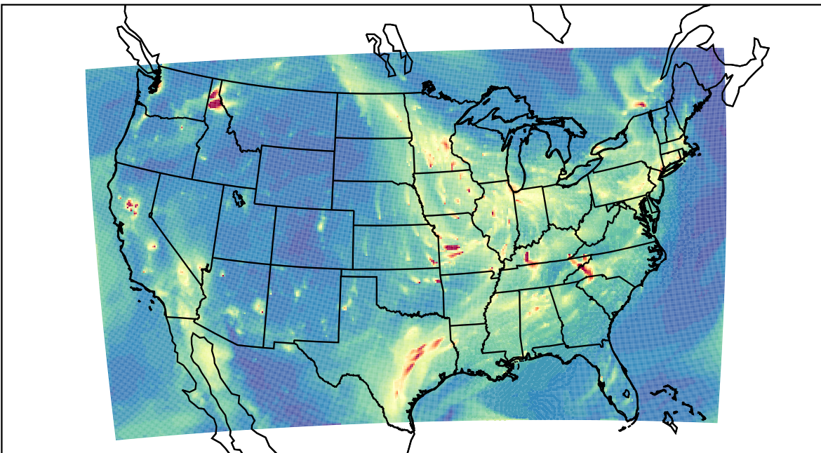
WRF 2023-11-14_02:00:00
