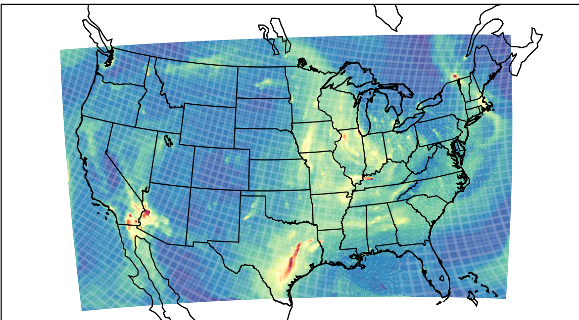
WRF 2023-11-14_14:00:00
