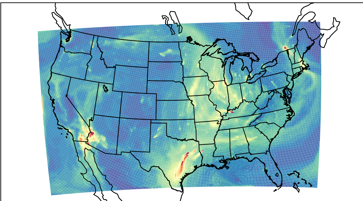
WRF 2023-11-14_15:00:00
