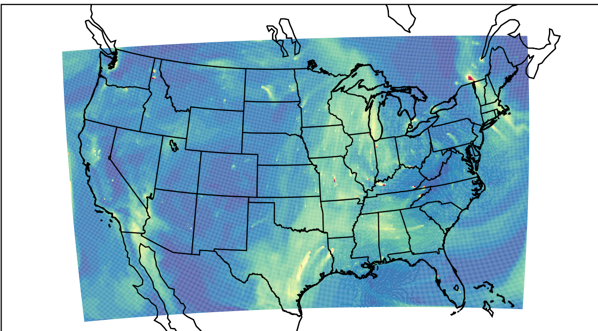
WRF 2023-11-14_20:00:00
