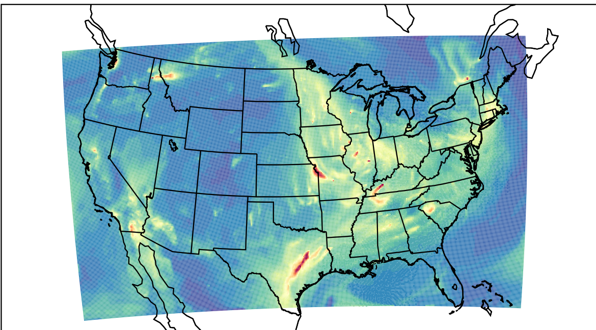
WRF 2023-11-14_07:00:00
