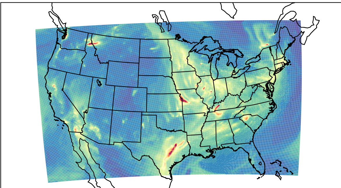
WRF 2023-11-14_06:00:00
