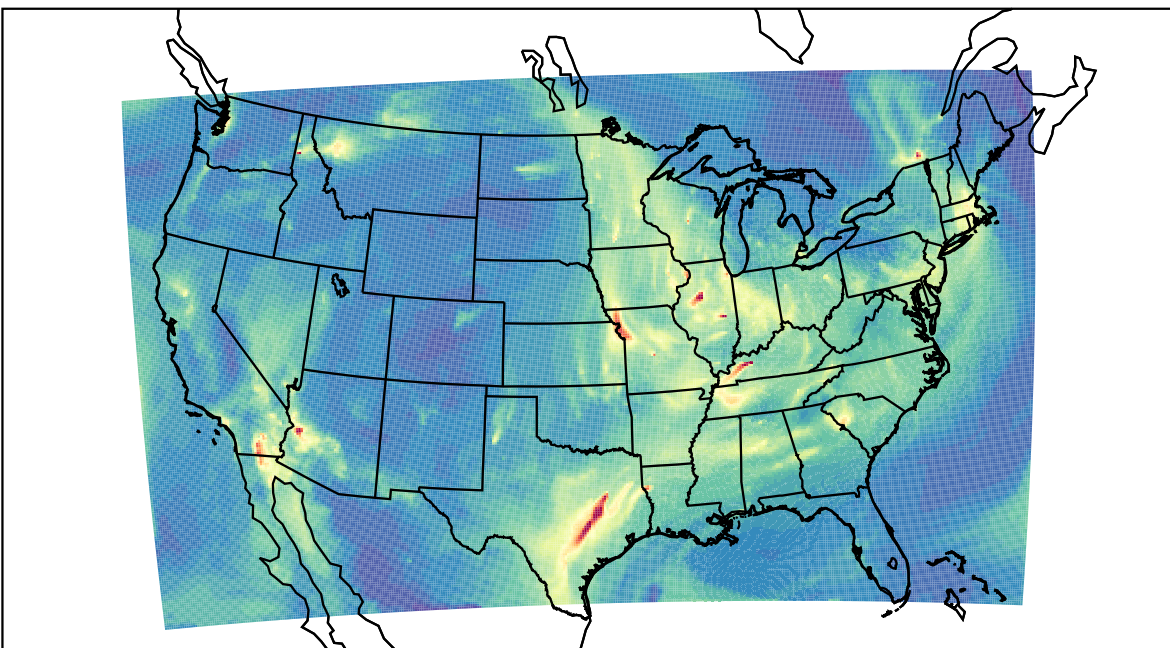
WRF 2023-11-14_09:00:00
