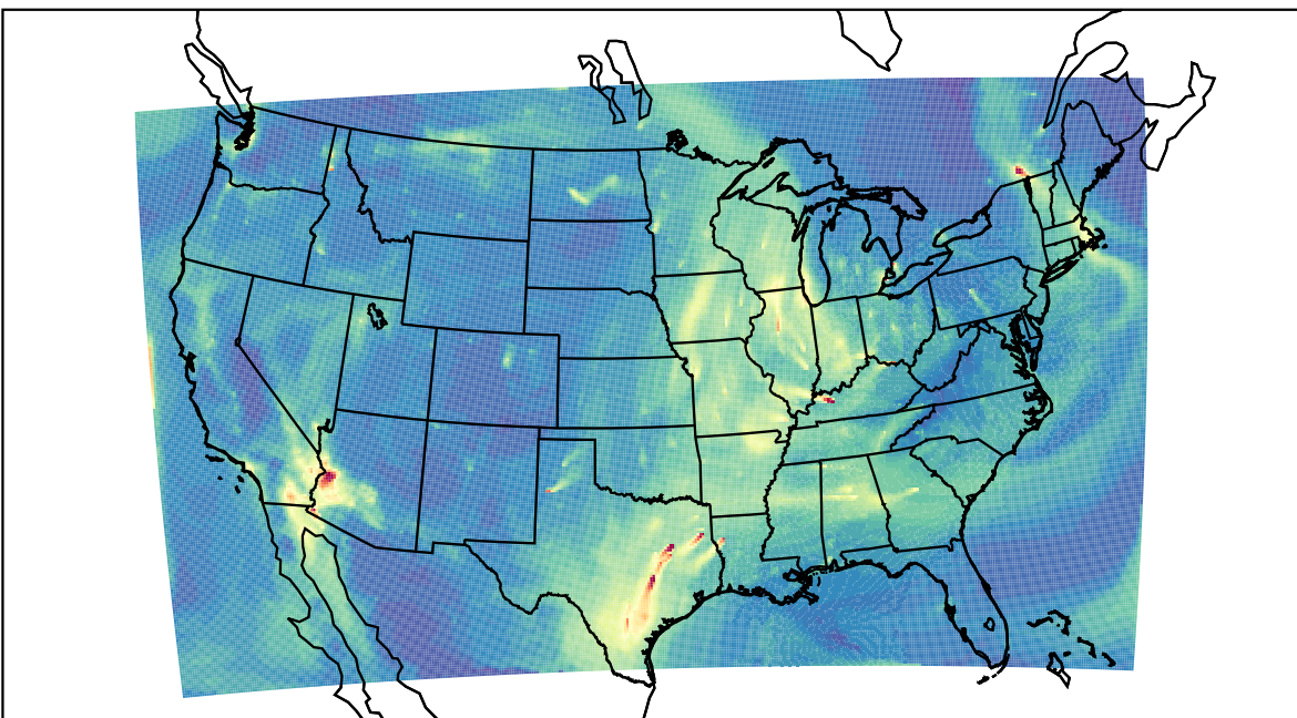
WRF 2023-11-14_16:00:00
