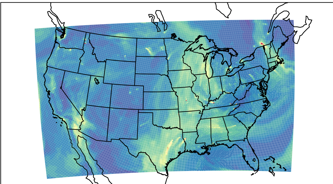
WRF 2023-11-14_19:00:00
