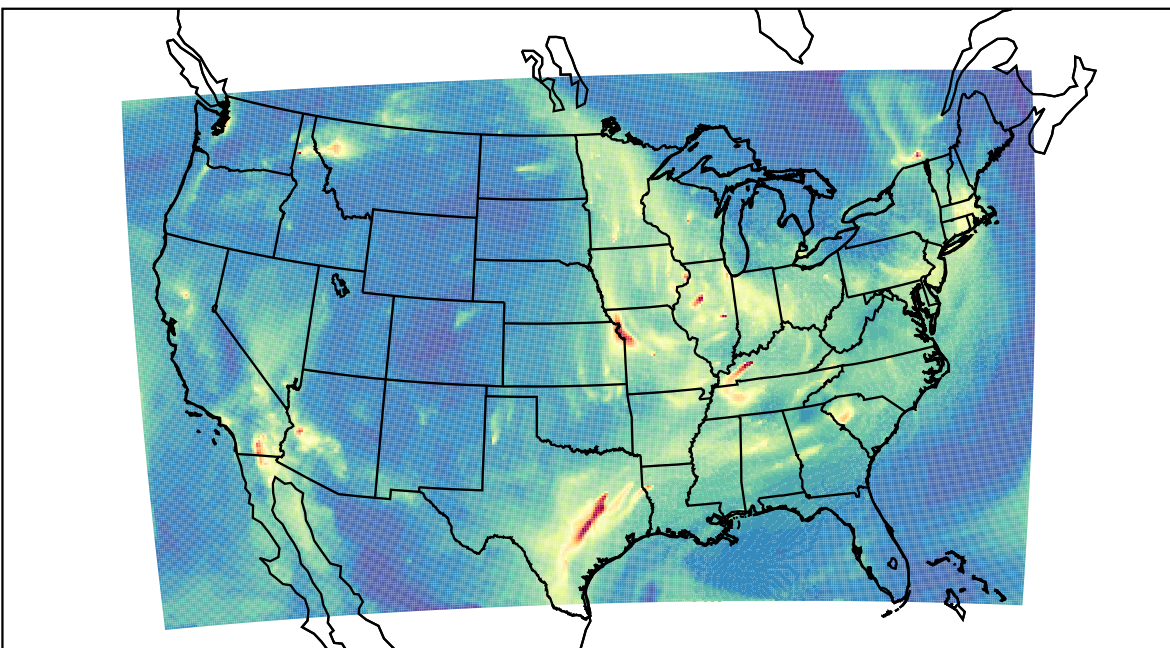
WRF 2023-11-14_08:00:00
