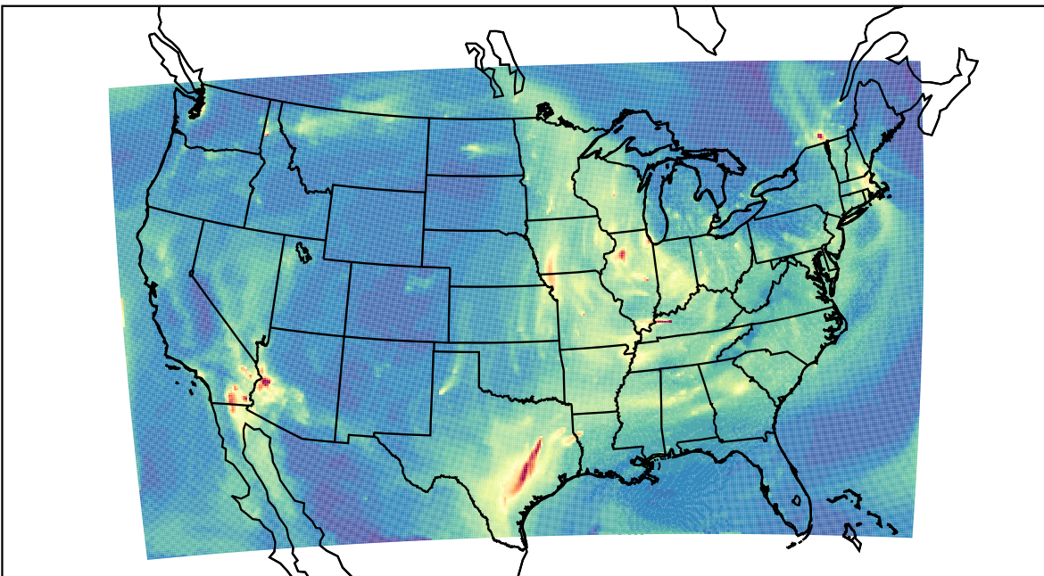
WRF 2023-11-14_12:00:00
