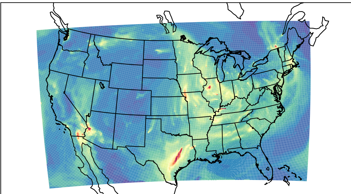
WRF 2023-11-14_11:00:00
