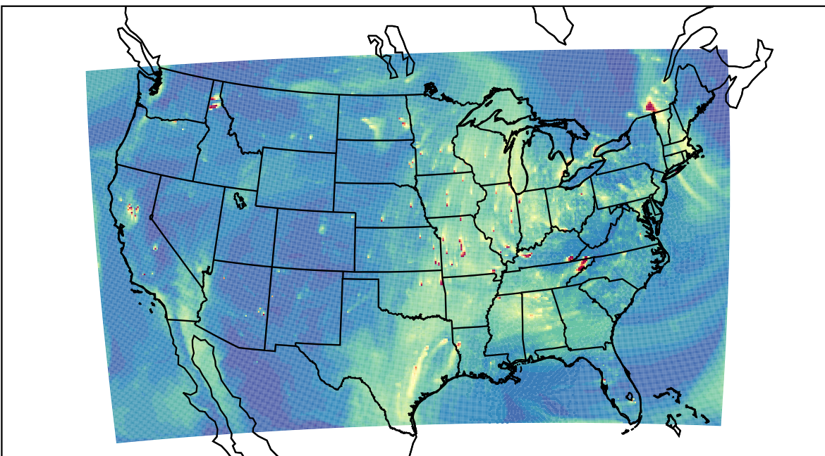
WRF 2023-11-14_23:00:00
