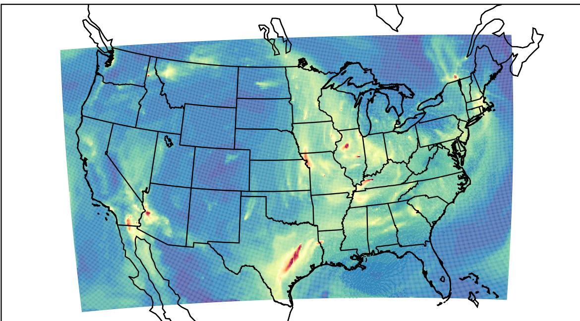
WRF 2023-11-14_10:00:00
