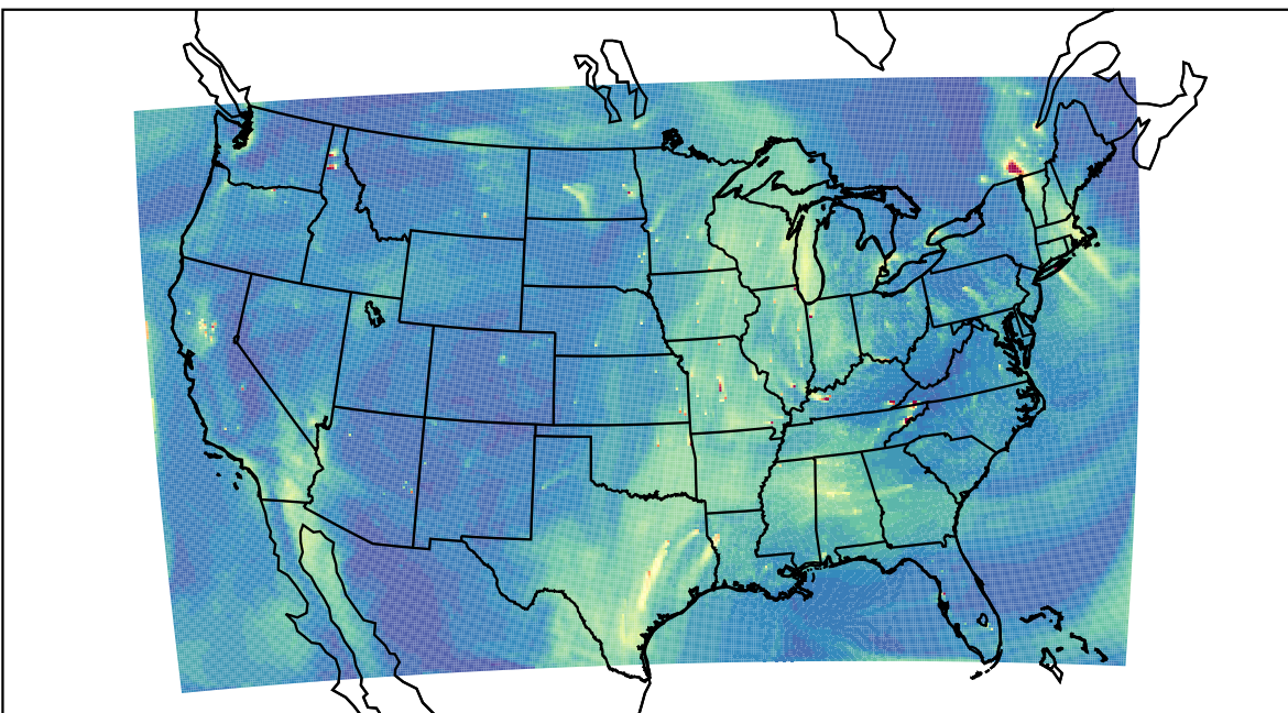
WRF 2023-11-14_21:00:00
