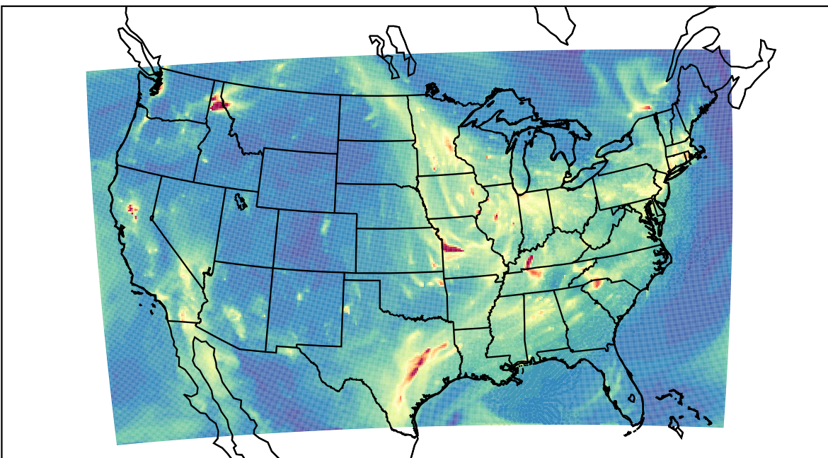
WRF 2023-11-14_04:00:00
