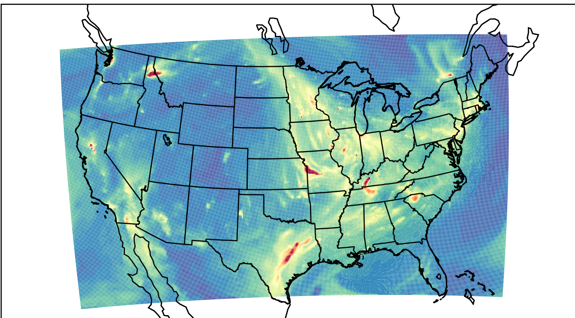
WRF 2023-11-14_05:00:00
