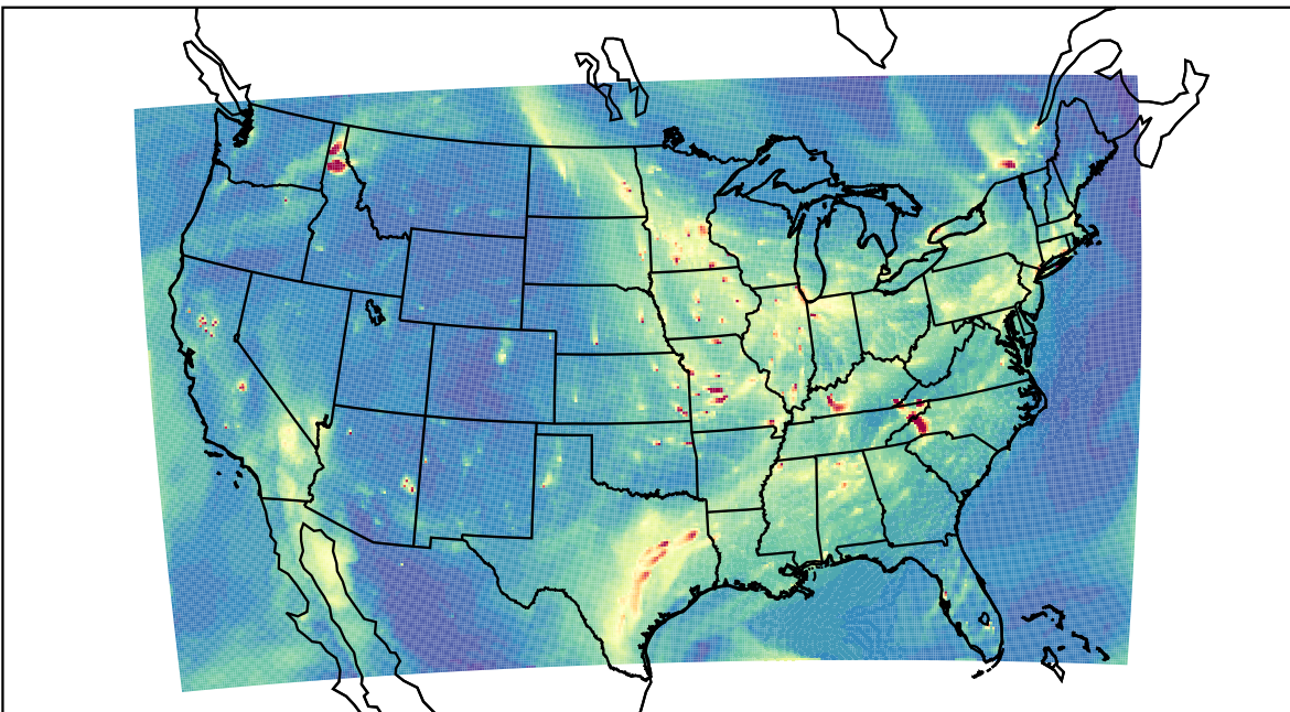
WRF 2023-11-14_00:00:00
