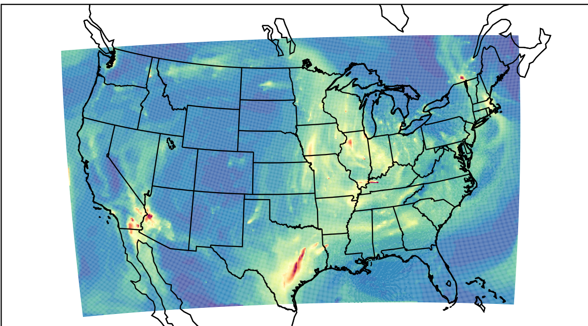
WRF 2023-11-14_13:00:00
