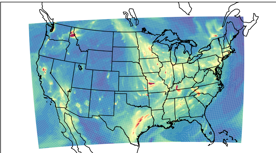
WRF 2023-11-14_03:00:00
