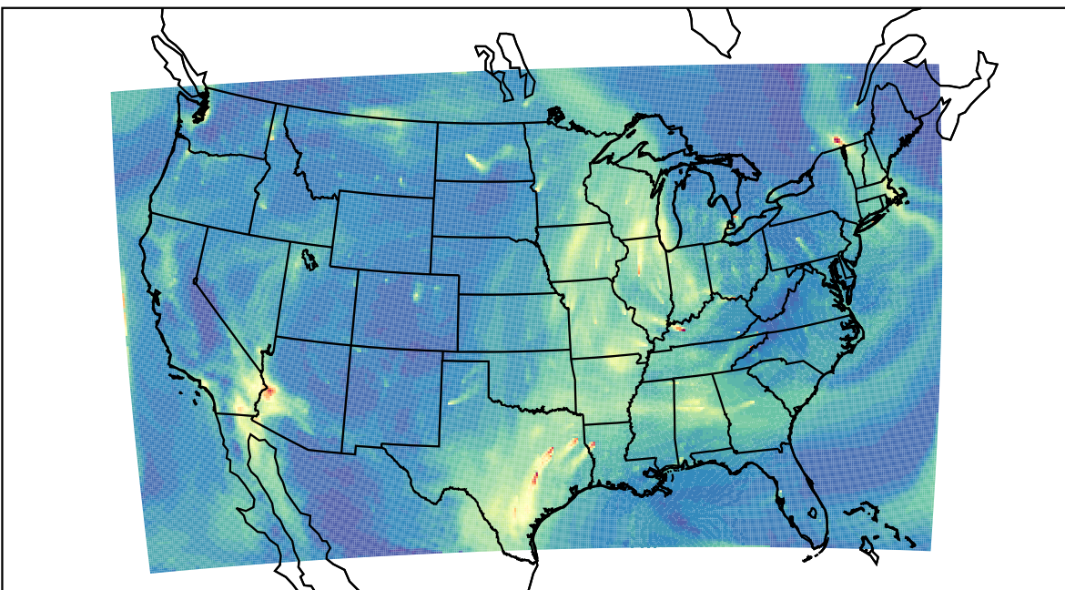
WRF 2023-11-14_17:00:00
