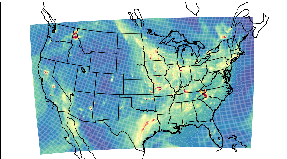
WRF 2023-11-14_01:00:00
