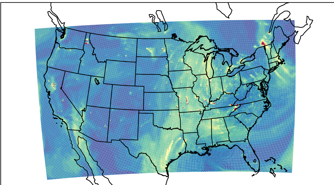
WRF 2023-11-14_22:00:00
