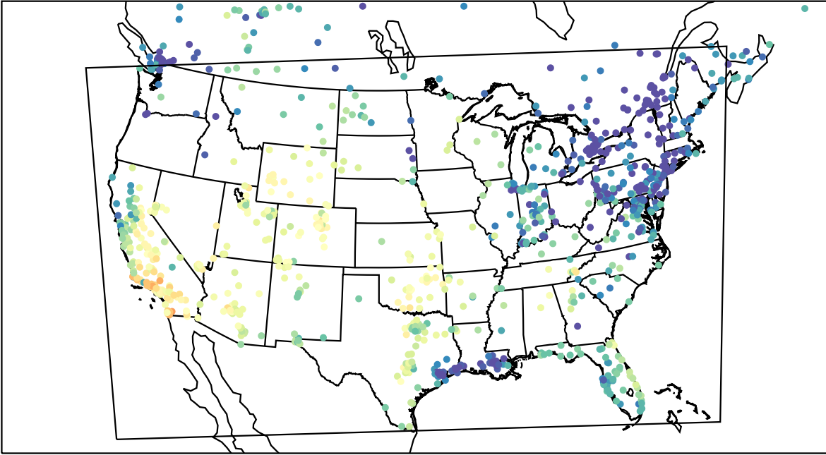
AirNOW (2023-11-14_22:00:00)
