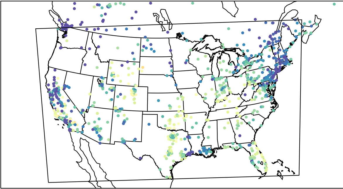
AirNOW (2023-11-15_17:00:00)
