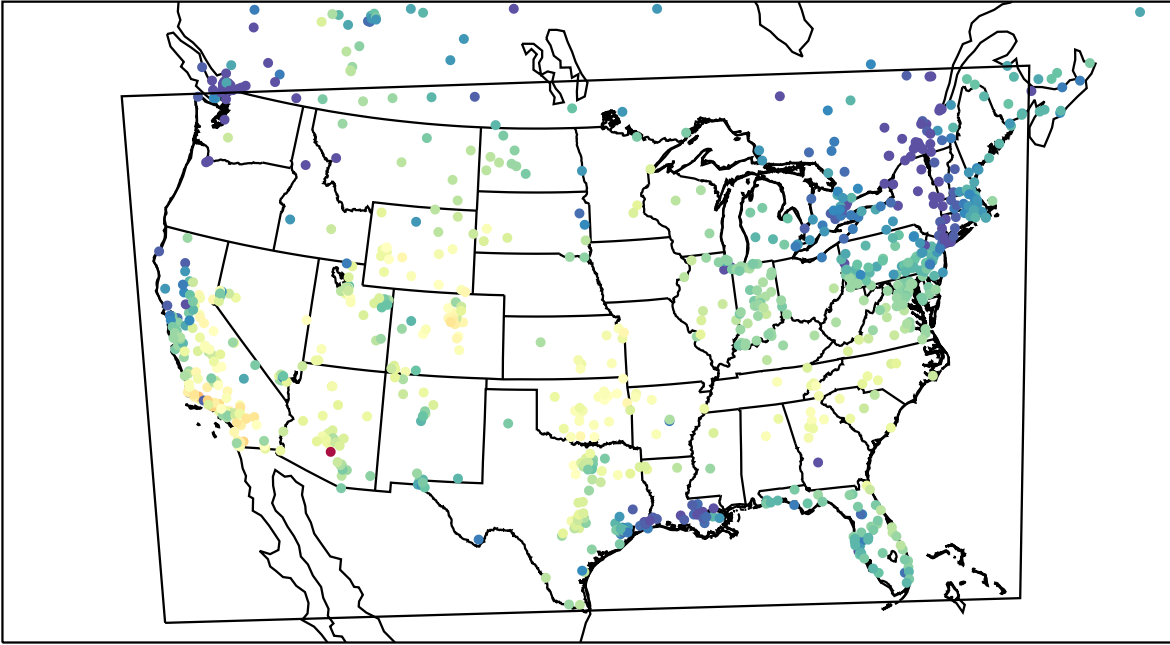
AirNOW (2023-11-14_19:00:00)
