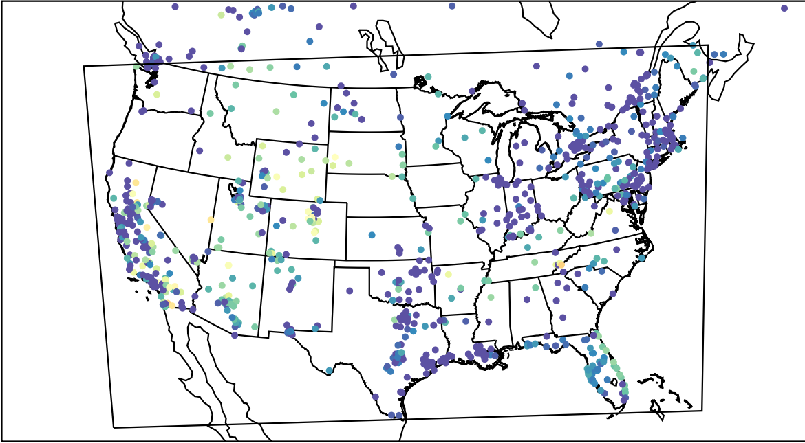
AirNOW (2023-11-14_09:00:00)
