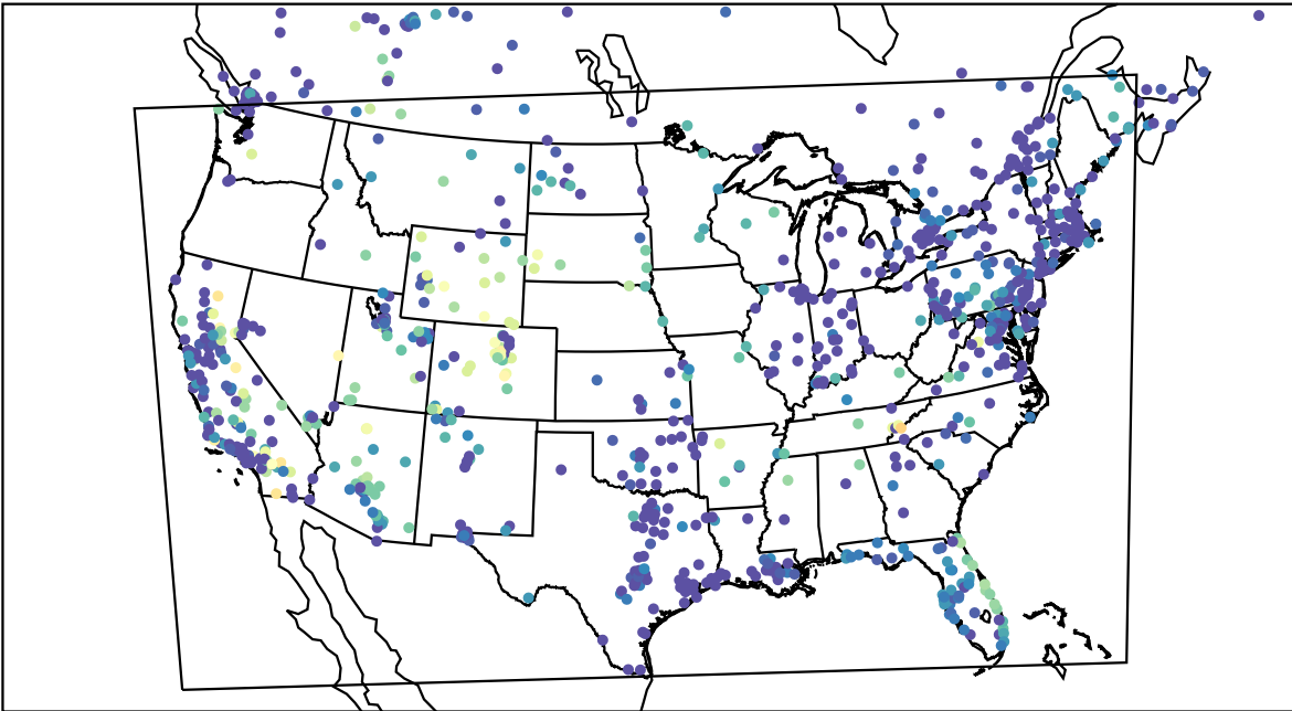
AirNOW (2023-11-14_11:00:00)
