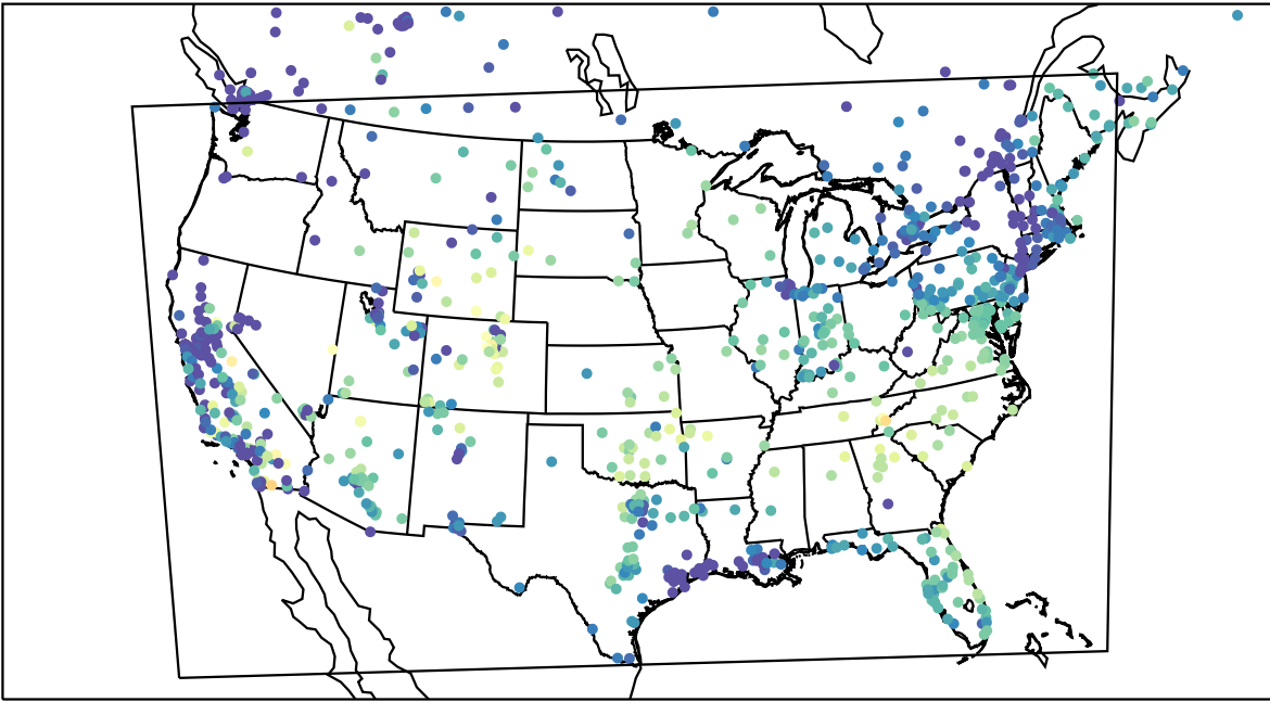
AirNOW (2023-11-14_16:00:00)
