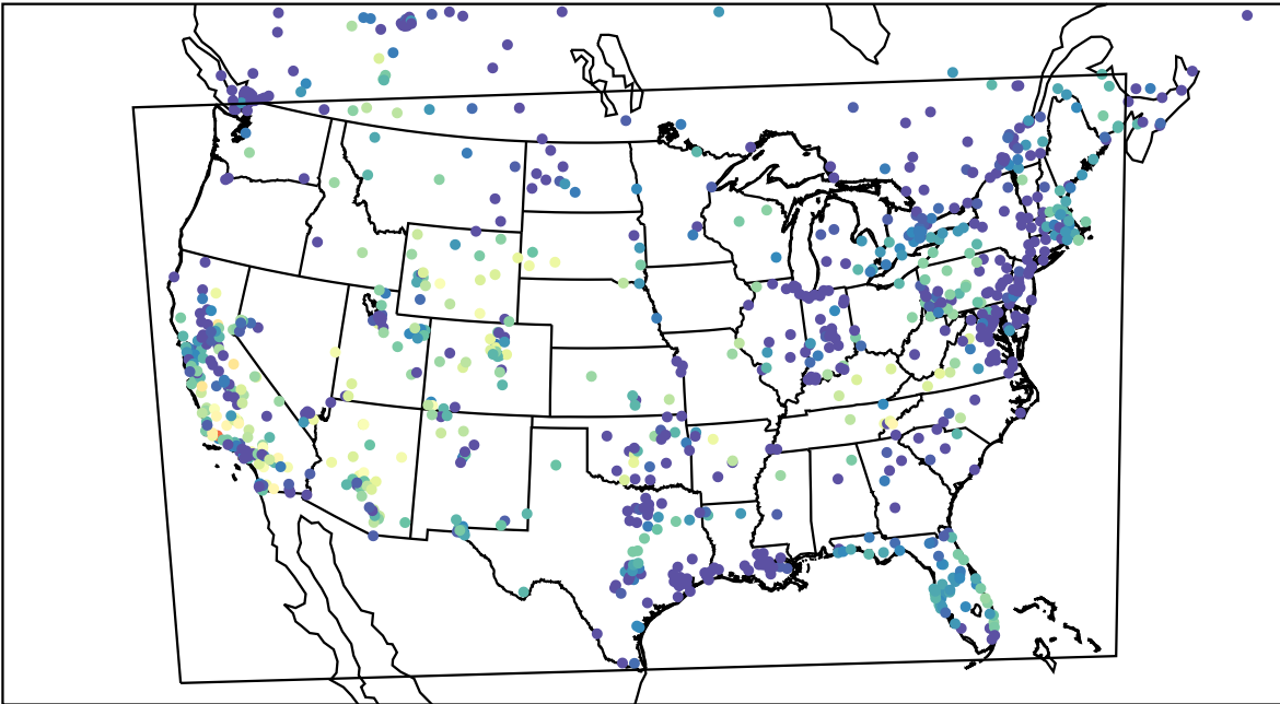
AirNOW (2023-11-14_02:00:00)
