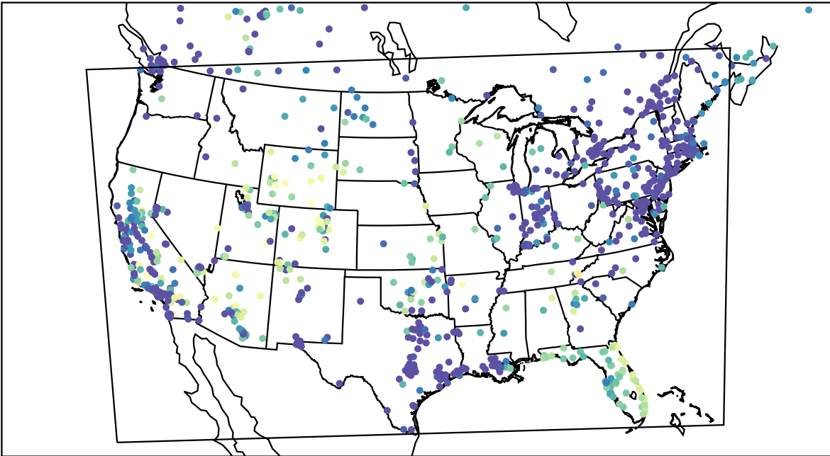
AirNOW (2023-11-15_03:00:00)
