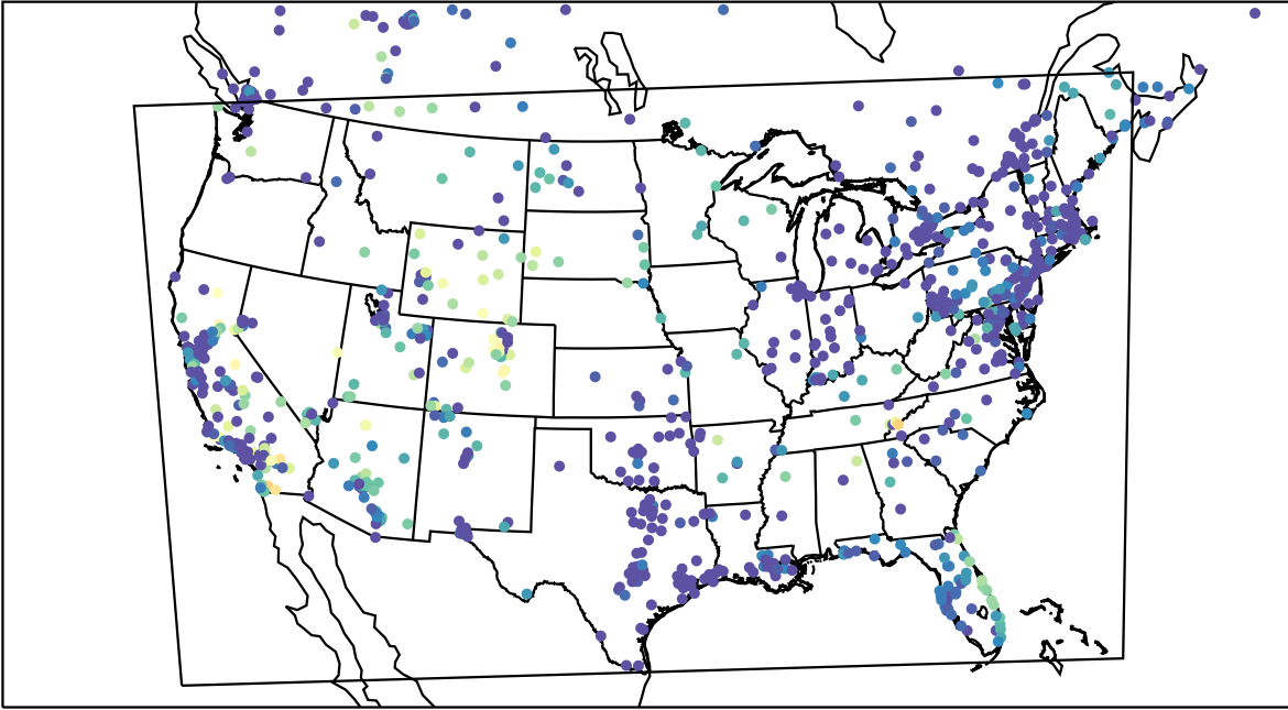
AirNOW (2023-11-14_12:00:00)
