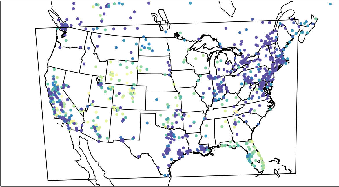
AirNOW (2023-11-15_02:00:00)
