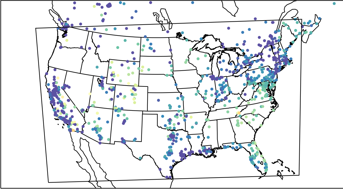
AirNOW (2023-11-14_15:00:00)
