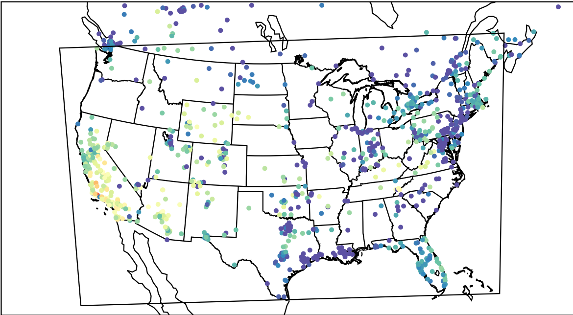
AirNOW (2023-11-14_00:00:00)
