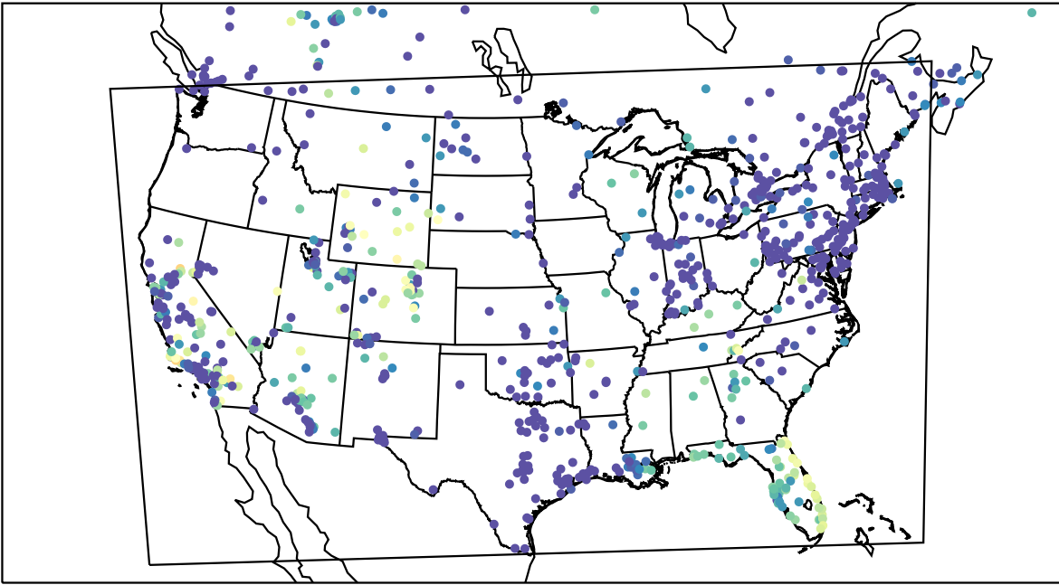
AirNOW (2023-11-15_12:00:00)
