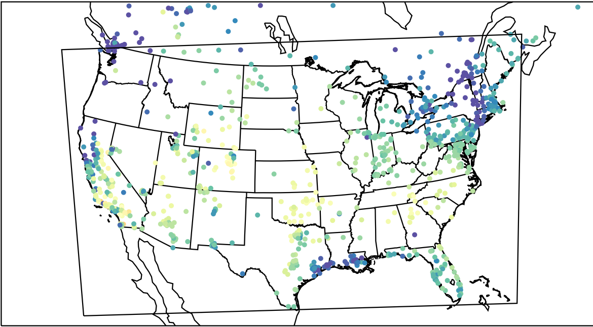
AirNOW (2023-11-14_18:00:00)
