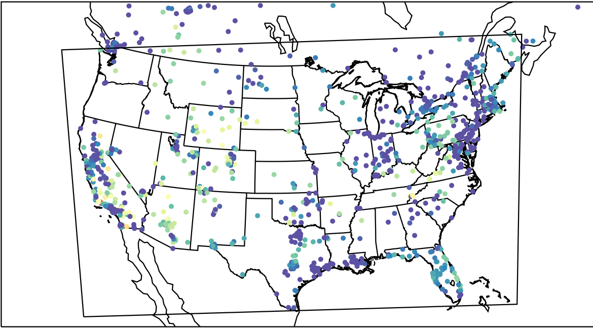
AirNOW (2023-11-14_03:00:00)
