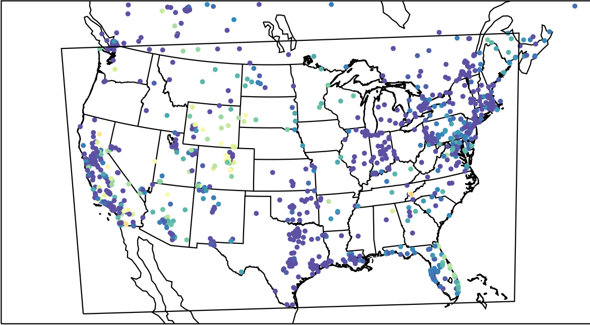
AirNOW (2023-11-14_13:00:00)
