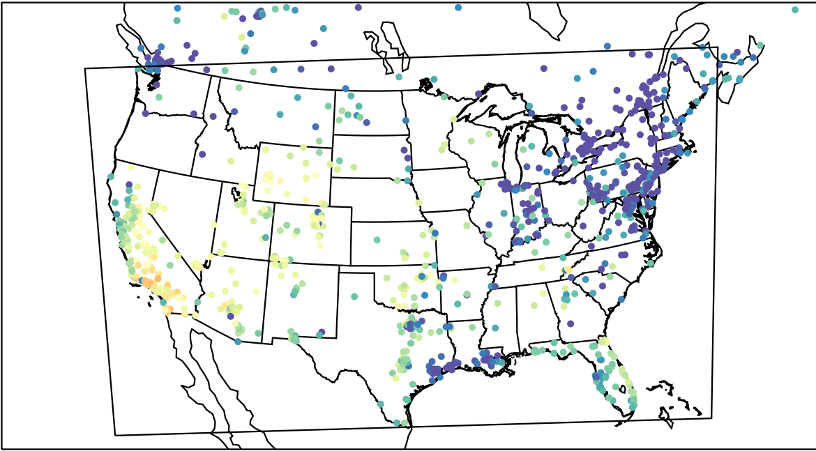
AirNOW (2023-11-14_23:00:00)
