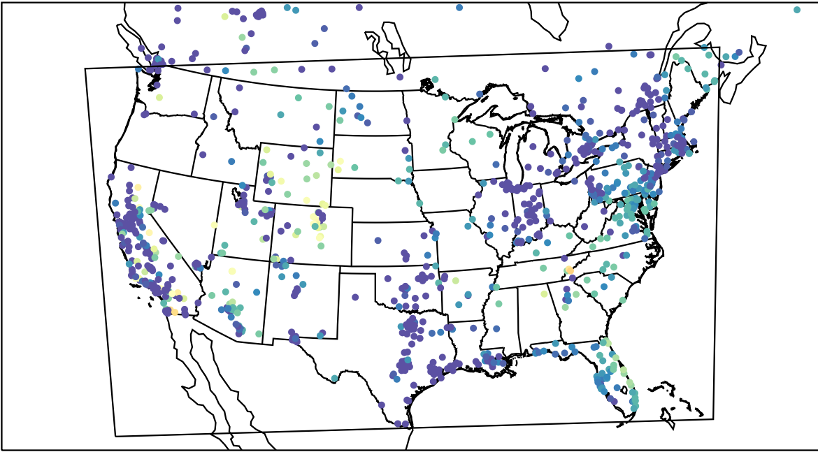
AirNOW (2023-11-14_14:00:00)
