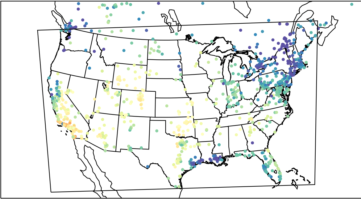
AirNOW (2023-11-14_21:00:00)
