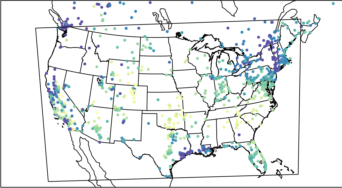
AirNOW (2023-11-14_17:00:00)
