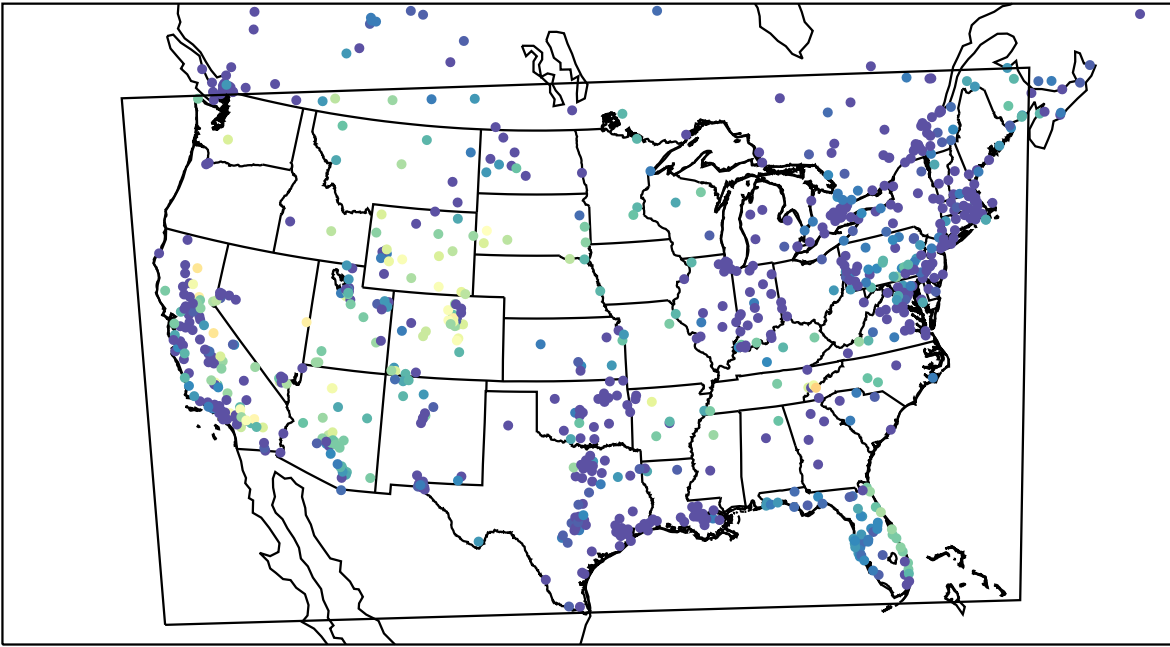
AirNOW (2023-11-14_10:00:00)
