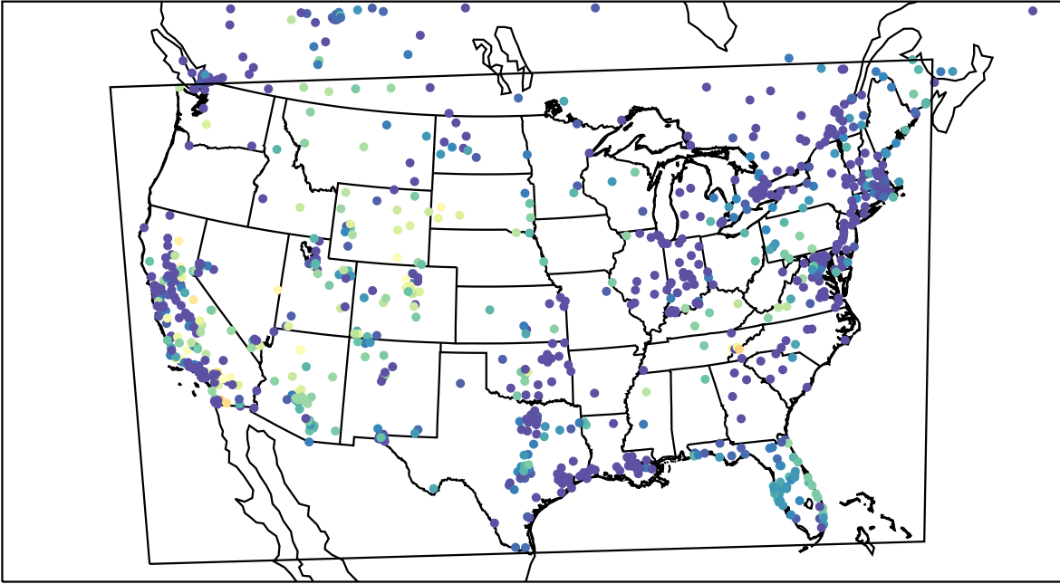
AirNOW (2023-11-14_06:00:00)
