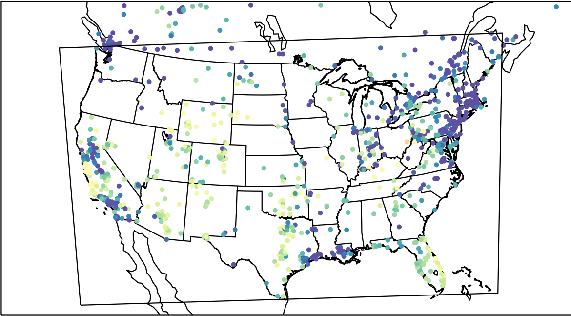
AirNOW (2023-11-15_23:00:00)
