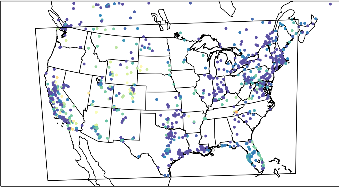
AirNOW (2023-11-14_08:00:00)
