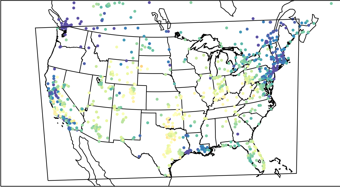
AirNOW (2023-11-15_19:00:00)
