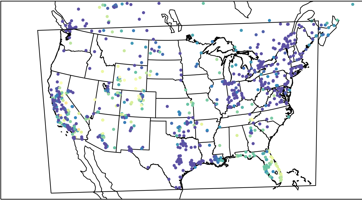
AirNOW (2023-11-15_08:00:00)
