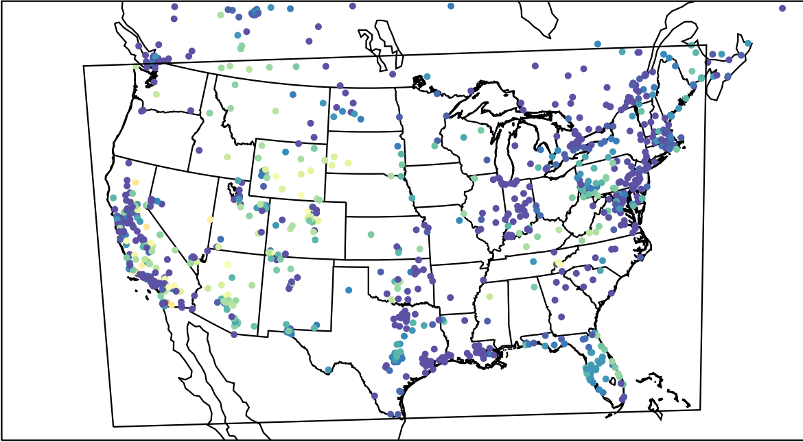
AirNOW (2023-11-14_05:00:00)
