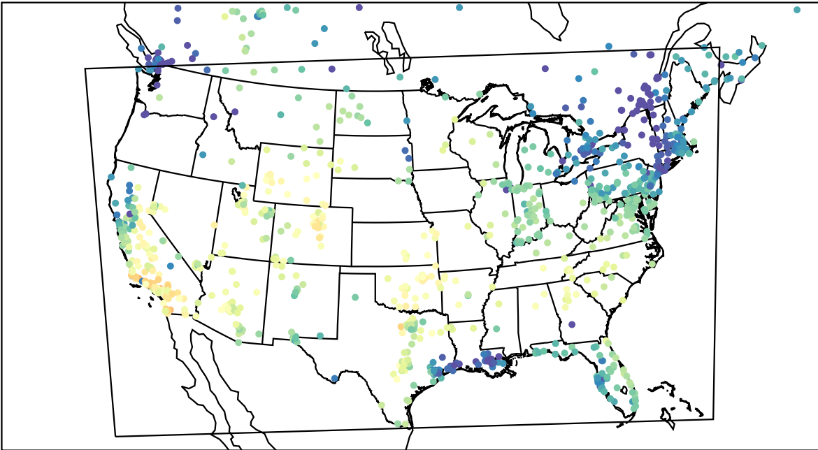
AirNOW (2023-11-14_20:00:00)
