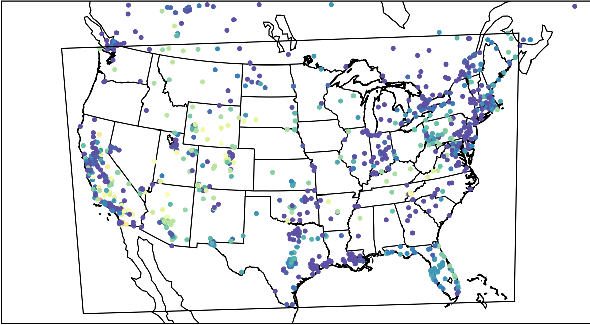
AirNOW (2023-11-14_04:00:00)
