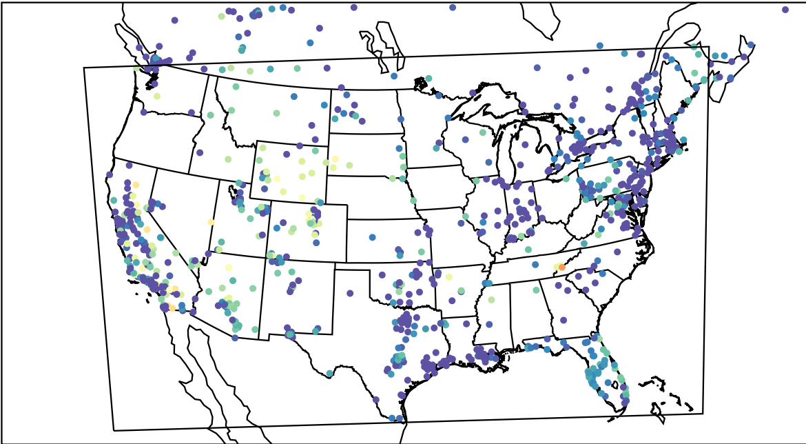
AirNOW (2023-11-14_07:00:00)
