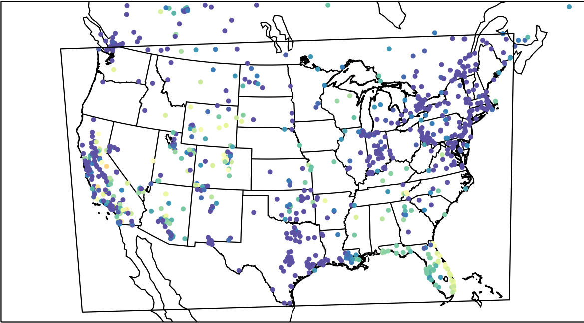
AirNOW (2023-11-15_09:00:00)
