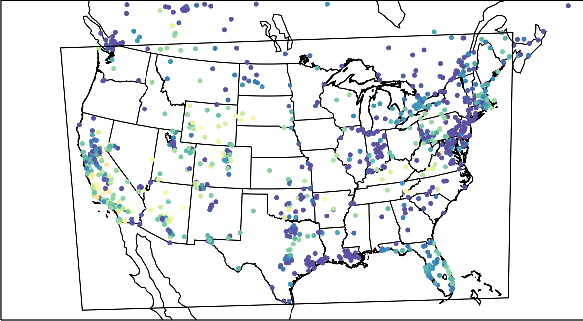
AirNOW (2023-11-14_01:00:00)
