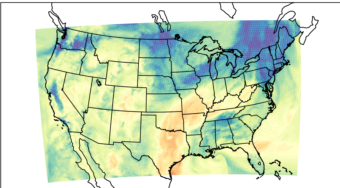
WRF (2023-11-15_20:00:00)
