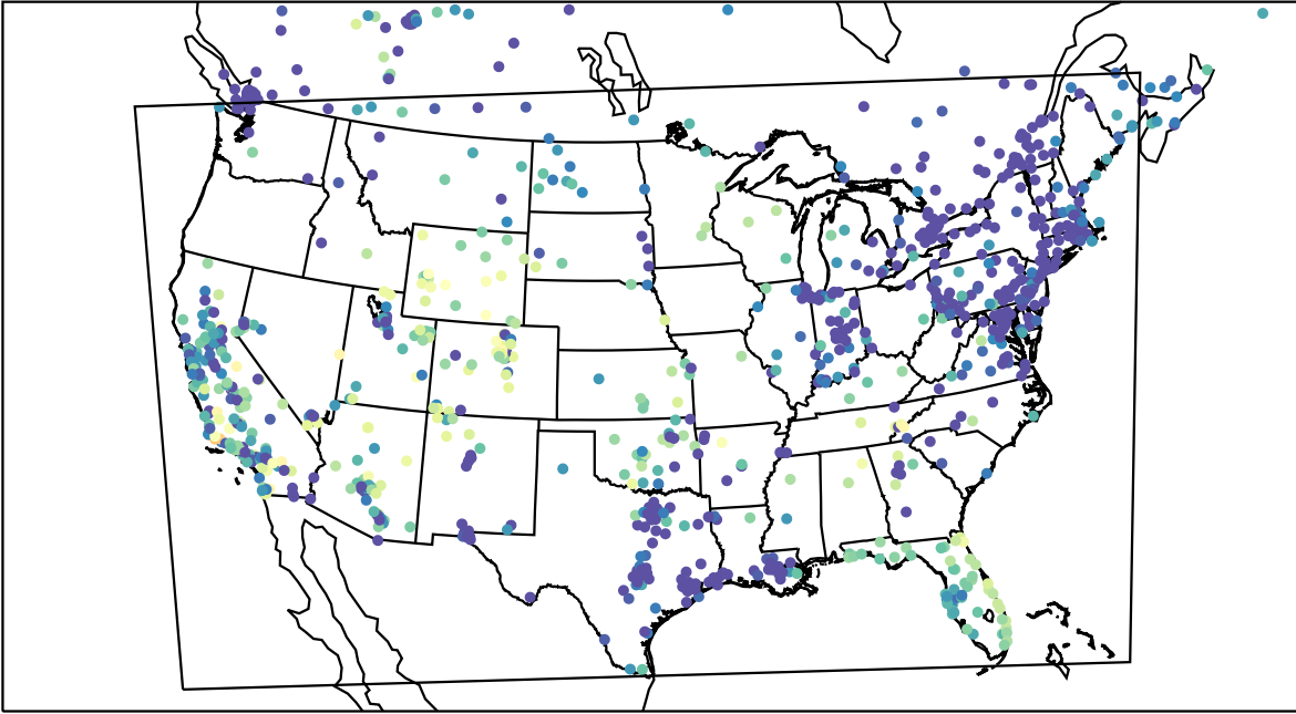
AirNOW (2023-11-15_01:00:00)
