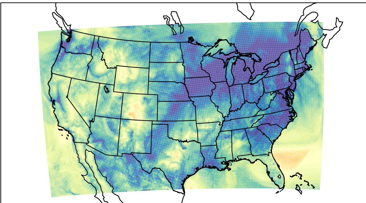
WRF (2023-11-15_12:00:00)
