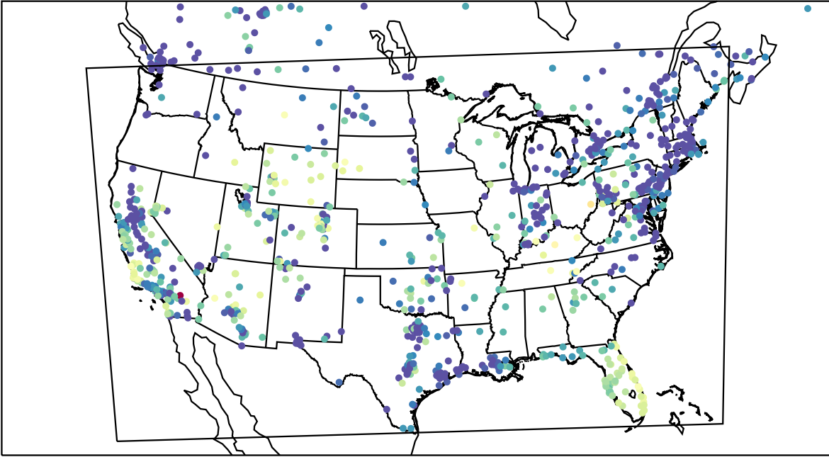
AirNOW (2023-11-16_02:00:00)
