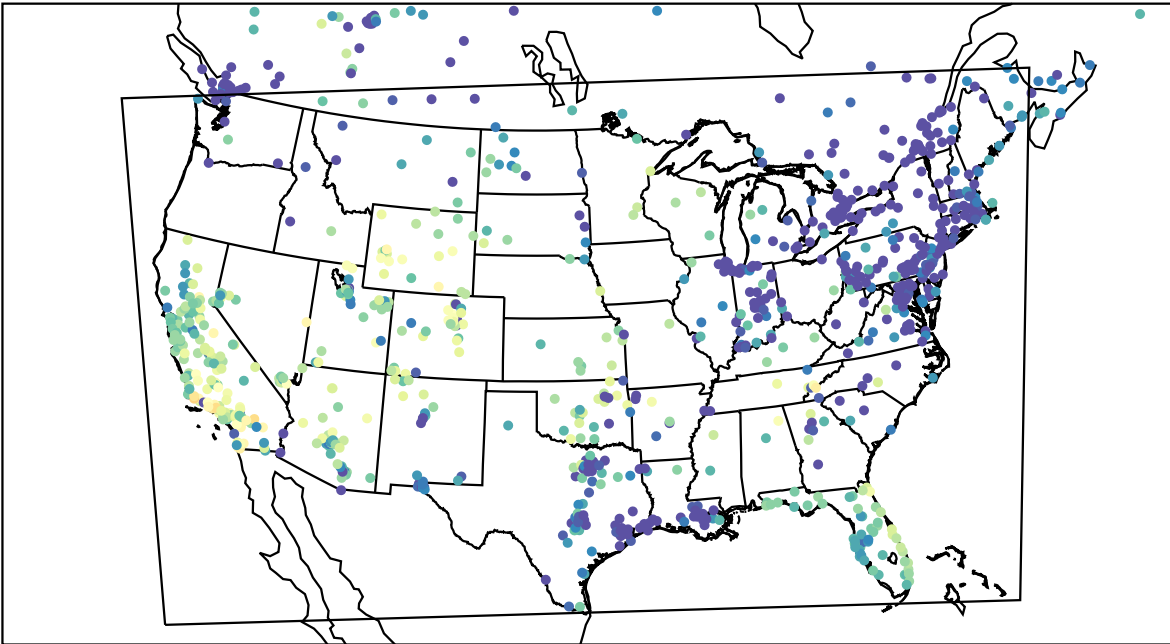
AirNOW (2023-11-15_00:00:00)
