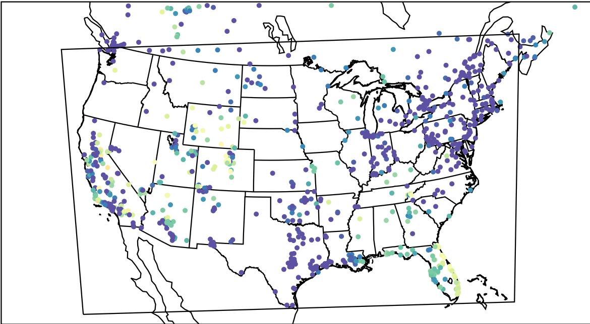
AirNOW (2023-11-15_11:00:00)
