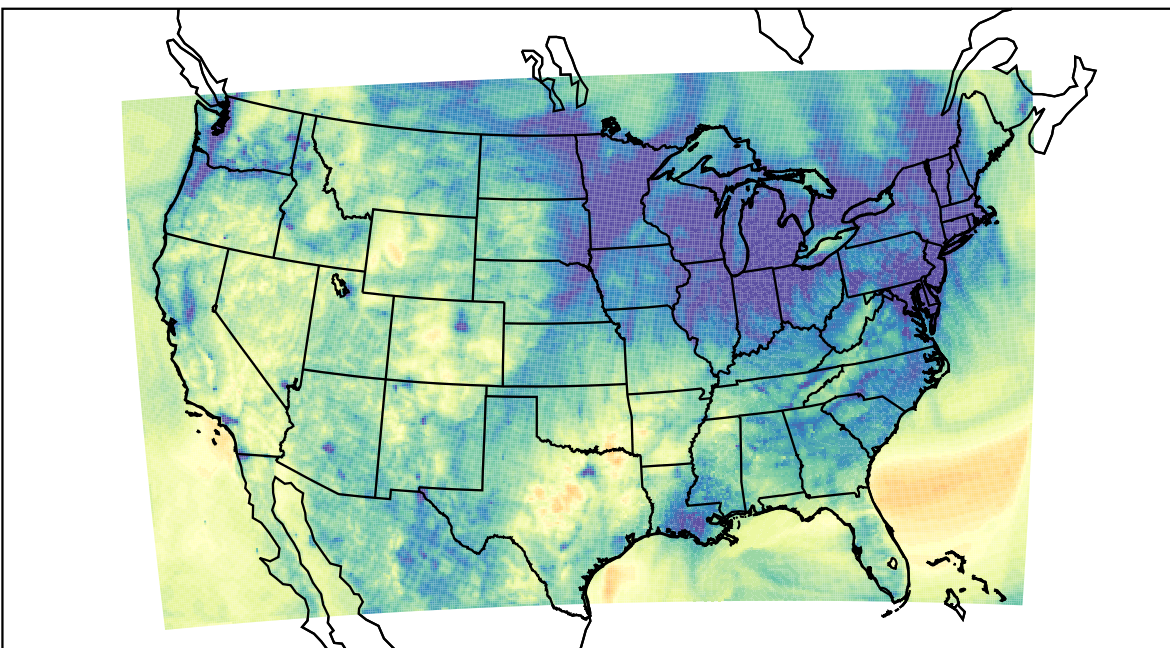
WRF (2023-11-15_03:00:00)
