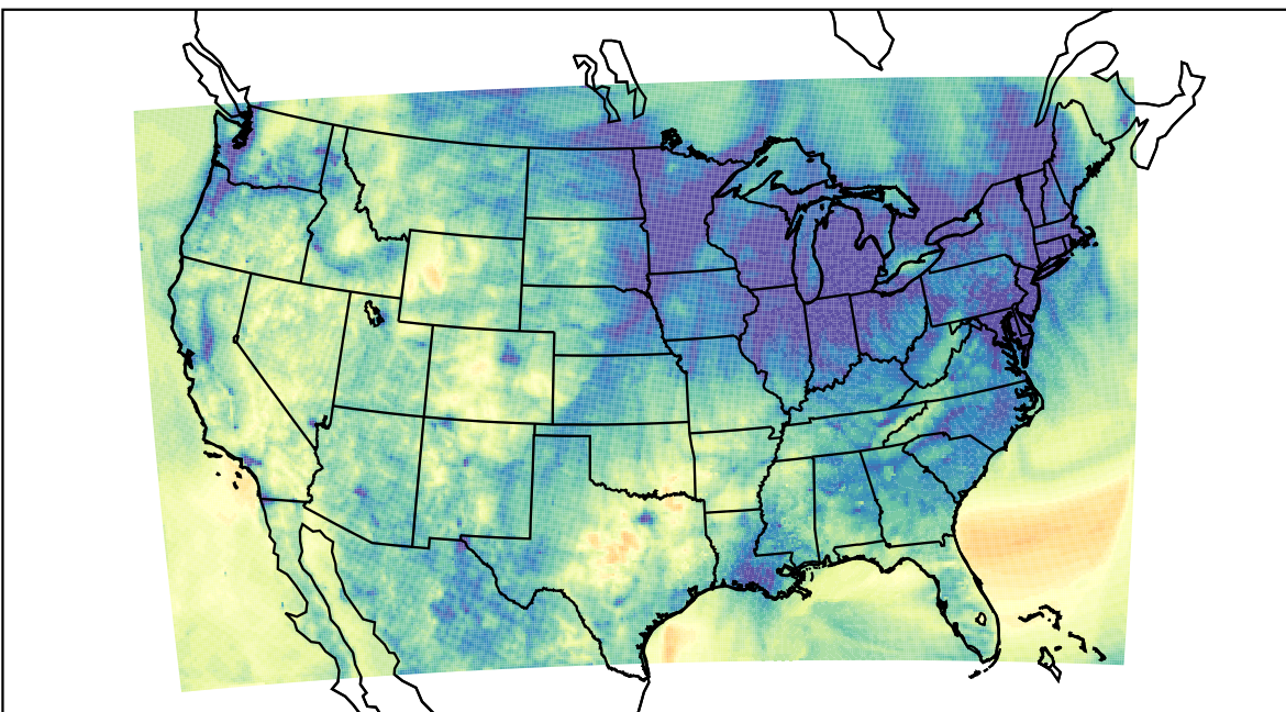
WRF (2023-11-15_04:00:00)
