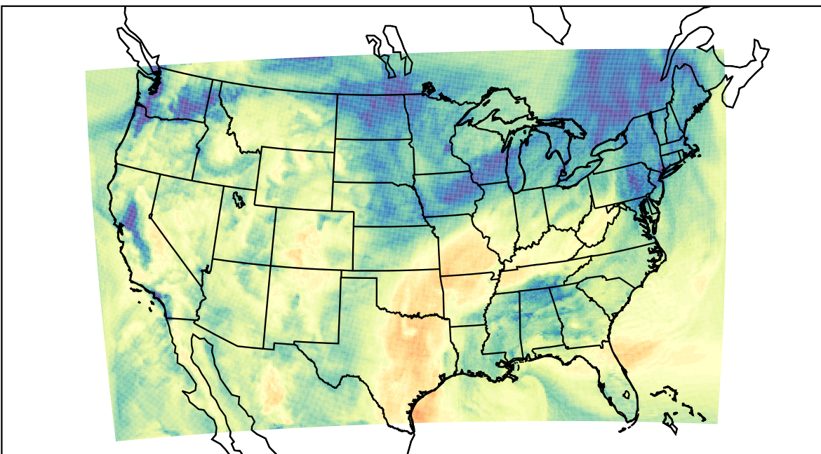
WRF (2023-11-15_19:00:00)
