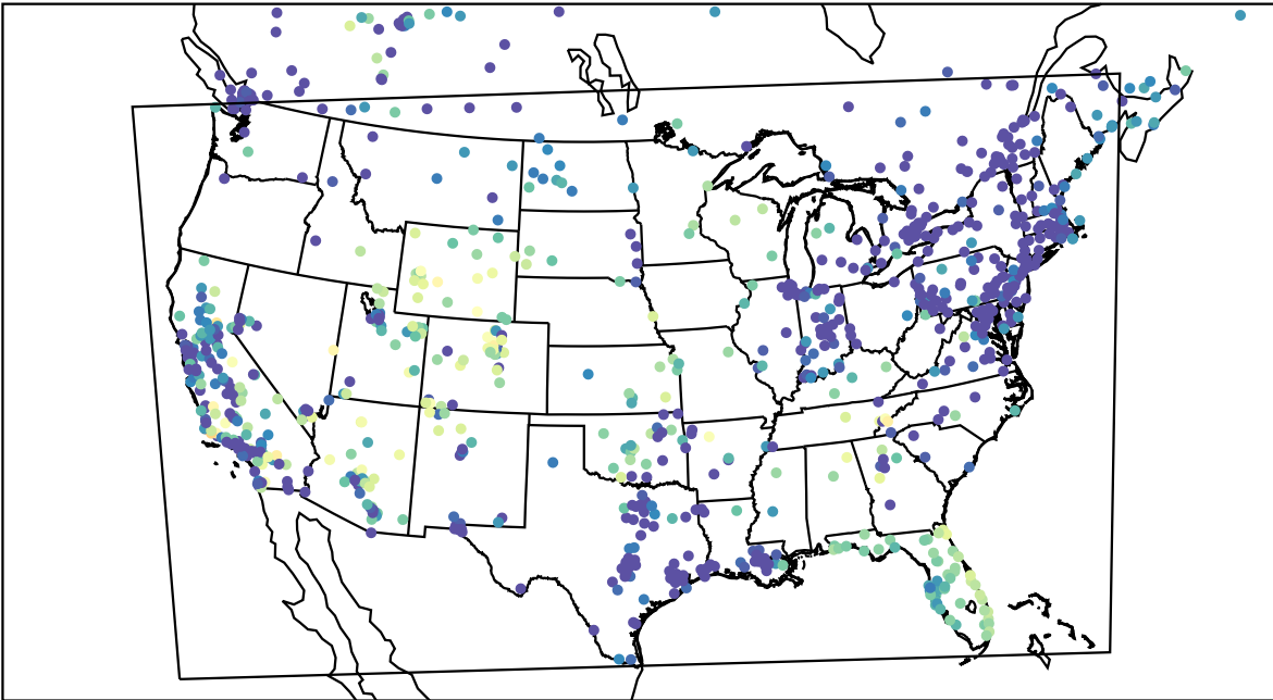
AirNOW (2023-11-15_02:00:00)
