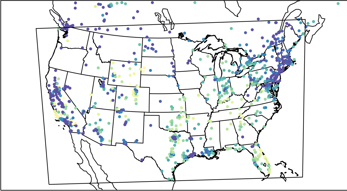
AirNOW (2023-11-15_16:00:00)
