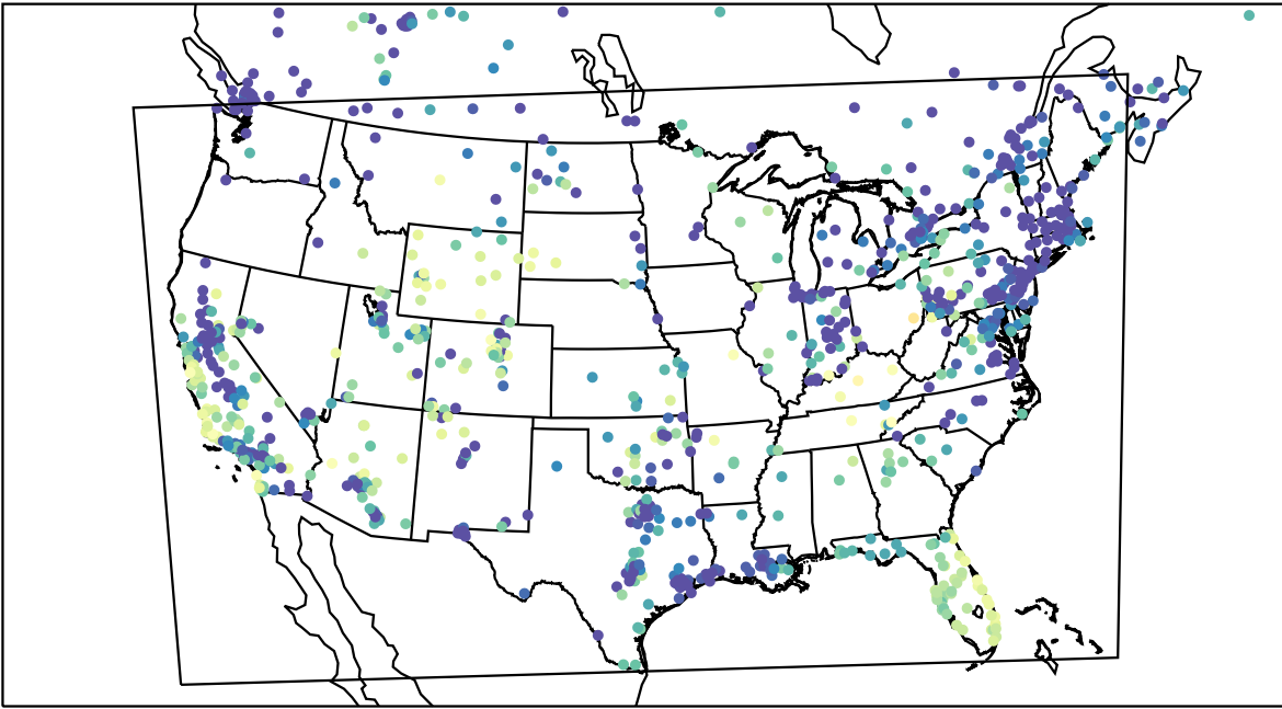
AirNOW (2023-11-16_01:00:00)
