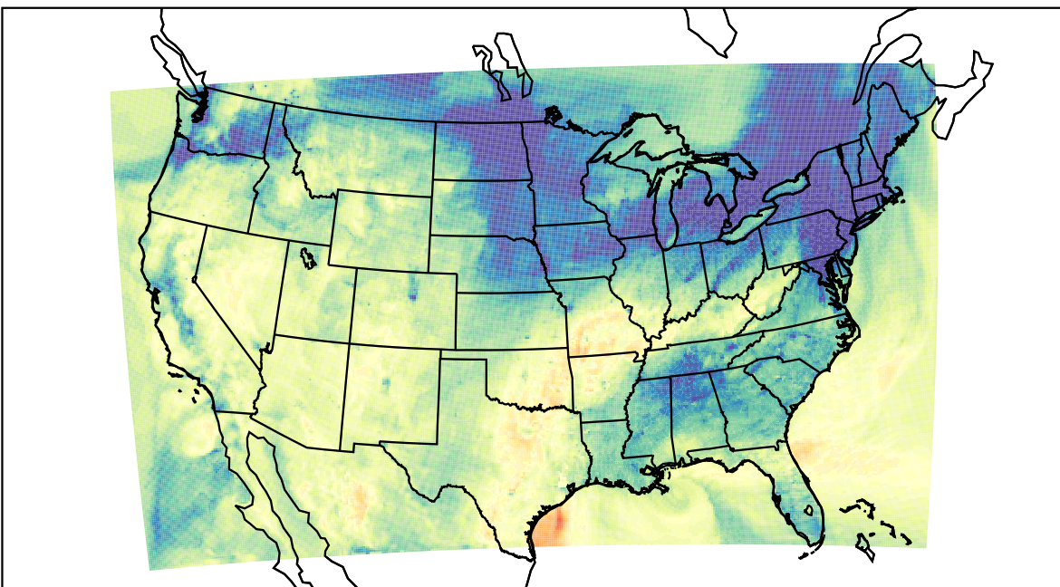
WRF (2023-11-15_23:00:00)
