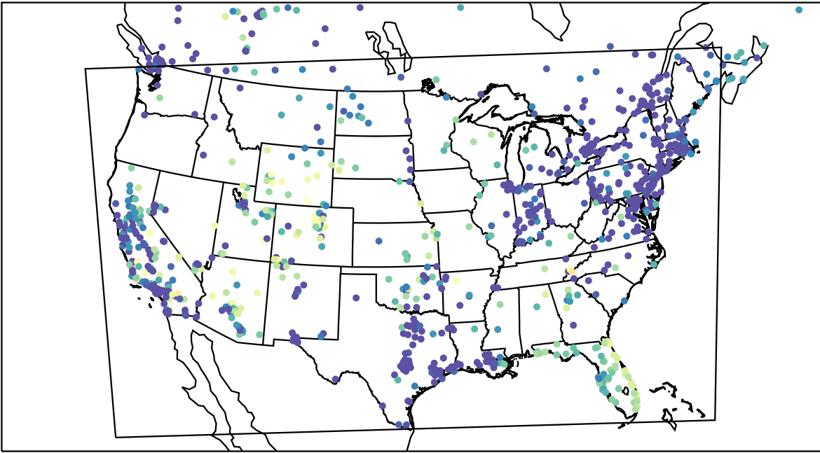
AirNOW (2023-11-15_03:00:00)
