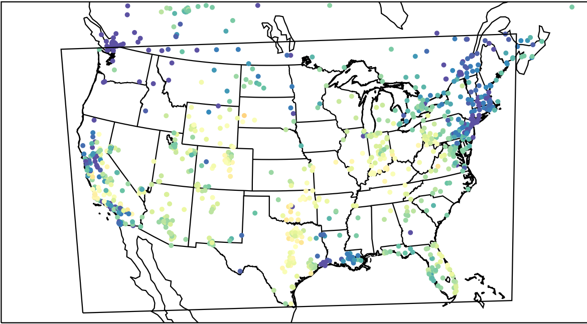
AirNOW (2023-11-15_19:00:00)
