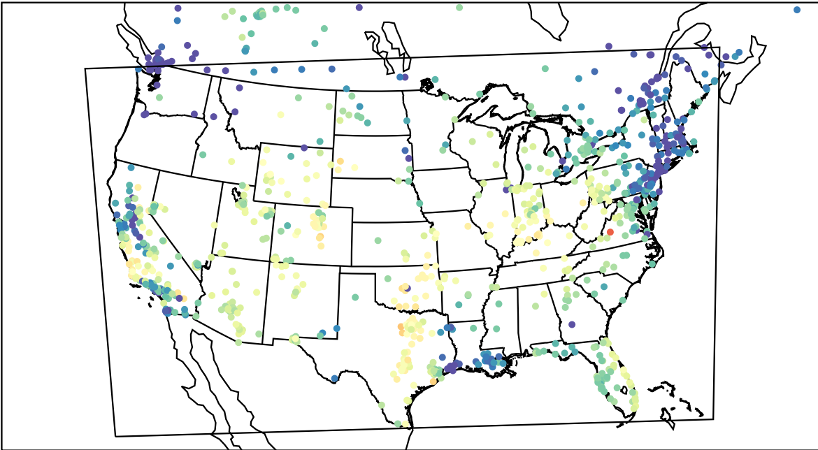
AirNOW (2023-11-15_20:00:00)
