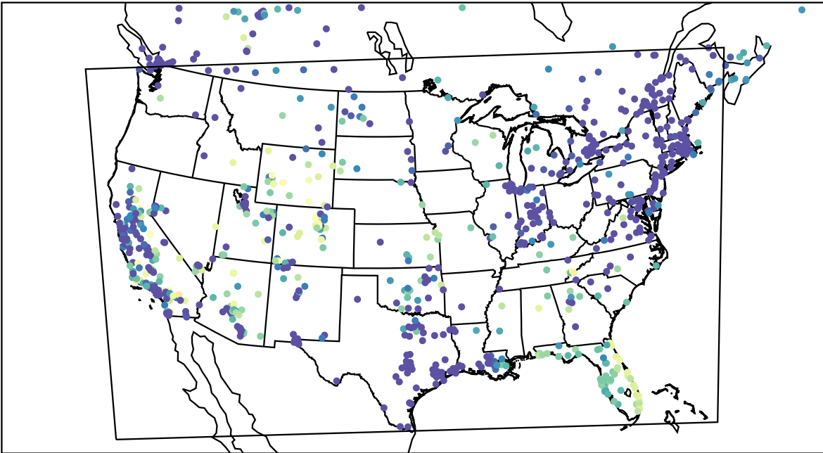
AirNOW (2023-11-15_06:00:00)
