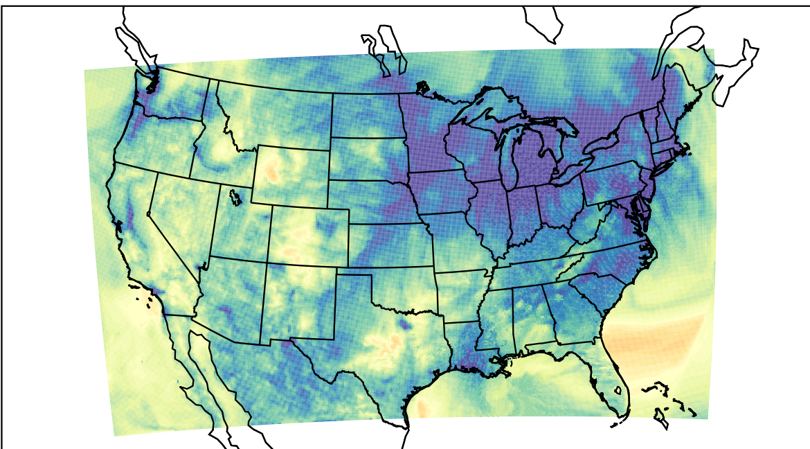
WRF (2023-11-15_07:00:00)
