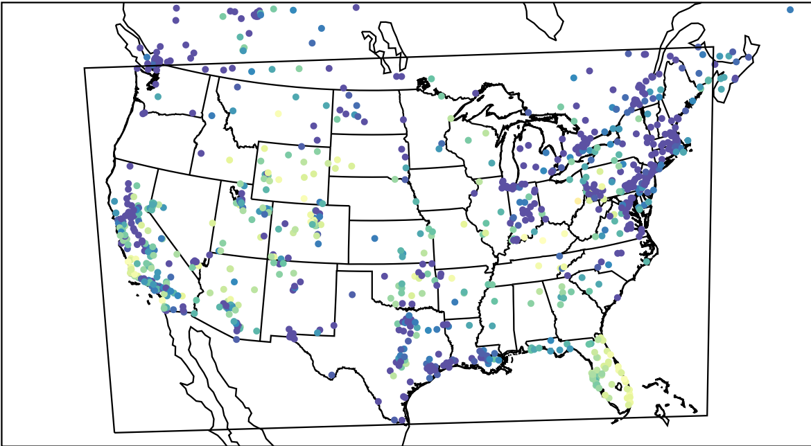
AirNOW (2023-11-16_03:00:00)
