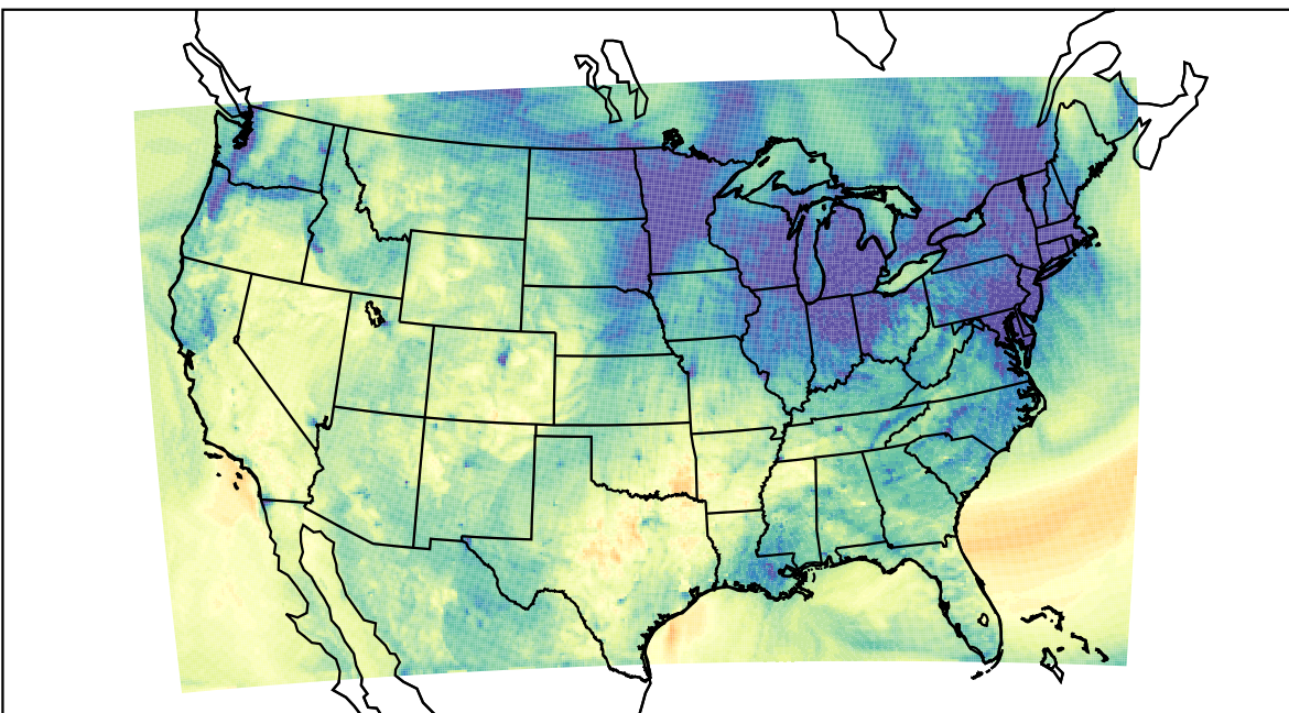
WRF (2023-11-15_00:00:00)
