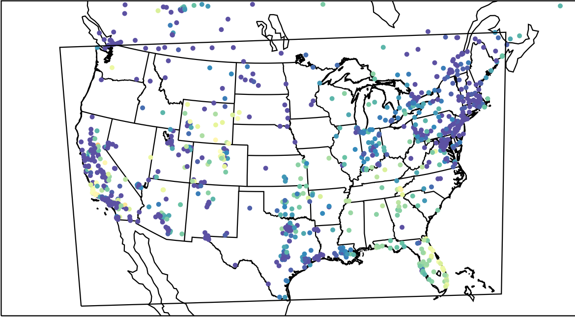
AirNOW (2023-11-15_15:00:00)
