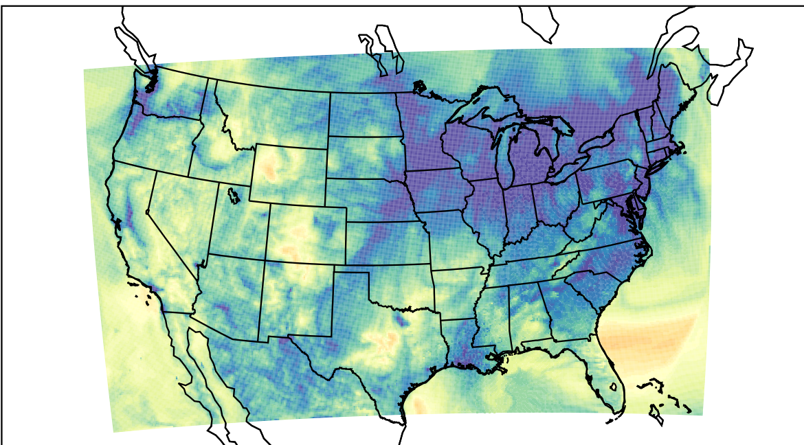
WRF (2023-11-15_08:00:00)
