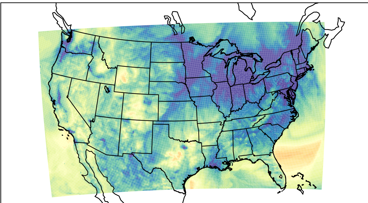
WRF (2023-11-15_06:00:00)
