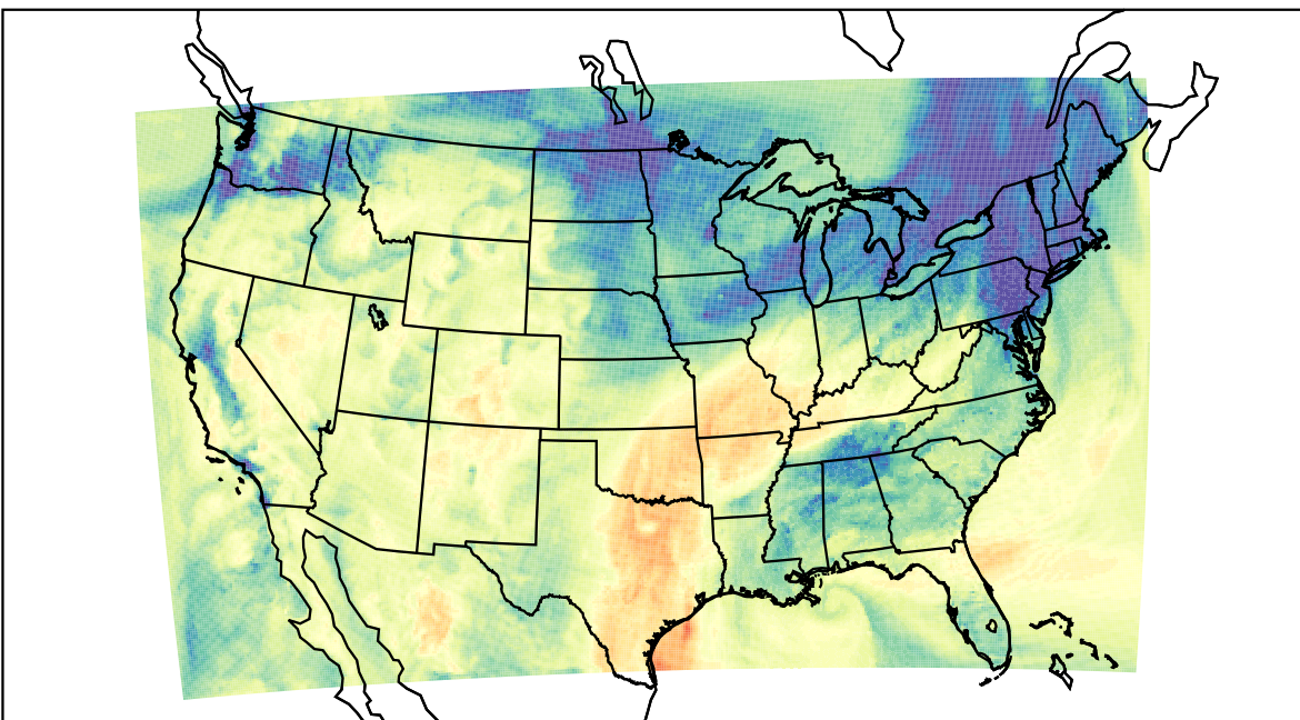
WRF (2023-11-15_21:00:00)
