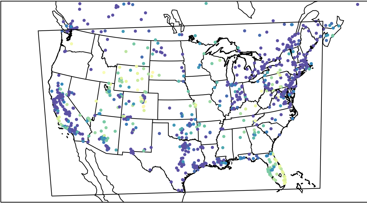
AirNOW (2023-11-16_10:00:00)
