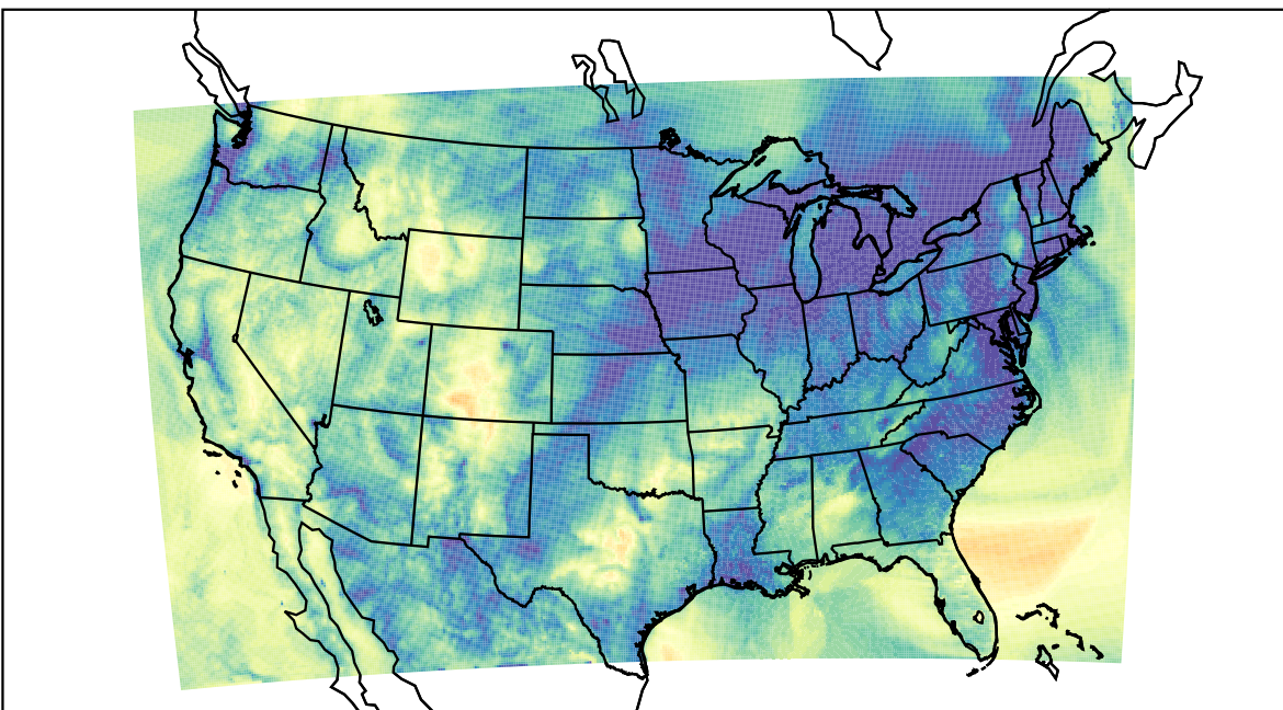
WRF (2023-11-15_11:00:00)
