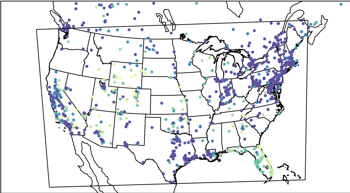
AirNOW (2023-11-15_04:00:00)
