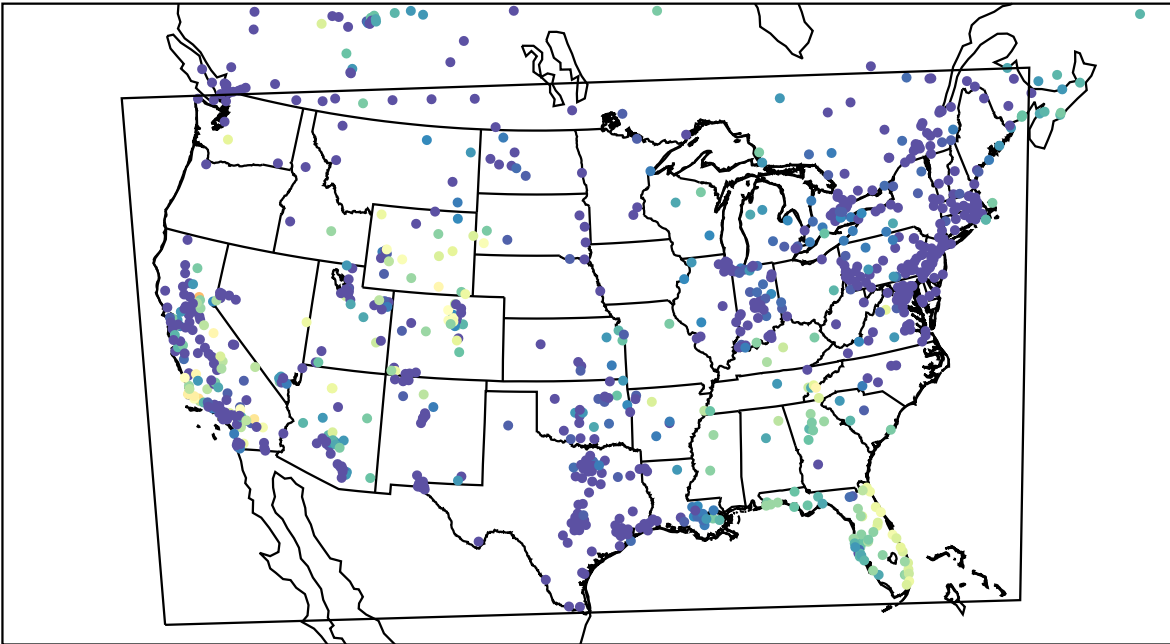
AirNOW (2023-11-15_14:00:00)
