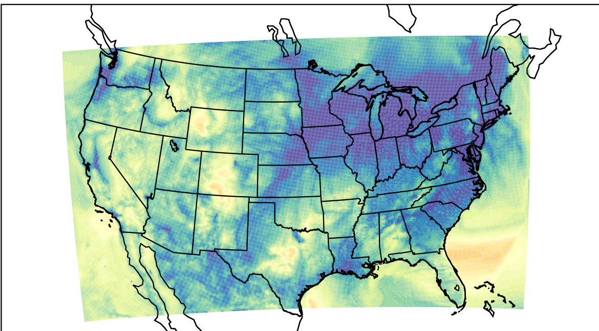
WRF (2023-11-15_09:00:00)
