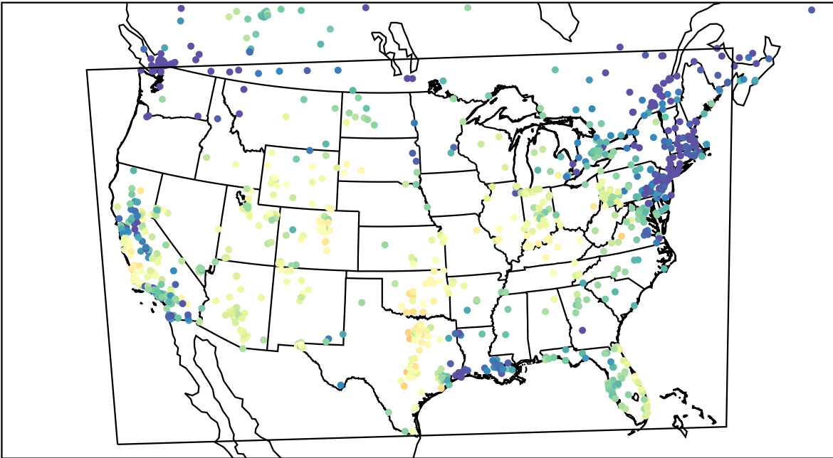
AirNOW (2023-11-15_21:00:00)
