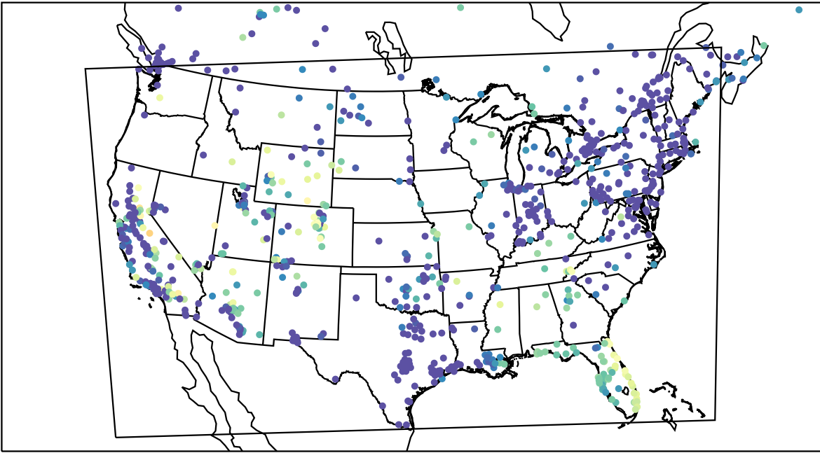
AirNOW (2023-11-15_10:00:00)
