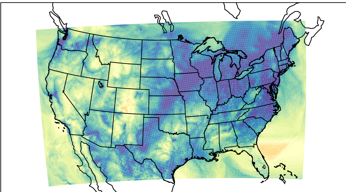
WRF (2023-11-15_14:00:00)
