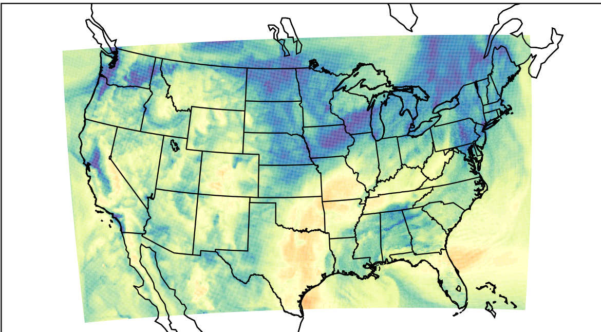
WRF (2023-11-15_18:00:00)
