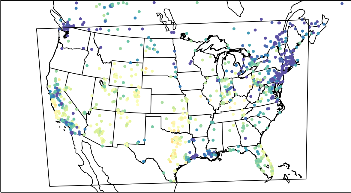
AirNOW (2023-11-15_22:00:00)
