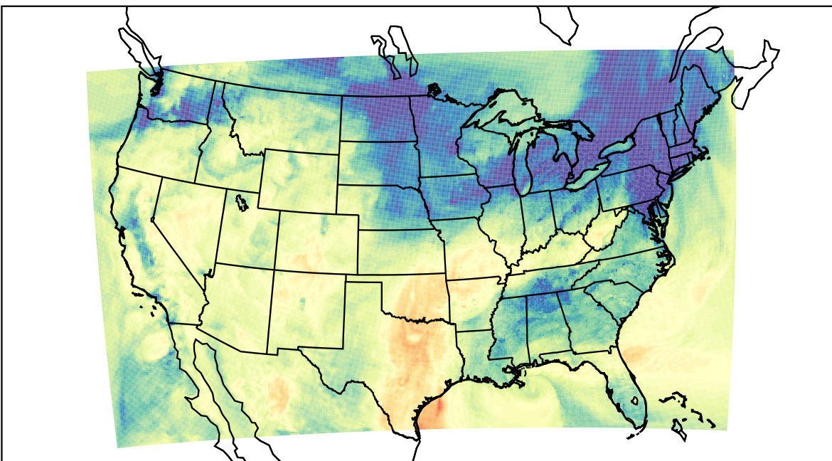
WRF (2023-11-15_22:00:00)
