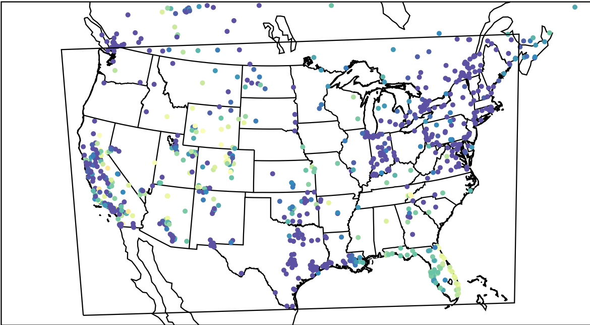
AirNOW (2023-11-15_08:00:00)
