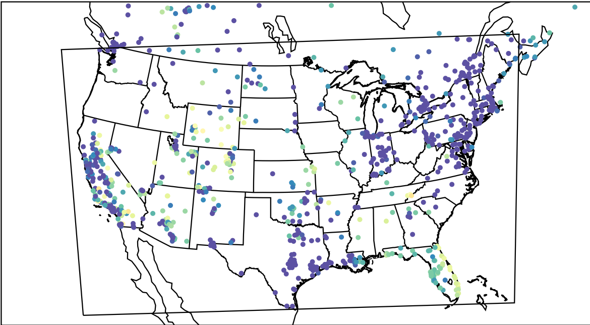
AirNOW (2023-11-15_07:00:00)
