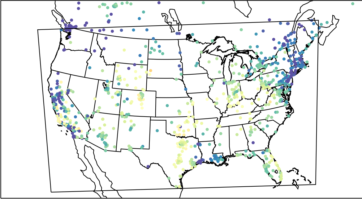
AirNOW (2023-11-15_18:00:00)
