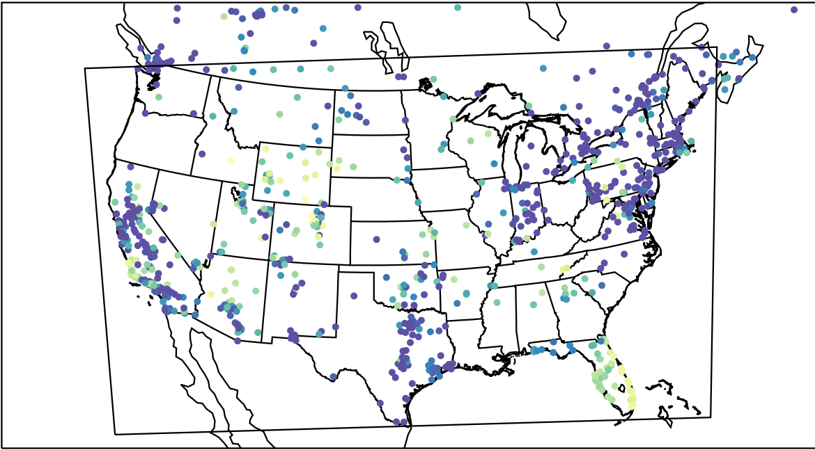
AirNOW (2023-11-16_07:00:00)
