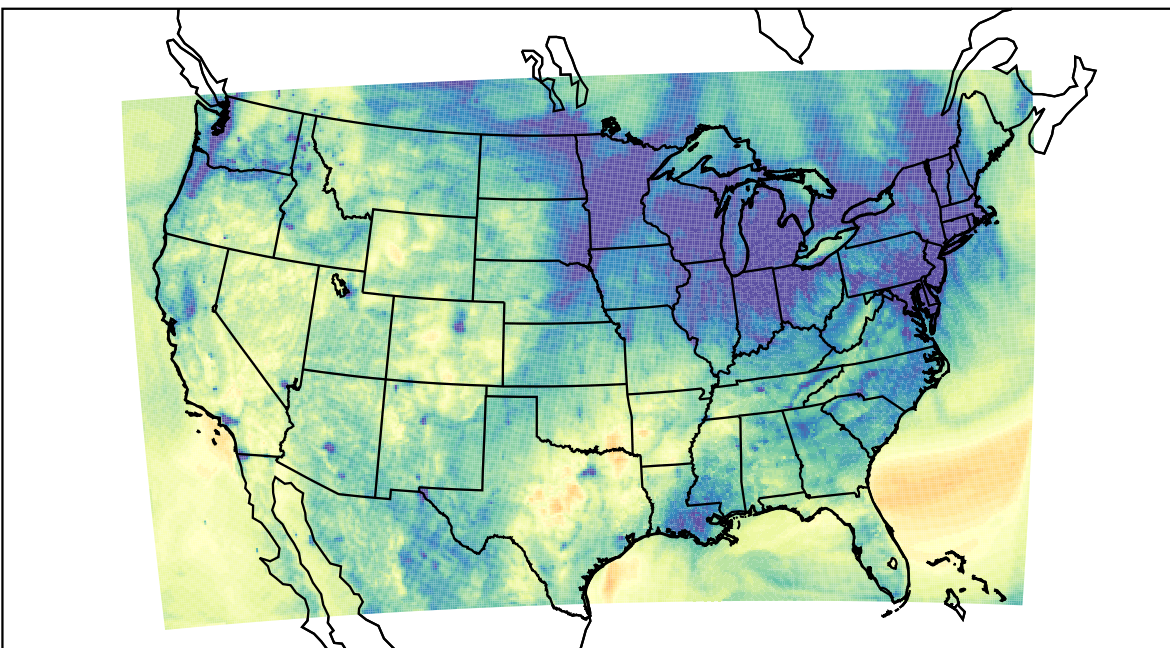
WRF (2023-11-15_02:00:00)
