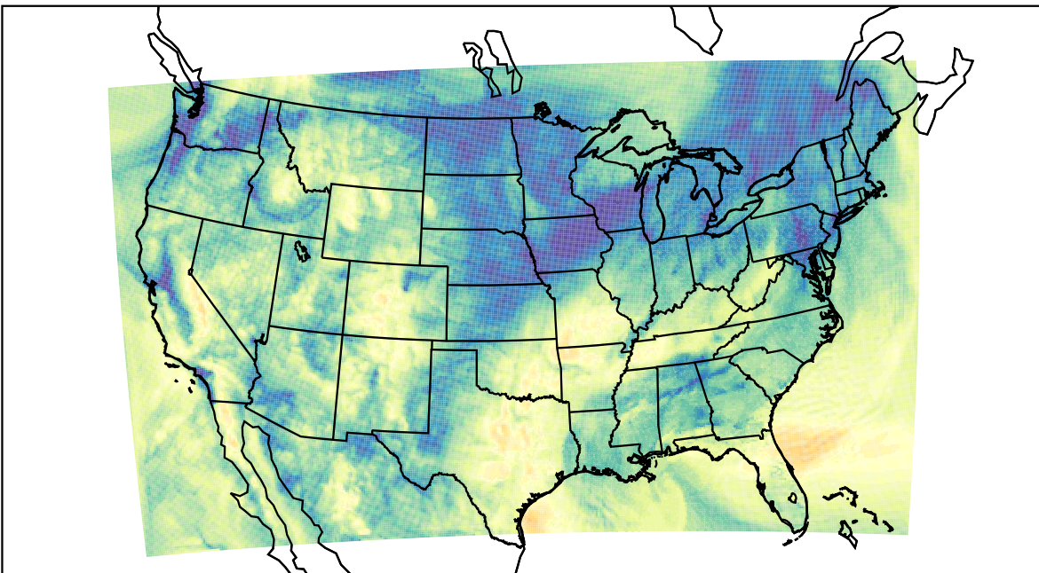
WRF (2023-11-15_17:00:00)
