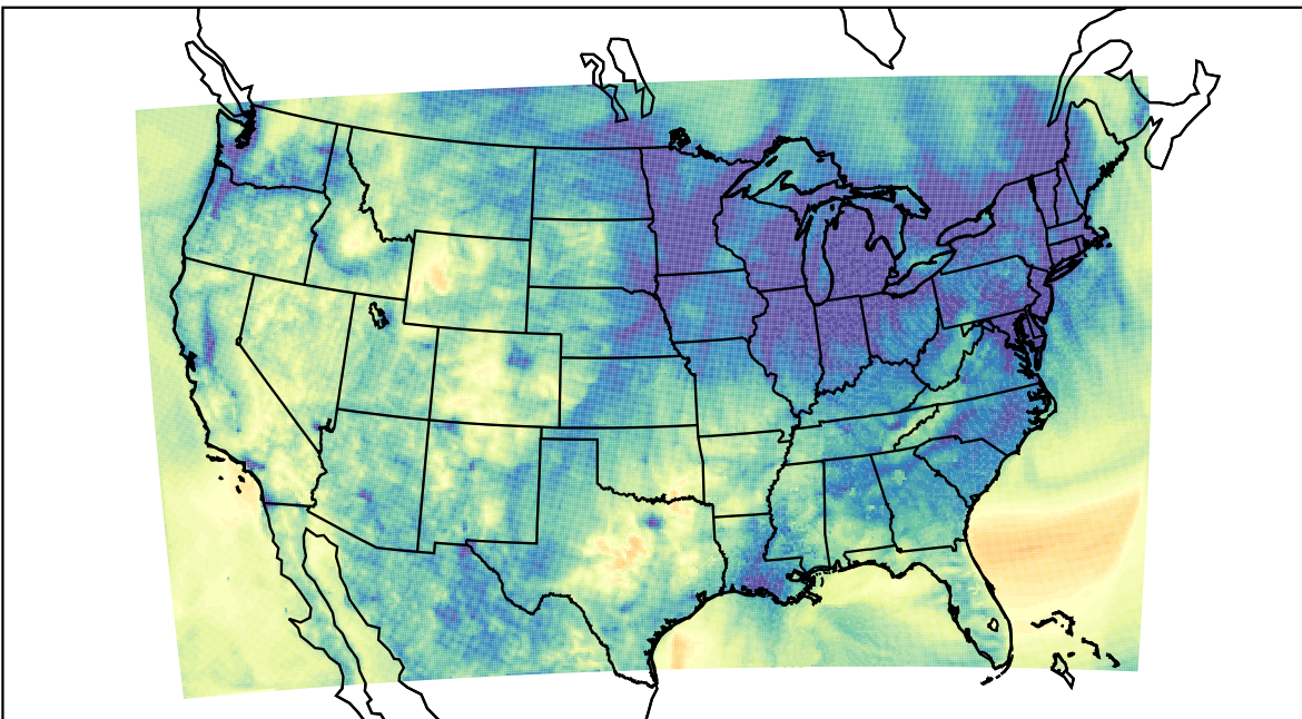
WRF (2023-11-15_05:00:00)
