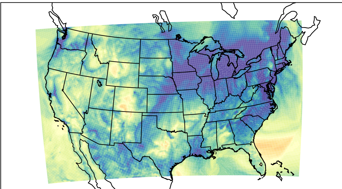
WRF (2023-11-15_10:00:00)
