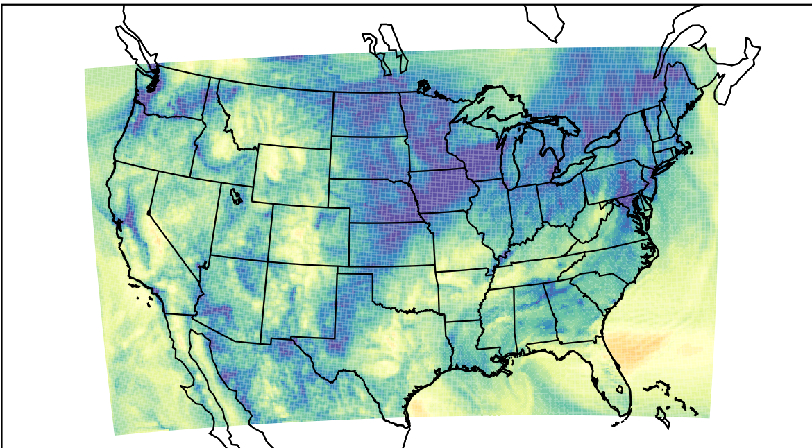
WRF (2023-11-15_16:00:00)
