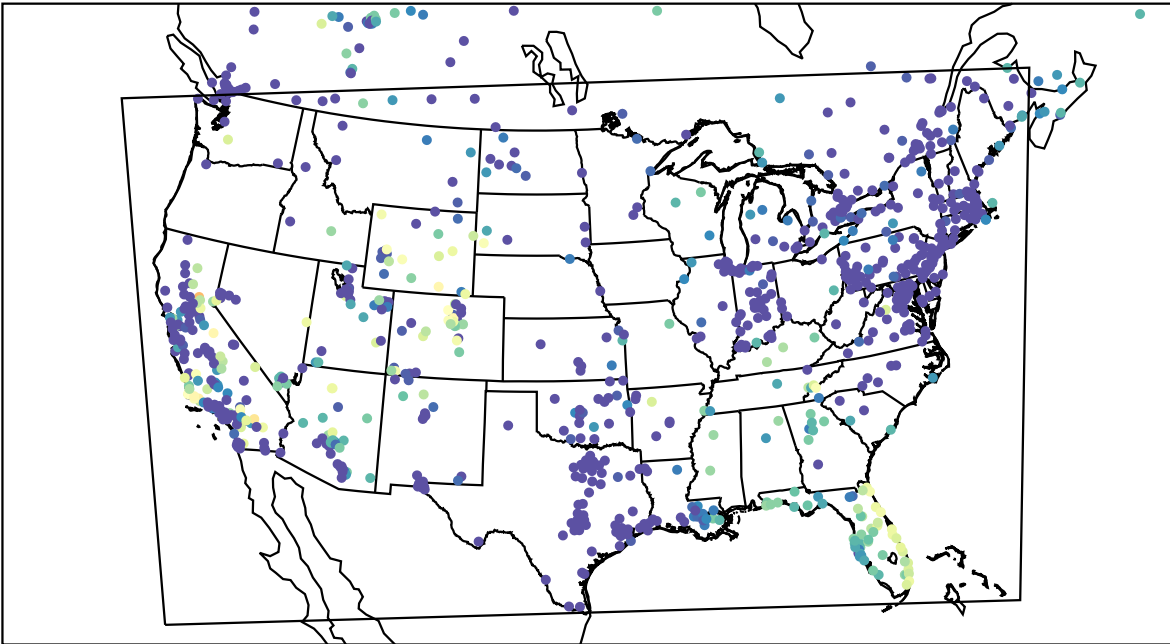
AirNOW (2023-11-15_13:00:00)
