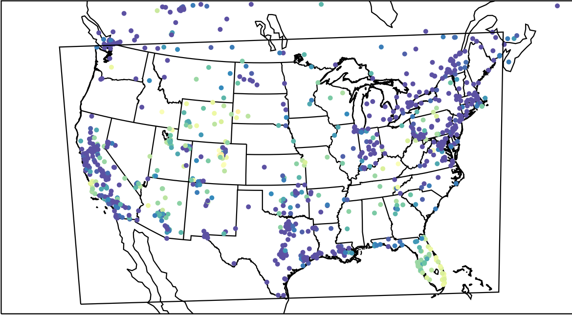
AirNOW (2023-11-16_09:00:00)
