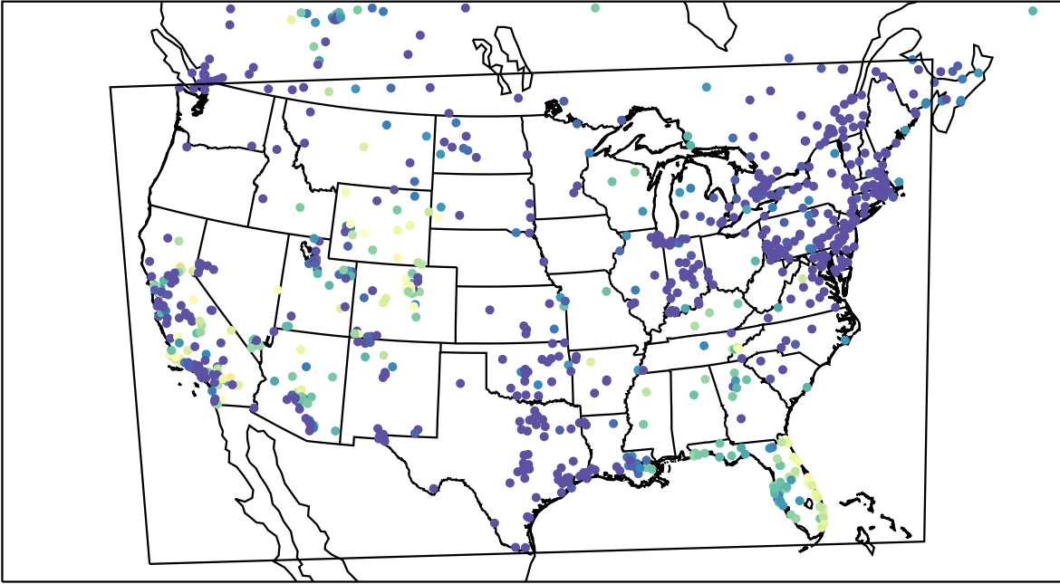
AirNOW (2023-11-15_12:00:00)
