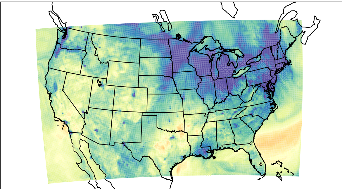
WRF (2023-11-15_01:00:00)
