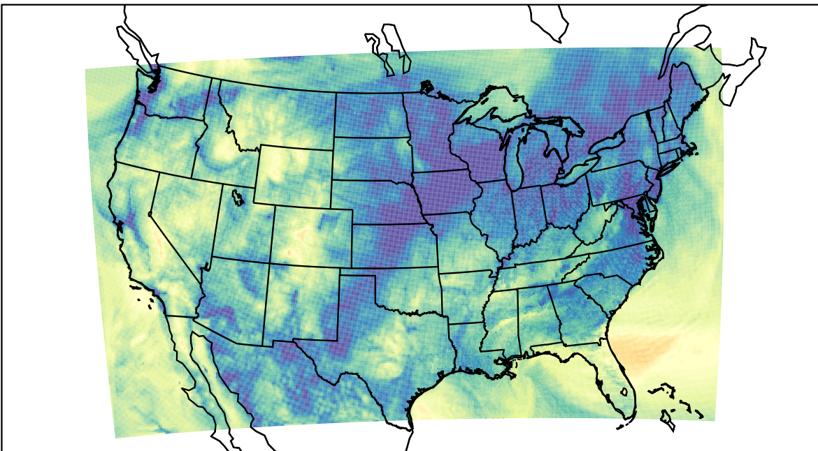
WRF (2023-11-15_15:00:00)
