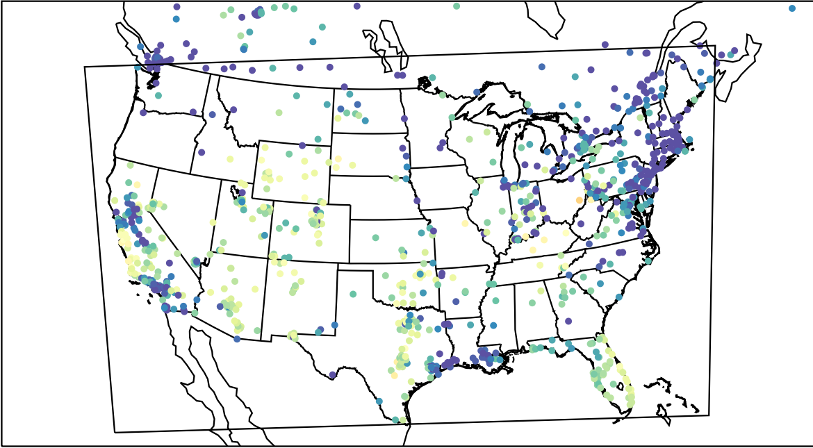
AirNOW (2023-11-15_23:00:00)
