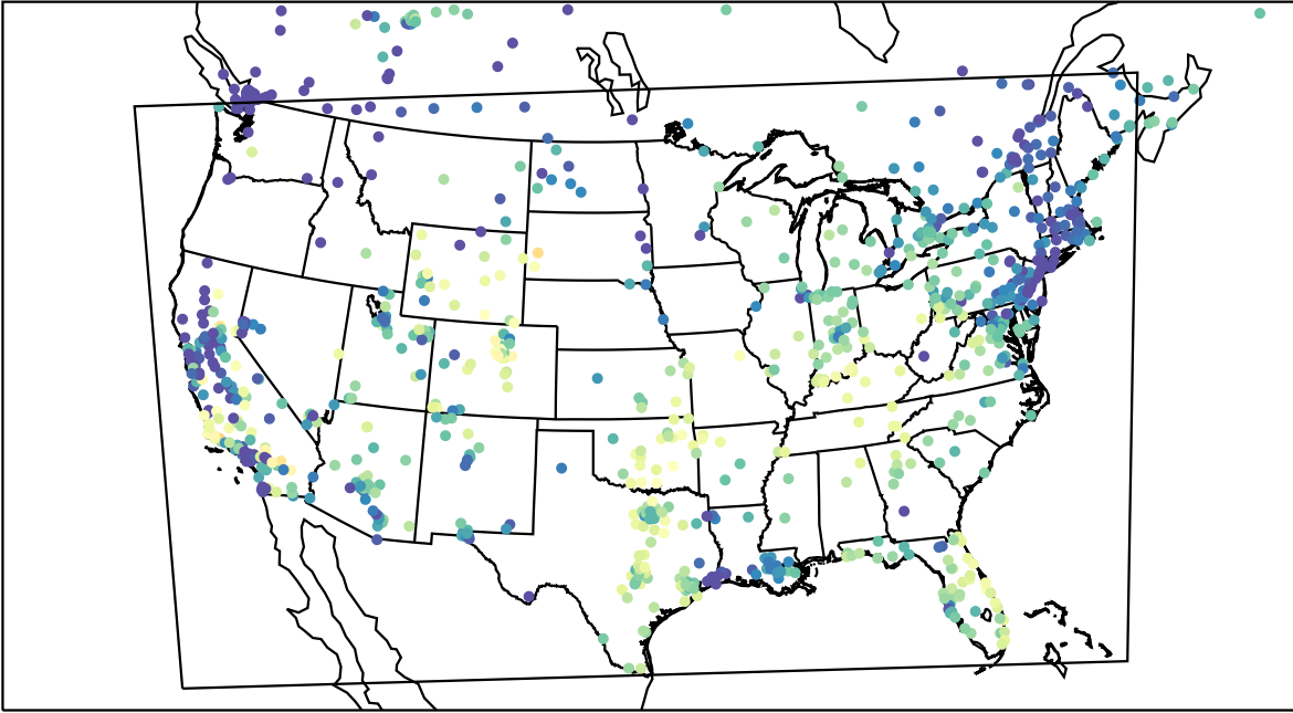
AirNOW (2023-11-15_17:00:00)
