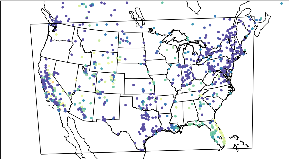
AirNOW (2023-11-15_09:00:00)
