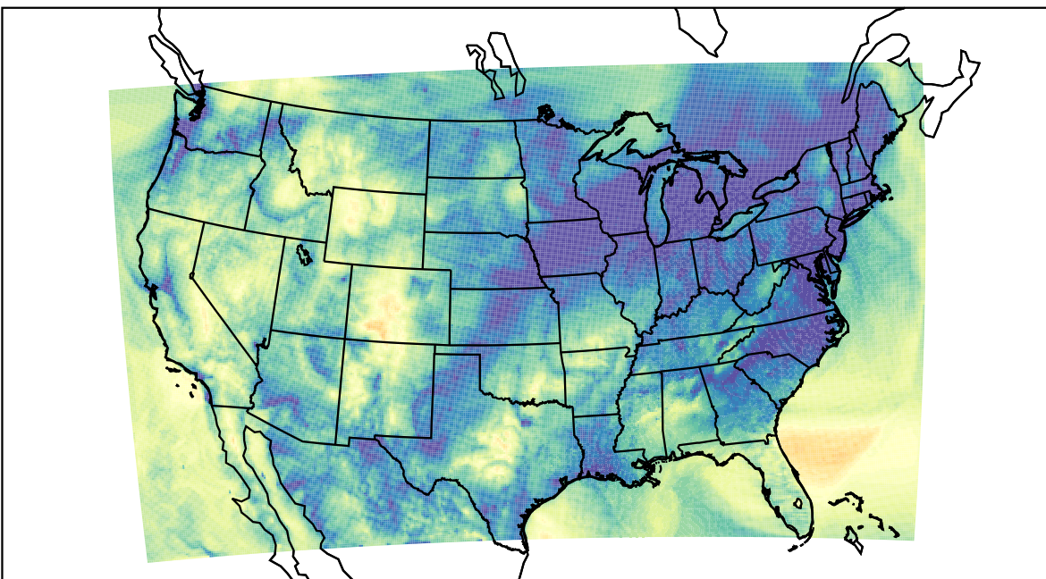
WRF (2023-11-15_13:00:00)
