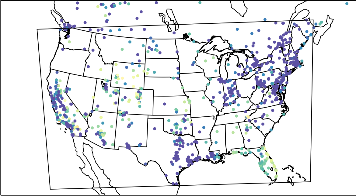
AirNOW (2023-11-15_05:00:00)
