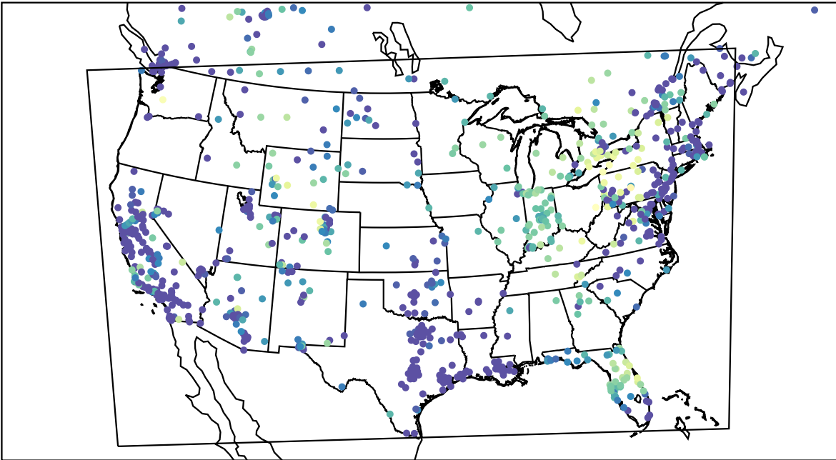
AirNOW (2023-11-17_05:00:00)
