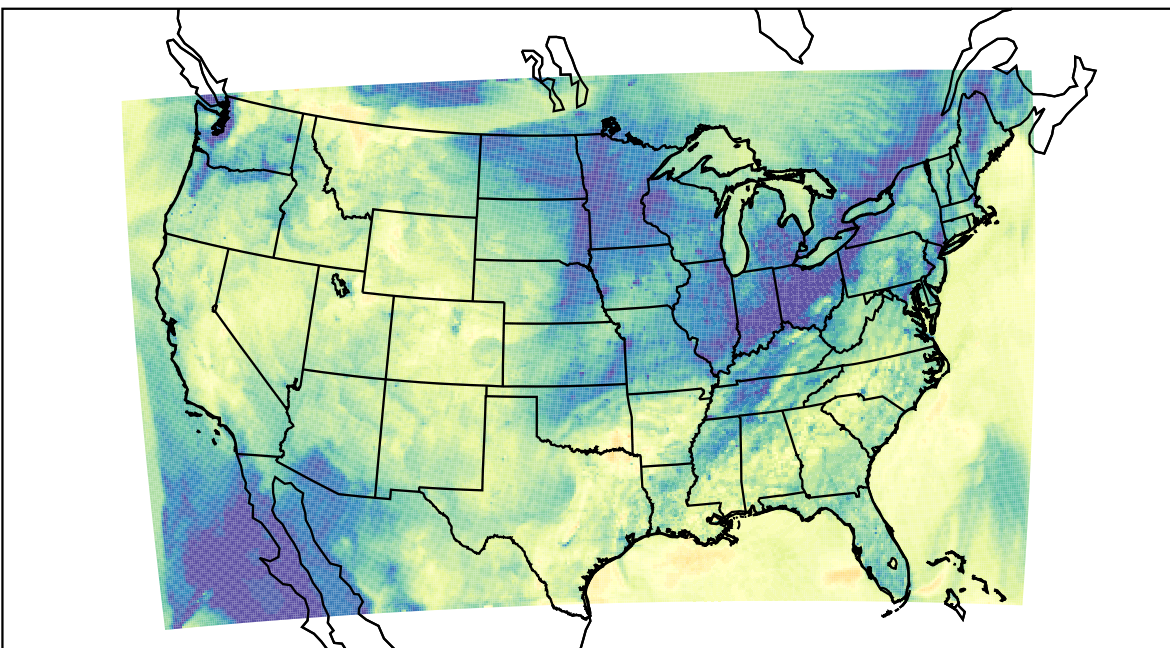
WRF (2023-11-17_23:00:00)
