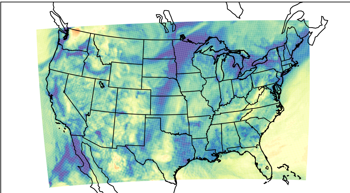
WRF (2023-11-16_16:00:00)
