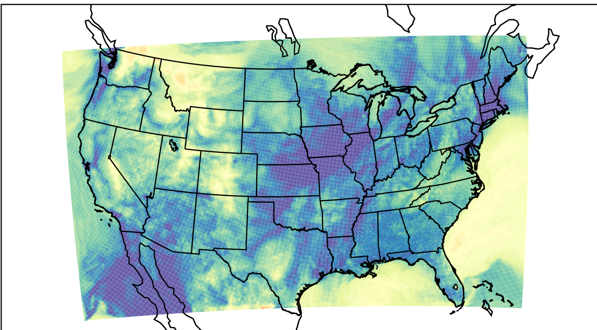
WRF (2023-11-17_10:00:00)
