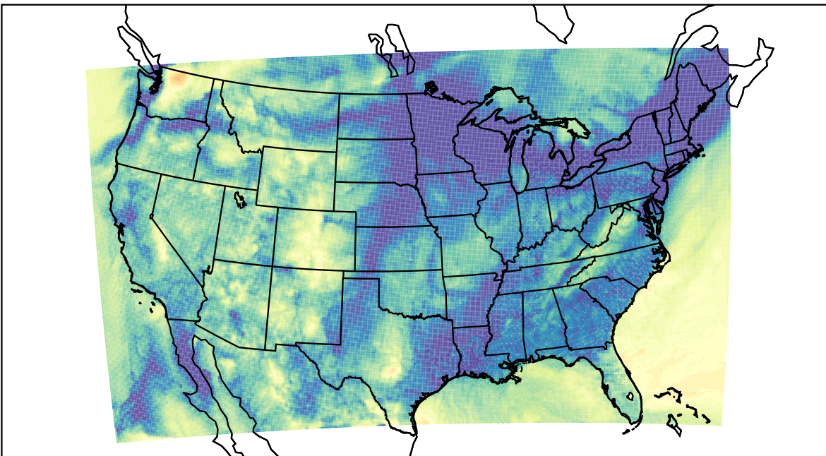
WRF (2023-11-16_12:00:00)
