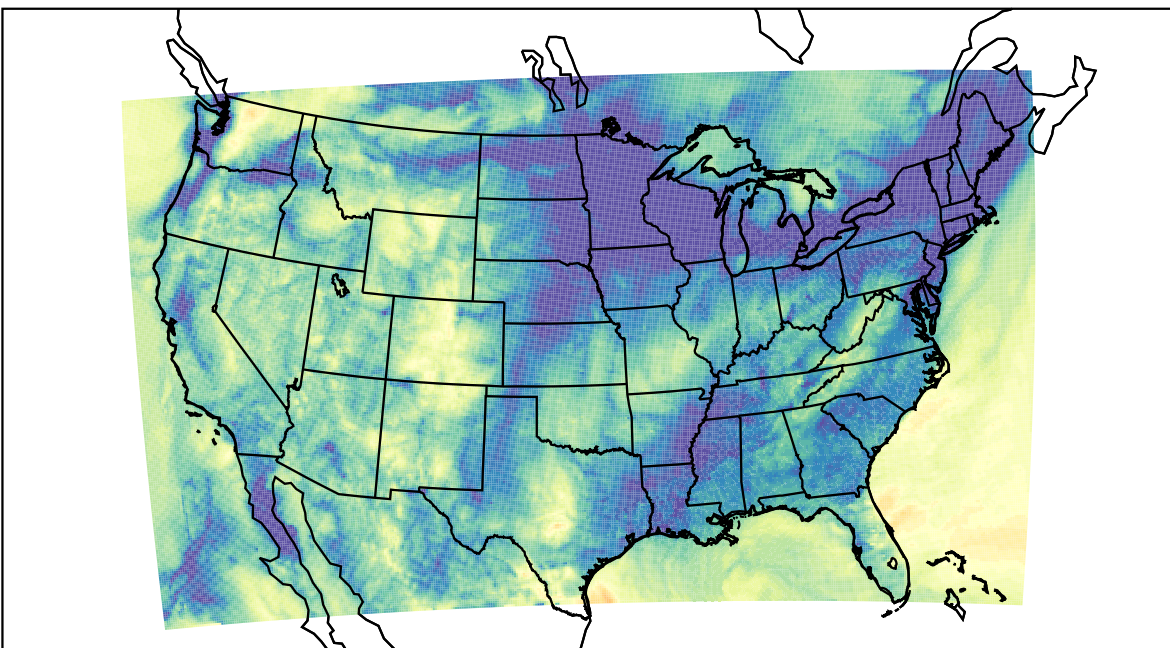
WRF (2023-11-16_09:00:00)
