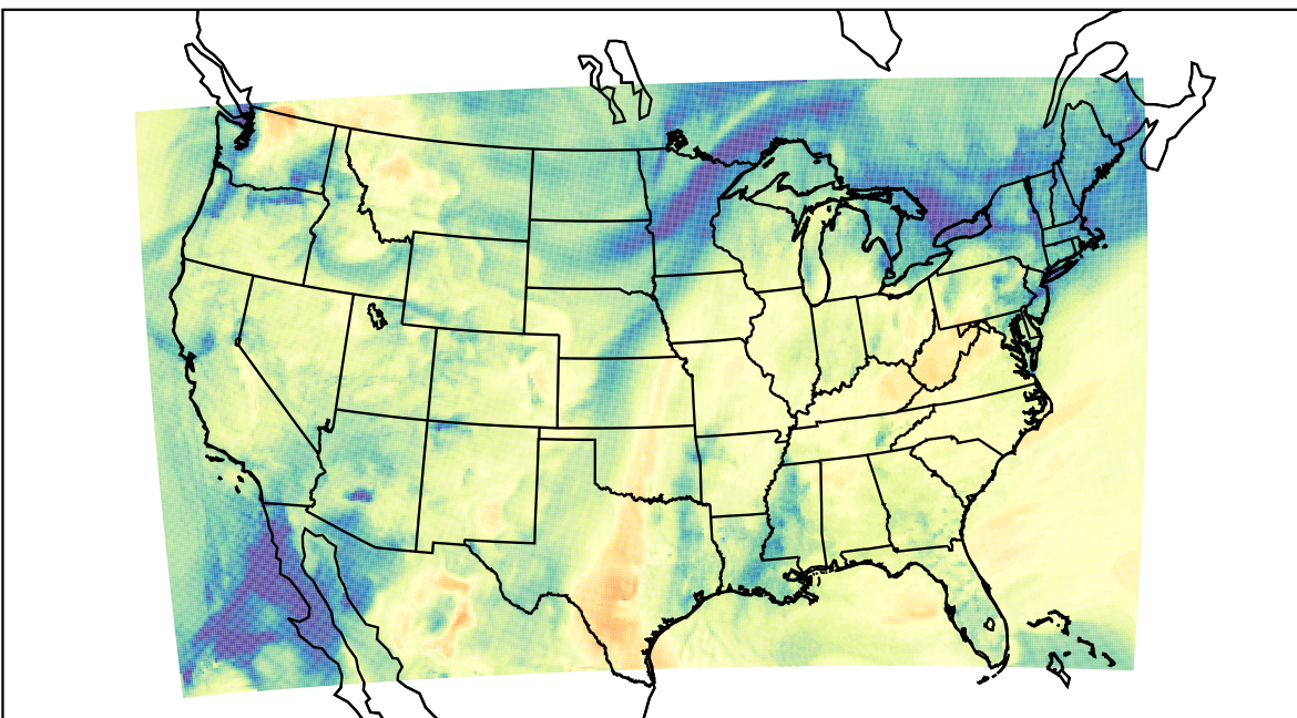
WRF (2023-11-16_20:00:00)
