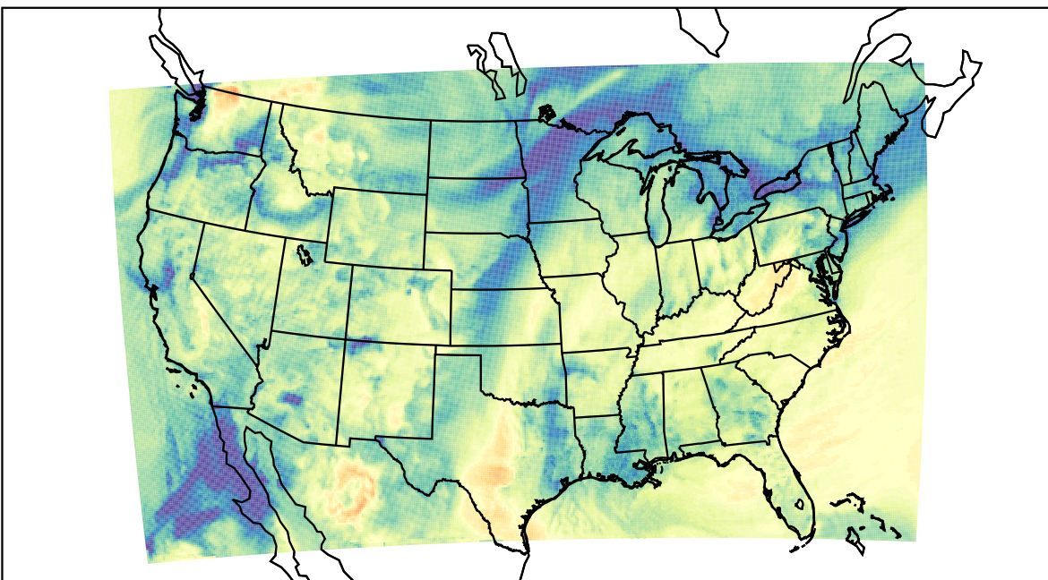
WRF (2023-11-16_18:00:00)
