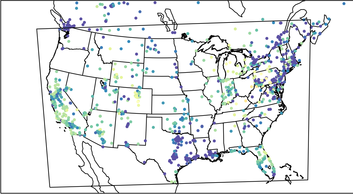
AirNOW (2023-11-17_00:00:00)
