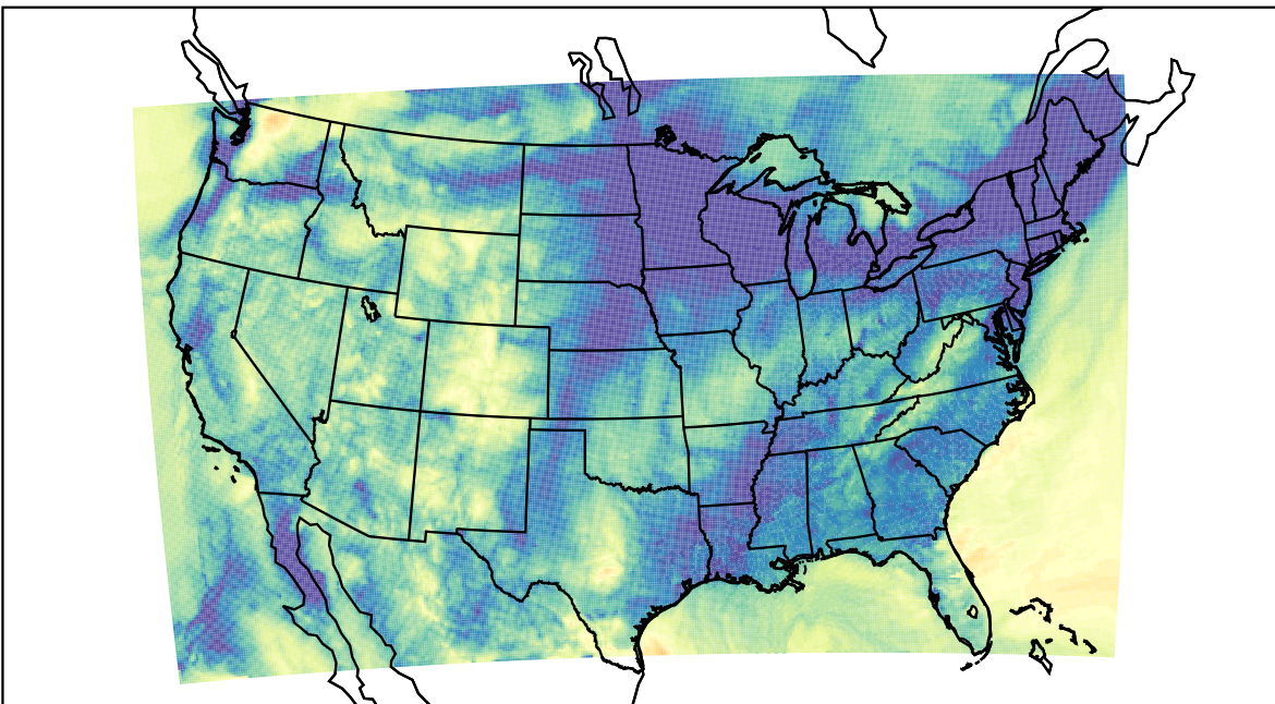
WRF (2023-11-16_10:00:00)
