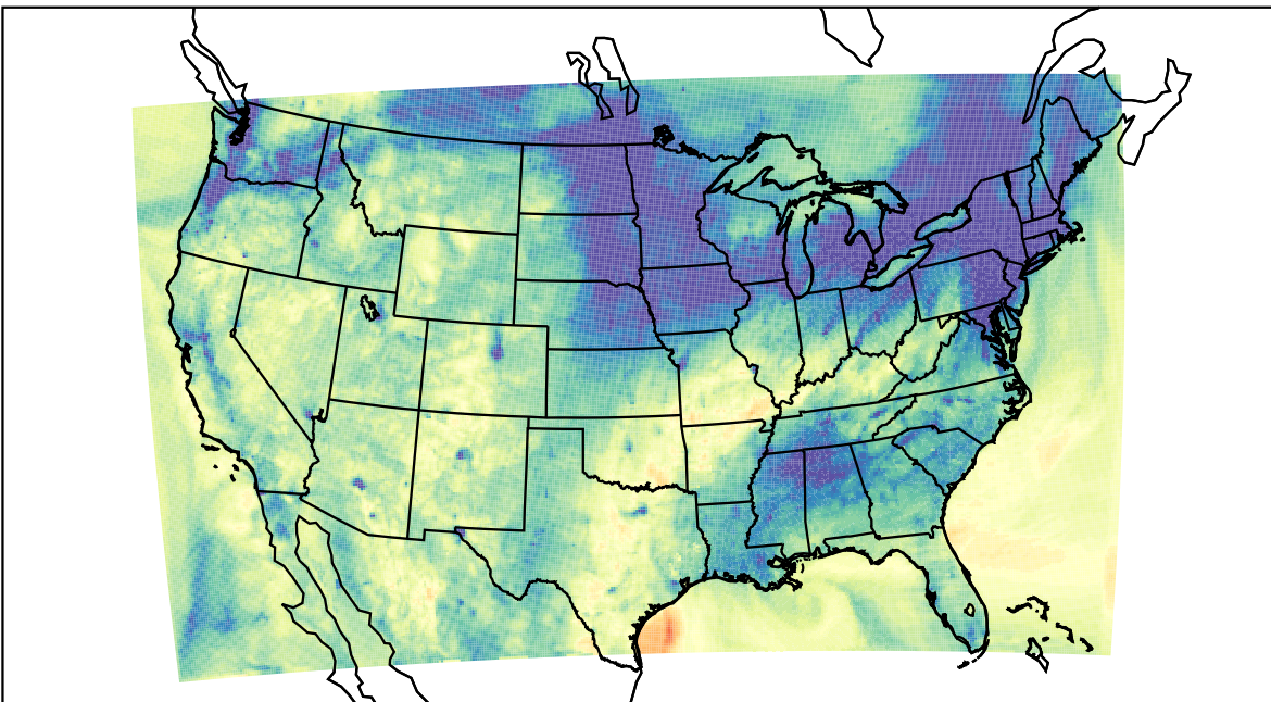
WRF (2023-11-16_01:00:00)
