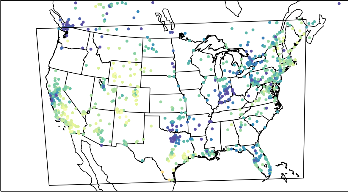
AirNOW (2023-11-17_22:00:00)
