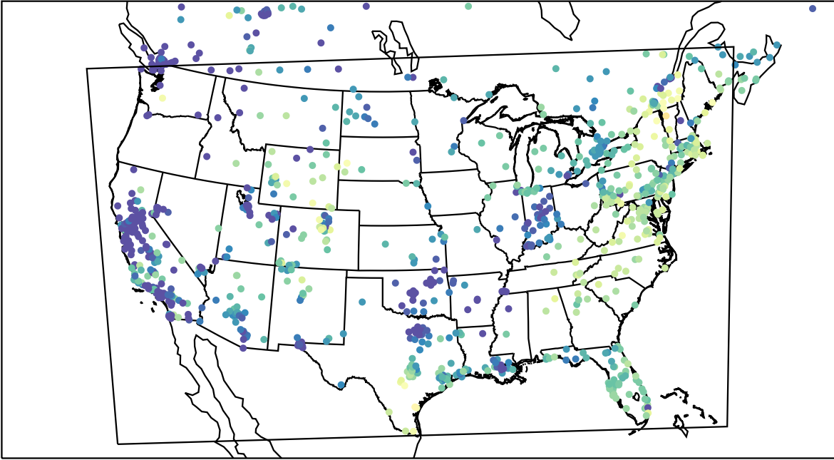
AirNOW (2023-11-17_17:00:00)
