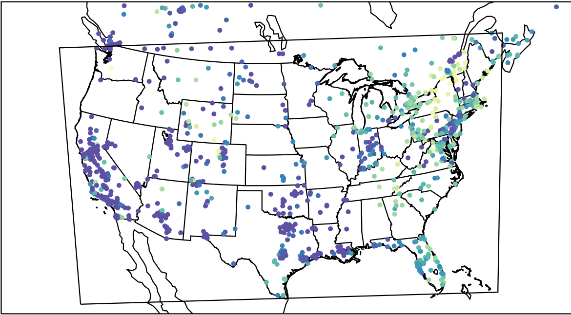
AirNOW (2023-11-17_15:00:00)
