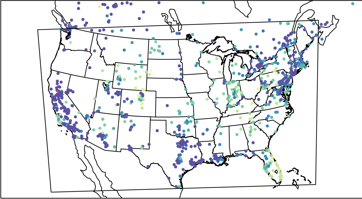
AirNOW (2023-11-16_15:00:00)
