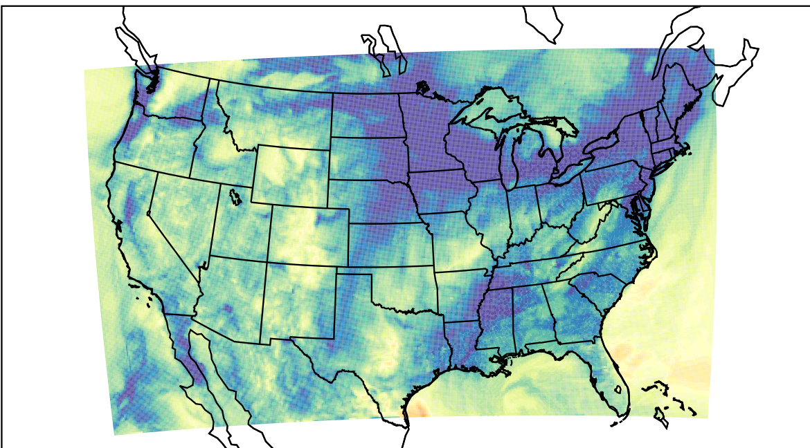
WRF (2023-11-16_07:00:00)
