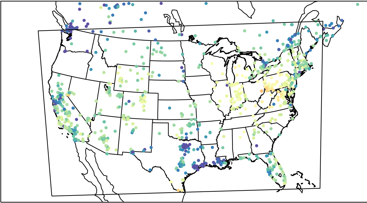
AirNOW (2023-11-16_19:00:00)
