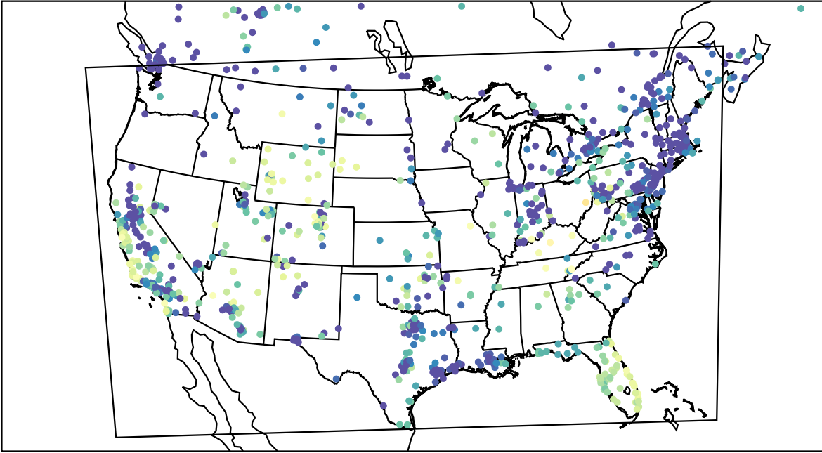
AirNOW (2023-11-16_01:00:00)
