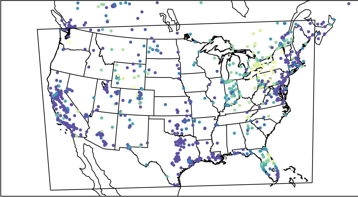
AirNOW (2023-11-17_08:00:00)
