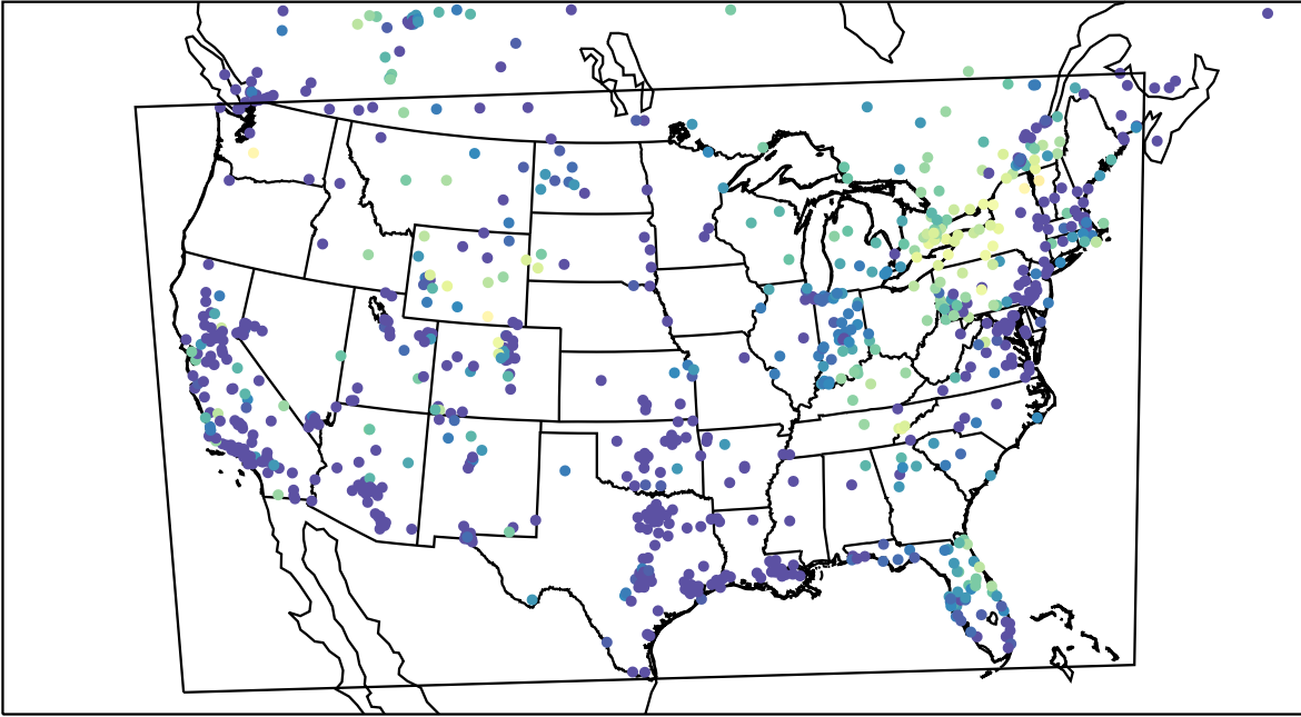
AirNOW (2023-11-17_11:00:00)
