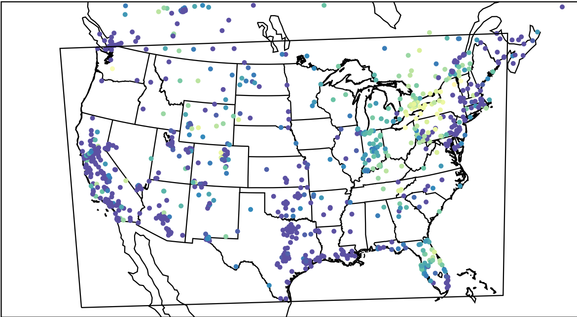
AirNOW (2023-11-17_09:00:00)
