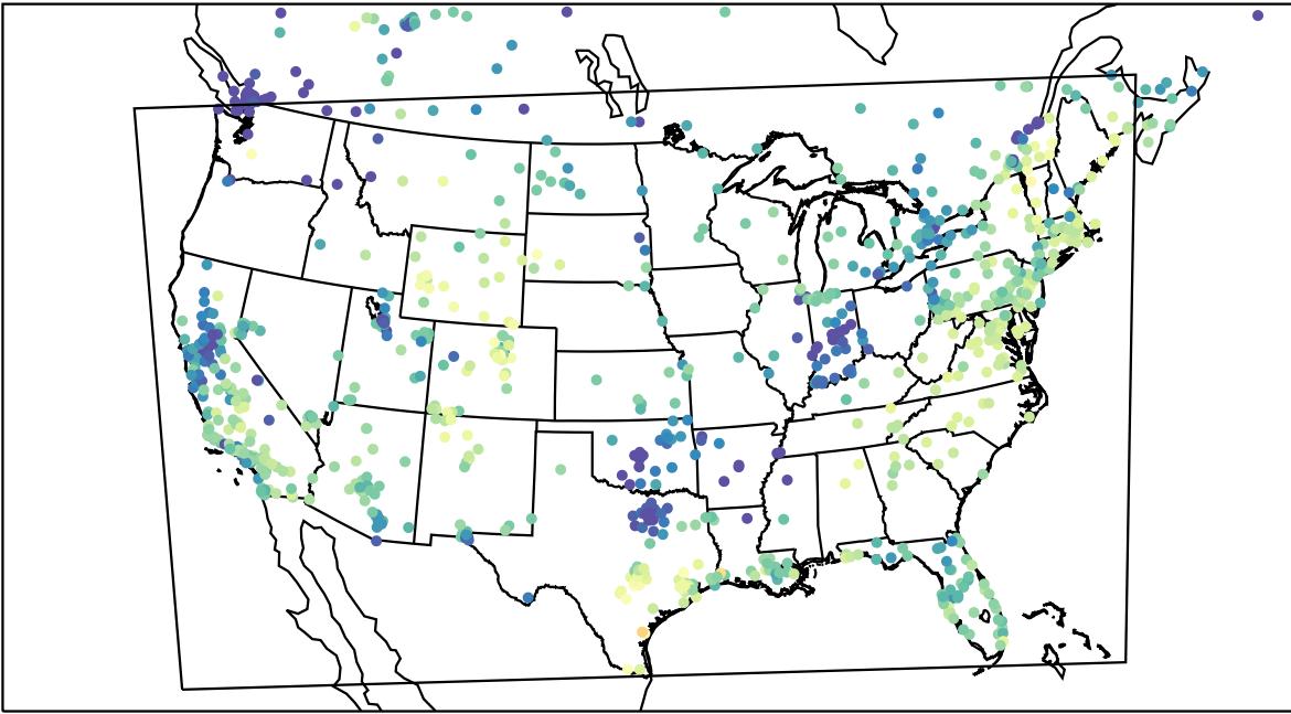
AirNOW (2023-11-17_19:00:00)
