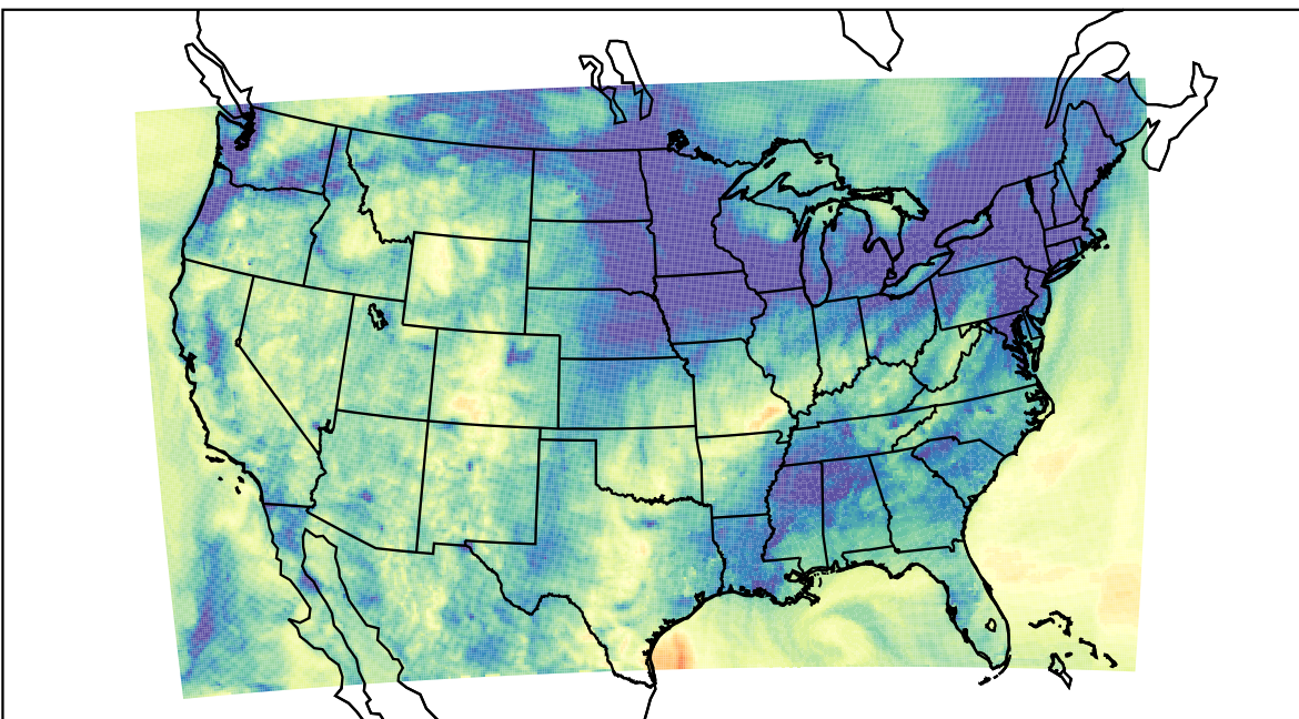
WRF (2023-11-16_04:00:00)
