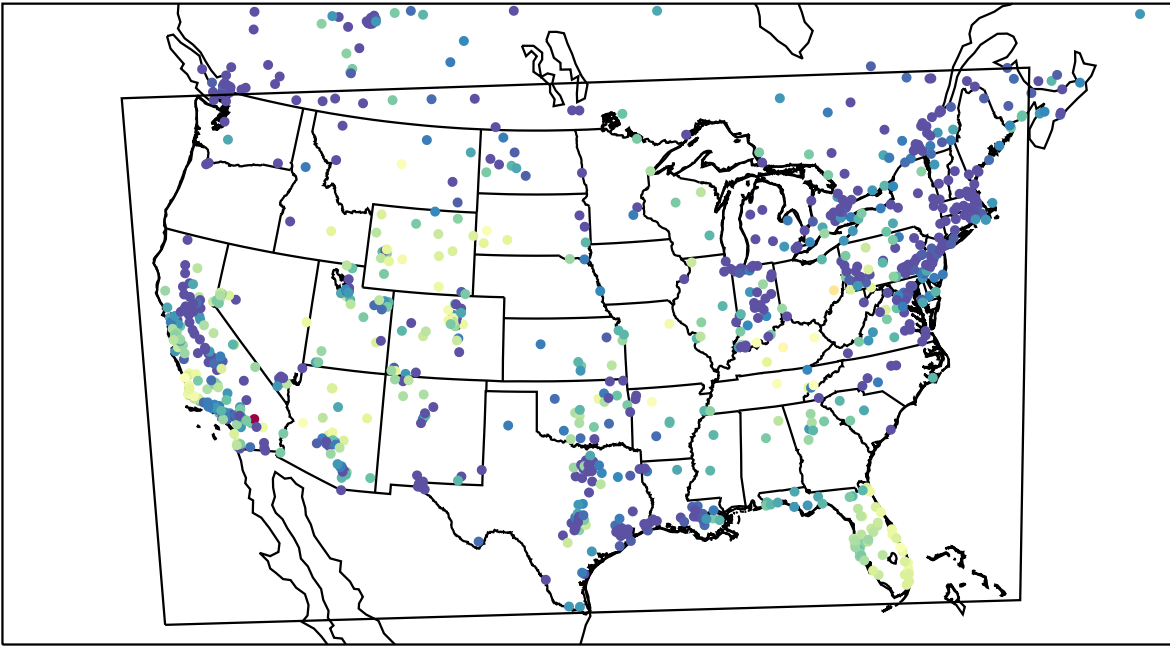
AirNOW (2023-11-16_02:00:00)
