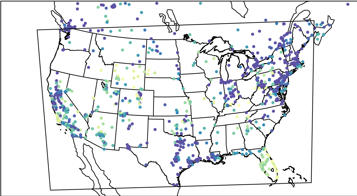
AirNOW (2023-11-16_05:00:00)
