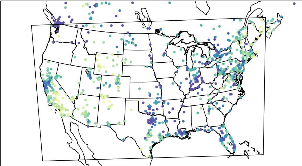
AirNOW (2023-11-17_23:00:00)
