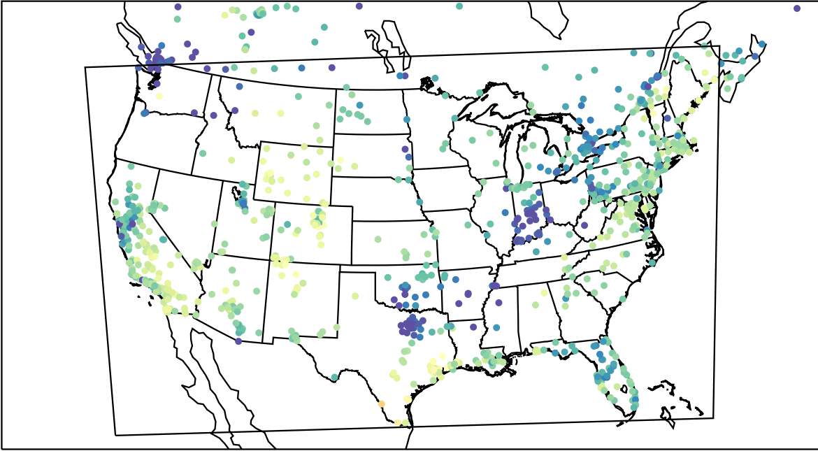
AirNOW (2023-11-17_21:00:00)
