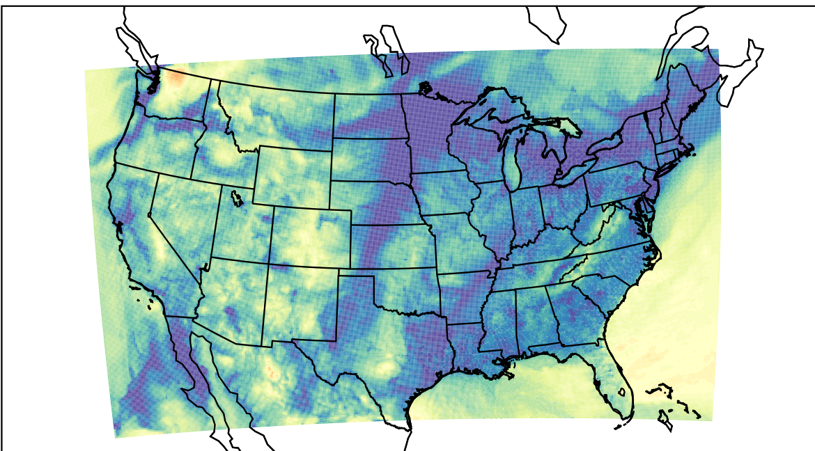
WRF (2023-11-16_14:00:00)
