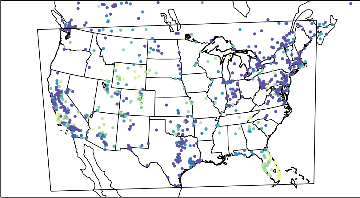
AirNOW (2023-11-16_07:00:00)
