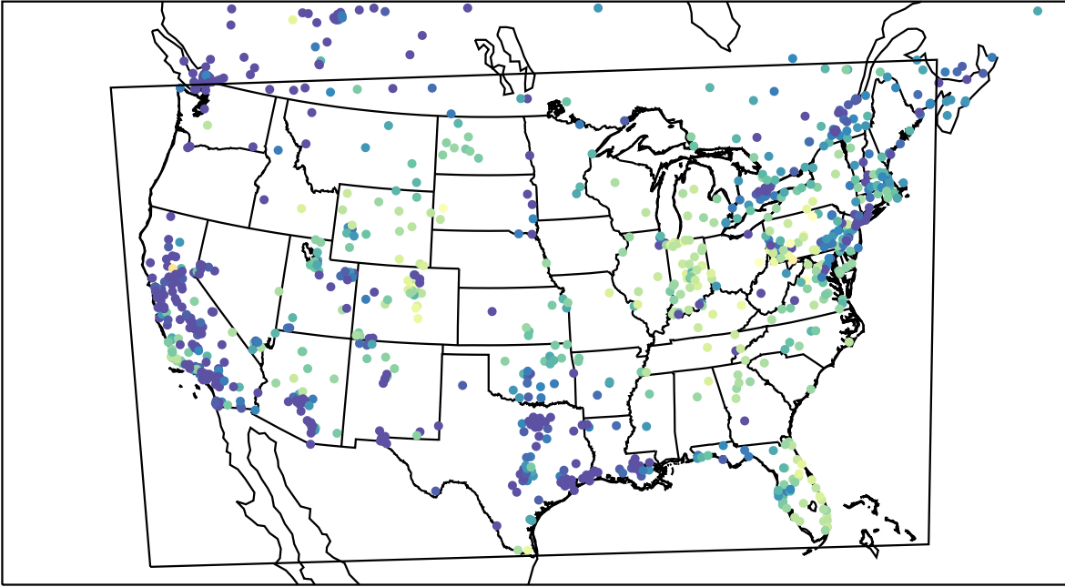
AirNOW (2023-11-16_16:00:00)
