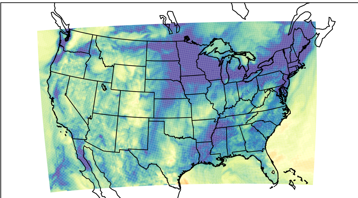
WRF (2023-11-16_08:00:00)
