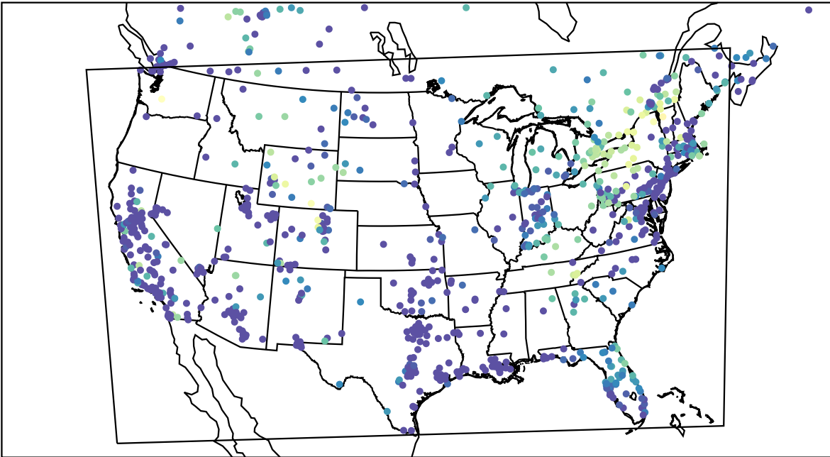
AirNOW (2023-11-17_13:00:00)
