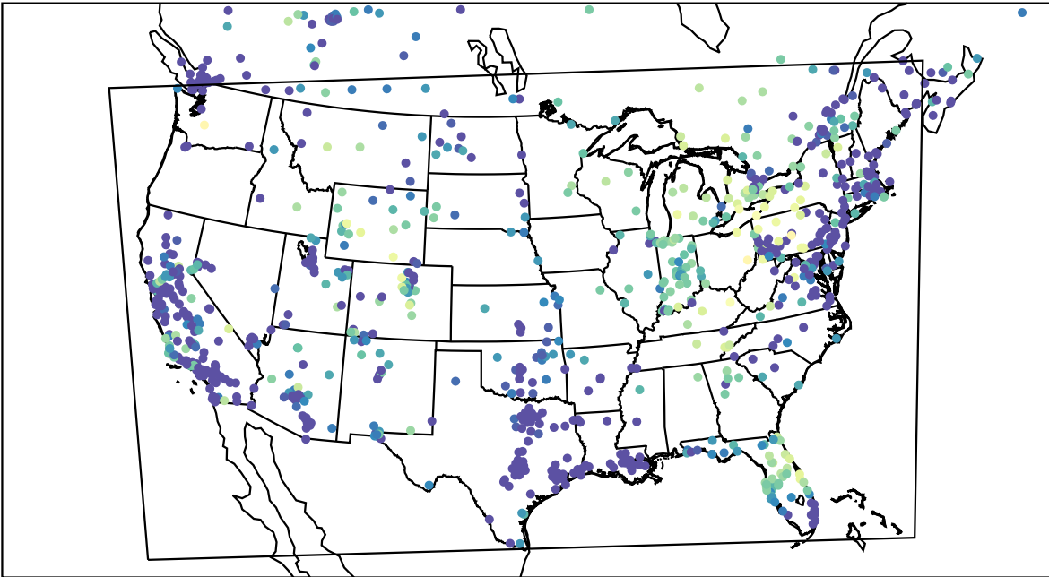
AirNOW (2023-11-17_04:00:00)
