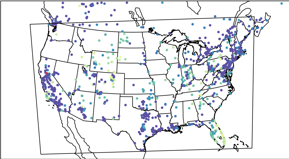
AirNOW (2023-11-16_14:00:00)
