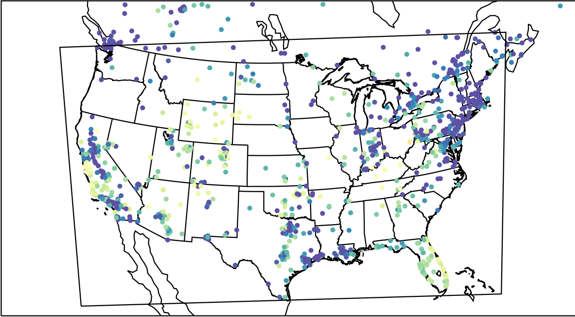
AirNOW (2023-11-16_00:00:00)
