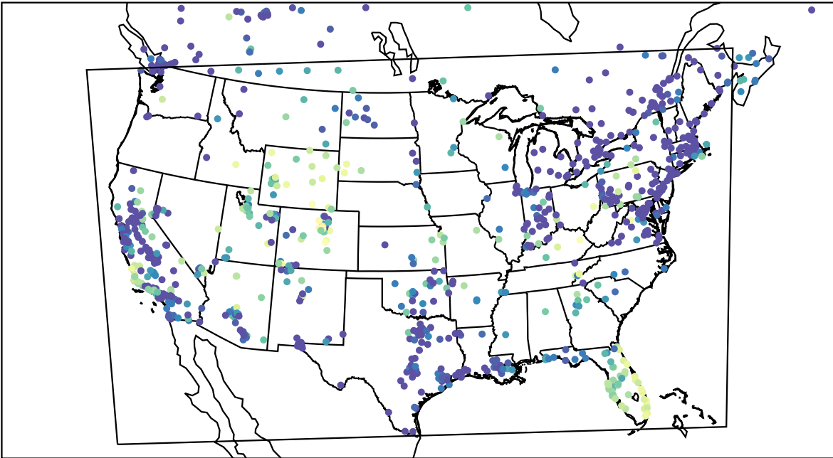
AirNOW (2023-11-16_08:00:00)
