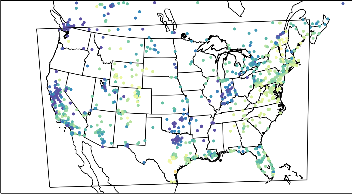
AirNOW (2023-11-17_18:00:00)
