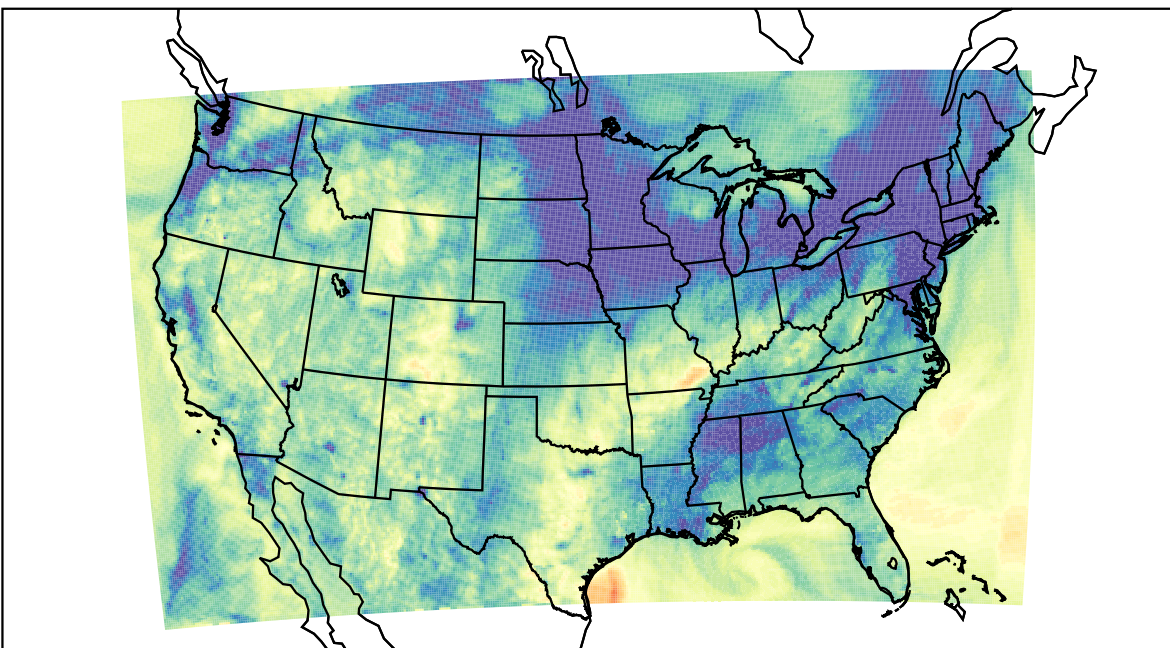
WRF (2023-11-16_03:00:00)
