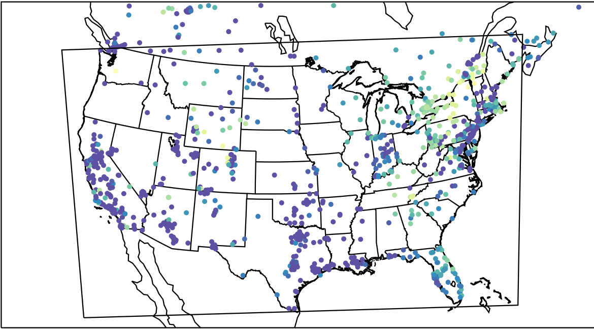
AirNOW (2023-11-17_14:00:00)
