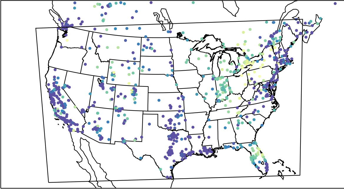
AirNOW (2023-11-17_06:00:00)
