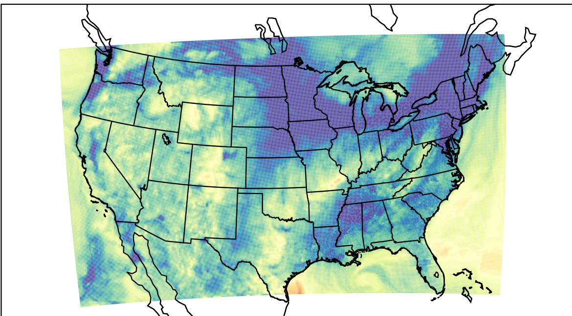
WRF (2023-11-16_05:00:00)
