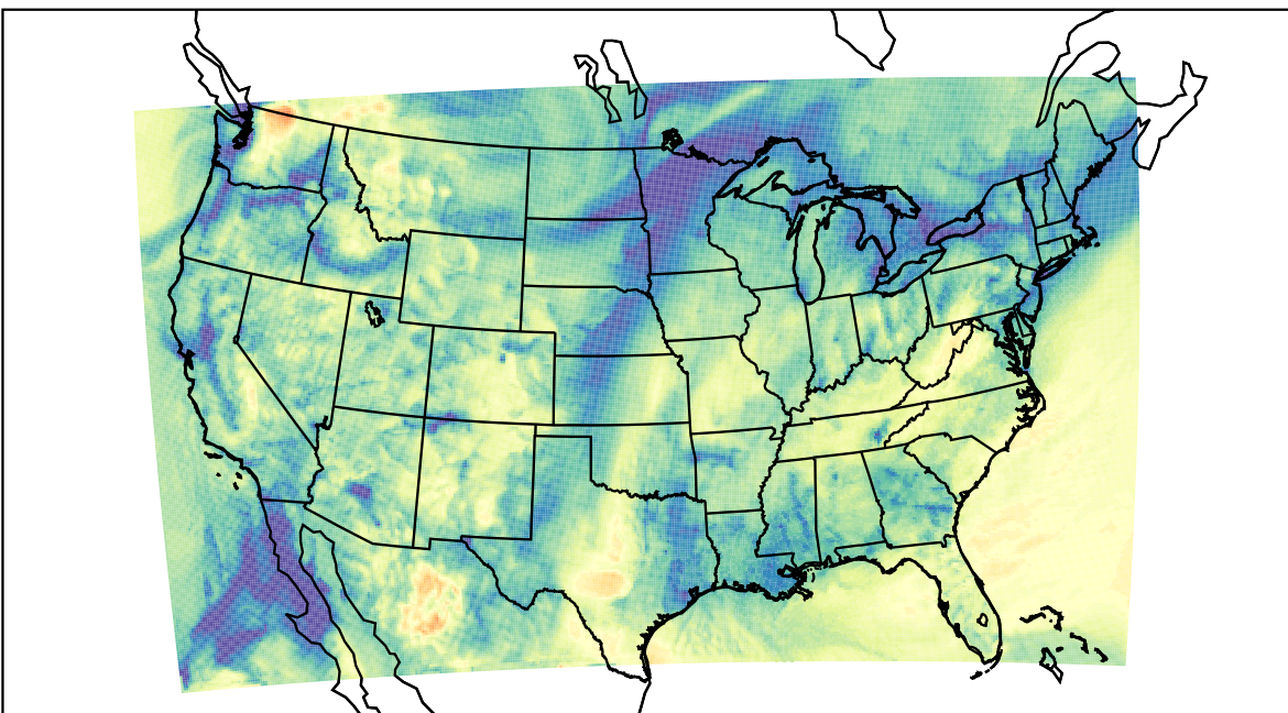
WRF (2023-11-16_17:00:00)
