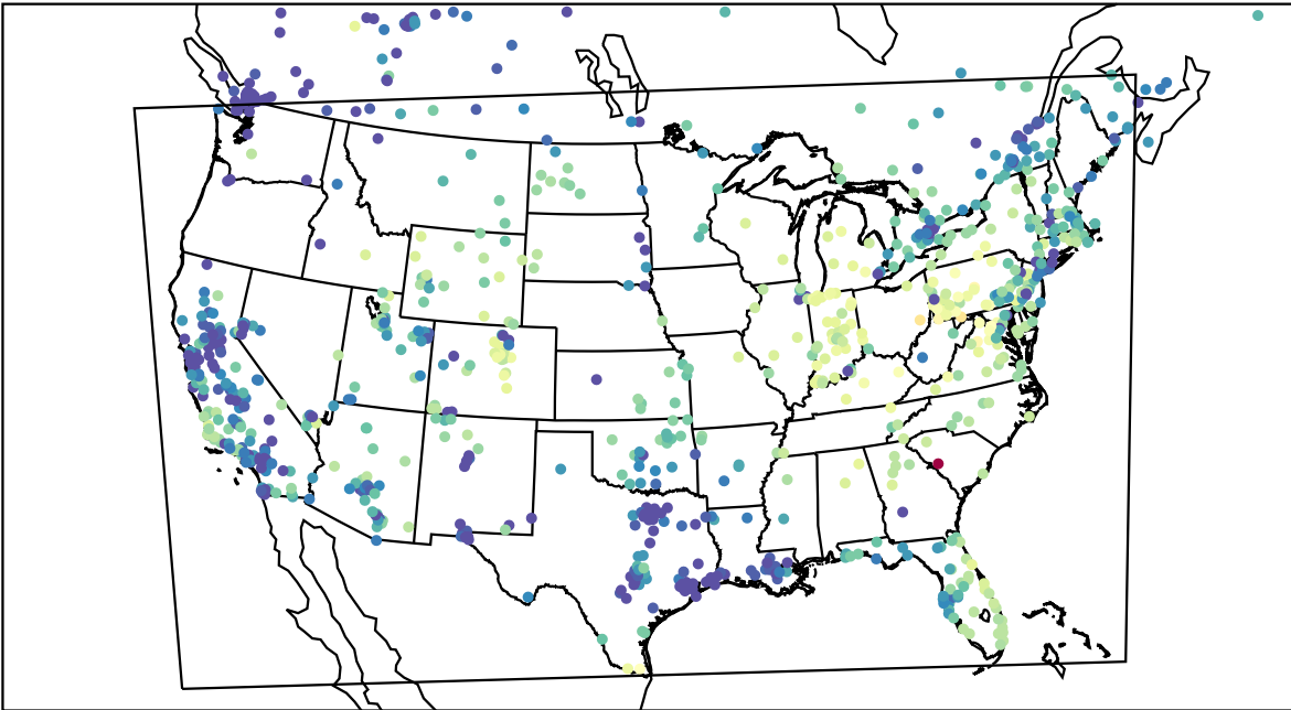
AirNOW (2023-11-16_17:00:00)
