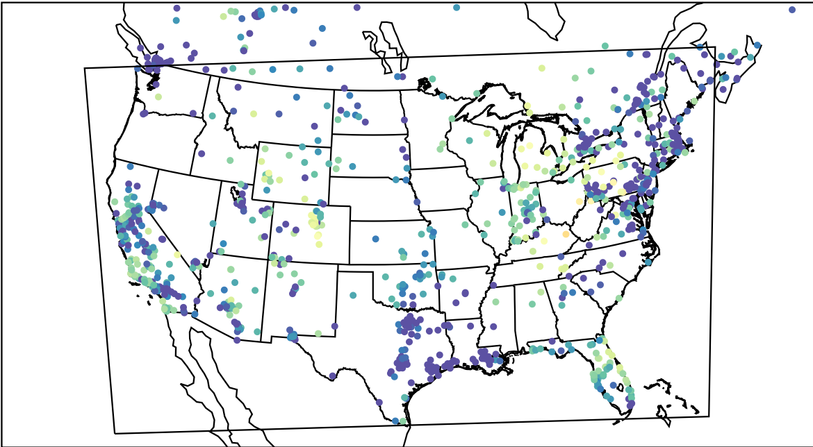
AirNOW (2023-11-17_01:00:00)
