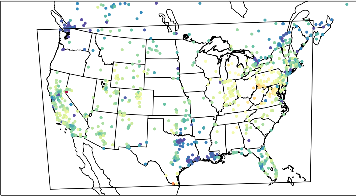
AirNOW (2023-11-16_20:00:00)
