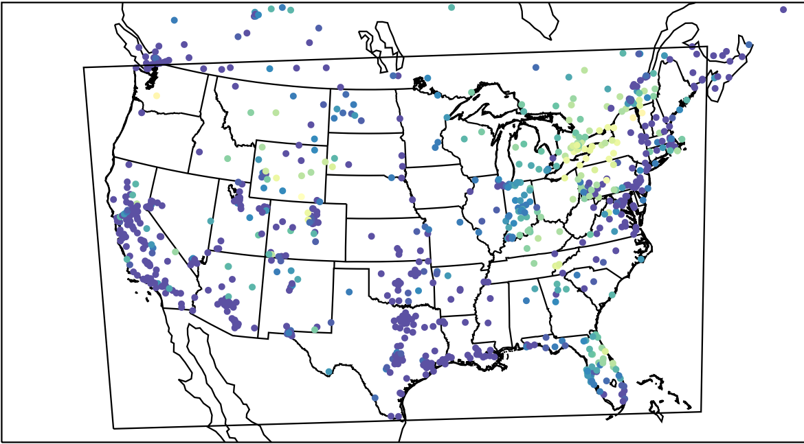
AirNOW (2023-11-17_10:00:00)
