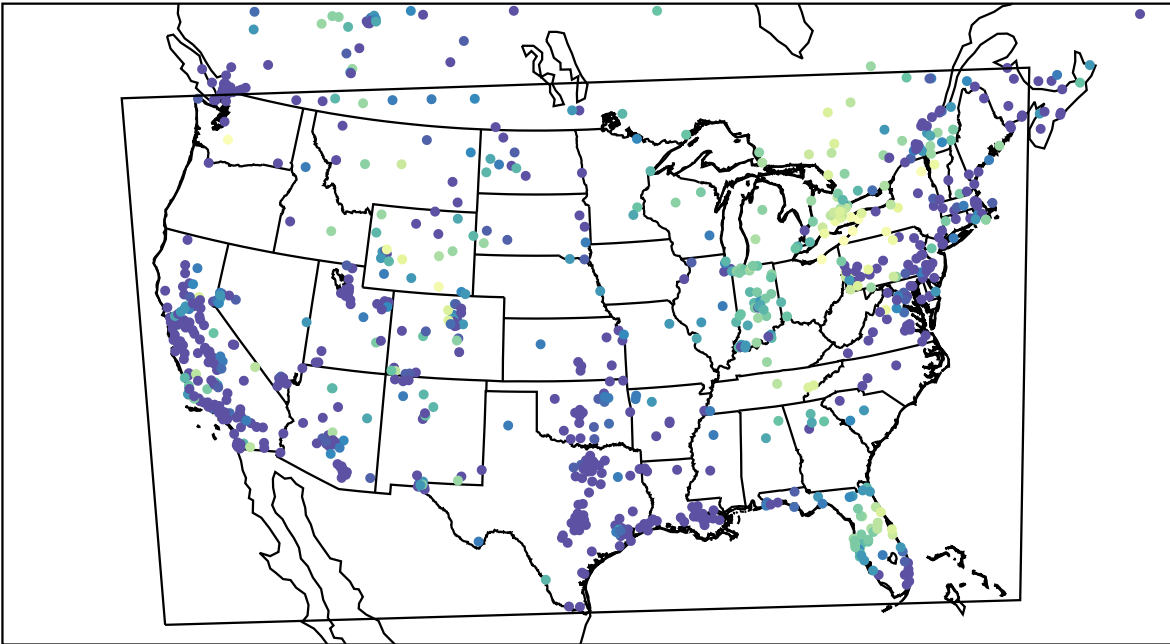
AirNOW (2023-11-17_07:00:00)
