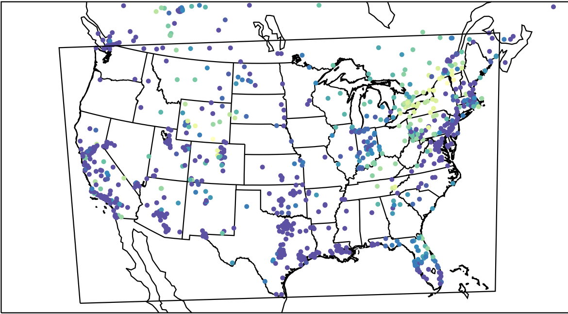
AirNOW (2023-11-17_12:00:00)
