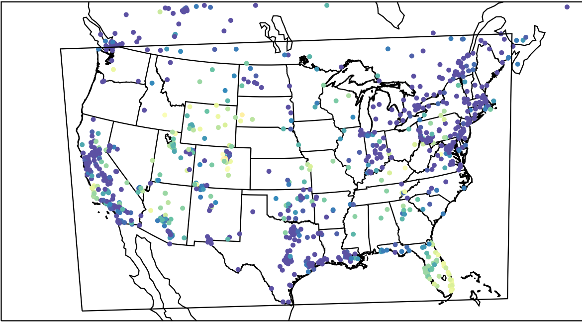
AirNOW (2023-11-16_09:00:00)
