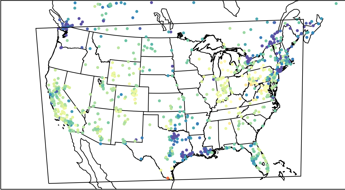
AirNOW (2023-11-16_21:00:00)
