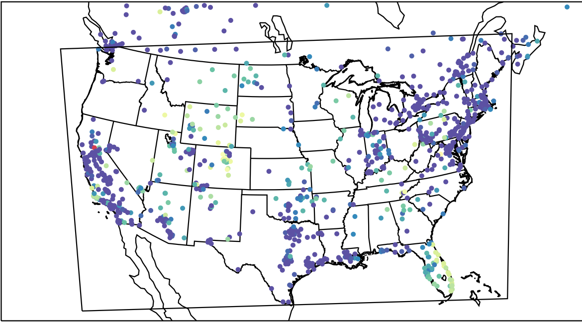
AirNOW (2023-11-16_13:00:00)
