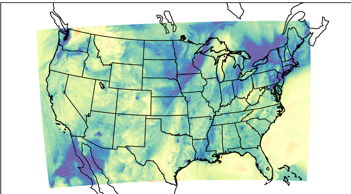
WRF (2023-11-17_00:00:00)
