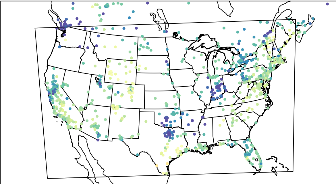
AirNOW (2023-11-17_20:00:00)
