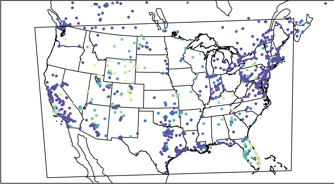
AirNOW (2023-11-16_12:00:00)
