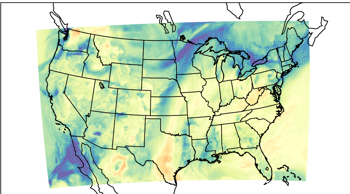
WRF (2023-11-16_19:00:00)
