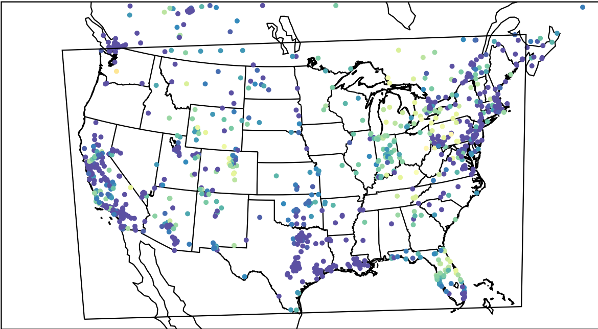
AirNOW (2023-11-17_03:00:00)
