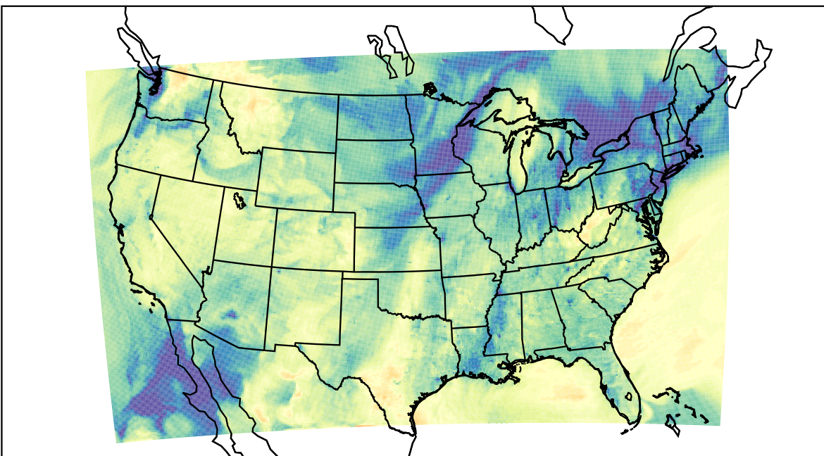
WRF (2023-11-16_23:00:00)
