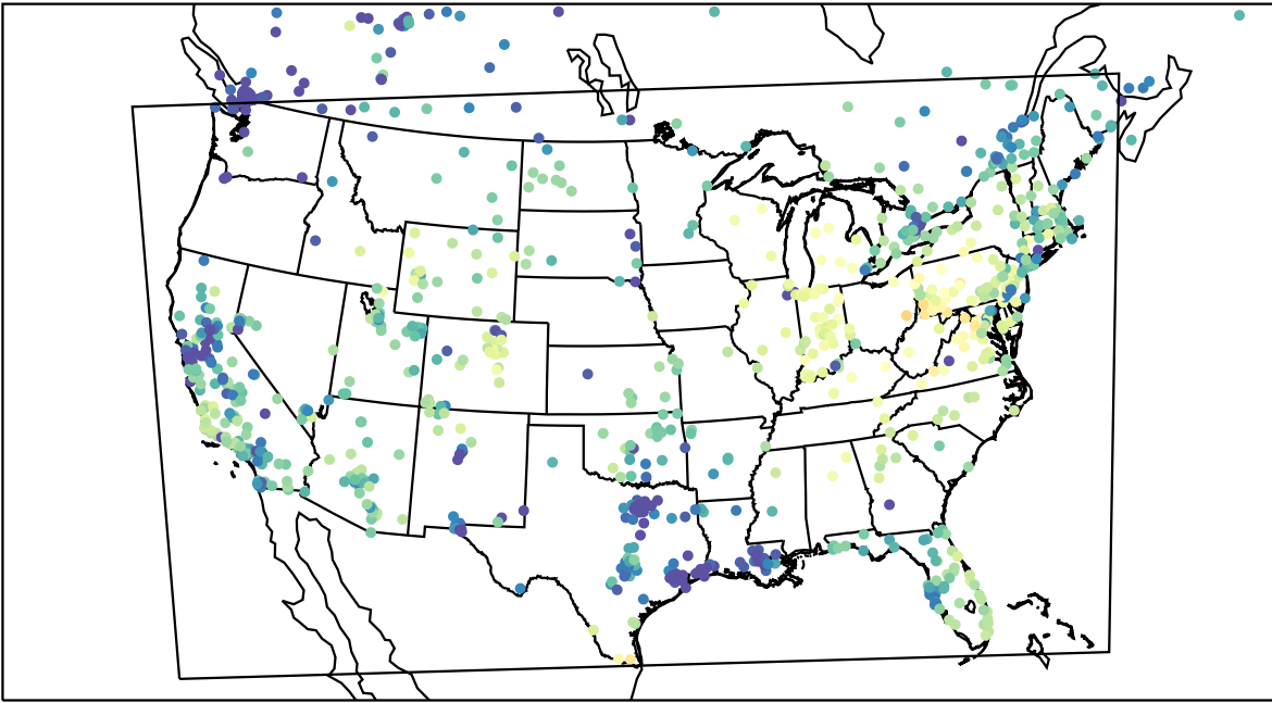
AirNOW (2023-11-16_18:00:00)
