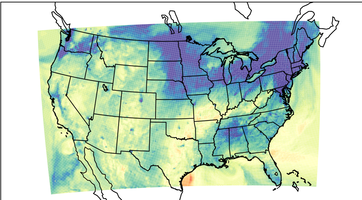
WRF (2023-11-16_00:00:00)
