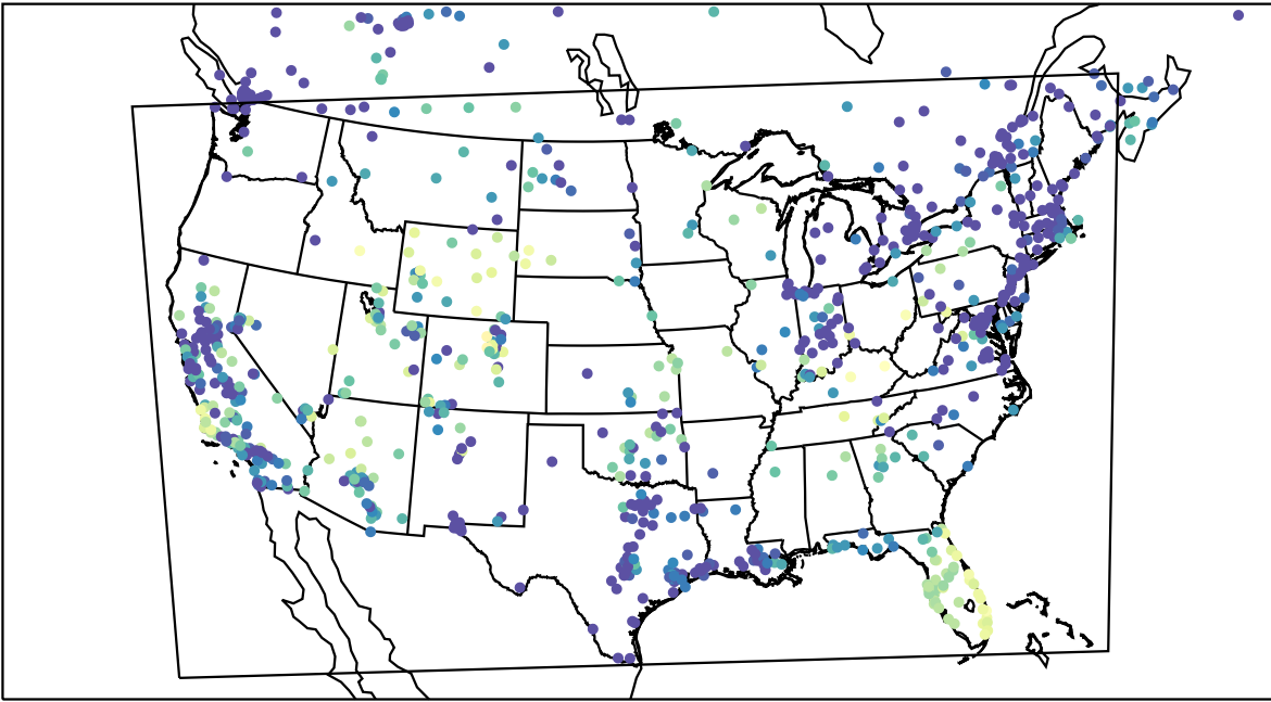
AirNOW (2023-11-16_06:00:00)
