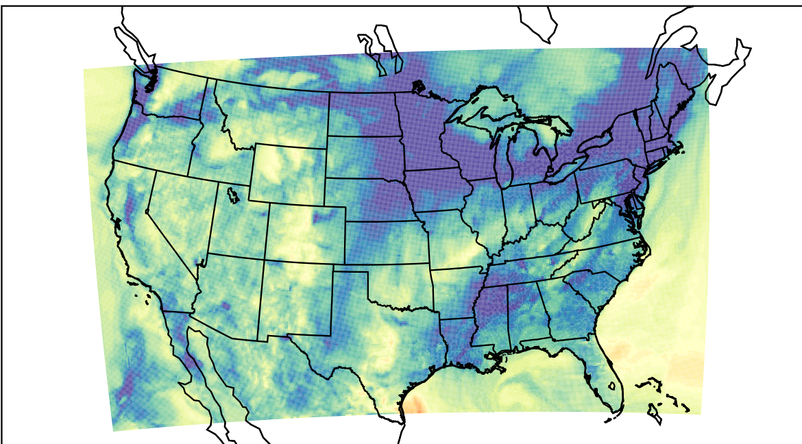
WRF (2023-11-16_06:00:00)
