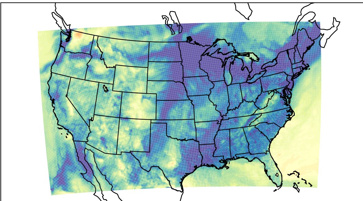
WRF (2023-11-16_13:00:00)
