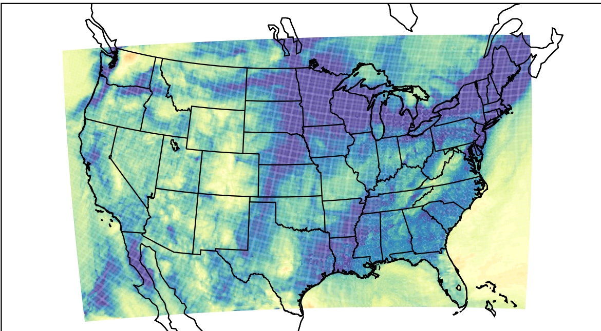
WRF (2023-11-16_11:00:00)
