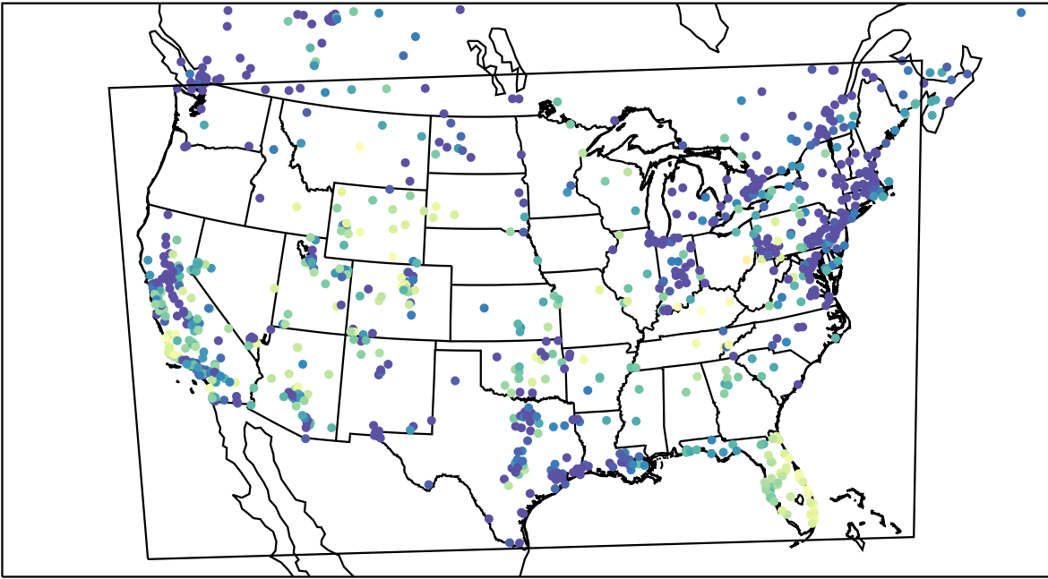
AirNOW (2023-11-16_03:00:00)
