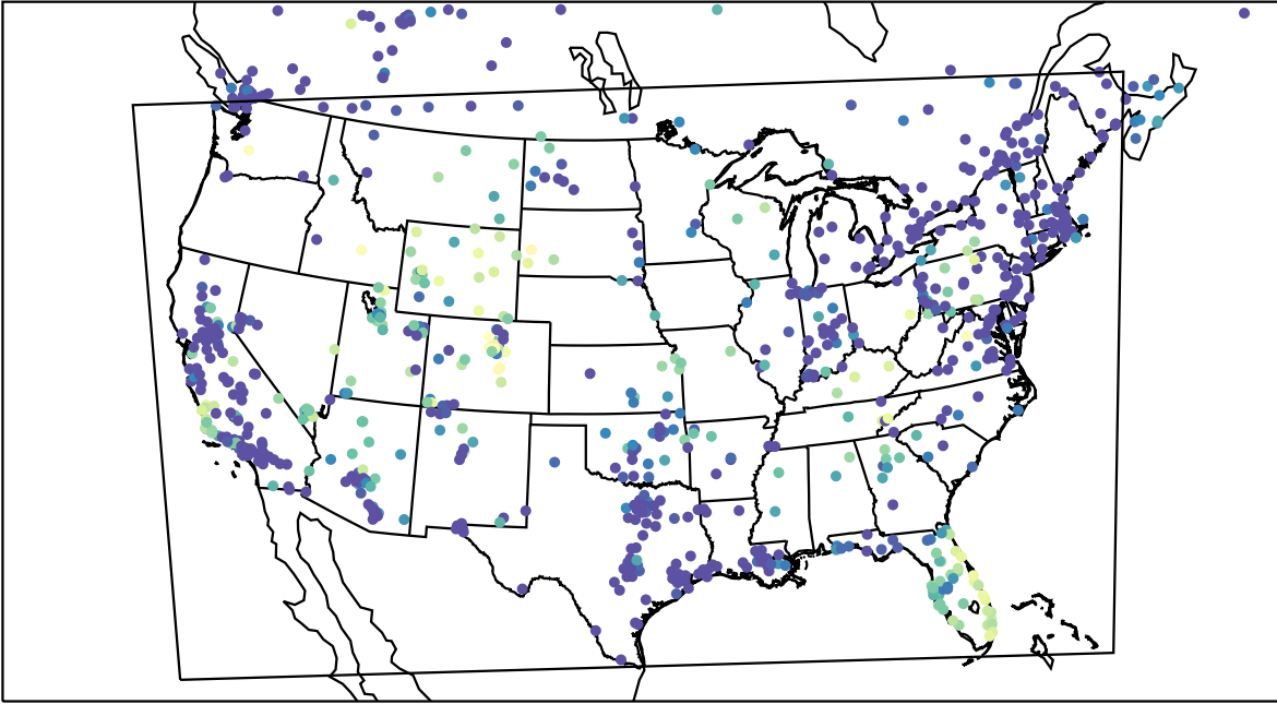
AirNOW (2023-11-16_11:00:00)
