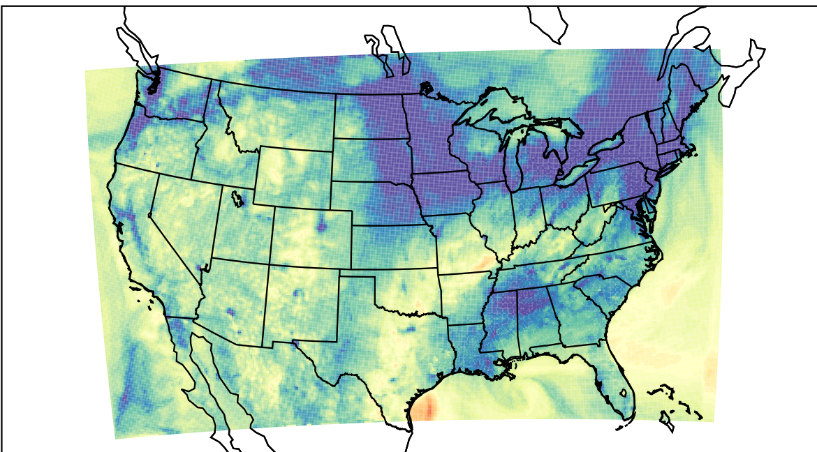
WRF (2023-11-16_02:00:00)
