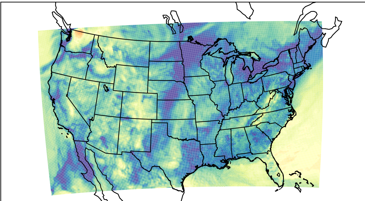
WRF (2023-11-16_15:00:00)
