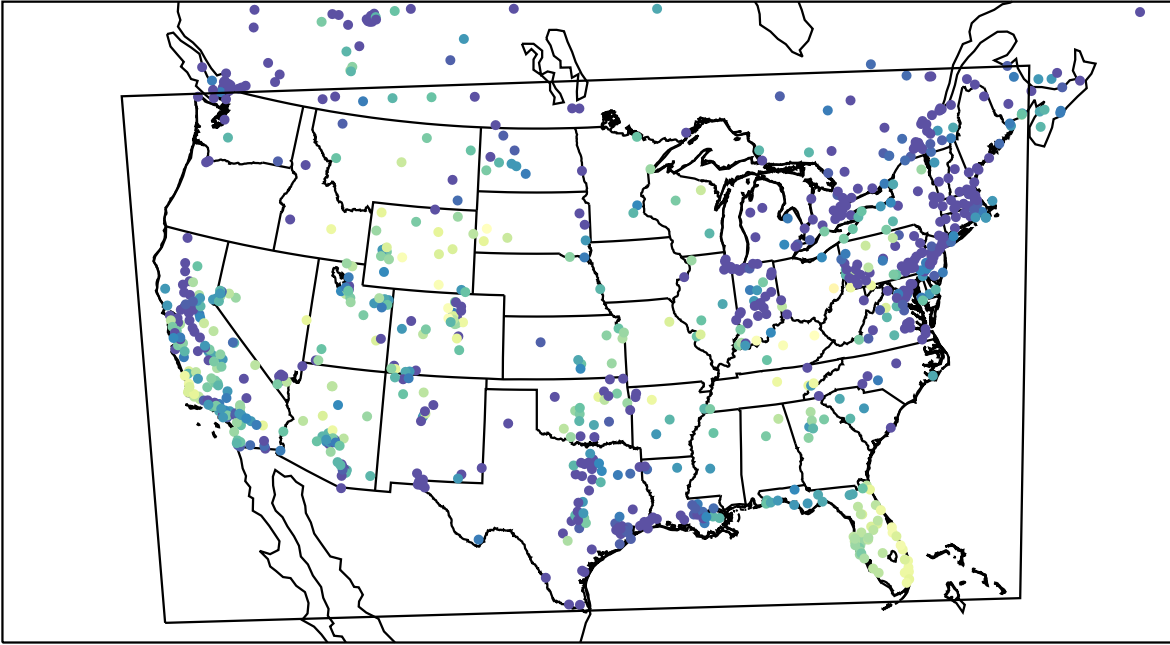
AirNOW (2023-11-16_04:00:00)
