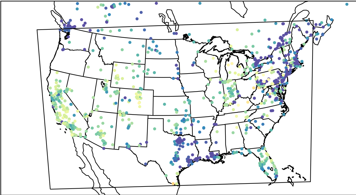
AirNOW (2023-11-16_23:00:00)
