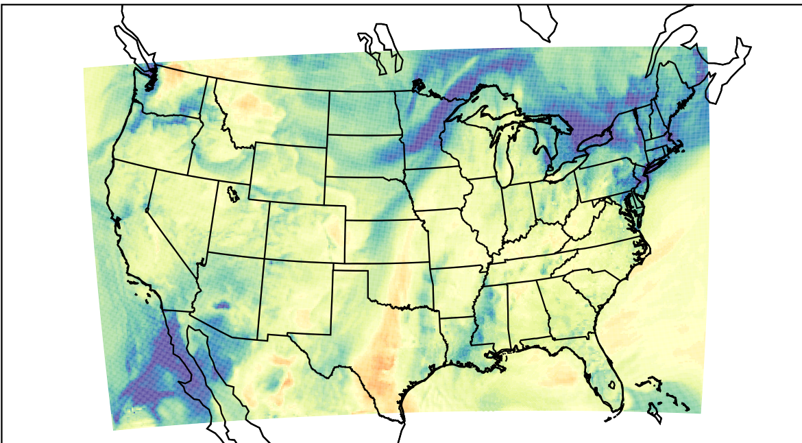
WRF (2023-11-16_21:00:00)
