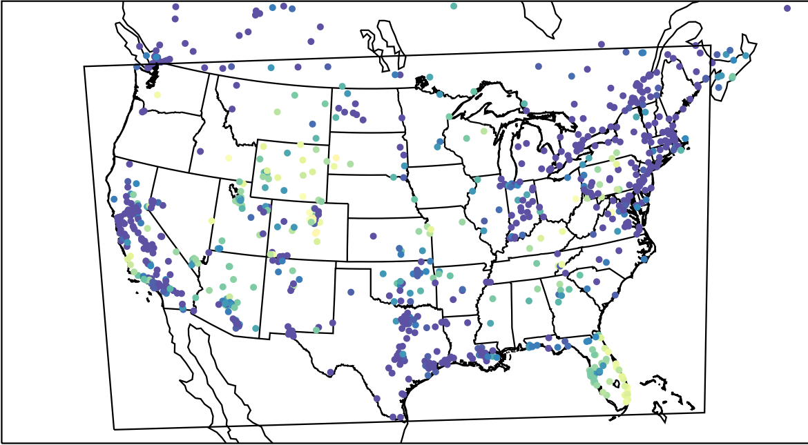
AirNOW (2023-11-16_10:00:00)
