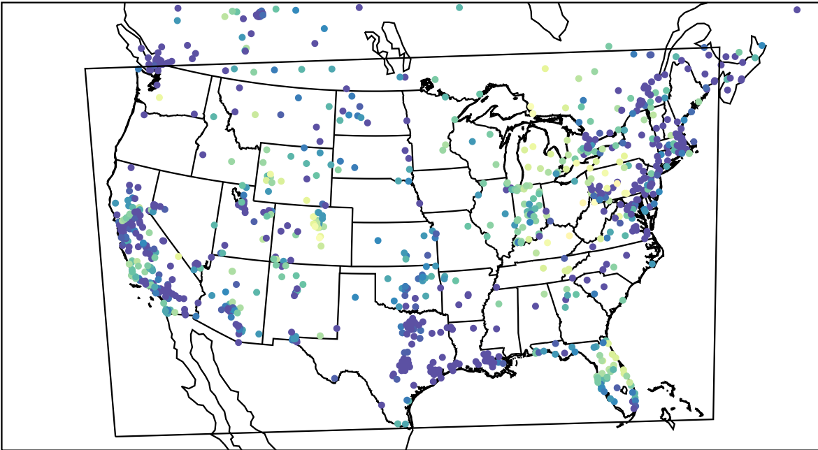
AirNOW (2023-11-17_02:00:00)
