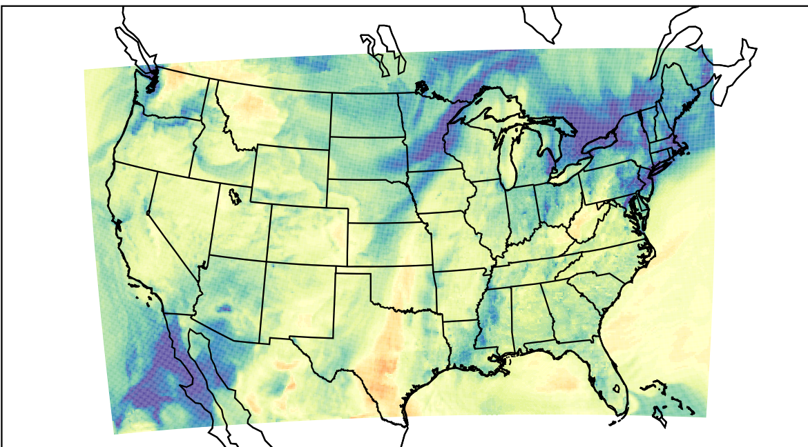
WRF (2023-11-16_22:00:00)
