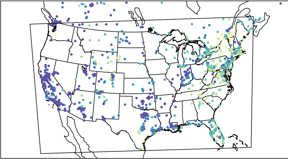
AirNOW (2023-11-17_16:00:00)
