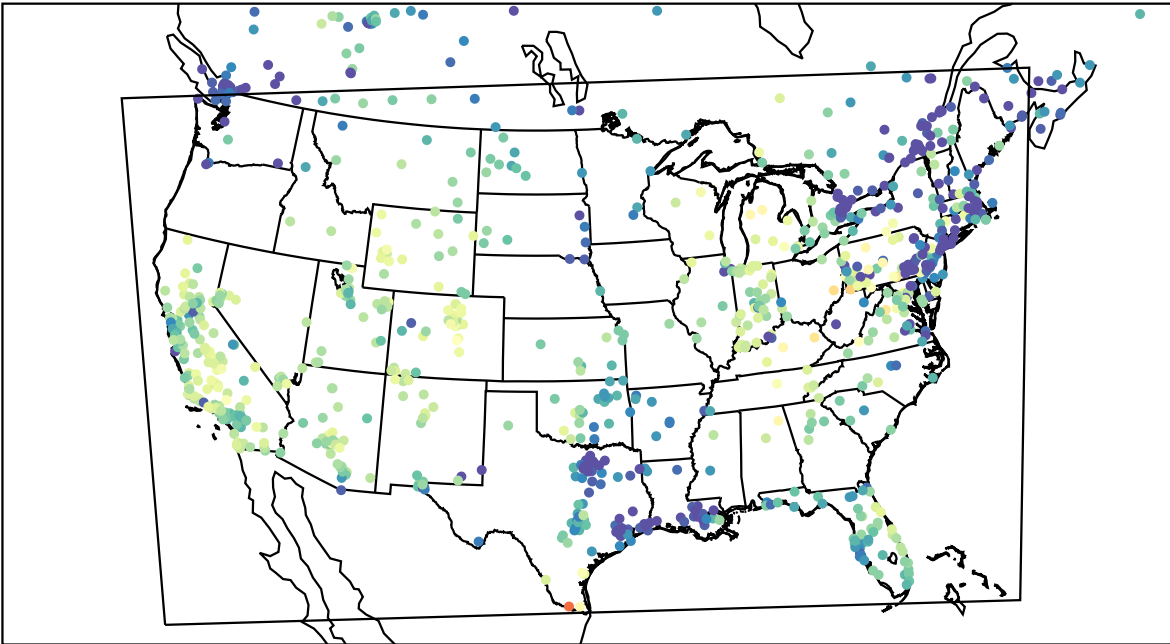
AirNOW (2023-11-16_22:00:00)
