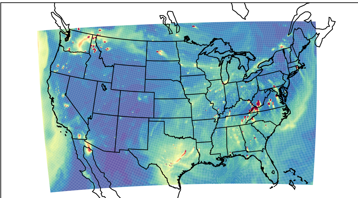
WRF 2023-11-18_22:00:00
