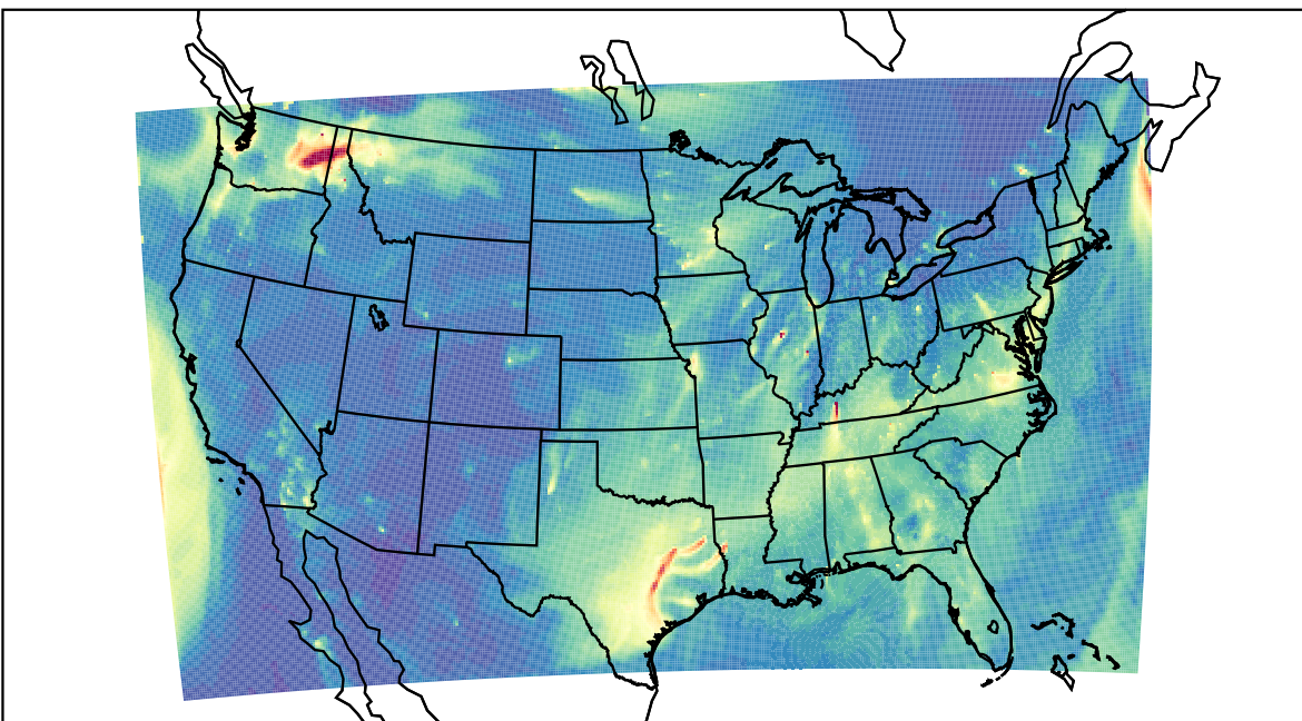
WRF 2023-11-18_12:00:00
