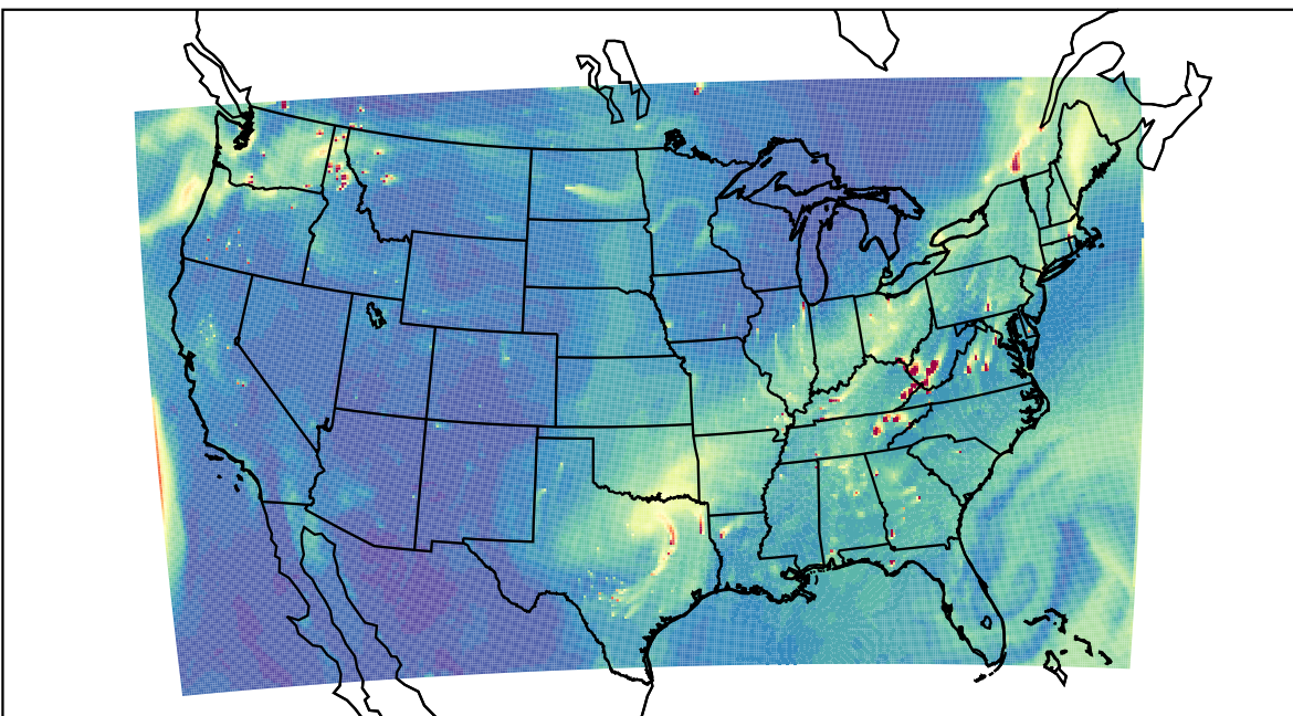
WRF 2023-11-17_21:00:00
