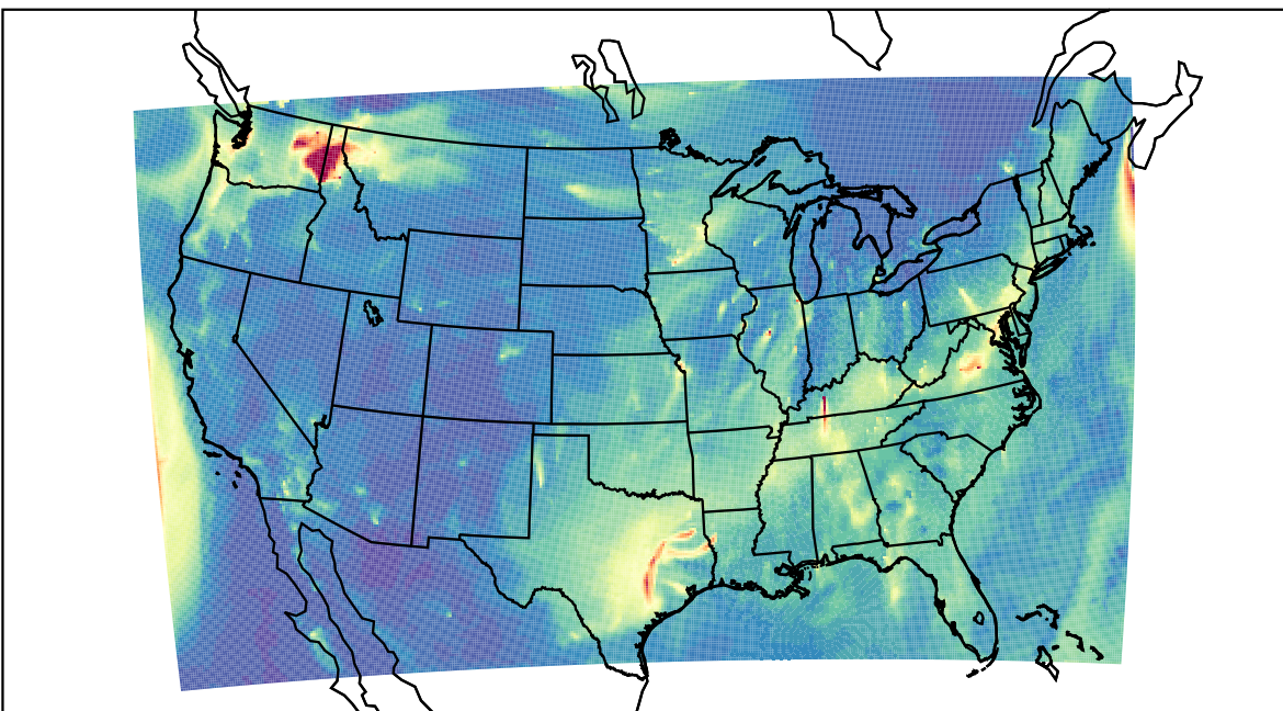
WRF 2023-11-18_09:00:00
