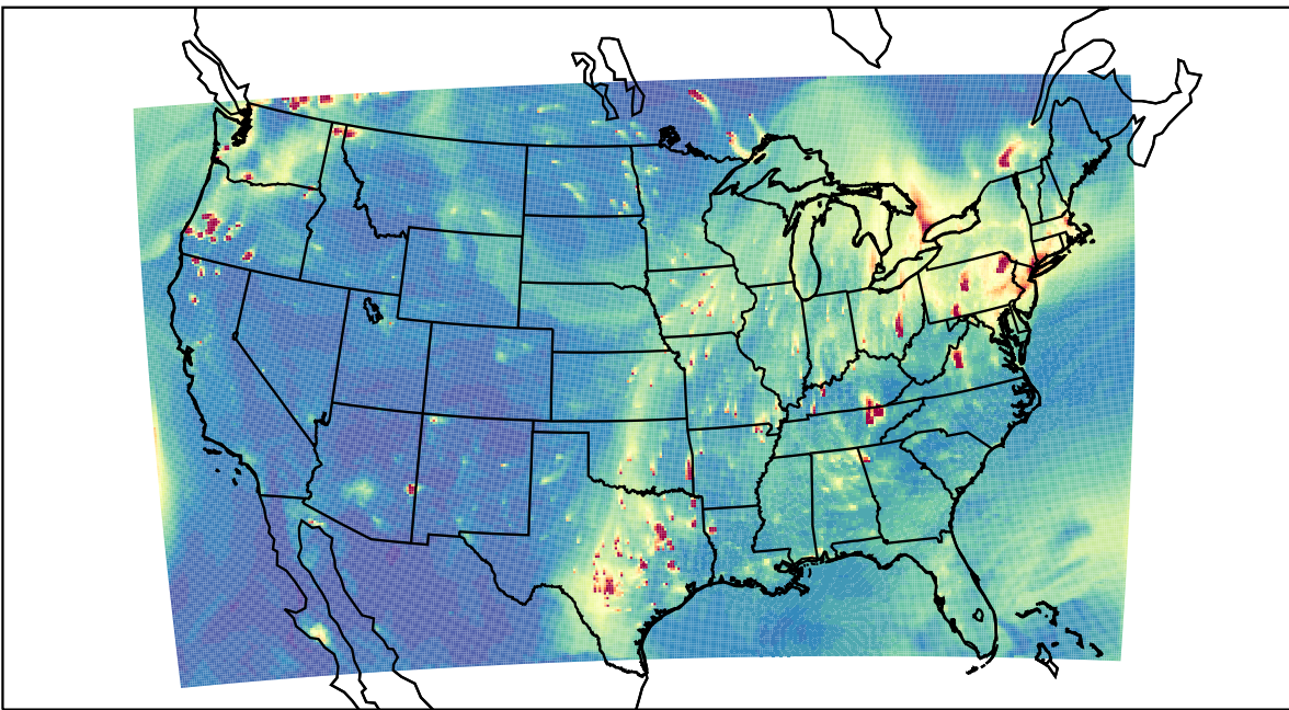
WRF 2023-11-17_00:00:00
