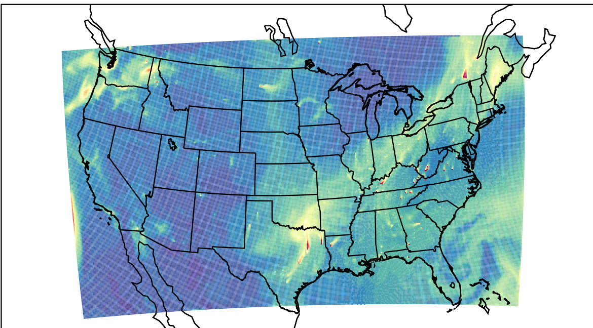
WRF 2023-11-17_18:00:00
