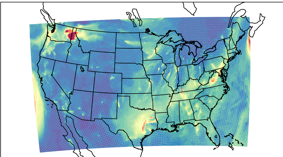
WRF 2023-11-18_08:00:00
