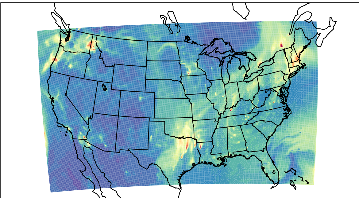
WRF 2023-11-17_13:00:00
