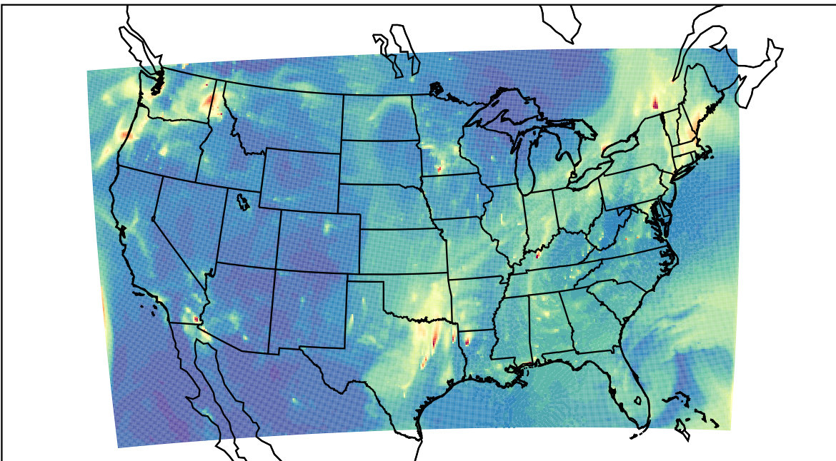
WRF 2023-11-17_14:00:00
