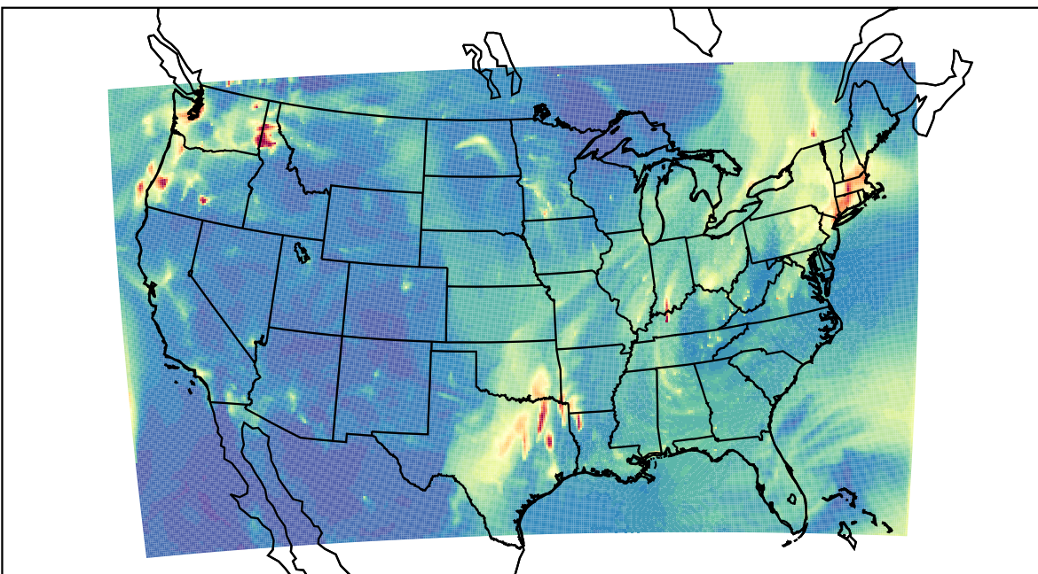
WRF 2023-11-17_09:00:00
