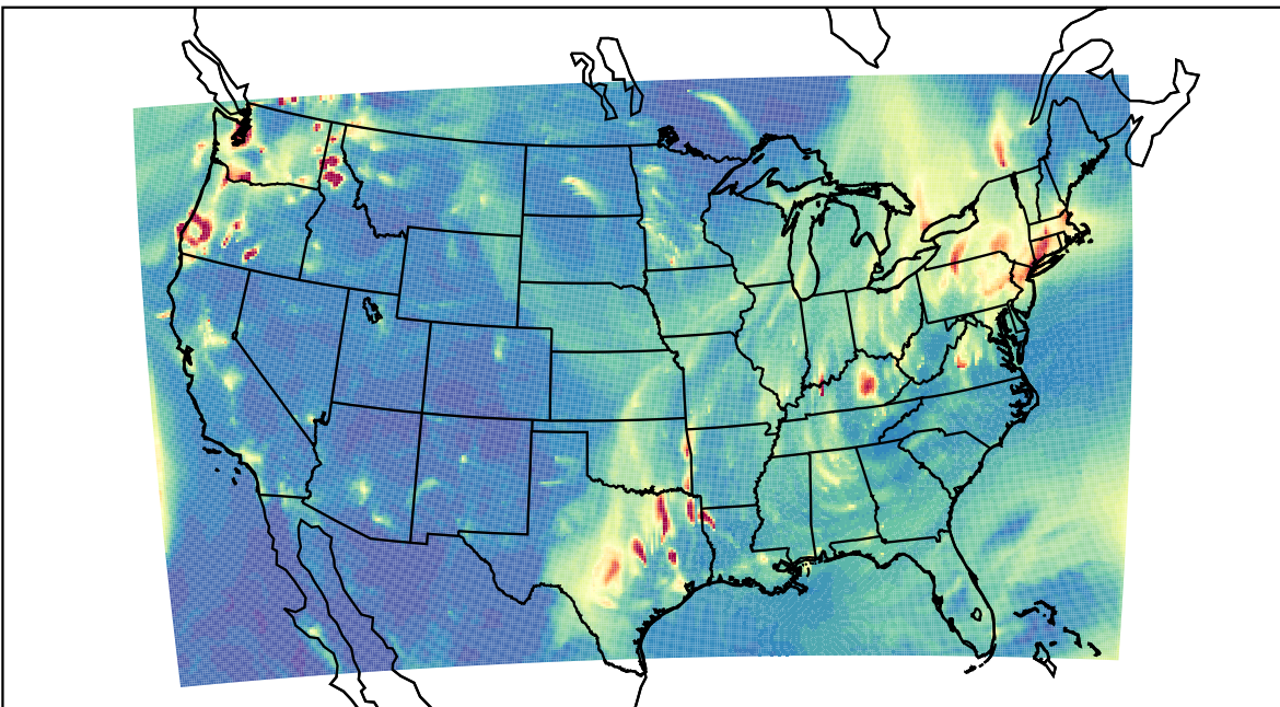
WRF 2023-11-17_05:00:00
