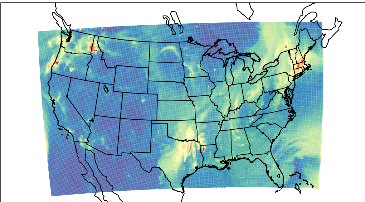
WRF 2023-11-17_11:00:00
