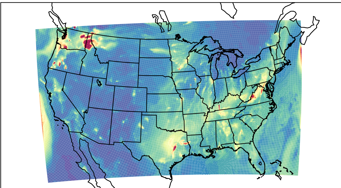
WRF 2023-11-18_05:00:00
