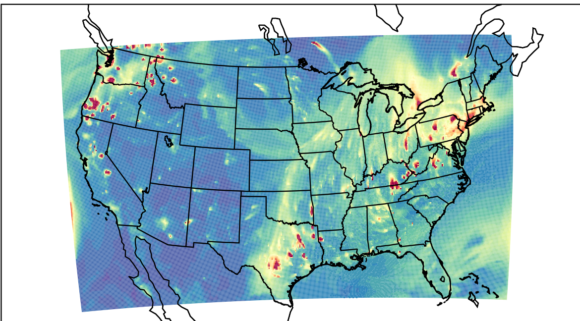
WRF 2023-11-17_02:00:00
