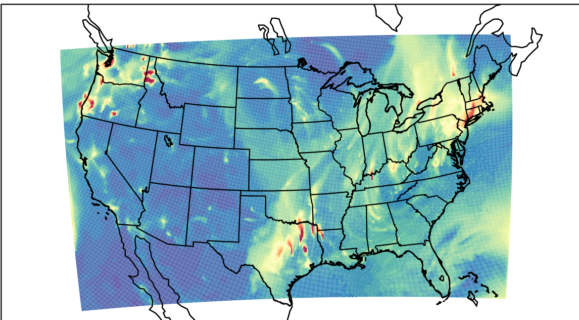
WRF 2023-11-17_07:00:00
