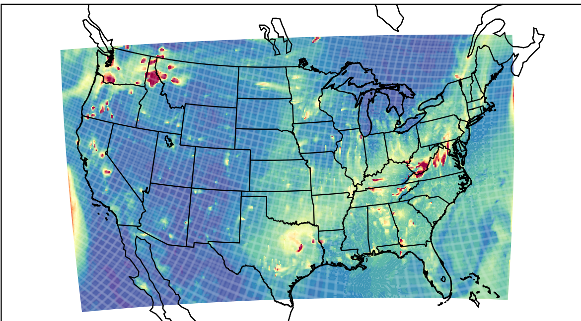
WRF 2023-11-18_02:00:00
