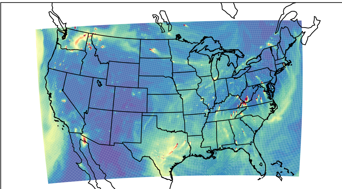
WRF 2023-11-18_21:00:00
