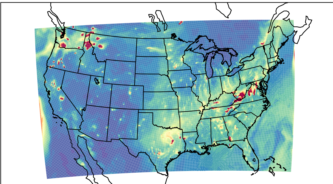
WRF 2023-11-18_01:00:00
