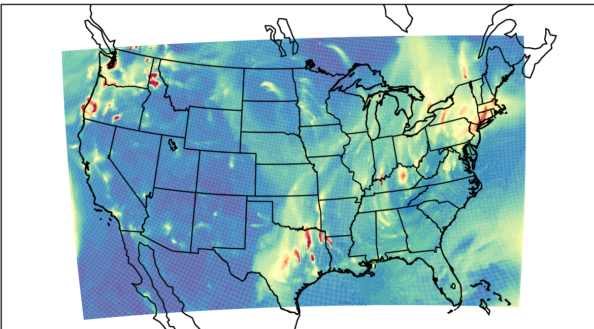
WRF 2023-11-17_06:00:00
