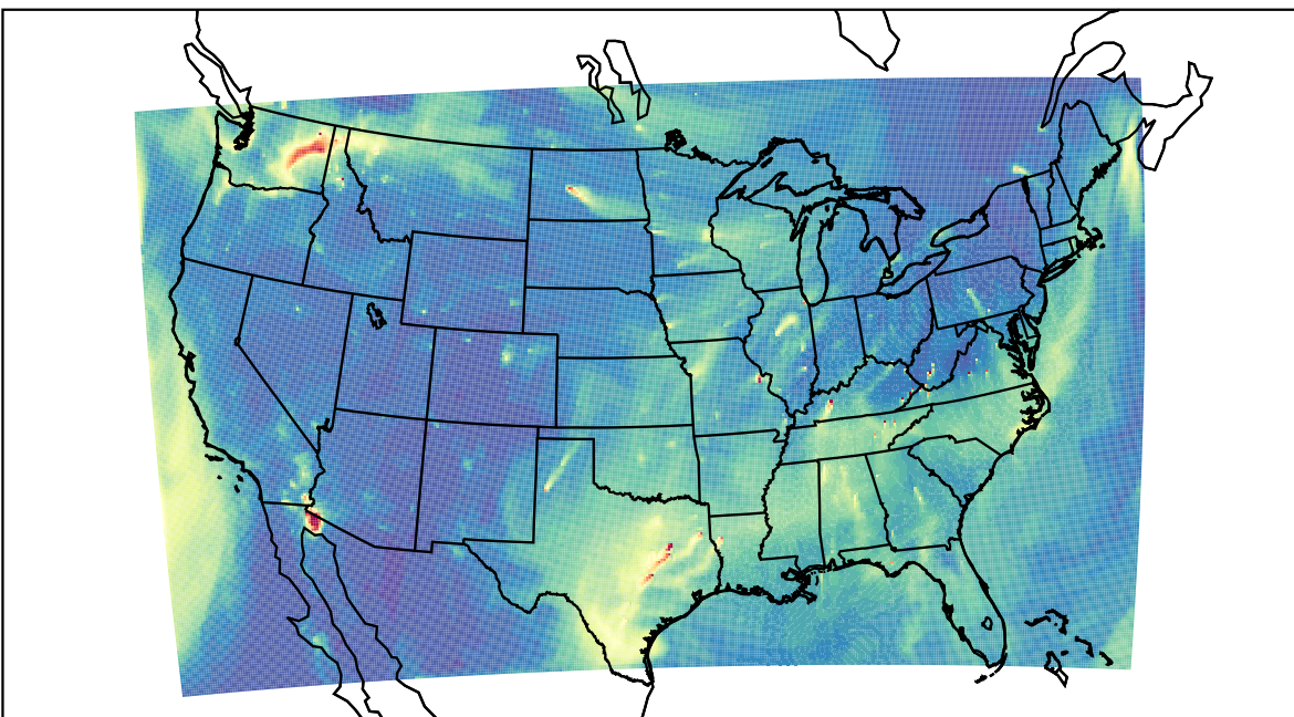
WRF 2023-11-18_17:00:00
