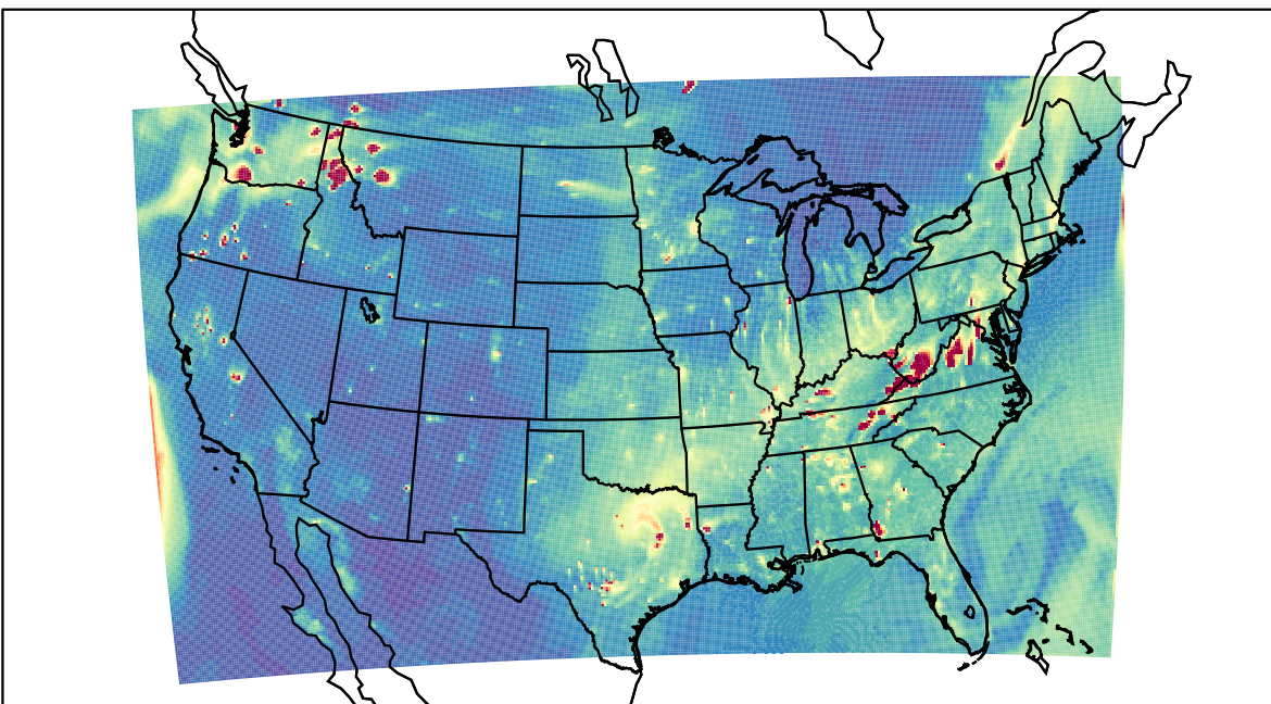
WRF 2023-11-18_00:00:00
