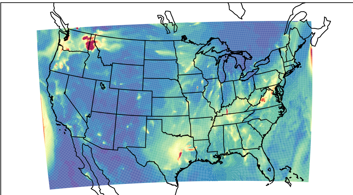
WRF 2023-11-18_06:00:00
