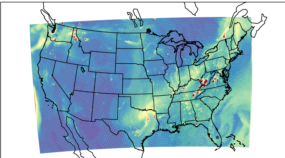
WRF 2023-11-17_22:00:00
