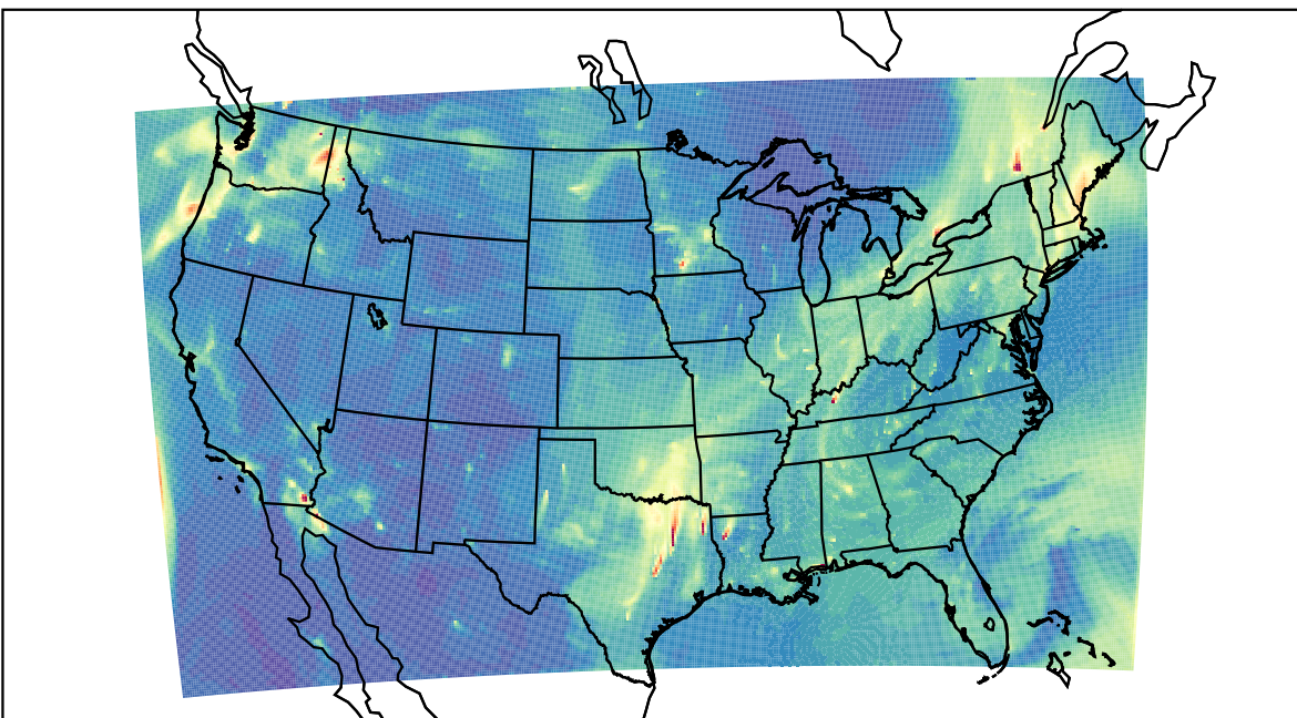
WRF 2023-11-17_15:00:00
