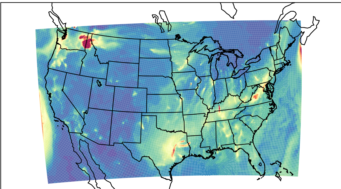
WRF 2023-11-18_07:00:00
