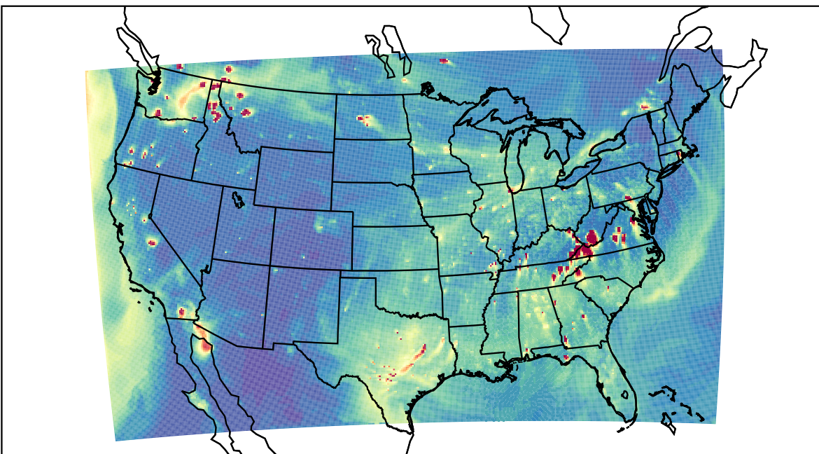
WRF 2023-11-18_23:00:00
