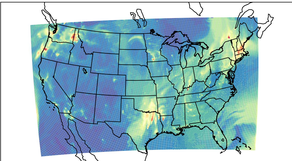
WRF 2023-11-17_12:00:00
