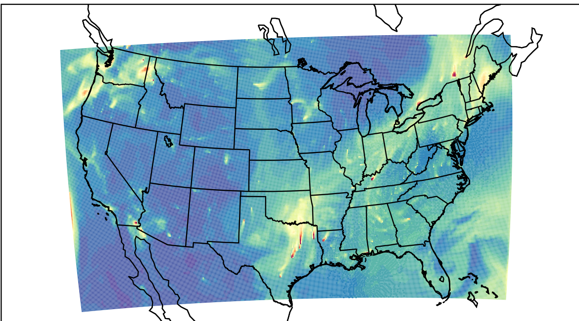
WRF 2023-11-17_16:00:00
