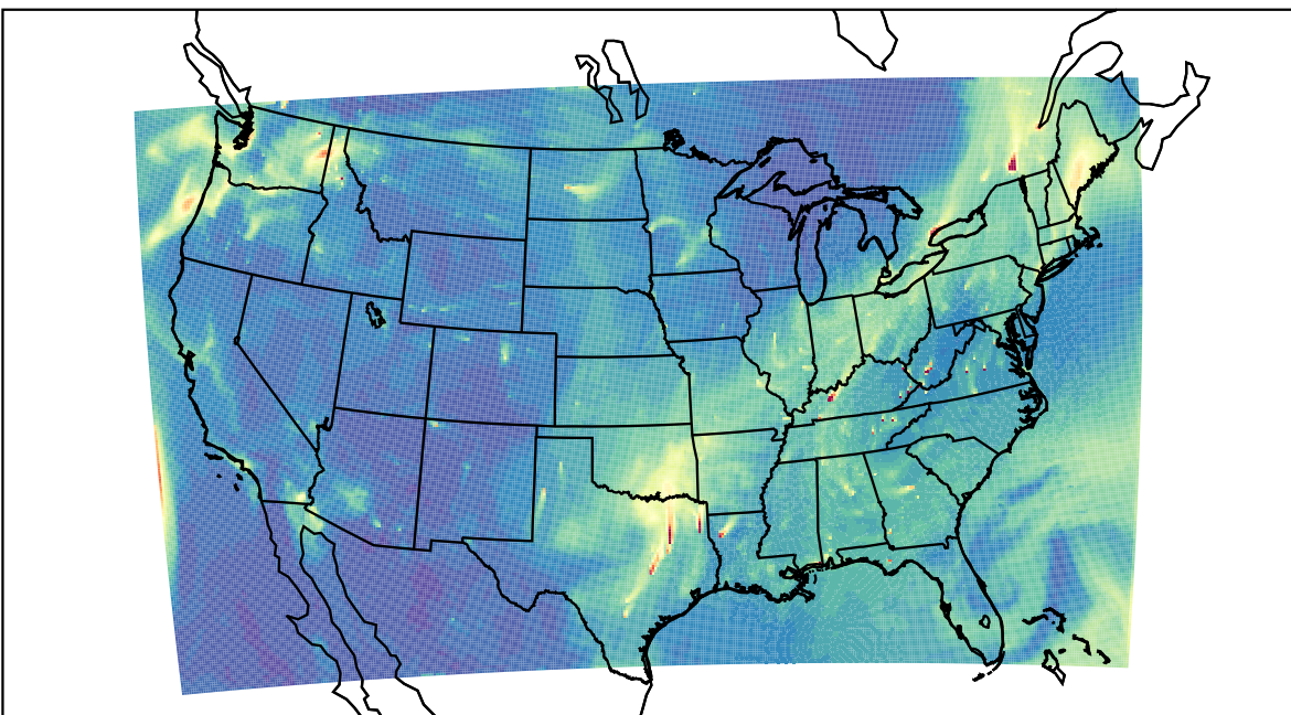
WRF 2023-11-17_17:00:00
