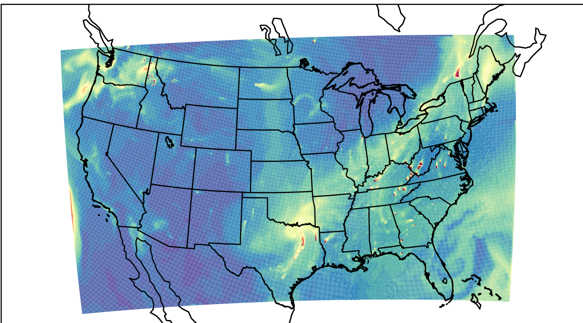
WRF 2023-11-17_19:00:00
