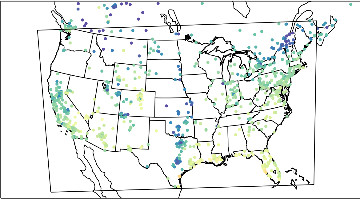
AirNOW (2023-11-19_19:00:00)
