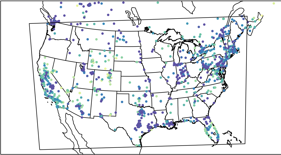
AirNOW (2023-11-19_02:00:00)
