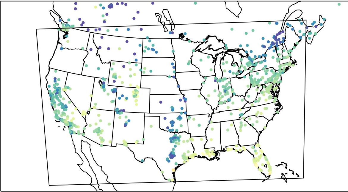
AirNOW (2023-11-19_18:00:00)
