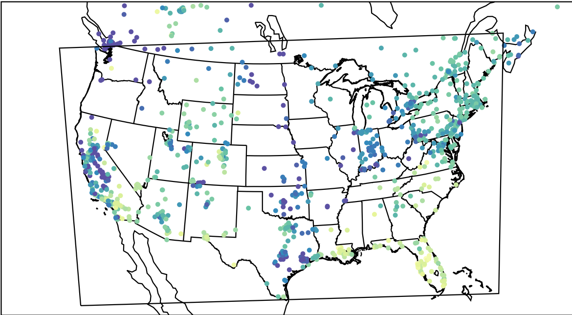
AirNOW (2023-11-20_17:00:00)
