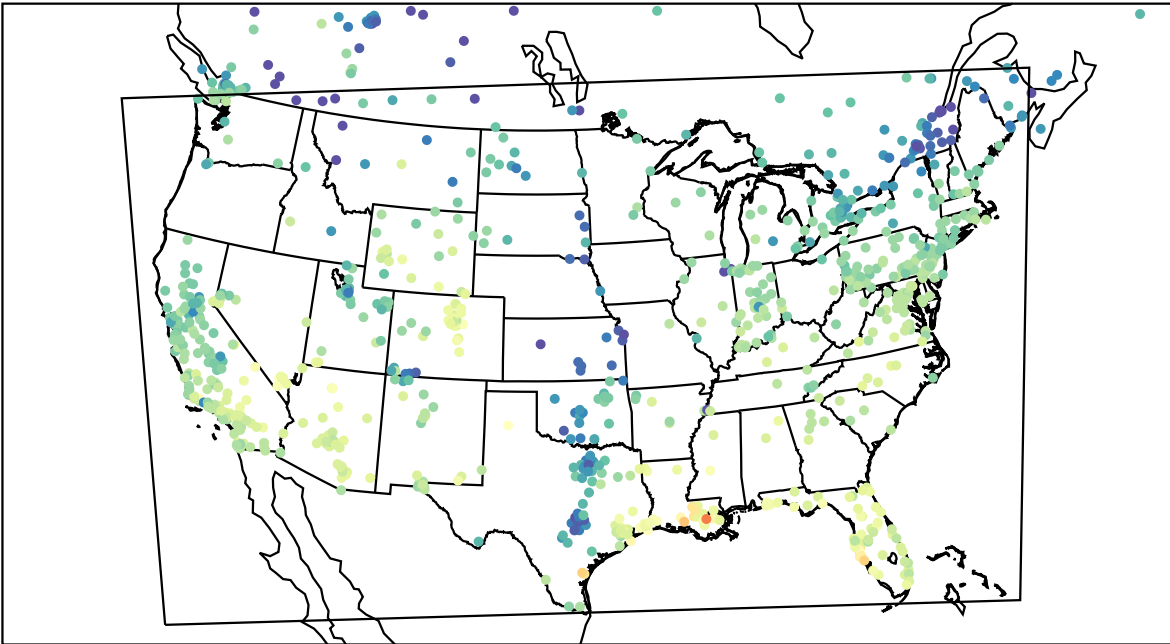
AirNOW (2023-11-19_20:00:00)
