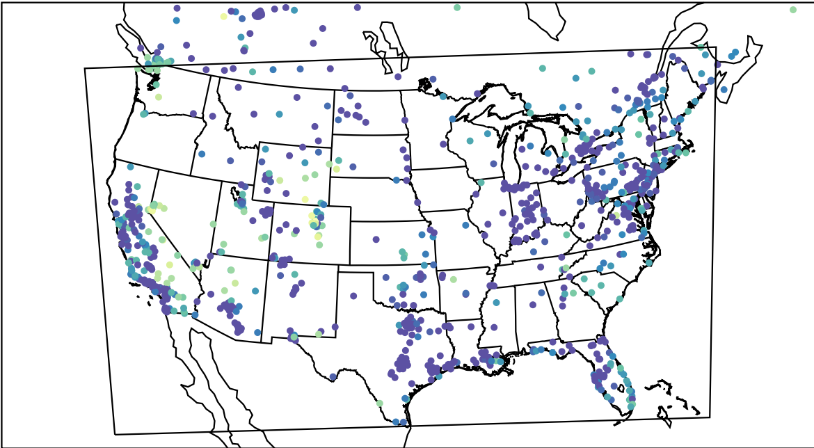
AirNOW (2023-11-19_13:00:00)
