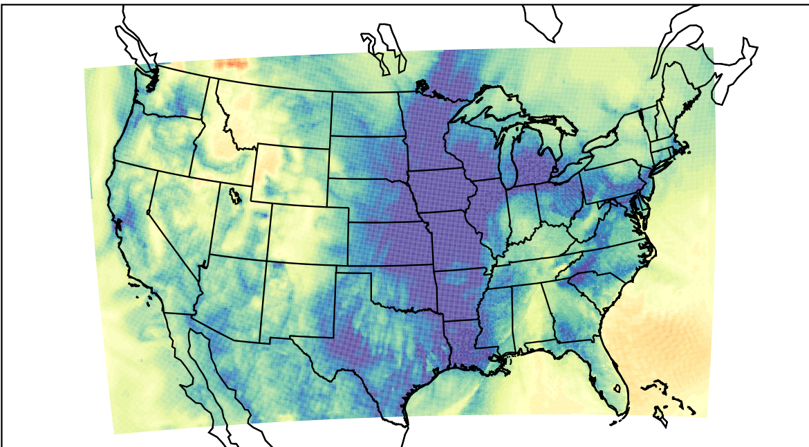
WRF (2023-11-21_10:00:00)
