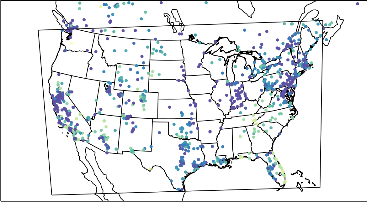
AirNOW (2023-11-21_05:00:00)
