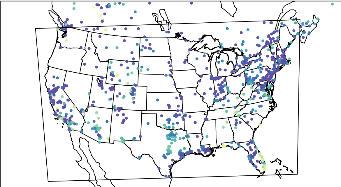
AirNOW (2023-11-21_12:00:00)
