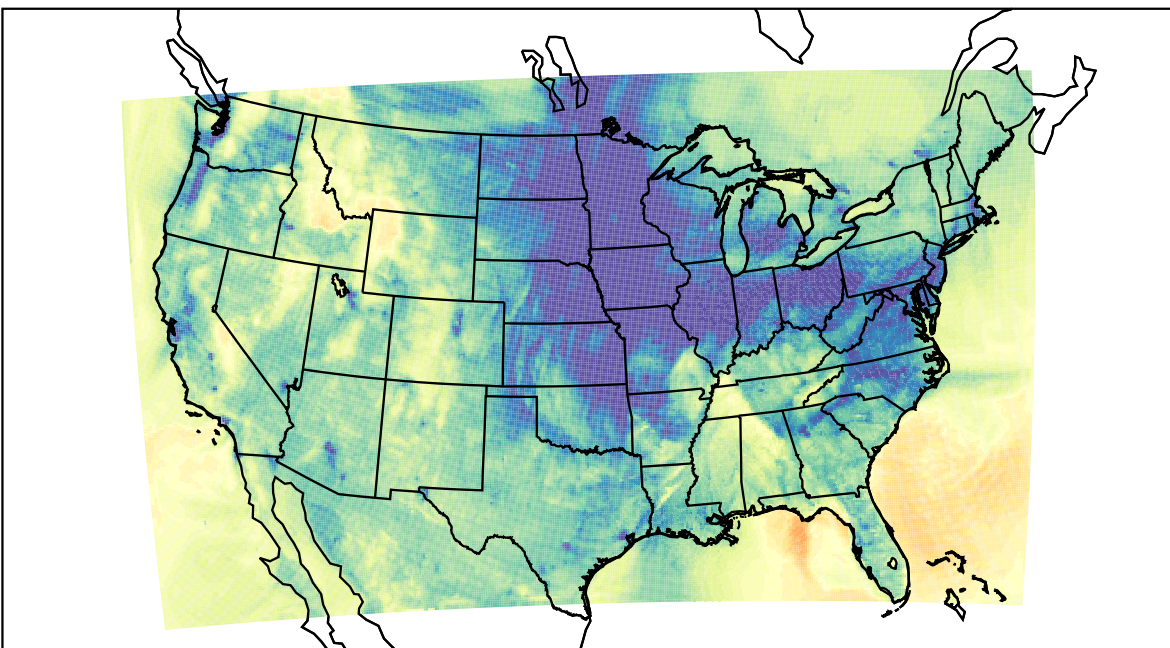
WRF (2023-11-21_01:00:00)
