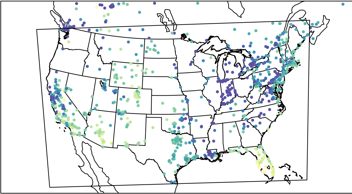
AirNOW (2023-11-21_19:00:00)
