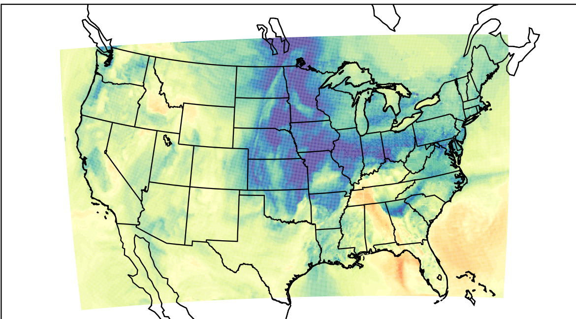
WRF (2023-11-20_21:00:00)
