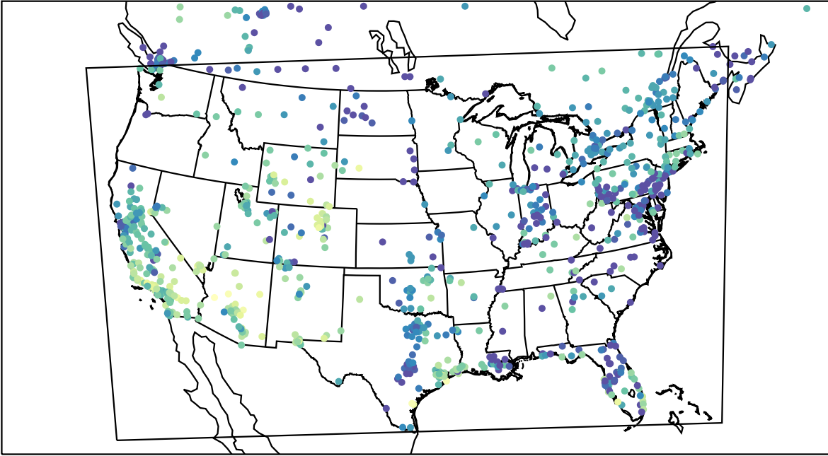
AirNOW (2023-11-20_01:00:00)
