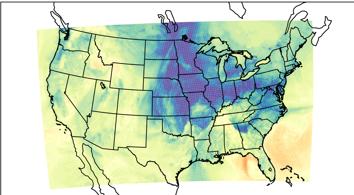
WRF (2023-11-20_22:00:00)
