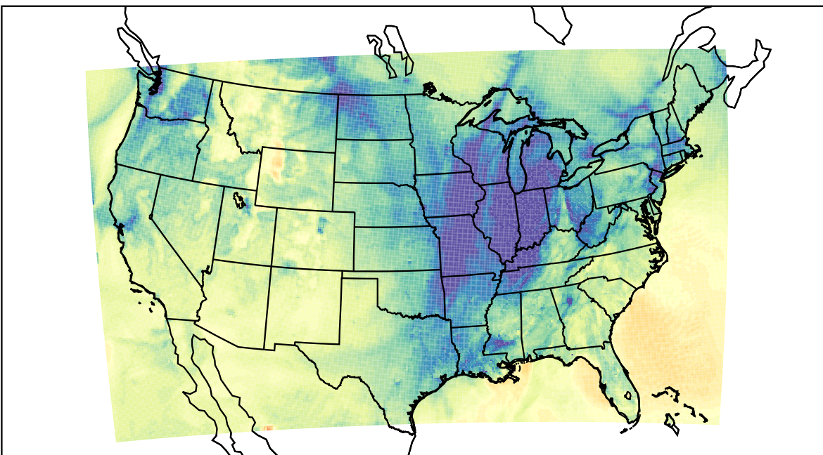
WRF (2023-11-21_23:00:00)
