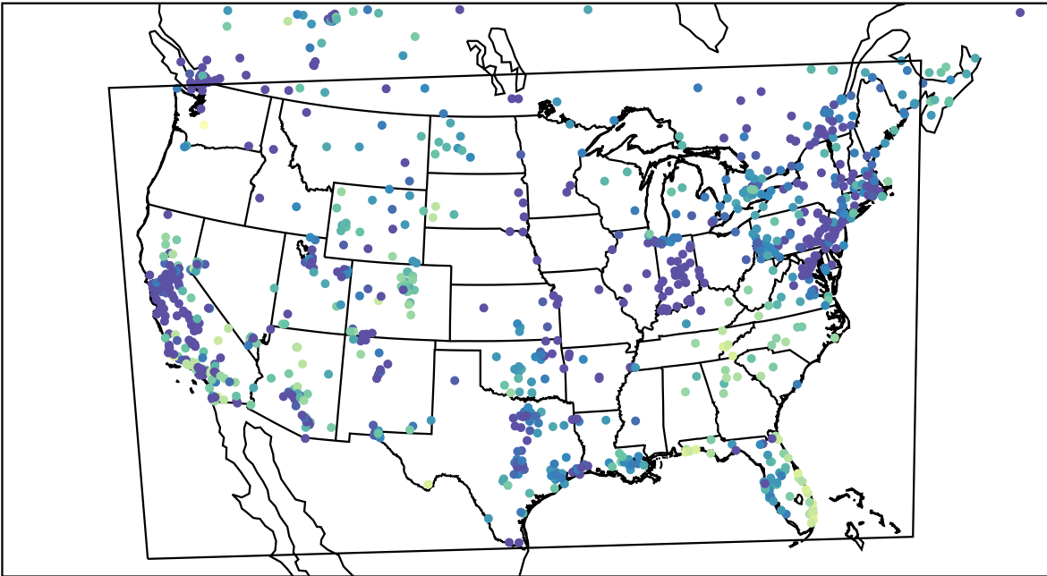
AirNOW (2023-11-21_04:00:00)
