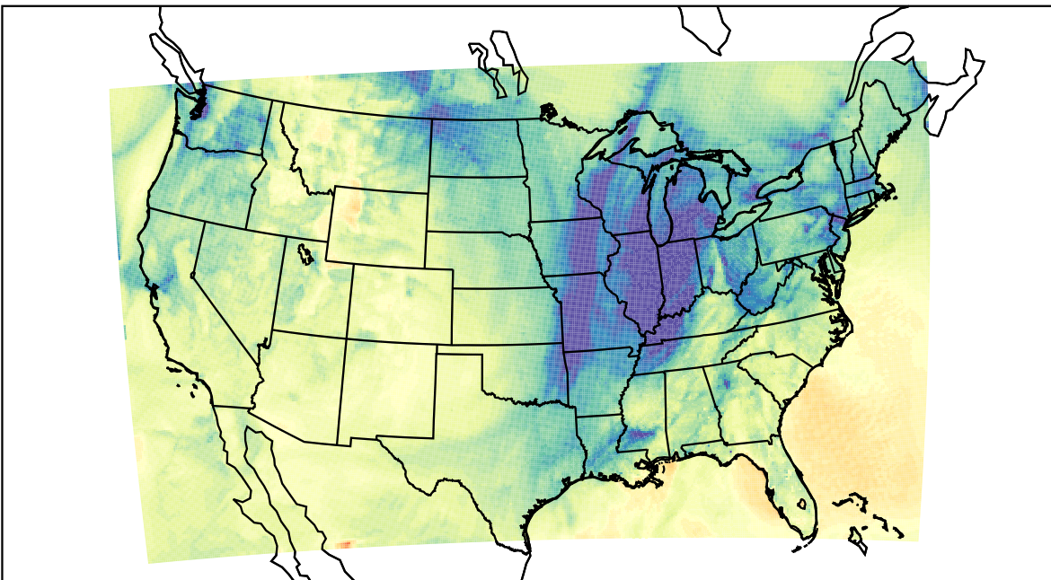
WRF (2023-11-21_22:00:00)
