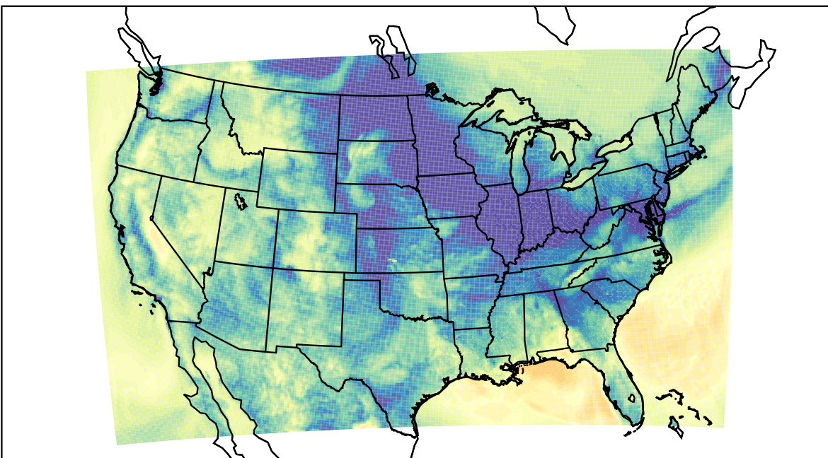
WRF (2023-11-20_07:00:00)
