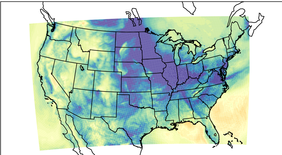
WRF (2023-11-20_11:00:00)
