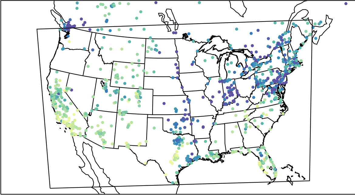
AirNOW (2023-11-20_22:00:00)
