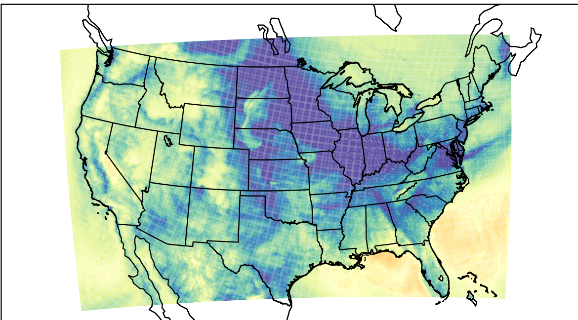
WRF (2023-11-20_09:00:00)
