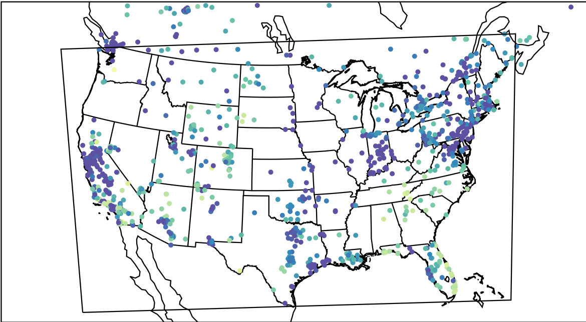
AirNOW (2023-11-21_02:00:00)
