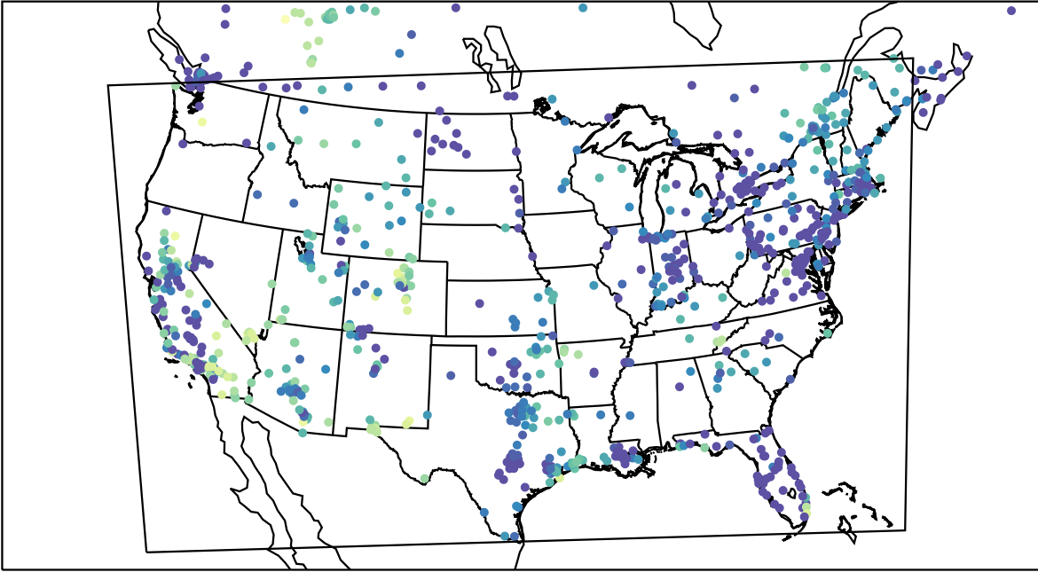
AirNOW (2023-11-20_11:00:00)
