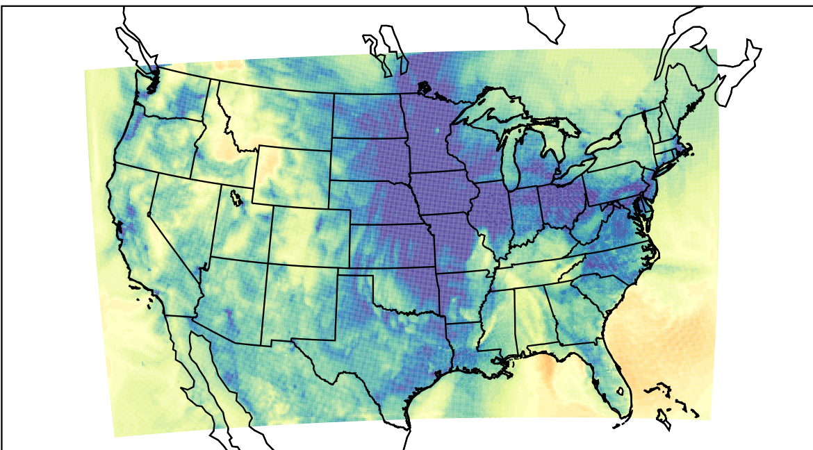
WRF (2023-11-21_04:00:00)
