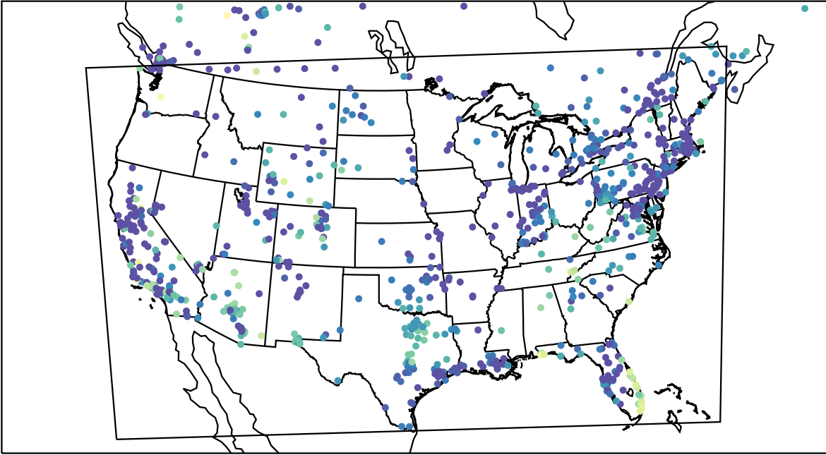
AirNOW (2023-11-21_11:00:00)
