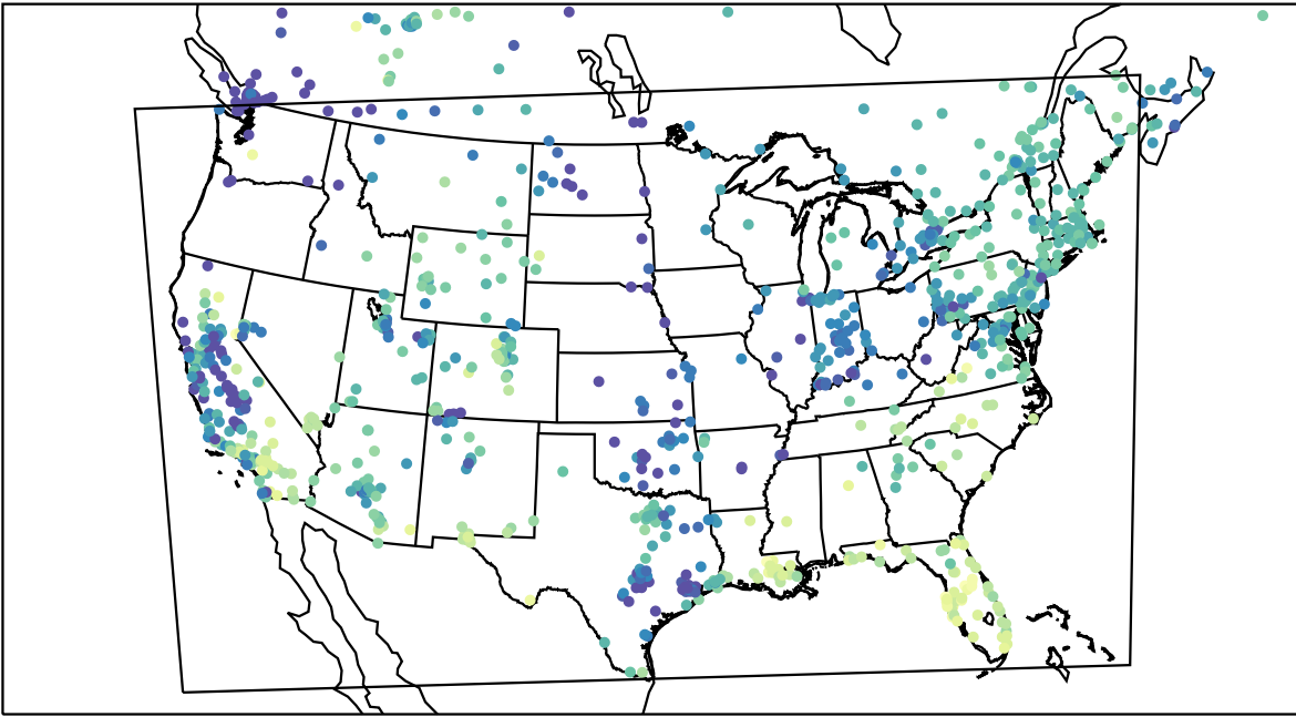
AirNOW (2023-11-20_17:00:00)
