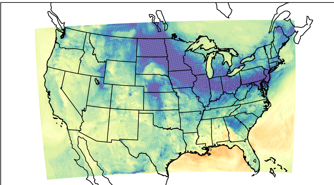
WRF (2023-11-20_00:00:00)
