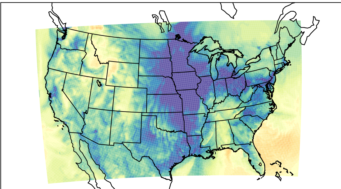
WRF (2023-11-21_06:00:00)
