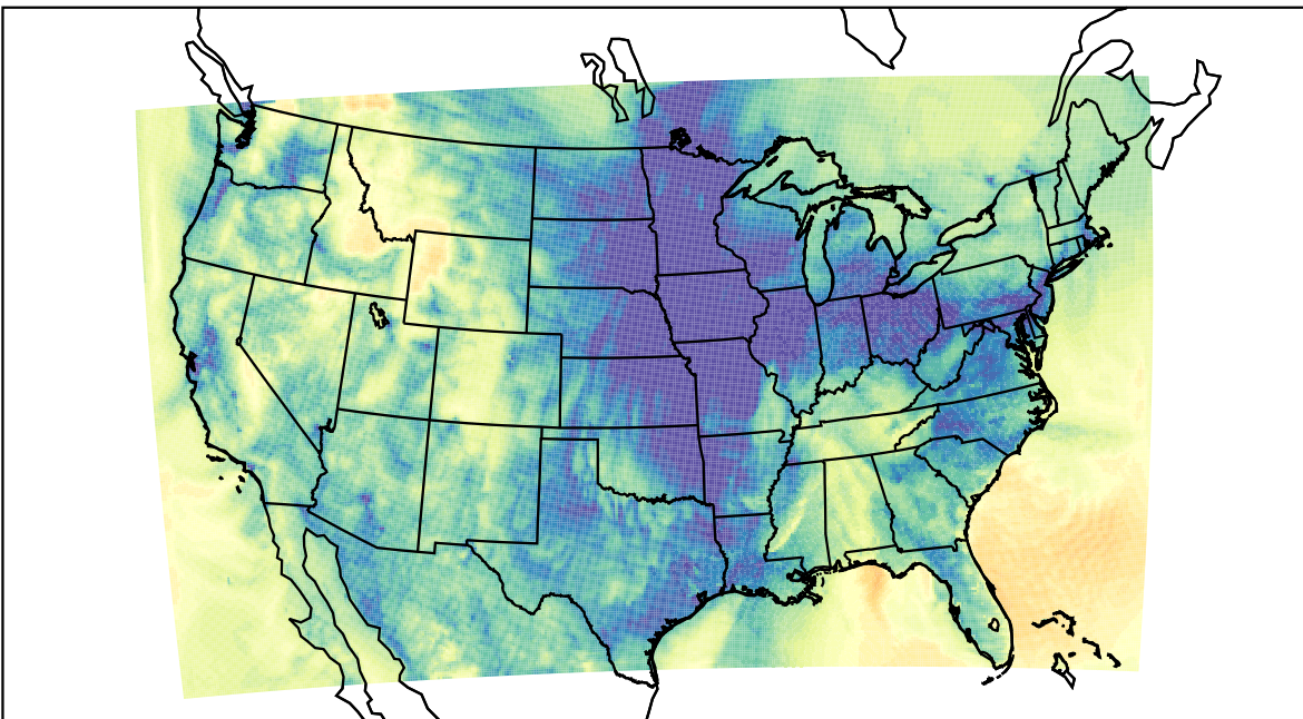
WRF (2023-11-21_05:00:00)
