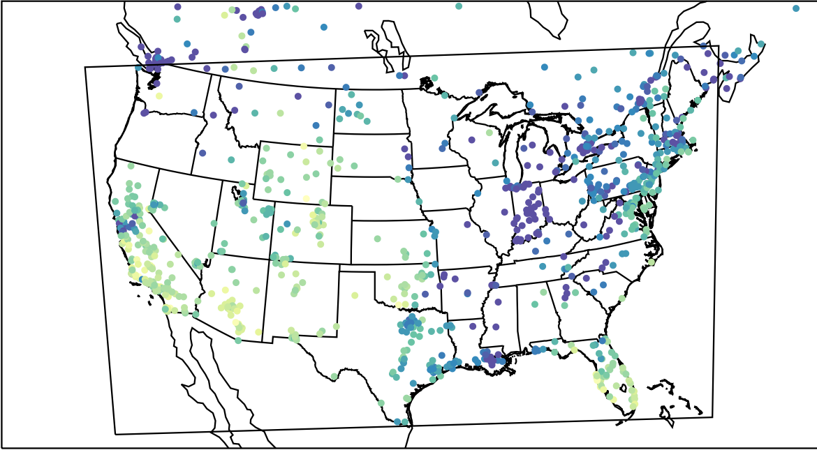
AirNOW (2023-11-21_22:00:00)
