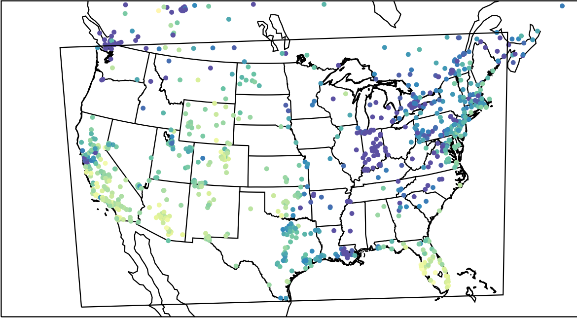
AirNOW (2023-11-21_21:00:00)
