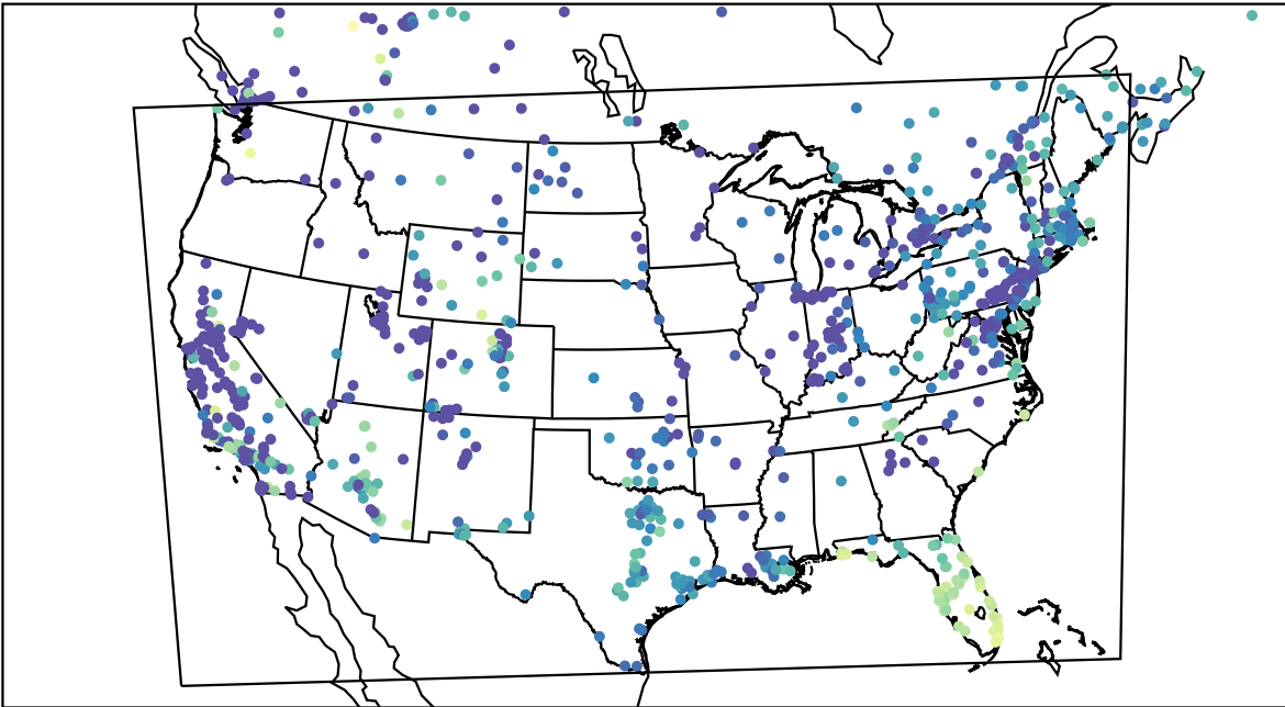
AirNOW (2023-11-21_15:00:00)
