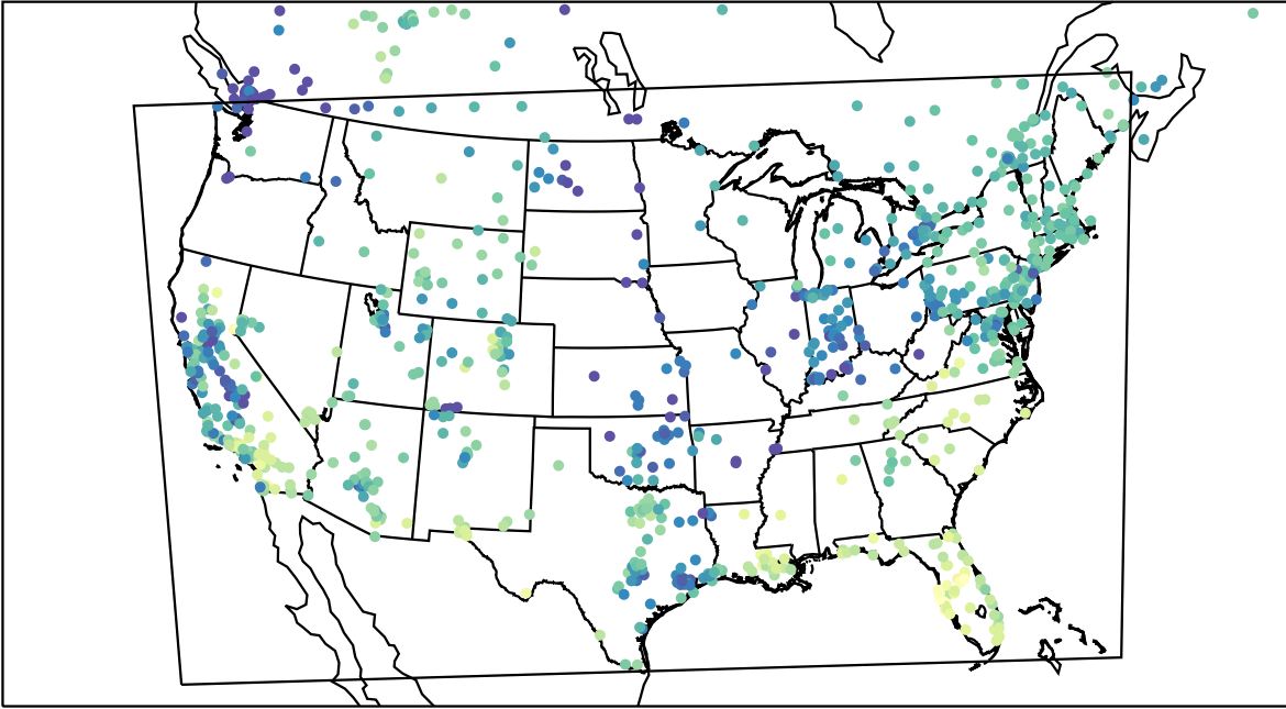
AirNOW (2023-11-20_18:00:00)
