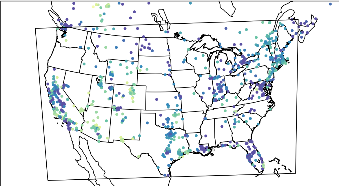
AirNOW (2023-11-20_06:00:00)
