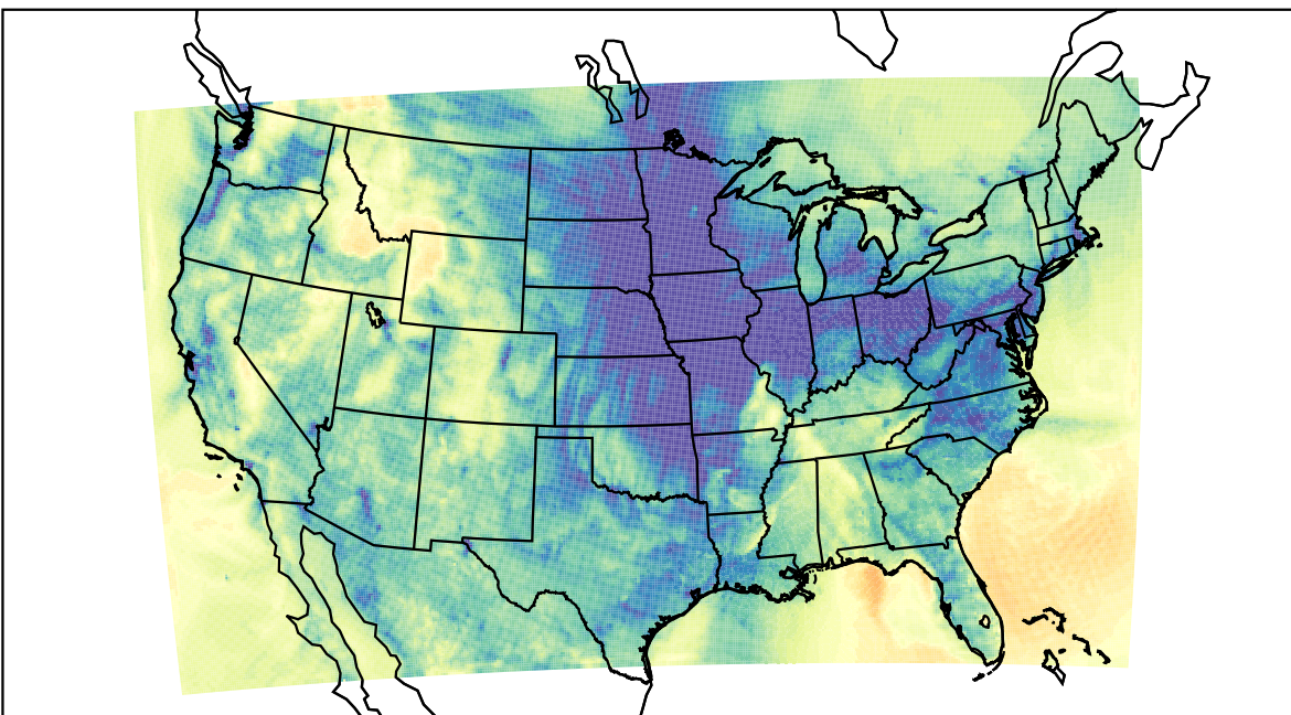
WRF (2023-11-21_03:00:00)
