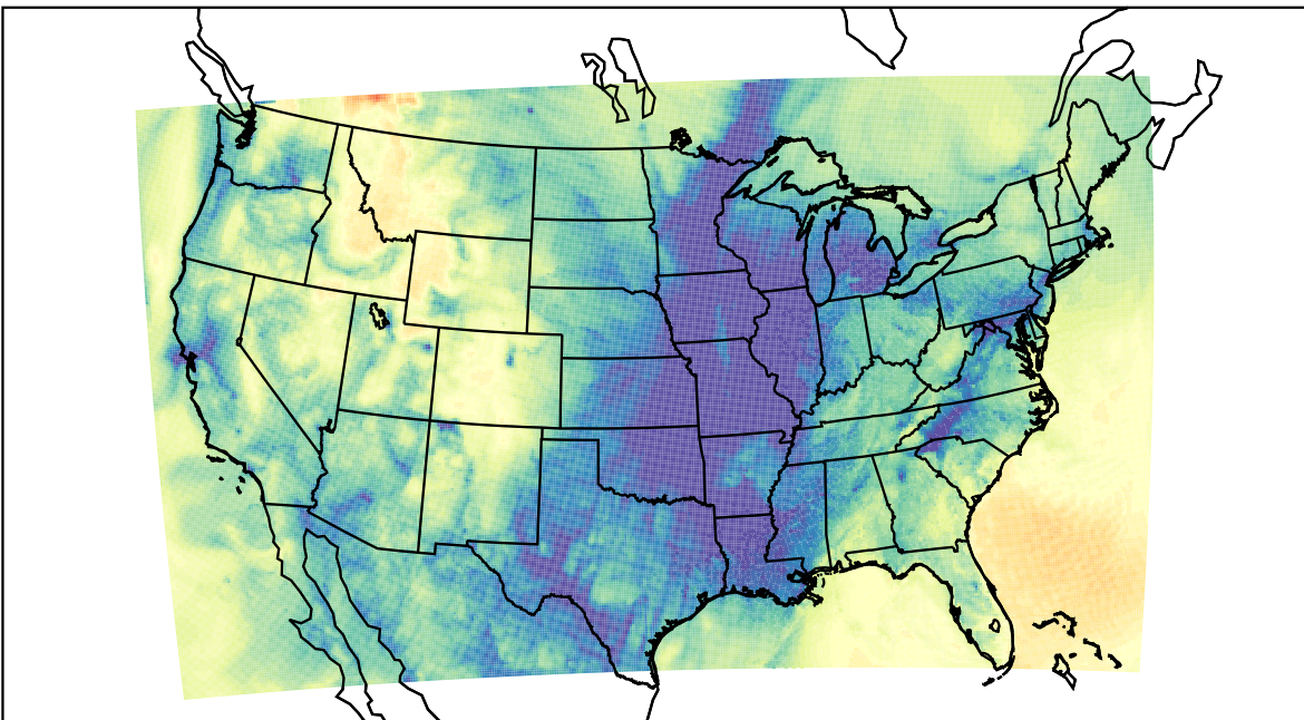
WRF (2023-11-21_14:00:00)
