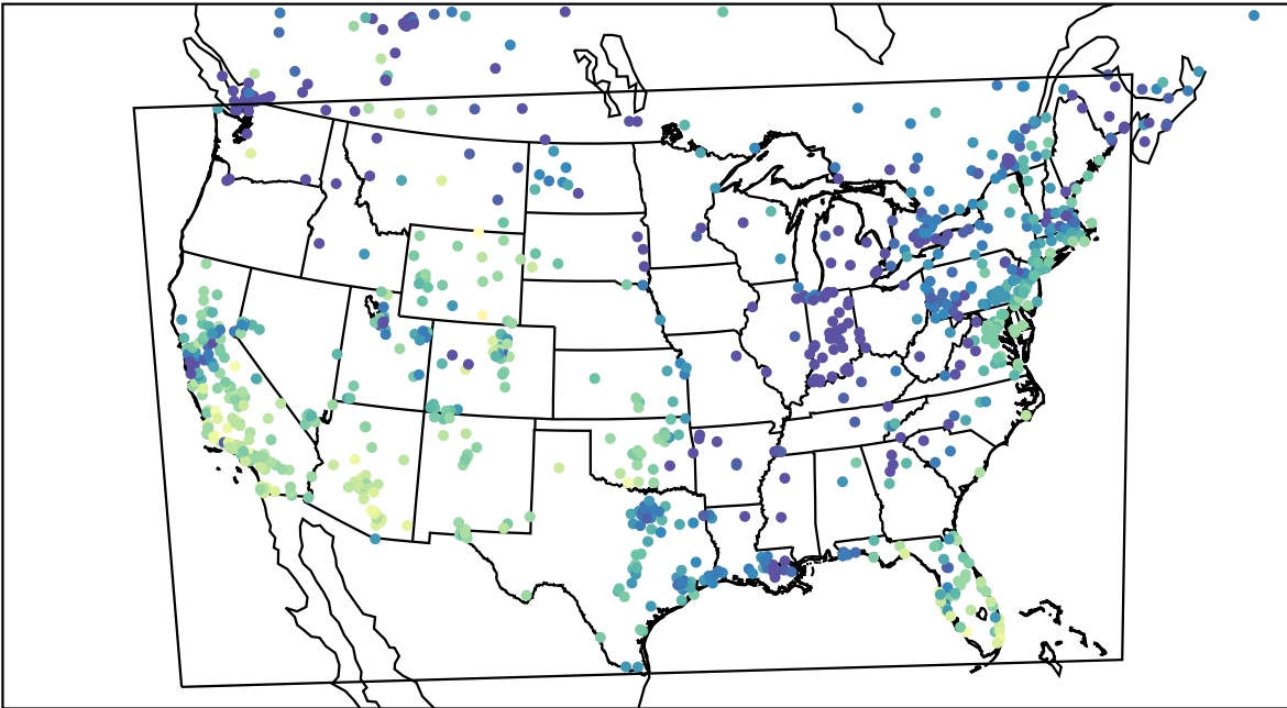
AirNOW (2023-11-21_23:00:00)
