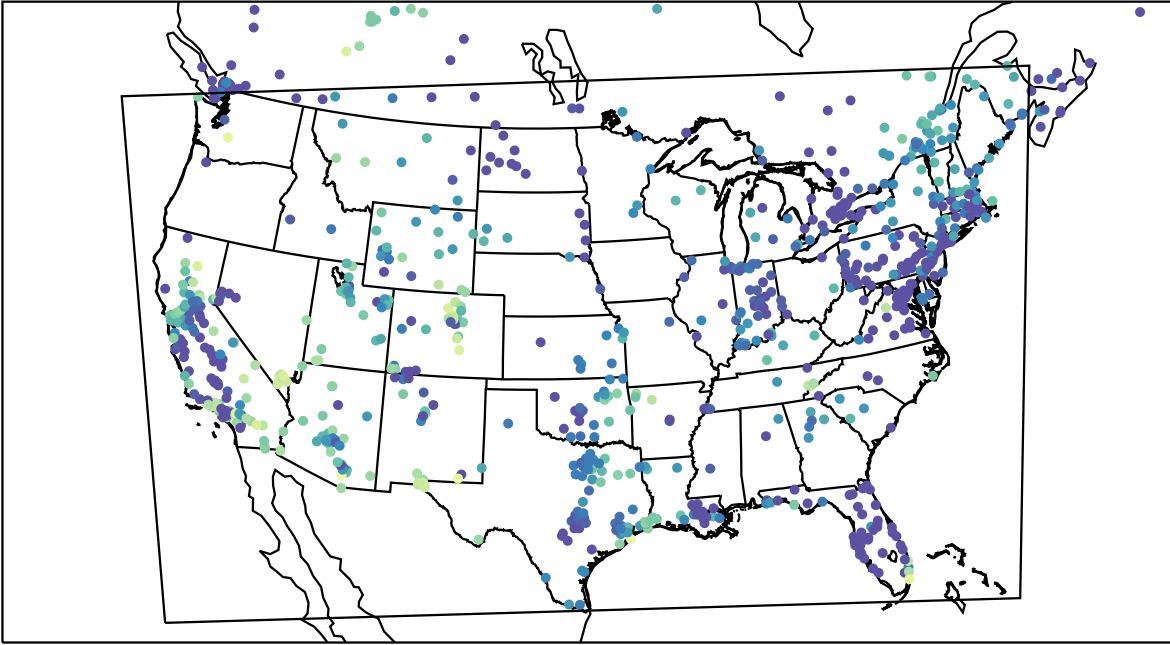
AirNOW (2023-11-20_10:00:00)
