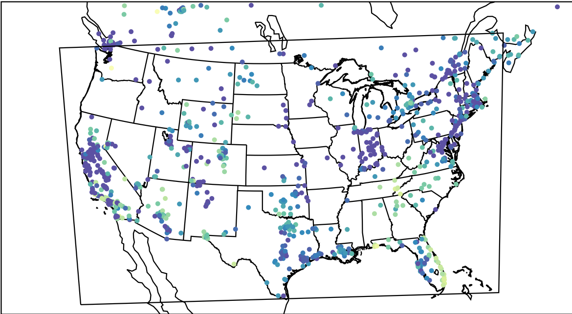
AirNOW (2023-11-21_06:00:00)
