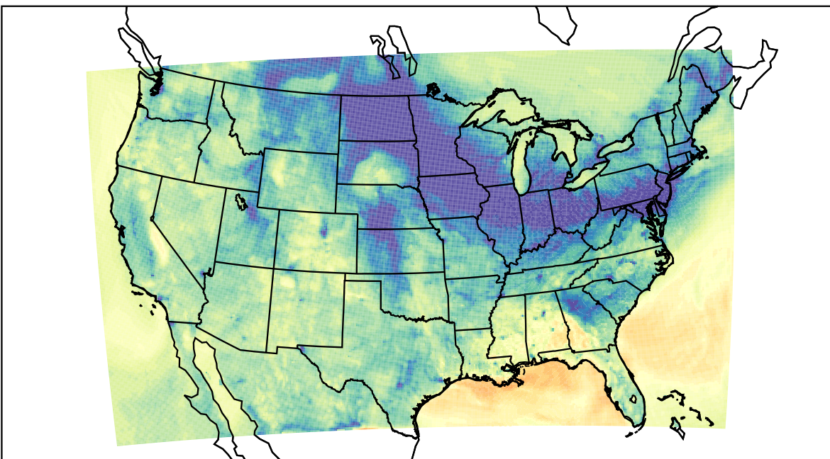
WRF (2023-11-20_01:00:00)
