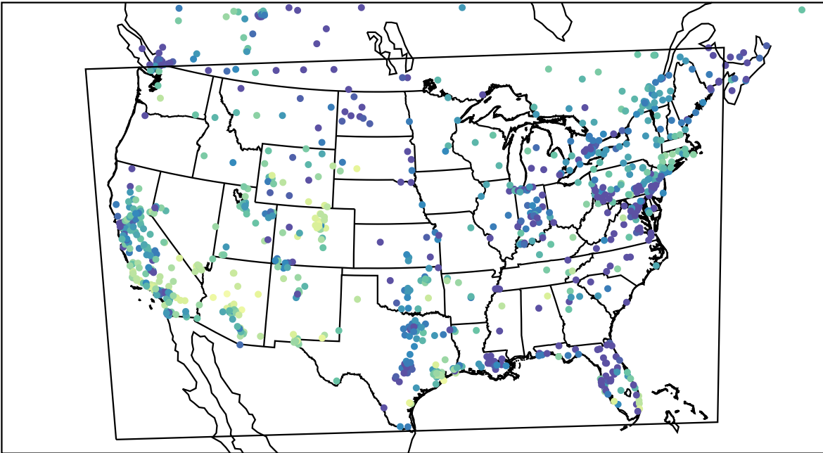
AirNOW (2023-11-20_02:00:00)
