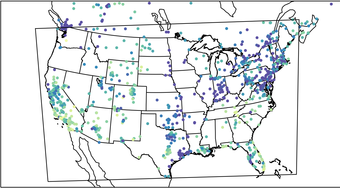
AirNOW (2023-11-21_00:00:00)
