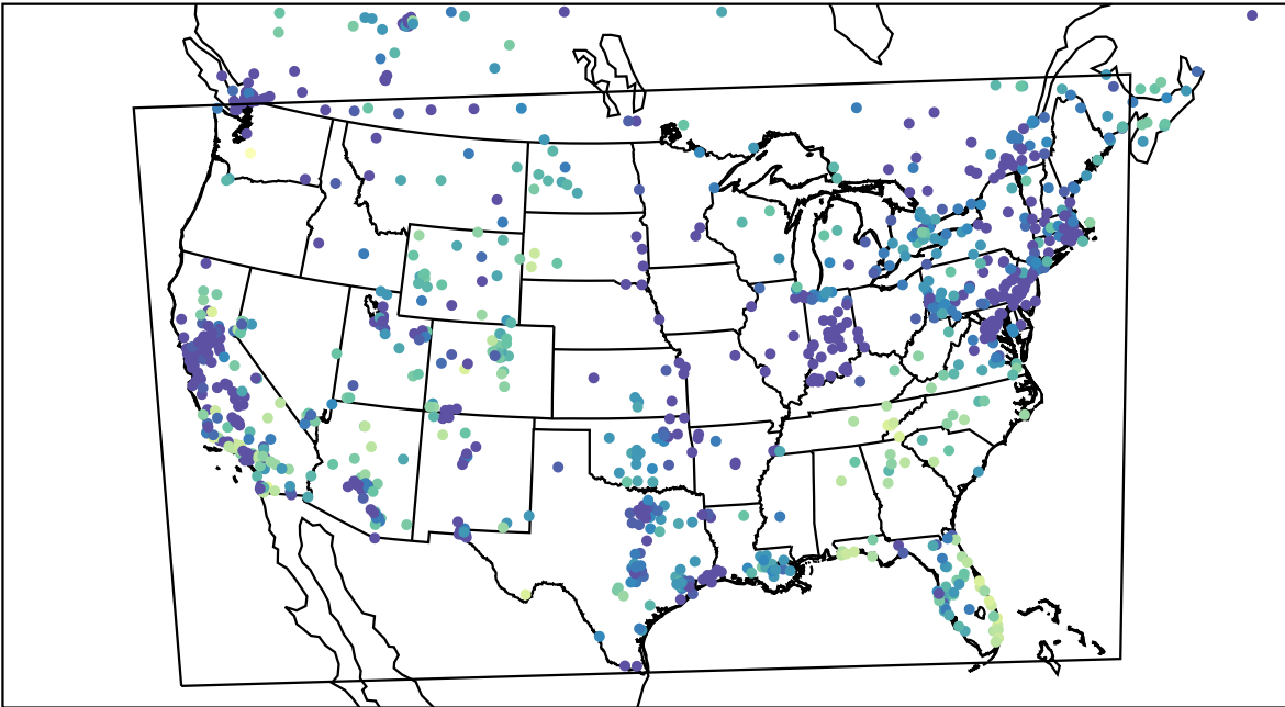
AirNOW (2023-11-21_03:00:00)
