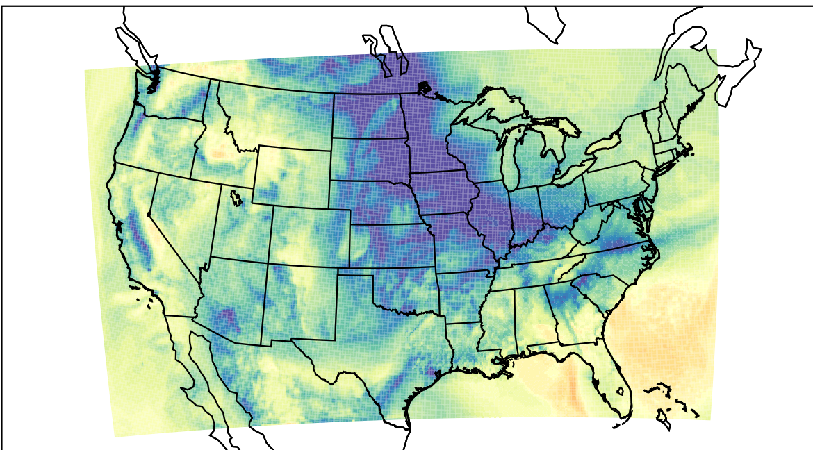
WRF (2023-11-20_16:00:00)
