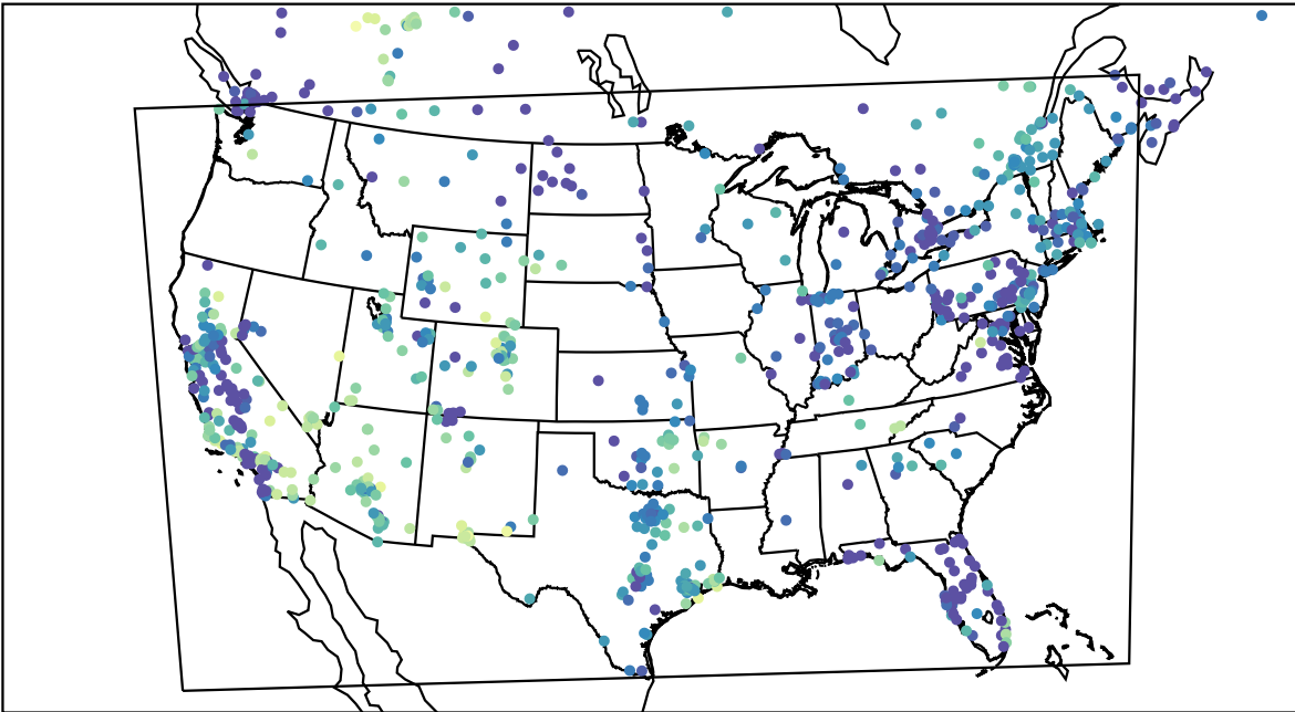
AirNOW (2023-11-20_07:00:00)
