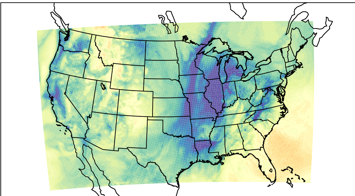
WRF (2023-11-21_17:00:00)
