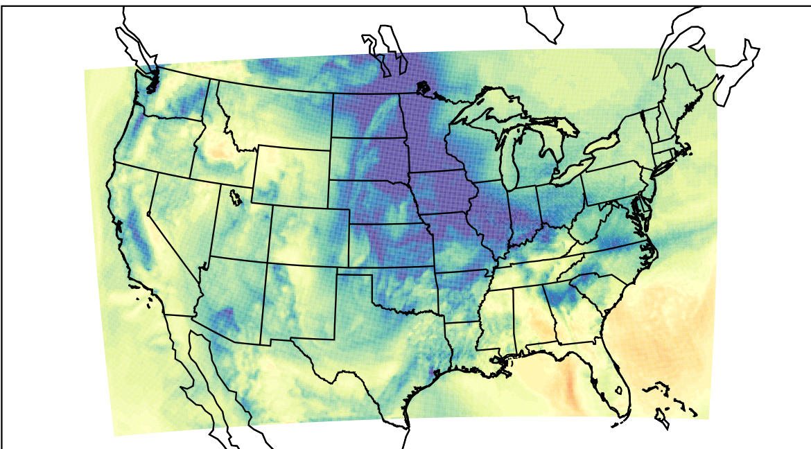
WRF (2023-11-20_17:00:00)
