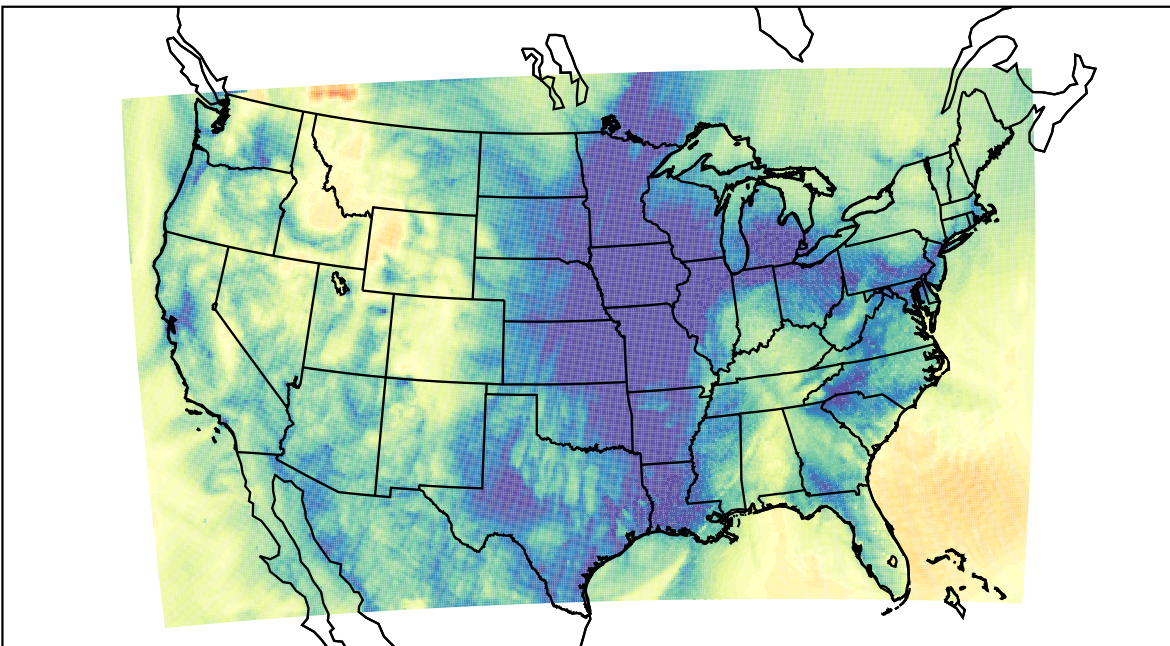
WRF (2023-11-21_09:00:00)
