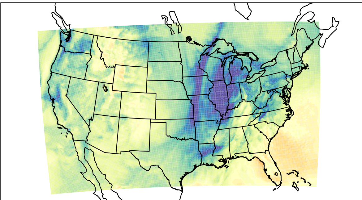
WRF (2023-11-21_19:00:00)
