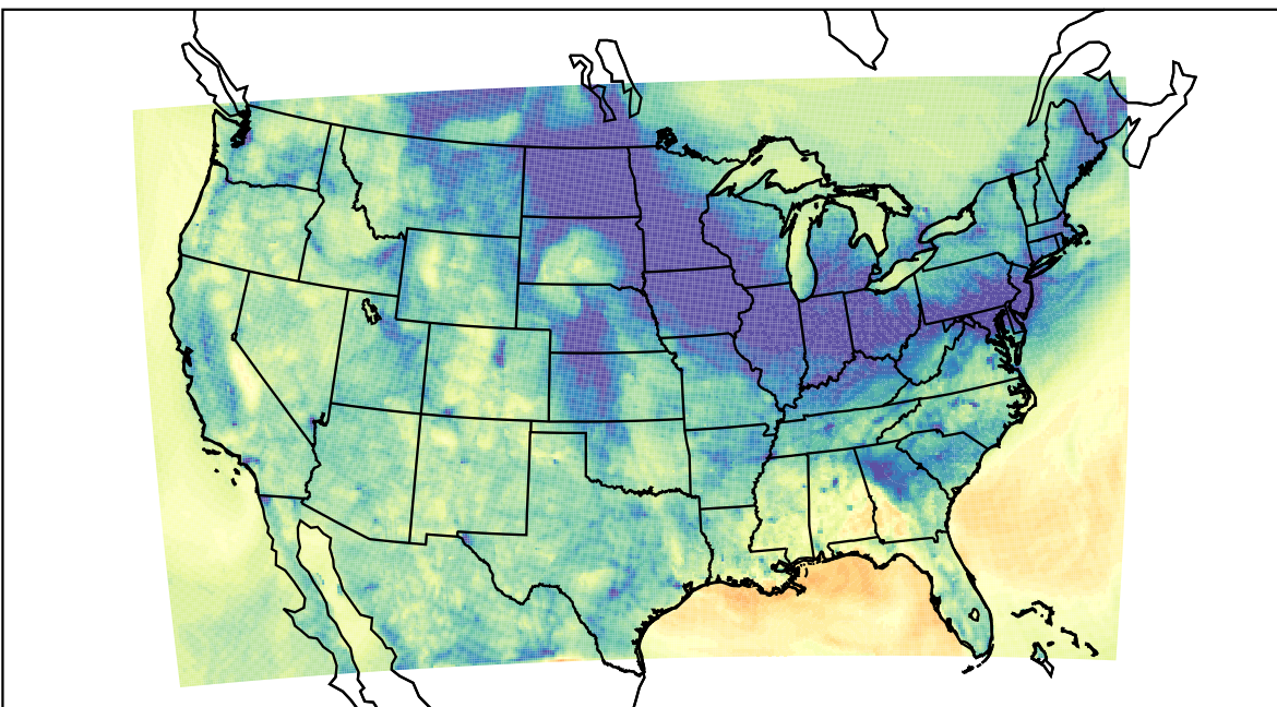
WRF (2023-11-20_02:00:00)
