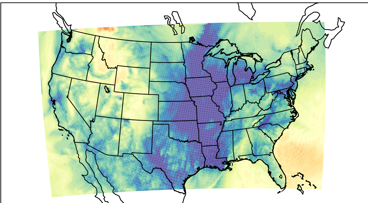
WRF (2023-11-21_12:00:00)
