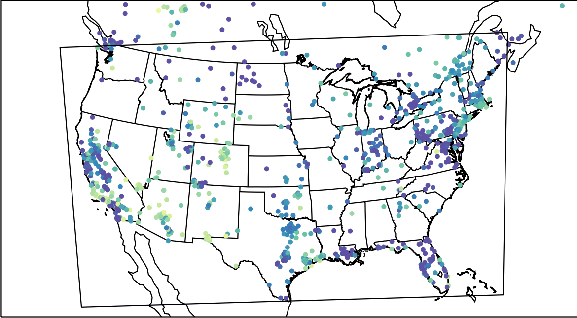
AirNOW (2023-11-20_05:00:00)
