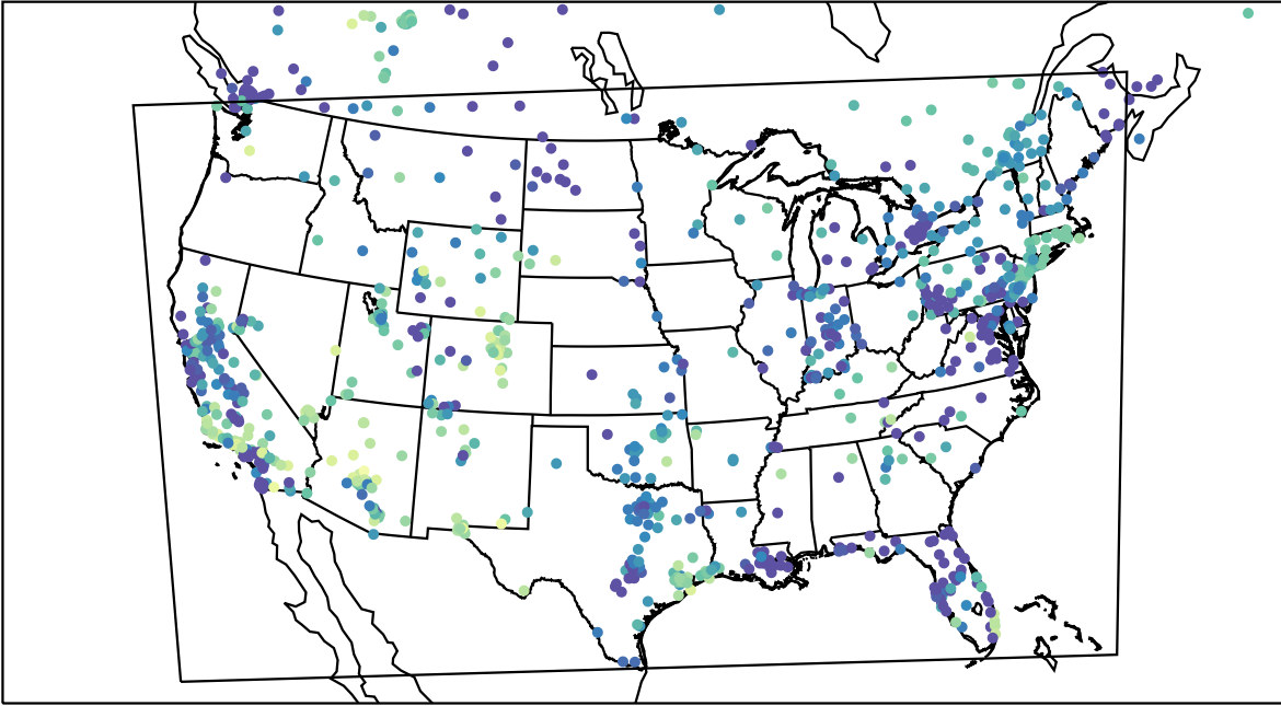
AirNOW (2023-11-20_04:00:00)
