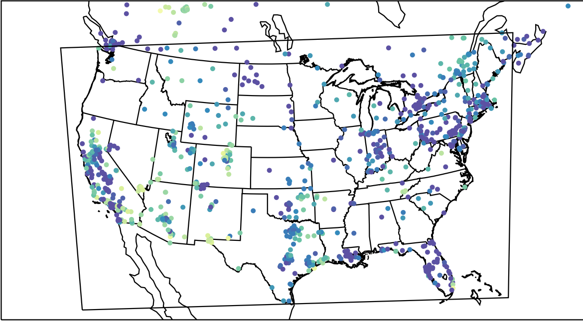
AirNOW (2023-11-20_09:00:00)
