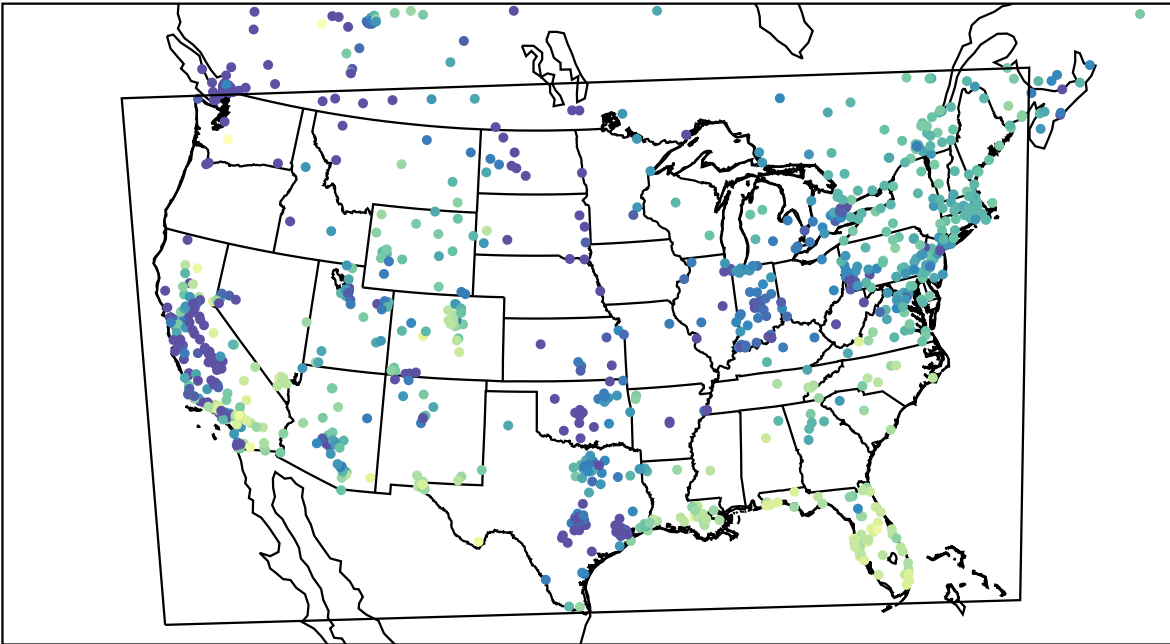
AirNOW (2023-11-20_16:00:00)
