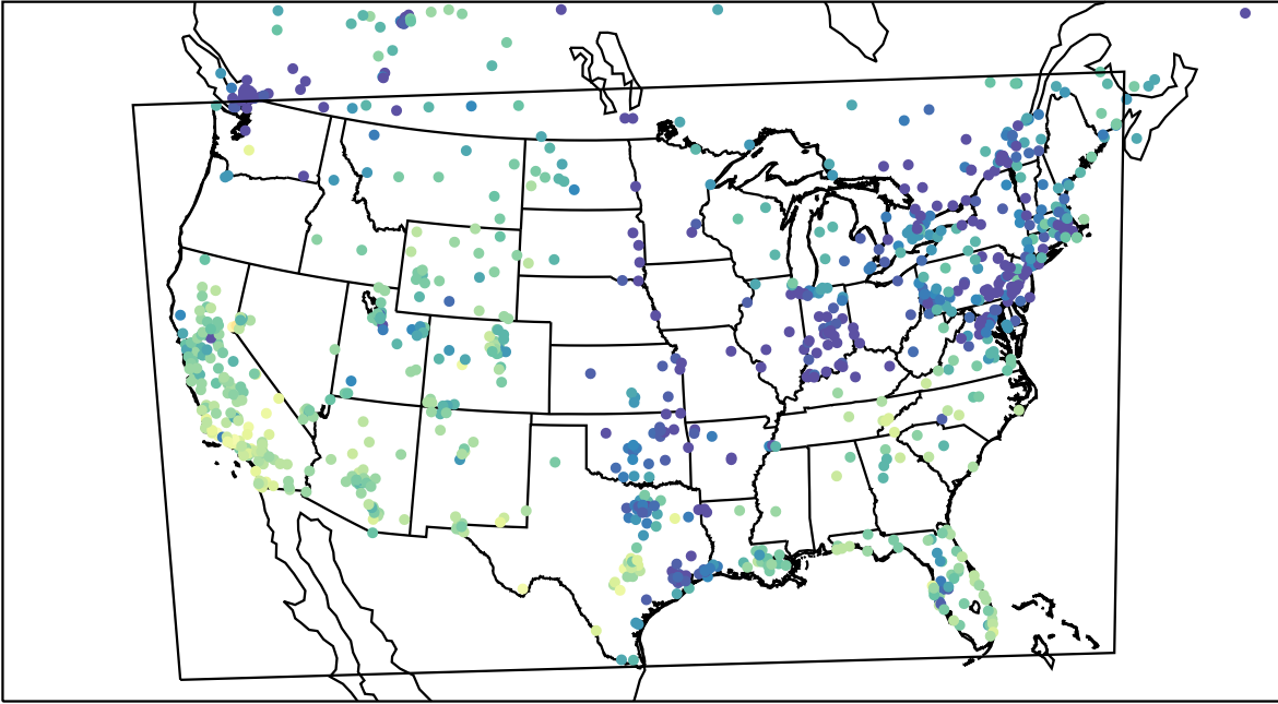
AirNOW (2023-11-20_23:00:00)
