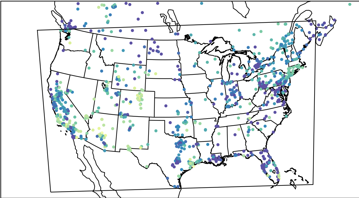
AirNOW (2023-11-20_03:00:00)
