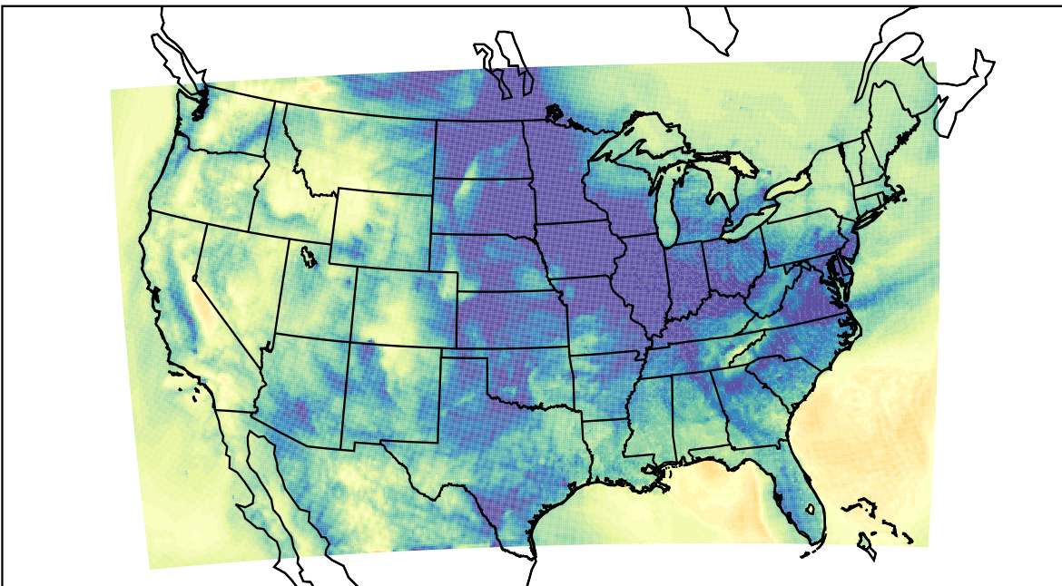
WRF (2023-11-20_13:00:00)
