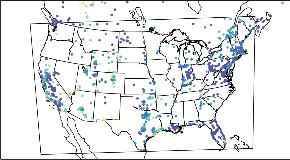
AirNOW (2023-11-20_08:00:00)
