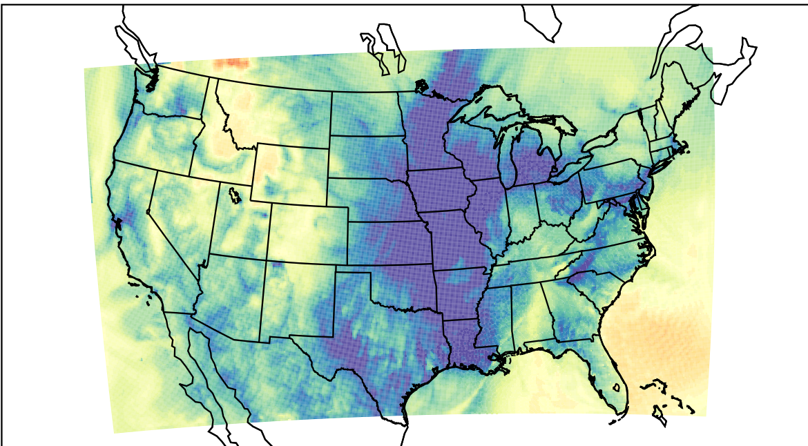
WRF (2023-11-21_11:00:00)
