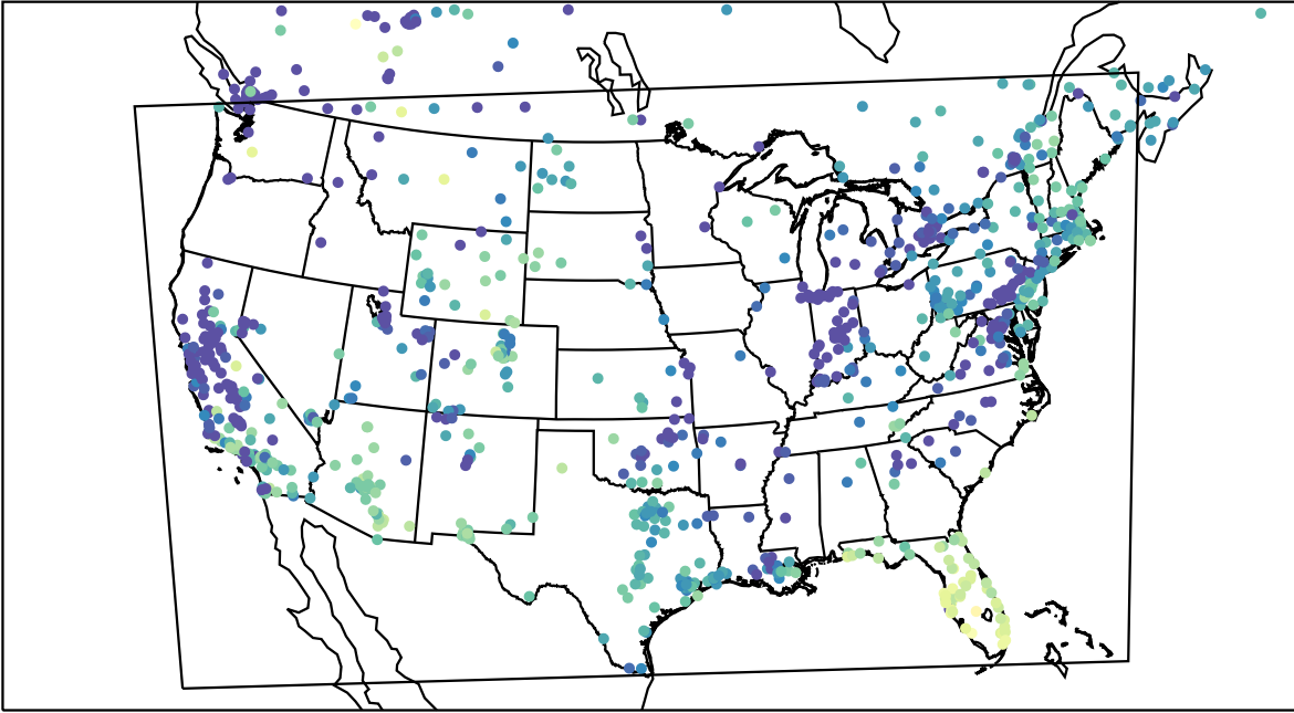
AirNOW (2023-11-21_17:00:00)
