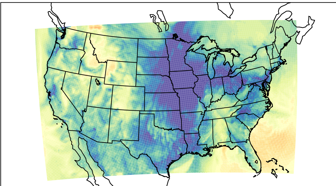
WRF (2023-11-21_07:00:00)
