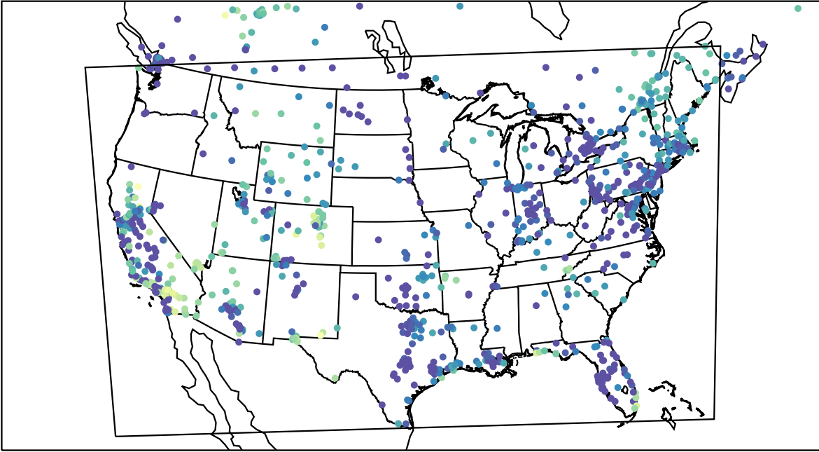
AirNOW (2023-11-20_13:00:00)
