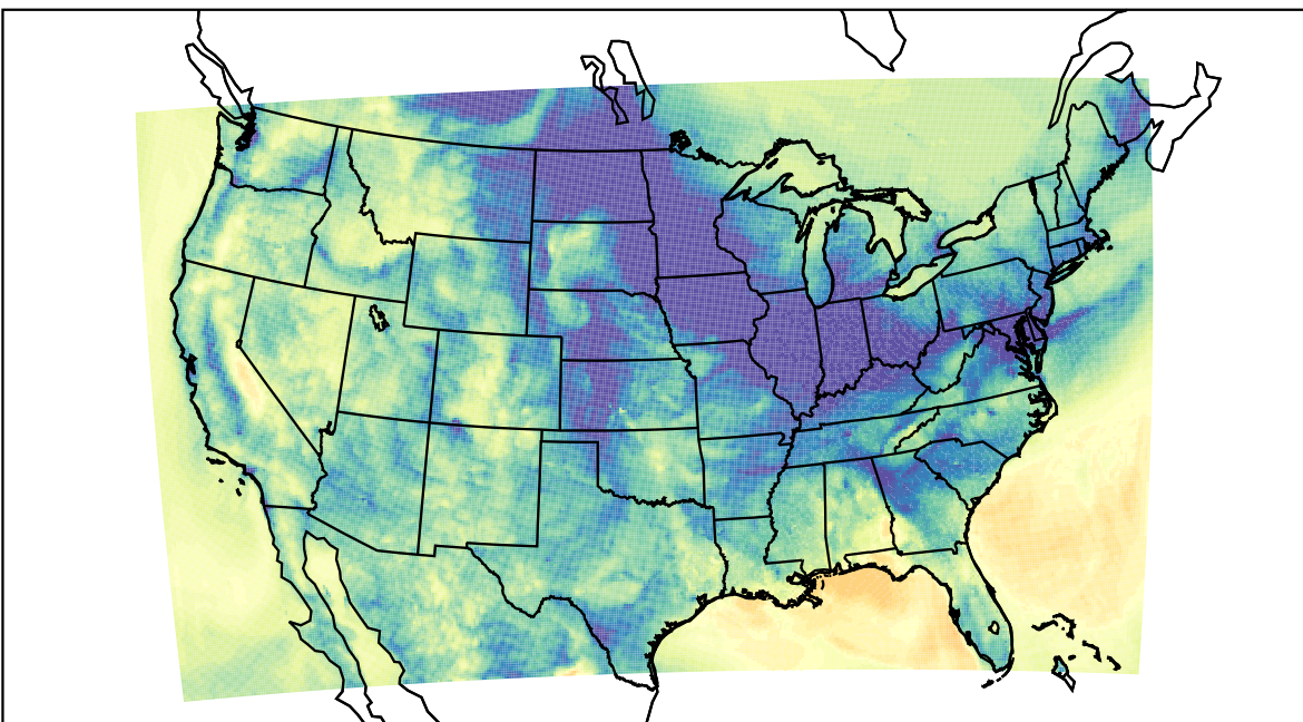
WRF (2023-11-20_06:00:00)
