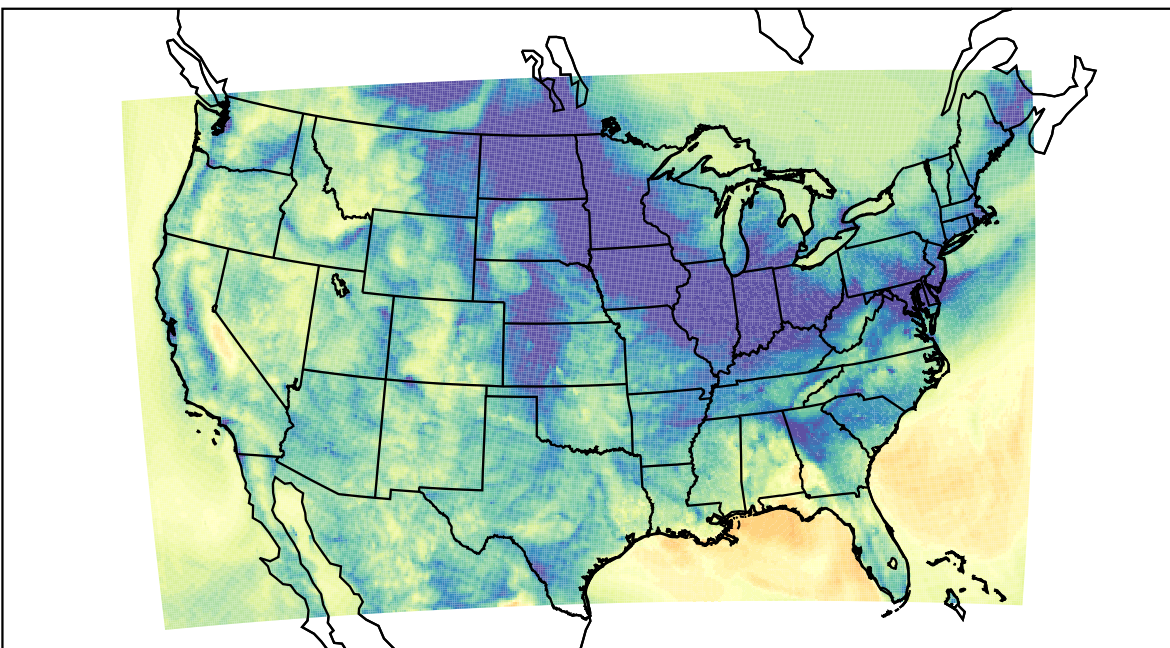
WRF (2023-11-20_05:00:00)
