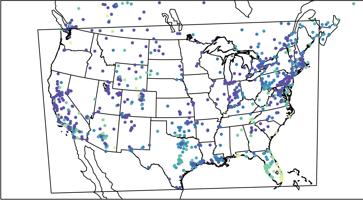
AirNOW (2023-11-21_14:00:00)
