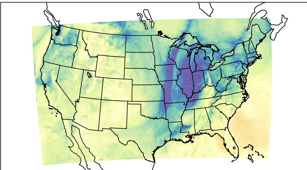
WRF (2023-11-21_21:00:00)
