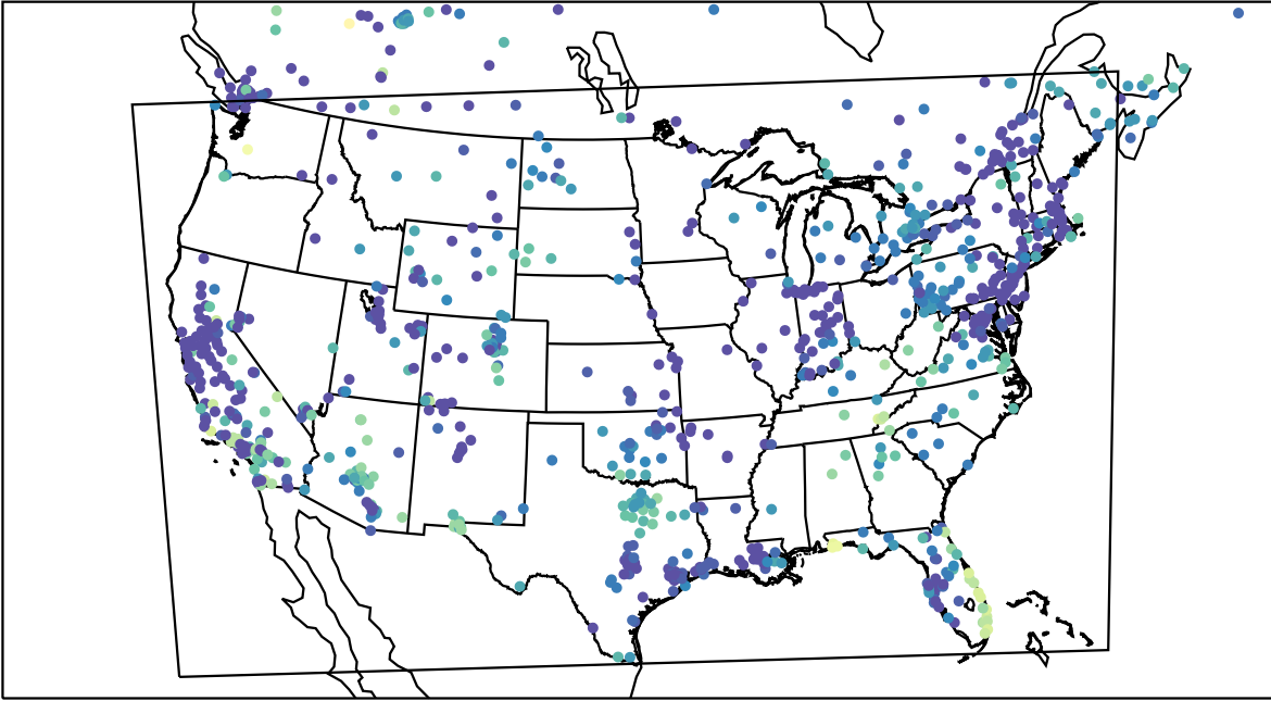
AirNOW (2023-11-21_09:00:00)
