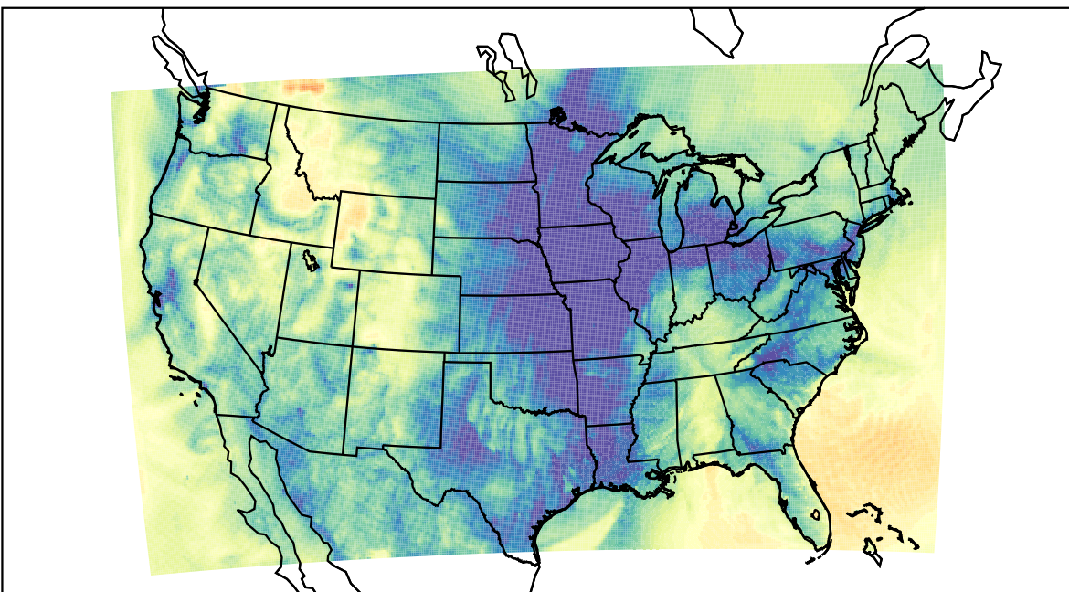
WRF (2023-11-21_08:00:00)
