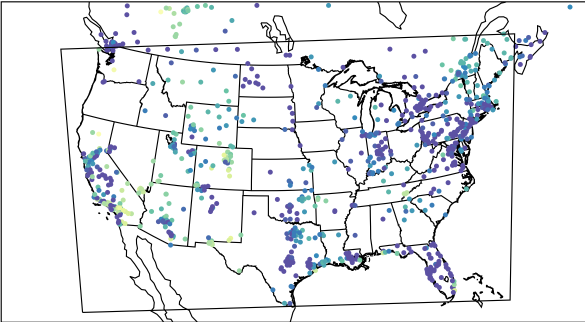
AirNOW (2023-11-20_12:00:00)
