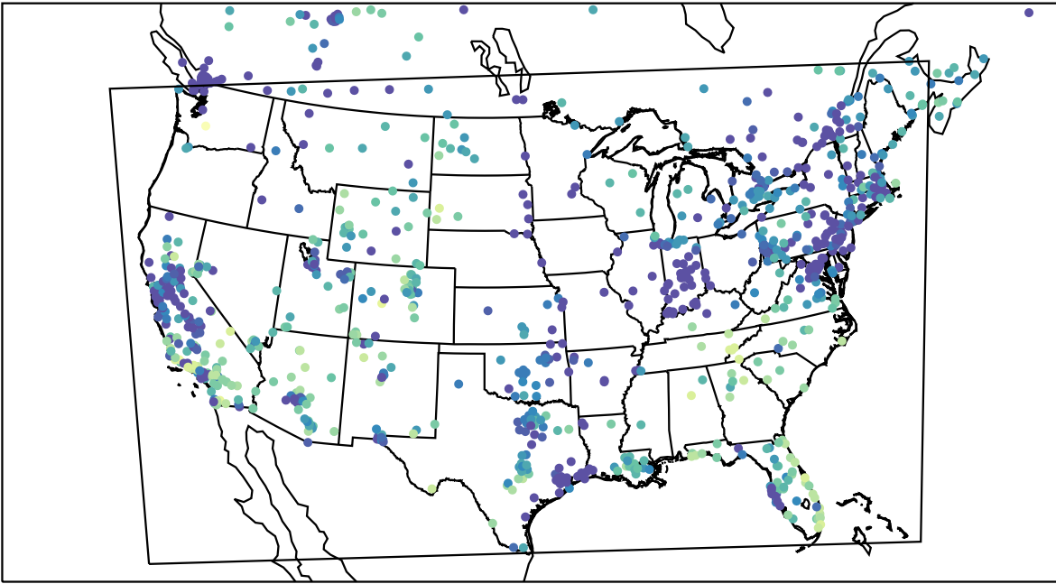
AirNOW (2023-11-21_01:00:00)
