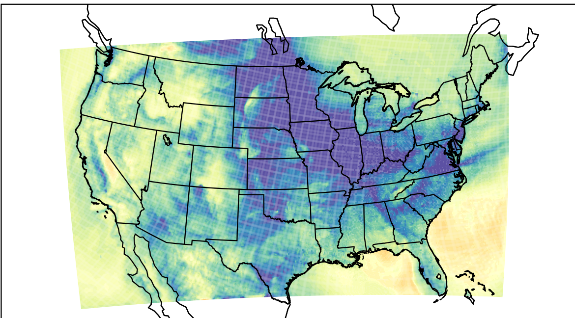
WRF (2023-11-20_12:00:00)
