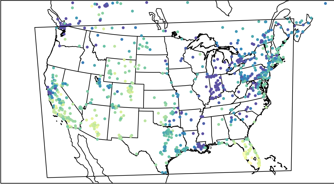
AirNOW (2023-11-21_20:00:00)
