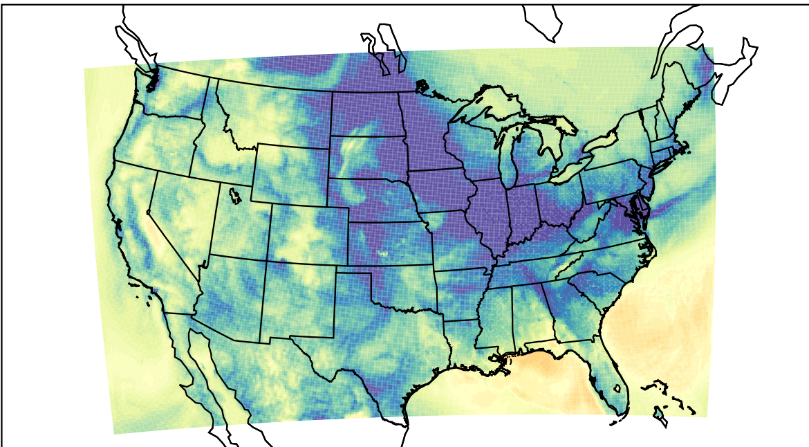
WRF (2023-11-20_08:00:00)
