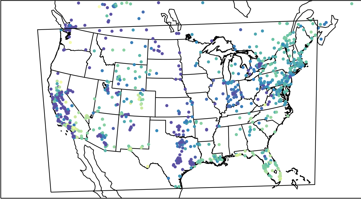
AirNOW (2023-11-20_15:00:00)
