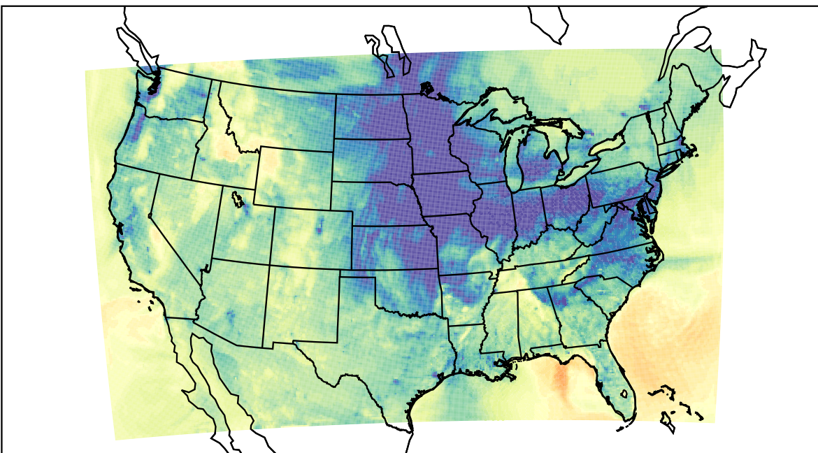
WRF (2023-11-21_00:00:00)
