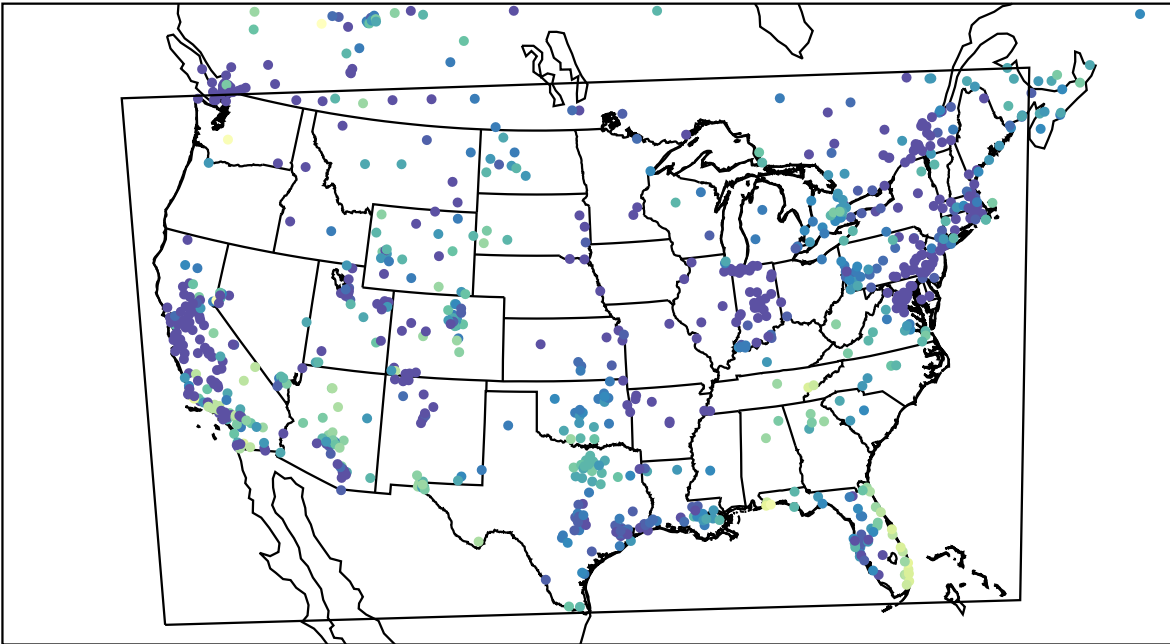
AirNOW (2023-11-21_07:00:00)
