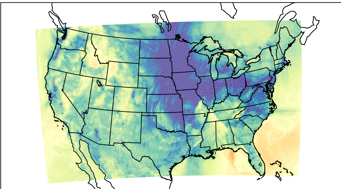
WRF (2023-11-21_02:00:00)
