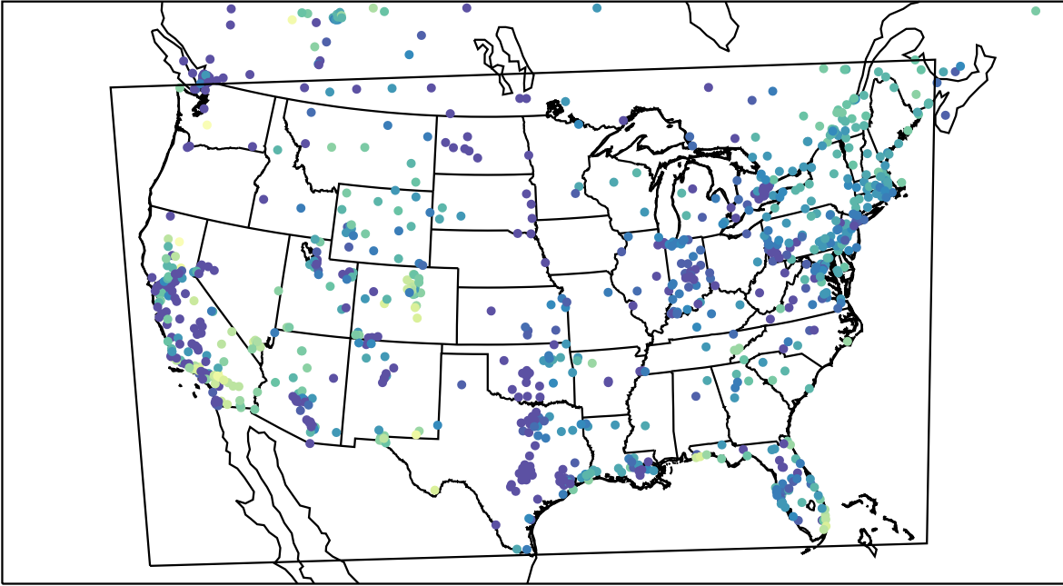
AirNOW (2023-11-20_14:00:00)
