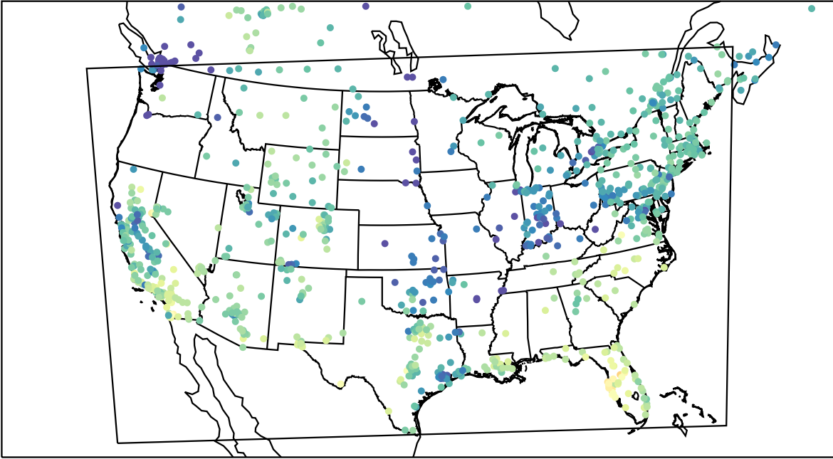
AirNOW (2023-11-20_19:00:00)
