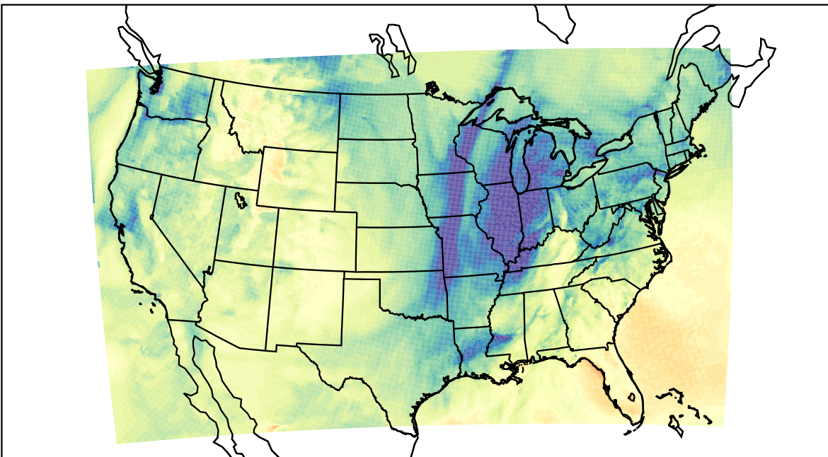
WRF (2023-11-21_20:00:00)
