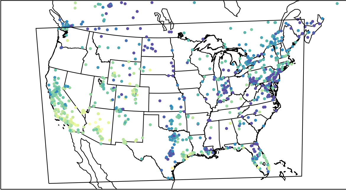
AirNOW (2023-11-20_00:00:00)
