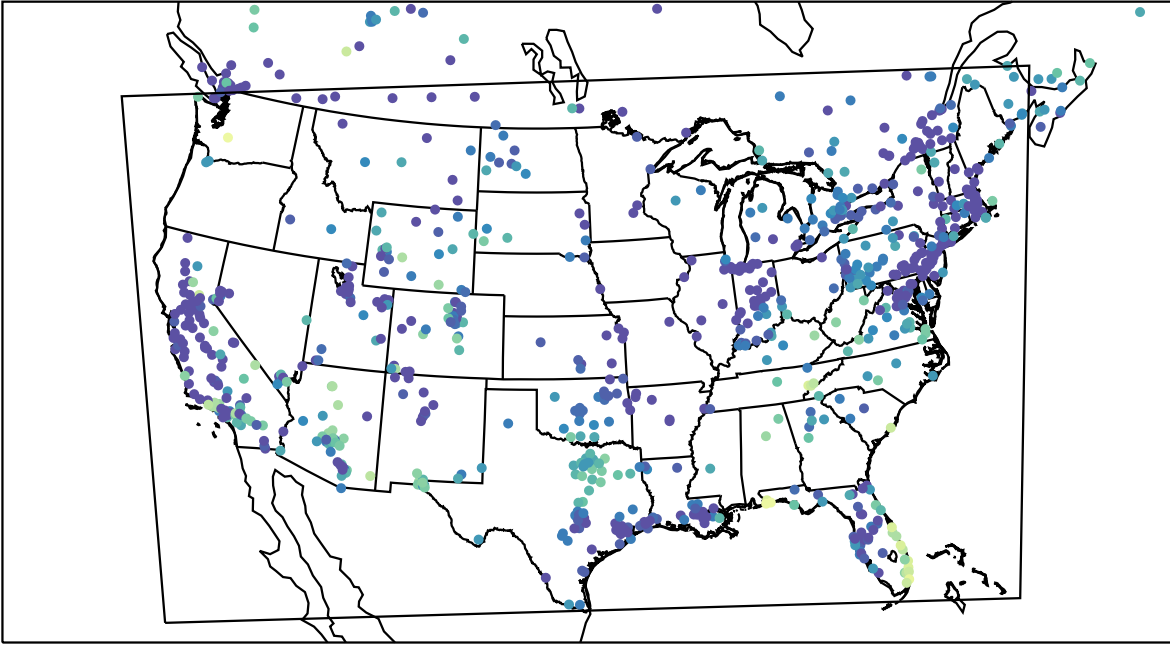
AirNOW (2023-11-21_10:00:00)
