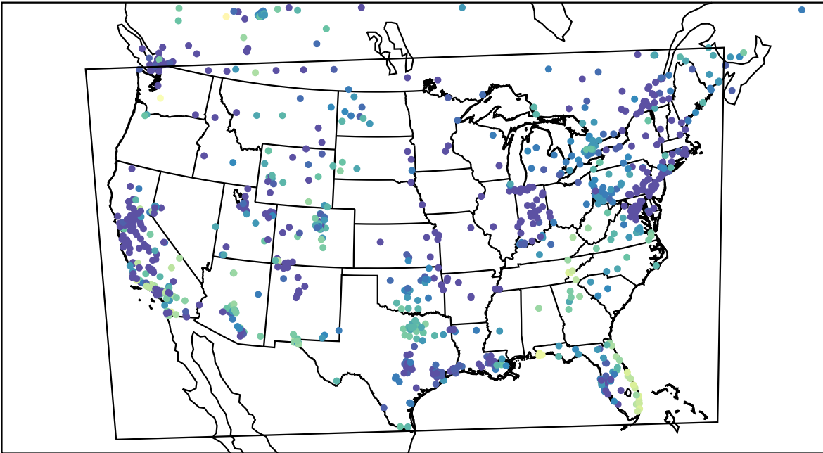
AirNOW (2023-11-21_08:00:00)
