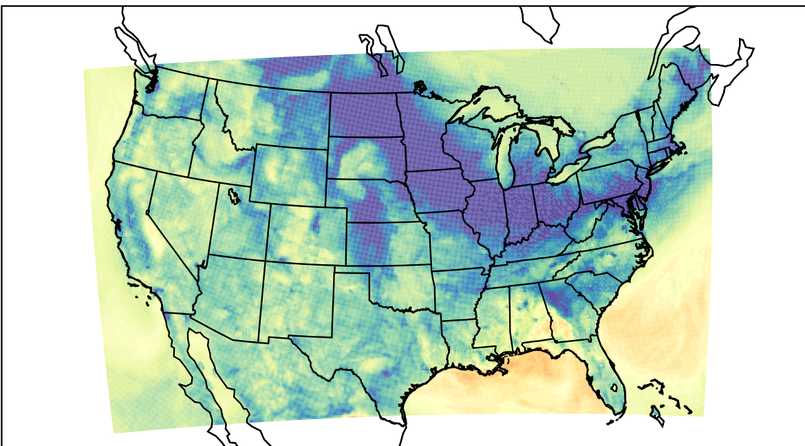
WRF (2023-11-20_03:00:00)
