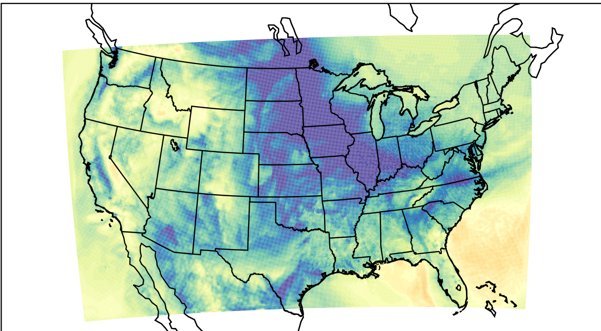
WRF (2023-11-20_15:00:00)
