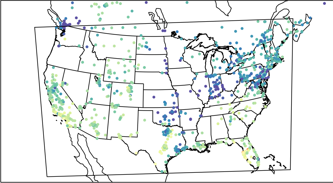
AirNOW (2023-11-20_21:00:00)
