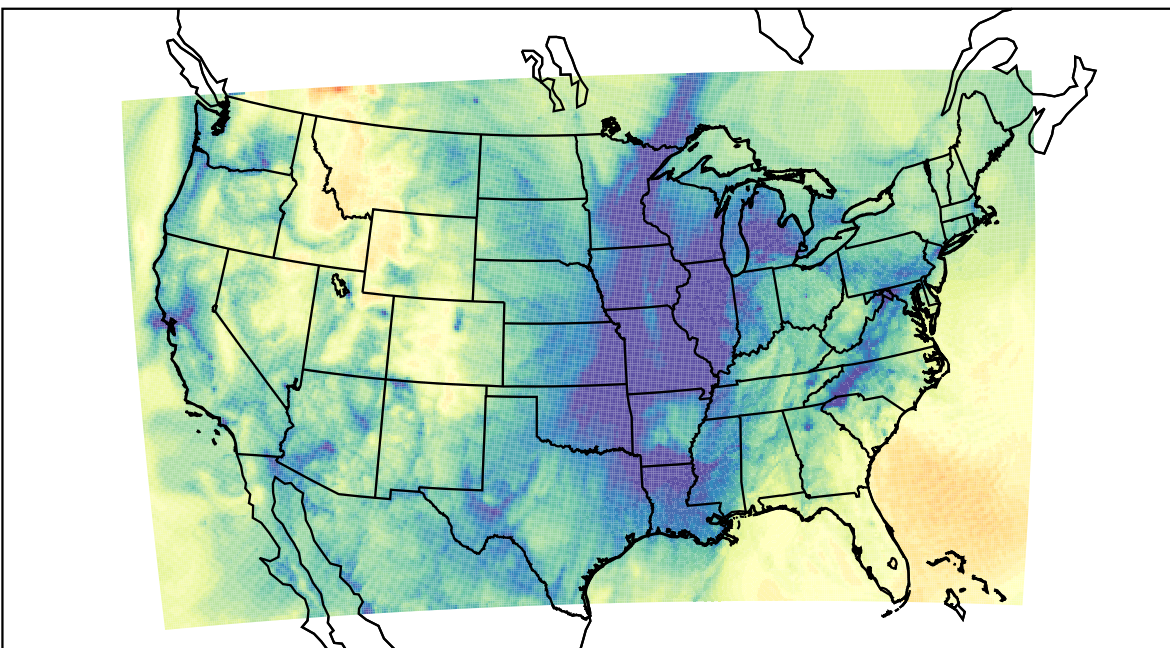
WRF (2023-11-21_15:00:00)
