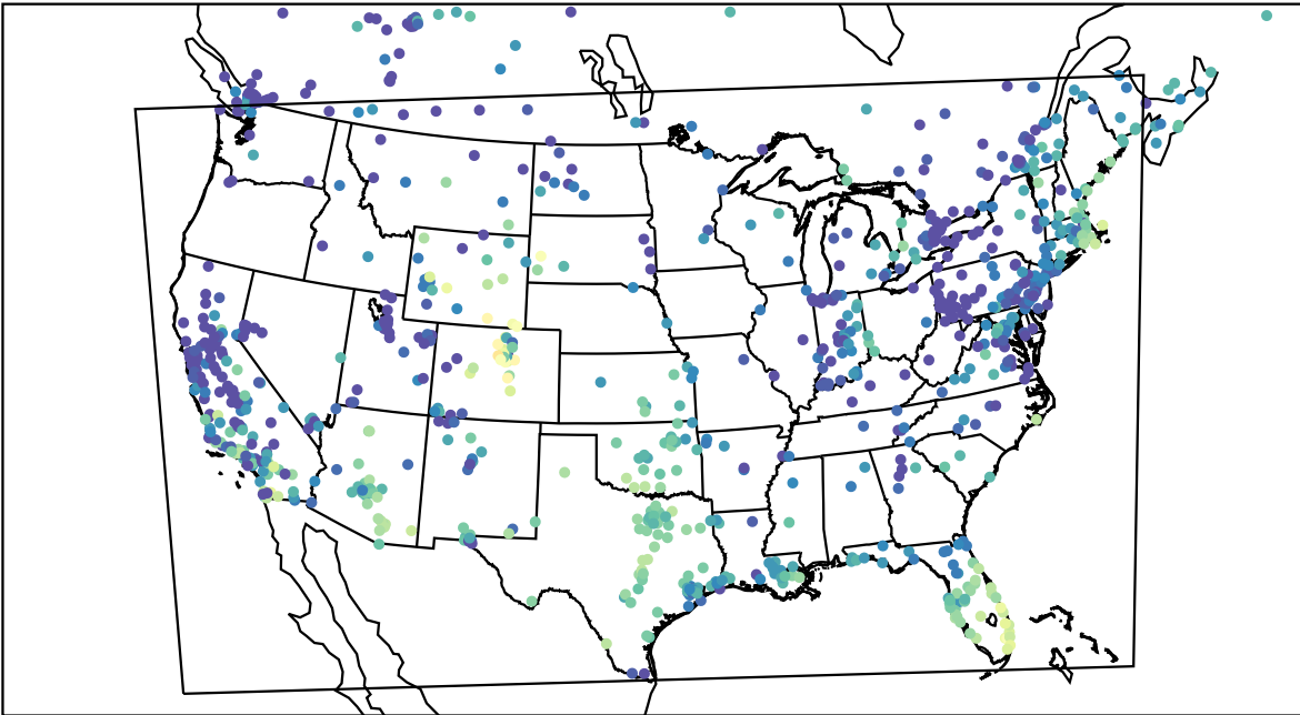
AirNOW (2023-11-22_17:00:00)
