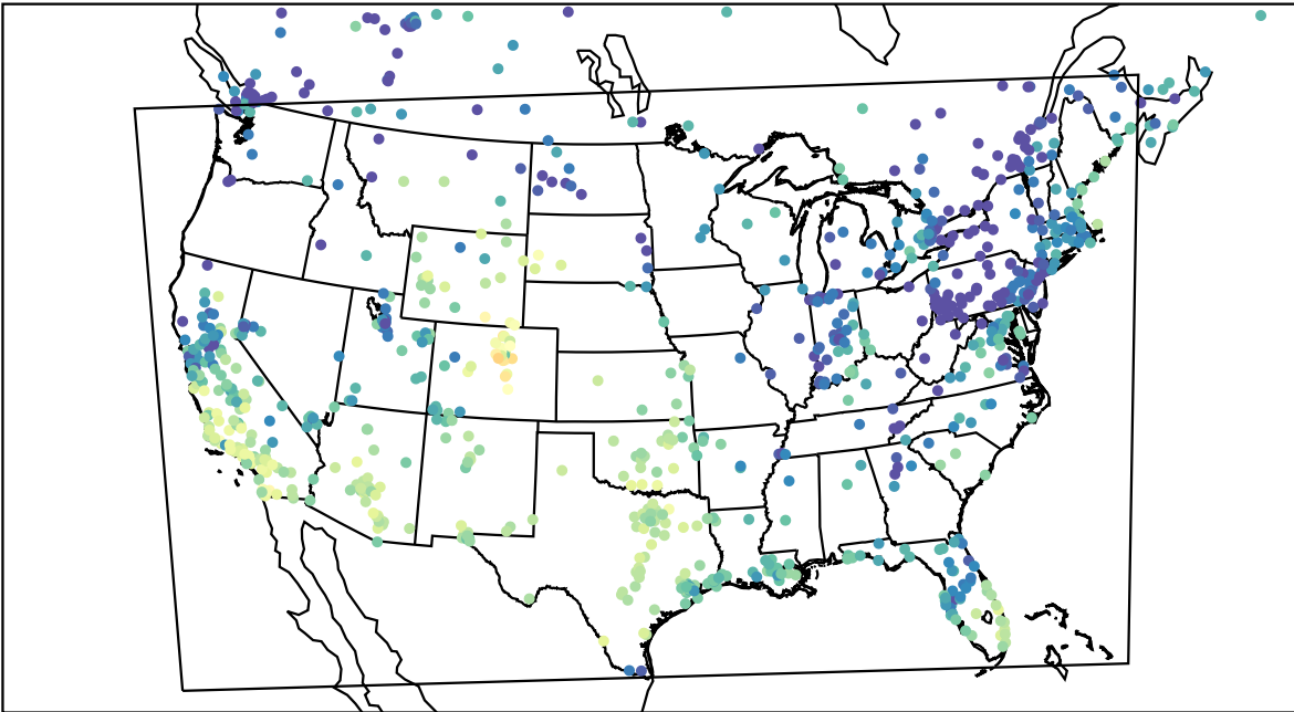
AirNOW (2023-11-22_20:00:00)
