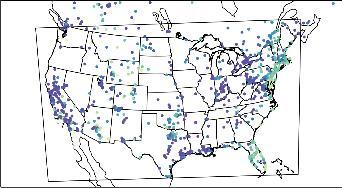
AirNOW (2023-11-22_04:00:00)
