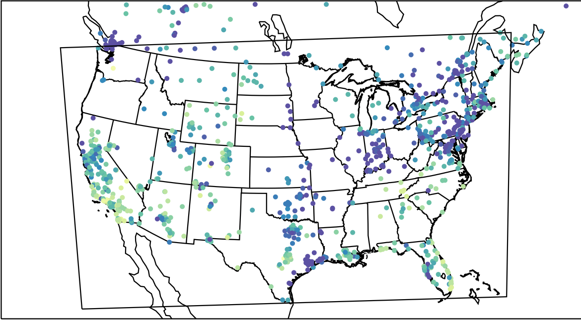
AirNOW (2023-11-21_00:00:00)
