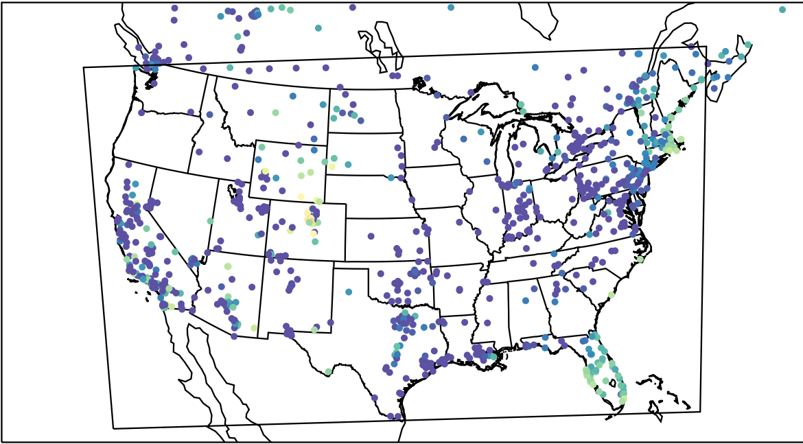
AirNOW (2023-11-22_14:00:00)
