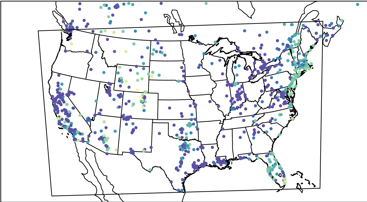
AirNOW (2023-11-22_06:00:00)
