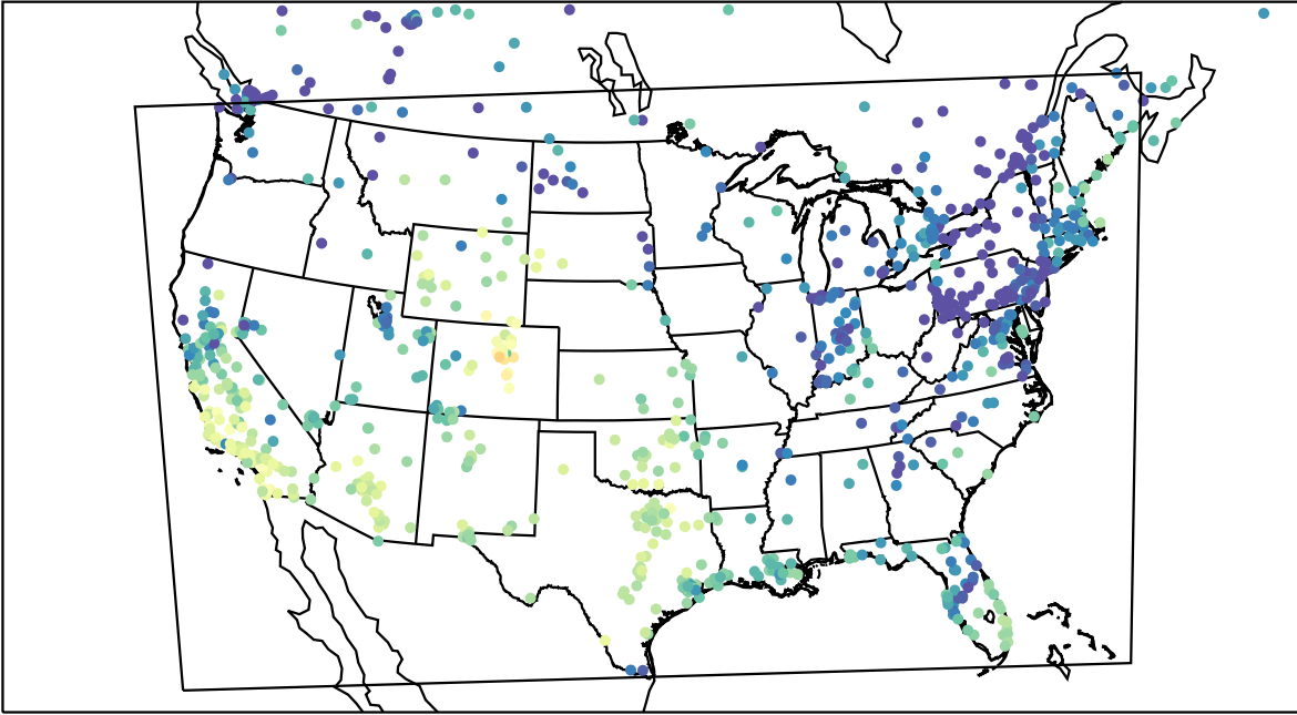
AirNOW (2023-11-22_21:00:00)
