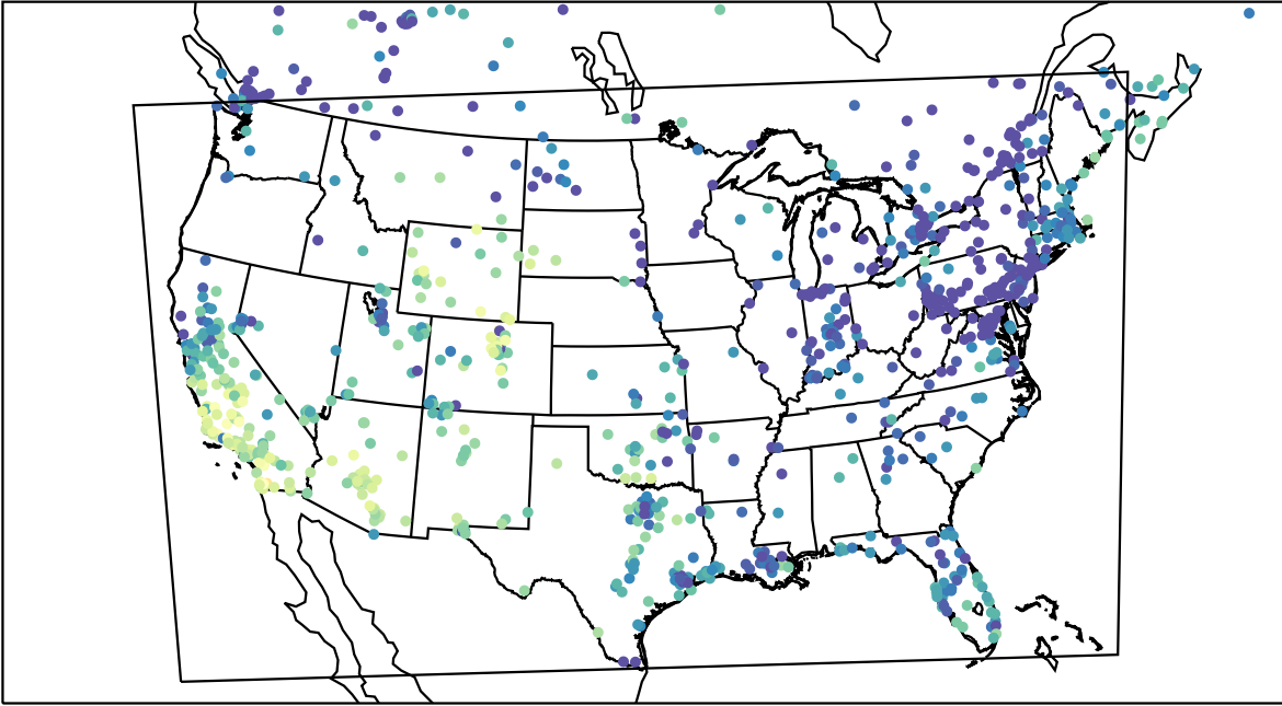
AirNOW (2023-11-22_23:00:00)
