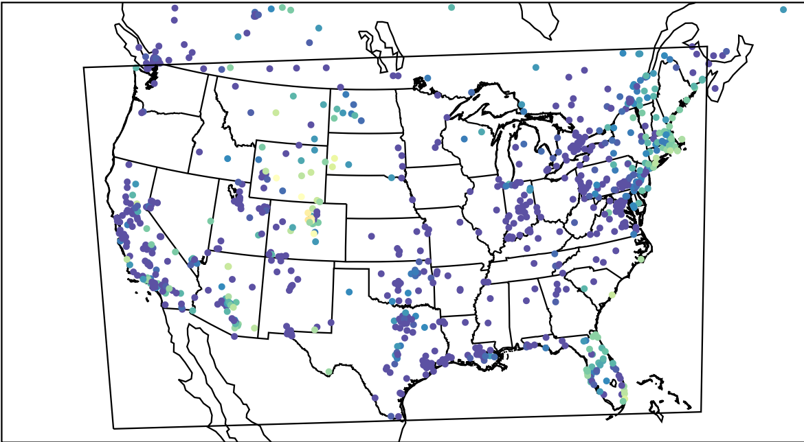
AirNOW (2023-11-22_10:00:00)
