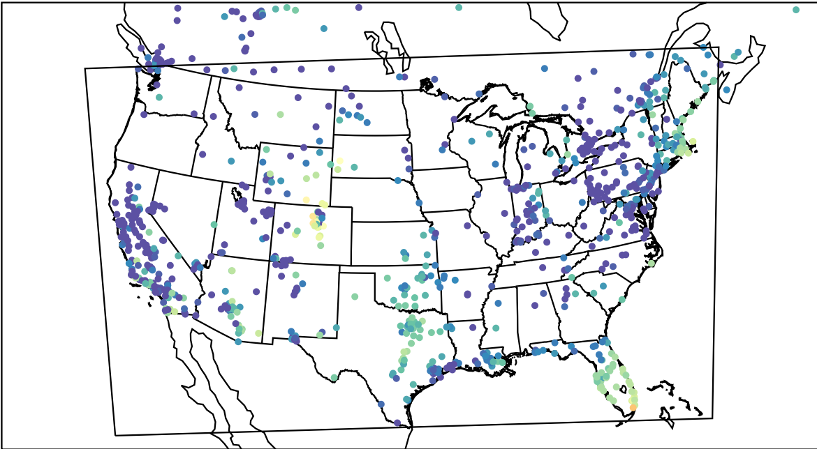
AirNOW (2023-11-22_16:00:00)
