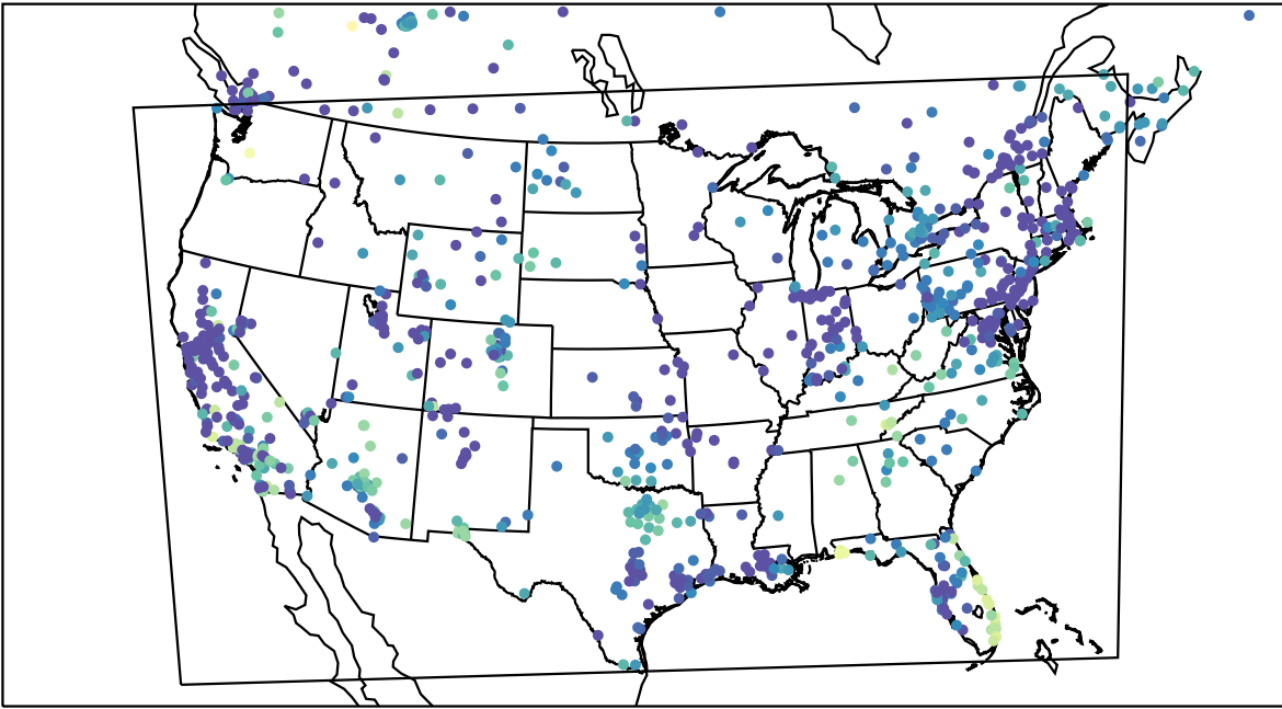
AirNOW (2023-11-21_09:00:00)
