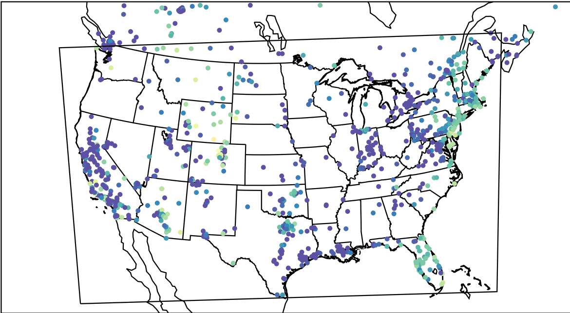
AirNOW (2023-11-22_05:00:00)
