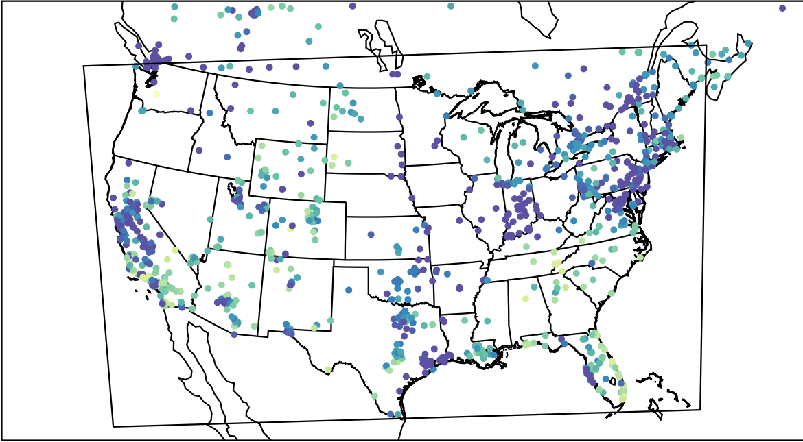
AirNOW (2023-11-21_01:00:00)
