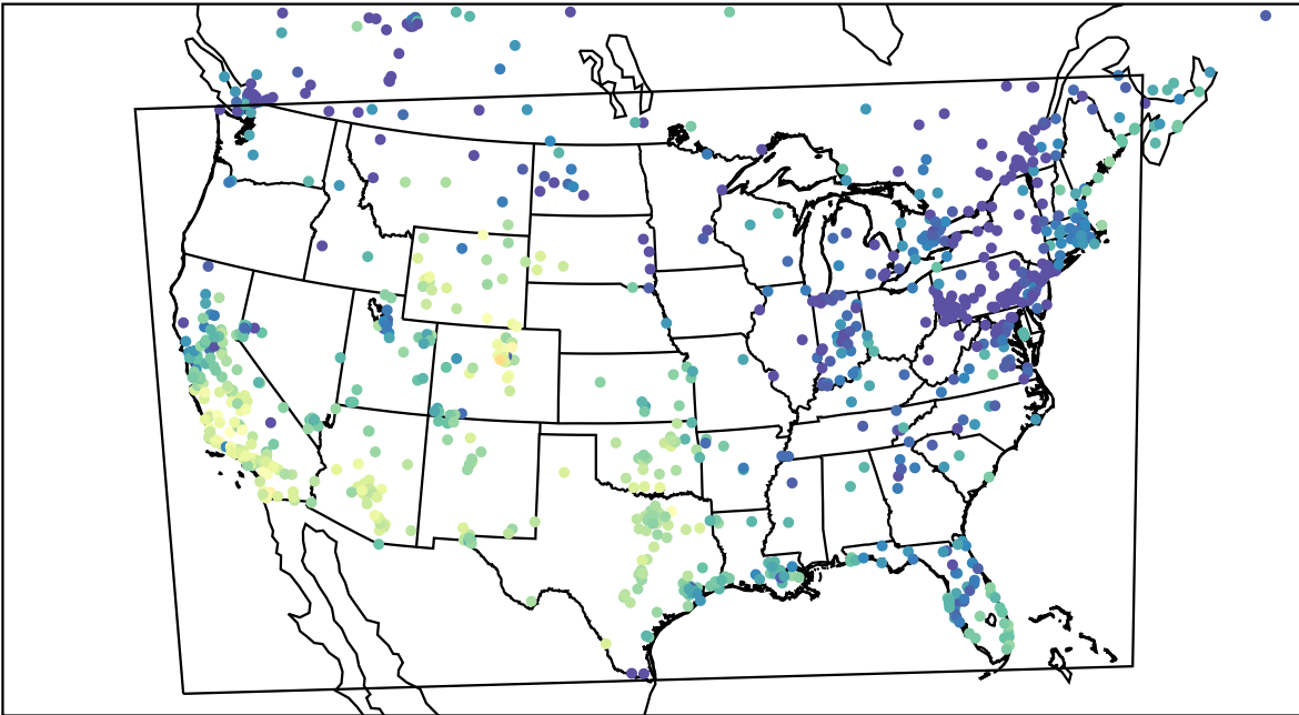
AirNOW (2023-11-22_22:00:00)
