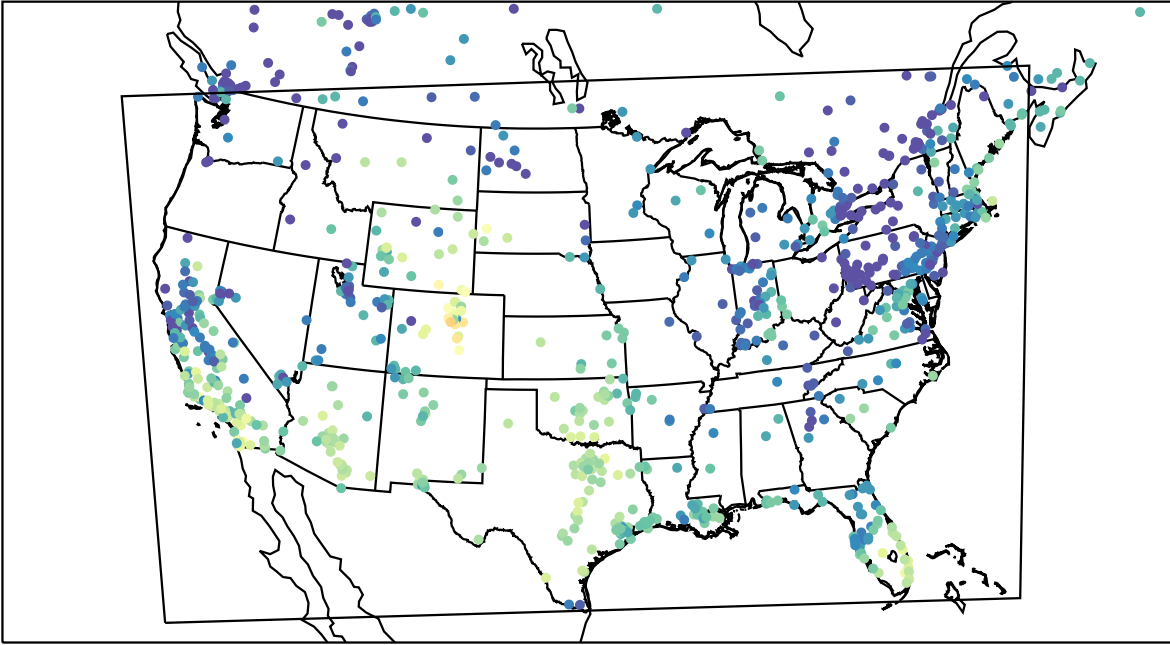
AirNOW (2023-11-22_19:00:00)
