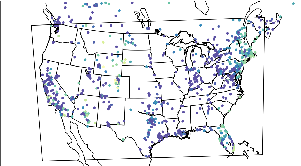
AirNOW (2023-11-22_09:00:00)
