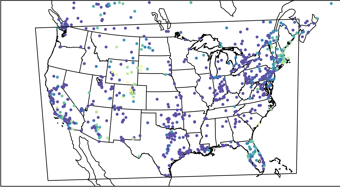
AirNOW (2023-11-22_12:00:00)
