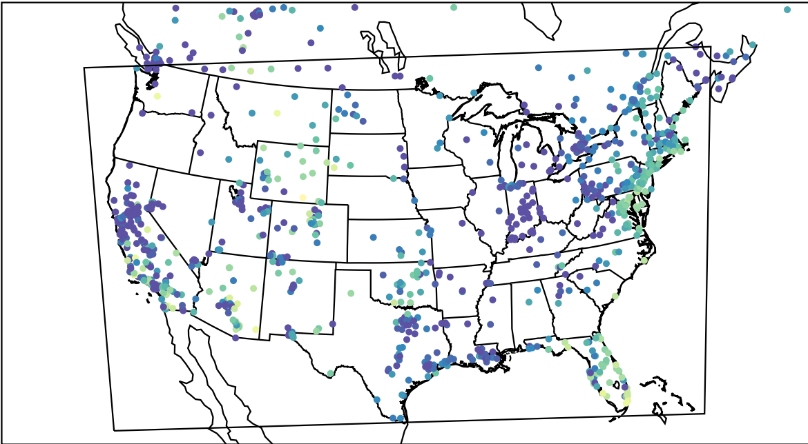
AirNOW (2023-11-22_01:00:00)
