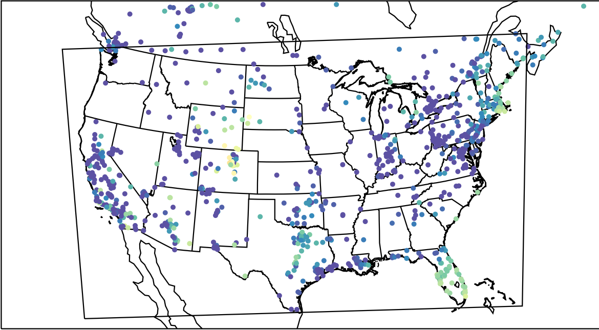
AirNOW (2023-11-22_15:00:00)
