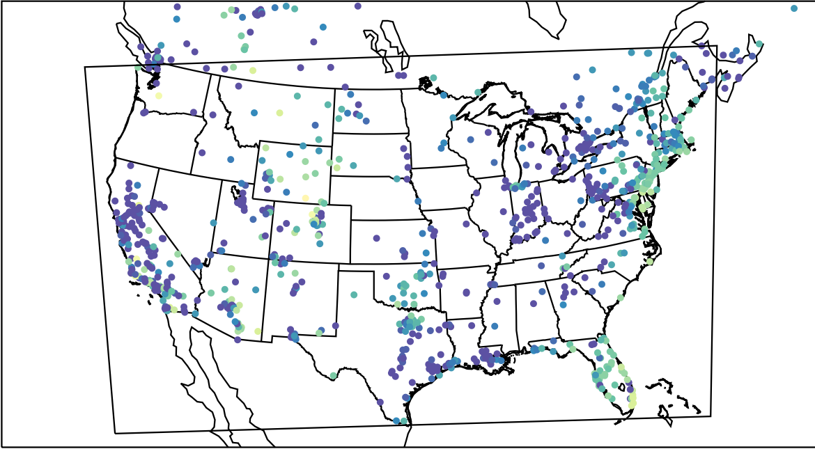
AirNOW (2023-11-22_03:00:00)
