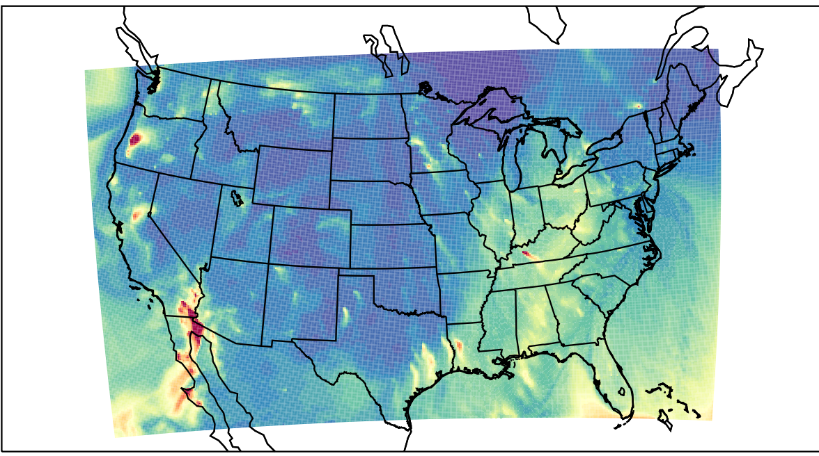
WRF 2023-11-22_08:00:00
