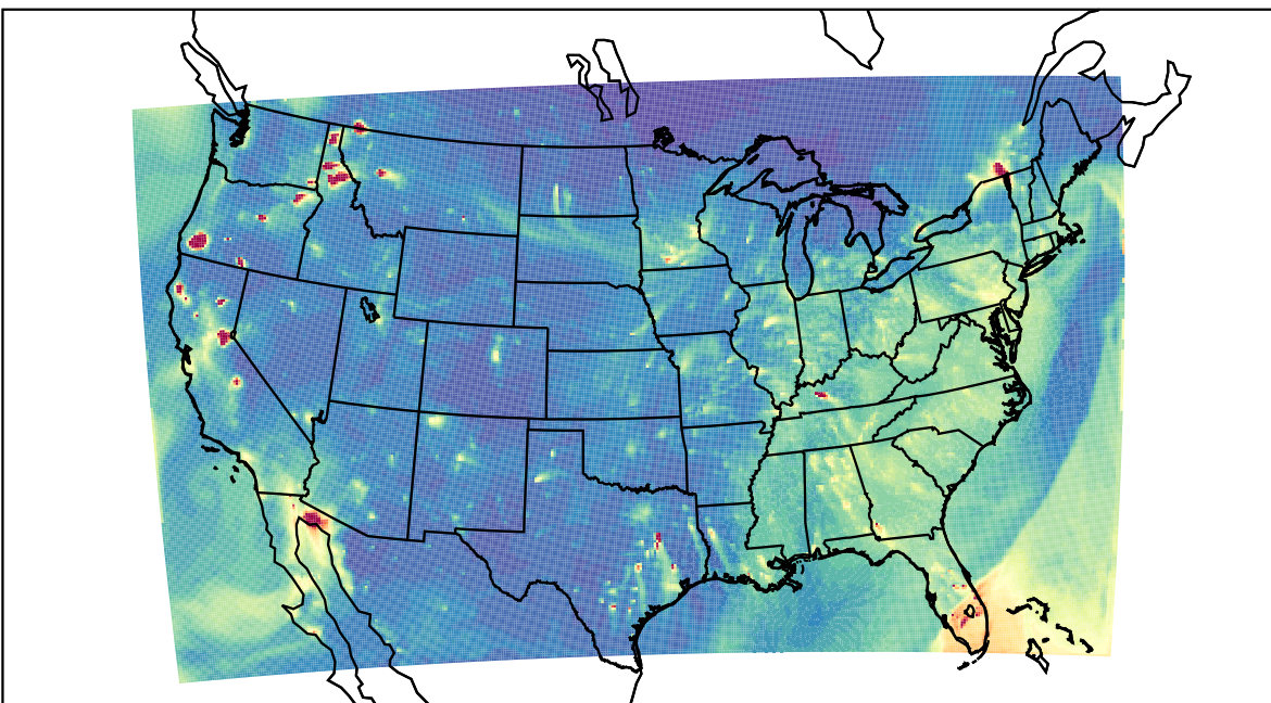
WRF 2023-11-23_01:00:00
