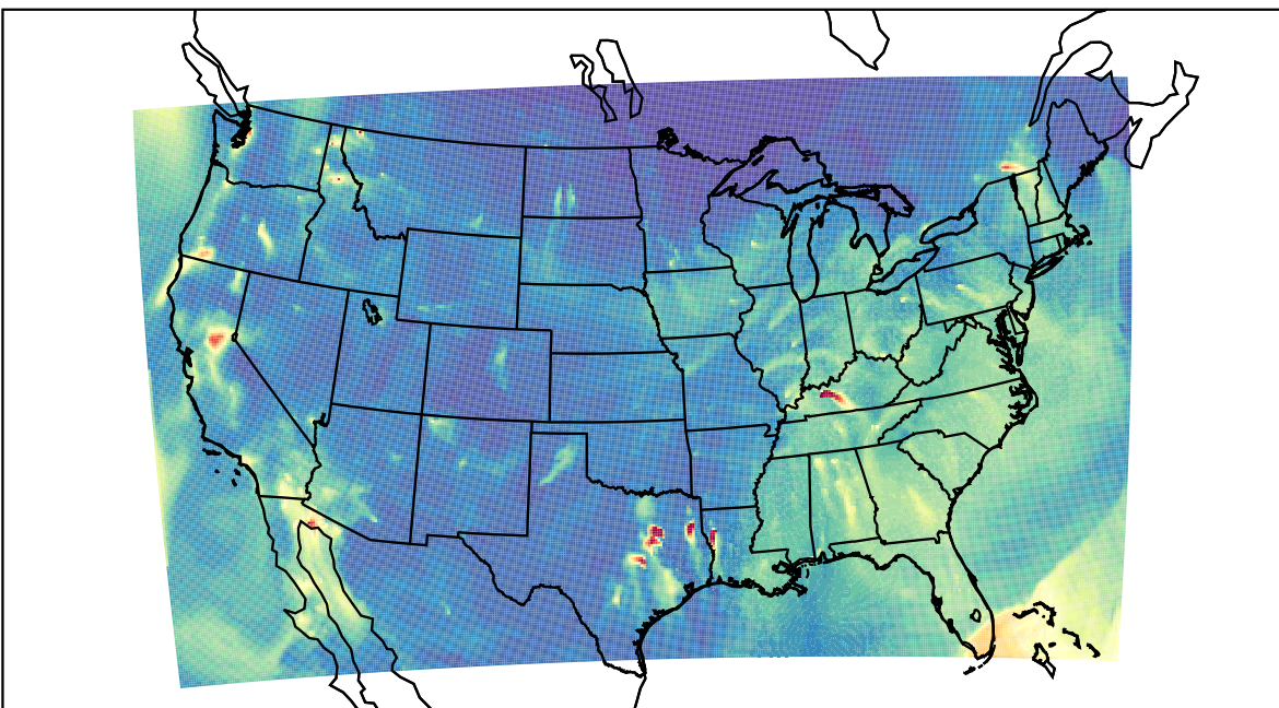
WRF 2023-11-23_08:00:00
