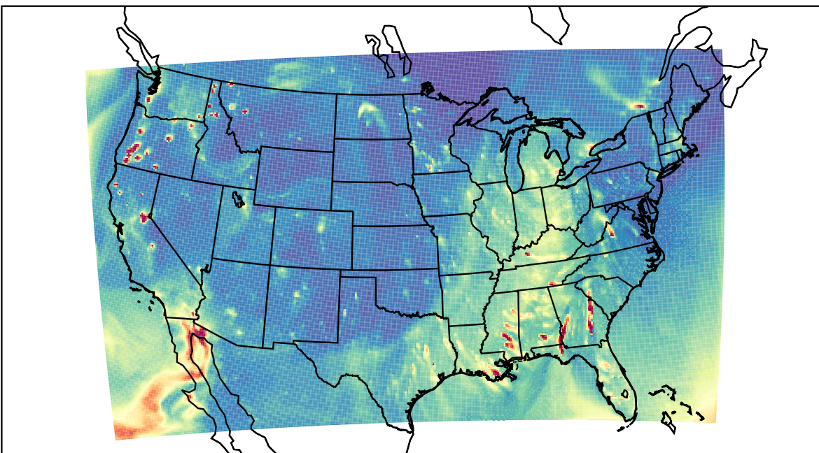
WRF 2023-11-22_01:00:00
