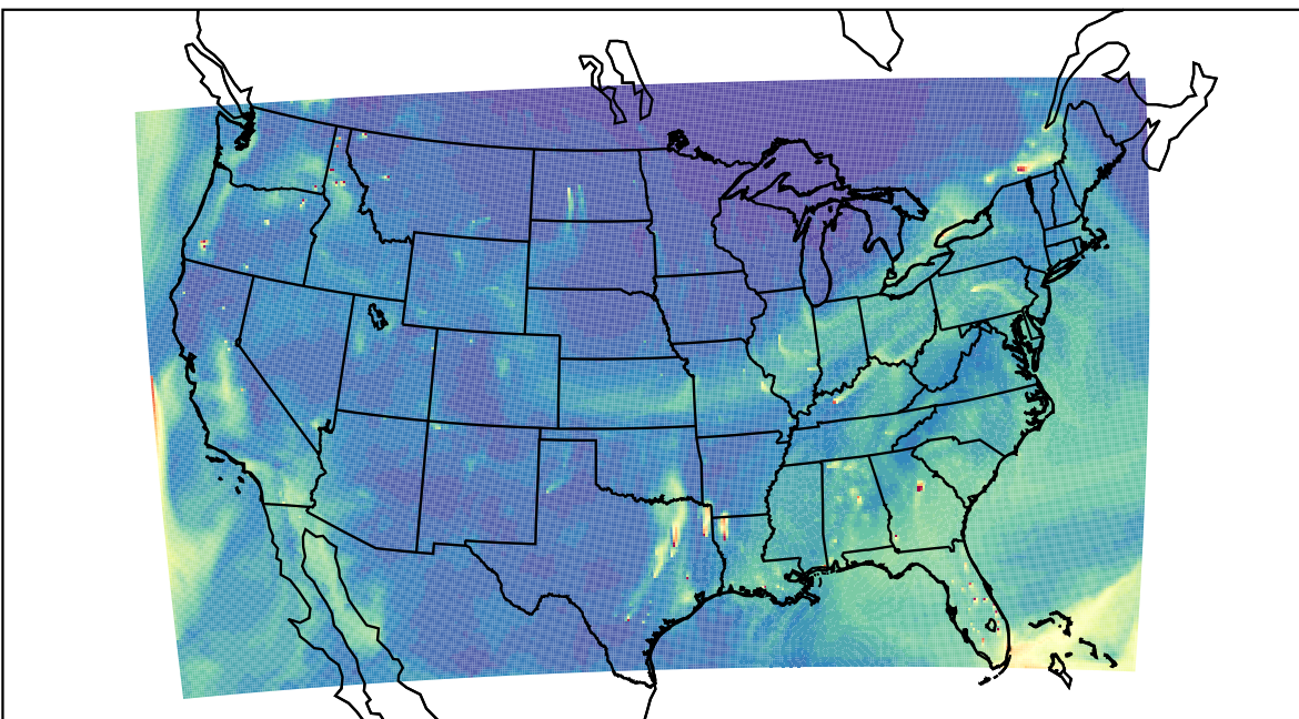
WRF 2023-11-23_20:00:00
