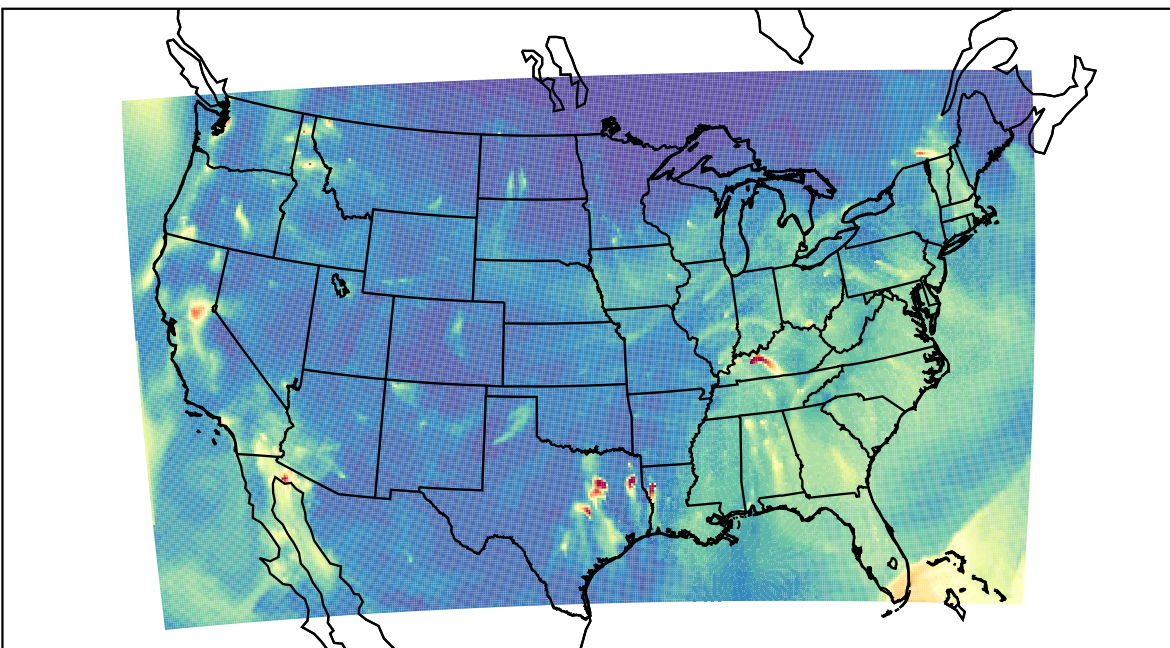
WRF 2023-11-23_09:00:00
