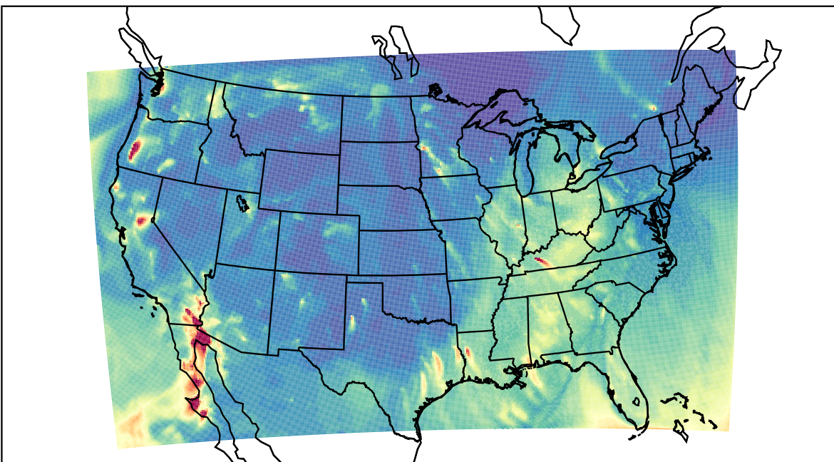
WRF 2023-11-22_06:00:00
