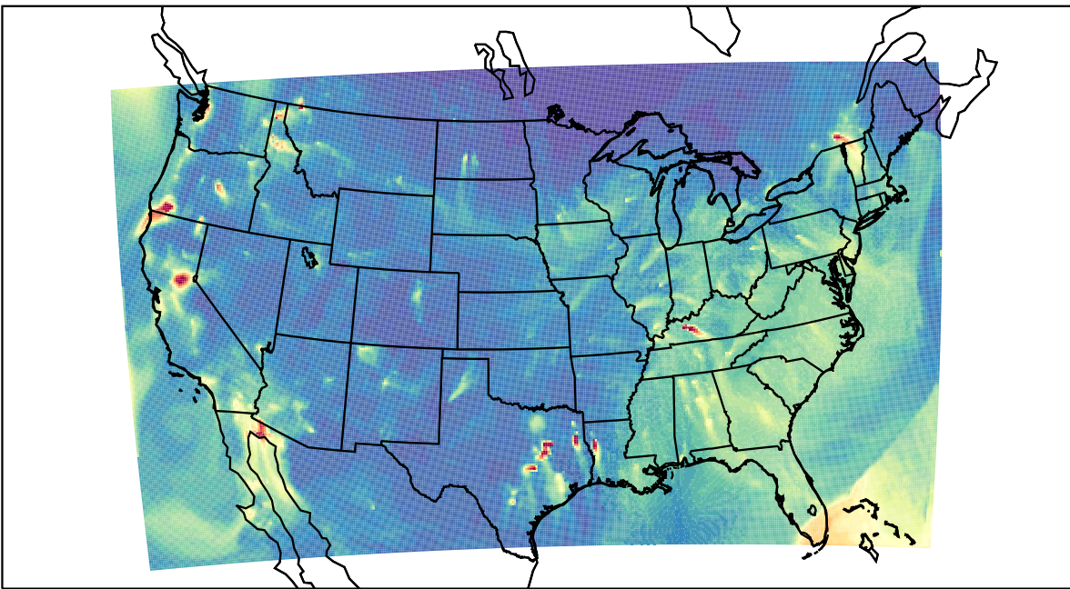
WRF 2023-11-23_06:00:00
