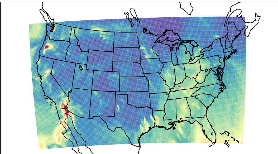
WRF 2023-11-22_09:00:00
