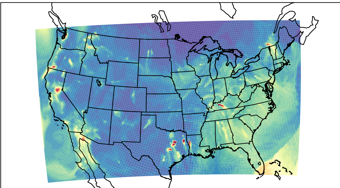
WRF 2023-11-23_07:00:00
