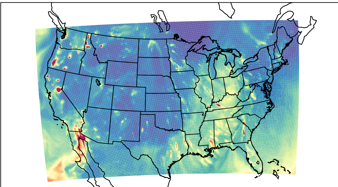
WRF 2023-11-22_03:00:00
