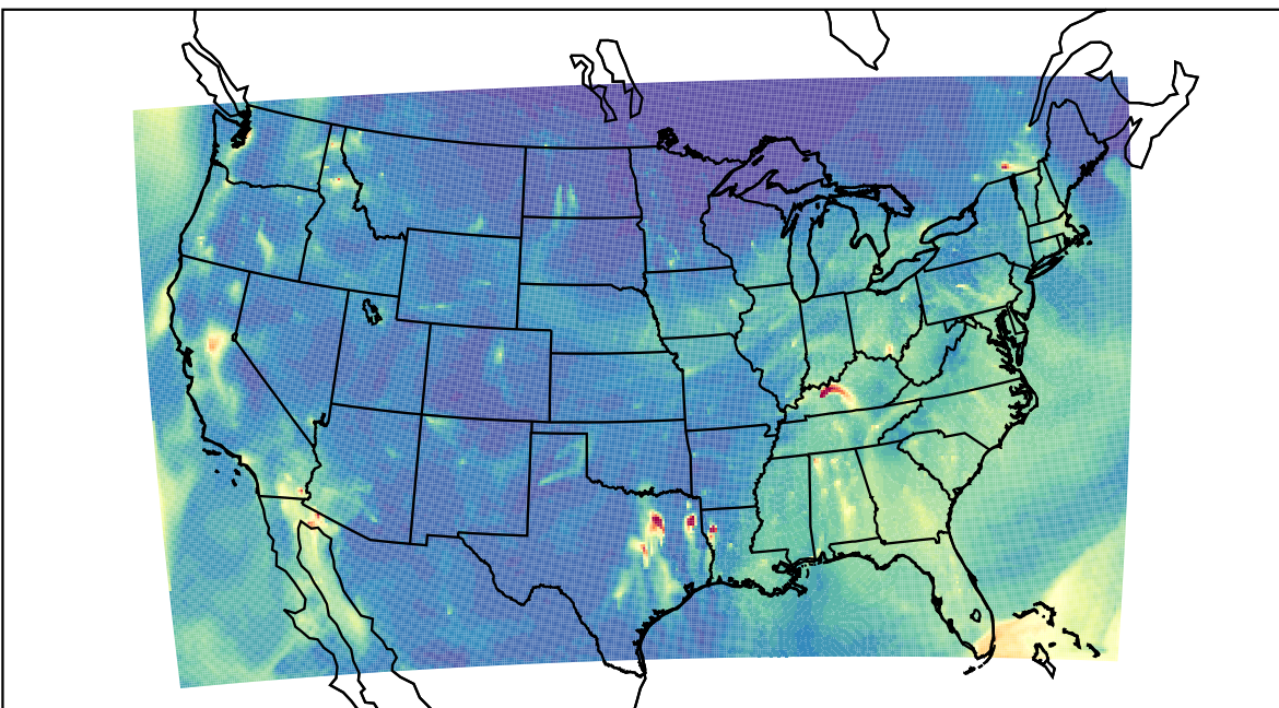
WRF 2023-11-23_11:00:00
