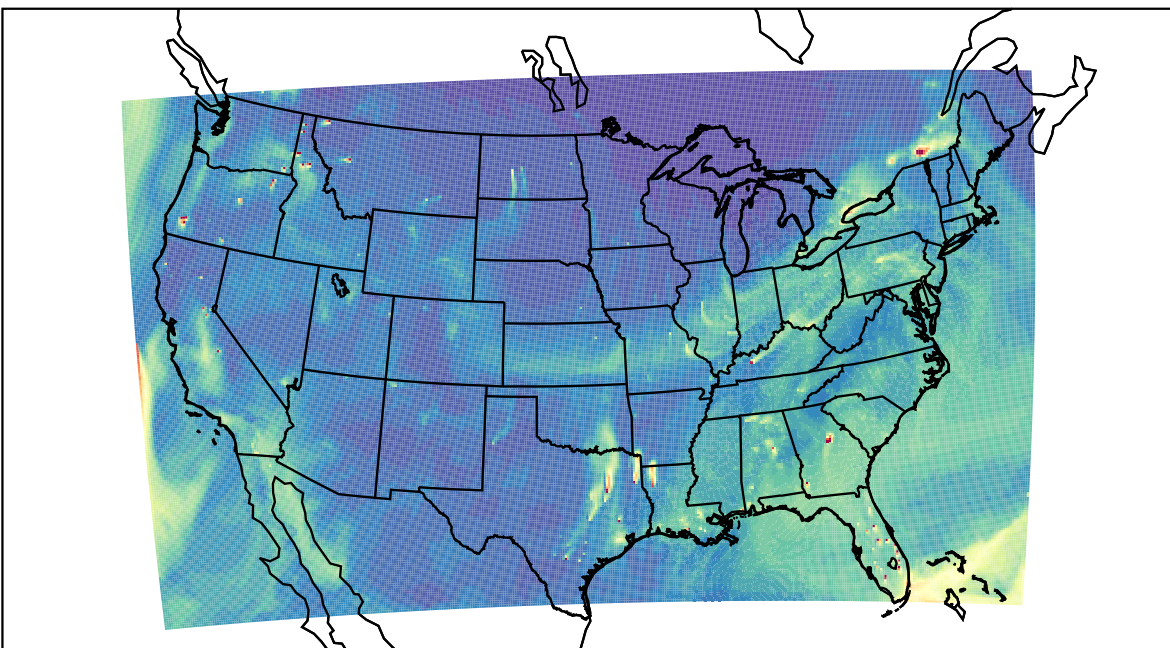
WRF 2023-11-23_21:00:00
