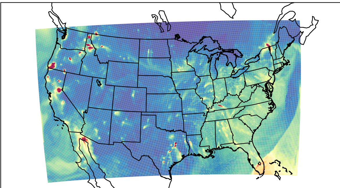
WRF 2023-11-23_03:00:00
