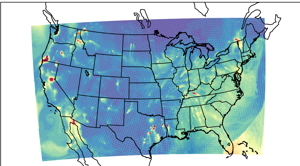
WRF 2023-11-23_05:00:00
