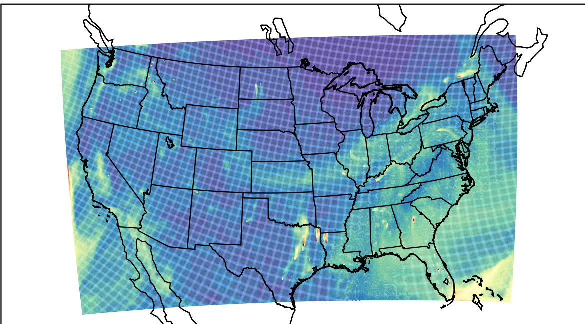
WRF 2023-11-23_19:00:00
