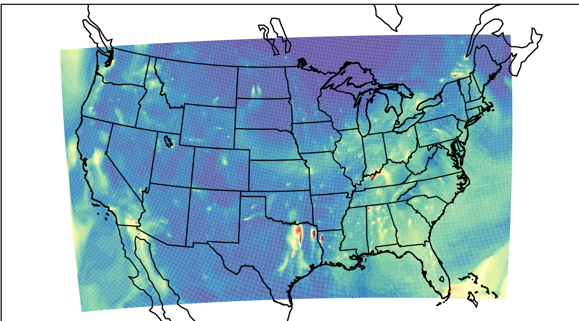
WRF 2023-11-23_14:00:00
