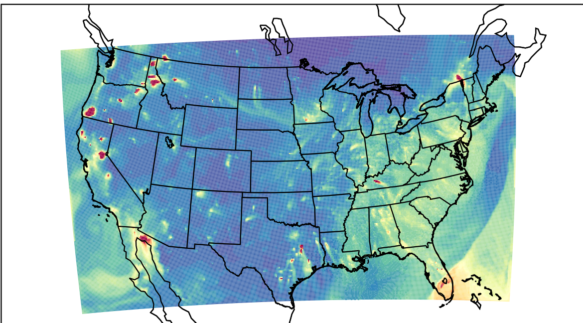
WRF 2023-11-23_02:00:00
