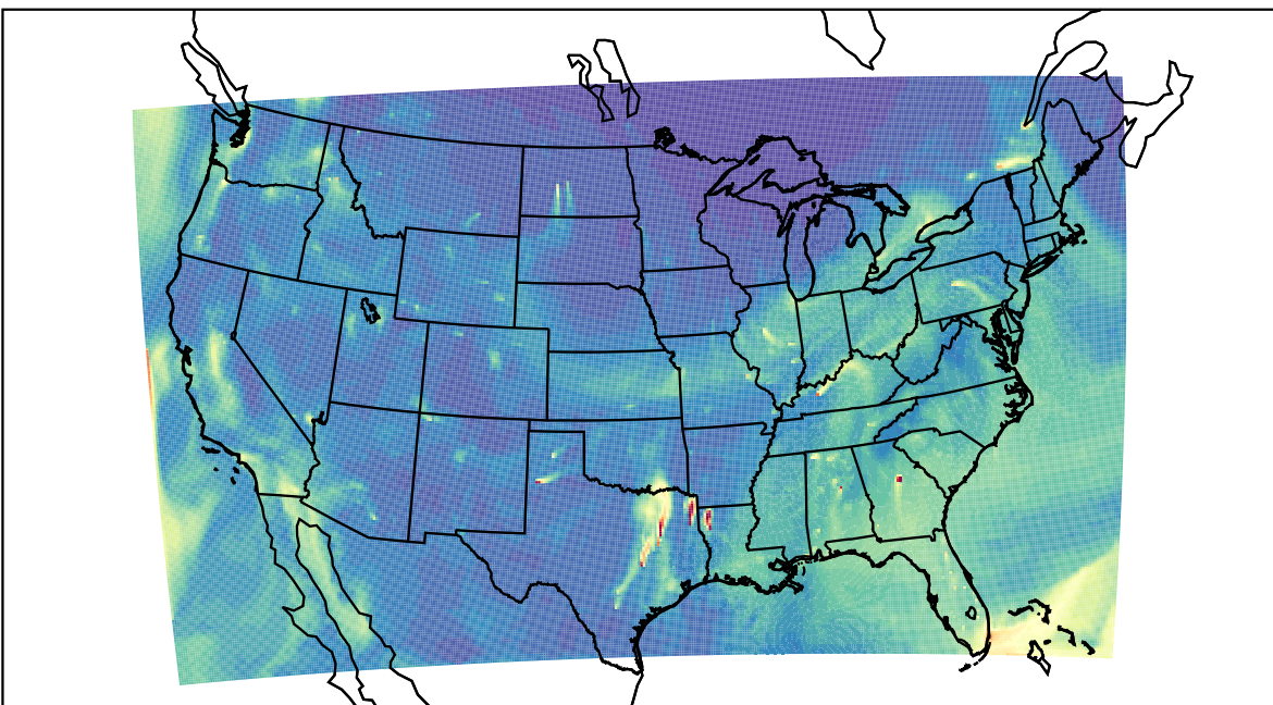
WRF 2023-11-23_17:00:00
