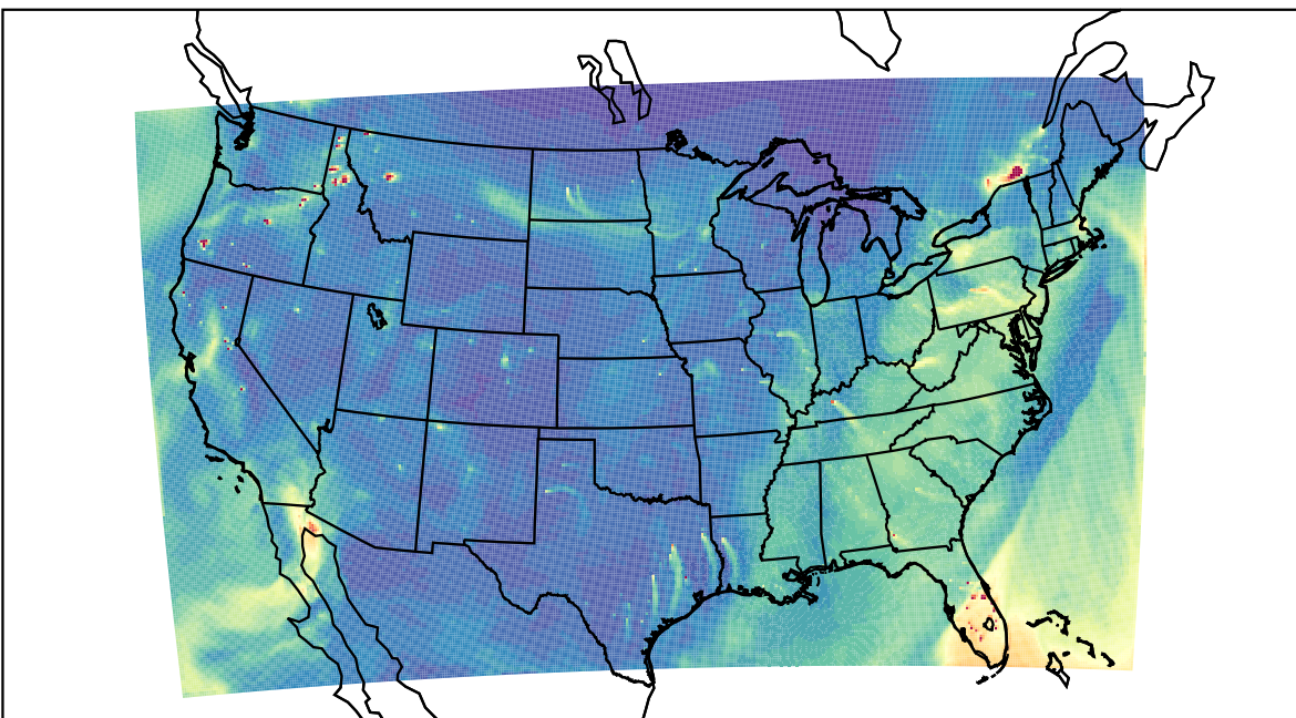
WRF 2023-11-22_21:00:00
