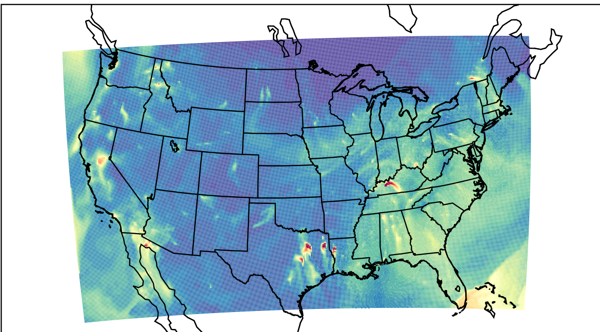
WRF 2023-11-23_10:00:00
