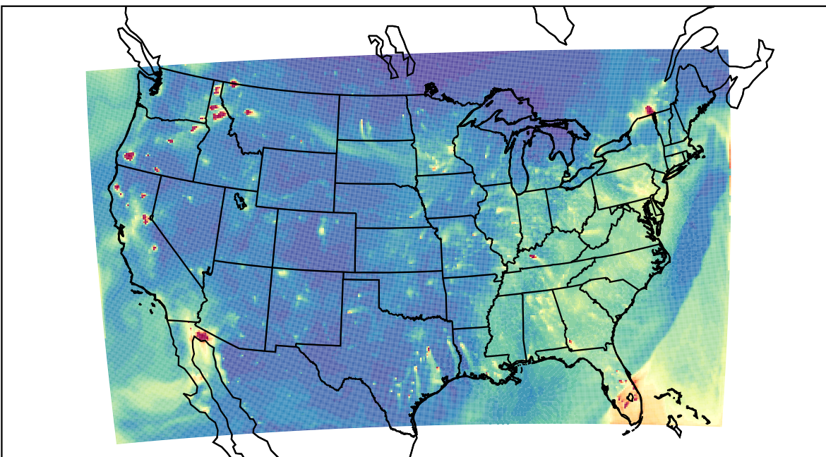
WRF 2023-11-23_00:00:00
