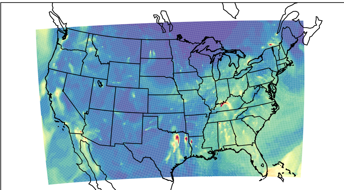
WRF 2023-11-23_13:00:00
