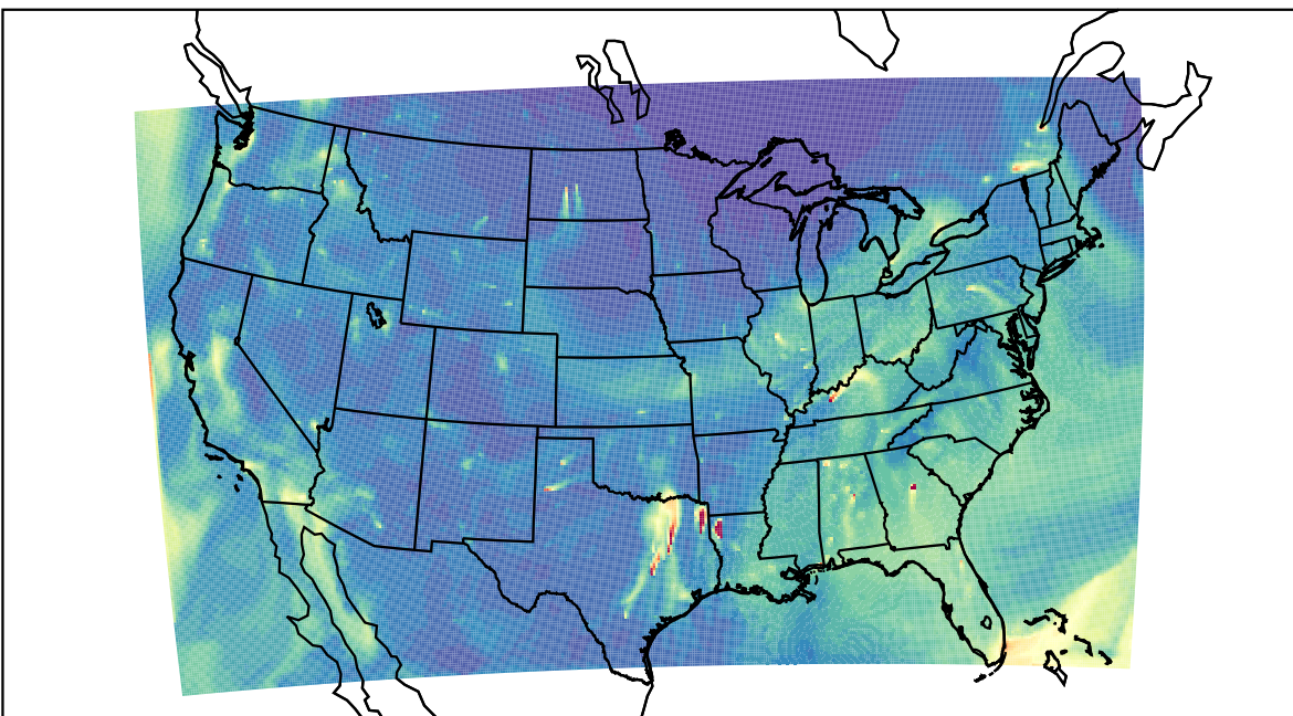
WRF 2023-11-23_16:00:00
