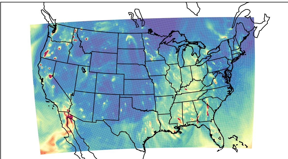
WRF 2023-11-22_02:00:00
