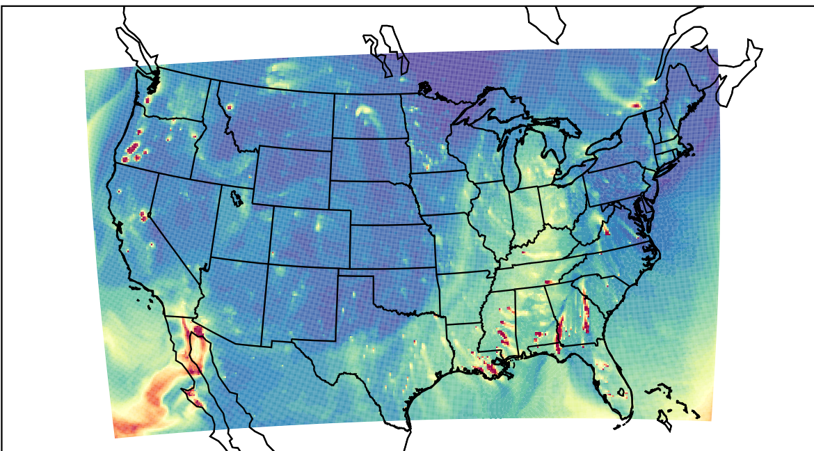
WRF 2023-11-22_00:00:00
