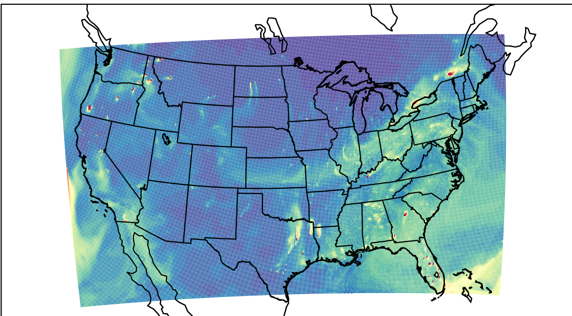
WRF 2023-11-23_22:00:00
