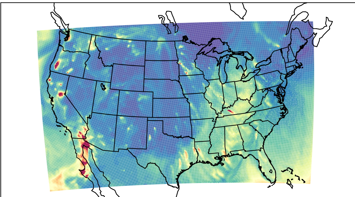
WRF 2023-11-22_05:00:00
