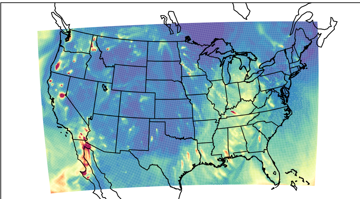
WRF 2023-11-22_04:00:00
