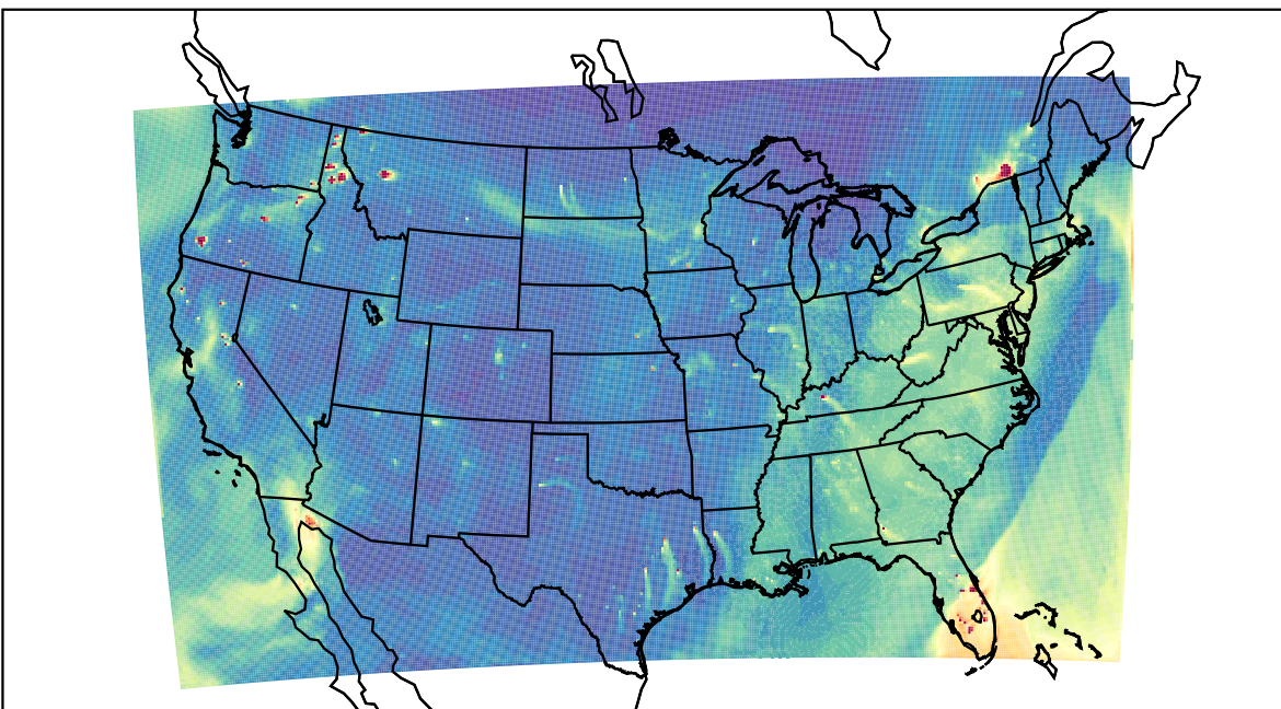
WRF 2023-11-22_22:00:00
