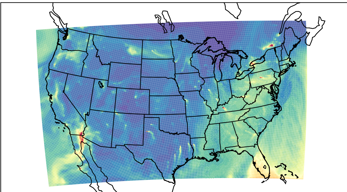
WRF 2023-11-22_17:00:00
