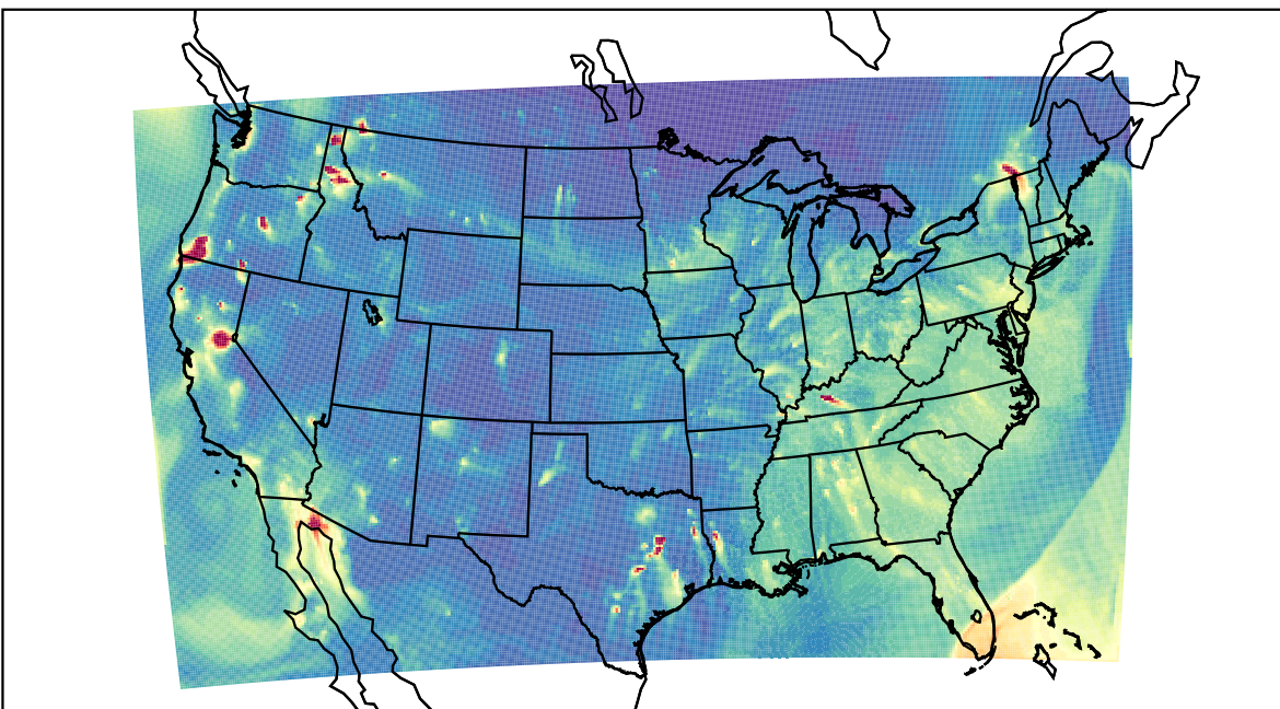
WRF 2023-11-23_04:00:00
