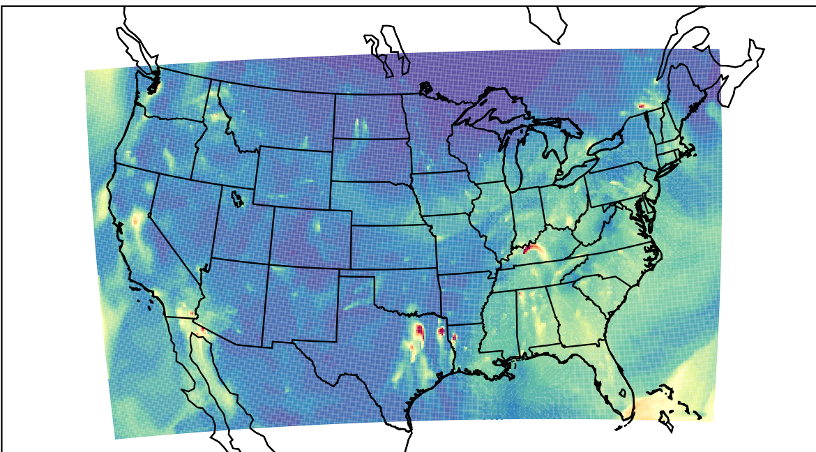
WRF 2023-11-23_12:00:00
