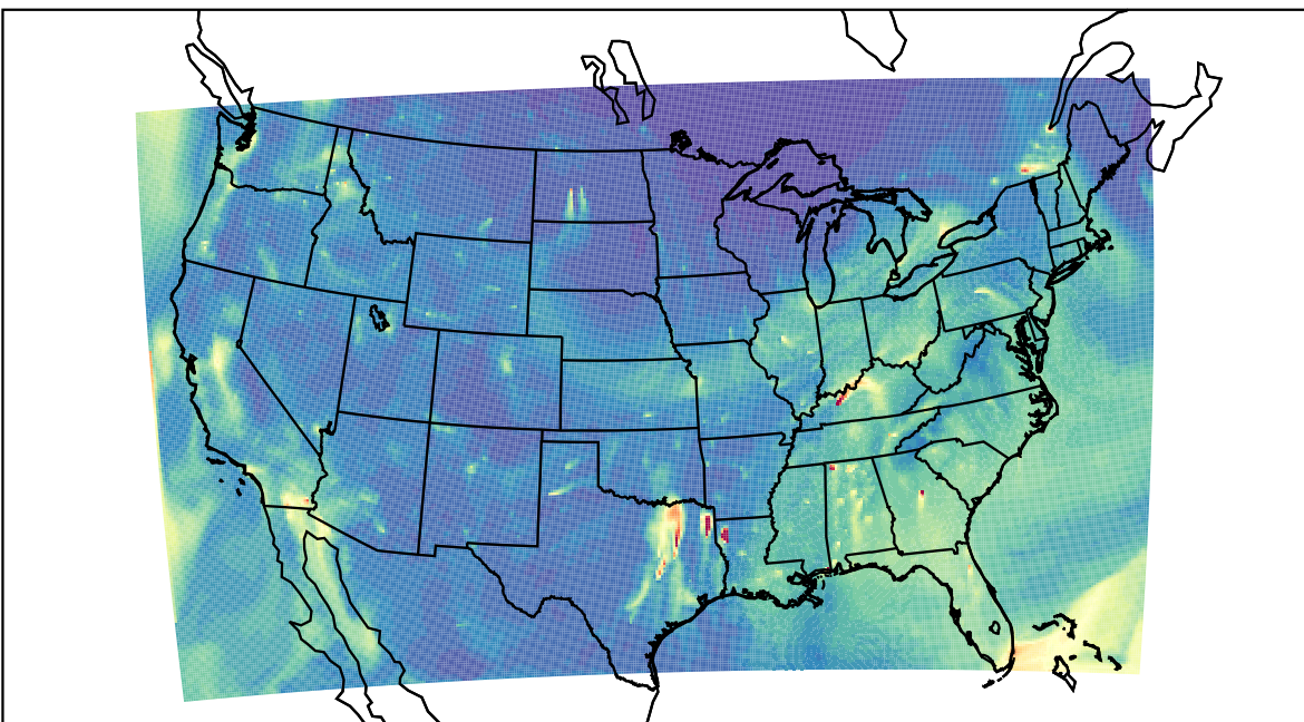
WRF 2023-11-23_15:00:00
