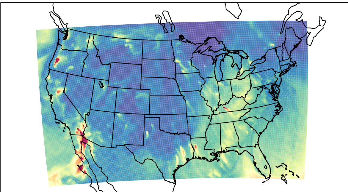
WRF 2023-11-22_07:00:00
