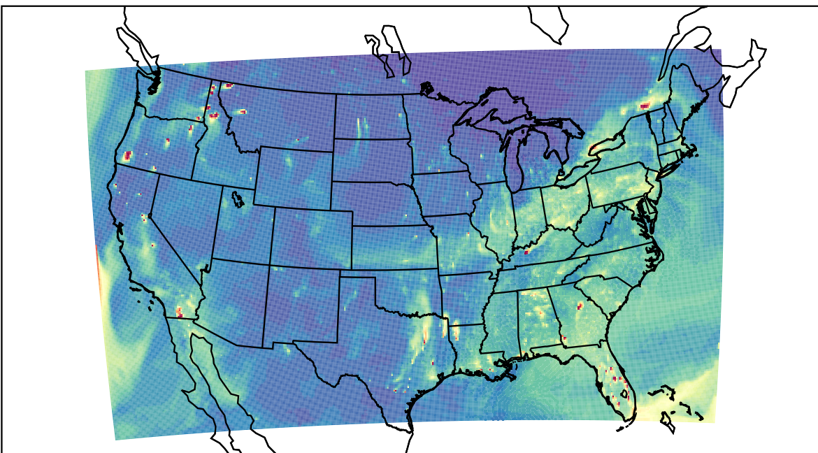
WRF 2023-11-23_23:00:00
