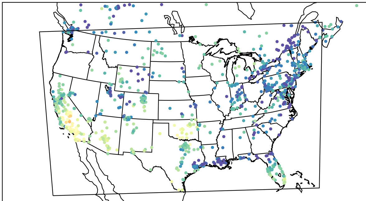
AirNOW (2023-11-23_22:00:00)
