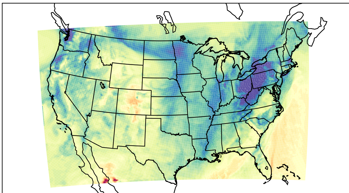
WRF (2023-11-22_19:00:00)
