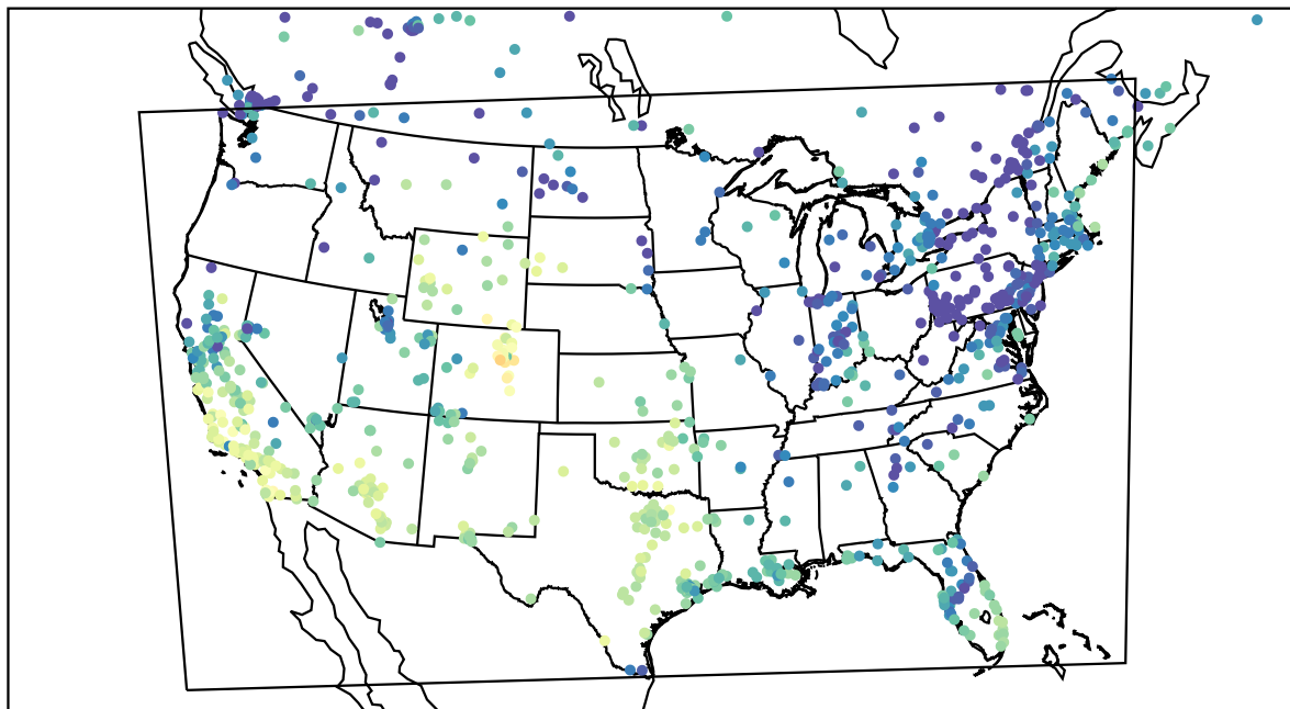
AirNOW (2023-11-22_21:00:00)
