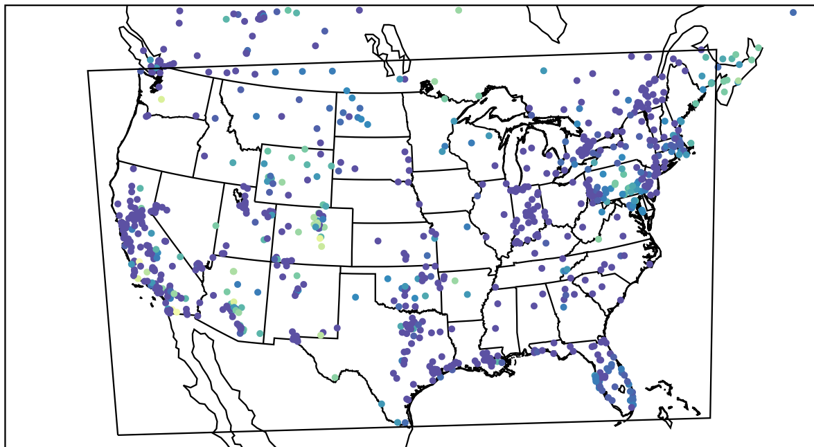
AirNOW (2023-11-23_09:00:00)
