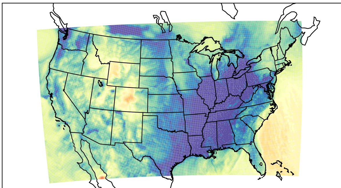
WRF (2023-11-22_11:00:00)
