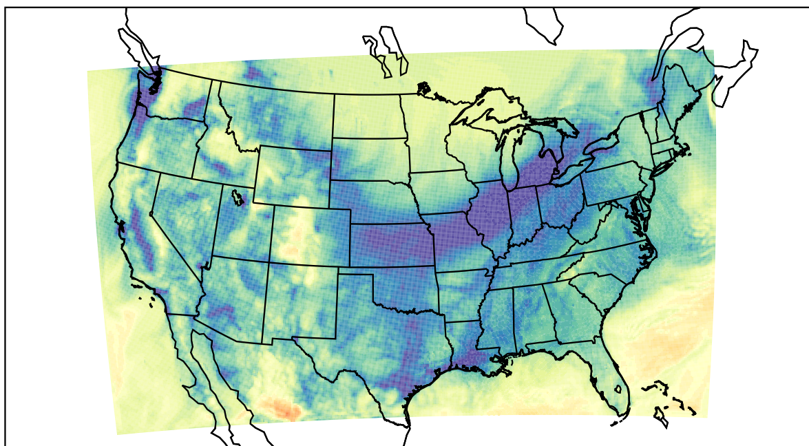
WRF (2023-11-23_16:00:00)
