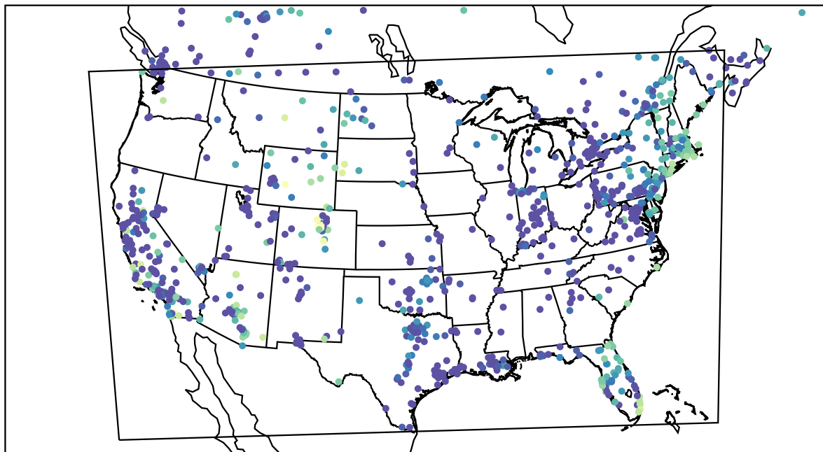
AirNOW (2023-11-22_09:00:00)
