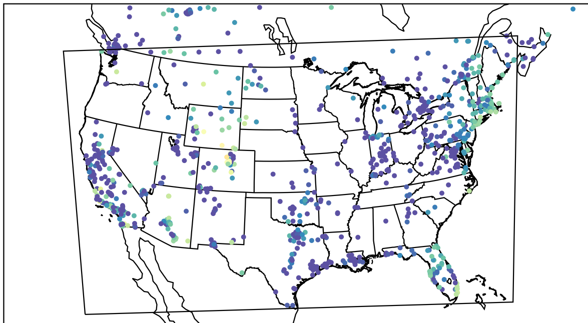
AirNOW (2023-11-22_08:00:00)
