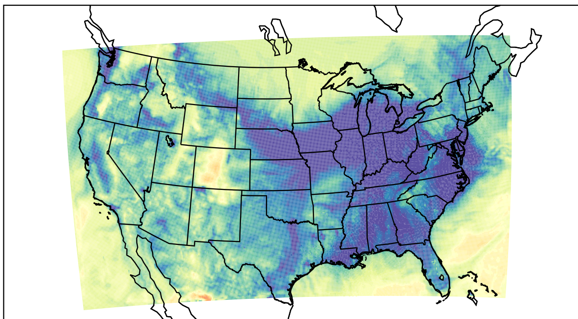
WRF (2023-11-23_10:00:00)
