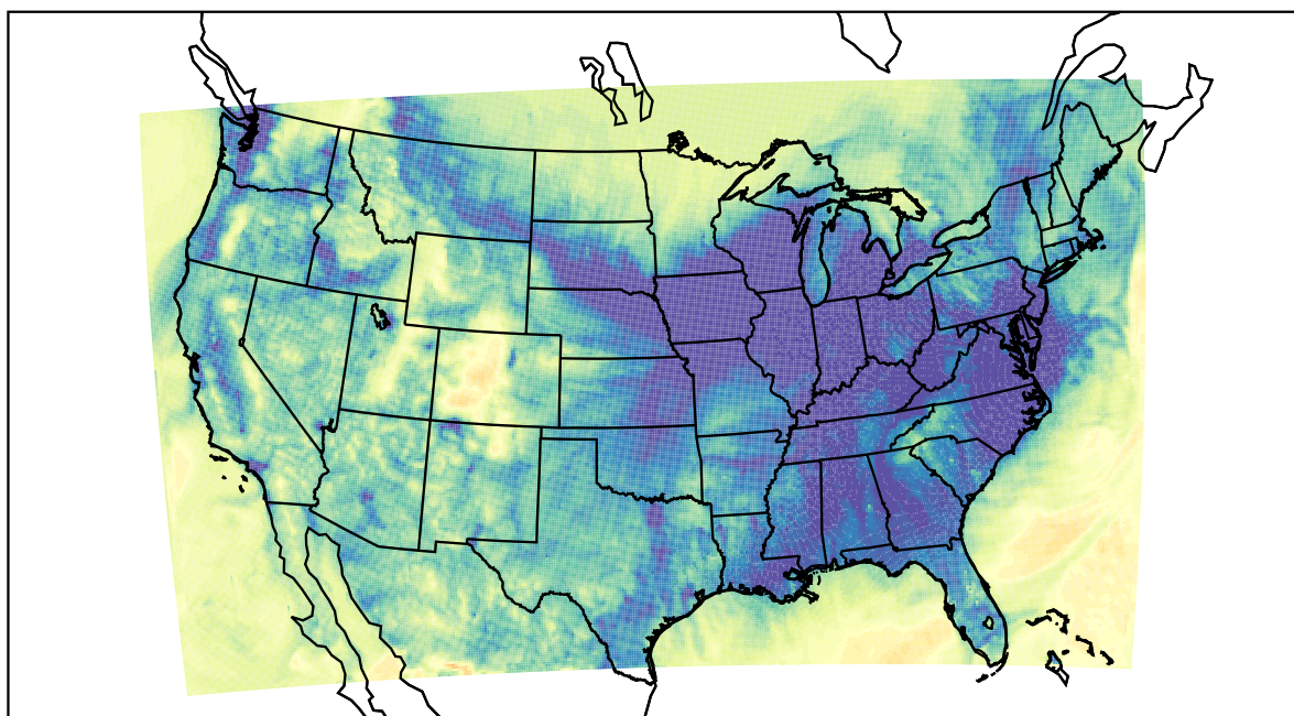
WRF (2023-11-23_07:00:00)
