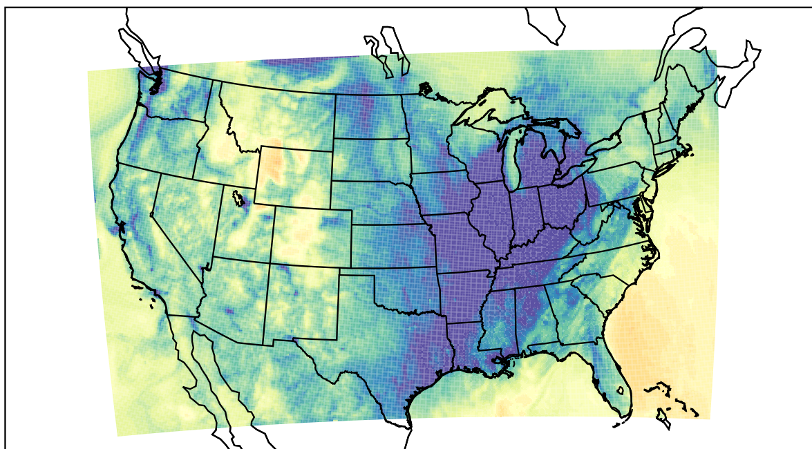
WRF (2023-11-22_05:00:00)
