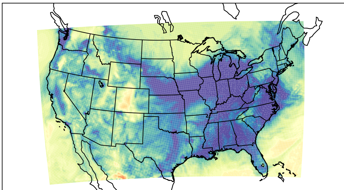
WRF (2023-11-23_11:00:00)
