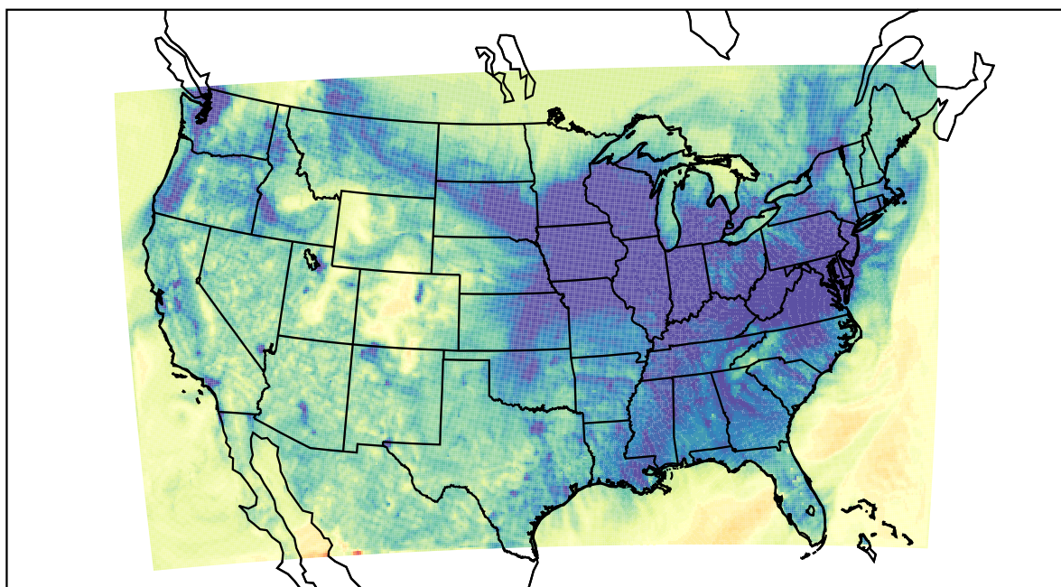
WRF (2023-11-23_03:00:00)
