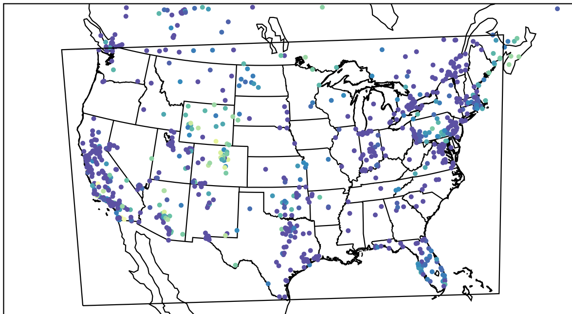
AirNOW (2023-11-23_07:00:00)
