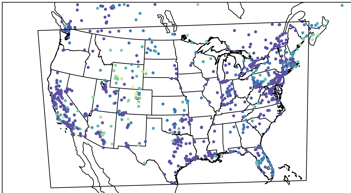
AirNOW (2023-11-23_04:00:00)
