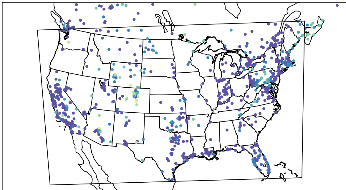
AirNOW (2023-11-23_08:00:00)
