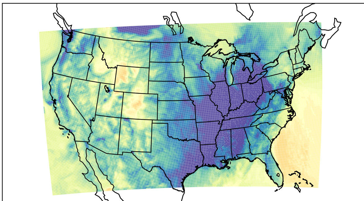
WRF (2023-11-22_08:00:00)
