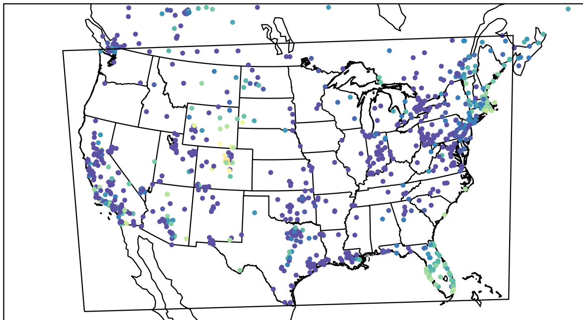
AirNOW (2023-11-22_14:00:00)
