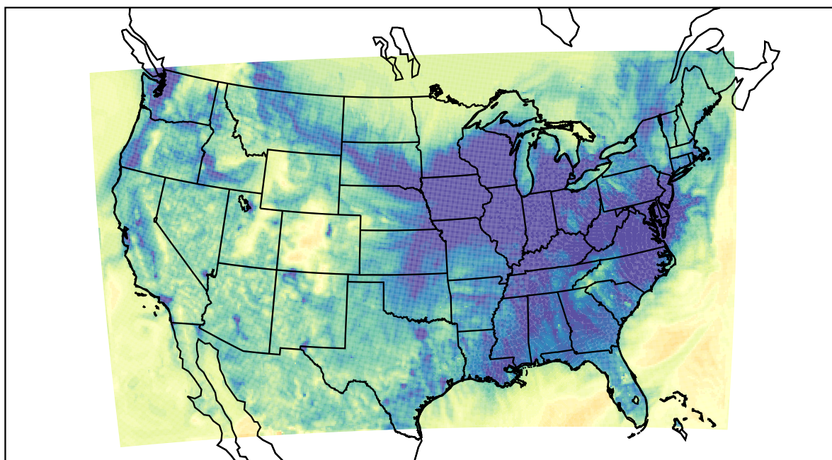
WRF (2023-11-23_05:00:00)
