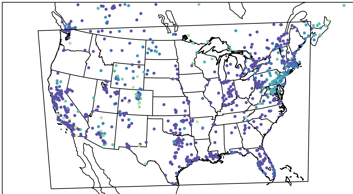
AirNOW (2023-11-23_13:00:00)
