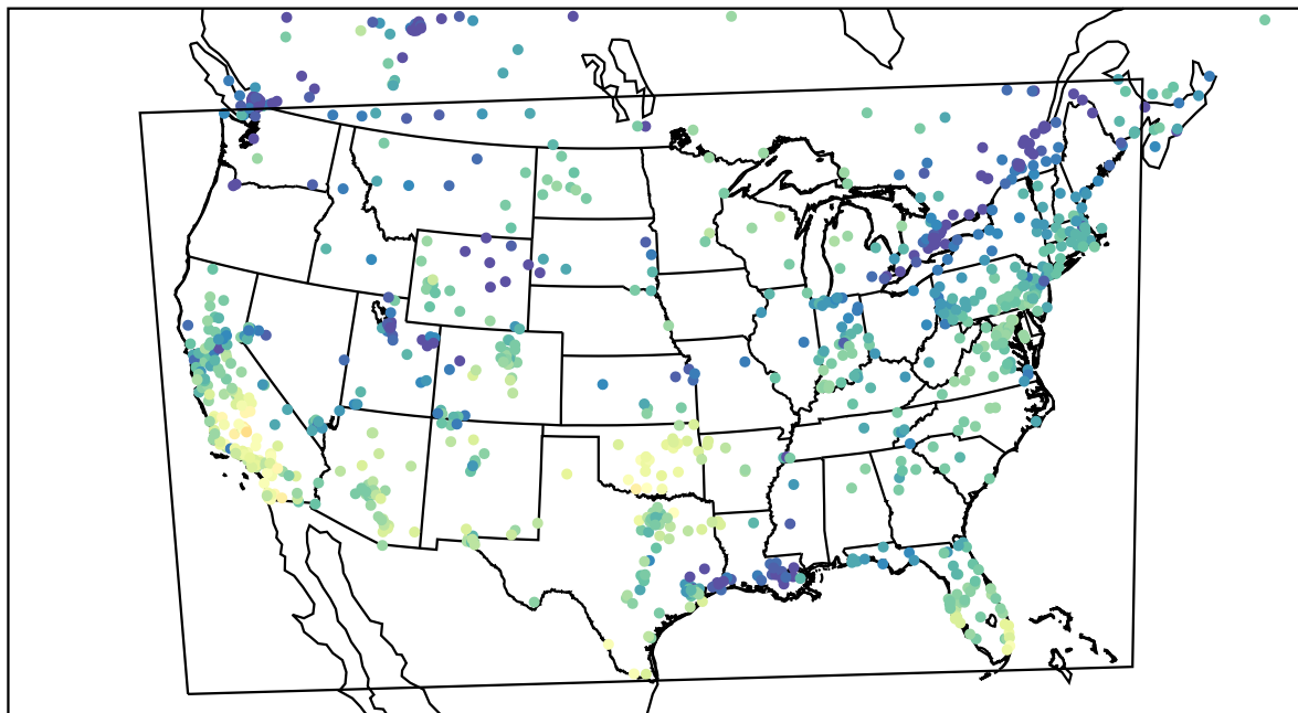
AirNOW (2023-11-23_20:00:00)
