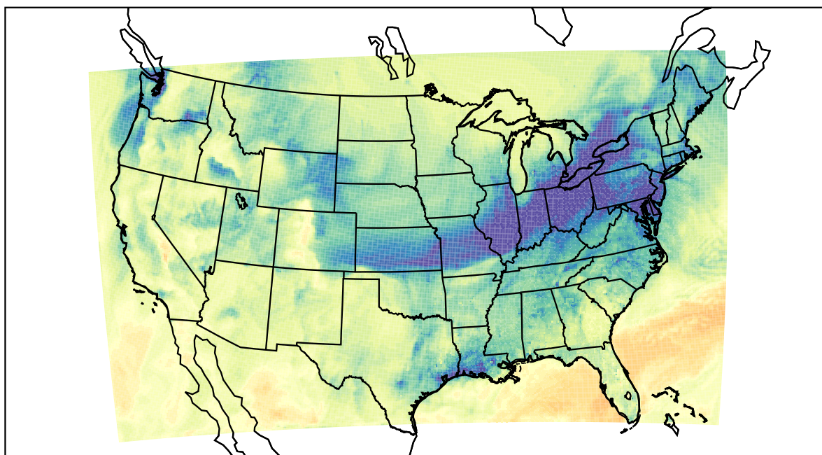
WRF (2023-11-23_22:00:00)
