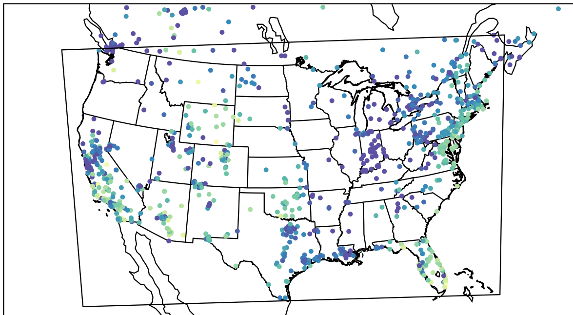
AirNOW (2023-11-22_00:00:00)
