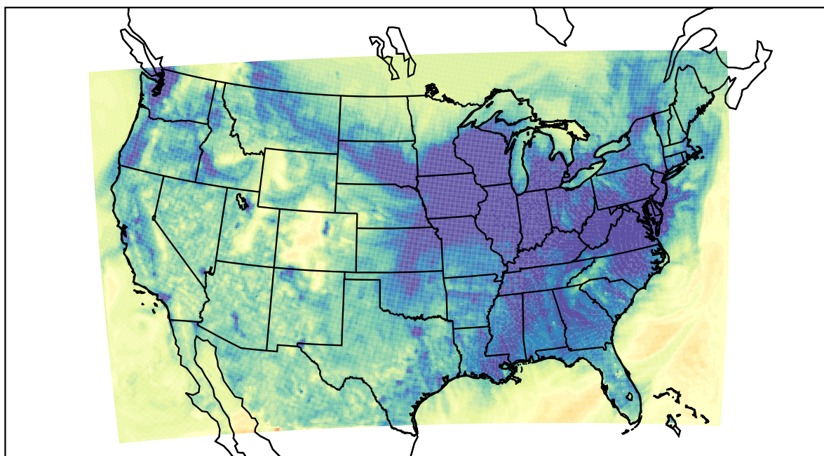
WRF (2023-11-23_04:00:00)
