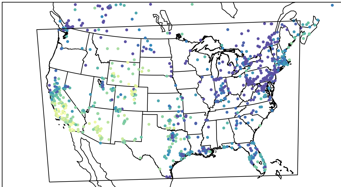
AirNOW (2023-11-22_23:00:00)
