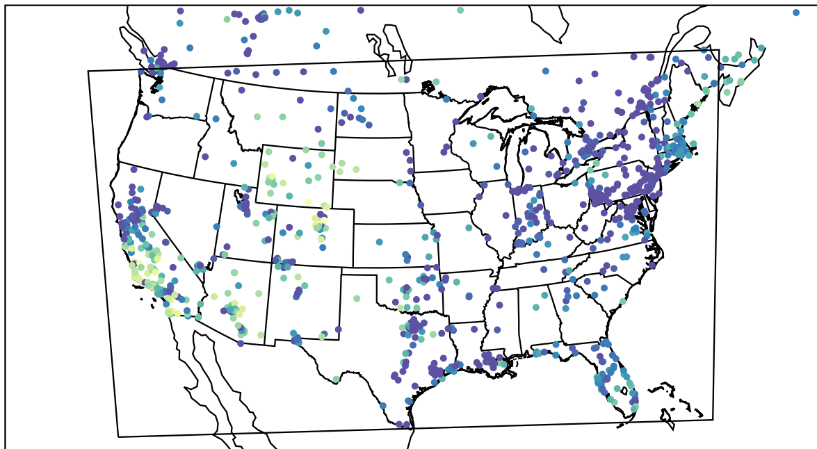
AirNOW (2023-11-23_00:00:00)
