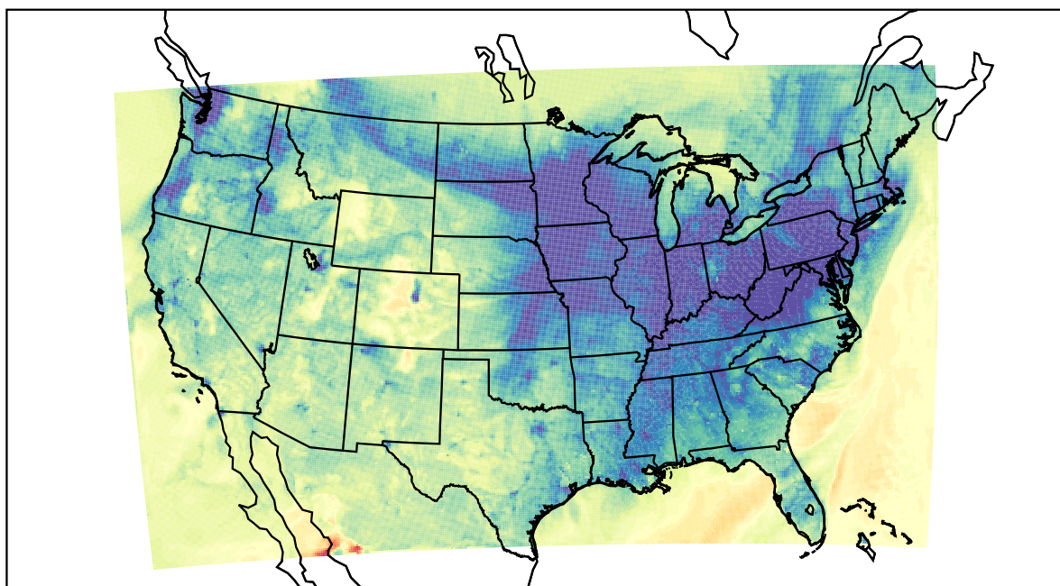
WRF (2023-11-23_00:00:00)
