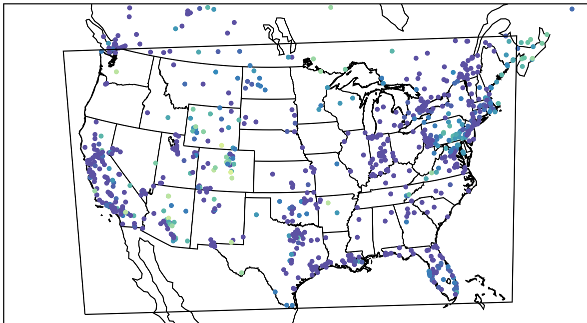
AirNOW (2023-11-23_10:00:00)
