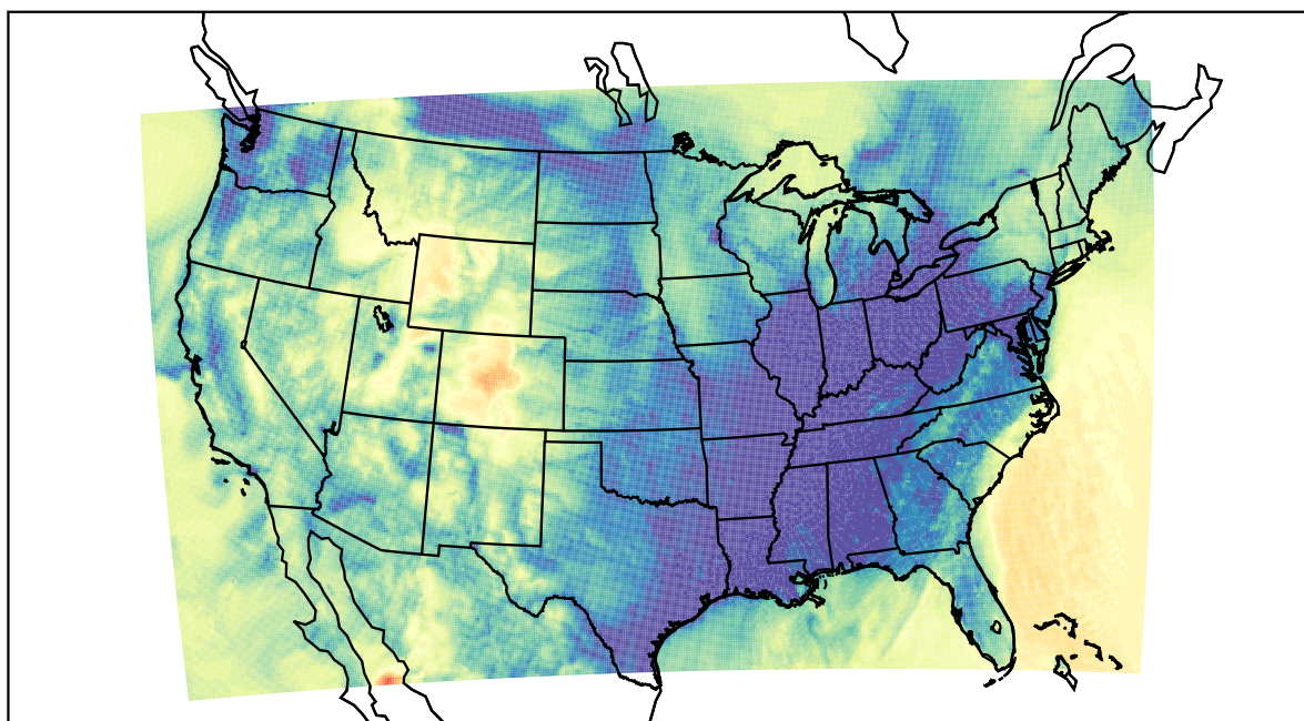
WRF (2023-11-22_12:00:00)
