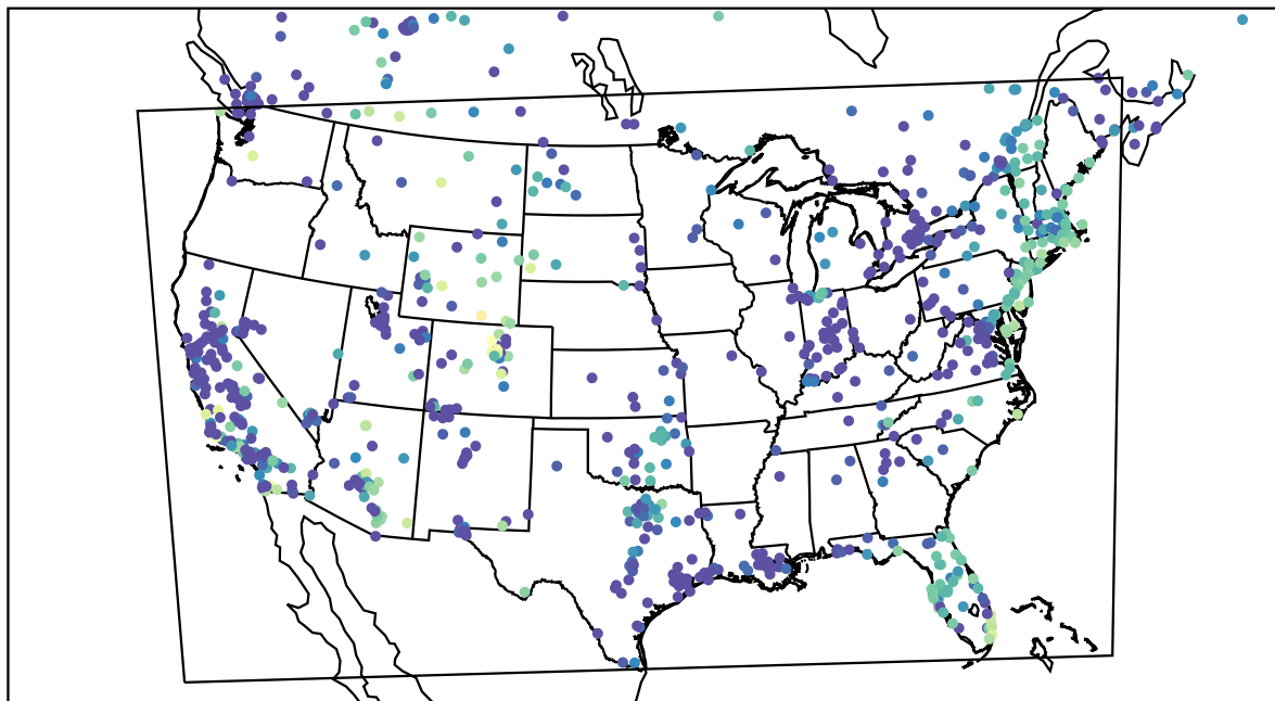
AirNOW (2023-11-22_06:00:00)
