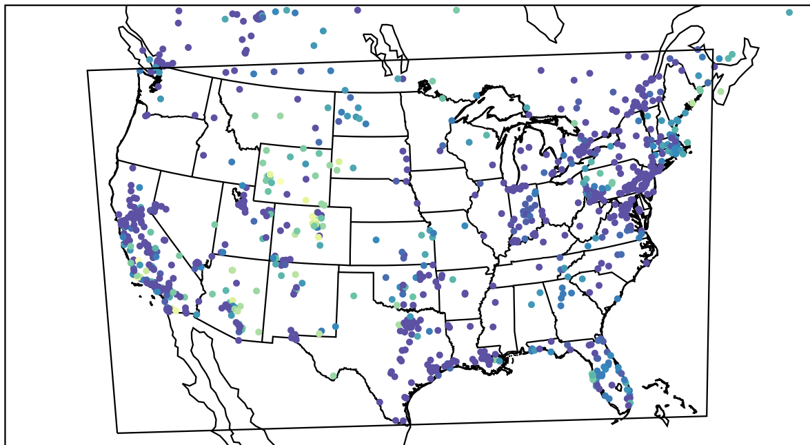
AirNOW (2023-11-23_03:00:00)
