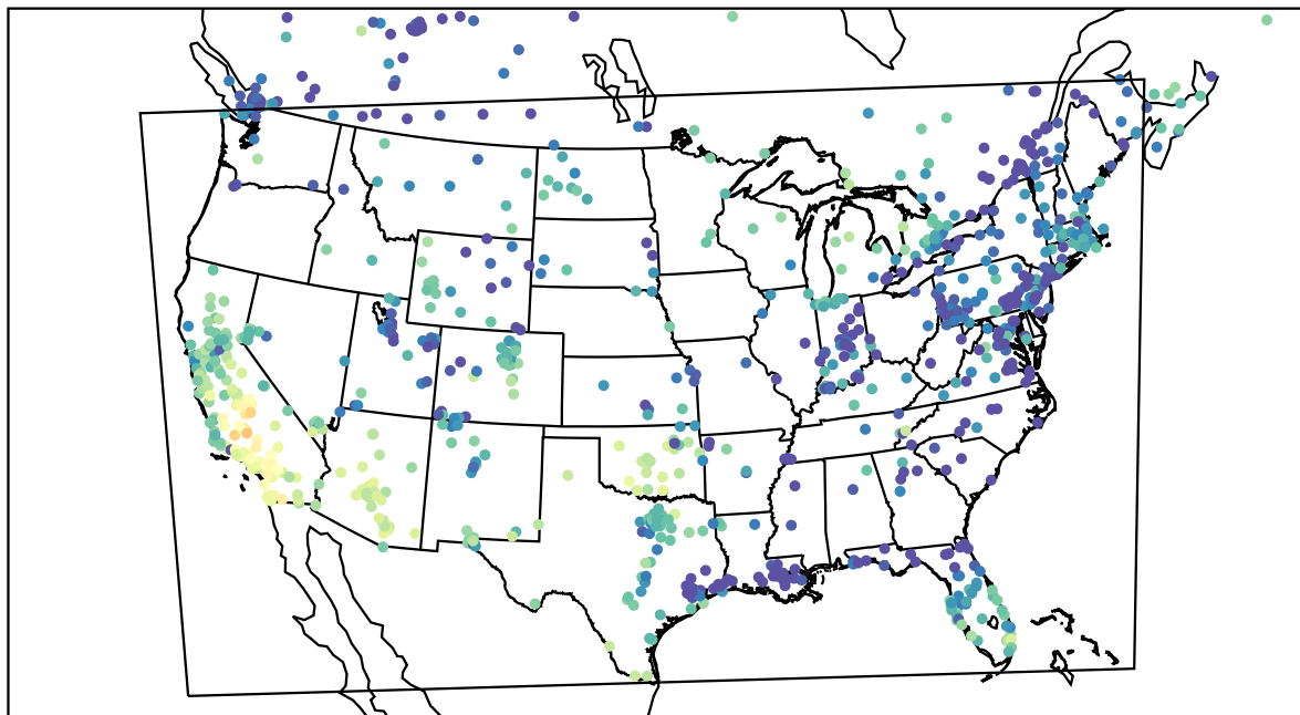
AirNOW (2023-11-23_23:00:00)
