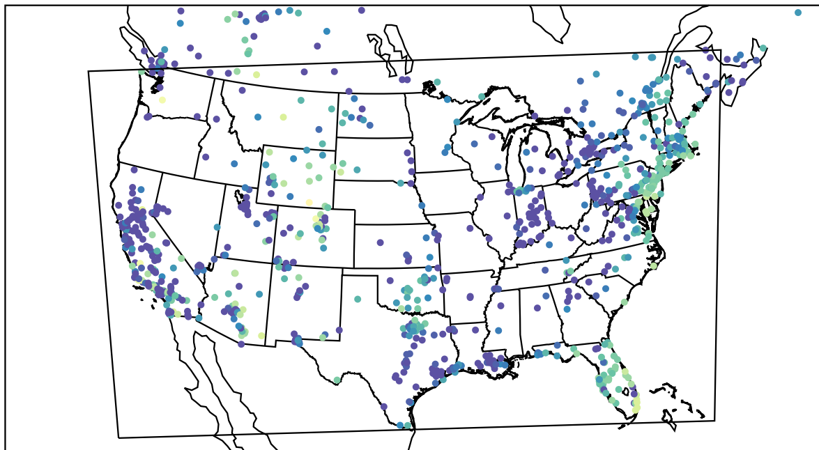
AirNOW (2023-11-22_03:00:00)
