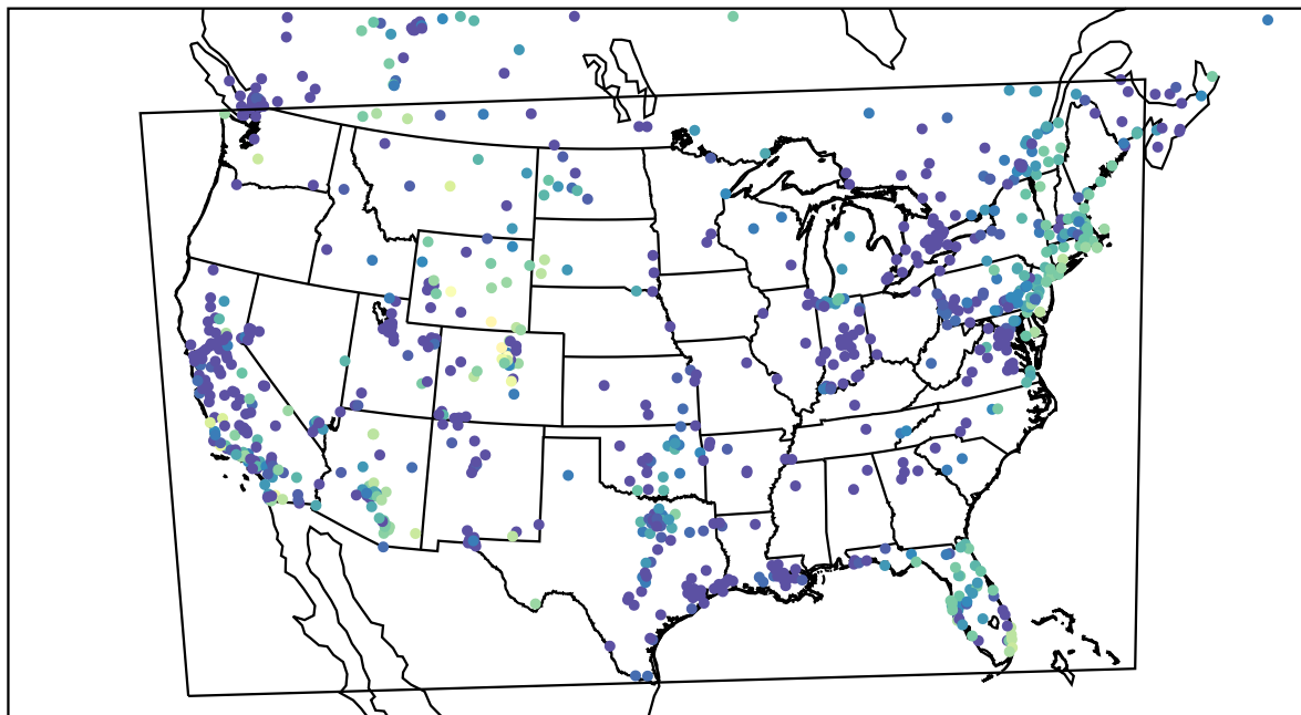
AirNOW (2023-11-22_07:00:00)
