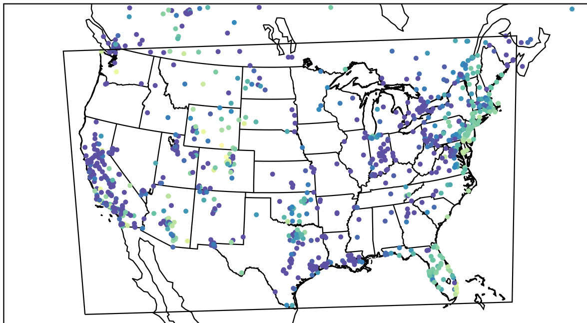
AirNOW (2023-11-22_04:00:00)
