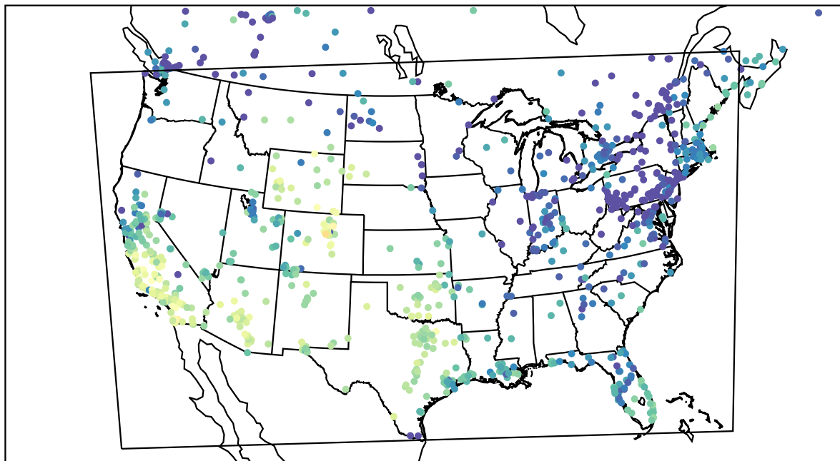
AirNOW (2023-11-22_22:00:00)
