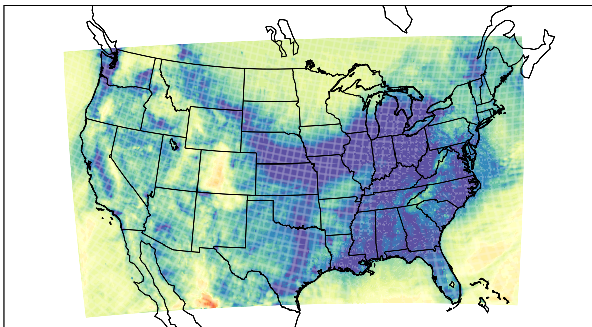
WRF (2023-11-23_13:00:00)
