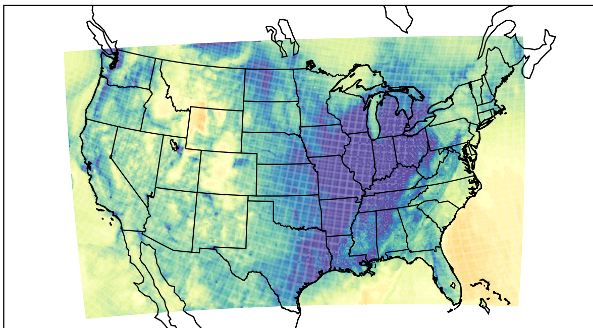
WRF (2023-11-22_04:00:00)
