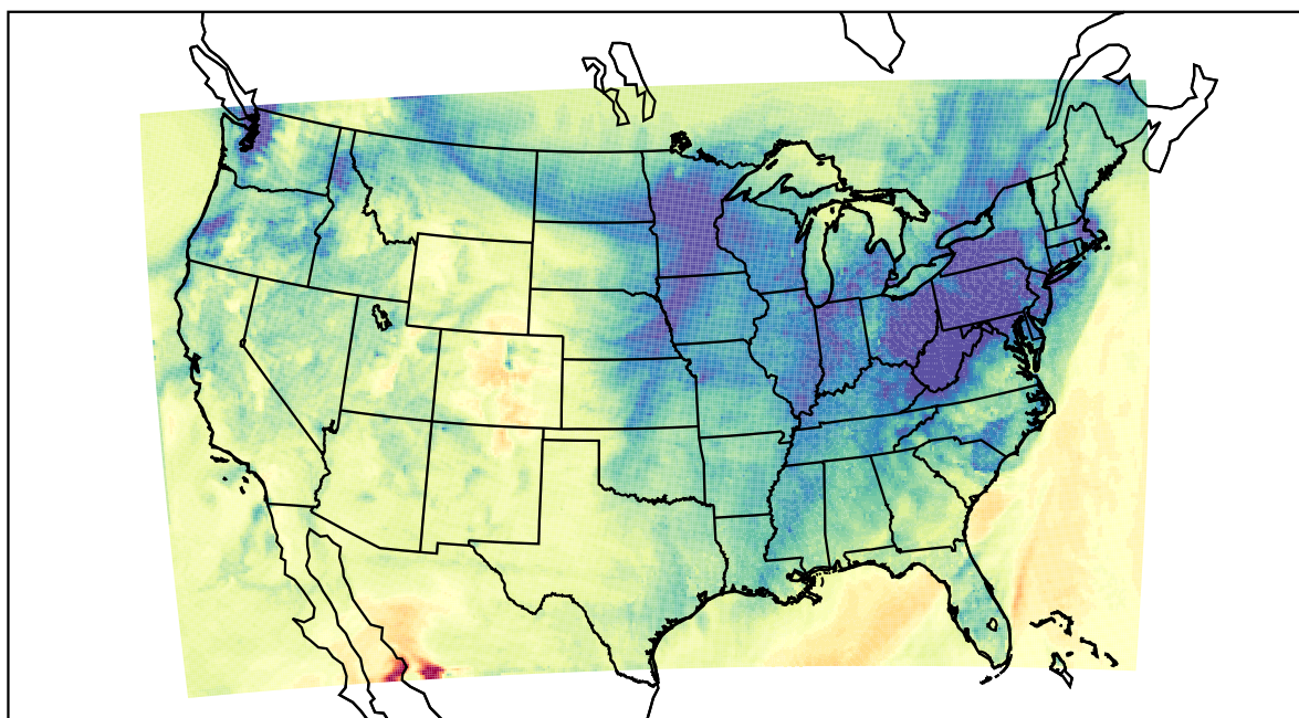
WRF (2023-11-22_22:00:00)
