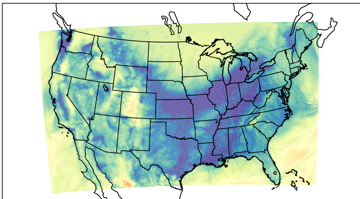
WRF (2023-11-23_15:00:00)
