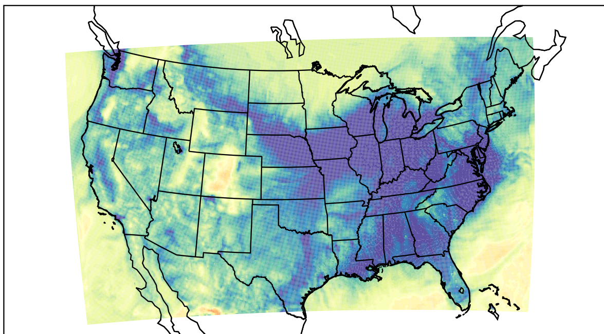
WRF (2023-11-23_09:00:00)
