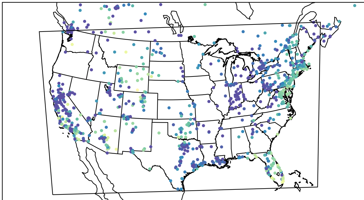
AirNOW (2023-11-22_01:00:00)
