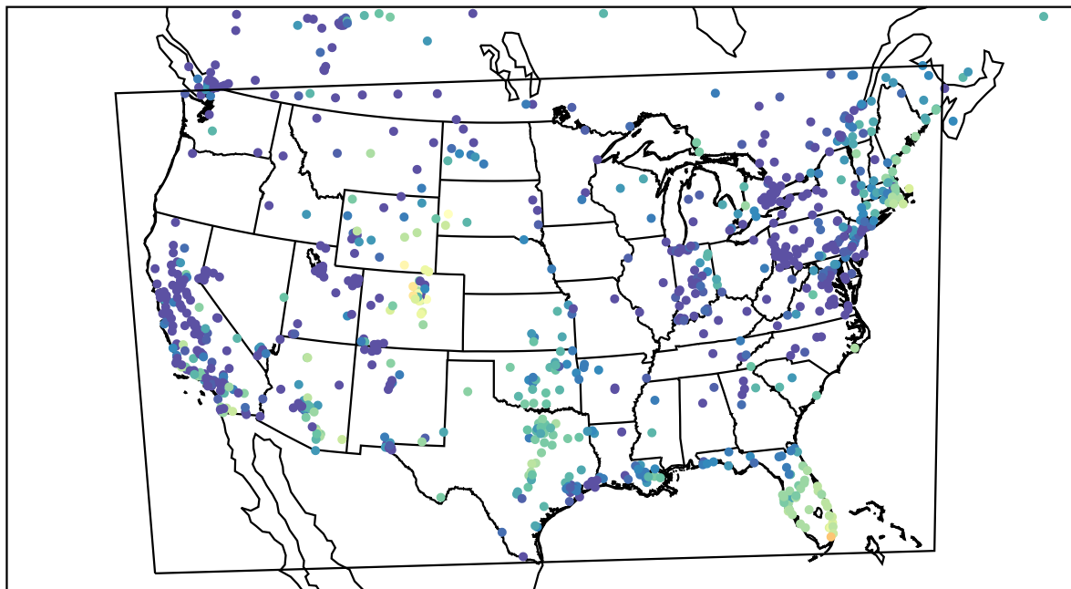
AirNOW (2023-11-22_16:00:00)
