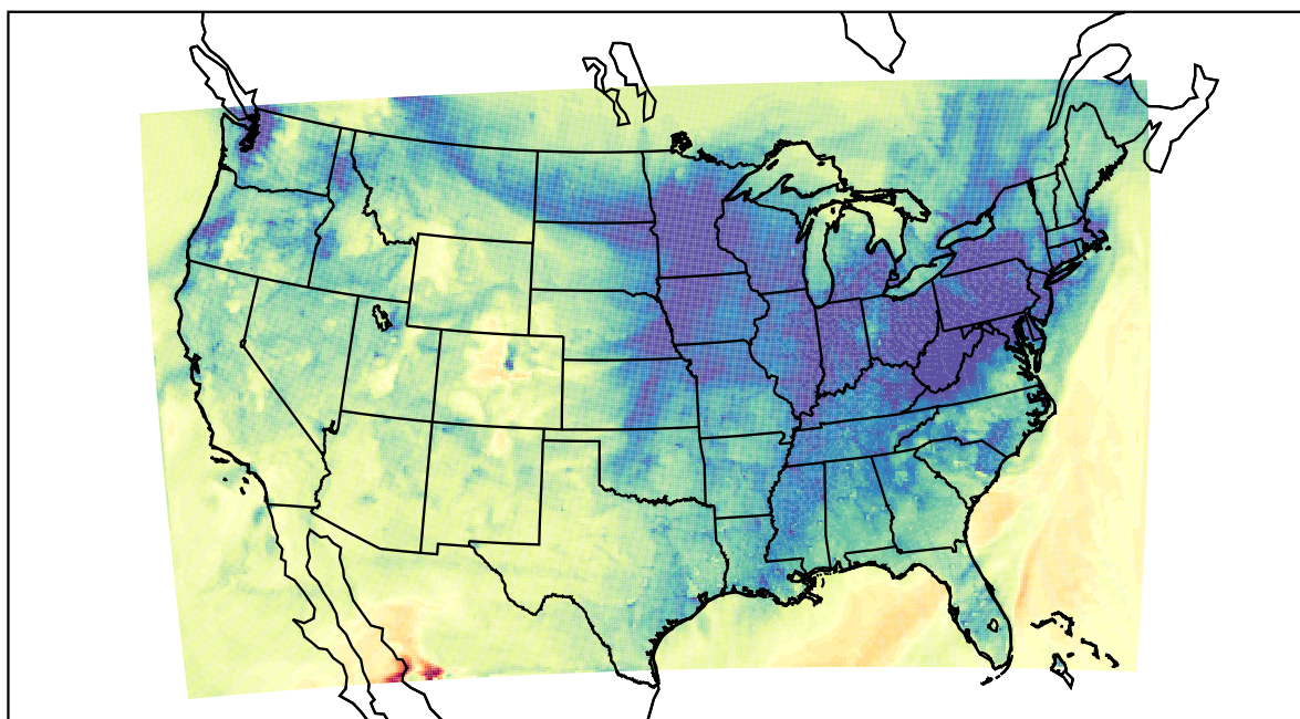
WRF (2023-11-22_23:00:00)
