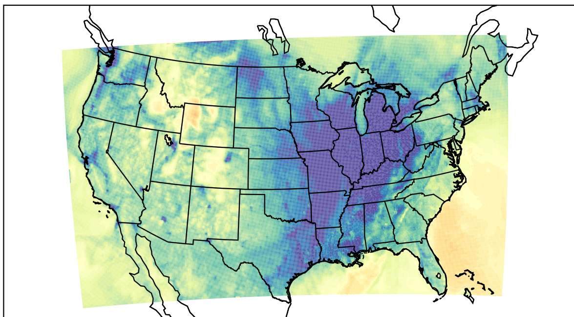
WRF (2023-11-22_02:00:00)
