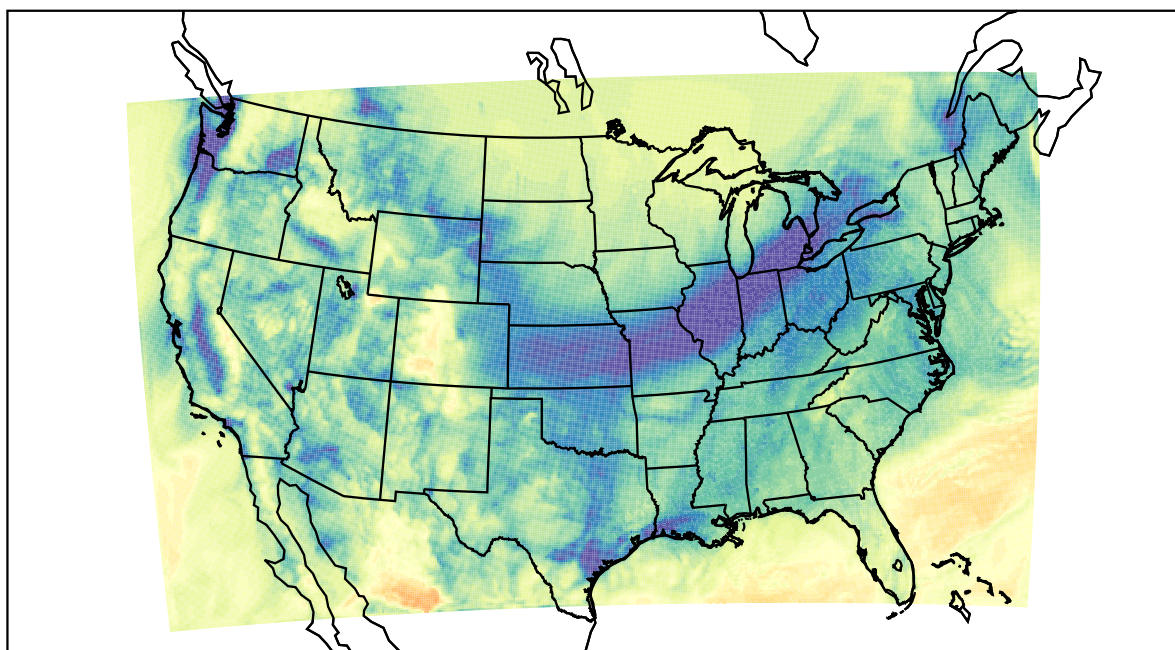
WRF (2023-11-23_17:00:00)
