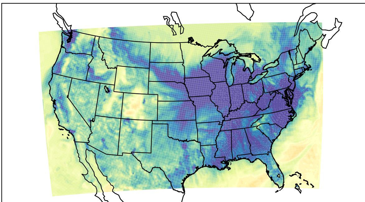
WRF (2023-11-23_06:00:00)
