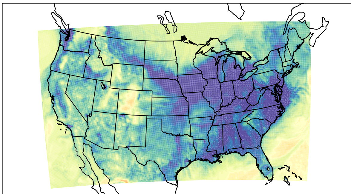
WRF (2023-11-23_08:00:00)
