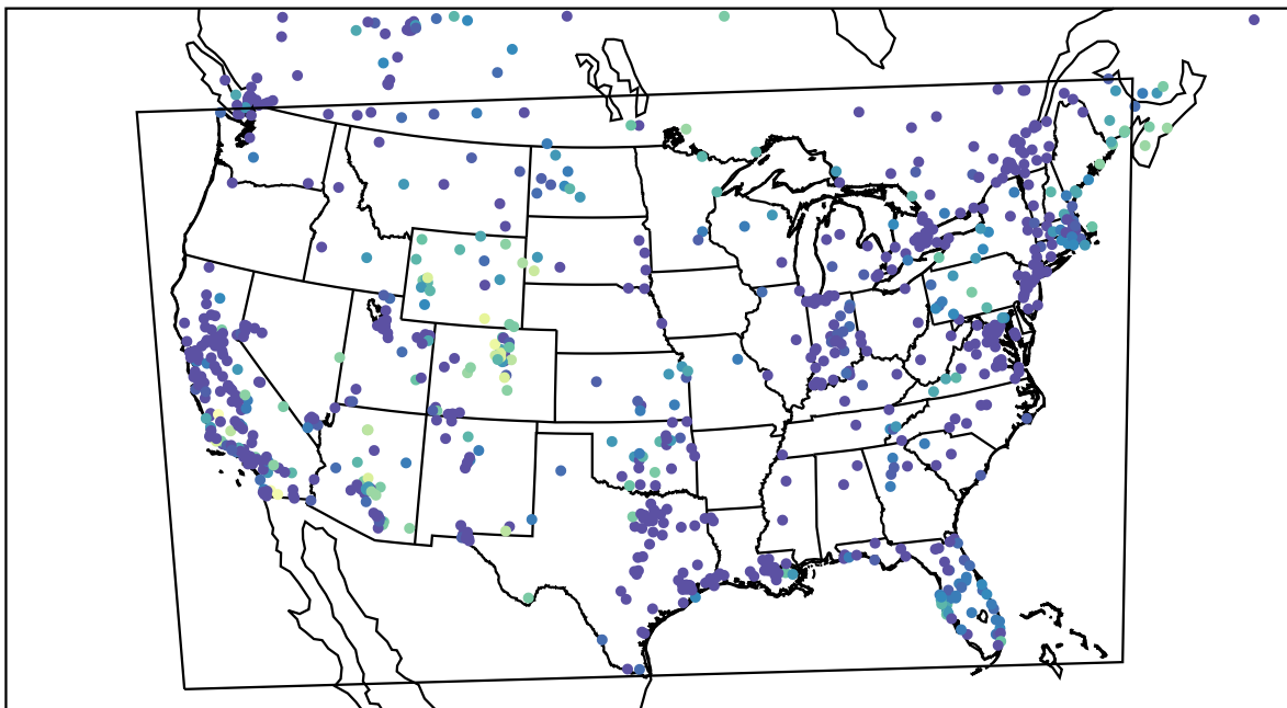
AirNOW (2023-11-23_06:00:00)
