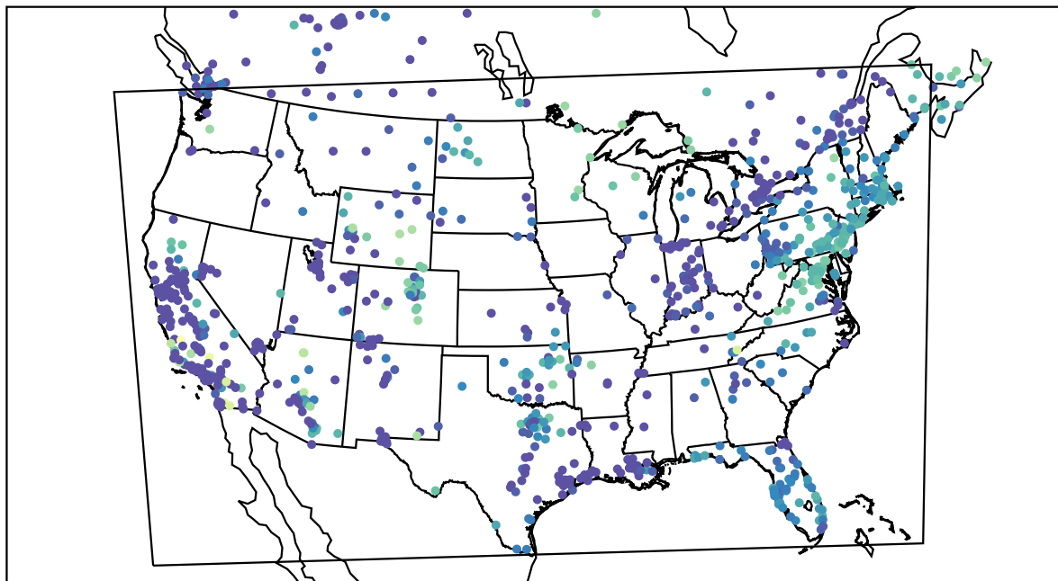
AirNOW (2023-11-23_15:00:00)
