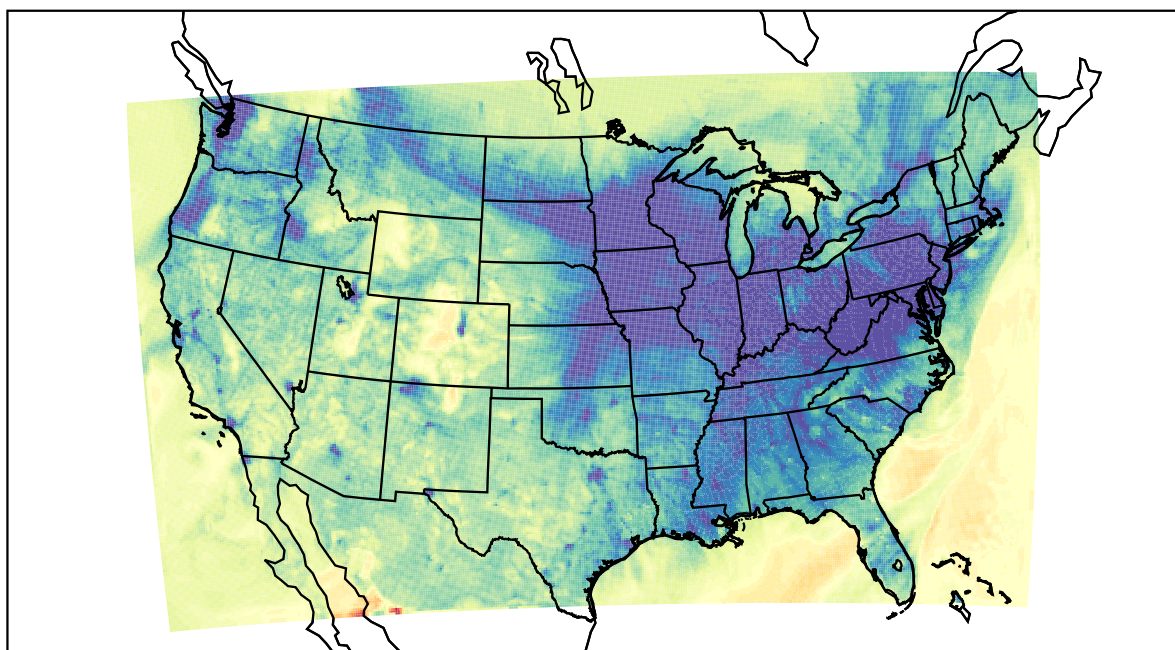
WRF (2023-11-23_01:00:00)
