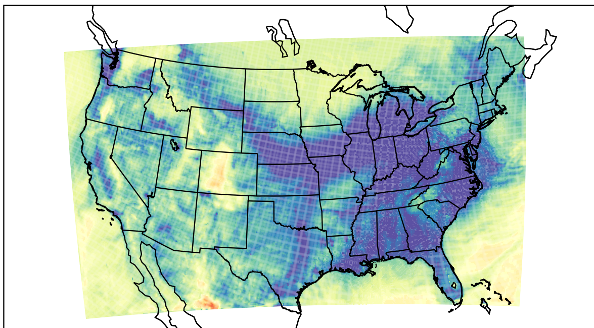
WRF (2023-11-23_12:00:00)
