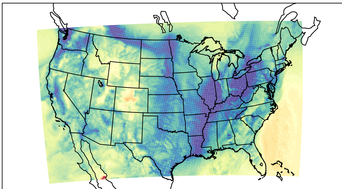
WRF (2023-11-22_16:00:00)
