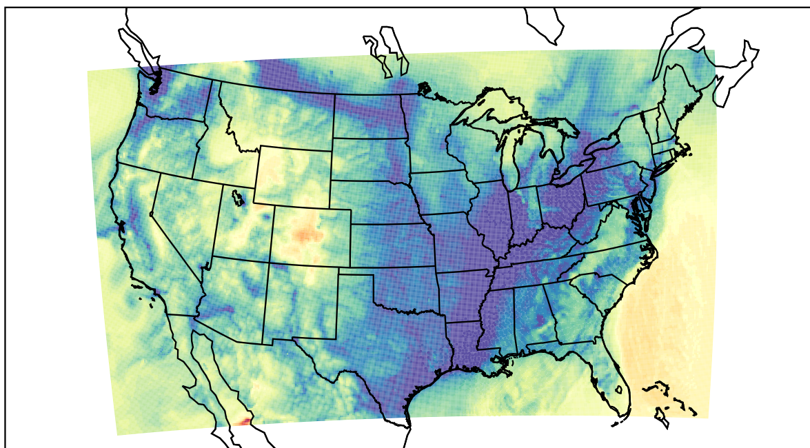
WRF (2023-11-22_15:00:00)
