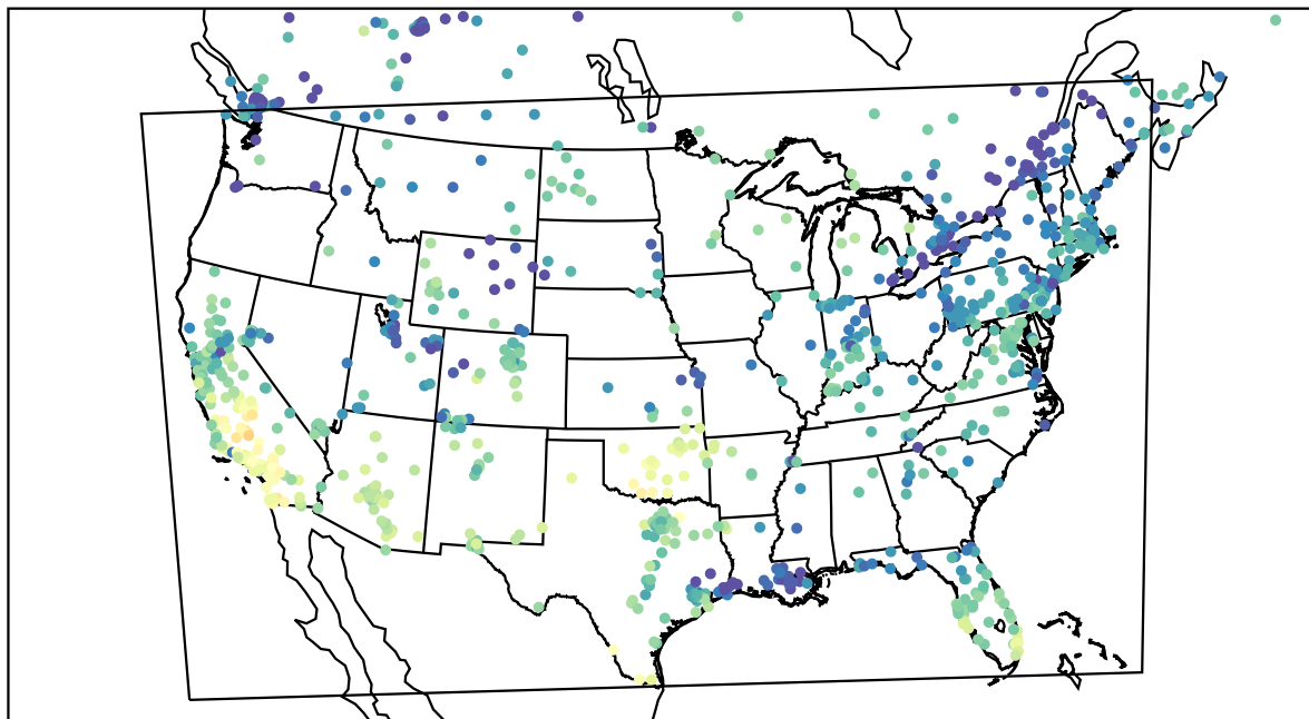
AirNOW (2023-11-23_21:00:00)
