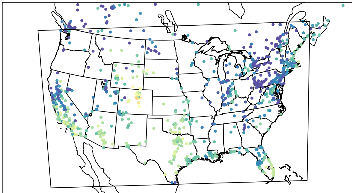
AirNOW (2023-11-22_19:00:00)
