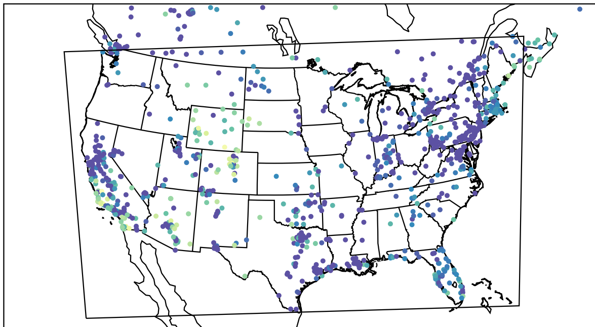
AirNOW (2023-11-23_01:00:00)
