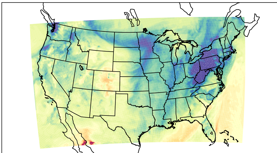
WRF (2023-11-22_21:00:00)
