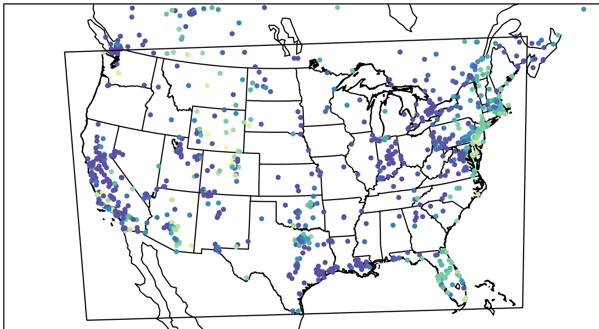
AirNOW (2023-11-22_05:00:00)
