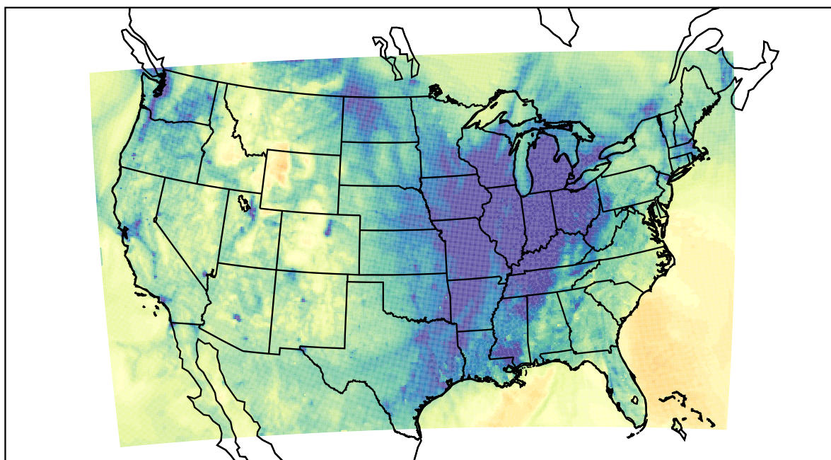
WRF (2023-11-22_01:00:00)
