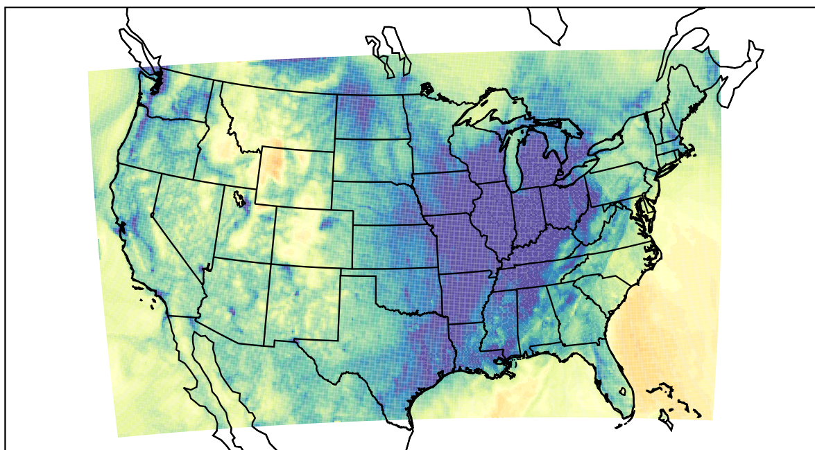
WRF (2023-11-22_03:00:00)
