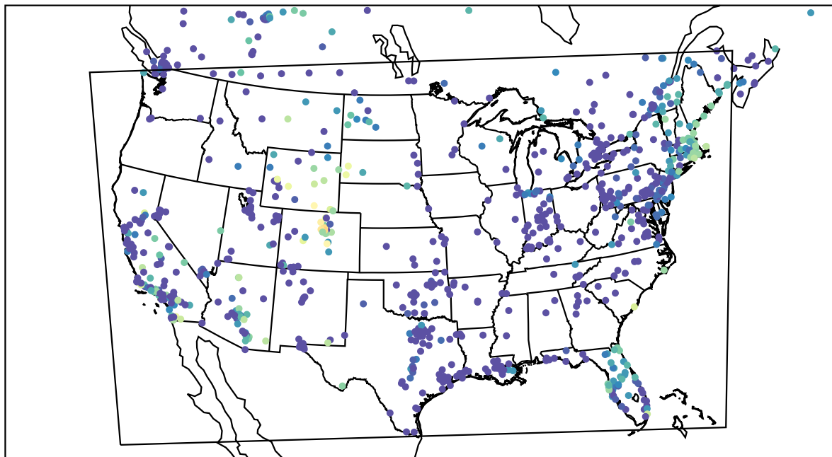
AirNOW (2023-11-22_12:00:00)
