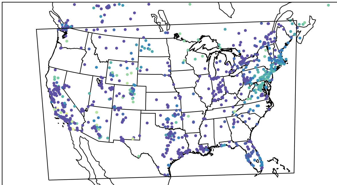
AirNOW (2023-11-23_14:00:00)
