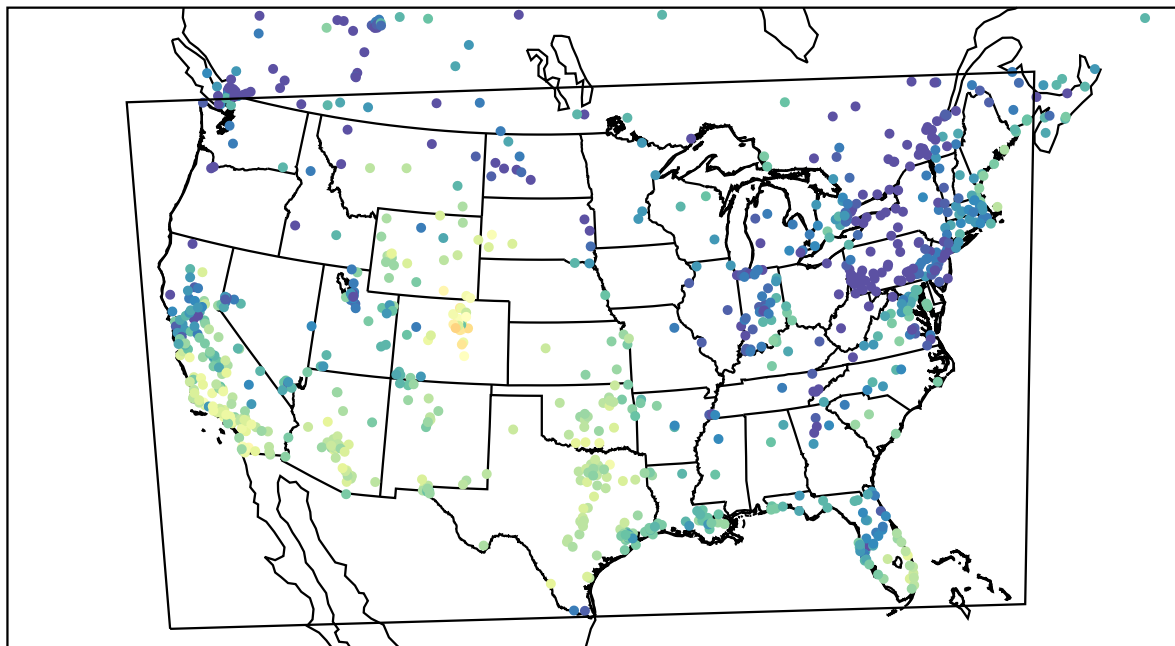
AirNOW (2023-11-22_20:00:00)
