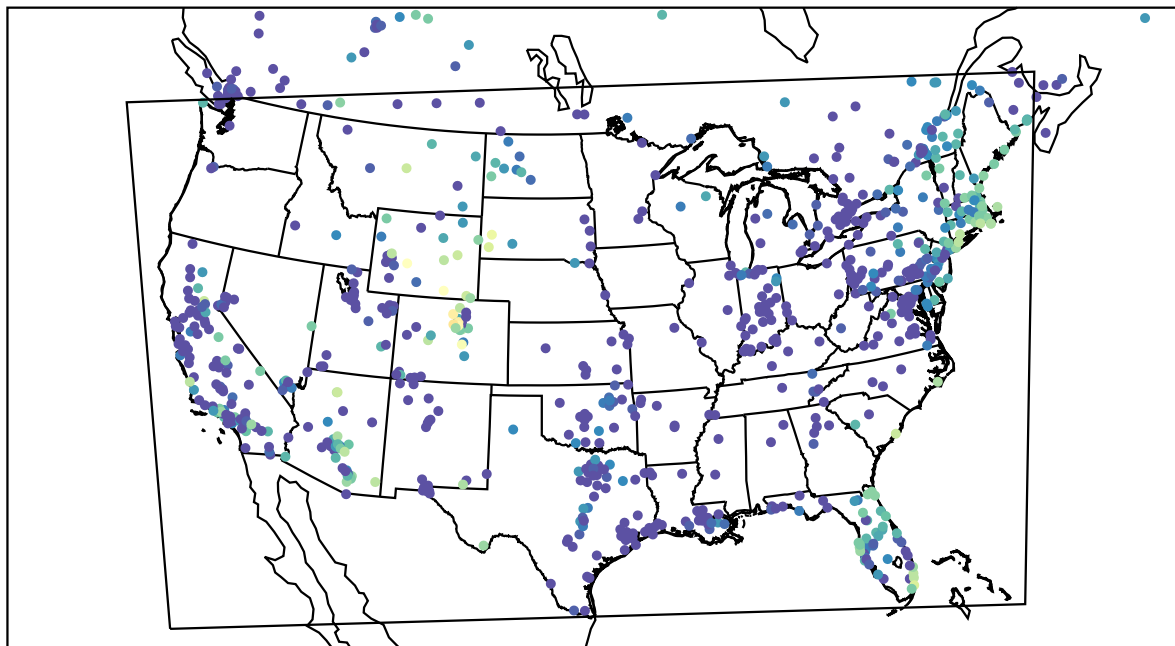
AirNOW (2023-11-22_10:00:00)
