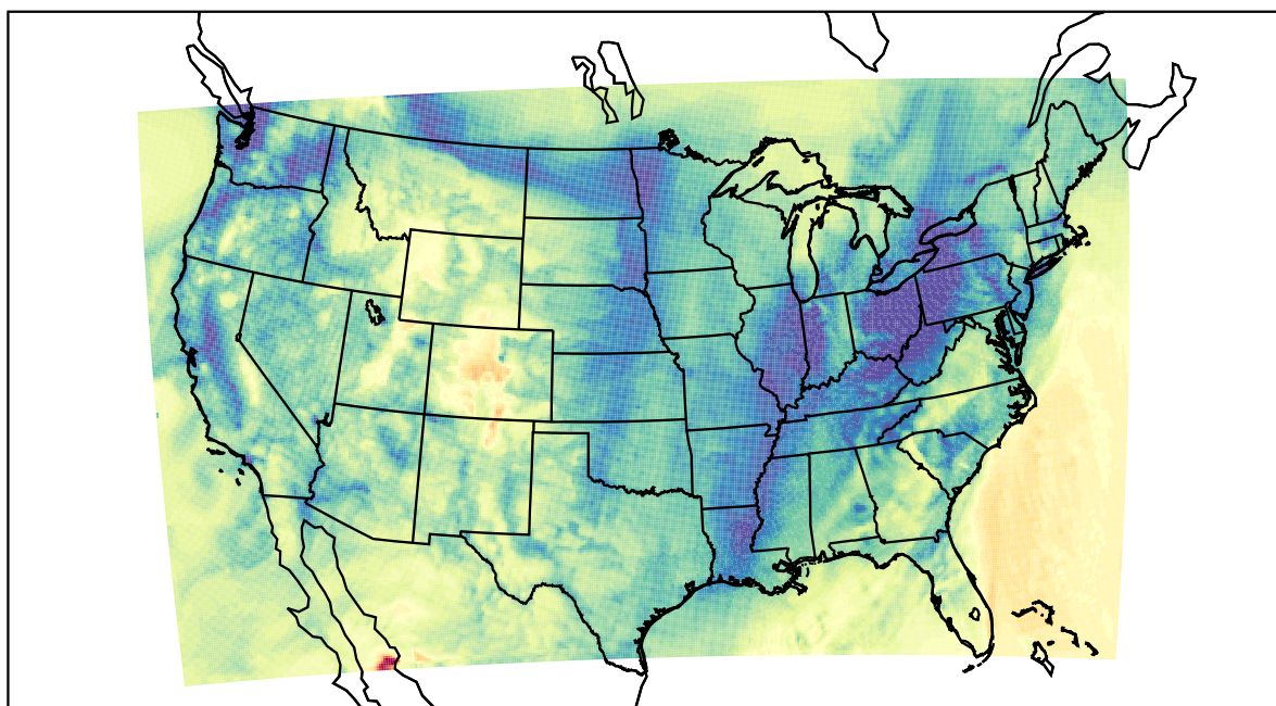
WRF (2023-11-22_17:00:00)
