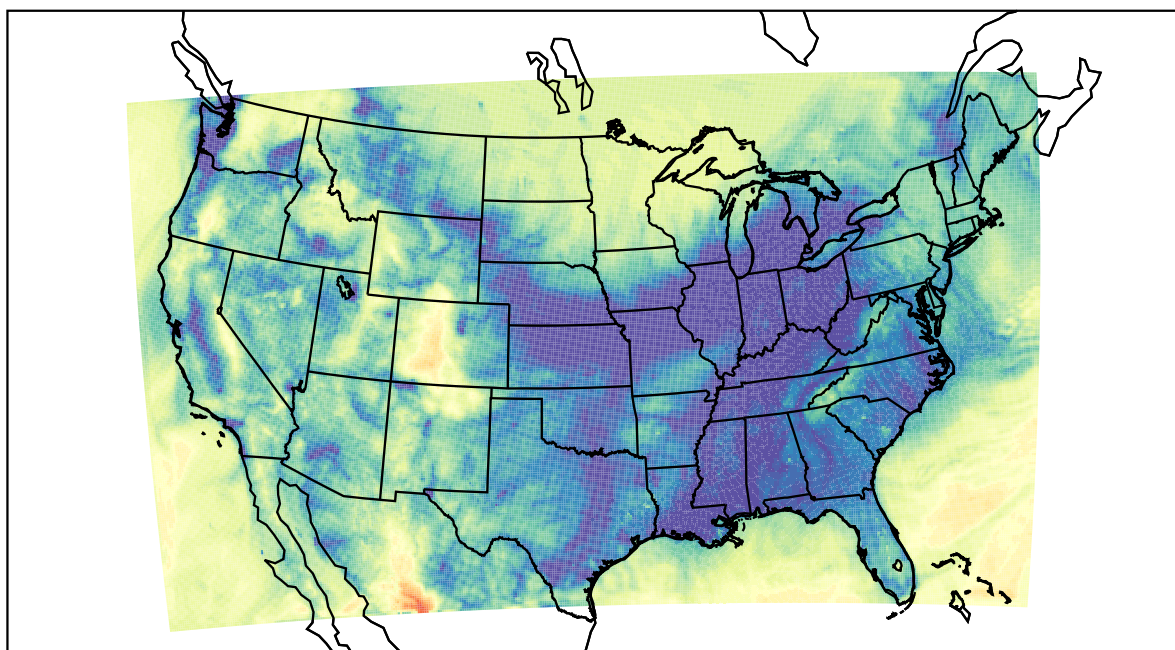
WRF (2023-11-23_14:00:00)
