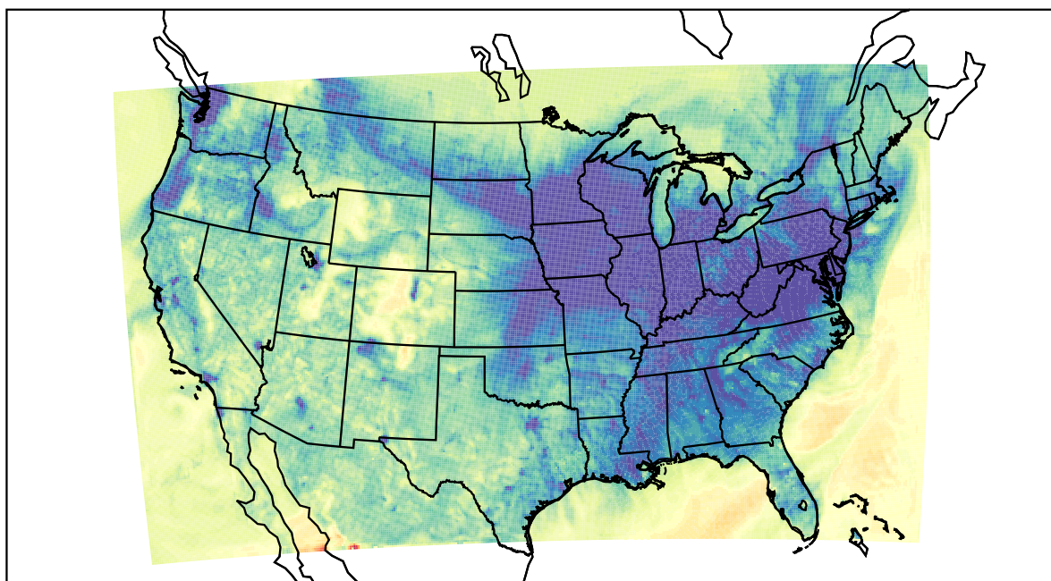
WRF (2023-11-23_02:00:00)
