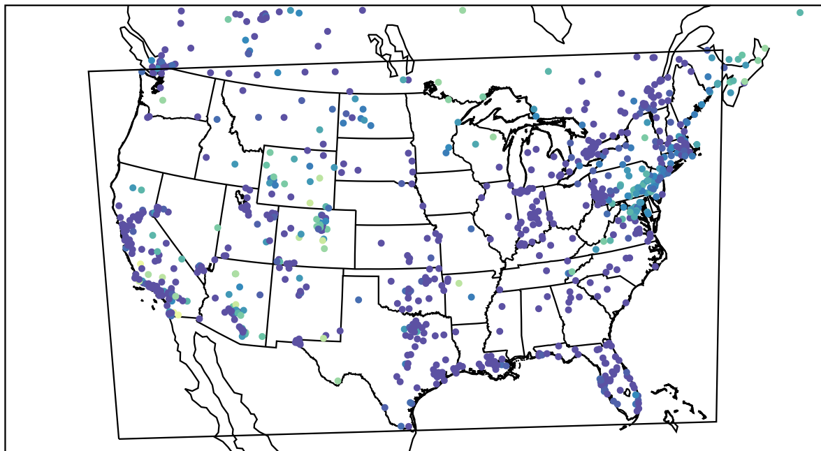
AirNOW (2023-11-23_12:00:00)
