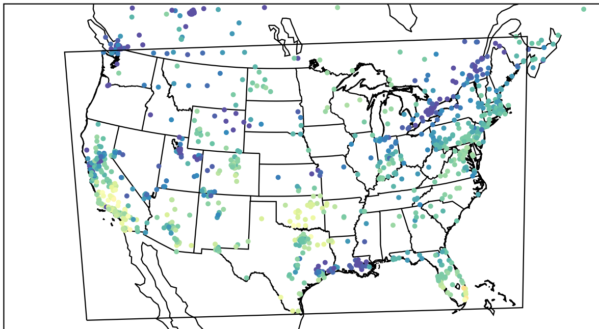
AirNOW (2023-11-23_19:00:00)
