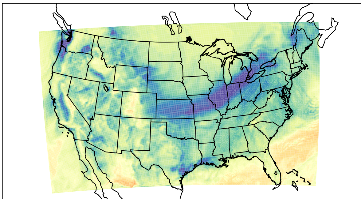
WRF (2023-11-23_18:00:00)
