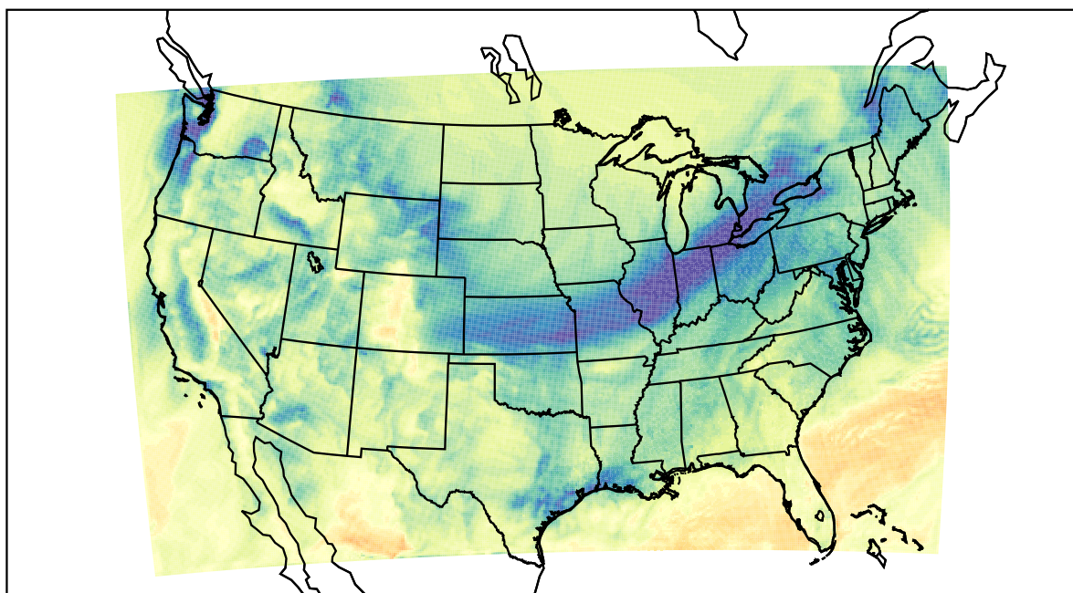
WRF (2023-11-23_19:00:00)
