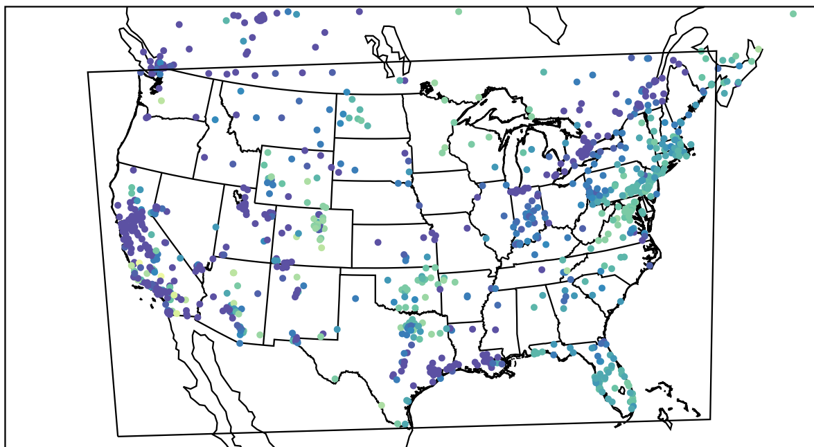
AirNOW (2023-11-23_16:00:00)
