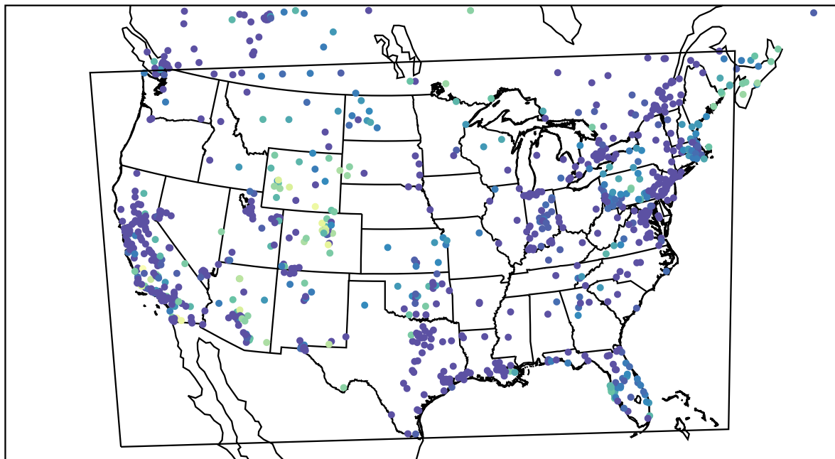
AirNOW (2023-11-23_05:00:00)
