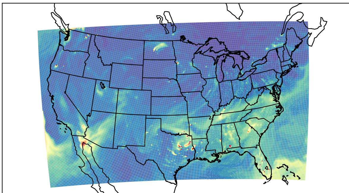
WRF 2023-11-24_22:00:00
