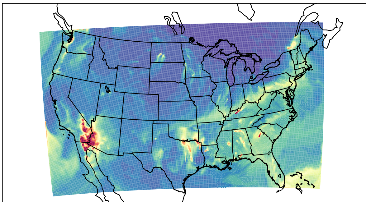
WRF 2023-11-24_07:00:00
