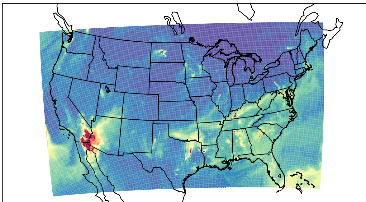
WRF 2023-11-24_14:00:00
