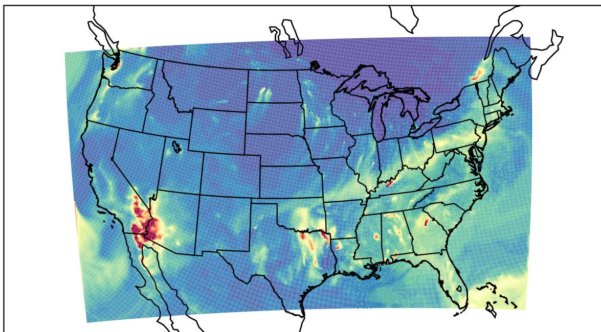
WRF 2023-11-24_06:00:00
