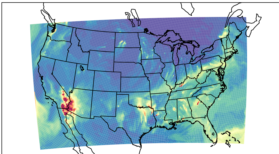
WRF 2023-11-24_08:00:00
