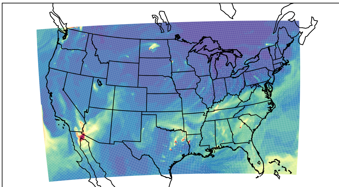
WRF 2023-11-24_19:00:00
