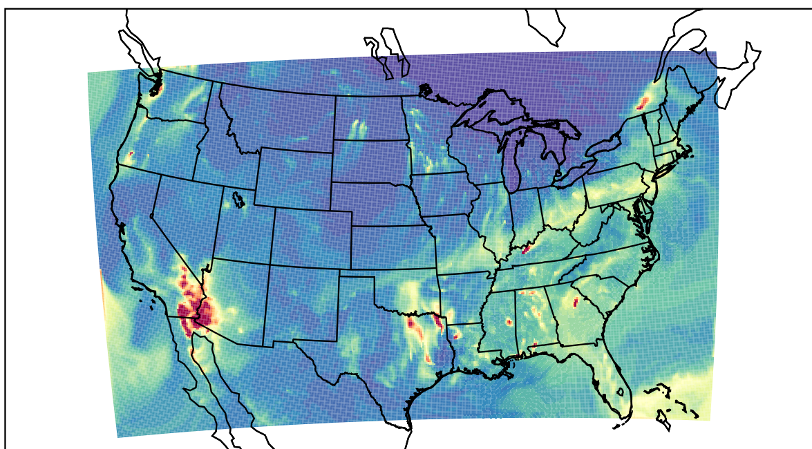
WRF 2023-11-24_05:00:00
