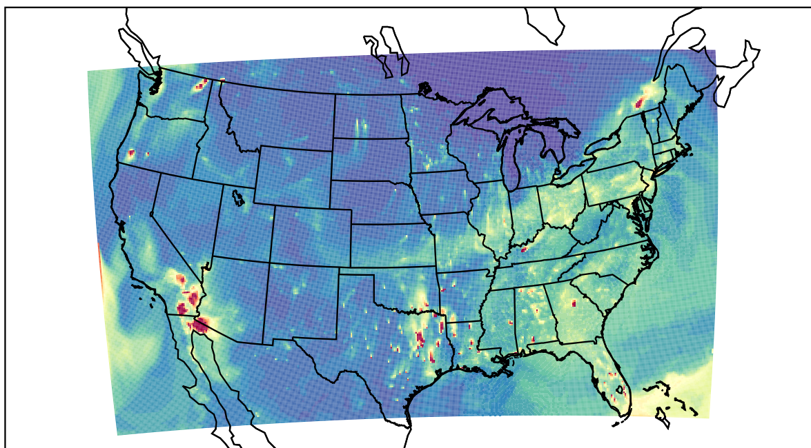
WRF 2023-11-24_00:00:00
