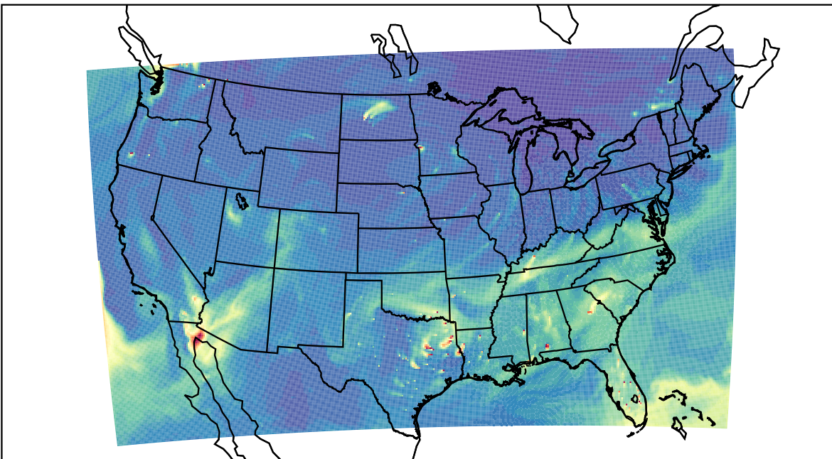
WRF 2023-11-24_21:00:00
