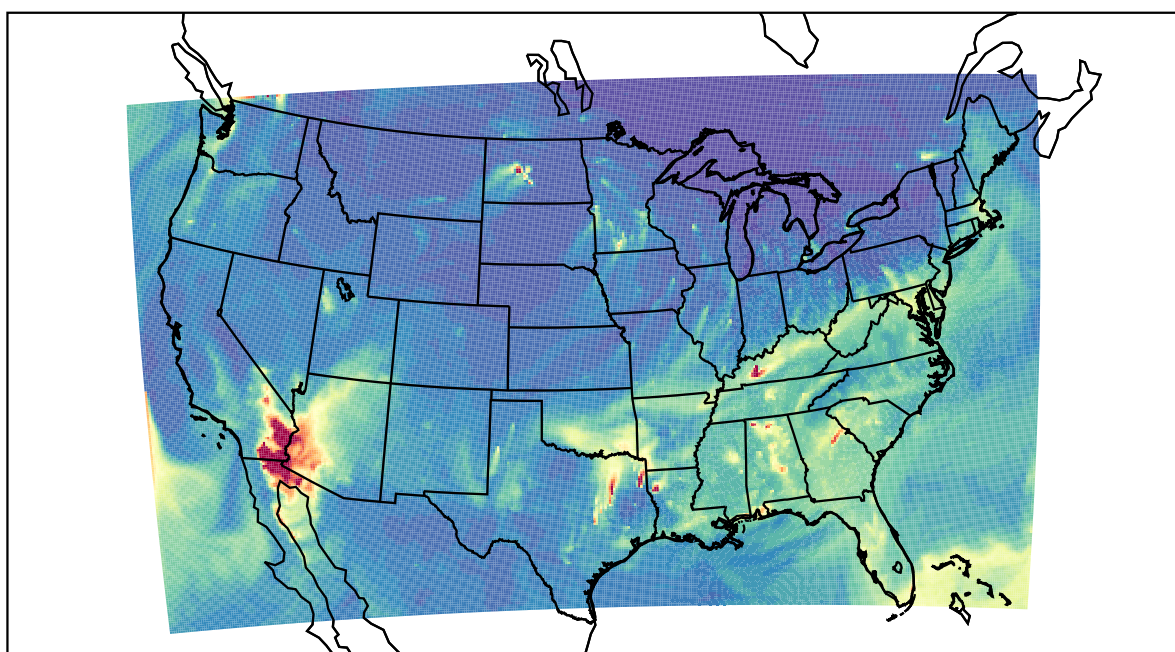
WRF 2023-11-24_13:00:00
