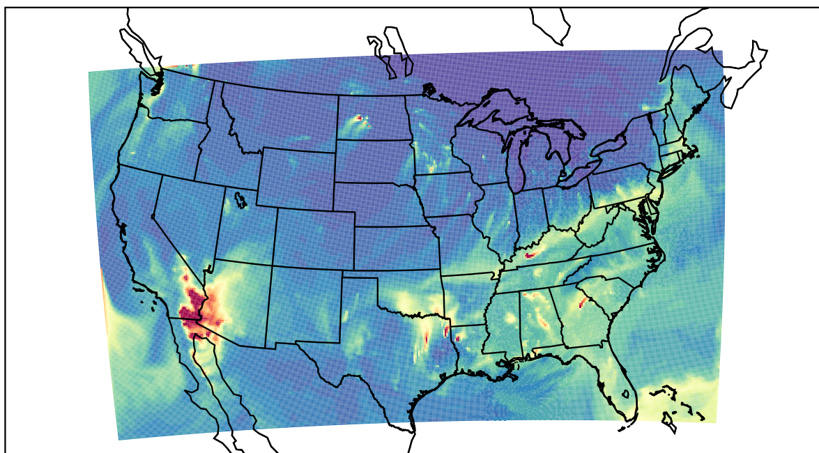
WRF 2023-11-24_11:00:00
