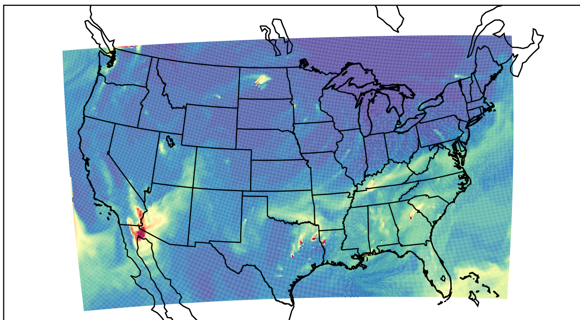
WRF 2023-11-24_18:00:00
