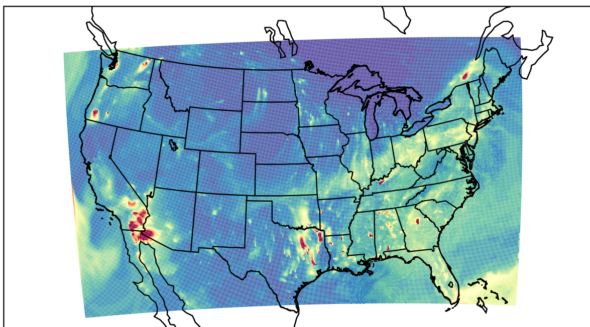
WRF 2023-11-24_02:00:00
