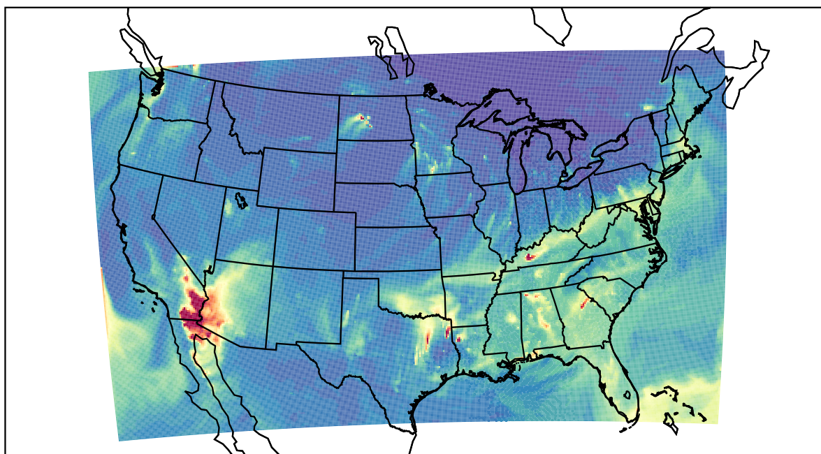
WRF 2023-11-24_12:00:00
