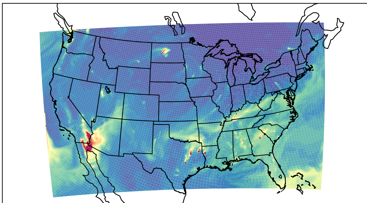
WRF 2023-11-24_17:00:00
