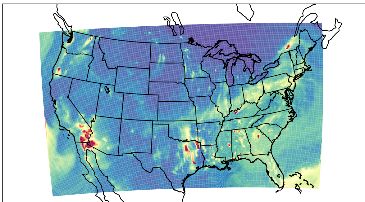
WRF 2023-11-24_03:00:00
