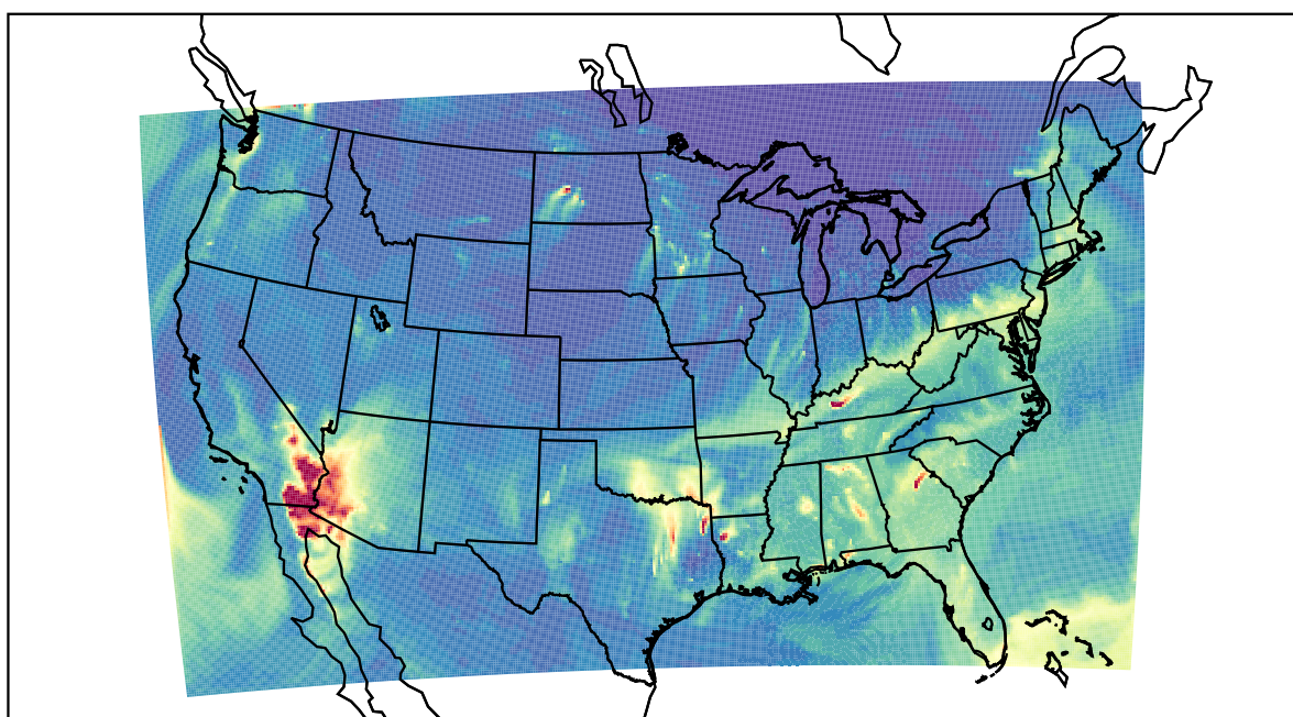
WRF 2023-11-24_10:00:00
