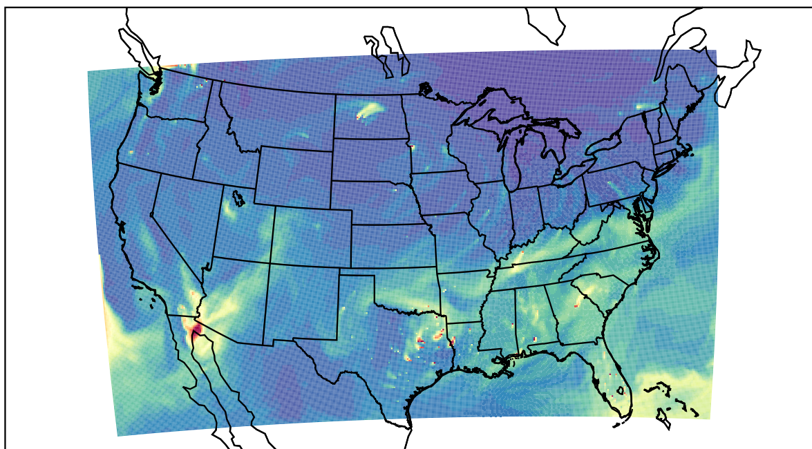
WRF 2023-11-24_20:00:00
