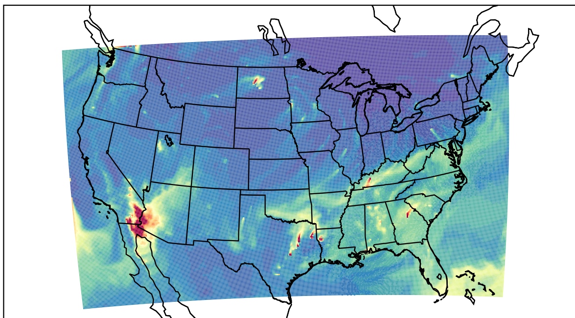
WRF 2023-11-24_16:00:00
