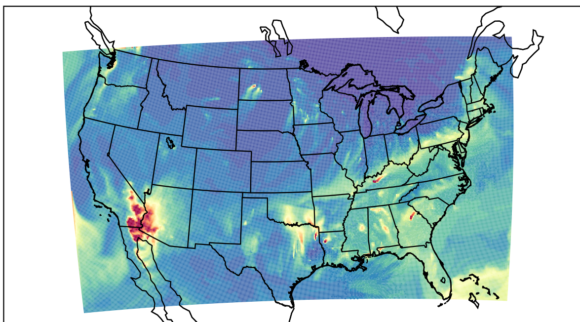
WRF 2023-11-24_09:00:00
