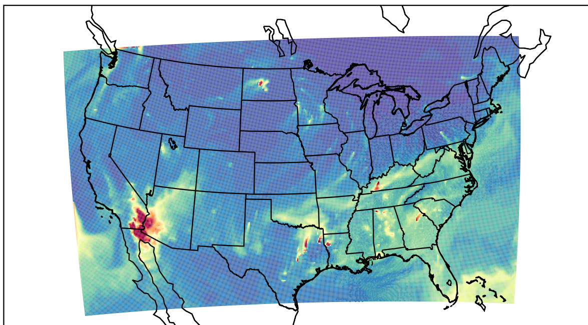
WRF 2023-11-24_15:00:00
