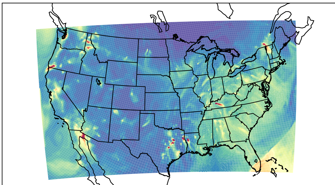
WRF 2023-11-23_06:00:00
