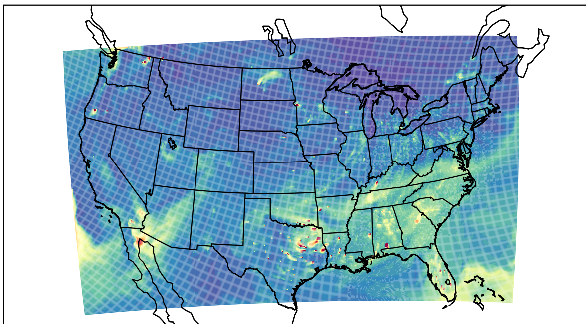
WRF 2023-11-24_23:00:00
