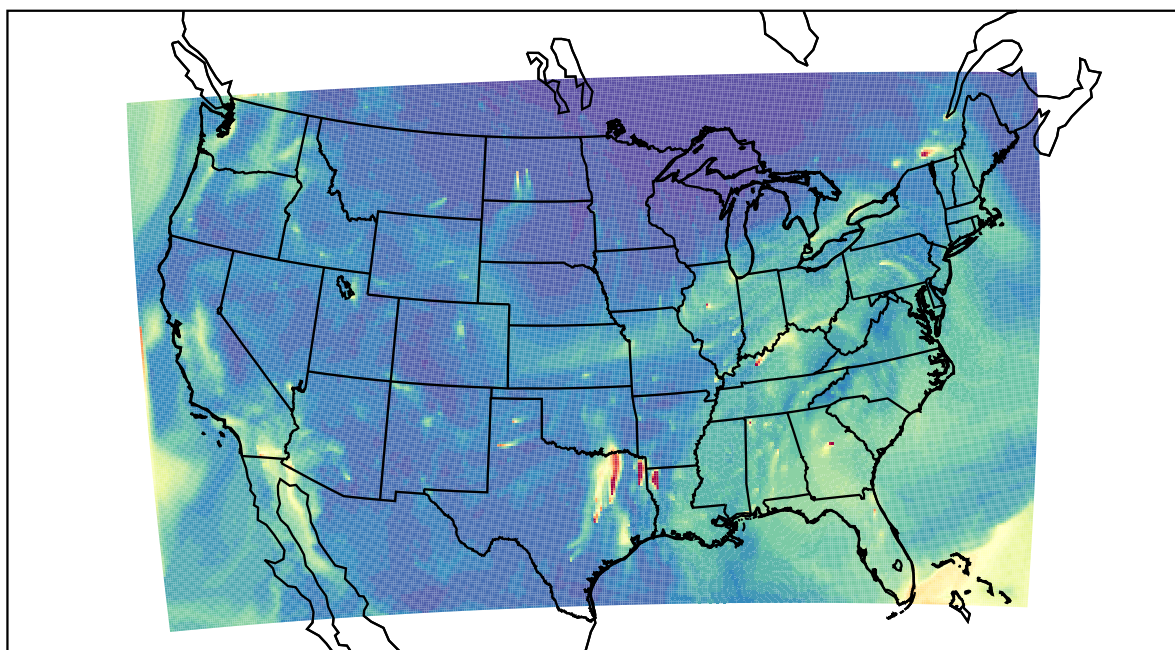
WRF 2023-11-23_16:00:00
