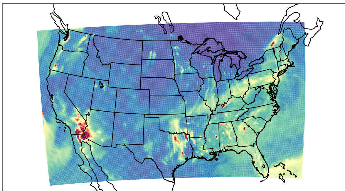
WRF 2023-11-24_04:00:00
