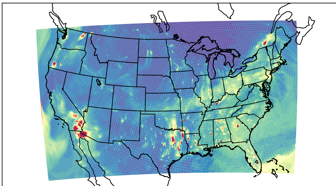
WRF 2023-11-24_01:00:00
