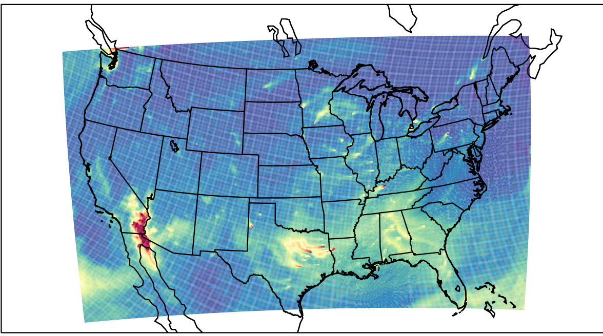
WRF 2023-11-25_15:00:00
