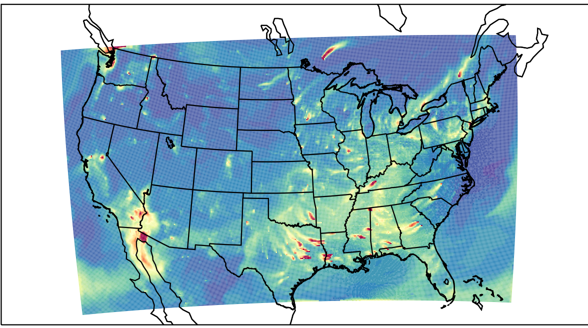
WRF 2023-11-26_02:00:00
