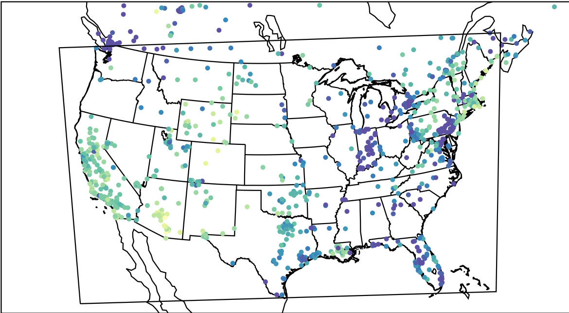
AirNOW (2023-11-26_23:00:00)
