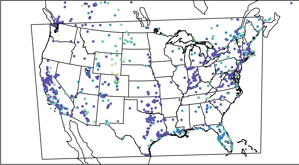
AirNOW (2023-11-26_06:00:00)
