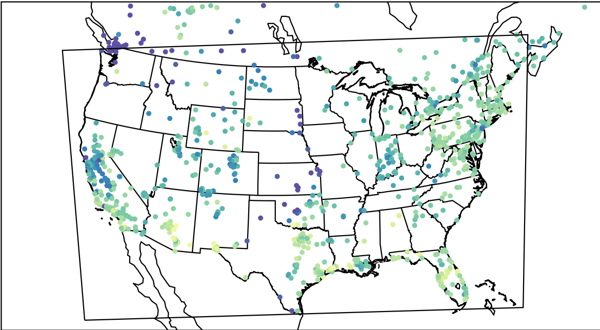
AirNOW (2023-11-25_19:00:00)
