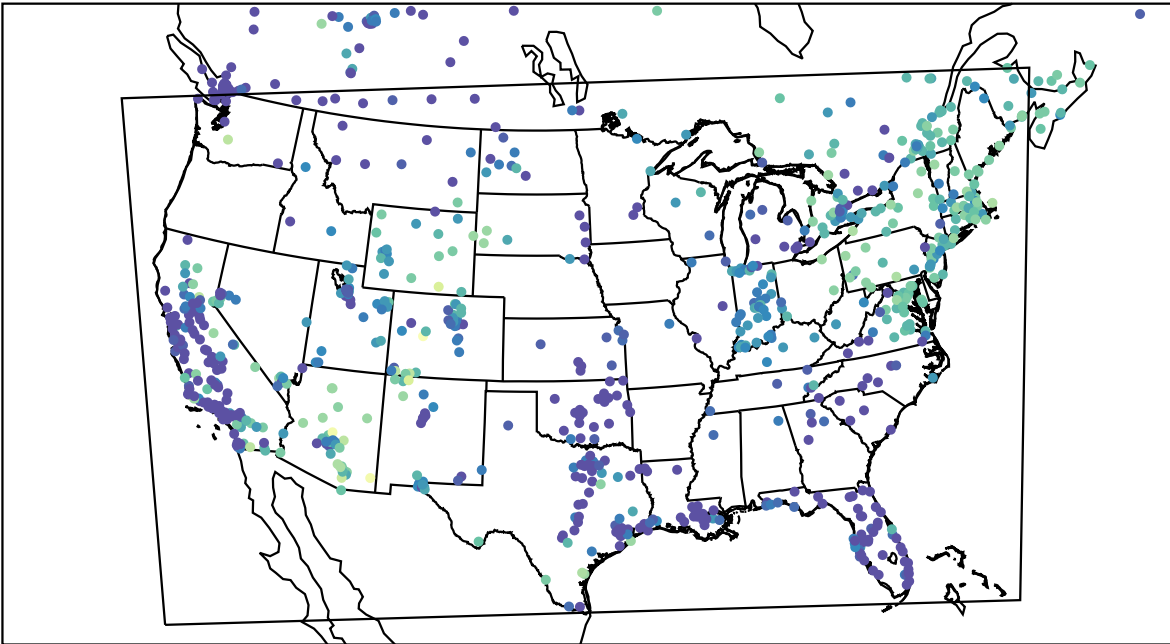
AirNOW (2023-11-25_06:00:00)
