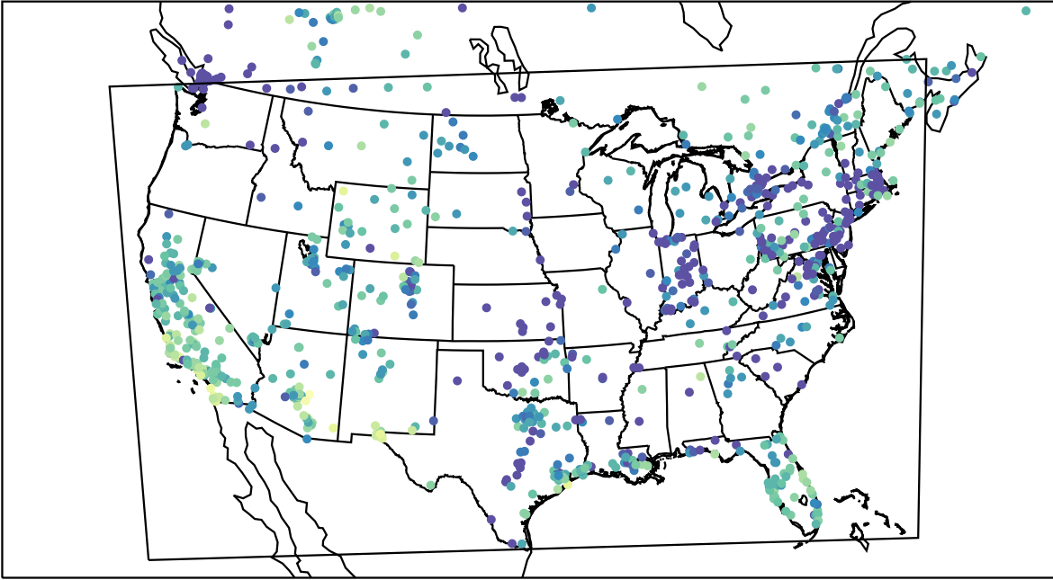
AirNOW (2023-11-26_00:00:00)
