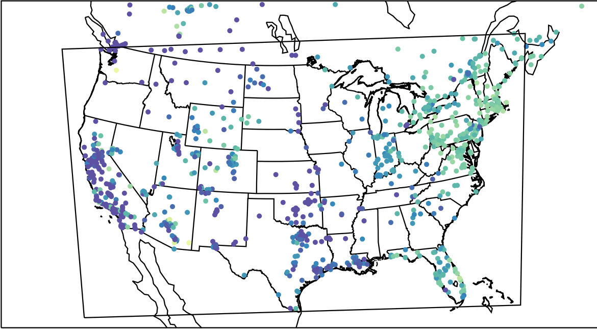
AirNOW (2023-11-25_15:00:00)
