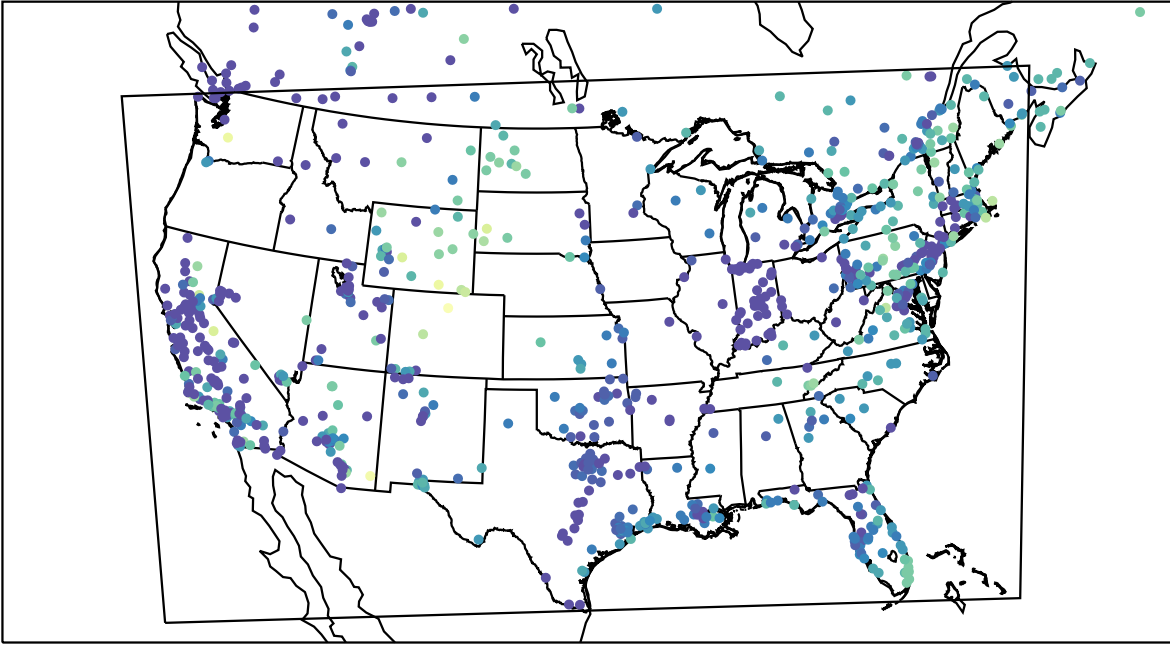
AirNOW (2023-11-26_15:00:00)
