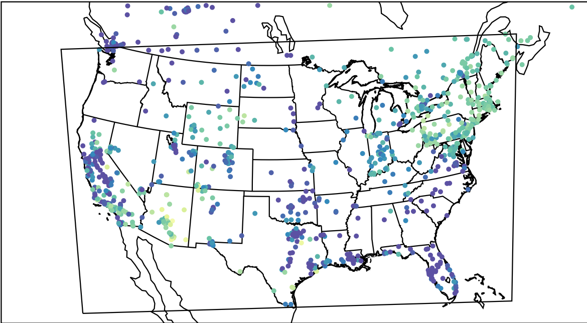
AirNOW (2023-11-25_02:00:00)
