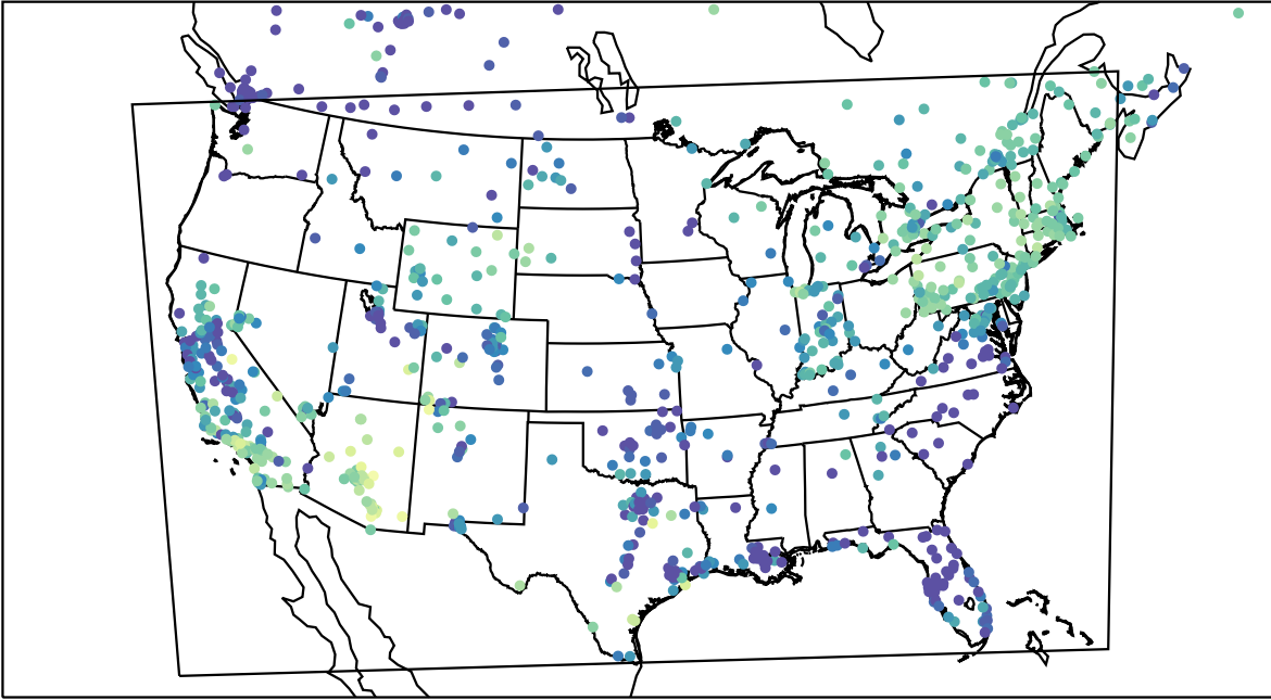
AirNOW (2023-11-25_01:00:00)
