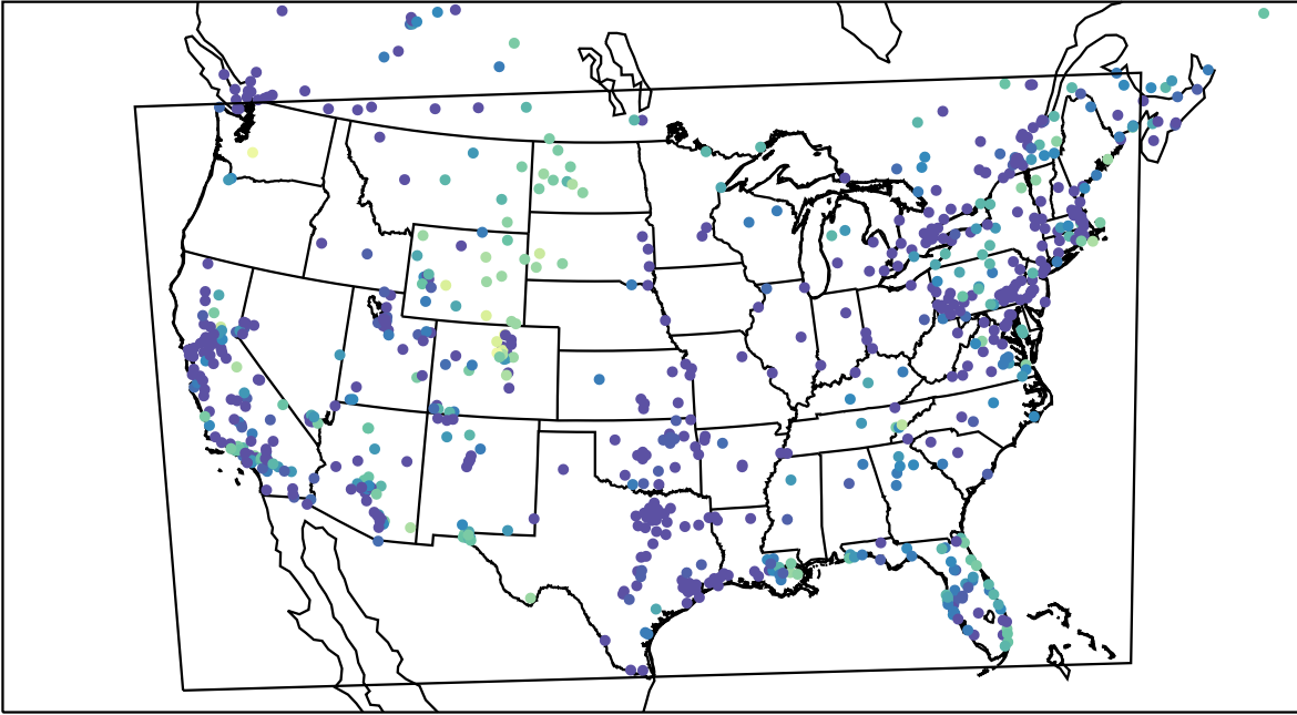
AirNOW (2023-11-26_10:00:00)
