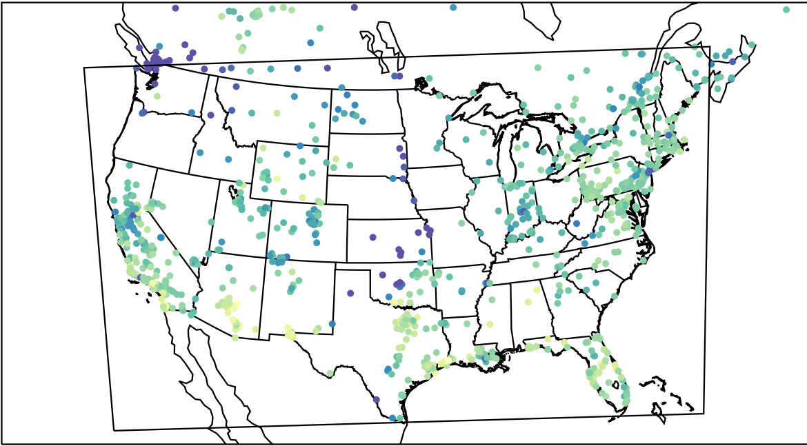
AirNOW (2023-11-25_20:00:00)
