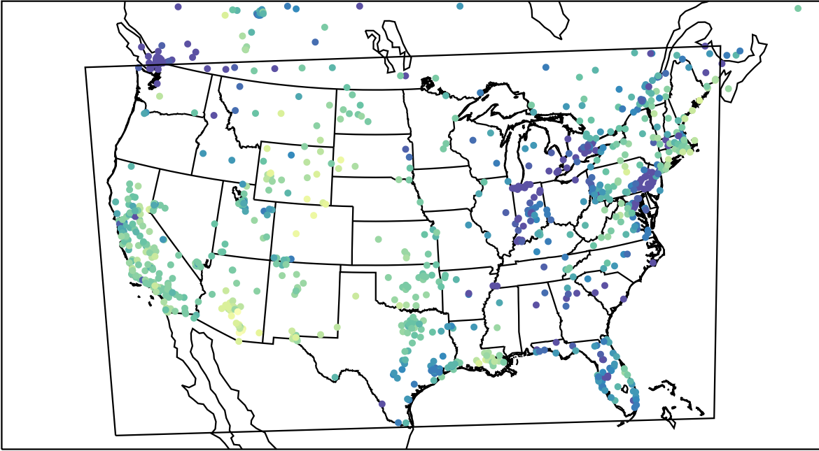
AirNOW (2023-11-26_21:00:00)
