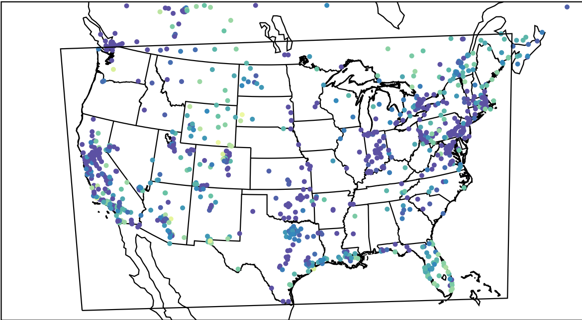
AirNOW (2023-11-26_03:00:00)
