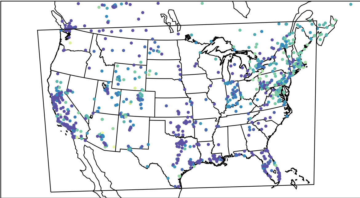
AirNOW (2023-11-25_08:00:00)
