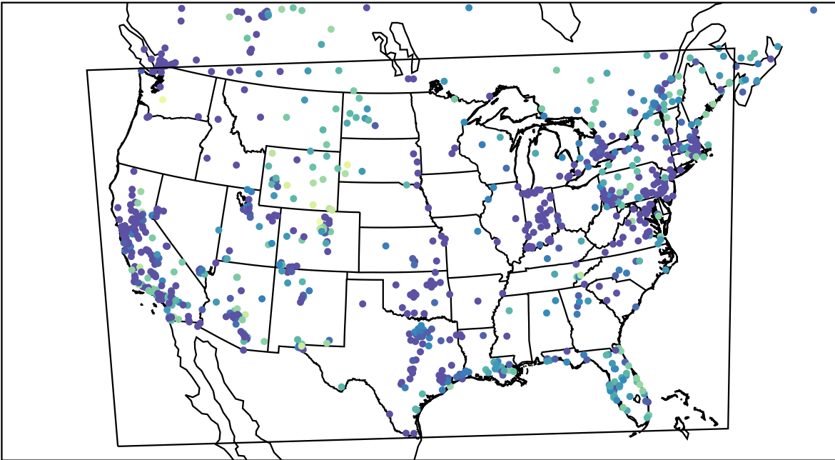
AirNOW (2023-11-26_05:00:00)
