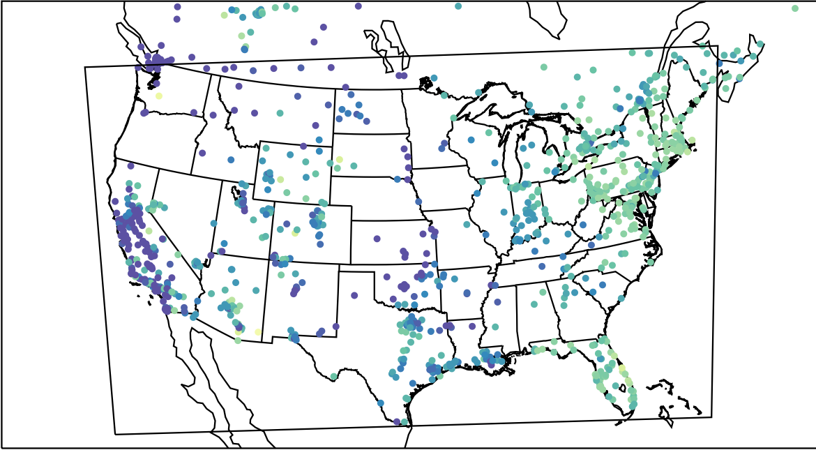
AirNOW (2023-11-25_16:00:00)
