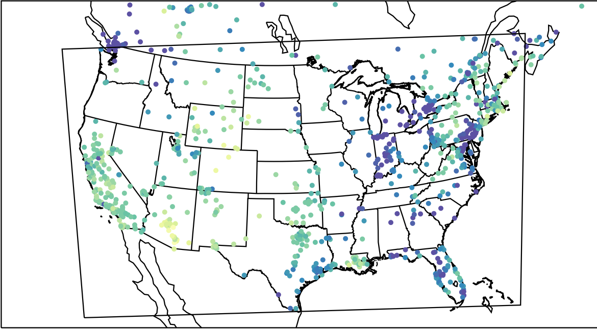
AirNOW (2023-11-26_22:00:00)
