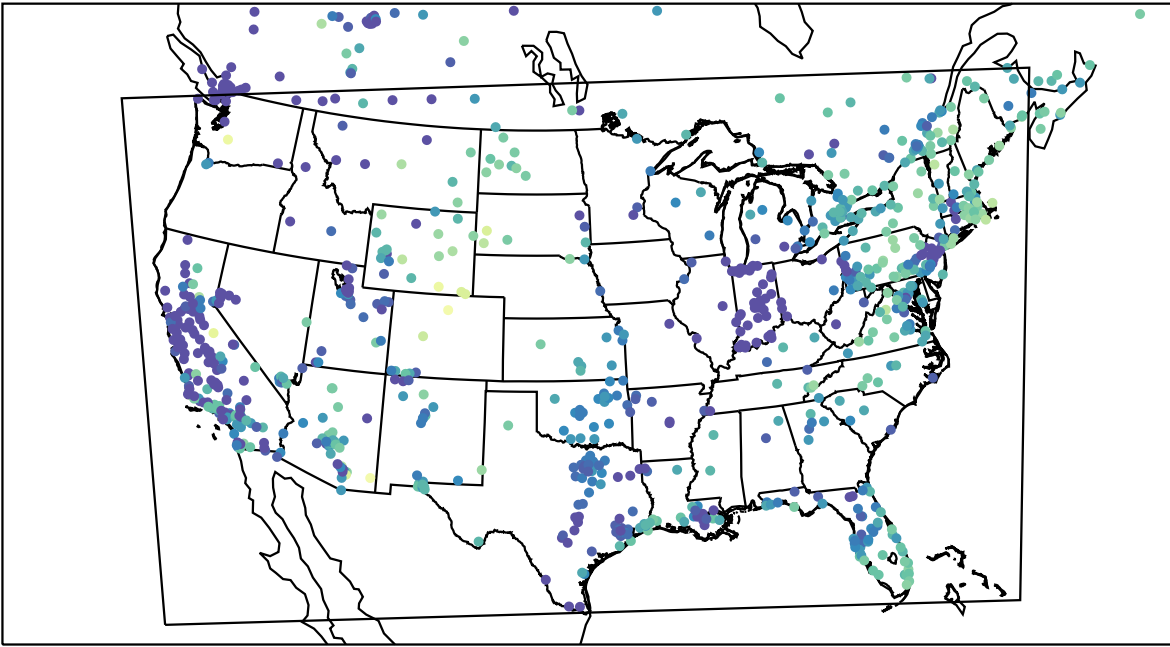
AirNOW (2023-11-26_16:00:00)
