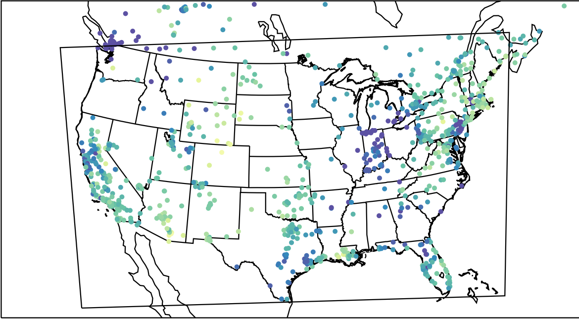
AirNOW (2023-11-26_19:00:00)
