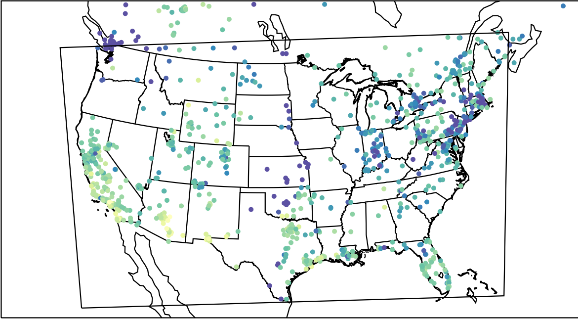
AirNOW (2023-11-25_22:00:00)
