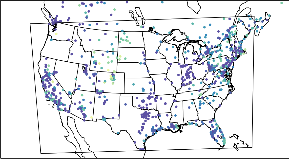
AirNOW (2023-11-26_14:00:00)
