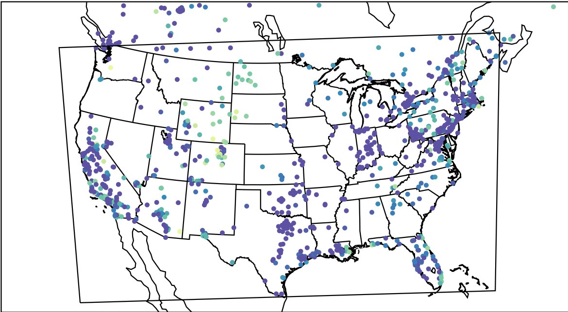
AirNOW (2023-11-26_13:00:00)
