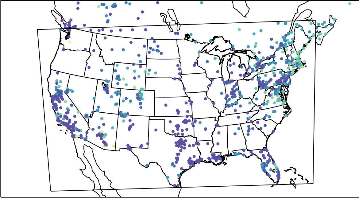
AirNOW (2023-11-25_13:00:00)
