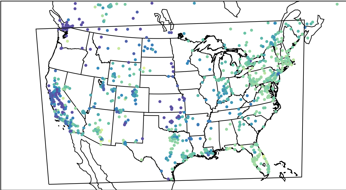
AirNOW (2023-11-25_17:00:00)
