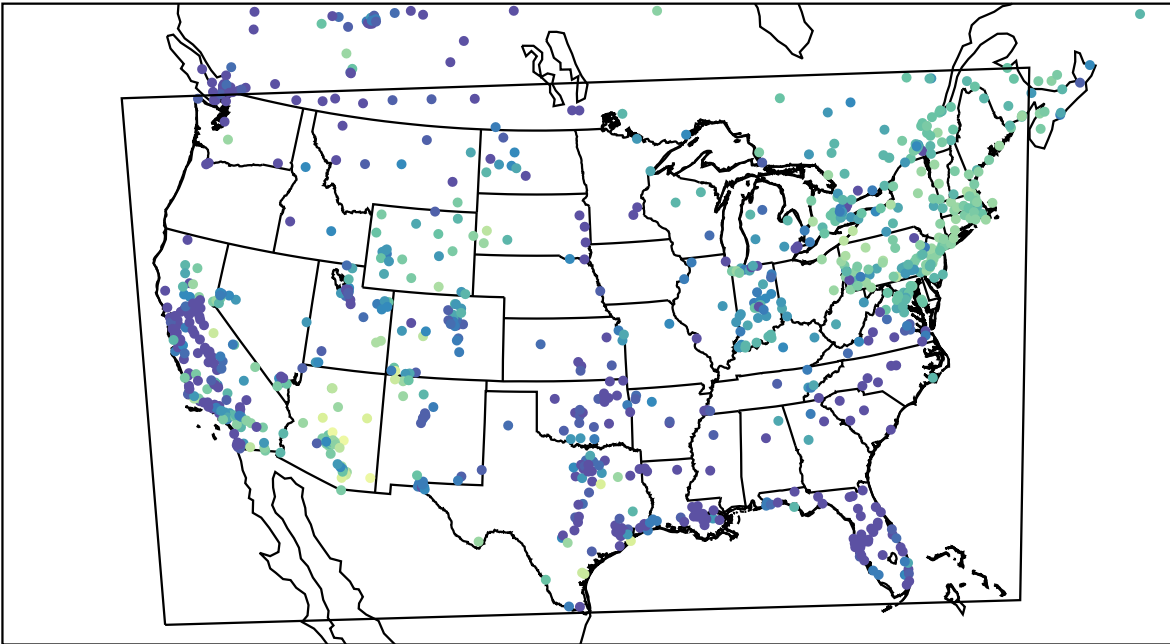
AirNOW (2023-11-25_03:00:00)
