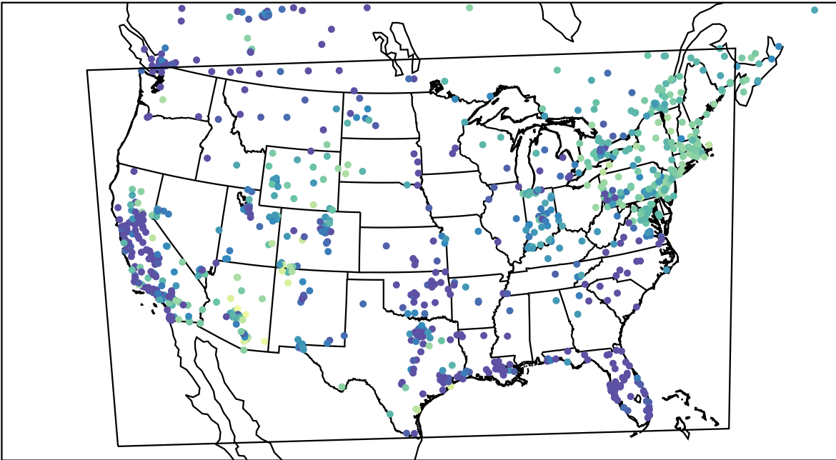
AirNOW (2023-11-25_04:00:00)
