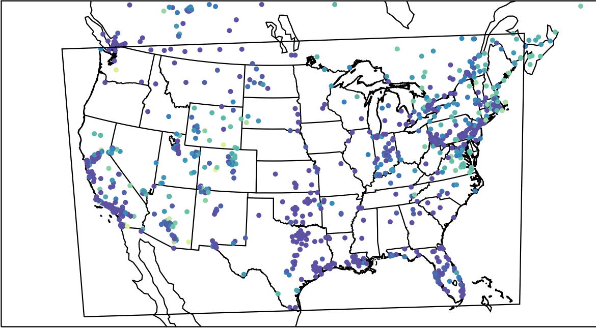
AirNOW (2023-11-25_12:00:00)
