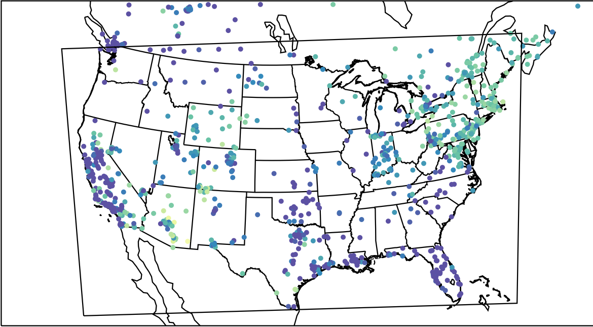
AirNOW (2023-11-25_05:00:00)
