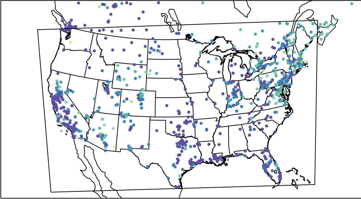
AirNOW (2023-11-25_09:00:00)
