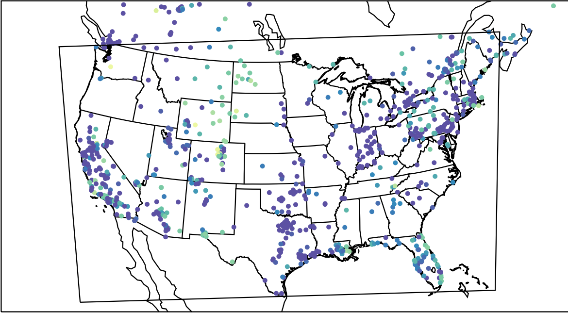
AirNOW (2023-11-26_09:00:00)
