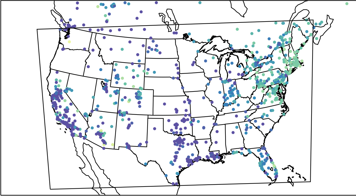
AirNOW (2023-11-25_14:00:00)
