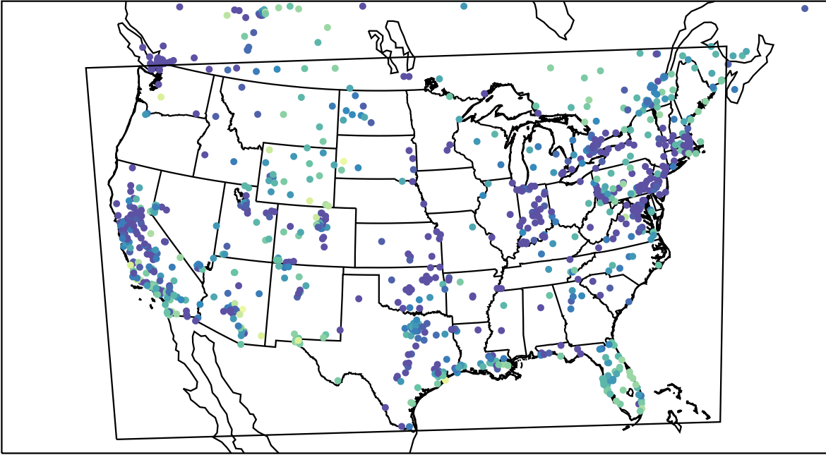
AirNOW (2023-11-26_02:00:00)
