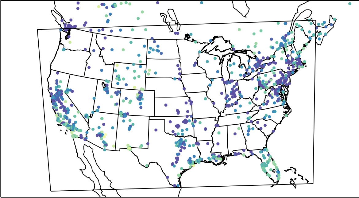
AirNOW (2023-11-26_01:00:00)
