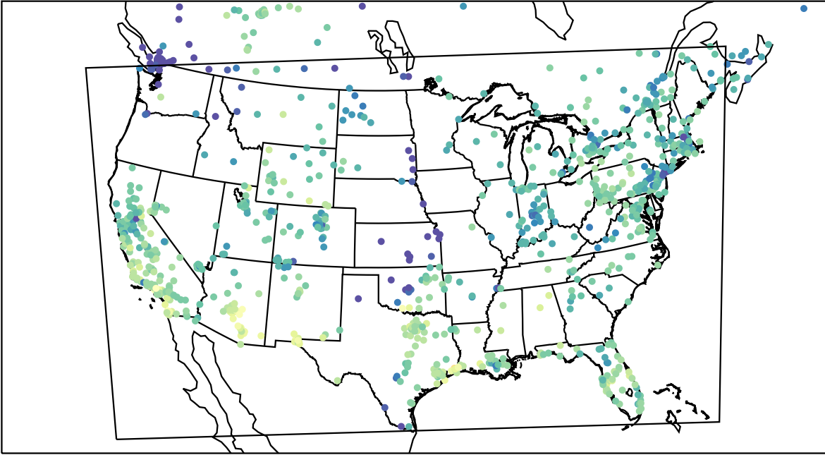
AirNOW (2023-11-25_21:00:00)
