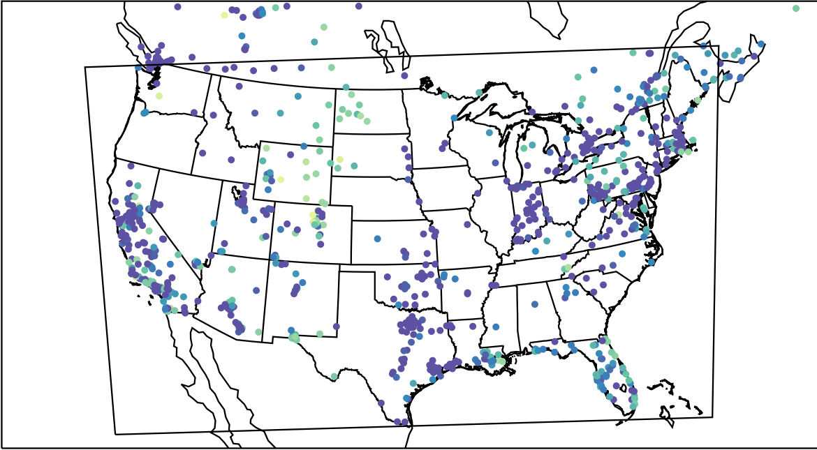
AirNOW (2023-11-26_08:00:00)
