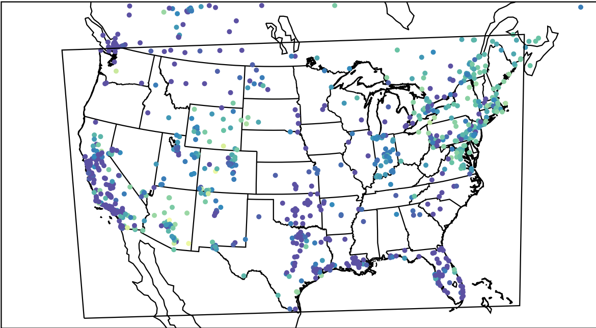
AirNOW (2023-11-25_07:00:00)
