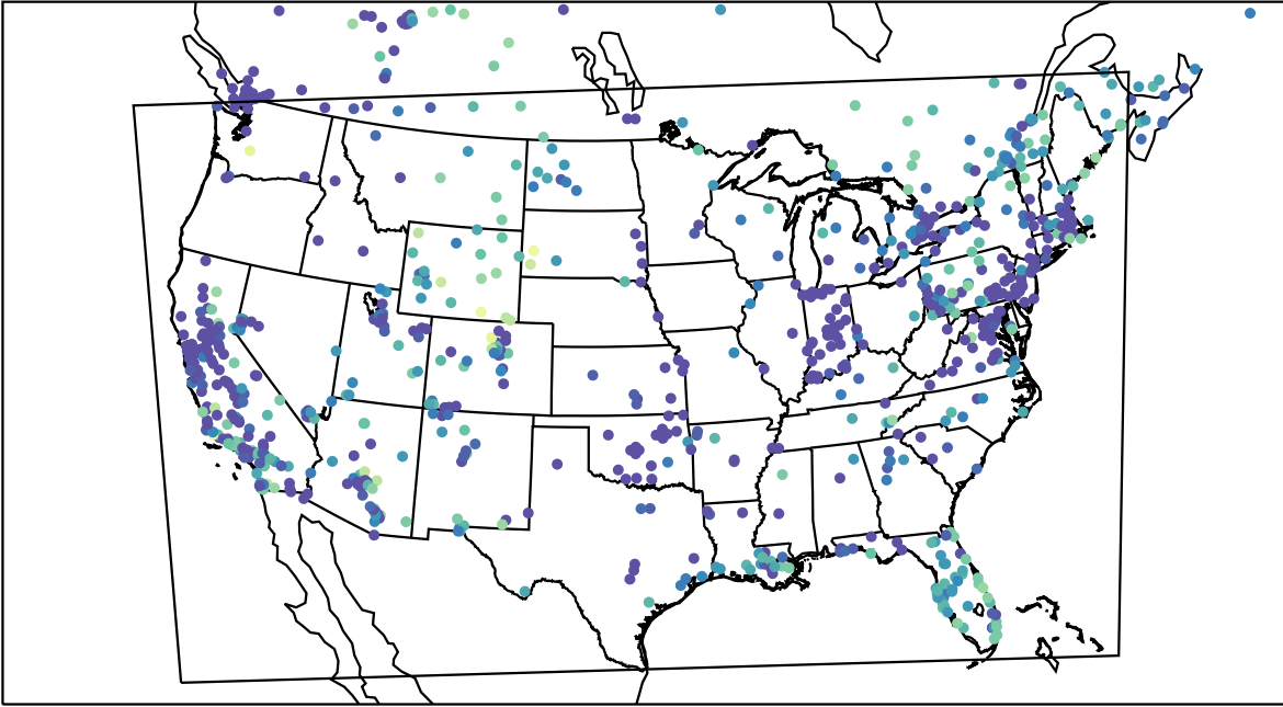
AirNOW (2023-11-26_04:00:00)
