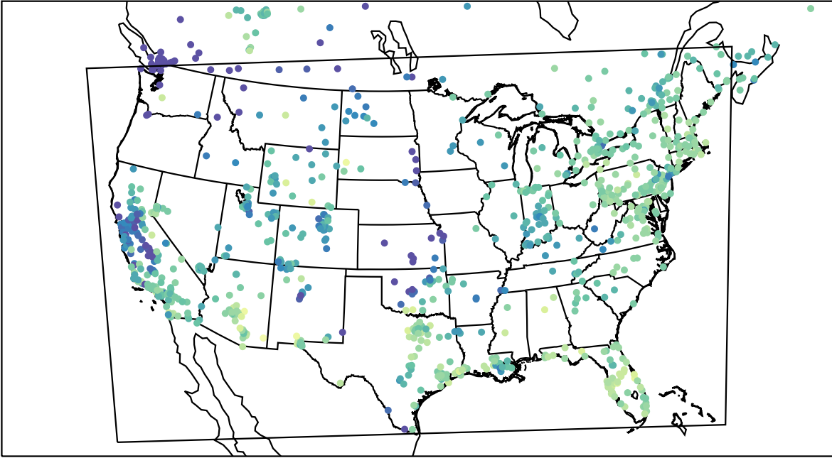
AirNOW (2023-11-25_18:00:00)
