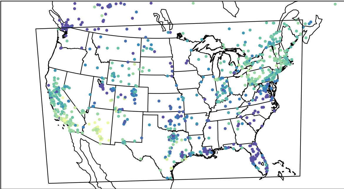
AirNOW (2023-11-25_00:00:00)
