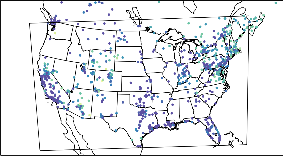
AirNOW (2023-11-25_10:00:00)
