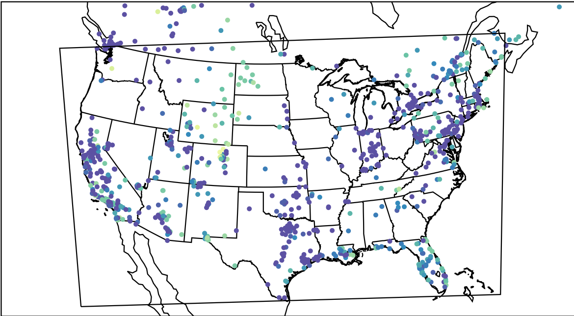
AirNOW (2023-11-26_07:00:00)
