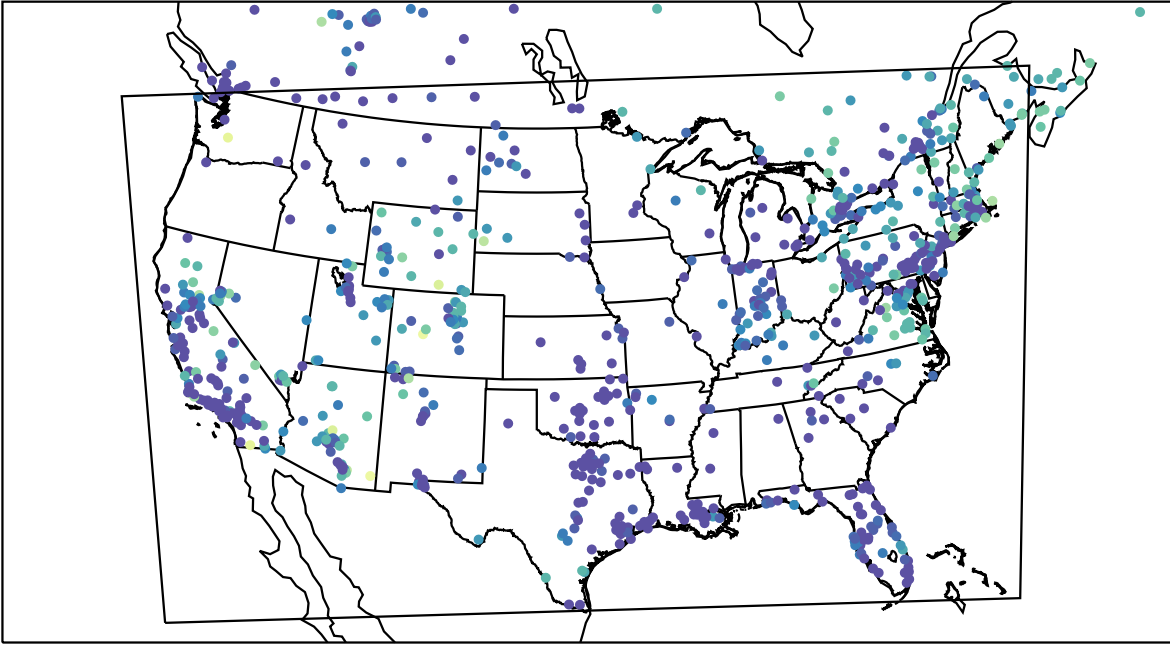
AirNOW (2023-11-25_11:00:00)
