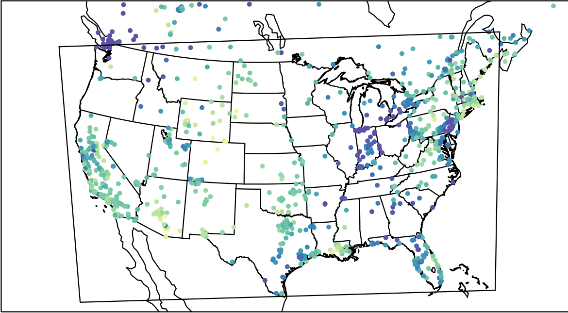
AirNOW (2023-11-26_20:00:00)
