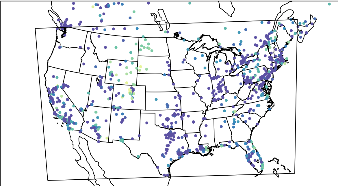
AirNOW (2023-11-26_12:00:00)
