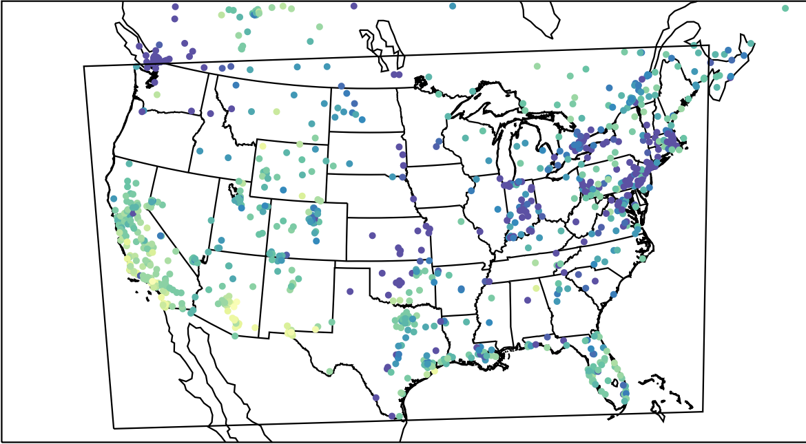
AirNOW (2023-11-25_23:00:00)
