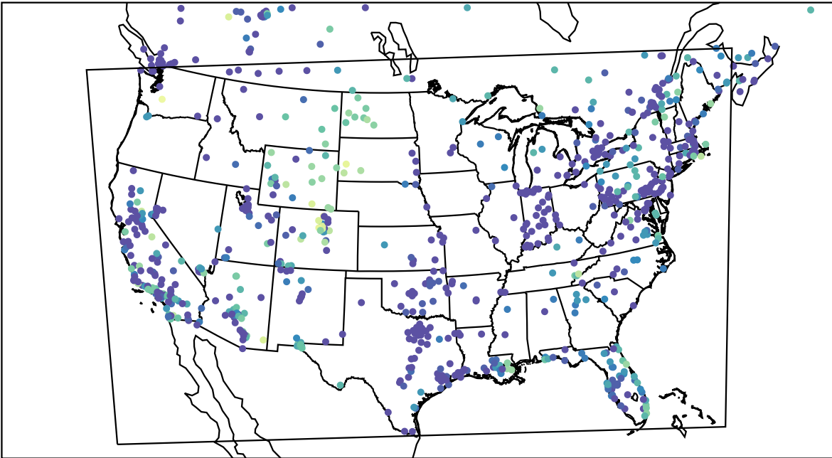
AirNOW (2023-11-26_11:00:00)
