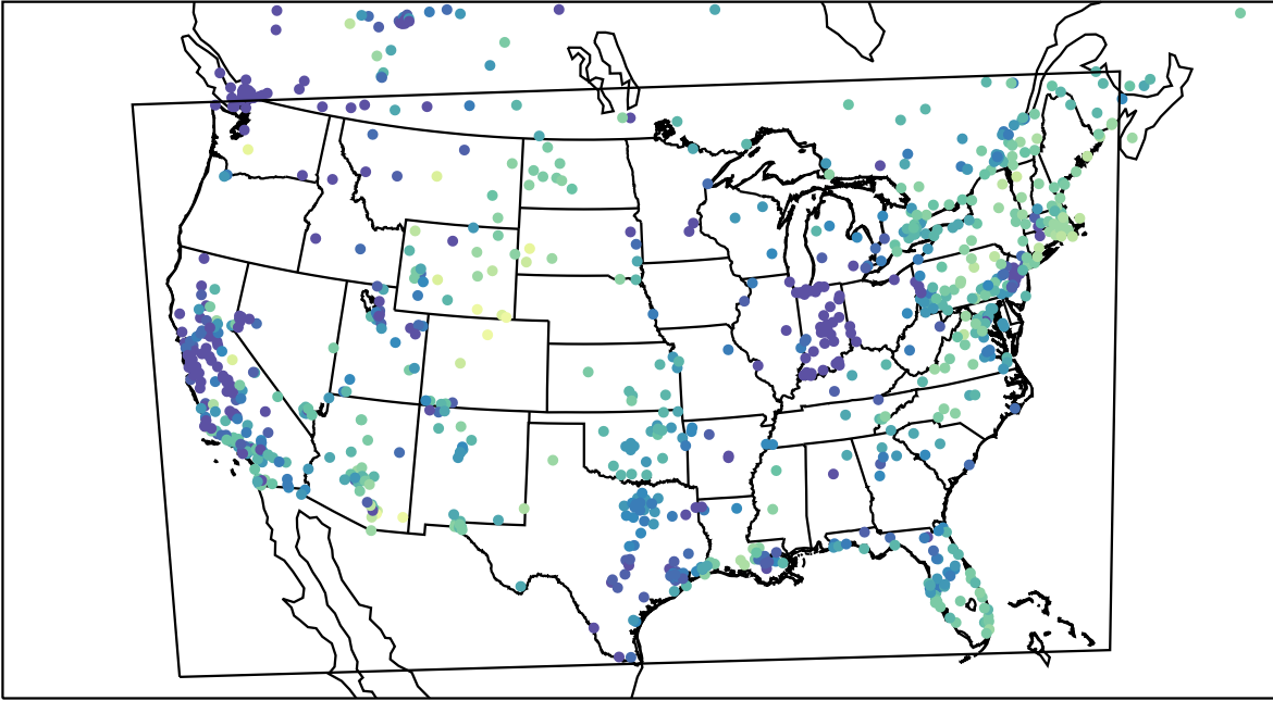
AirNOW (2023-11-26_17:00:00)
