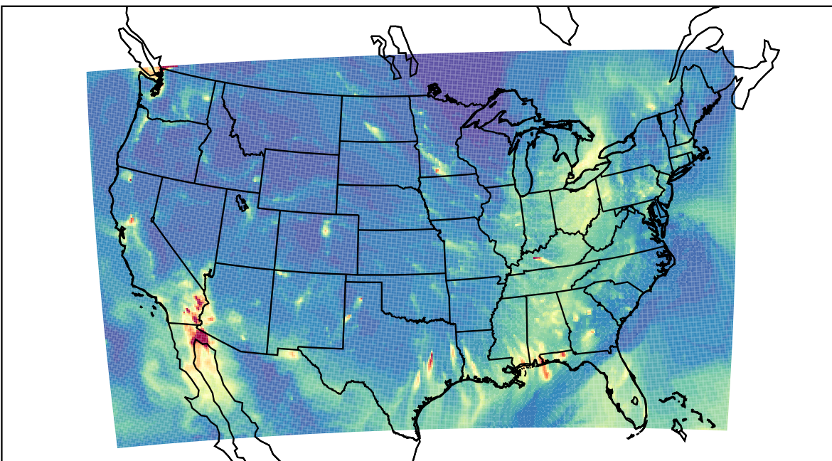
WRF 2023-11-27_04:00:00
