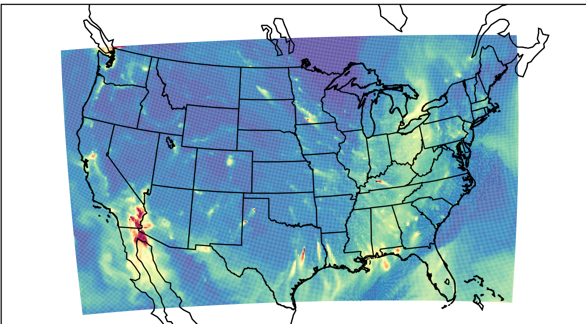
WRF 2023-11-27_05:00:00
