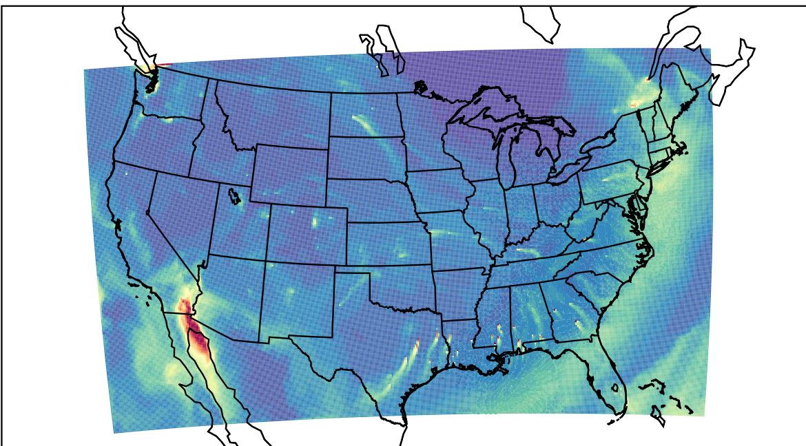
WRF 2023-11-27_20:00:00
