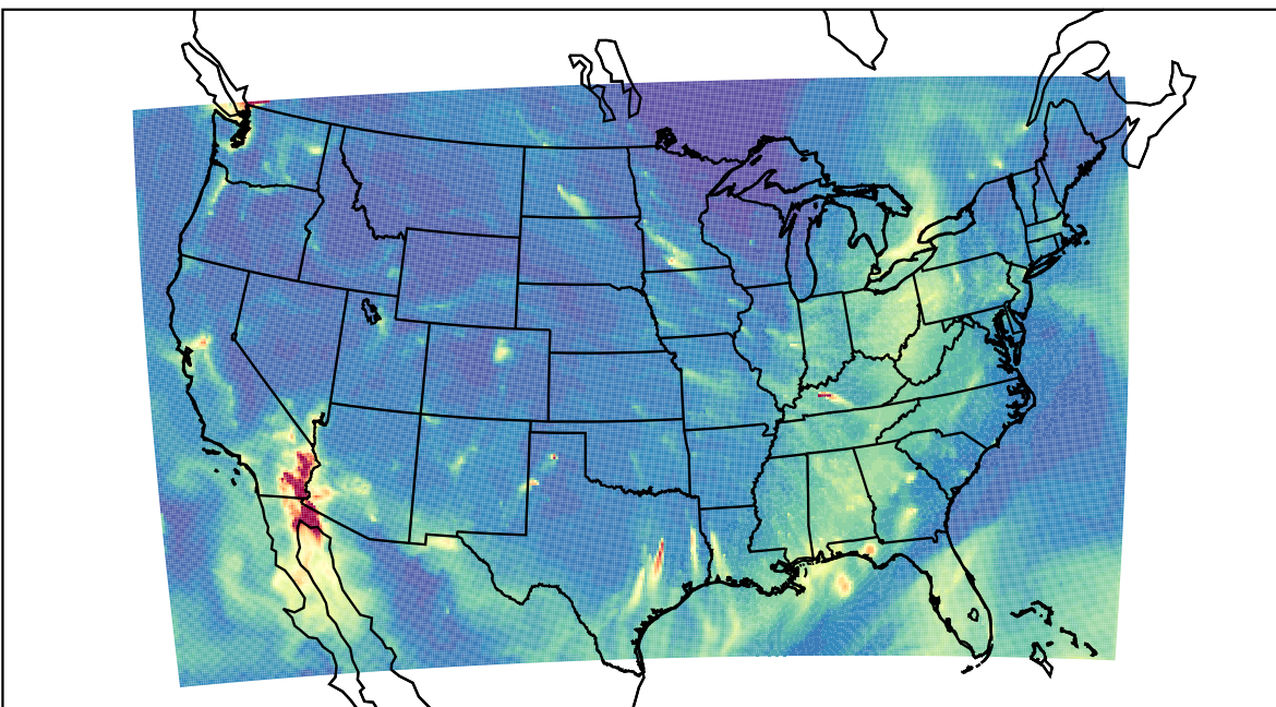
WRF 2023-11-27_06:00:00
