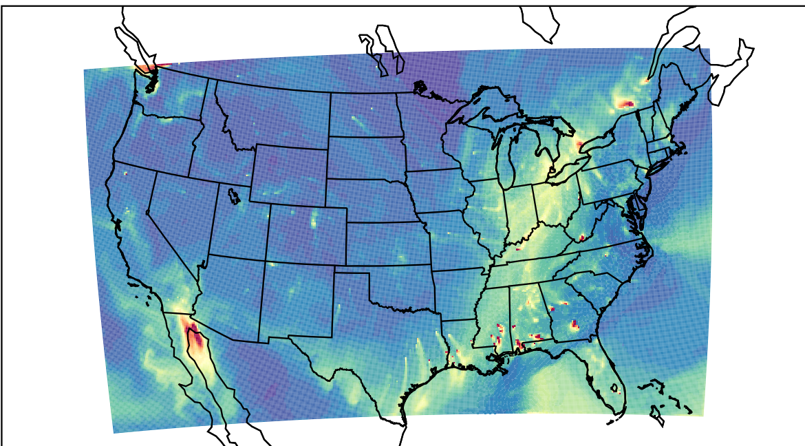
WRF 2023-11-26_22:00:00
