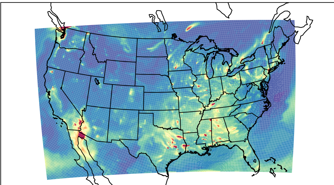
WRF 2023-11-26_03:00:00
