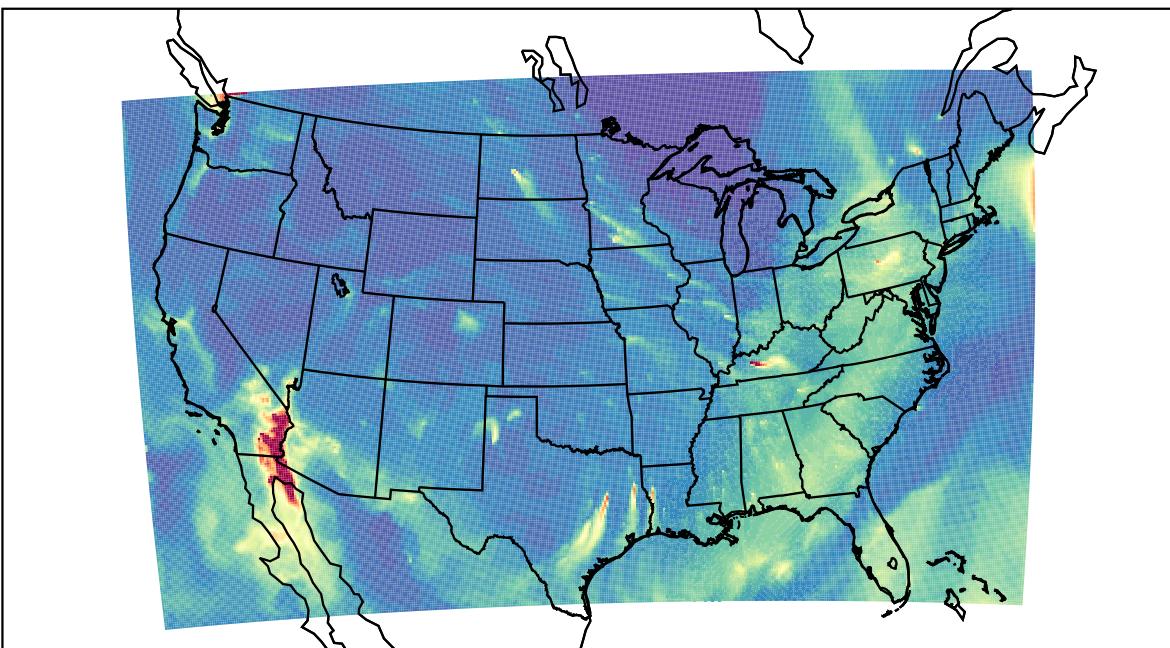
WRF 2023-11-27_11:00:00
