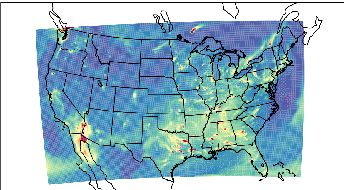
WRF 2023-11-26_02:00:00
