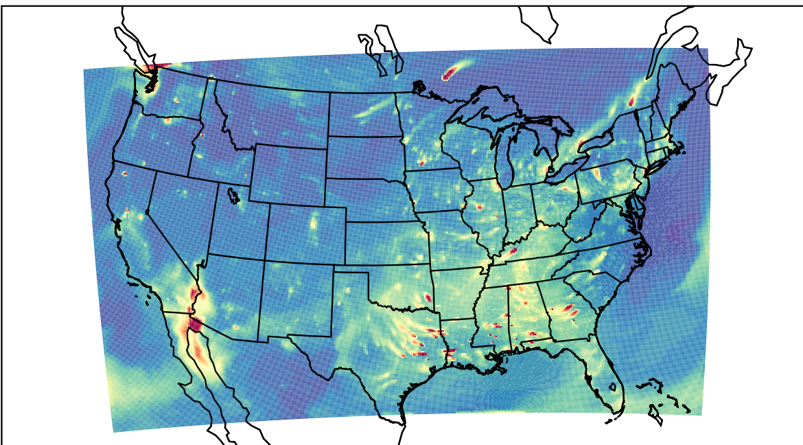
WRF 2023-11-26_01:00:00
