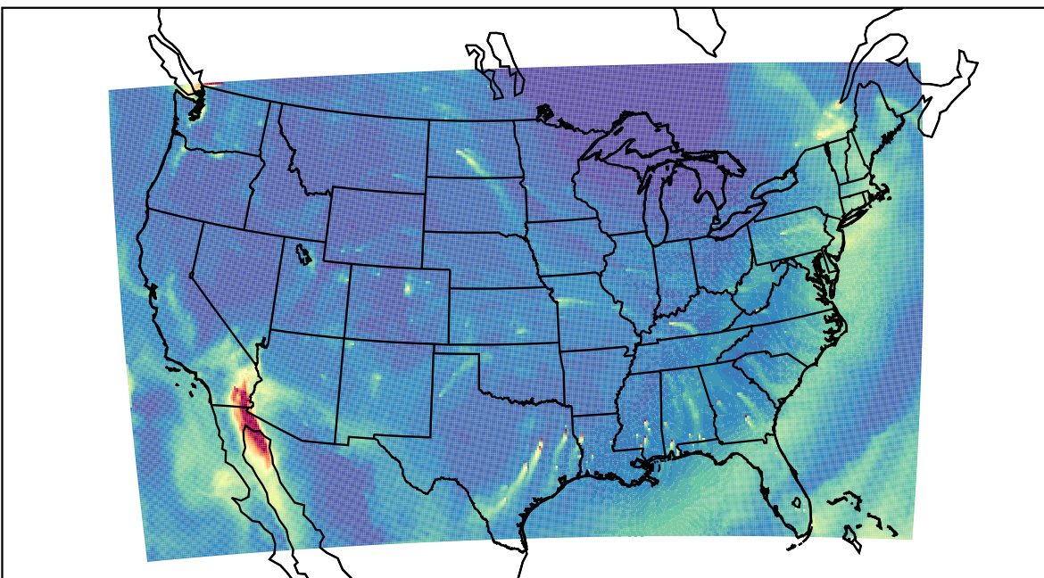
WRF 2023-11-27_19:00:00
