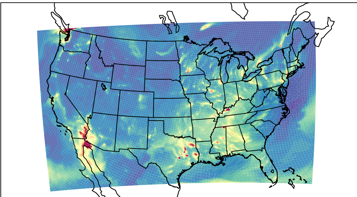
WRF 2023-11-26_05:00:00
