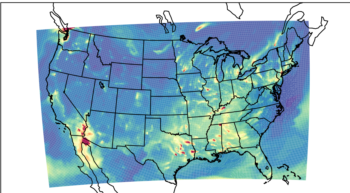
WRF 2023-11-26_04:00:00
