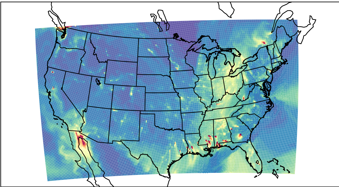
WRF 2023-11-27_00:00:00
