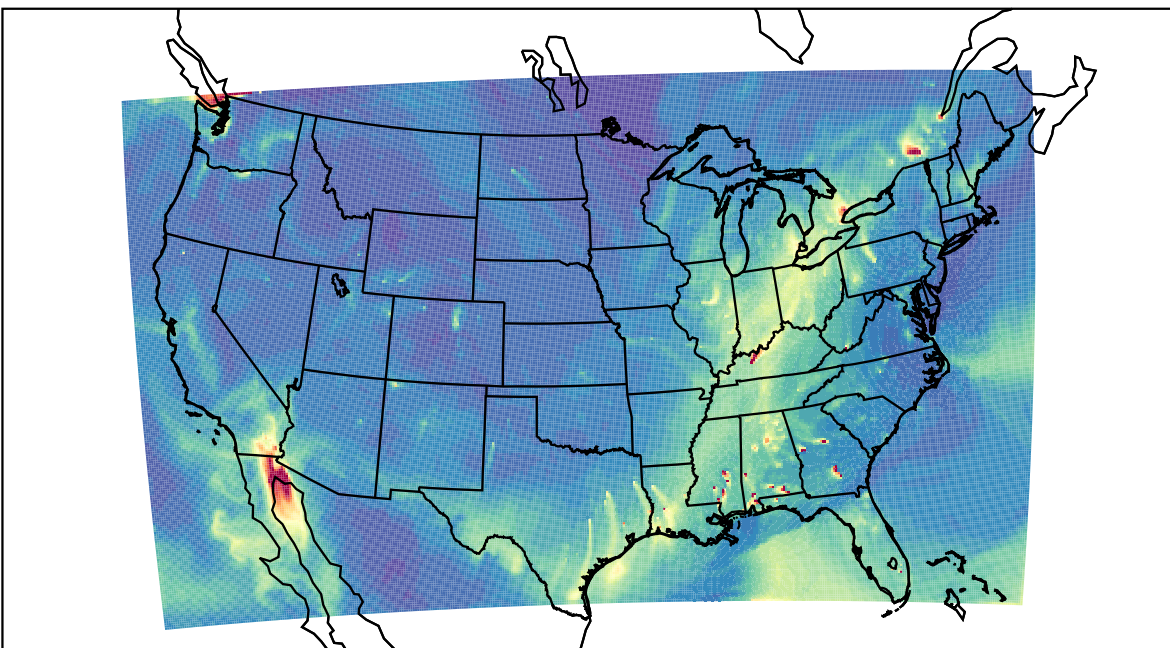
WRF 2023-11-26_20:00:00
