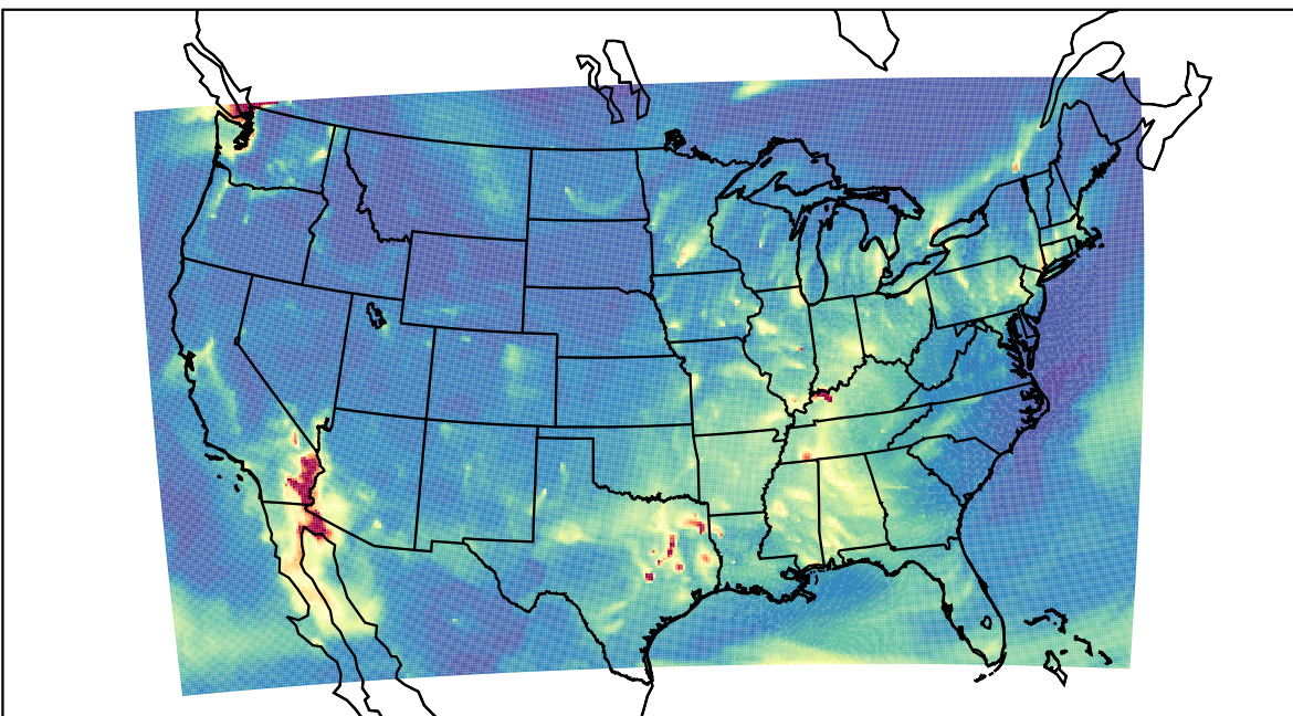
WRF 2023-11-26_07:00:00
