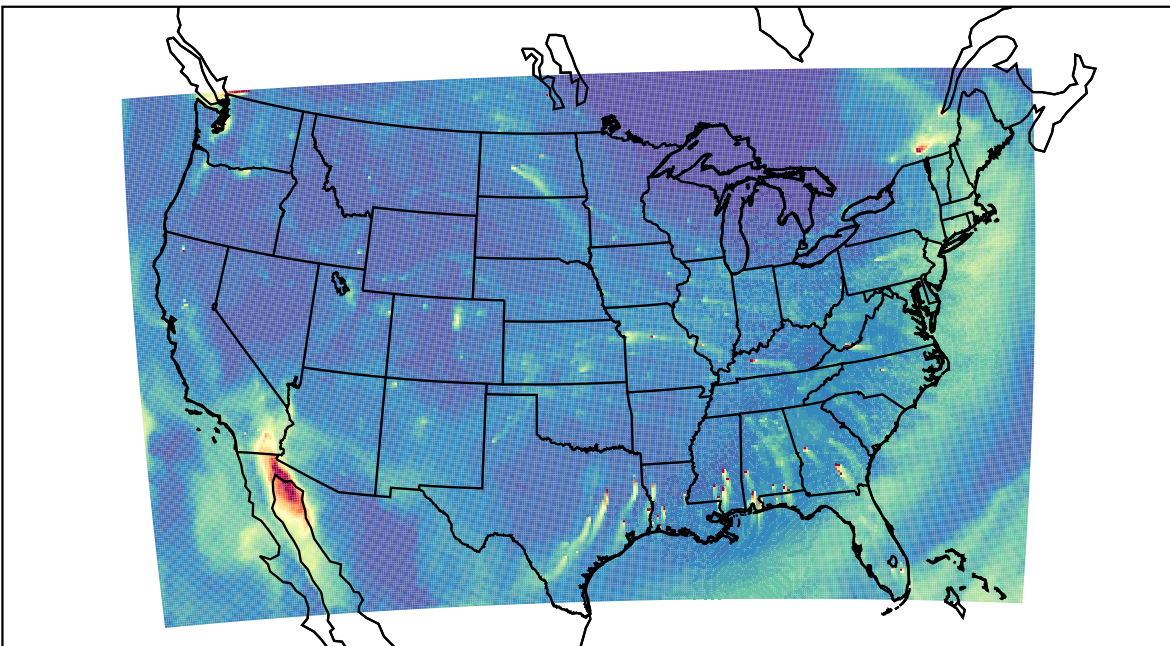
WRF 2023-11-27_22:00:00
