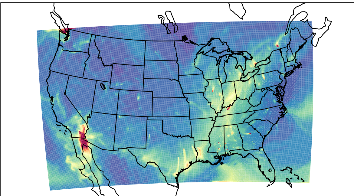
WRF 2023-11-26_17:00:00
