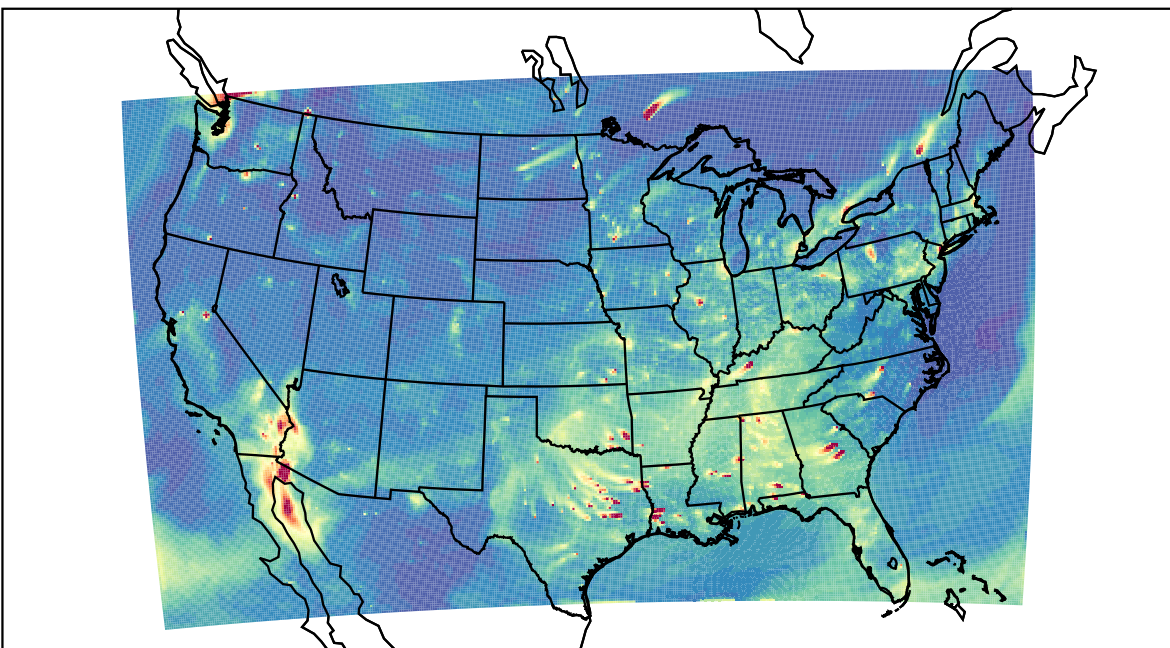
WRF 2023-11-26_00:00:00
