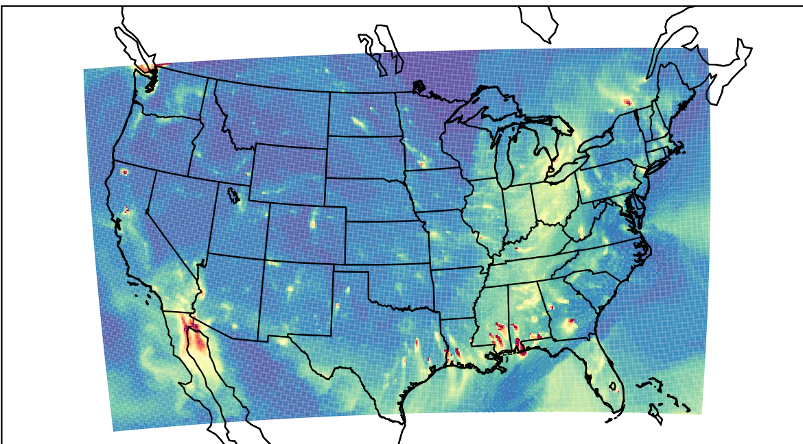
WRF 2023-11-27_01:00:00
