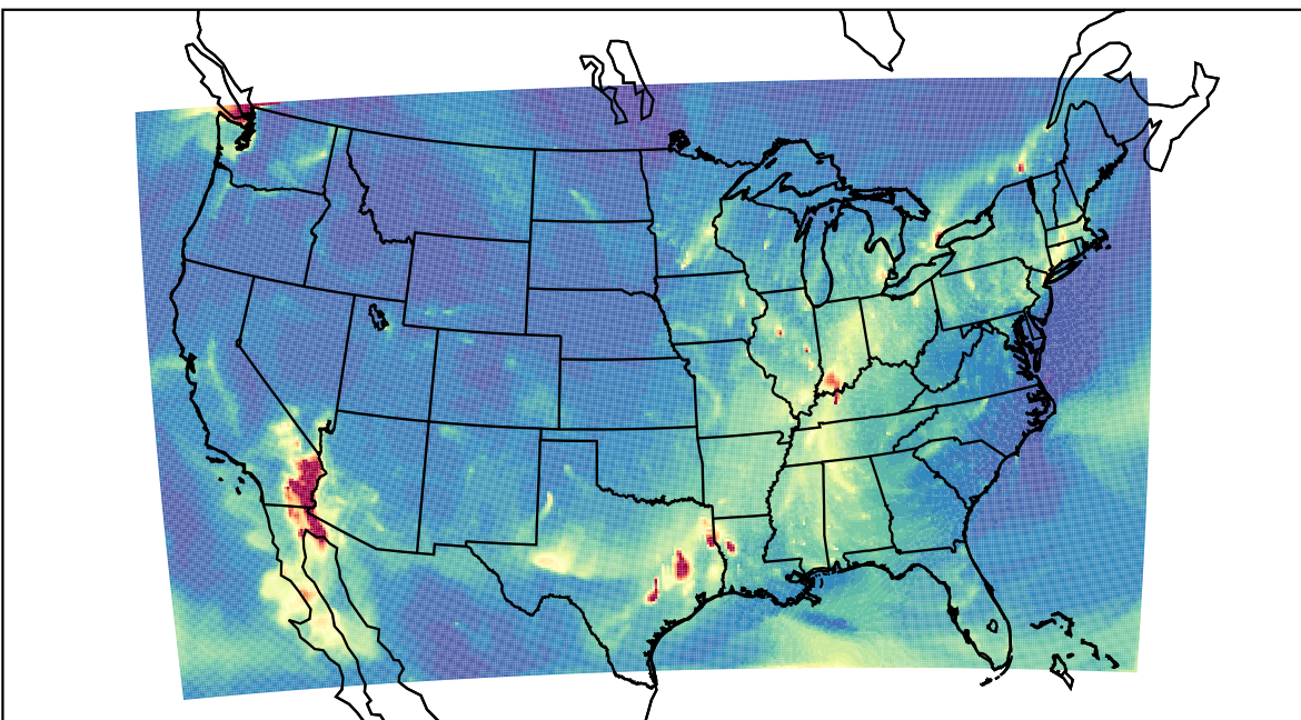
WRF 2023-11-26_12:00:00
