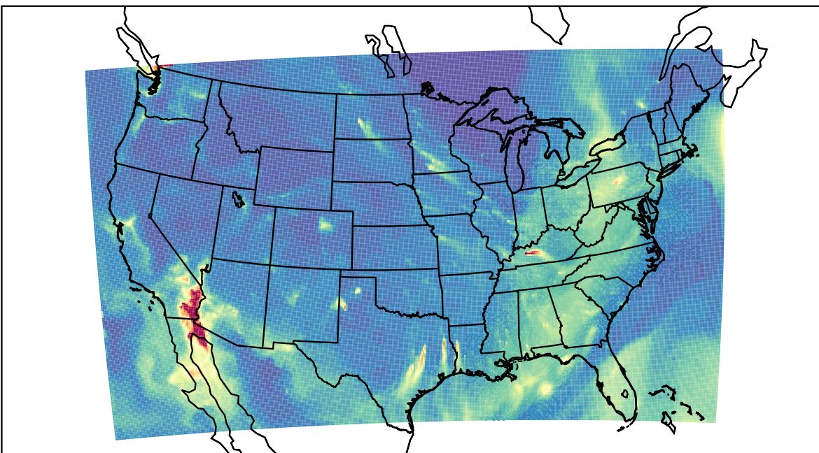
WRF 2023-11-27_09:00:00
