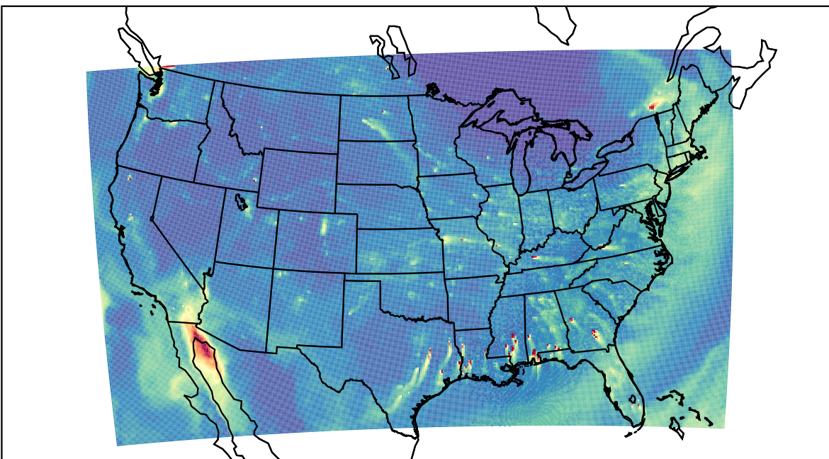
WRF 2023-11-27_23:00:00
