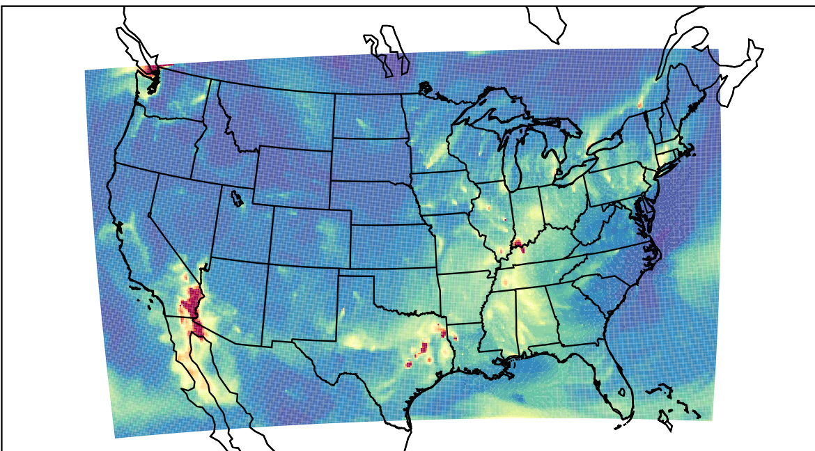
WRF 2023-11-26_09:00:00
