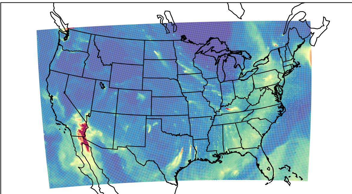
WRF 2023-11-27_12:00:00
