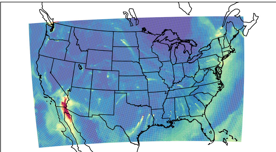
WRF 2023-11-27_18:00:00
