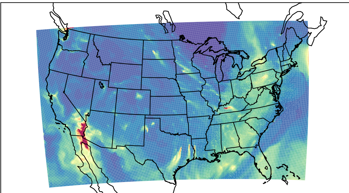
WRF 2023-11-27_10:00:00
