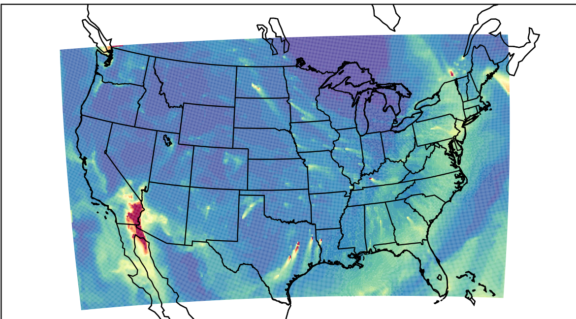
WRF 2023-11-27_15:00:00
