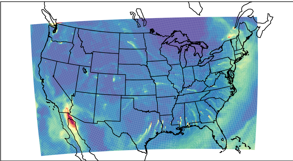
WRF 2023-11-27_21:00:00
