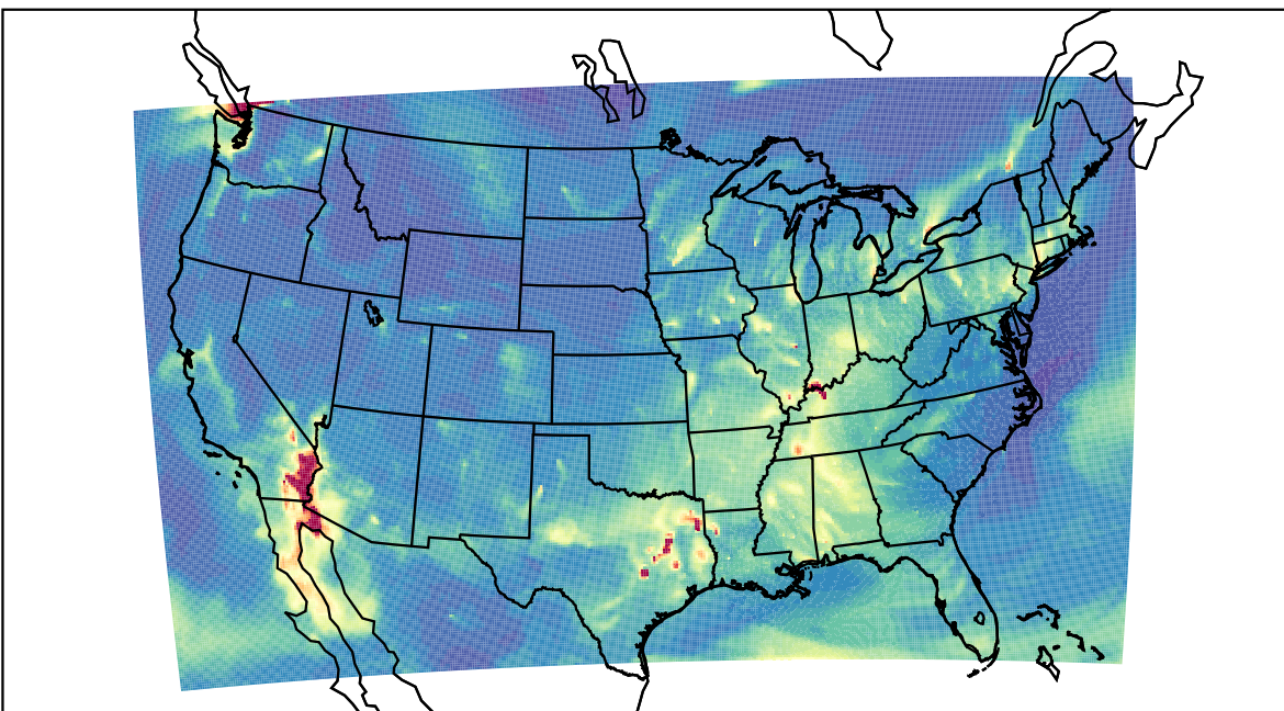
WRF 2023-11-26_08:00:00
