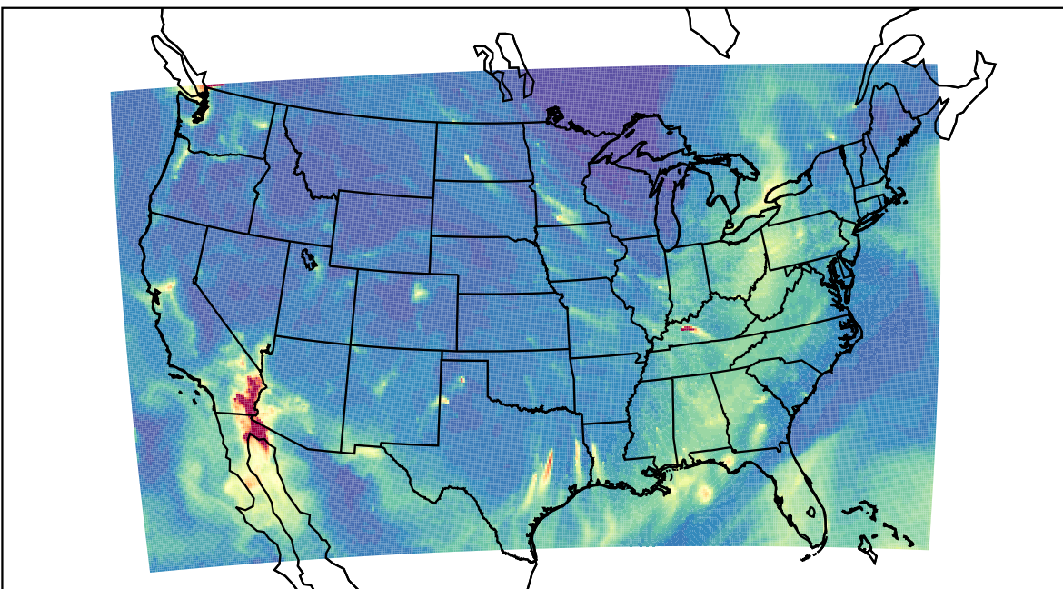
WRF 2023-11-27_07:00:00
