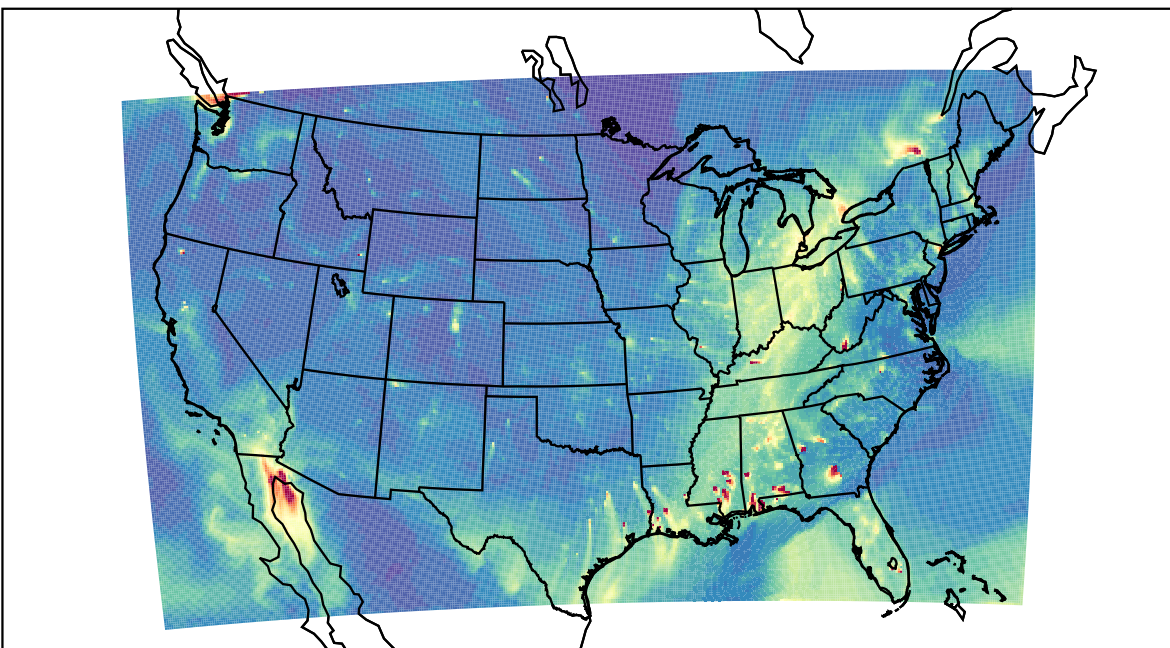
WRF 2023-11-26_23:00:00
