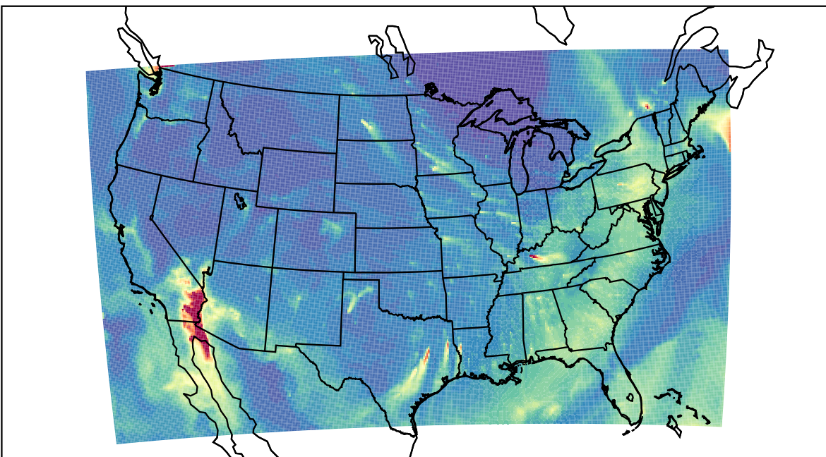
WRF 2023-11-27_13:00:00
