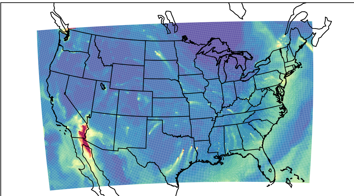
WRF 2023-11-27_17:00:00
