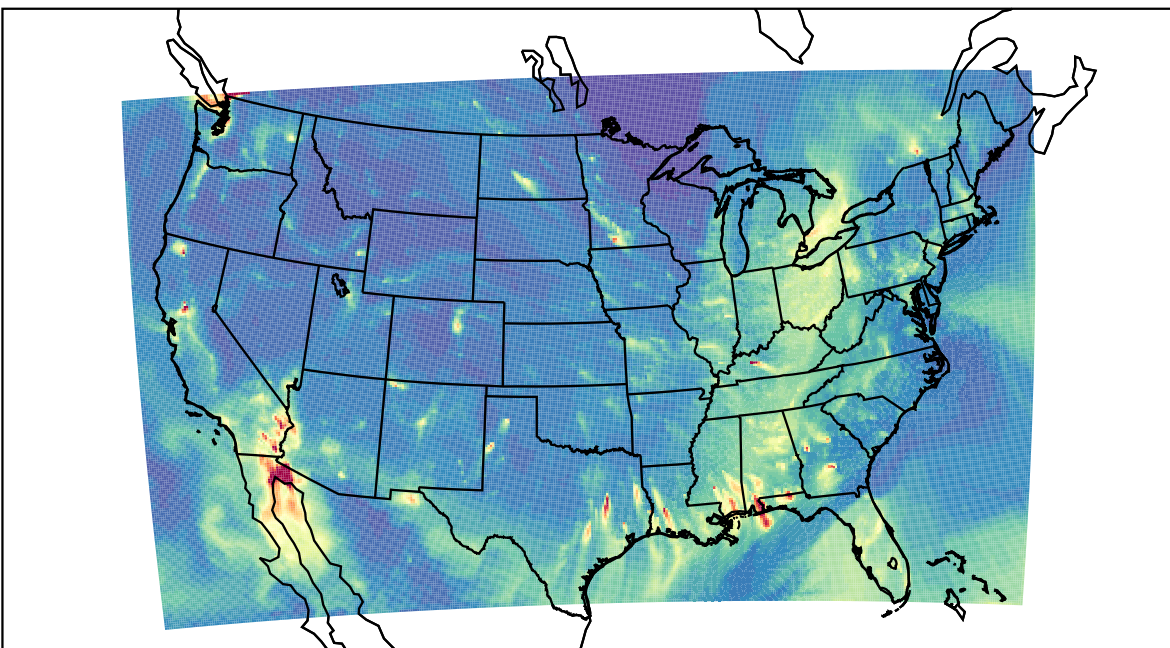
WRF 2023-11-27_03:00:00
