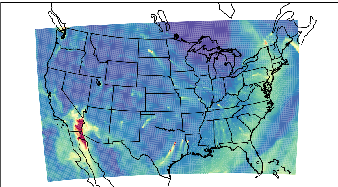
WRF 2023-11-27_16:00:00
