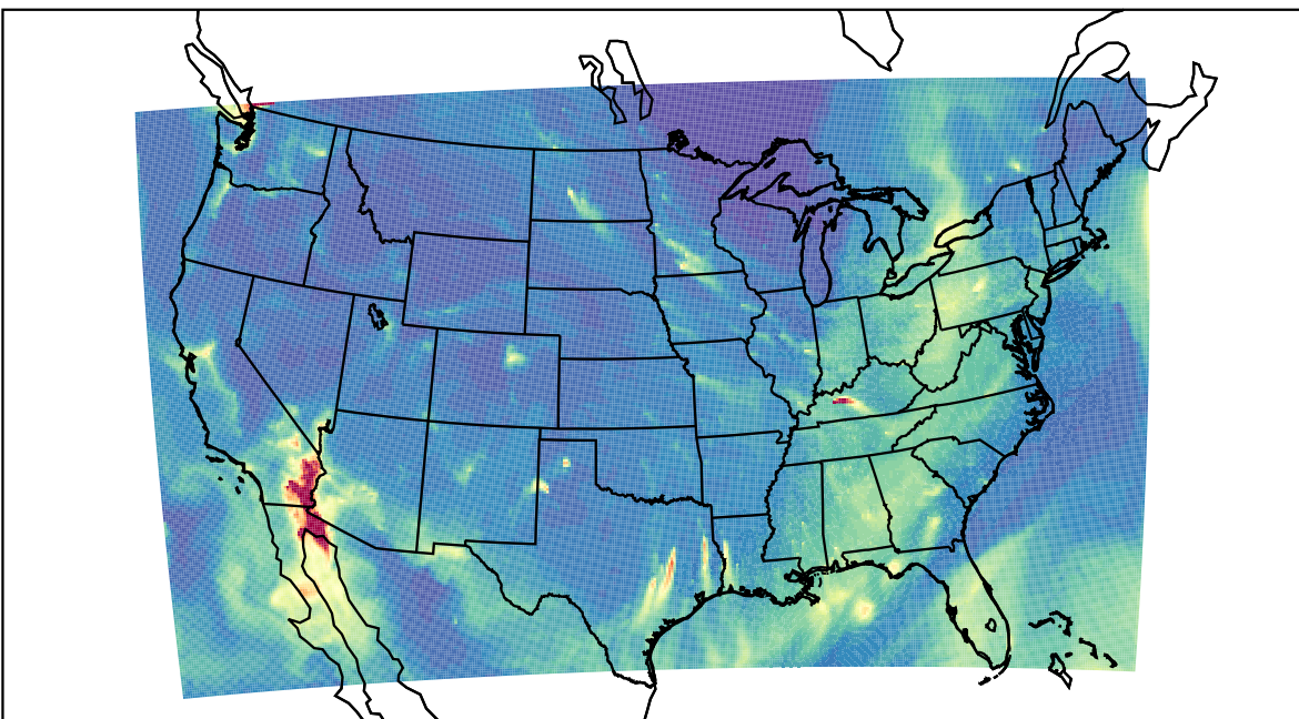
WRF 2023-11-27_08:00:00
