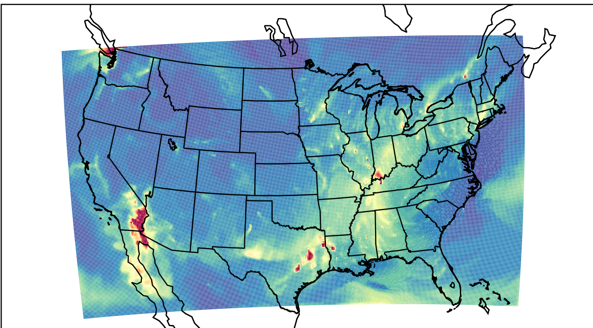
WRF 2023-11-26_11:00:00
