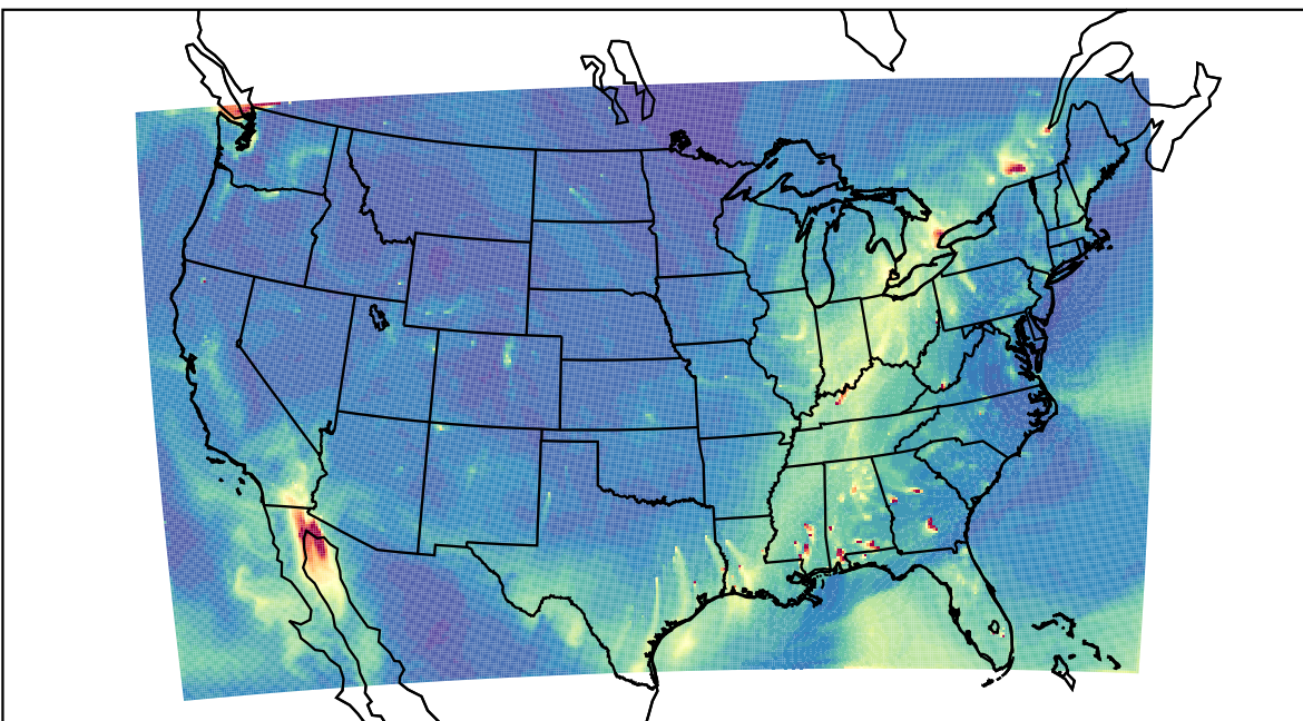
WRF 2023-11-26_21:00:00
