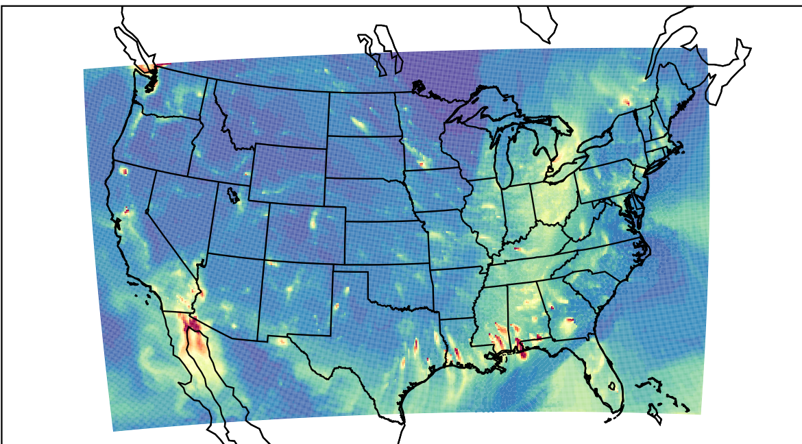
WRF 2023-11-27_02:00:00
