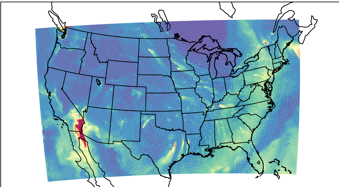
WRF 2023-11-27_14:00:00
