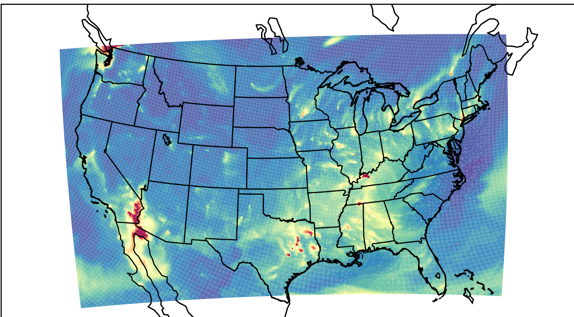
WRF 2023-11-26_06:00:00
