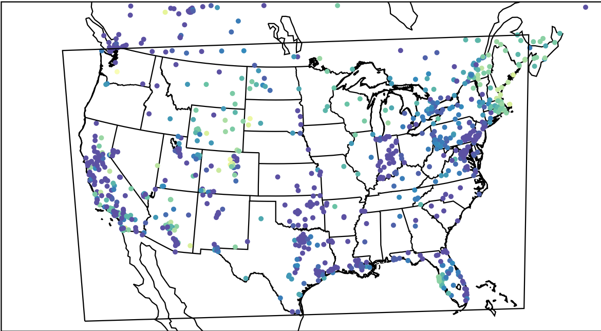
AirNOW (2023-11-27_09:00:00)
