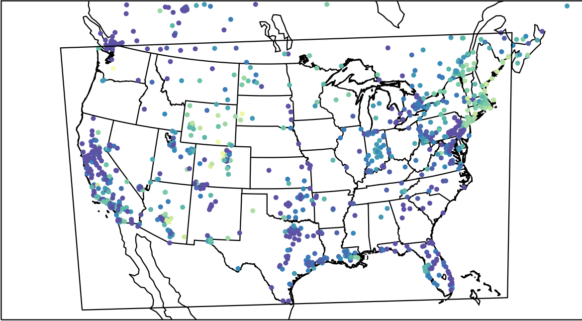
AirNOW (2023-11-27_03:00:00)
