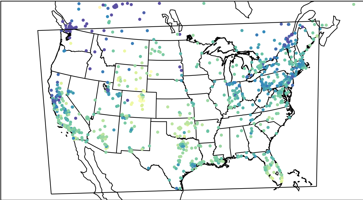
AirNOW (2023-11-27_19:00:00)
