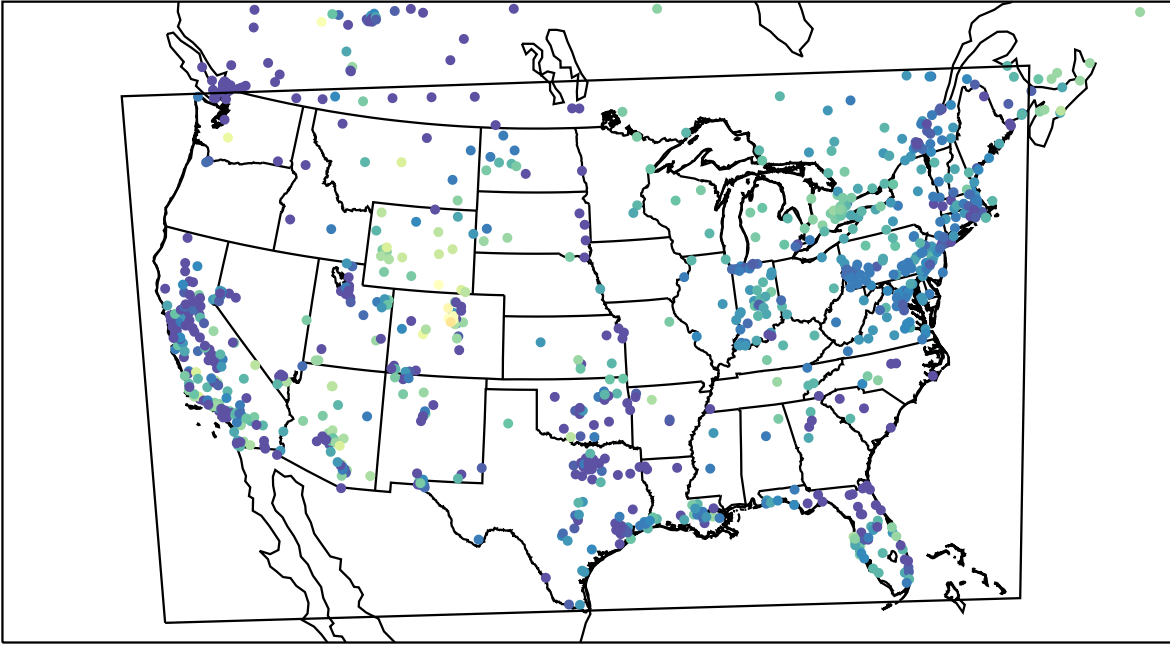
AirNOW (2023-11-28_01:00:00)
