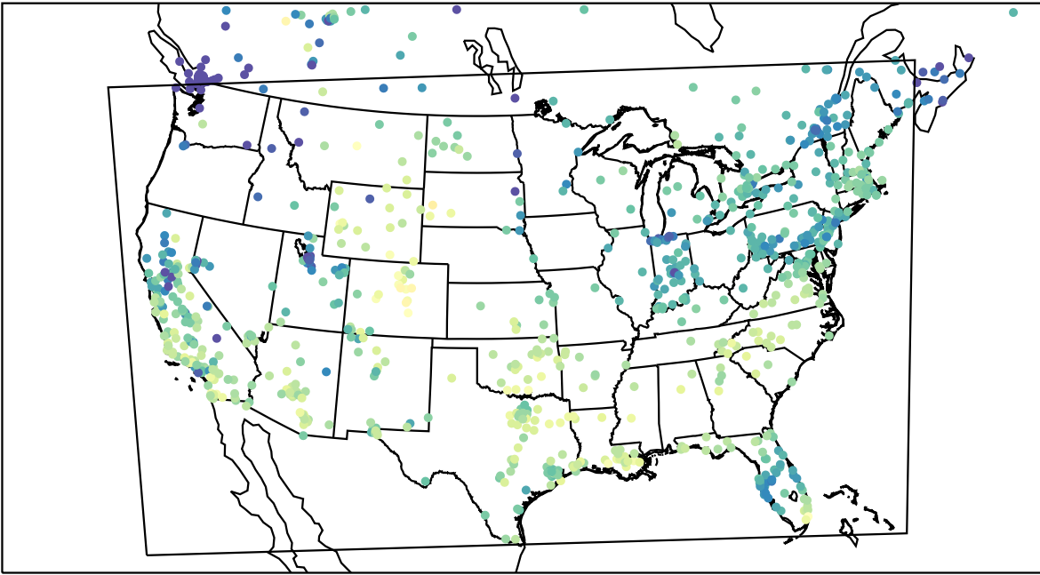
AirNOW (2023-11-28_20:00:00)
