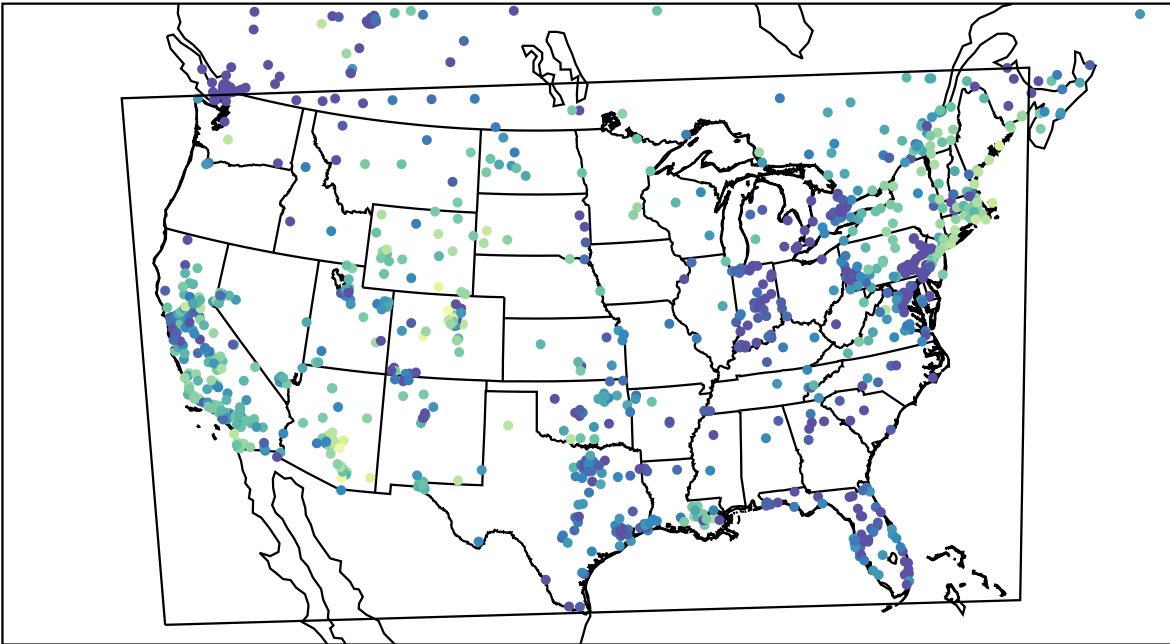
AirNOW (2023-11-27_00:00:00)
