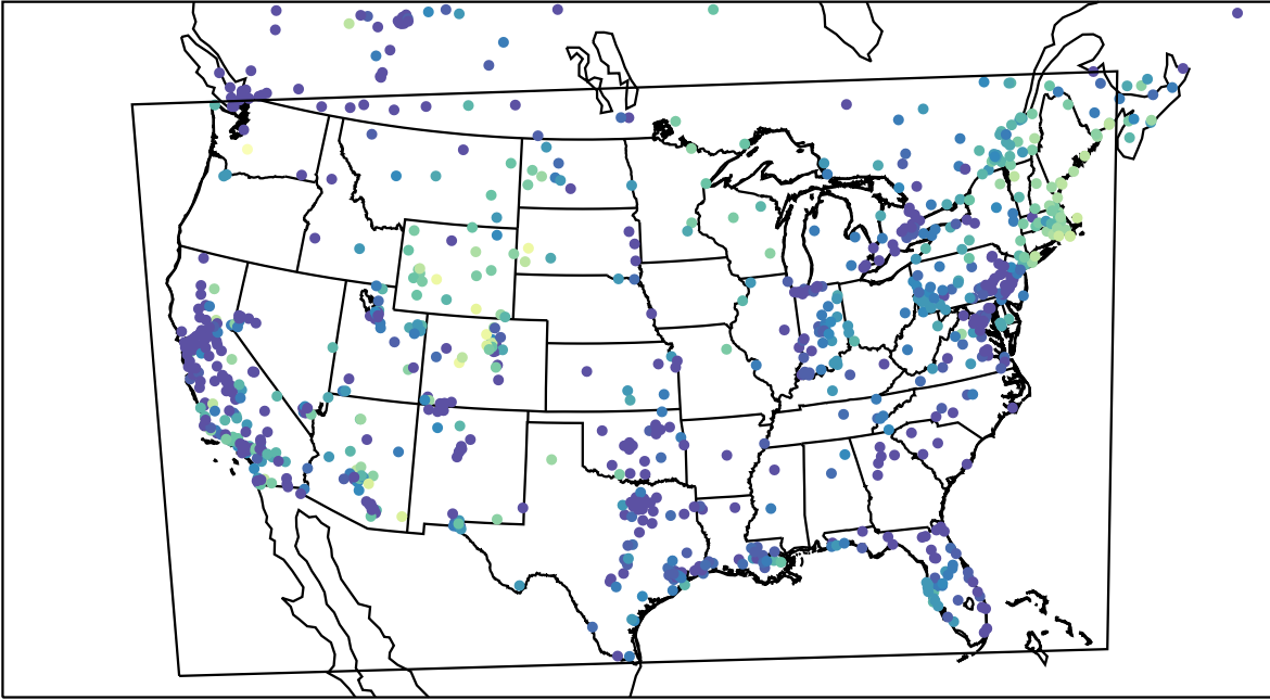
AirNOW (2023-11-27_05:00:00)
