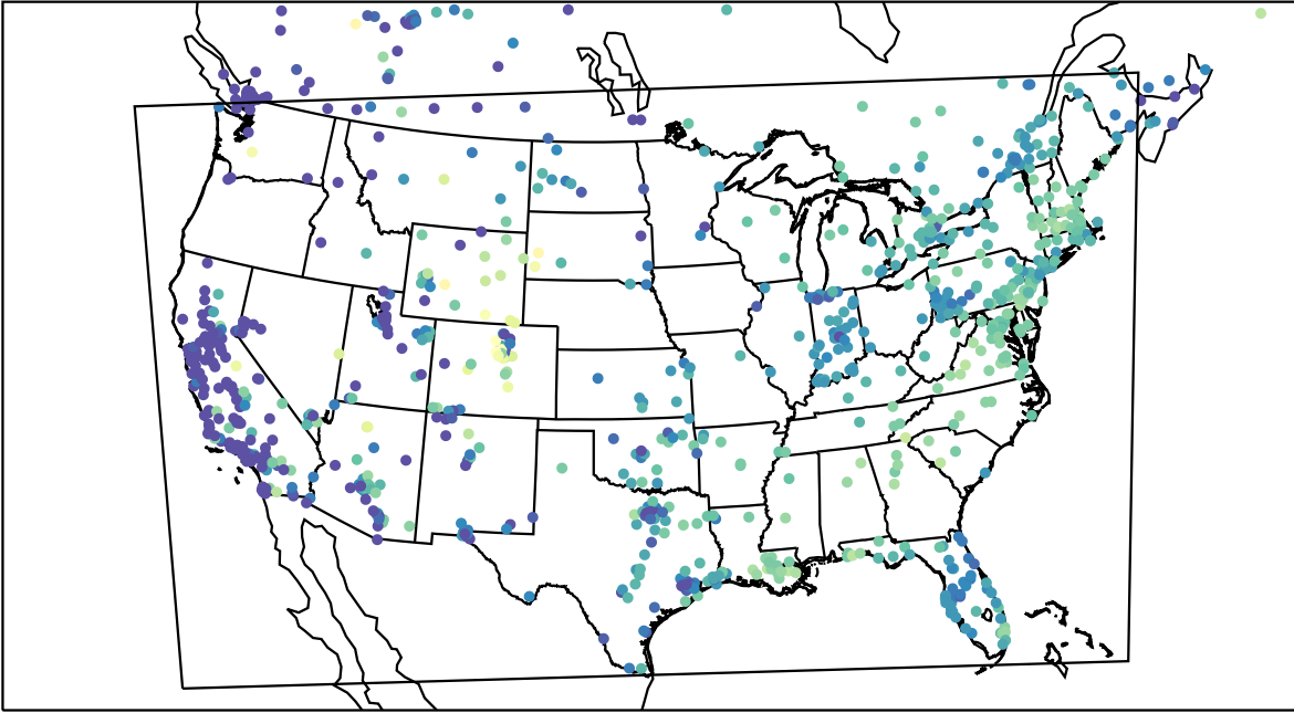
AirNOW (2023-11-28_16:00:00)
