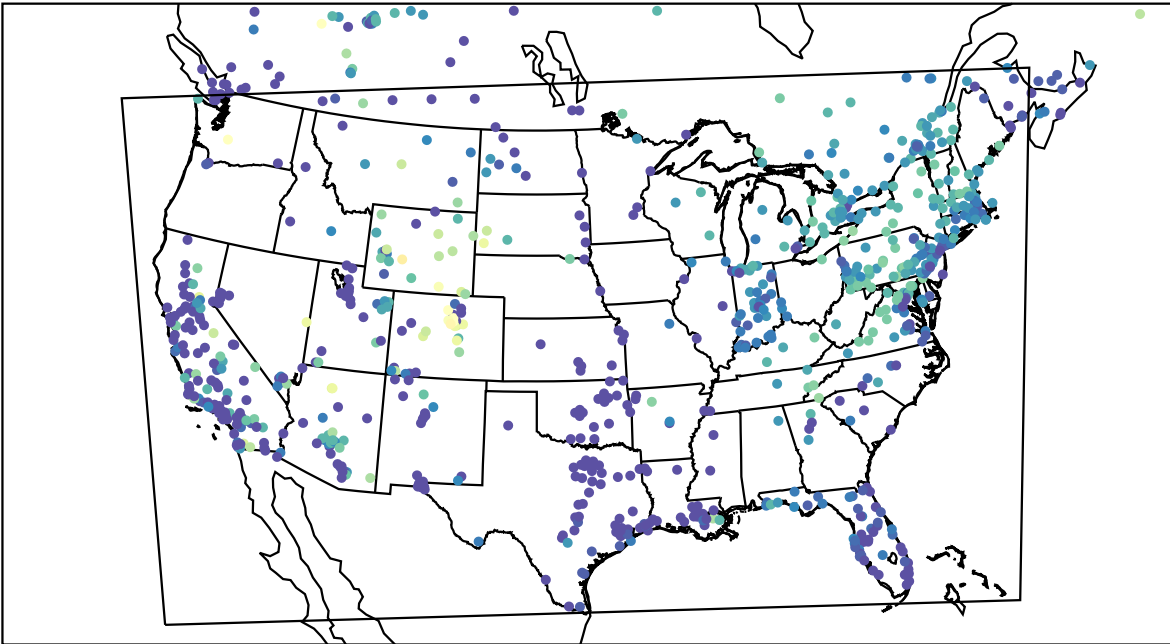
AirNOW (2023-11-28_13:00:00)
