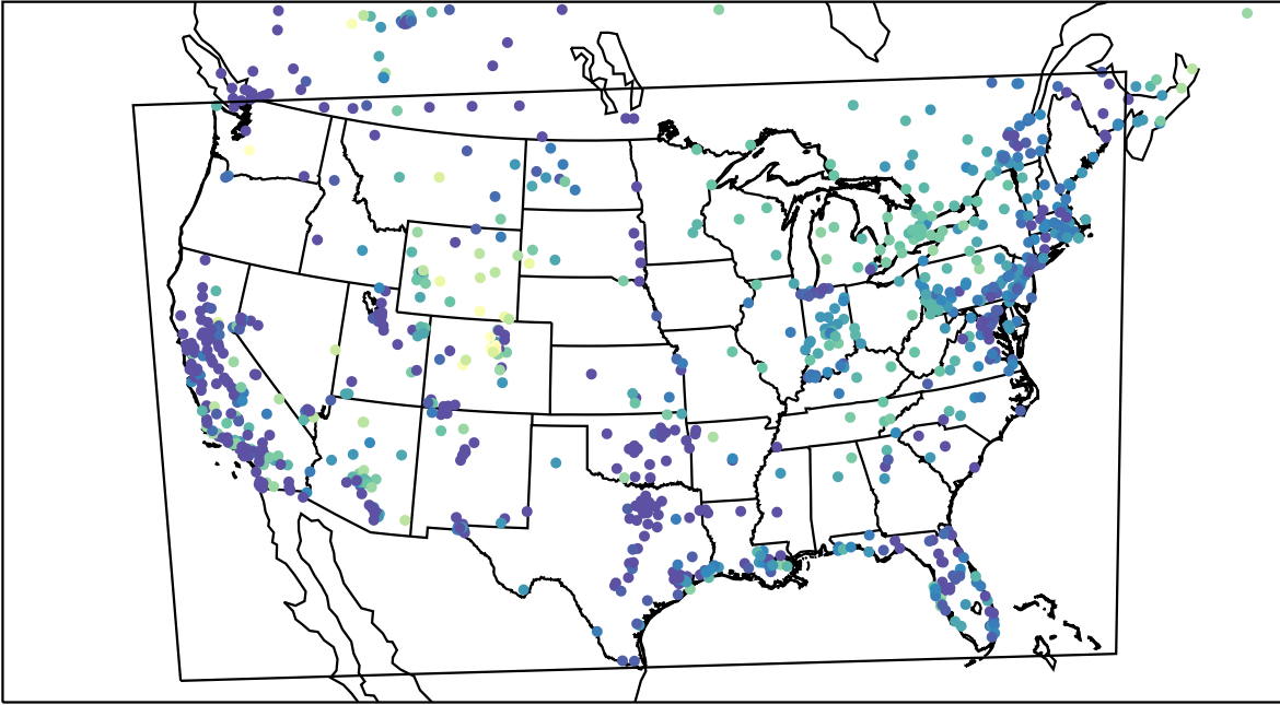
AirNOW (2023-11-28_04:00:00)
