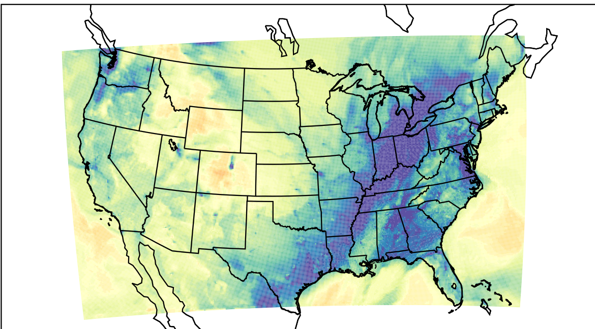
WRF (2023-11-27_00:00:00)
