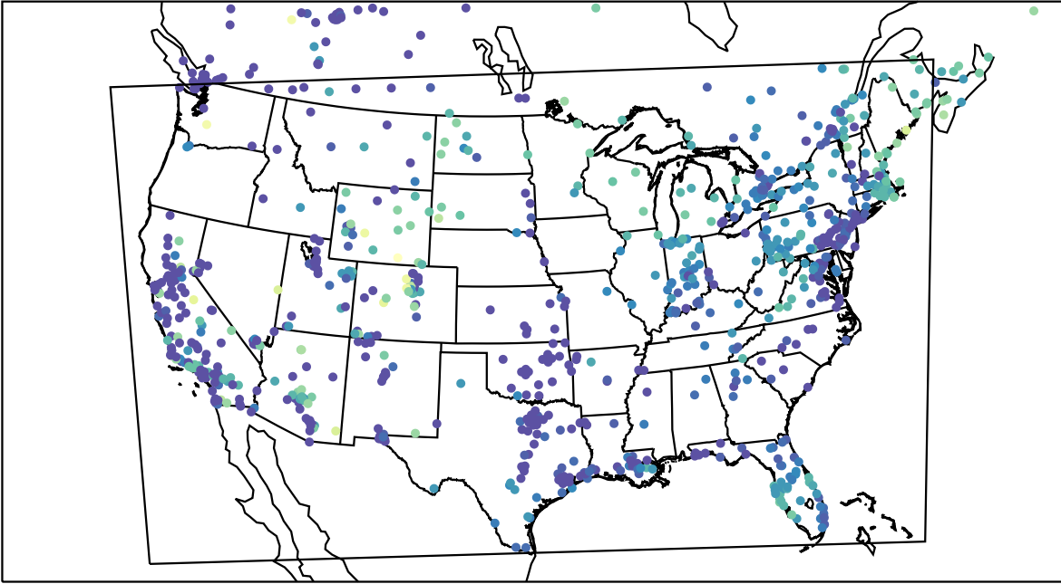
AirNOW (2023-11-27_14:00:00)
