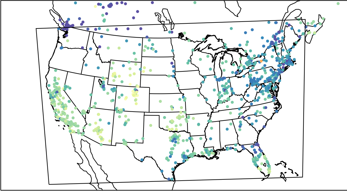
AirNOW (2023-11-27_22:00:00)
