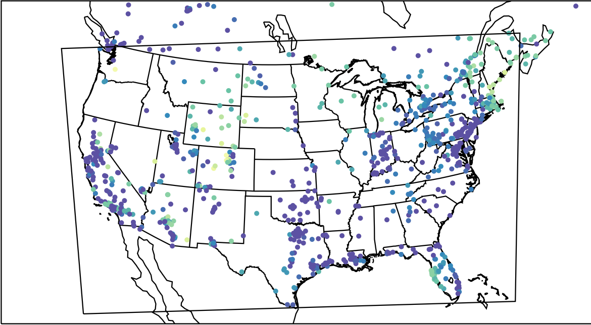
AirNOW (2023-11-27_10:00:00)
