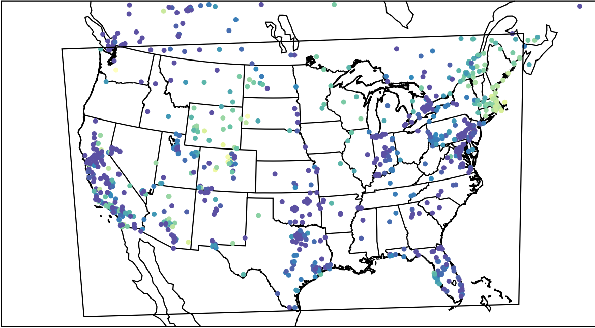
AirNOW (2023-11-27_07:00:00)
