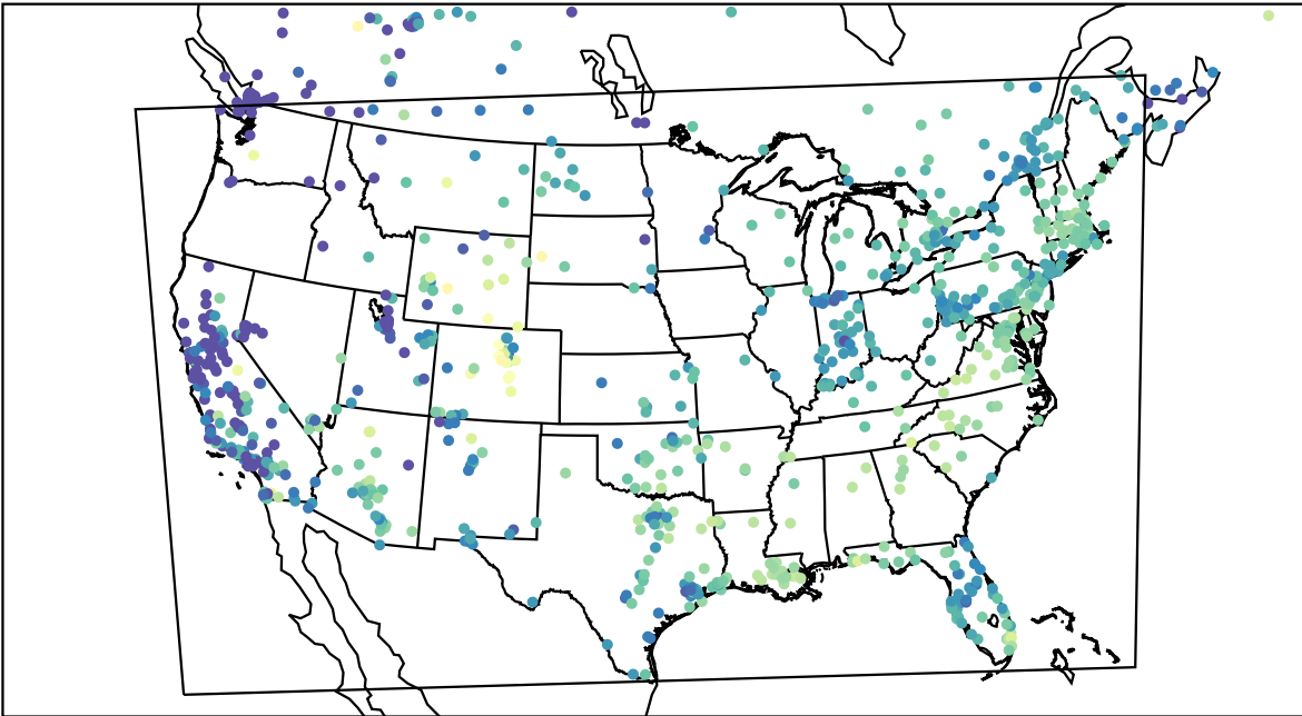
AirNOW (2023-11-28_17:00:00)
