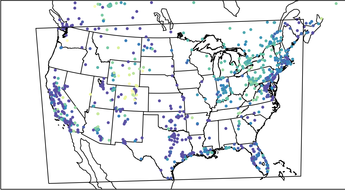
AirNOW (2023-11-28_08:00:00)
