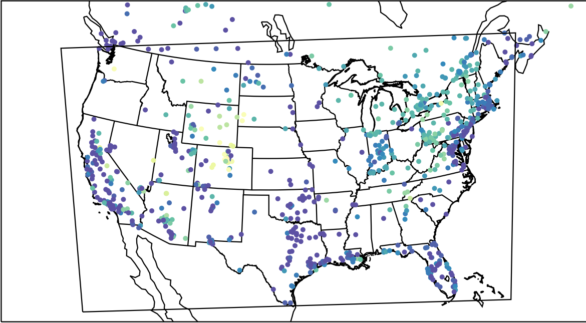
AirNOW (2023-11-28_10:00:00)
