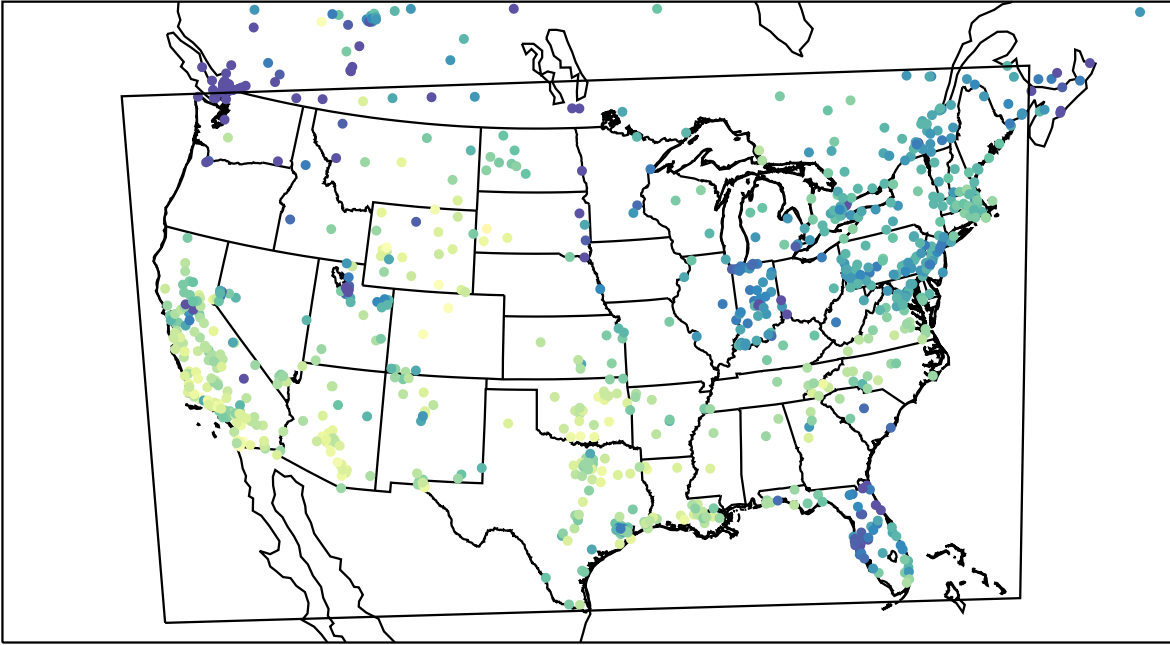
AirNOW (2023-11-28_22:00:00)
