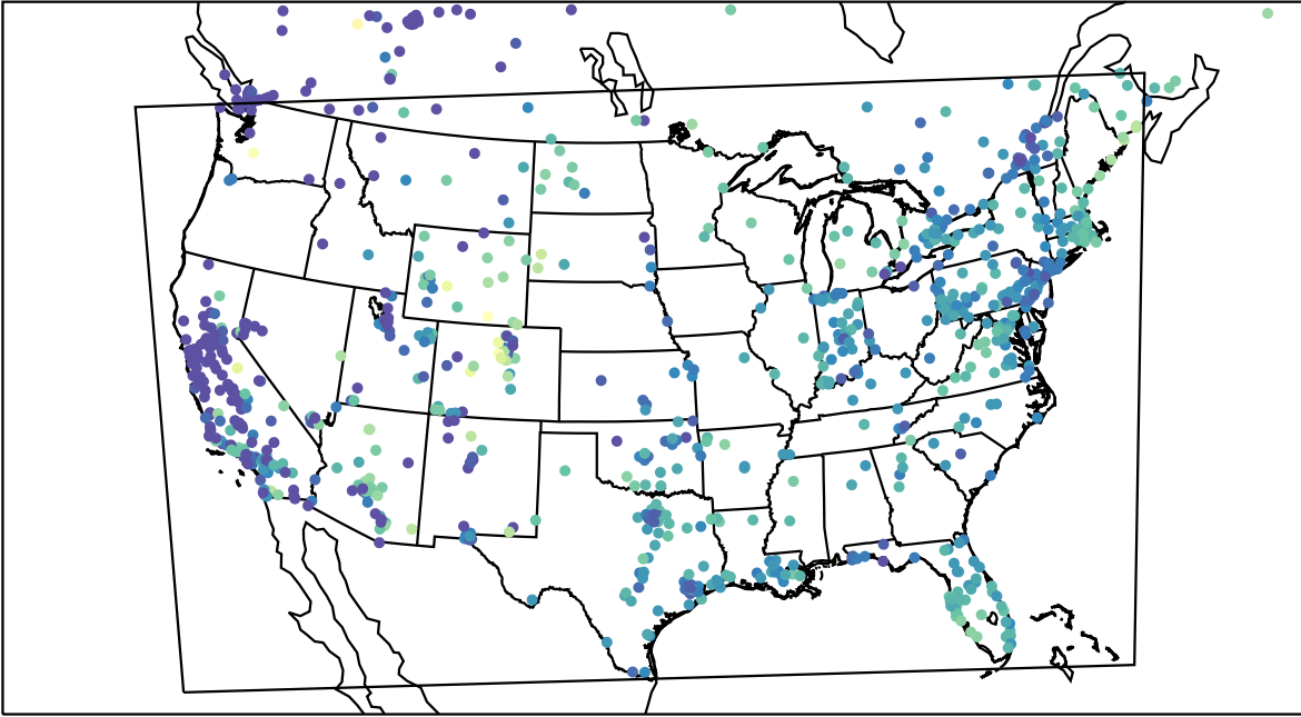
AirNOW (2023-11-27_16:00:00)
