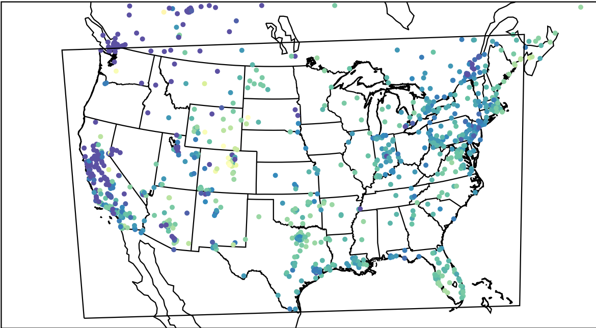
AirNOW (2023-11-27_17:00:00)
