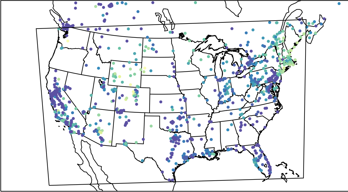
AirNOW (2023-11-27_04:00:00)
