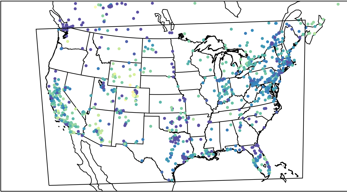
AirNOW (2023-11-28_00:00:00)
