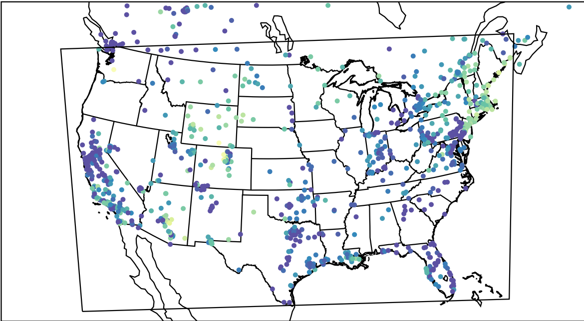
AirNOW (2023-11-27_02:00:00)
