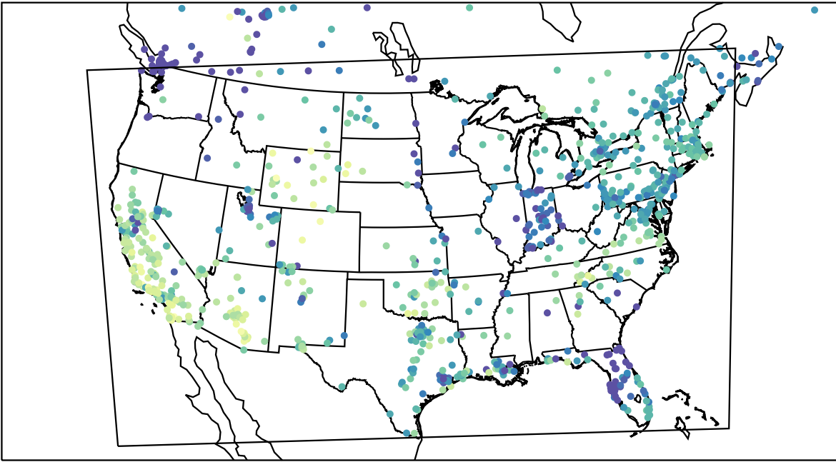
AirNOW (2023-11-28_23:00:00)
