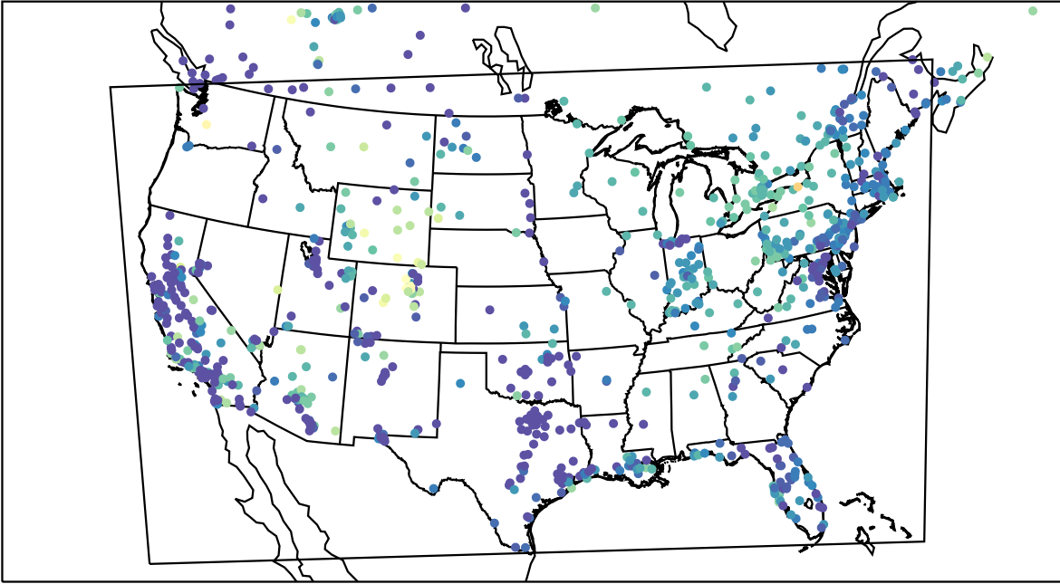
AirNOW (2023-11-28_05:00:00)
