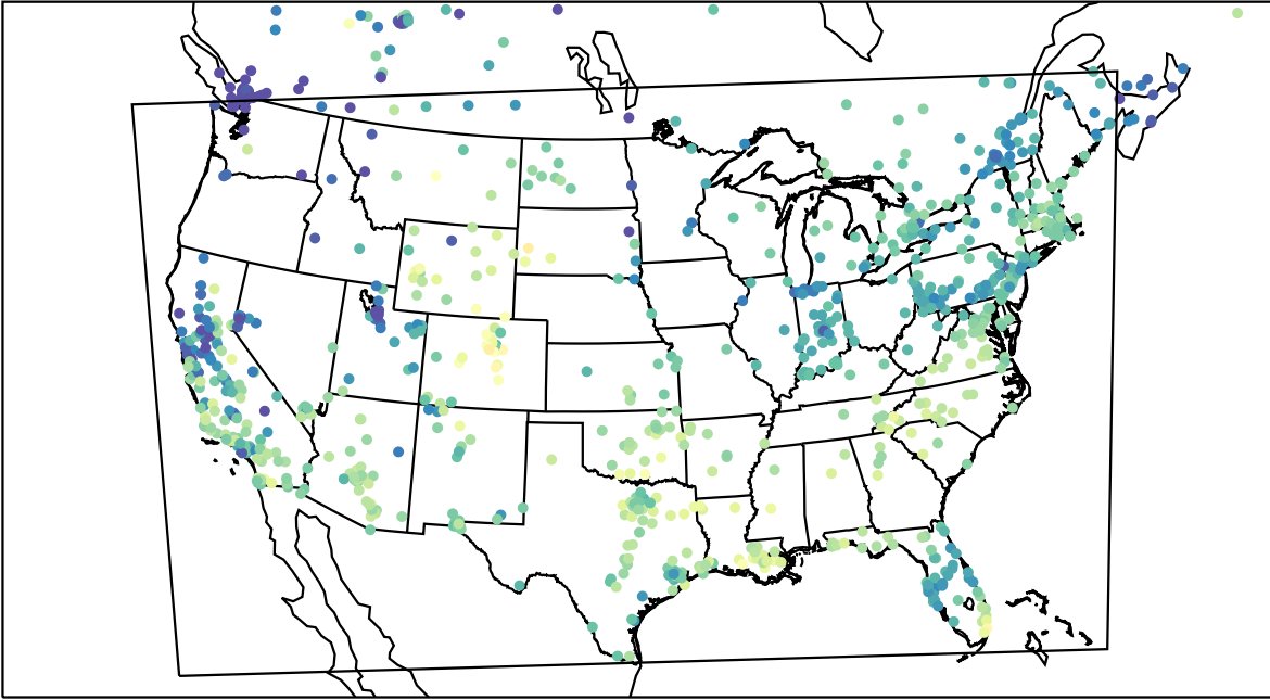
AirNOW (2023-11-28_19:00:00)
