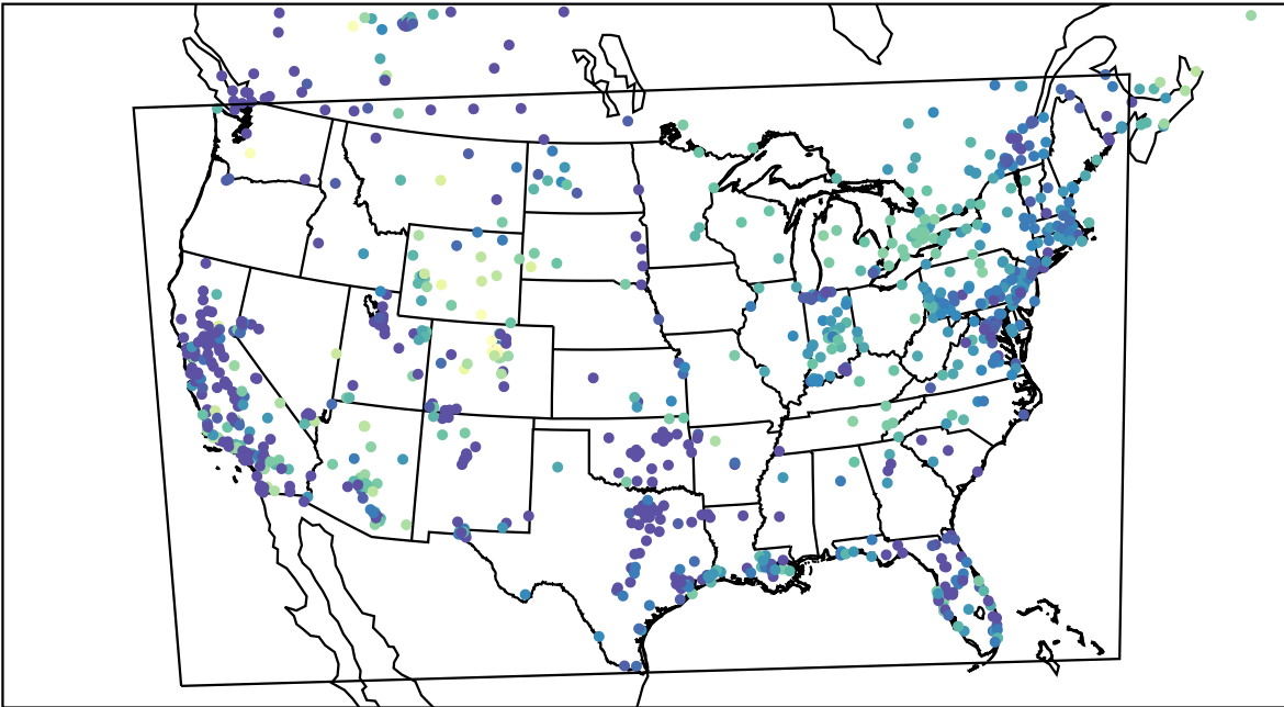
AirNOW (2023-11-28_03:00:00)
