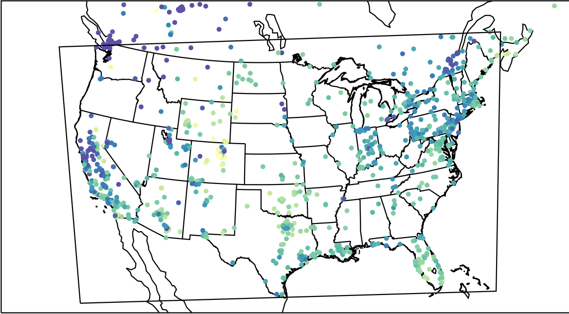
AirNOW (2023-11-27_18:00:00)
