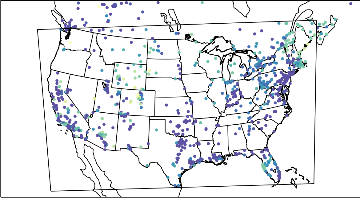
AirNOW (2023-11-27_11:00:00)
