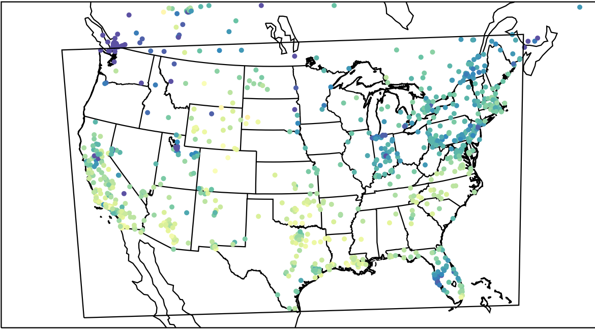
AirNOW (2023-11-28_21:00:00)
