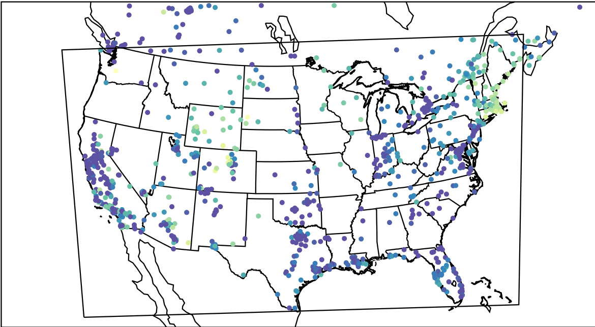
AirNOW (2023-11-27_06:00:00)
