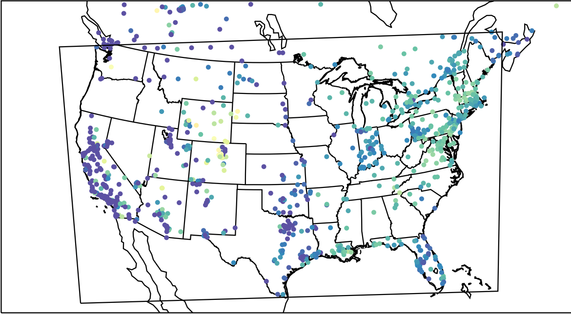
AirNOW (2023-11-28_15:00:00)
