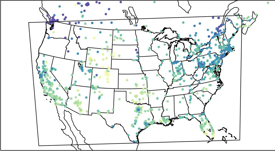
AirNOW (2023-11-27_20:00:00)
