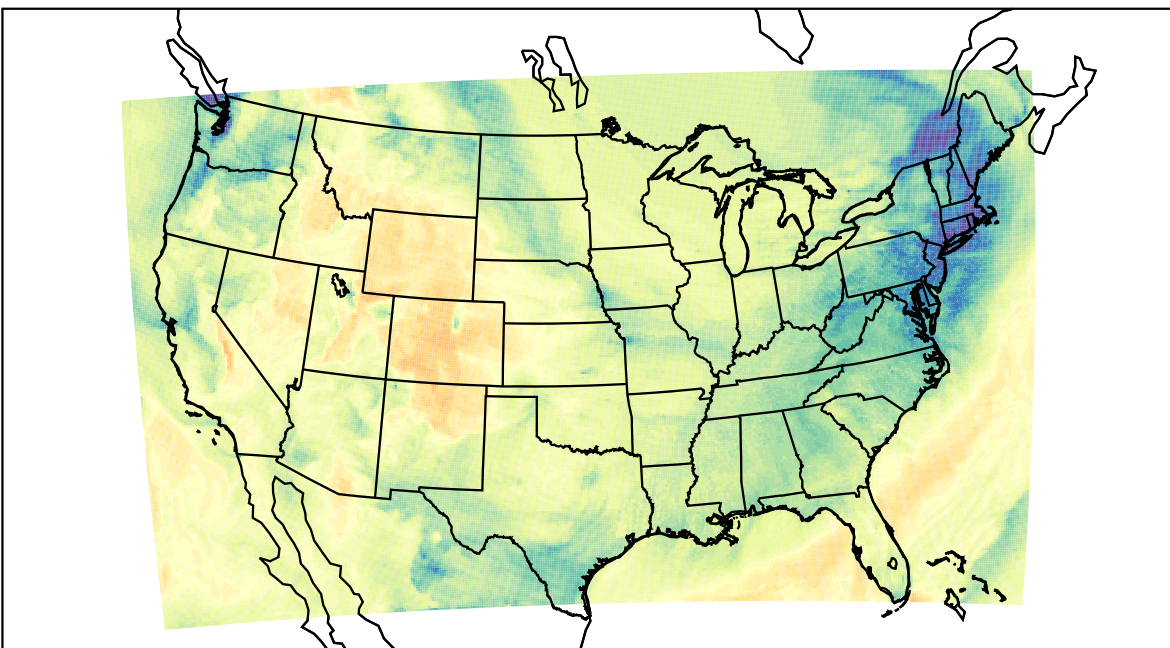
WRF (2023-11-27_21:00:00)
