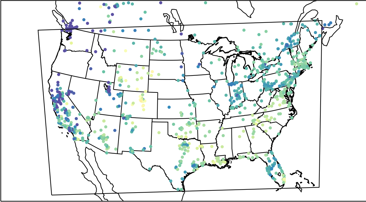
AirNOW (2023-11-28_18:00:00)
