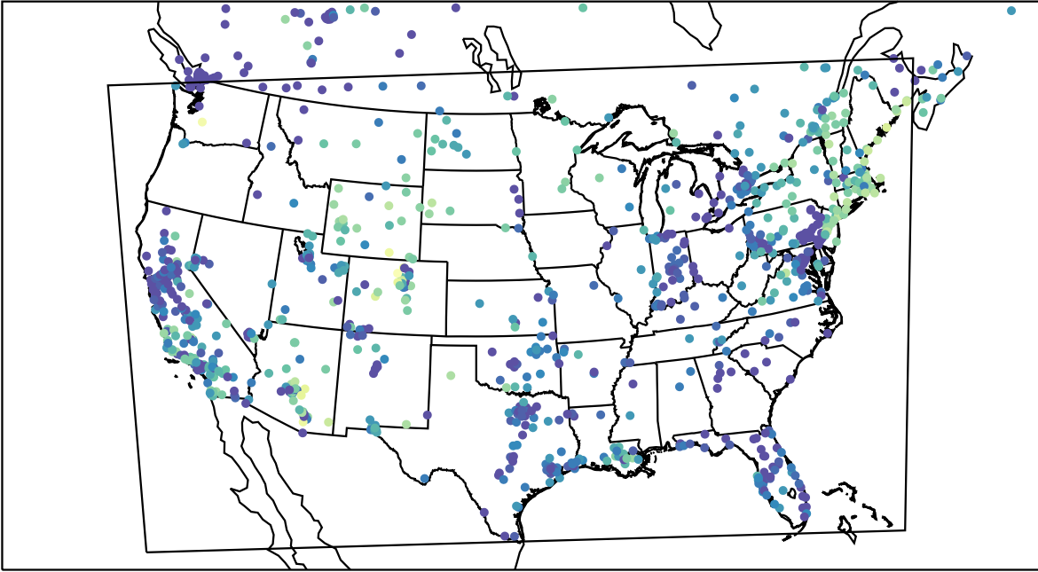
AirNOW (2023-11-27_01:00:00)
