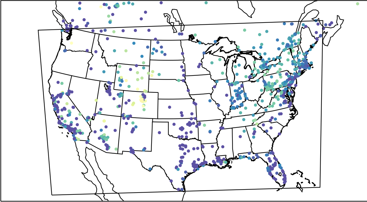
AirNOW (2023-11-28_12:00:00)
