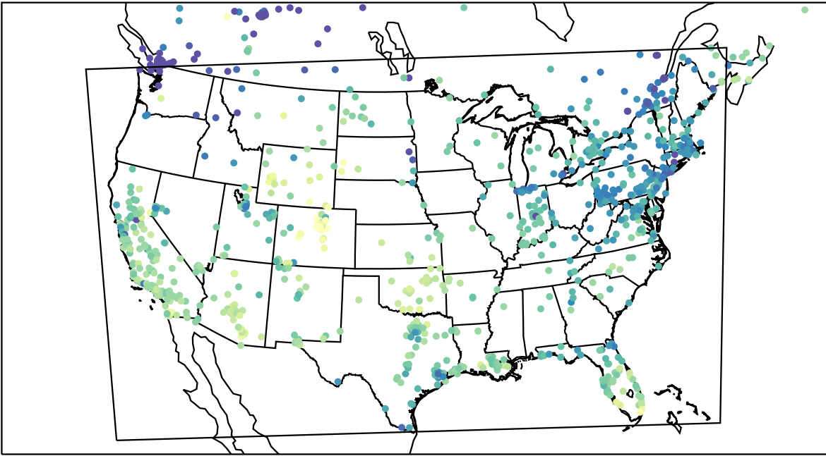
AirNOW (2023-11-27_21:00:00)
