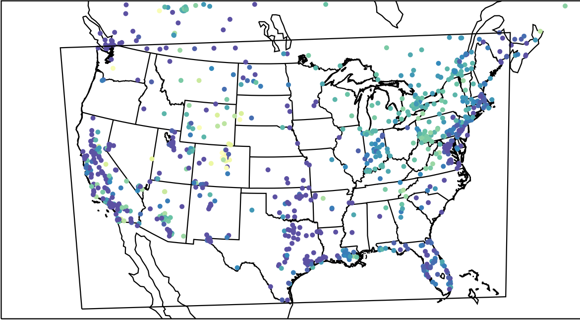
AirNOW (2023-11-28_09:00:00)
