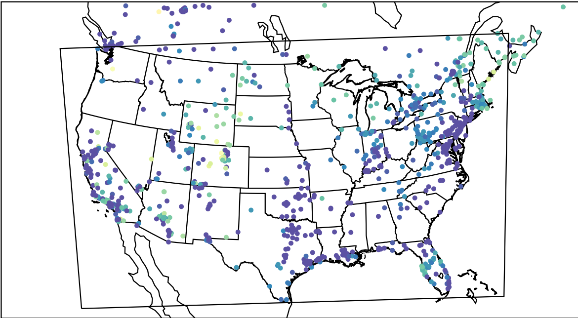
AirNOW (2023-11-27_12:00:00)
