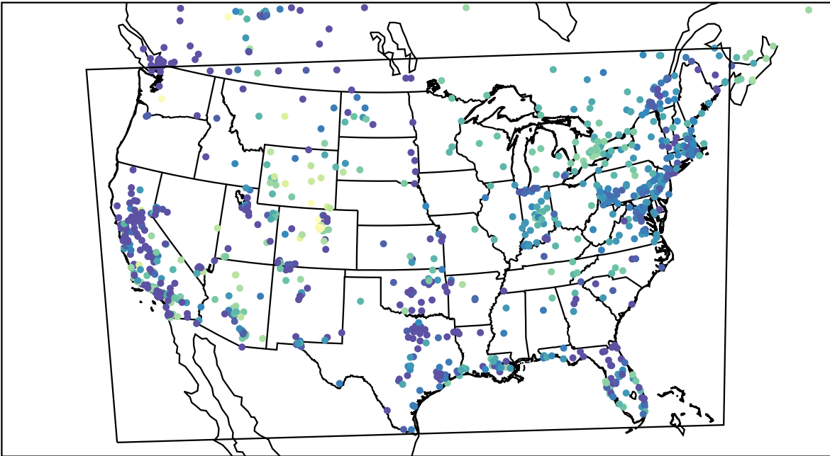
AirNOW (2023-11-28_02:00:00)
