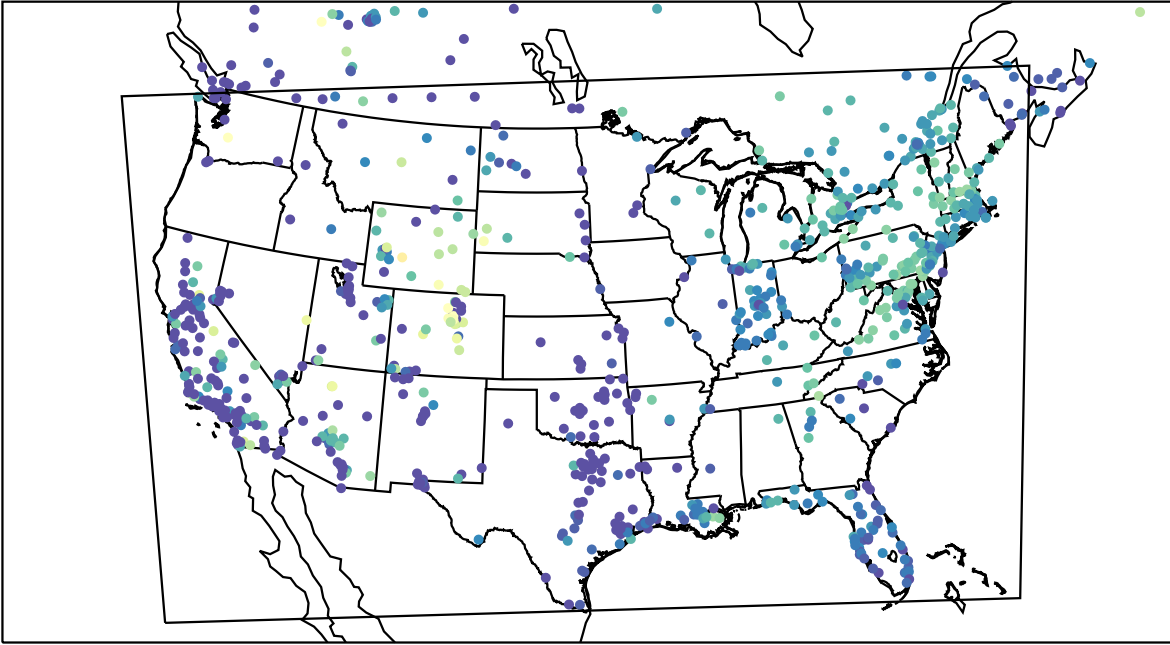
AirNOW (2023-11-28_14:00:00)
