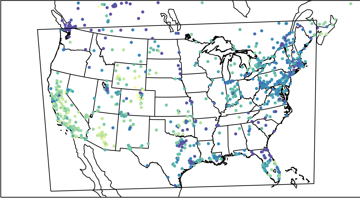
AirNOW (2023-11-27_23:00:00)
