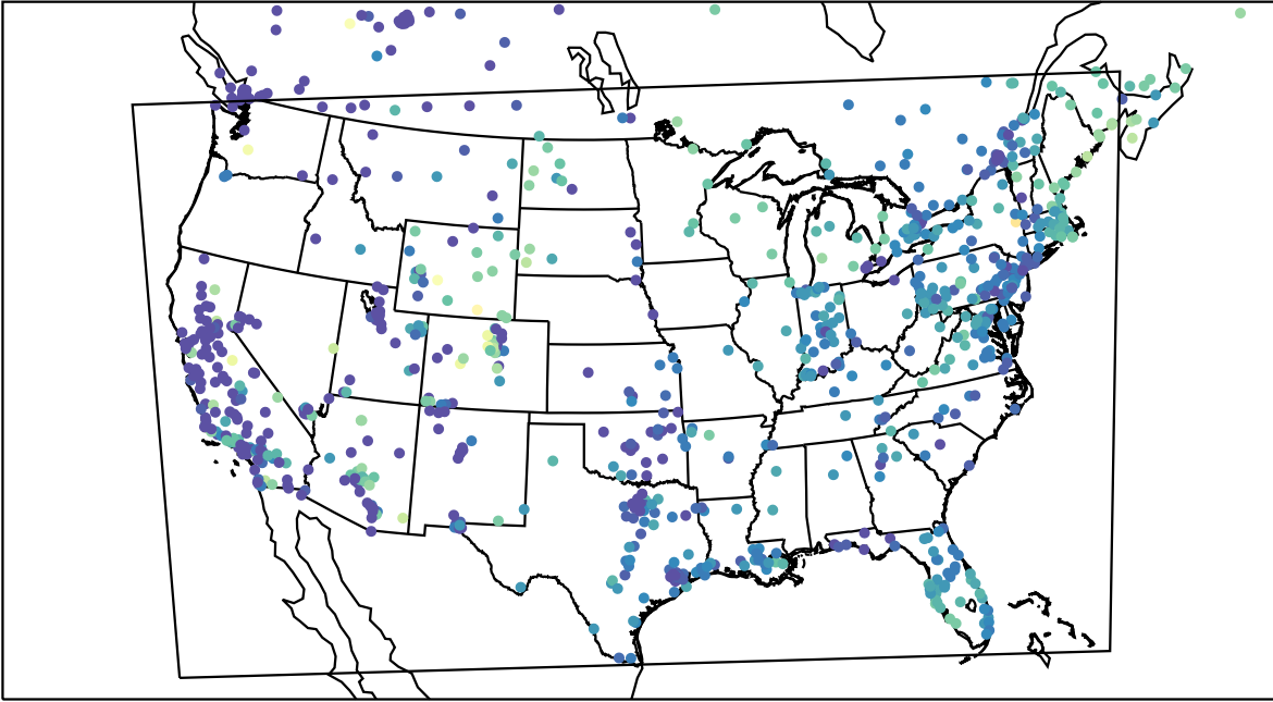
AirNOW (2023-11-27_15:00:00)
