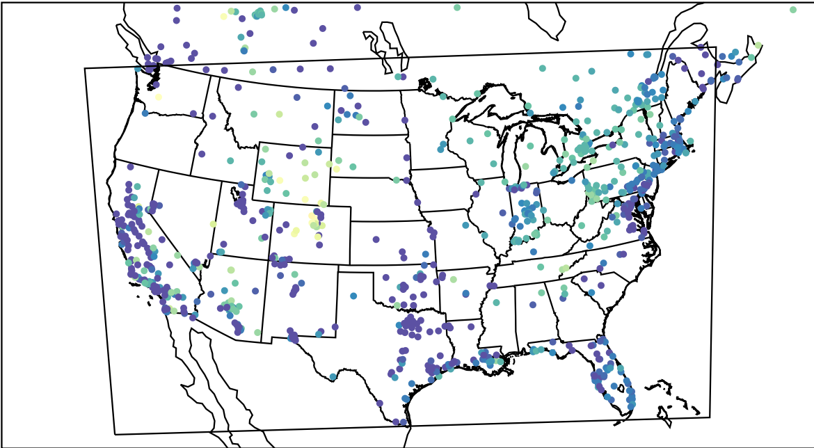
AirNOW (2023-11-28_07:00:00)
