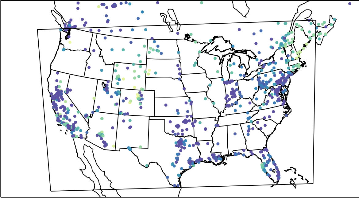
AirNOW (2023-11-27_08:00:00)
