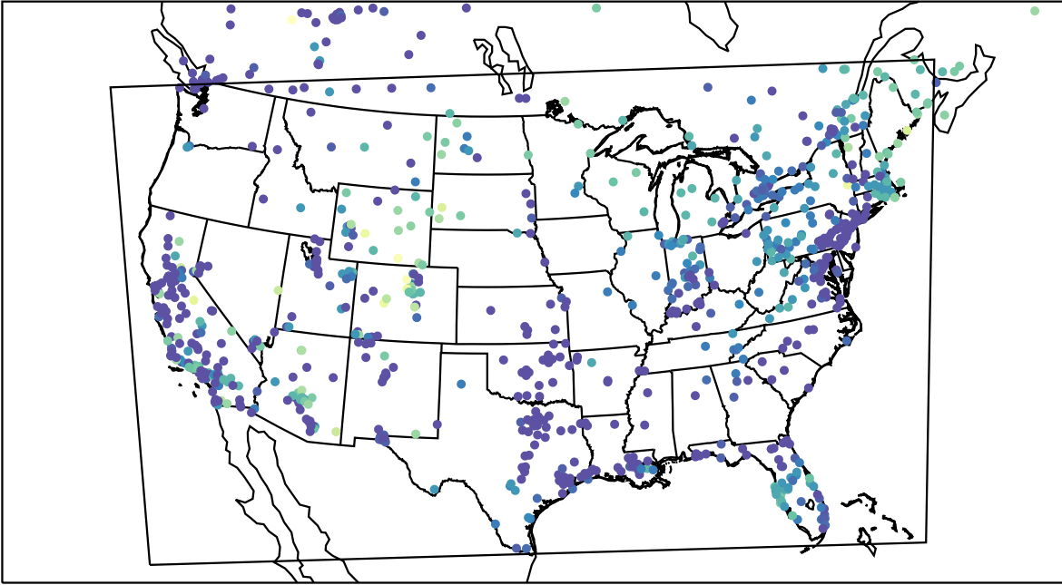
AirNOW (2023-11-27_13:00:00)
