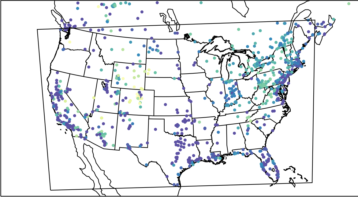
AirNOW (2023-11-28_11:00:00)
