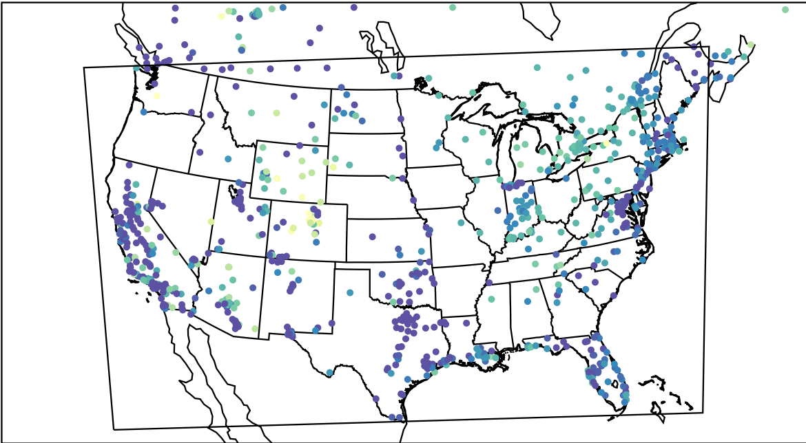
AirNOW (2023-11-28_06:00:00)
