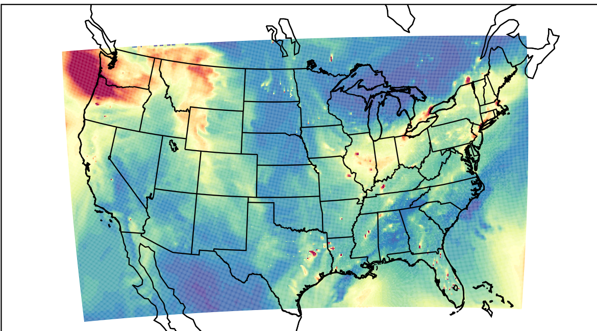
WRF 2023-12-02_21:00:00
