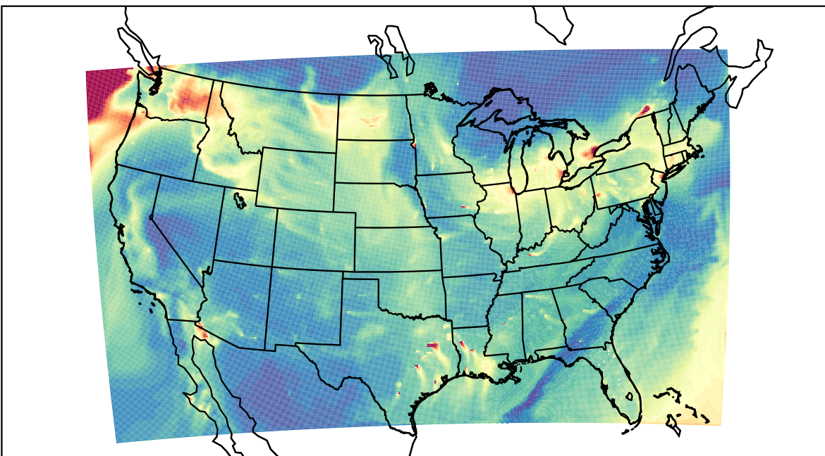
WRF 2023-12-03_17:00:00
