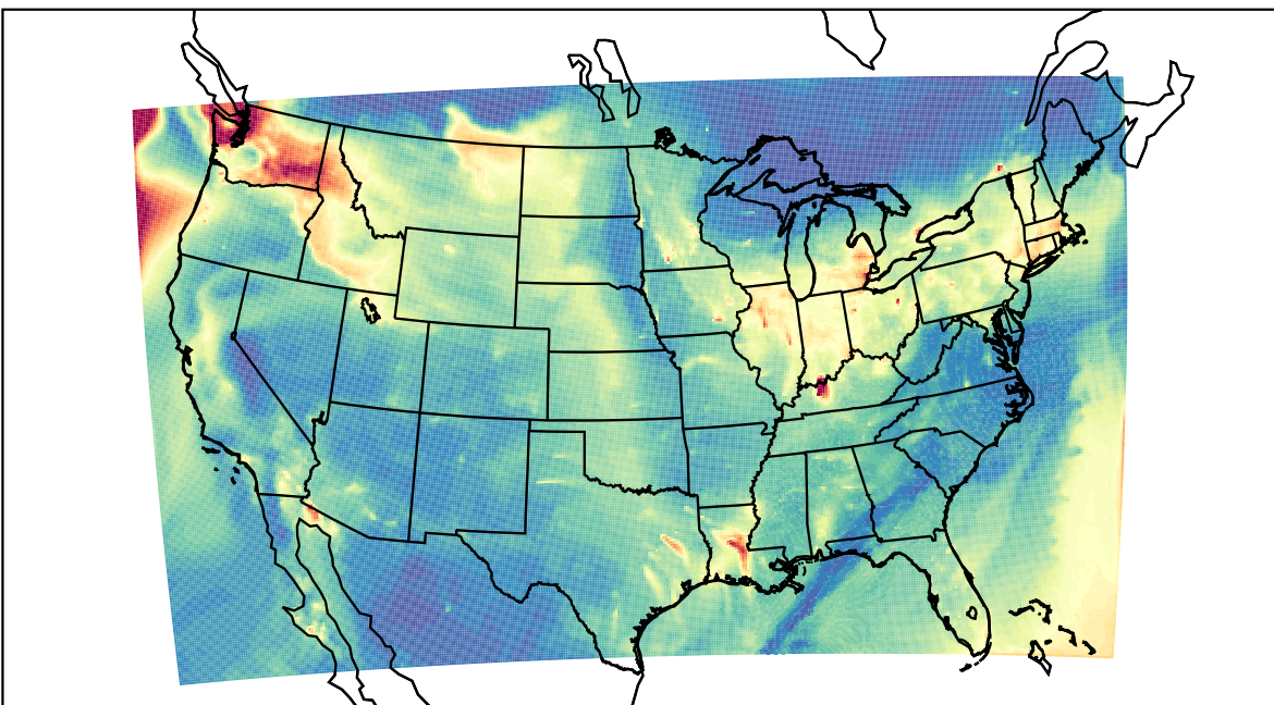
WRF 2023-12-03_12:00:00
