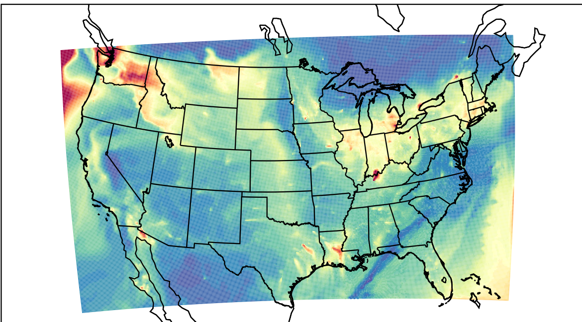
WRF 2023-12-03_13:00:00
