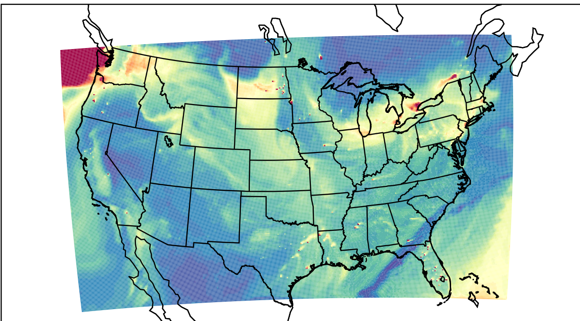
WRF 2023-12-03_21:00:00
