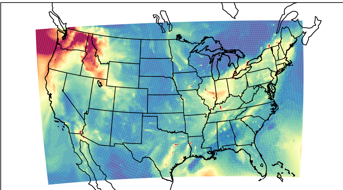
WRF 2023-12-02_15:00:00
