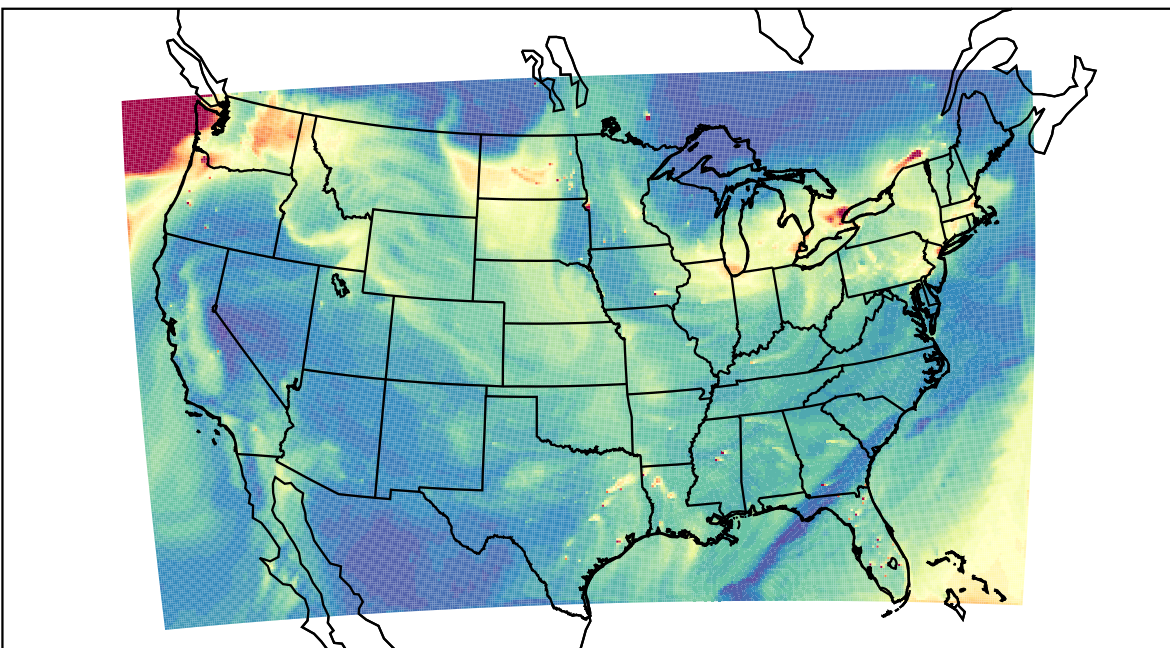
WRF 2023-12-03_20:00:00
