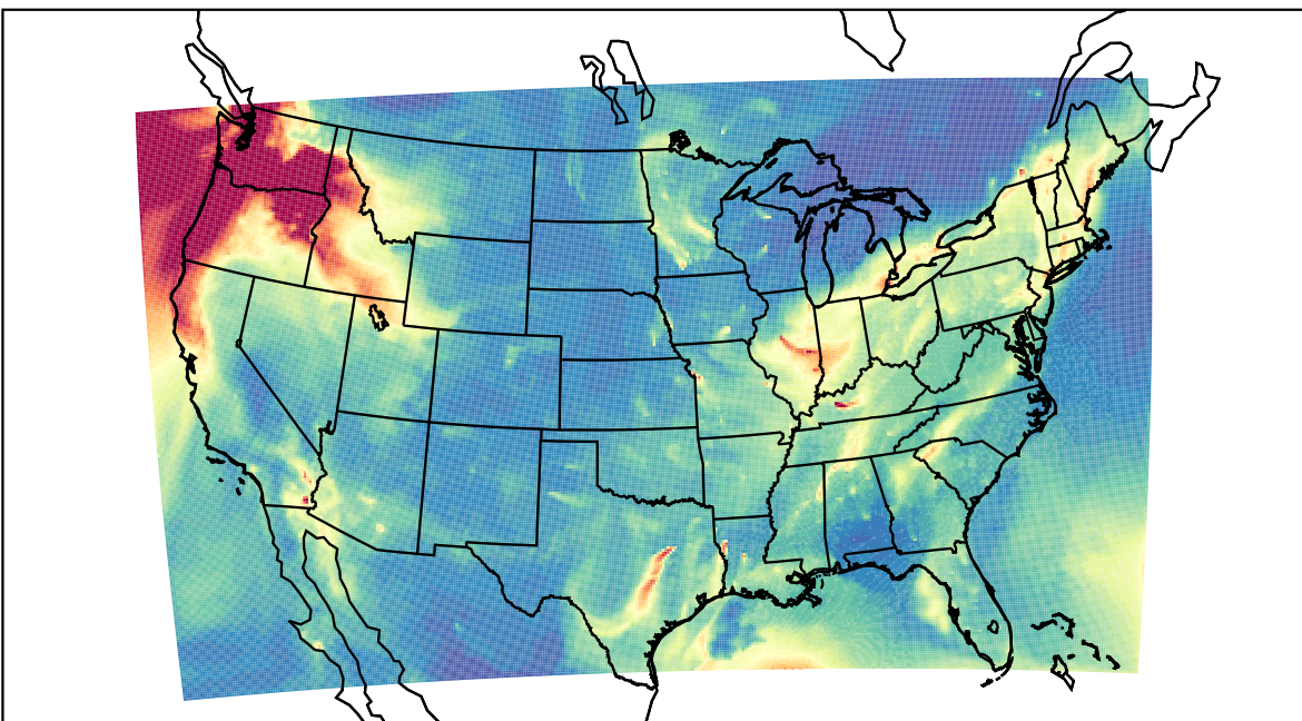
WRF 2023-12-02_11:00:00
