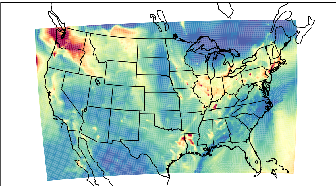
WRF 2023-12-03_06:00:00
