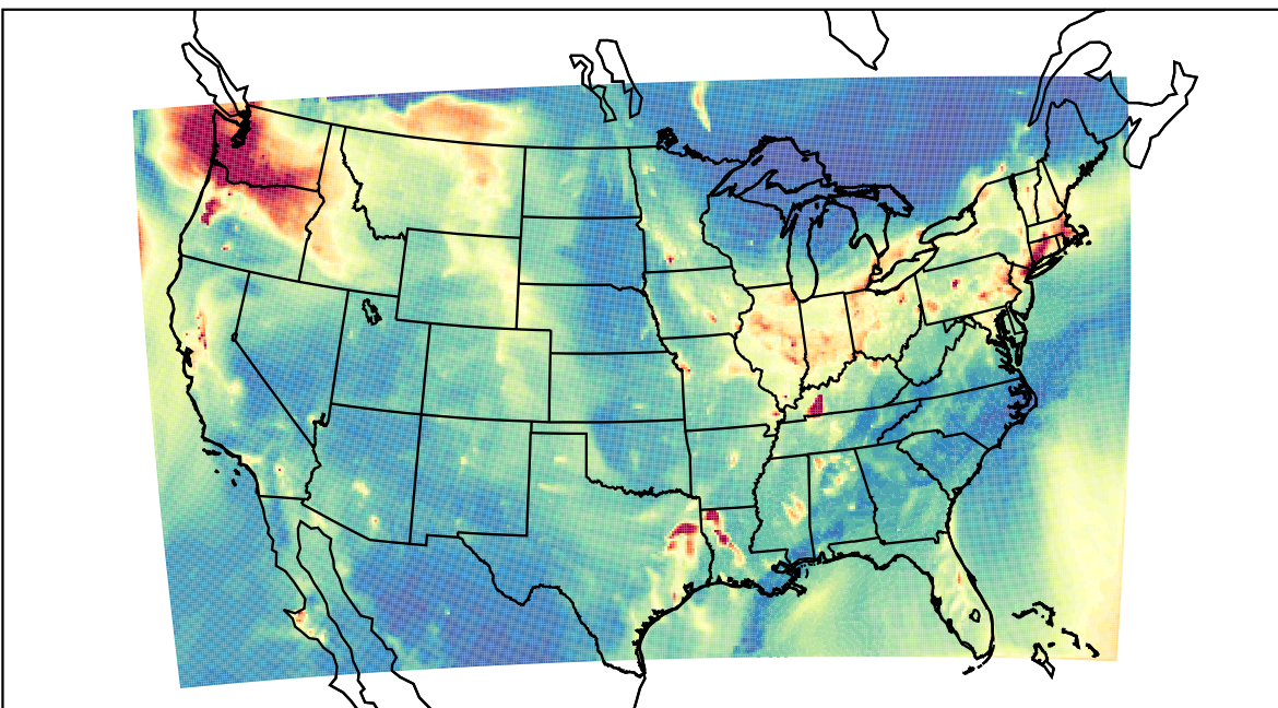
WRF 2023-12-03_04:00:00
