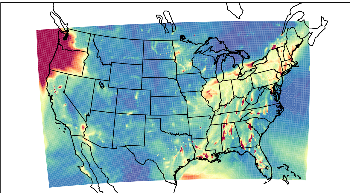
WRF 2023-12-02_01:00:00
