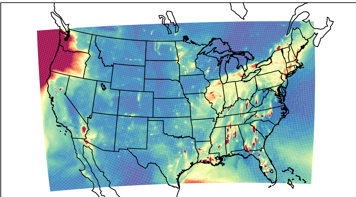
WRF 2023-12-02_00:00:00
