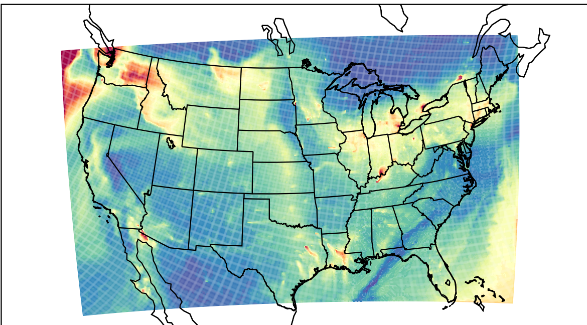
WRF 2023-12-03_14:00:00
