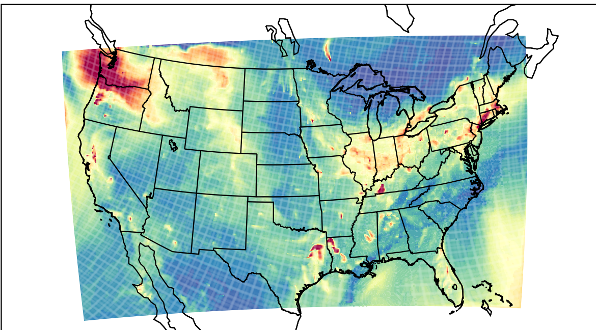
WRF 2023-12-03_03:00:00
