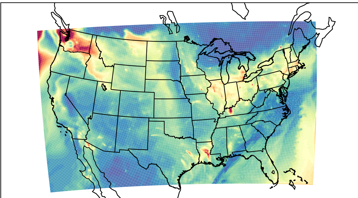
WRF 2023-12-03_11:00:00
