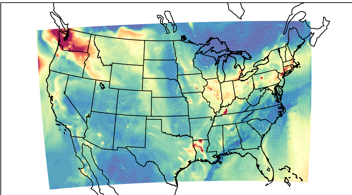
WRF 2023-12-03_07:00:00
