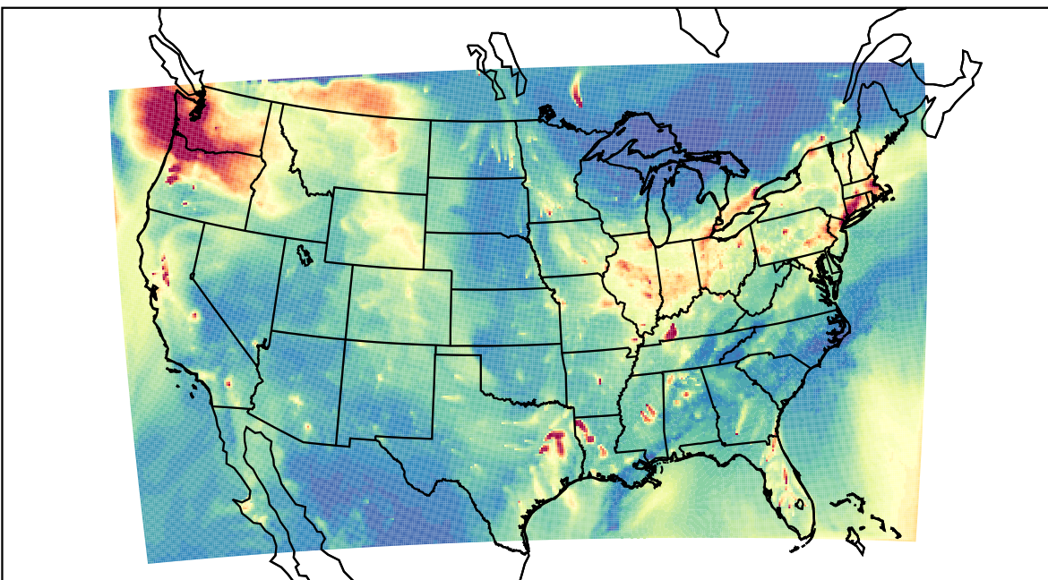
WRF 2023-12-03_02:00:00
