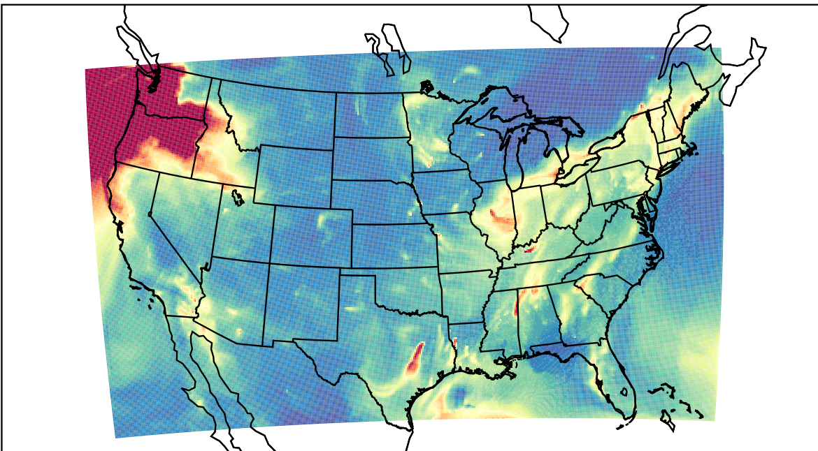
WRF 2023-12-02_08:00:00
