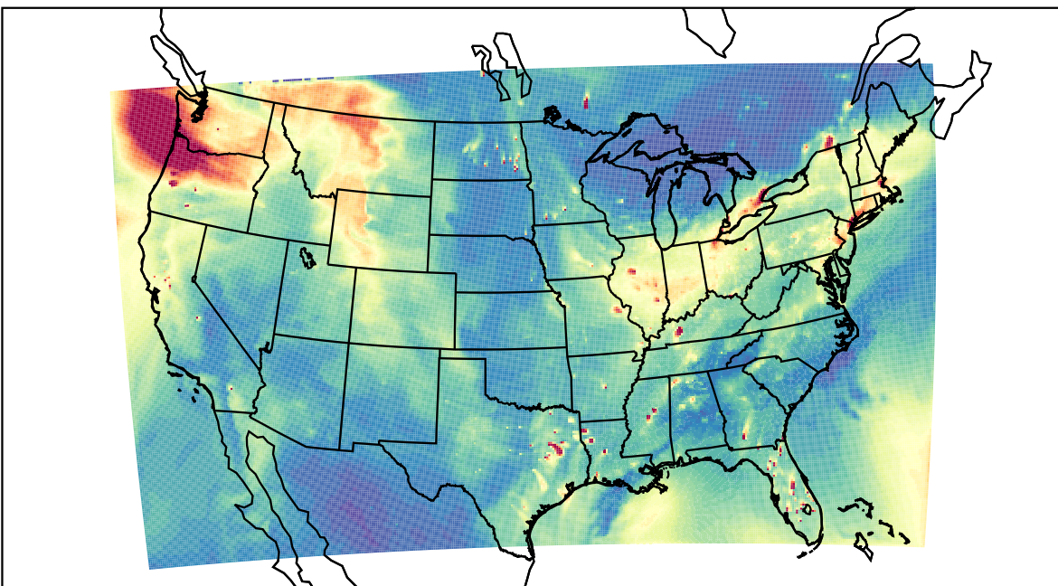
WRF 2023-12-02_22:00:00
