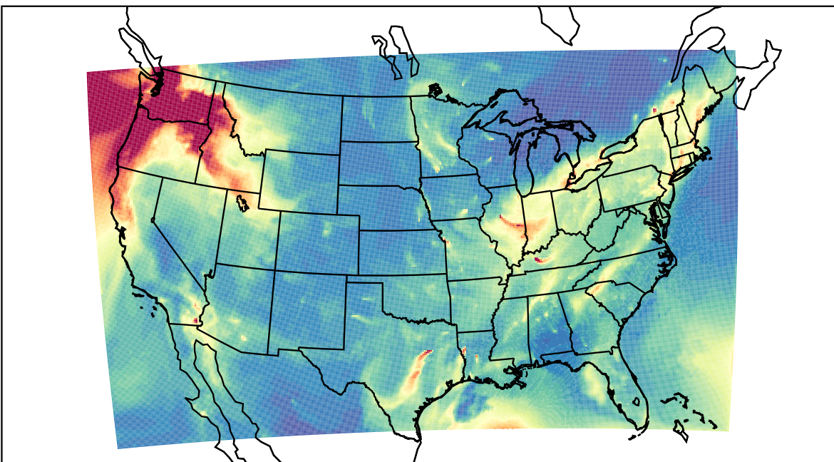
WRF 2023-12-02_12:00:00
