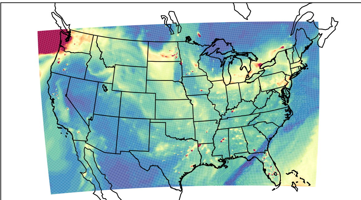
WRF 2023-12-03_23:00:00
