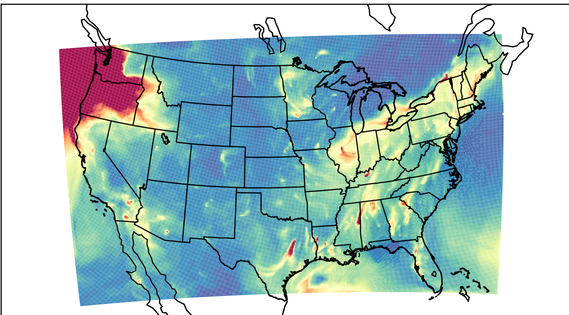
WRF 2023-12-02_06:00:00
