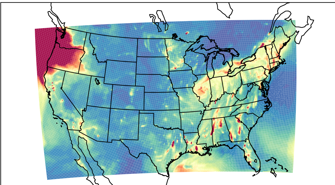
WRF 2023-12-02_03:00:00
