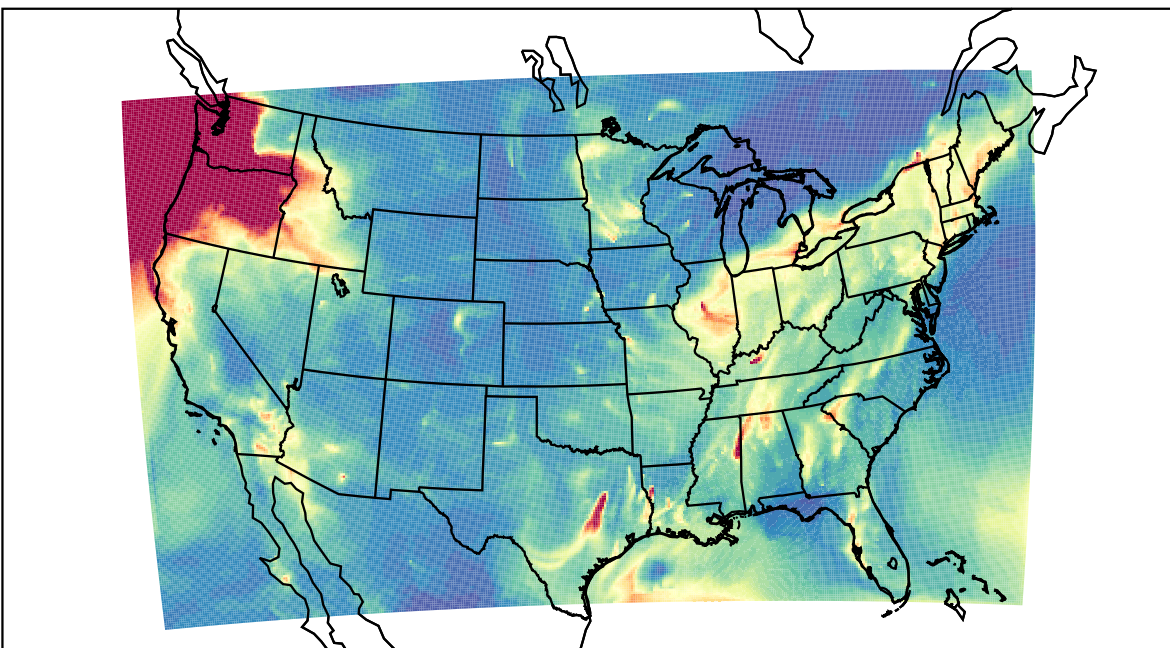
WRF 2023-12-02_07:00:00
