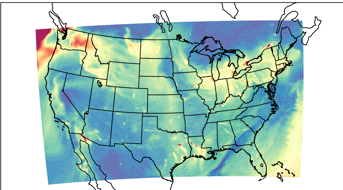
WRF 2023-12-03_16:00:00
