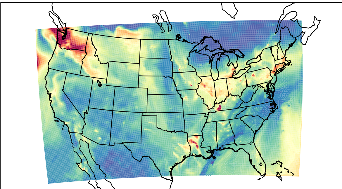
WRF 2023-12-03_08:00:00
