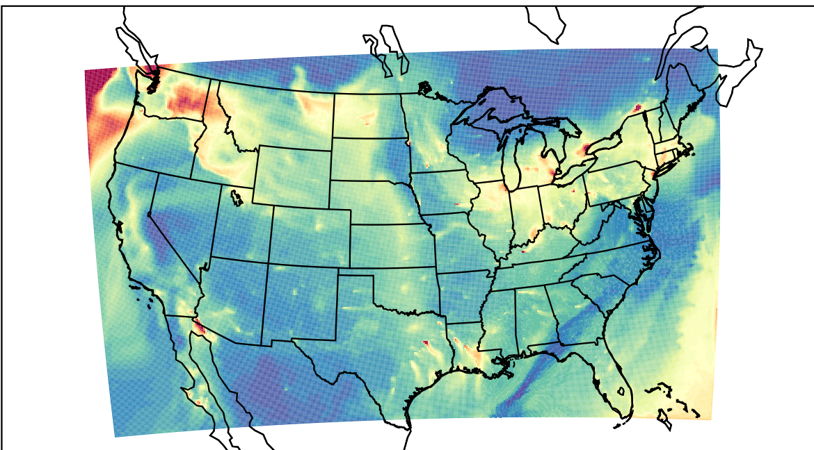
WRF 2023-12-03_15:00:00
