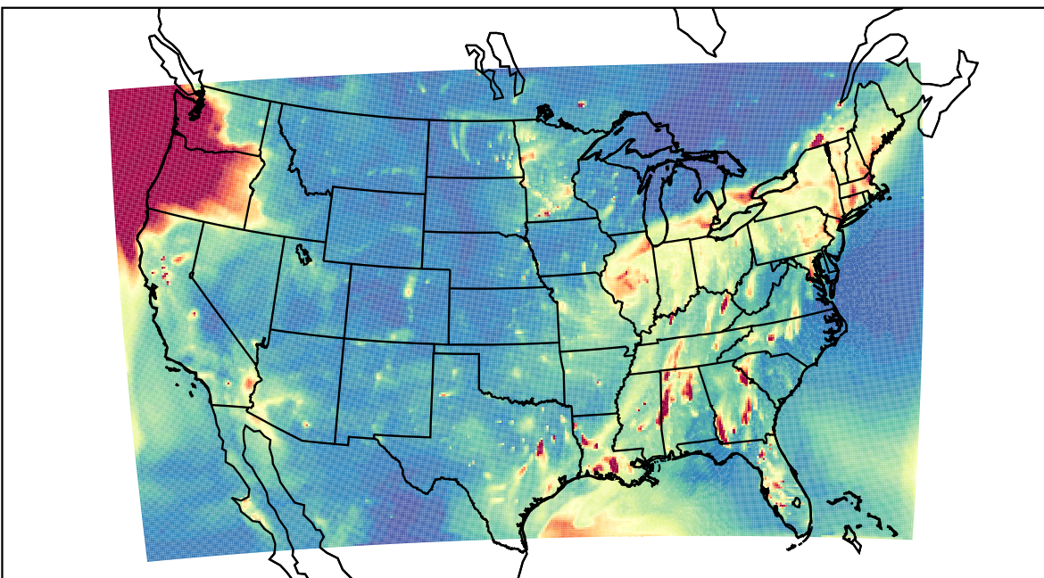
WRF 2023-12-02_02:00:00
