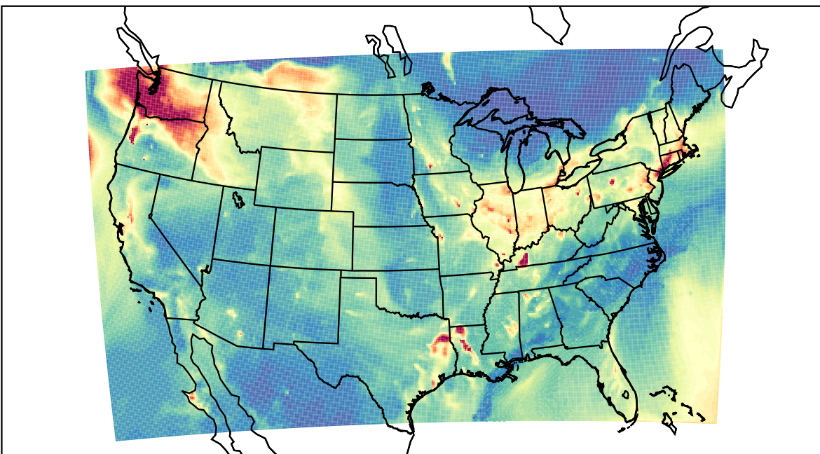
WRF 2023-12-03_05:00:00
