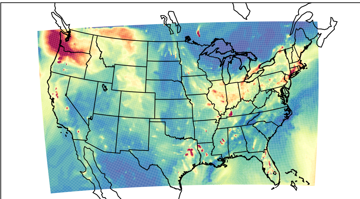
WRF 2023-12-03_01:00:00
