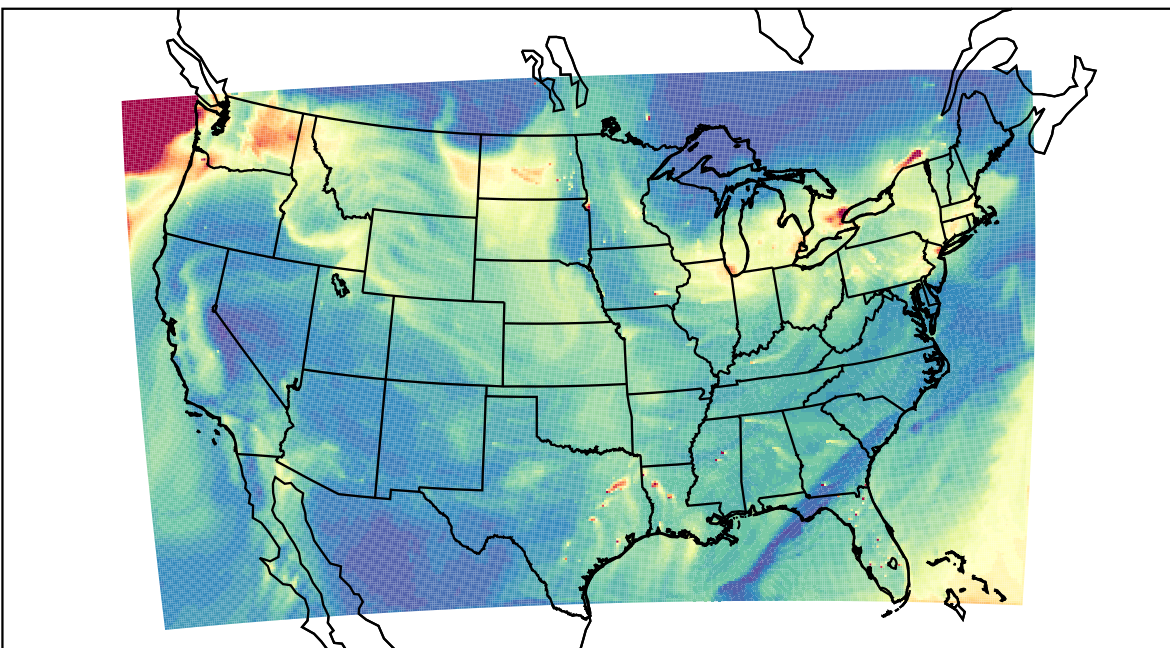
WRF 2023-12-03_19:00:00
