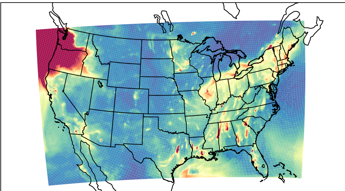
WRF 2023-12-02_04:00:00
