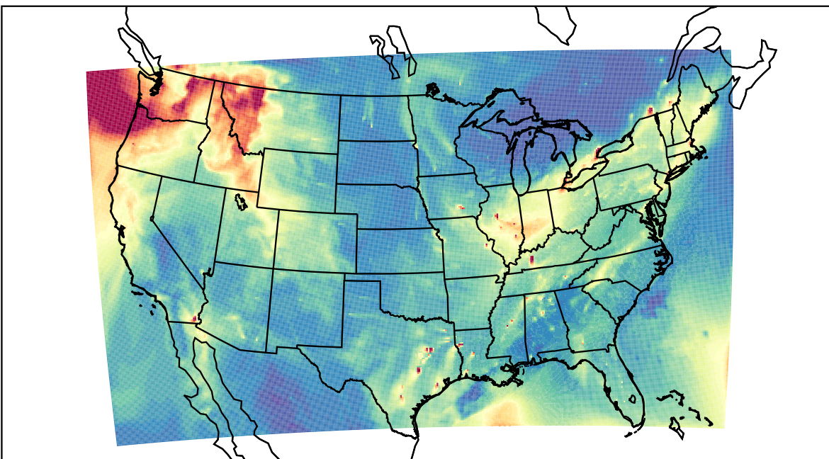
WRF 2023-12-02_17:00:00
