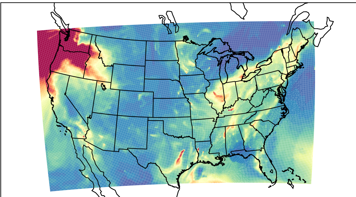
WRF 2023-12-02_09:00:00
