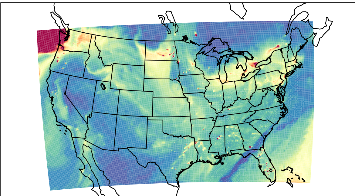
WRF 2023-12-03_22:00:00
