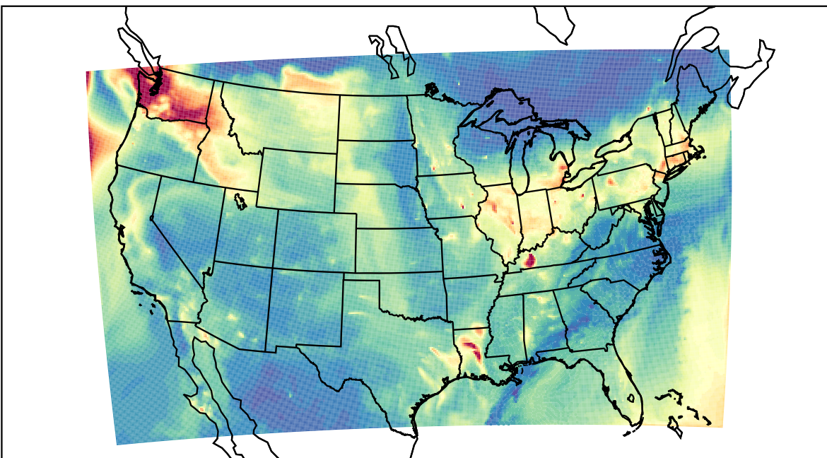
WRF 2023-12-03_09:00:00
