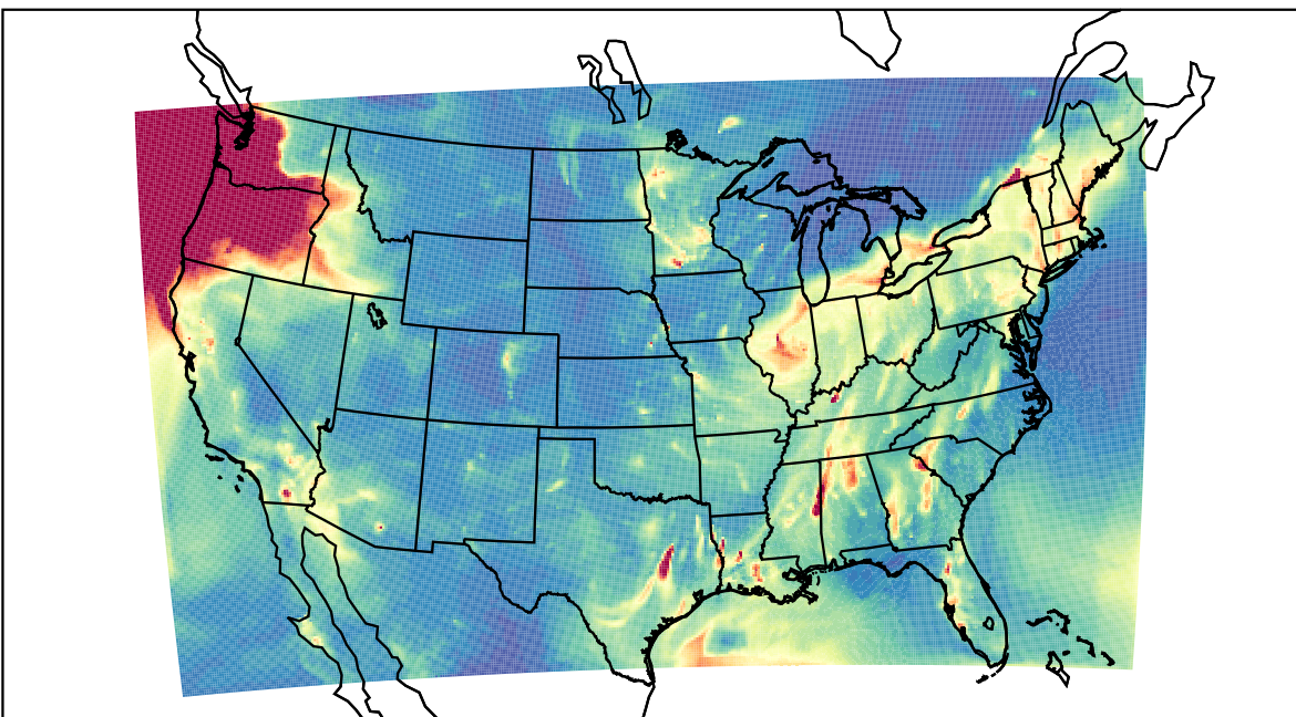
WRF 2023-12-02_05:00:00
