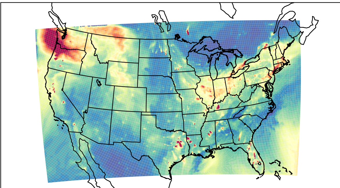
WRF 2023-12-03_00:00:00
