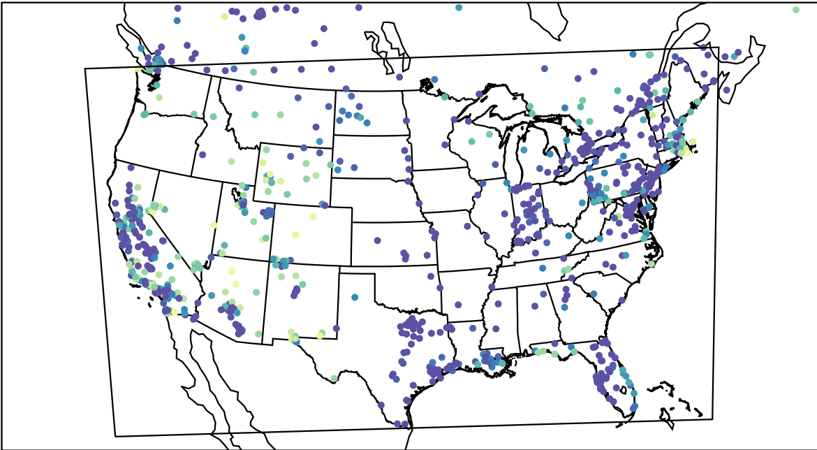
AirNOW (2023-12-02_05:00:00)
