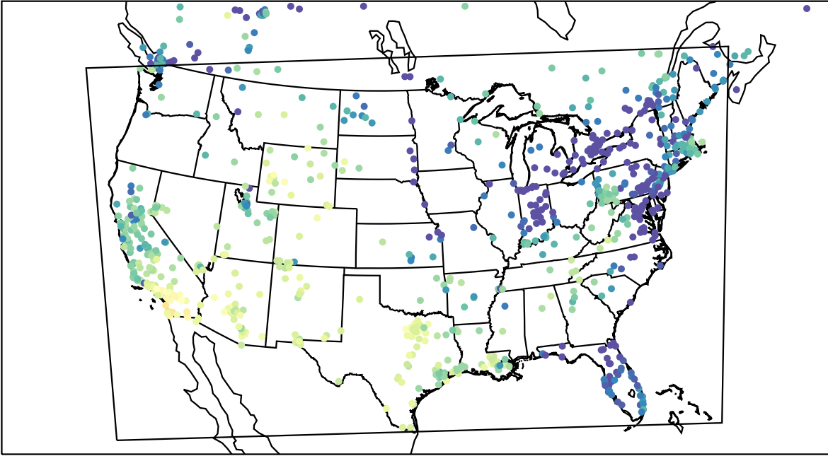
AirNOW (2023-12-03_21:00:00)
