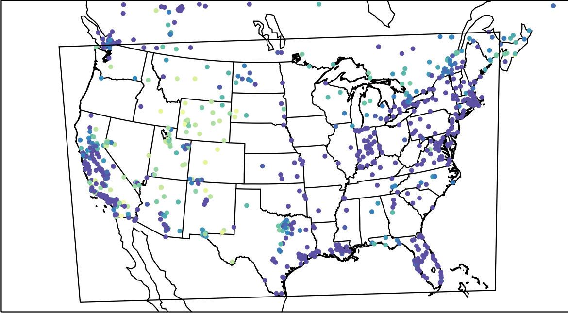
AirNOW (2023-12-03_06:00:00)
