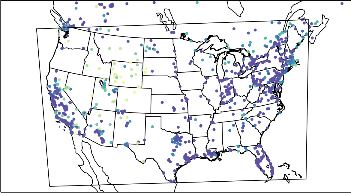
AirNOW (2023-12-03_13:00:00)
