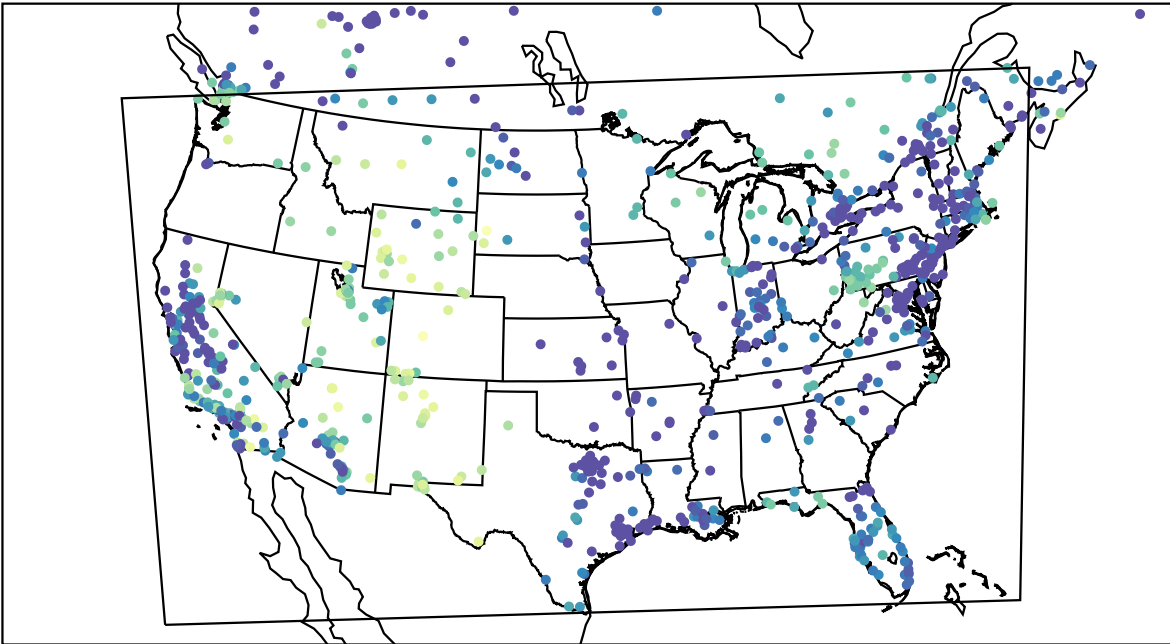
AirNOW (2023-12-02_17:00:00)
