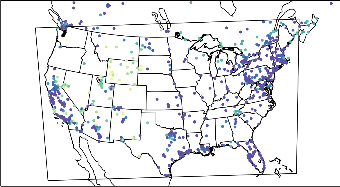
AirNOW (2023-12-03_10:00:00)
