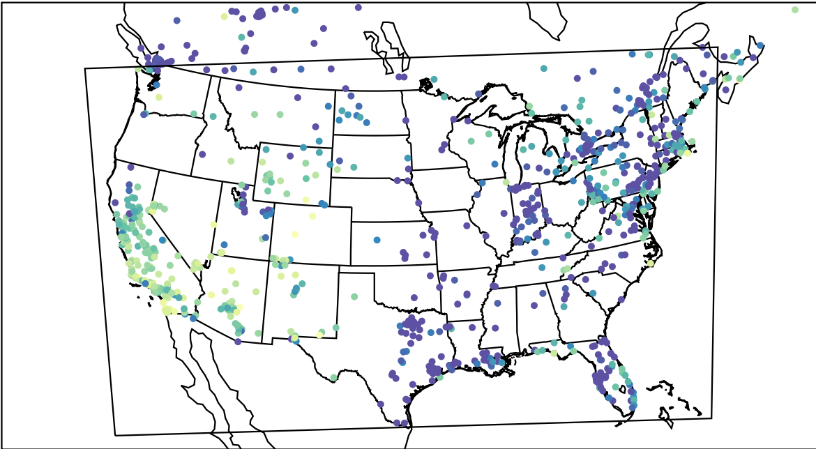
AirNOW (2023-12-02_00:00:00)
