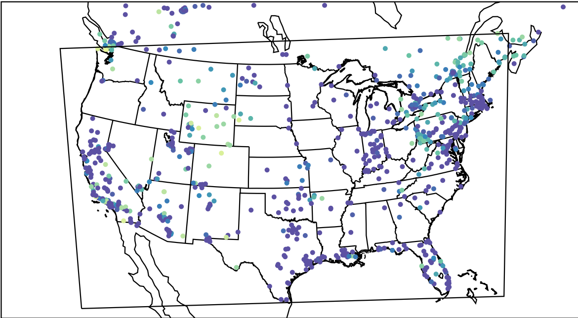
AirNOW (2023-12-05_11:00:00)
