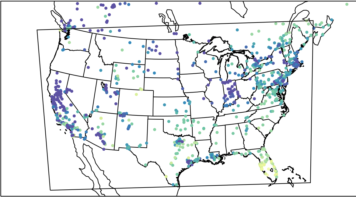
AirNOW (2023-12-05_17:00:00)
