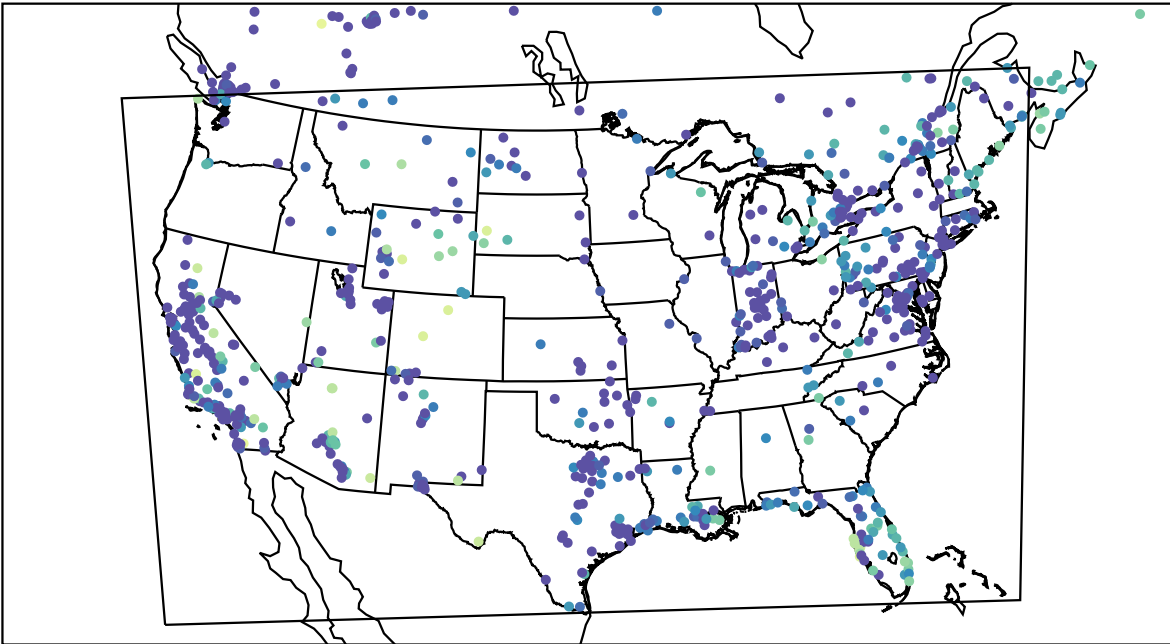
AirNOW (2023-12-06_08:00:00)
