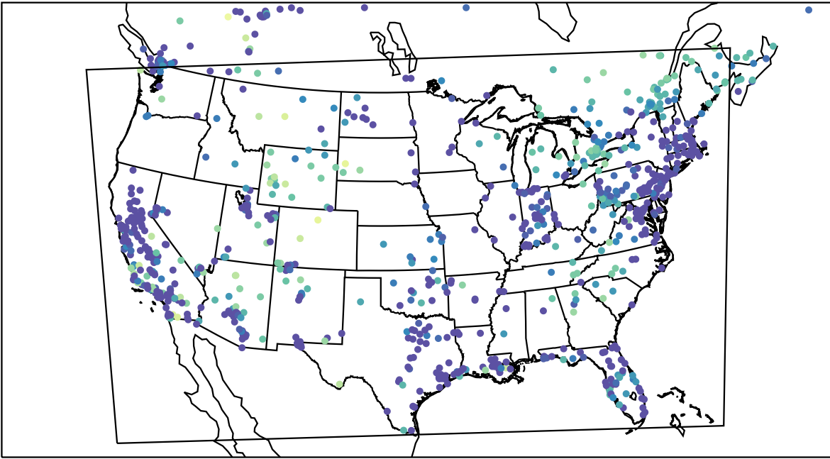
AirNOW (2023-12-05_03:00:00)
