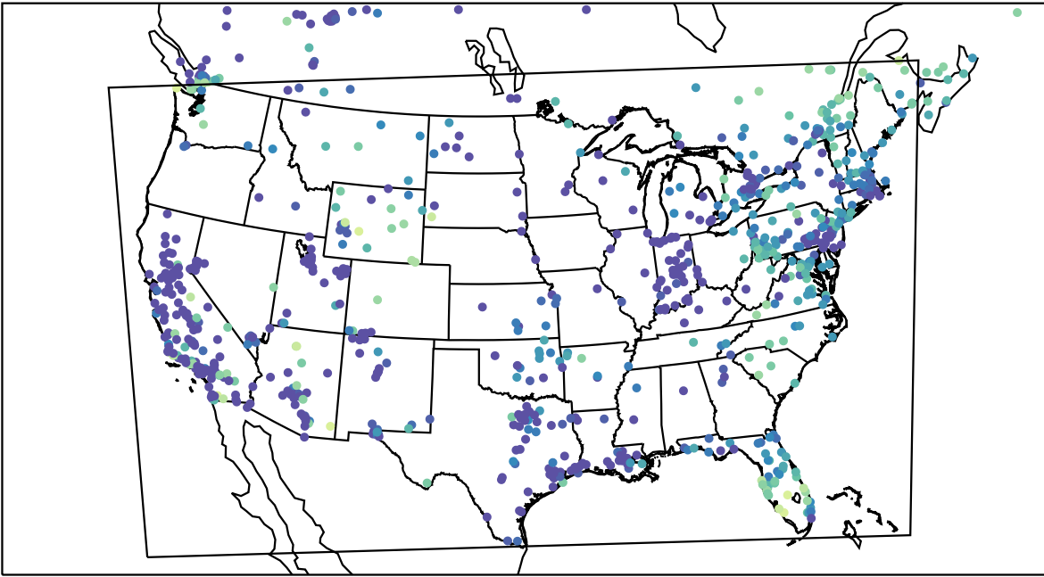
AirNOW (2023-12-05_15:00:00)
