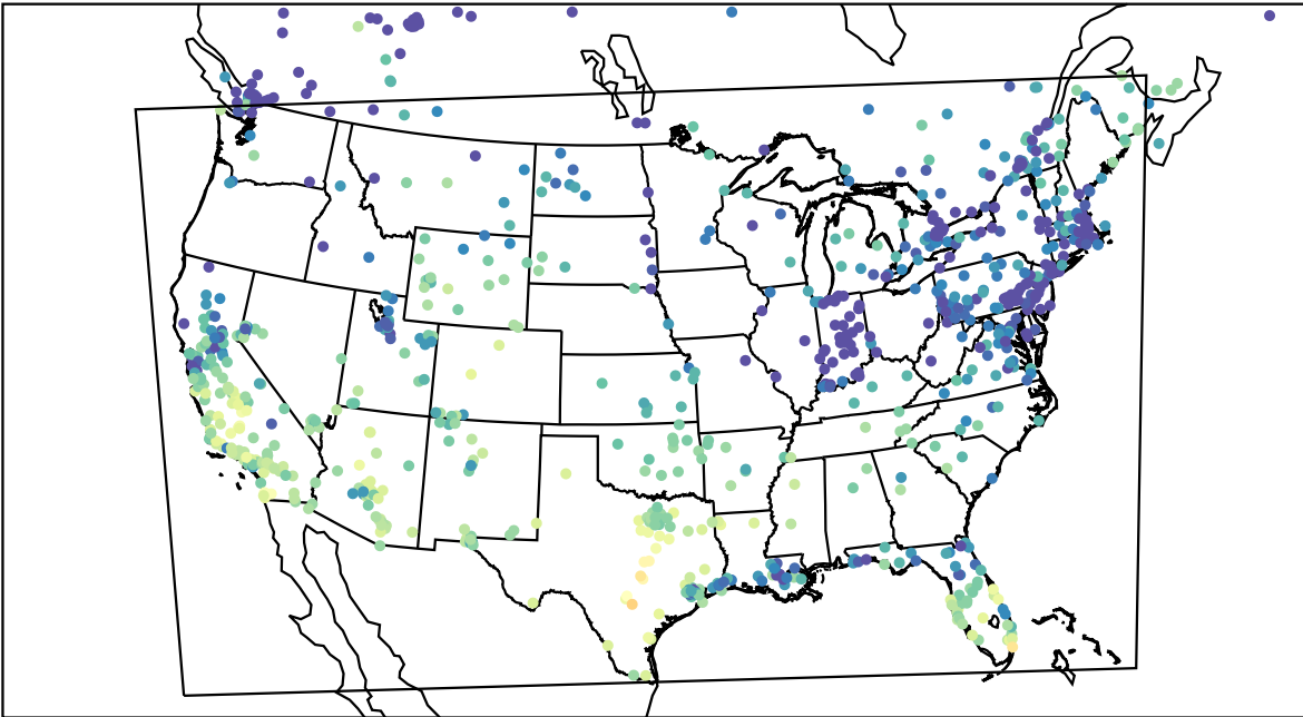
AirNOW (2023-12-05_22:00:00)
