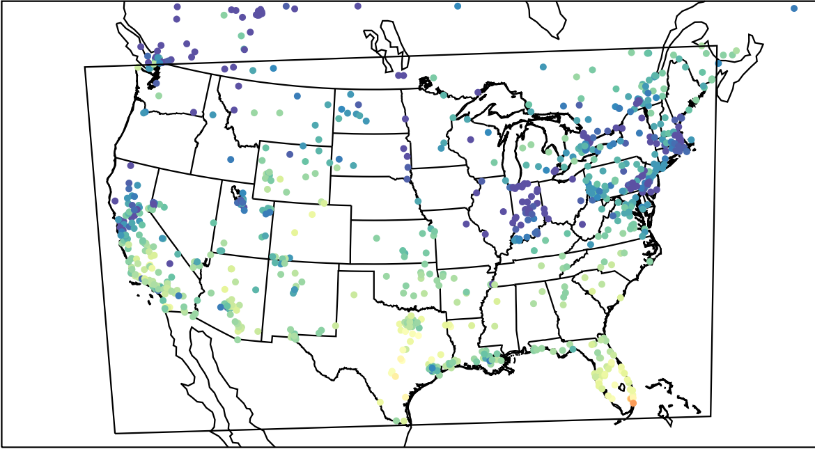
AirNOW (2023-12-05_20:00:00)
