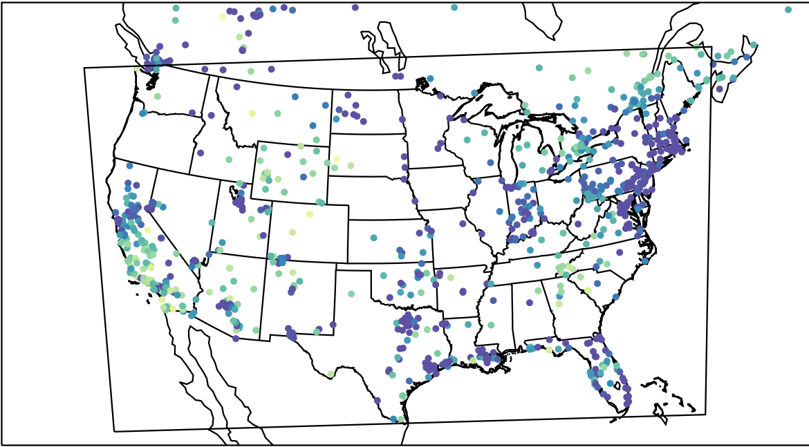
AirNOW (2023-12-05_00:00:00)
