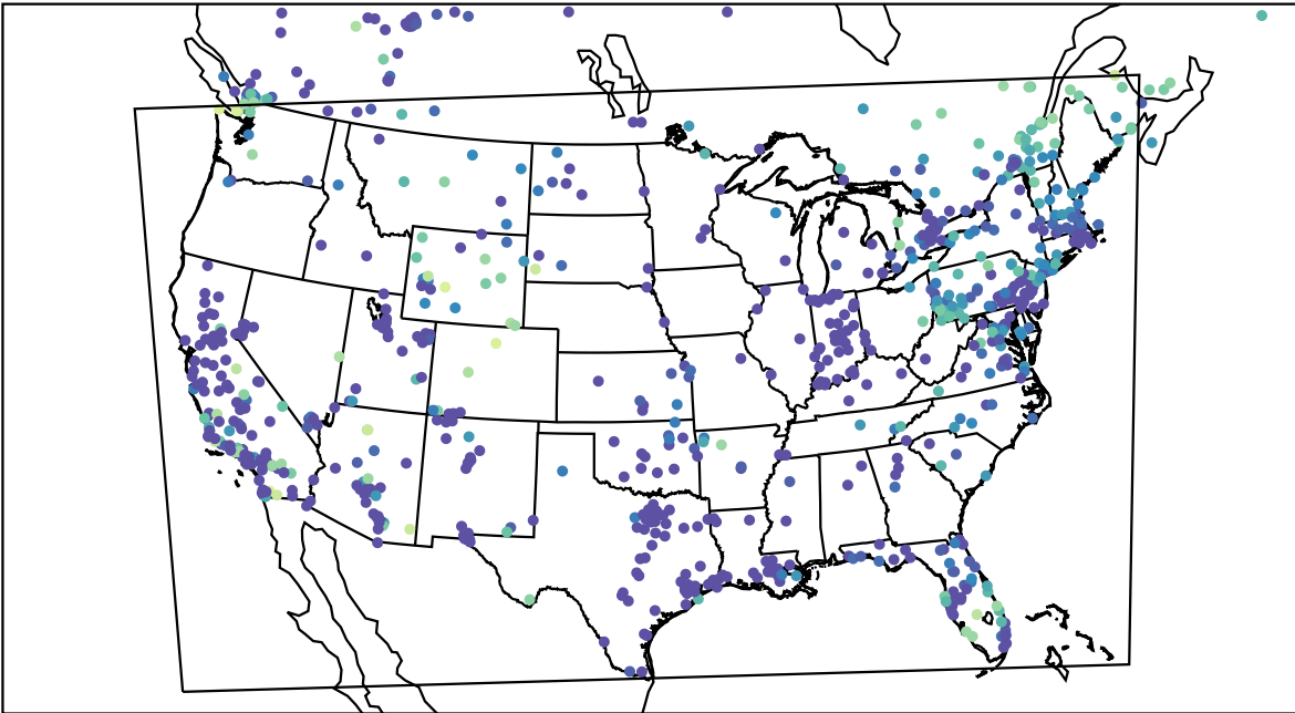
AirNOW (2023-12-05_14:00:00)
