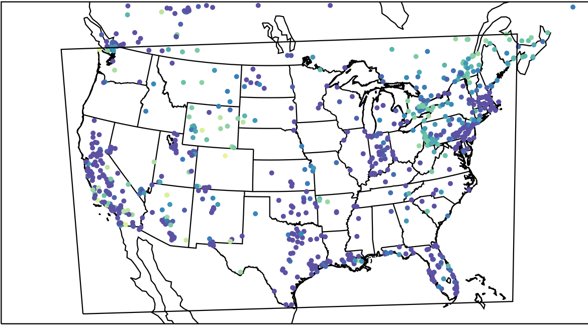
AirNOW (2023-12-05_09:00:00)
