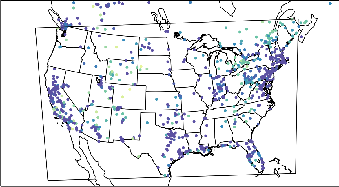
AirNOW (2023-12-05_04:00:00)
