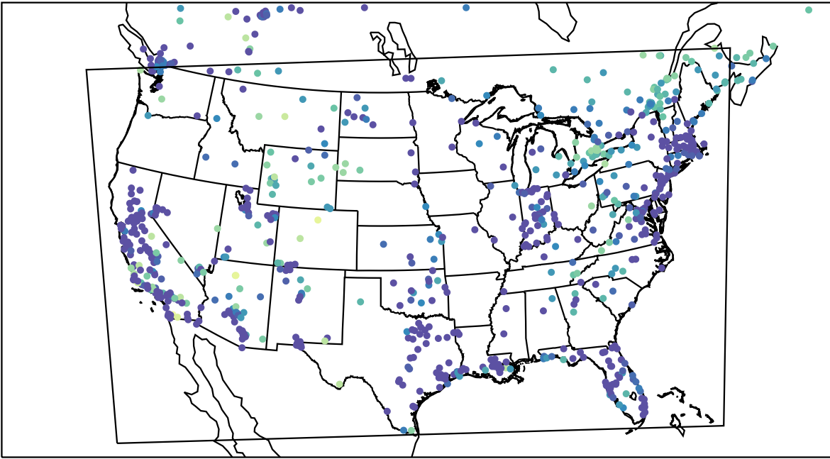
AirNOW (2023-12-05_06:00:00)
