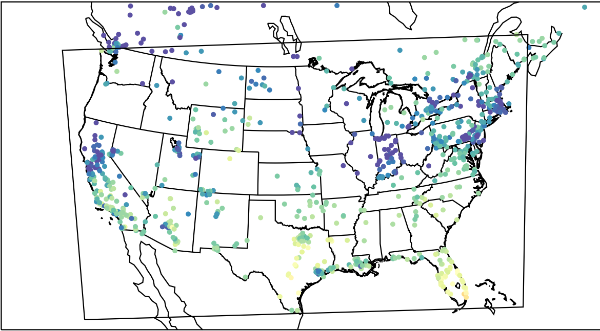
AirNOW (2023-12-05_19:00:00)
