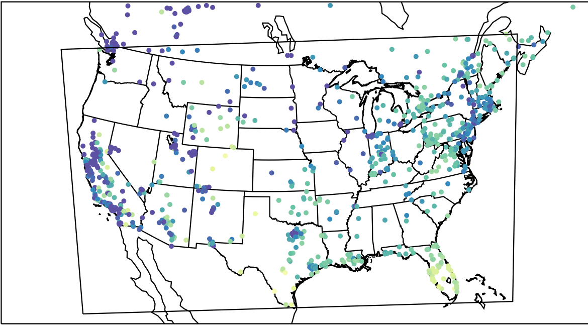
AirNOW (2023-12-06_17:00:00)
