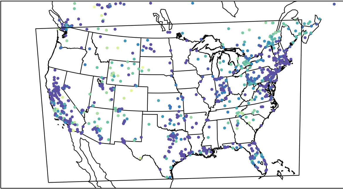
AirNOW (2023-12-05_02:00:00)
