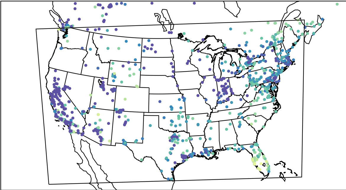
AirNOW (2023-12-05_16:00:00)
