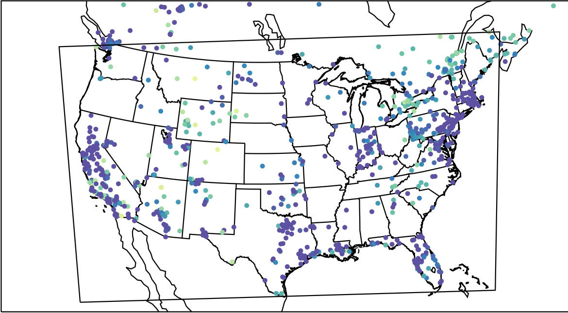
AirNOW (2023-12-05_05:00:00)
