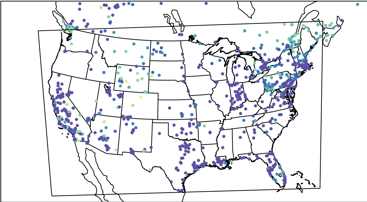
AirNOW (2023-12-05_13:00:00)
