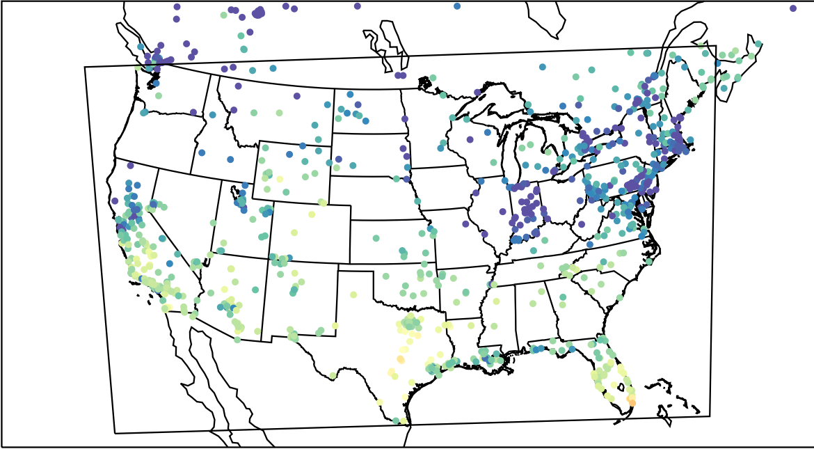
AirNOW (2023-12-05_21:00:00)
