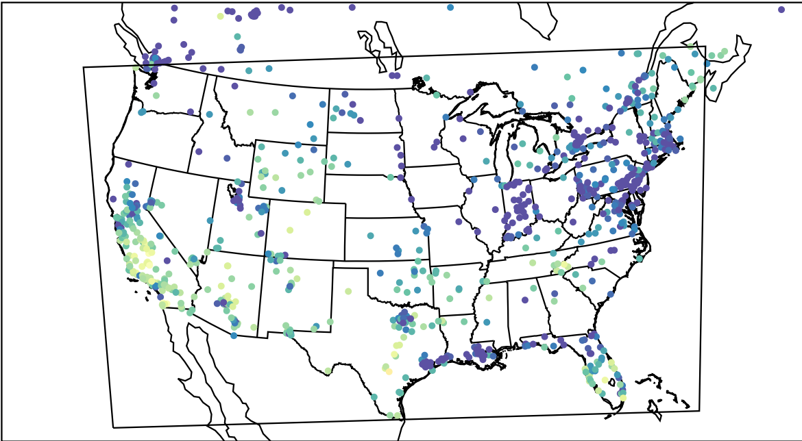
AirNOW (2023-12-05_23:00:00)
