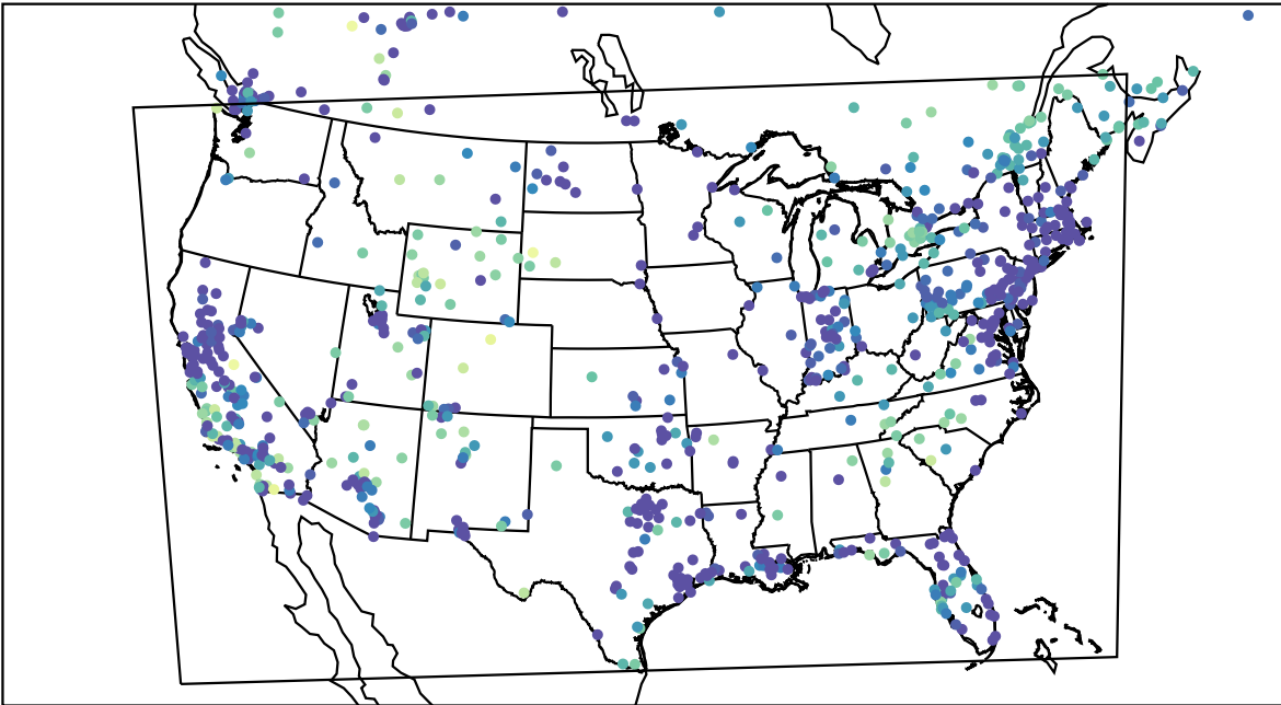
AirNOW (2023-12-05_01:00:00)
