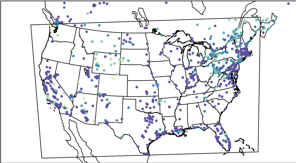
AirNOW (2023-12-05_10:00:00)
