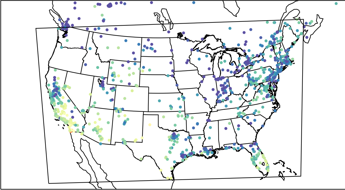
AirNOW (2023-12-06_23:00:00)
