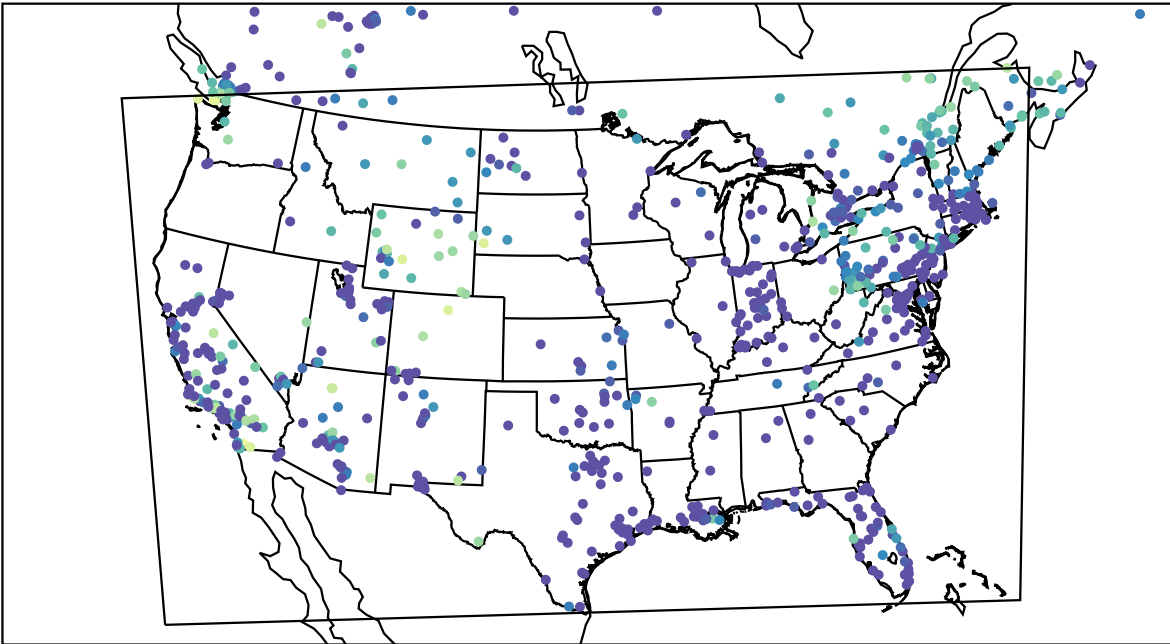
AirNOW (2023-12-05_12:00:00)
