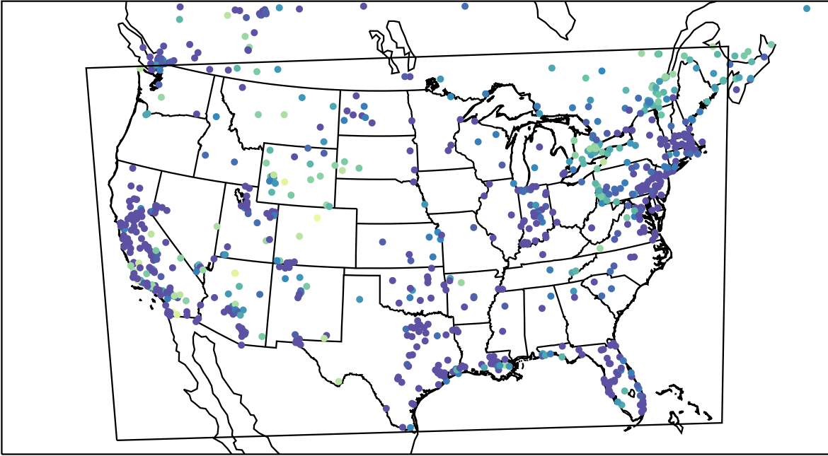
AirNOW (2023-12-05_07:00:00)
