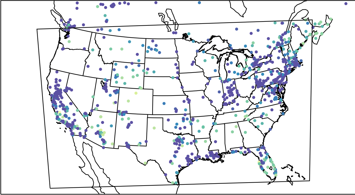
AirNOW (2023-12-06_02:00:00)
