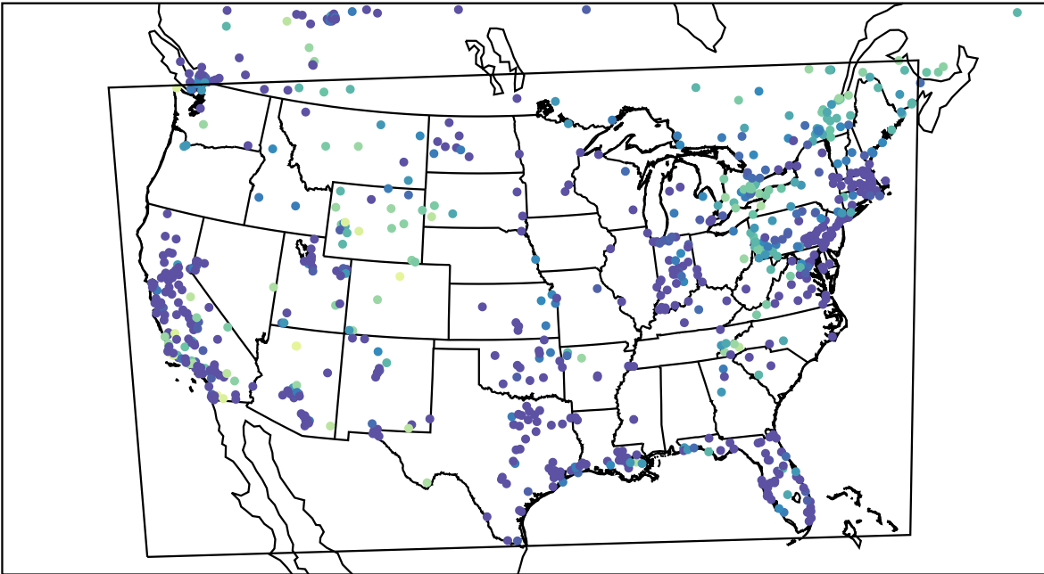
AirNOW (2023-12-05_08:00:00)
