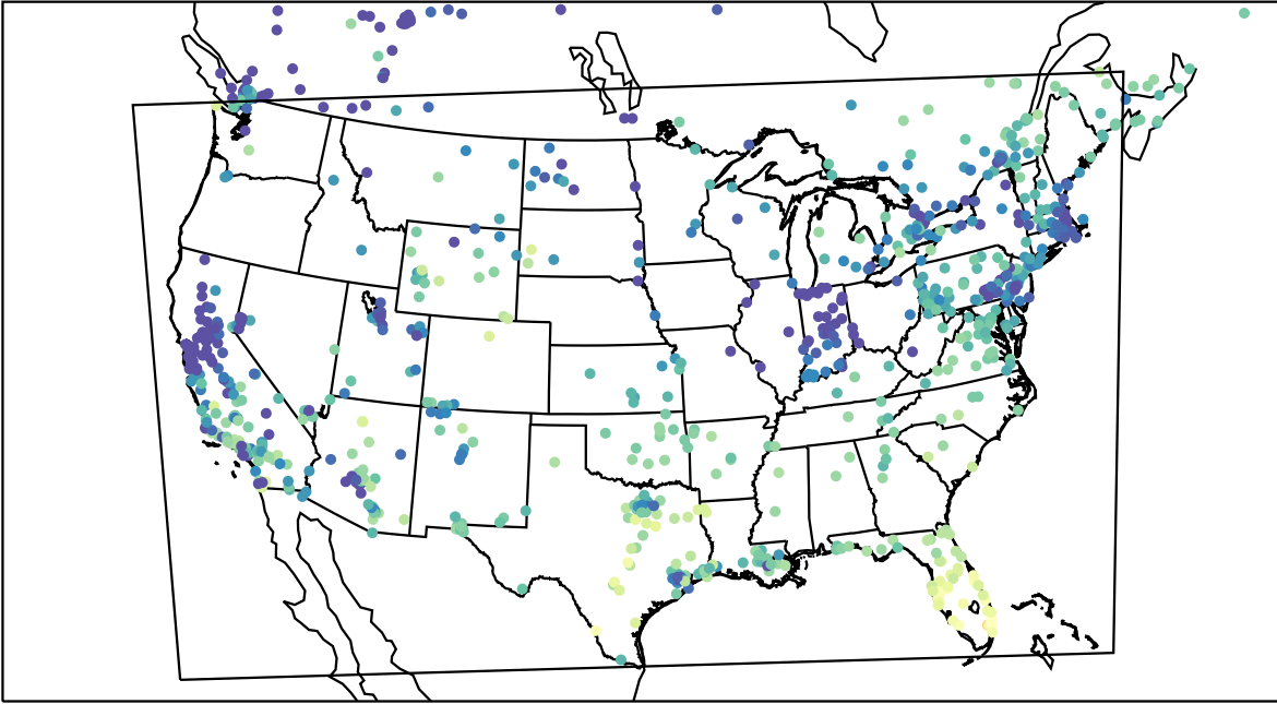
AirNOW (2023-12-05_18:00:00)
