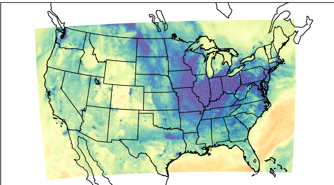
WRF (2023-12-06_00:00:00)
