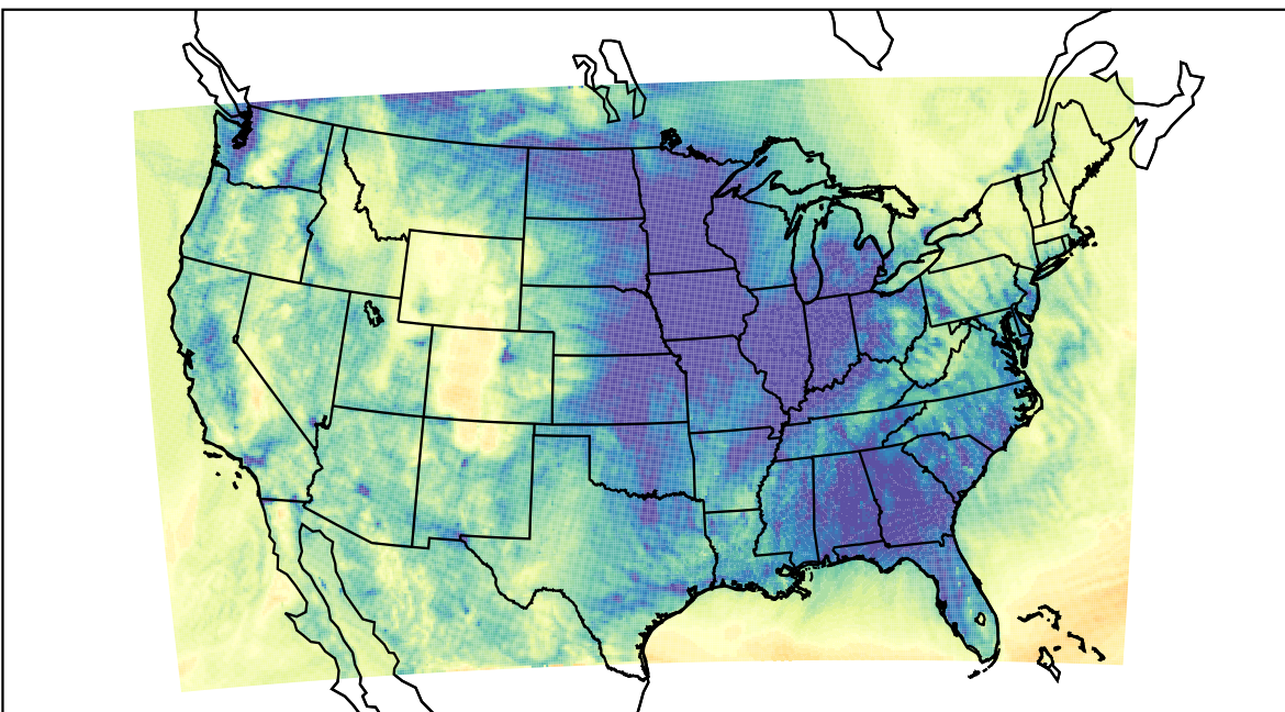
WRF (2023-12-07_03:00:00)
