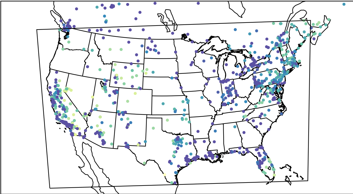
AirNOW (2023-12-07_05:00:00)
