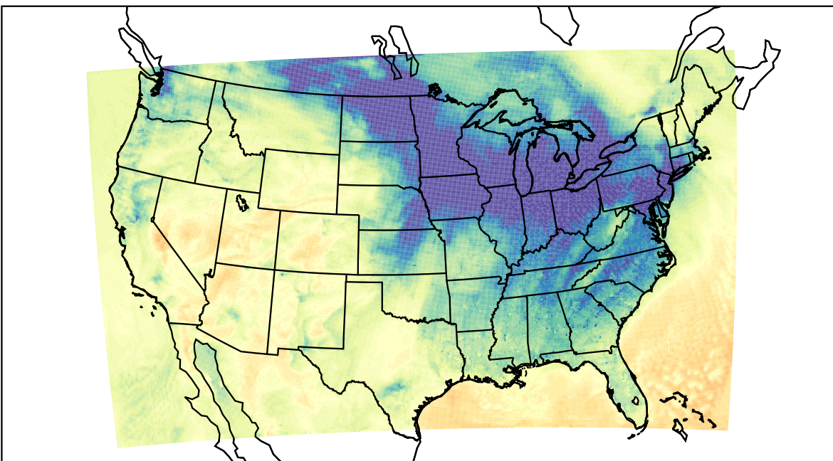
WRF (2023-12-07_22:00:00)
