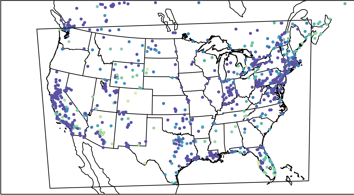
AirNOW (2023-12-06_04:00:00)
