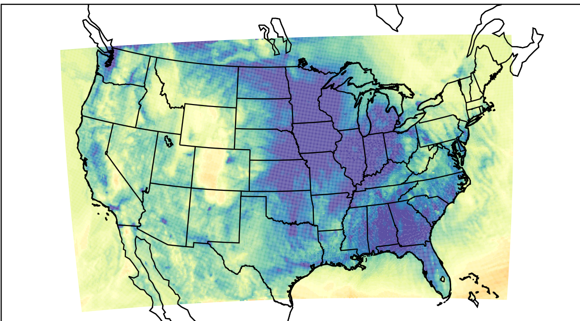
WRF (2023-12-07_04:00:00)
