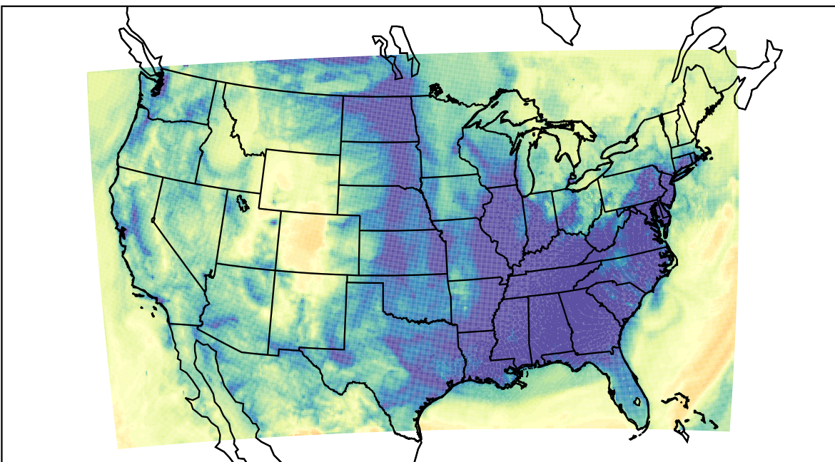
WRF (2023-12-06_11:00:00)
