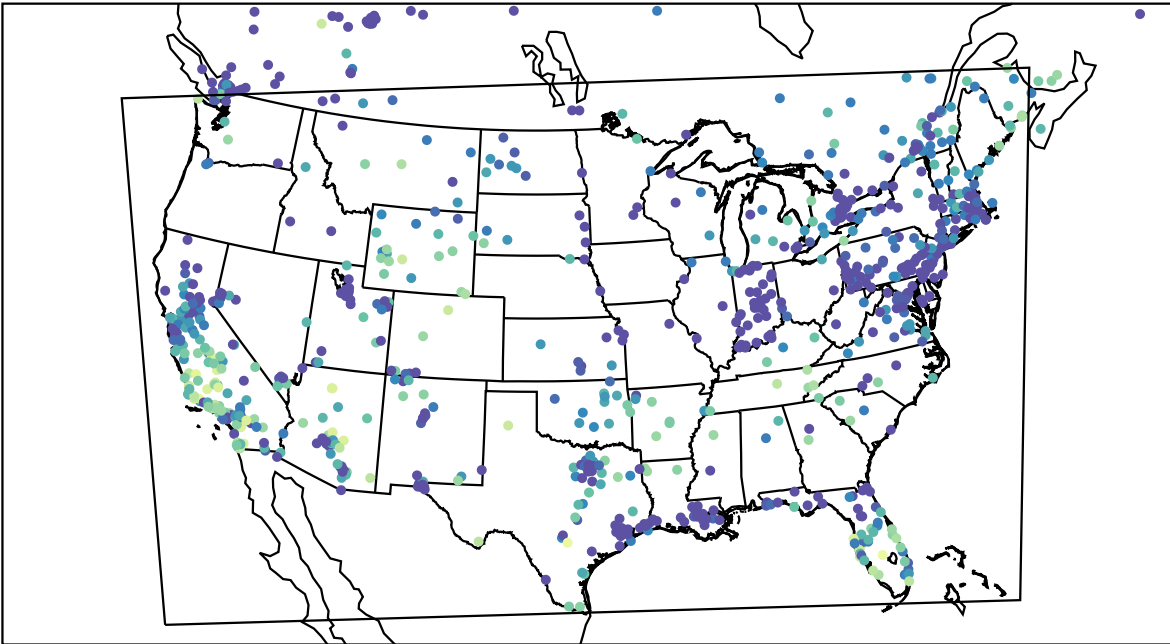
AirNOW (2023-12-06_00:00:00)
