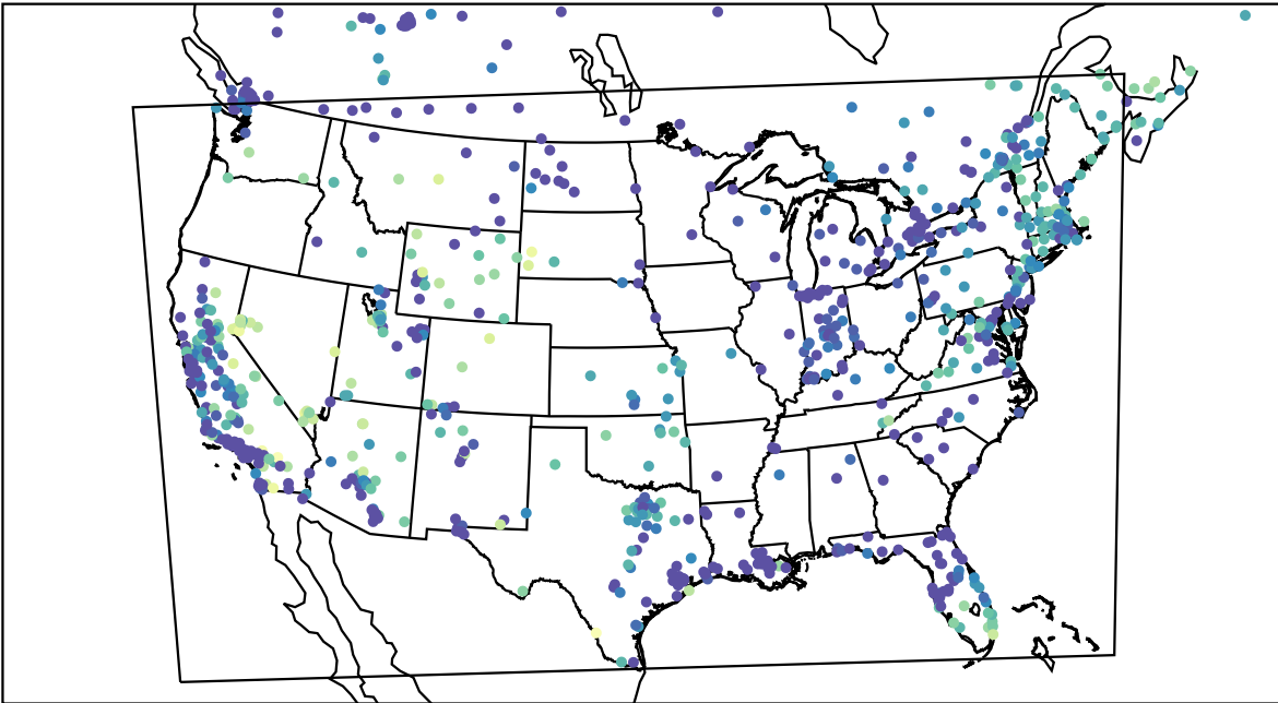
AirNOW (2023-12-07_06:00:00)
