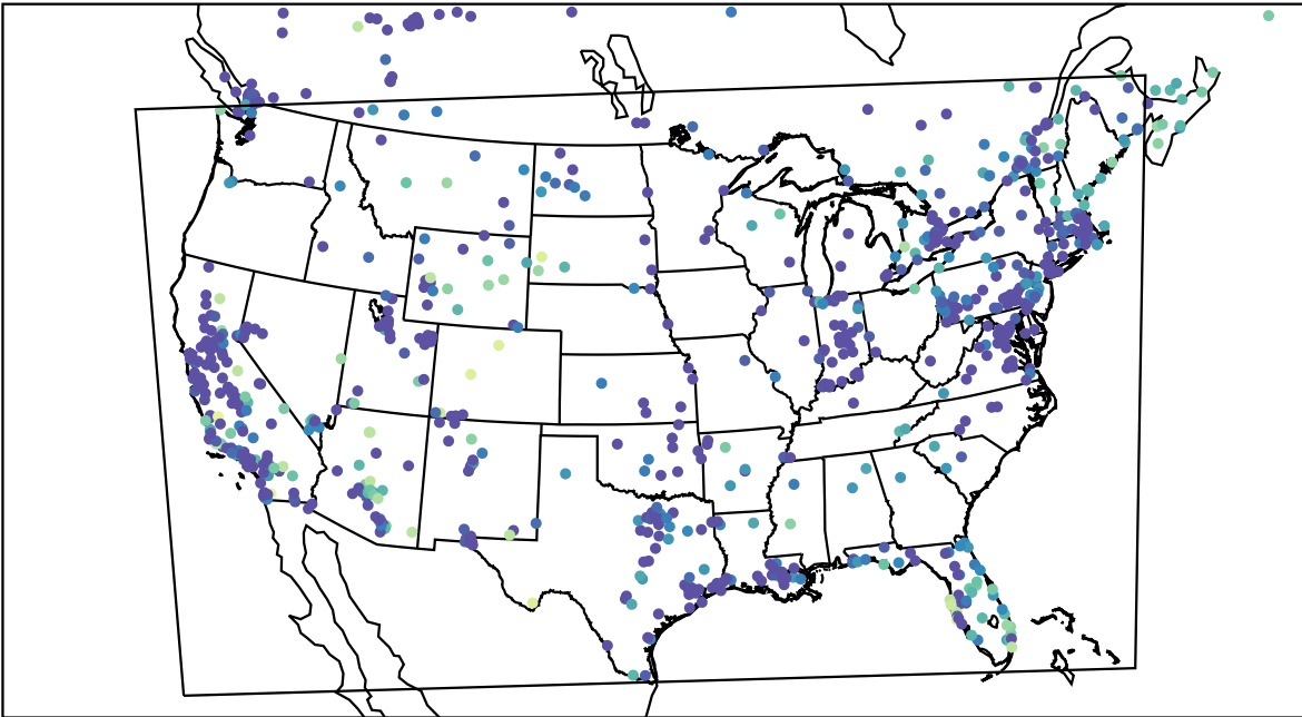
AirNOW (2023-12-06_07:00:00)
