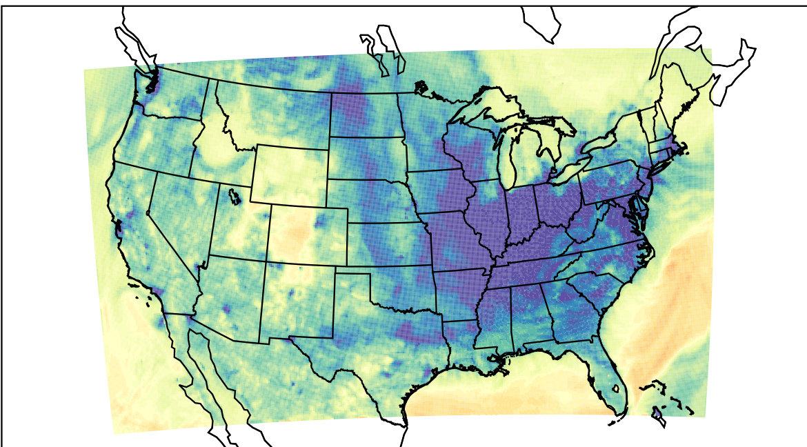
WRF (2023-12-06_03:00:00)
