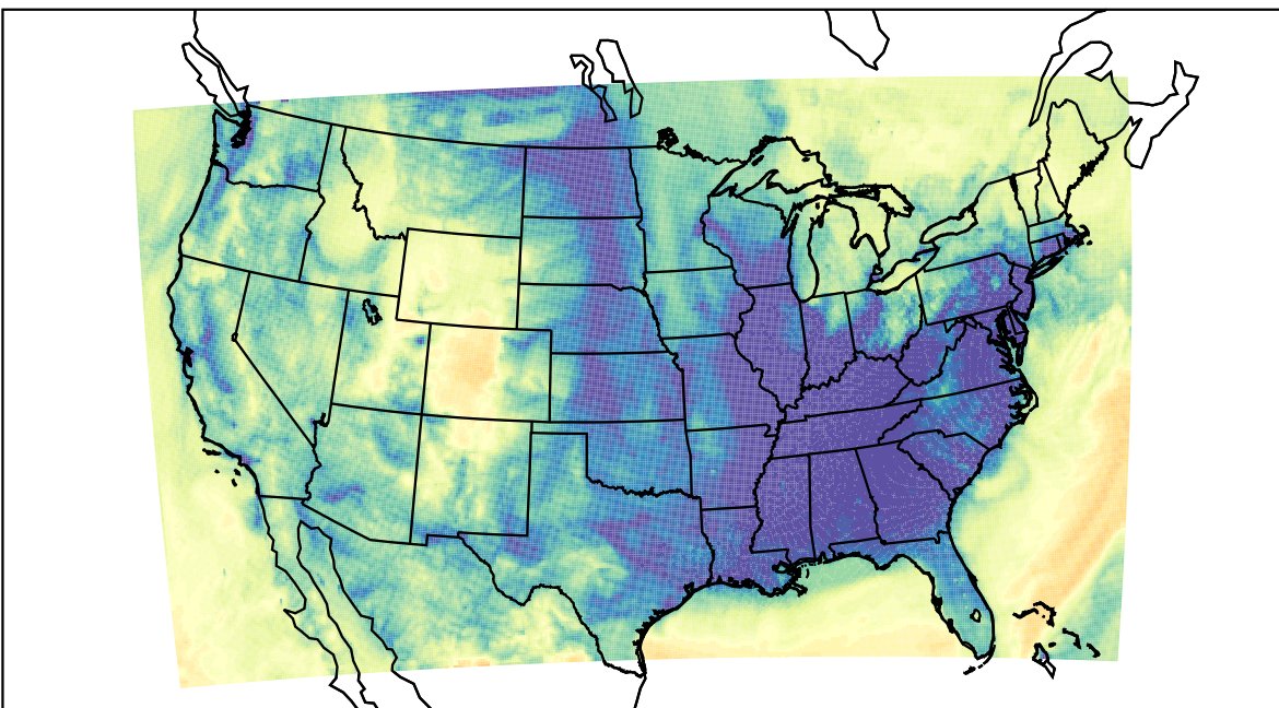
WRF (2023-12-06_09:00:00)
