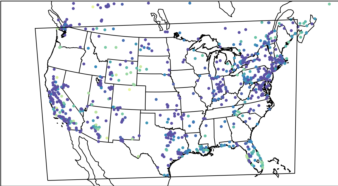
AirNOW (2023-12-06_09:00:00)
