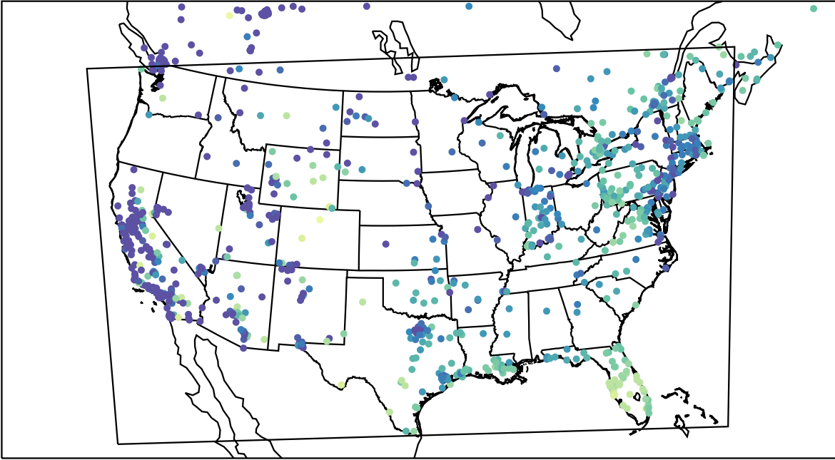
AirNOW (2023-12-06_16:00:00)
