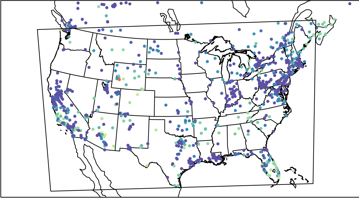
AirNOW (2023-12-06_01:00:00)
