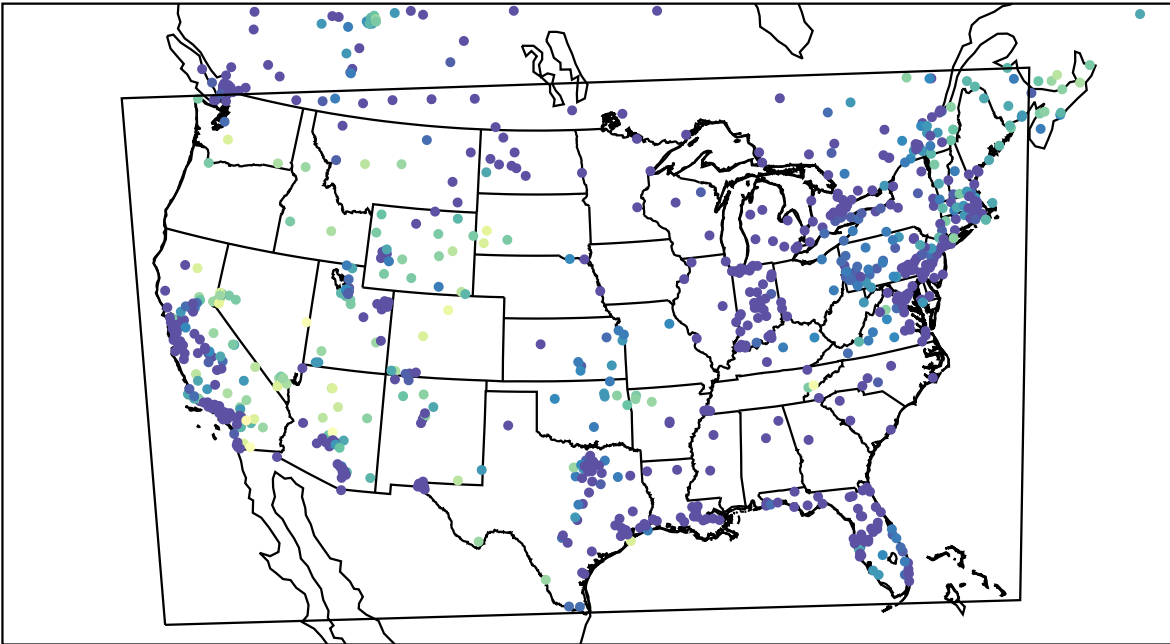
AirNOW (2023-12-07_12:00:00)
