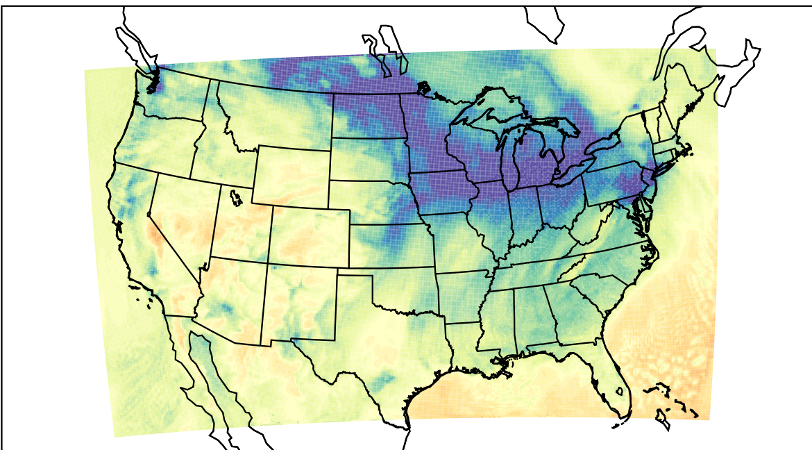
WRF (2023-12-07_20:00:00)
