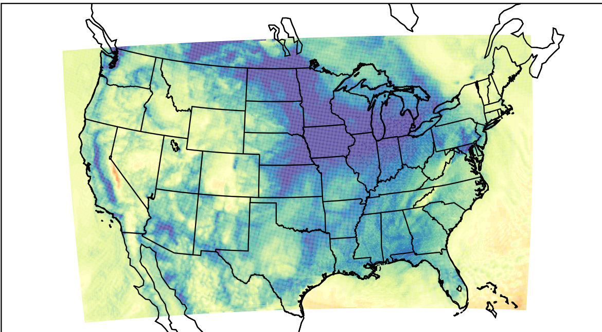
WRF (2023-12-07_16:00:00)
