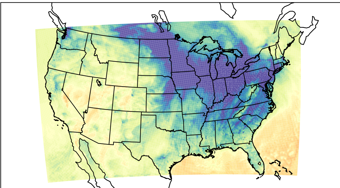
WRF (2023-12-07_23:00:00)
