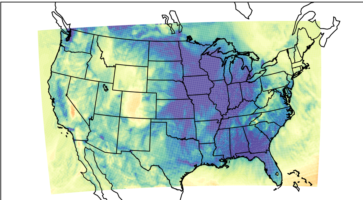
WRF (2023-12-07_07:00:00)
