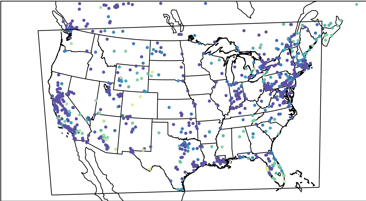
AirNOW (2023-12-06_05:00:00)
