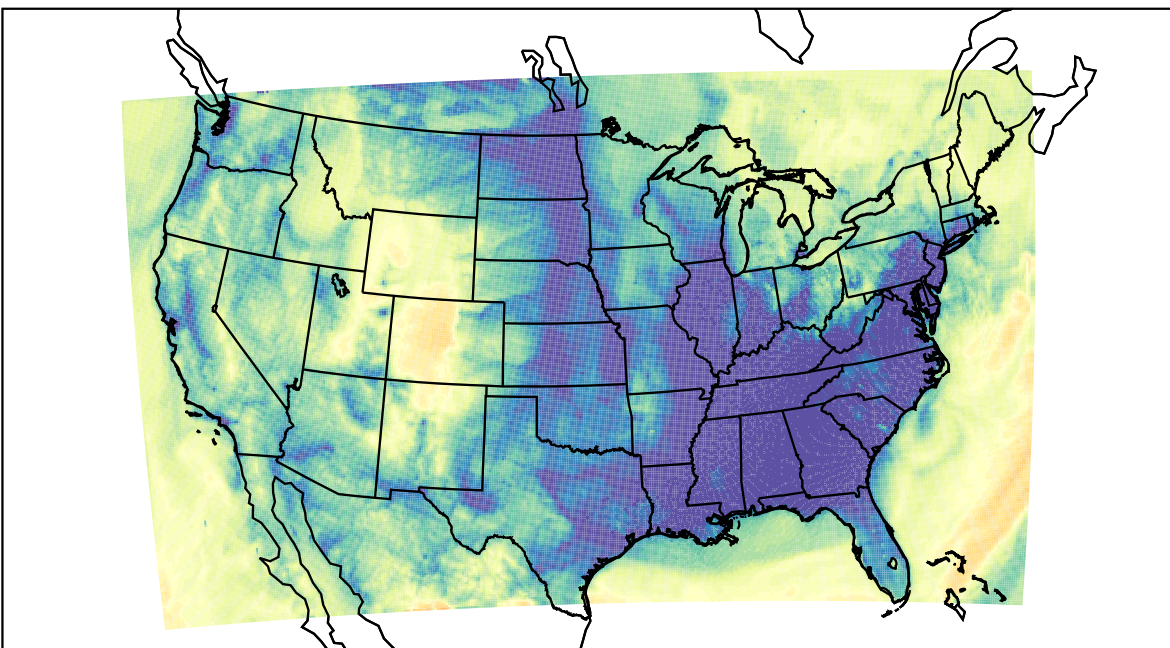
WRF (2023-12-06_12:00:00)
