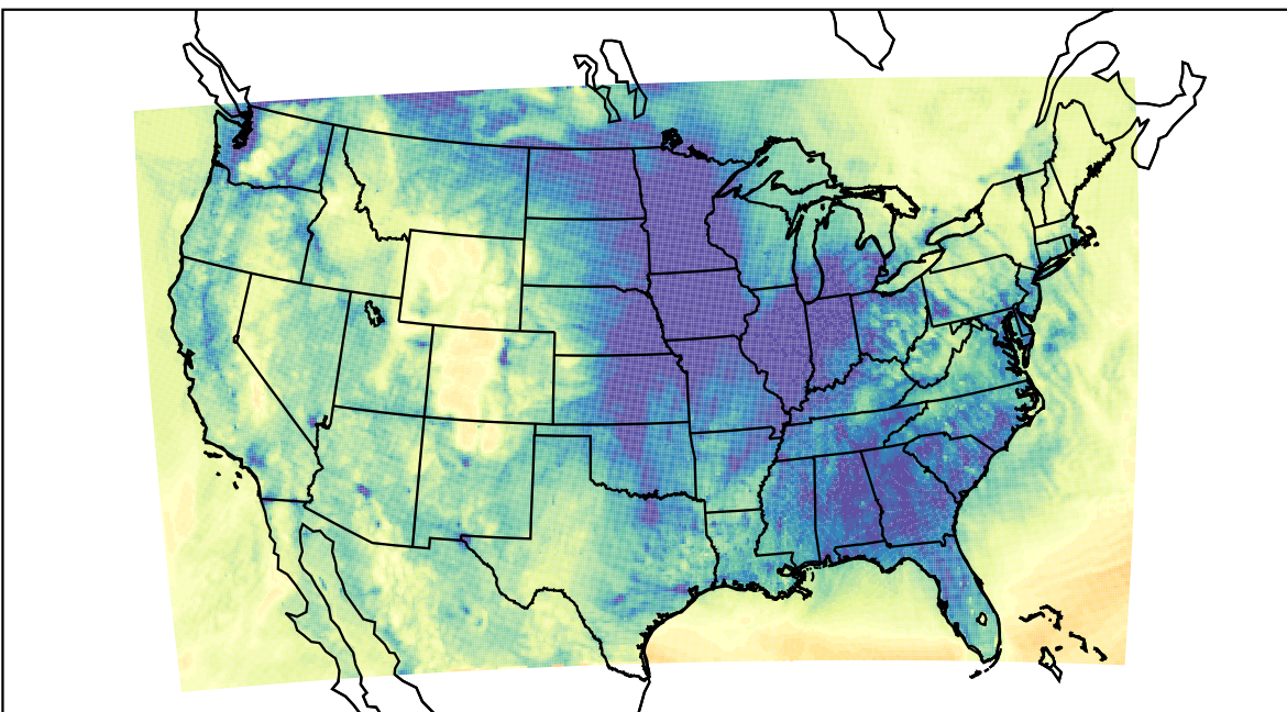
WRF (2023-12-07_01:00:00)
