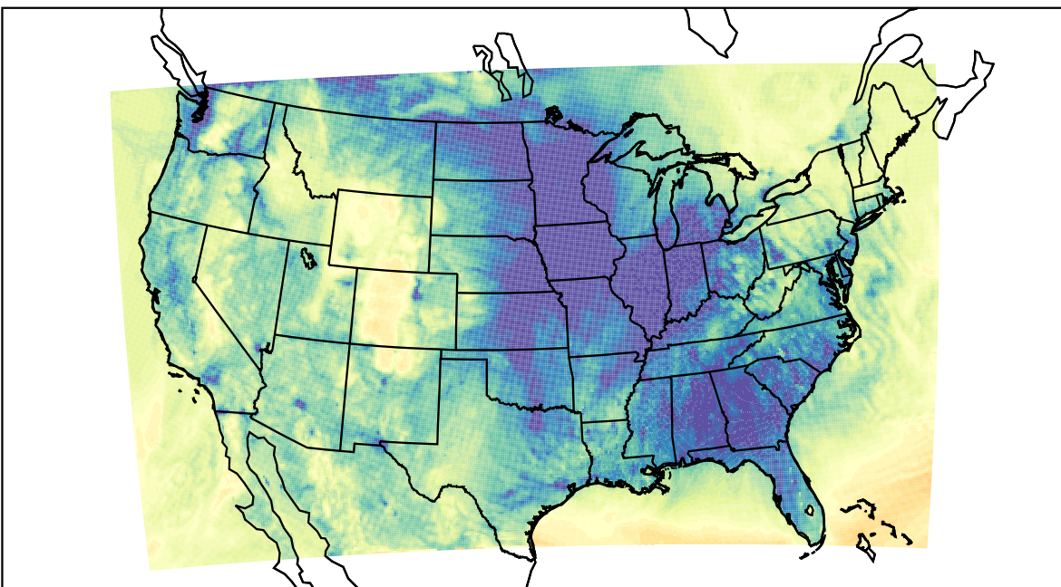
WRF (2023-12-07_02:00:00)
