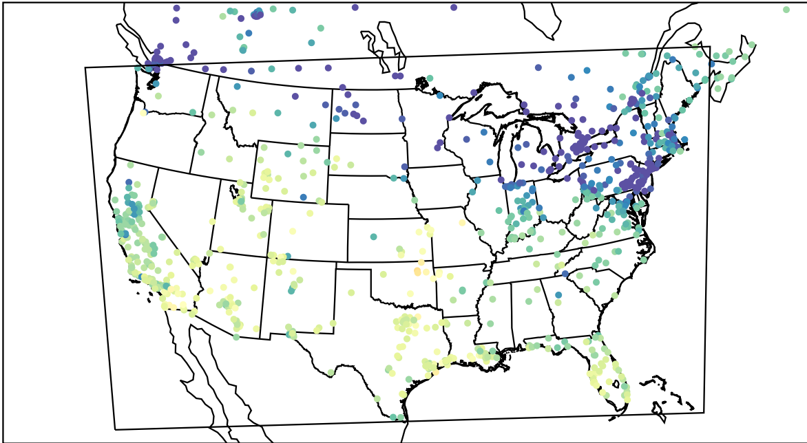
AirNOW (2023-12-07_21:00:00)
