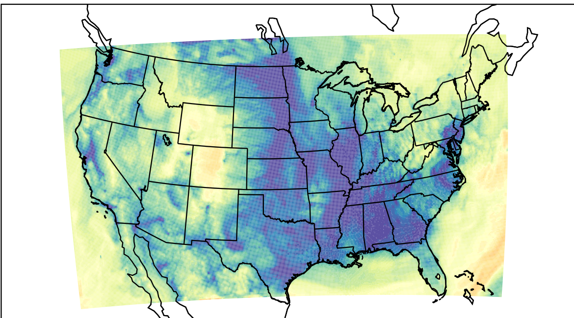
WRF (2023-12-06_15:00:00)
