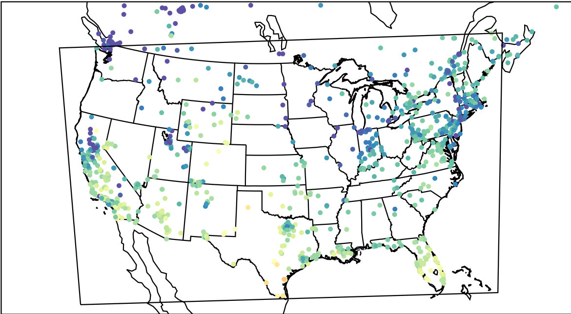
AirNOW (2023-12-06_20:00:00)
