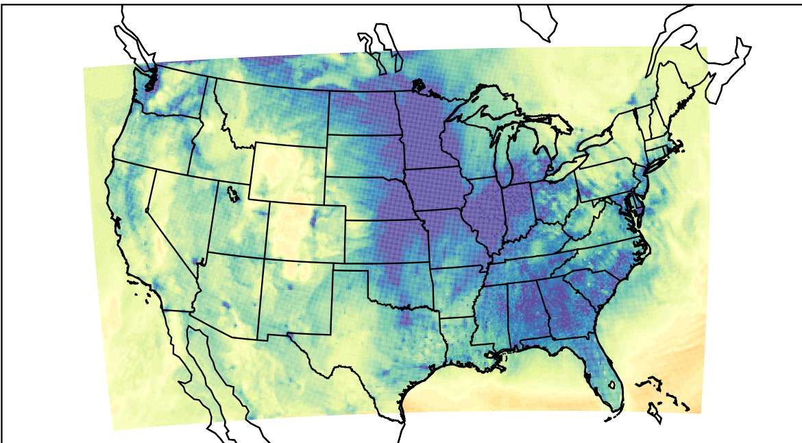
WRF (2023-12-07_00:00:00)
