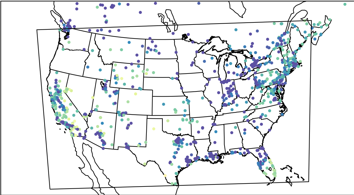
AirNOW (2023-12-07_02:00:00)
