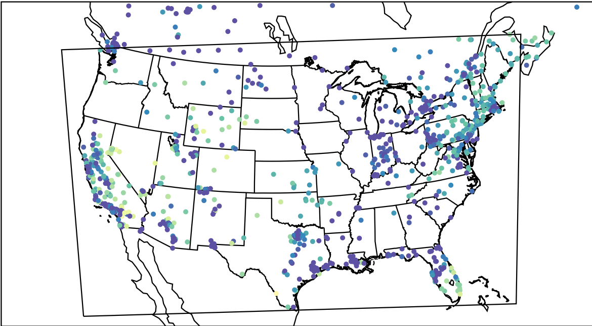
AirNOW (2023-12-07_04:00:00)
