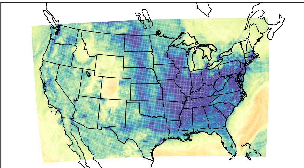
WRF (2023-12-06_05:00:00)
