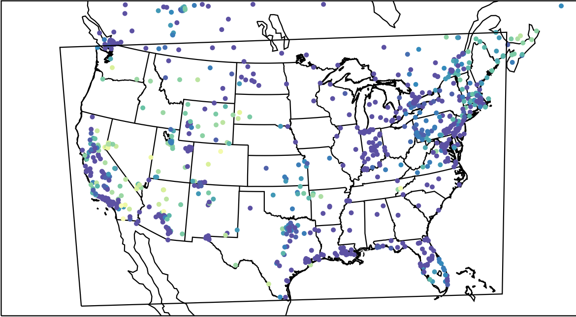
AirNOW (2023-12-07_11:00:00)
