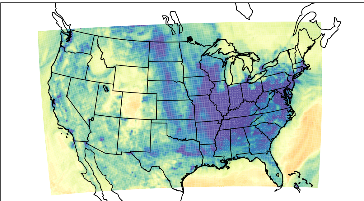
WRF (2023-12-06_04:00:00)
