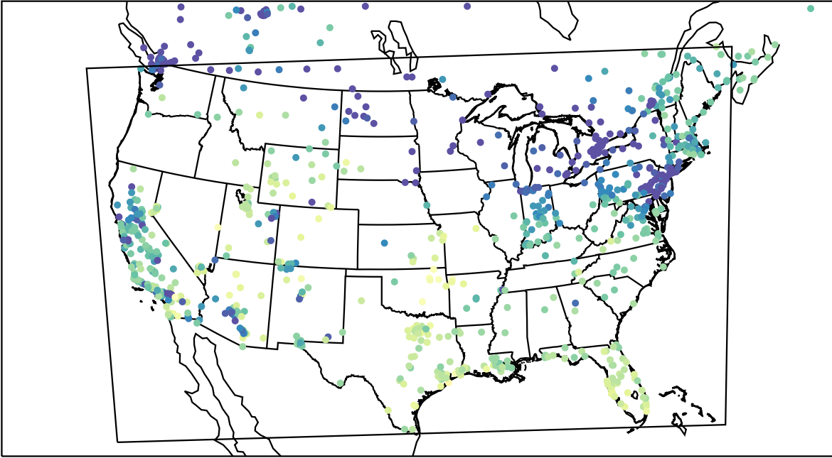
AirNOW (2023-12-07_18:00:00)
