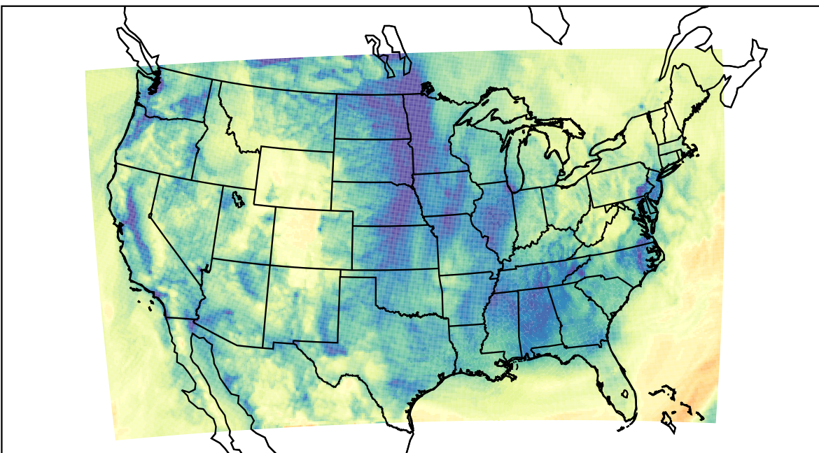
WRF (2023-12-06_17:00:00)
