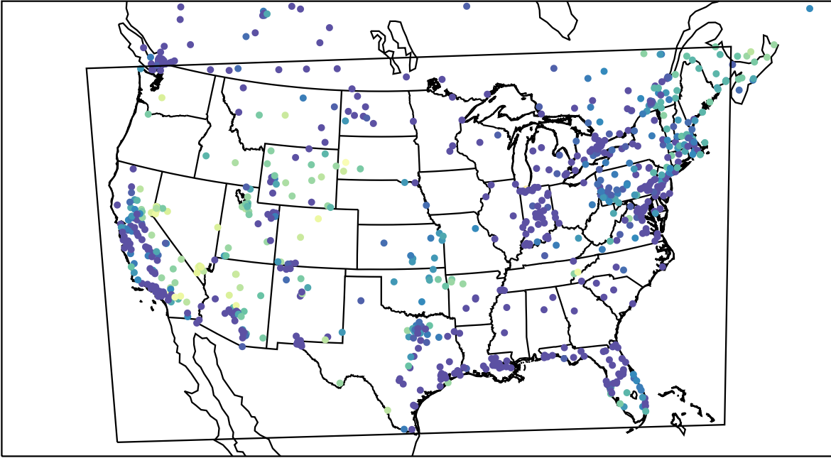
AirNOW (2023-12-07_10:00:00)
