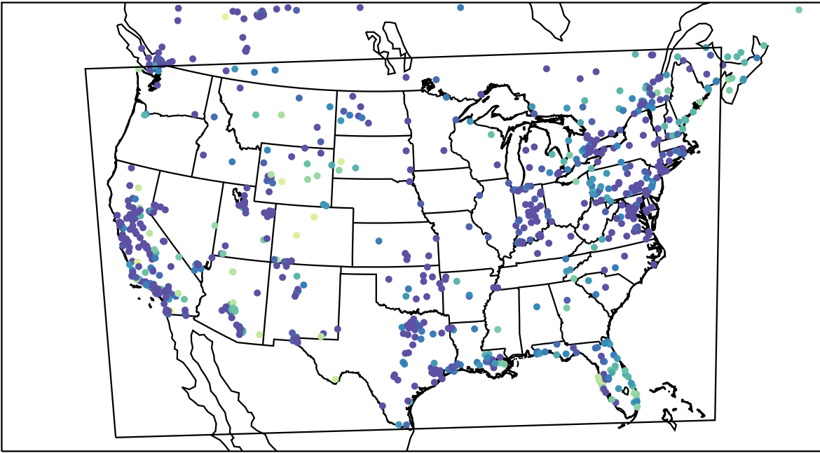
AirNOW (2023-12-06_08:00:00)
