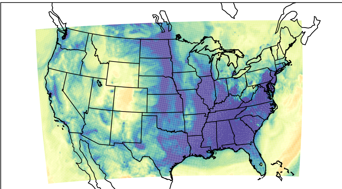
WRF (2023-12-06_13:00:00)
