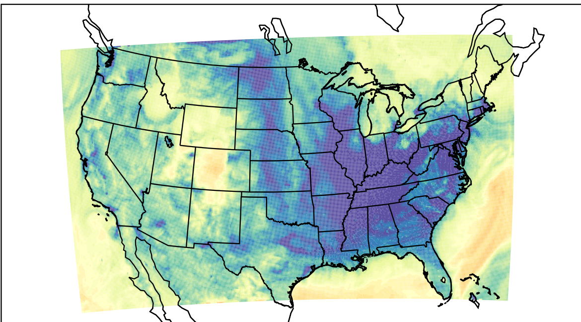
WRF (2023-12-06_06:00:00)
