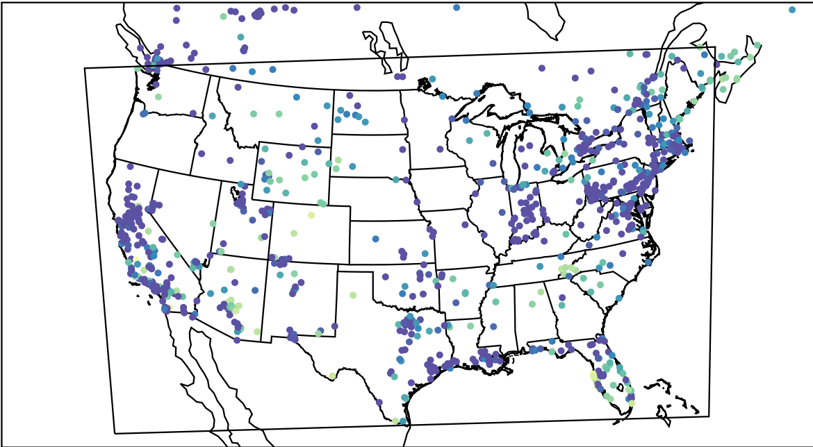
AirNOW (2023-12-06_03:00:00)
