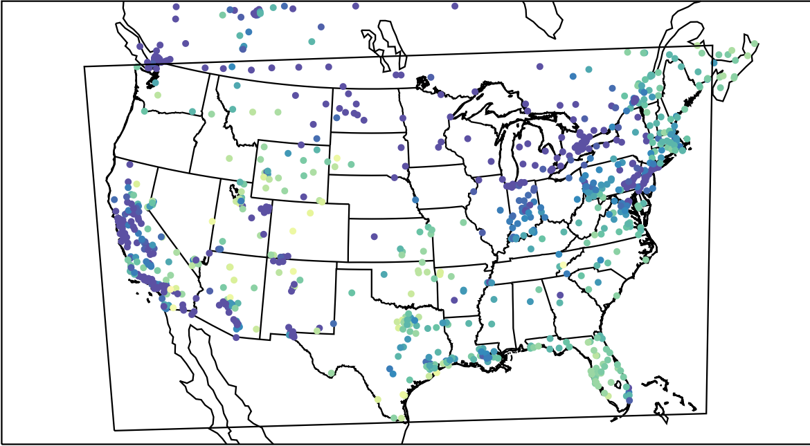
AirNOW (2023-12-07_16:00:00)
