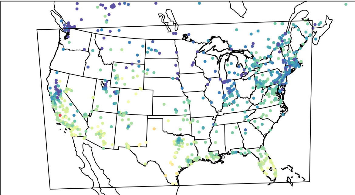
AirNOW (2023-12-06_21:00:00)
