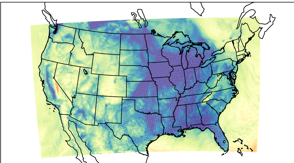
WRF (2023-12-07_14:00:00)
