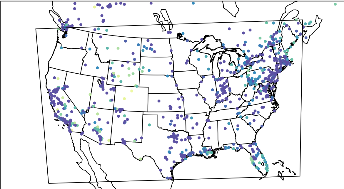
AirNOW (2023-12-06_12:00:00)
