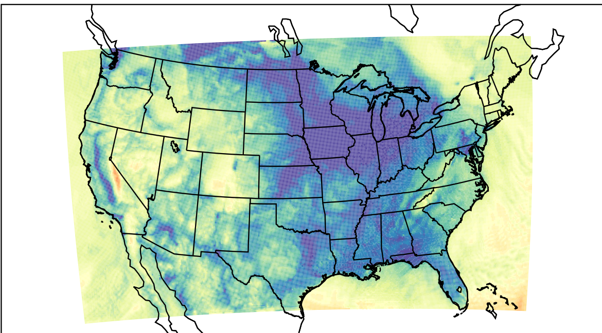
WRF (2023-12-07_15:00:00)
