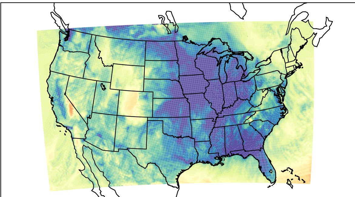
WRF (2023-12-07_08:00:00)
