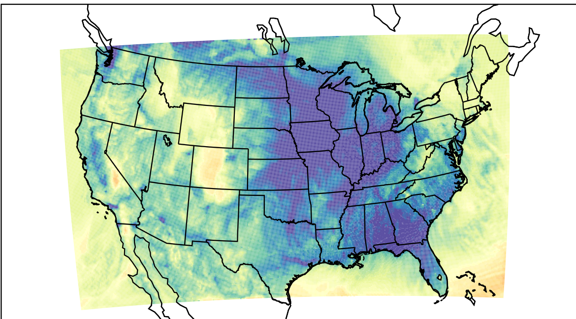
WRF (2023-12-07_06:00:00)
