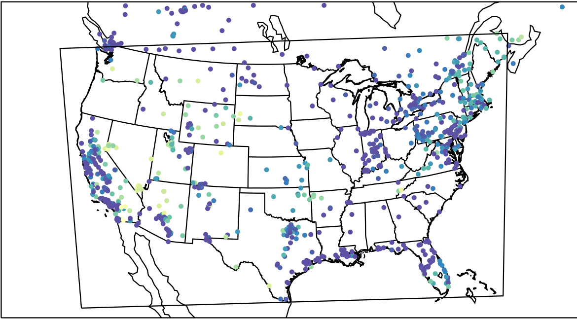
AirNOW (2023-12-07_09:00:00)
