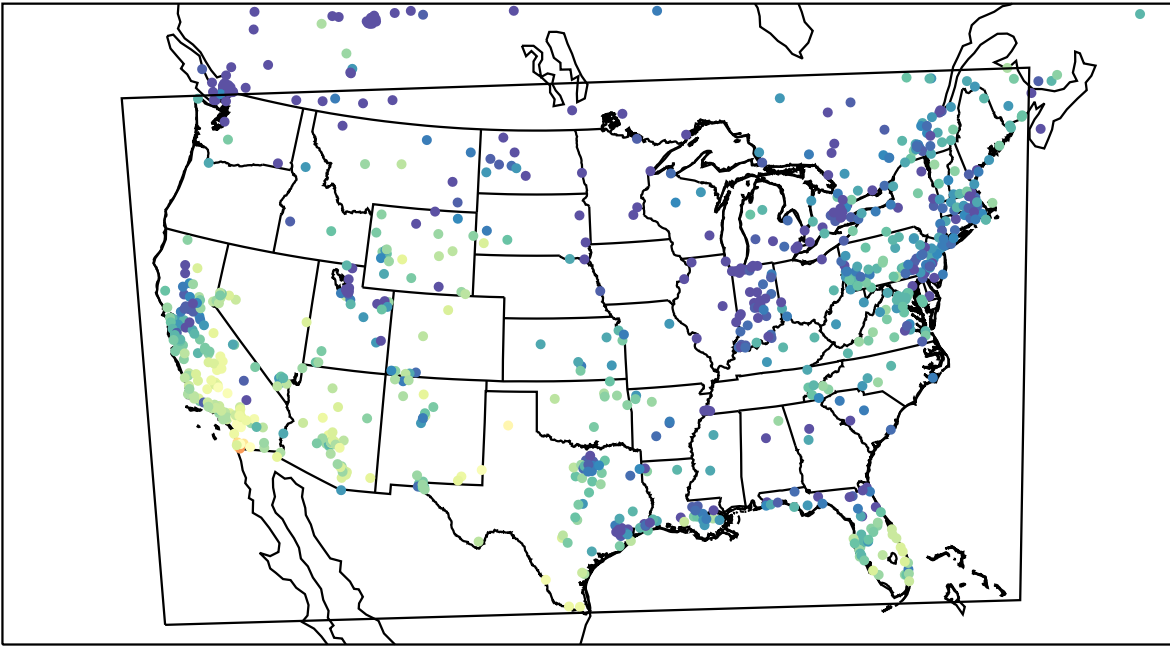
AirNOW (2023-12-06_23:00:00)
