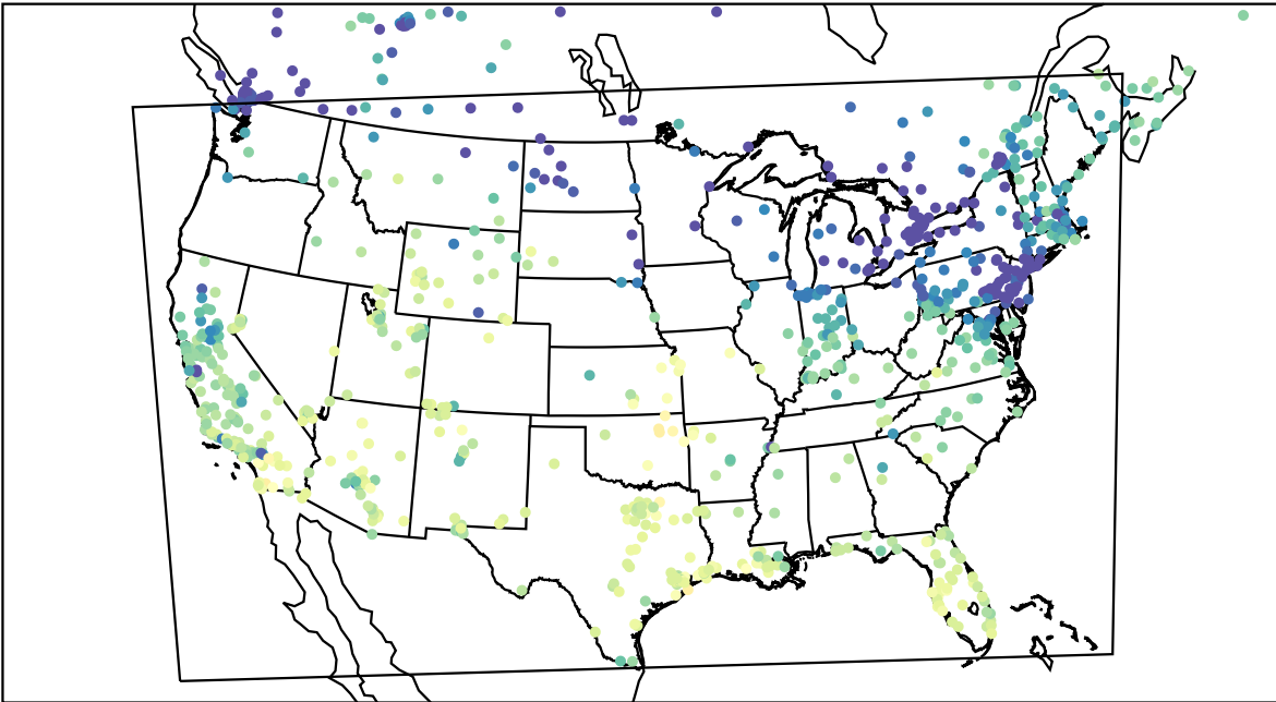
AirNOW (2023-12-07_20:00:00)
