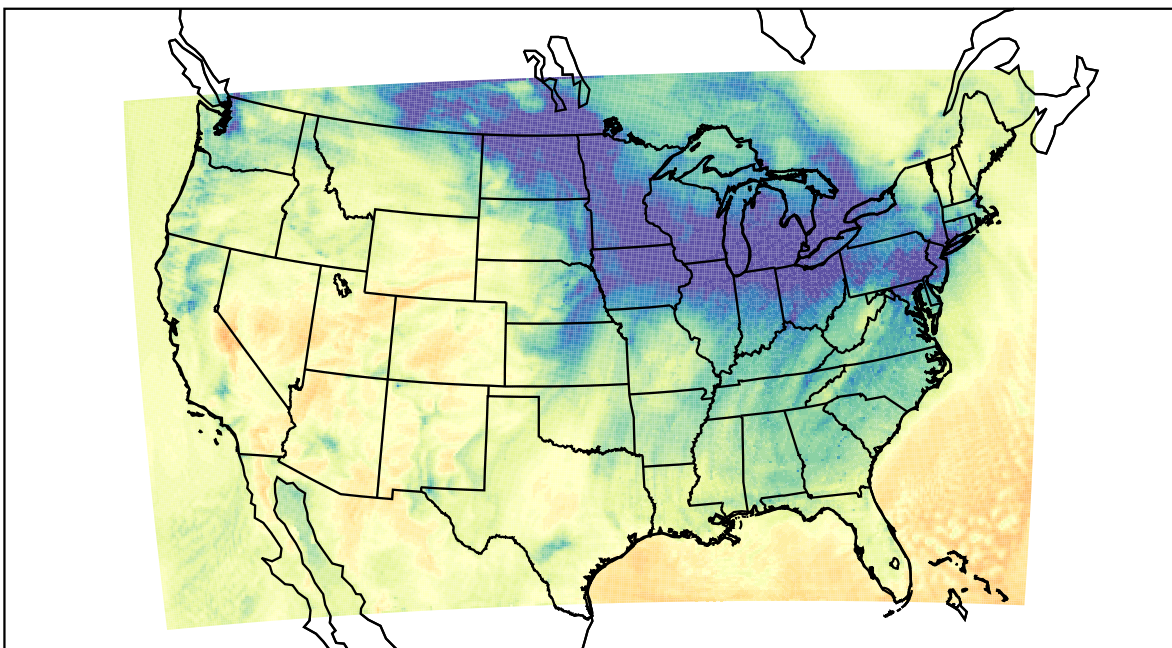
WRF (2023-12-07_21:00:00)
