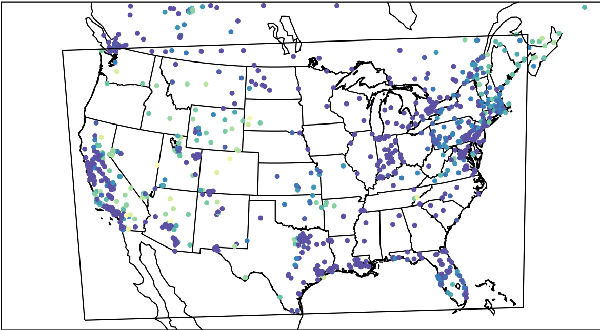
AirNOW (2023-12-07_13:00:00)
