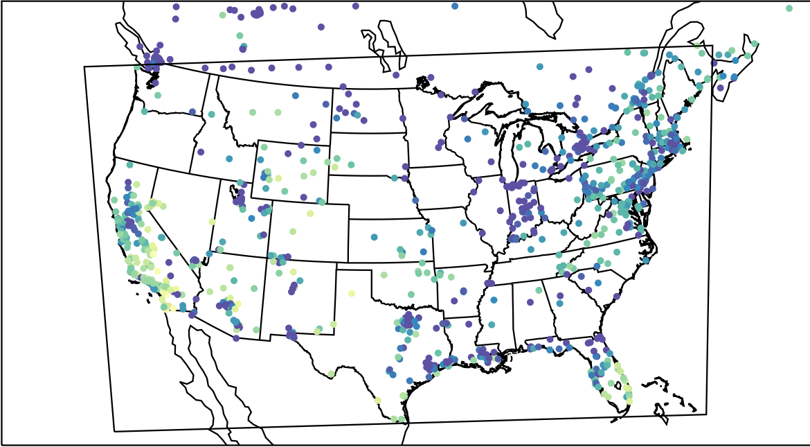
AirNOW (2023-12-07_00:00:00)
