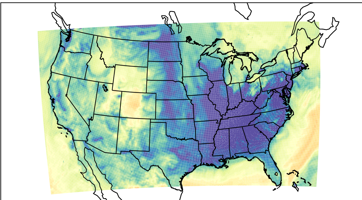
WRF (2023-12-06_08:00:00)
