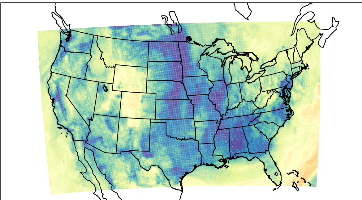
WRF (2023-12-06_16:00:00)
