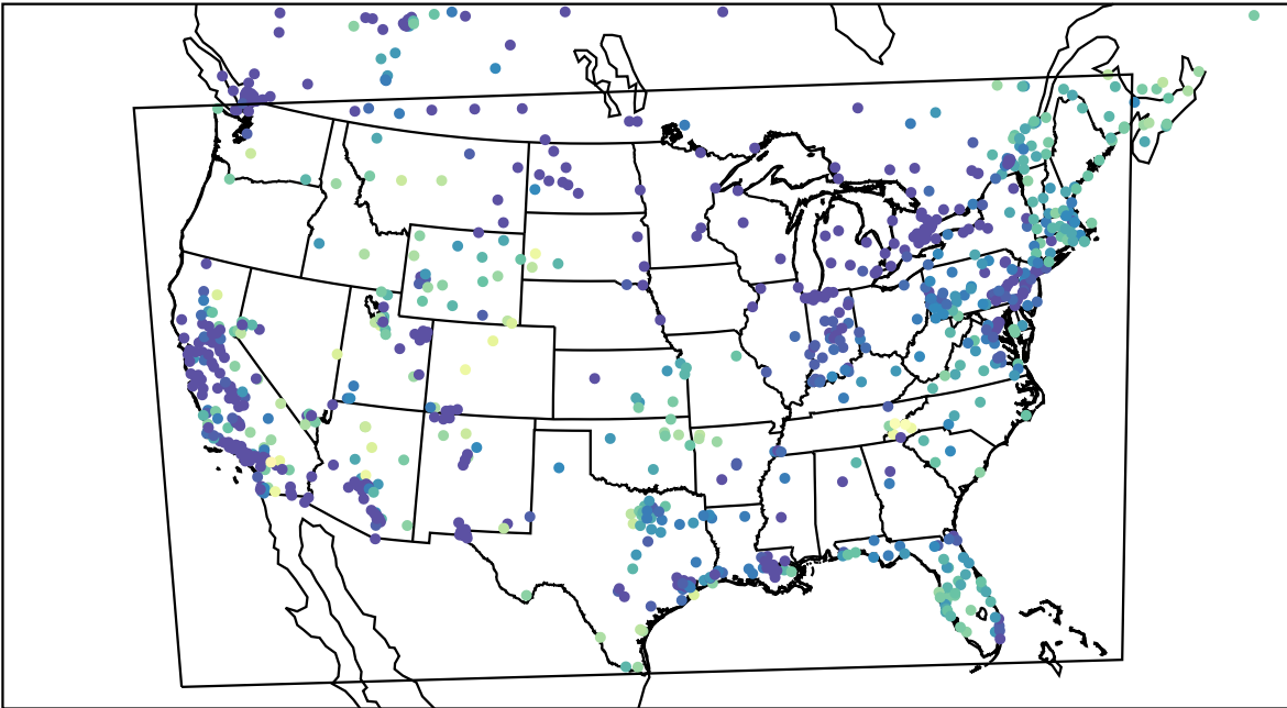
AirNOW (2023-12-07_15:00:00)
