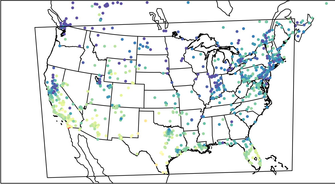
AirNOW (2023-12-06_22:00:00)
