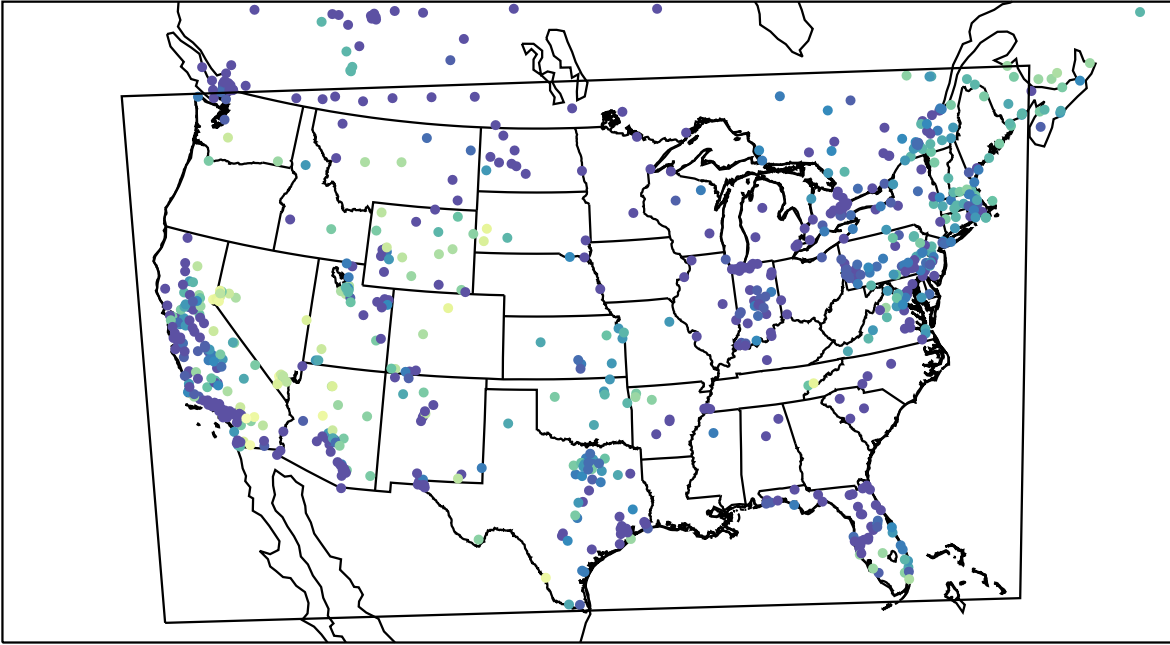
AirNOW (2023-12-07_07:00:00)
