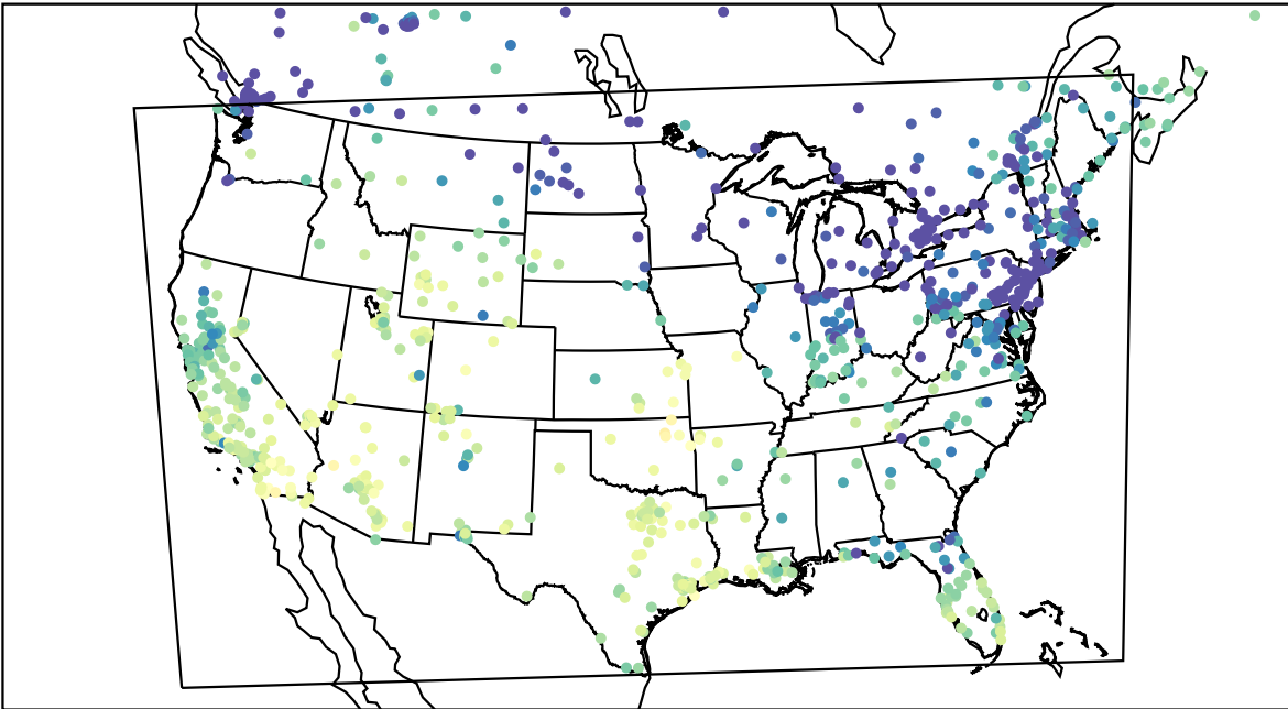
AirNOW (2023-12-07_22:00:00)
