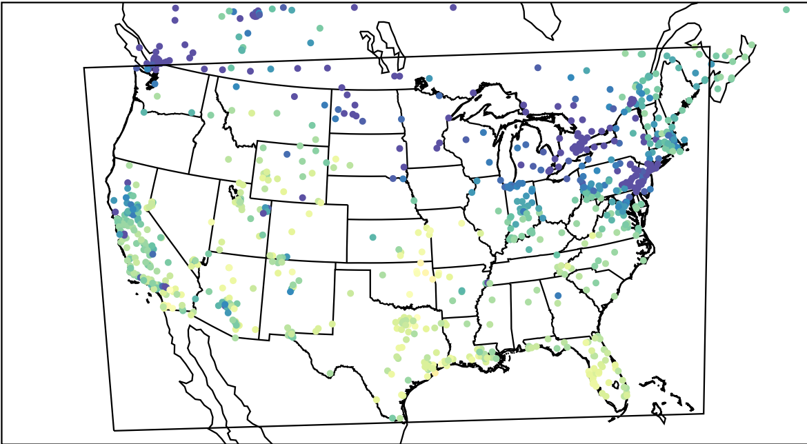
AirNOW (2023-12-07_19:00:00)
