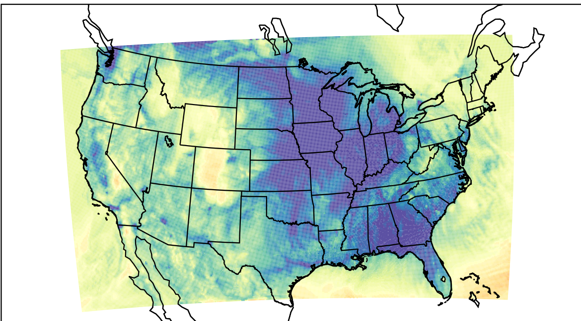
WRF (2023-12-07_05:00:00)
