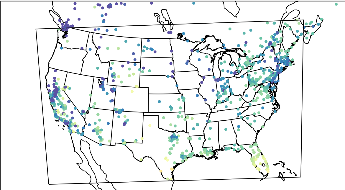
AirNOW (2023-12-06_18:00:00)
