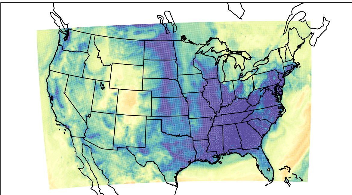
WRF (2023-12-06_10:00:00)
