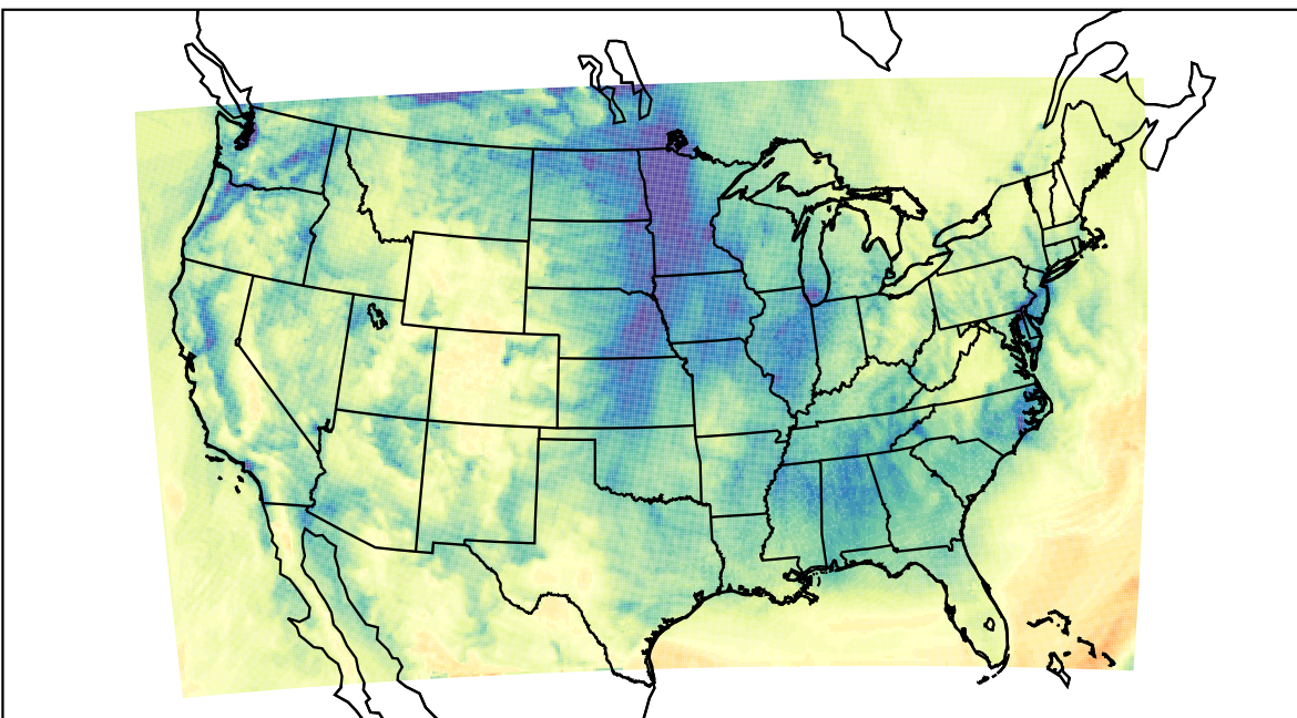
WRF (2023-12-06_19:00:00)
