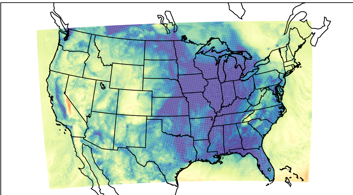
WRF (2023-12-07_13:00:00)
