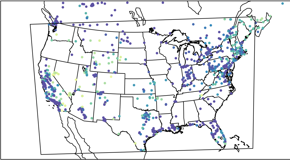
AirNOW (2023-12-07_08:00:00)
