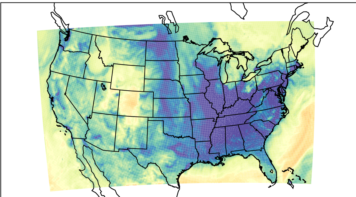
WRF (2023-12-06_07:00:00)
