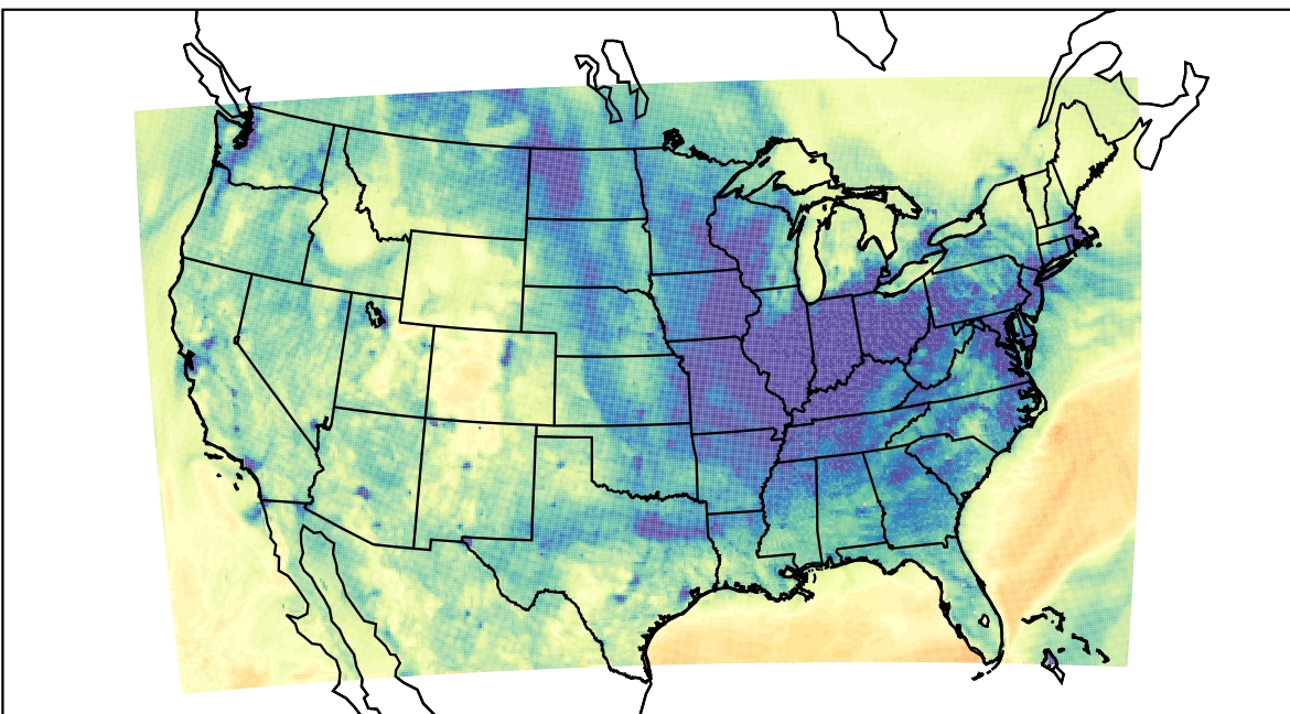
WRF (2023-12-06_01:00:00)
