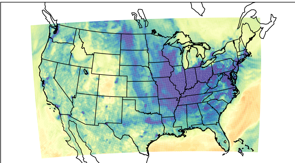
WRF (2023-12-06_02:00:00)
