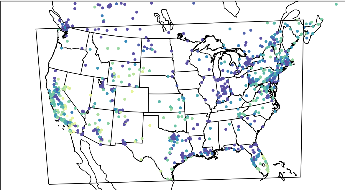
AirNOW (2023-12-07_01:00:00)
