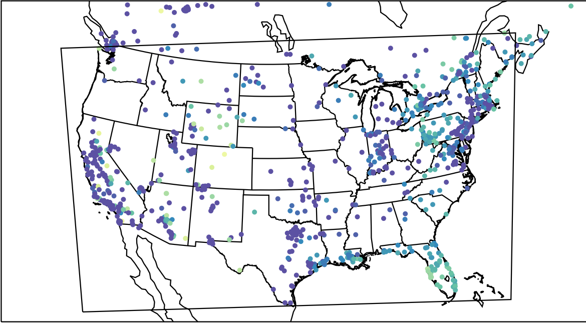
AirNOW (2023-12-06_14:00:00)
