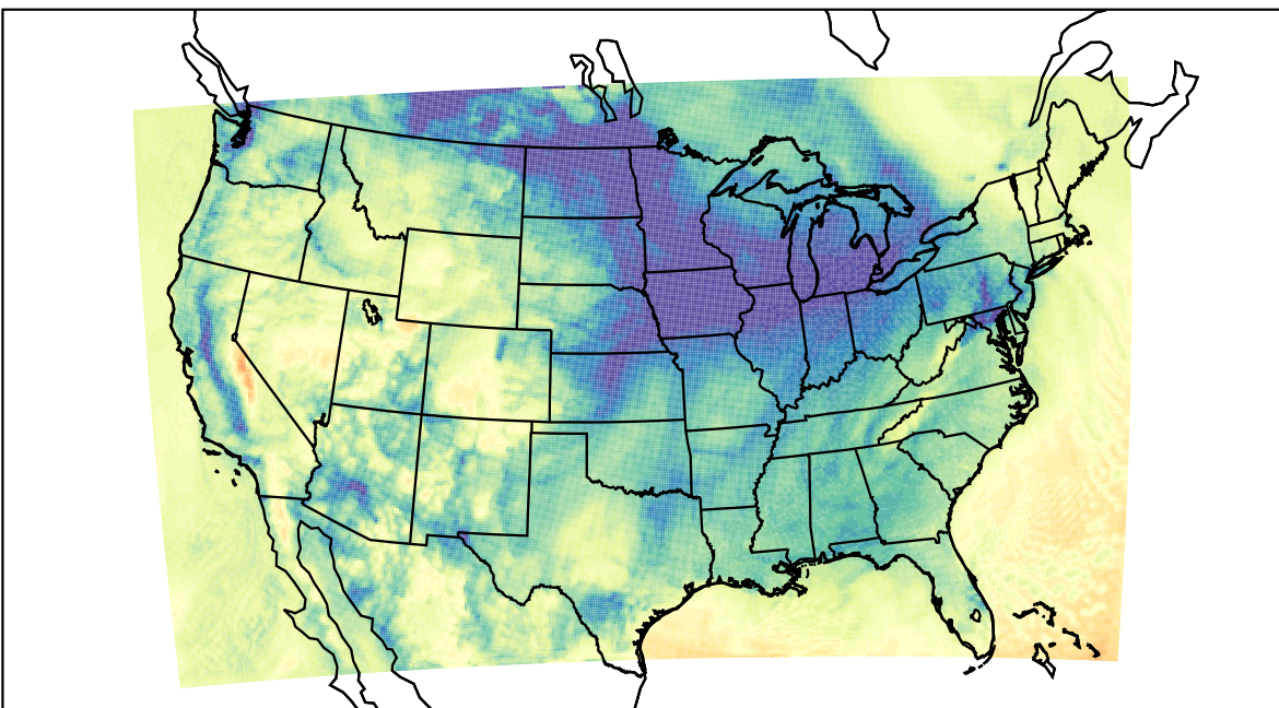
WRF (2023-12-07_17:00:00)
