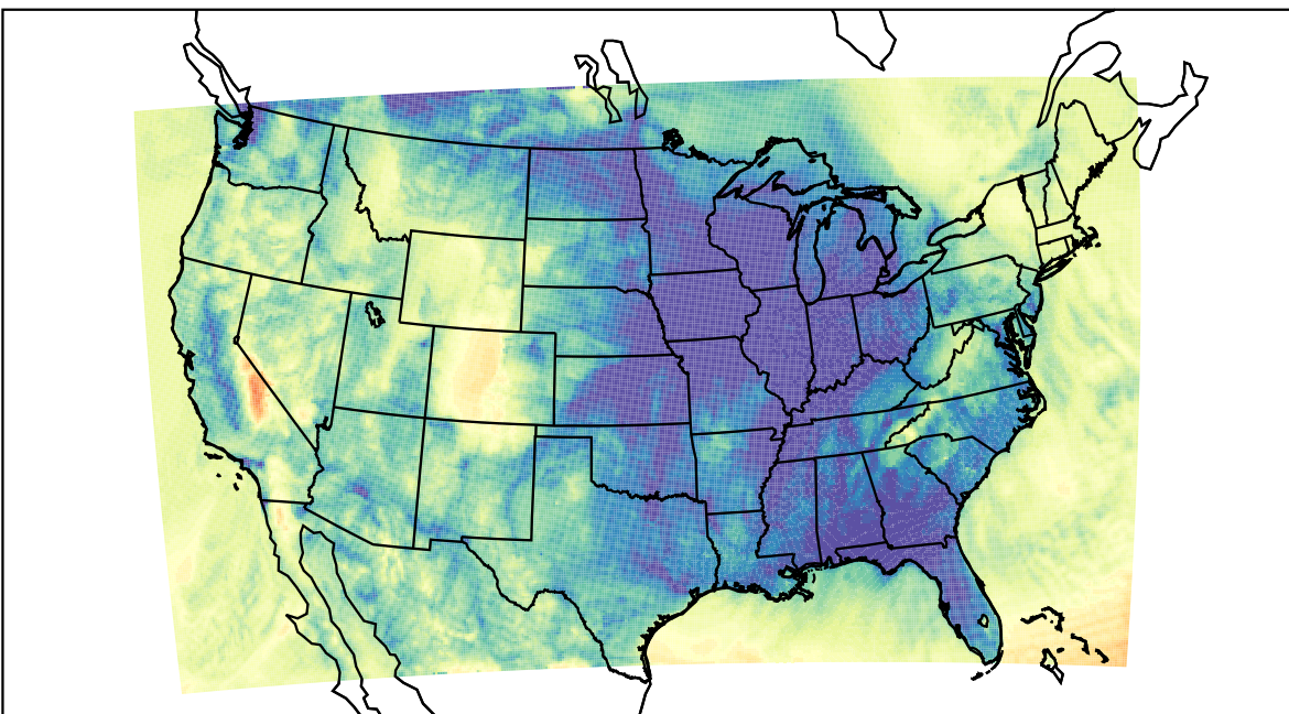
WRF (2023-12-07_09:00:00)
