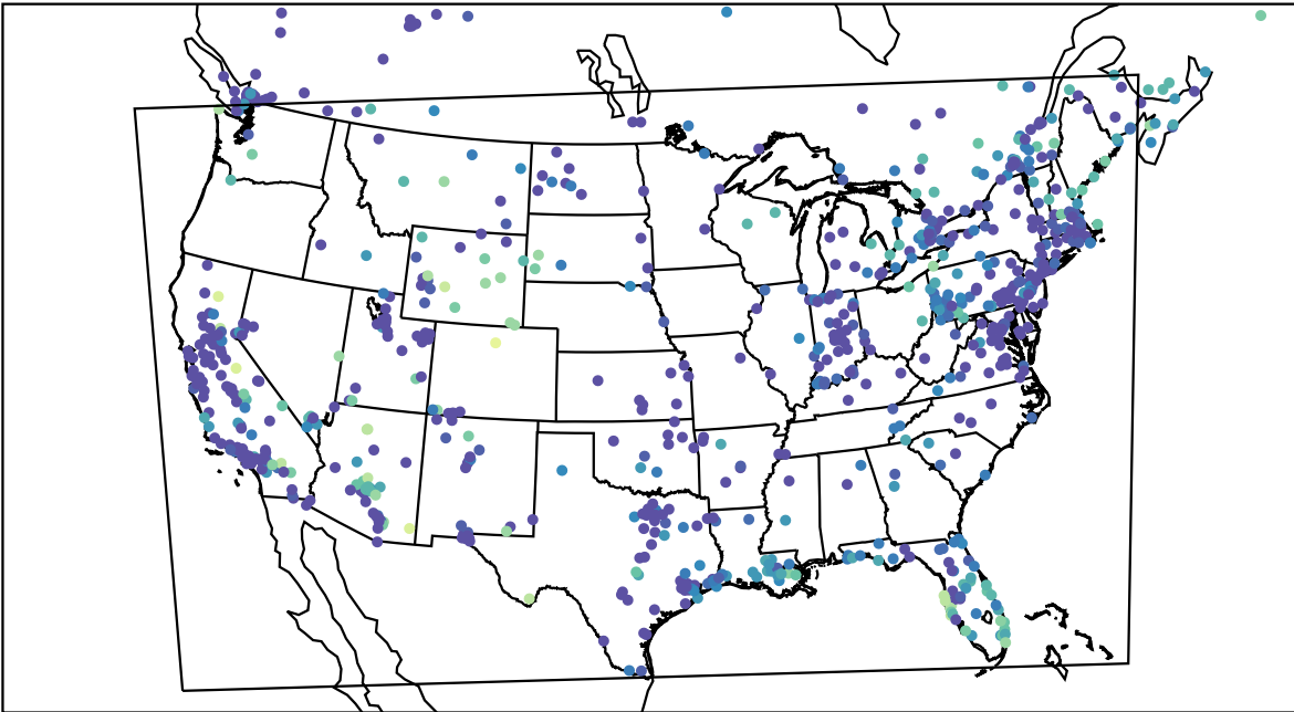
AirNOW (2023-12-06_10:00:00)
