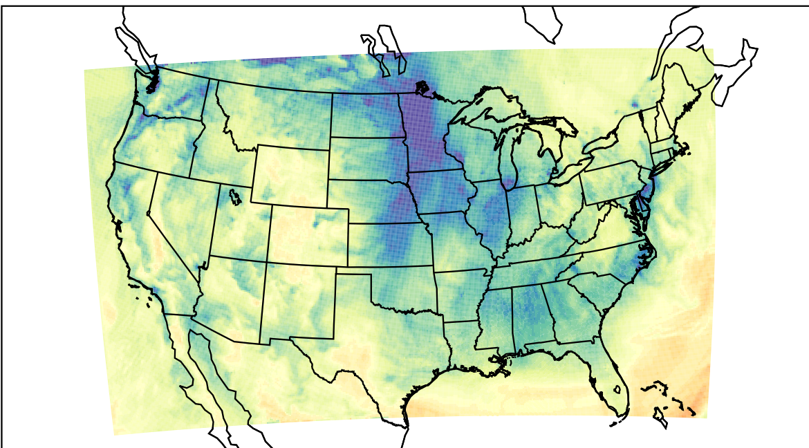
WRF (2023-12-06_20:00:00)
