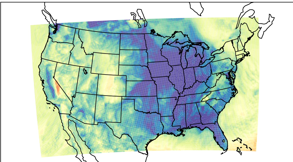
WRF (2023-12-07_11:00:00)
