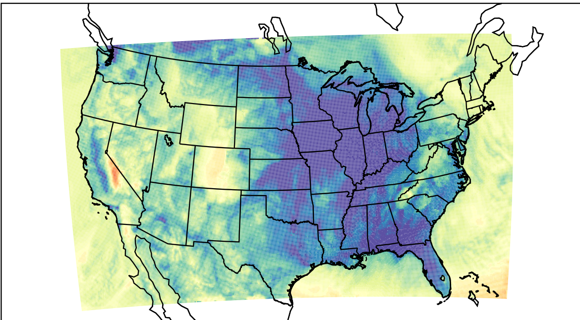
WRF (2023-12-07_10:00:00)
