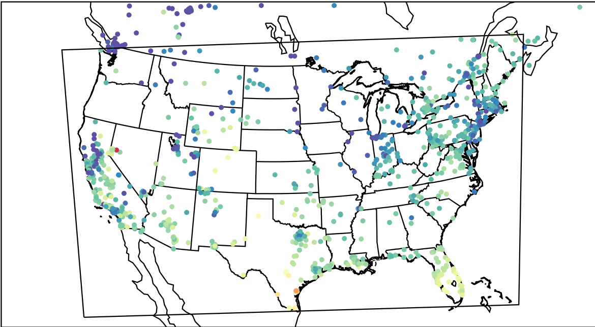
AirNOW (2023-12-06_19:00:00)
