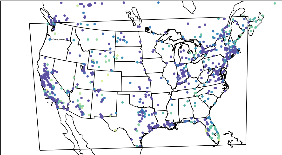
AirNOW (2023-12-06_06:00:00)
