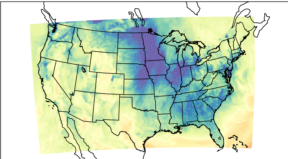
WRF (2023-12-06_22:00:00)
