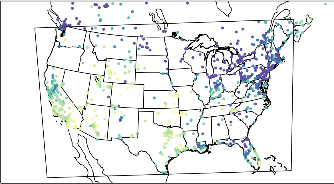
AirNOW (2023-12-07_23:00:00)
