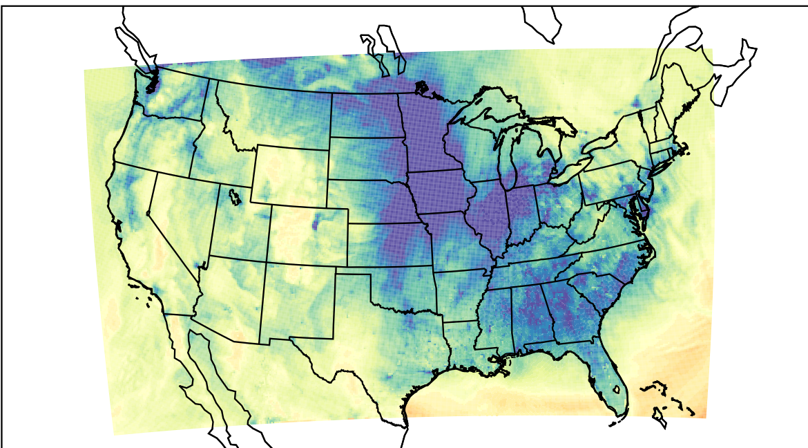
WRF (2023-12-06_23:00:00)
