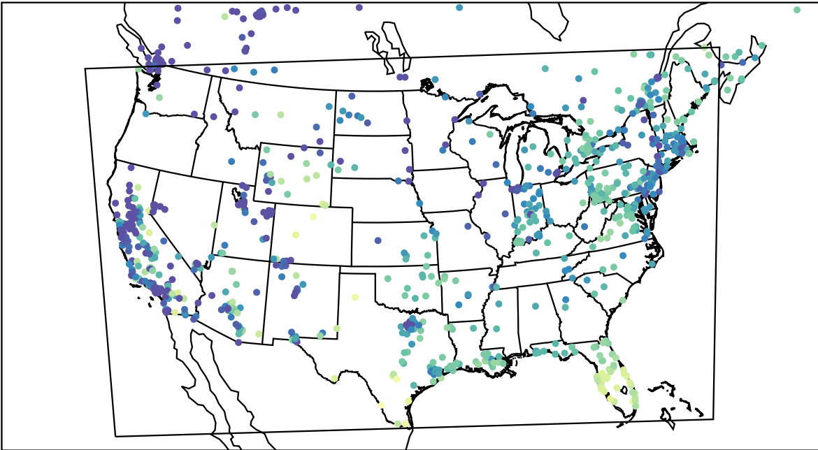
AirNOW (2023-12-06_17:00:00)
