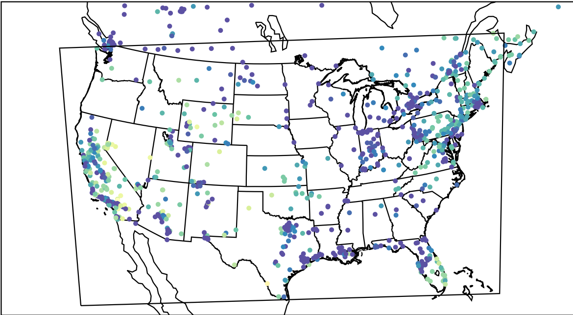
AirNOW (2023-12-07_03:00:00)
