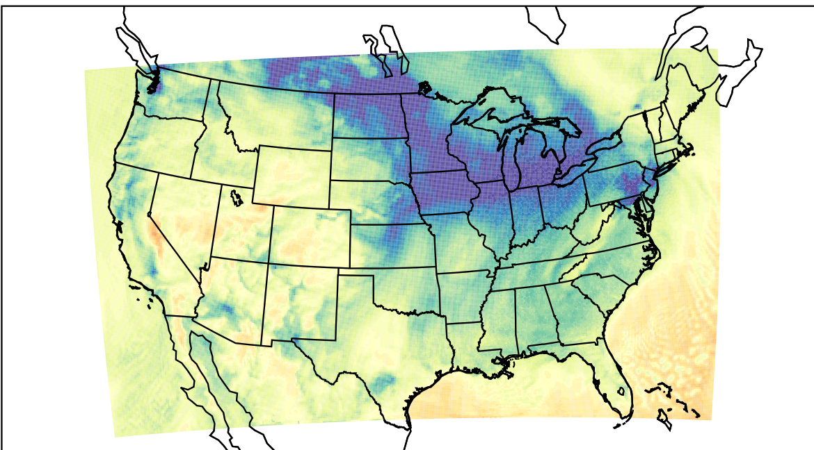
WRF (2023-12-07_19:00:00)
