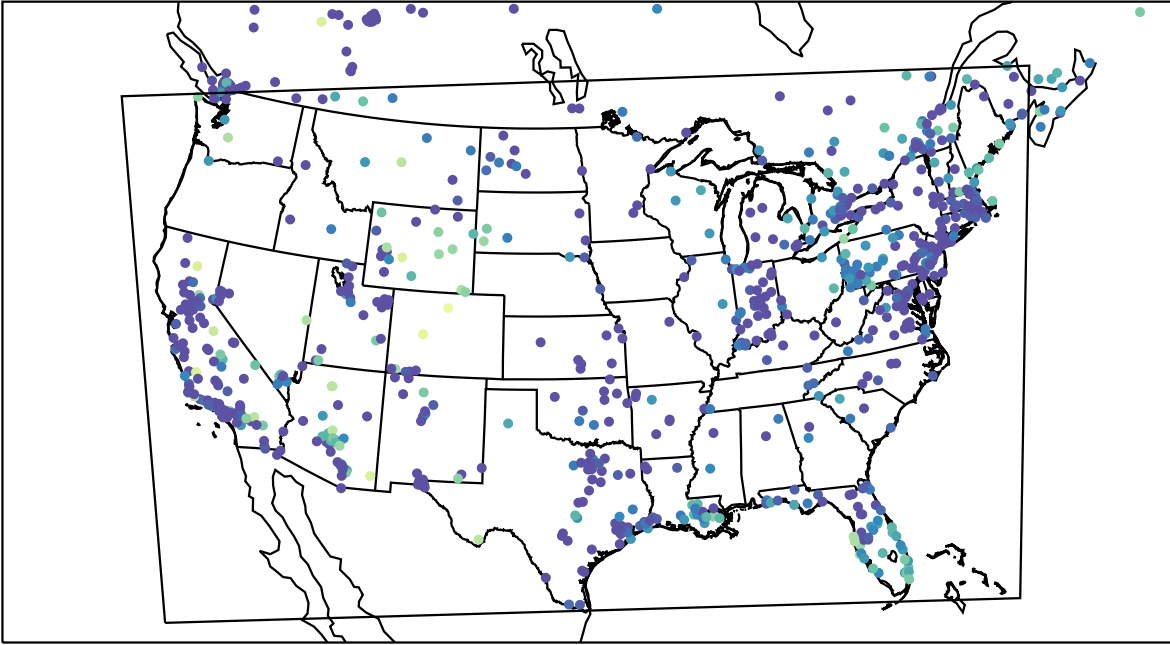
AirNOW (2023-12-06_11:00:00)
