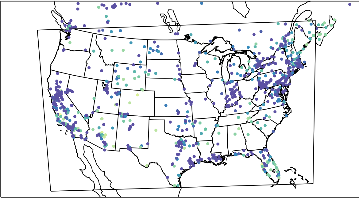
AirNOW (2023-12-06_02:00:00)
