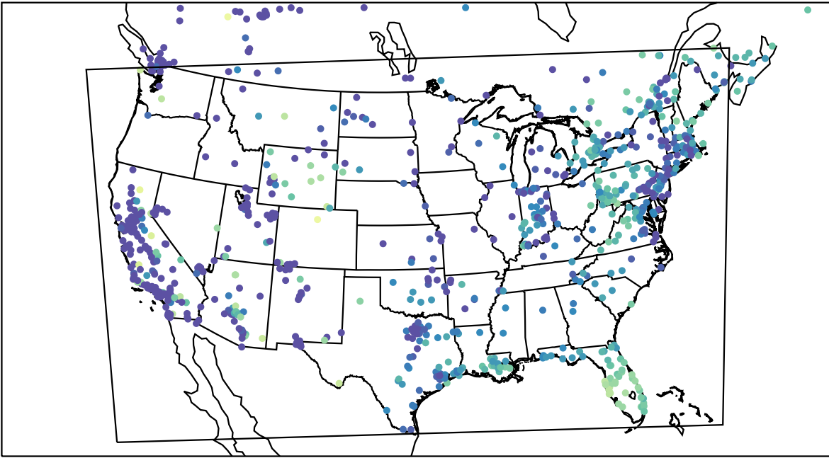
AirNOW (2023-12-06_15:00:00)
