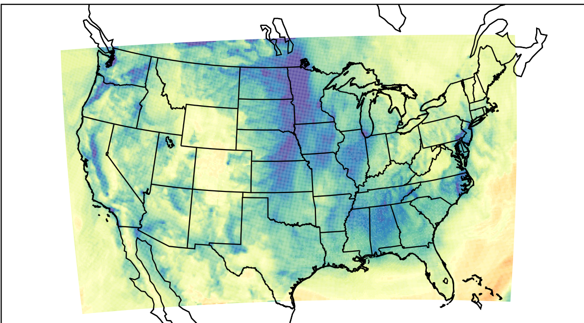
WRF (2023-12-06_18:00:00)
