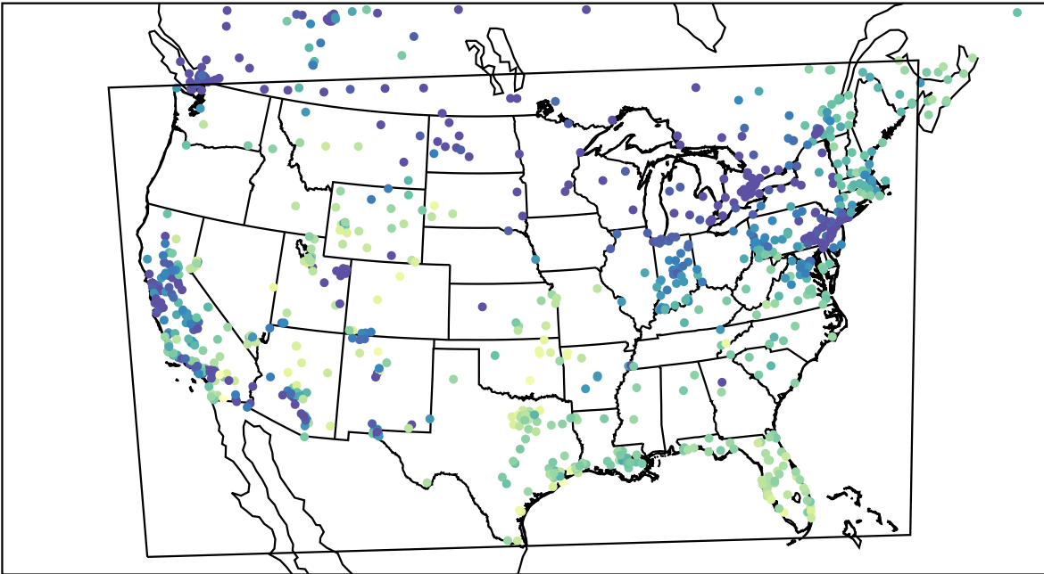
AirNOW (2023-12-07_17:00:00)
