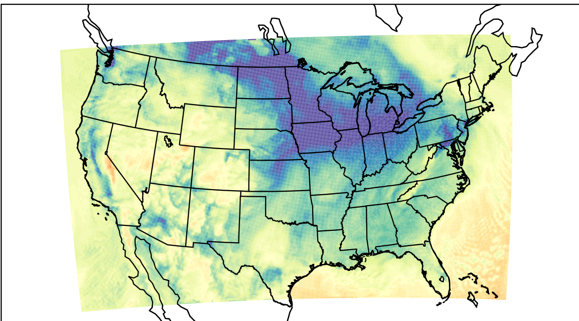
WRF (2023-12-07_18:00:00)
