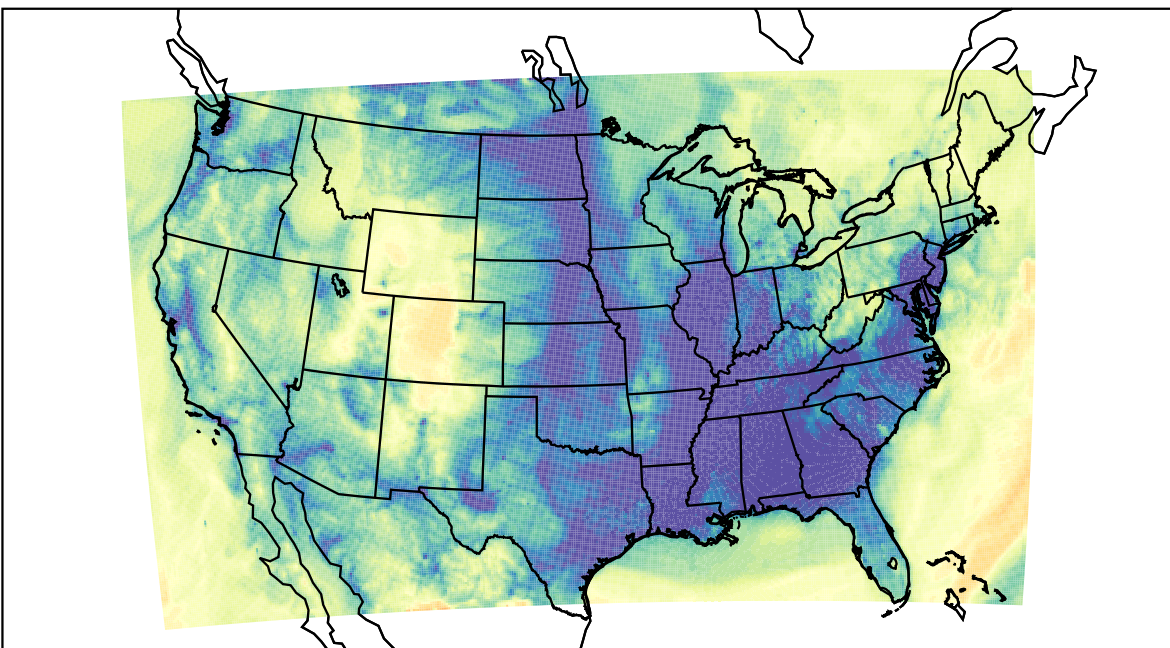
WRF (2023-12-06_14:00:00)
