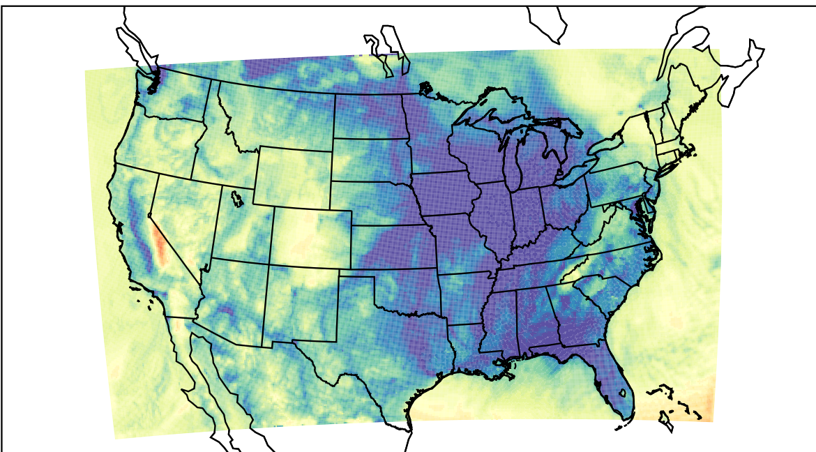
WRF (2023-12-07_12:00:00)
