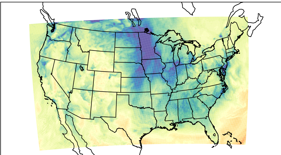
WRF (2023-12-06_21:00:00)
