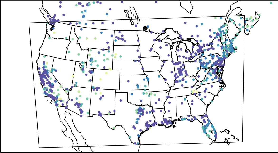
AirNOW (2023-12-07_14:00:00)
