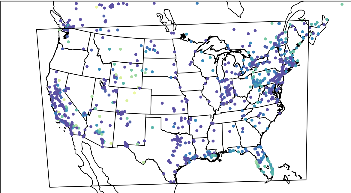
AirNOW (2023-12-06_13:00:00)
