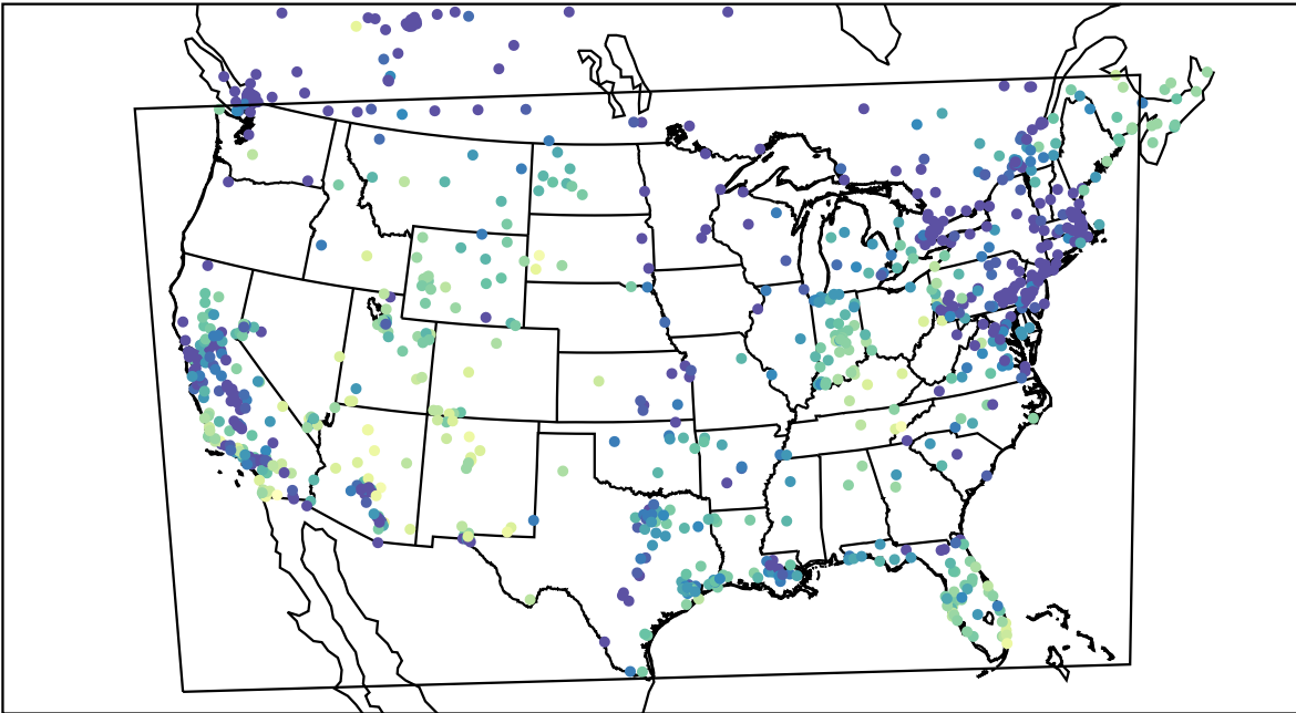
AirNOW (2023-12-09_01:00:00)
