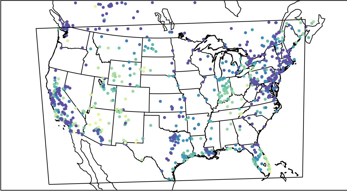
AirNOW (2023-12-09_04:00:00)
