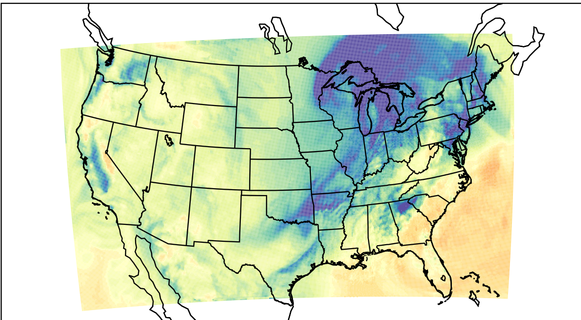
WRF (2023-12-09_18:00:00)
