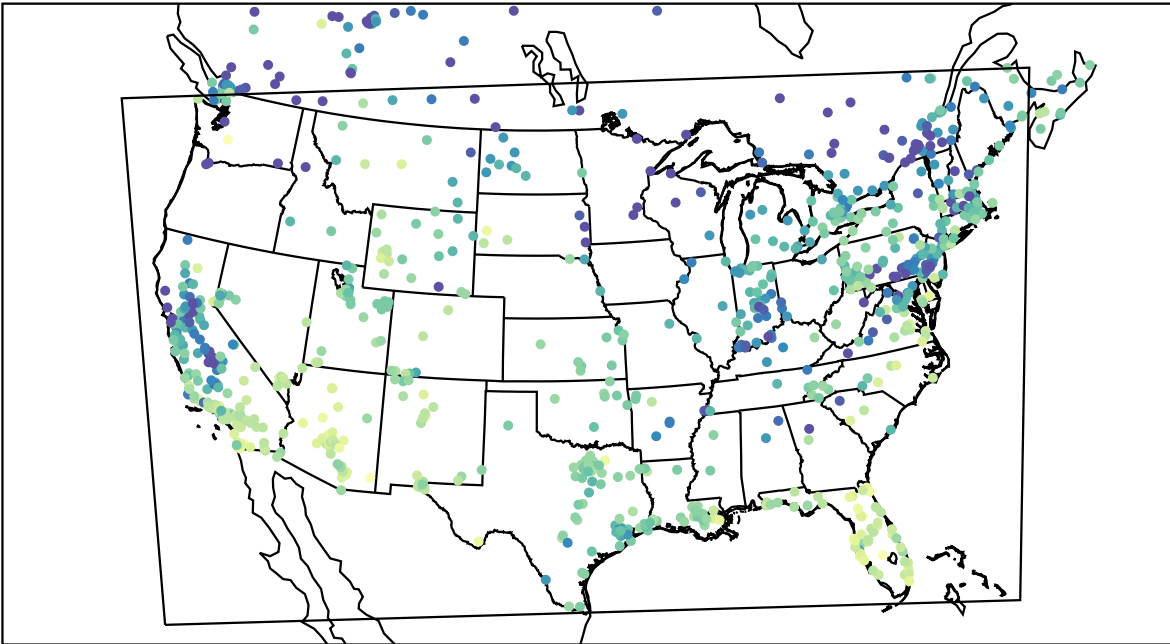
AirNOW (2023-12-09_19:00:00)
