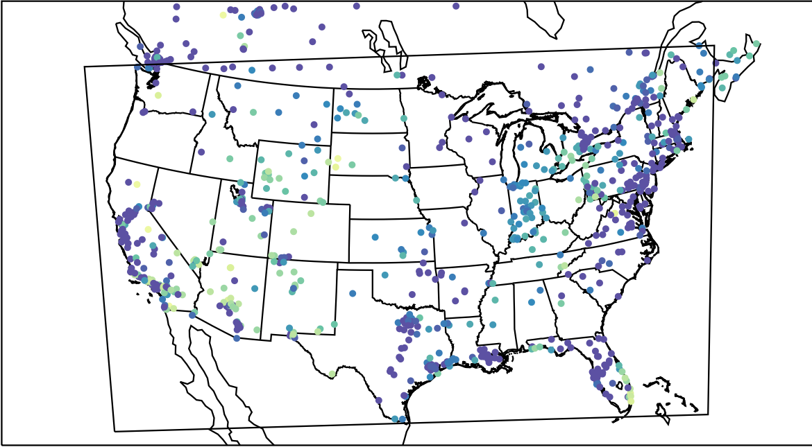
AirNOW (2023-12-09_12:00:00)
