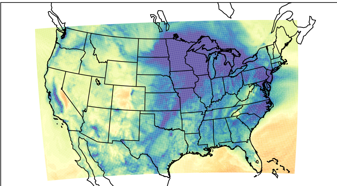
WRF (2023-12-08_15:00:00)
