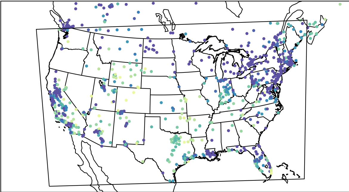
AirNOW (2023-12-08_04:00:00)
