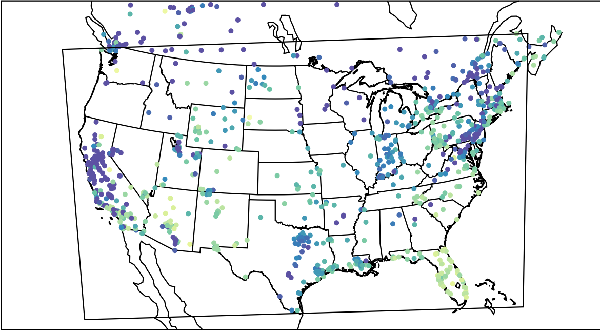
AirNOW (2023-12-09_16:00:00)
