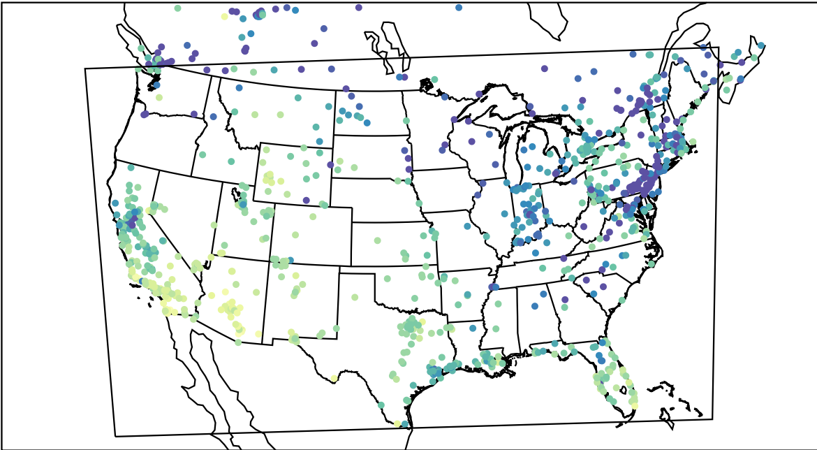
AirNOW (2023-12-09_22:00:00)
