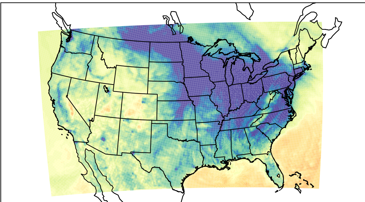
WRF (2023-12-08_02:00:00)
