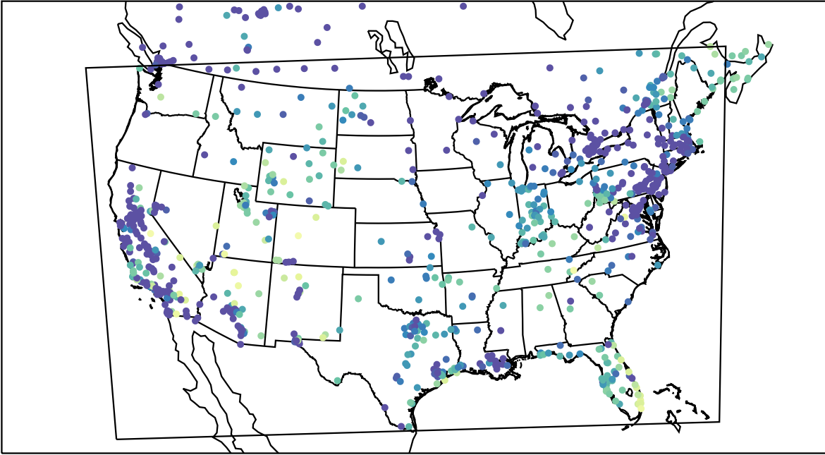
AirNOW (2023-12-08_15:00:00)
