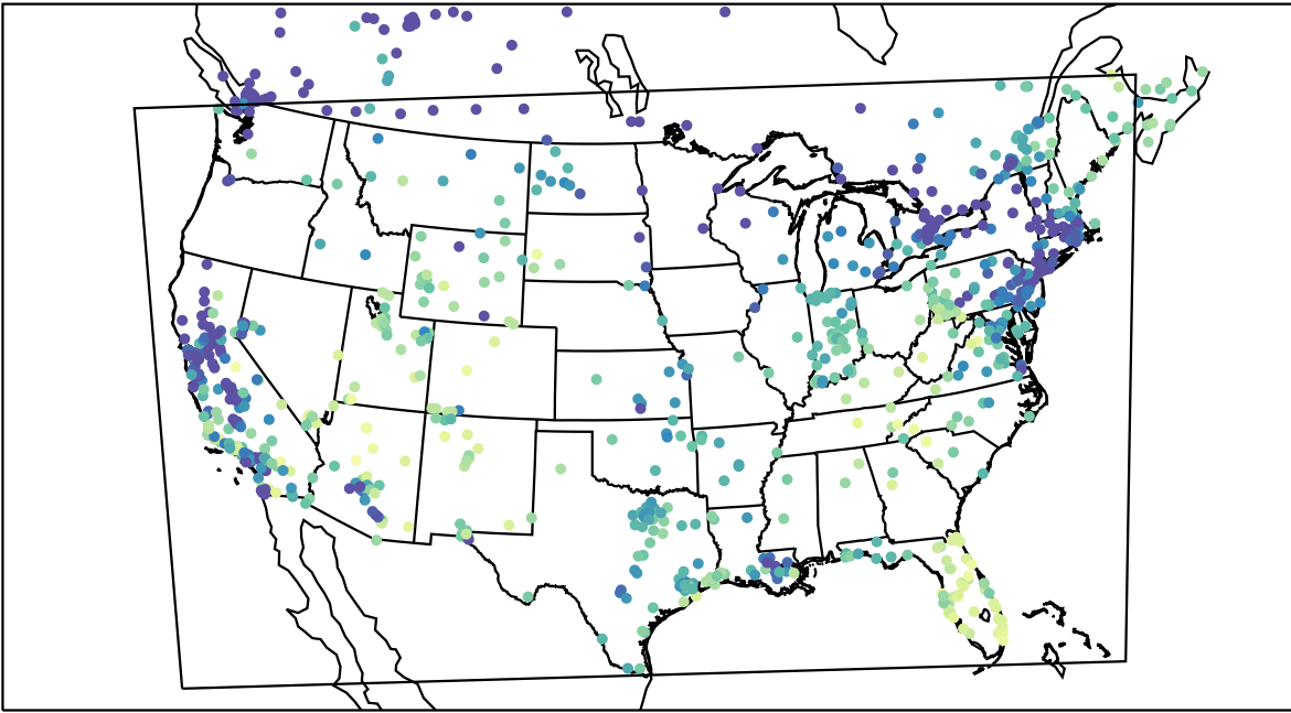
AirNOW (2023-12-08_17:00:00)
