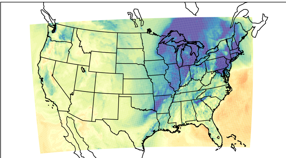
WRF (2023-12-09_22:00:00)
