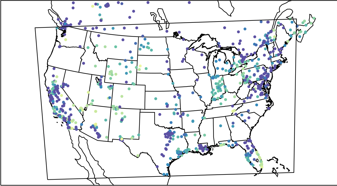
AirNOW (2023-12-09_08:00:00)
