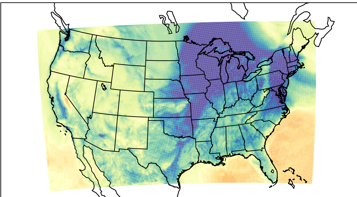
WRF (2023-12-09_05:00:00)
