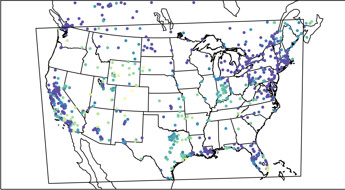
AirNOW (2023-12-08_08:00:00)
