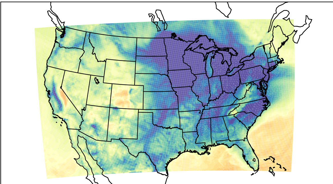
WRF (2023-12-08_13:00:00)
