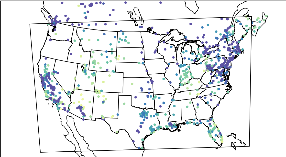
AirNOW (2023-12-09_02:00:00)
