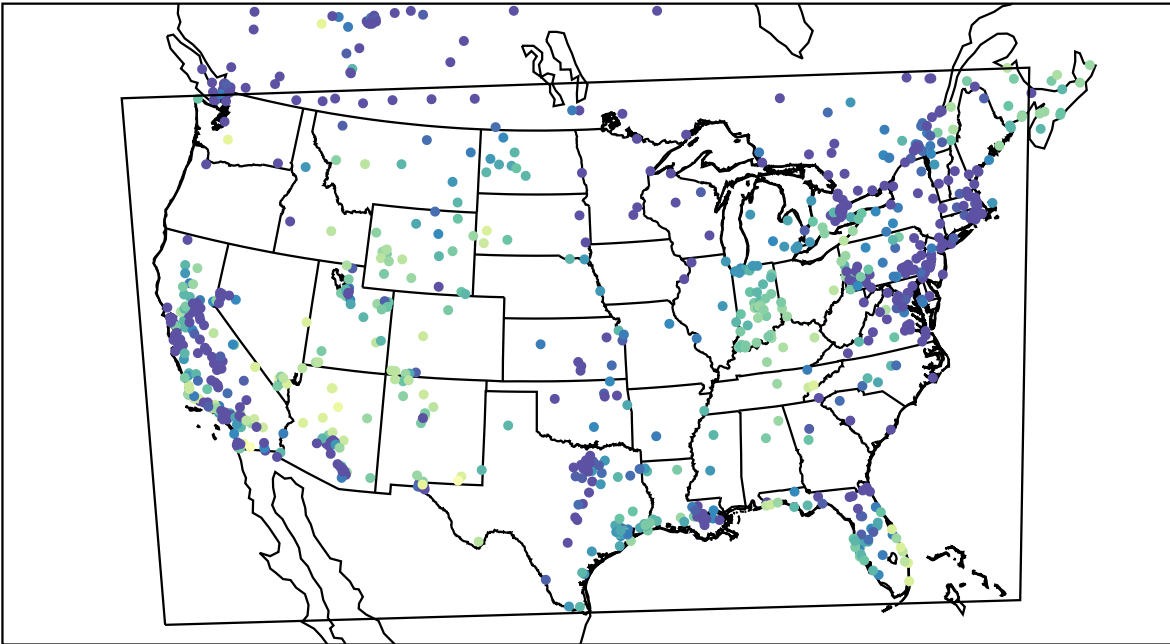
AirNOW (2023-12-09_05:00:00)
