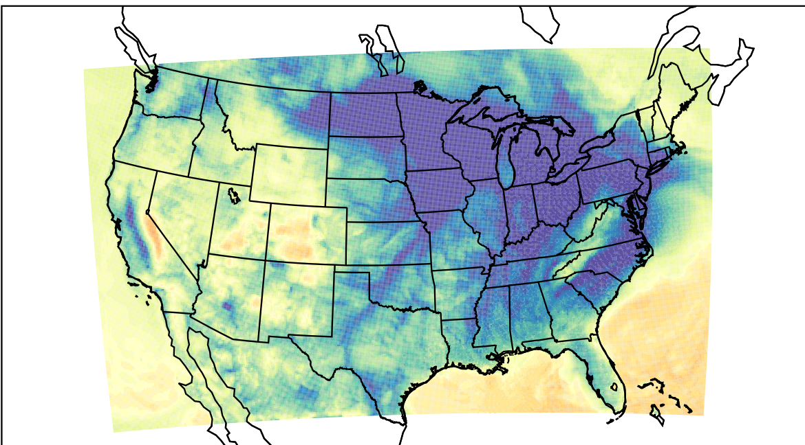
WRF (2023-12-08_09:00:00)
