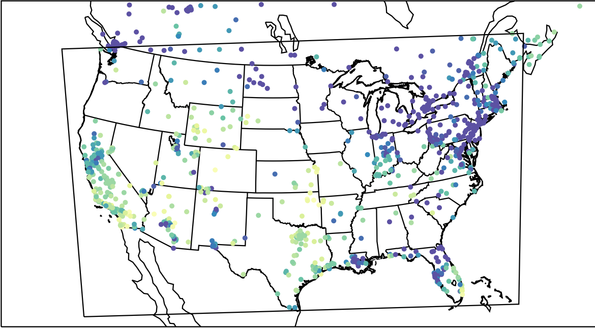
AirNOW (2023-12-08_00:00:00)
