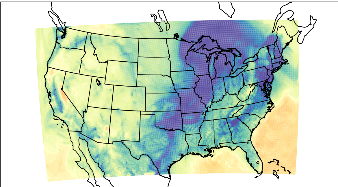
WRF (2023-12-09_14:00:00)
