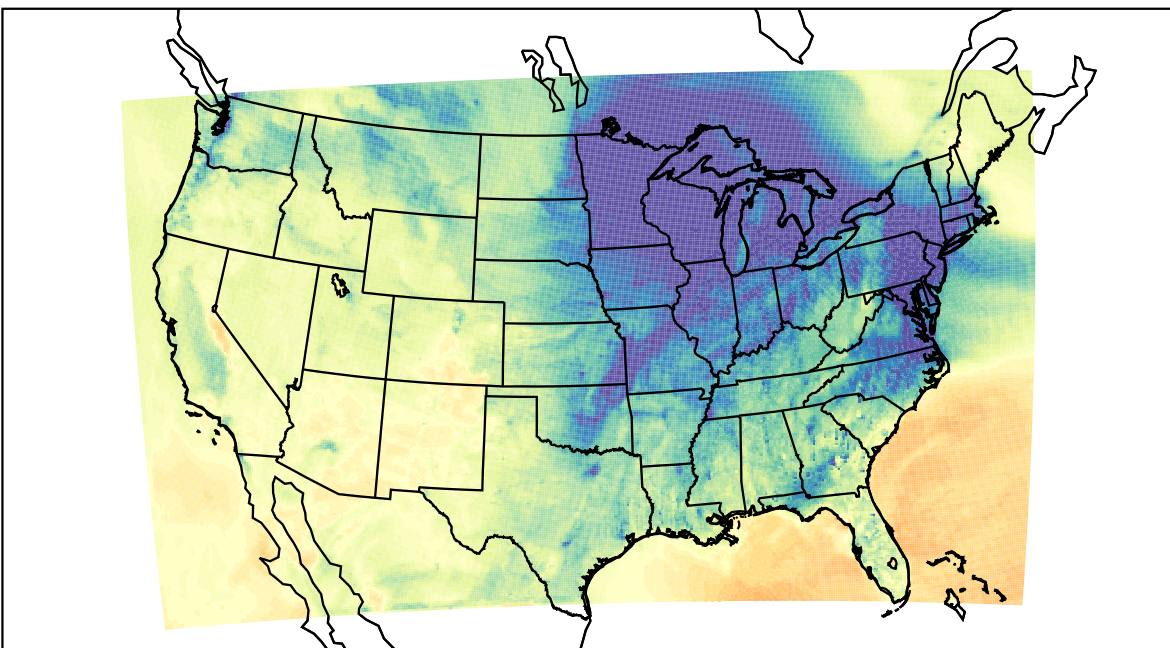
WRF (2023-12-08_23:00:00)
