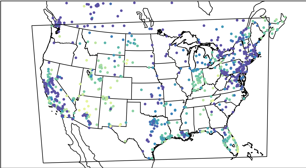
AirNOW (2023-12-09_03:00:00)
