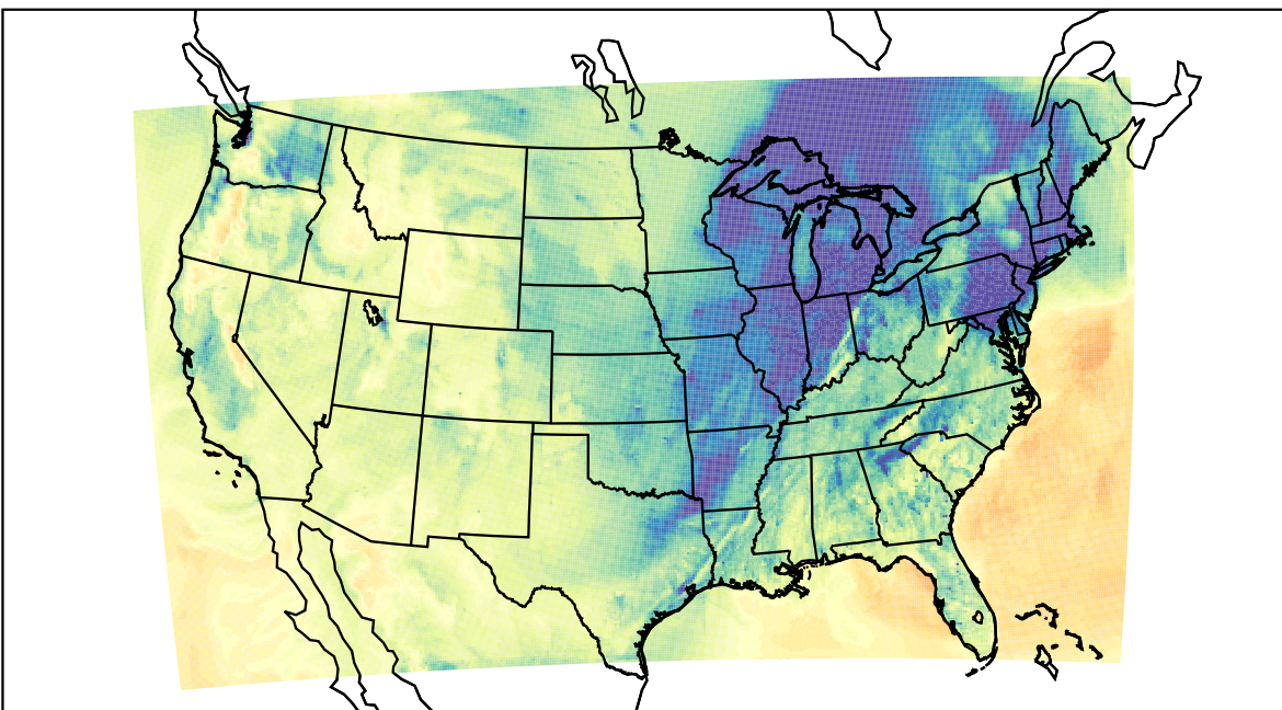
WRF (2023-12-09_23:00:00)
