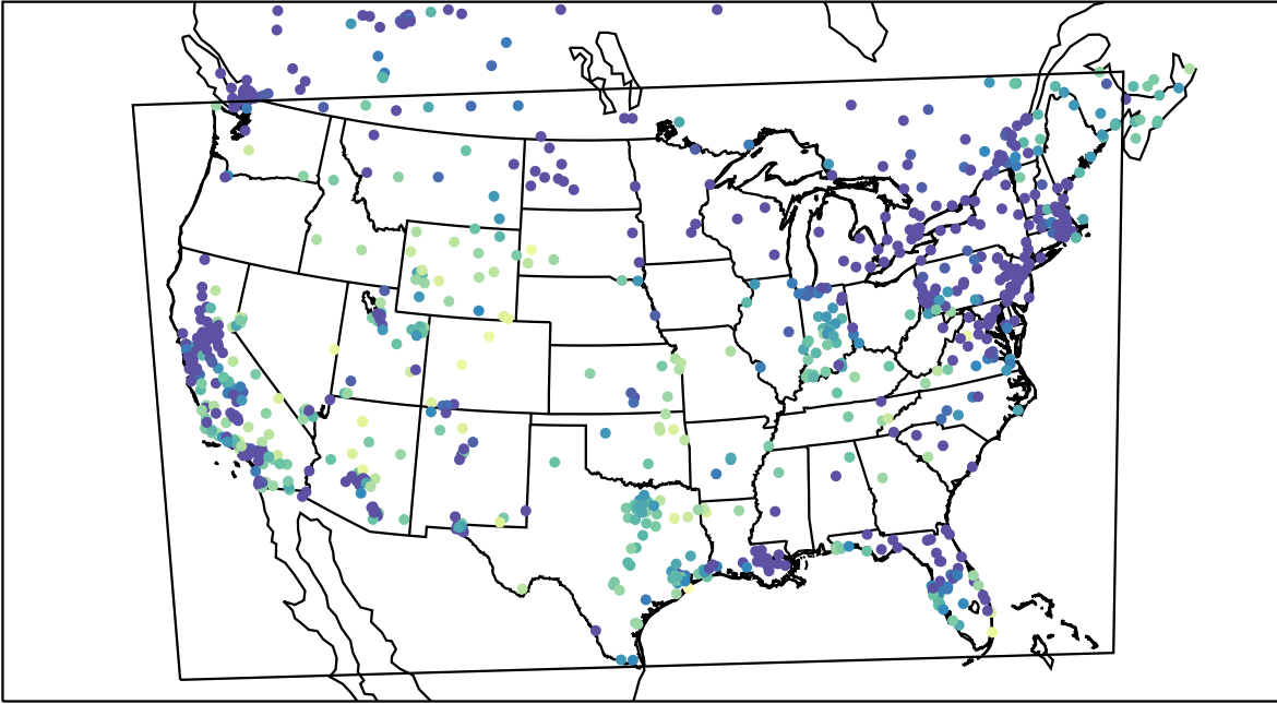
AirNOW (2023-12-08_05:00:00)
