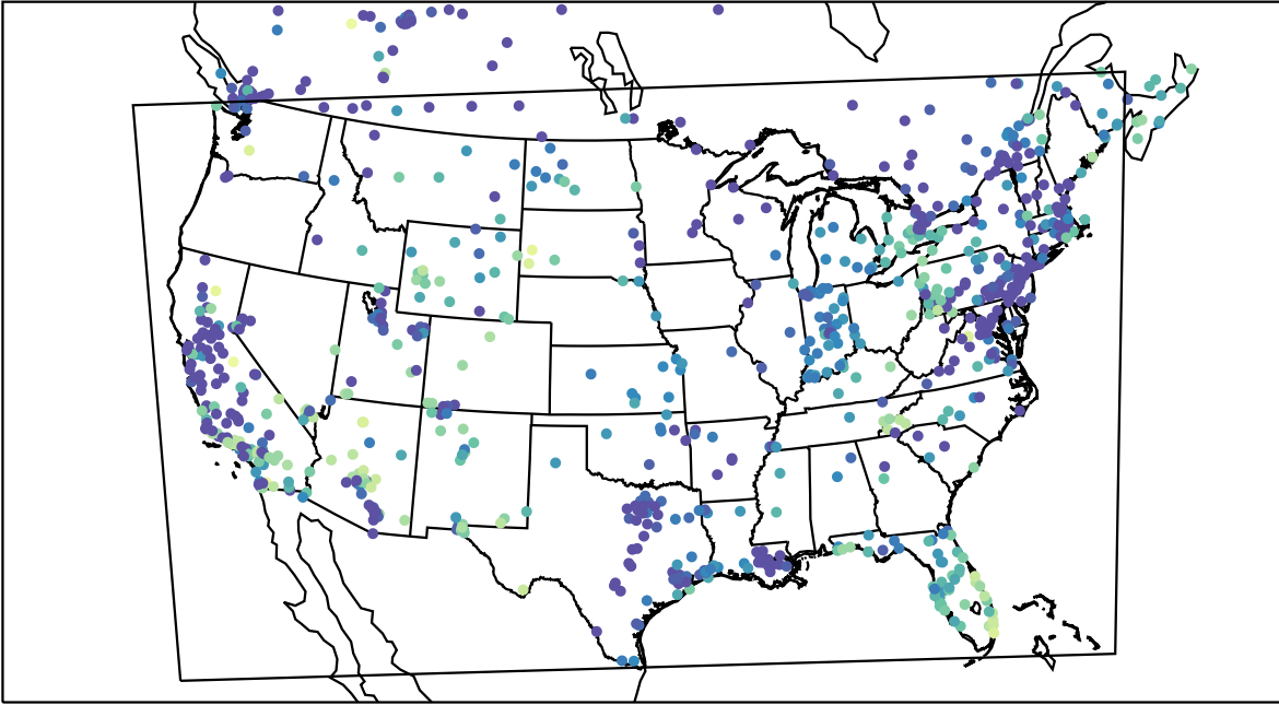
AirNOW (2023-12-09_14:00:00)
