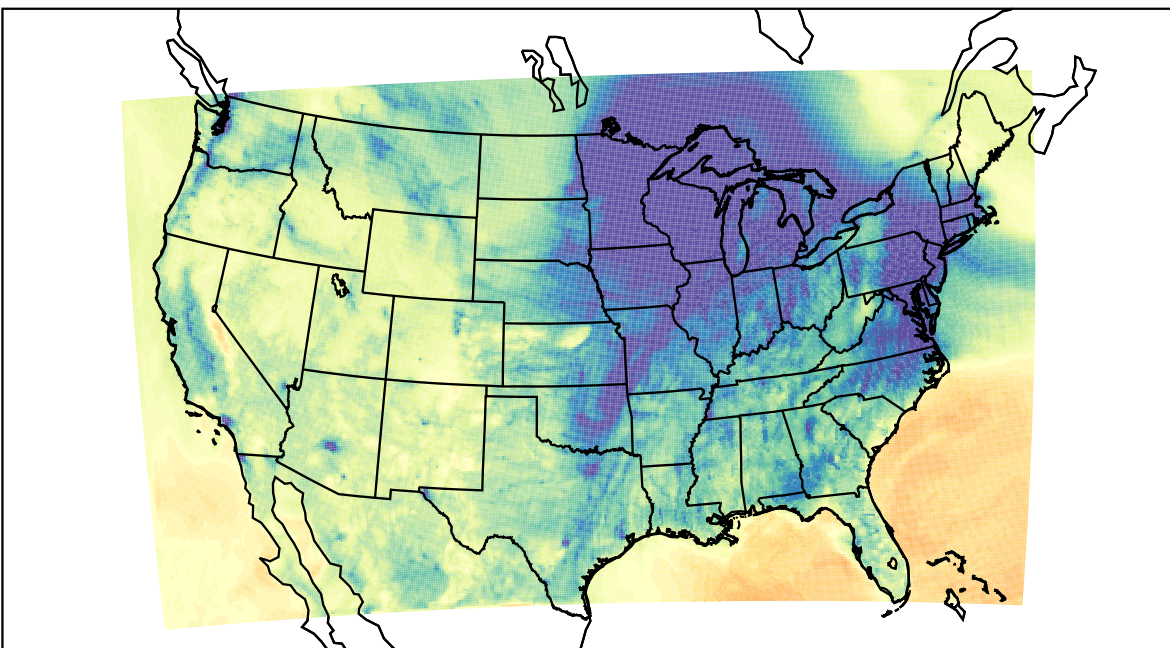
WRF (2023-12-09_01:00:00)
