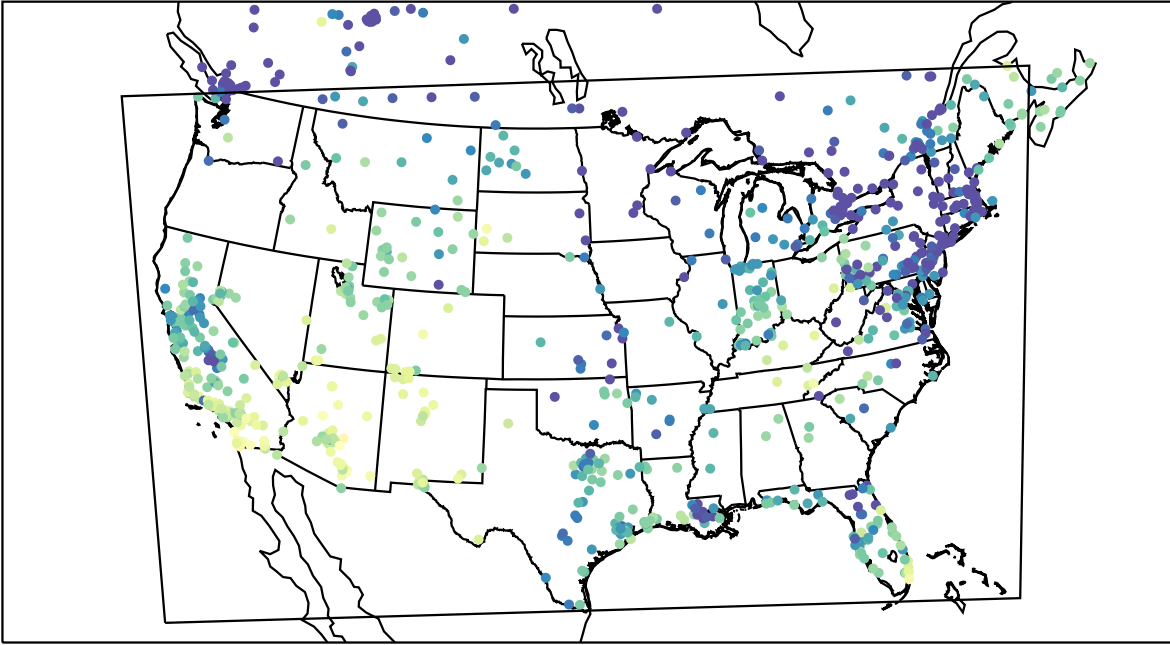
AirNOW (2023-12-08_23:00:00)
