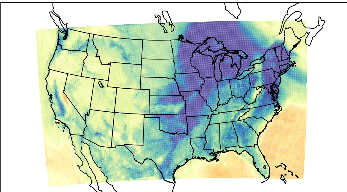
WRF (2023-12-09_08:00:00)
