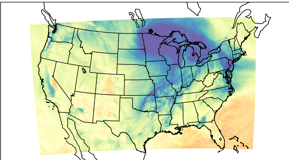
WRF (2023-12-08_19:00:00)
