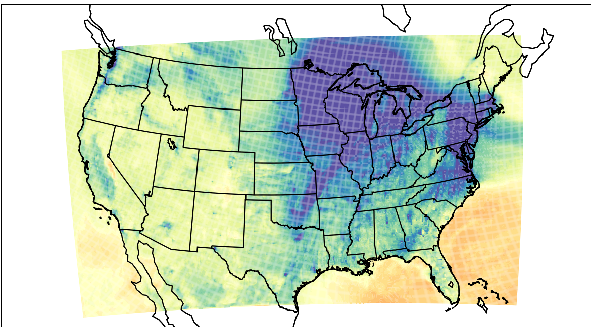
WRF (2023-12-09_00:00:00)
