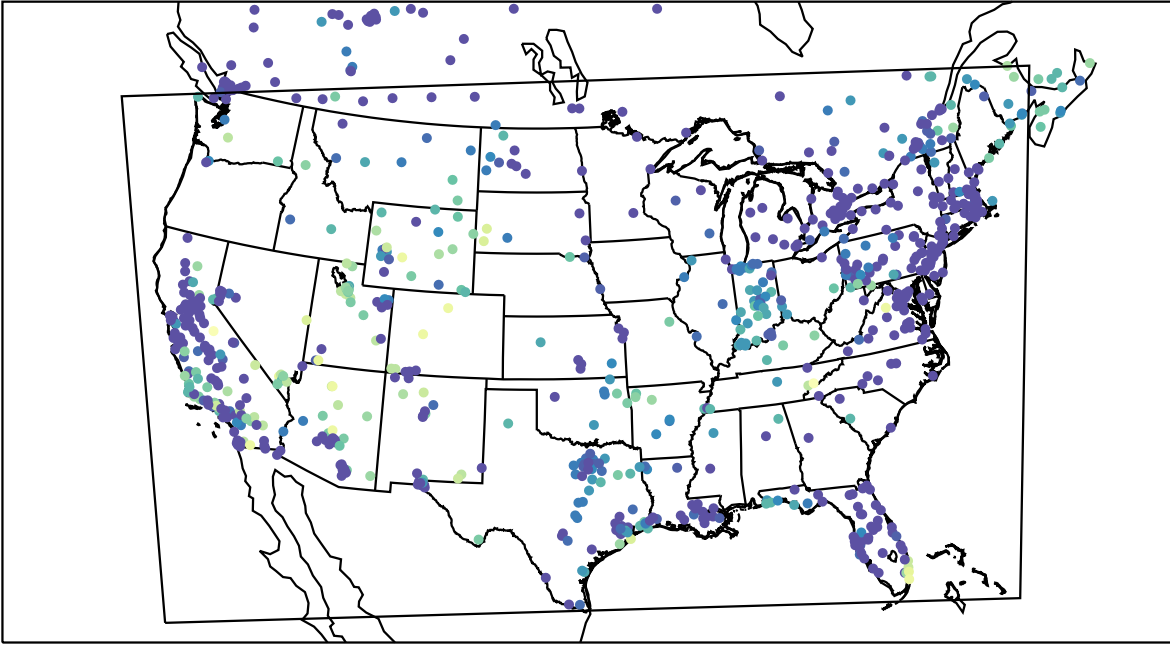
AirNOW (2023-12-08_13:00:00)
