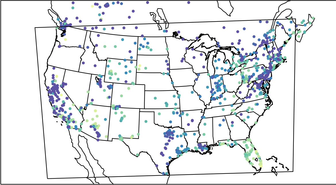
AirNOW (2023-12-09_15:00:00)
