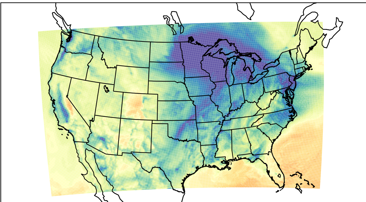
WRF (2023-12-08_17:00:00)
