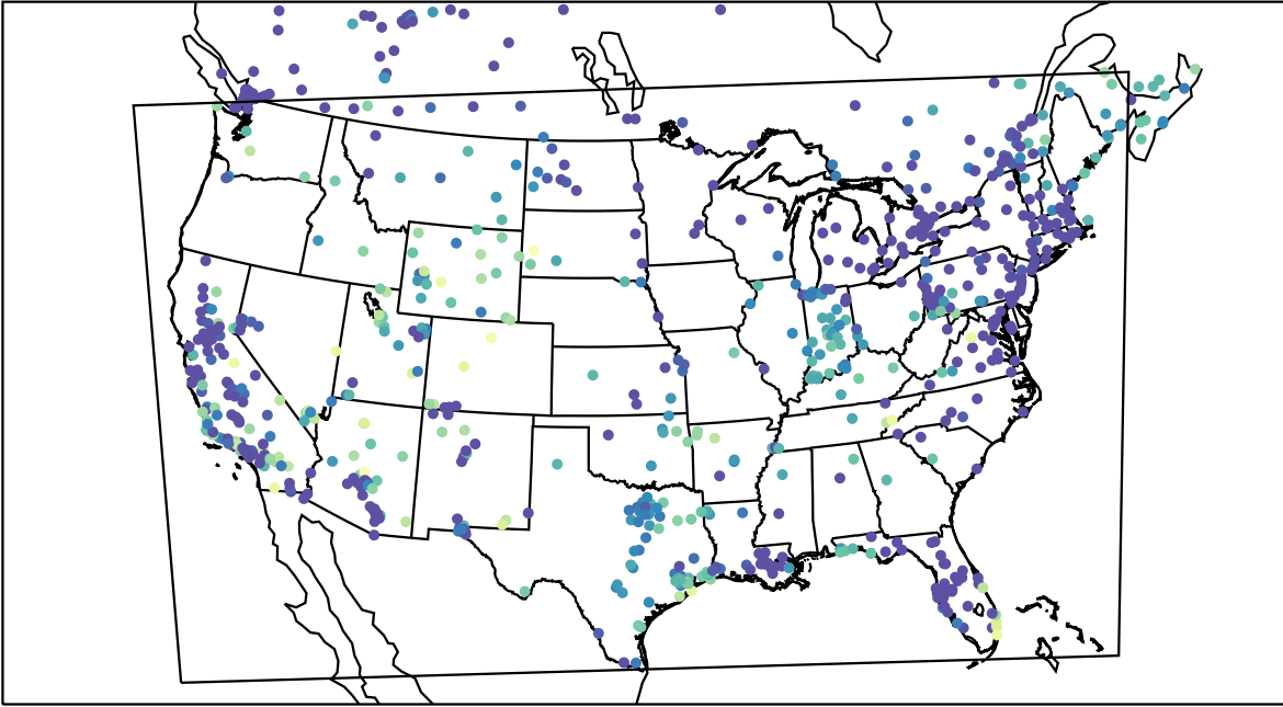
AirNOW (2023-12-08_11:00:00)
