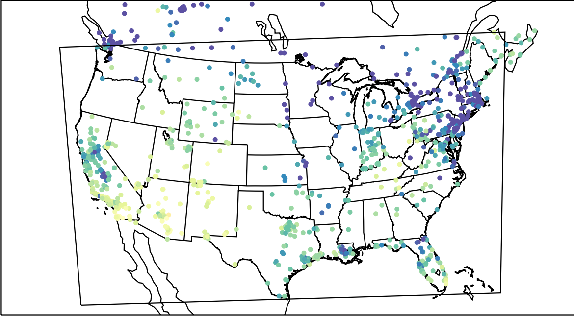
AirNOW (2023-12-08_22:00:00)
