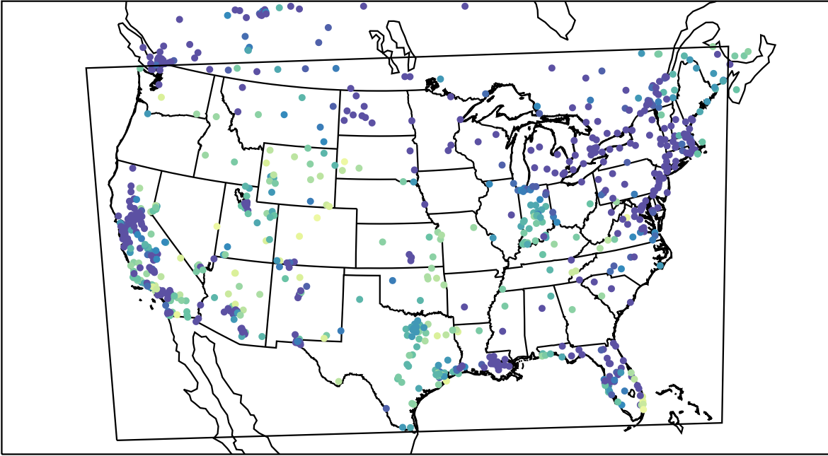
AirNOW (2023-12-08_06:00:00)
