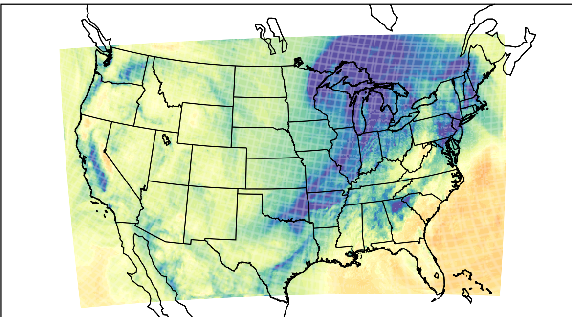
WRF (2023-12-09_17:00:00)
