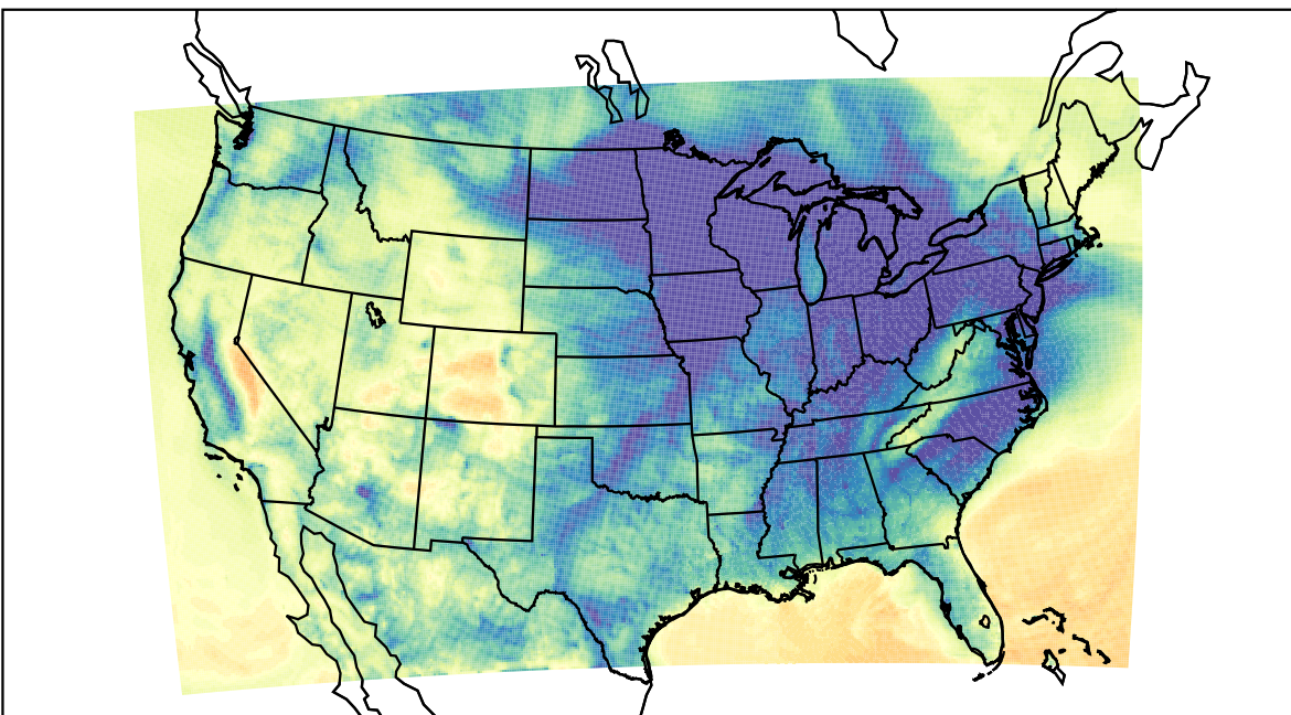
WRF (2023-12-08_11:00:00)
