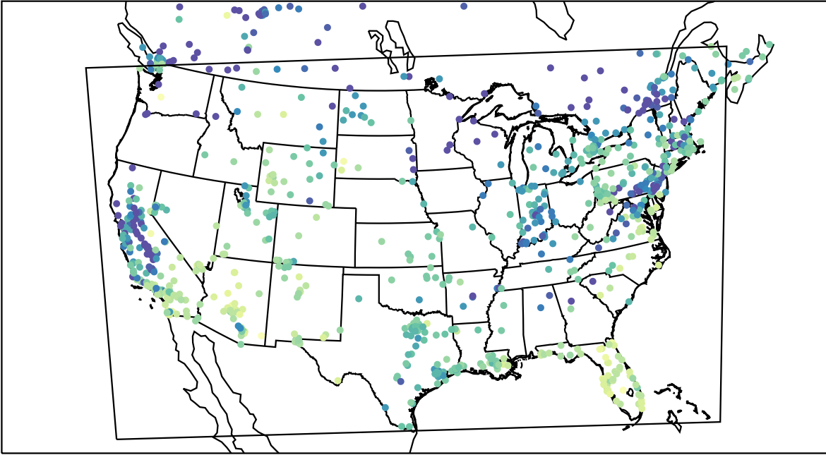
AirNOW (2023-12-09_18:00:00)
