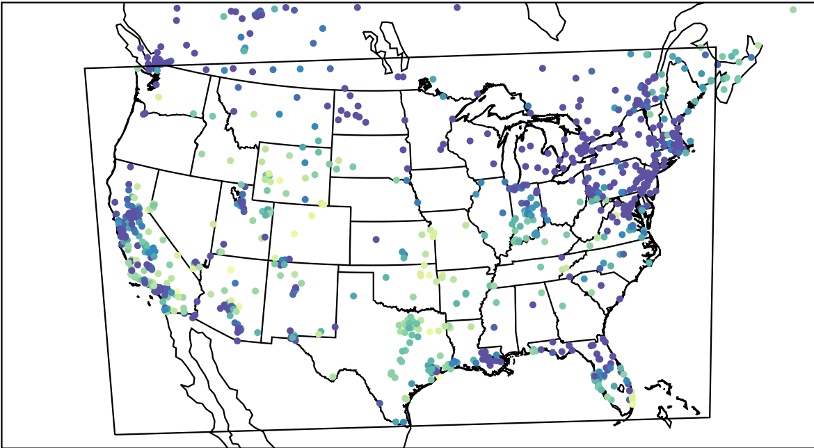
AirNOW (2023-12-08_03:00:00)
