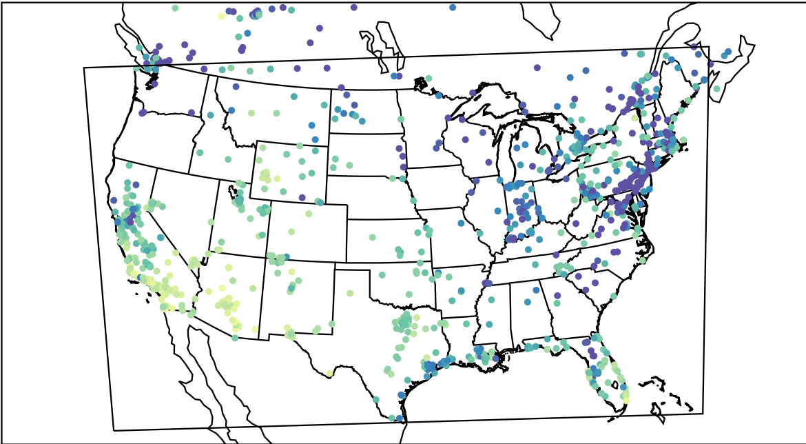
AirNOW (2023-12-09_23:00:00)
