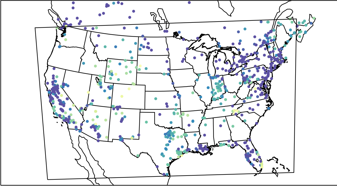
AirNOW (2023-12-08_10:00:00)
