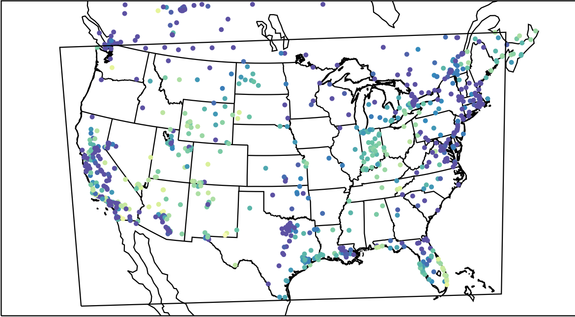
AirNOW (2023-12-09_06:00:00)
