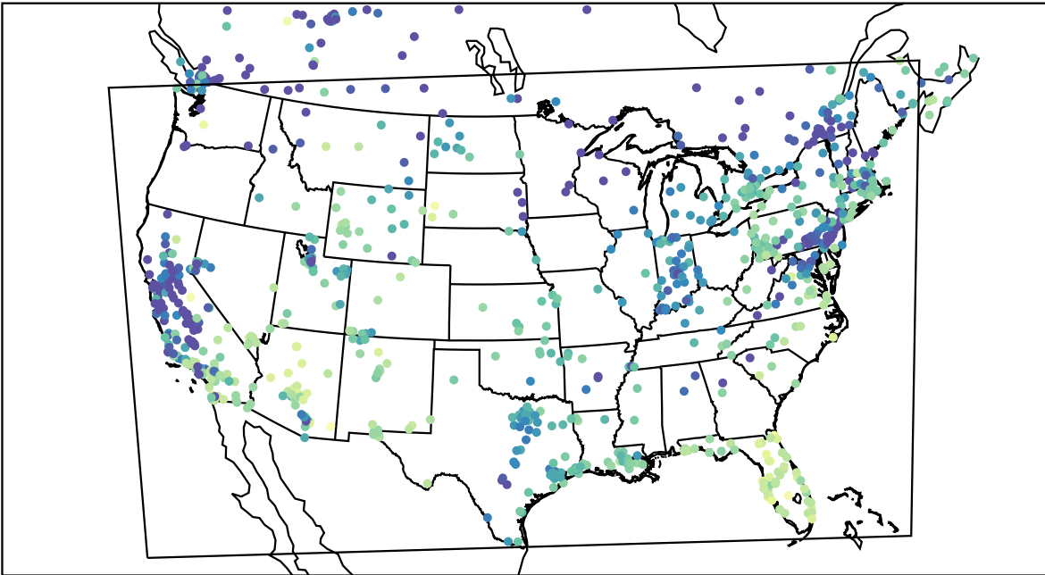
AirNOW (2023-12-09_17:00:00)
