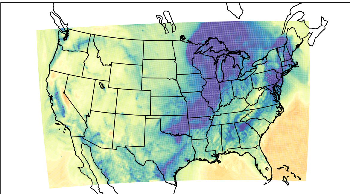
WRF (2023-12-09_15:00:00)
