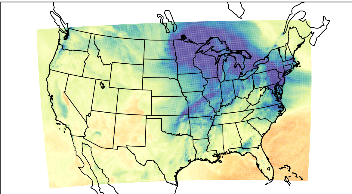
WRF (2023-12-08_21:00:00)
