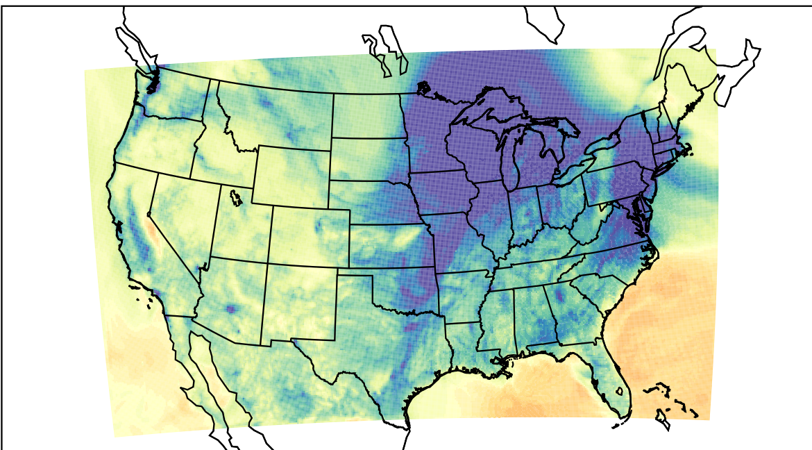
WRF (2023-12-09_03:00:00)
