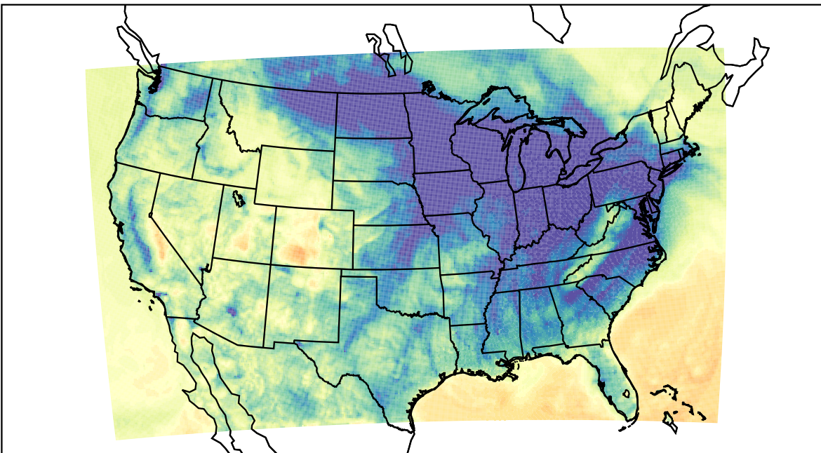
WRF (2023-12-08_05:00:00)
