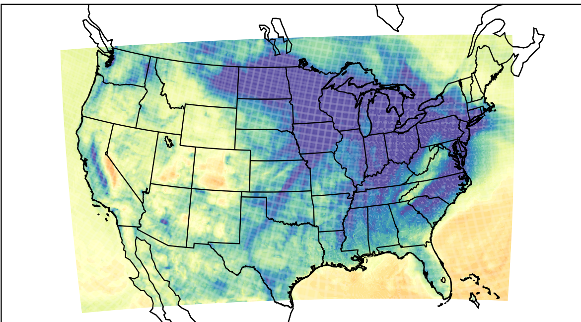
WRF (2023-12-08_08:00:00)
