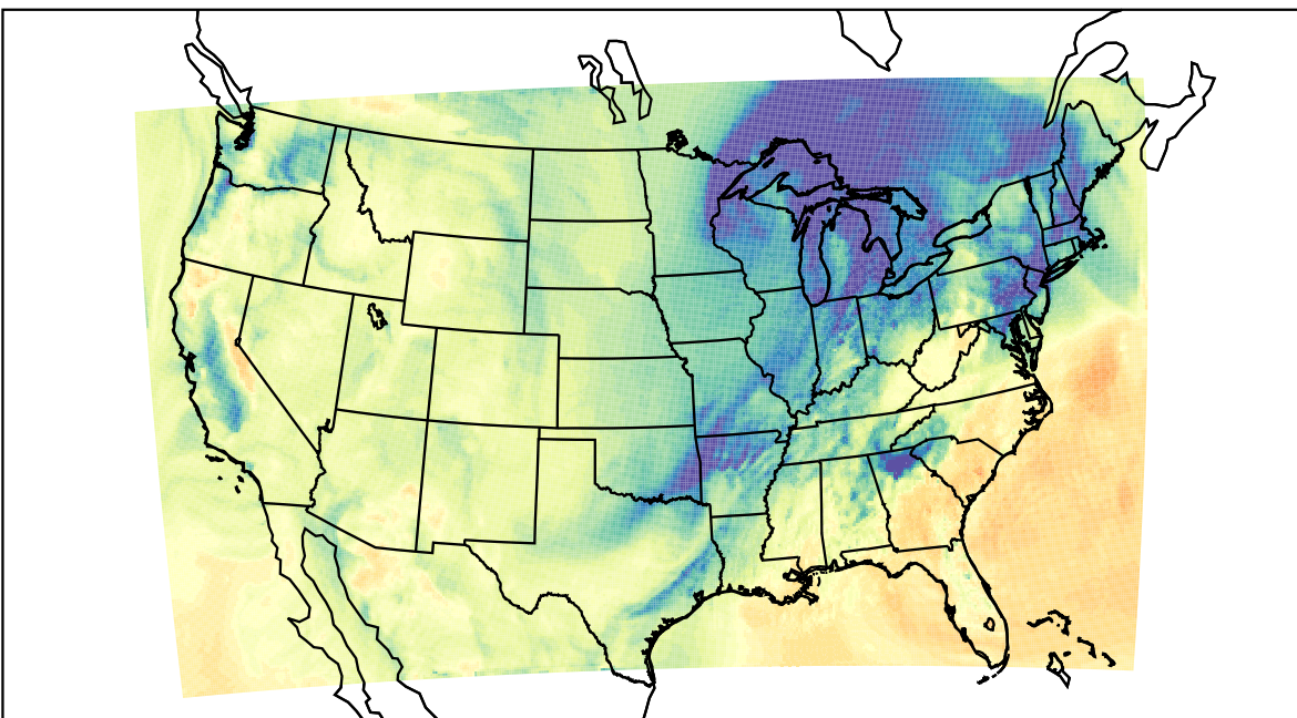
WRF (2023-12-09_19:00:00)
