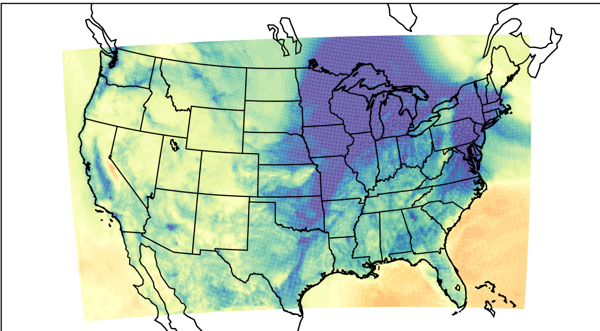
WRF (2023-12-09_04:00:00)
