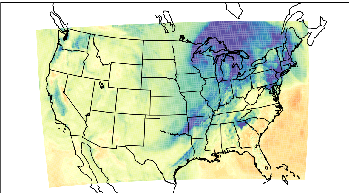
WRF (2023-12-09_20:00:00)
