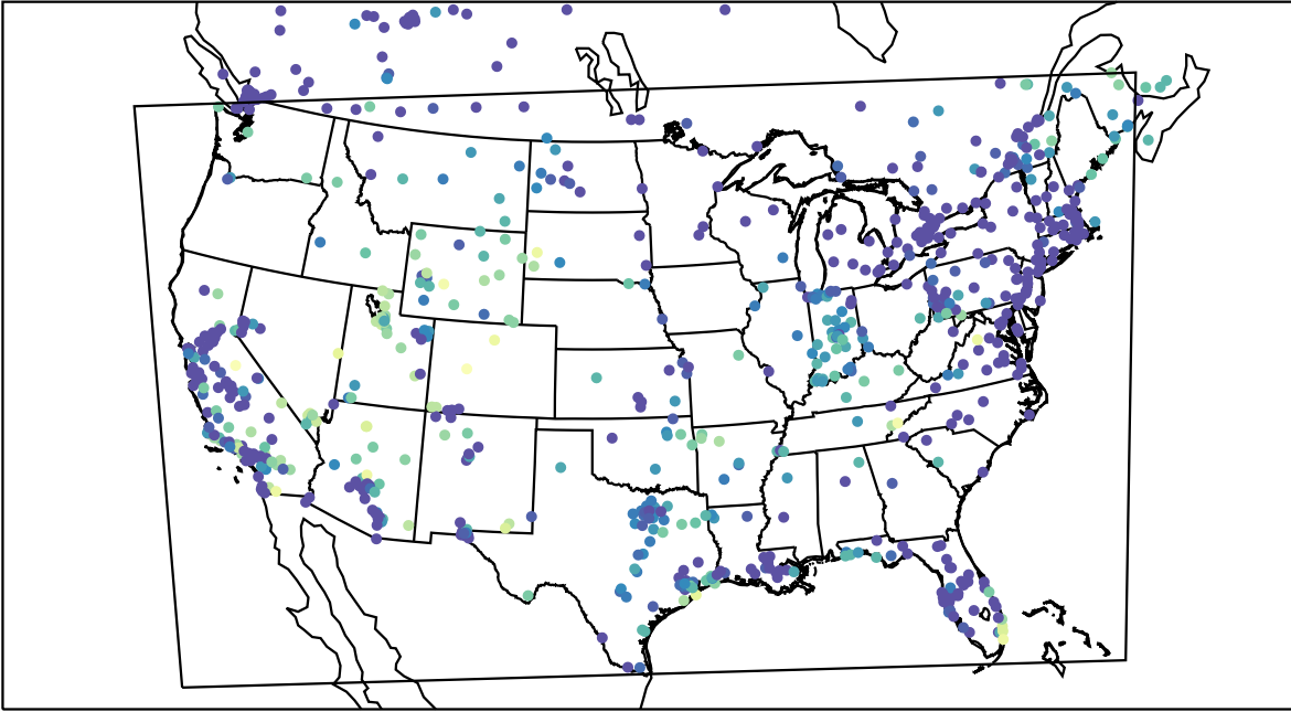
AirNOW (2023-12-08_12:00:00)
