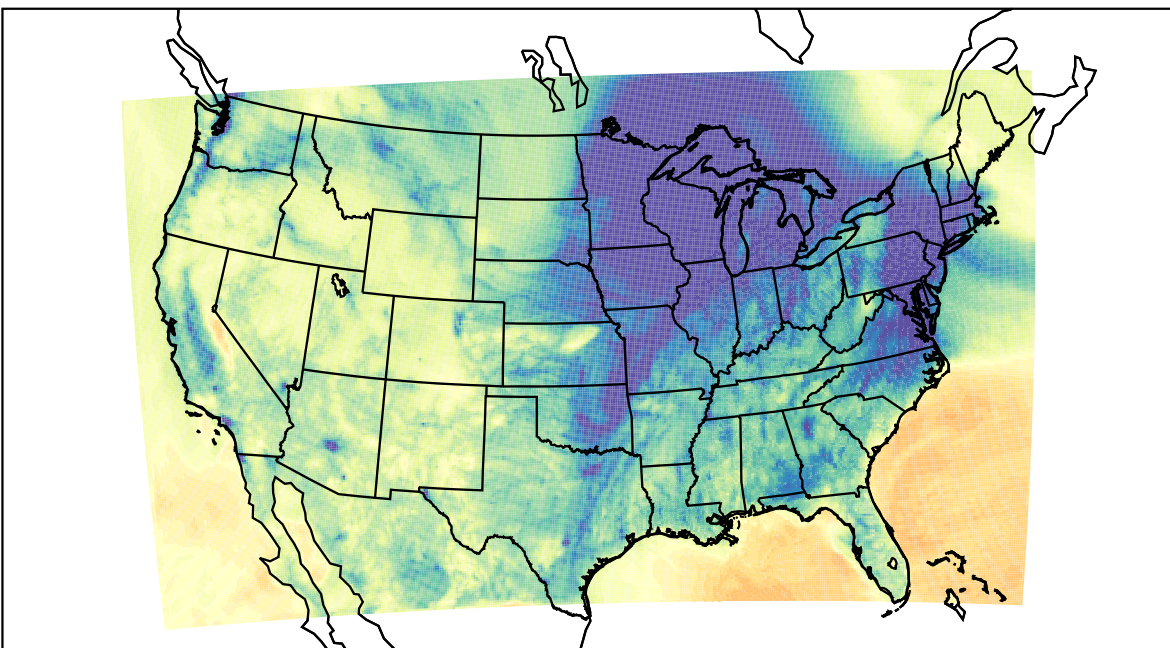
WRF (2023-12-09_02:00:00)
