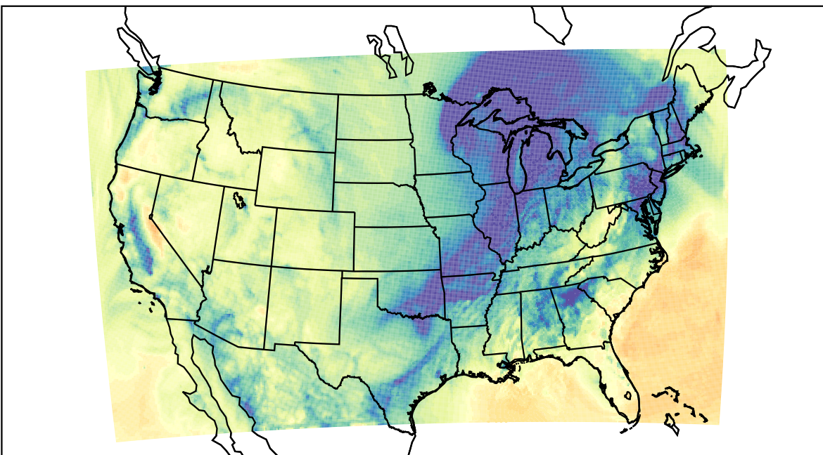
WRF (2023-12-09_16:00:00)
