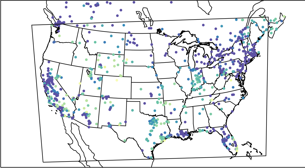
AirNOW (2023-12-08_09:00:00)
