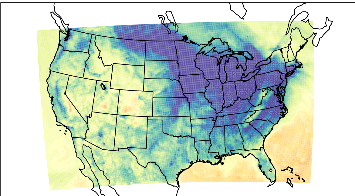
WRF (2023-12-08_03:00:00)
