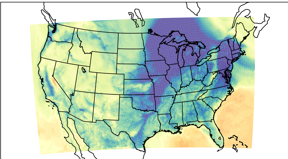
WRF (2023-12-09_06:00:00)
