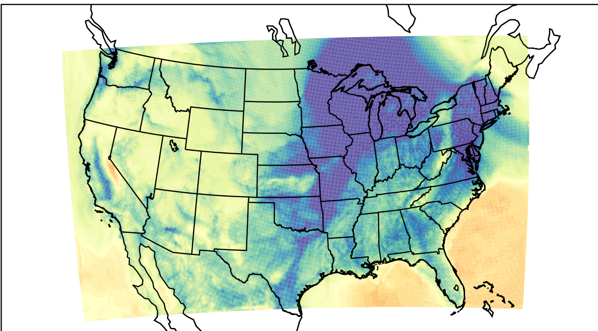
WRF (2023-12-09_07:00:00)
