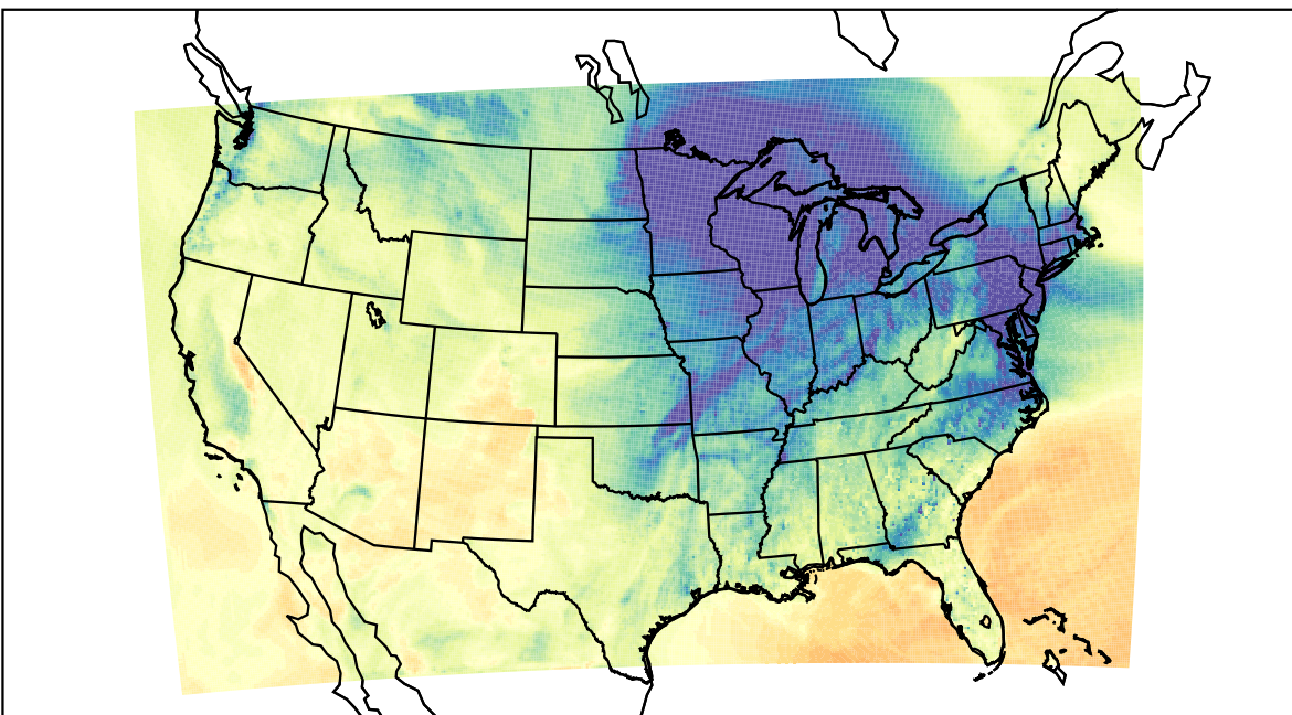
WRF (2023-12-08_22:00:00)
