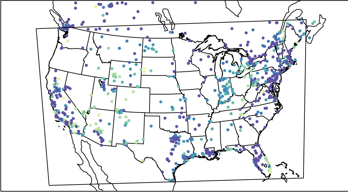
AirNOW (2023-12-09_11:00:00)
