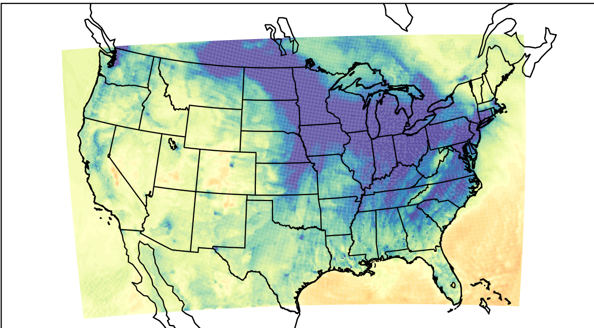
WRF (2023-12-08_00:00:00)
