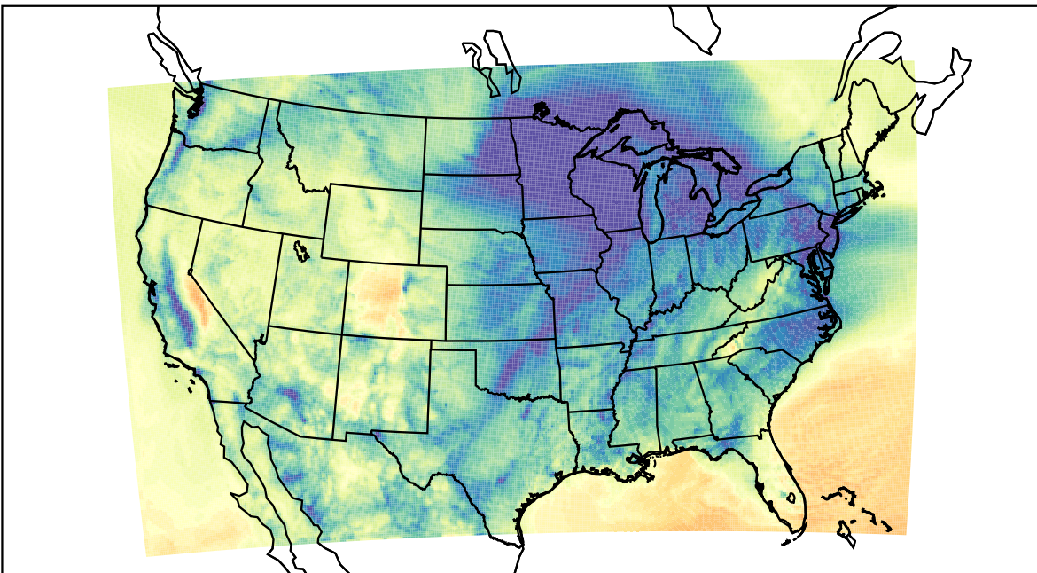
WRF (2023-12-08_16:00:00)
