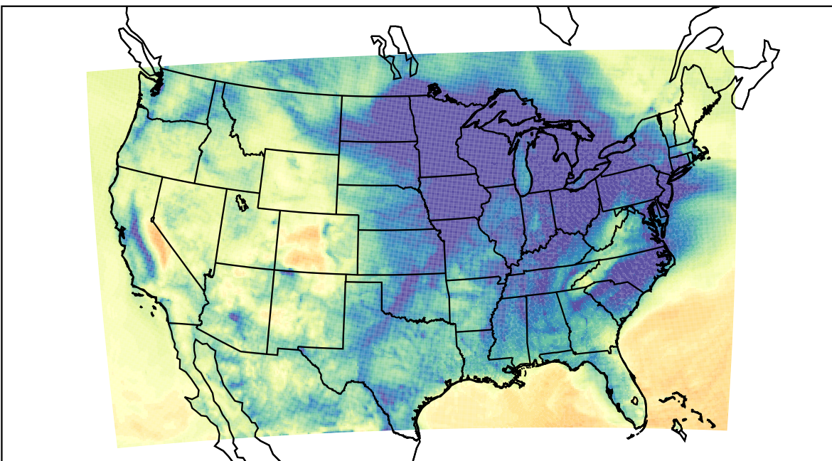
WRF (2023-12-08_12:00:00)
