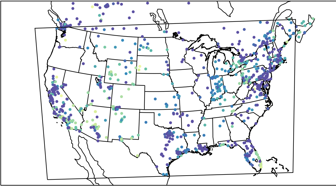
AirNOW (2023-12-09_13:00:00)
