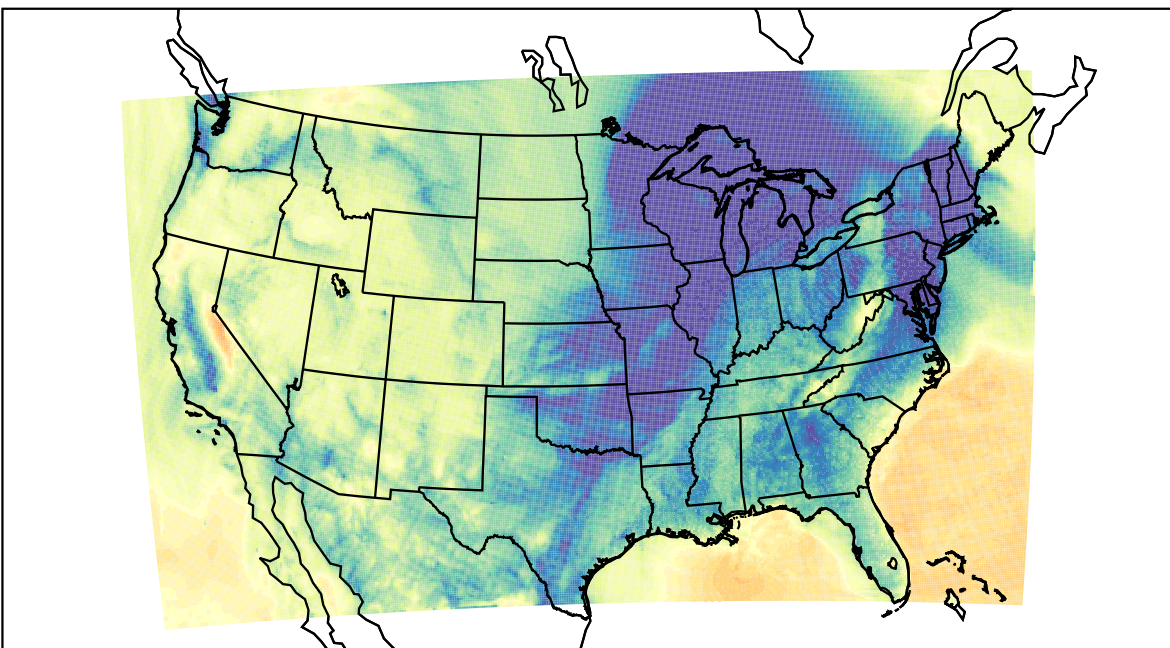
WRF (2023-12-09_10:00:00)
