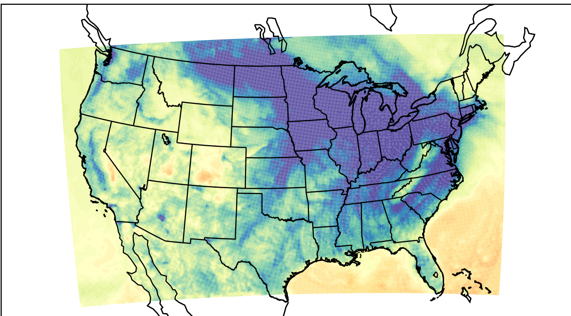
WRF (2023-12-08_04:00:00)
