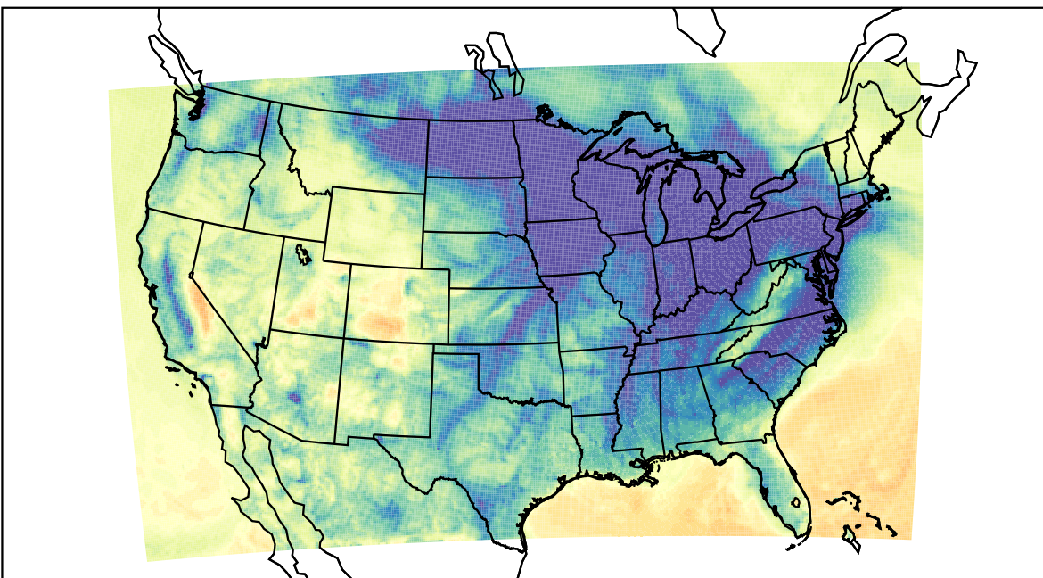
WRF (2023-12-08_07:00:00)
