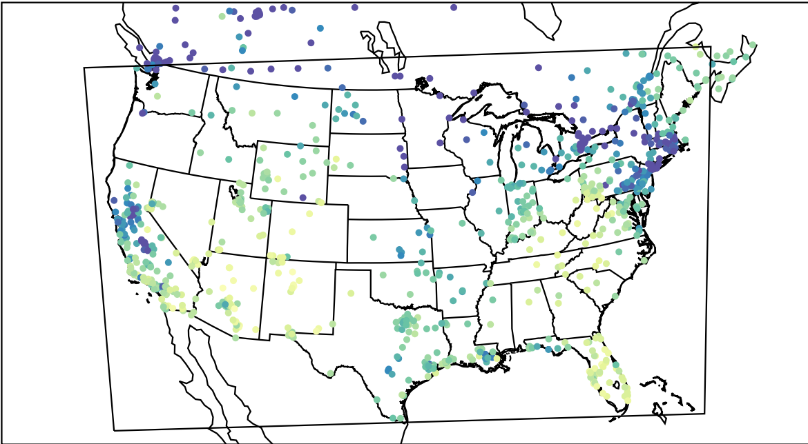
AirNOW (2023-12-08_19:00:00)
