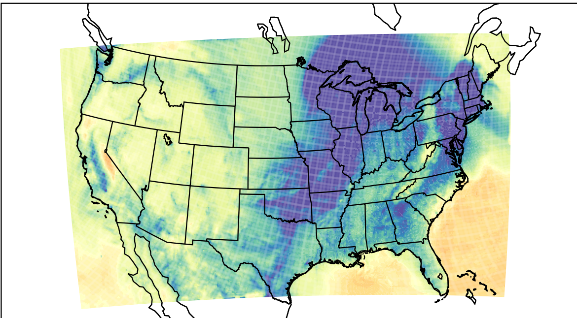
WRF (2023-12-09_12:00:00)
