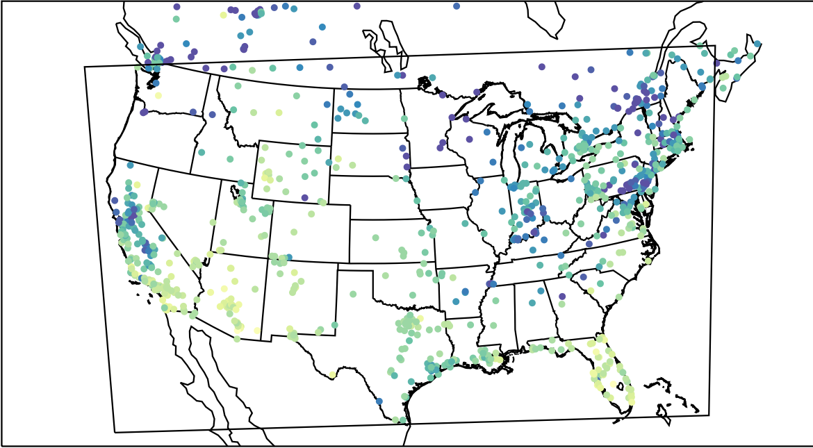
AirNOW (2023-12-09_20:00:00)
