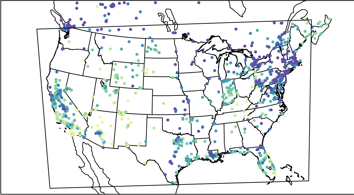
AirNOW (2023-12-09_00:00:00)
