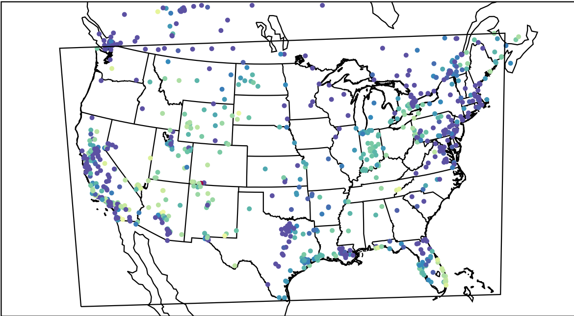
AirNOW (2023-12-09_07:00:00)
