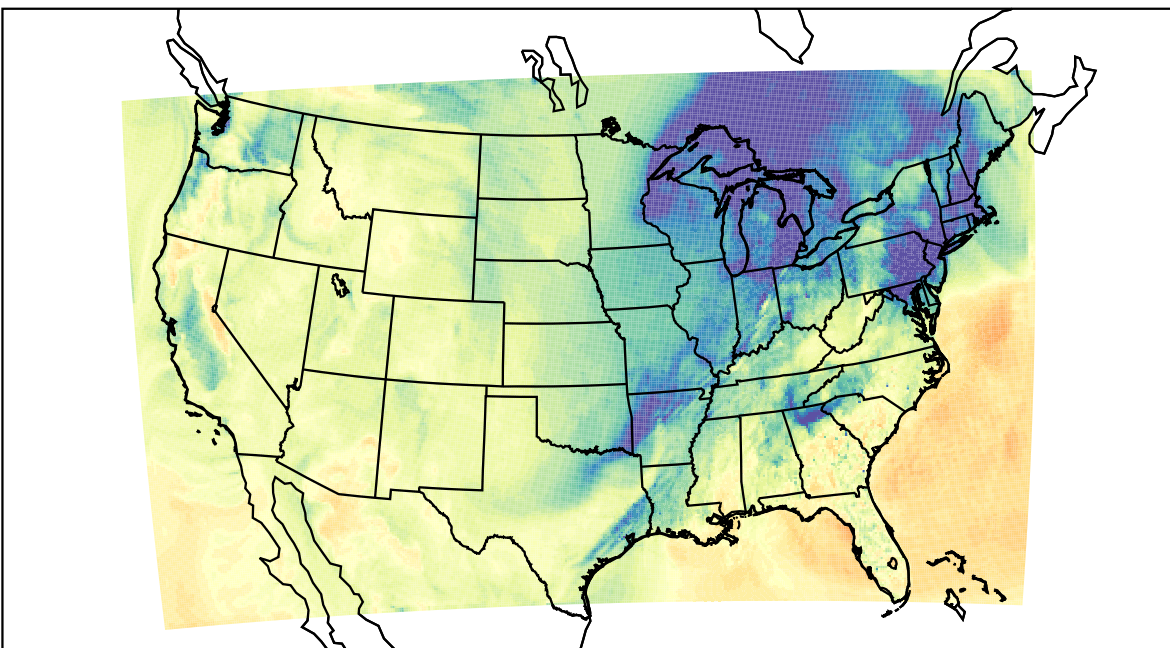
WRF (2023-12-09_21:00:00)
