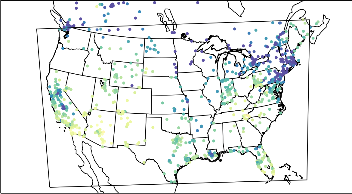
AirNOW (2023-12-08_21:00:00)
