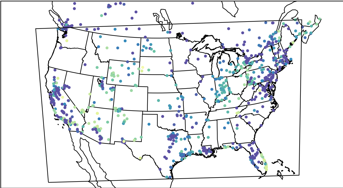
AirNOW (2023-12-09_10:00:00)
