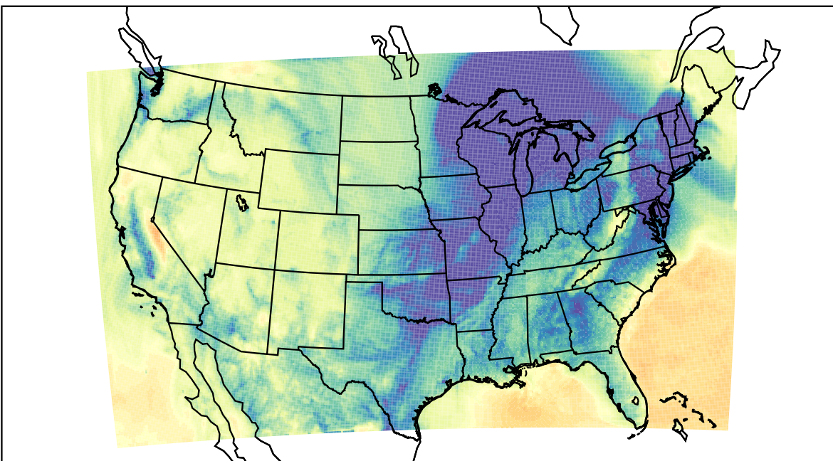
WRF (2023-12-09_11:00:00)
