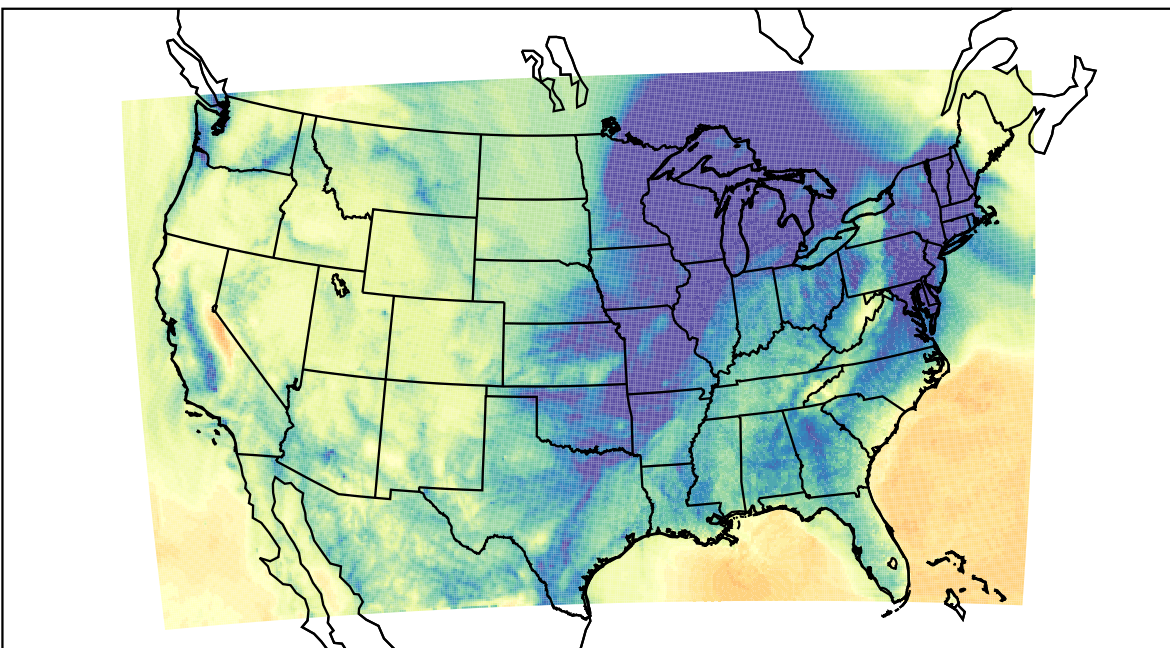
WRF (2023-12-09_09:00:00)
