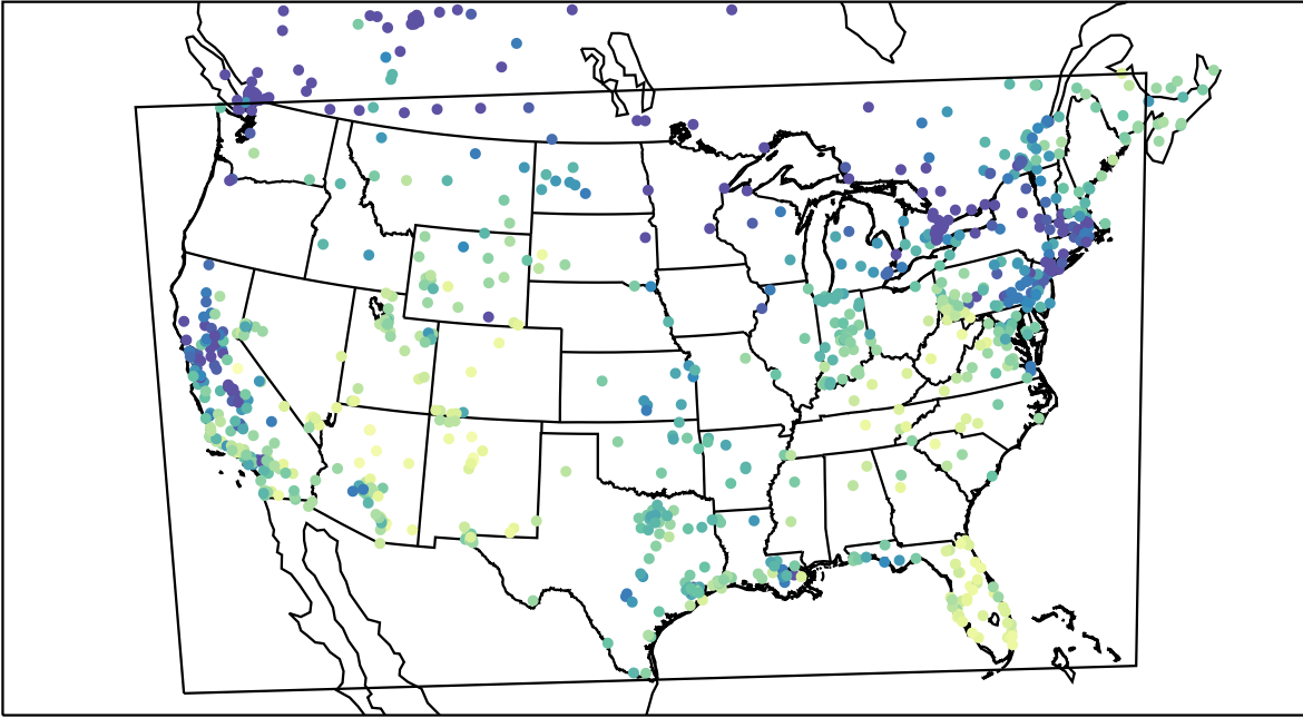
AirNOW (2023-12-08_18:00:00)
