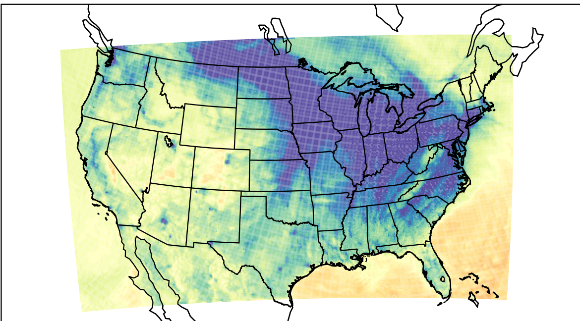
WRF (2023-12-08_01:00:00)
