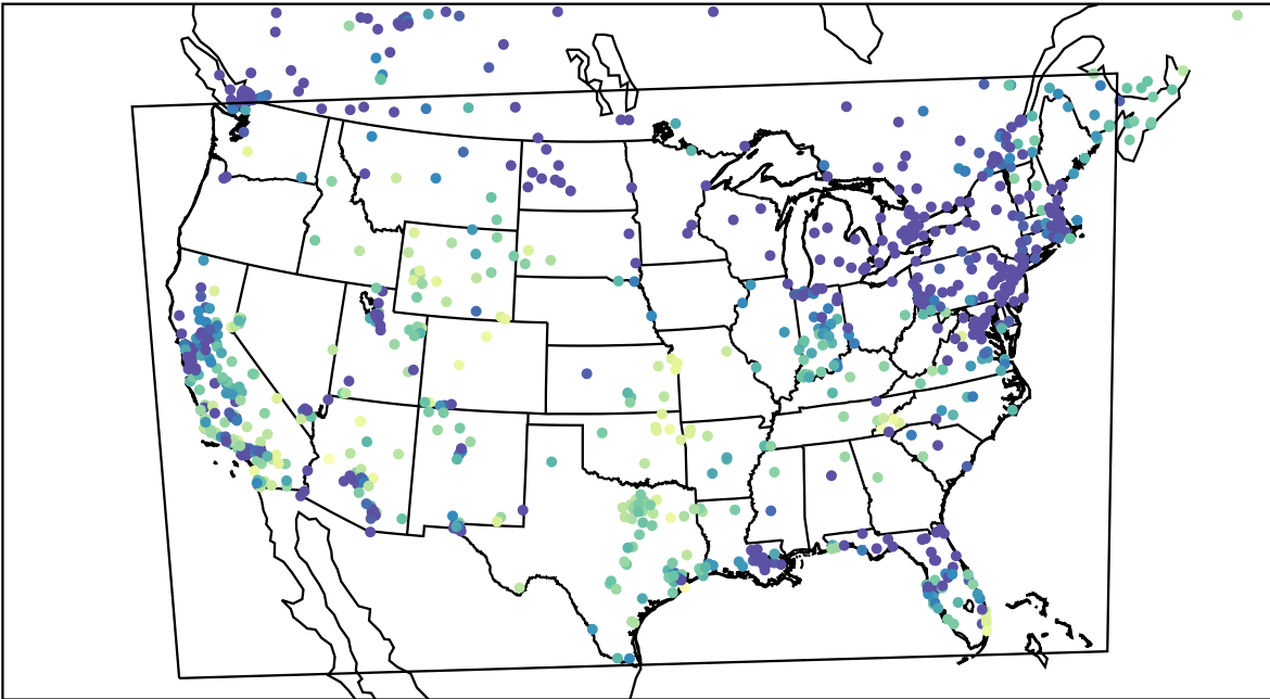
AirNOW (2023-12-08_02:00:00)
