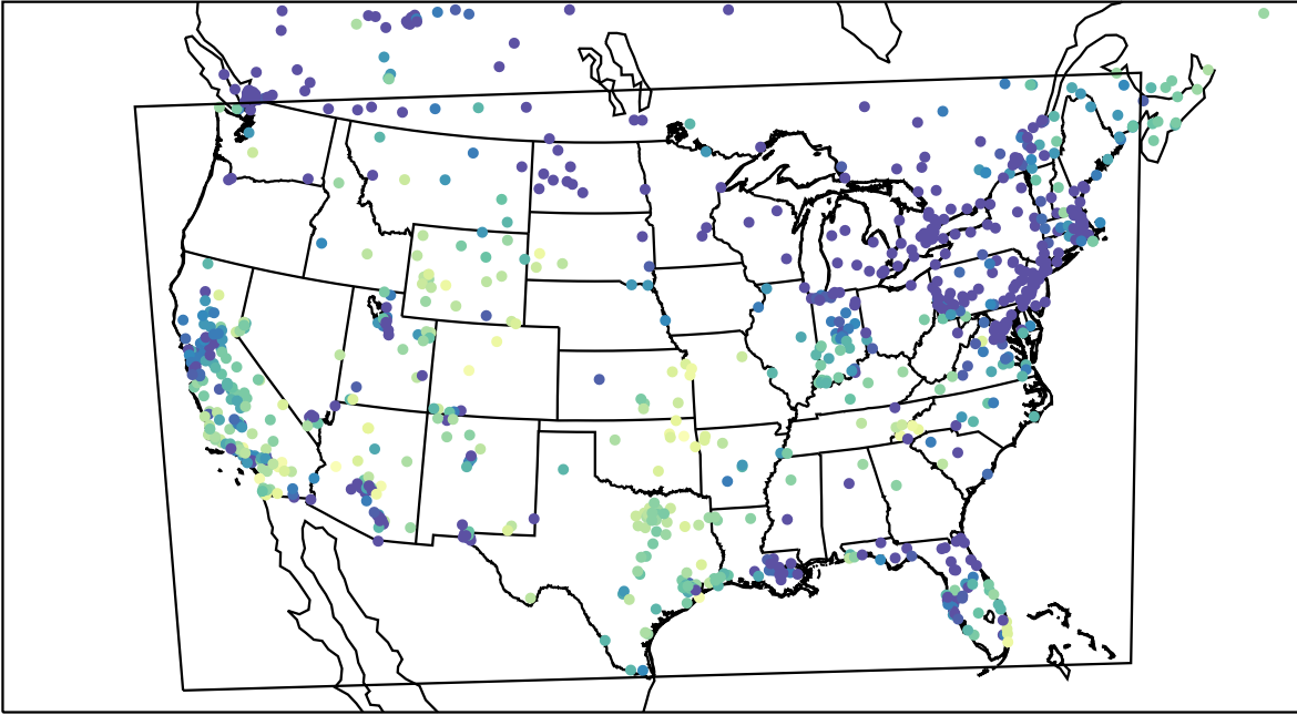
AirNOW (2023-12-08_01:00:00)
