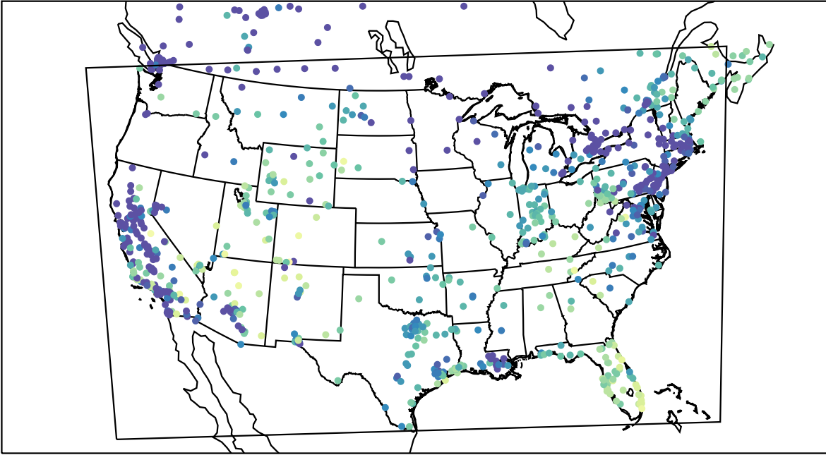
AirNOW (2023-12-08_16:00:00)
