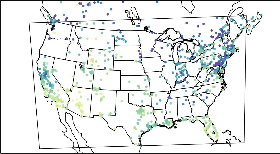
AirNOW (2023-12-09_21:00:00)
