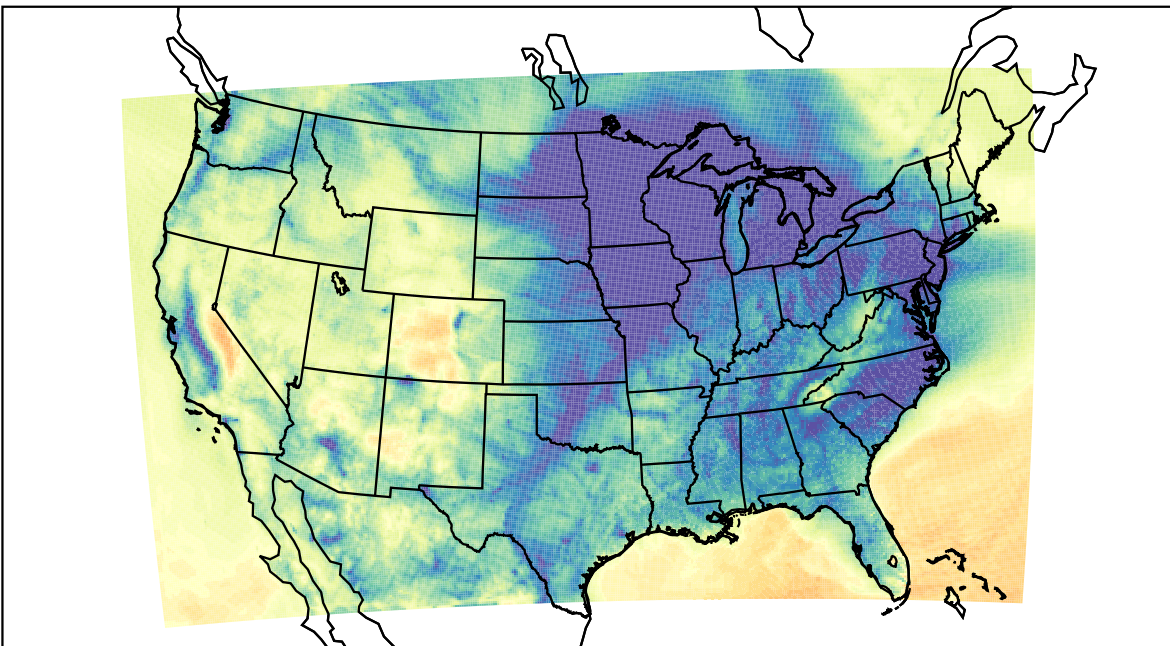
WRF (2023-12-08_14:00:00)
