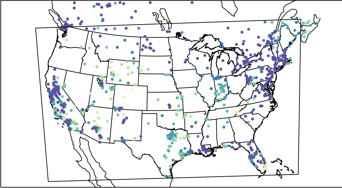
AirNOW (2023-12-08_07:00:00)
