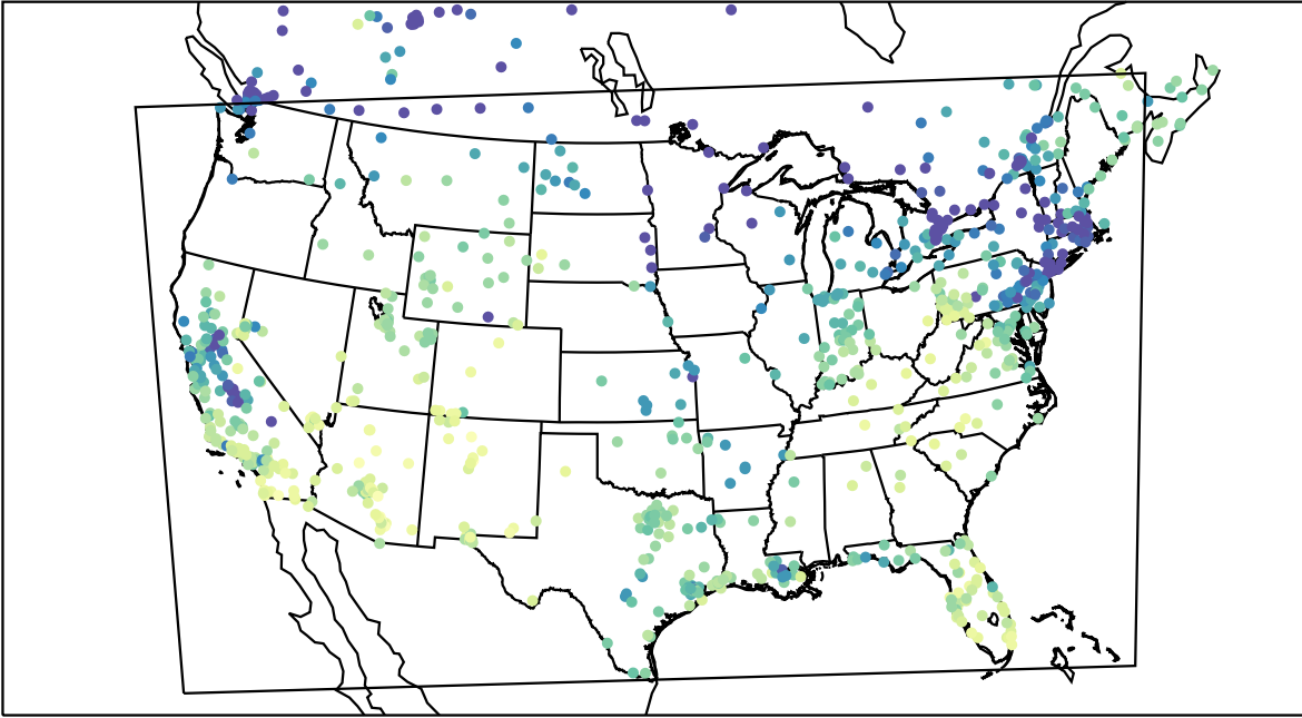
AirNOW (2023-12-08_20:00:00)
