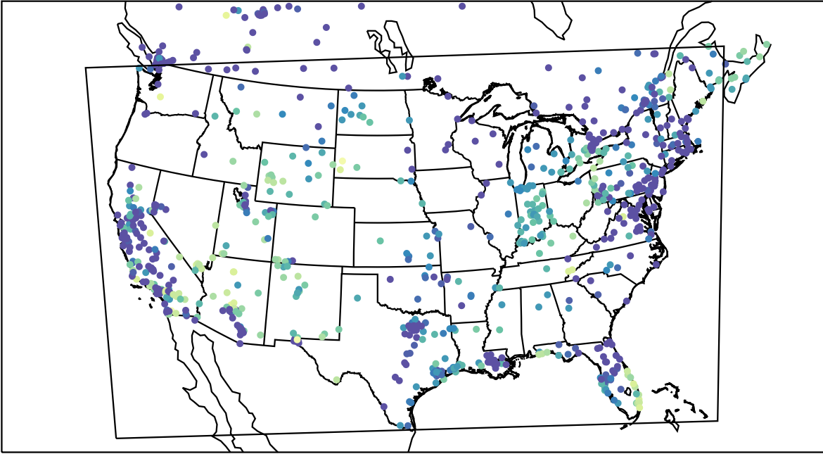
AirNOW (2023-12-09_09:00:00)
