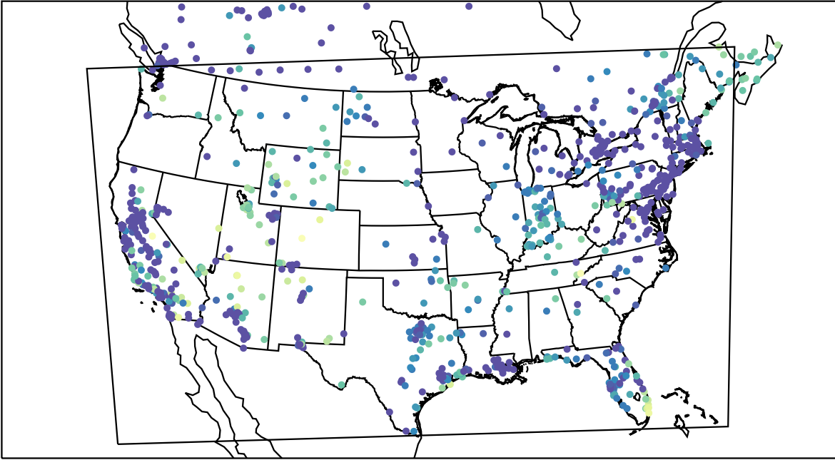
AirNOW (2023-12-08_14:00:00)
