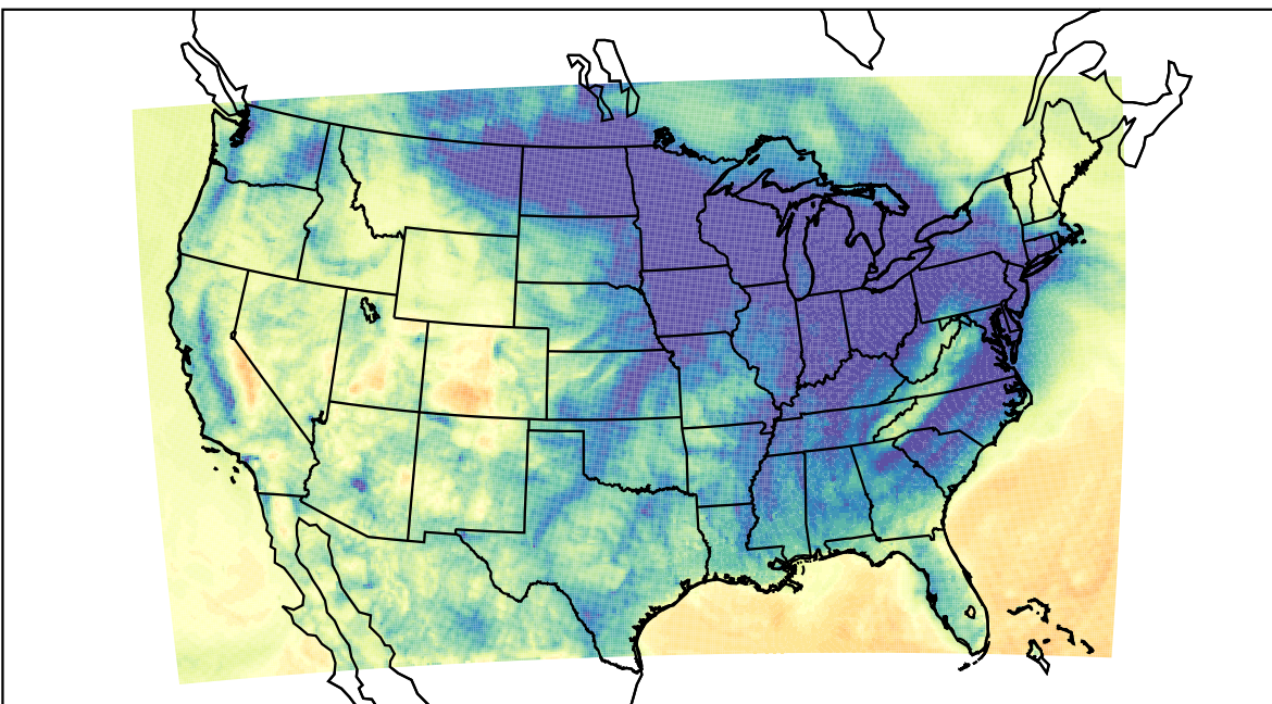
WRF (2023-12-08_06:00:00)
