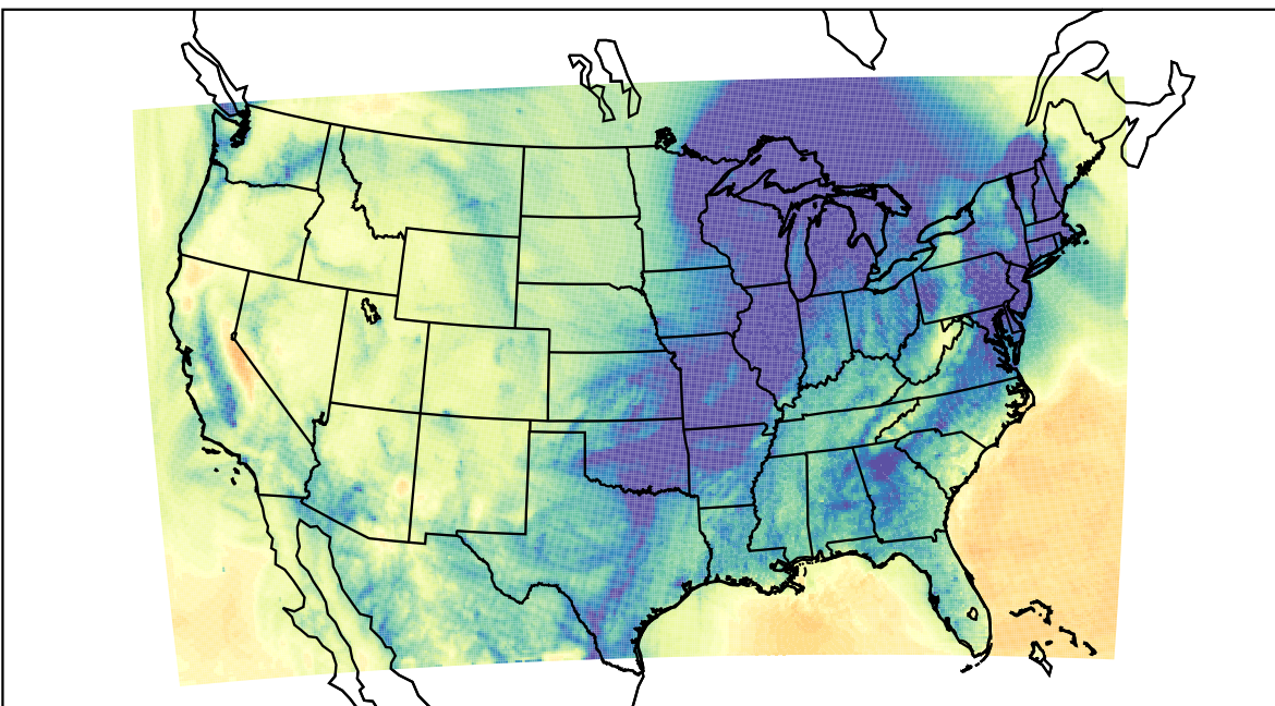
WRF (2023-12-09_13:00:00)
