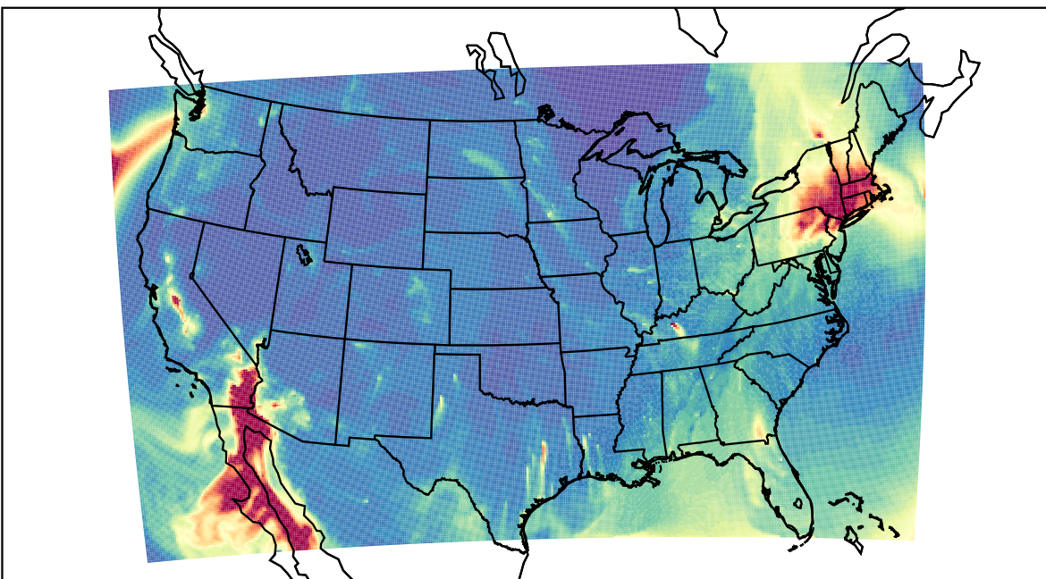
WRF 2023-12-10_07:00:00
