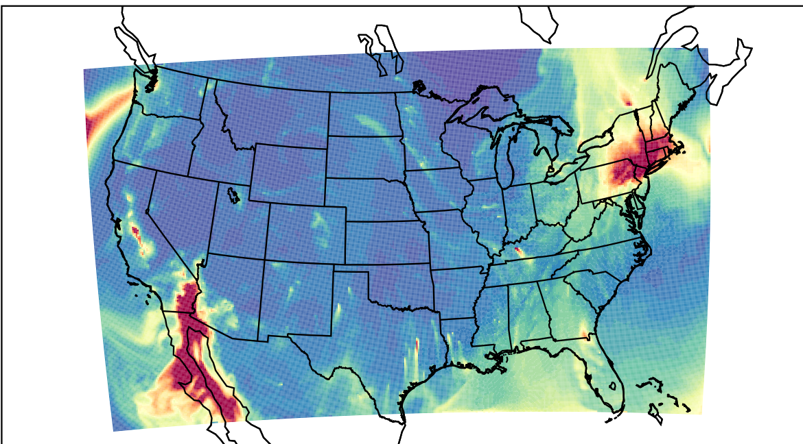
WRF 2023-12-10_06:00:00
