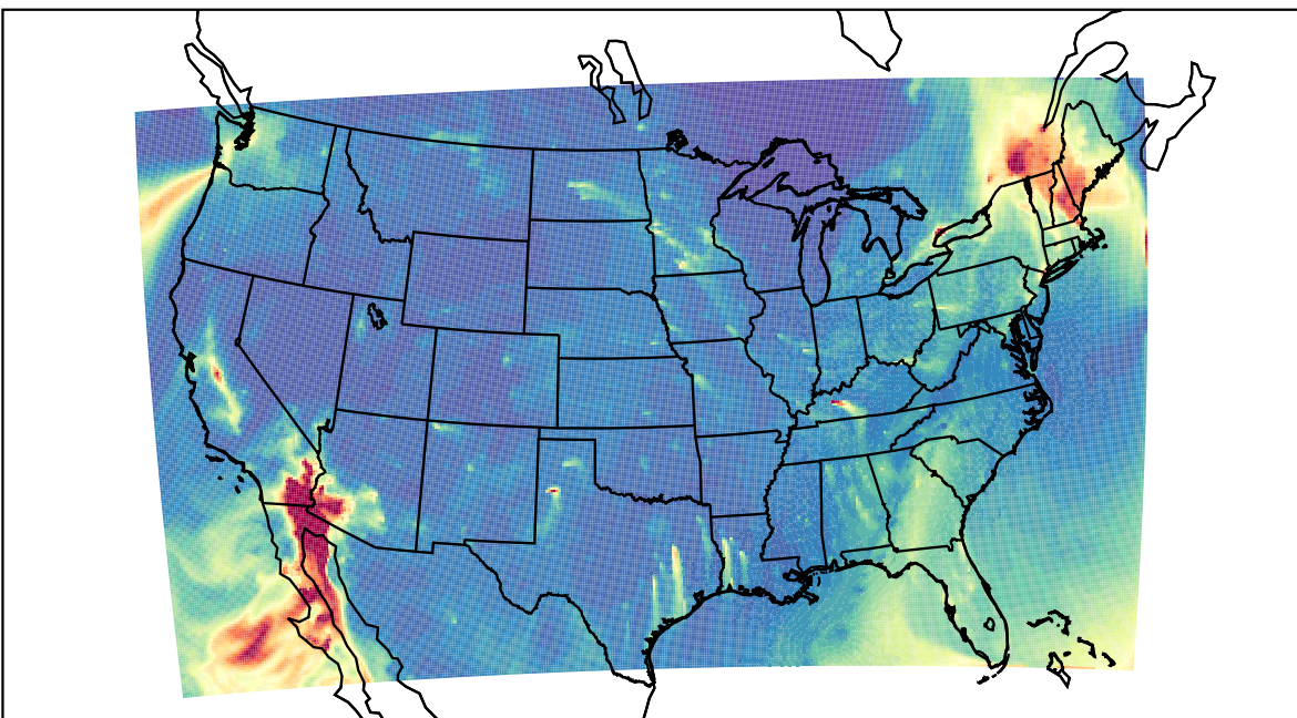
WRF 2023-12-10_14:00:00
