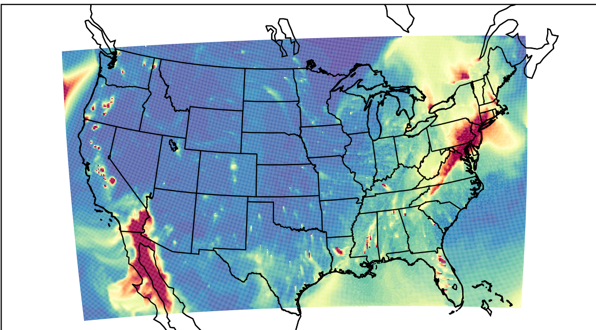
WRF 2023-12-10_01:00:00
