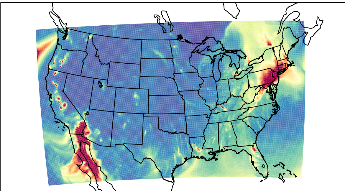
WRF 2023-12-10_03:00:00
