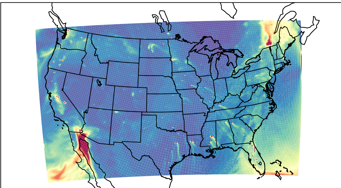
WRF 2023-12-10_21:00:00
