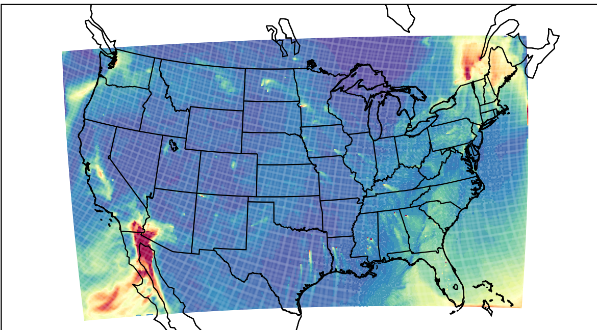
WRF 2023-12-10_18:00:00
