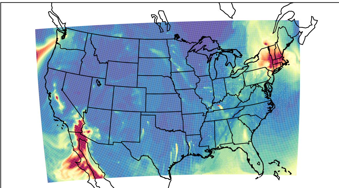
WRF 2023-12-10_09:00:00
