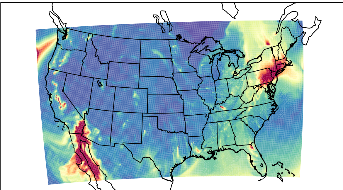
WRF 2023-12-10_04:00:00
