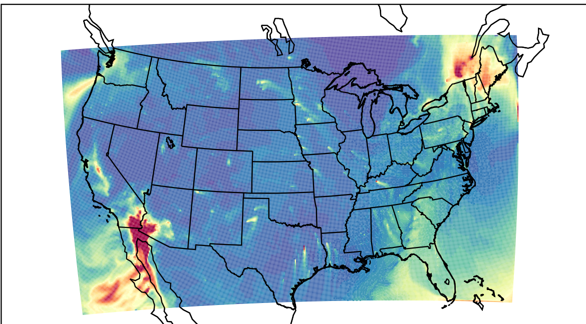
WRF 2023-12-10_16:00:00
