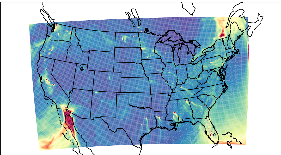
WRF 2023-12-10_22:00:00
