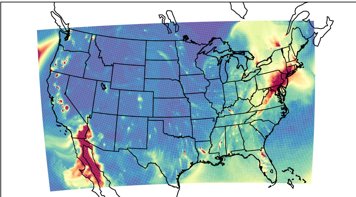
WRF 2023-12-10_02:00:00
