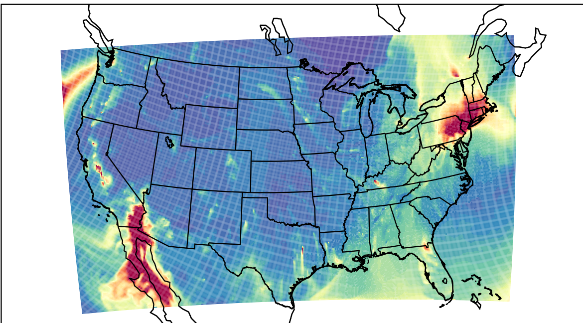
WRF 2023-12-10_05:00:00
