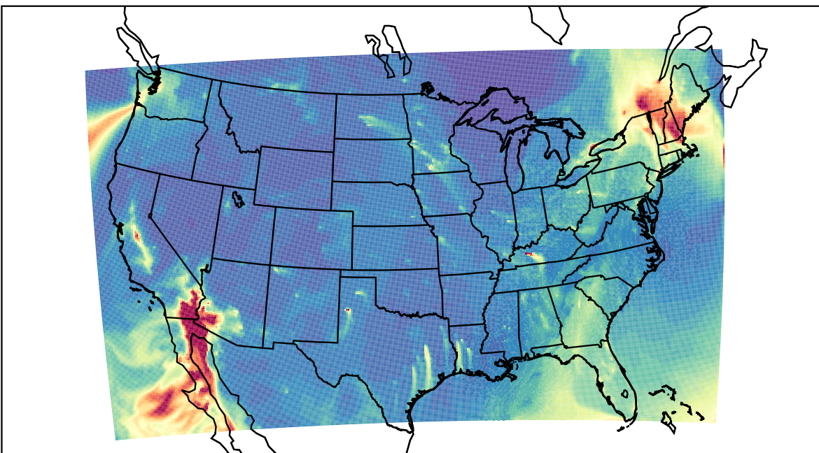
WRF 2023-12-10_13:00:00
