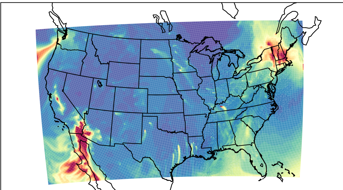
WRF 2023-12-10_11:00:00
