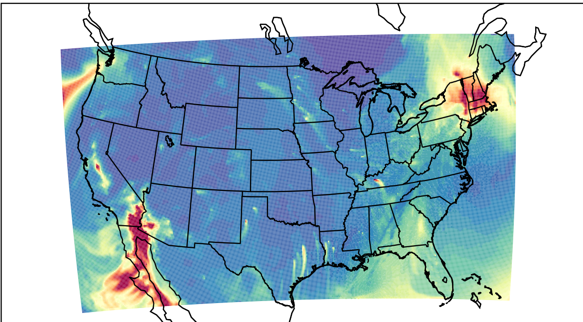
WRF 2023-12-10_10:00:00
