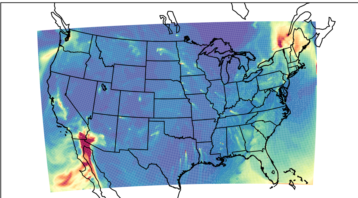
WRF 2023-12-10_17:00:00
