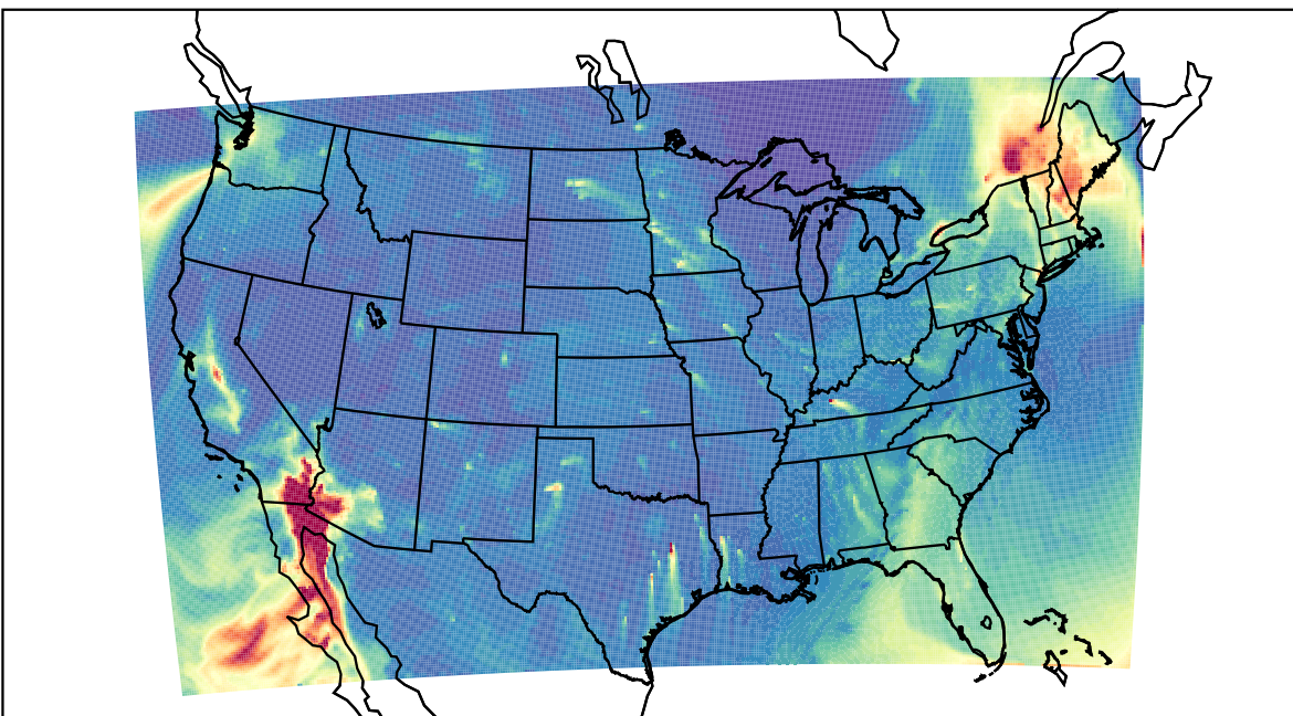
WRF 2023-12-10_15:00:00
