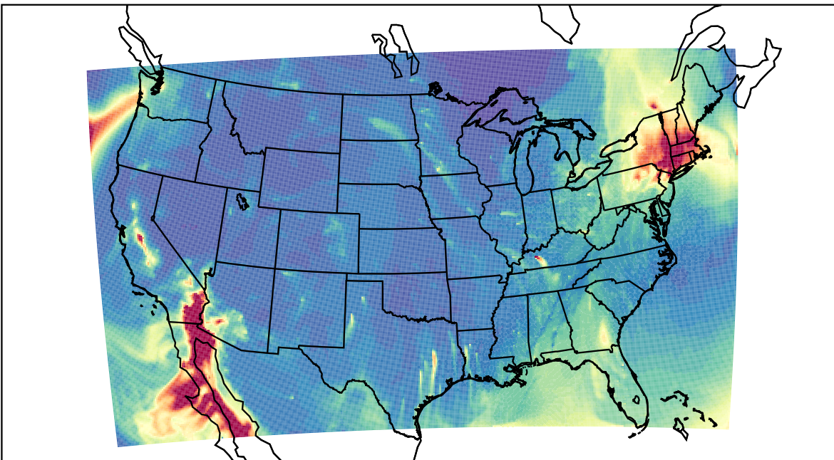
WRF 2023-12-10_08:00:00
