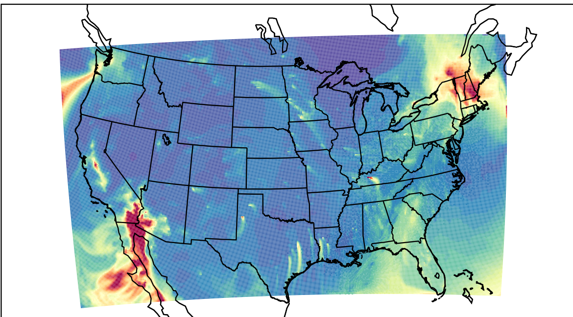
WRF 2023-12-10_12:00:00
