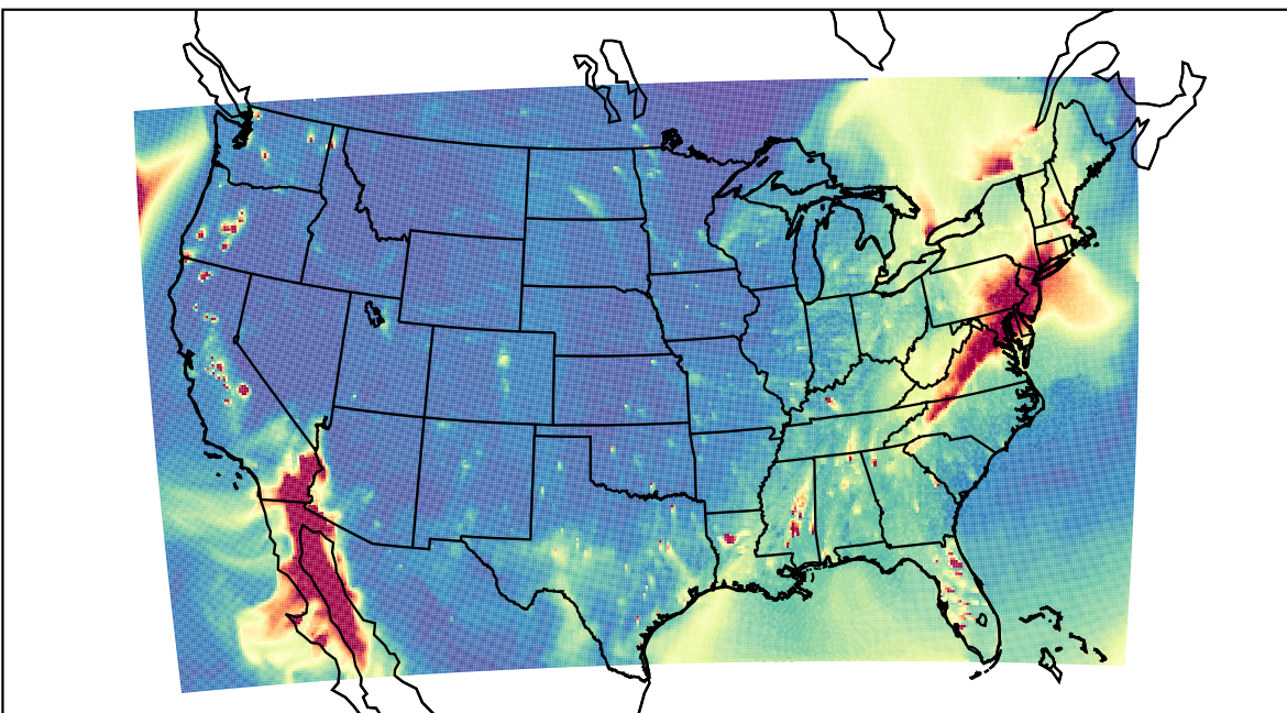
WRF 2023-12-10_00:00:00
