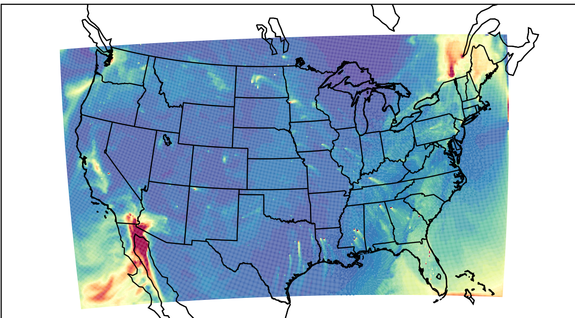
WRF 2023-12-10_19:00:00
