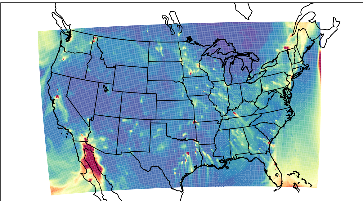
WRF 2023-12-11_02:00:00
