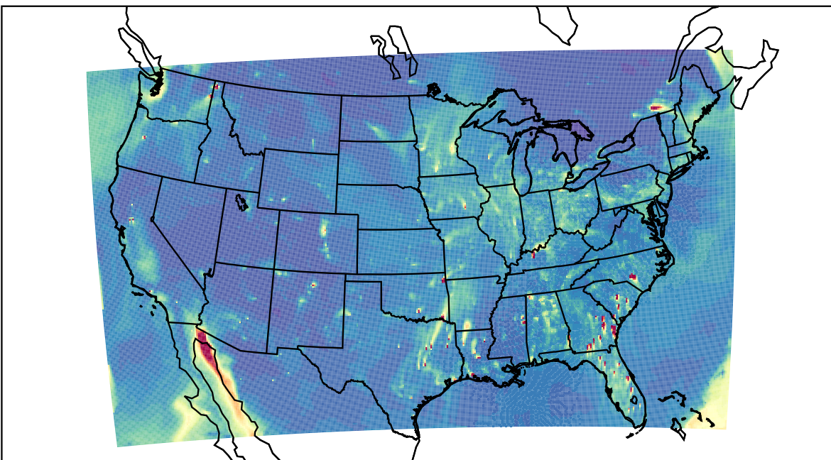
WRF 2023-12-11_23:00:00
