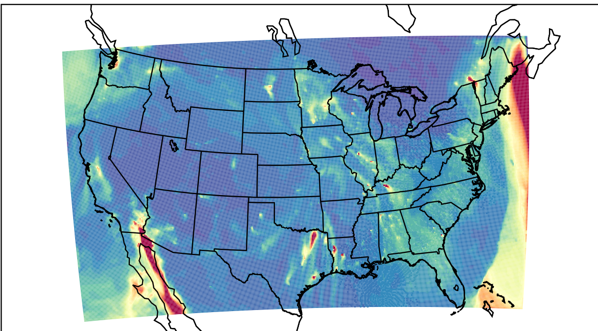
WRF 2023-12-11_12:00:00
