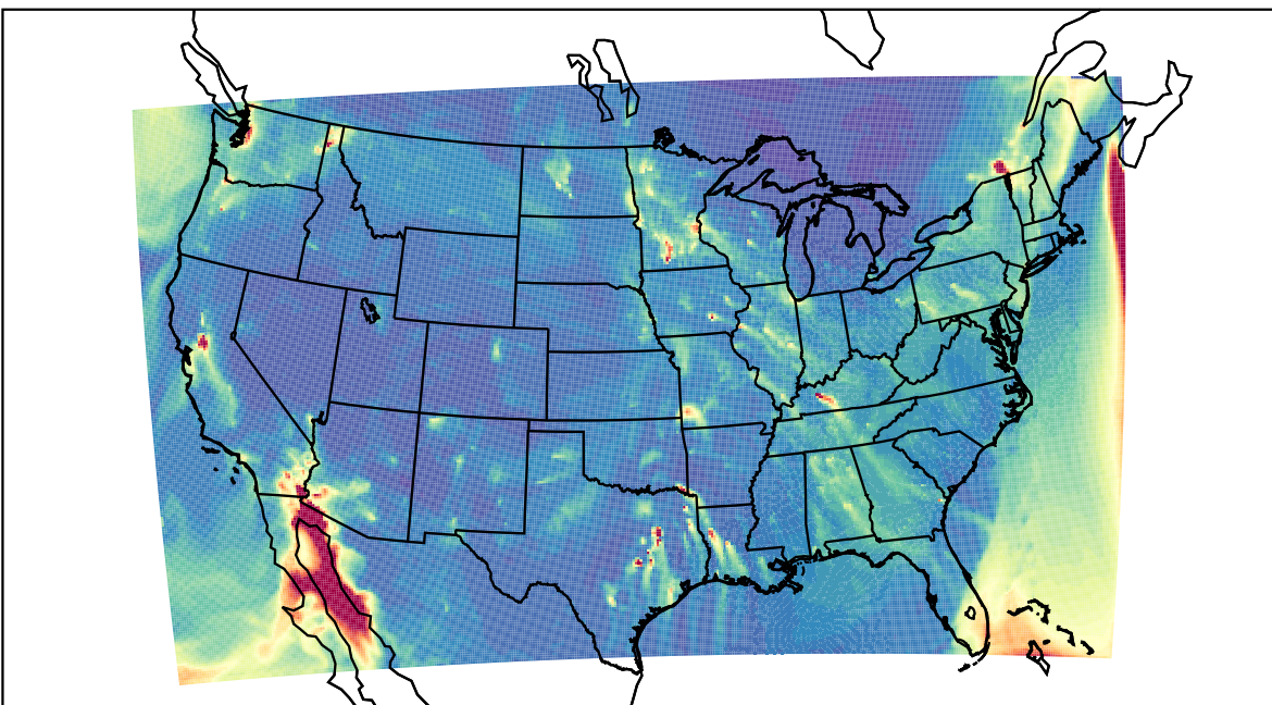
WRF 2023-12-11_05:00:00
