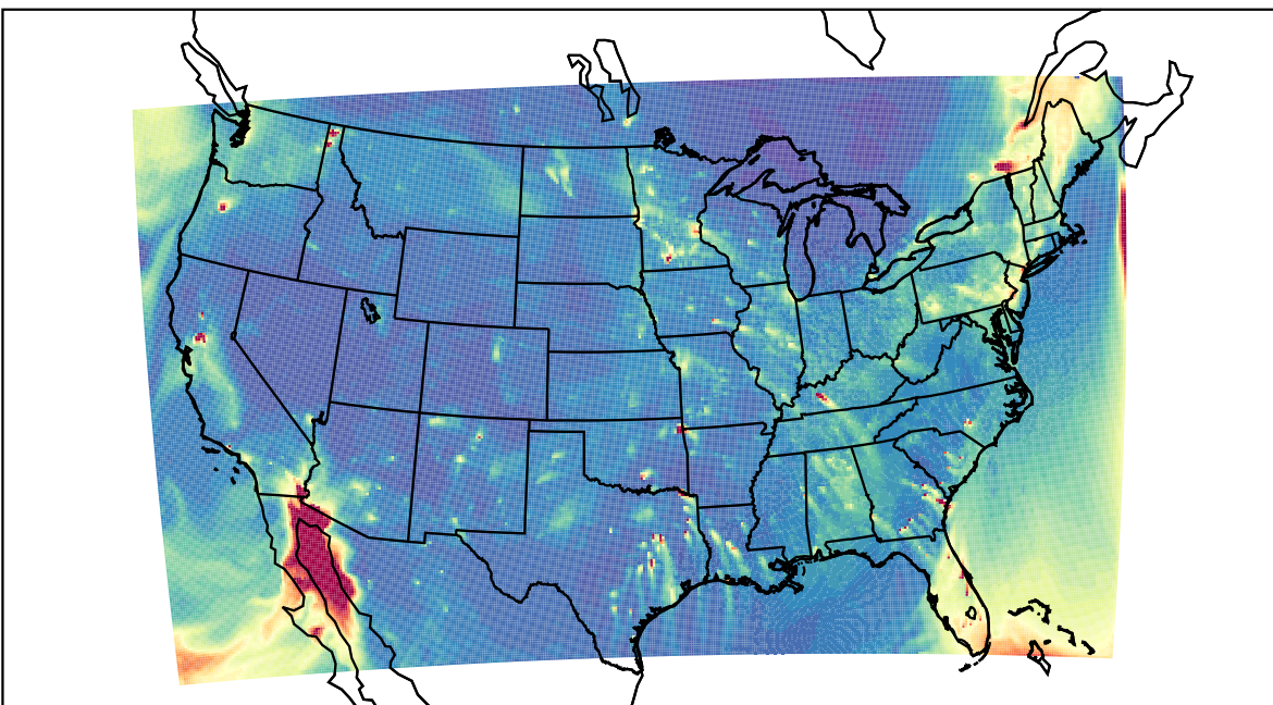
WRF 2023-12-11_01:00:00
