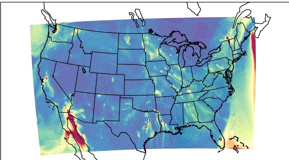
WRF 2023-12-11_06:00:00
