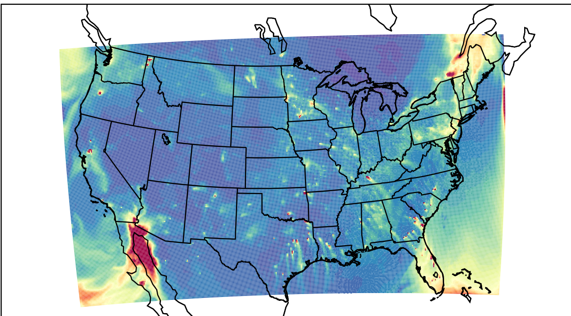
WRF 2023-12-11_00:00:00
