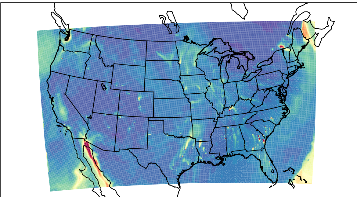
WRF 2023-12-11_20:00:00
