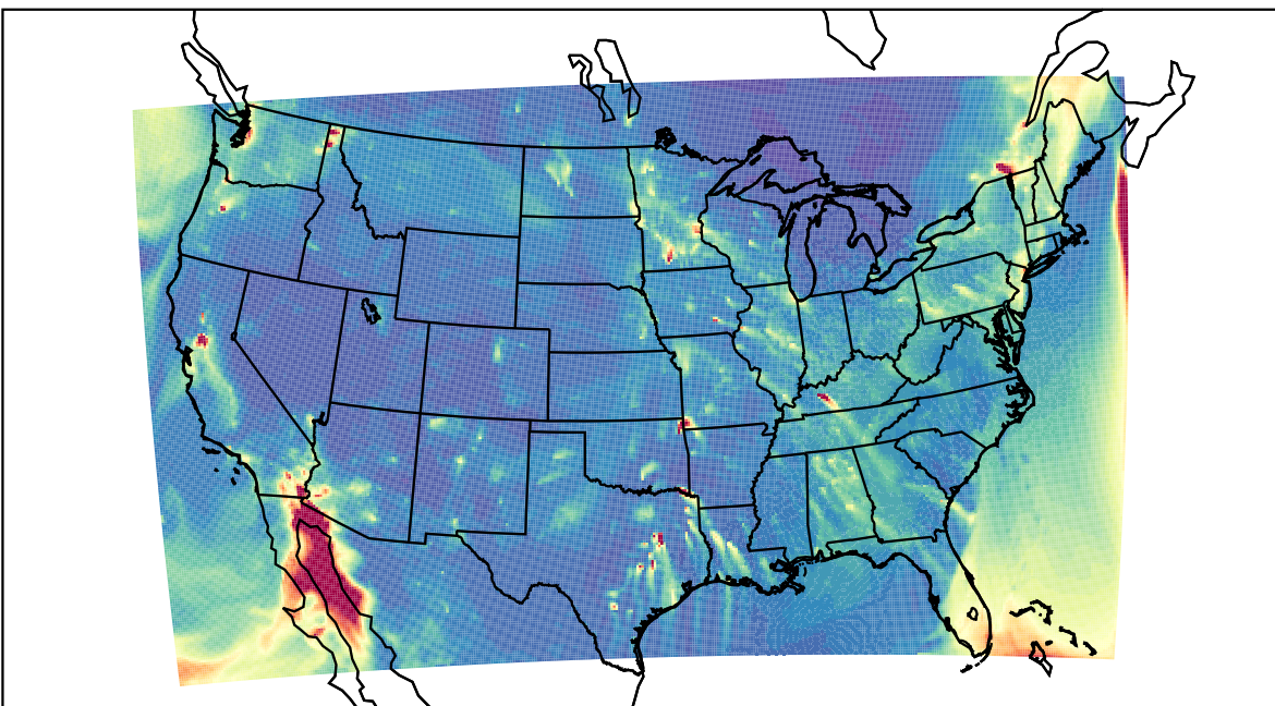
WRF 2023-12-11_03:00:00
