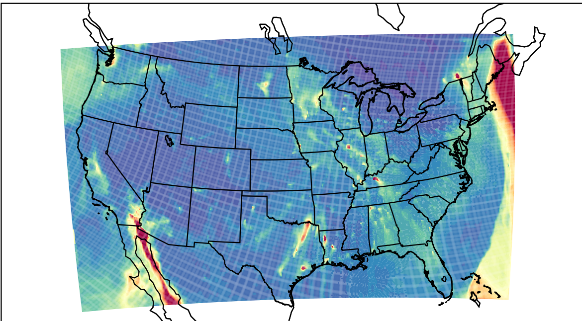
WRF 2023-12-11_14:00:00
