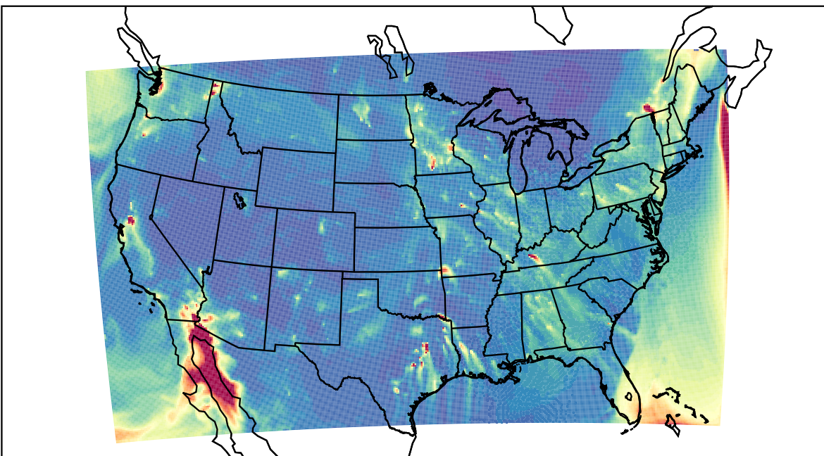
WRF 2023-12-11_04:00:00
