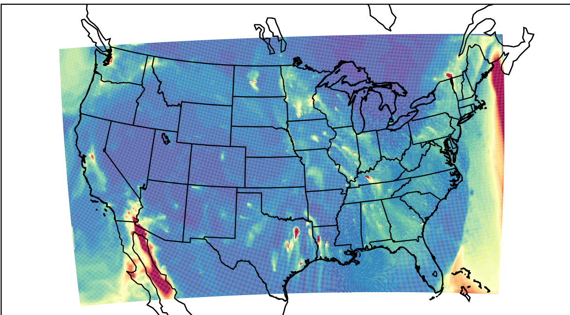
WRF 2023-12-11_09:00:00
