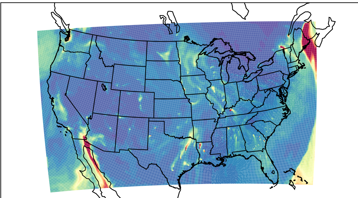
WRF 2023-12-11_17:00:00
