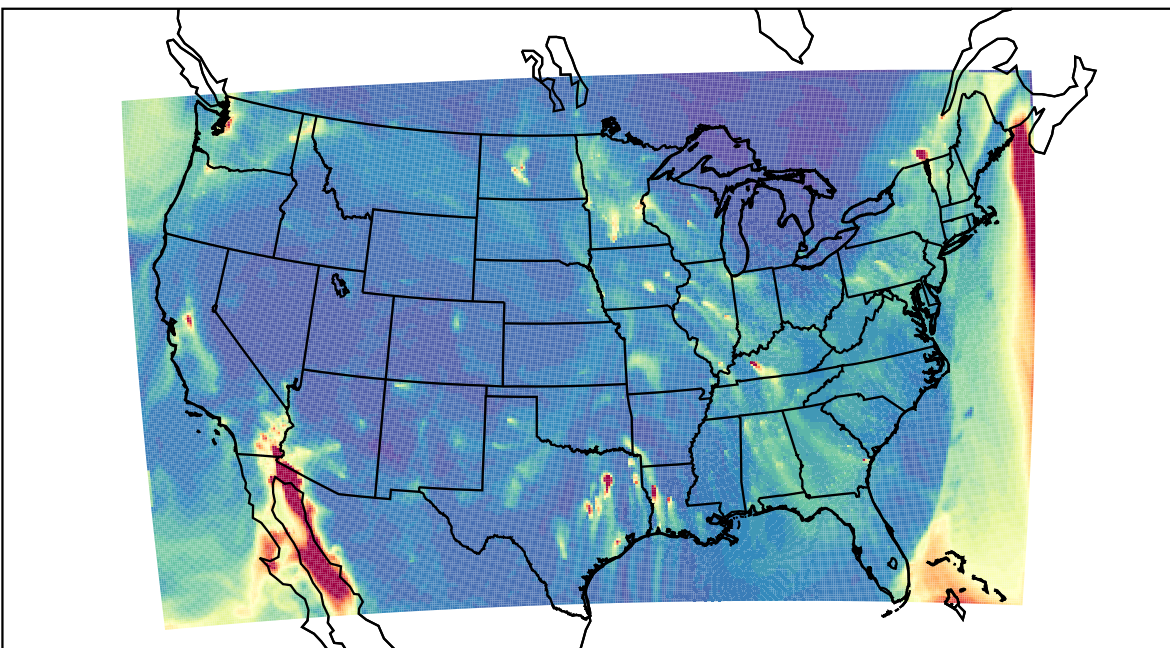
WRF 2023-12-11_08:00:00
