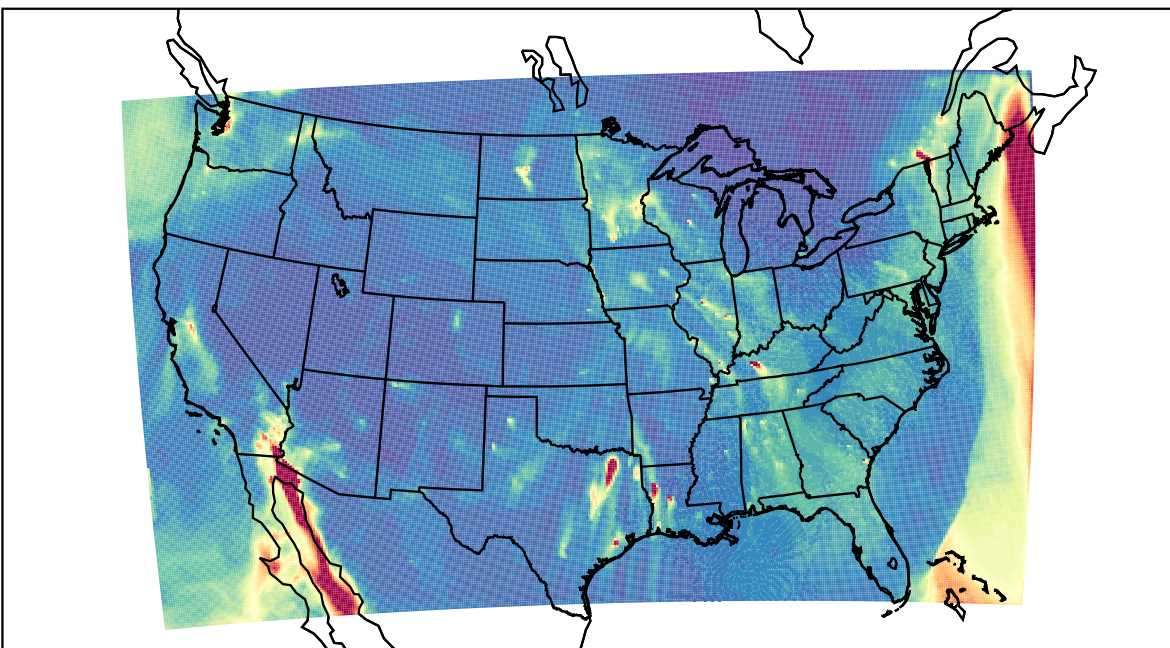
WRF 2023-12-11_11:00:00
