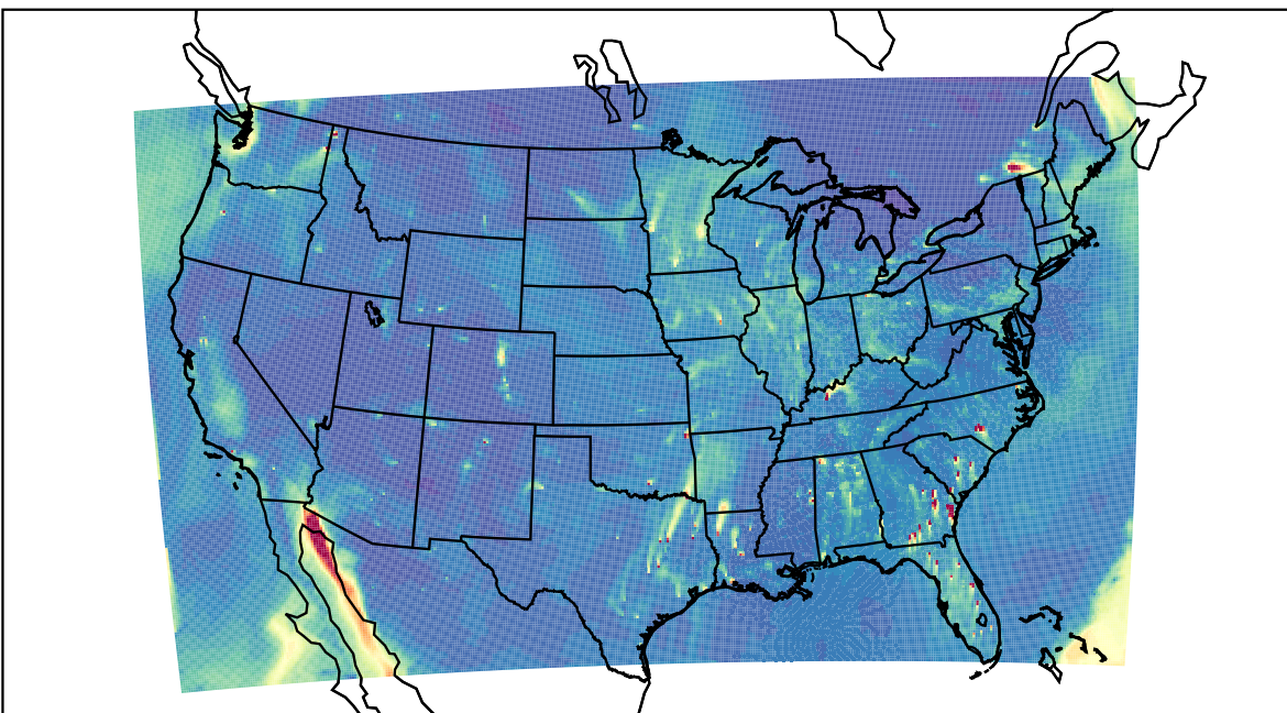
WRF 2023-12-11_22:00:00
