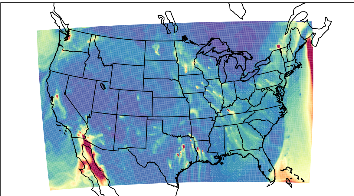
WRF 2023-12-11_07:00:00
