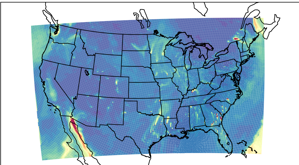
WRF 2023-12-11_21:00:00
