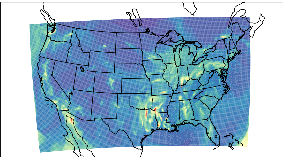
WRF 2023-12-12_08:00:00
