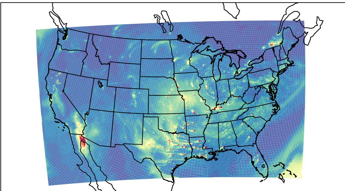
WRF 2023-12-13_22:00:00
