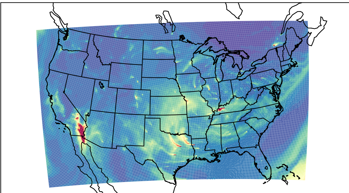
WRF 2023-12-13_17:00:00
