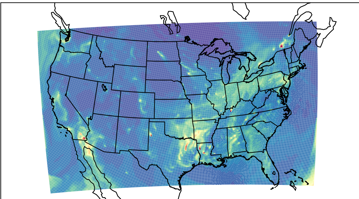
WRF 2023-12-12_14:00:00
