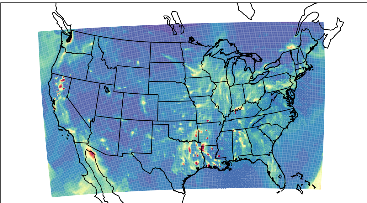
WRF 2023-12-12_03:00:00
