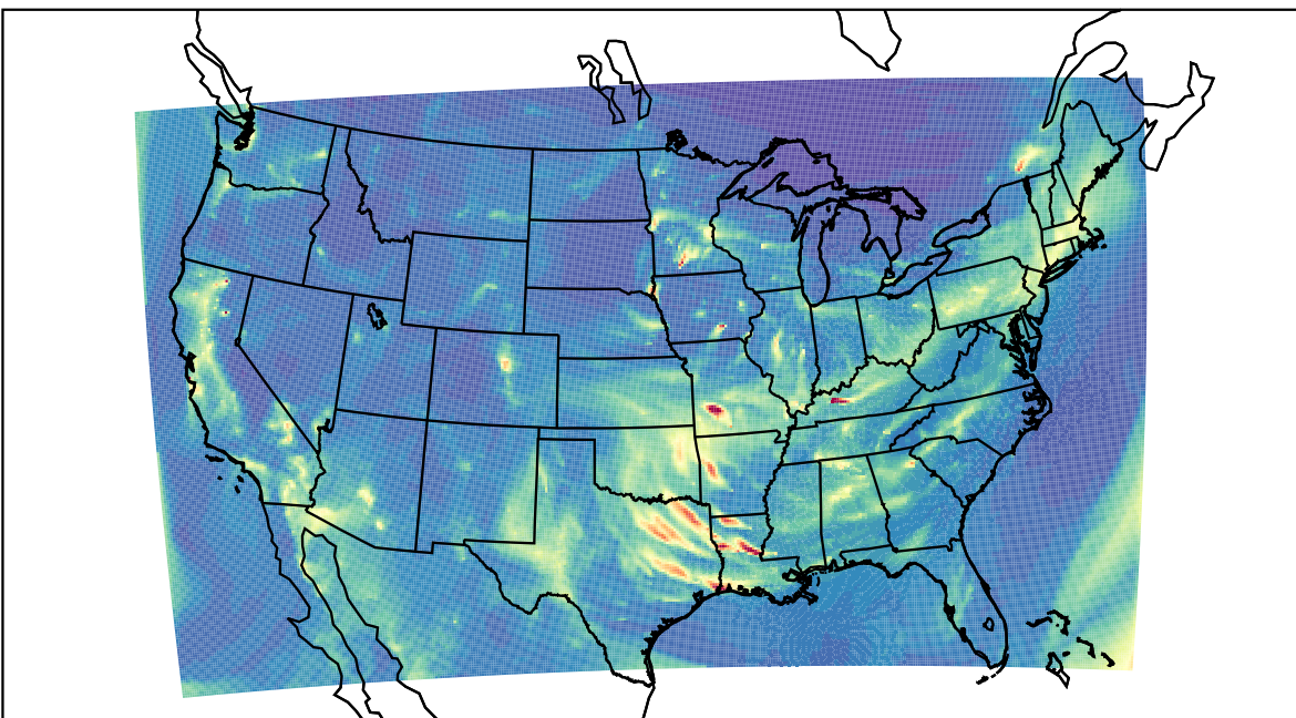
WRF 2023-12-13_05:00:00
