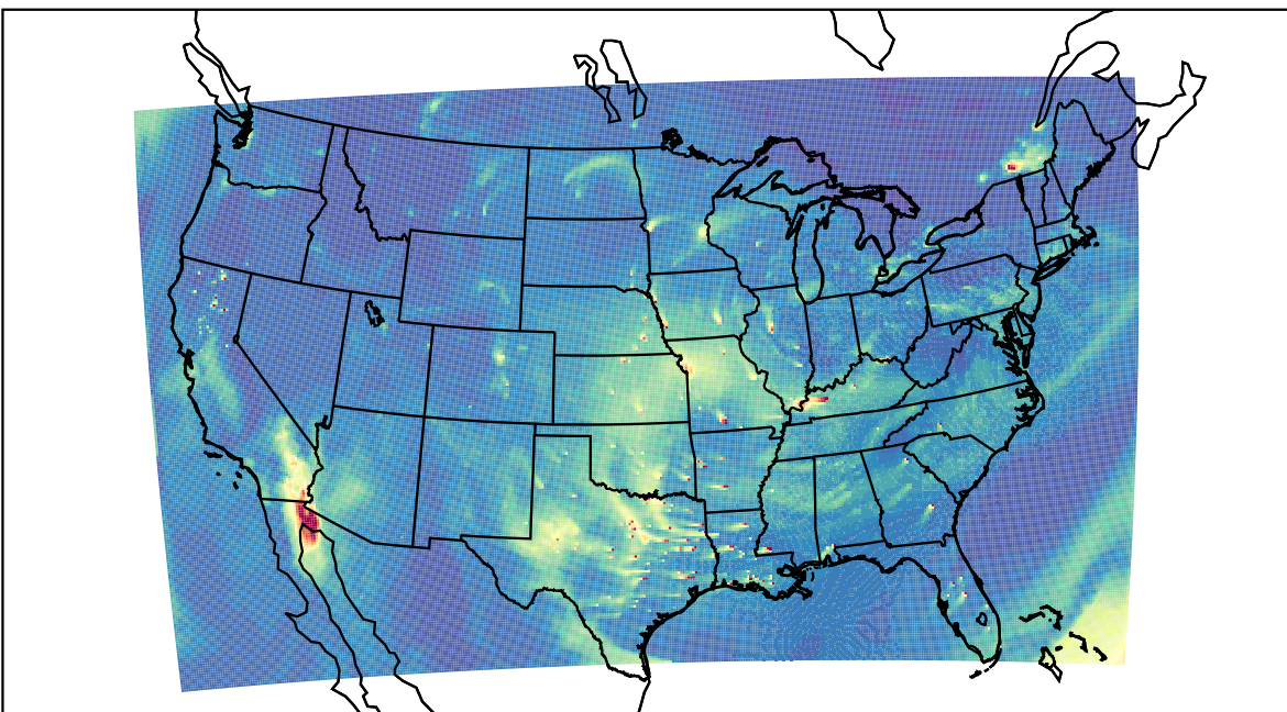
WRF 2023-12-13_21:00:00
