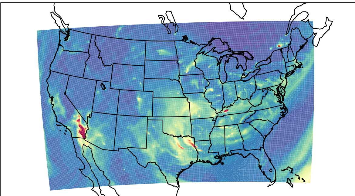
WRF 2023-12-13_14:00:00
