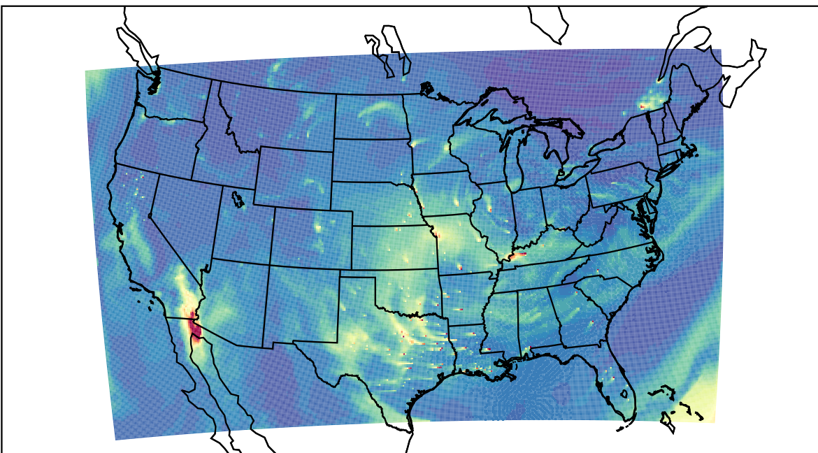
WRF 2023-12-13_20:00:00
