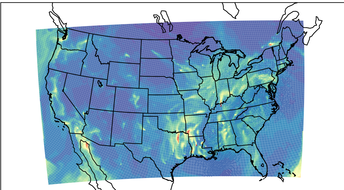
WRF 2023-12-12_09:00:00
