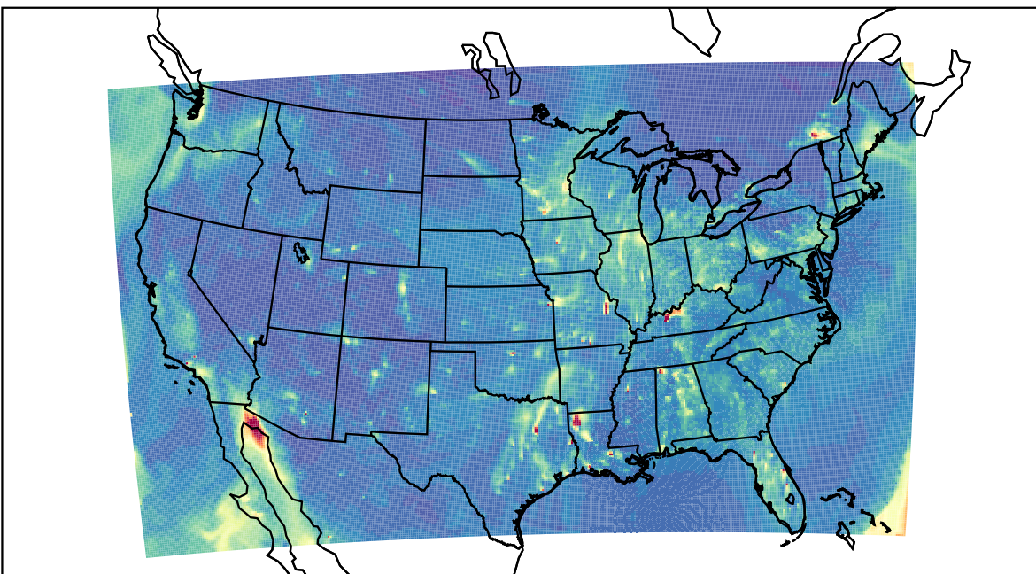
WRF 2023-12-12_00:00:00
