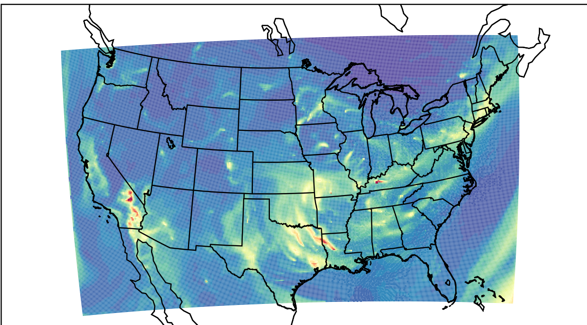
WRF 2023-12-13_09:00:00
