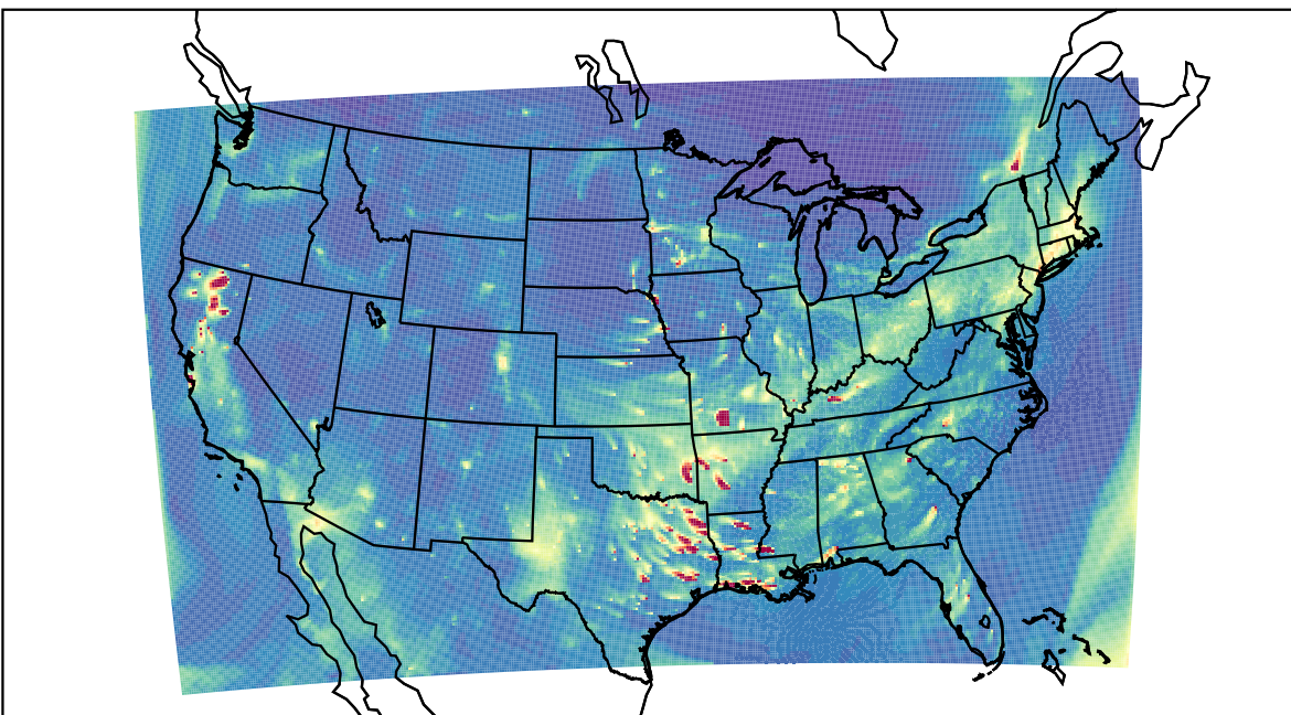
WRF 2023-12-13_01:00:00
