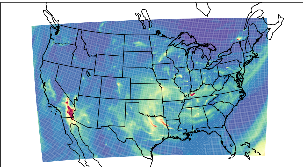
WRF 2023-12-13_15:00:00
