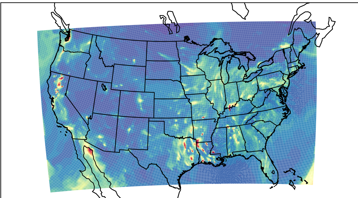
WRF 2023-12-12_04:00:00
