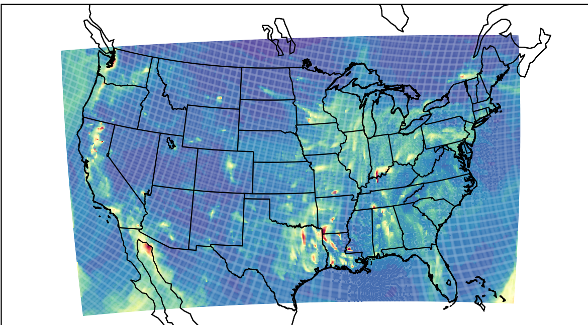
WRF 2023-12-12_05:00:00
