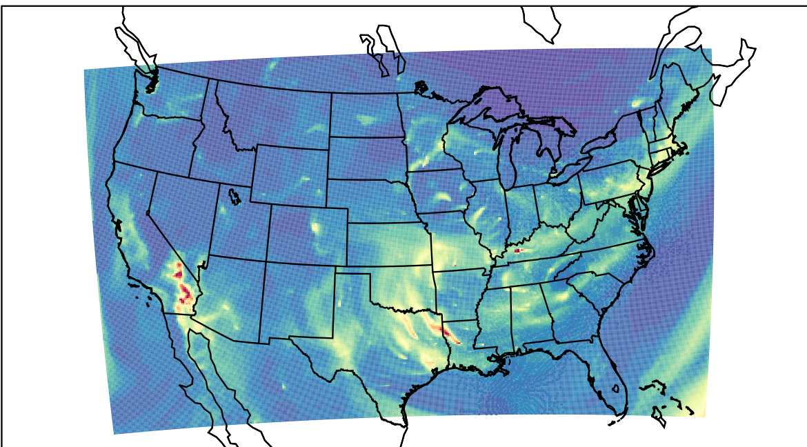
WRF 2023-12-13_10:00:00
