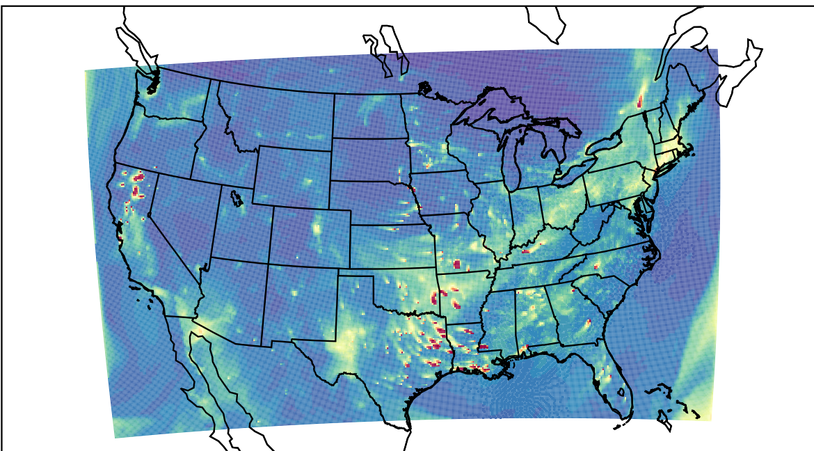
WRF 2023-12-13_00:00:00
