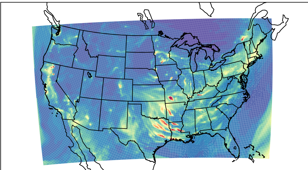
WRF 2023-12-13_04:00:00
