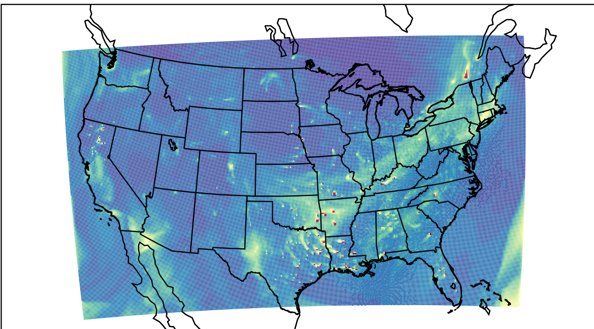
WRF 2023-12-12_22:00:00
