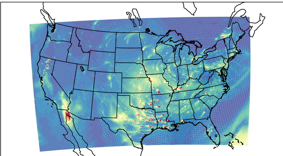
WRF 2023-12-13_23:00:00
