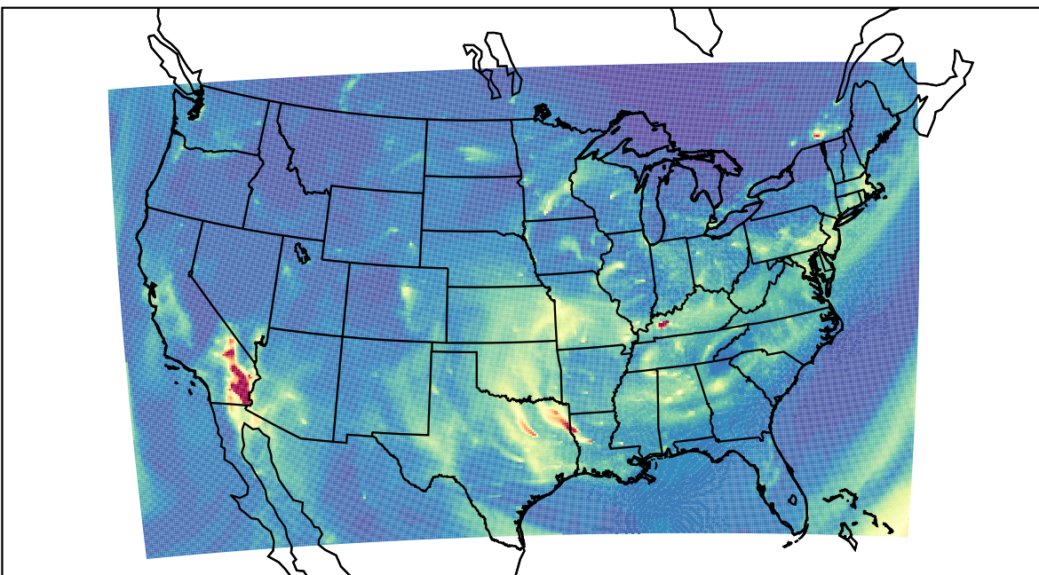
WRF 2023-12-13_13:00:00
