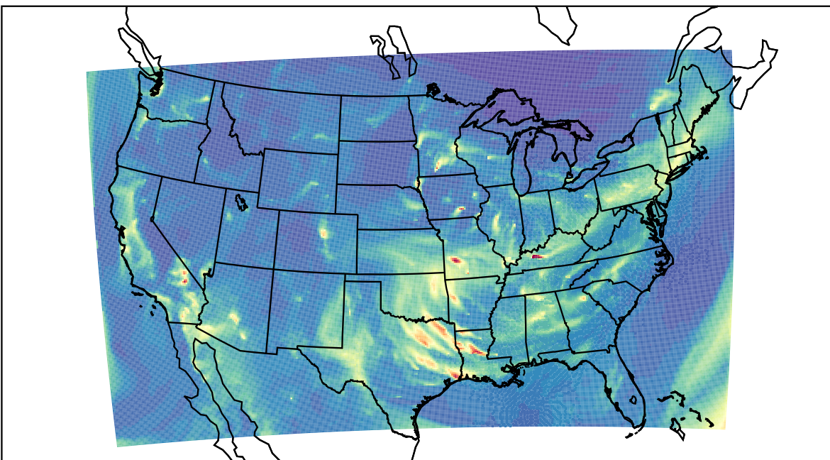
WRF 2023-12-13_06:00:00
