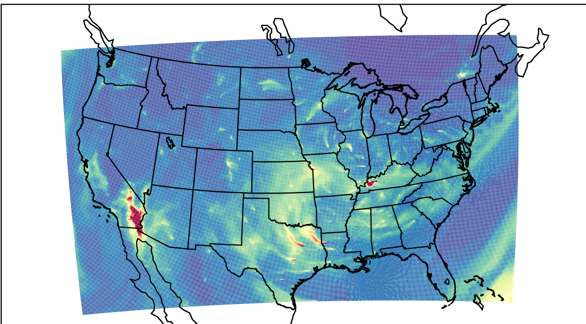
WRF 2023-12-13_16:00:00
