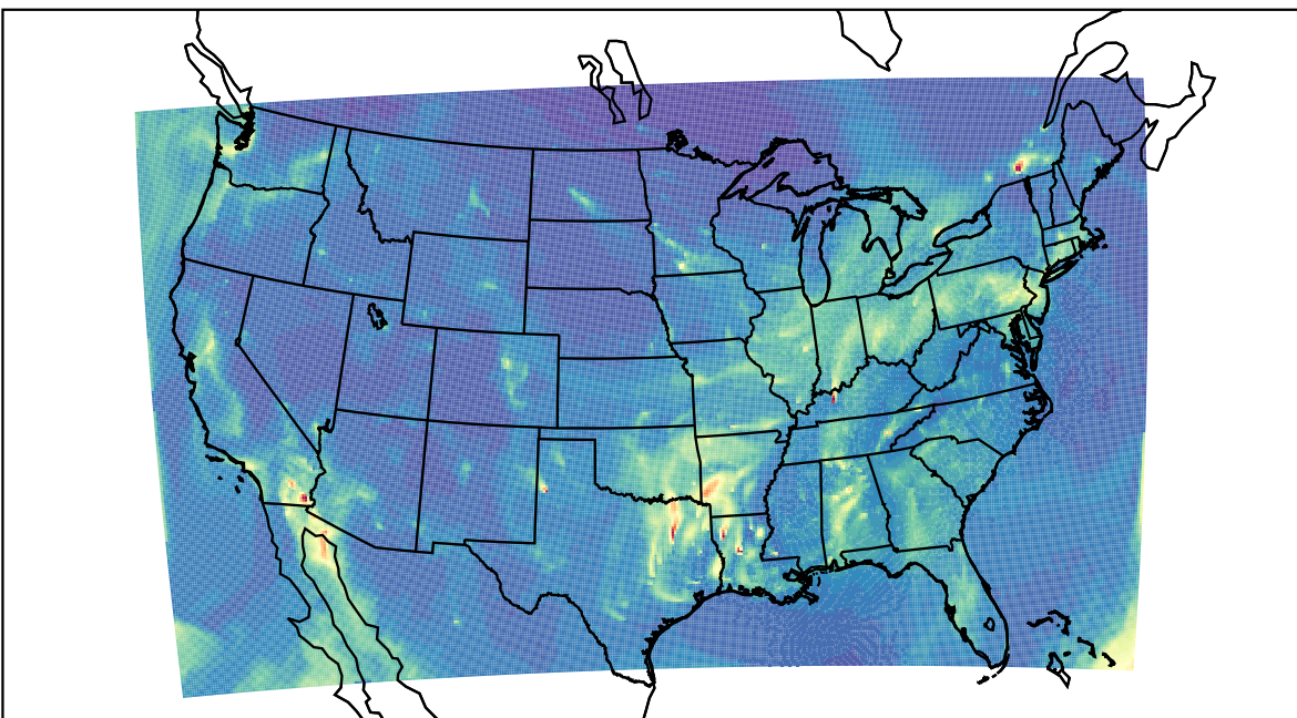
WRF 2023-12-12_12:00:00
