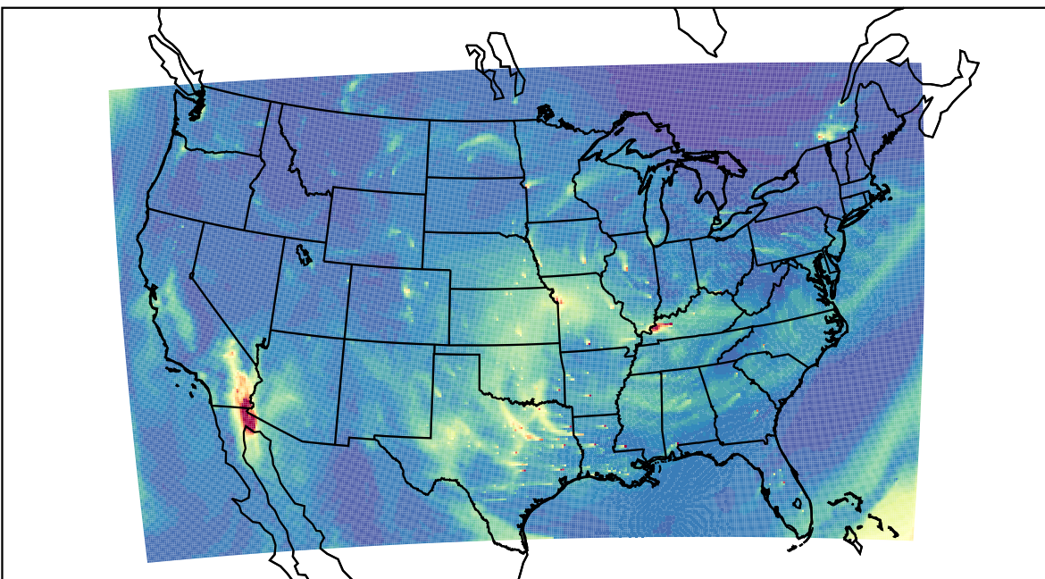
WRF 2023-12-13_19:00:00
