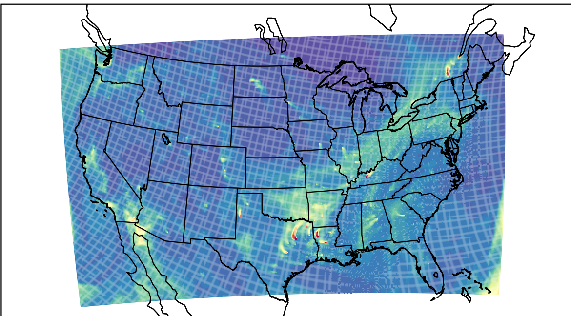
WRF 2023-12-12_17:00:00
