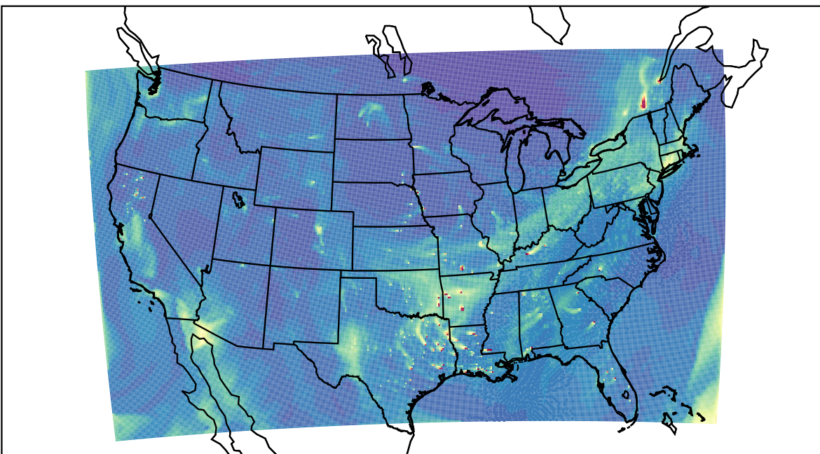
WRF 2023-12-12_21:00:00
