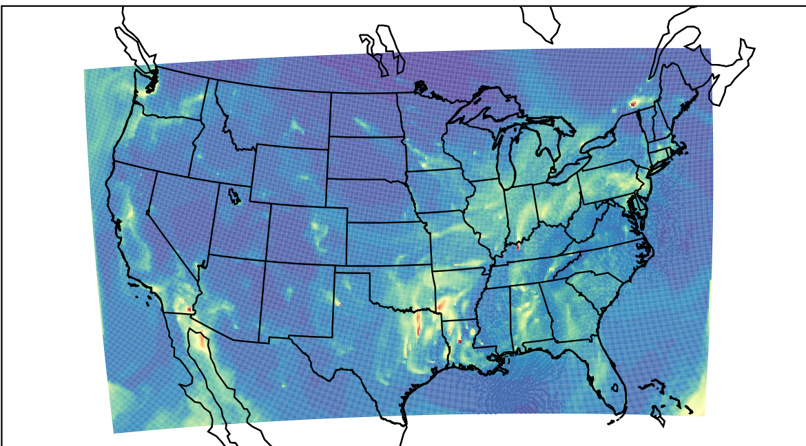
WRF 2023-12-12_11:00:00
