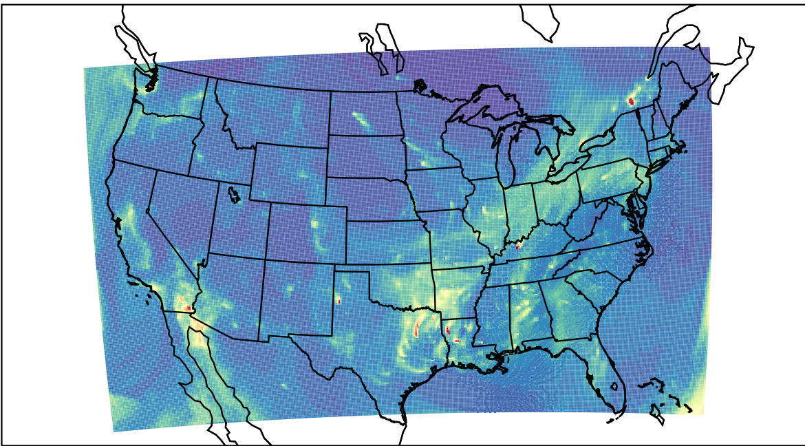
WRF 2023-12-12_15:00:00
