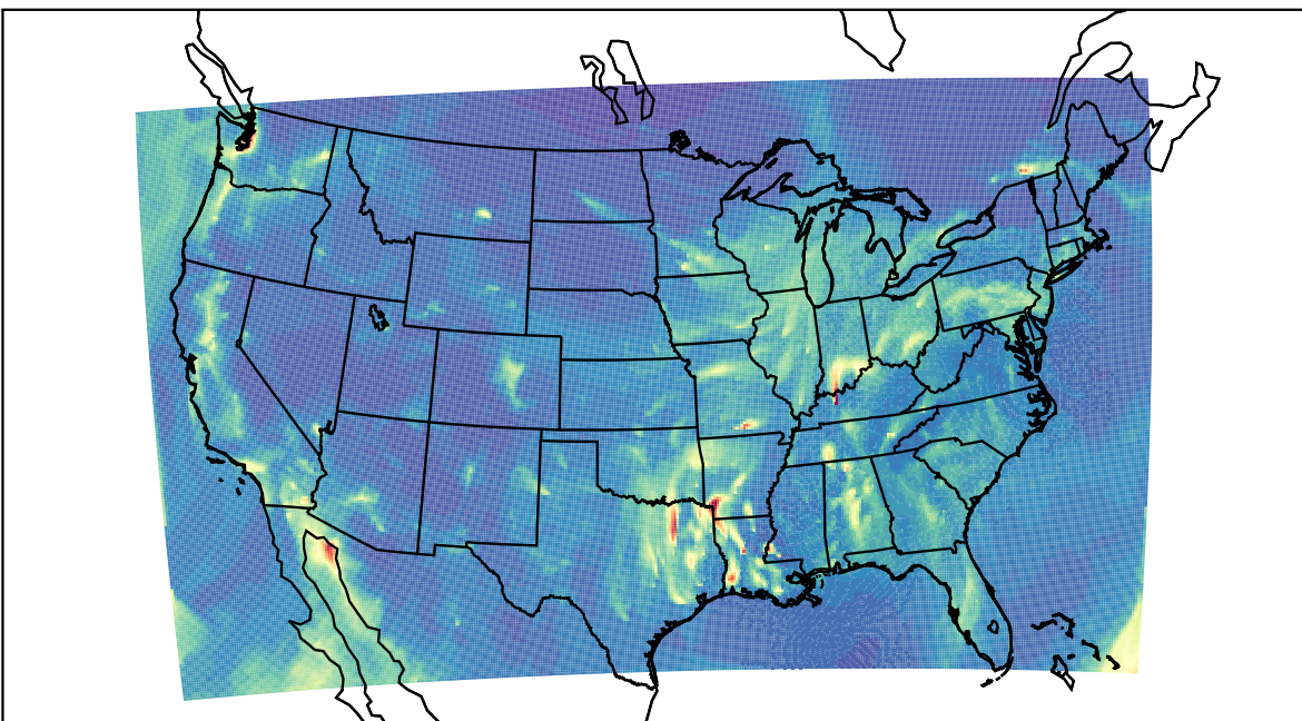
WRF 2023-12-12_07:00:00
