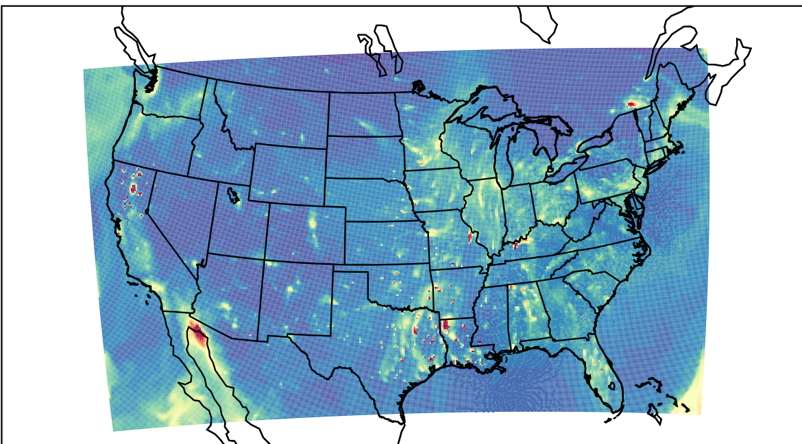
WRF 2023-12-12_01:00:00
