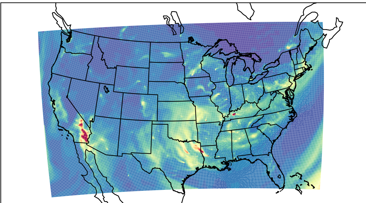
WRF 2023-12-13_12:00:00
