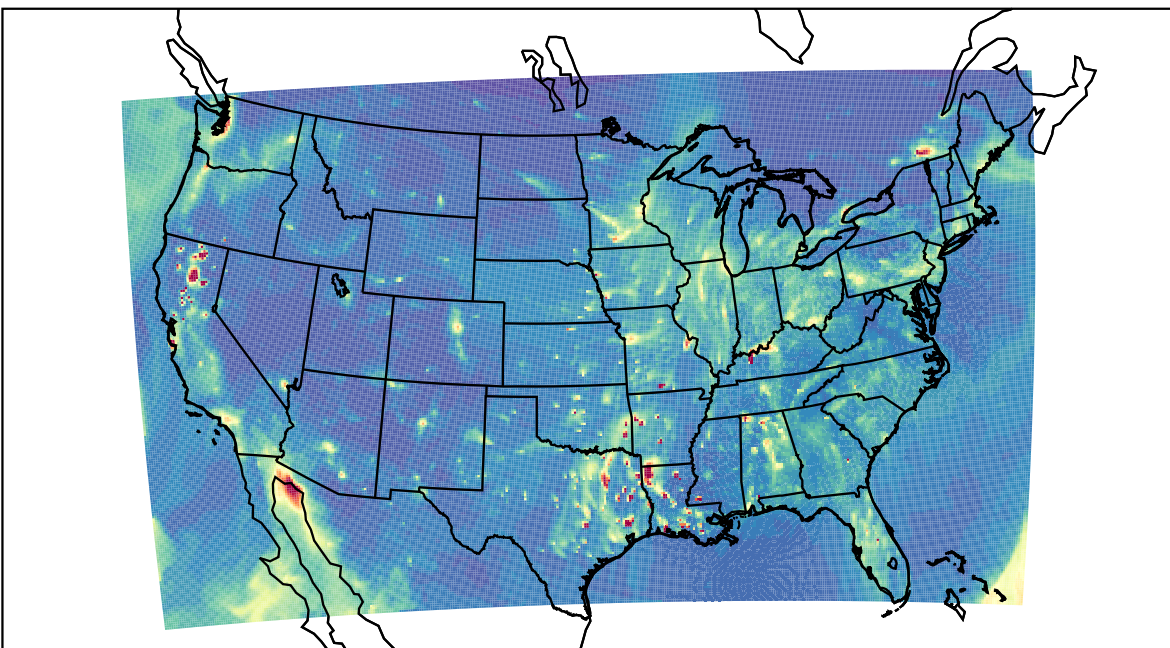
WRF 2023-12-12_02:00:00
