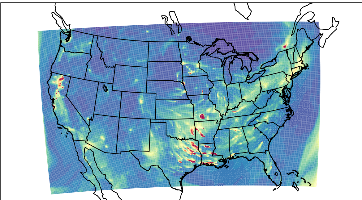
WRF 2023-12-13_02:00:00
