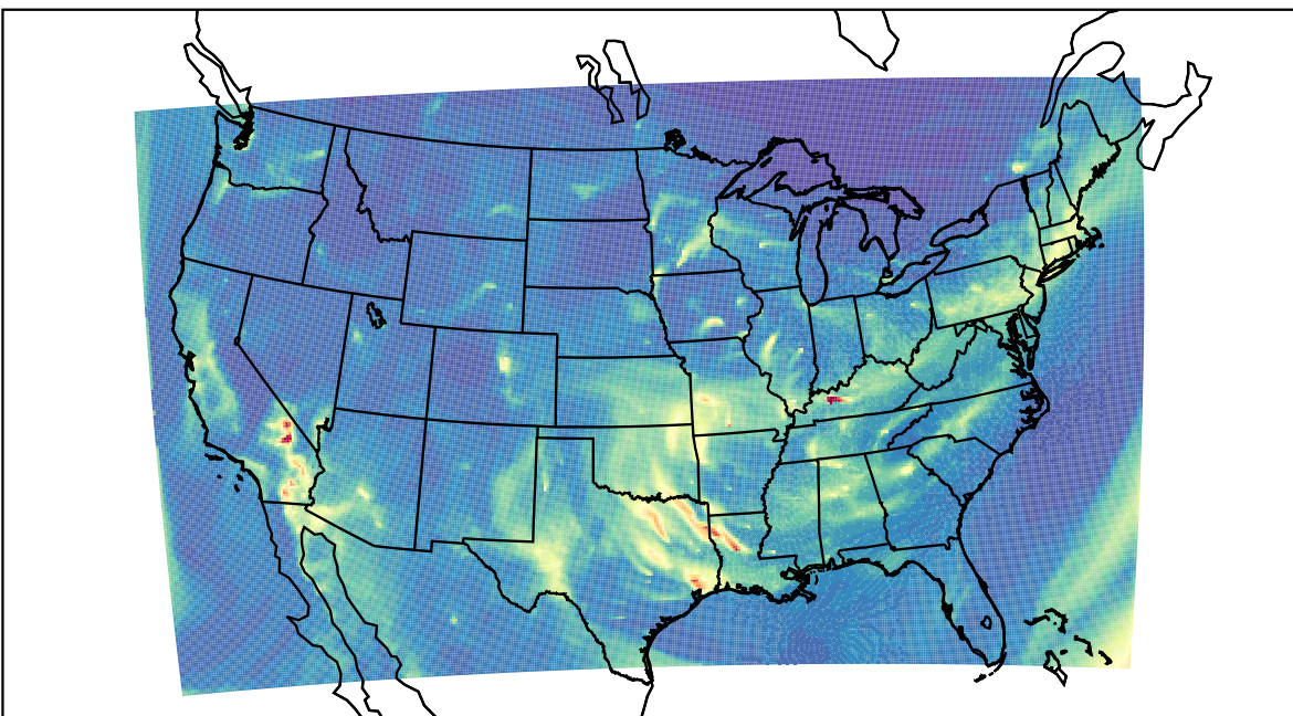
WRF 2023-12-13_08:00:00
