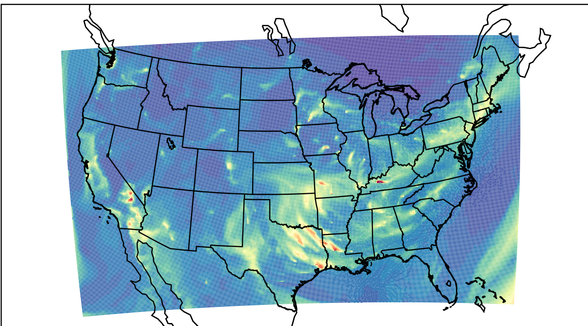
WRF 2023-12-13_07:00:00
