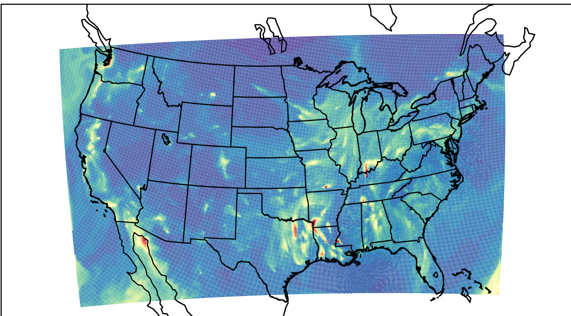
WRF 2023-12-12_06:00:00
