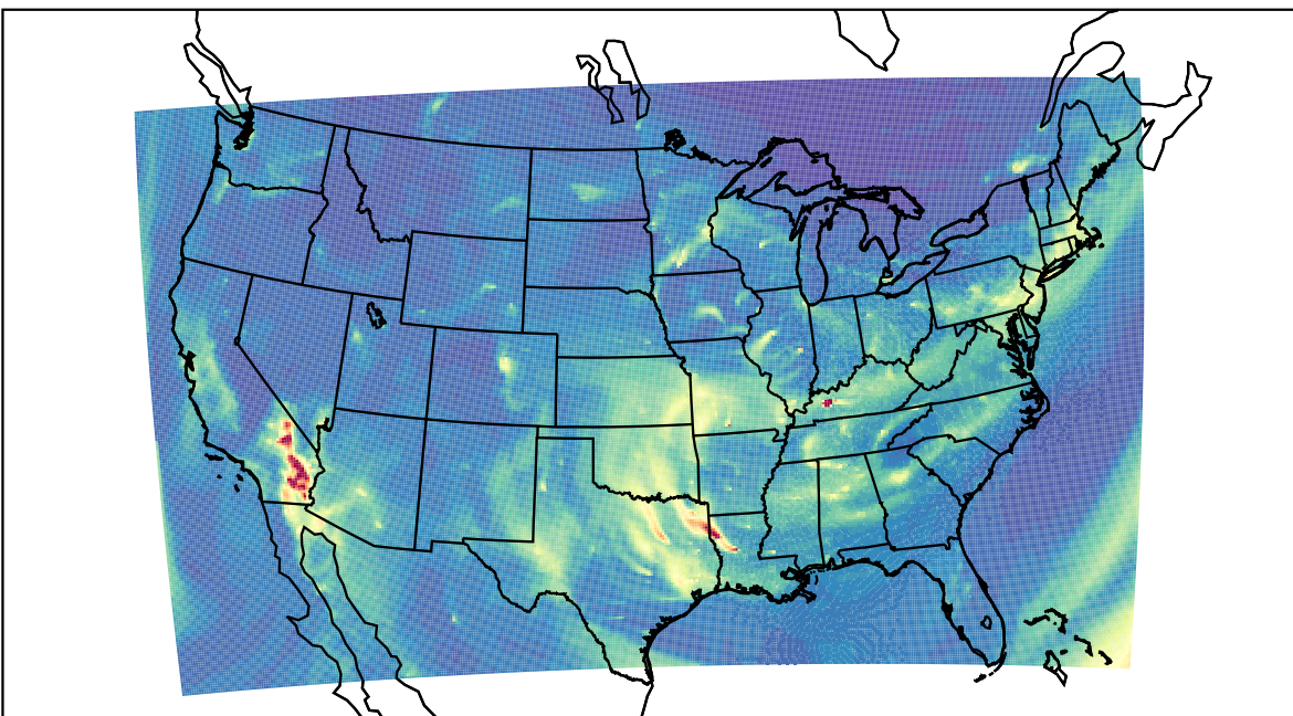
WRF 2023-12-13_11:00:00
