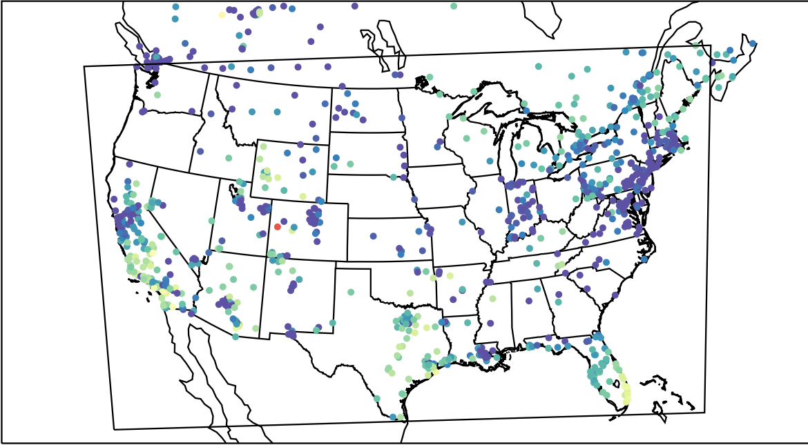
AirNOW (2023-12-13_00:00:00)
