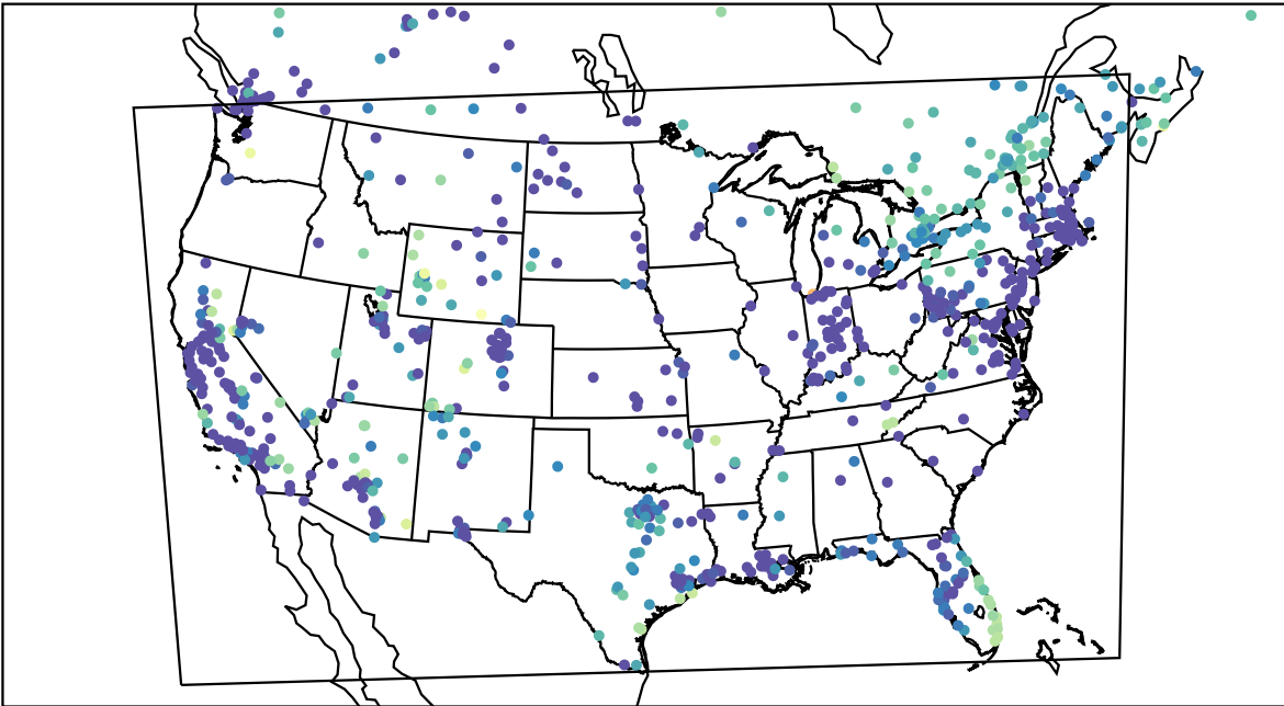
AirNOW (2023-12-13_10:00:00)
