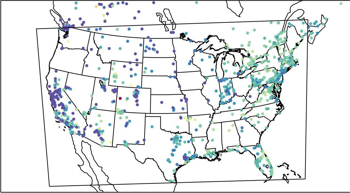
AirNOW (2023-12-13_17:00:00)
