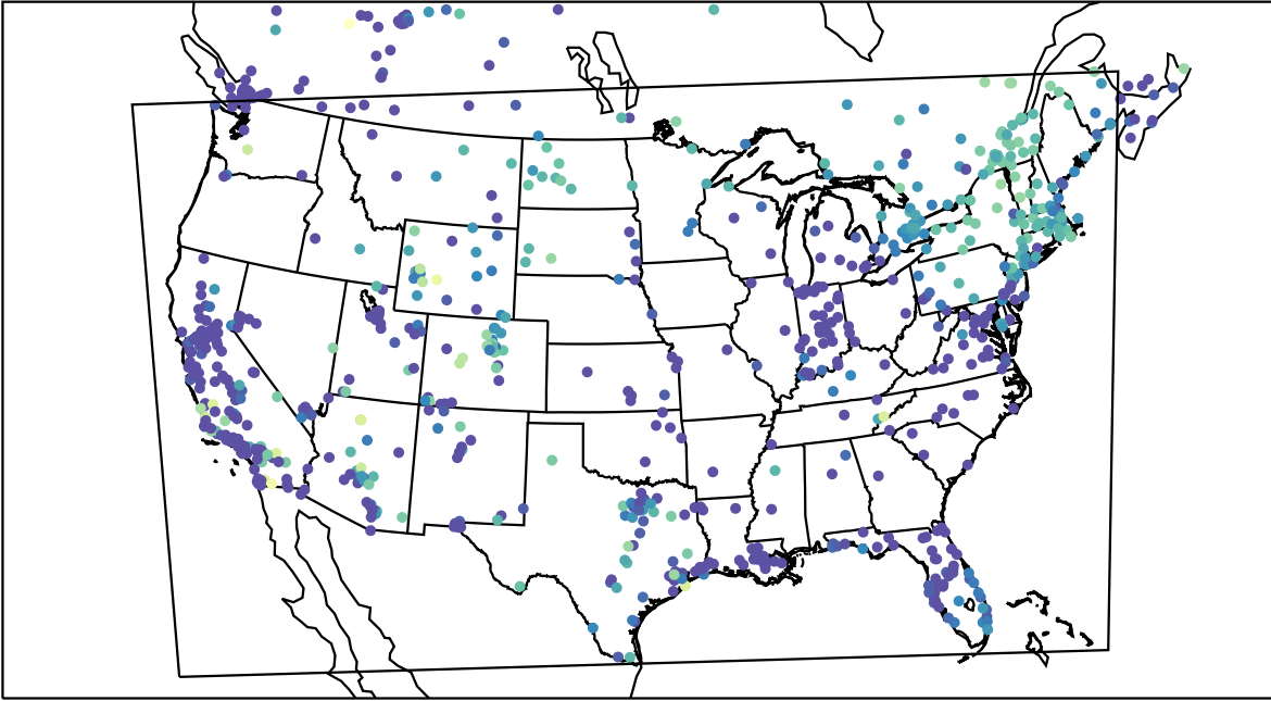
AirNOW (2023-12-12_06:00:00)
