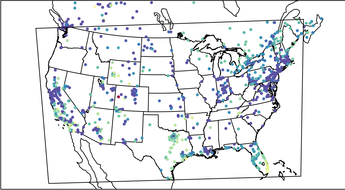
AirNOW (2023-12-13_01:00:00)
