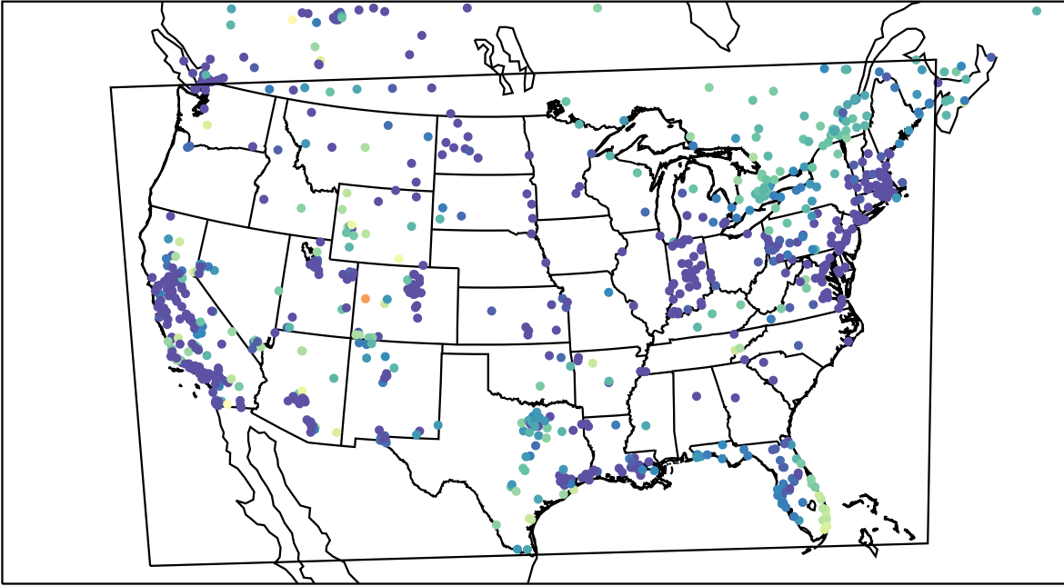
AirNOW (2023-12-13_08:00:00)
