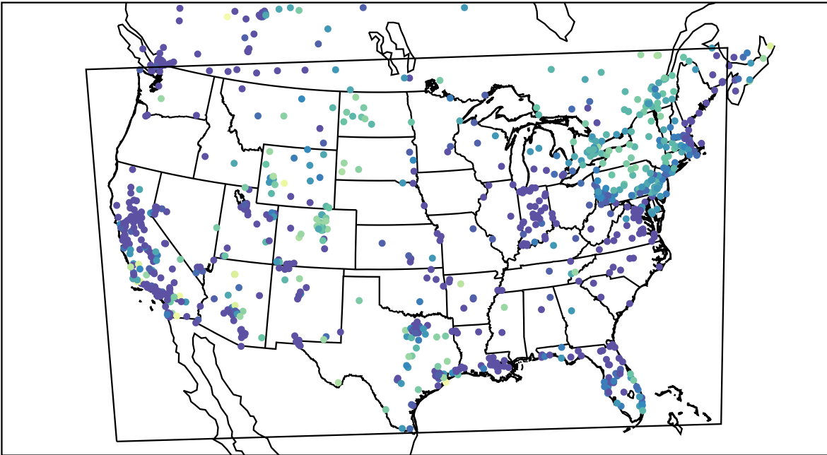
AirNOW (2023-12-12_03:00:00)
