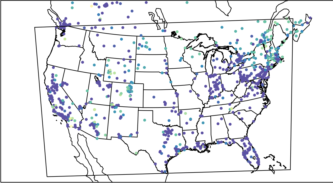
AirNOW (2023-12-12_11:00:00)
