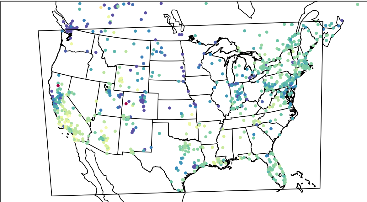
AirNOW (2023-12-13_21:00:00)
