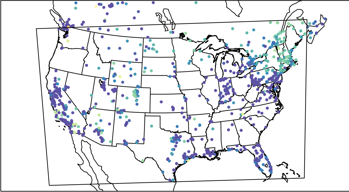
AirNOW (2023-12-12_09:00:00)
