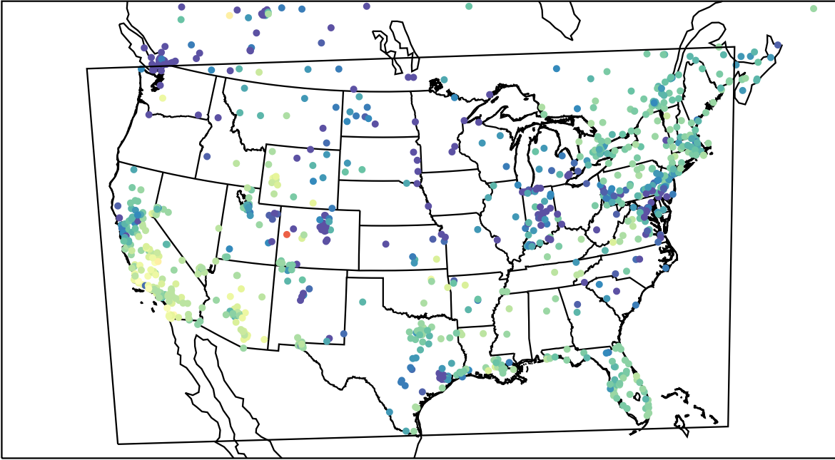
AirNOW (2023-12-13_22:00:00)
