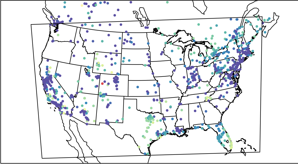
AirNOW (2023-12-13_03:00:00)
