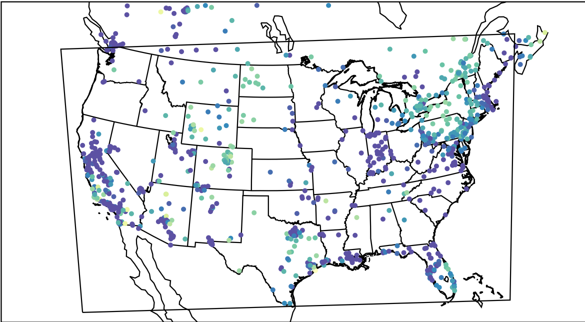
AirNOW (2023-12-12_02:00:00)
