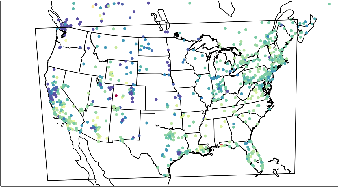
AirNOW (2023-12-13_19:00:00)
