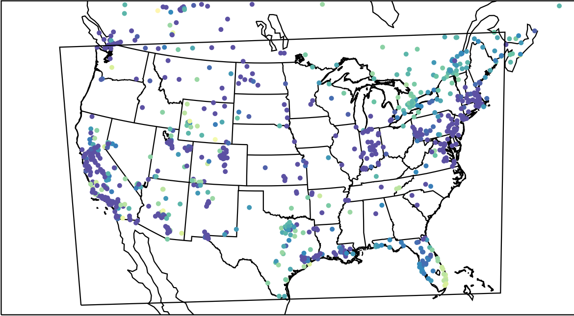
AirNOW (2023-12-13_07:00:00)
