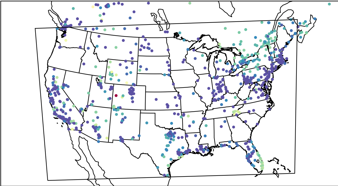
AirNOW (2023-12-13_11:00:00)
