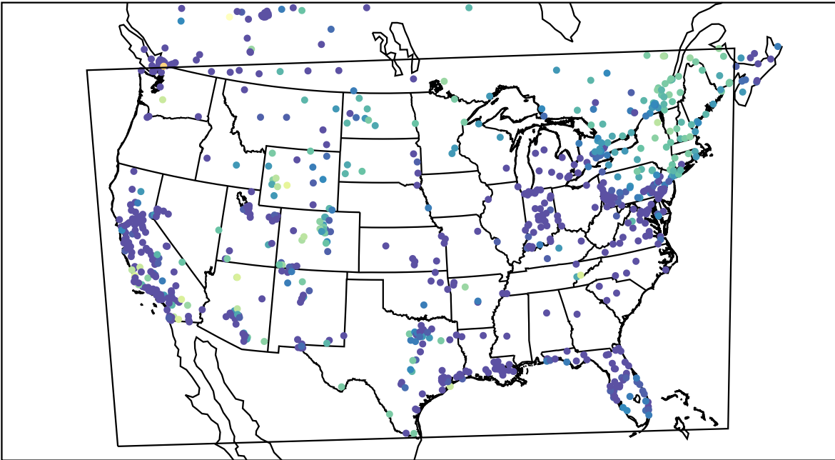
AirNOW (2023-12-12_08:00:00)
