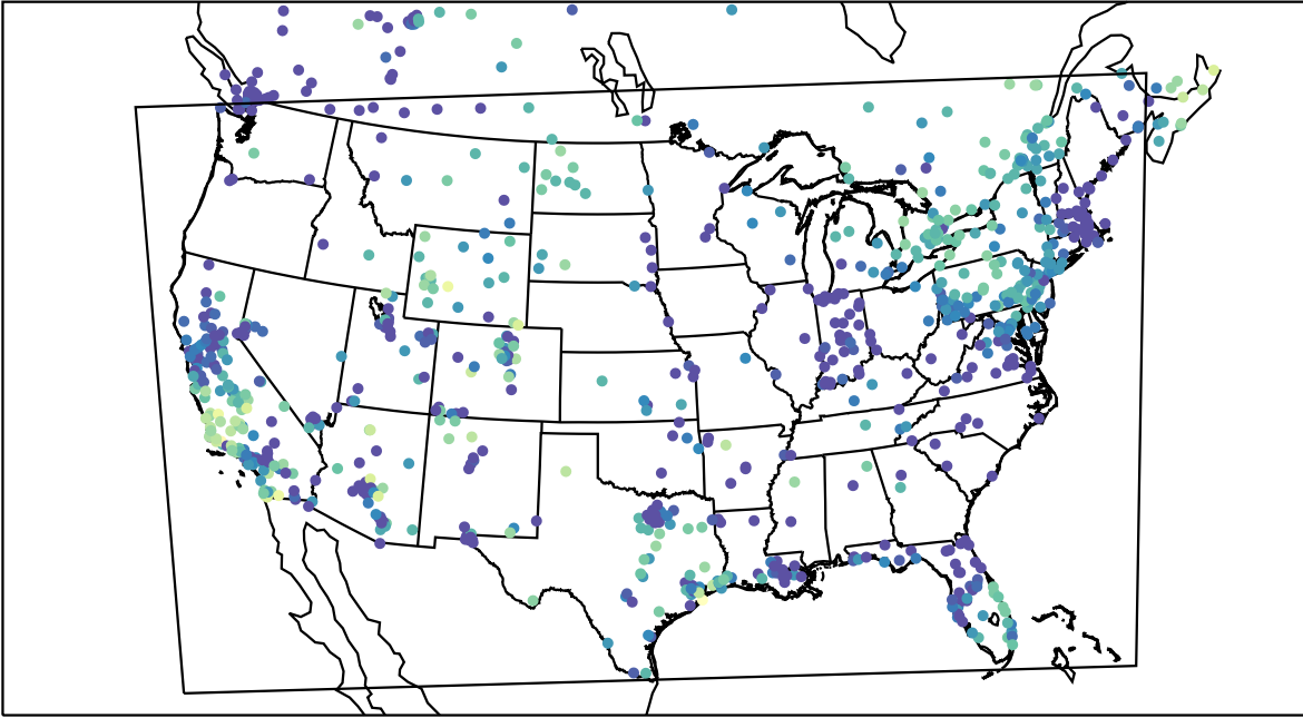
AirNOW (2023-12-12_00:00:00)
