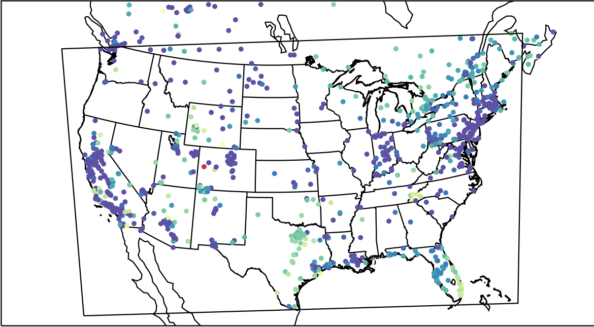
AirNOW (2023-12-13_04:00:00)
