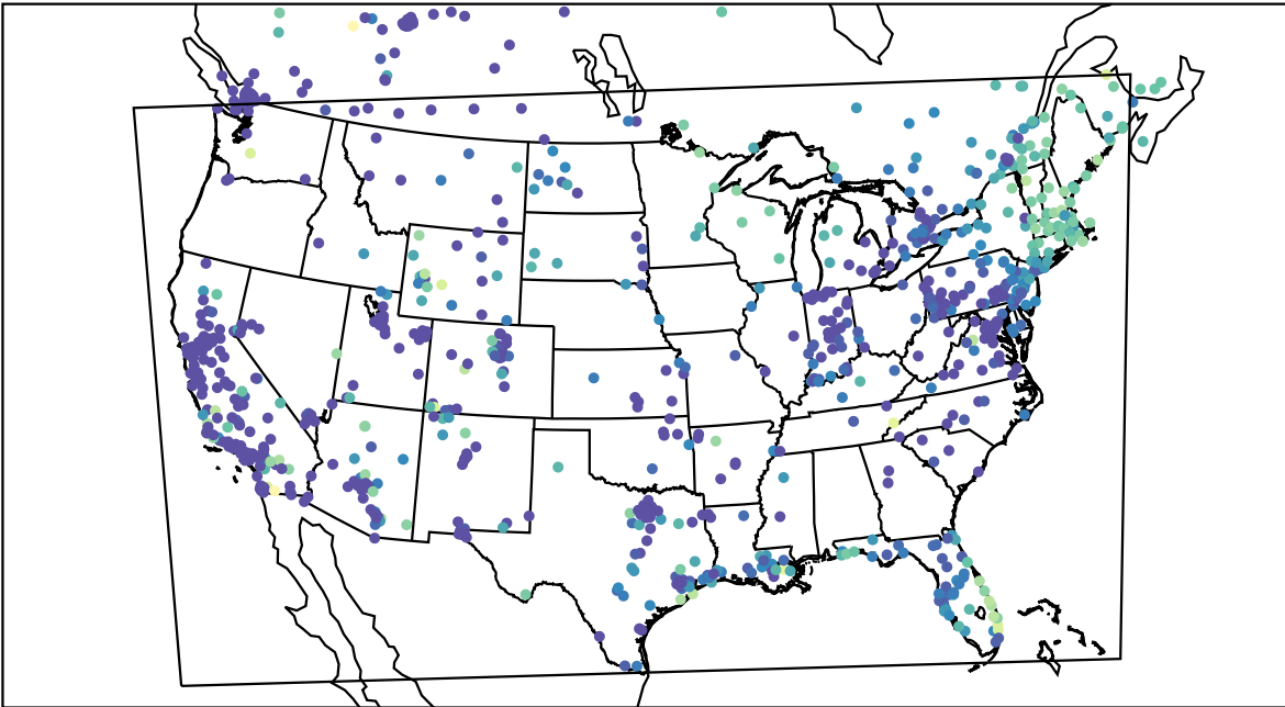
AirNOW (2023-12-12_15:00:00)
