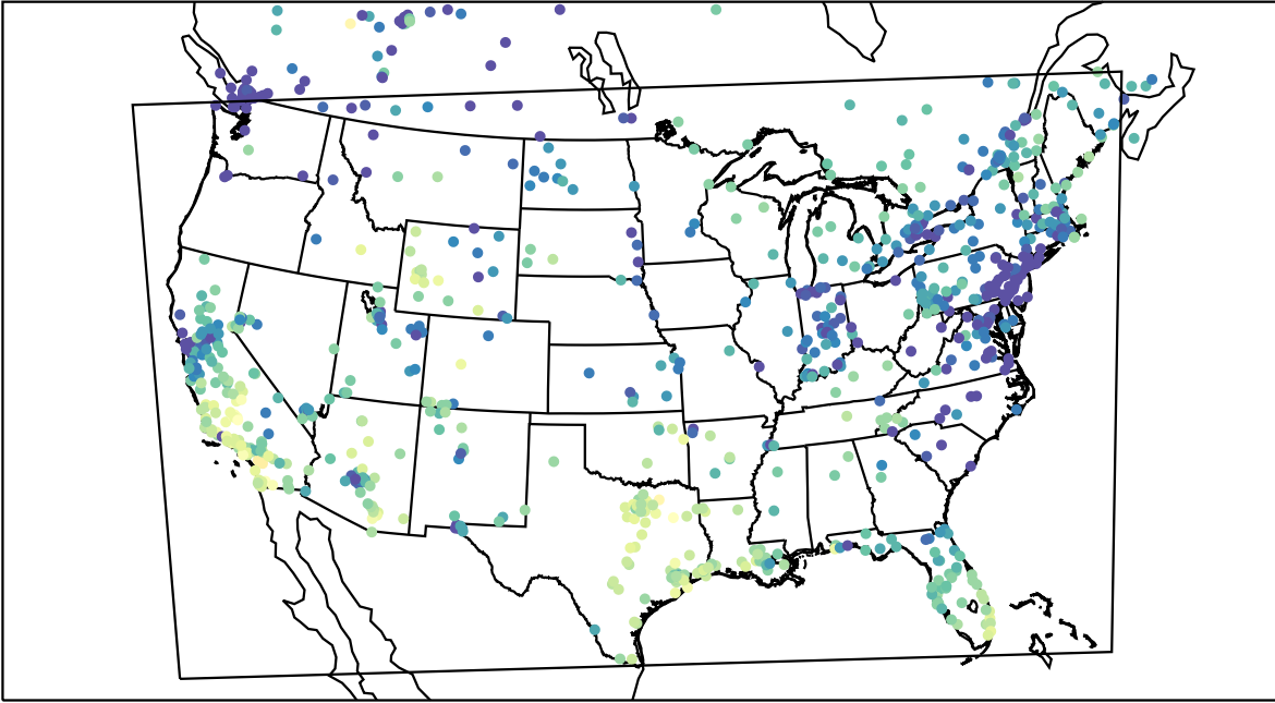
AirNOW (2023-12-12_22:00:00)
