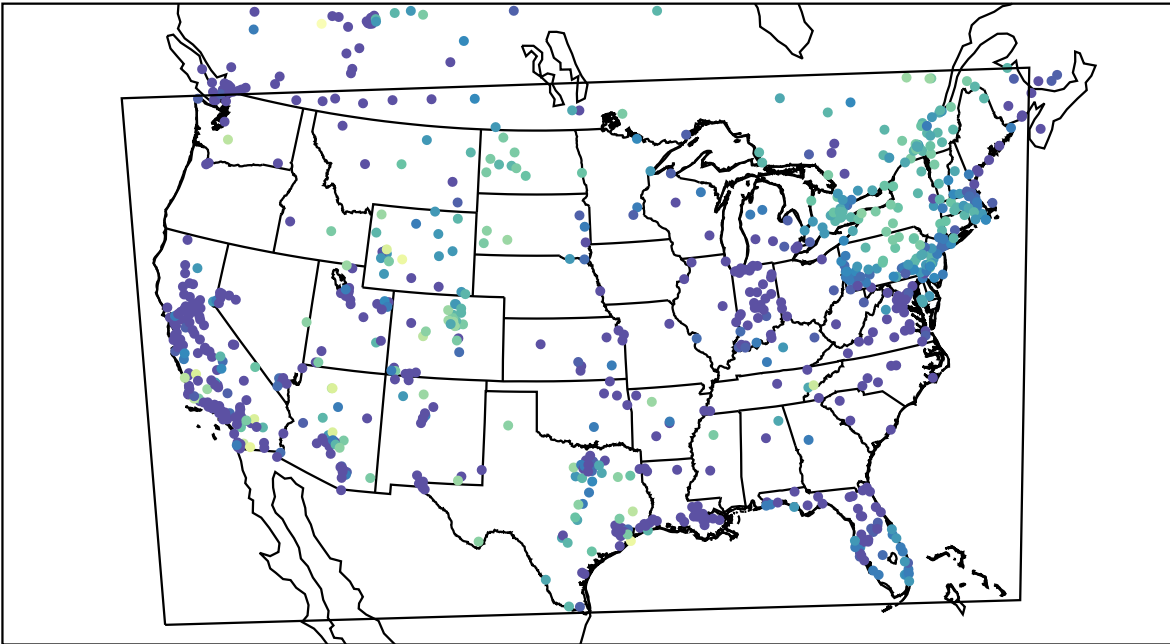
AirNOW (2023-12-12_04:00:00)
