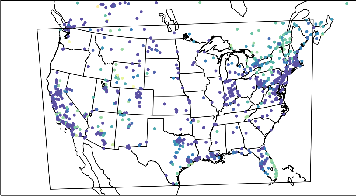
AirNOW (2023-12-13_13:00:00)
