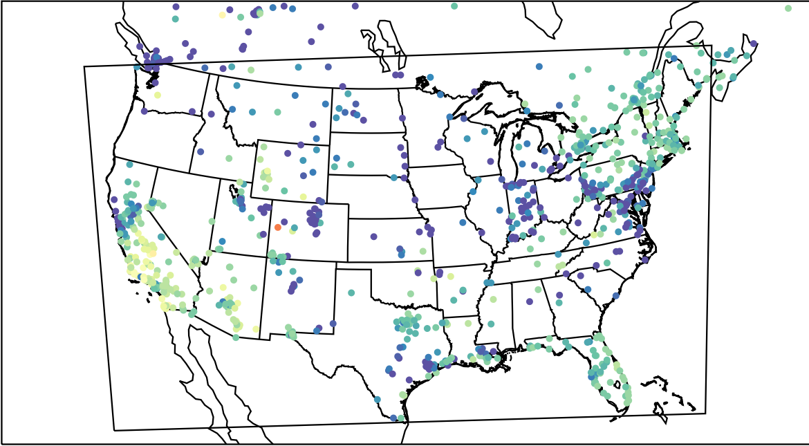
AirNOW (2023-12-13_23:00:00)
