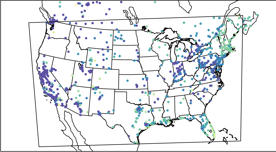
AirNOW (2023-12-12_16:00:00)
