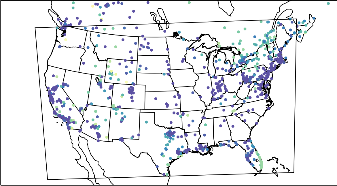
AirNOW (2023-12-13_12:00:00)
