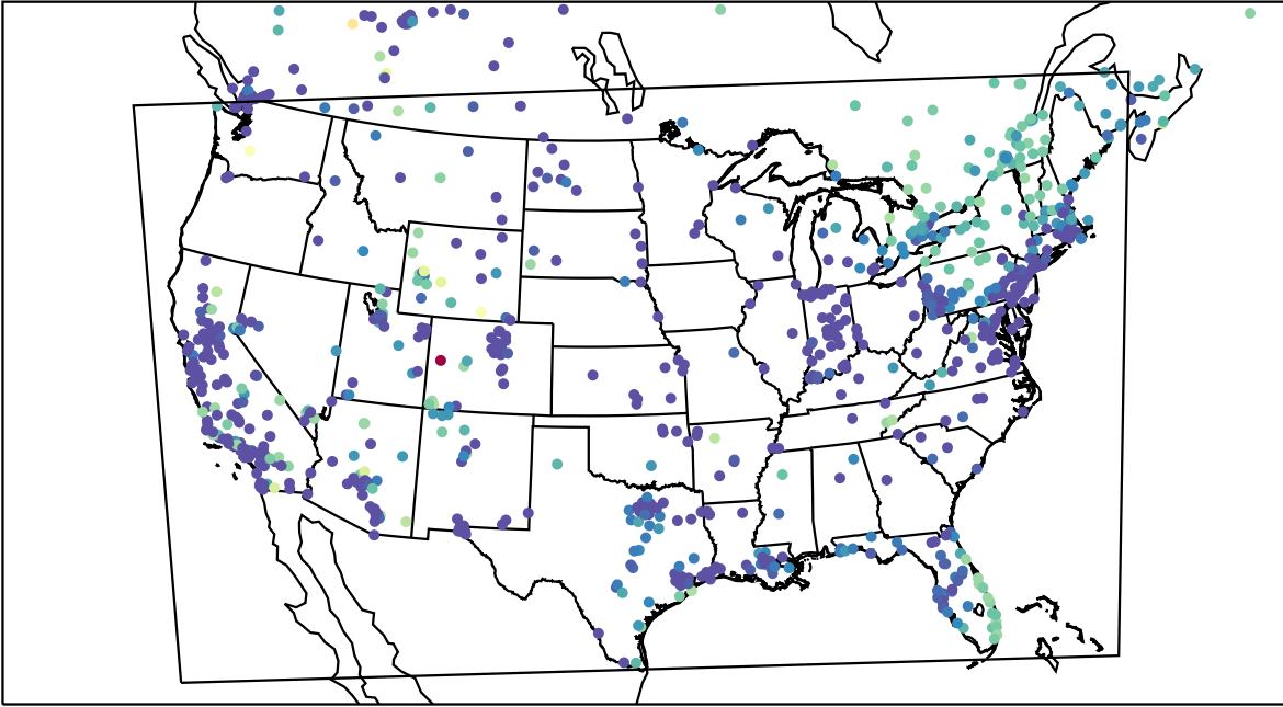
AirNOW (2023-12-13_14:00:00)
