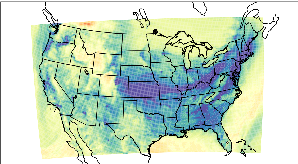
WRF (2023-12-13_03:00:00)
