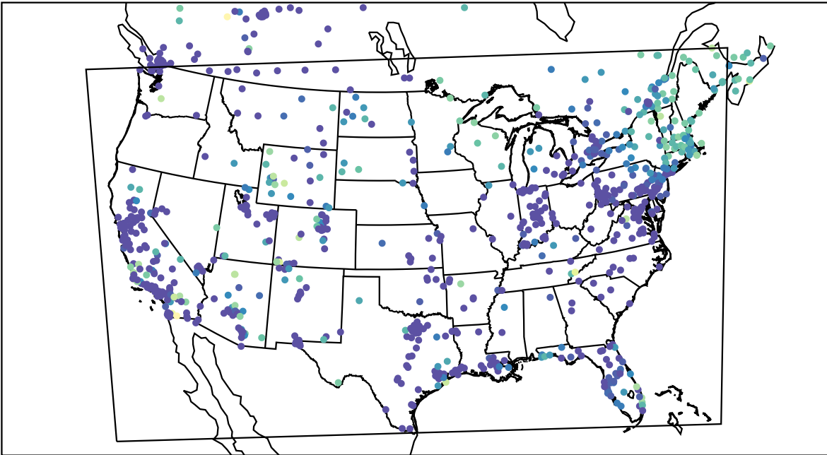
AirNOW (2023-12-12_14:00:00)
