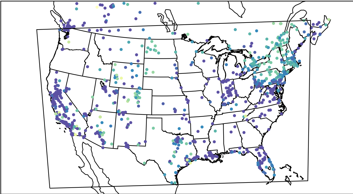
AirNOW (2023-12-12_05:00:00)
