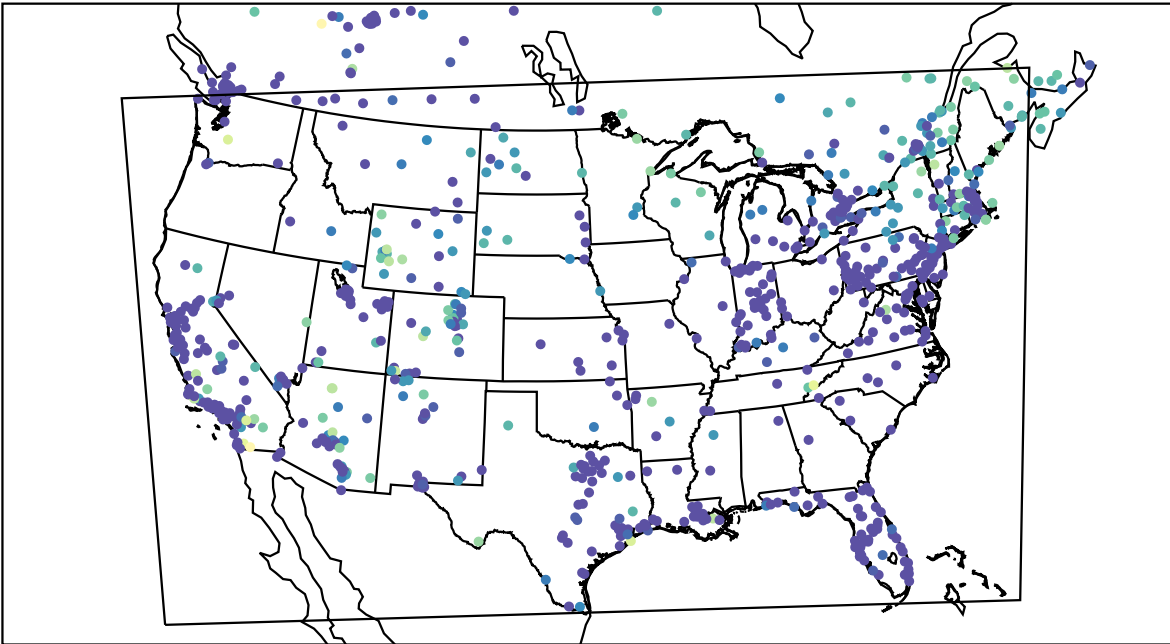
AirNOW (2023-12-12_12:00:00)
