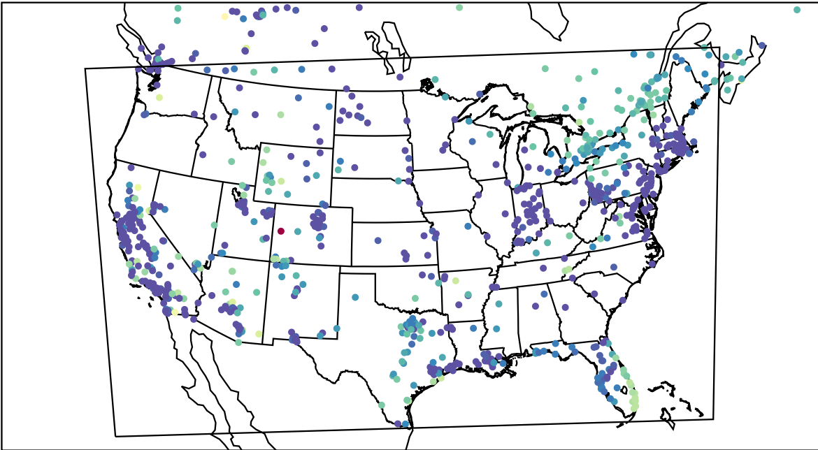
AirNOW (2023-12-13_09:00:00)
