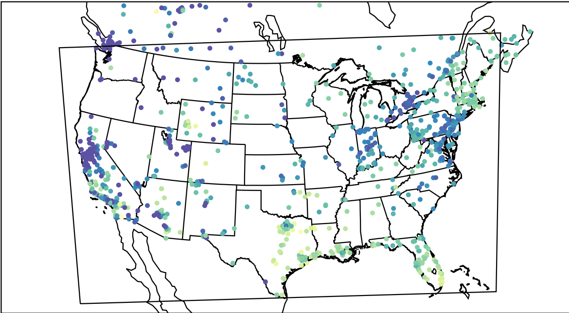
AirNOW (2023-12-12_18:00:00)
