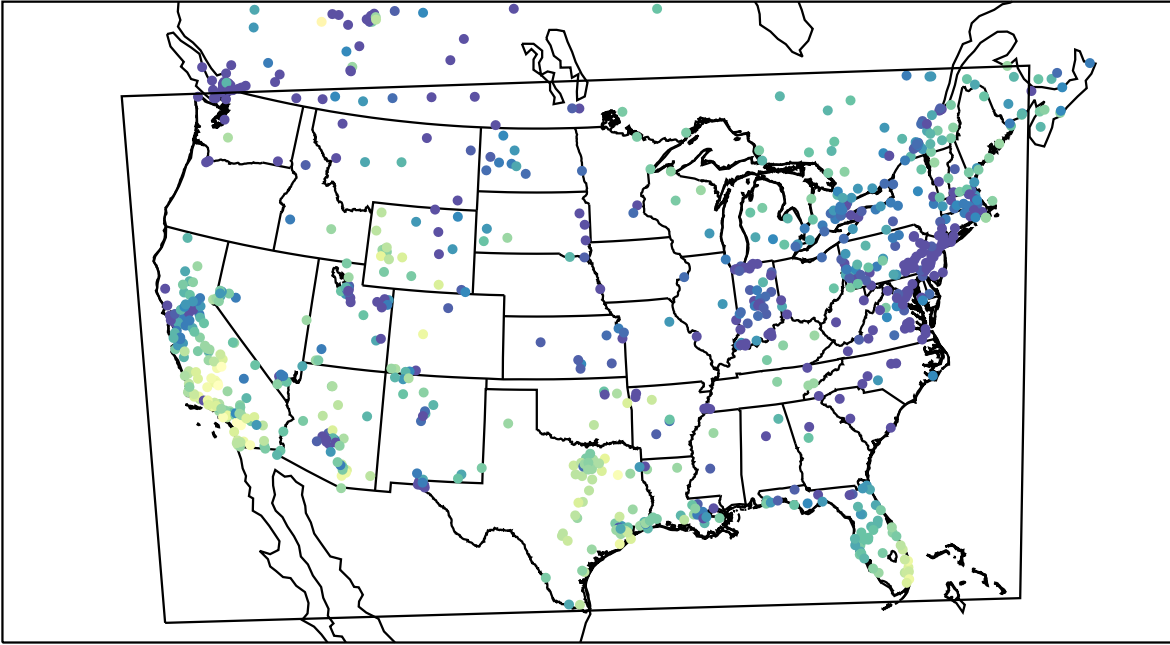
AirNOW (2023-12-12_23:00:00)
