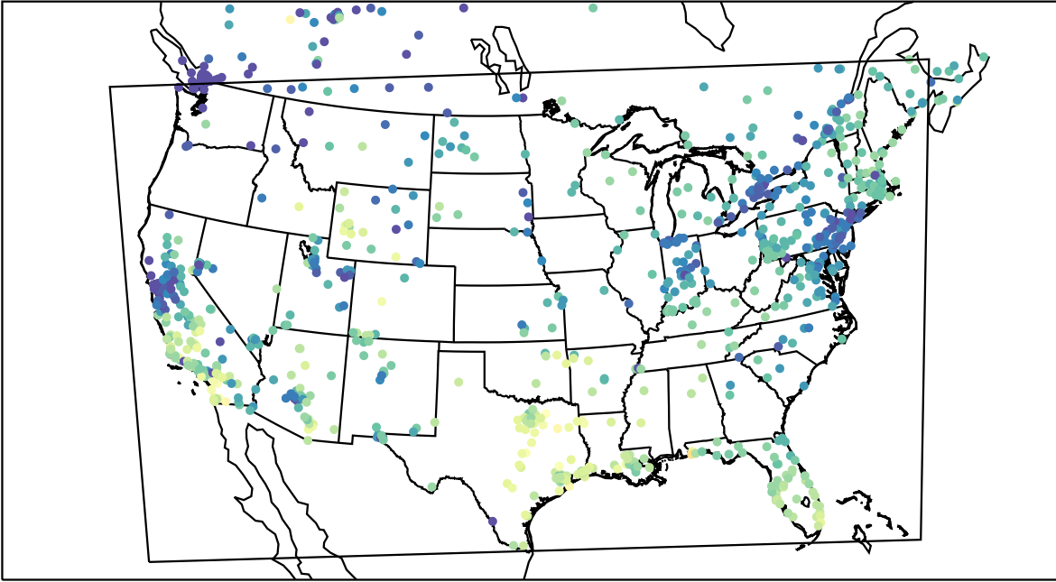
AirNOW (2023-12-12_20:00:00)
