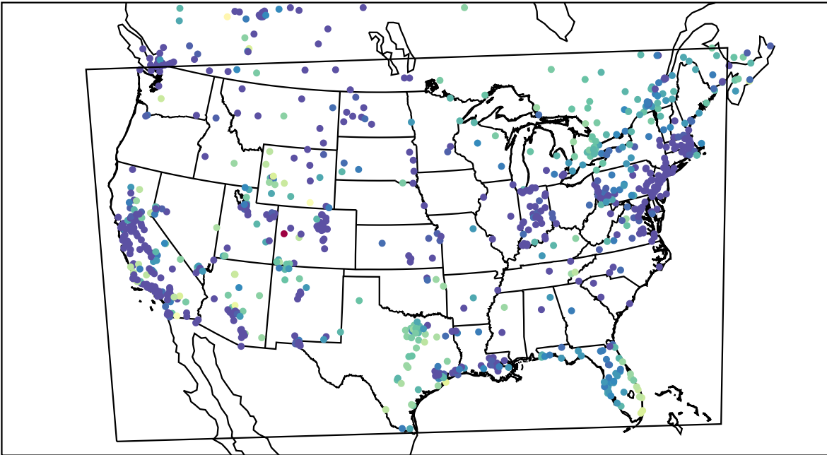
AirNOW (2023-12-13_05:00:00)
