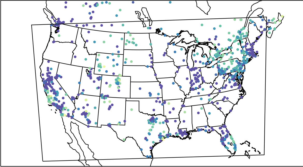
AirNOW (2023-12-12_01:00:00)
