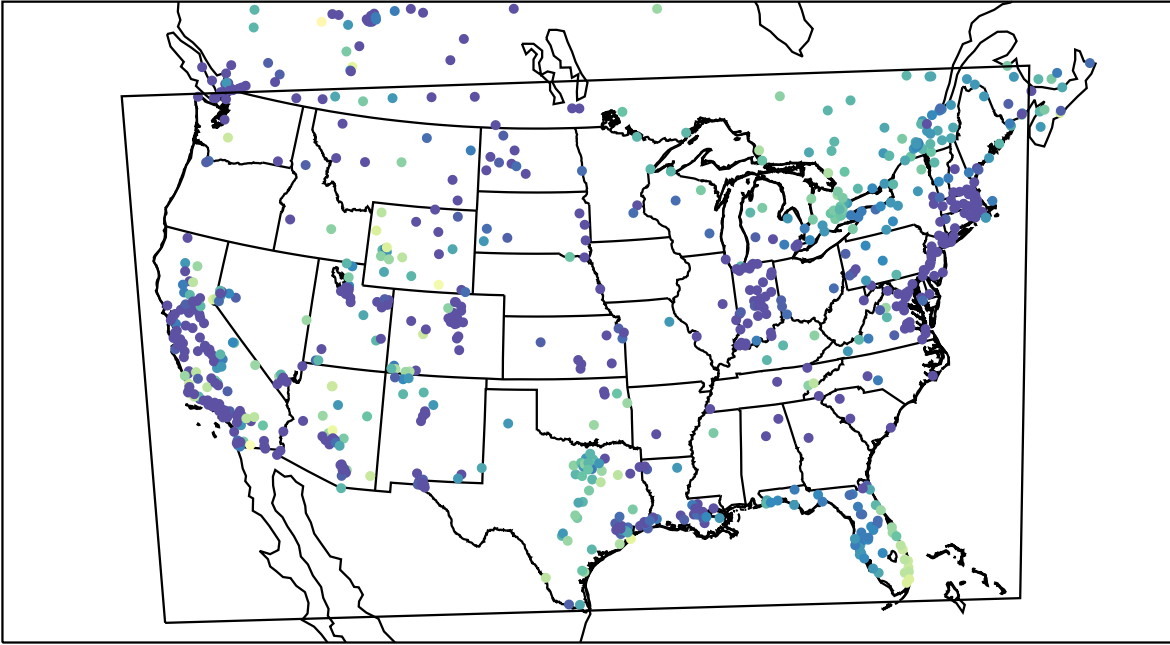
AirNOW (2023-12-13_06:00:00)
