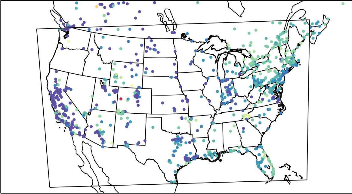
AirNOW (2023-12-13_16:00:00)
