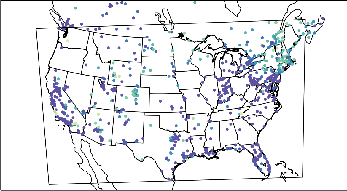
AirNOW (2023-12-12_10:00:00)
