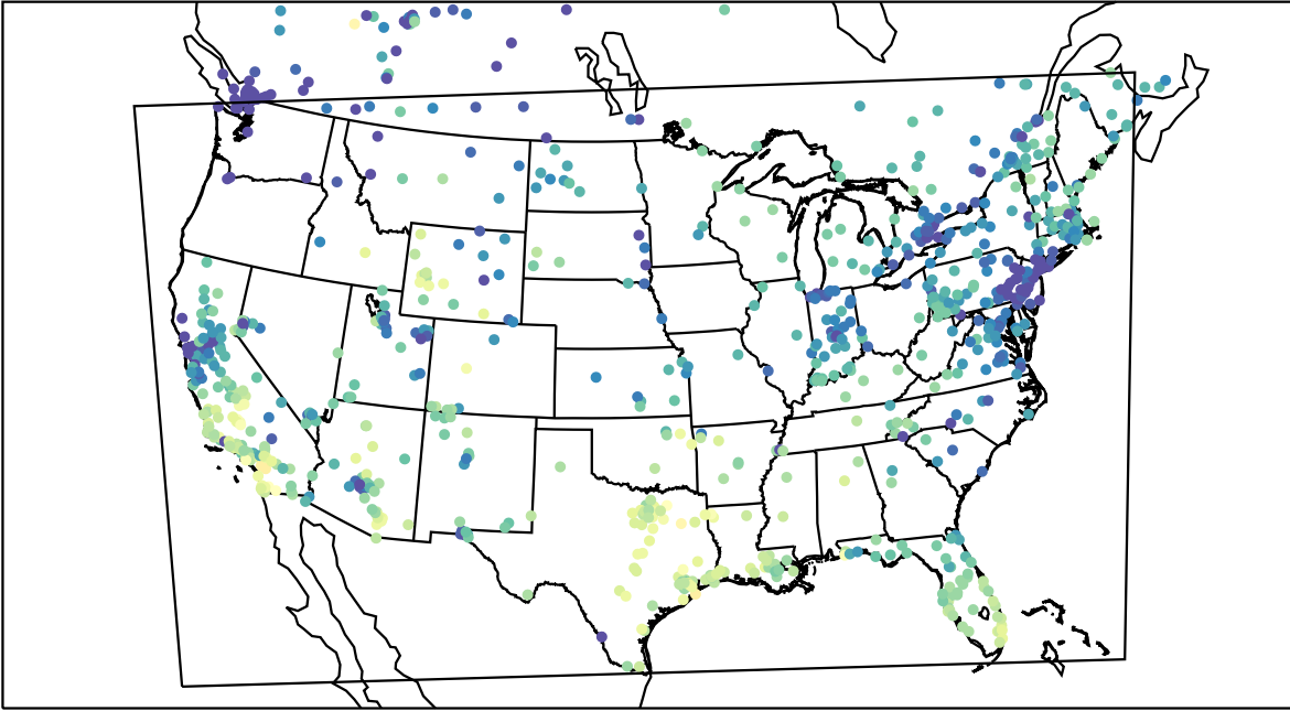
AirNOW (2023-12-12_21:00:00)
