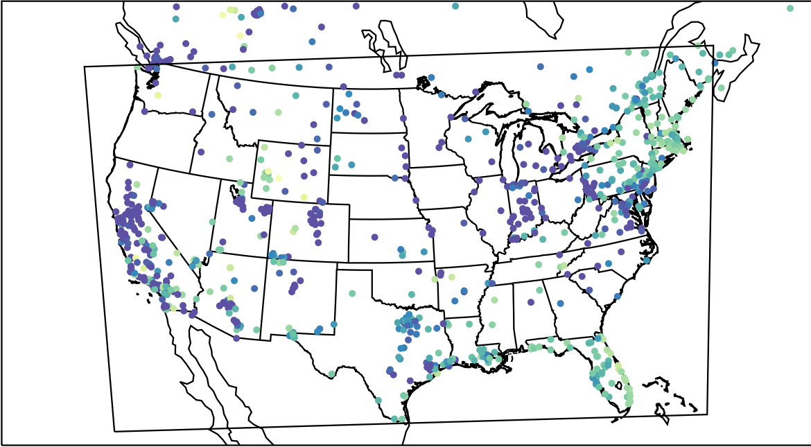
AirNOW (2023-12-14_03:00:00)
