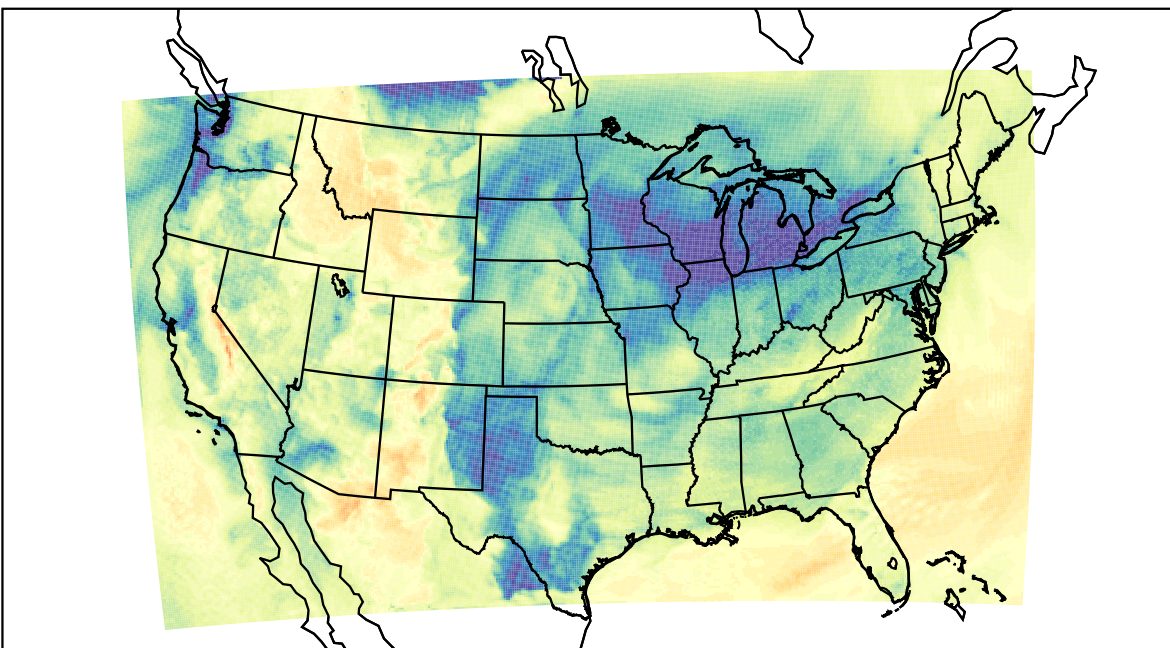
WRF (2023-12-14_20:00:00)
