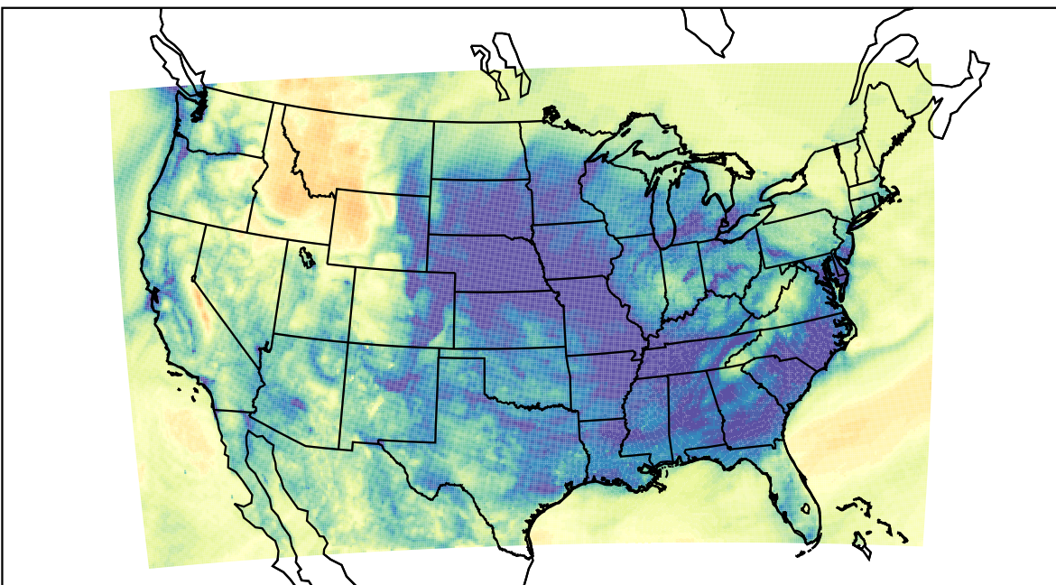
WRF (2023-12-14_05:00:00)
