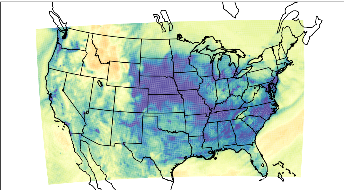
WRF (2023-12-14_02:00:00)
