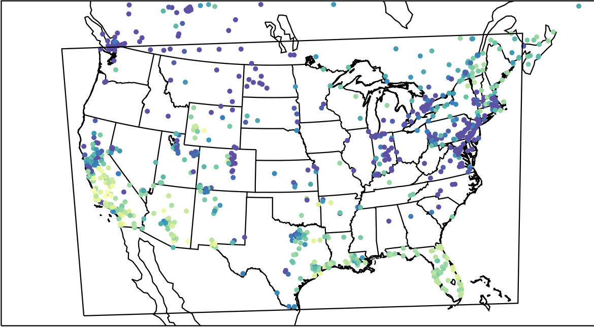
AirNOW (2023-12-14_23:00:00)
