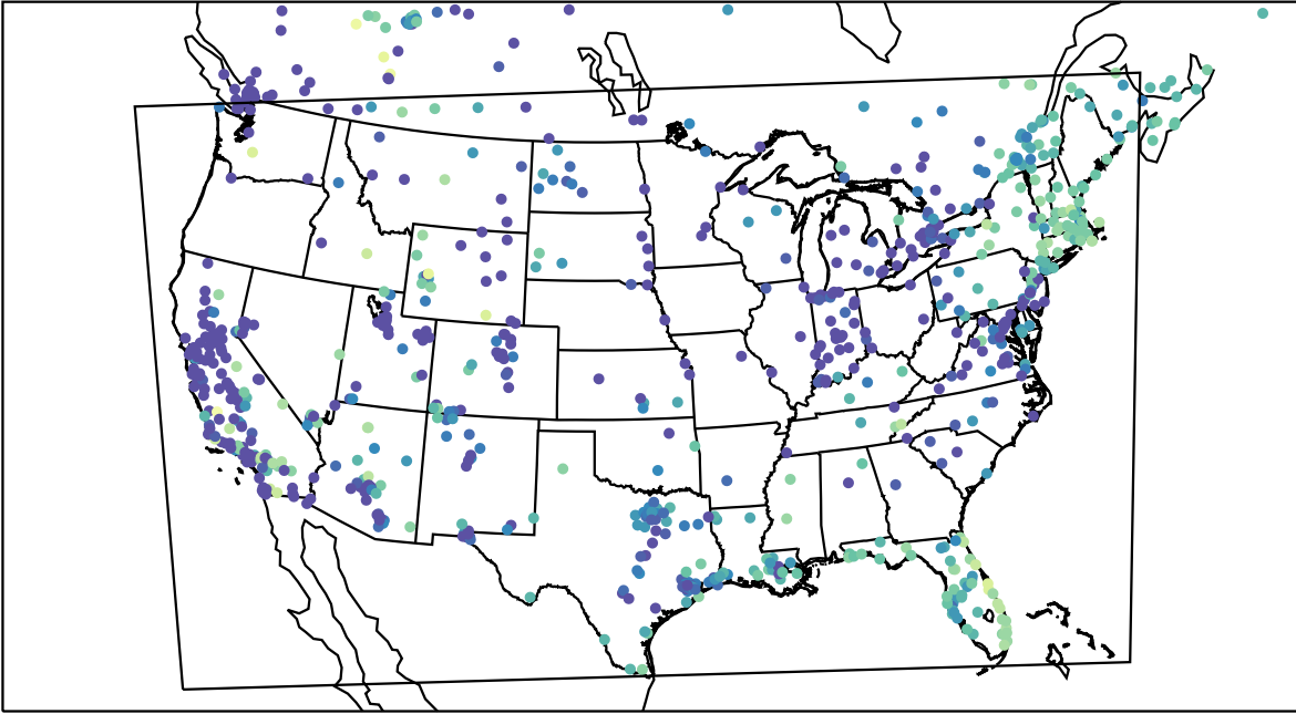
AirNOW (2023-12-14_06:00:00)
