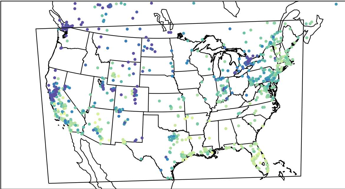
AirNOW (2023-12-14_19:00:00)
