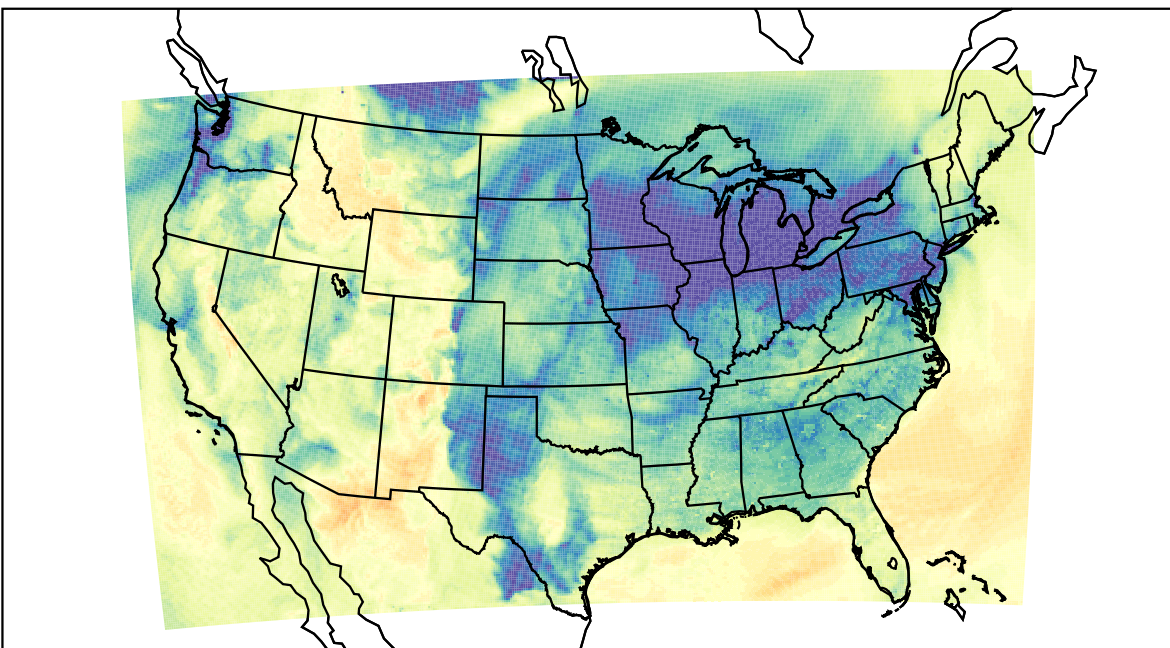
WRF (2023-12-14_22:00:00)
