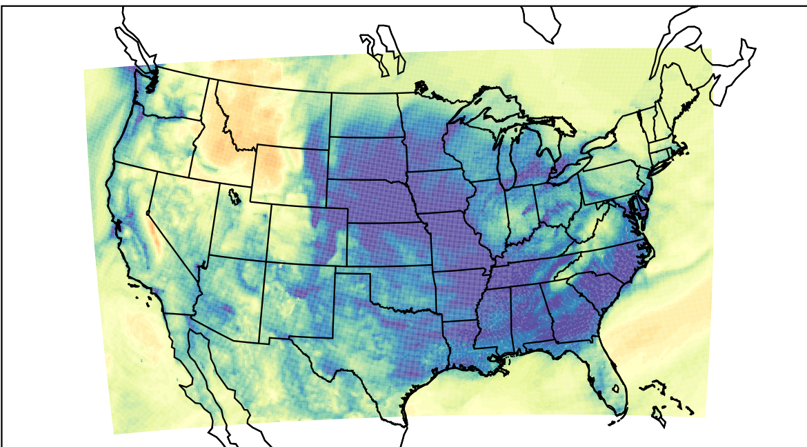
WRF (2023-12-14_06:00:00)
