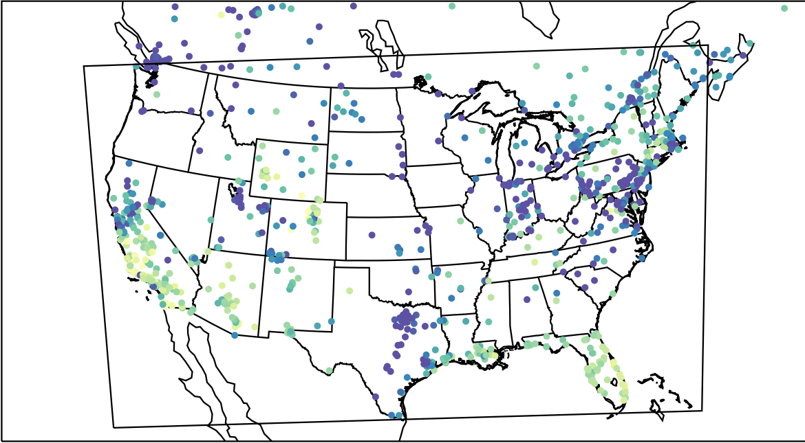
AirNOW (2023-12-15_23:00:00)
