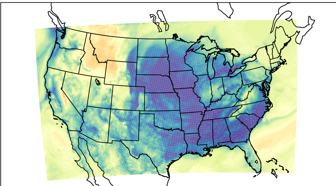
WRF (2023-12-14_08:00:00)
