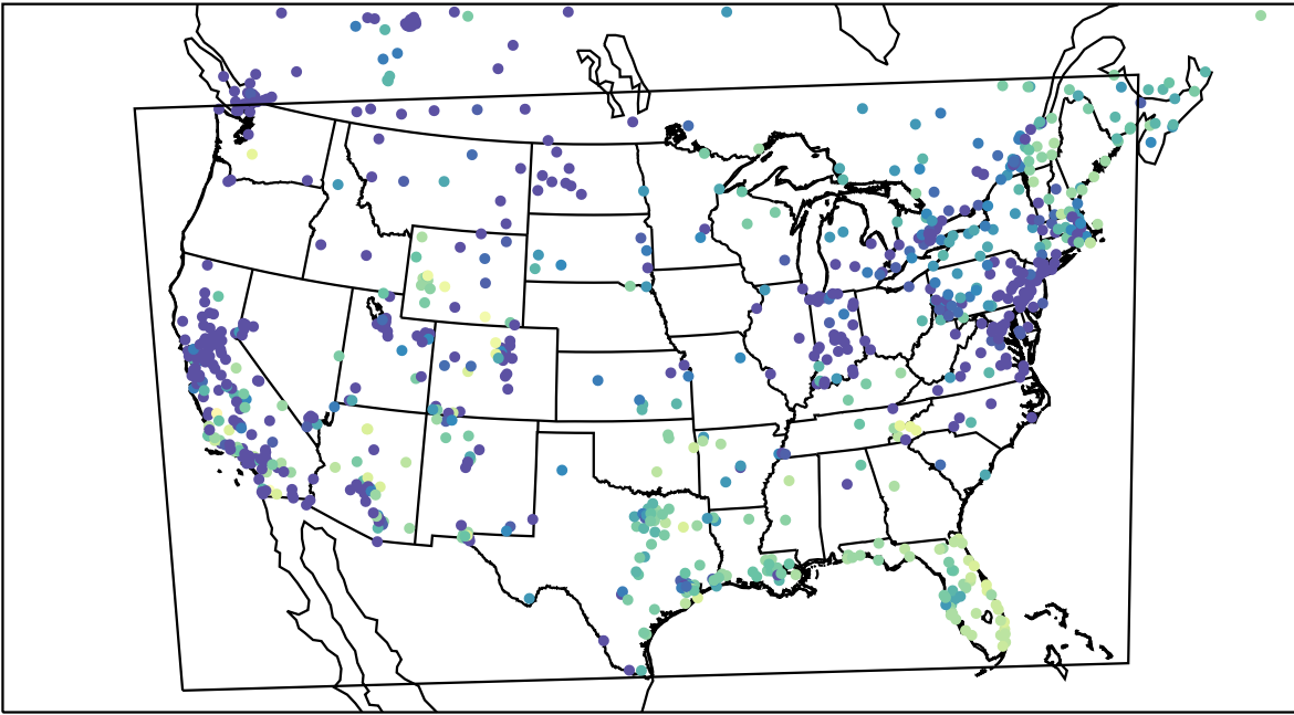
AirNOW (2023-12-15_02:00:00)
