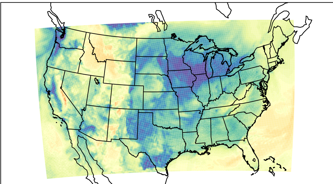
WRF (2023-12-14_18:00:00)
