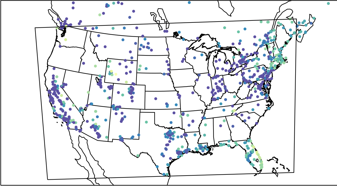
AirNOW (2023-12-14_10:00:00)
