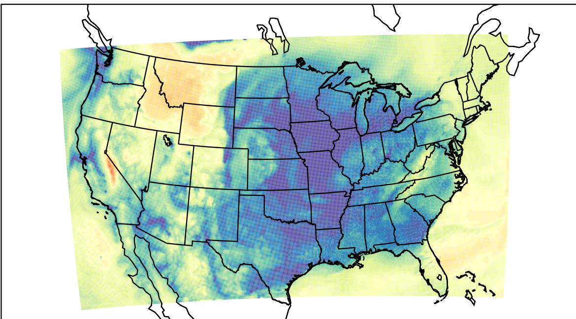
WRF (2023-12-14_15:00:00)
