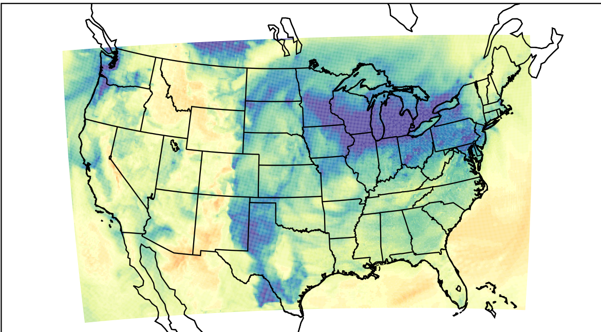
WRF (2023-12-14_21:00:00)
