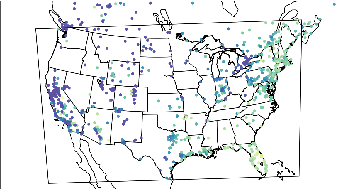
AirNOW (2023-12-14_17:00:00)
