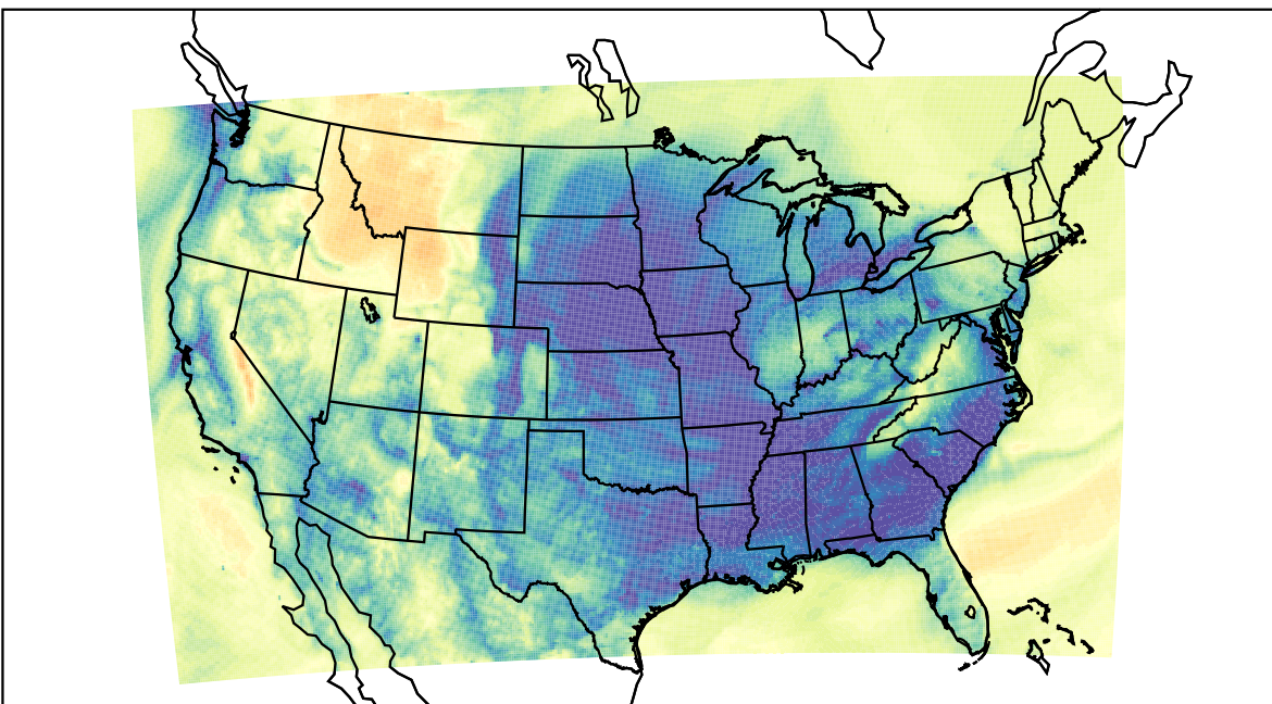
WRF (2023-12-14_09:00:00)
