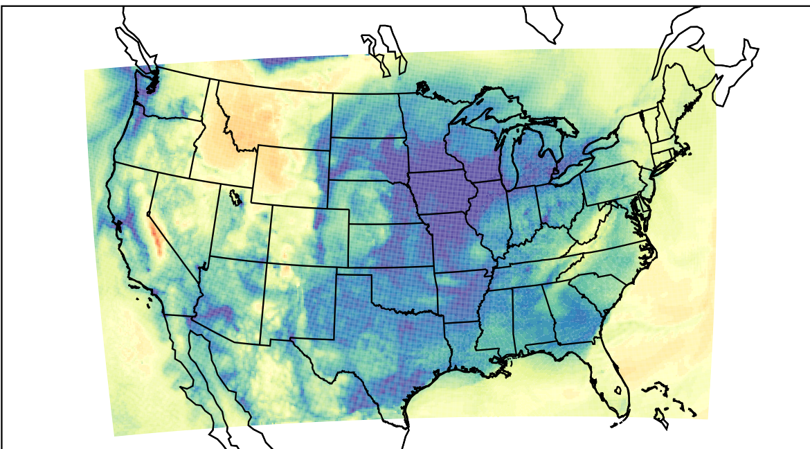
WRF (2023-12-14_16:00:00)
