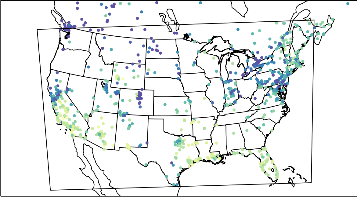
AirNOW (2023-12-14_21:00:00)
