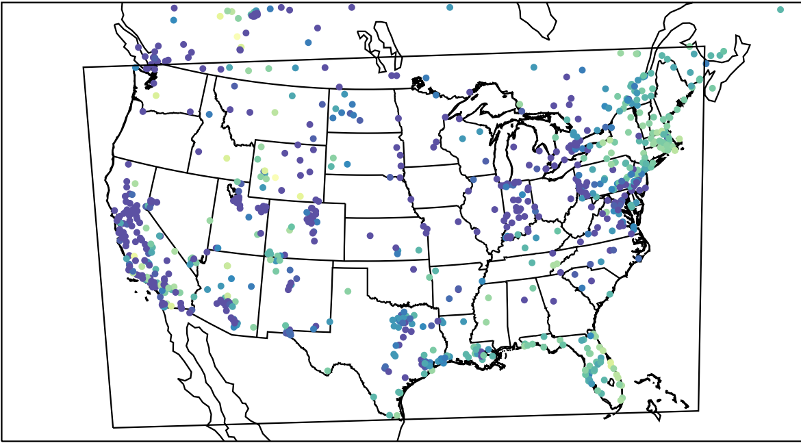
AirNOW (2023-12-14_05:00:00)
