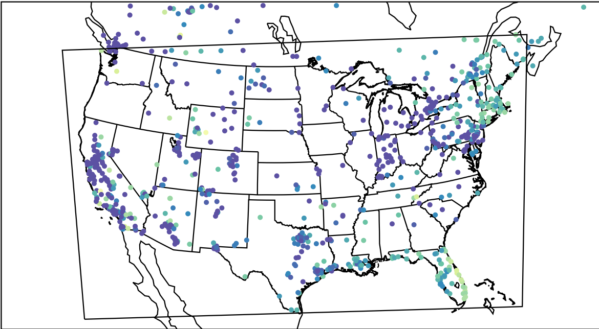
AirNOW (2023-12-14_09:00:00)
