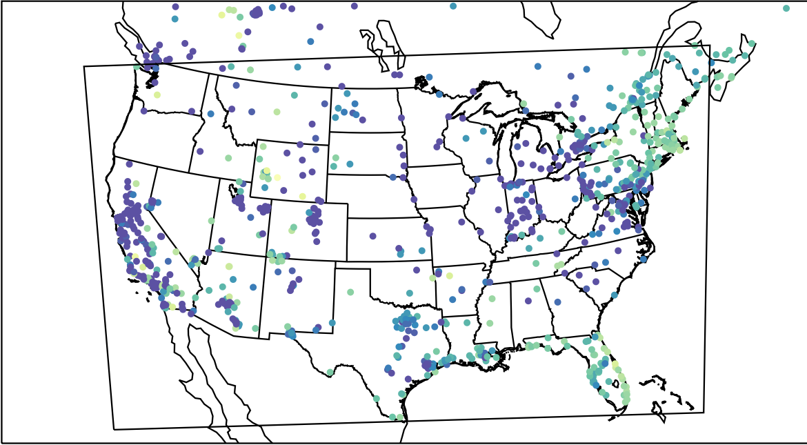
AirNOW (2023-12-14_04:00:00)
