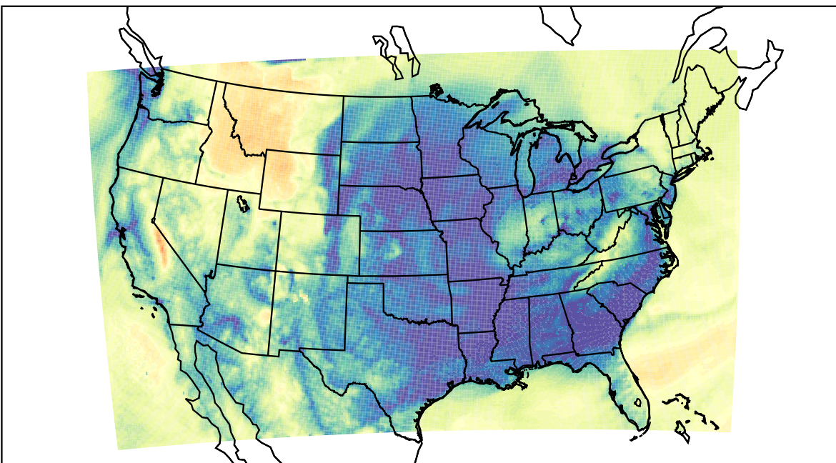
WRF (2023-12-14_12:00:00)
