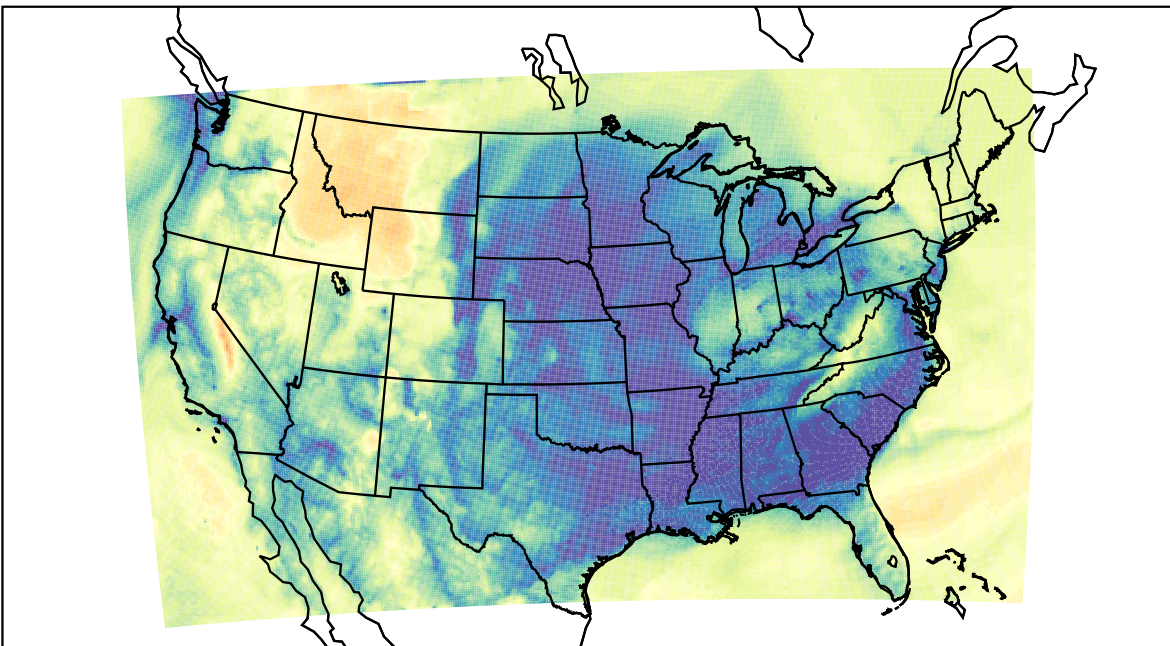
WRF (2023-12-14_11:00:00)
