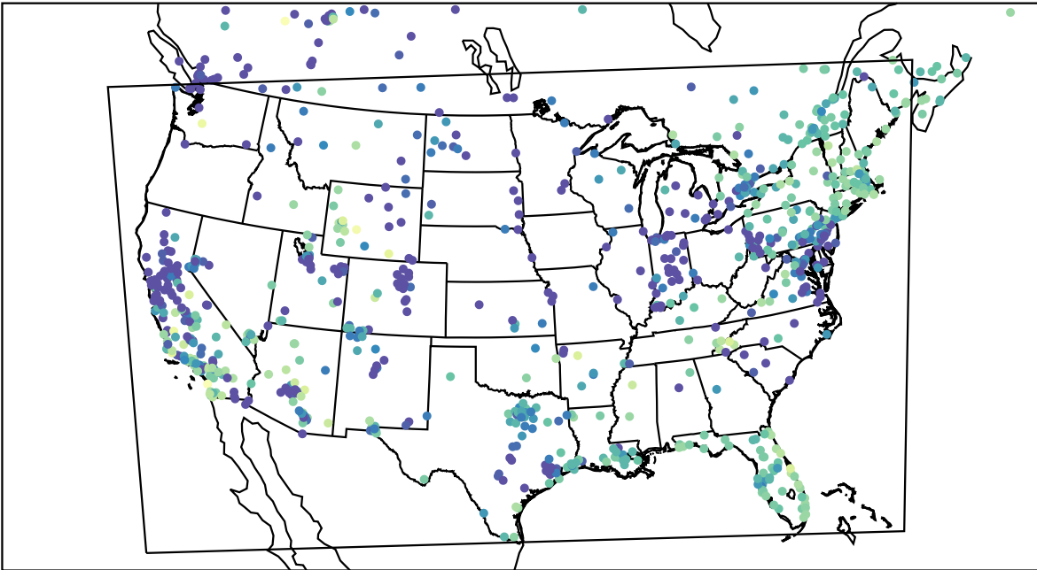
AirNOW (2023-12-14_01:00:00)
