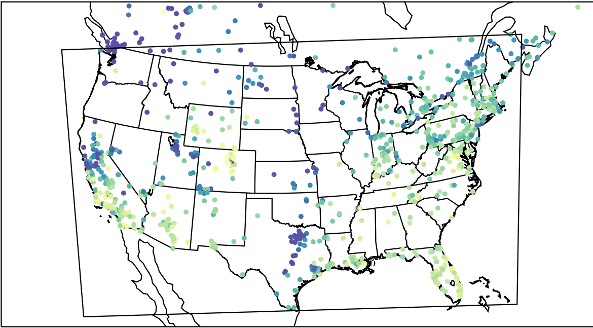
AirNOW (2023-12-15_20:00:00)
