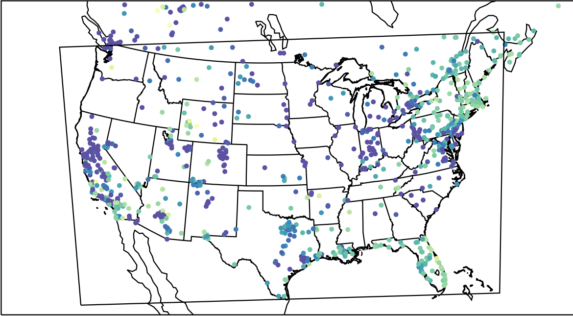
AirNOW (2023-12-14_02:00:00)
