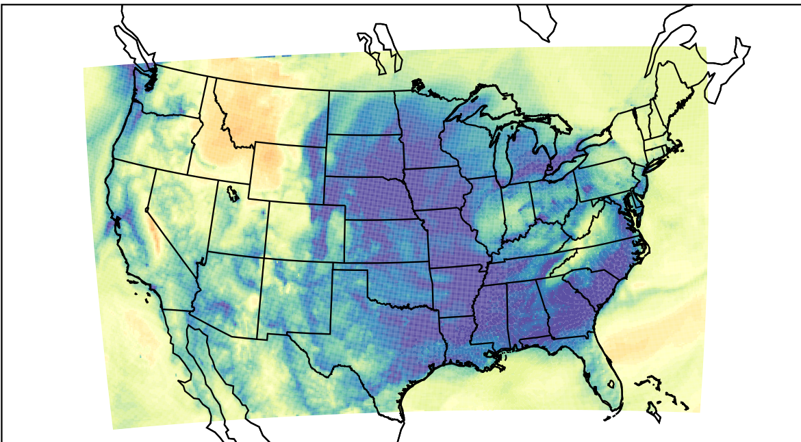
WRF (2023-12-14_10:00:00)
