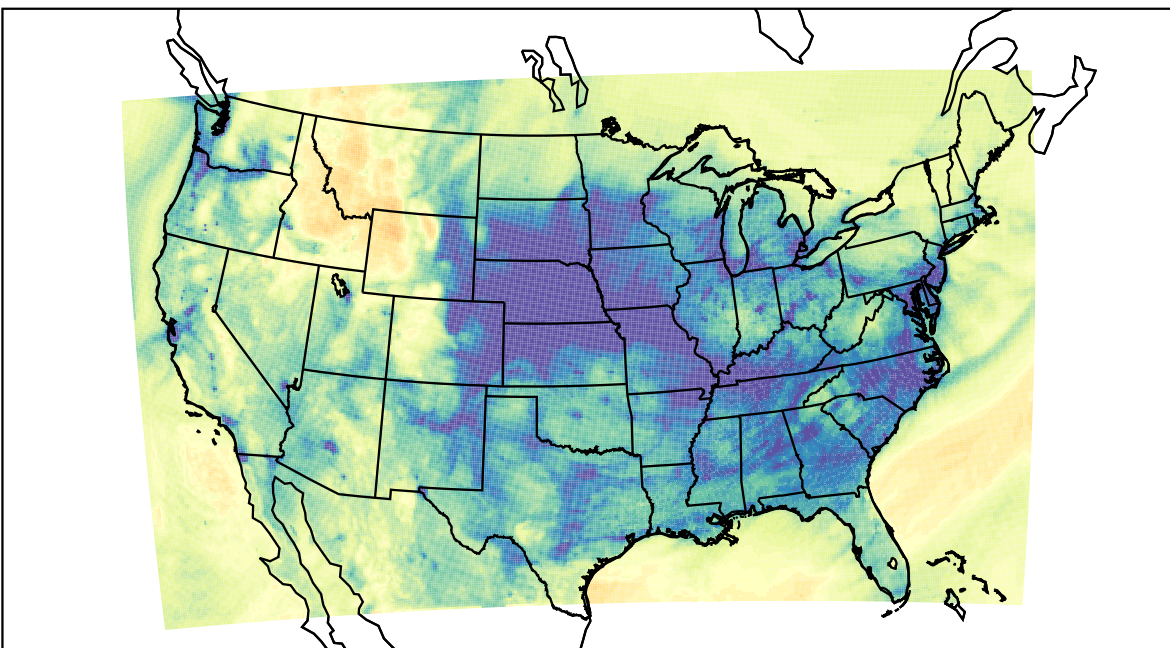
WRF (2023-12-14_01:00:00)
