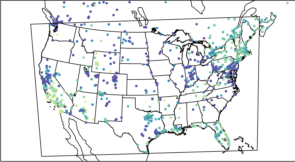
AirNOW (2023-12-14_00:00:00)
