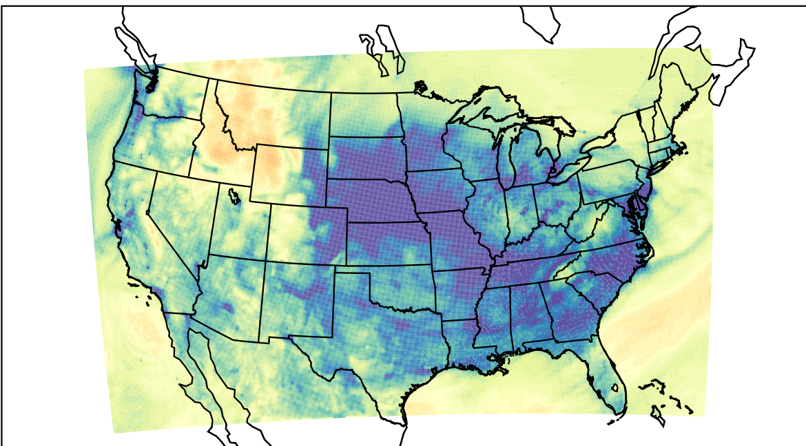
WRF (2023-12-14_03:00:00)
