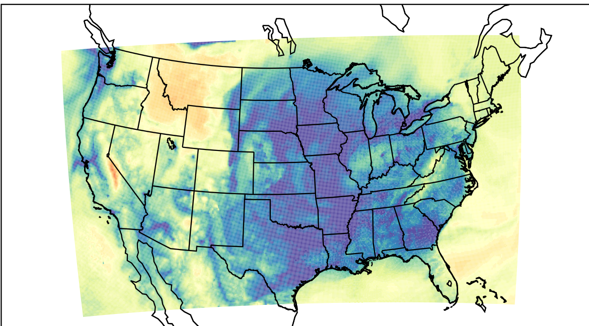
WRF (2023-12-14_14:00:00)
