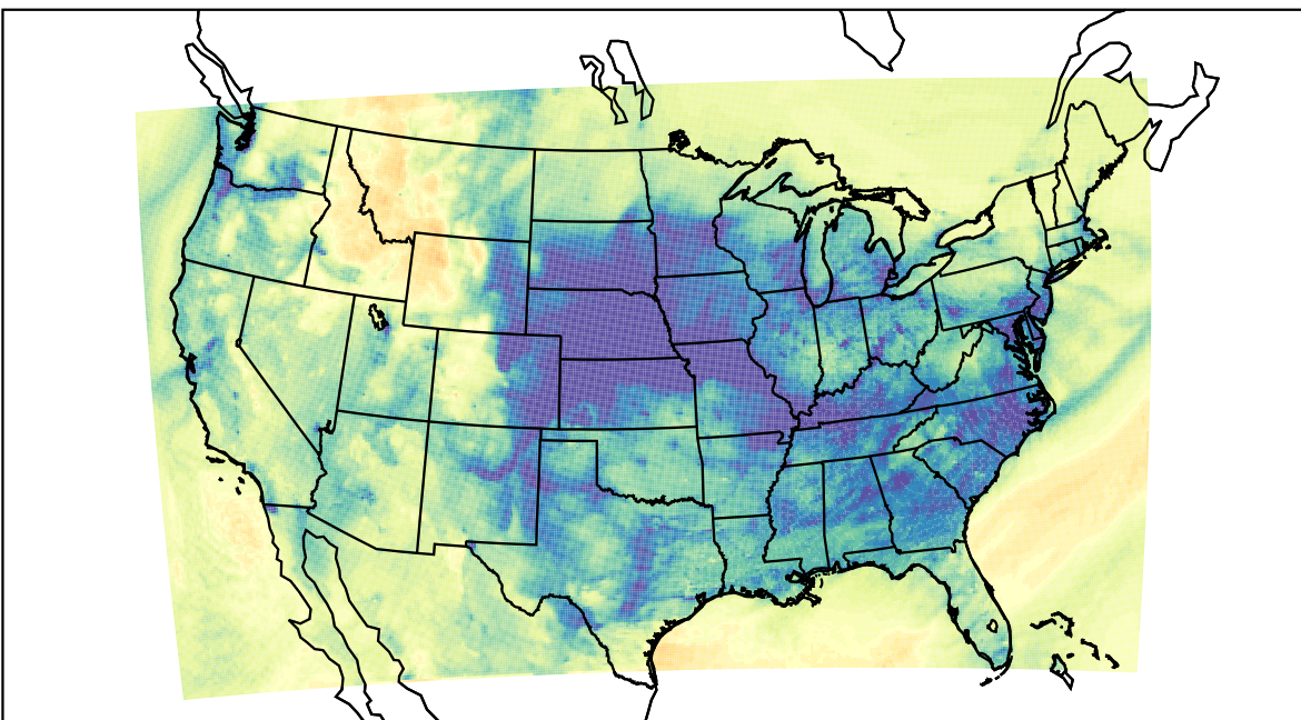
WRF (2023-12-14_00:00:00)
