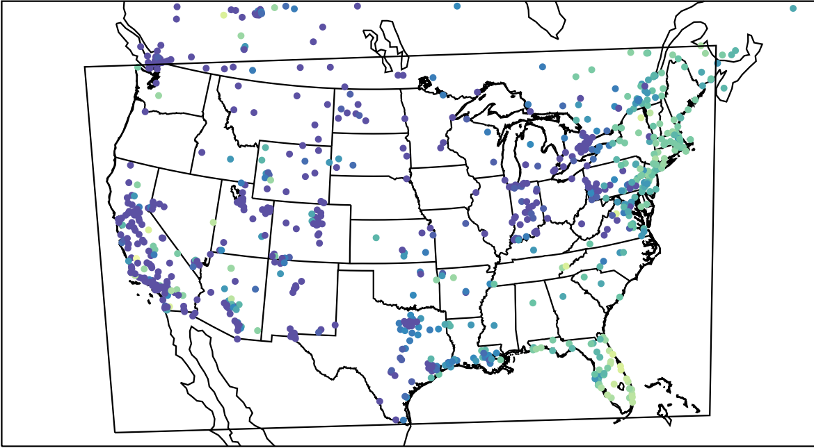
AirNOW (2023-12-14_15:00:00)
