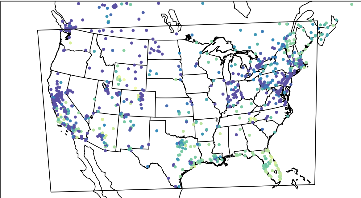
AirNOW (2023-12-15_01:00:00)
