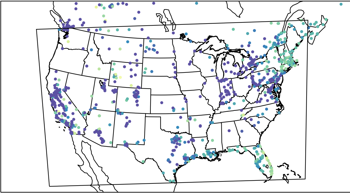
AirNOW (2023-12-14_08:00:00)
