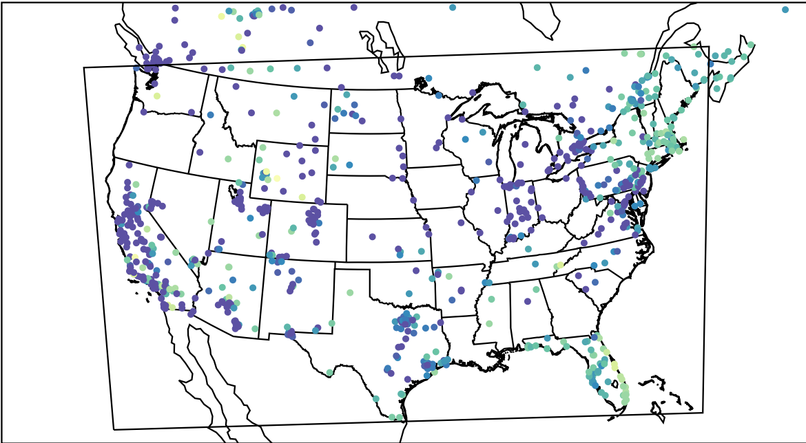
AirNOW (2023-12-14_07:00:00)
