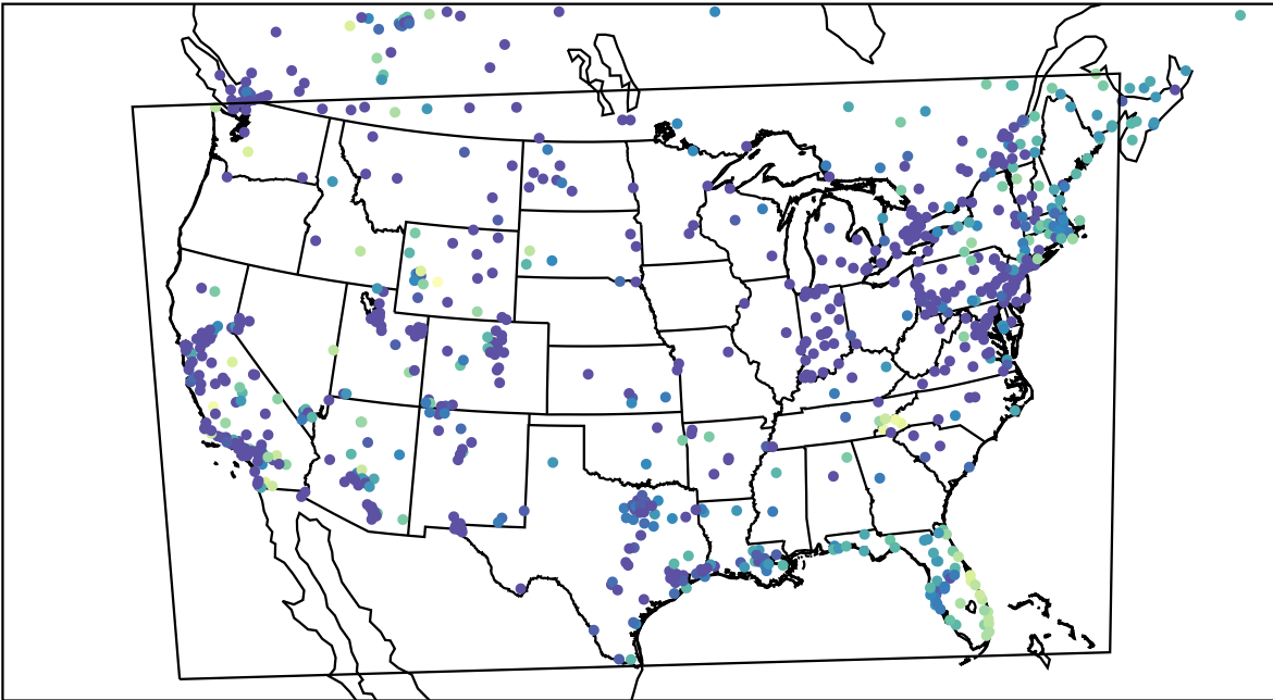
AirNOW (2023-12-14_12:00:00)
