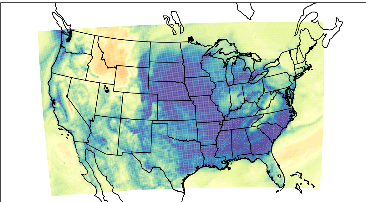
WRF (2023-12-14_07:00:00)
