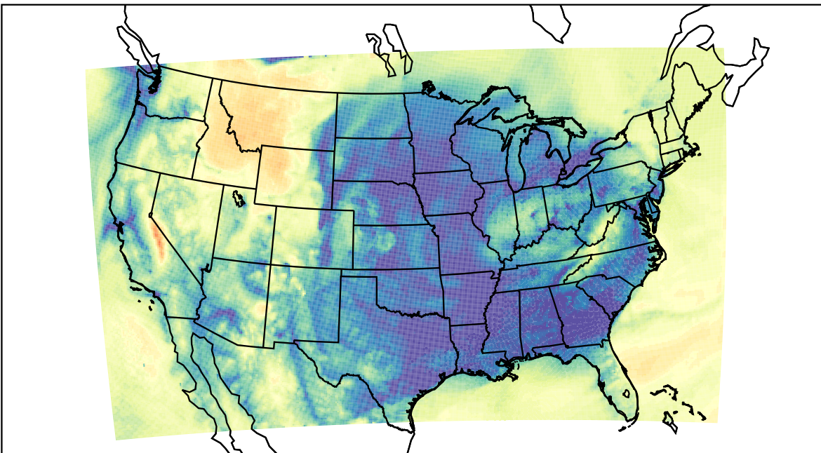
WRF (2023-12-14_13:00:00)
