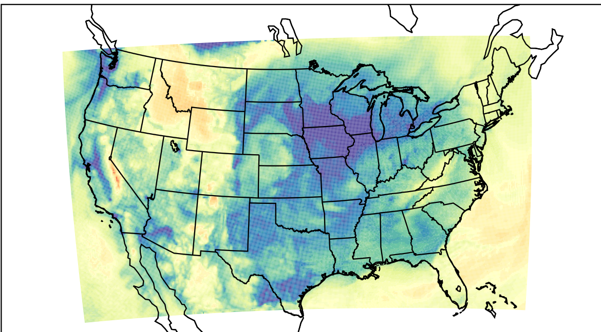
WRF (2023-12-14_17:00:00)
