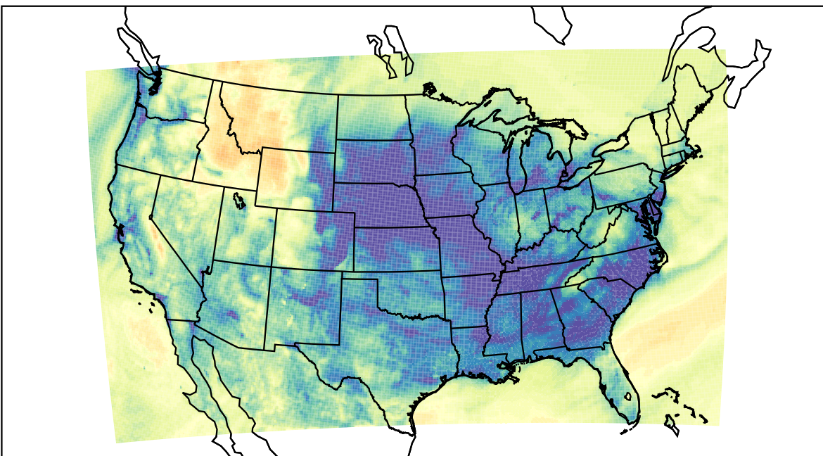
WRF (2023-12-14_04:00:00)
