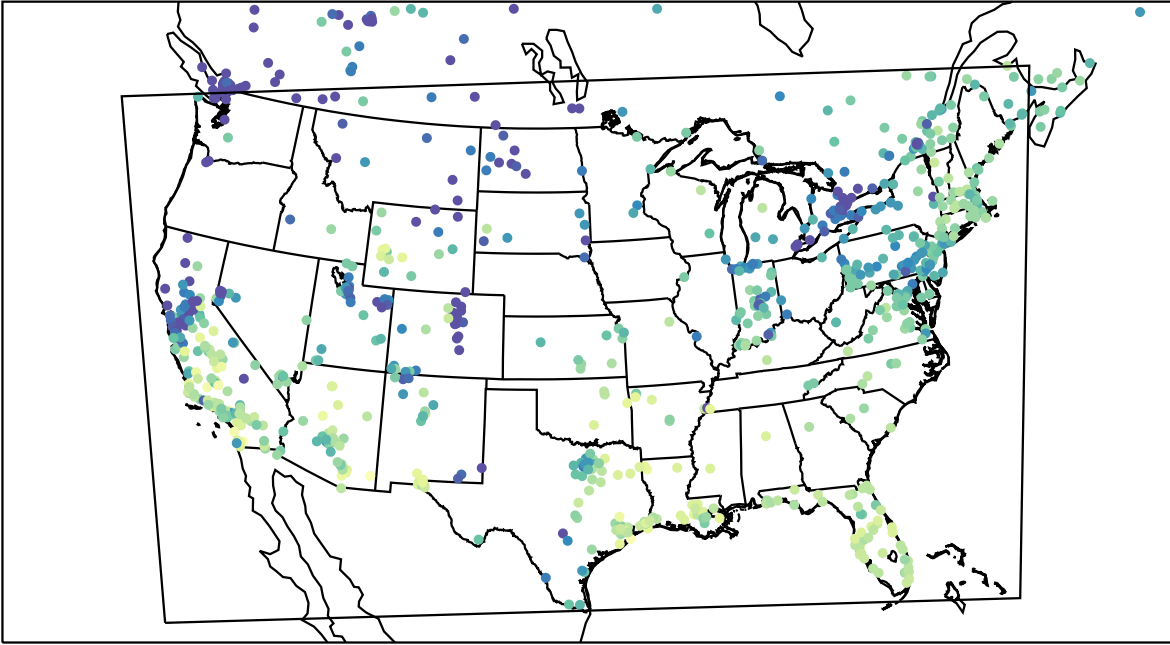
AirNOW (2023-12-14_20:00:00)
