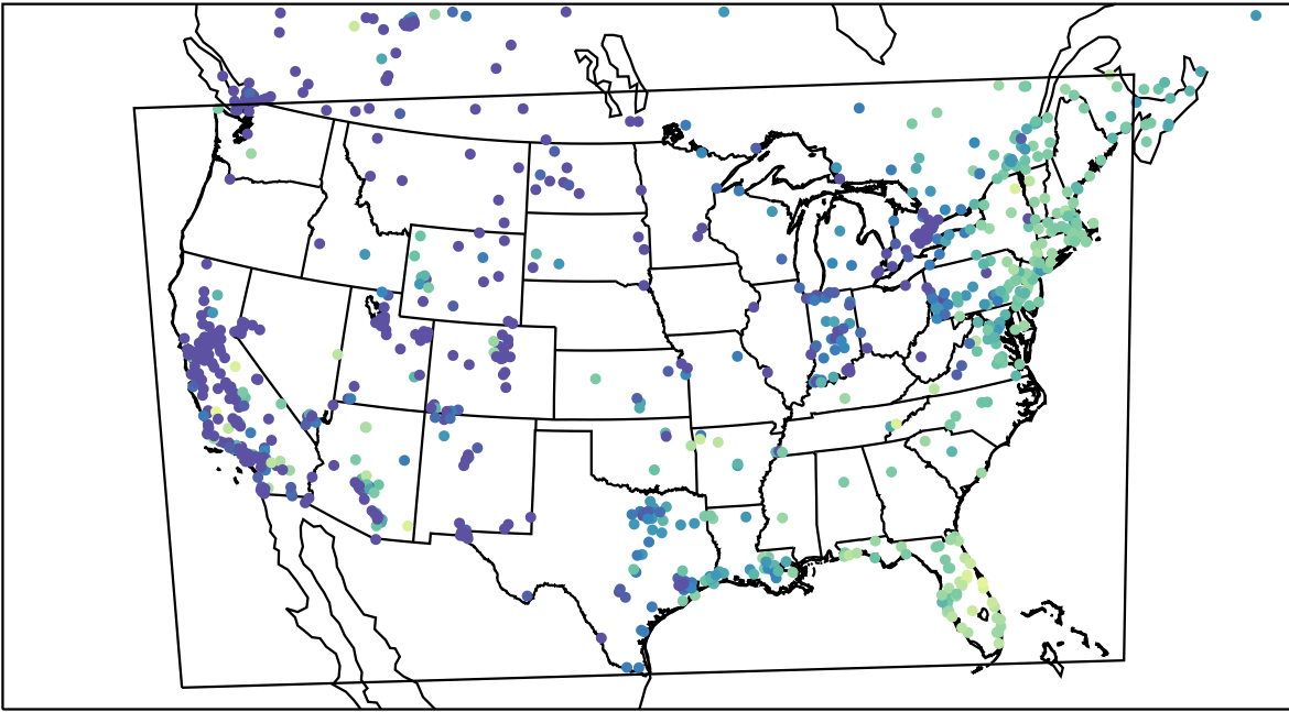
AirNOW (2023-12-14_16:00:00)
