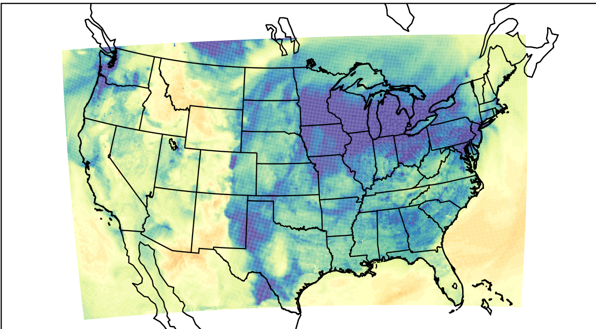
WRF (2023-12-14_23:00:00)
