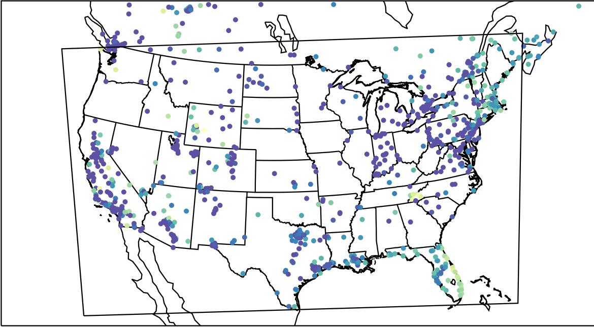
AirNOW (2023-12-14_11:00:00)
