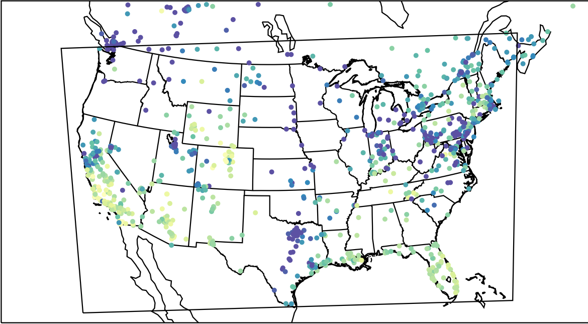
AirNOW (2023-12-15_22:00:00)
