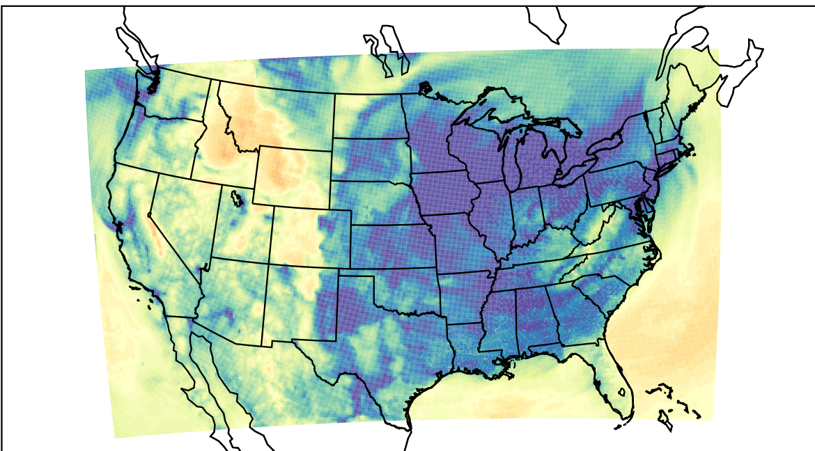
WRF (2023-12-15_05:00:00)
