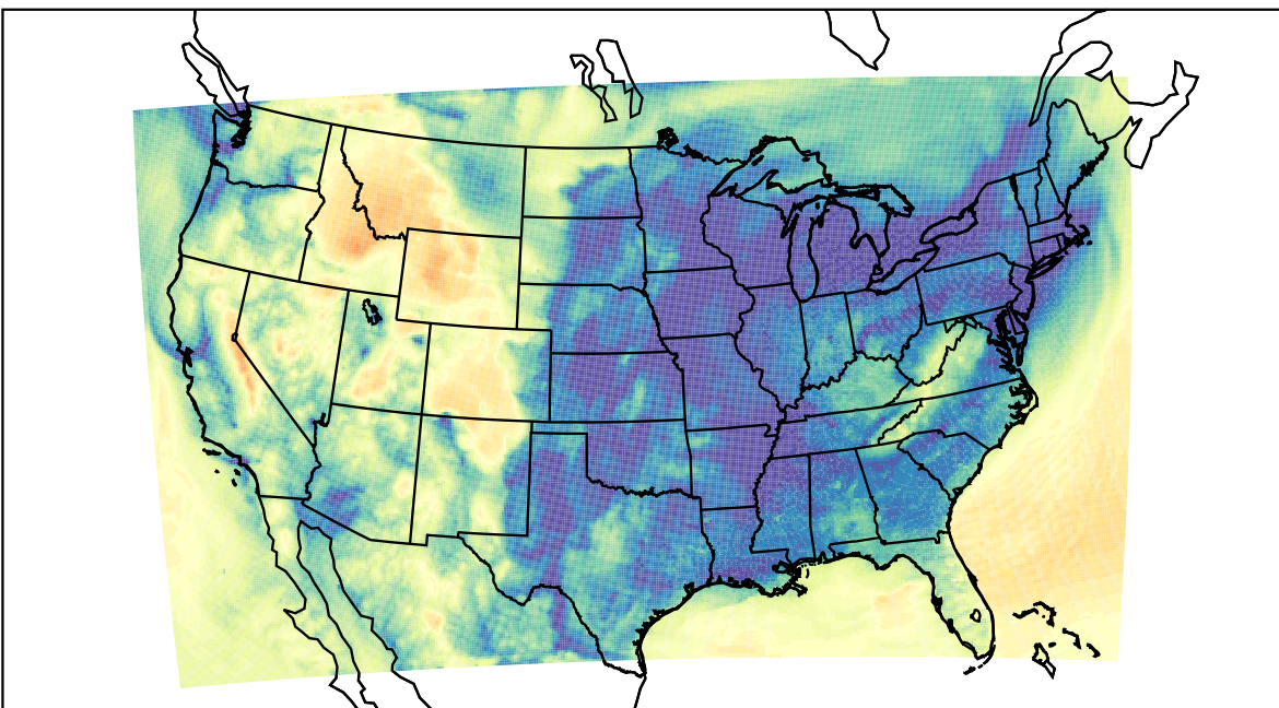
WRF (2023-12-15_10:00:00)
