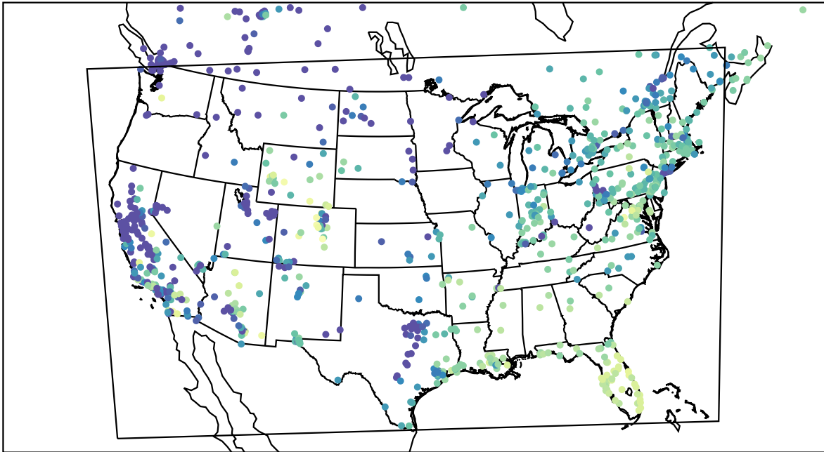
AirNOW (2023-12-15_17:00:00)
