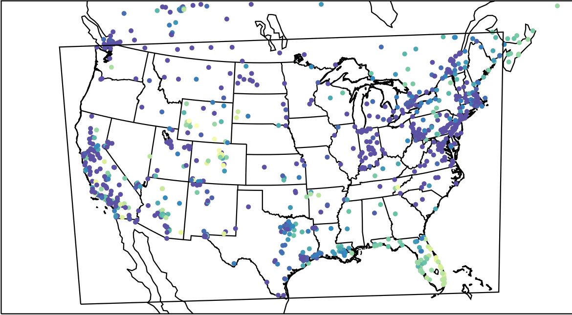
AirNOW (2023-12-15_13:00:00)
