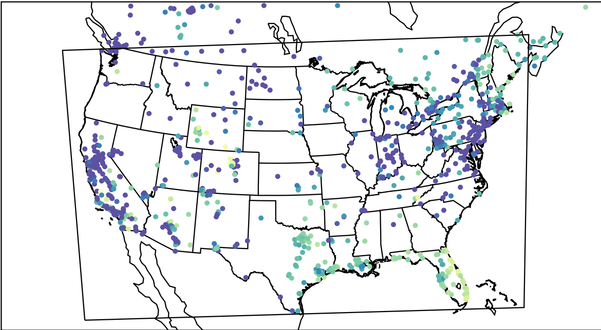
AirNOW (2023-12-15_04:00:00)
