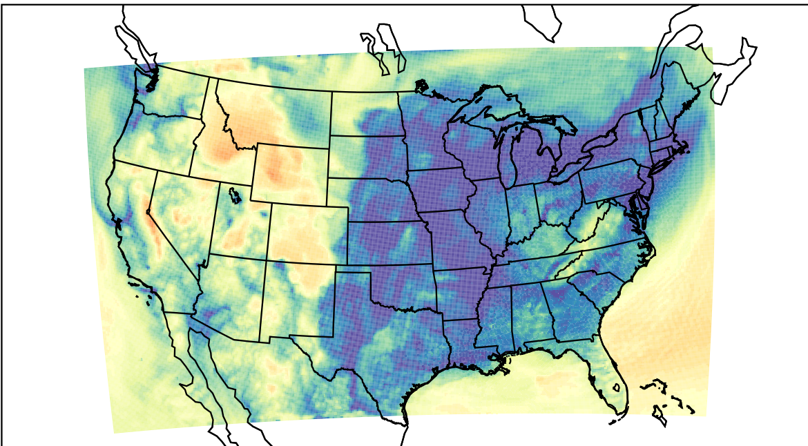
WRF (2023-12-15_12:00:00)
