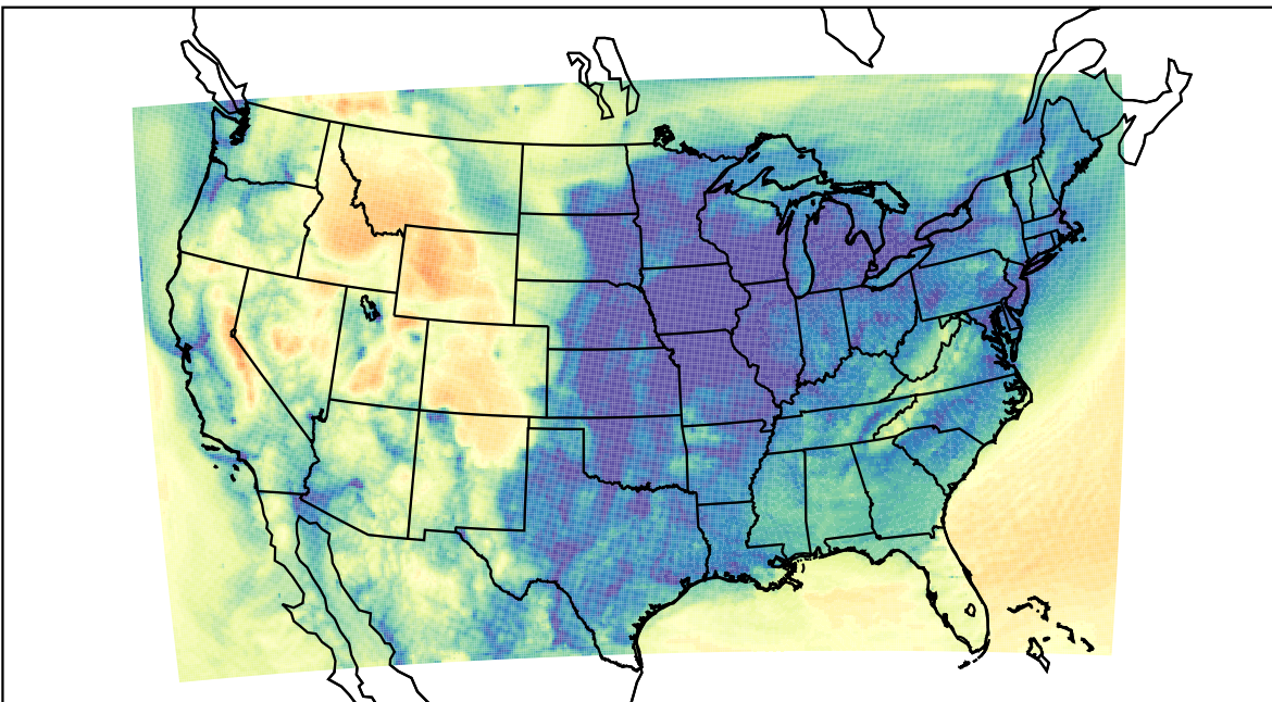
WRF (2023-12-15_15:00:00)
