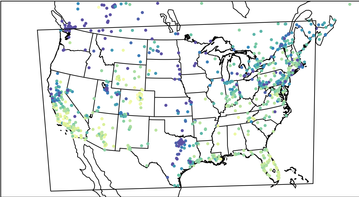
AirNOW (2023-12-15_21:00:00)
