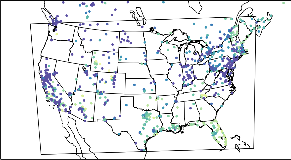
AirNOW (2023-12-15_02:00:00)
