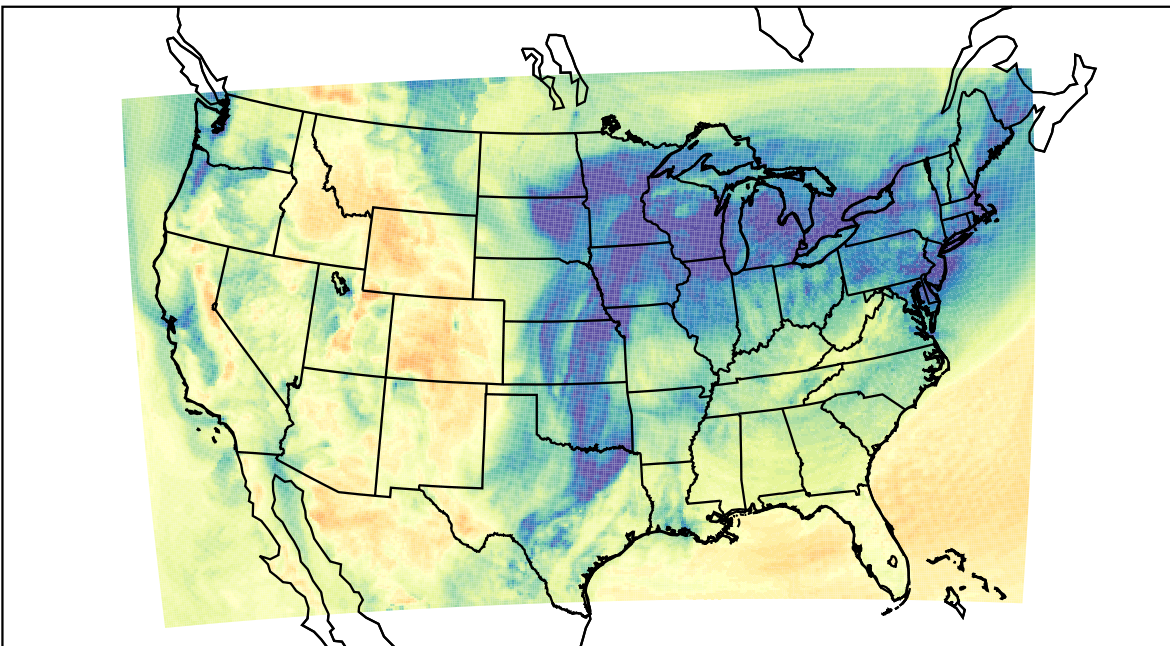
WRF (2023-12-15_20:00:00)
