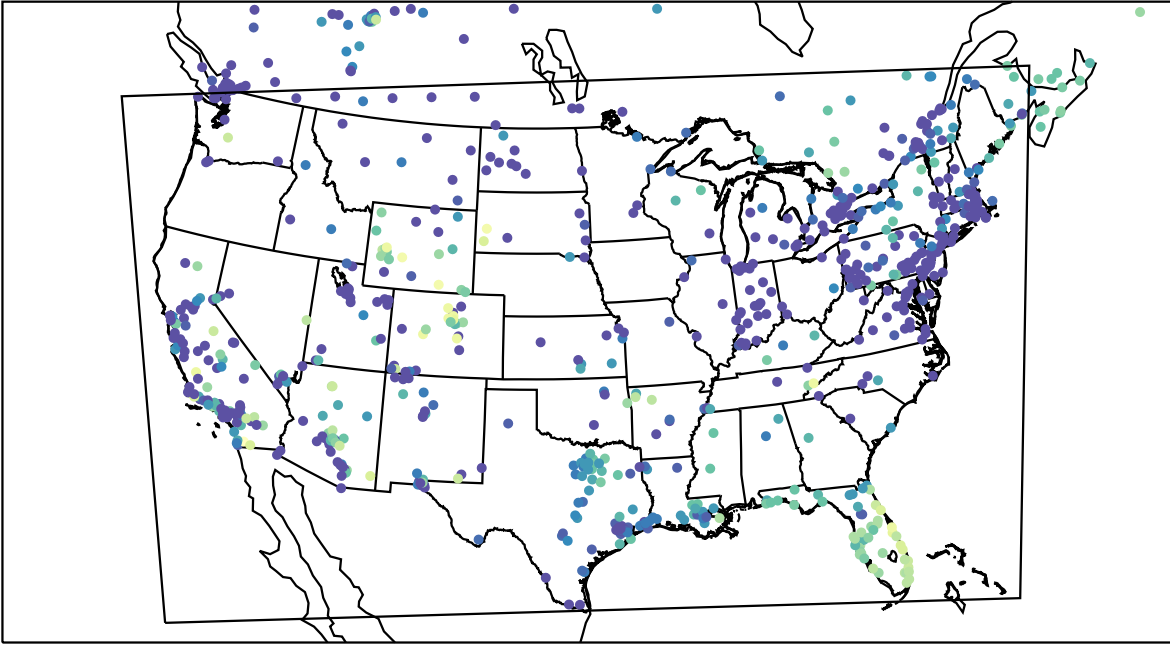
AirNOW (2023-12-15_12:00:00)
