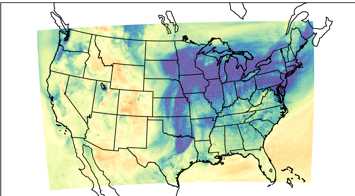
WRF (2023-12-15_22:00:00)
