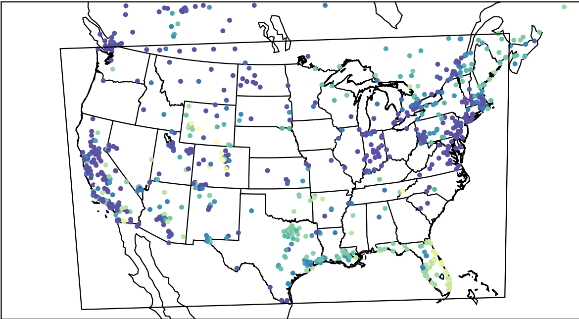
AirNOW (2023-12-15_07:00:00)
