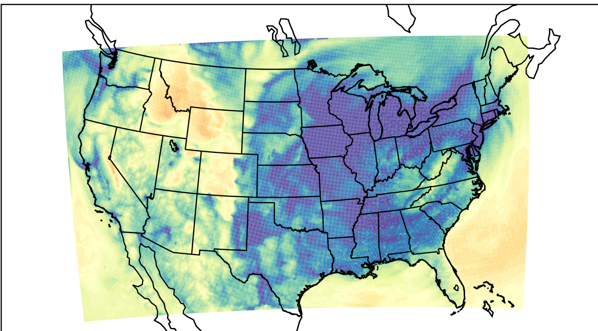
WRF (2023-12-15_06:00:00)
