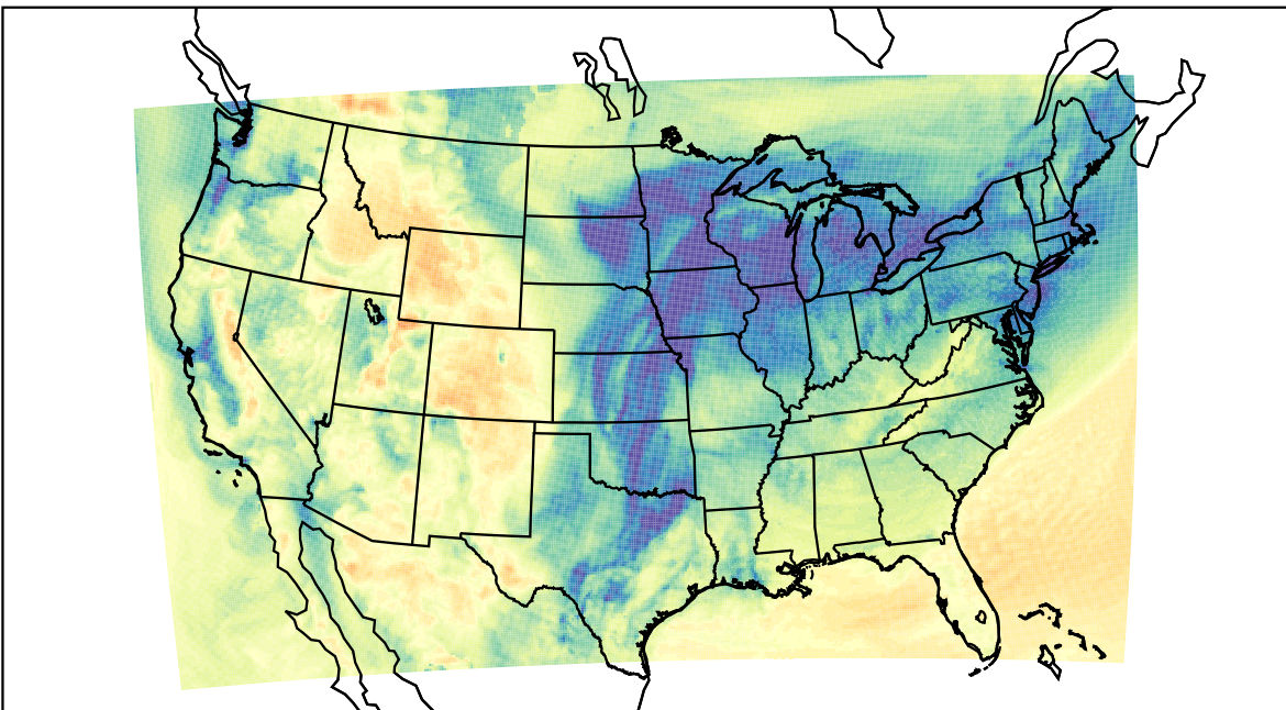
WRF (2023-12-15_19:00:00)
