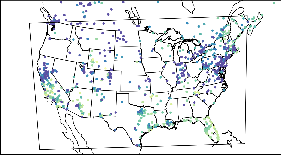
AirNOW (2023-12-15_00:00:00)
