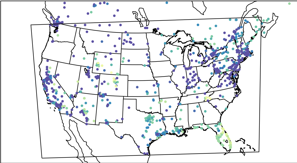
AirNOW (2023-12-15_10:00:00)
