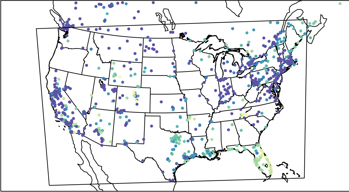
AirNOW (2023-12-15_09:00:00)
