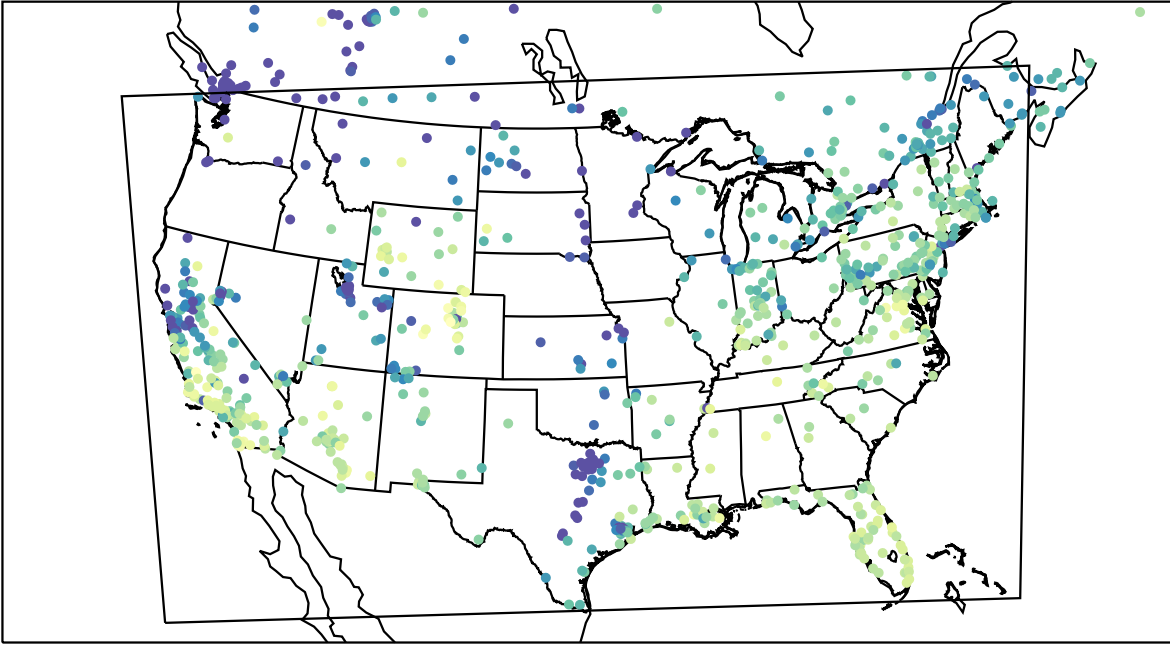
AirNOW (2023-12-15_20:00:00)
