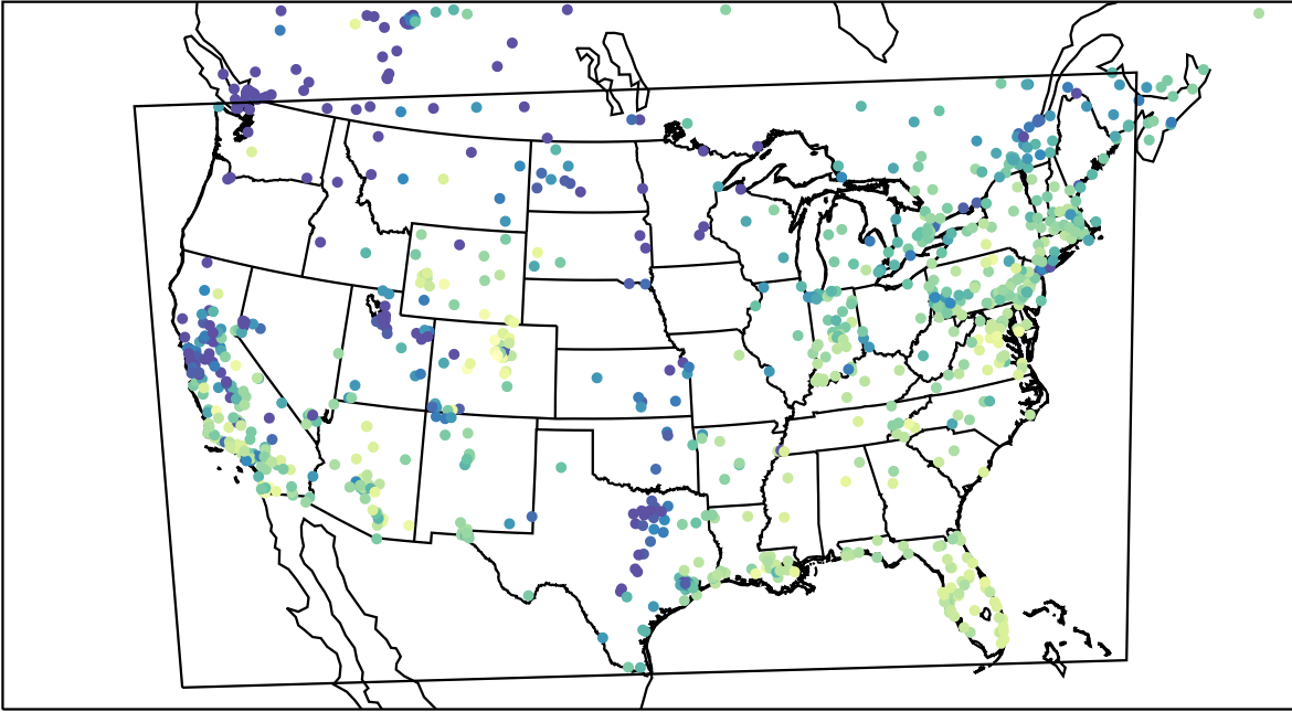
AirNOW (2023-12-15_19:00:00)
