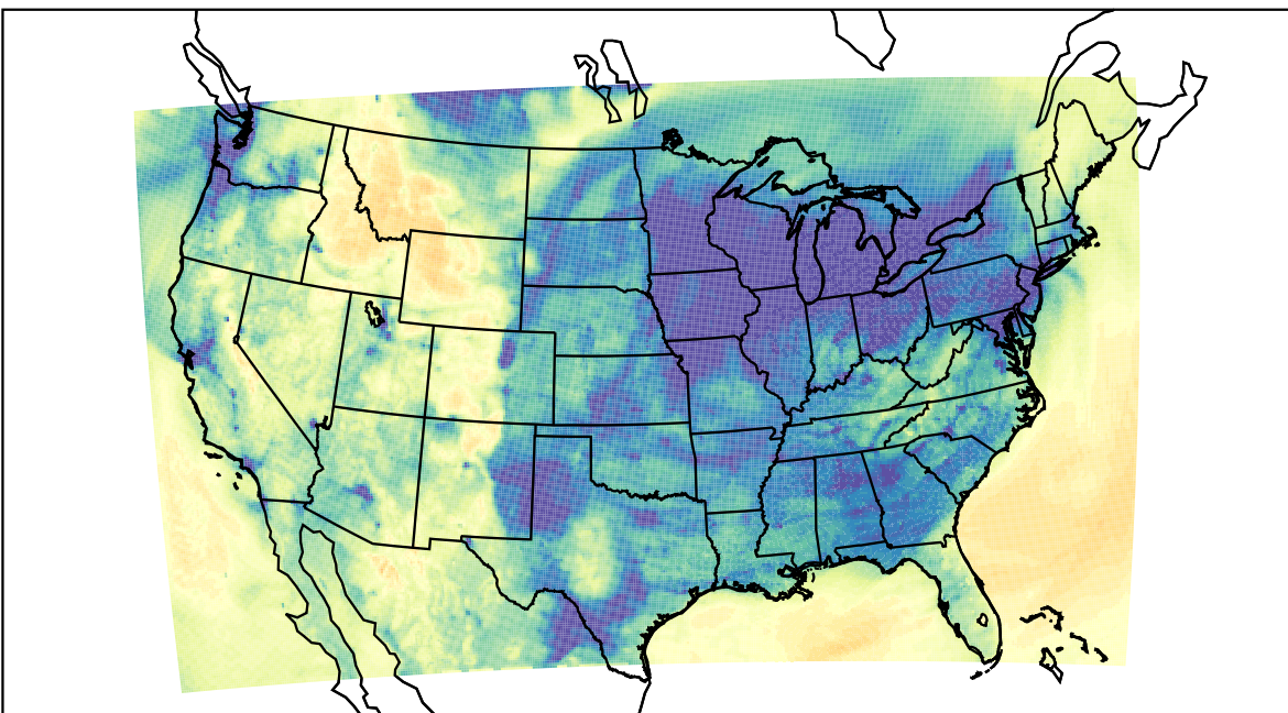
WRF (2023-12-15_01:00:00)
