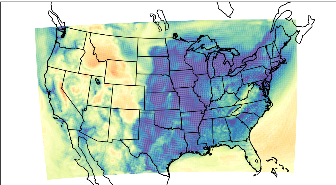
WRF (2023-12-15_13:00:00)
