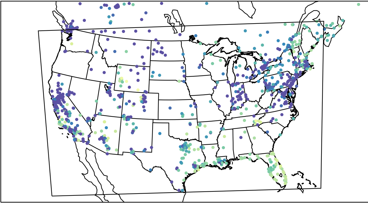
AirNOW (2023-12-15_01:00:00)
