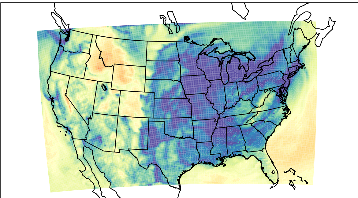
WRF (2023-12-15_07:00:00)
