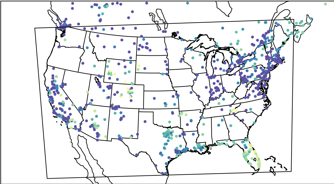
AirNOW (2023-12-15_11:00:00)
