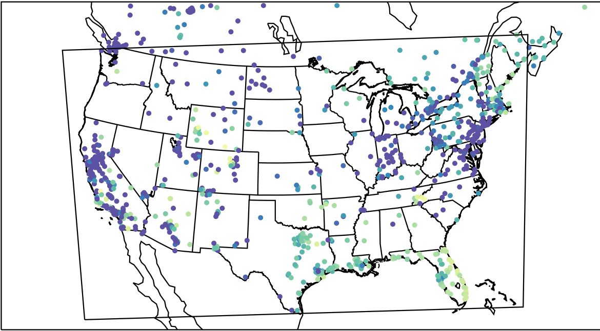
AirNOW (2023-12-15_03:00:00)
