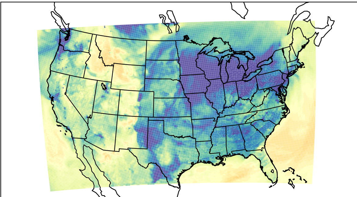
WRF (2023-12-15_00:00:00)
