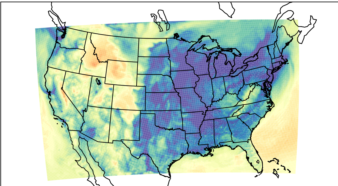
WRF (2023-12-15_09:00:00)
