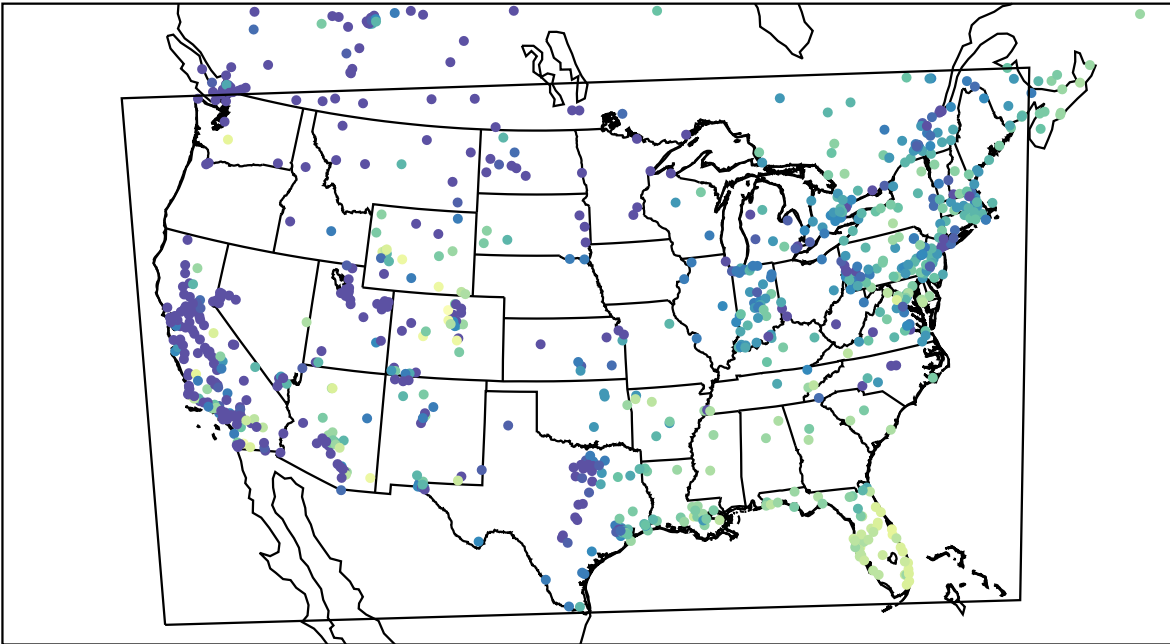
AirNOW (2023-12-15_16:00:00)
