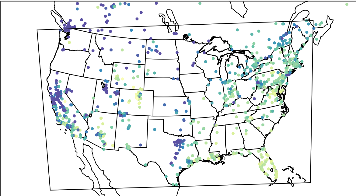
AirNOW (2023-12-15_18:00:00)
