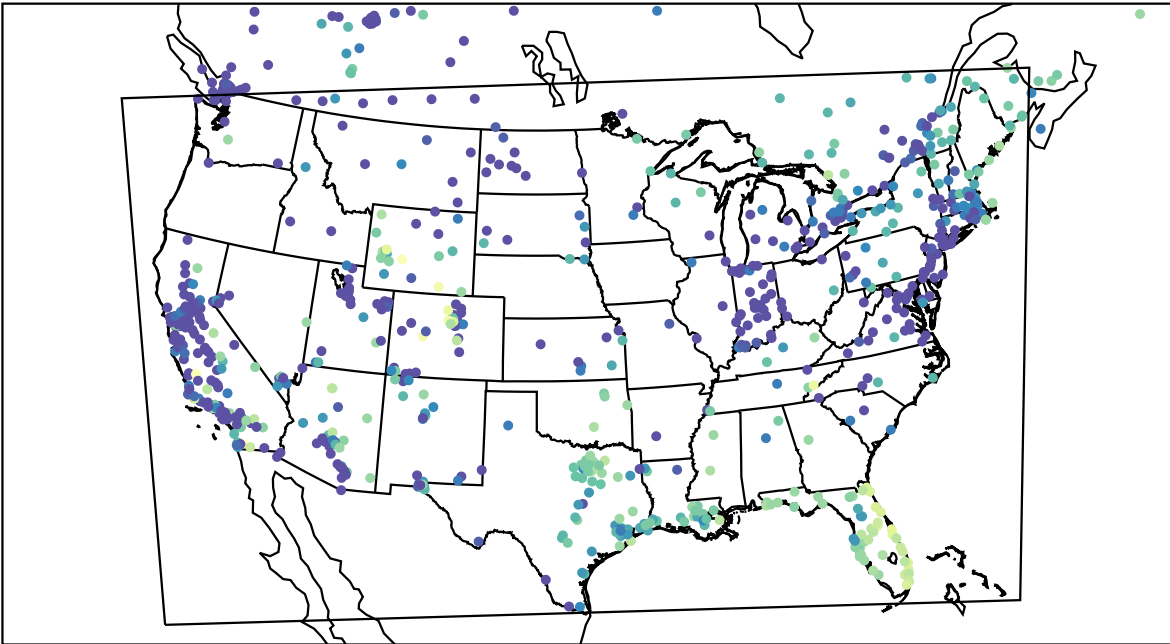
AirNOW (2023-12-15_06:00:00)
