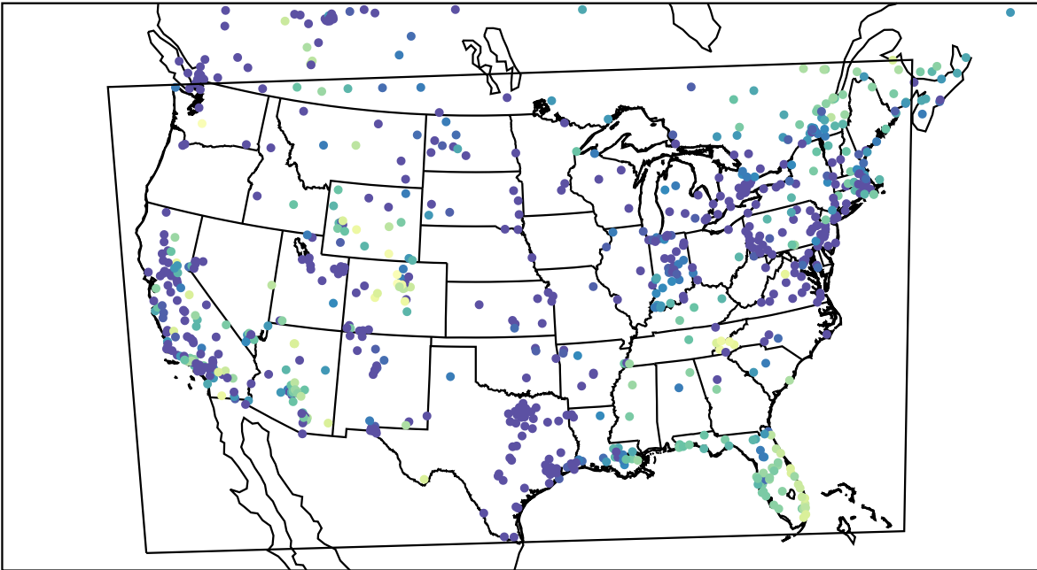
AirNOW (2023-12-16_11:00:00)
