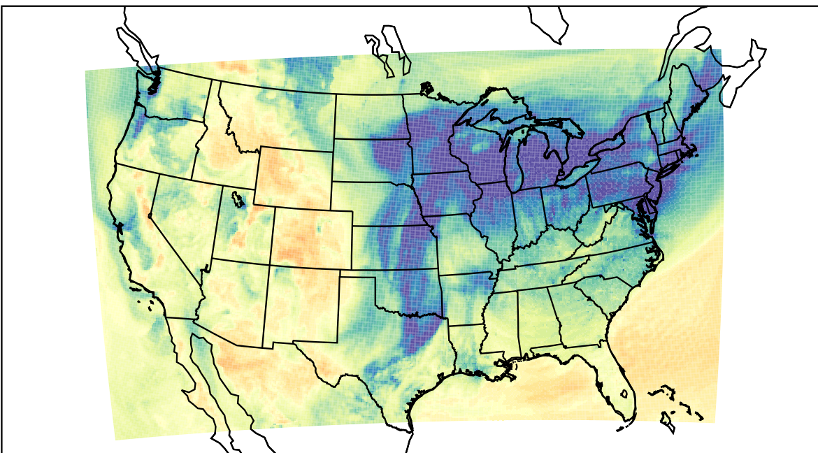
WRF (2023-12-15_21:00:00)
