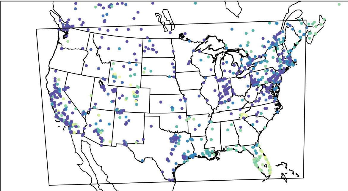
AirNOW (2023-12-15_14:00:00)
