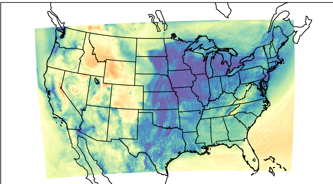
WRF (2023-12-15_16:00:00)
