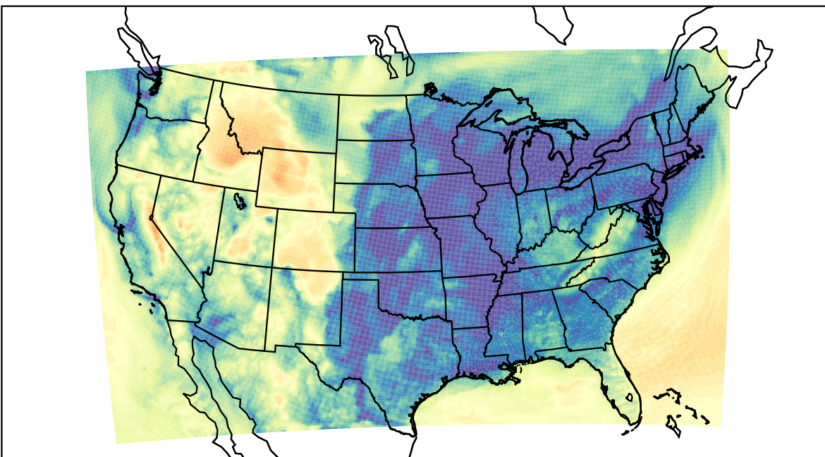
WRF (2023-12-15_11:00:00)
