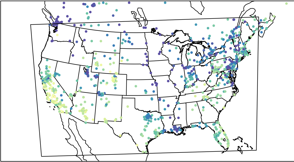
AirNOW (2023-12-16_22:00:00)
