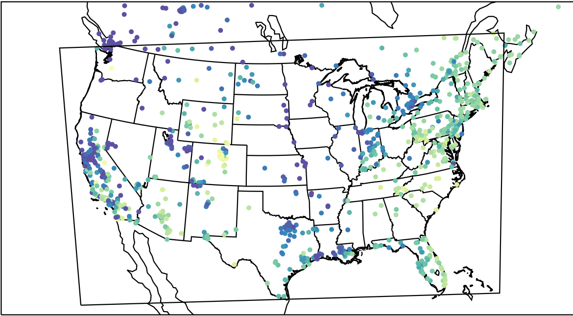
AirNOW (2023-12-16_18:00:00)
