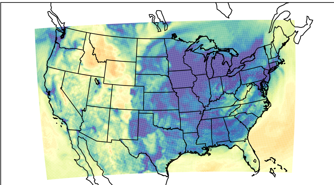
WRF (2023-12-15_04:00:00)
