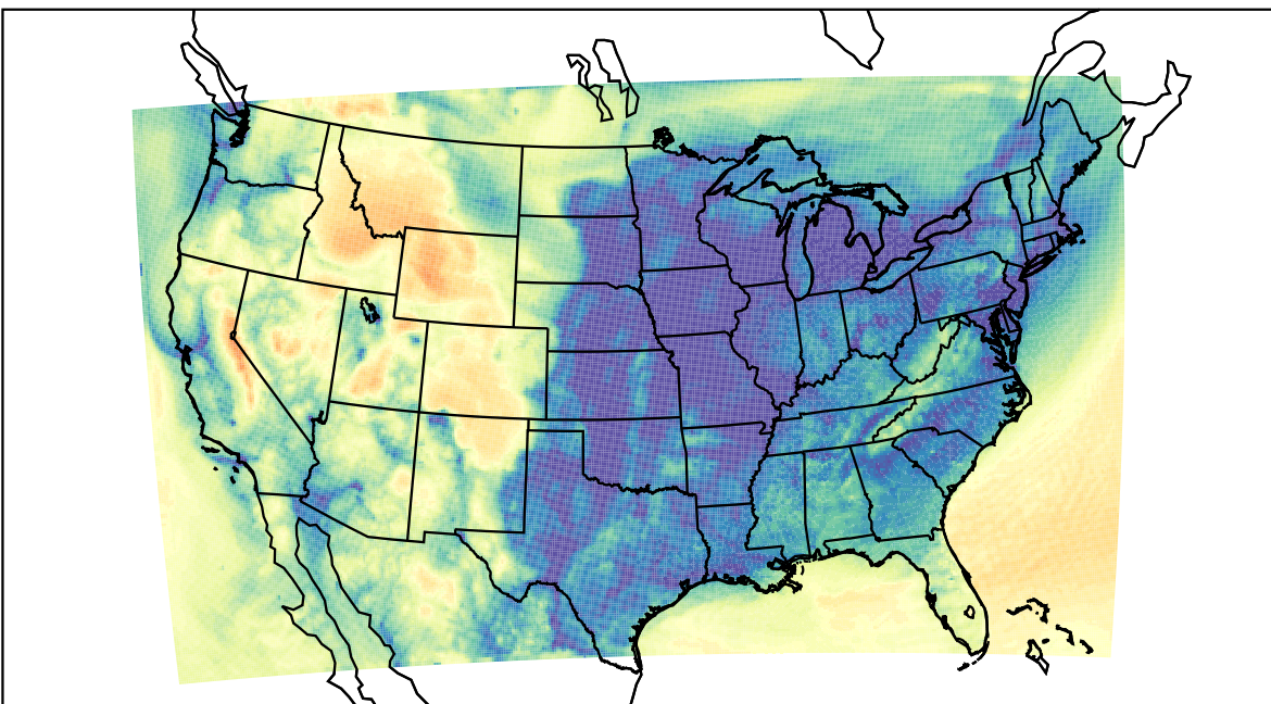
WRF (2023-12-15_14:00:00)
