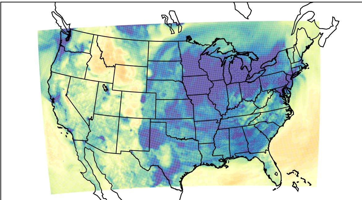
WRF (2023-12-15_02:00:00)
