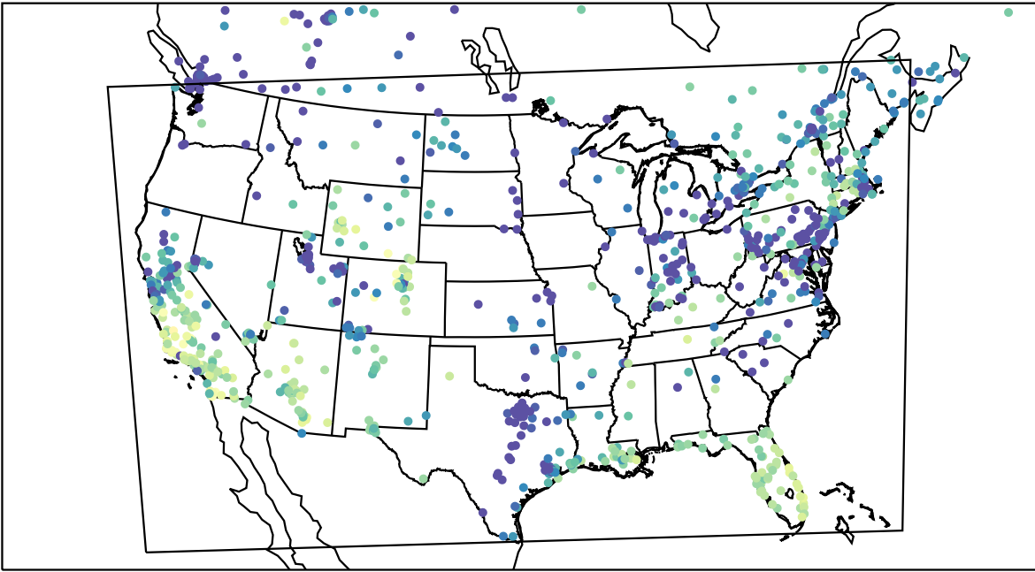
AirNOW (2023-12-15_23:00:00)
