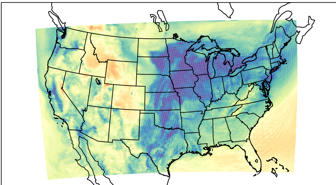
WRF (2023-12-15_17:00:00)
