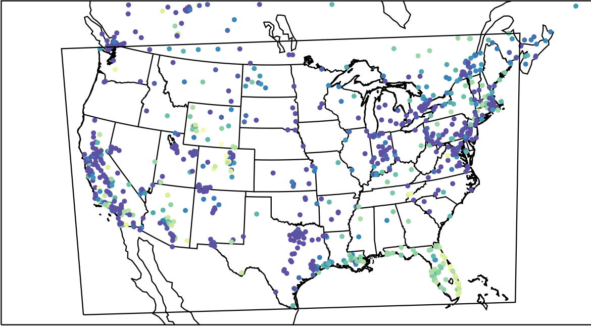
AirNOW (2023-12-16_04:00:00)
