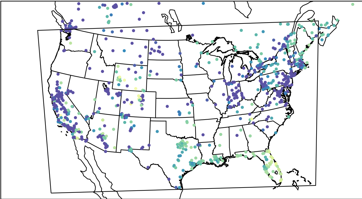
AirNOW (2023-12-15_05:00:00)
