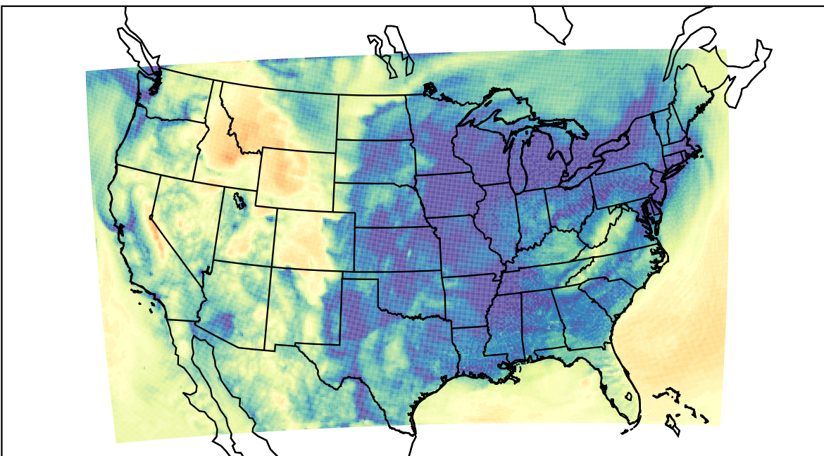
WRF (2023-12-15_08:00:00)
