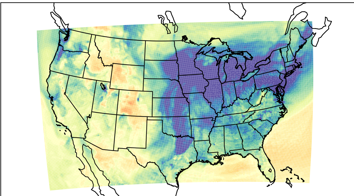
WRF (2023-12-15_23:00:00)
