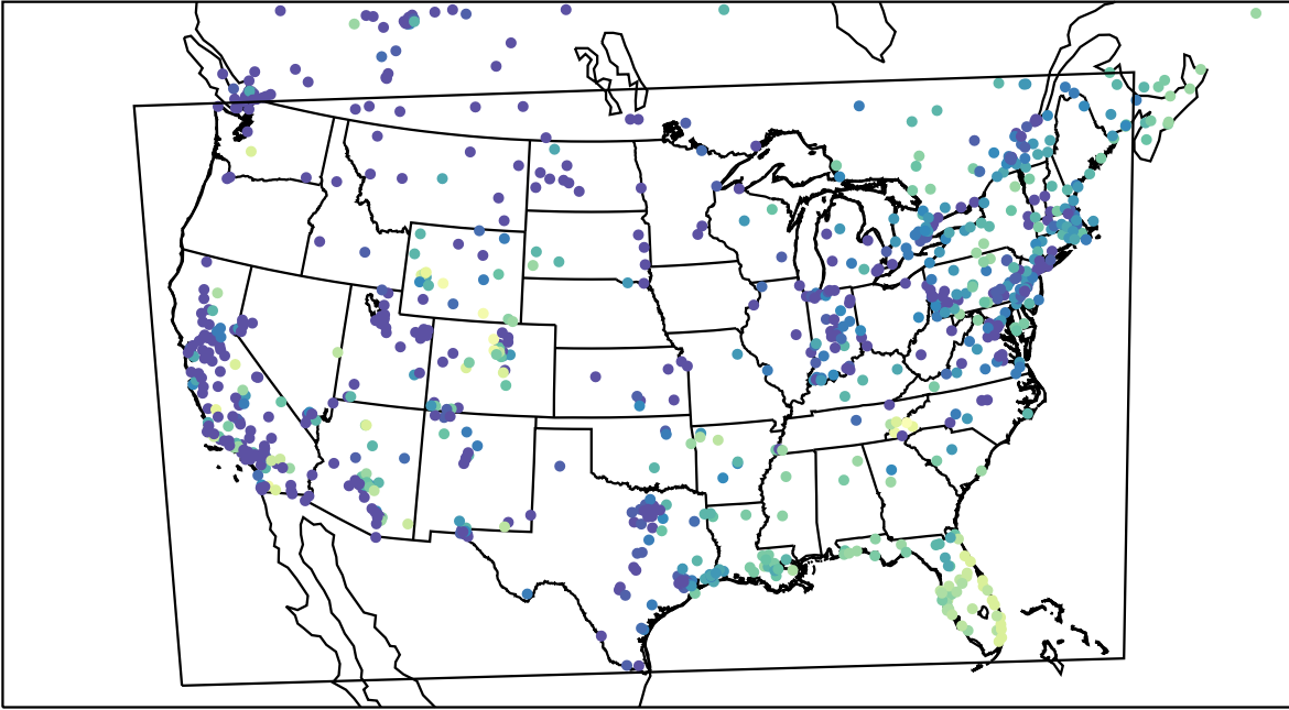
AirNOW (2023-12-15_15:00:00)
