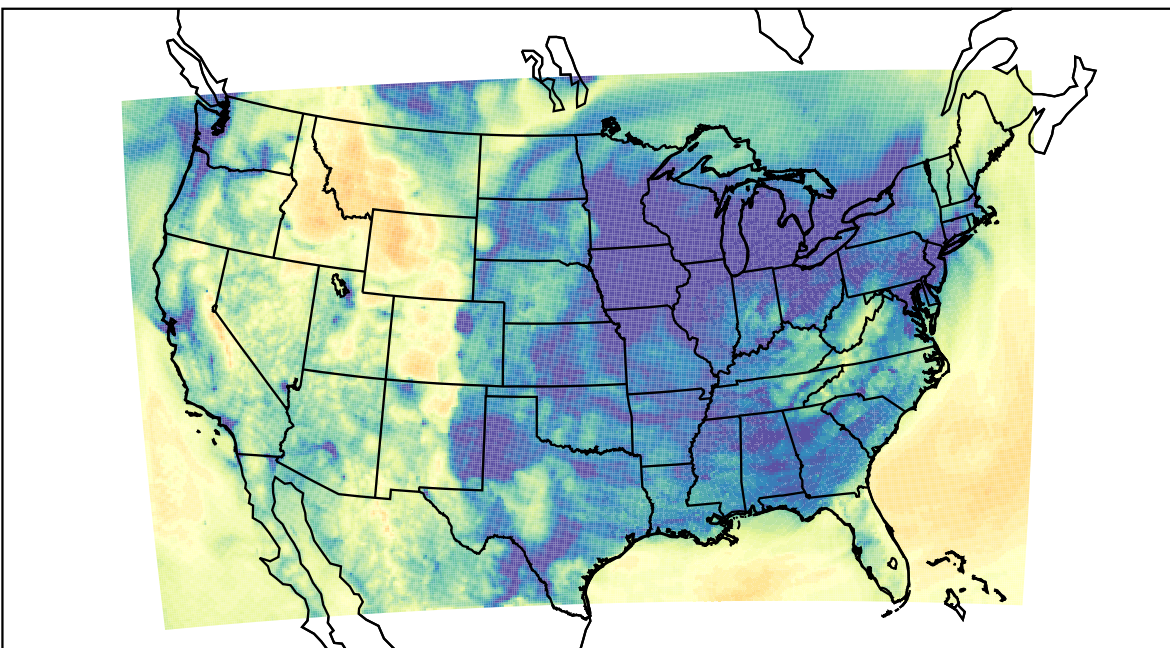
WRF (2023-12-15_03:00:00)
