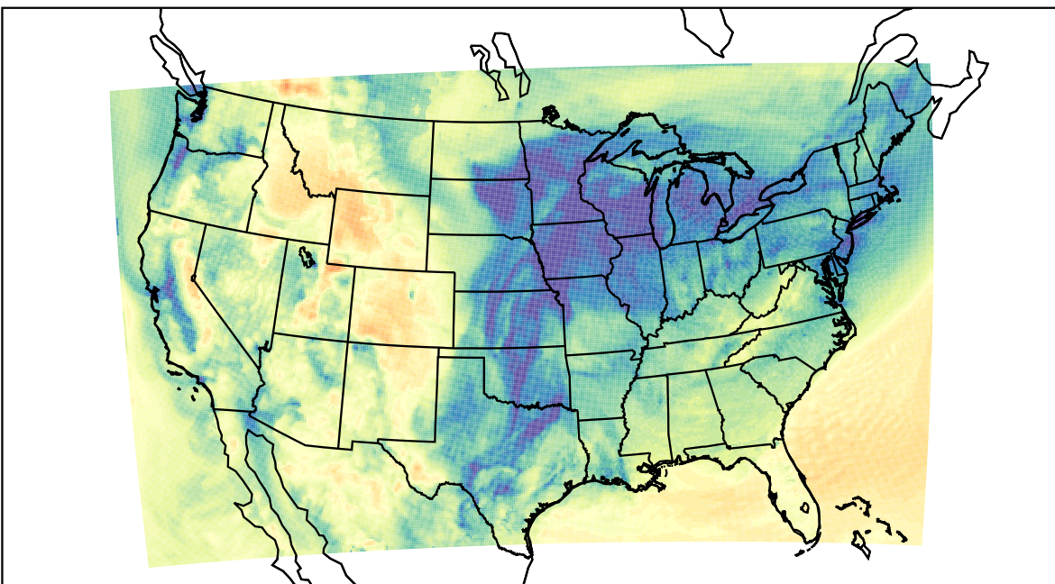
WRF (2023-12-15_18:00:00)
