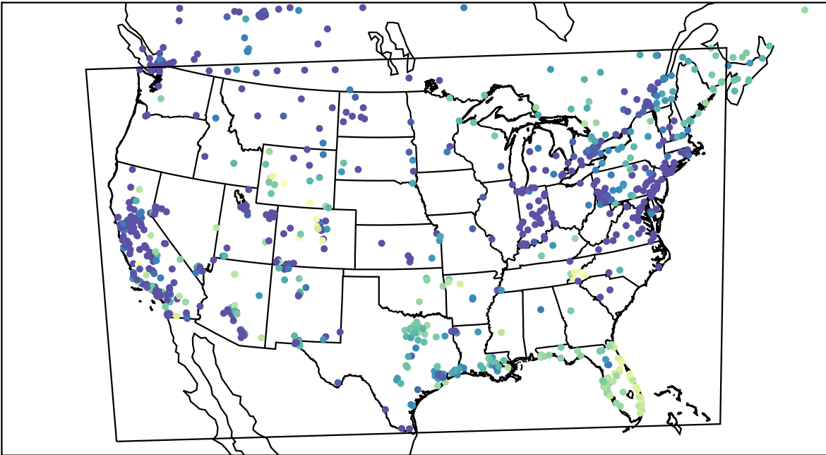
AirNOW (2023-12-15_08:00:00)
