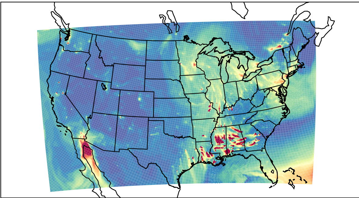
WRF 2023-12-16_23:00:00
