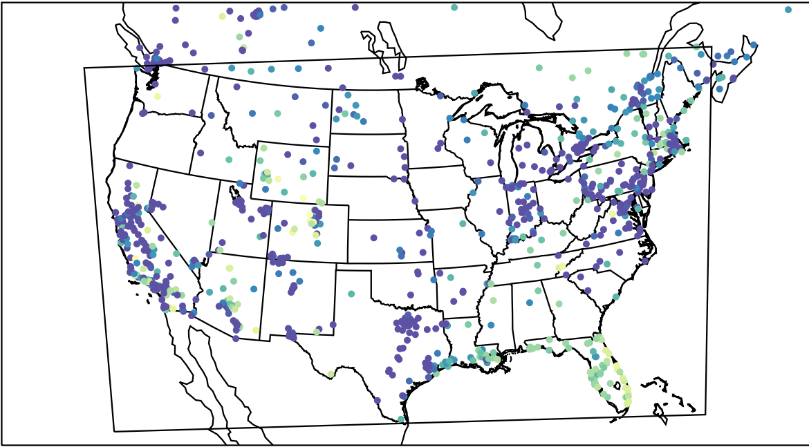
AirNOW (2023-12-16_04:00:00)
