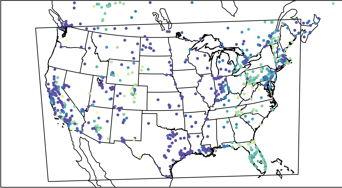
AirNOW (2023-12-17_09:00:00)
