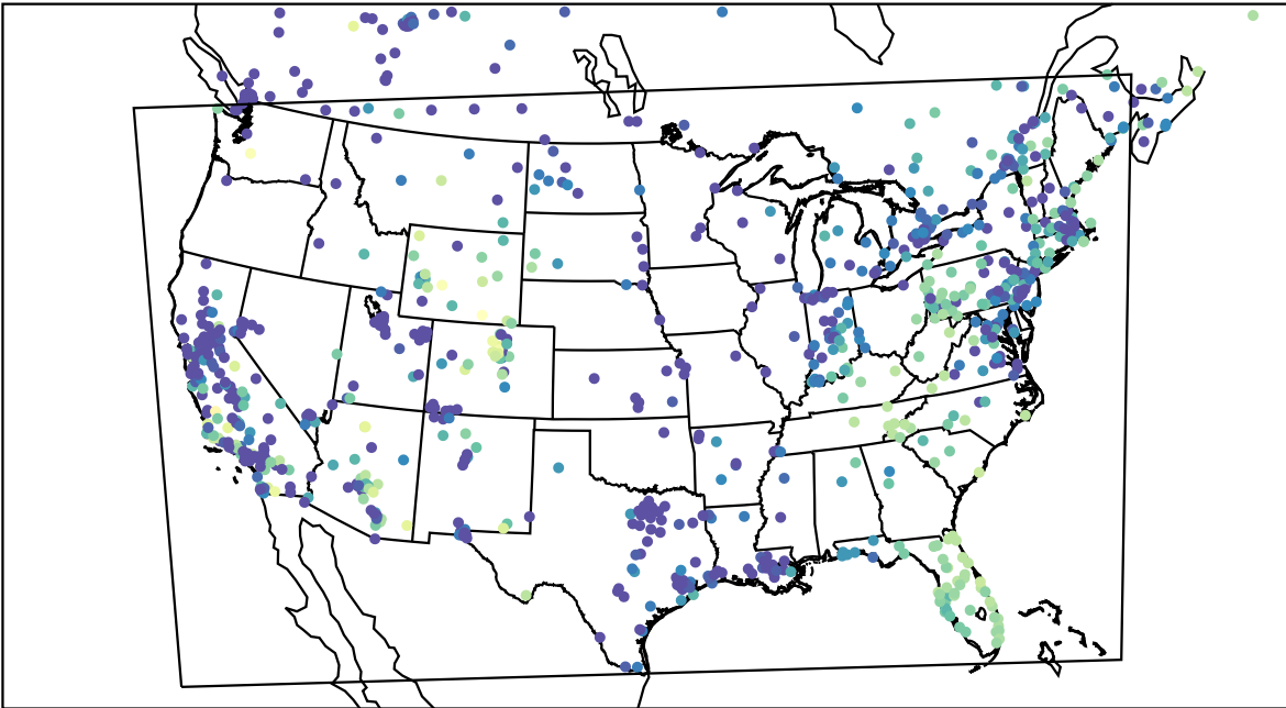
AirNOW (2023-12-17_02:00:00)
