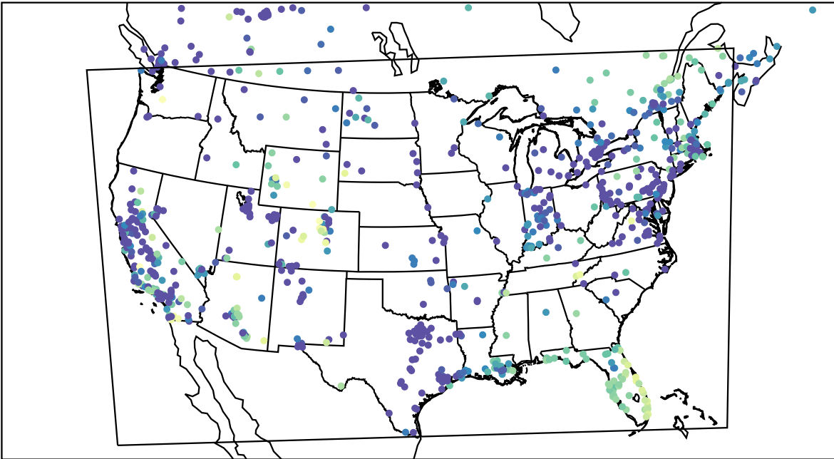
AirNOW (2023-12-16_08:00:00)
