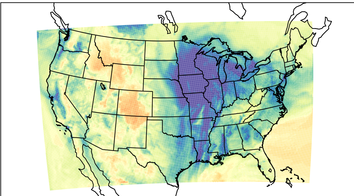
WRF (2023-12-16_18:00:00)
