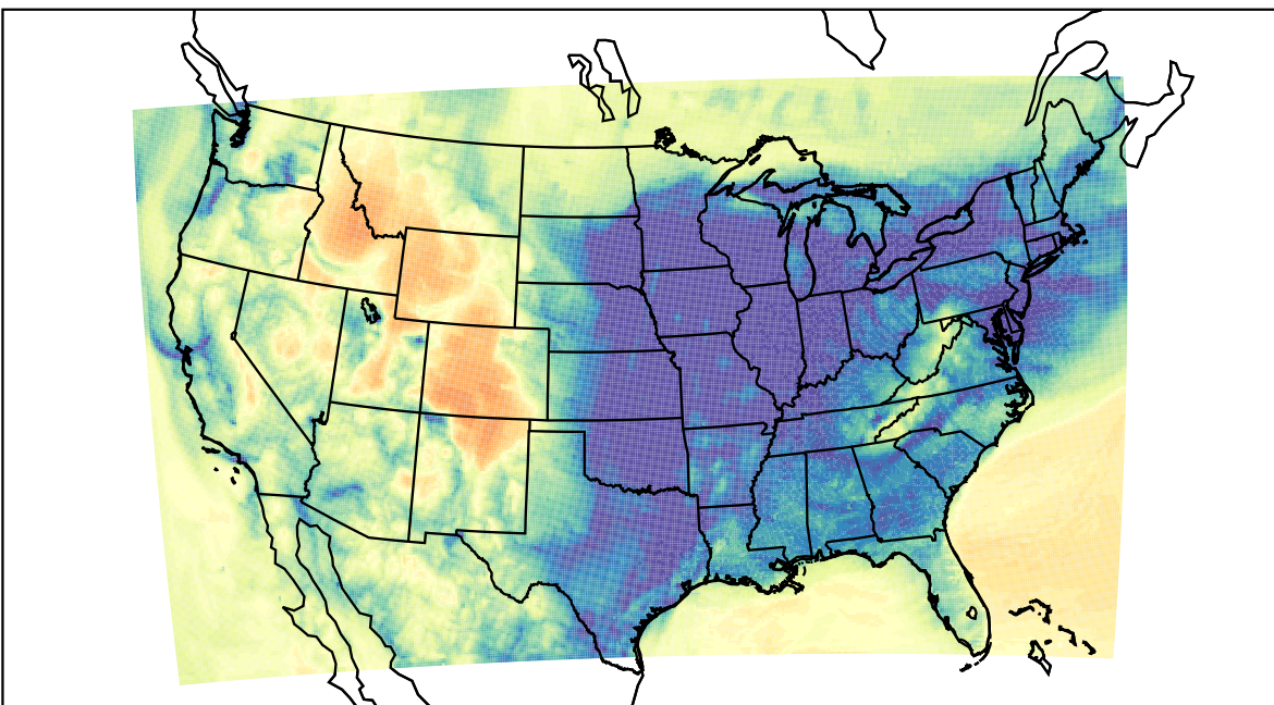
WRF (2023-12-16_07:00:00)
