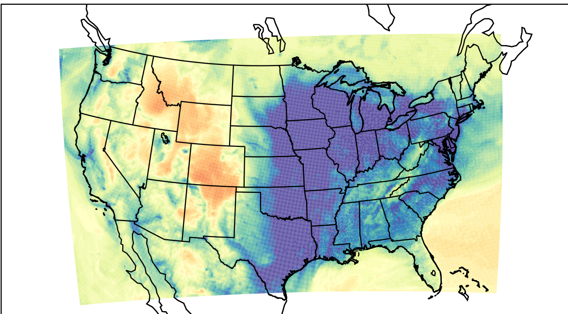
WRF (2023-12-16_14:00:00)
