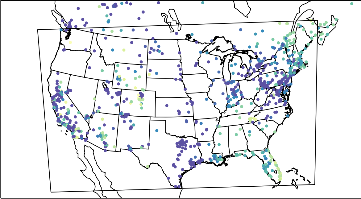
AirNOW (2023-12-16_14:00:00)
