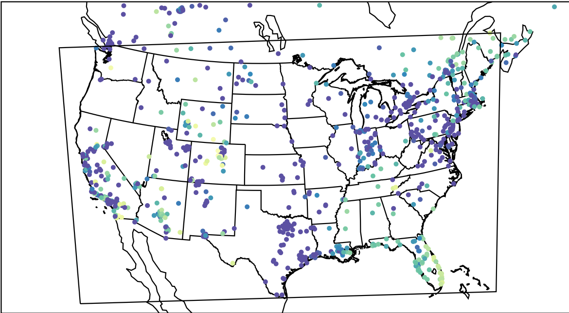
AirNOW (2023-12-16_12:00:00)
