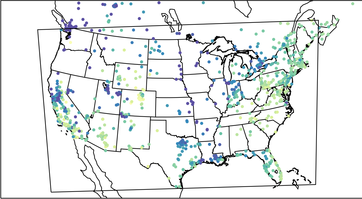
AirNOW (2023-12-16_19:00:00)
