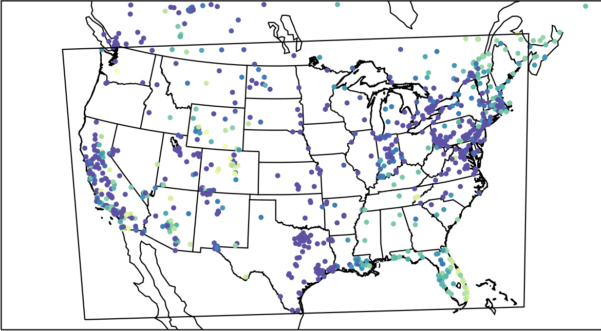
AirNOW (2023-12-16_13:00:00)
