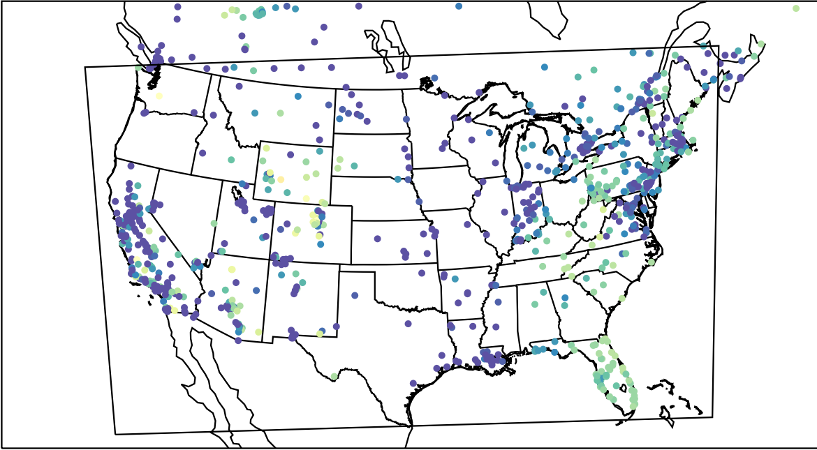
AirNOW (2023-12-17_04:00:00)
