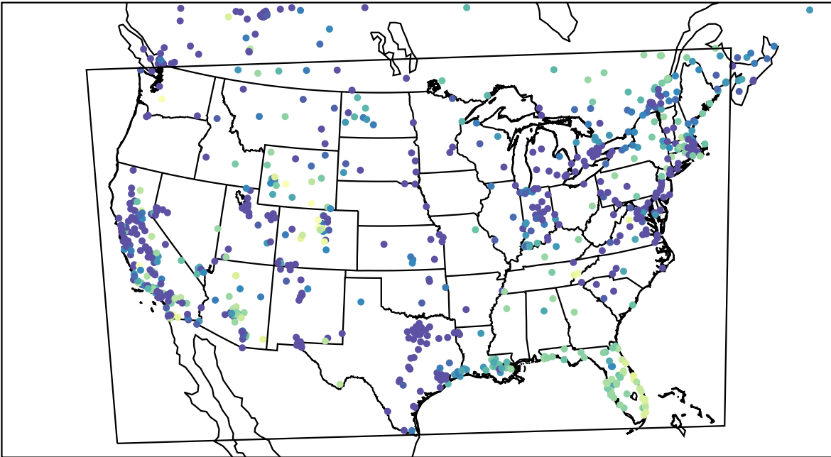
AirNOW (2023-12-16_06:00:00)
