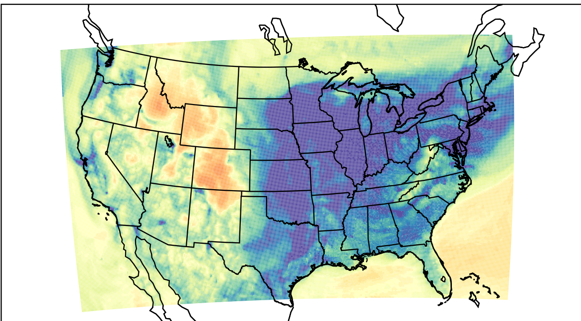
WRF (2023-12-16_04:00:00)
