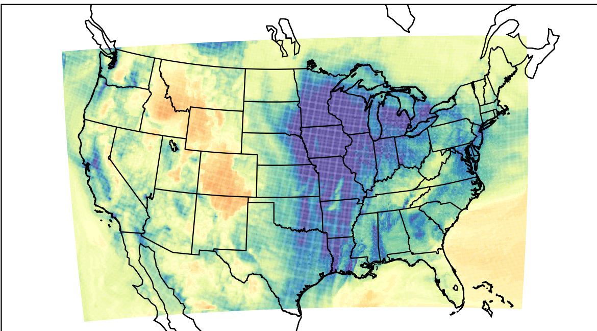
WRF (2023-12-16_17:00:00)
