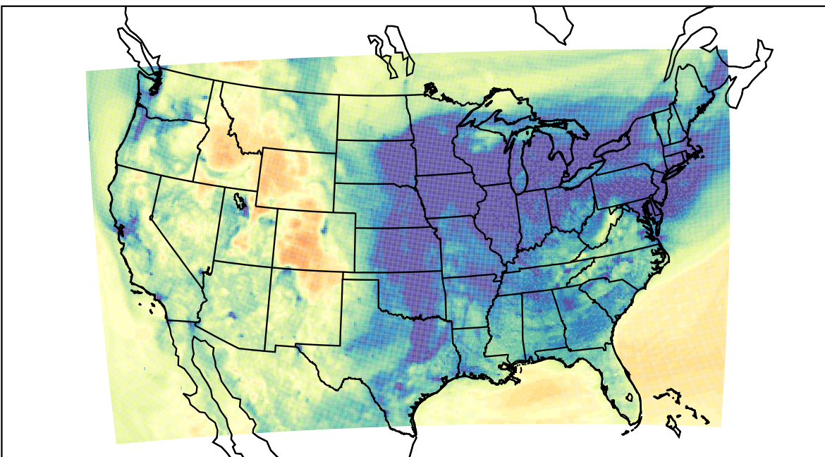
WRF (2023-12-16_01:00:00)
