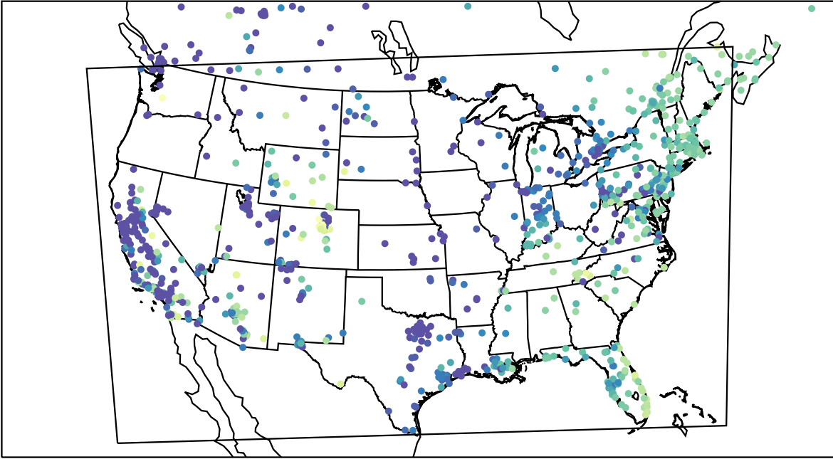
AirNOW (2023-12-16_16:00:00)
