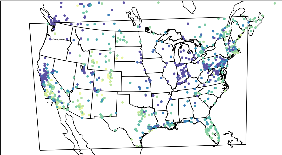
AirNOW (2023-12-17_23:00:00)
