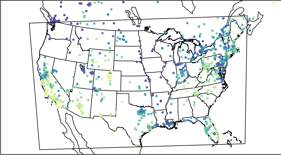
AirNOW (2023-12-16_21:00:00)
