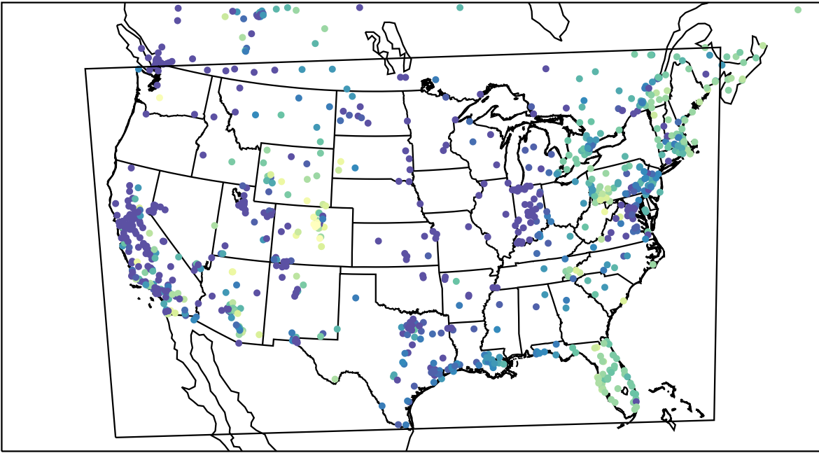
AirNOW (2023-12-17_16:00:00)
