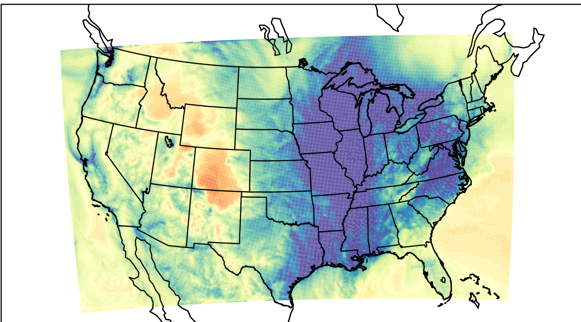
WRF (2023-12-17_07:00:00)
