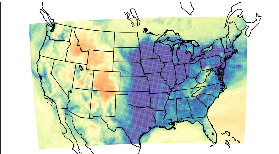
WRF (2023-12-16_11:00:00)
