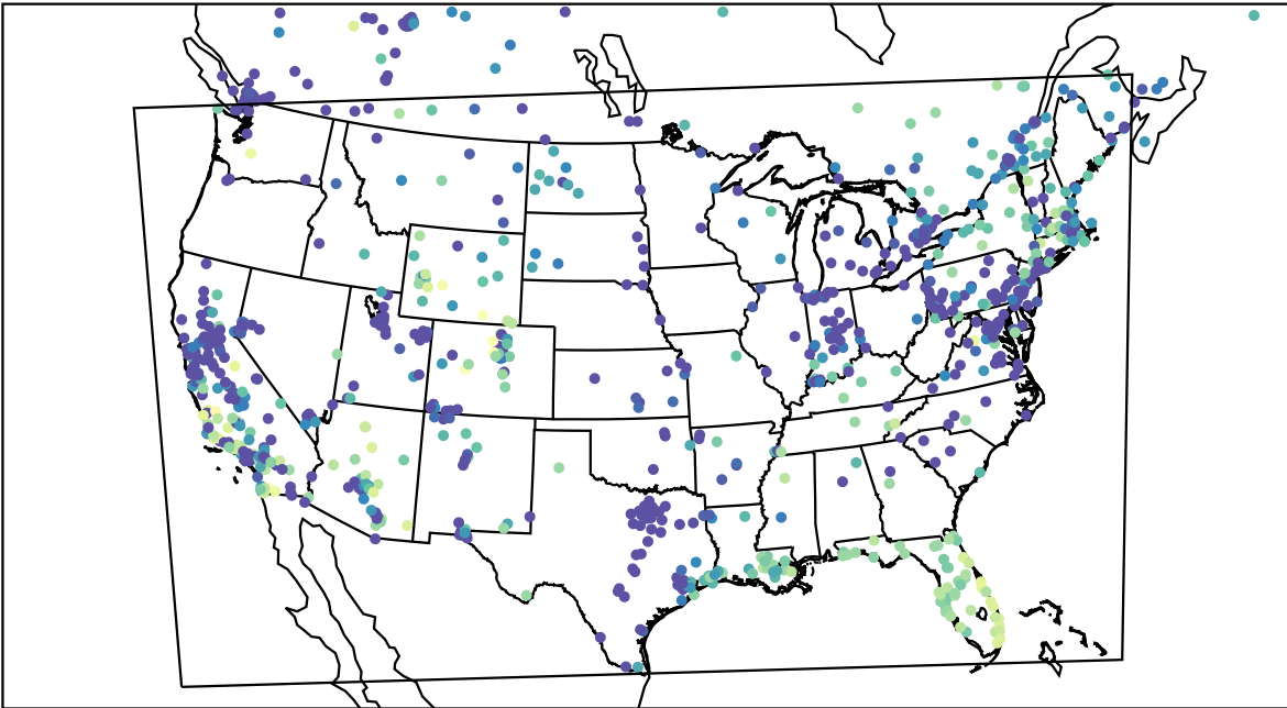
AirNOW (2023-12-16_01:00:00)
