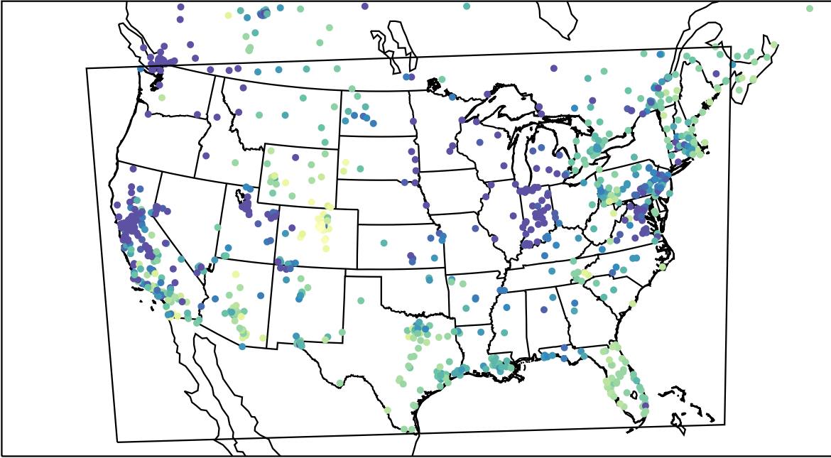
AirNOW (2023-12-17_18:00:00)
