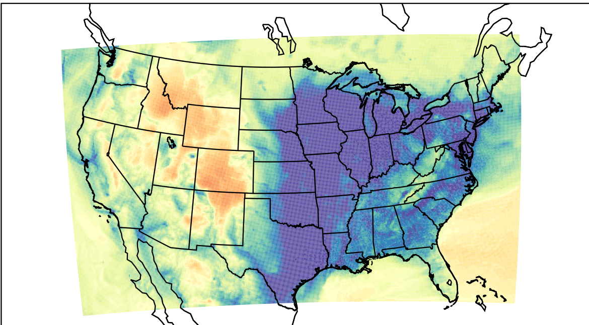
WRF (2023-12-16_13:00:00)
