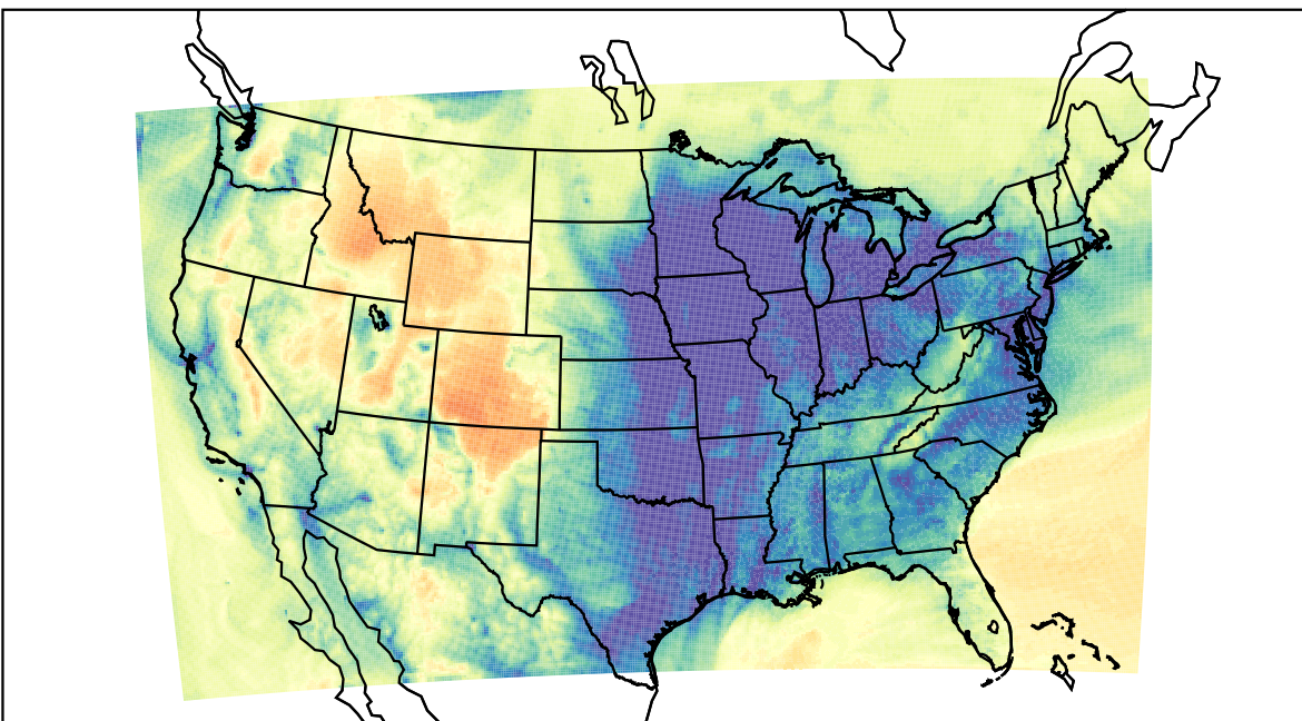
WRF (2023-12-16_15:00:00)
