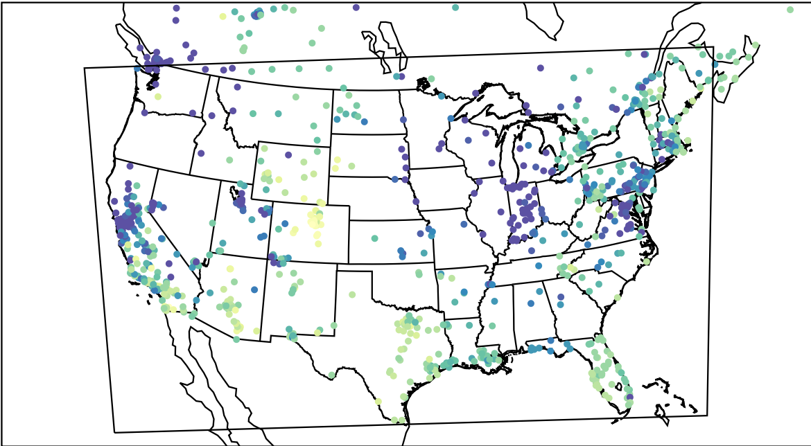
AirNOW (2023-12-17_19:00:00)
