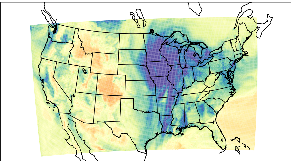
WRF (2023-12-16_19:00:00)
