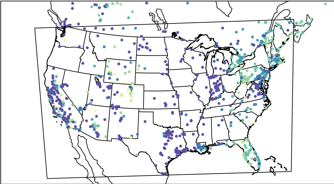
AirNOW (2023-12-17_14:00:00)
