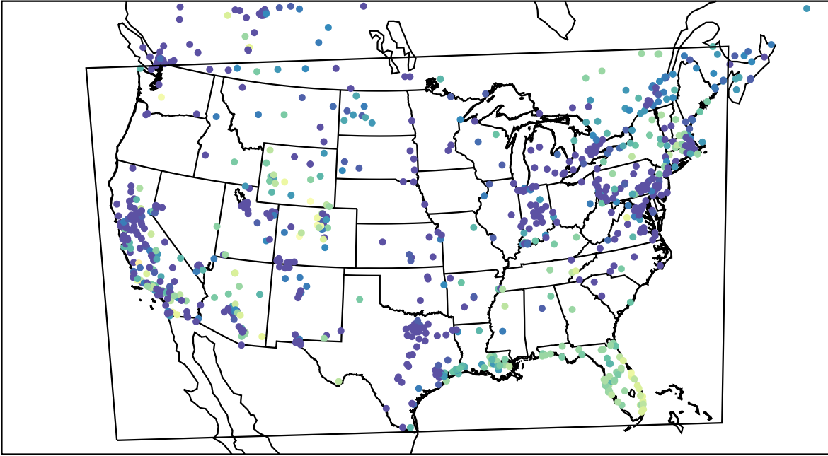
AirNOW (2023-12-16_03:00:00)
