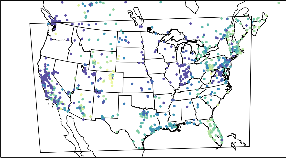
AirNOW (2023-12-17_17:00:00)
