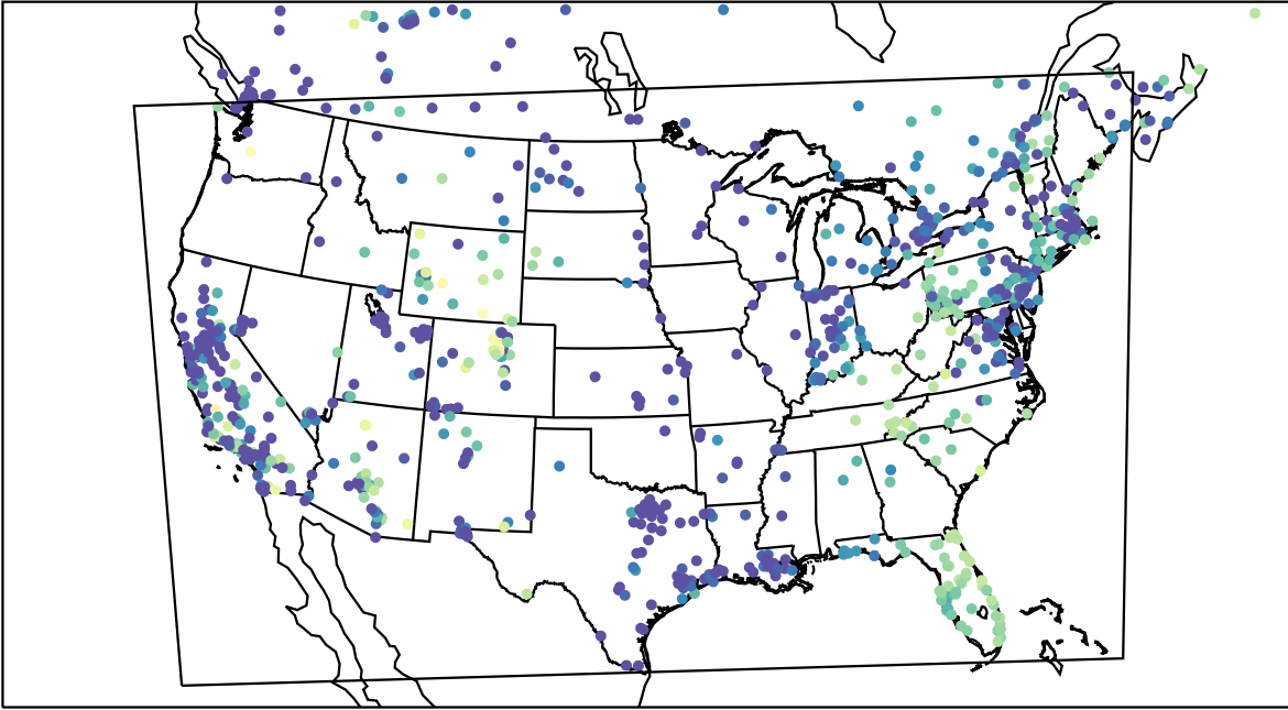
AirNOW (2023-12-17_03:00:00)
