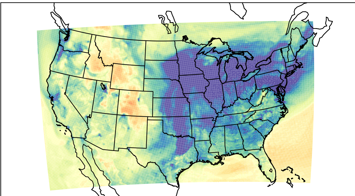
WRF (2023-12-16_00:00:00)
