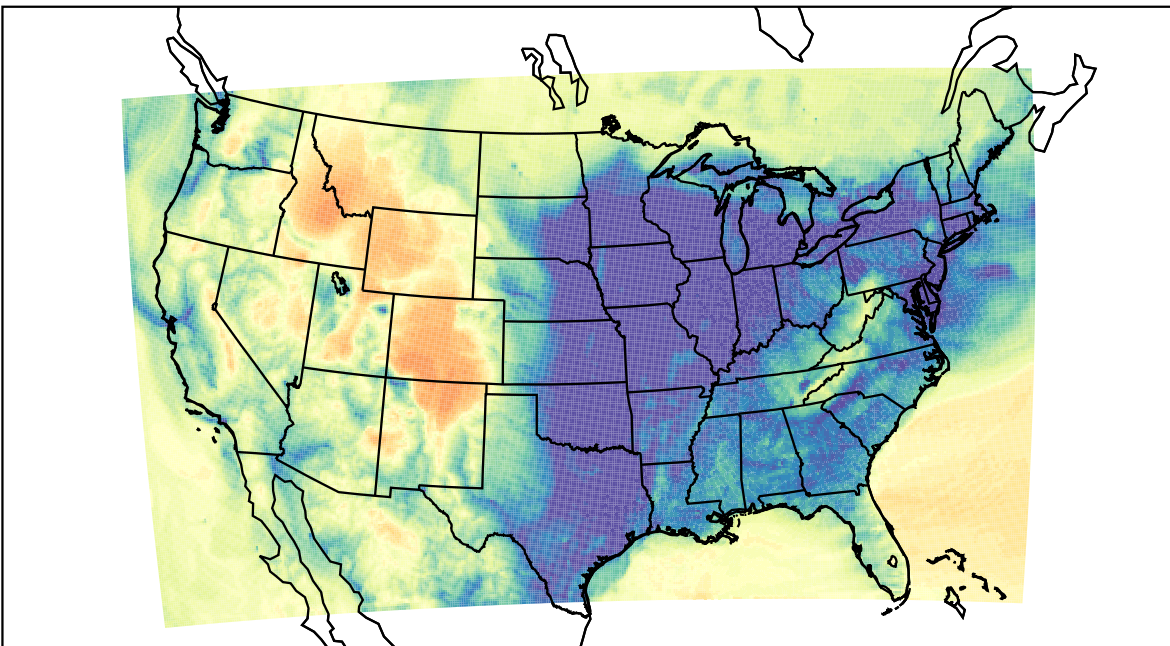
WRF (2023-12-16_10:00:00)
