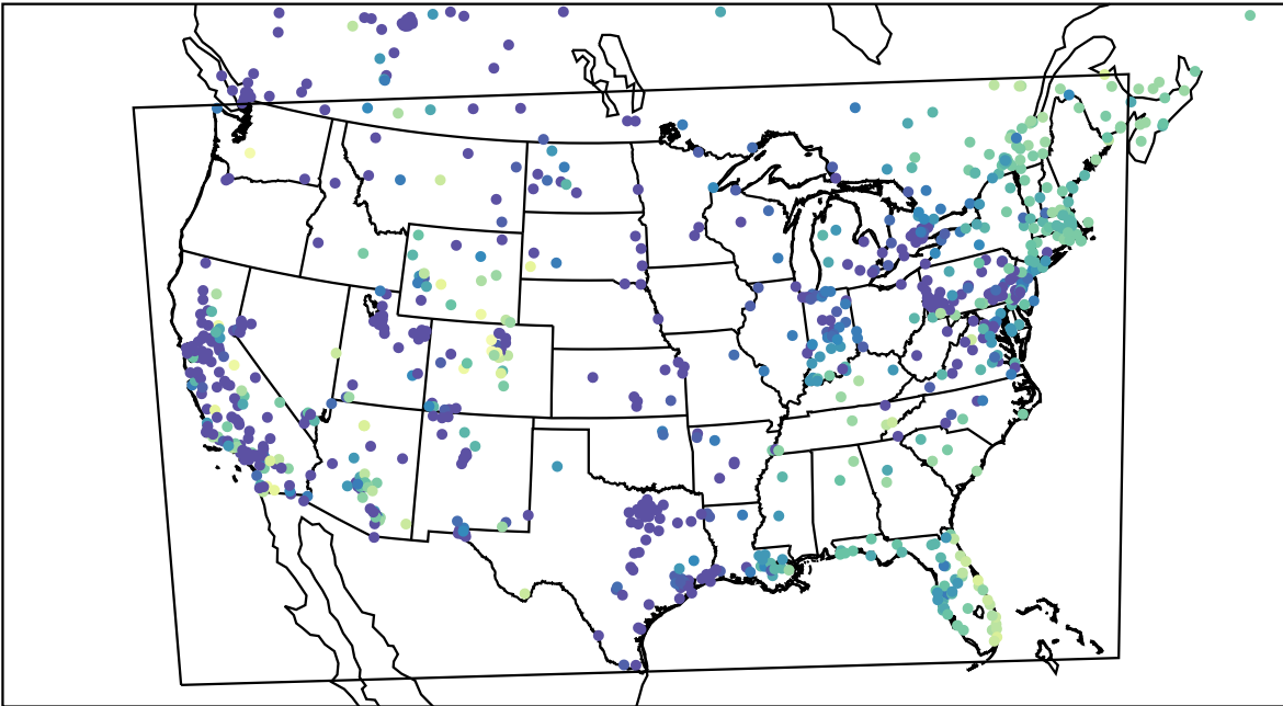
AirNOW (2023-12-16_15:00:00)
