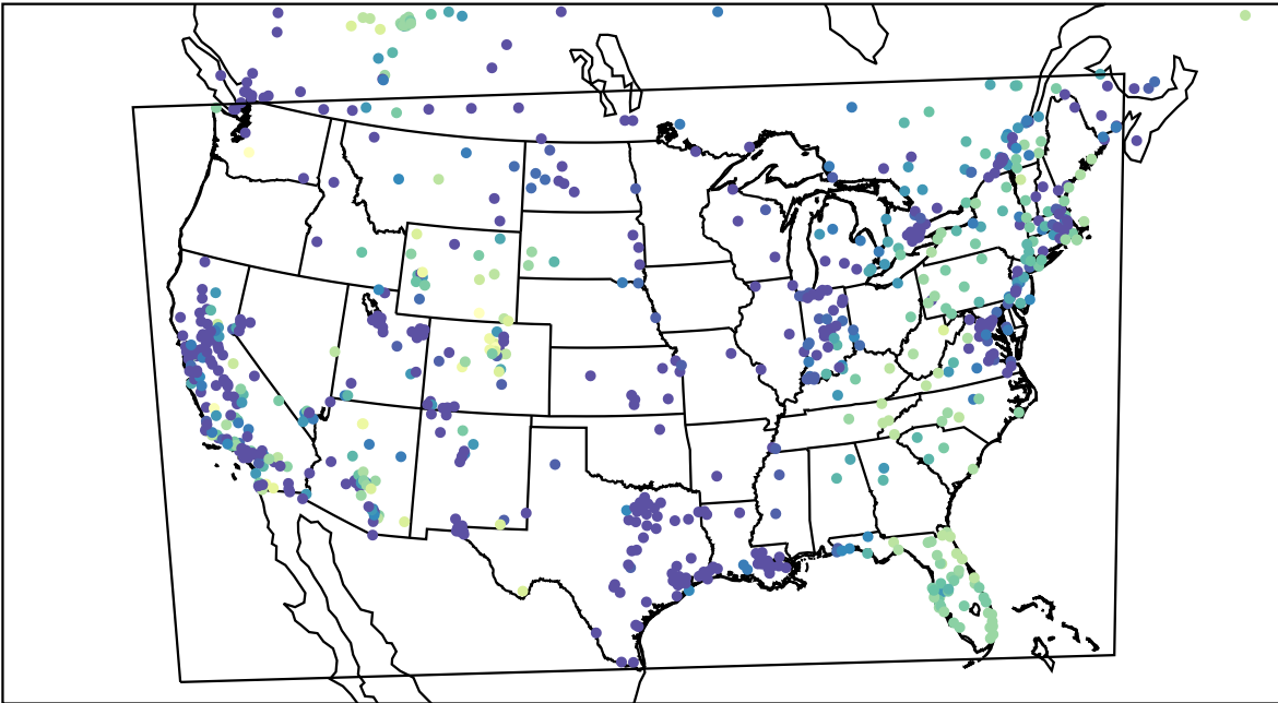
AirNOW (2023-12-17_06:00:00)
