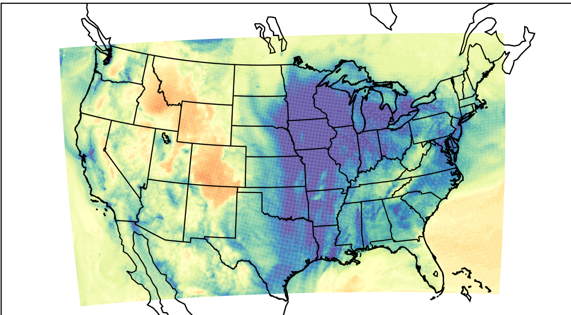
WRF (2023-12-16_16:00:00)
