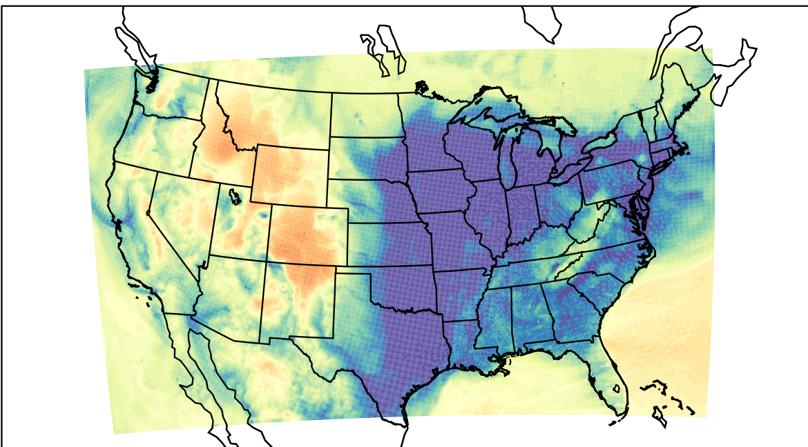
WRF (2023-12-16_12:00:00)
