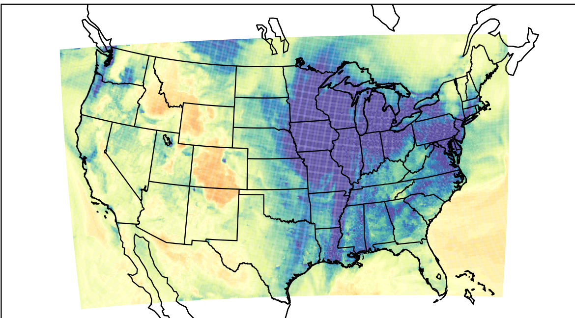
WRF (2023-12-16_23:00:00)
