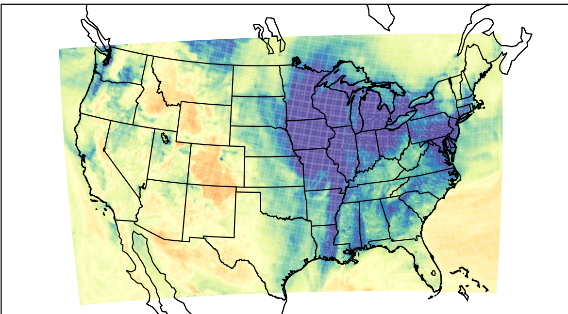
WRF (2023-12-16_22:00:00)
