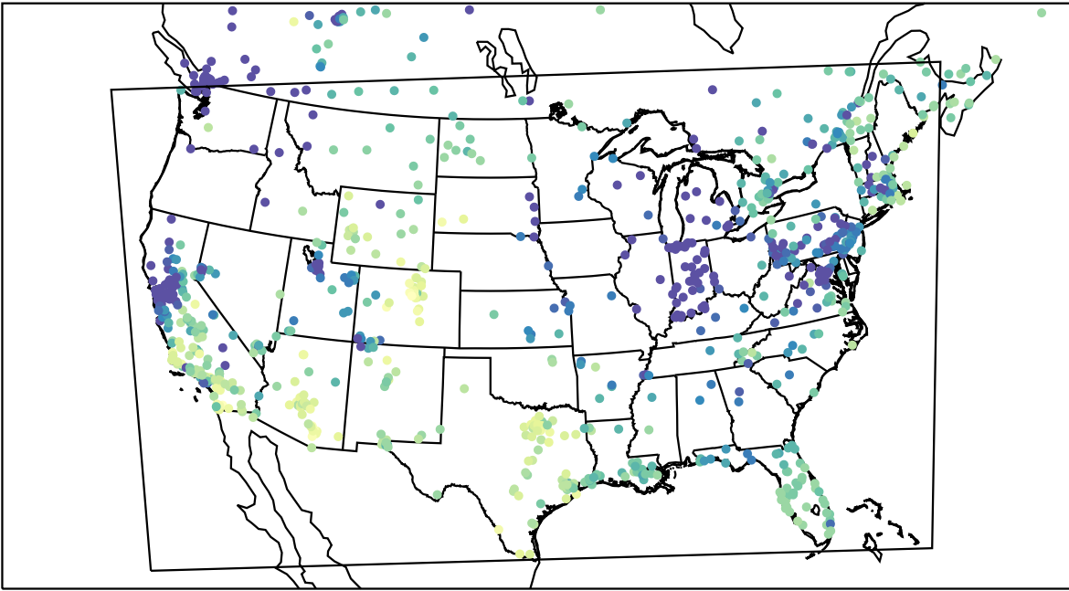
AirNOW (2023-12-17_22:00:00)
