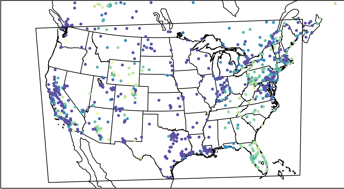
AirNOW (2023-12-17_05:00:00)
