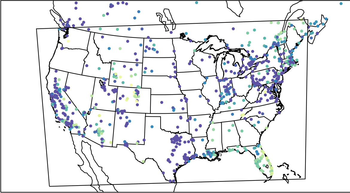
AirNOW (2023-12-16_10:00:00)
