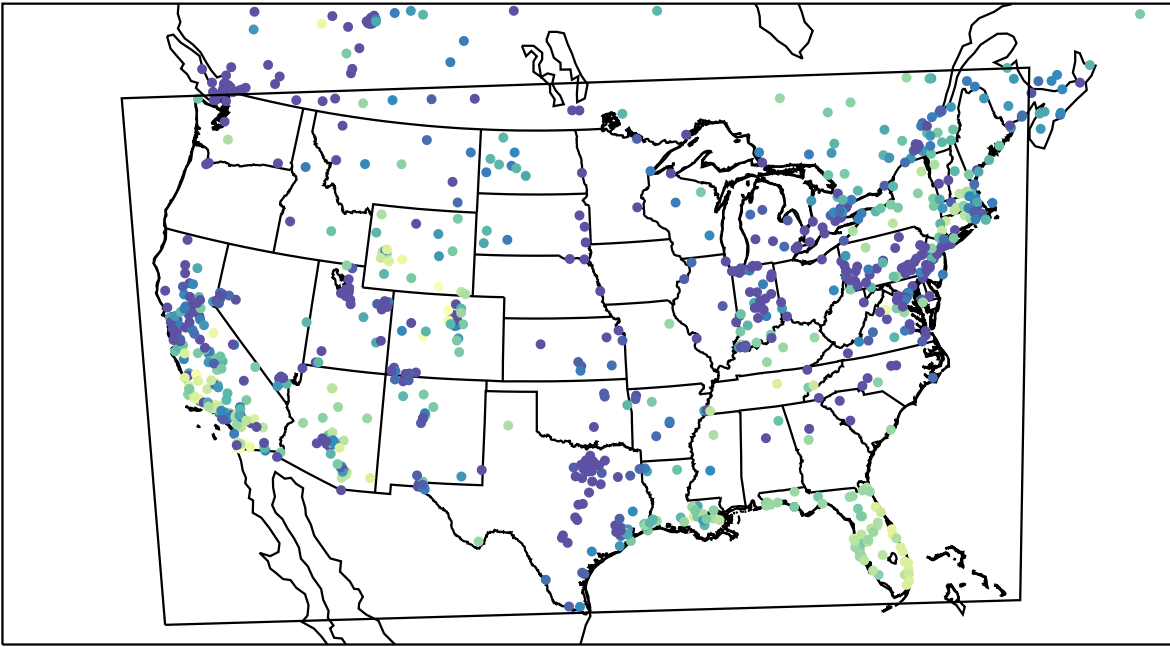
AirNOW (2023-12-16_00:00:00)
