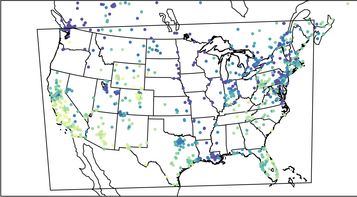
AirNOW (2023-12-16_22:00:00)
