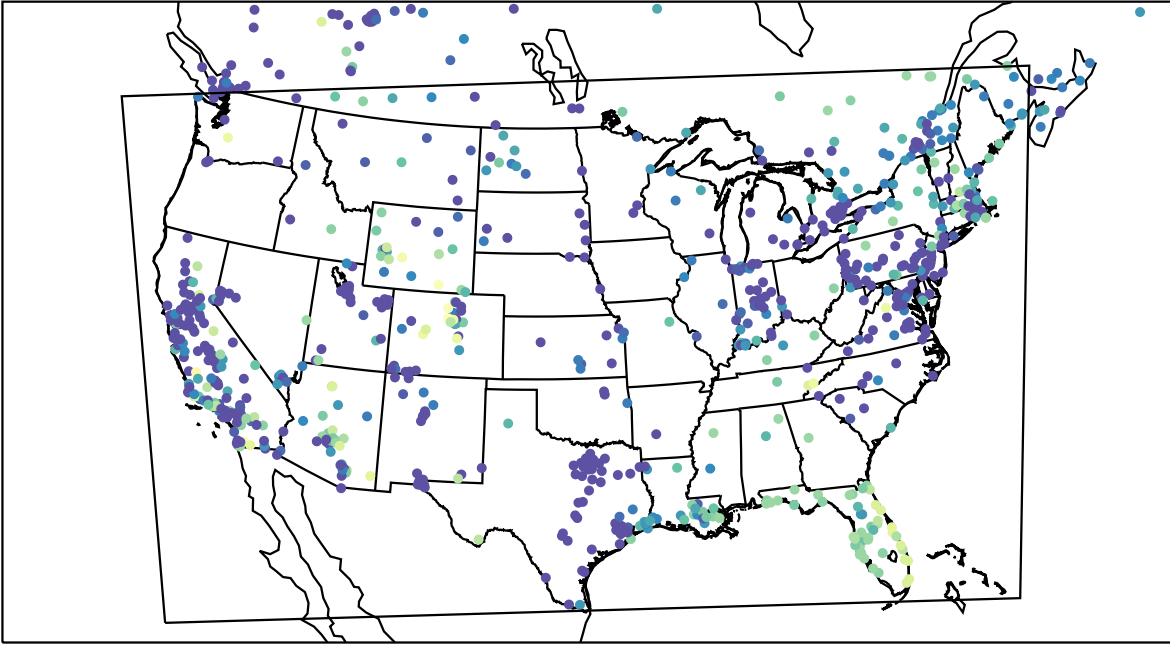
AirNOW (2023-12-16_05:00:00)
