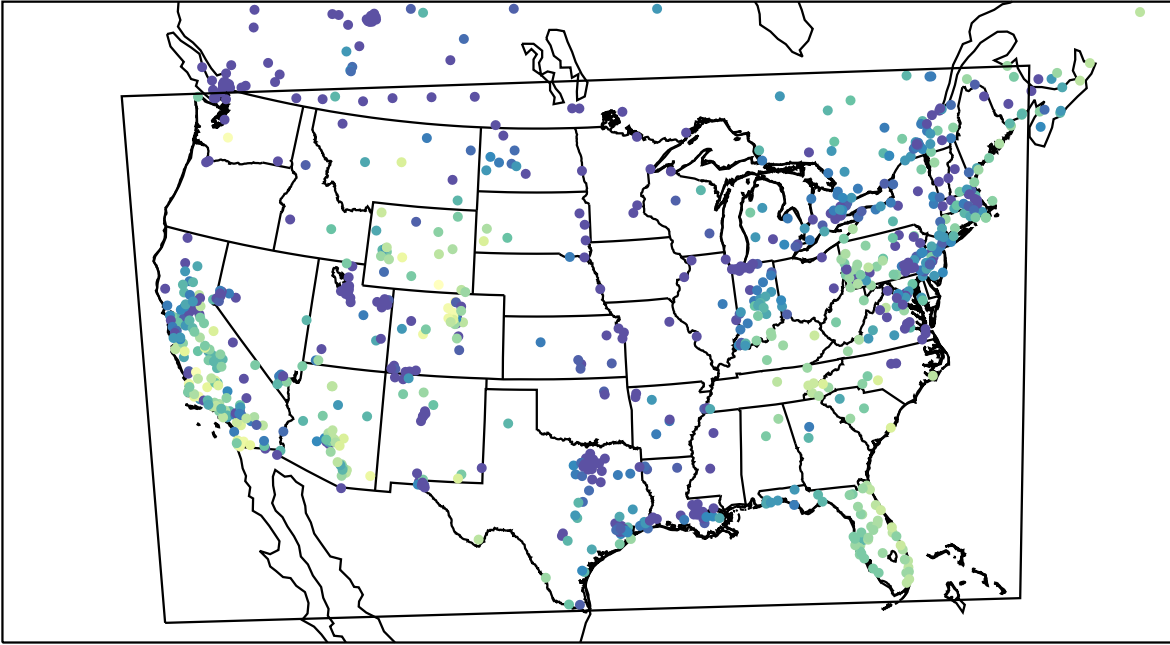
AirNOW (2023-12-17_00:00:00)
