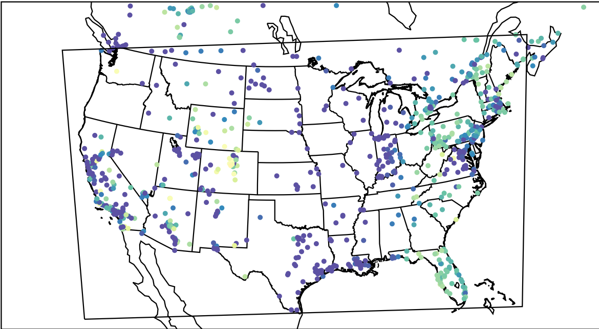
AirNOW (2023-12-17_12:00:00)
