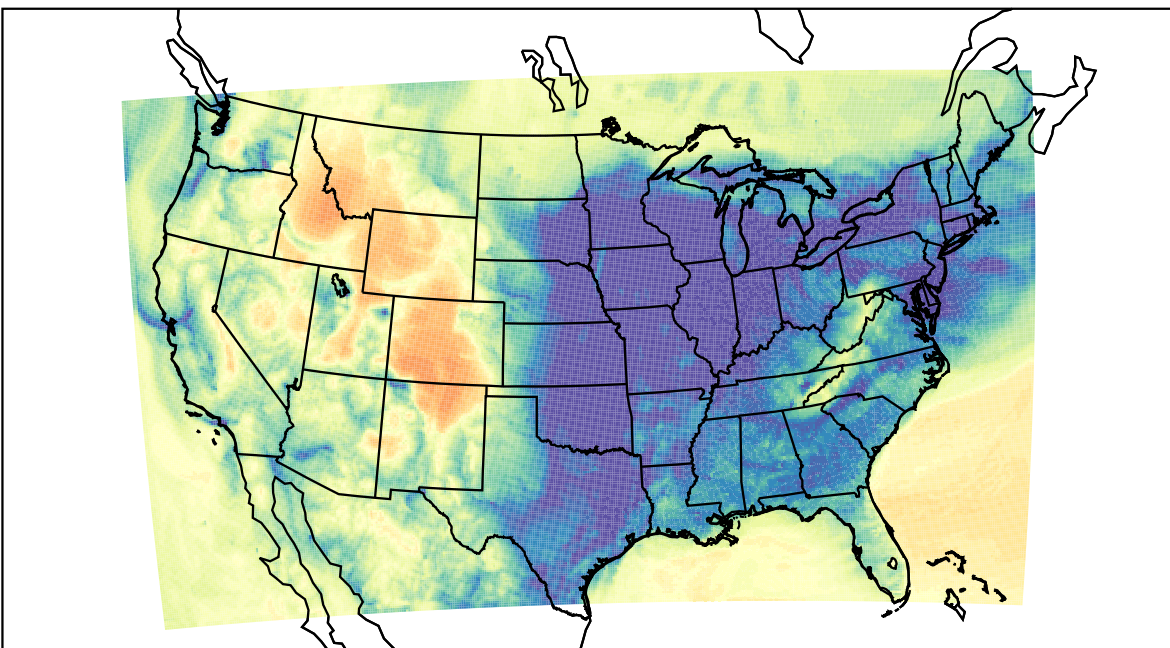
WRF (2023-12-16_08:00:00)
