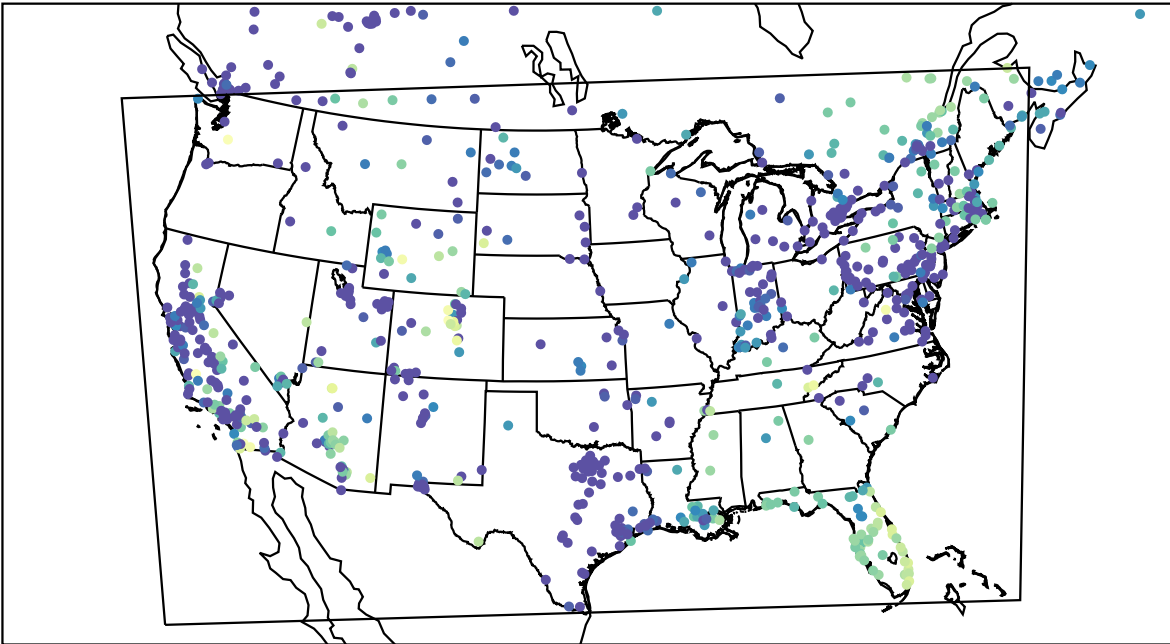
AirNOW (2023-12-16_09:00:00)
