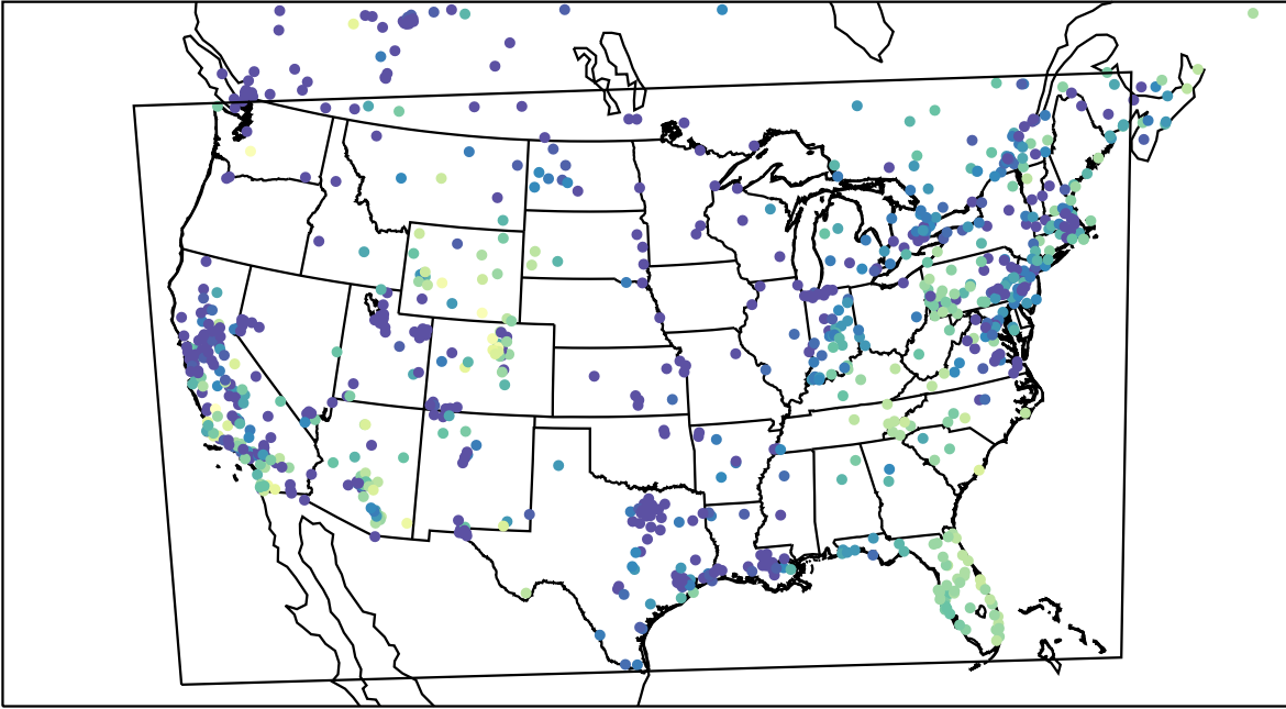
AirNOW (2023-12-17_01:00:00)
