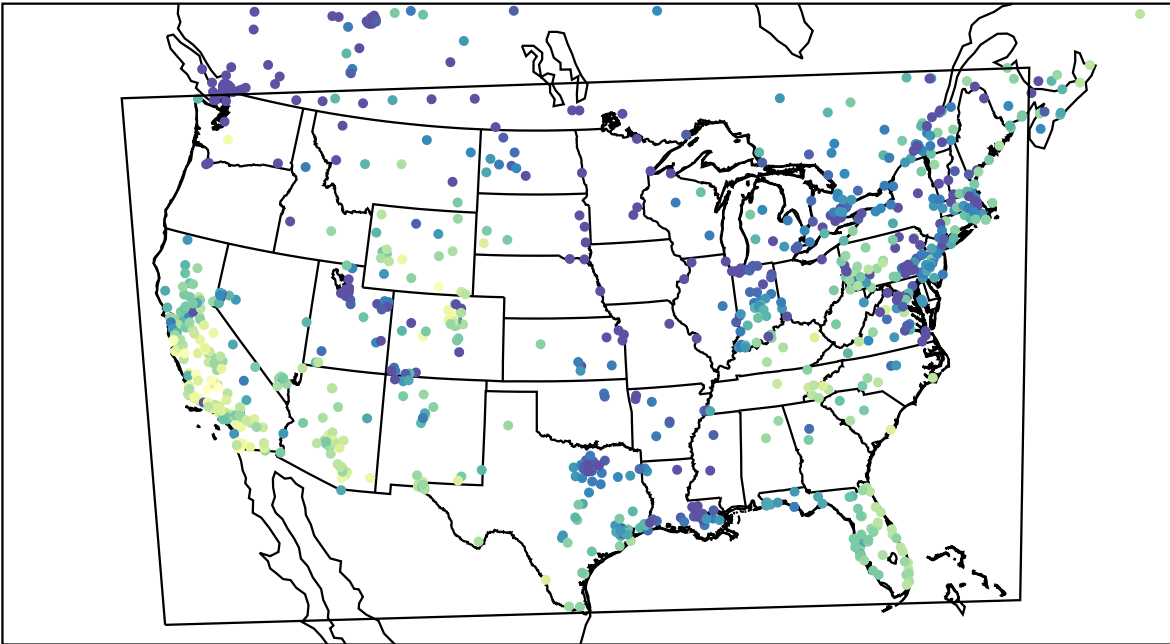
AirNOW (2023-12-16_23:00:00)
