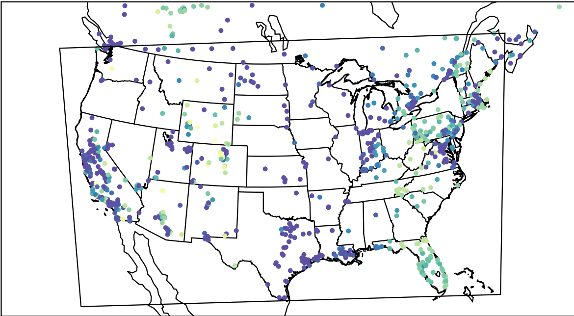
AirNOW (2023-12-17_08:00:00)
