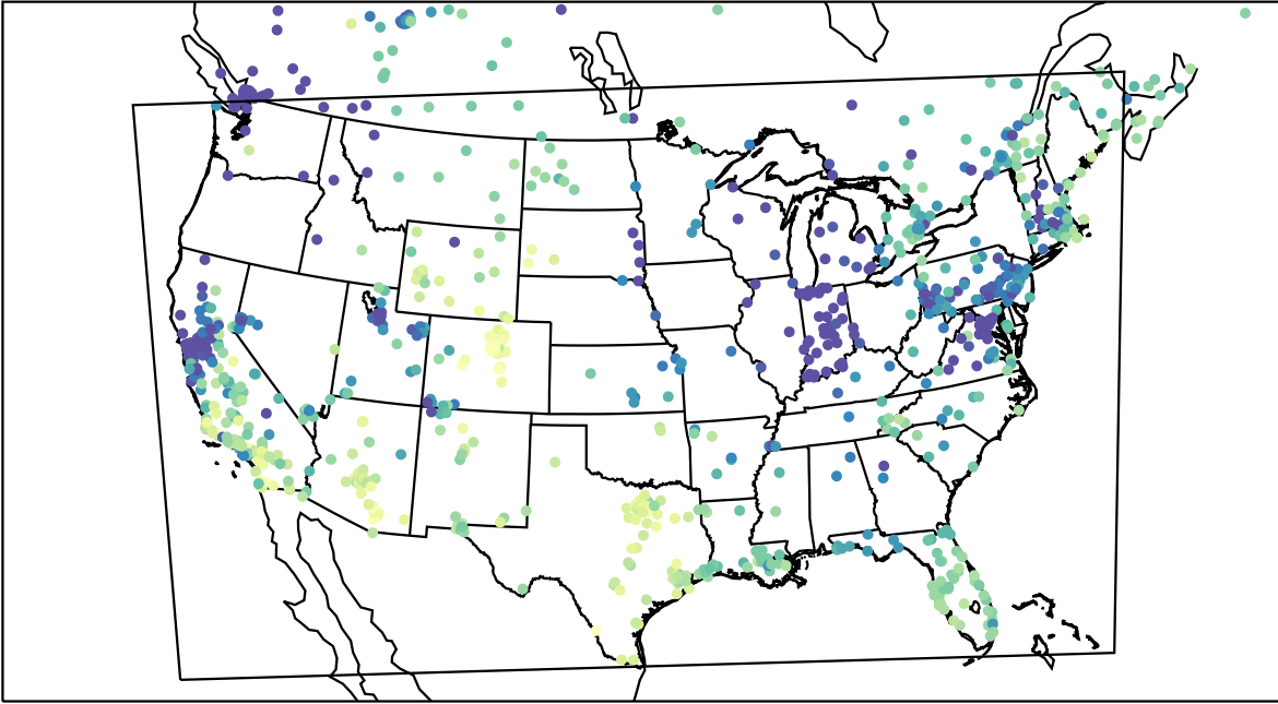
AirNOW (2023-12-17_21:00:00)
