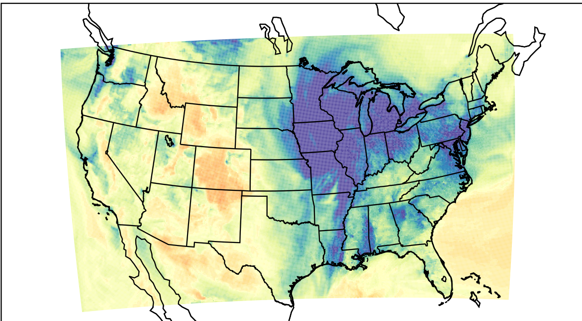
WRF (2023-12-16_21:00:00)
