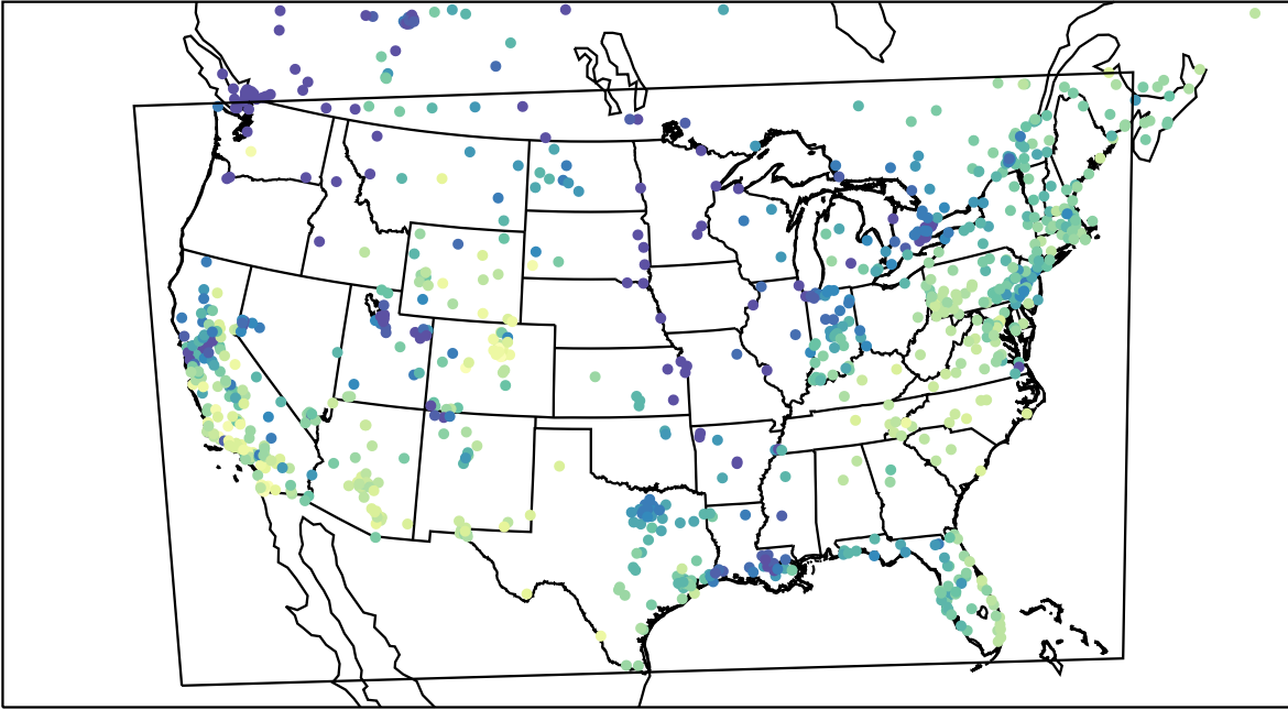
AirNOW (2023-12-16_20:00:00)
