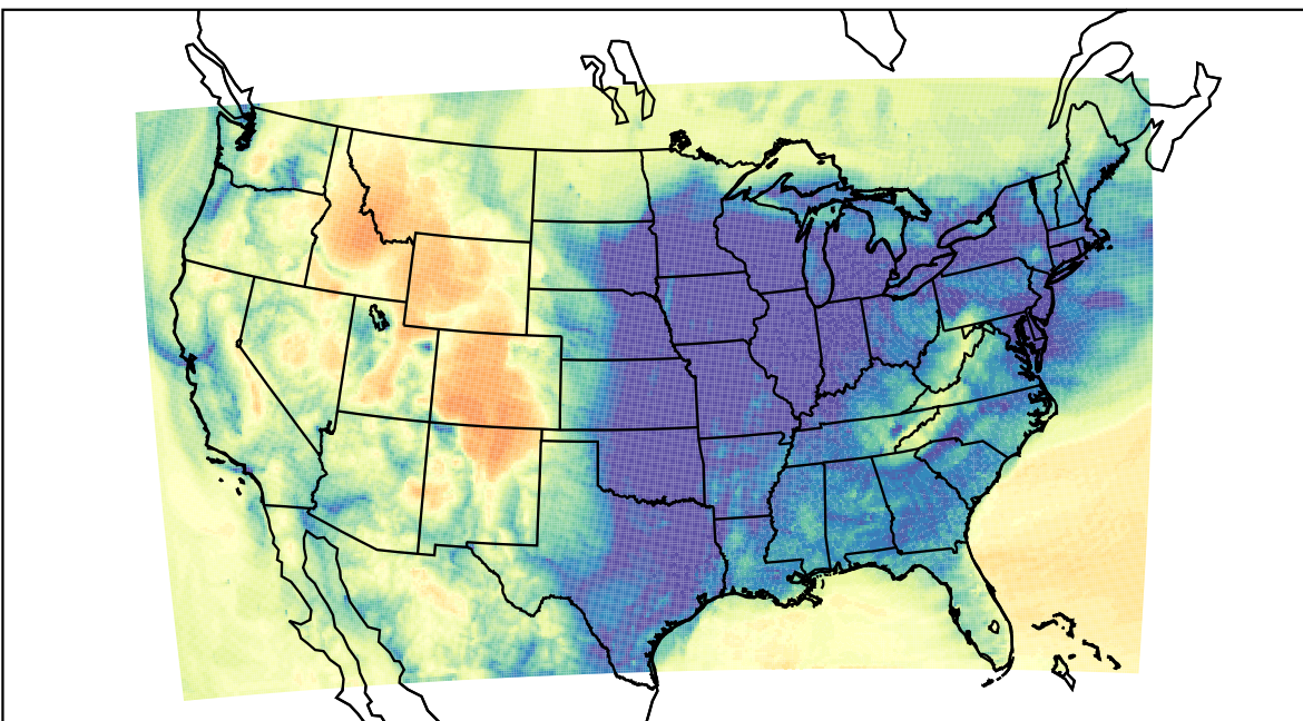
WRF (2023-12-16_09:00:00)
