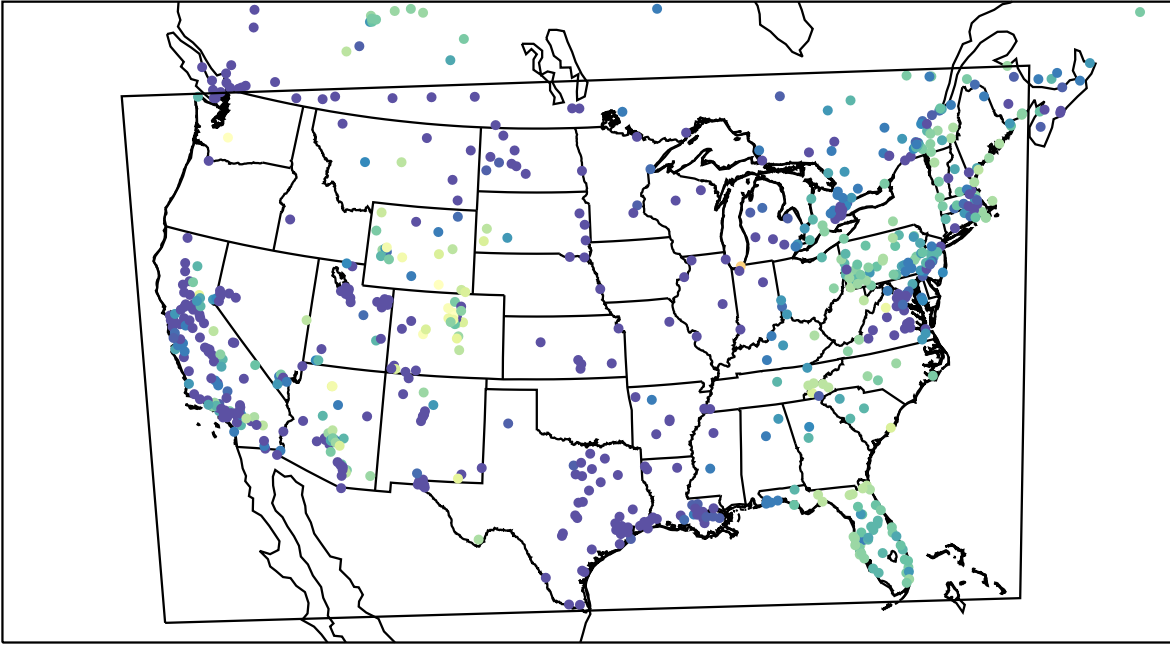
AirNOW (2023-12-17_10:00:00)
