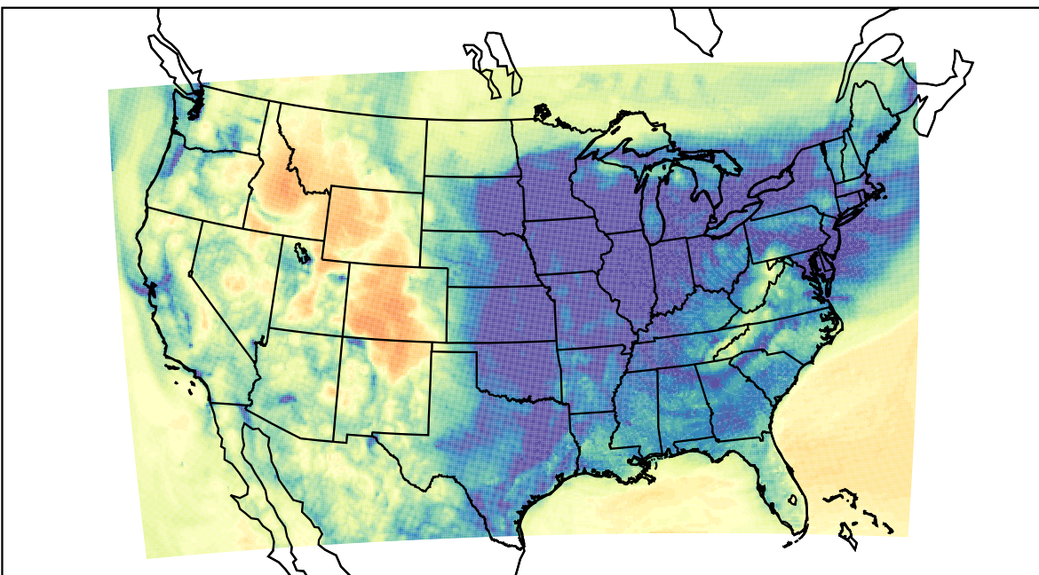
WRF (2023-12-16_05:00:00)
