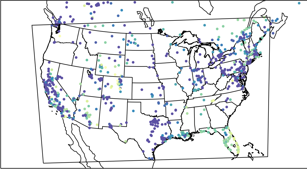
AirNOW (2023-12-16_07:00:00)
