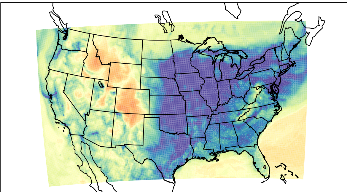
WRF (2023-12-16_06:00:00)
