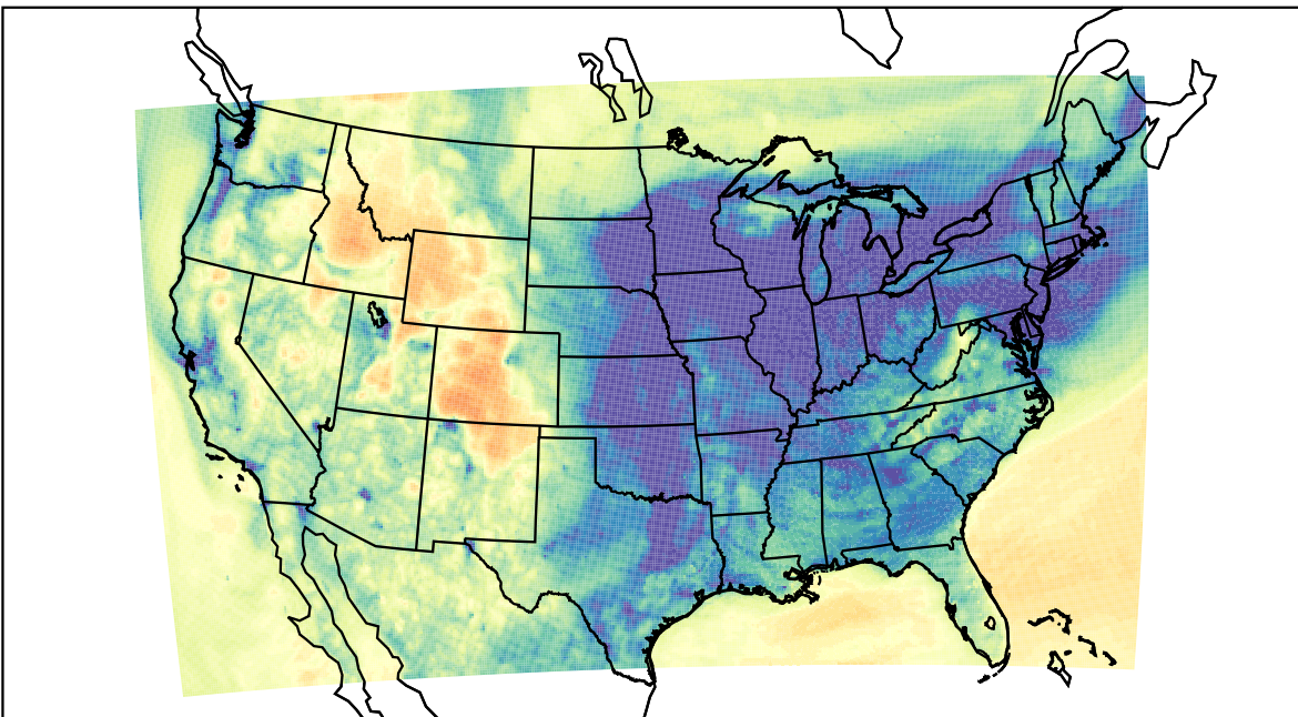
WRF (2023-12-16_02:00:00)
