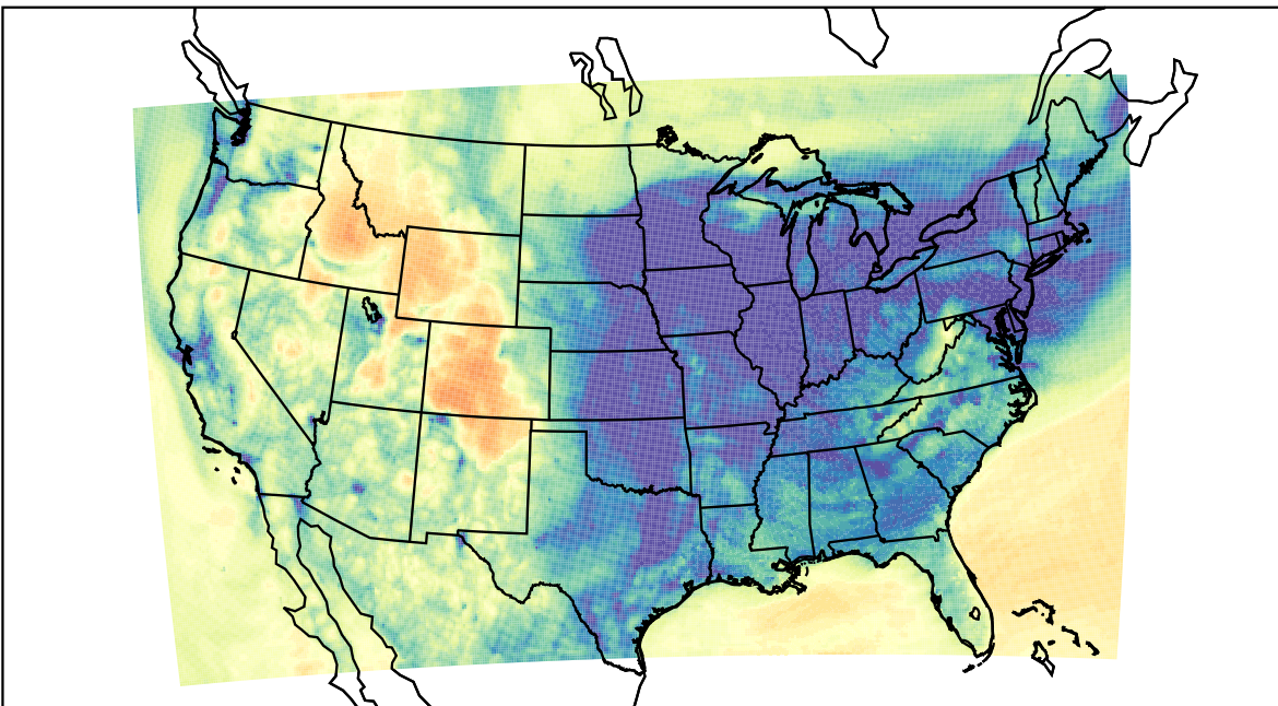
WRF (2023-12-16_03:00:00)
