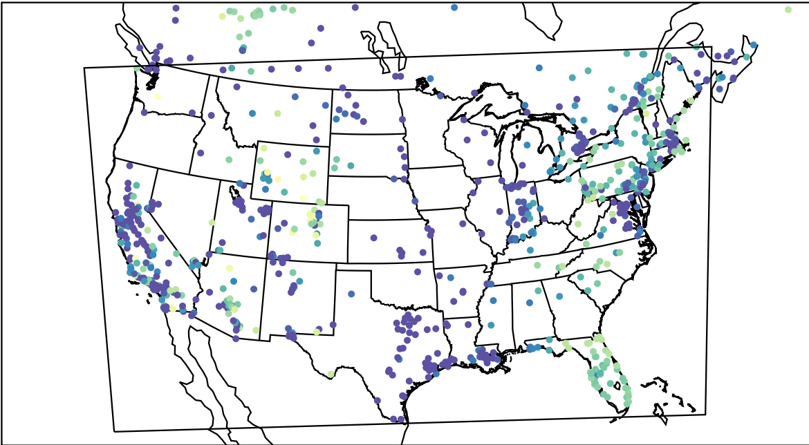
AirNOW (2023-12-17_07:00:00)
