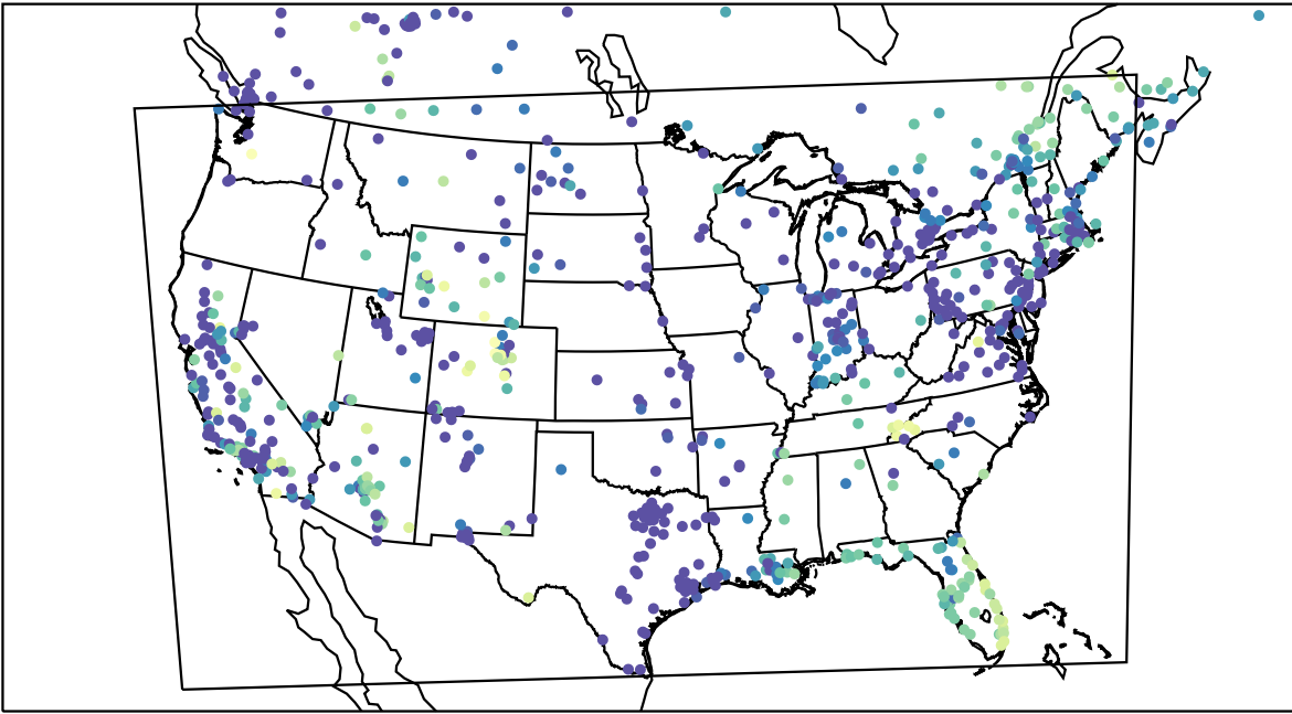
AirNOW (2023-12-16_11:00:00)
