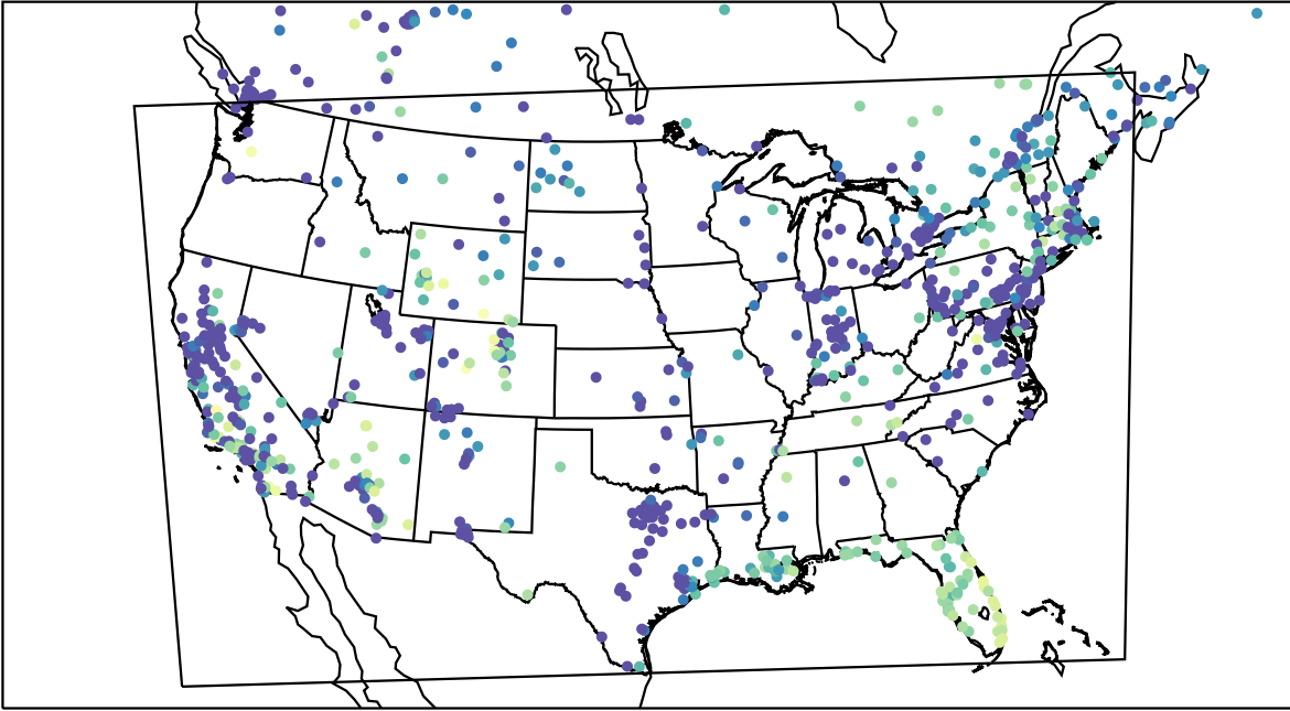
AirNOW (2023-12-16_02:00:00)
