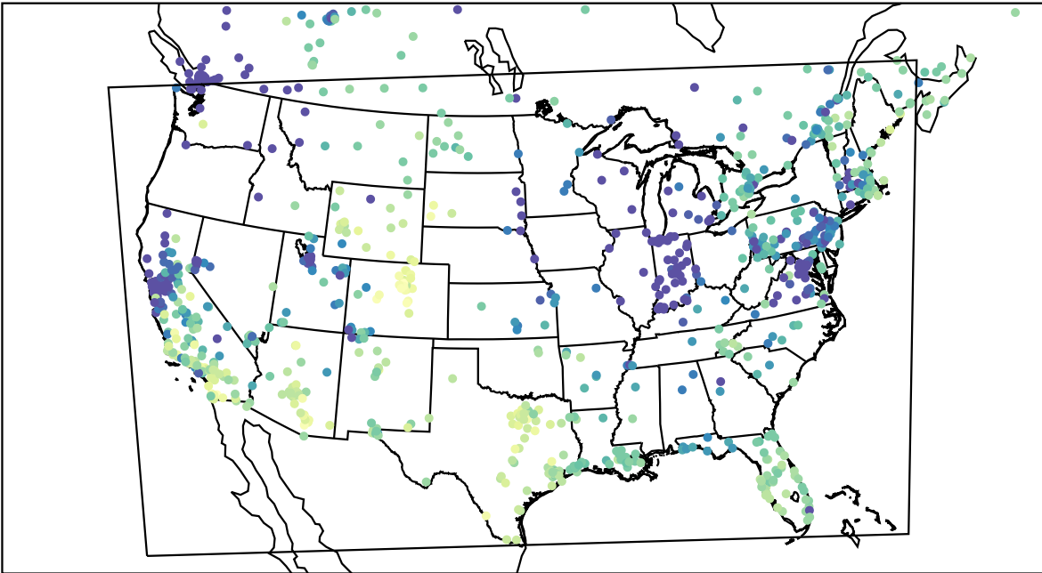
AirNOW (2023-12-17_20:00:00)
