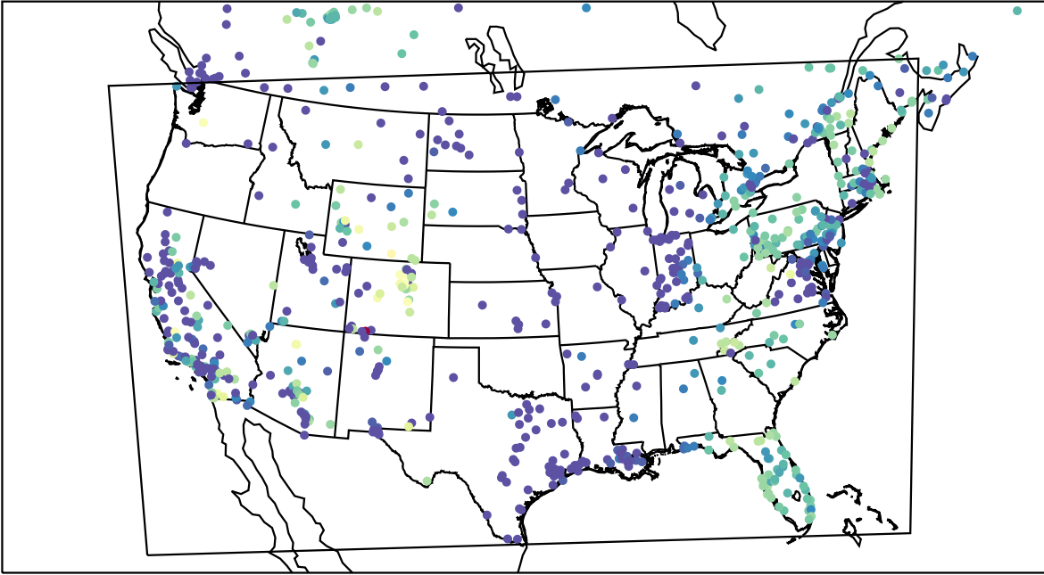
AirNOW (2023-12-17_11:00:00)
