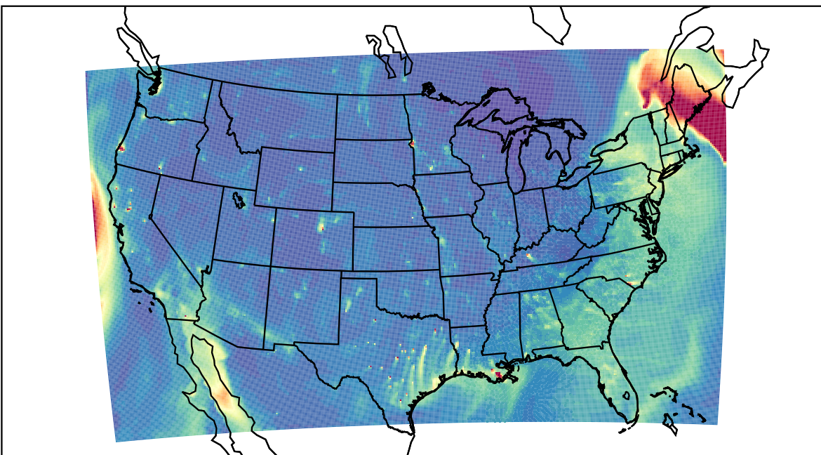
WRF 2023-12-18_23:00:00
