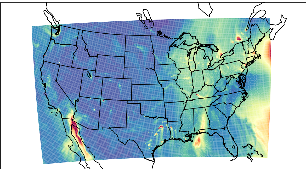
WRF 2023-12-17_20:00:00
