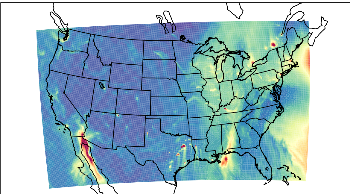
WRF 2023-12-17_19:00:00
