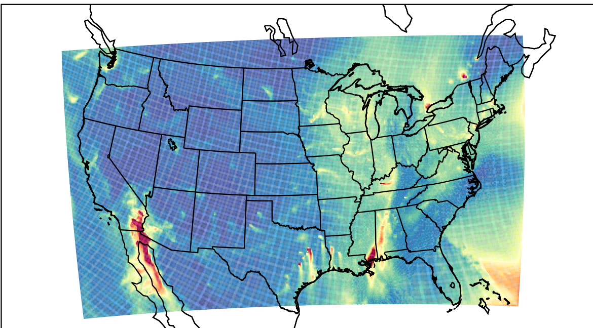
WRF 2023-12-17_14:00:00
