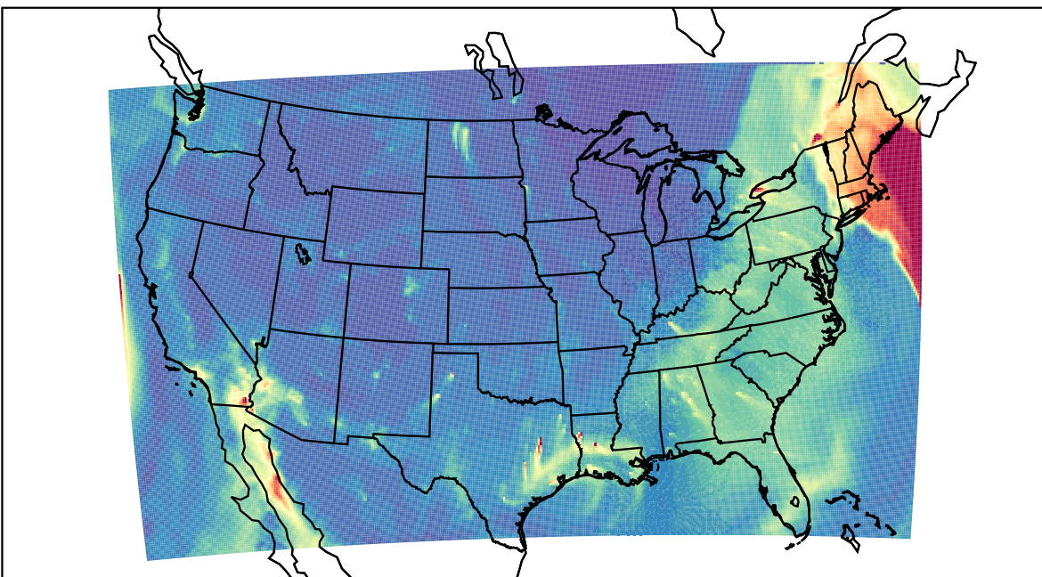
WRF 2023-12-18_16:00:00
