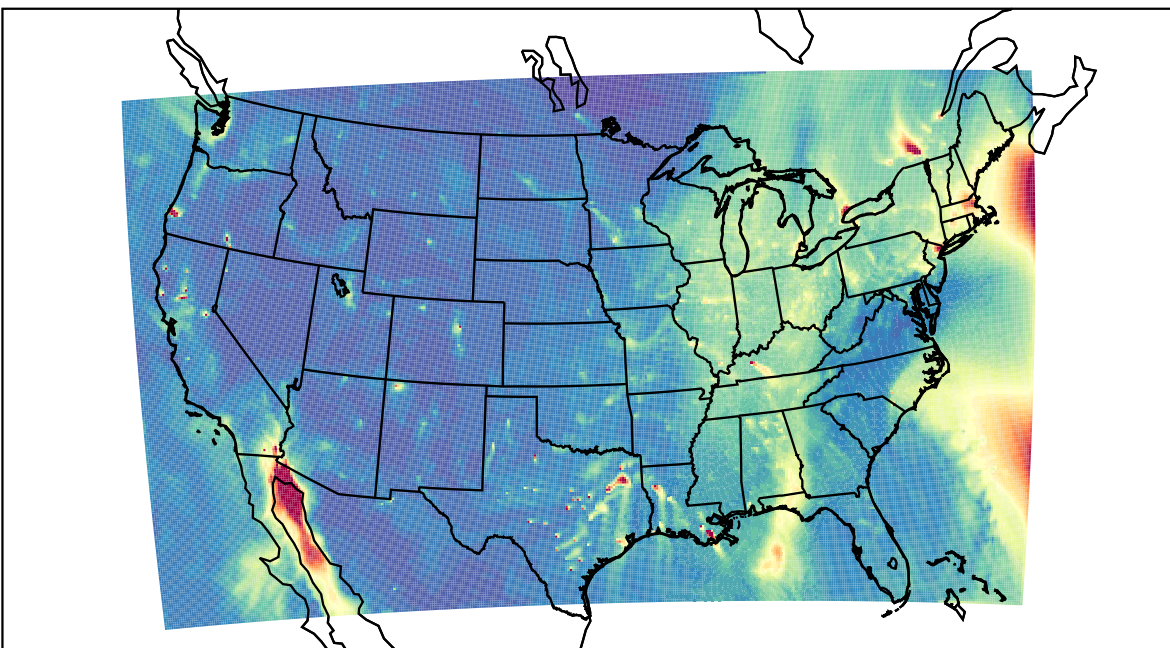
WRF 2023-12-17_23:00:00
