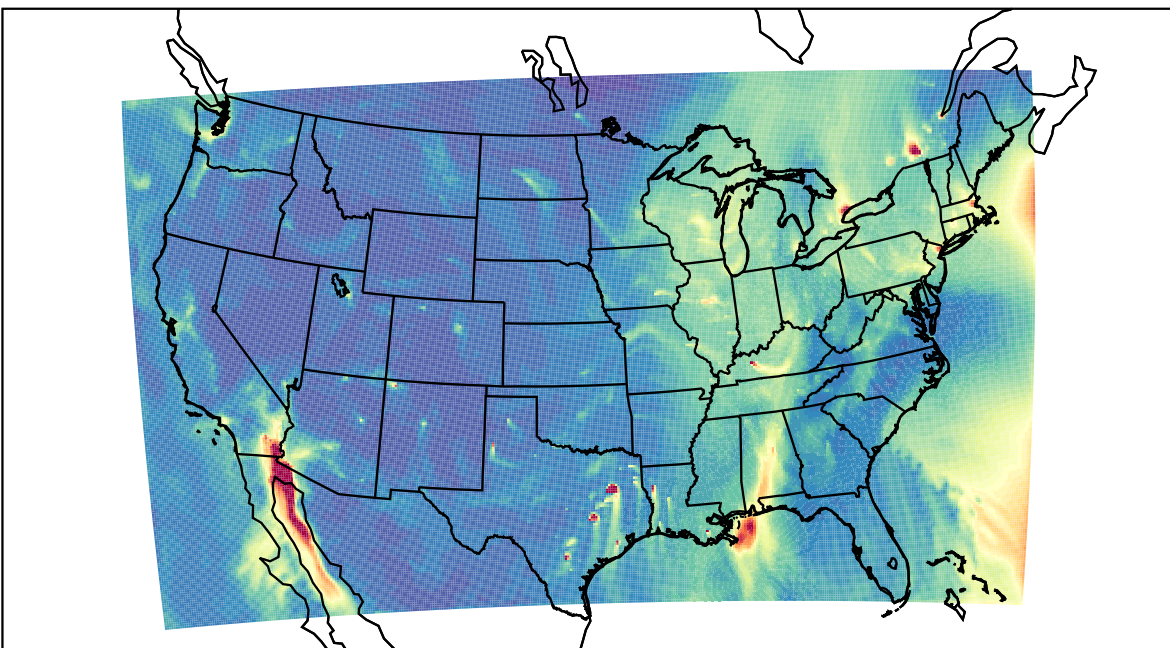
WRF 2023-12-17_18:00:00
