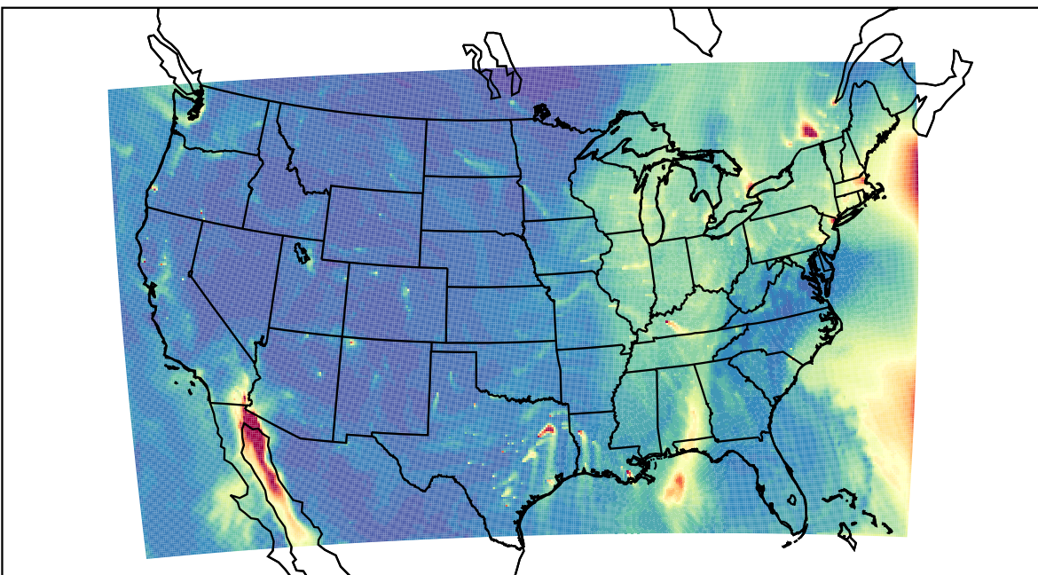
WRF 2023-12-17_21:00:00
