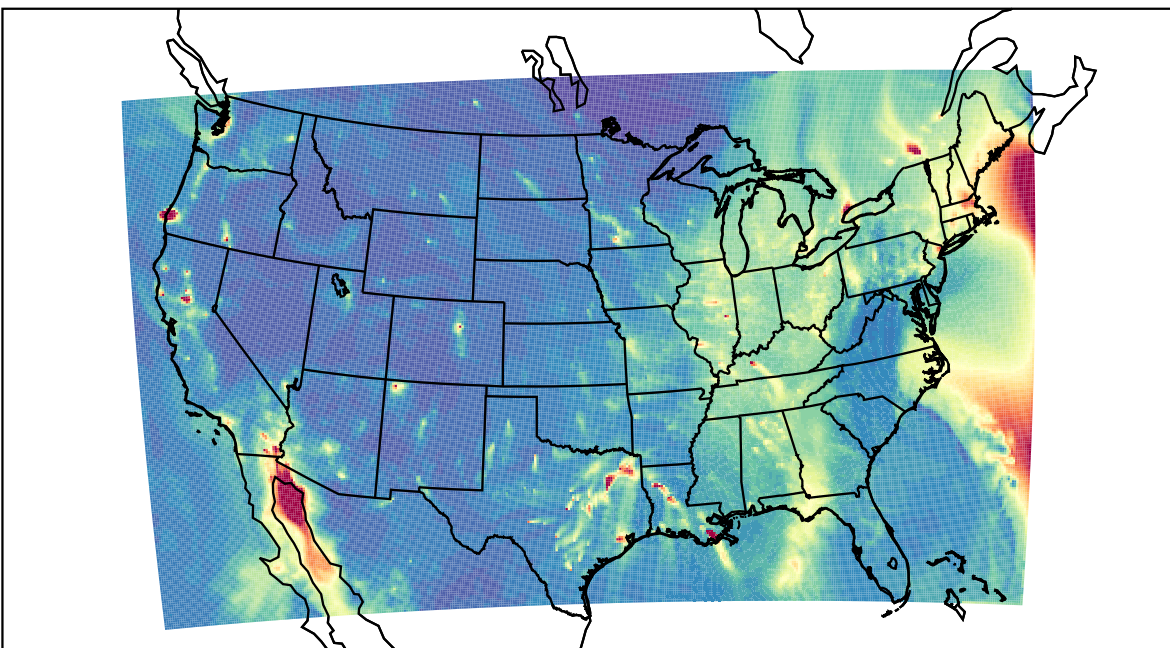
WRF 2023-12-18_02:00:00
