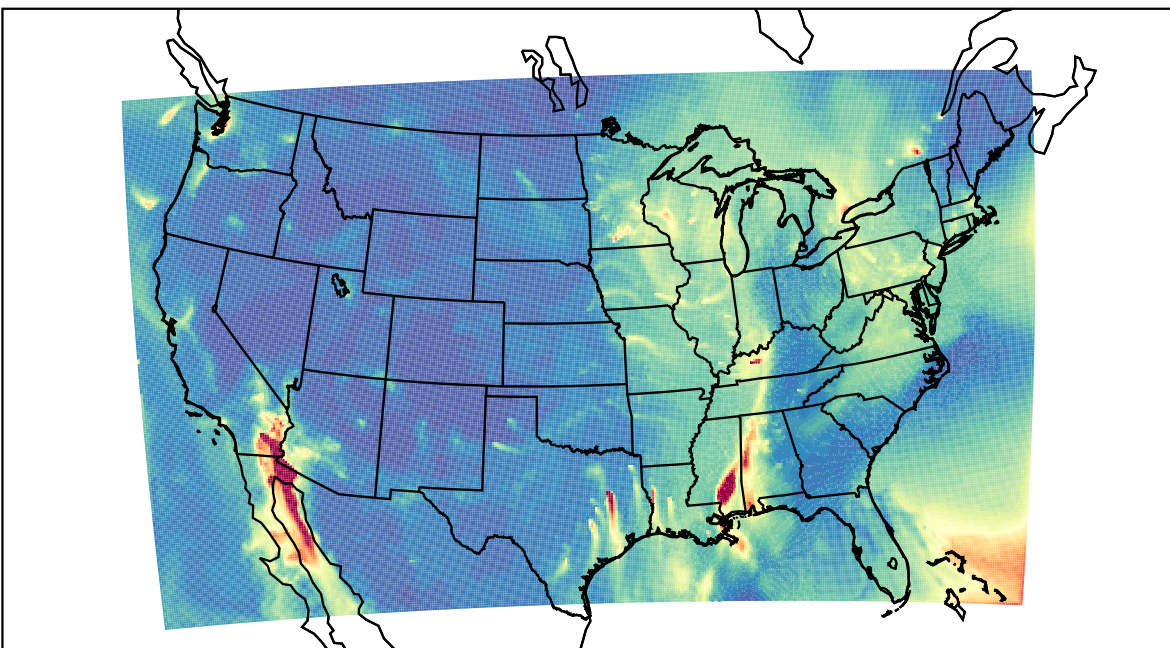
WRF 2023-12-17_11:00:00
