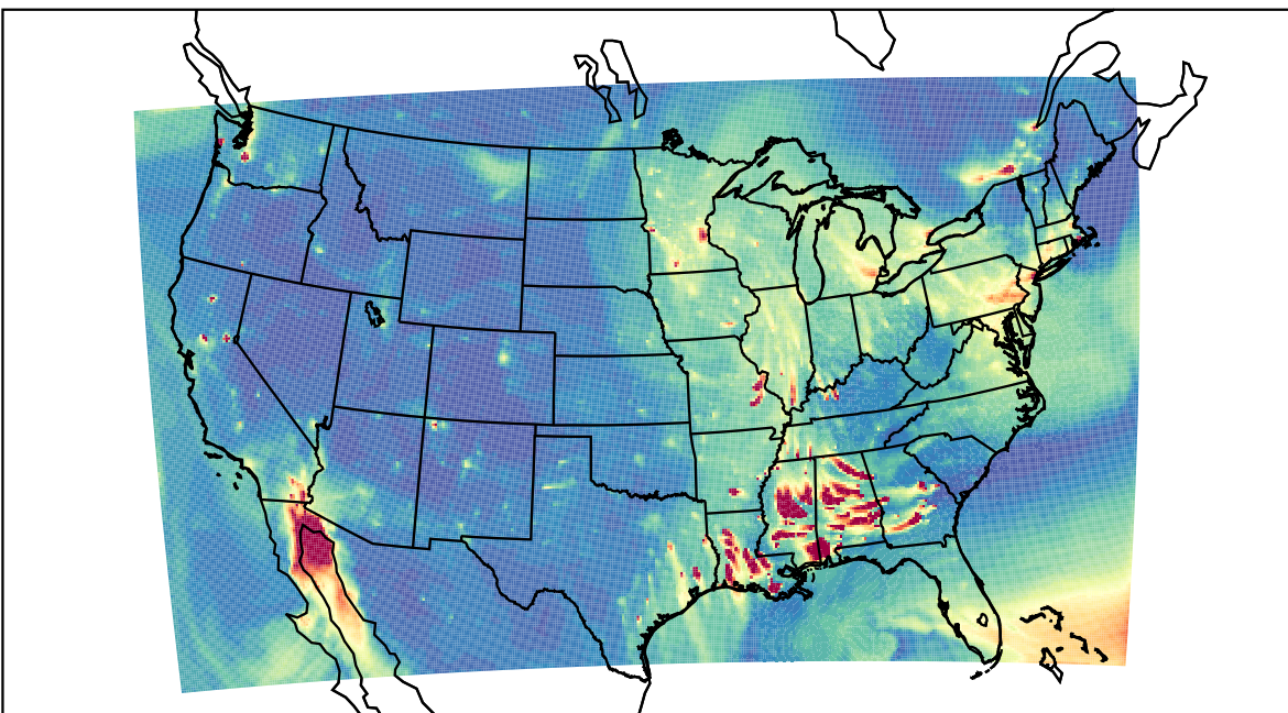
WRF 2023-12-17_00:00:00
