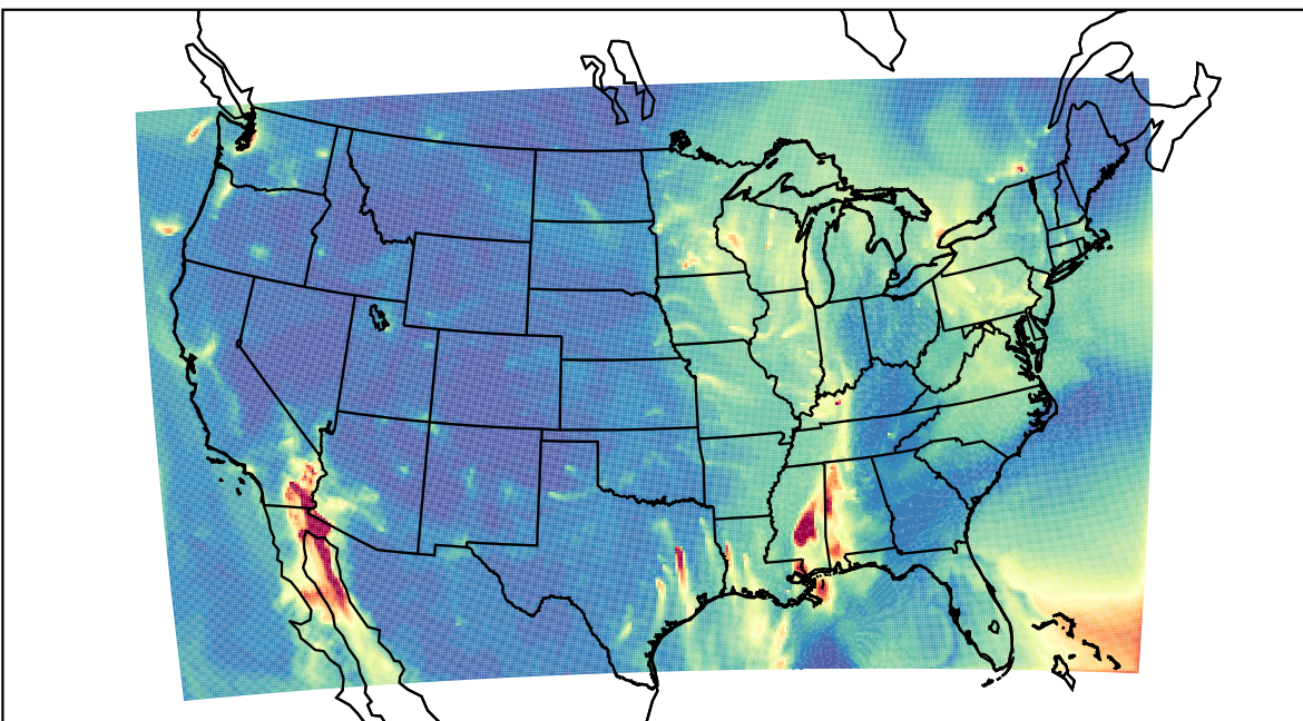
WRF 2023-12-17_09:00:00
