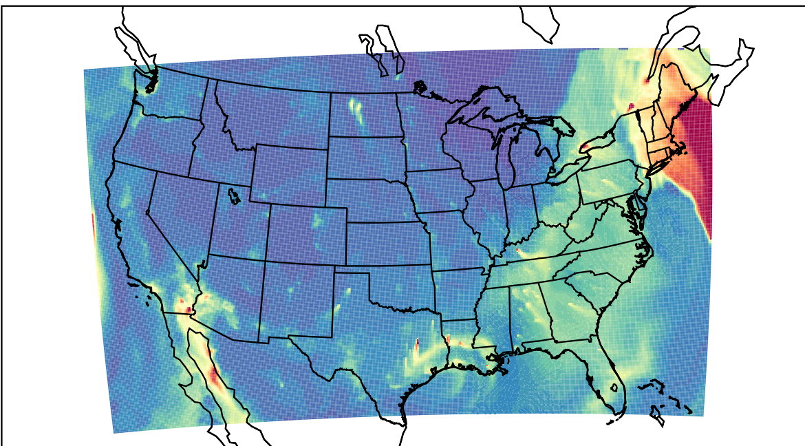
WRF 2023-12-18_15:00:00
