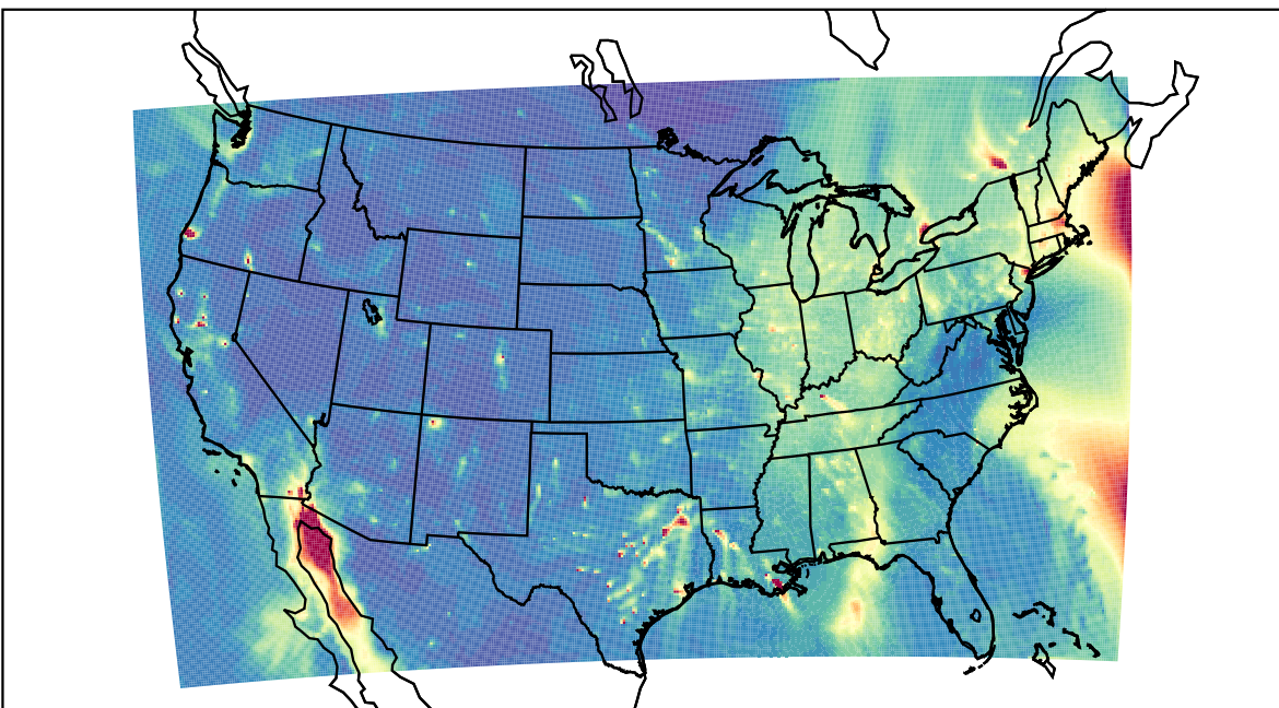
WRF 2023-12-18_00:00:00
