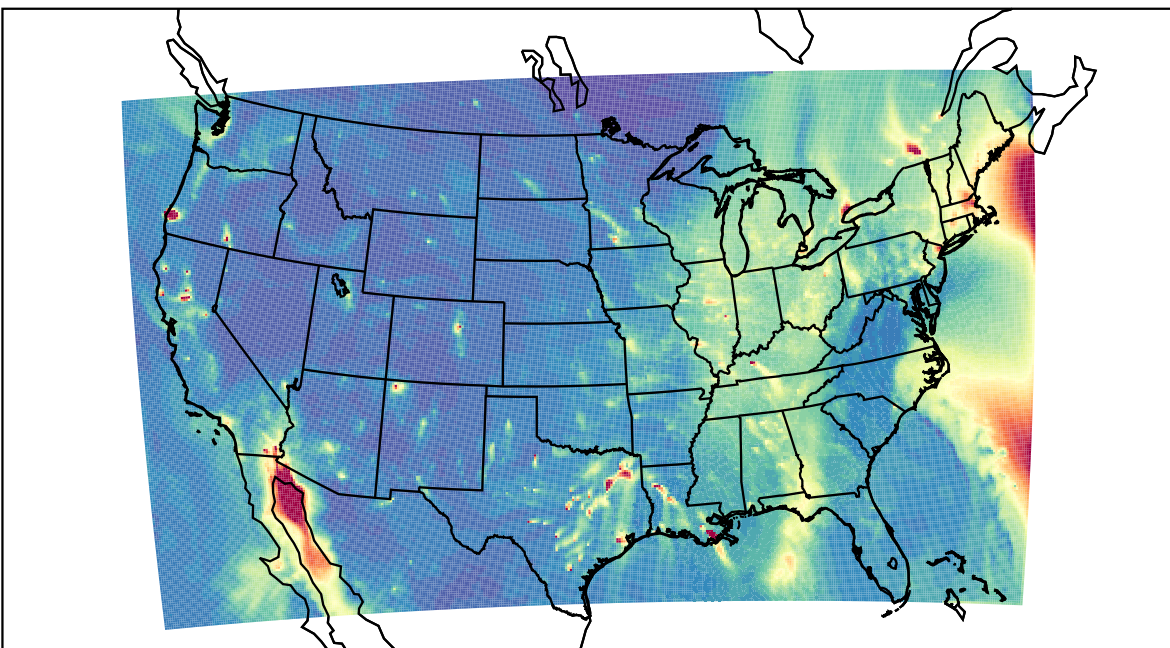
WRF 2023-12-18_01:00:00
