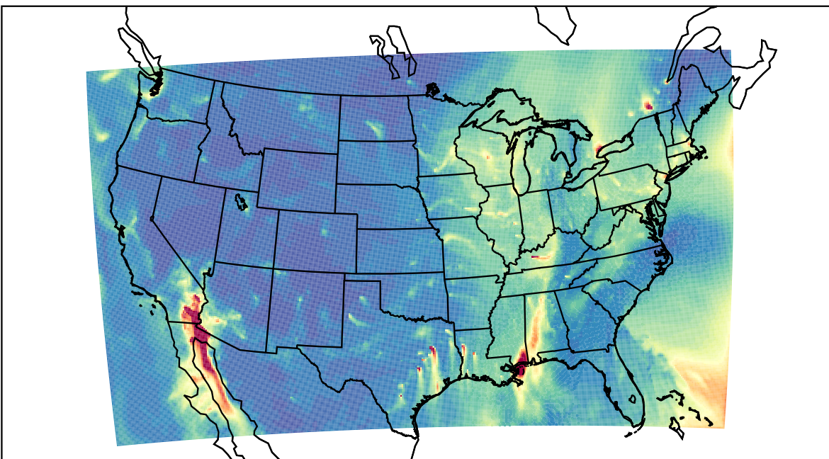
WRF 2023-12-17_15:00:00
