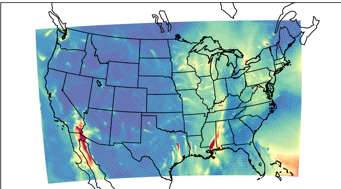
WRF 2023-12-17_12:00:00
