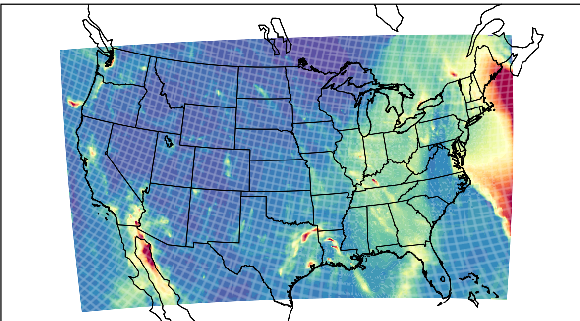
WRF 2023-12-18_06:00:00
