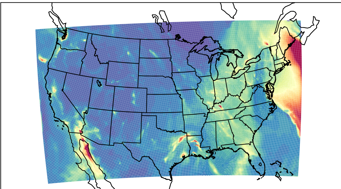
WRF 2023-12-18_07:00:00
