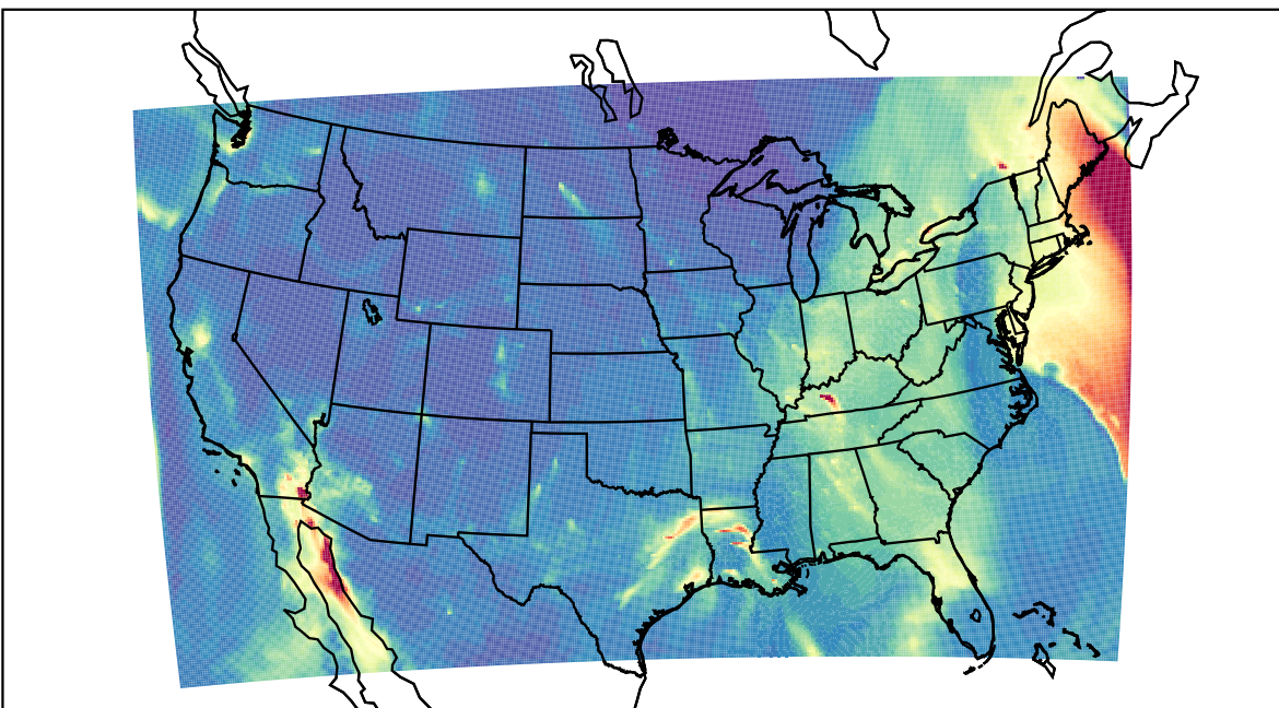
WRF 2023-12-18_09:00:00
