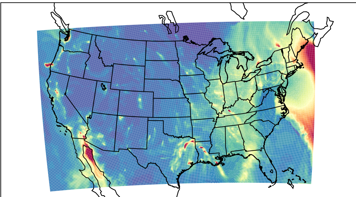
WRF 2023-12-18_04:00:00
