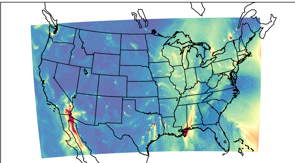
WRF 2023-12-17_16:00:00
