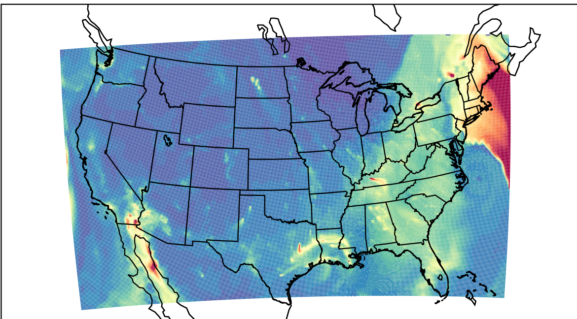
WRF 2023-12-18_13:00:00
