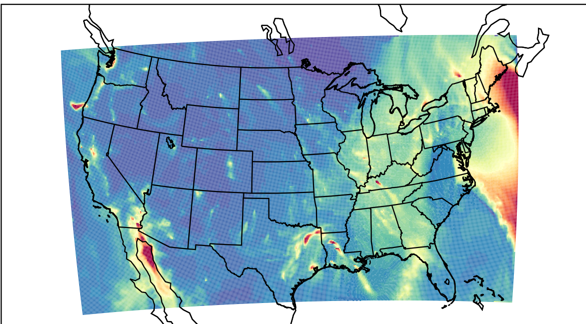
WRF 2023-12-18_05:00:00
