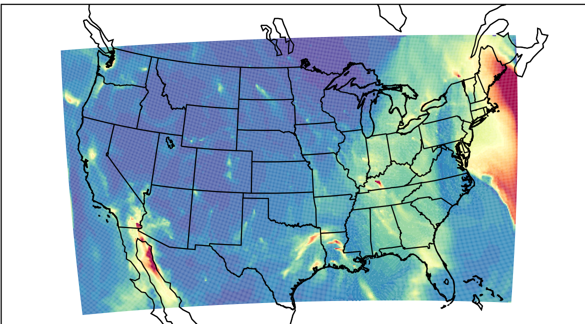
WRF 2023-12-18_08:00:00
