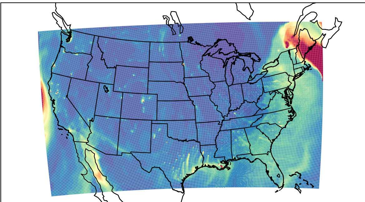
WRF 2023-12-18_22:00:00
