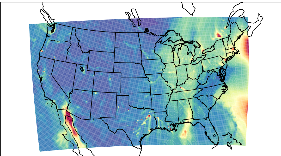
WRF 2023-12-17_22:00:00
