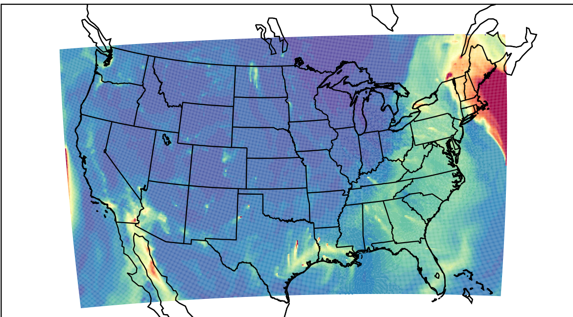
WRF 2023-12-18_17:00:00
