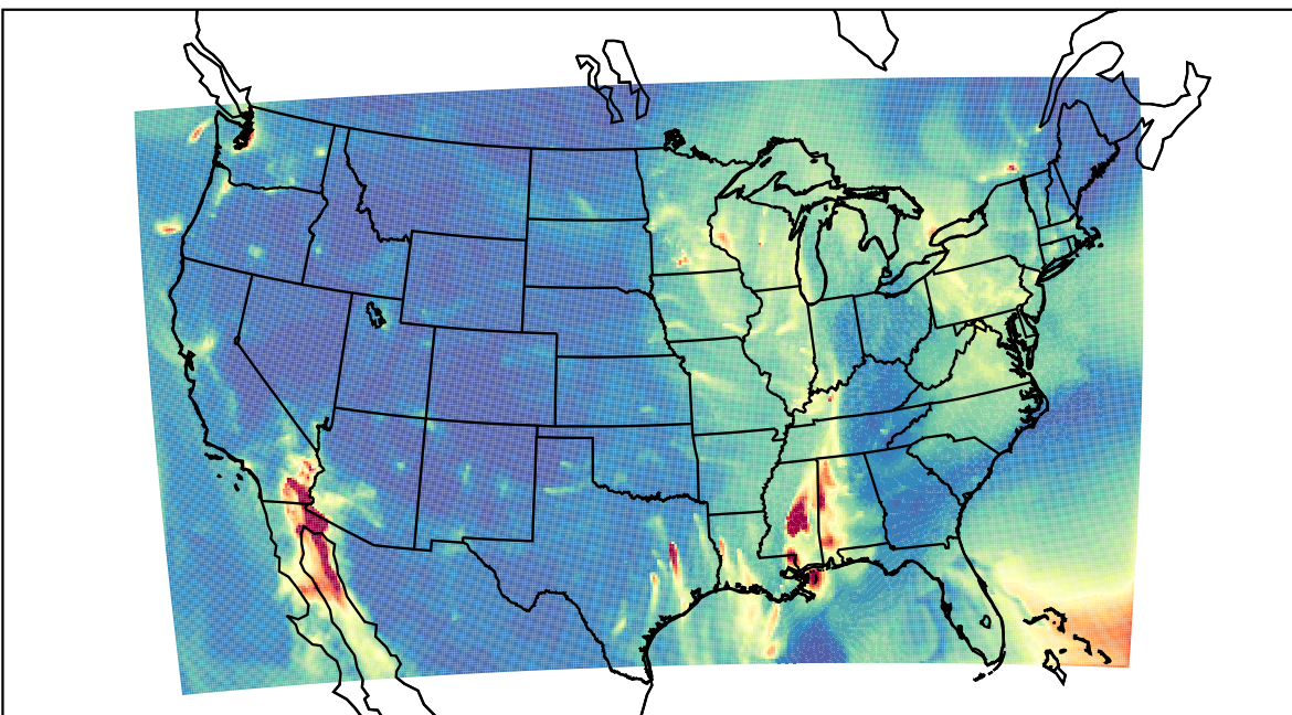
WRF 2023-12-17_08:00:00
