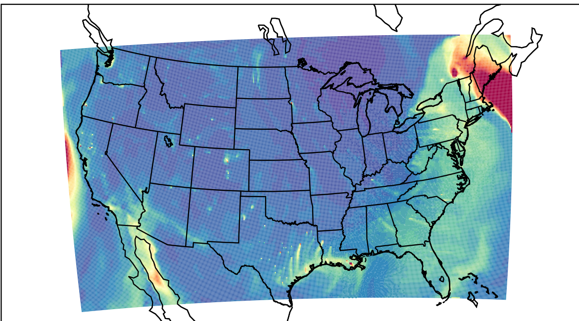
WRF 2023-12-18_21:00:00
