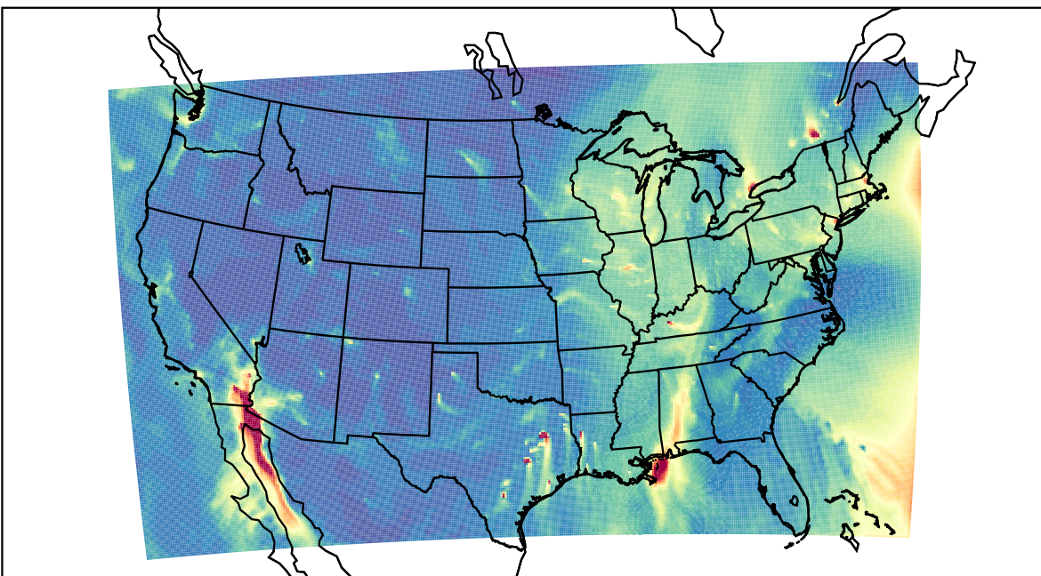
WRF 2023-12-17_17:00:00
