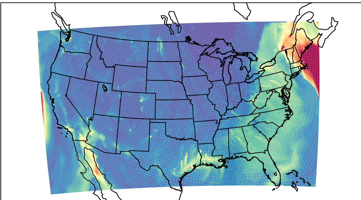
WRF 2023-12-18_18:00:00
