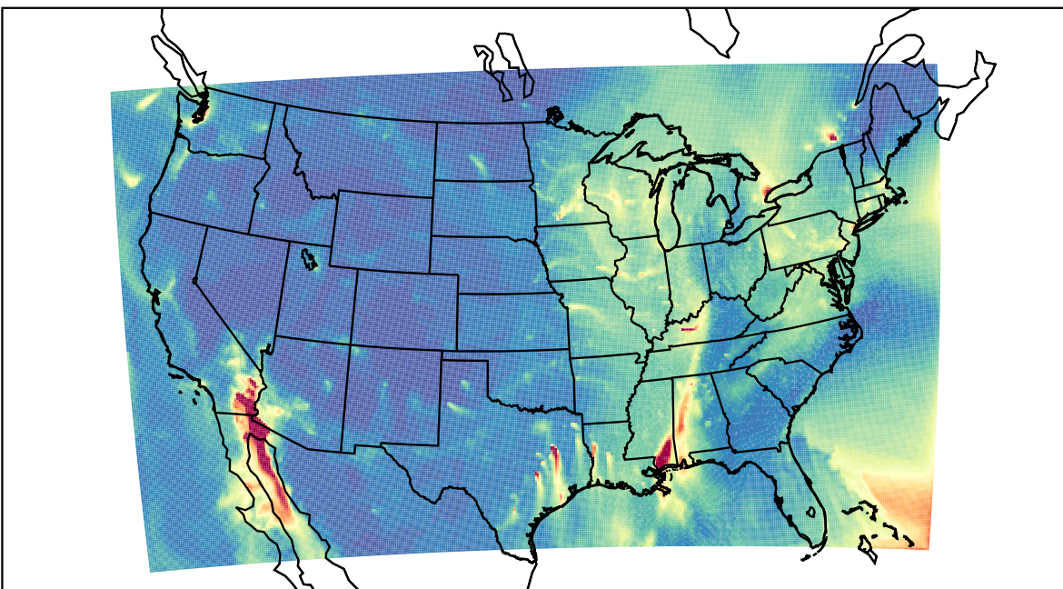
WRF 2023-12-17_13:00:00
