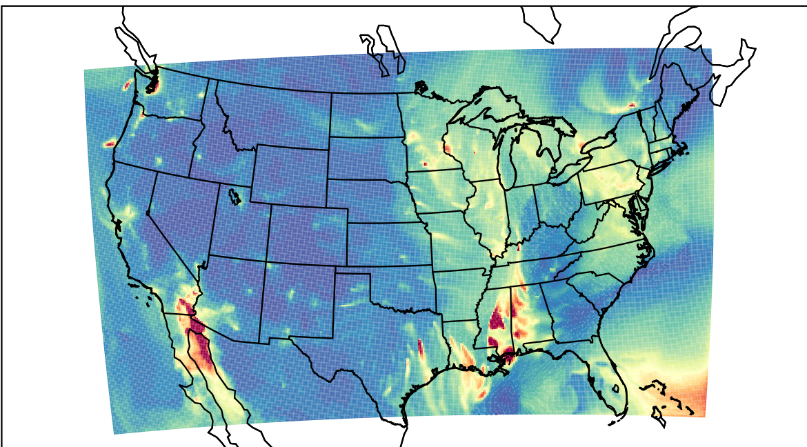
WRF 2023-12-17_06:00:00
