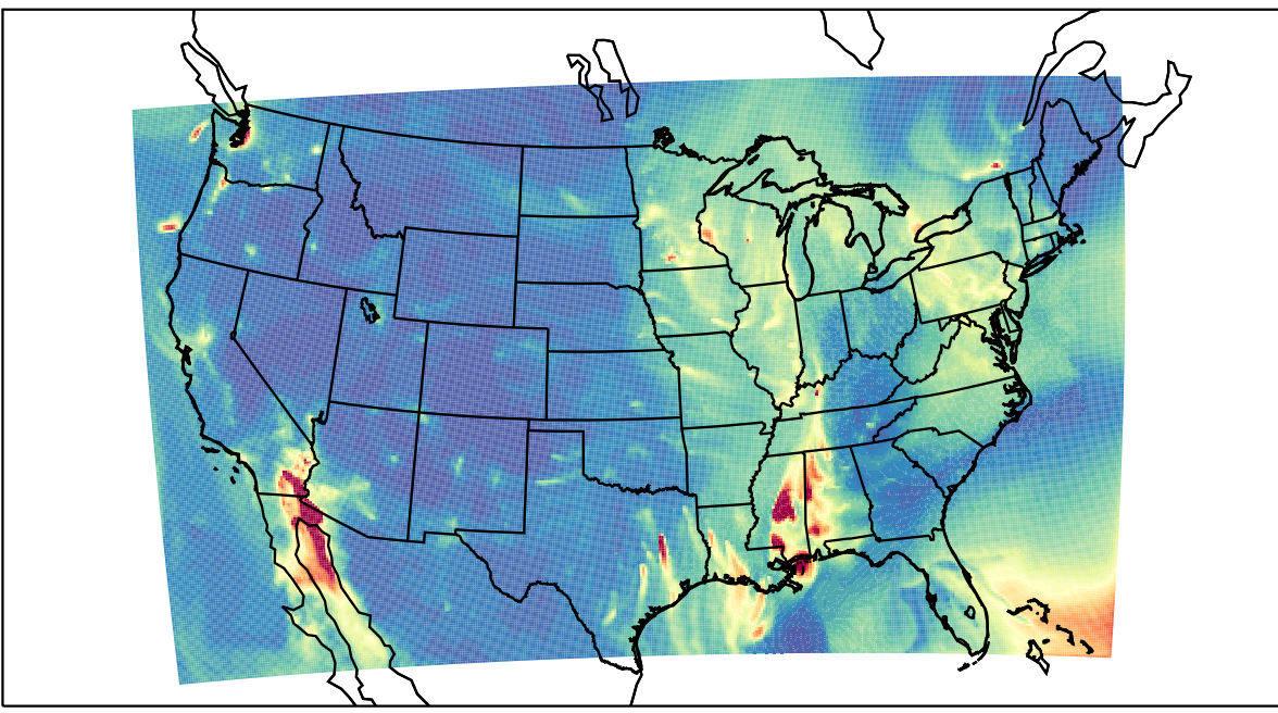
WRF 2023-12-17_07:00:00
