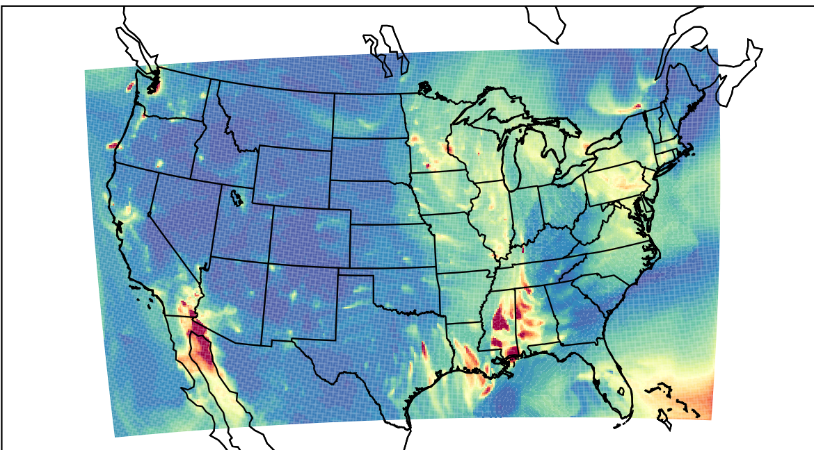
WRF 2023-12-17_05:00:00
