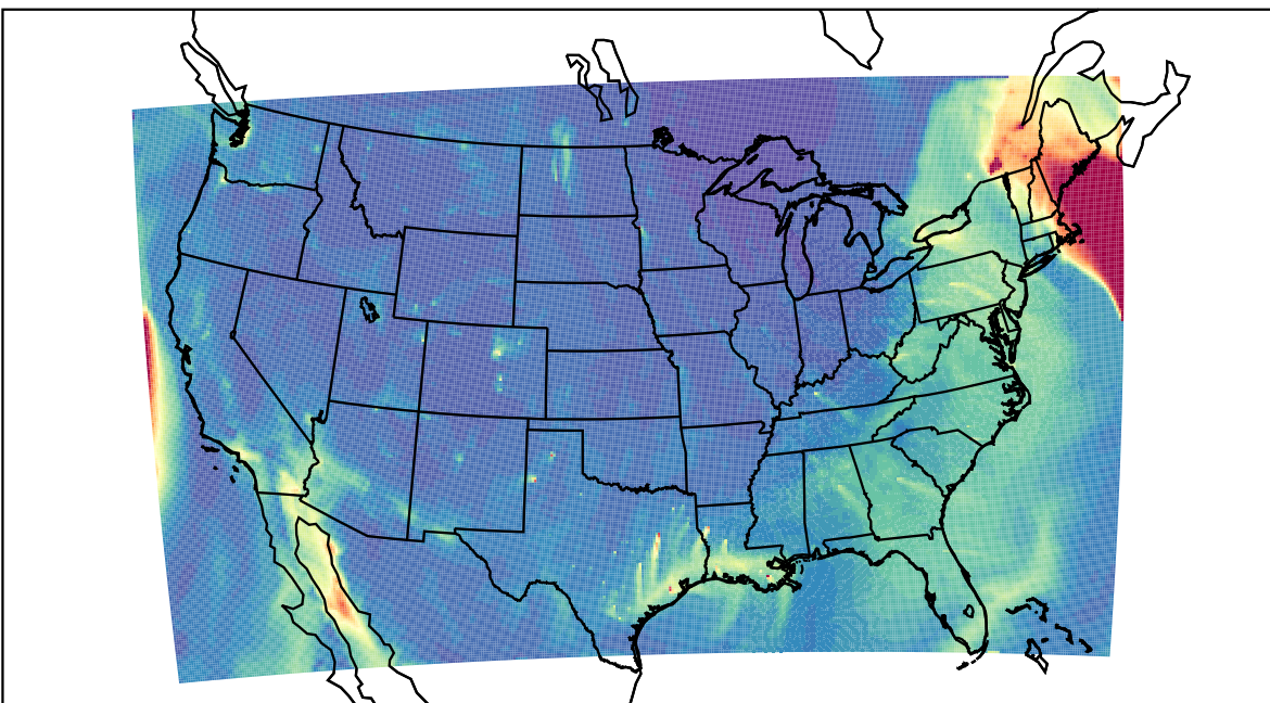
WRF 2023-12-18_19:00:00
