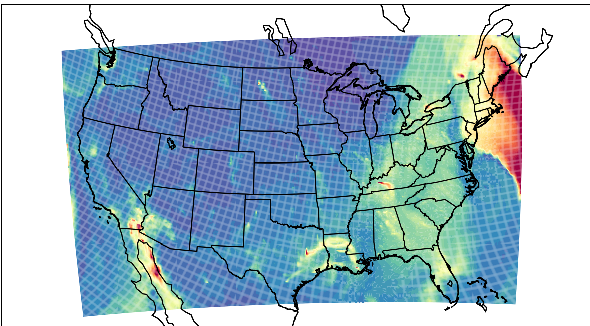
WRF 2023-12-18_12:00:00
