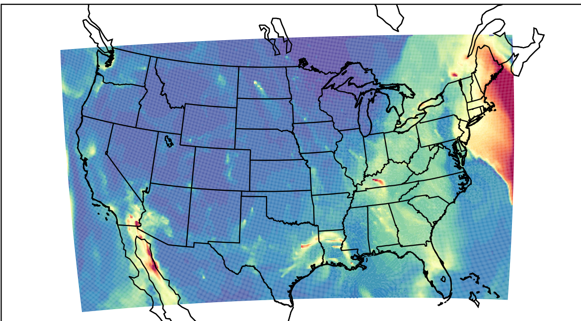
WRF 2023-12-18_11:00:00
