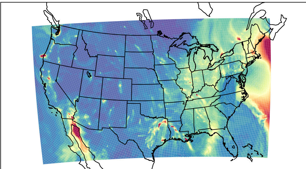
WRF 2023-12-18_03:00:00
