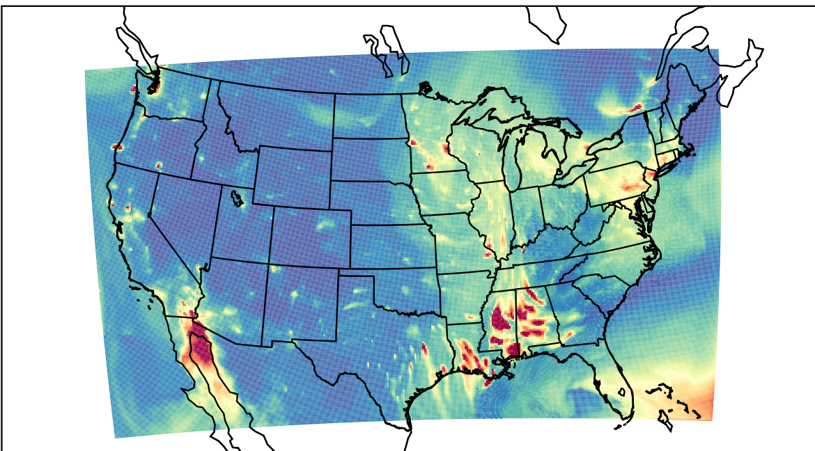
WRF 2023-12-17_03:00:00
