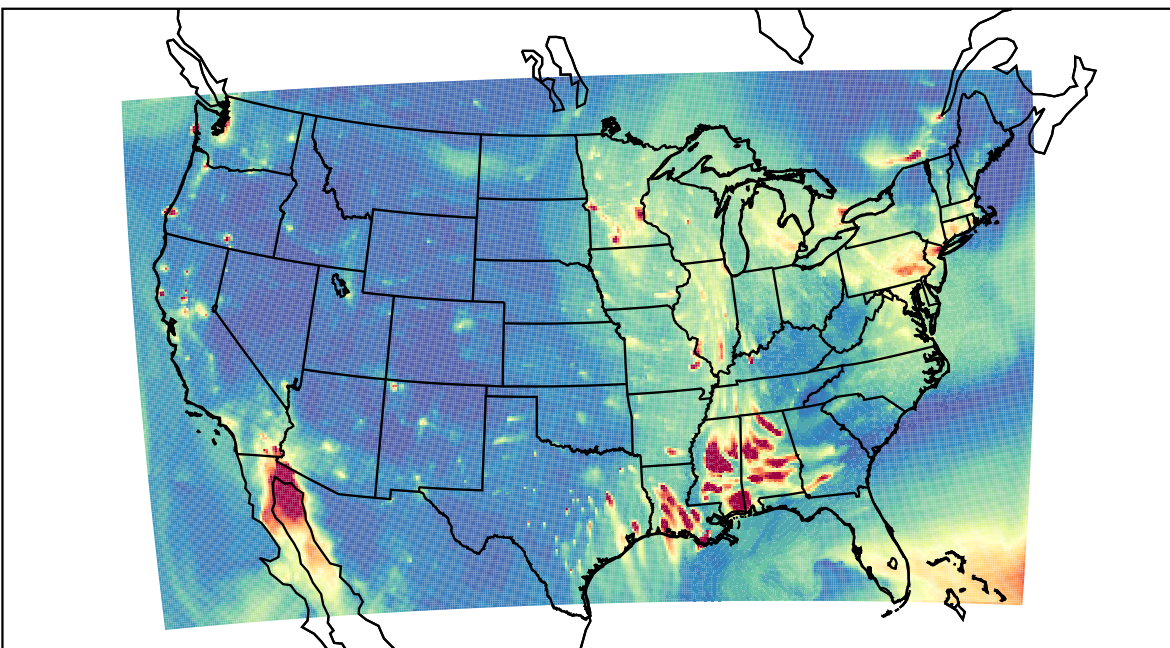
WRF 2023-12-17_02:00:00
