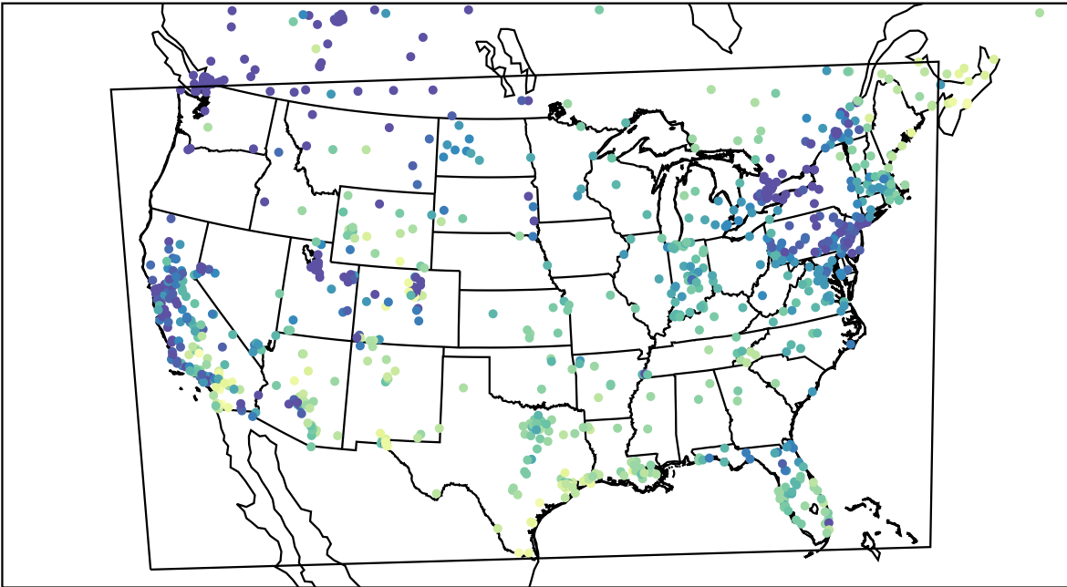
AirNOW (2023-12-18_22:00:00)
