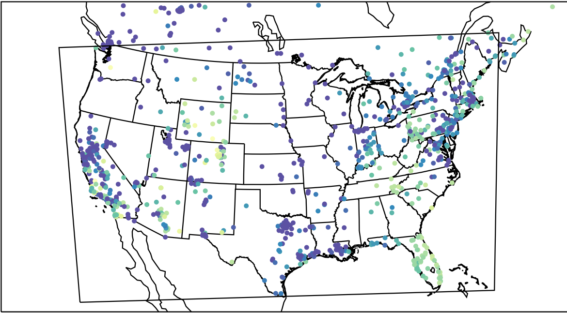
AirNOW (2023-12-17_01:00:00)
