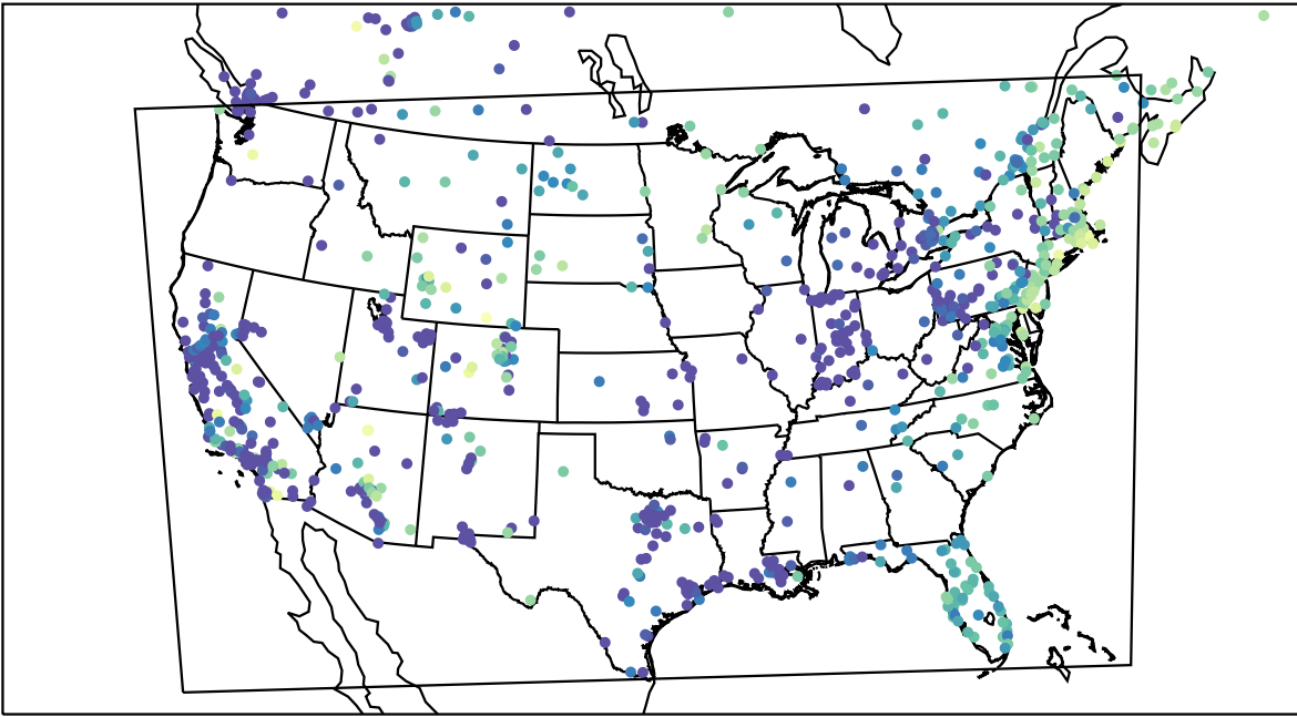
AirNOW (2023-12-18_04:00:00)
