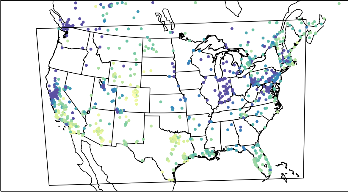
AirNOW (2023-12-17_22:00:00)
