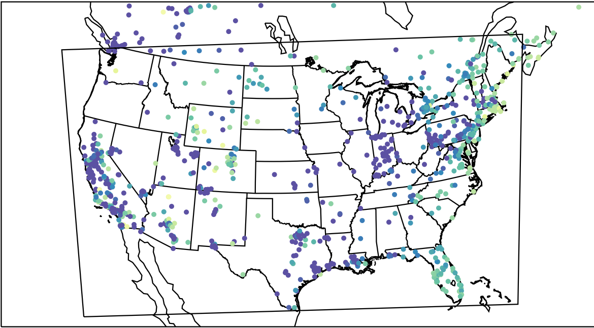
AirNOW (2023-12-18_02:00:00)
