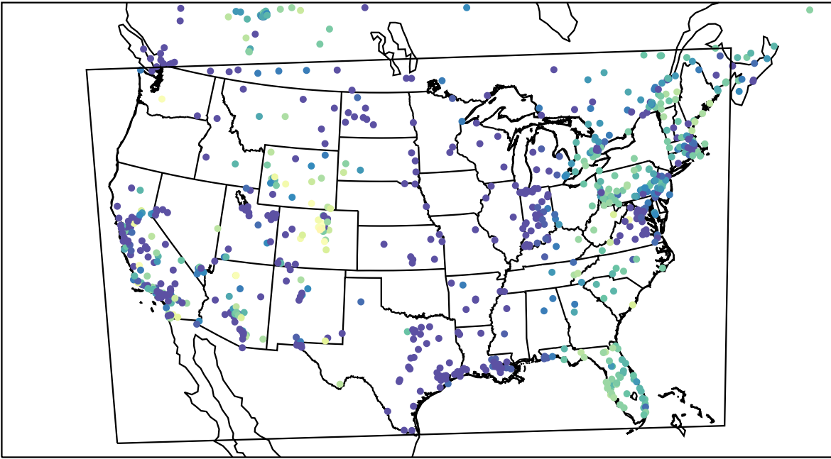
AirNOW (2023-12-17_12:00:00)
