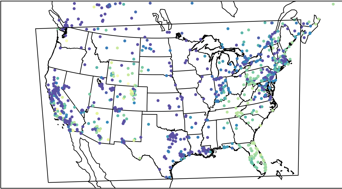
AirNOW (2023-12-17_02:00:00)
