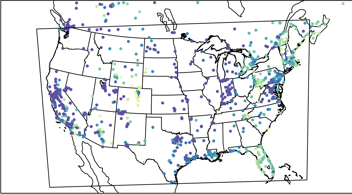
AirNOW (2023-12-17_16:00:00)
