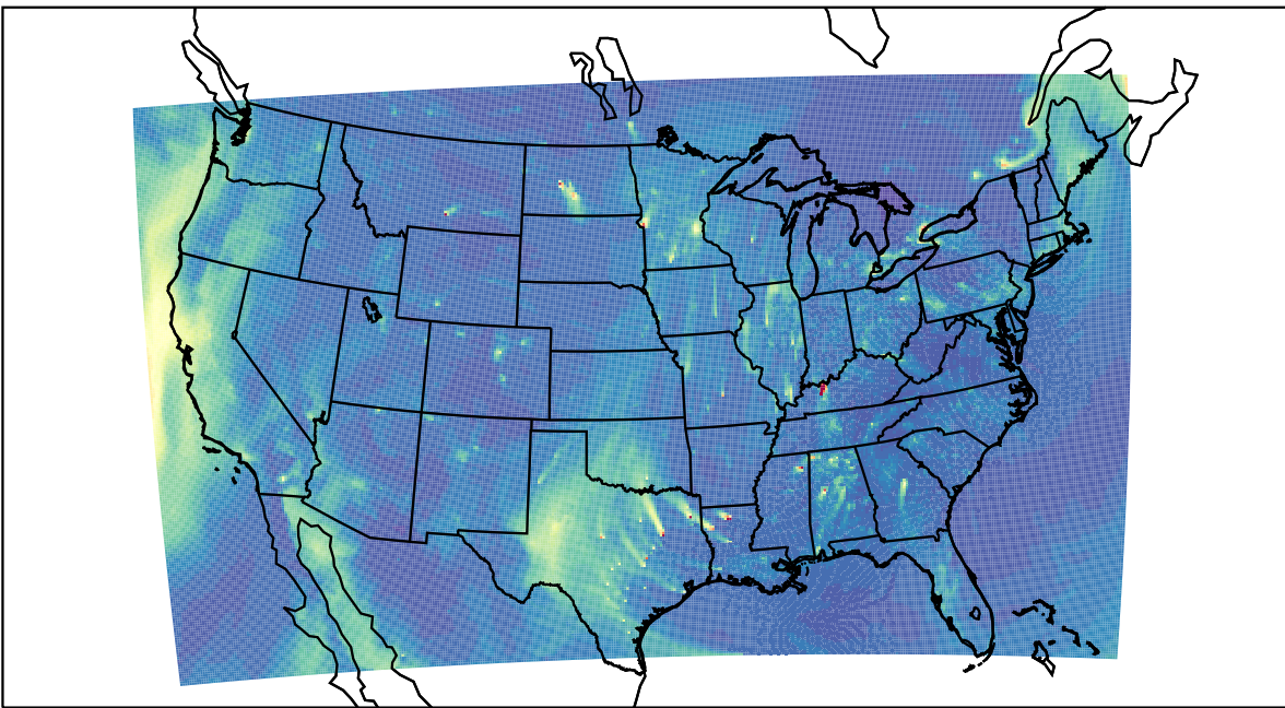
WRF 2023-12-19_22:00:00
