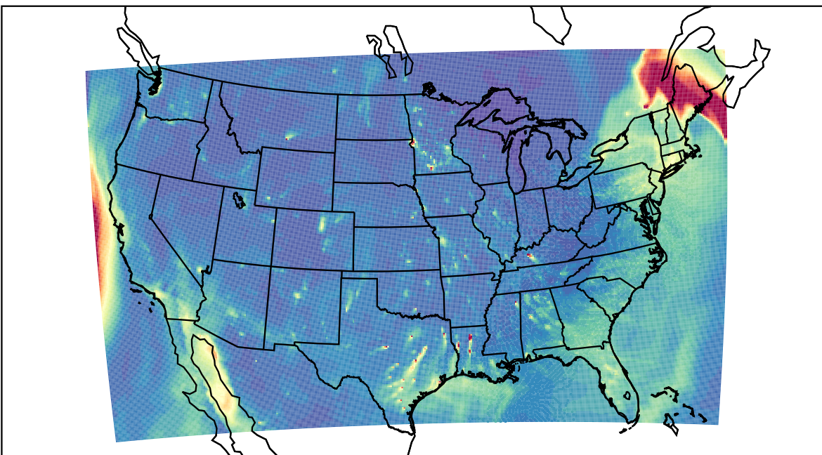
WRF 2023-12-19_00:00:00
