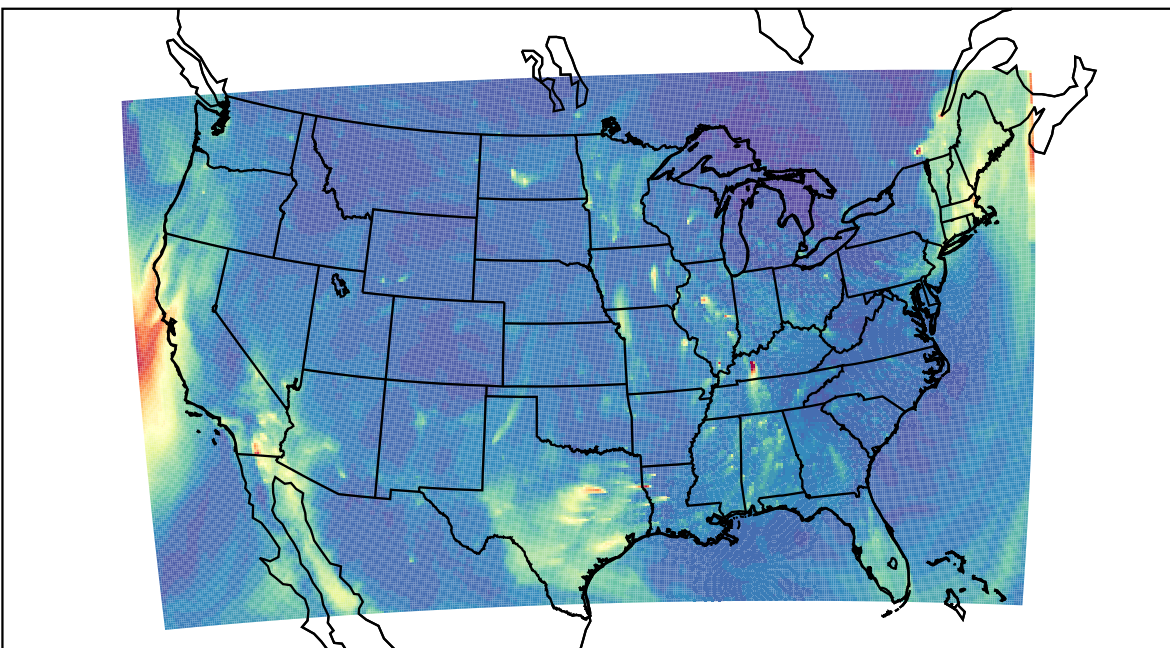
WRF 2023-12-19_13:00:00
