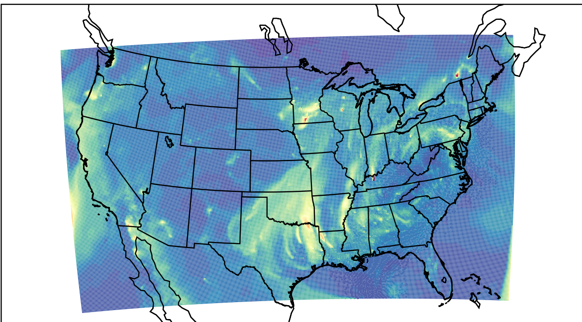
WRF 2023-12-20_12:00:00
