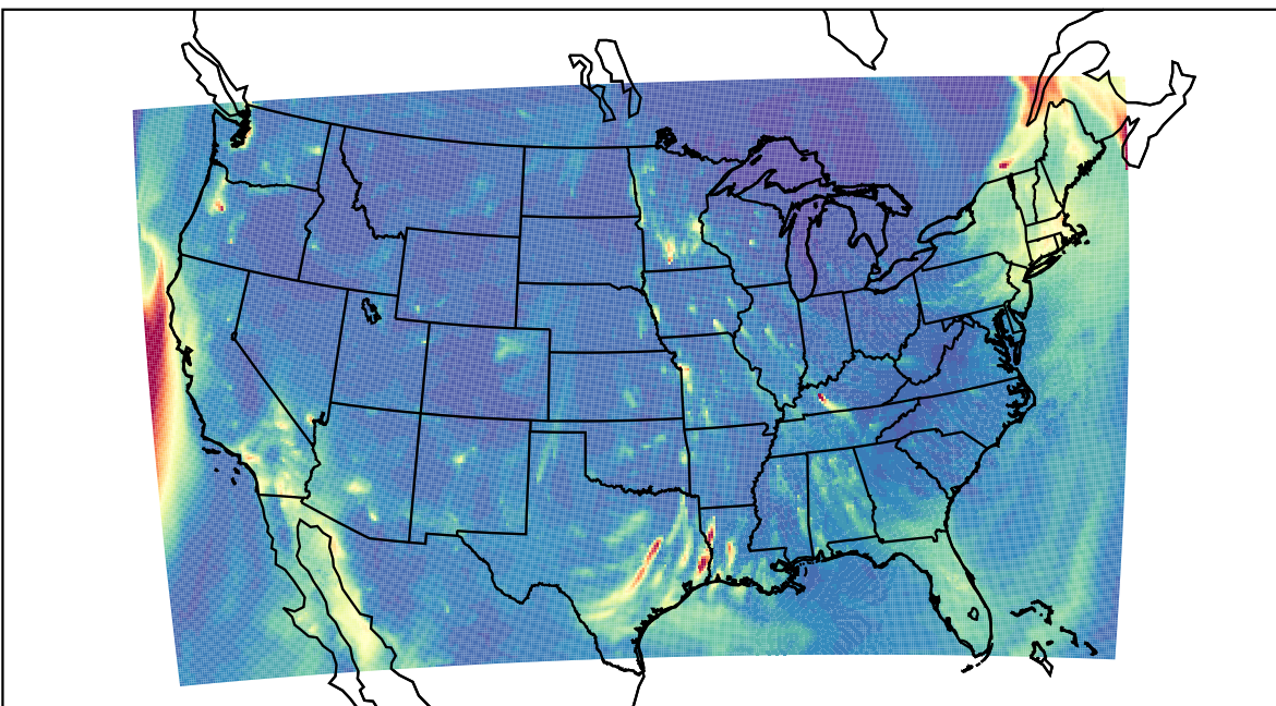
WRF 2023-12-19_05:00:00
