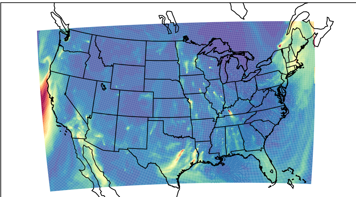
WRF 2023-12-19_08:00:00
