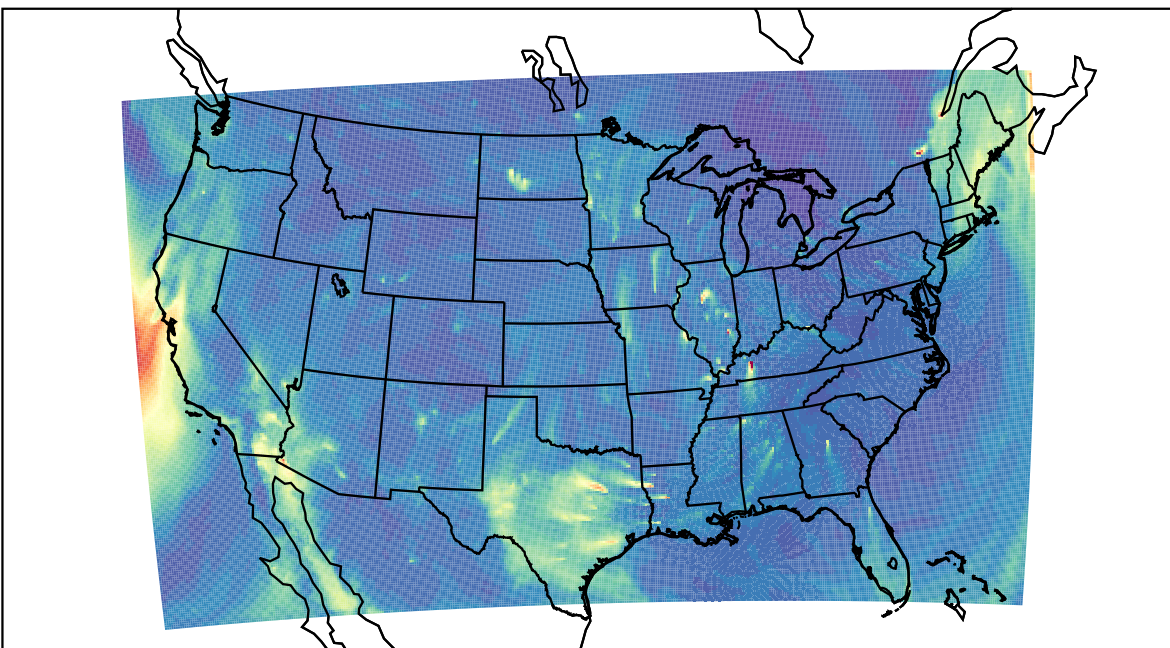
WRF 2023-12-19_15:00:00
