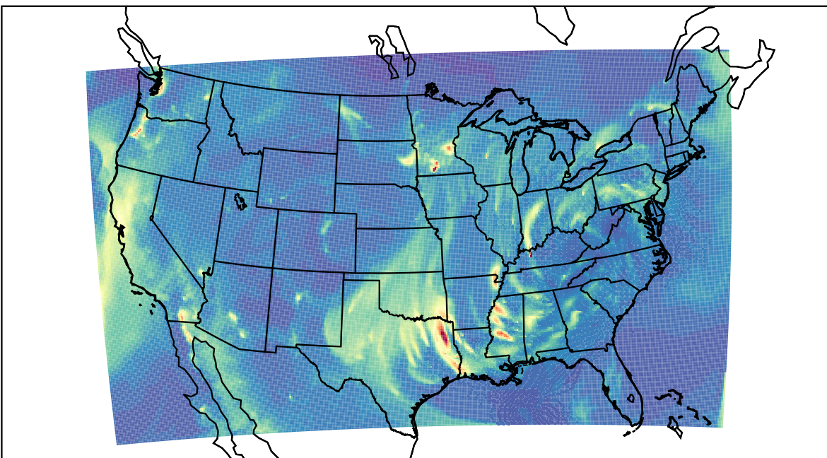
WRF 2023-12-20_07:00:00
