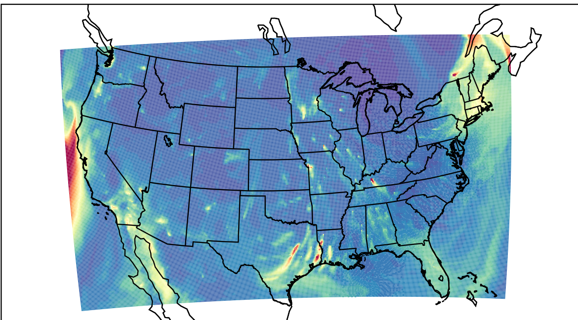
WRF 2023-12-19_06:00:00
