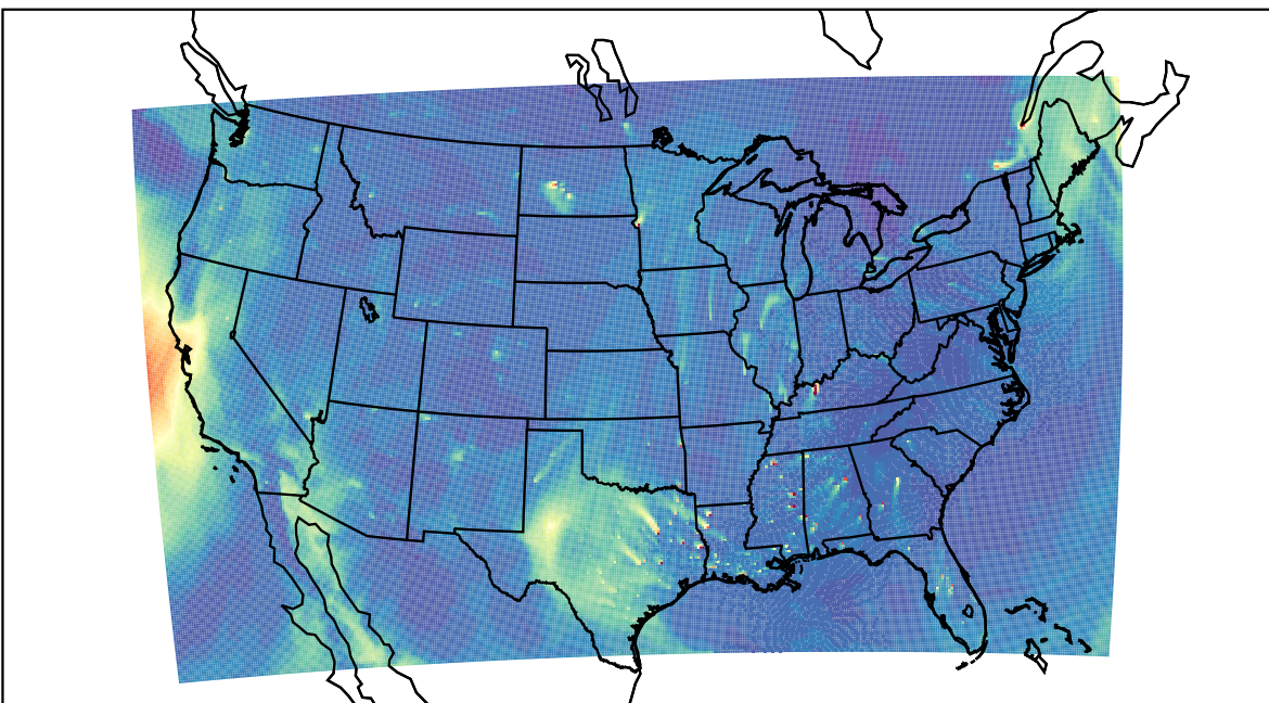
WRF 2023-12-19_19:00:00
