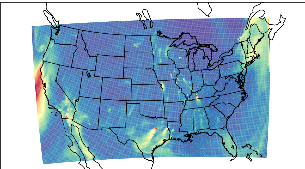
WRF 2023-12-19_10:00:00
