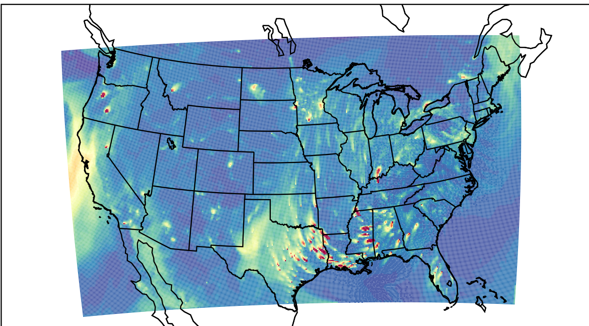
WRF 2023-12-20_01:00:00
