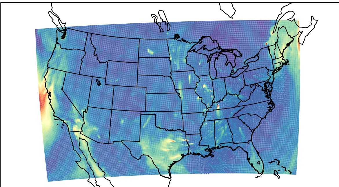
WRF 2023-12-19_14:00:00
