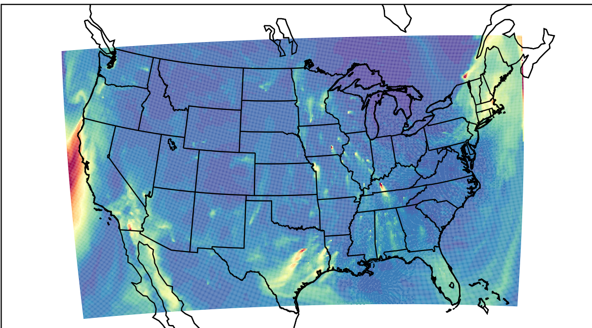
WRF 2023-12-19_09:00:00
