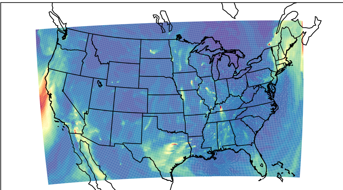
WRF 2023-12-19_12:00:00
