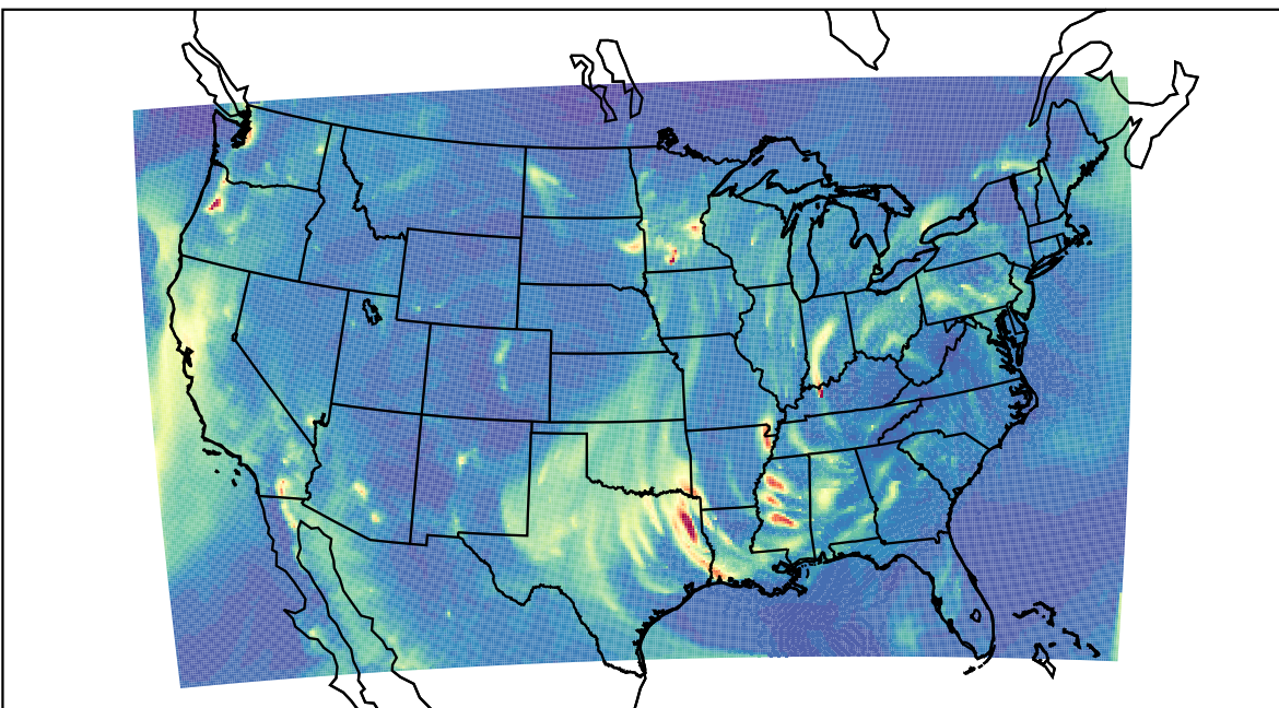
WRF 2023-12-20_06:00:00
