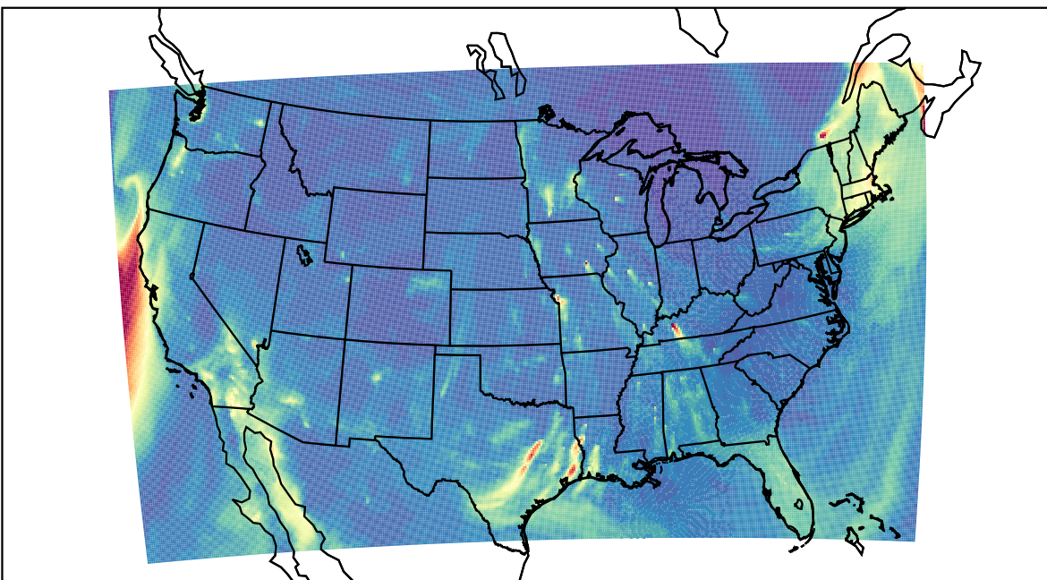
WRF 2023-12-19_07:00:00
