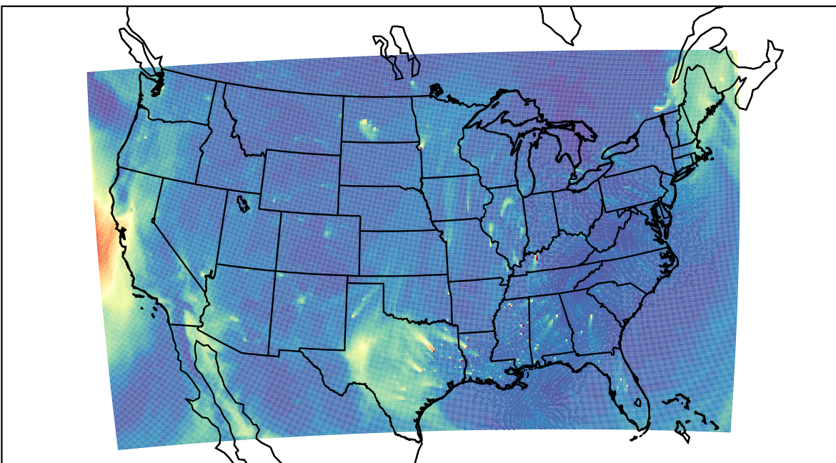
WRF 2023-12-19_18:00:00
