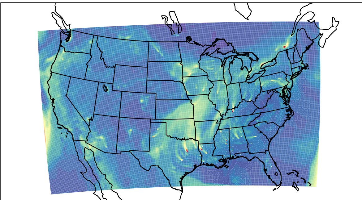
WRF 2023-12-20_17:00:00
