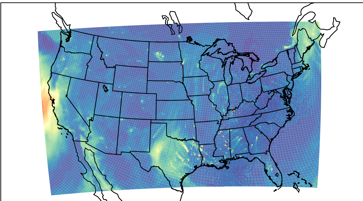
WRF 2023-12-19_20:00:00
