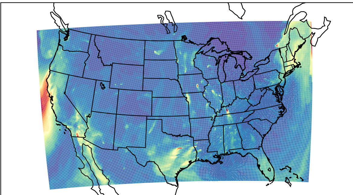
WRF 2023-12-19_11:00:00
