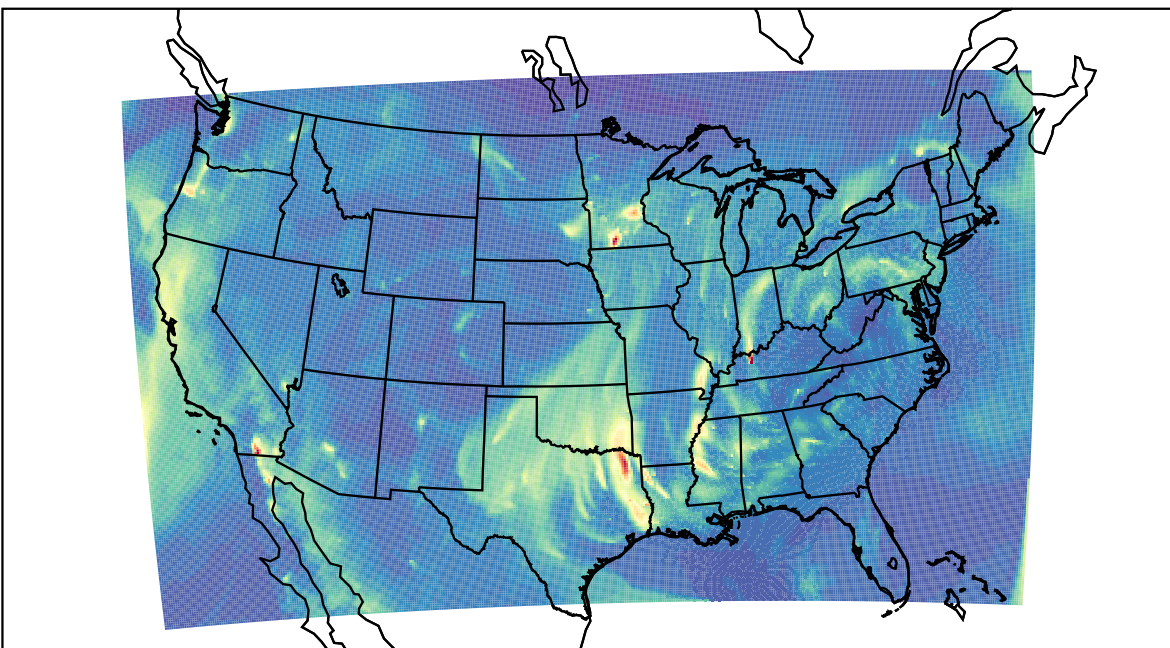
WRF 2023-12-20_09:00:00
