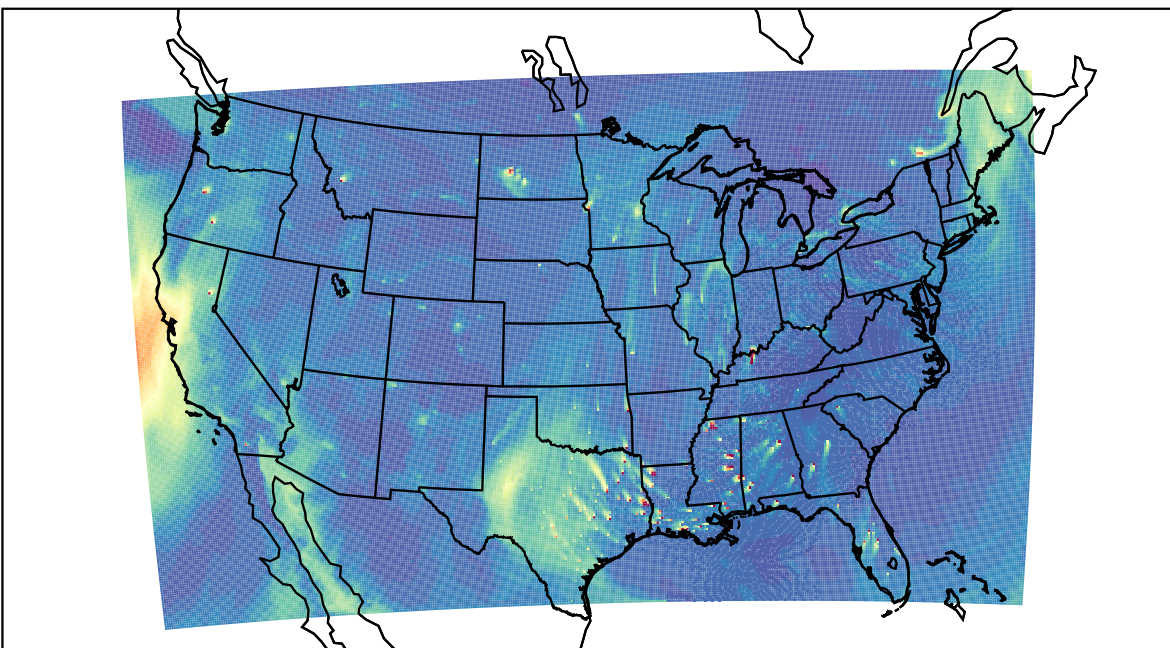
WRF 2023-12-19_21:00:00
