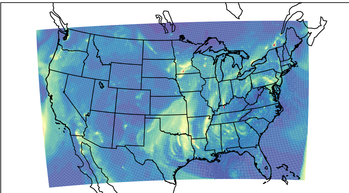
WRF 2023-12-20_13:00:00
