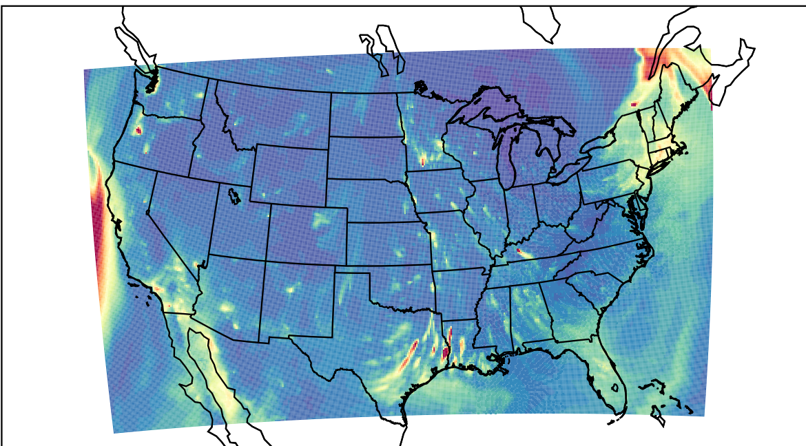
WRF 2023-12-19_04:00:00
