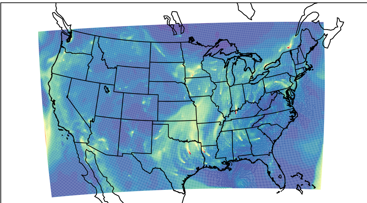
WRF 2023-12-20_16:00:00
