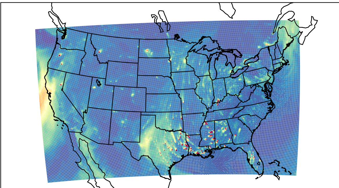
WRF 2023-12-19_23:00:00
