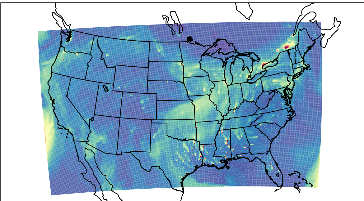
WRF 2023-12-20_21:00:00
