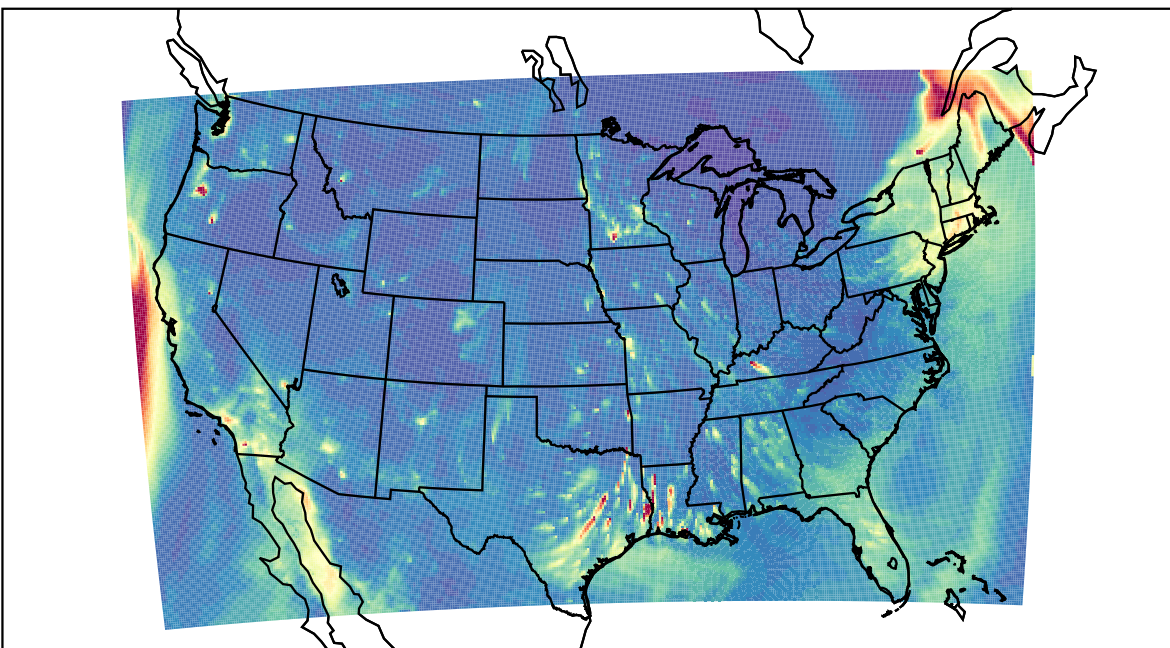
WRF 2023-12-19_03:00:00
