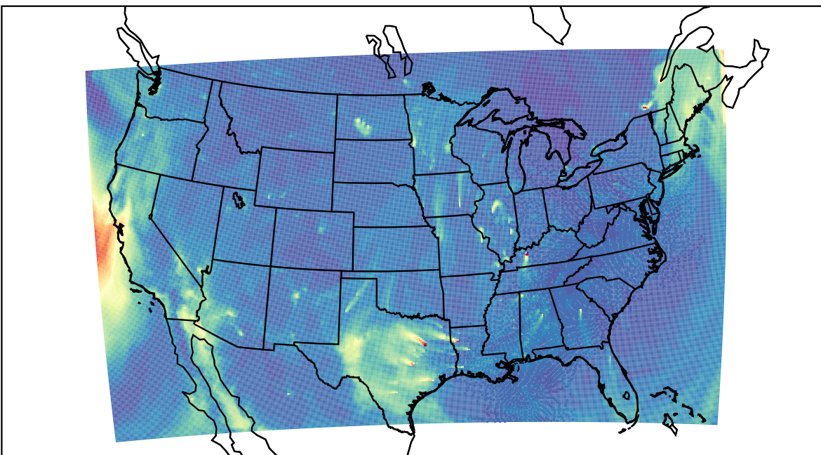
WRF 2023-12-19_16:00:00
