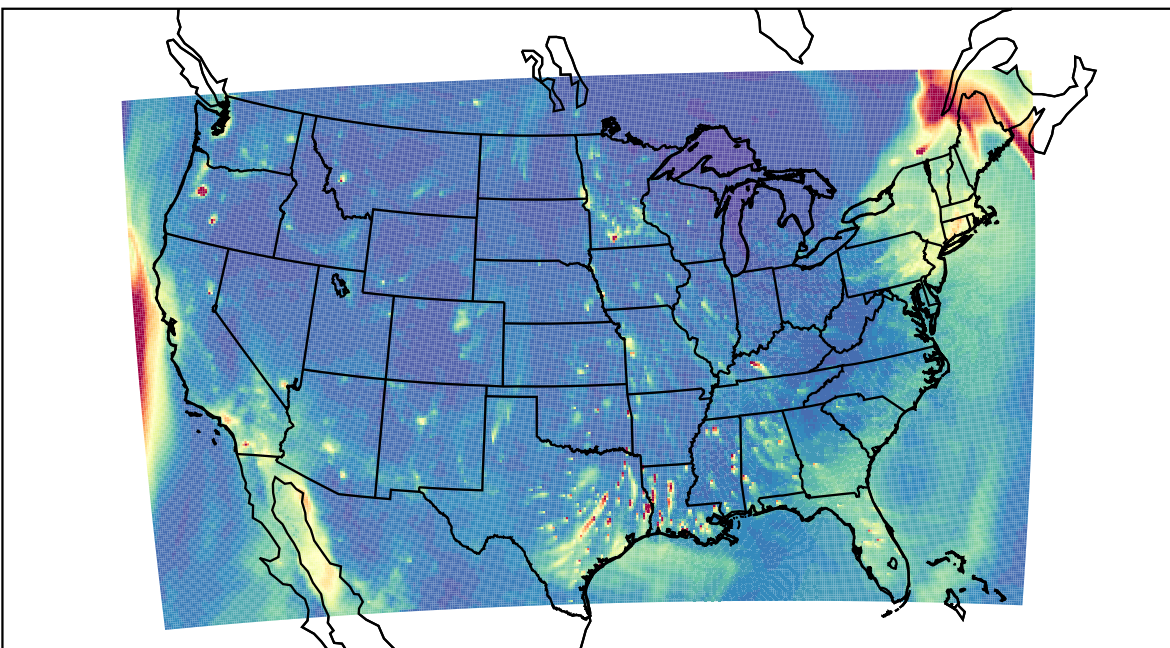
WRF 2023-12-19_02:00:00
