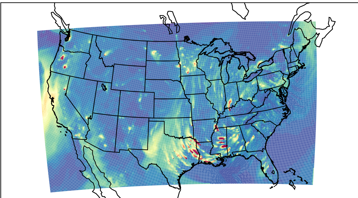
WRF 2023-12-20_02:00:00
