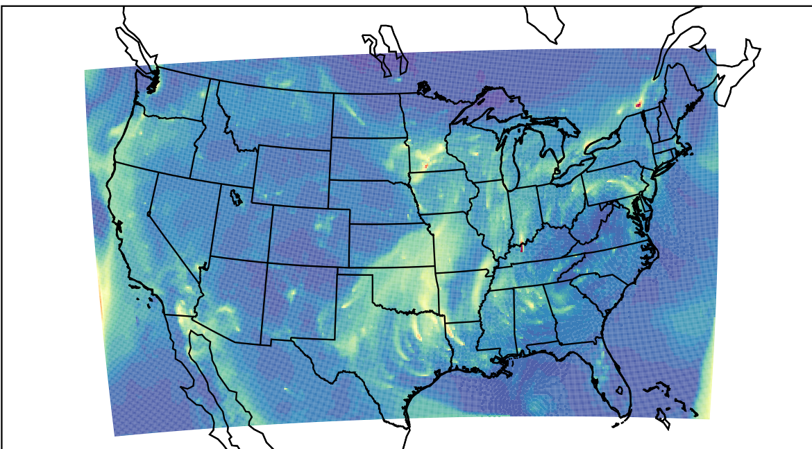
WRF 2023-12-20_15:00:00
