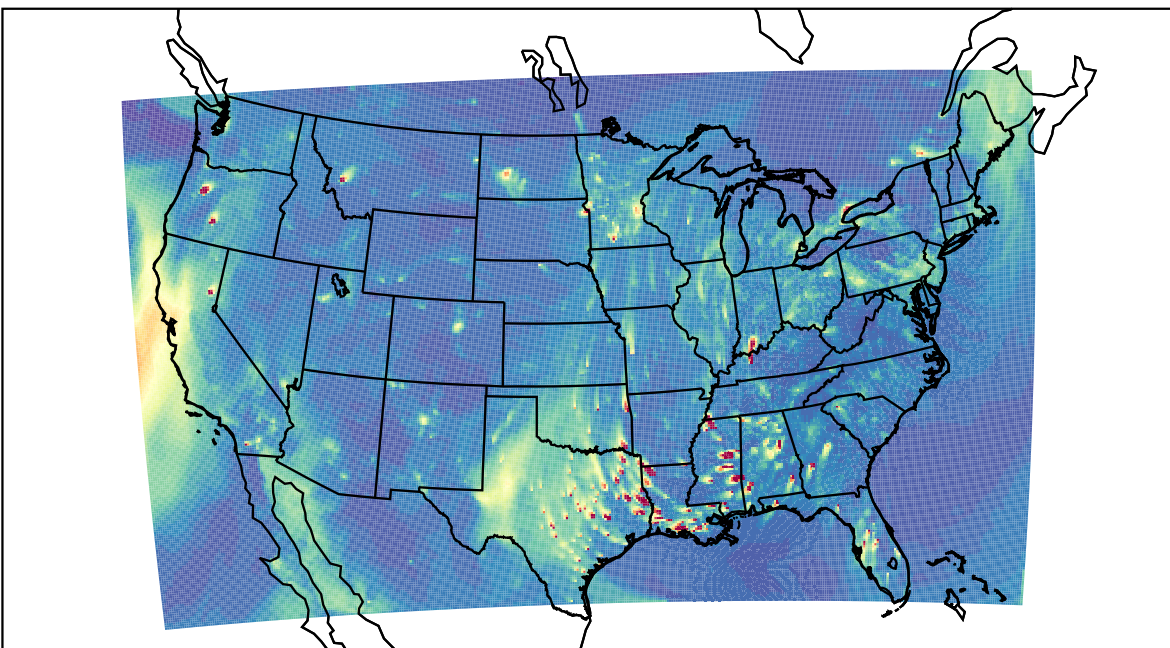
WRF 2023-12-20_00:00:00
