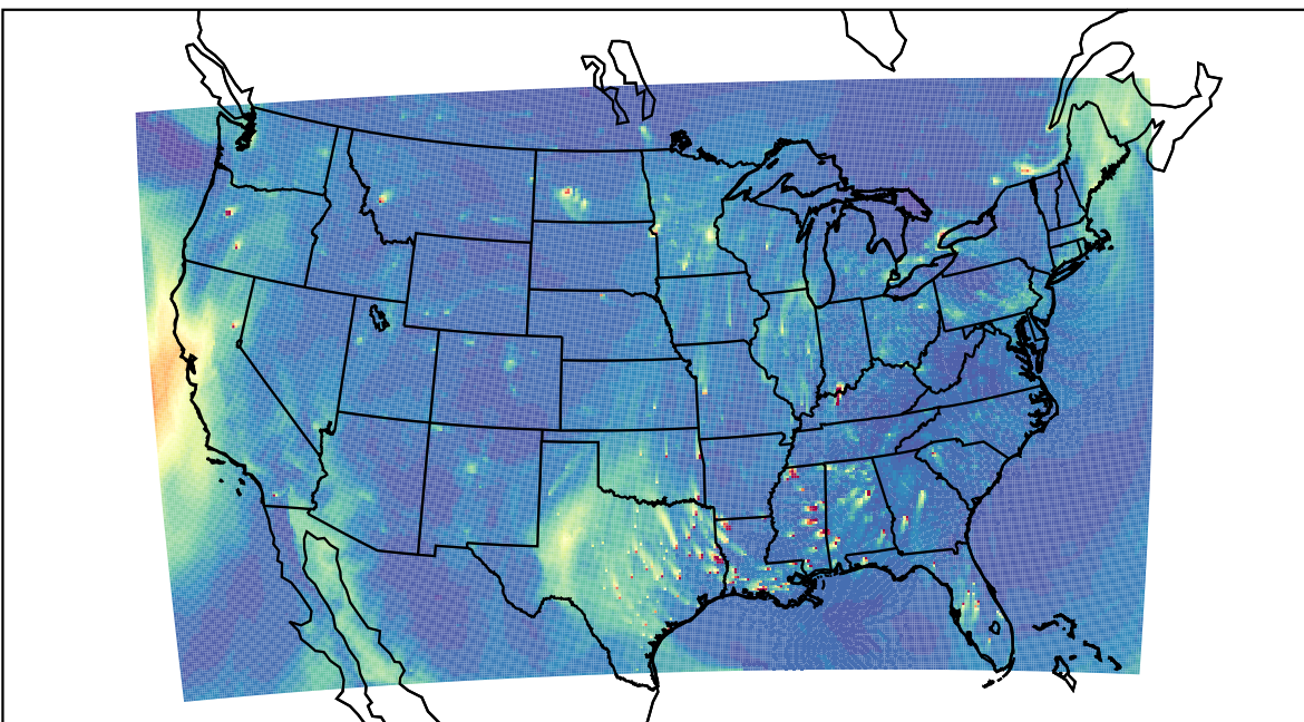
WRF 2023-12-19_22:00:00
