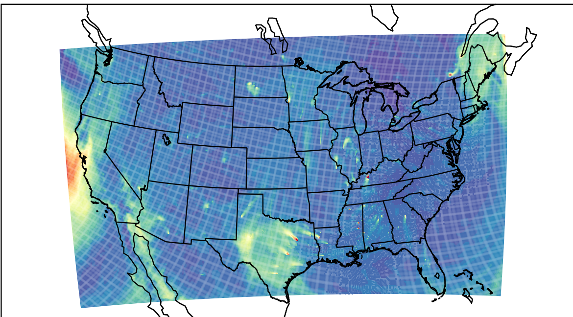
WRF 2023-12-19_17:00:00
