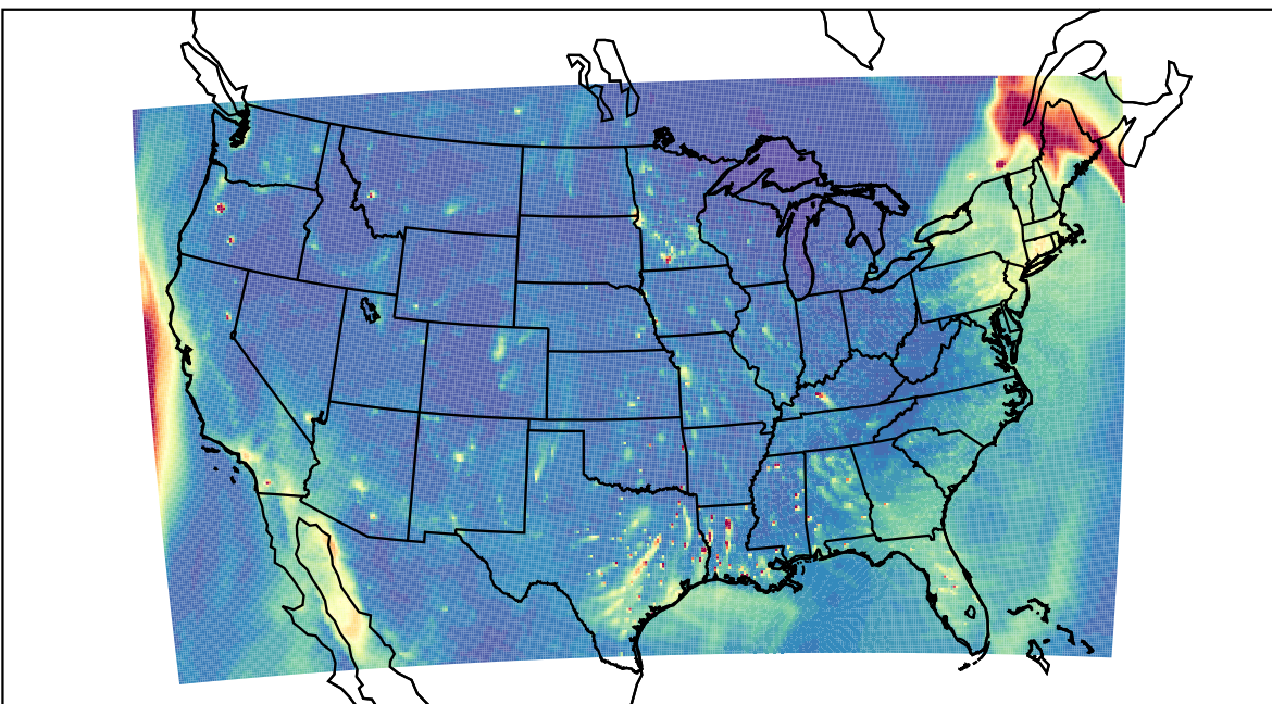
WRF 2023-12-19_01:00:00
