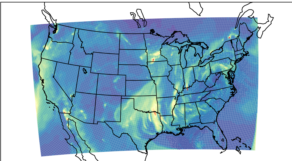
WRF 2023-12-20_11:00:00
