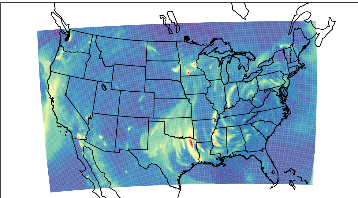
WRF 2023-12-20_08:00:00
