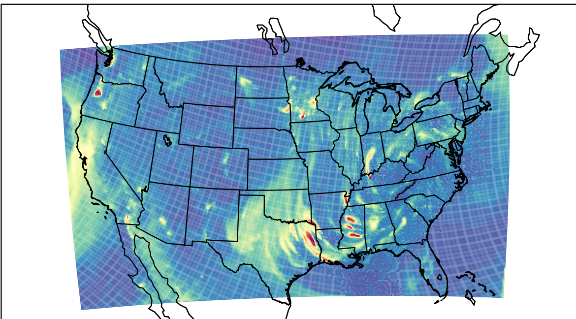
WRF 2023-12-20_05:00:00
