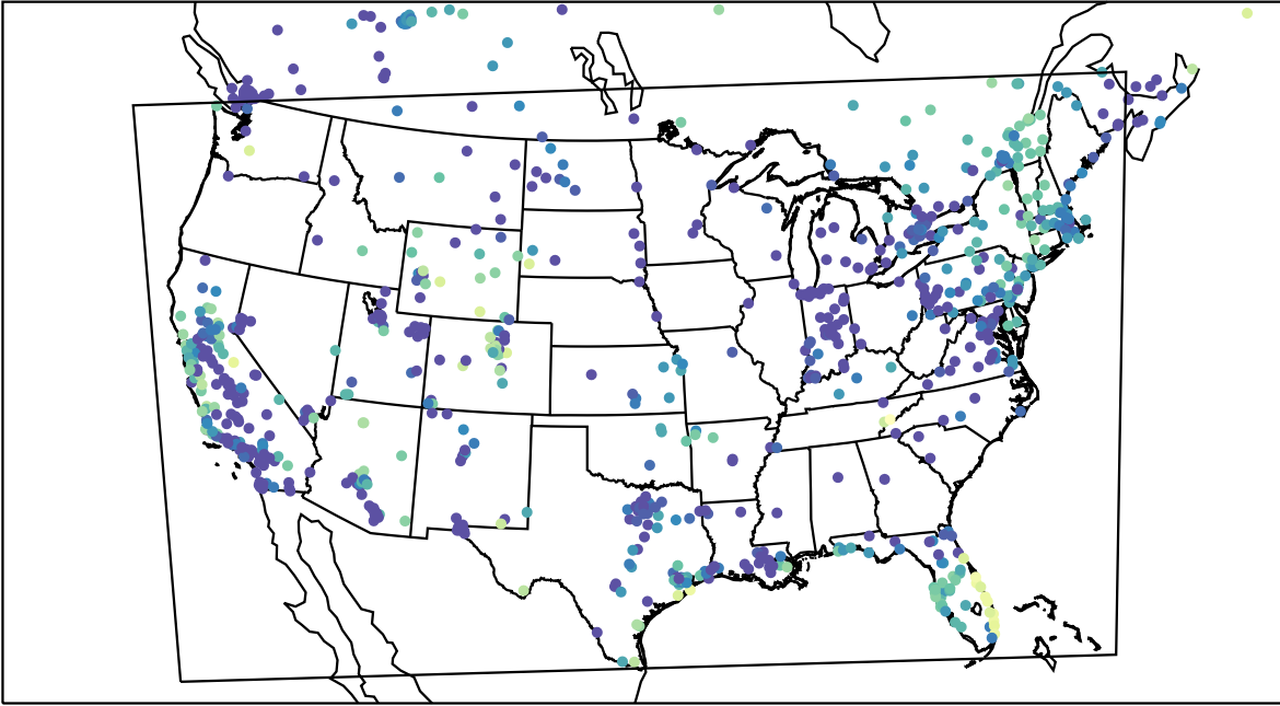
AirNOW (2023-12-20_08:00:00)
