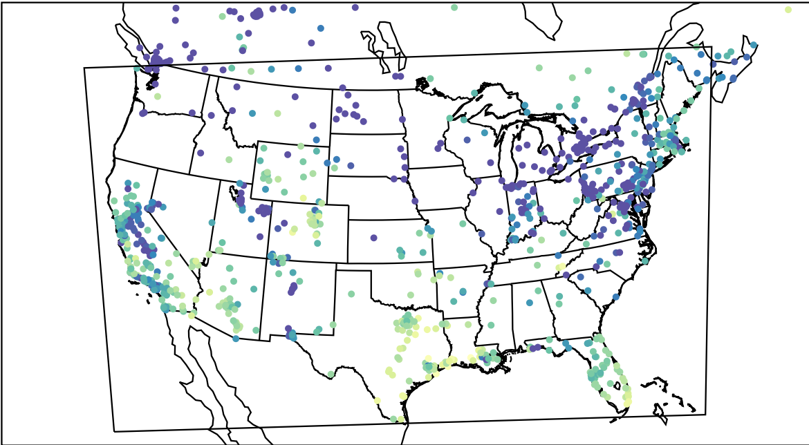
AirNOW (2023-12-20_22:00:00)
