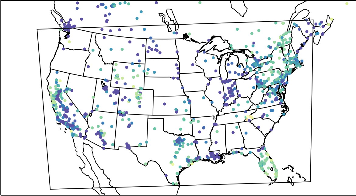
AirNOW (2023-12-20_01:00:00)
