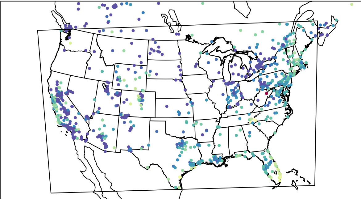
AirNOW (2023-12-20_16:00:00)
