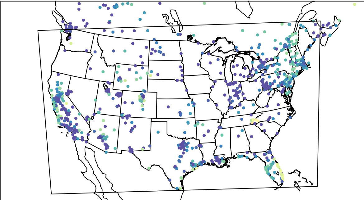
AirNOW (2023-12-20_09:00:00)
