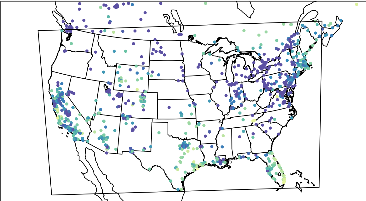
AirNOW (2023-12-21_00:00:00)
