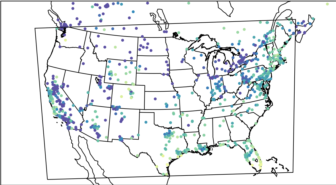
AirNOW (2023-12-20_17:00:00)
