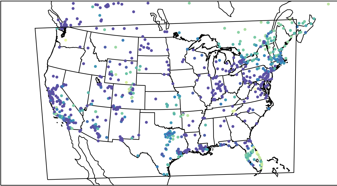
AirNOW (2023-12-21_12:00:00)
