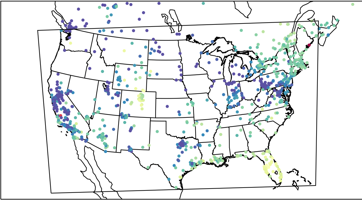
AirNOW (2023-12-21_19:00:00)
