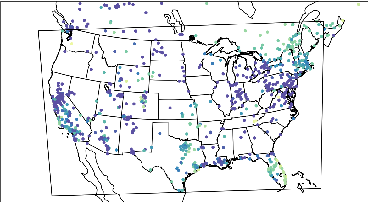
AirNOW (2023-12-21_09:00:00)
