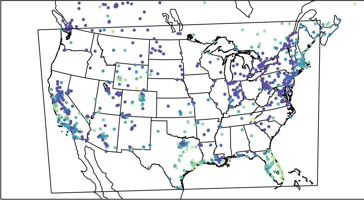
AirNOW (2023-12-21_01:00:00)
