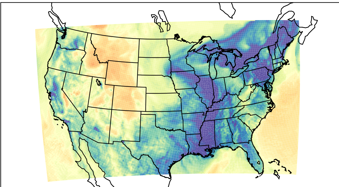
WRF (2023-12-26_06:00:00)
