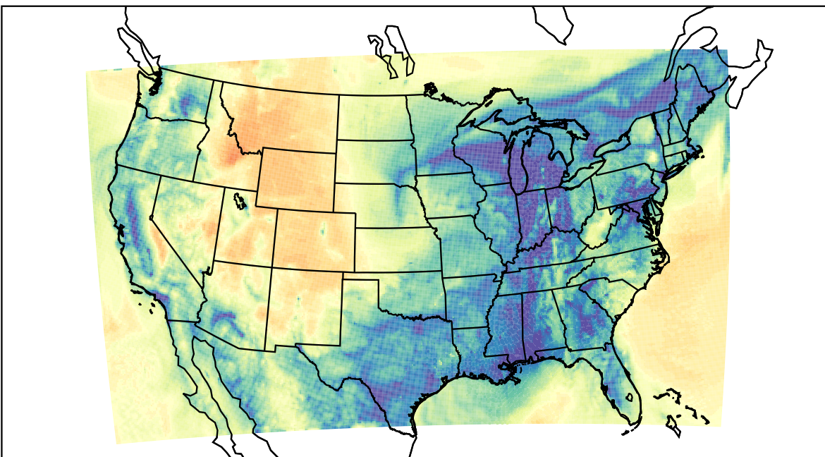
WRF (2023-12-26_15:00:00)
