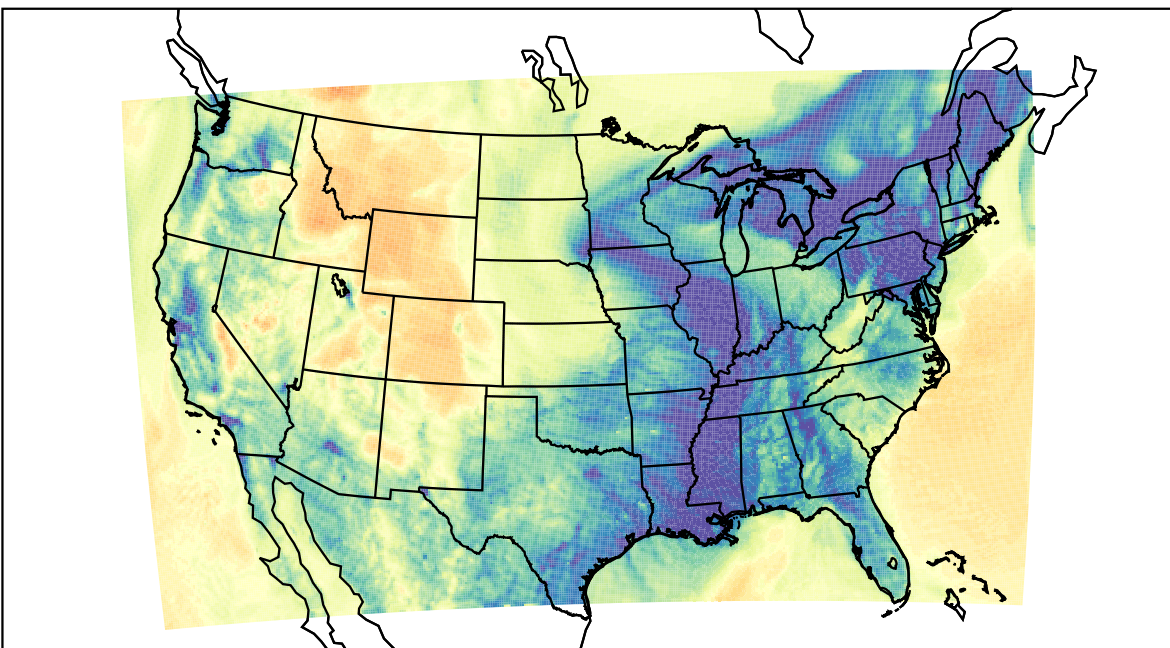
WRF (2023-12-26_05:00:00)
