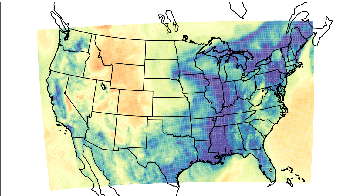
WRF (2023-12-26_08:00:00)
