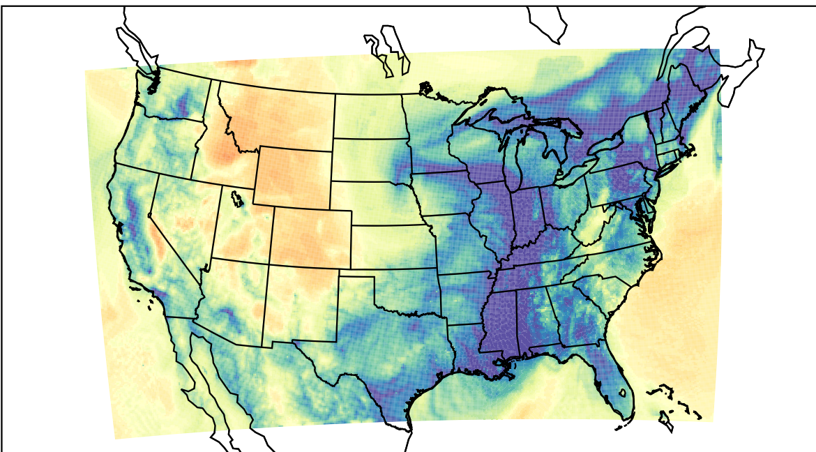
WRF (2023-12-26_10:00:00)
