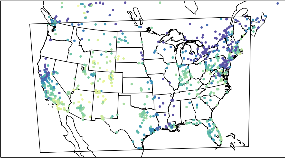
AirNOW (2023-12-25_21:00:00)
