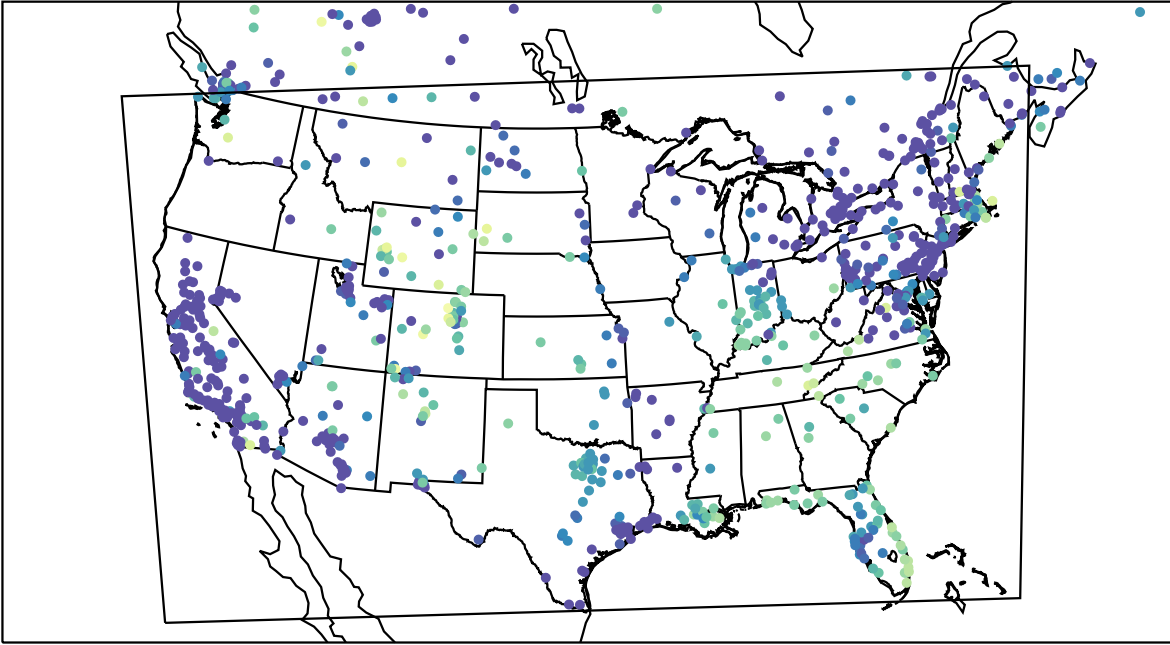
AirNOW (2023-12-25_15:00:00)
