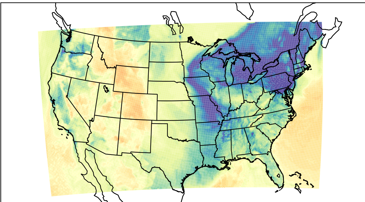
WRF (2023-12-25_22:00:00)
