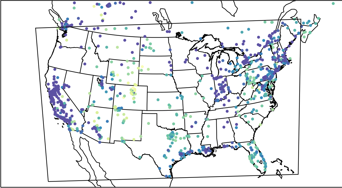
AirNOW (2023-12-26_17:00:00)
