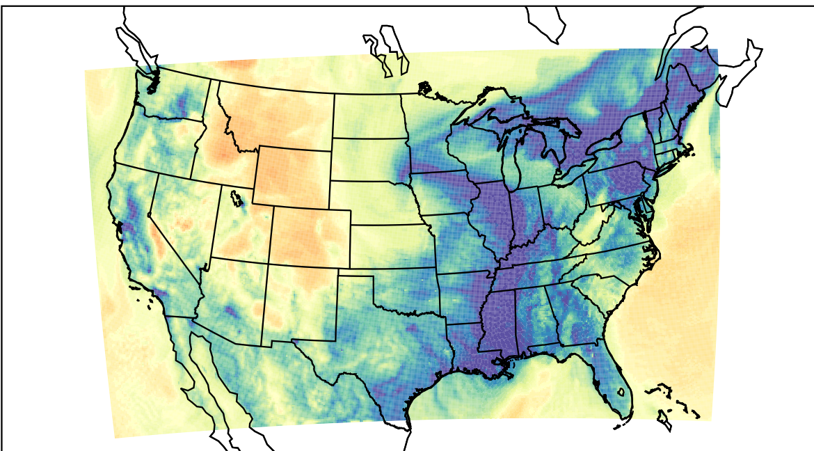
WRF (2023-12-26_07:00:00)
