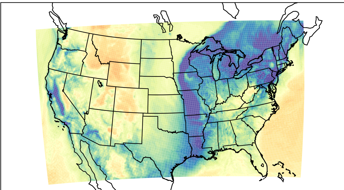
WRF (2023-12-25_17:00:00)
