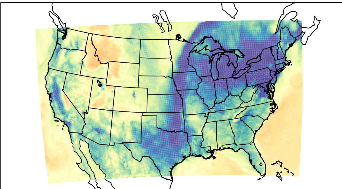
WRF (2023-12-25_05:00:00)
