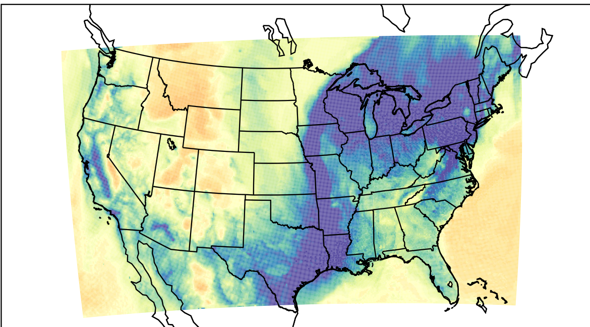
WRF (2023-12-25_13:00:00)
