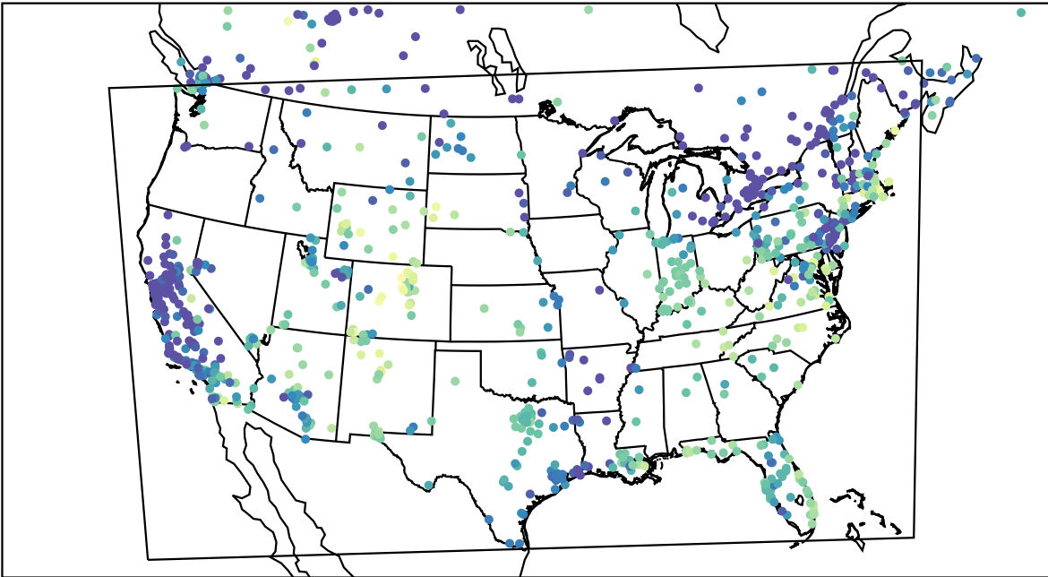
AirNOW (2023-12-25_18:00:00)
