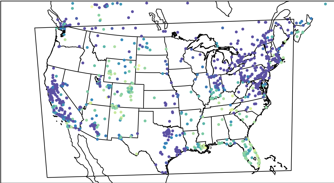
AirNOW (2023-12-25_02:00:00)
