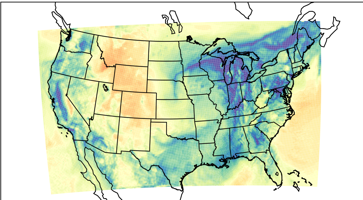
WRF (2023-12-26_17:00:00)
