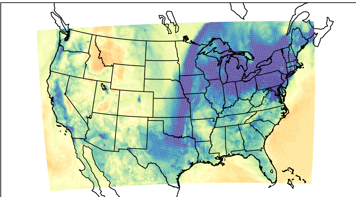
WRF (2023-12-25_03:00:00)
