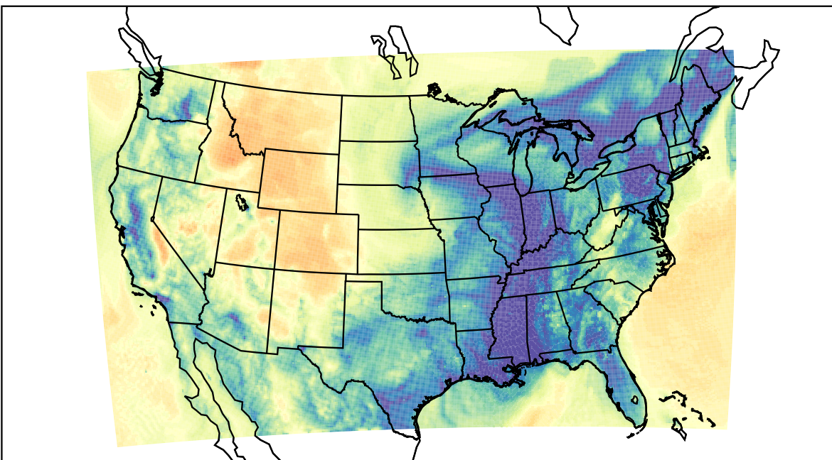
WRF (2023-12-26_09:00:00)
