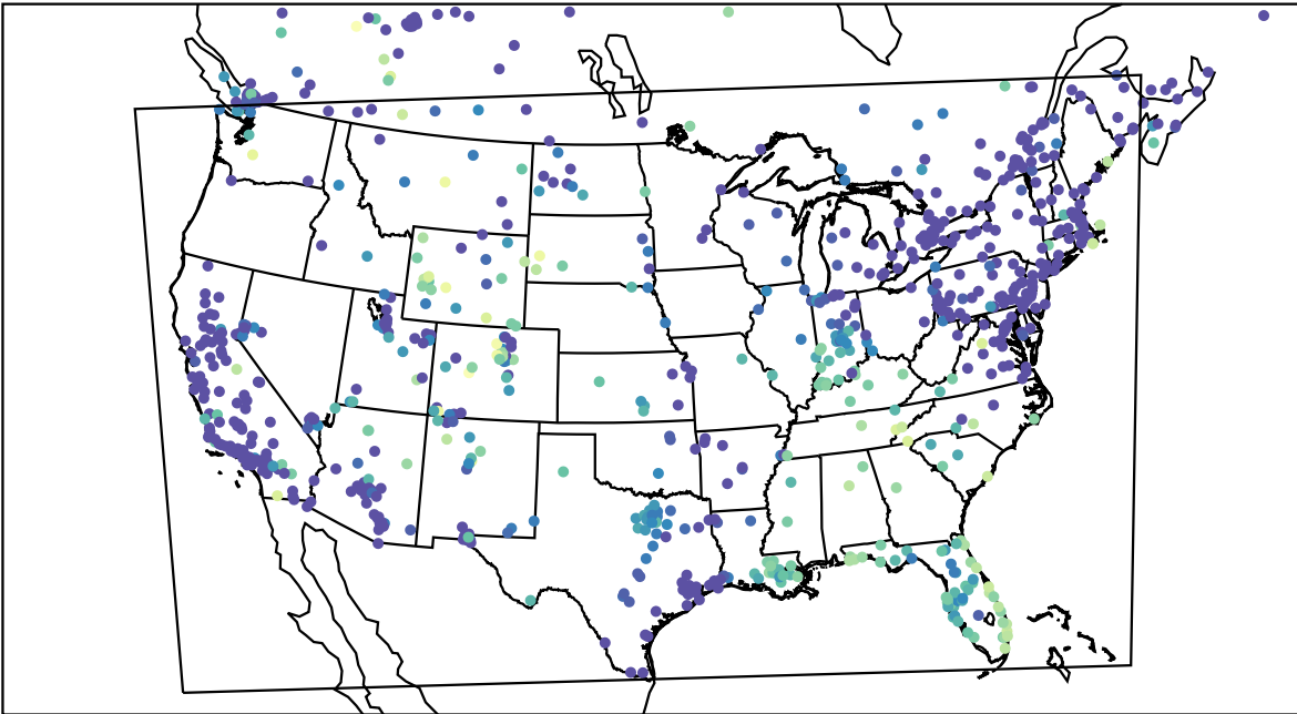
AirNOW (2023-12-25_11:00:00)
