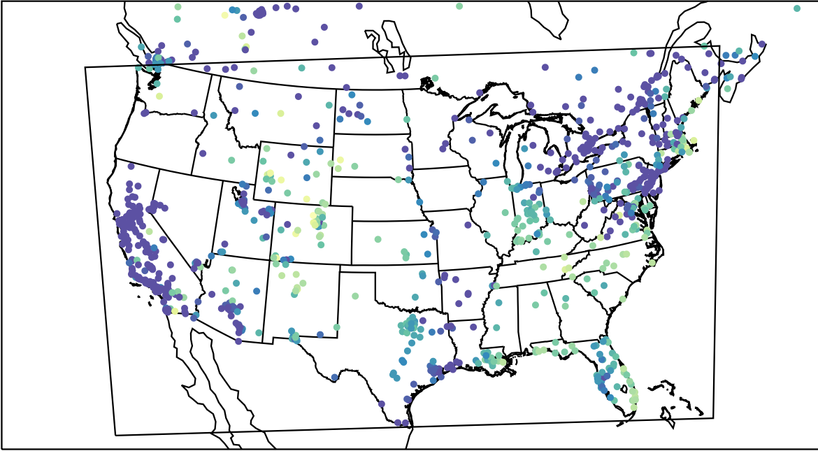
AirNOW (2023-12-25_16:00:00)
