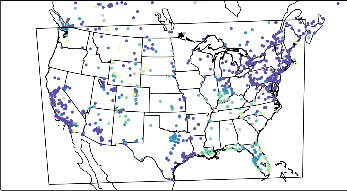
AirNOW (2023-12-25_12:00:00)
