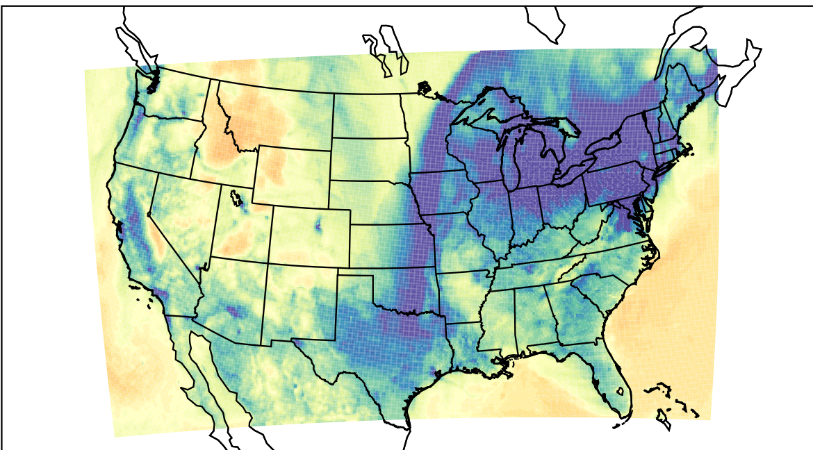
WRF (2023-12-25_04:00:00)
