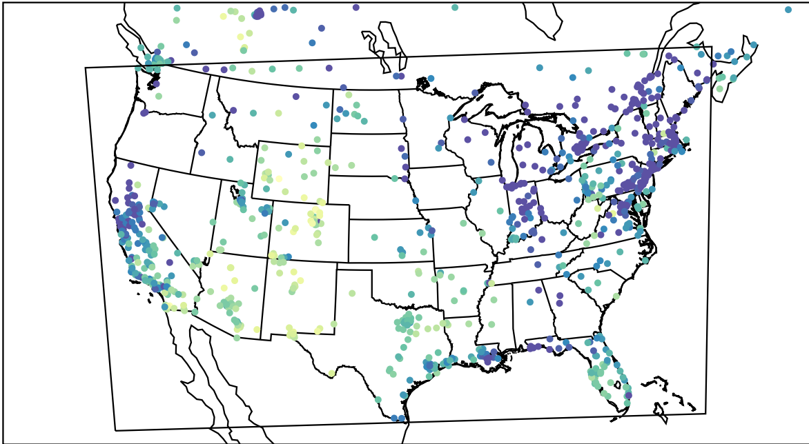
AirNOW (2023-12-26_21:00:00)
