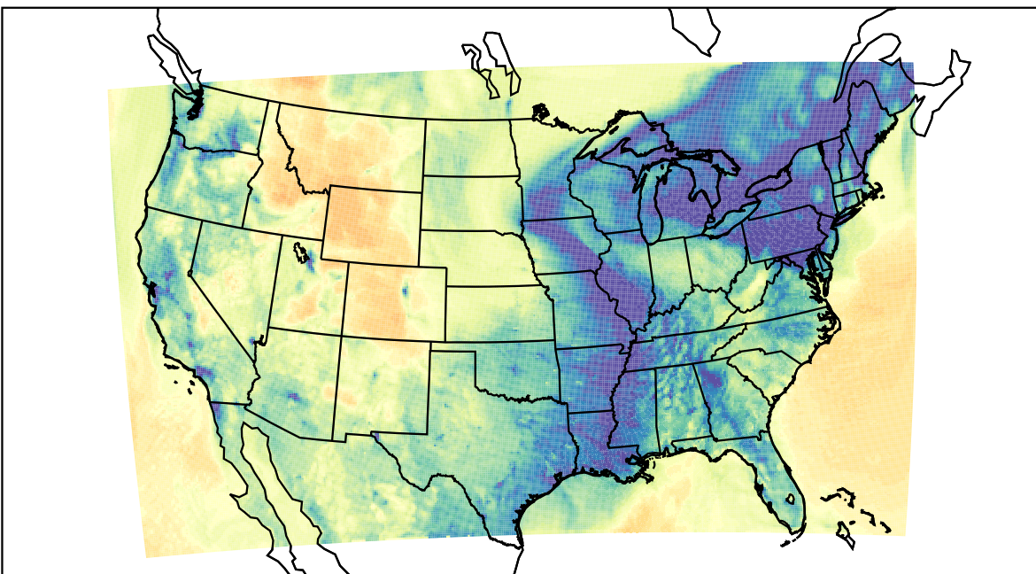
WRF (2023-12-26_01:00:00)
