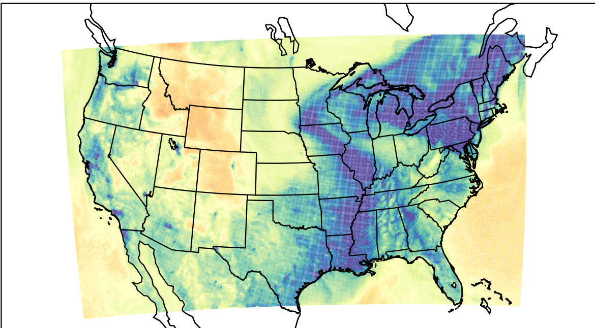
WRF (2023-12-26_02:00:00)
