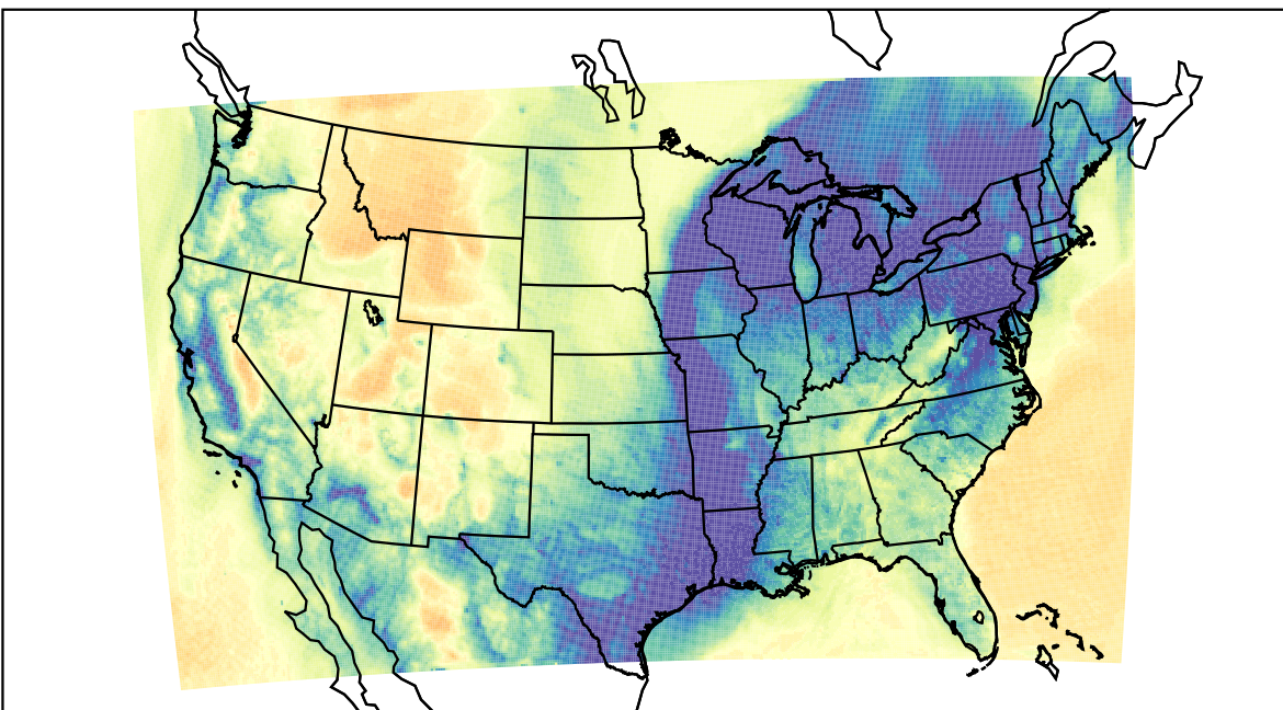
WRF (2023-12-25_14:00:00)
