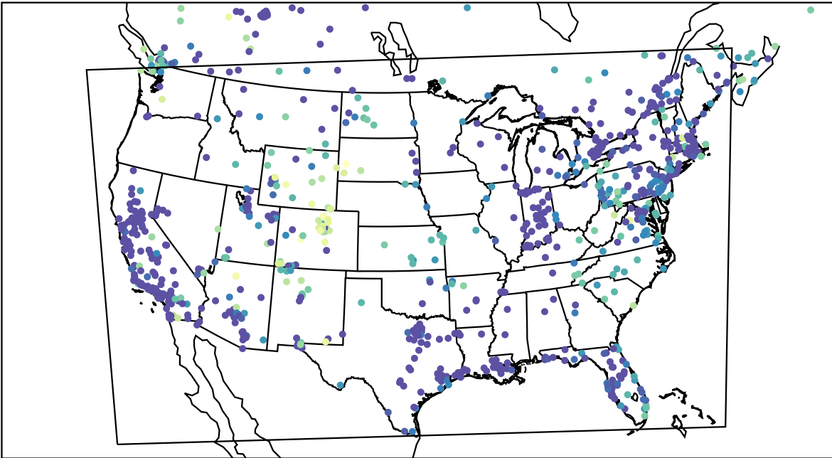
AirNOW (2023-12-26_14:00:00)
