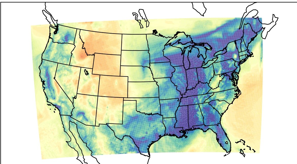
WRF (2023-12-26_13:00:00)
