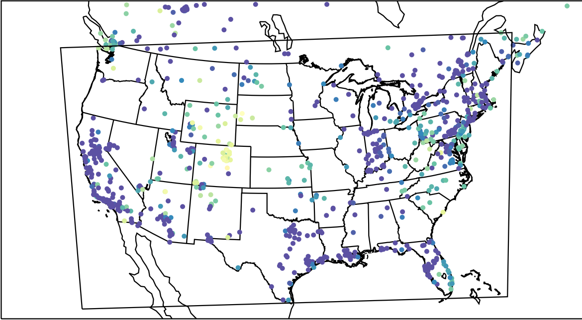
AirNOW (2023-12-26_11:00:00)
