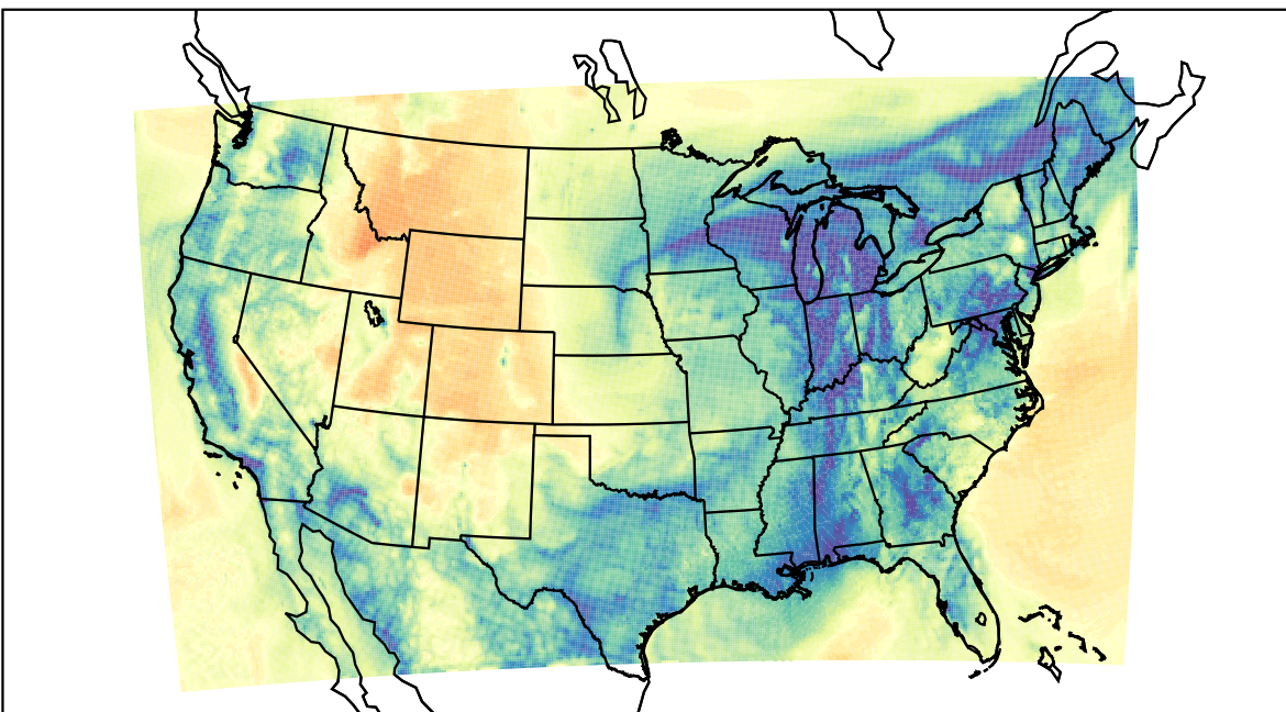
WRF (2023-12-26_16:00:00)
