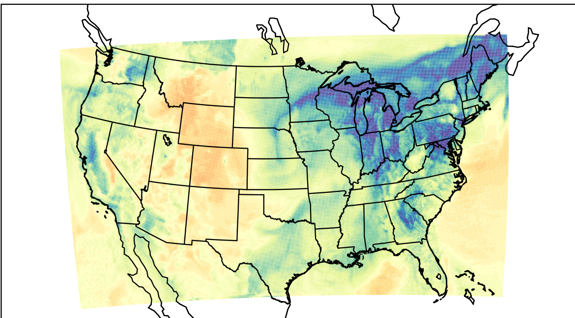
WRF (2023-12-26_20:00:00)
