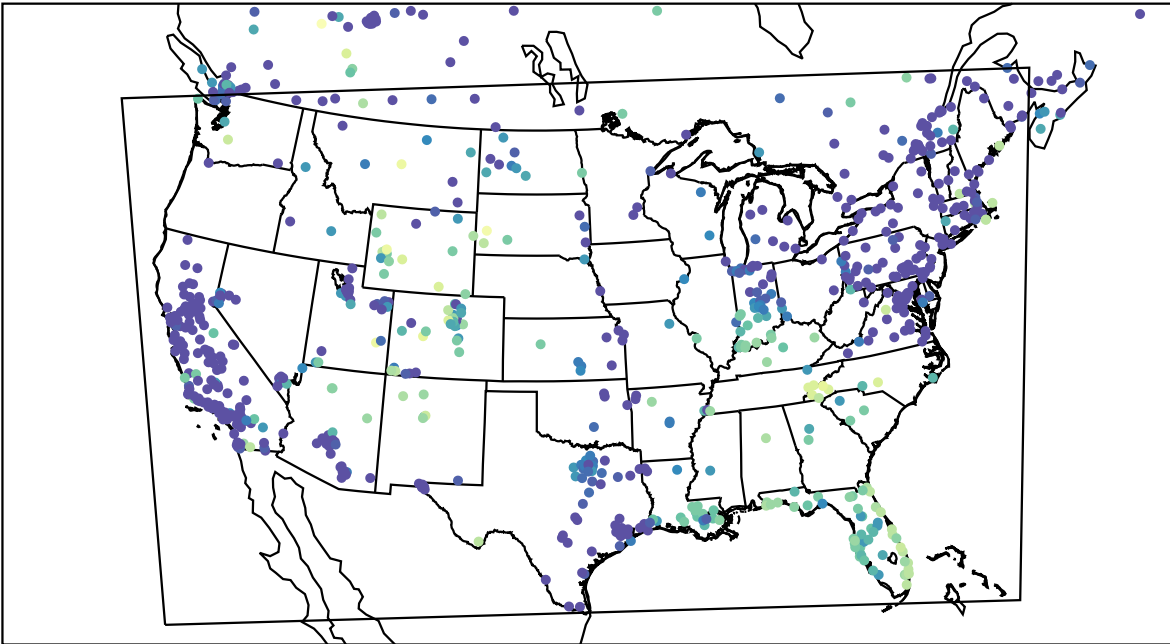
AirNOW (2023-12-25_08:00:00)
