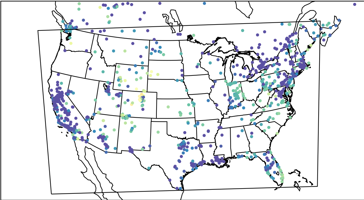
AirNOW (2023-12-26_03:00:00)
