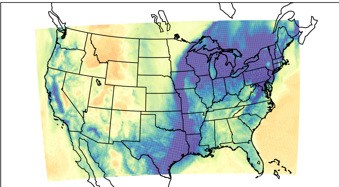
WRF (2023-12-25_12:00:00)
