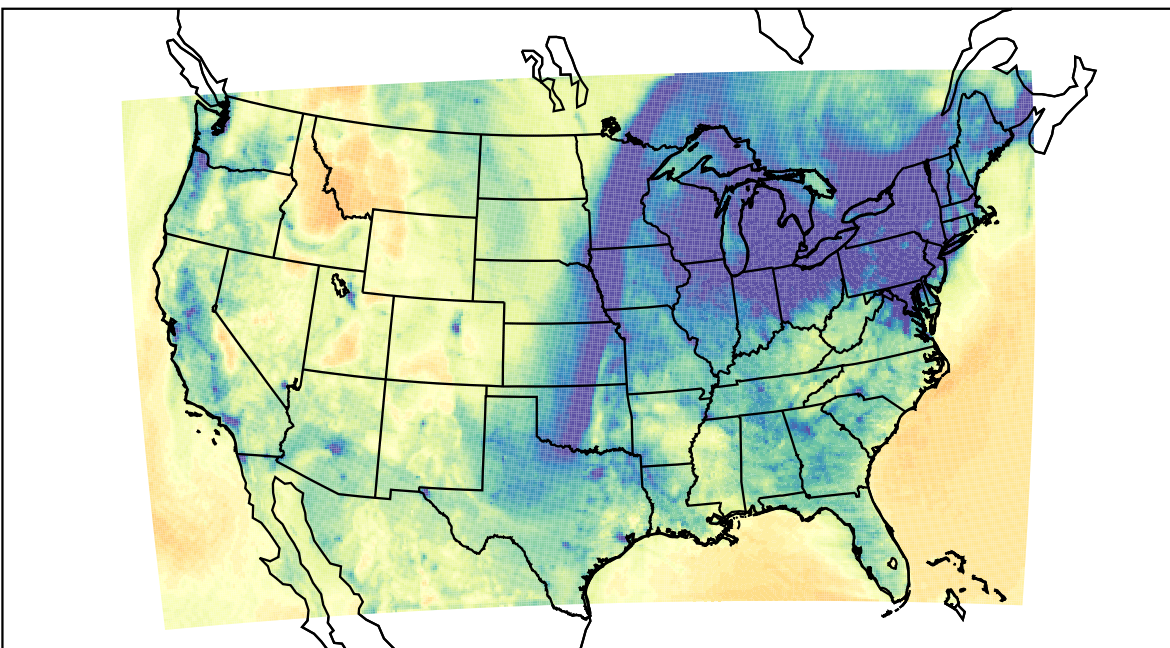
WRF (2023-12-25_01:00:00)
