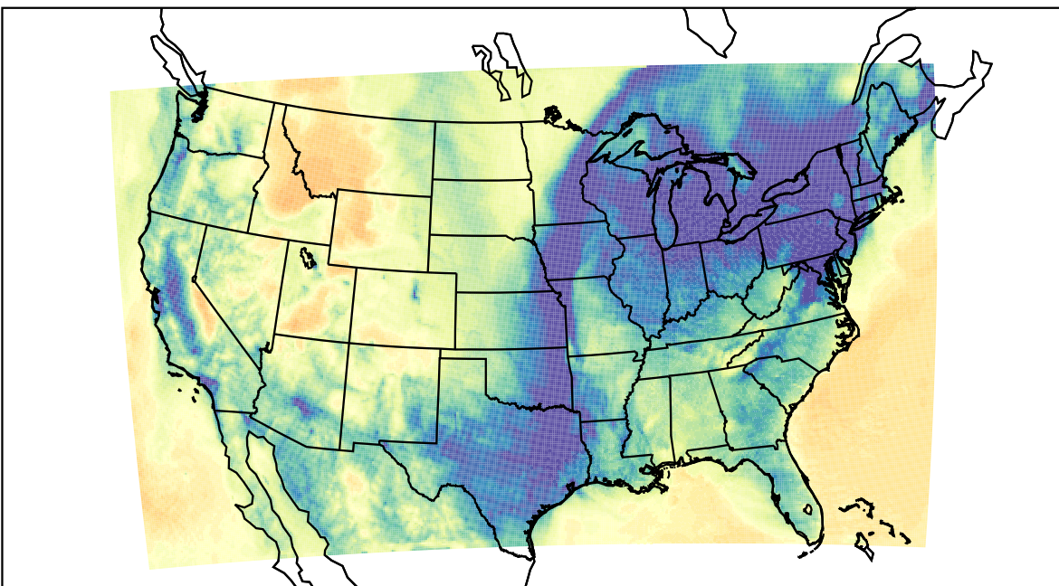
WRF (2023-12-25_07:00:00)
