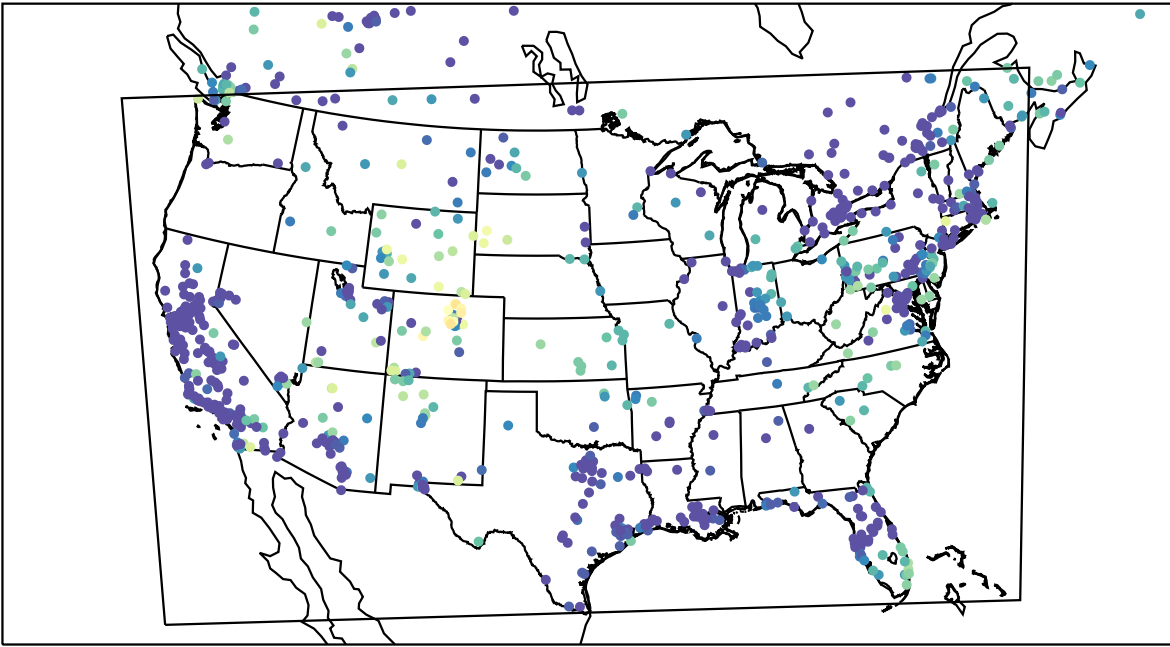
AirNOW (2023-12-26_07:00:00)
