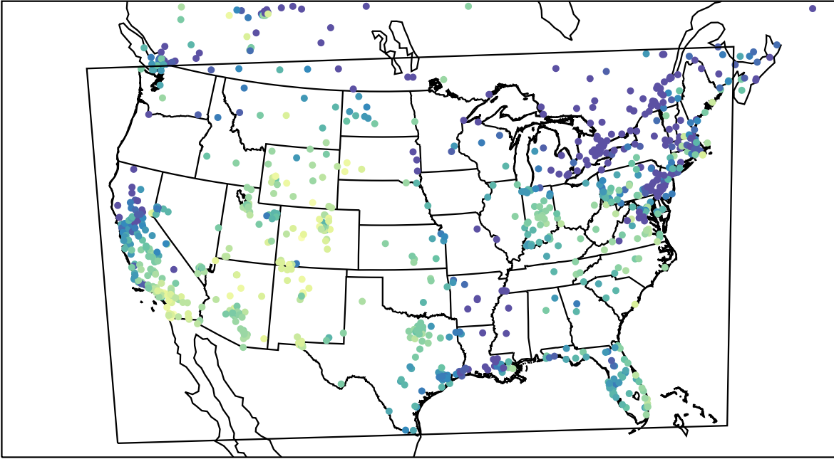
AirNOW (2023-12-25_22:00:00)
