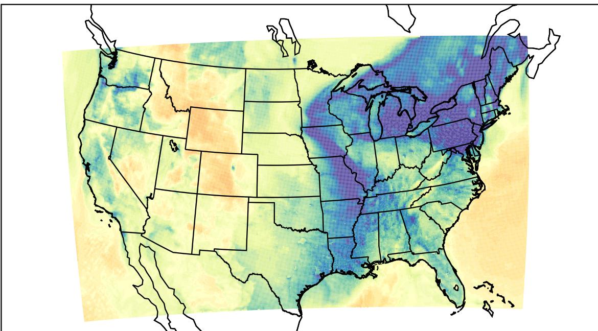
WRF (2023-12-25_23:00:00)
