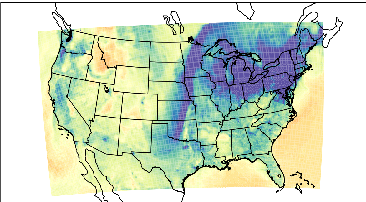
WRF (2023-12-25_00:00:00)
