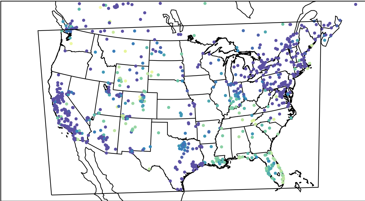
AirNOW (2023-12-25_09:00:00)
