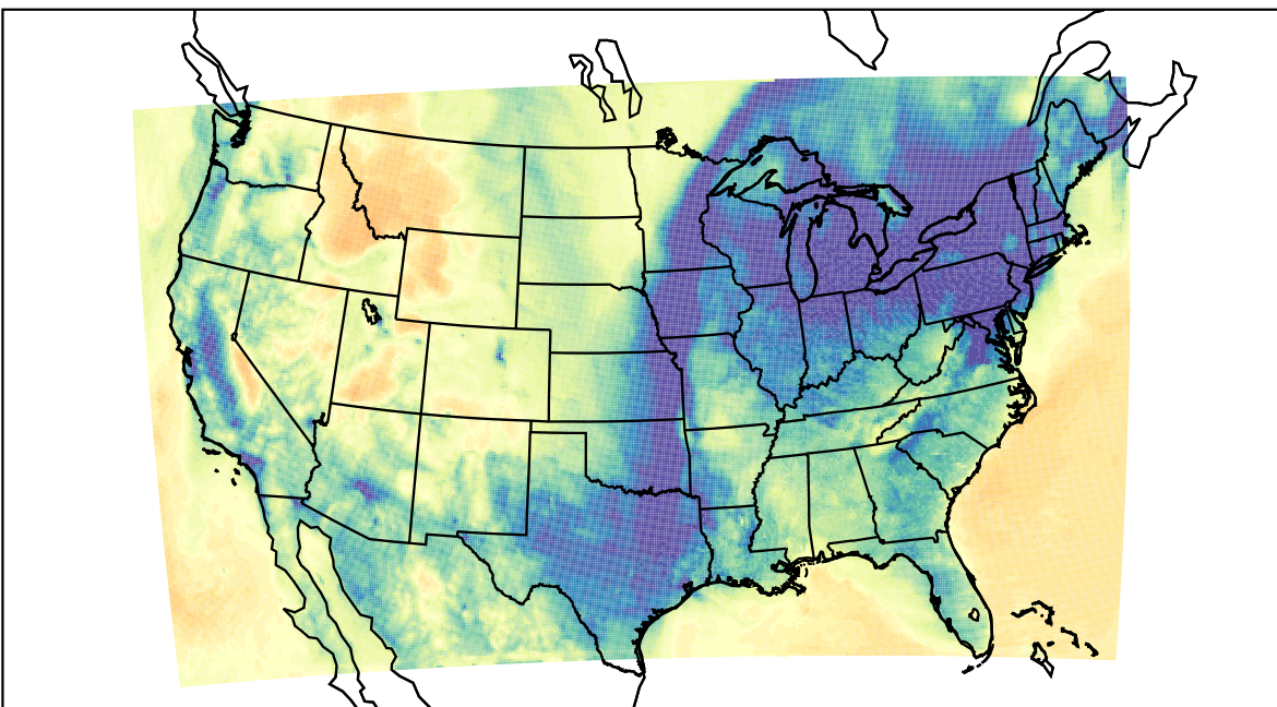
WRF (2023-12-25_06:00:00)
