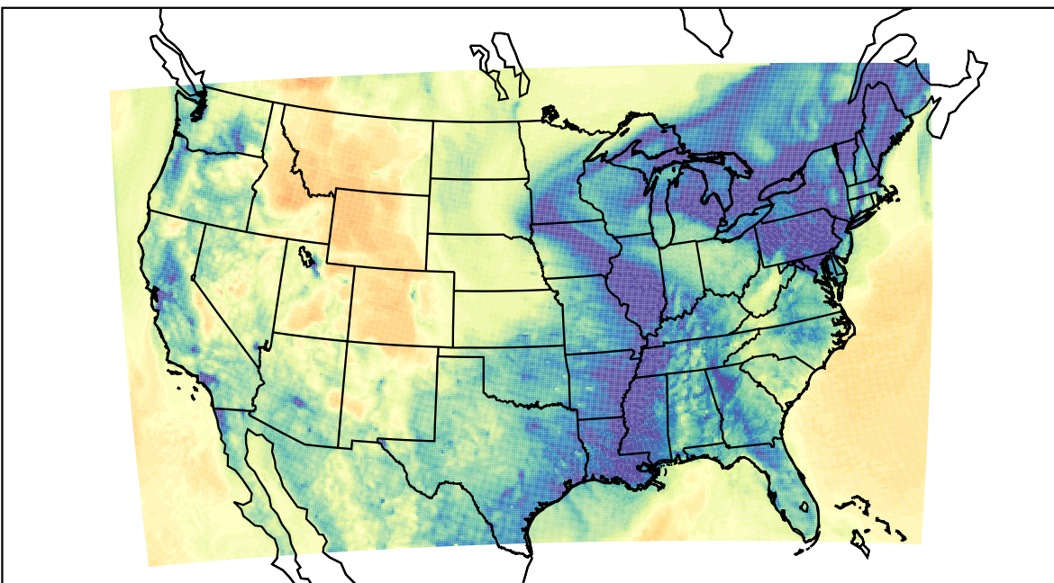
WRF (2023-12-26_03:00:00)
