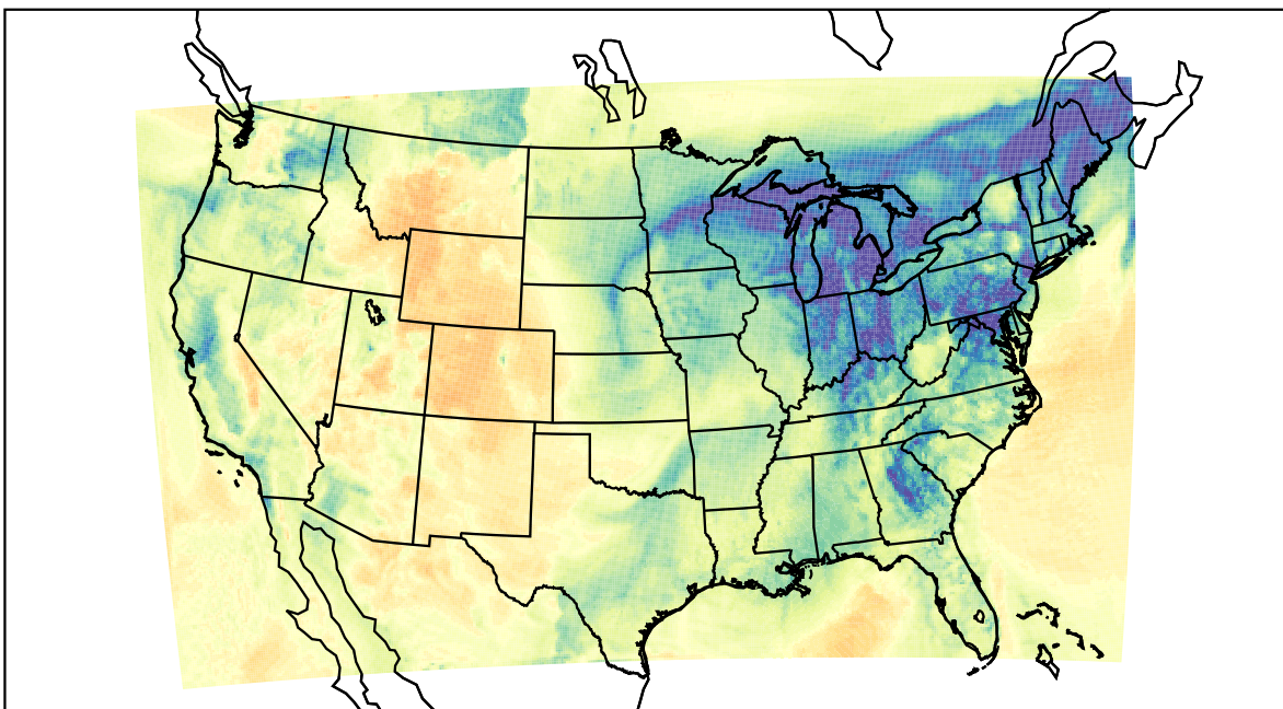
WRF (2023-12-26_21:00:00)
