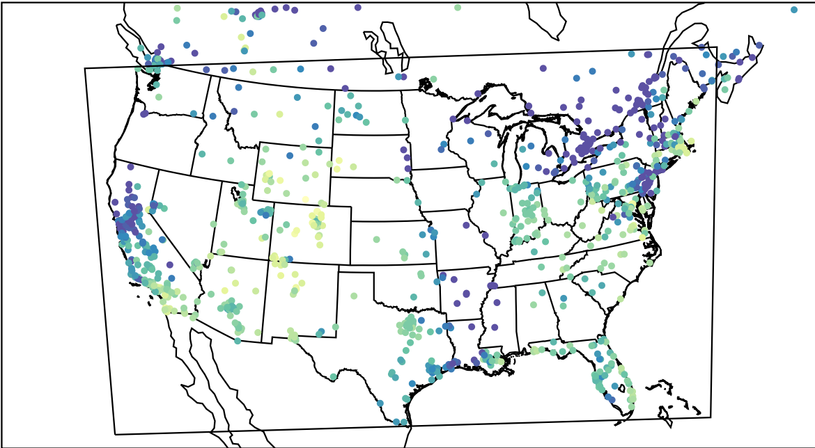
AirNOW (2023-12-25_20:00:00)
