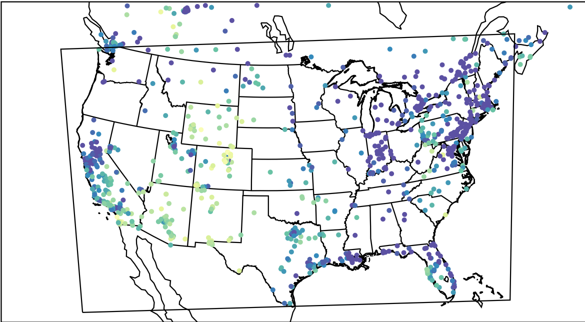
AirNOW (2023-12-26_23:00:00)
