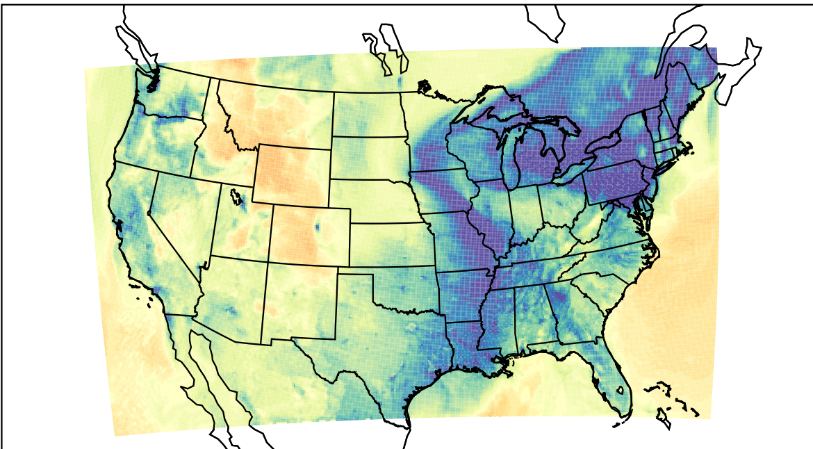
WRF (2023-12-26_00:00:00)
