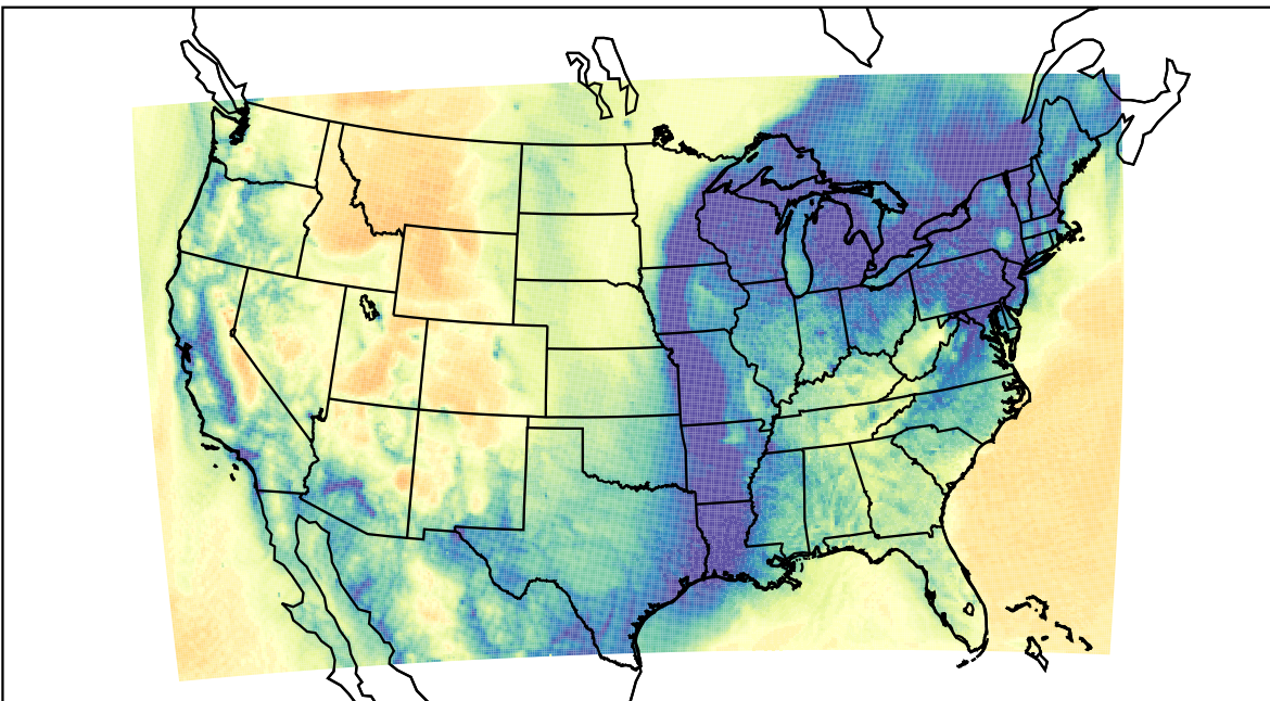
WRF (2023-12-25_15:00:00)
