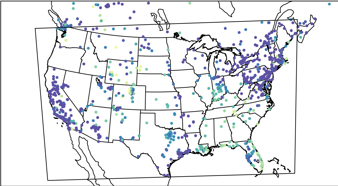
AirNOW (2023-12-25_14:00:00)
