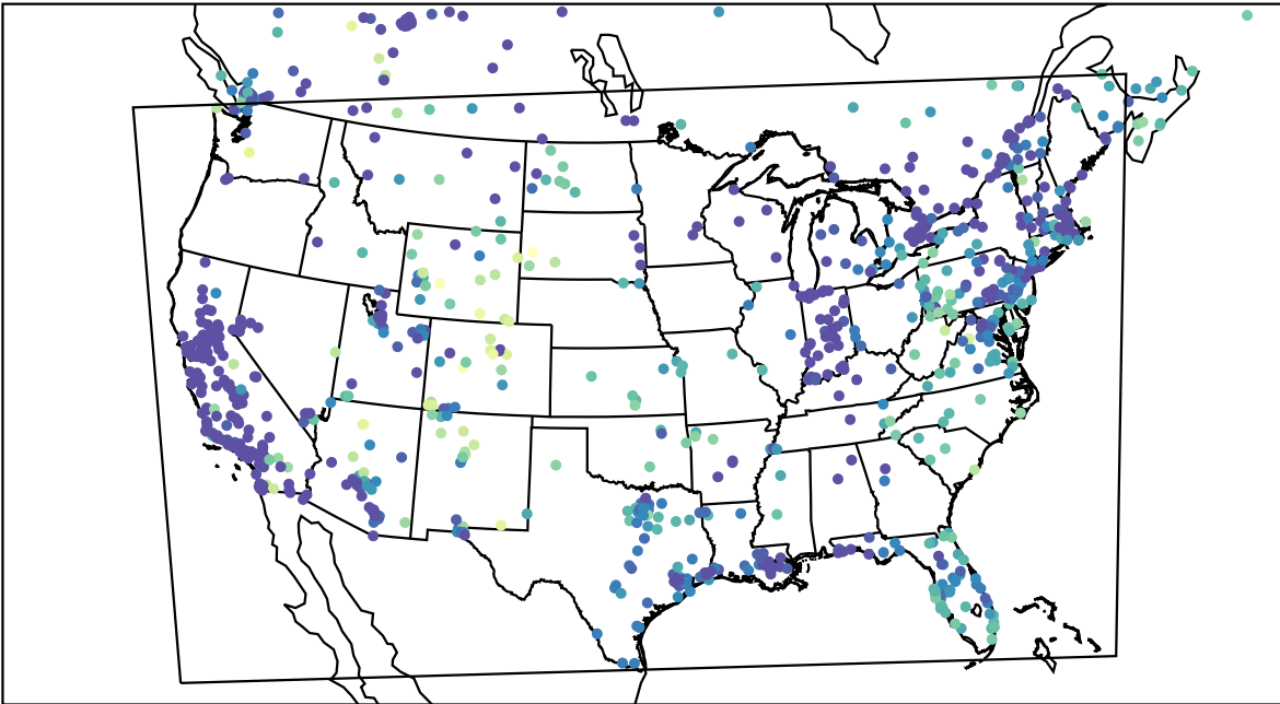
AirNOW (2023-12-26_16:00:00)
