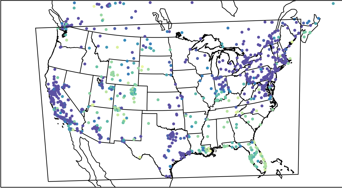
AirNOW (2023-12-25_03:00:00)
