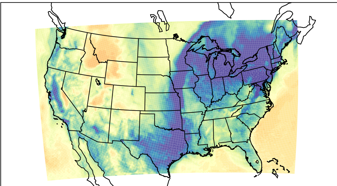
WRF (2023-12-25_08:00:00)
