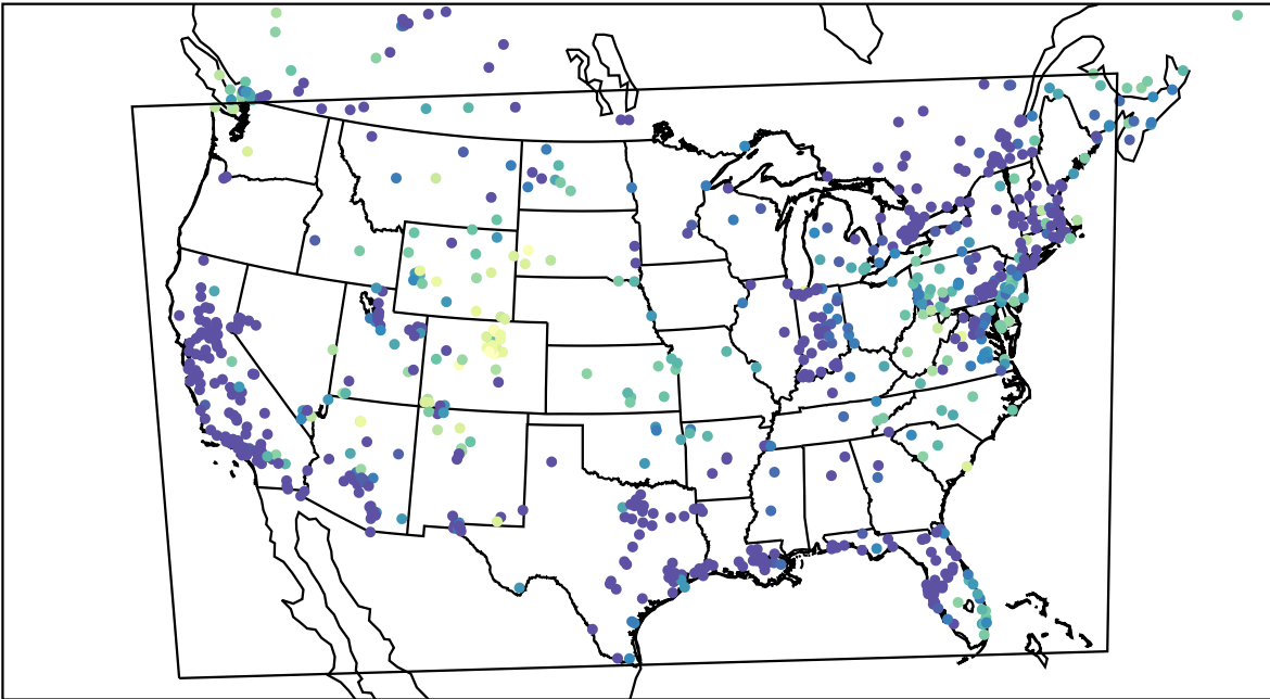
AirNOW (2023-12-26_10:00:00)
