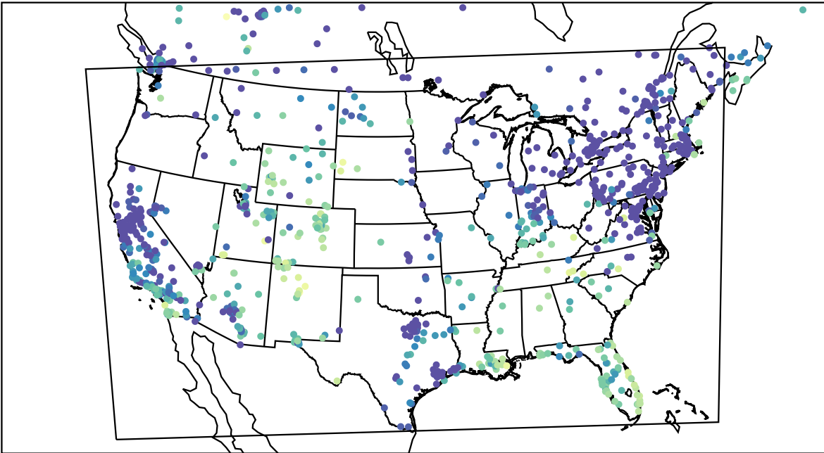
AirNOW (2023-12-25_01:00:00)
