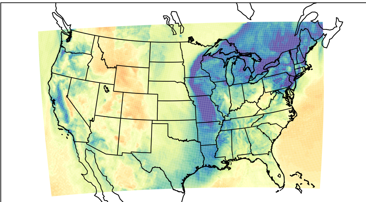
WRF (2023-12-25_19:00:00)
