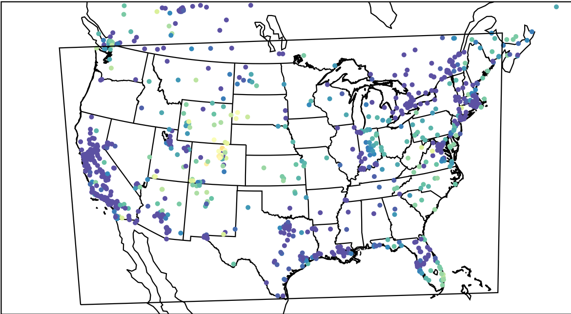
AirNOW (2023-12-26_06:00:00)
