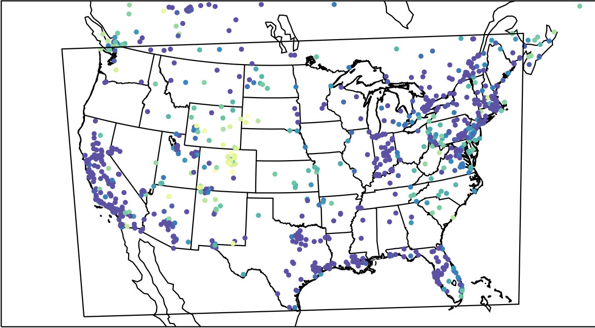
AirNOW (2023-12-26_13:00:00)
