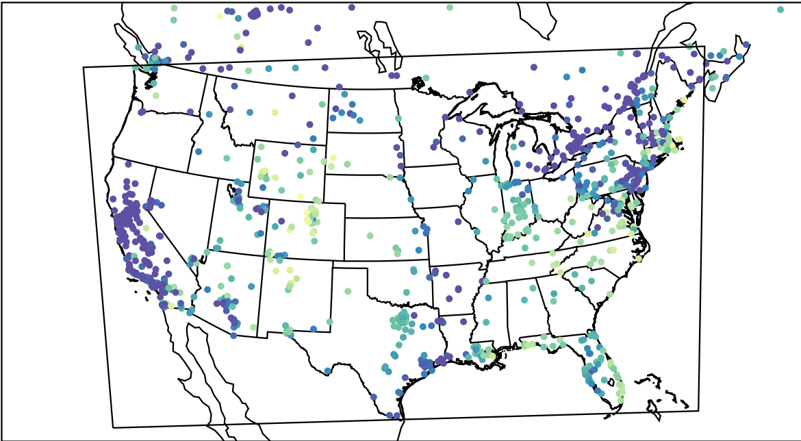
AirNOW (2023-12-25_17:00:00)
