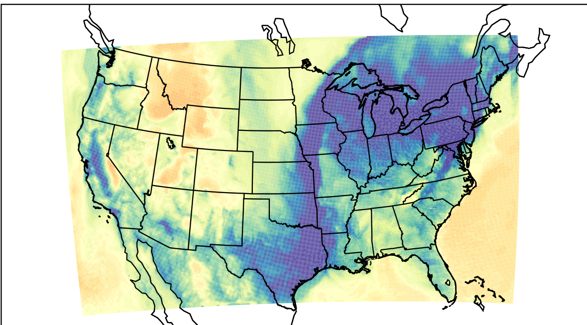
WRF (2023-12-25_09:00:00)
