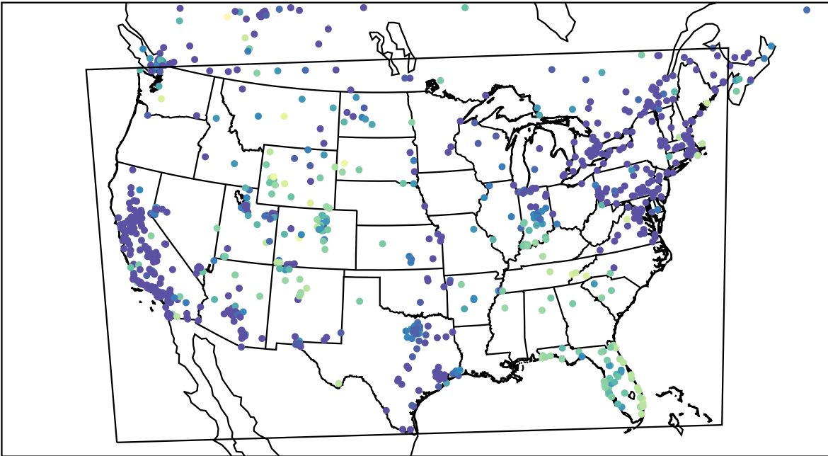
AirNOW (2023-12-25_07:00:00)
