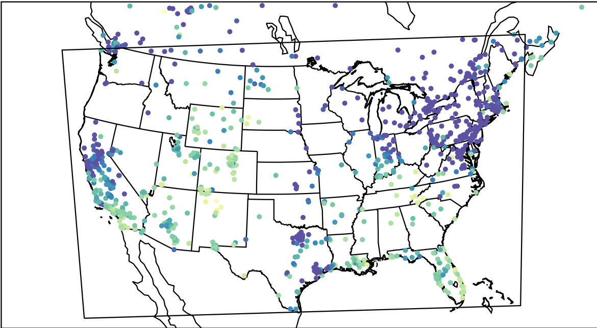
AirNOW (2023-12-25_00:00:00)
