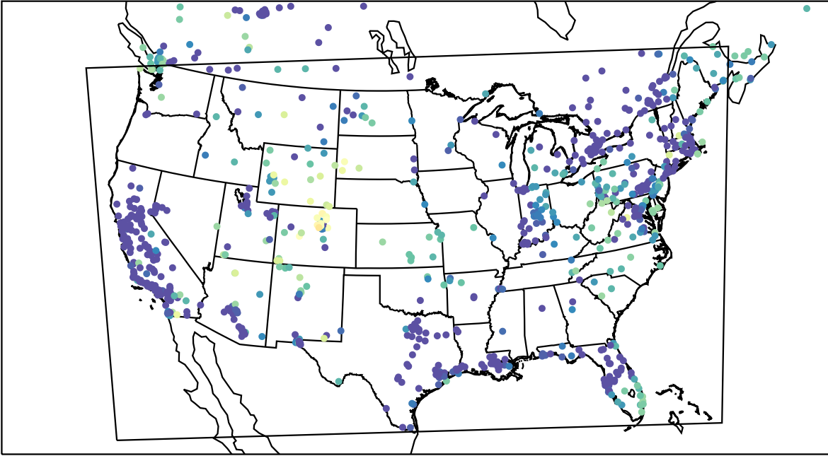
AirNOW (2023-12-26_08:00:00)
