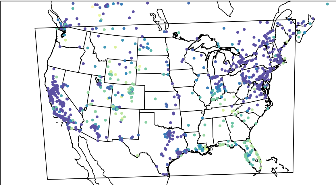
AirNOW (2023-12-25_05:00:00)
