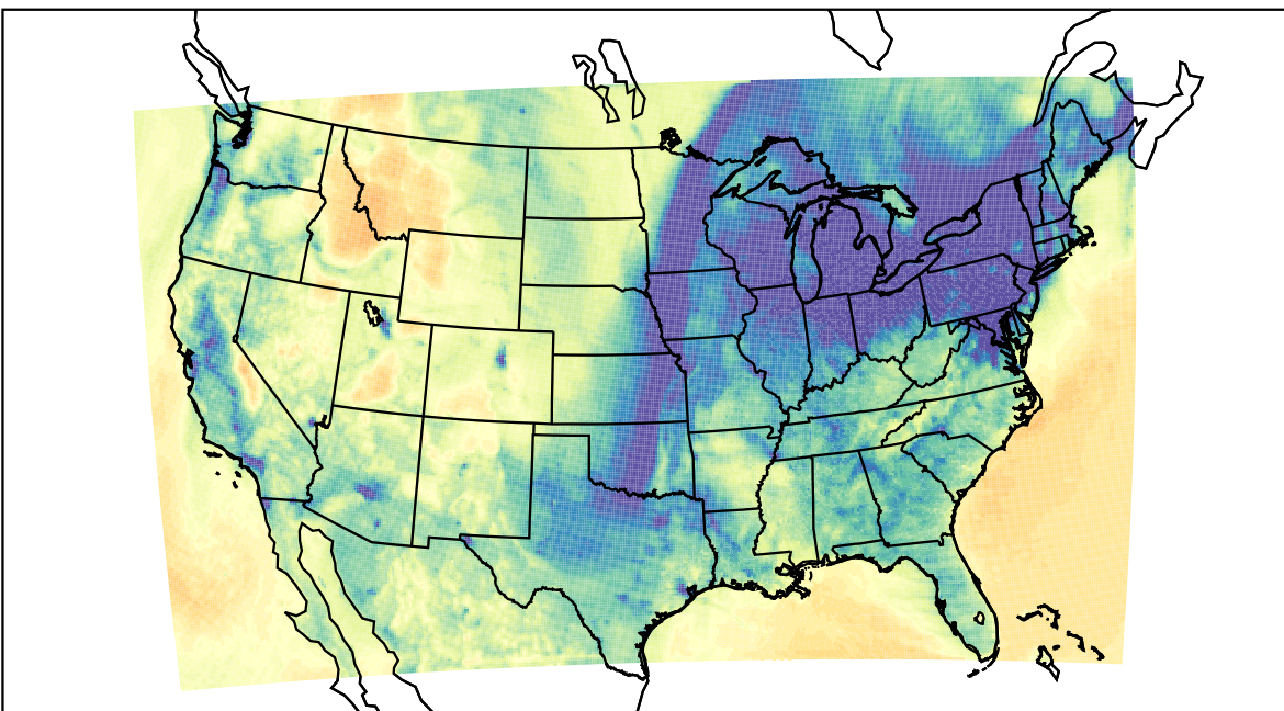
WRF (2023-12-25_02:00:00)
