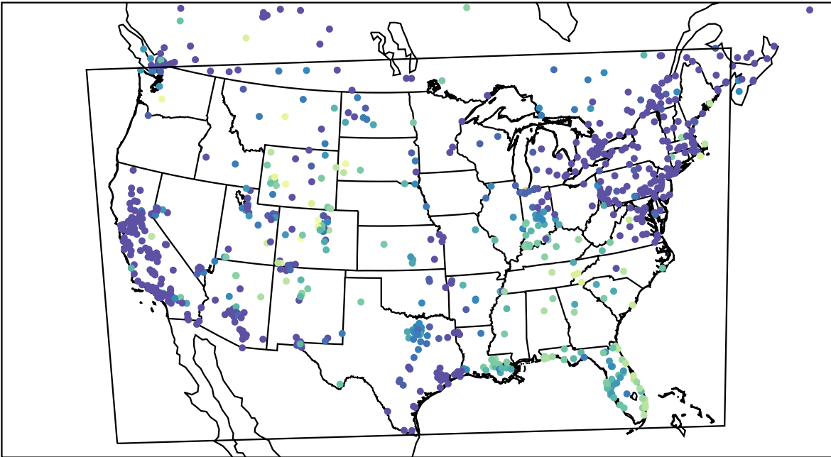
AirNOW (2023-12-25_10:00:00)
