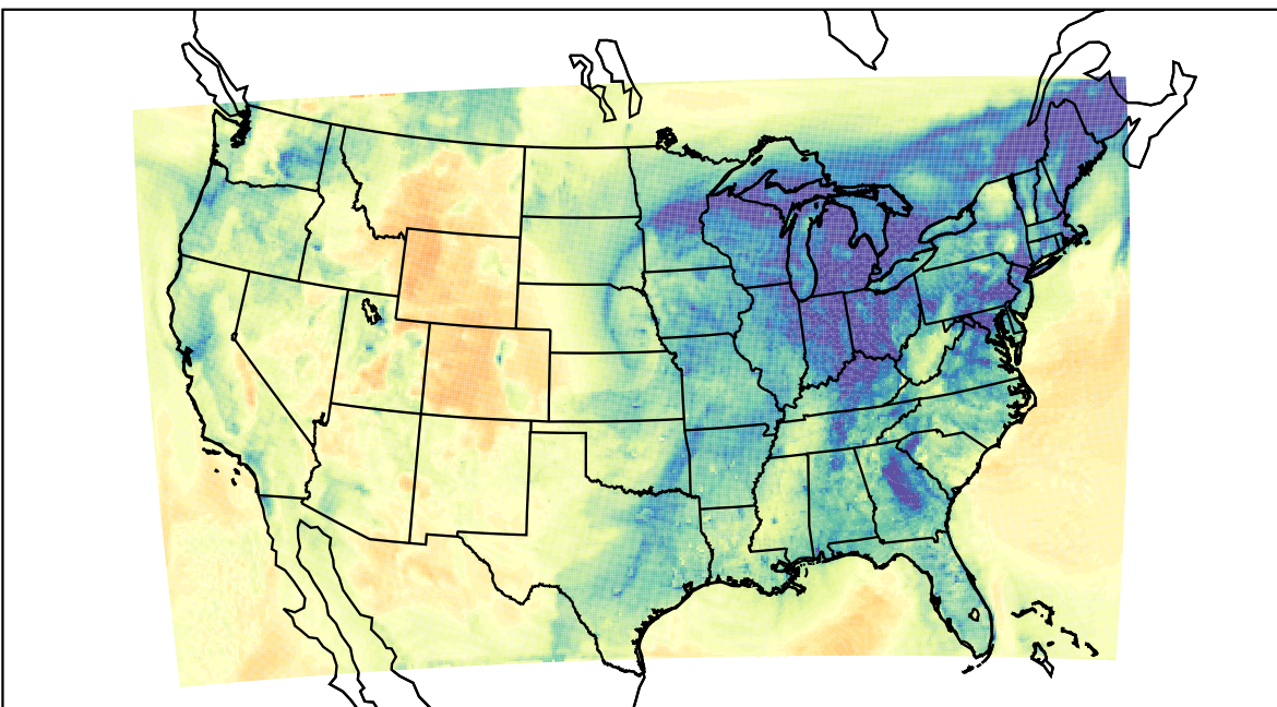
WRF (2023-12-26_23:00:00)
