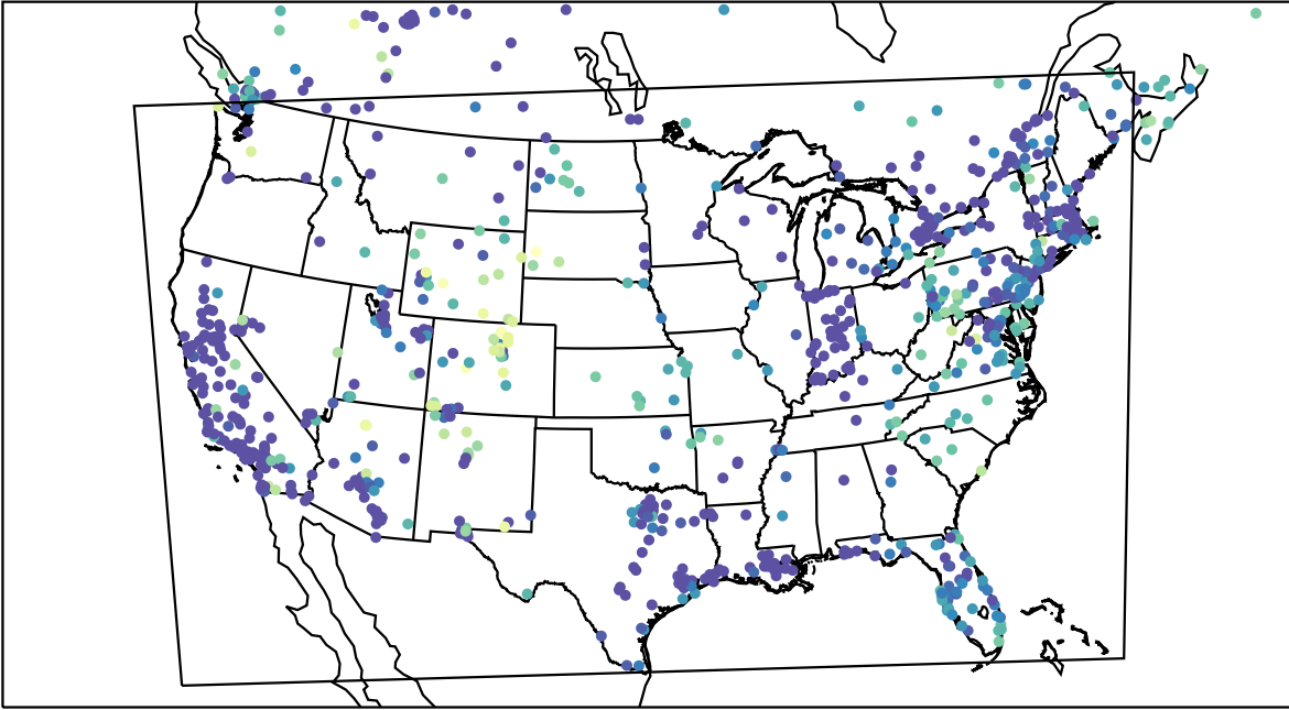
AirNOW (2023-12-26_15:00:00)
