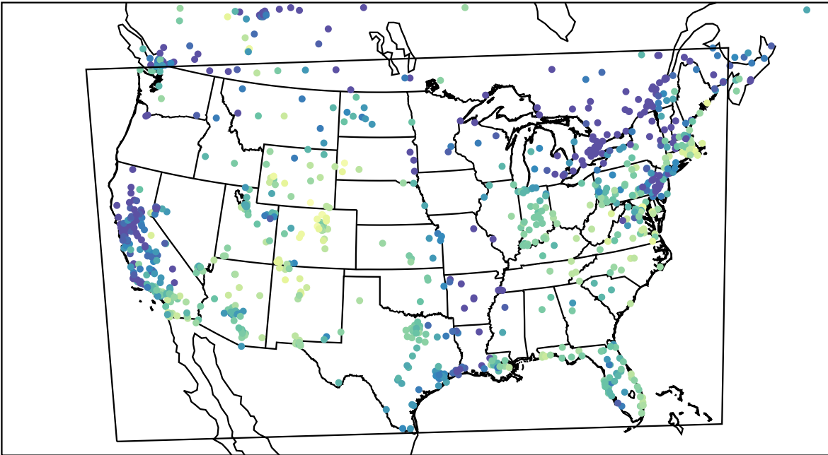
AirNOW (2023-12-25_19:00:00)
