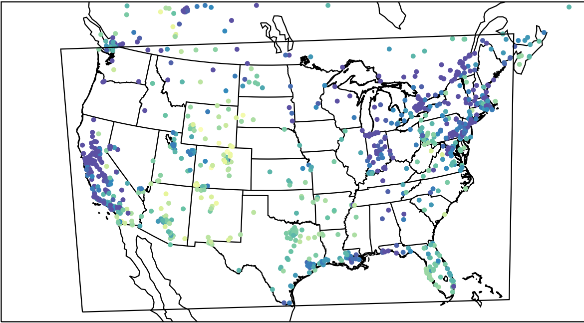
AirNOW (2023-12-26_19:00:00)
