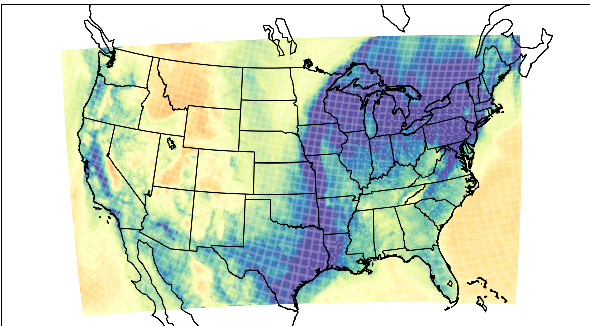
WRF (2023-12-25_11:00:00)
