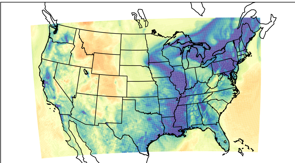
WRF (2023-12-26_04:00:00)
