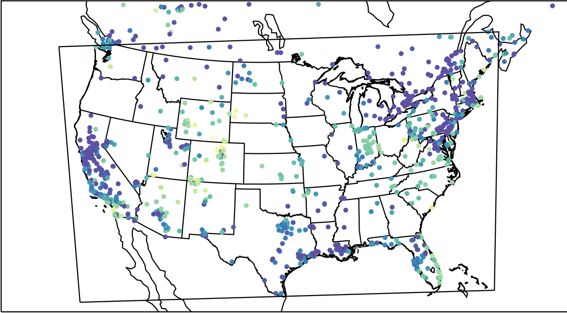
AirNOW (2023-12-26_01:00:00)
