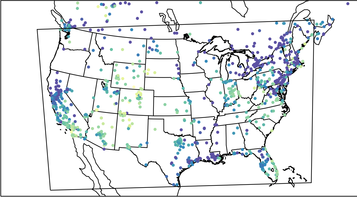
AirNOW (2023-12-26_00:00:00)
