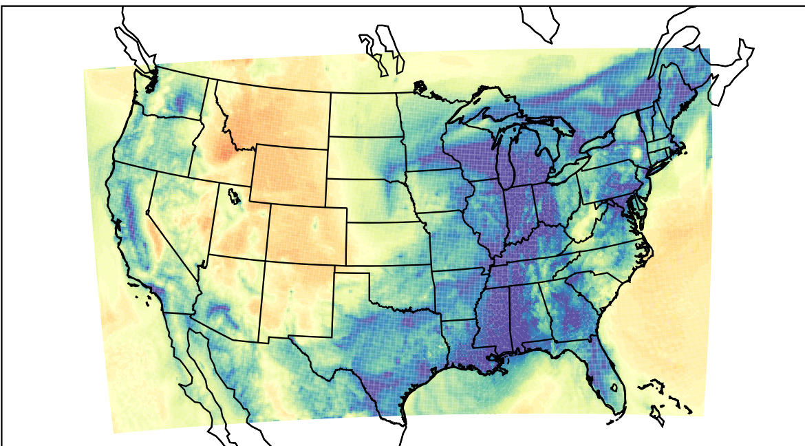
WRF (2023-12-26_14:00:00)
