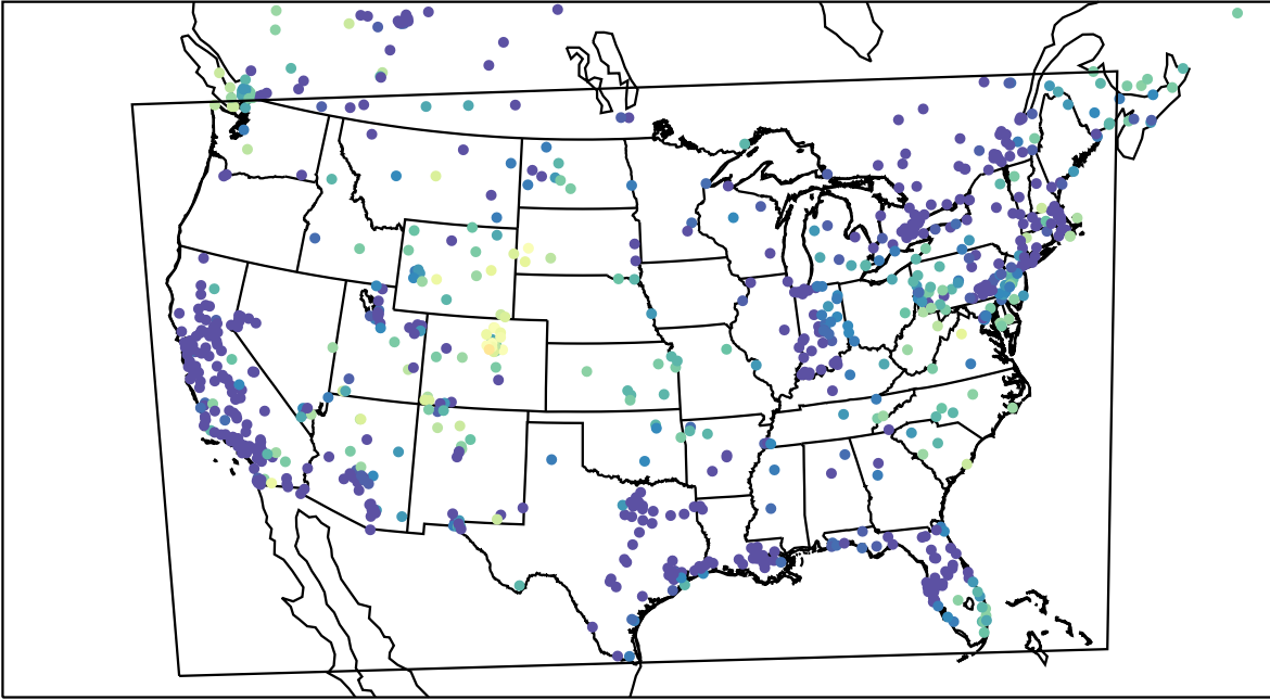
AirNOW (2023-12-26_09:00:00)
