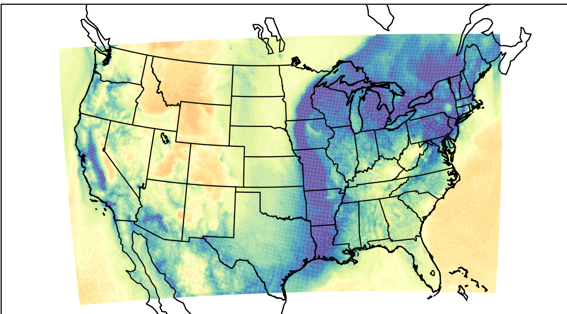
WRF (2023-12-25_16:00:00)
