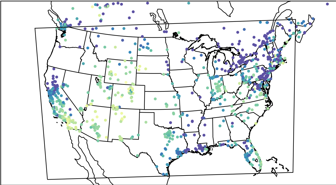
AirNOW (2023-12-25_23:00:00)
