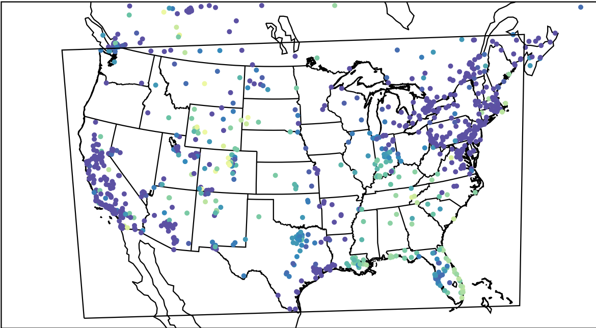
AirNOW (2023-12-25_13:00:00)
