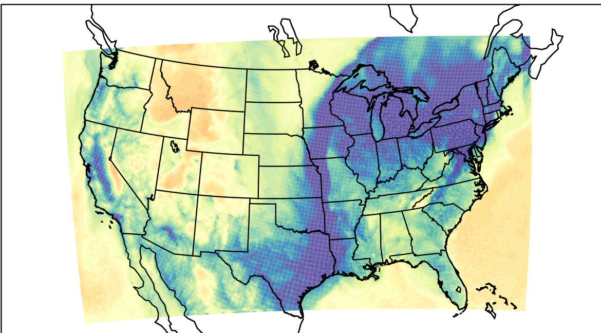
WRF (2023-12-25_10:00:00)
