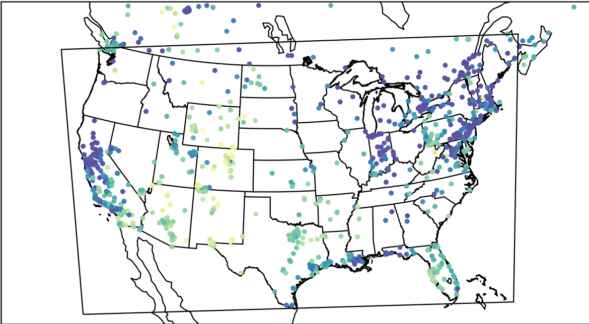
AirNOW (2023-12-26_20:00:00)
