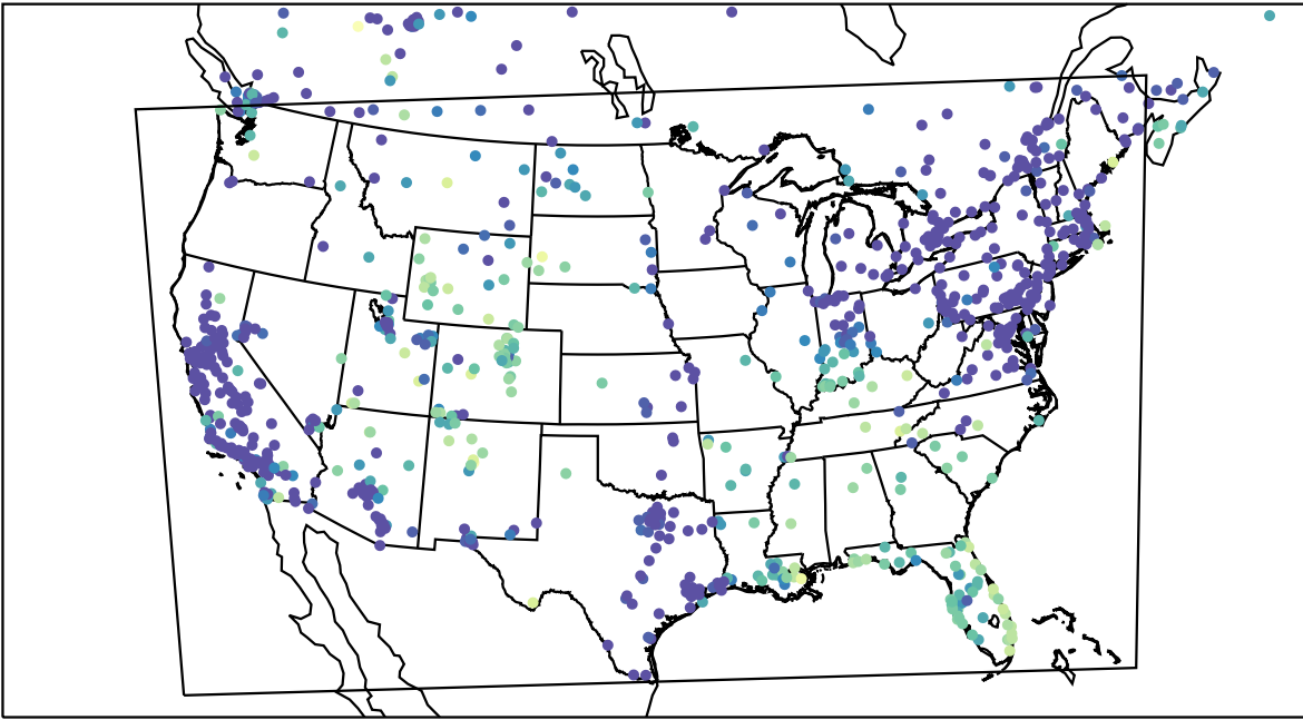
AirNOW (2023-12-25_04:00:00)
