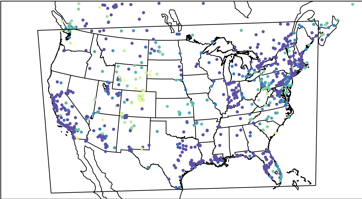
AirNOW (2023-12-26_12:00:00)
