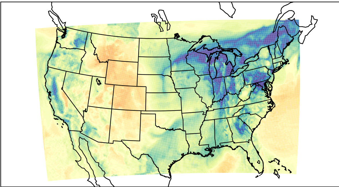
WRF (2023-12-26_19:00:00)
