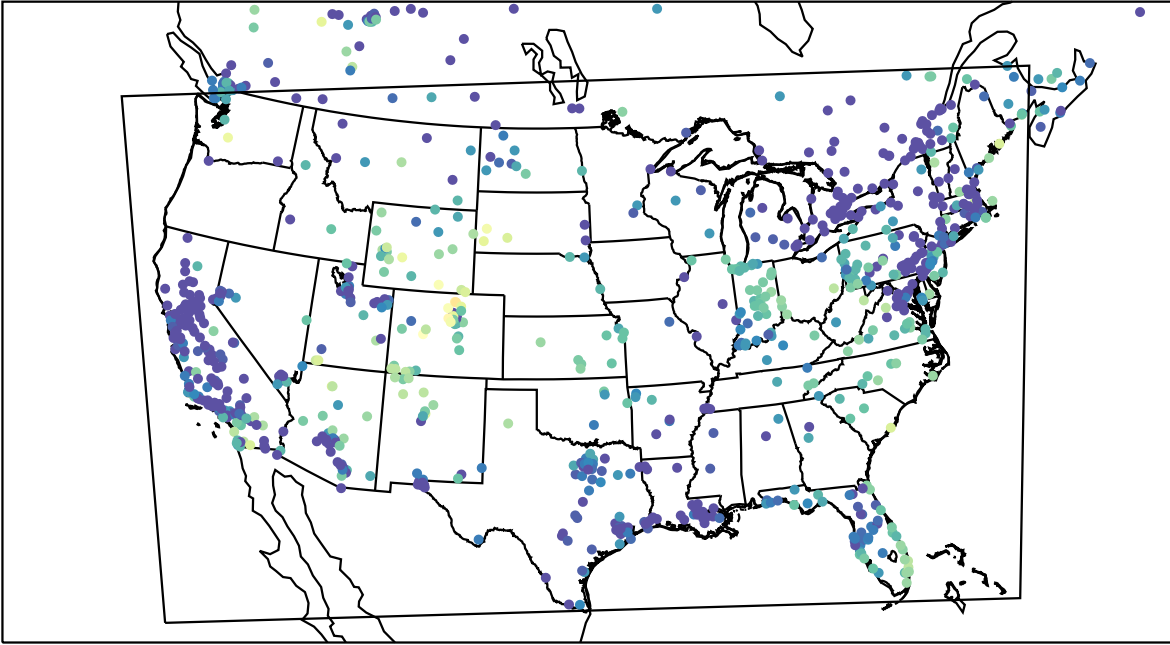
AirNOW (2023-12-26_02:00:00)
