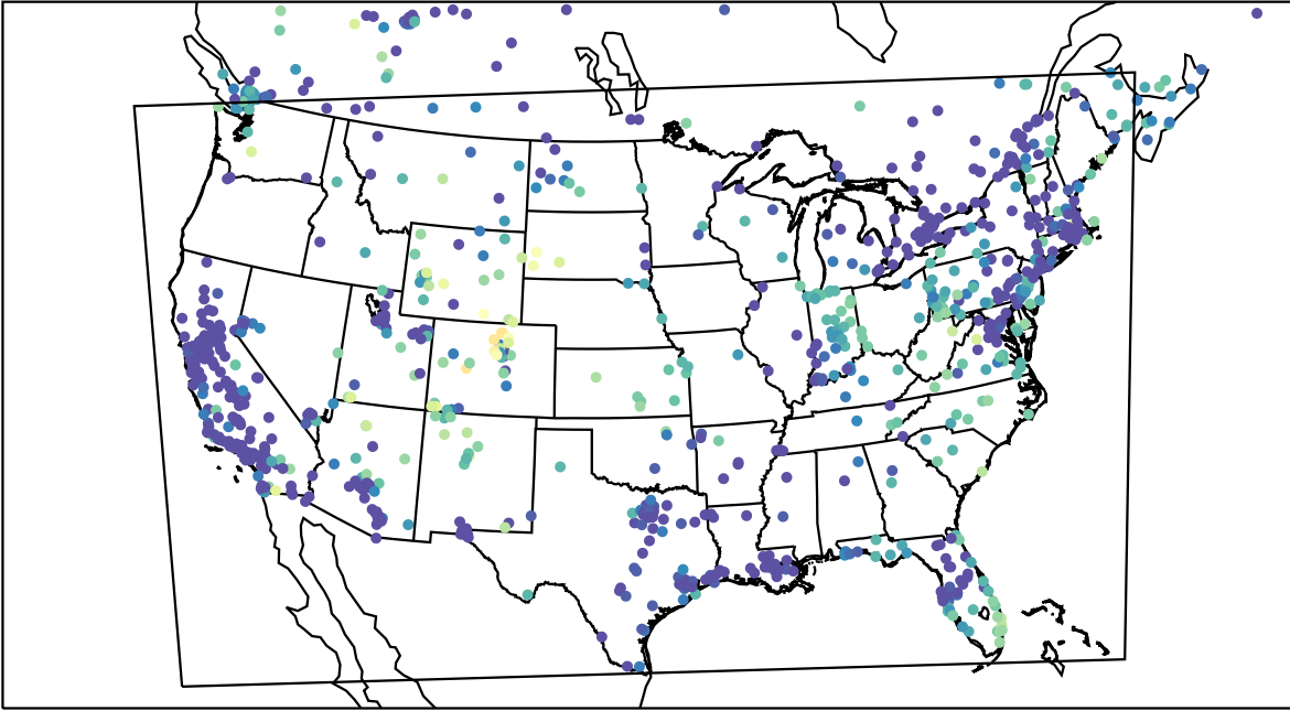
AirNOW (2023-12-26_04:00:00)
