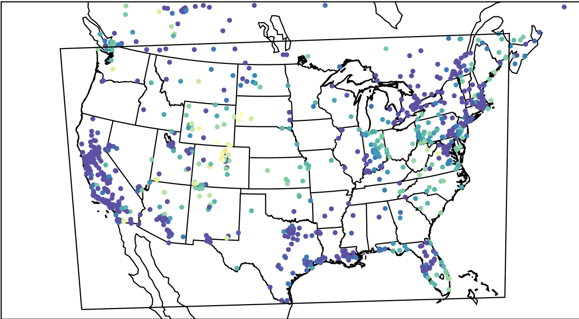
AirNOW (2023-12-26_05:00:00)
