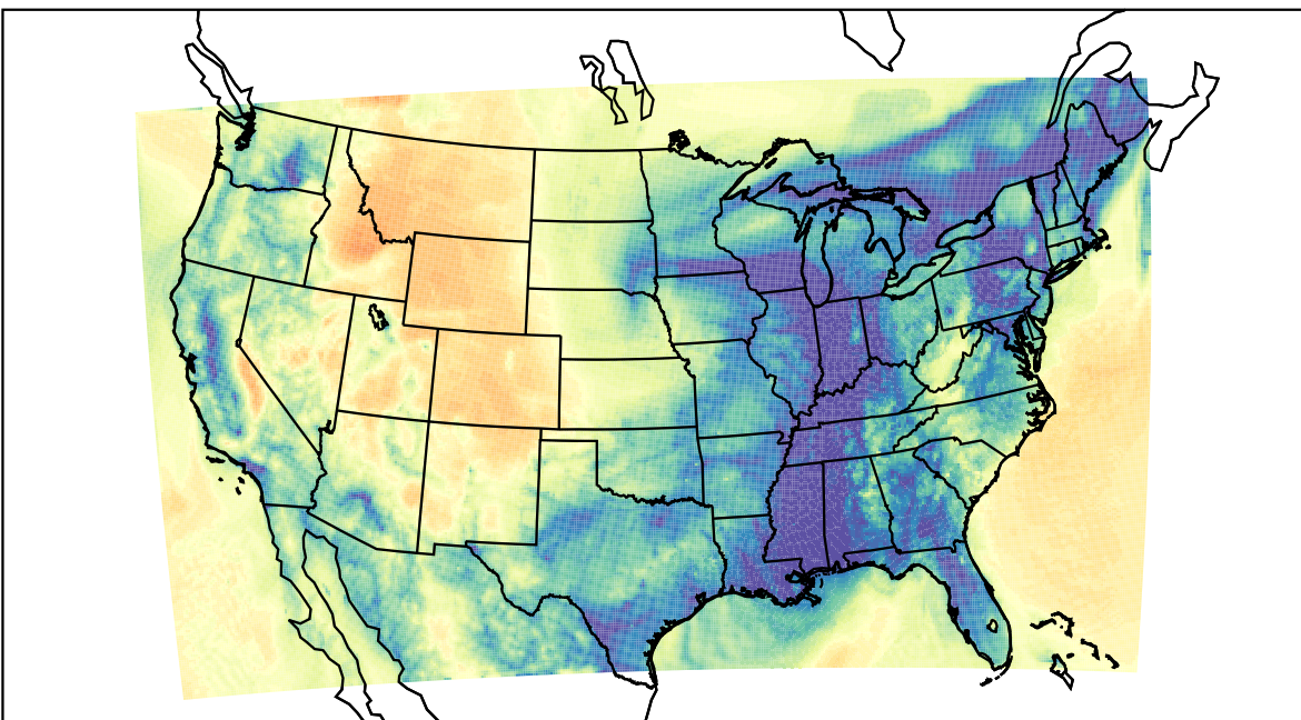
WRF (2023-12-26_11:00:00)
