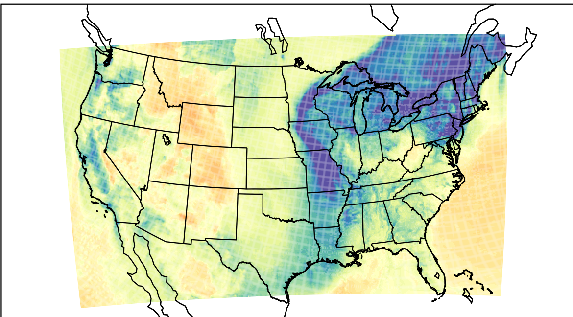
WRF (2023-12-25_20:00:00)
