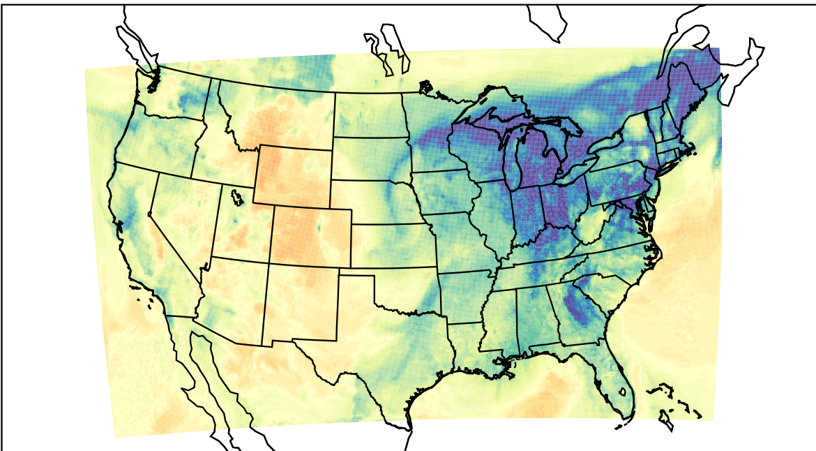
WRF (2023-12-26_22:00:00)
