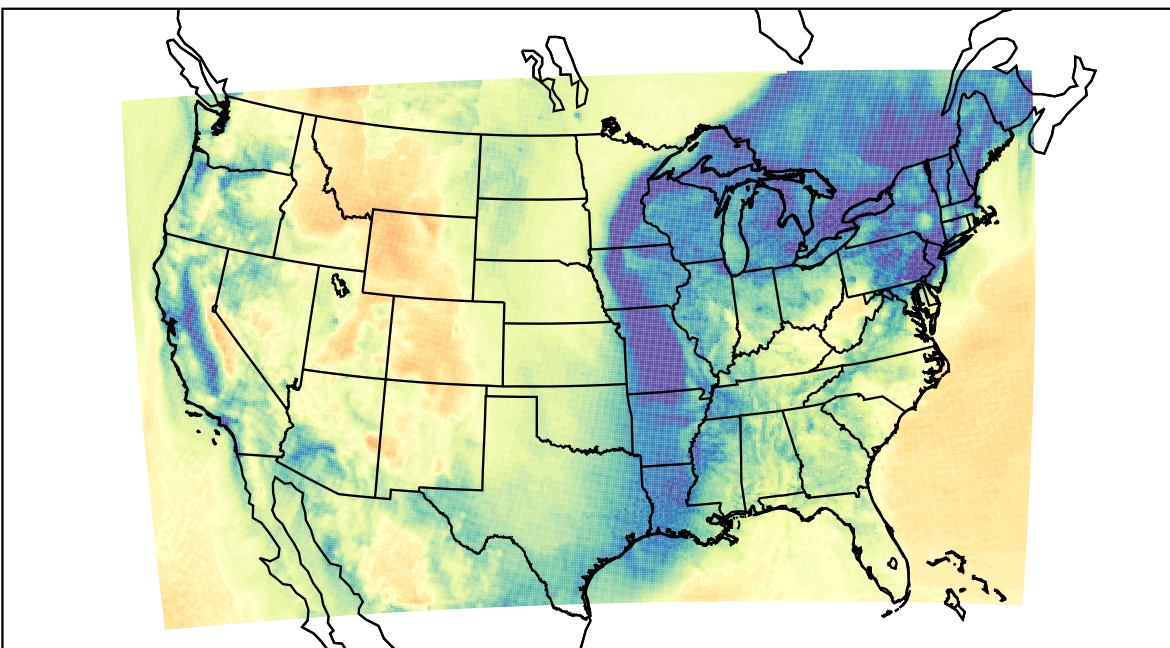
WRF (2023-12-25_18:00:00)
