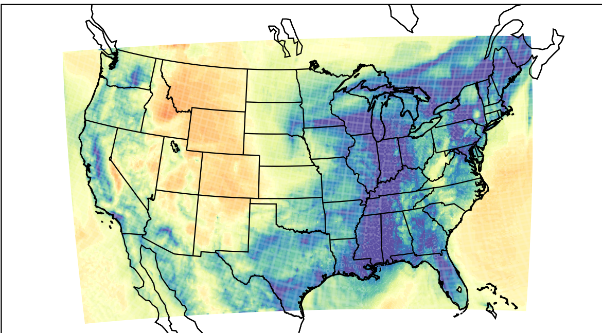
WRF (2023-12-26_12:00:00)
