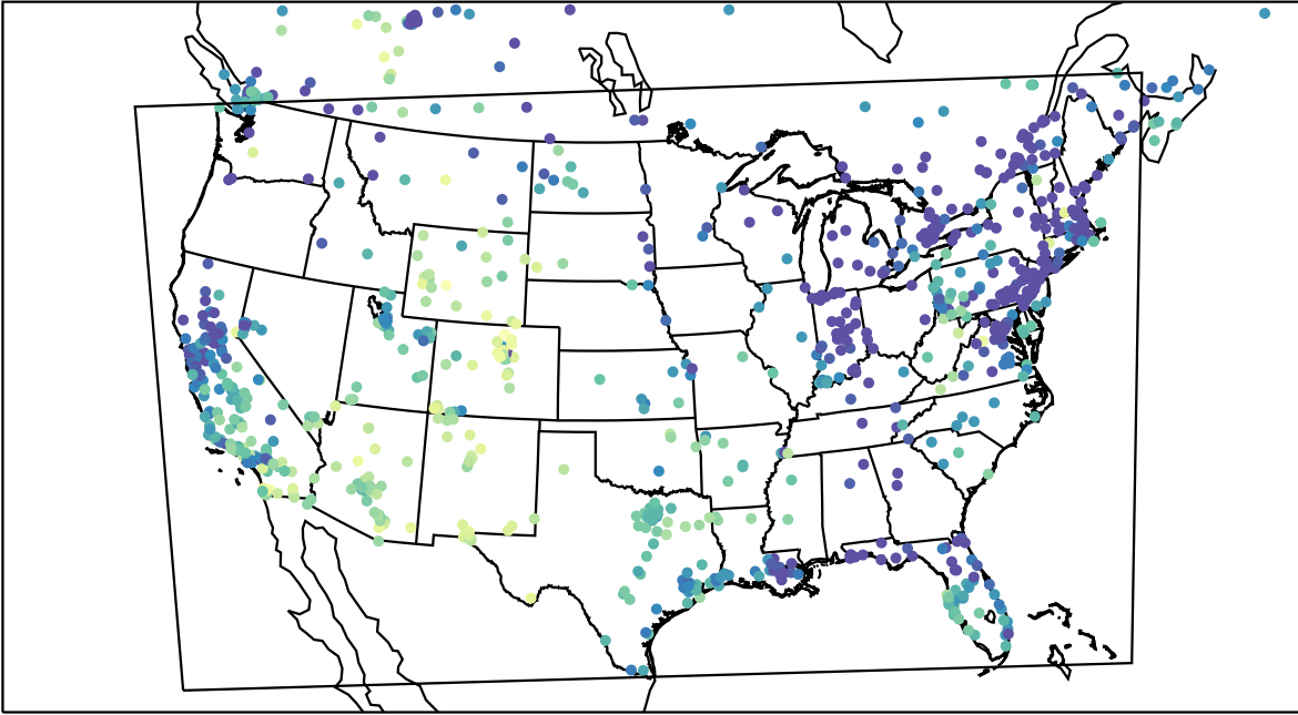
AirNOW (2023-12-26_22:00:00)
