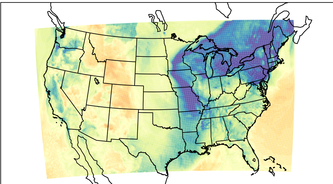
WRF (2023-12-25_21:00:00)
