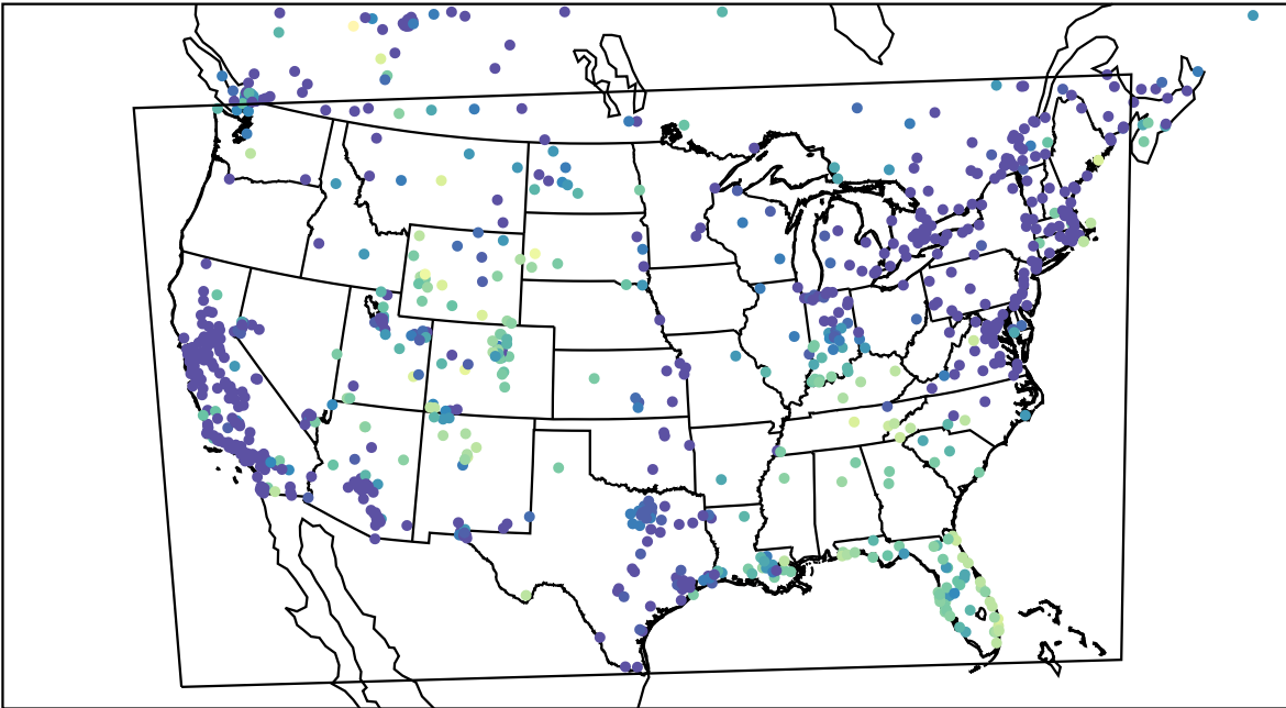
AirNOW (2023-12-25_06:00:00)
