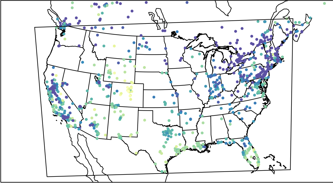
AirNOW (2023-12-27_19:00:00)
