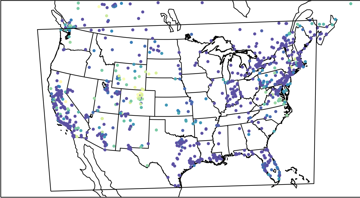
AirNOW (2023-12-27_14:00:00)
