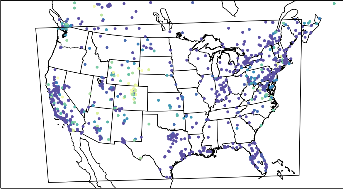
AirNOW (2023-12-27_13:00:00)
