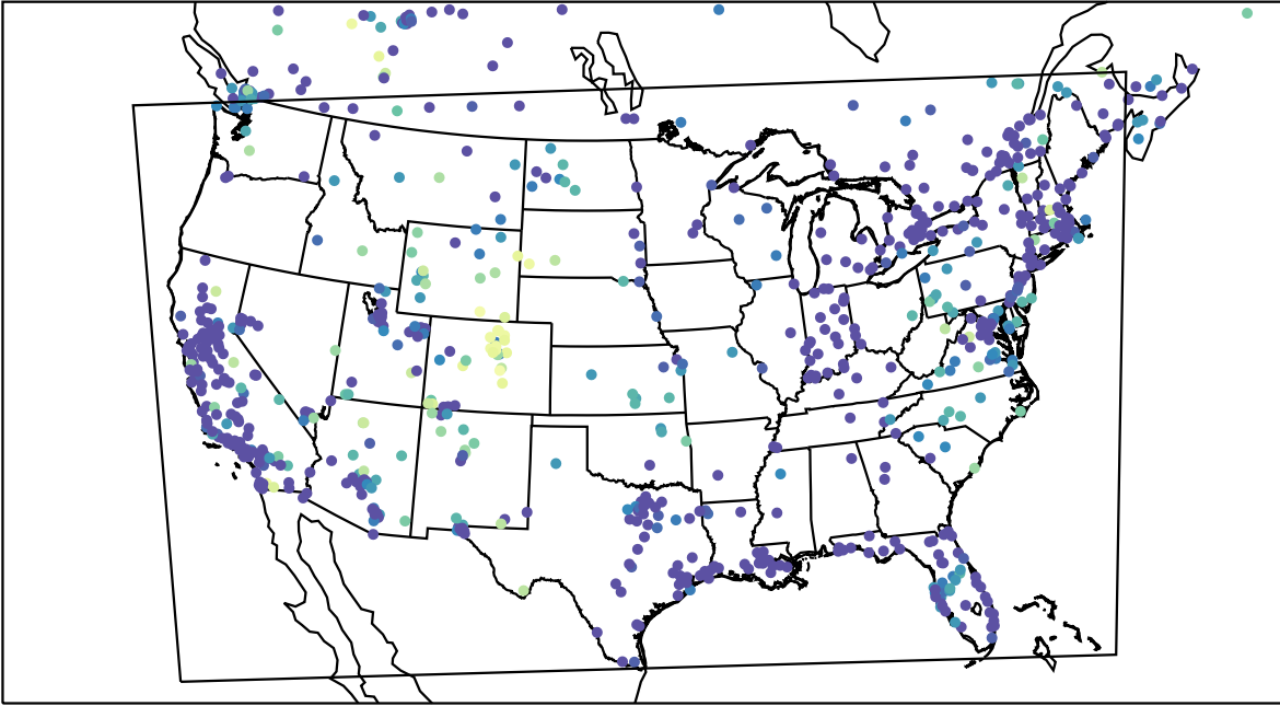
AirNOW (2023-12-27_06:00:00)
