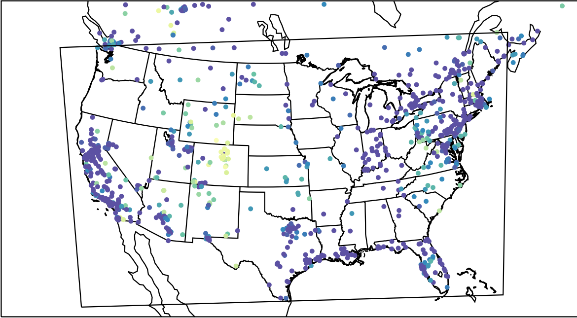
AirNOW (2023-12-27_05:00:00)
