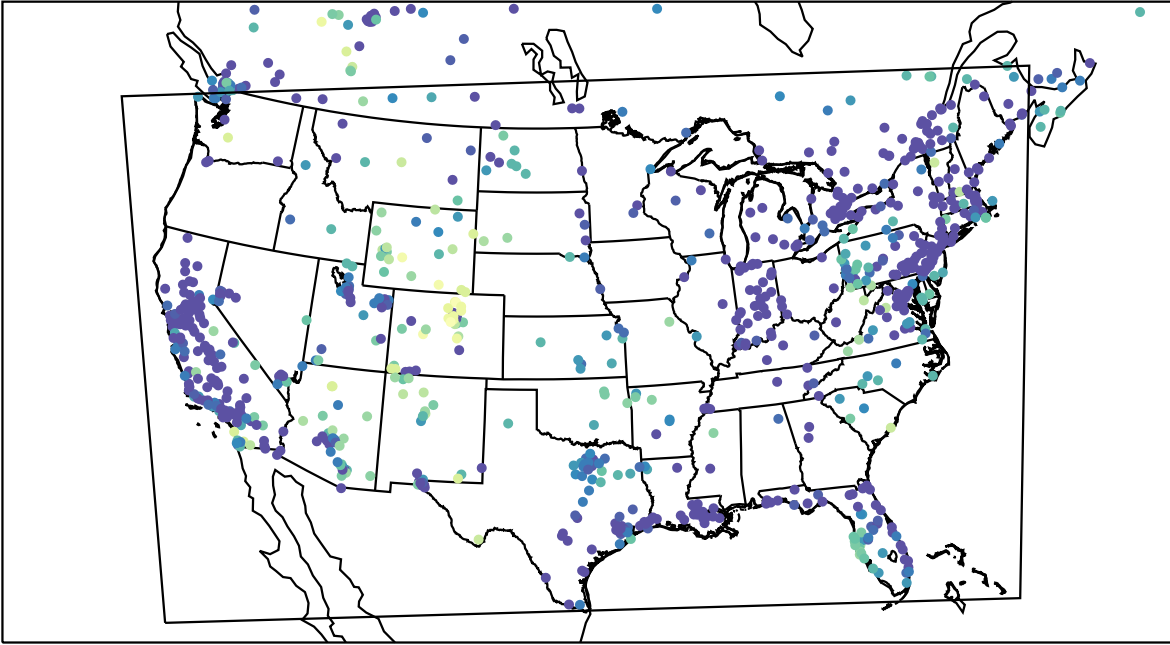
AirNOW (2023-12-27_01:00:00)
