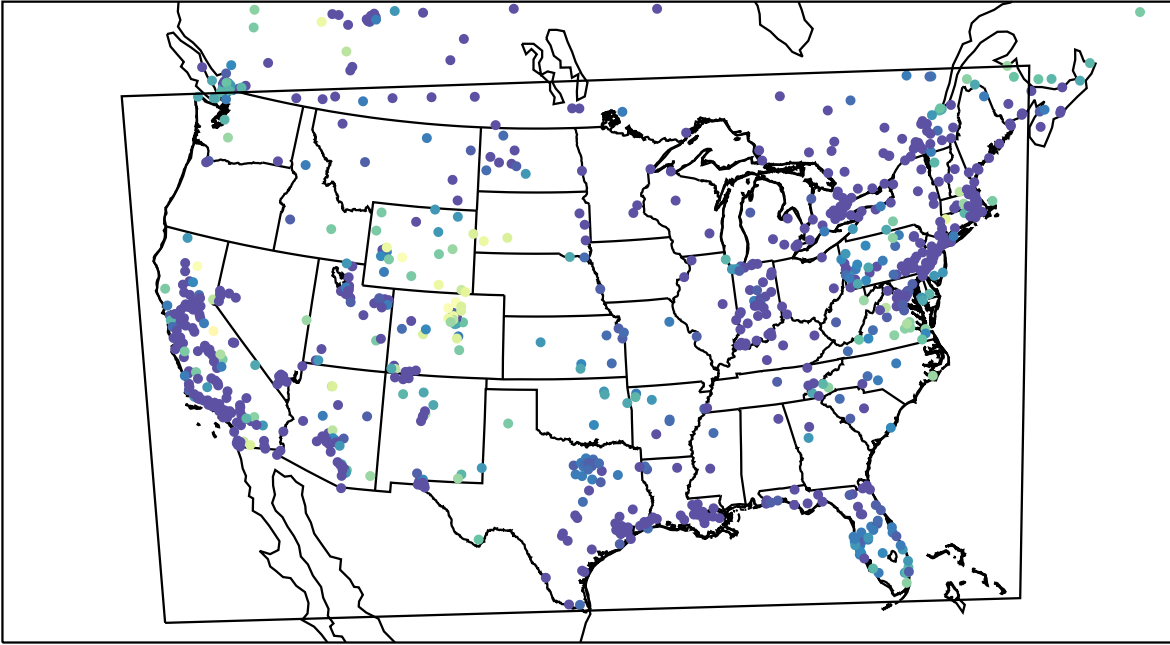
AirNOW (2023-12-27_15:00:00)
