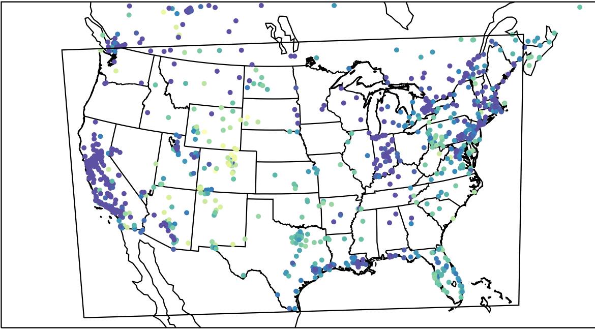
AirNOW (2023-12-26_17:00:00)
