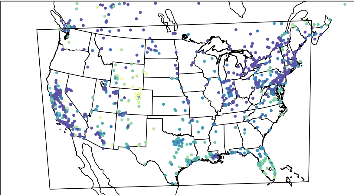
AirNOW (2023-12-27_17:00:00)
