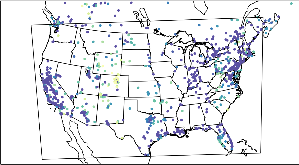
AirNOW (2023-12-27_02:00:00)
