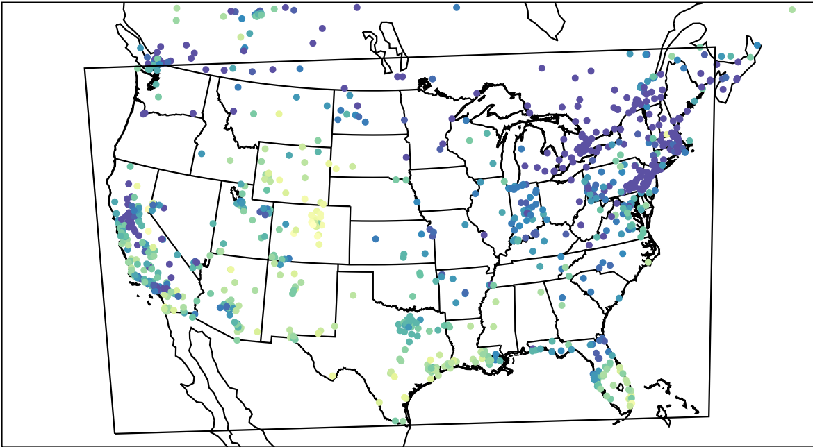
AirNOW (2023-12-27_20:00:00)
