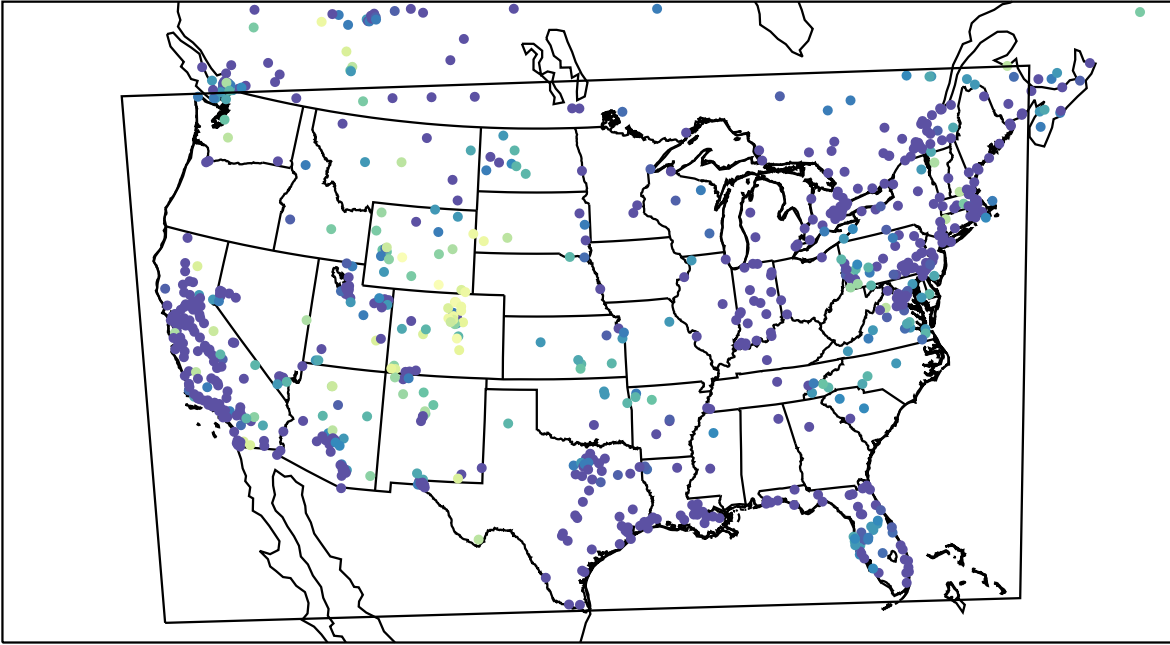
AirNOW (2023-12-27_07:00:00)
