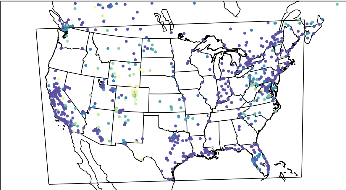
AirNOW (2023-12-27_08:00:00)
