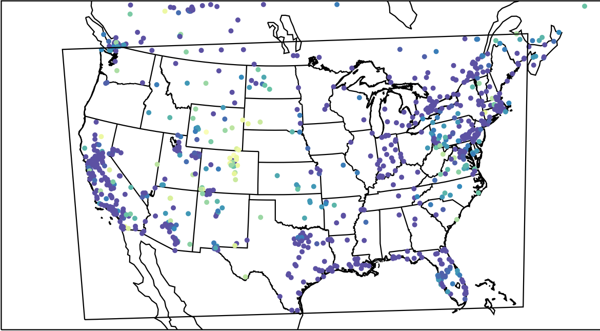
AirNOW (2023-12-27_09:00:00)
