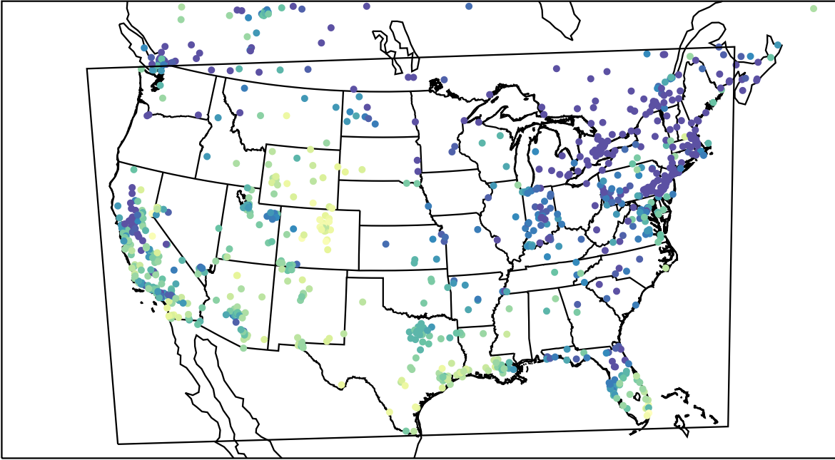
AirNOW (2023-12-27_21:00:00)
