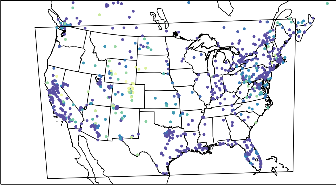
AirNOW (2023-12-27_10:00:00)
