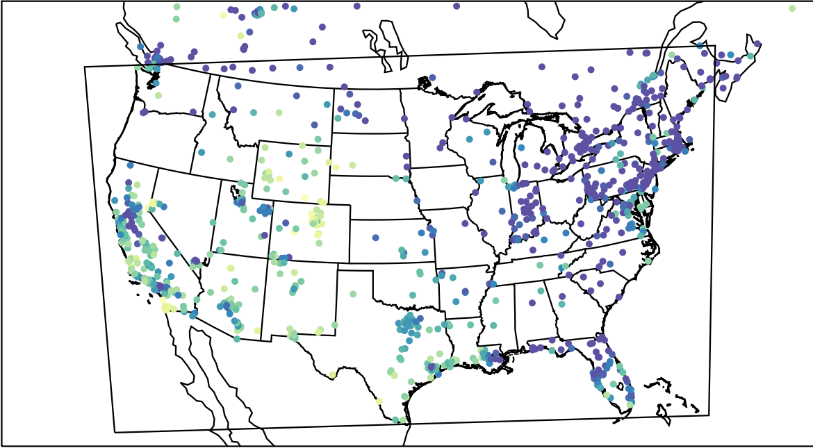
AirNOW (2023-12-27_23:00:00)
