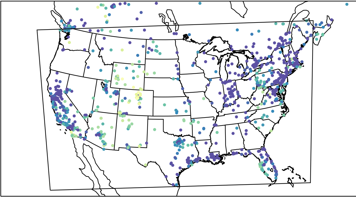
AirNOW (2023-12-27_00:00:00)
