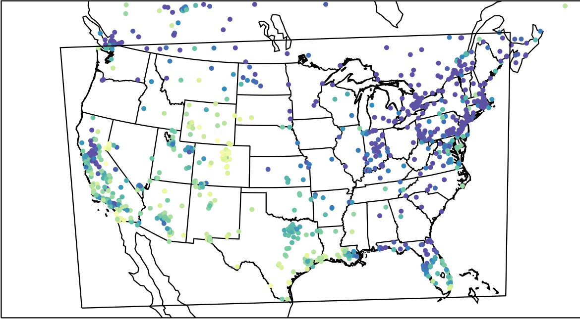
AirNOW (2023-12-27_22:00:00)
