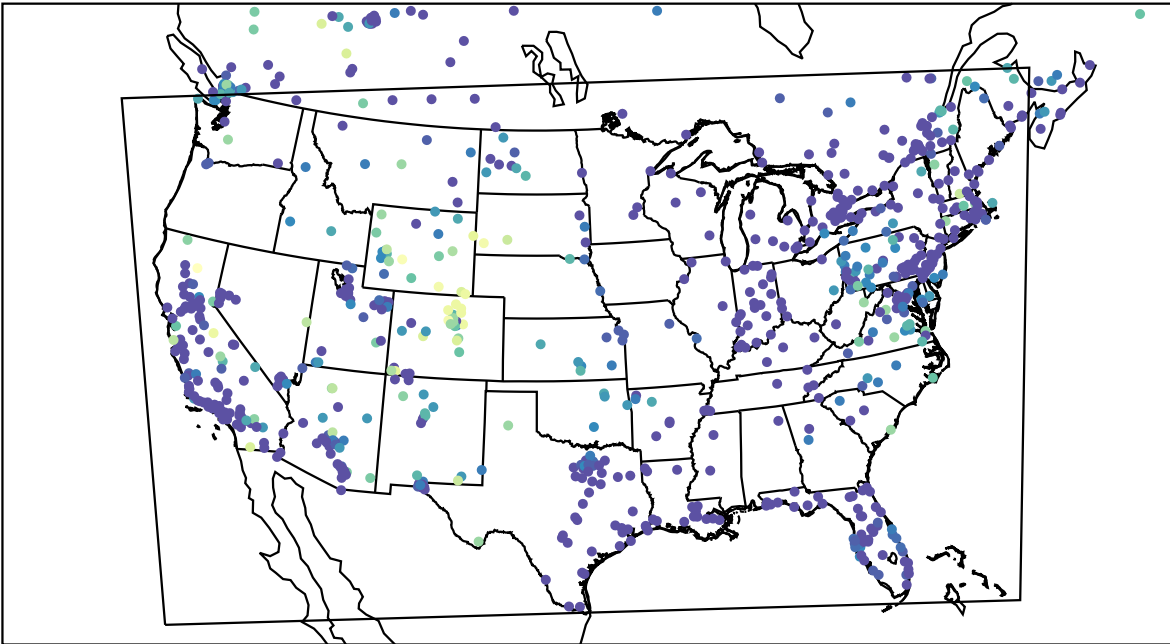
AirNOW (2023-12-27_11:00:00)
