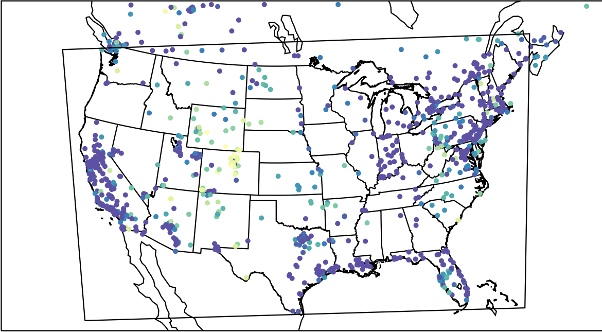
AirNOW (2023-12-27_03:00:00)
