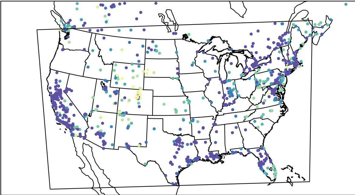
AirNOW (2023-12-26_07:00:00)
