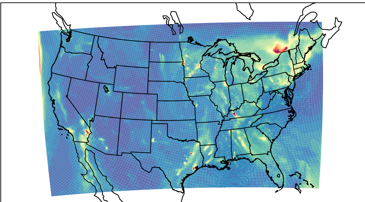
WRF 2023-12-27_10:00:00
