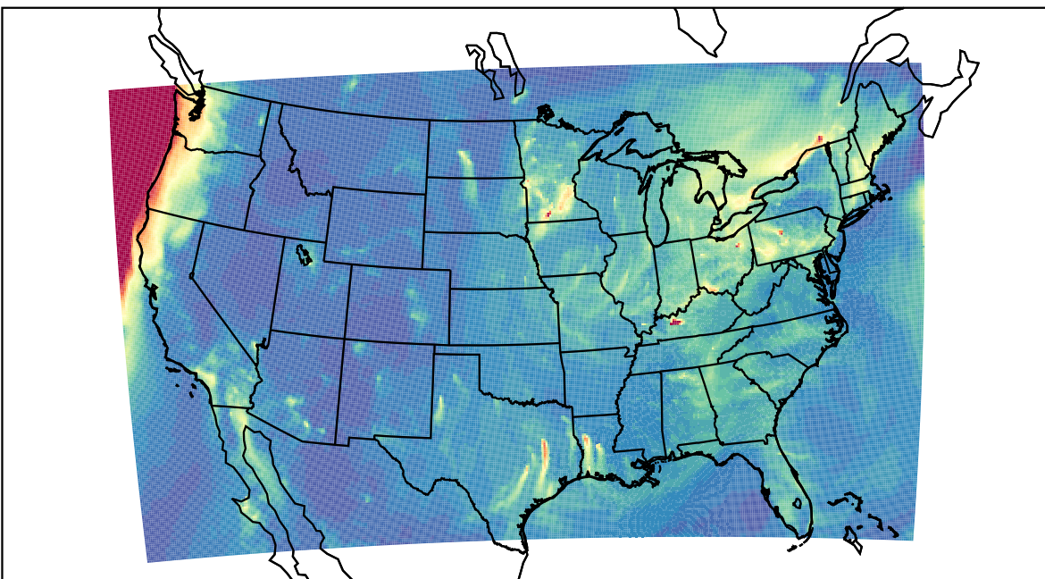
WRF 2023-12-28_08:00:00
