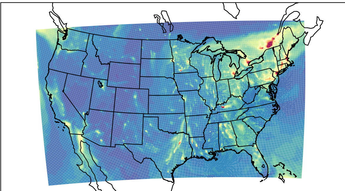
WRF 2023-12-27_01:00:00
