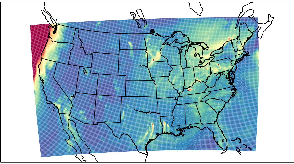
WRF 2023-12-28_09:00:00
