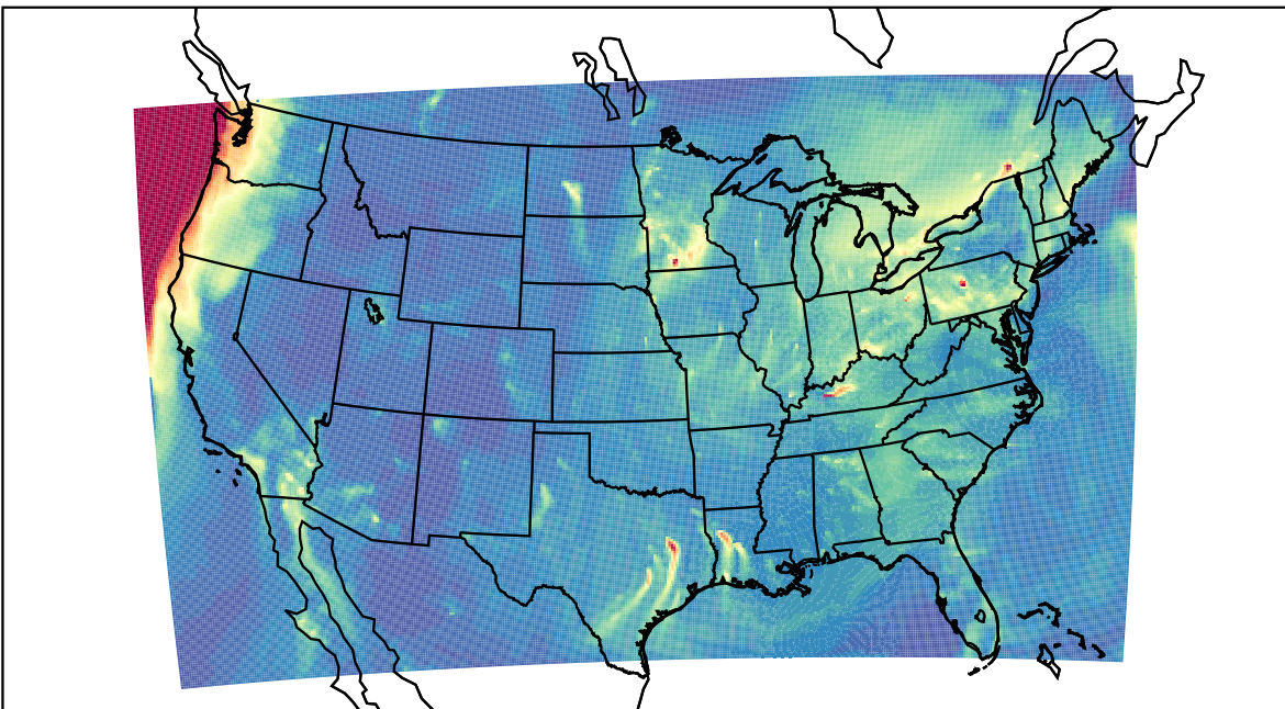
WRF 2023-12-28_11:00:00
