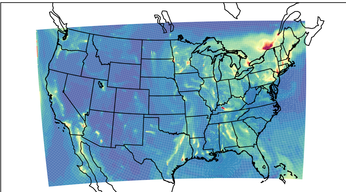
WRF 2023-12-27_06:00:00
