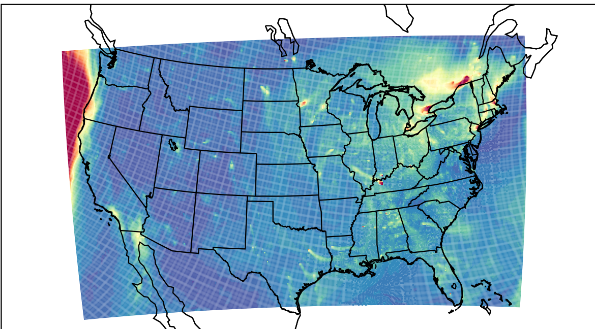
WRF 2023-12-27_22:00:00
