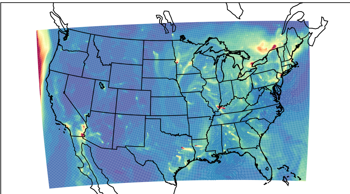
WRF 2023-12-27_16:00:00
