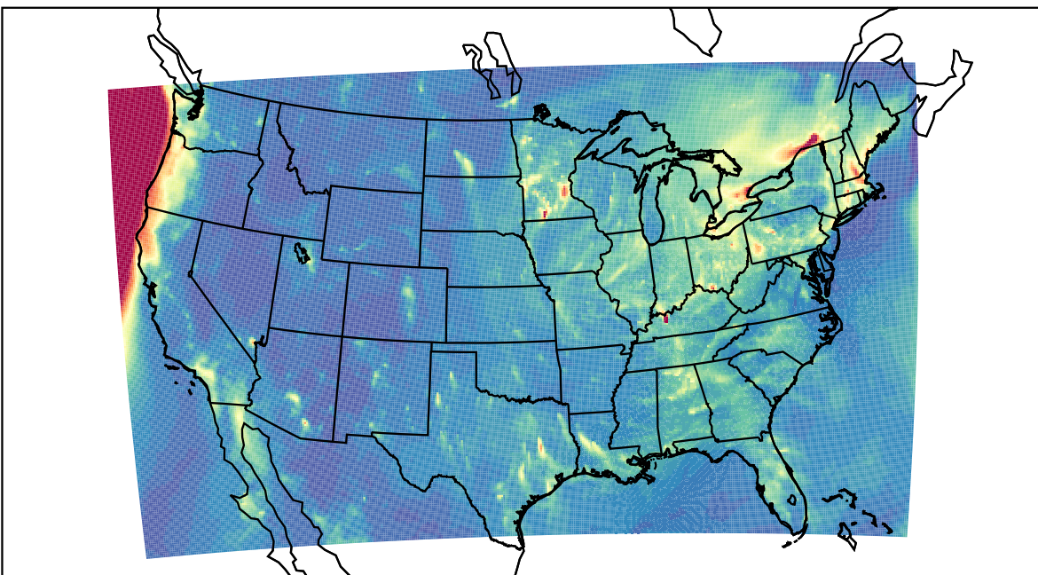
WRF 2023-12-28_03:00:00
