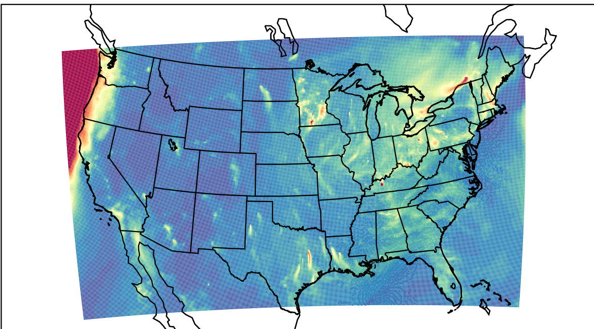
WRF 2023-12-28_05:00:00
