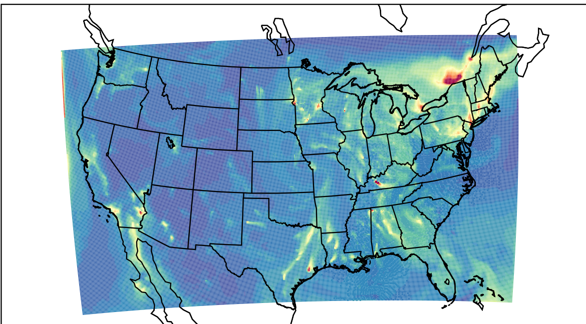
WRF 2023-12-27_07:00:00
