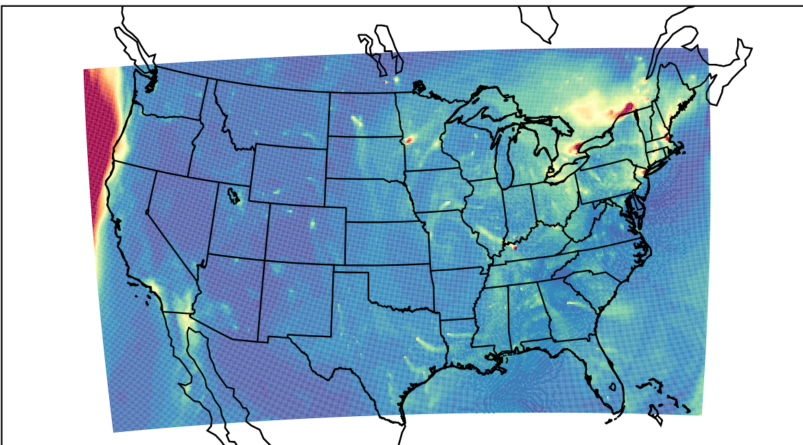
WRF 2023-12-27_21:00:00
