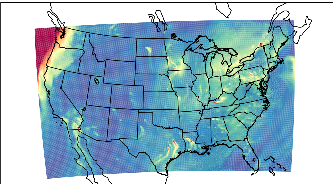
WRF 2023-12-28_14:00:00
