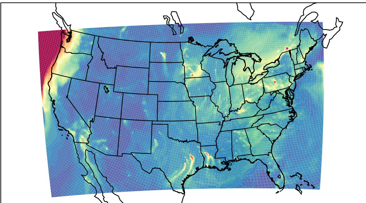
WRF 2023-12-28_12:00:00
