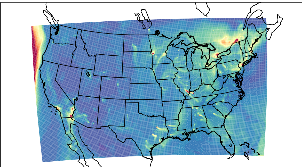
WRF 2023-12-27_17:00:00
