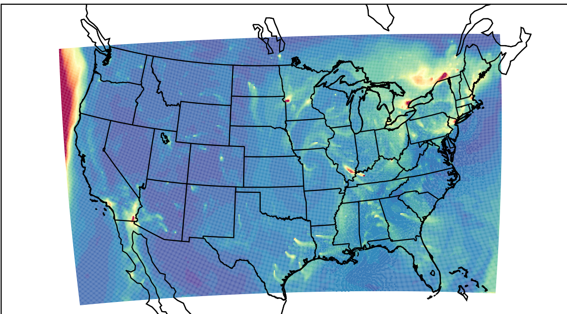
WRF 2023-12-27_18:00:00
