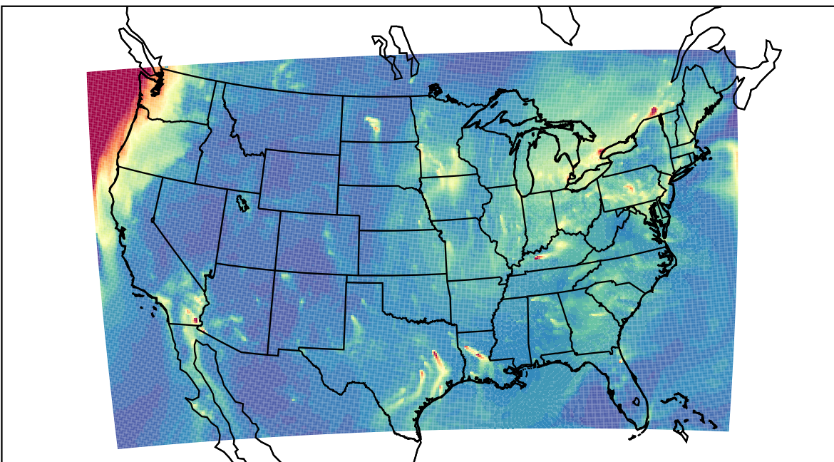
WRF 2023-12-28_15:00:00
