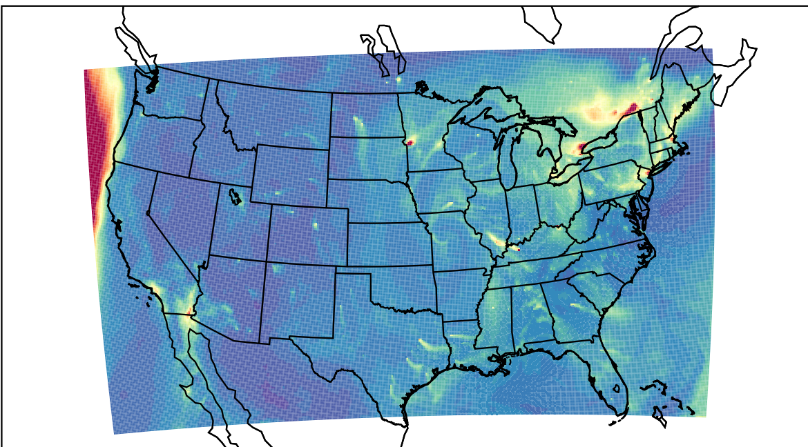
WRF 2023-12-27_19:00:00
