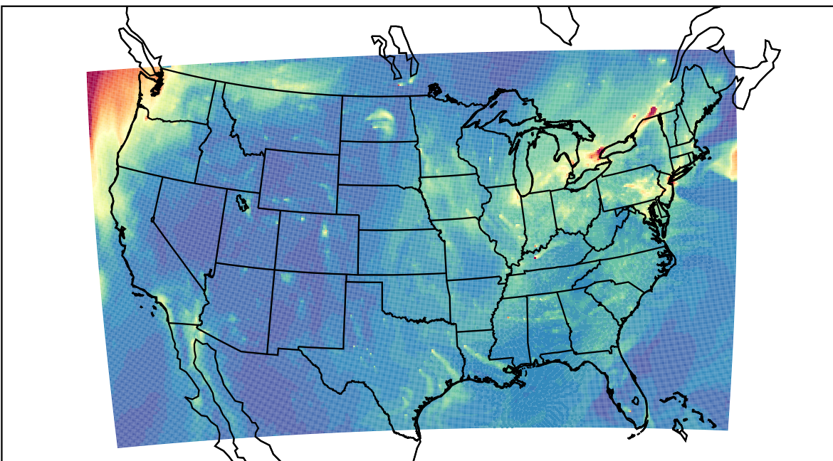
WRF 2023-12-28_22:00:00
