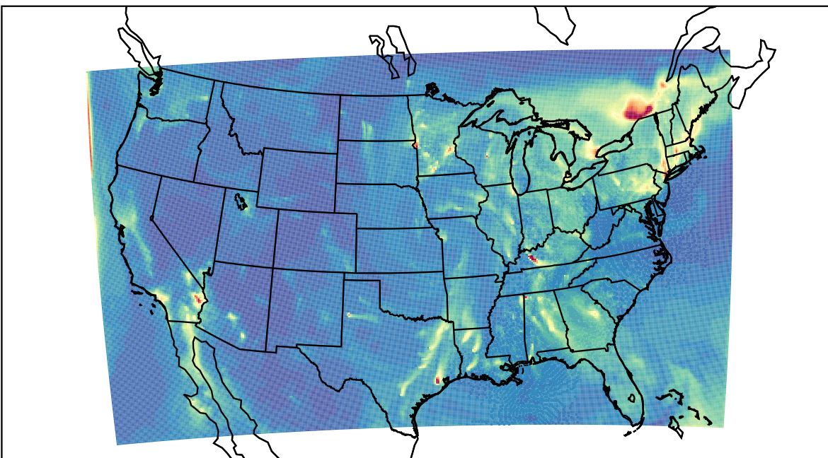
WRF 2023-12-27_08:00:00
