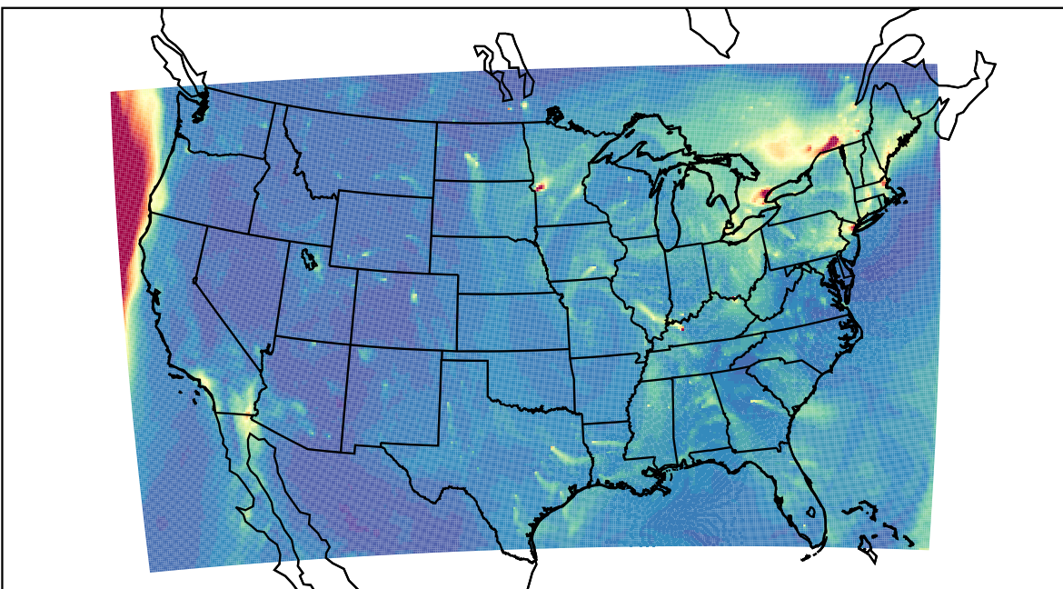
WRF 2023-12-27_20:00:00
