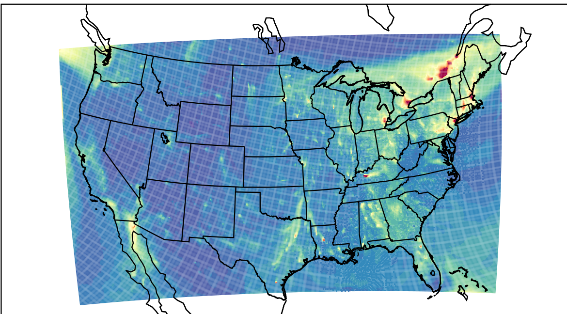
WRF 2023-12-27_00:00:00
