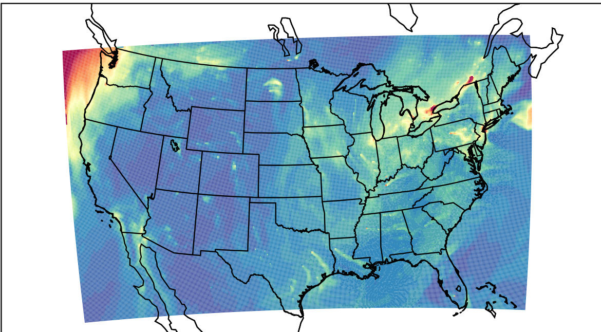
WRF 2023-12-28_21:00:00
