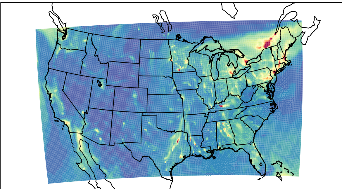
WRF 2023-12-27_02:00:00
