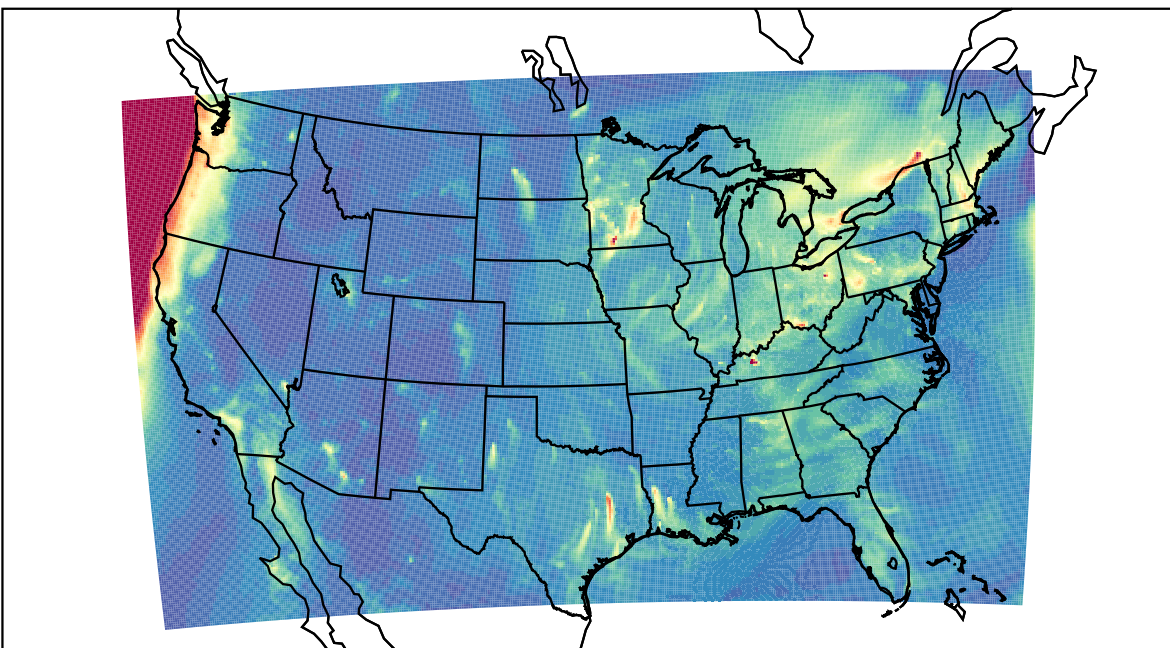
WRF 2023-12-28_06:00:00
