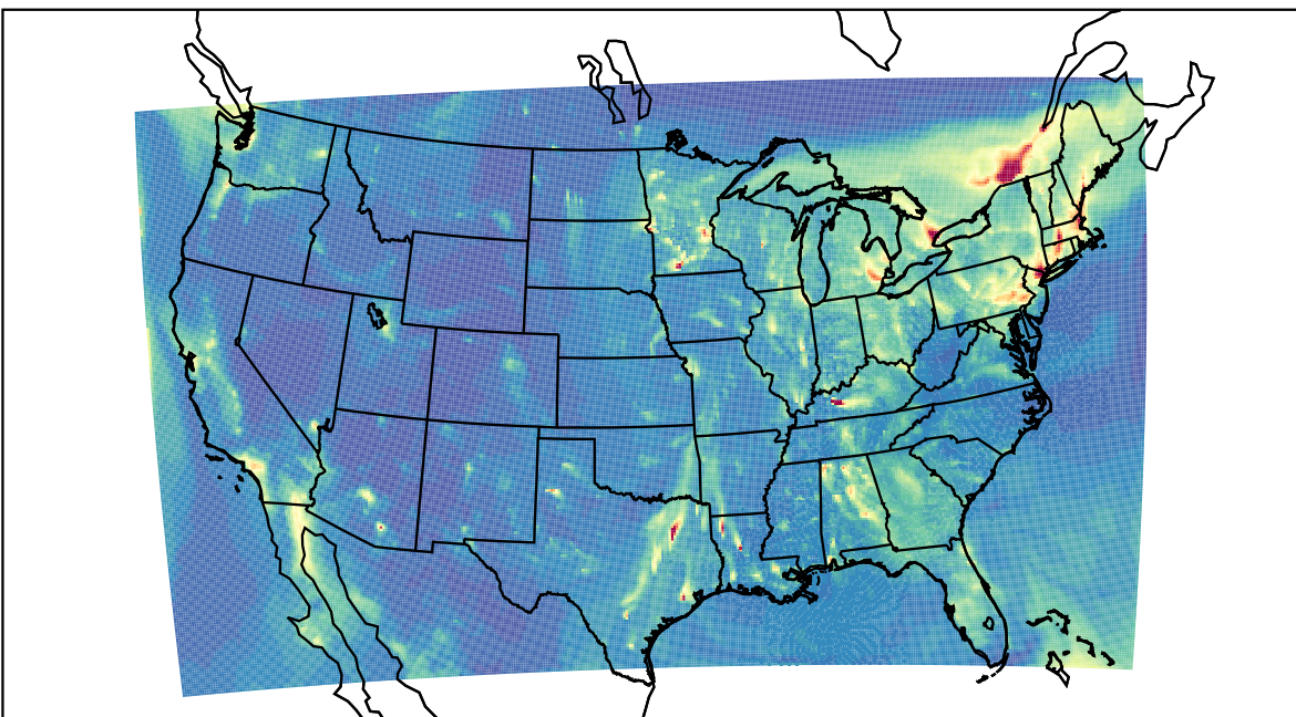
WRF 2023-12-27_03:00:00
