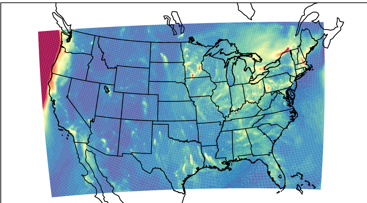
WRF 2023-12-28_04:00:00
