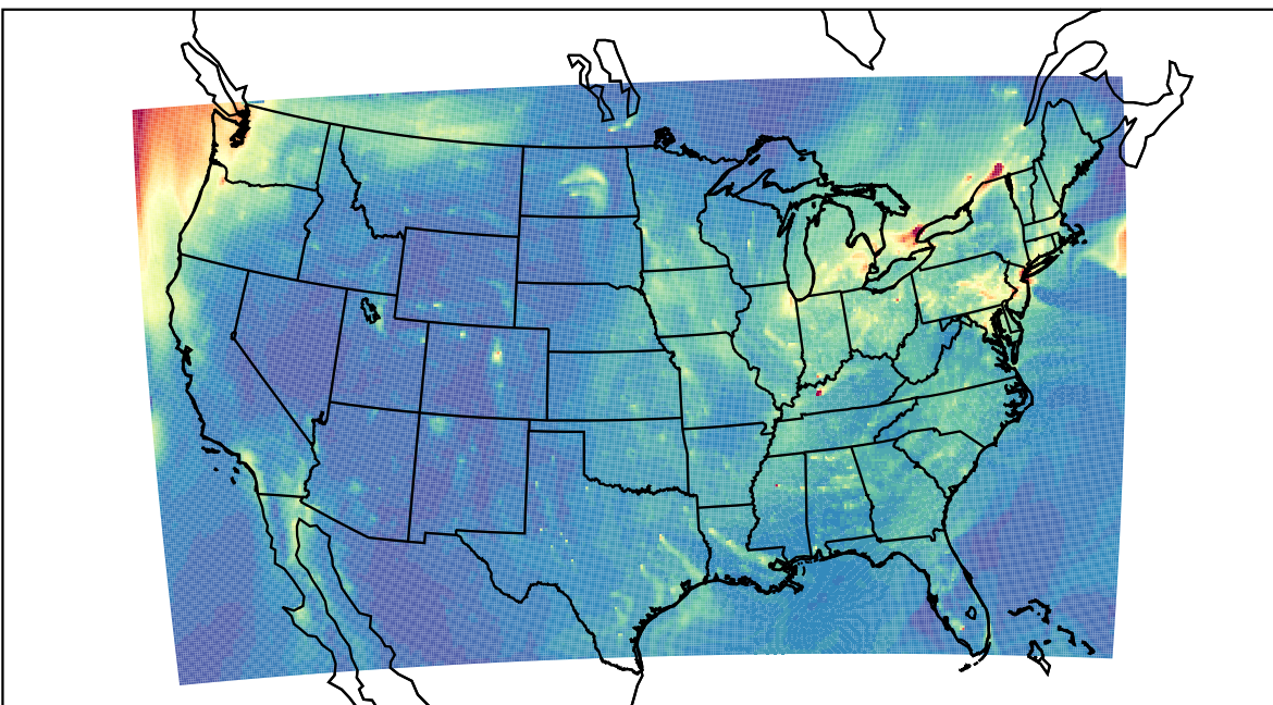
WRF 2023-12-28_23:00:00
