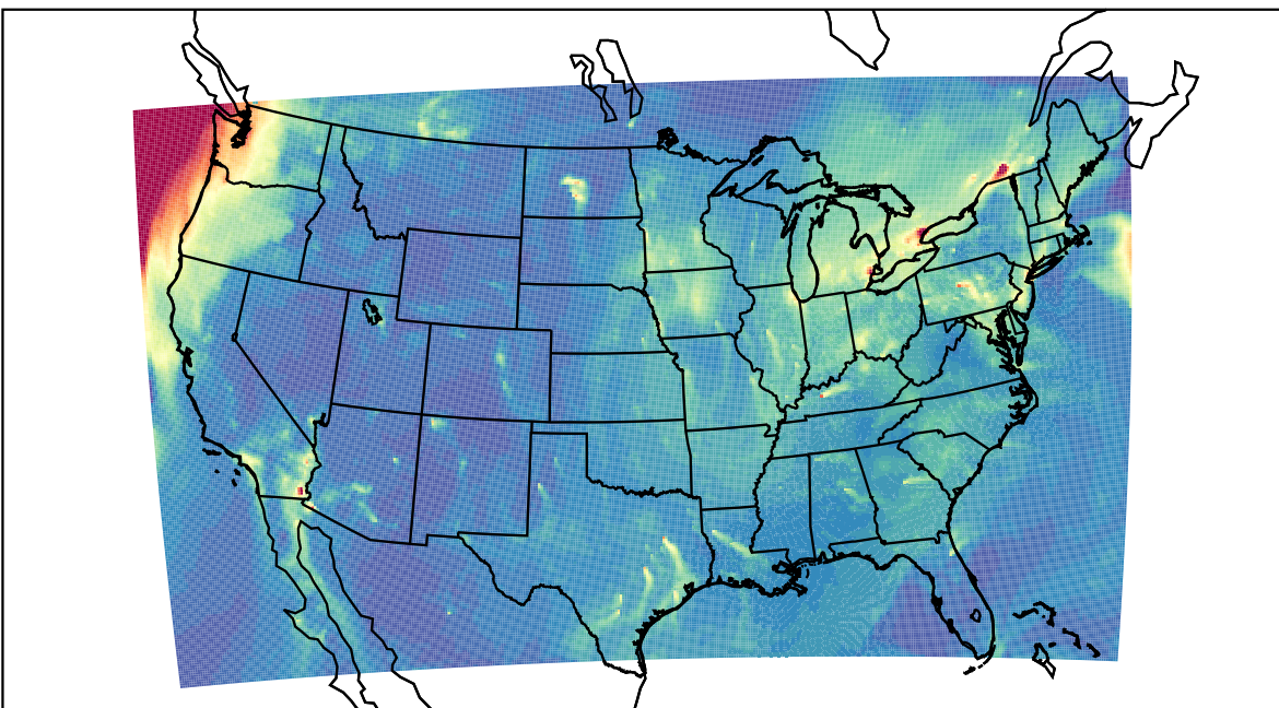
WRF 2023-12-28_17:00:00
