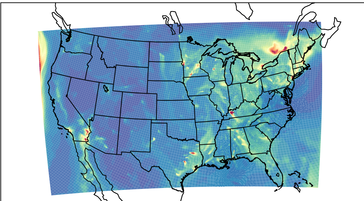
WRF 2023-12-27_13:00:00
