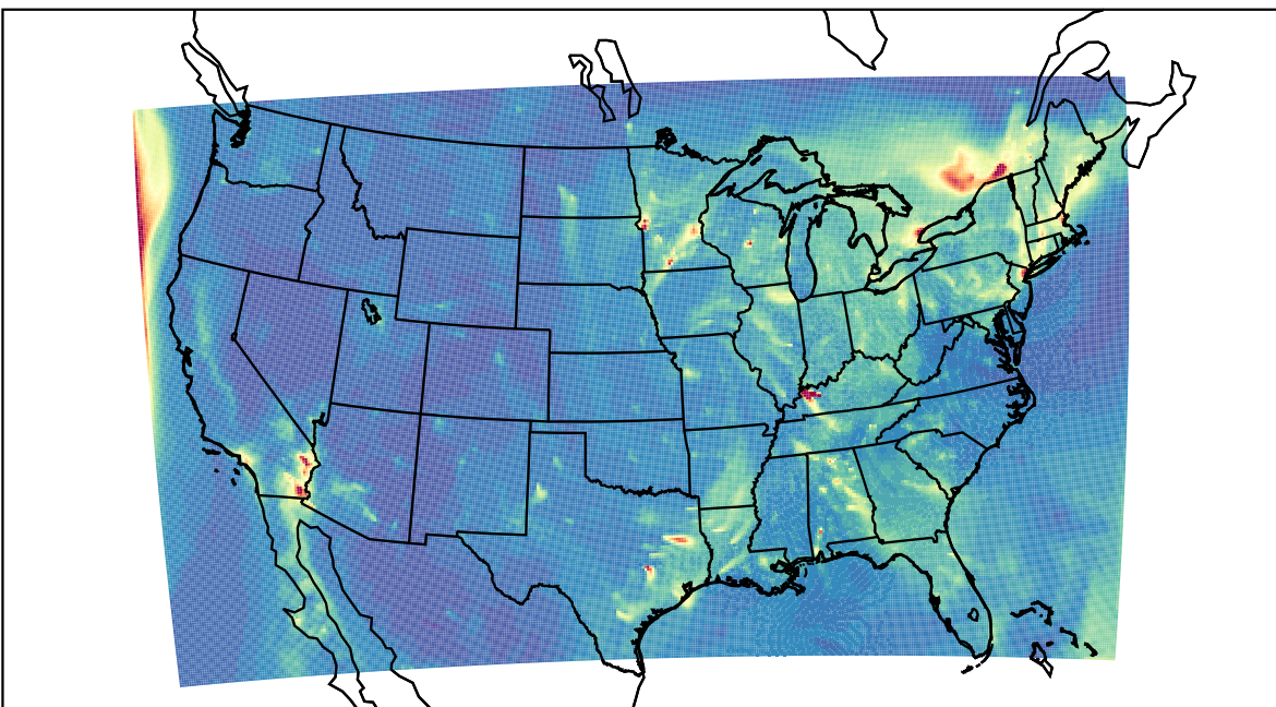
WRF 2023-12-27_14:00:00
