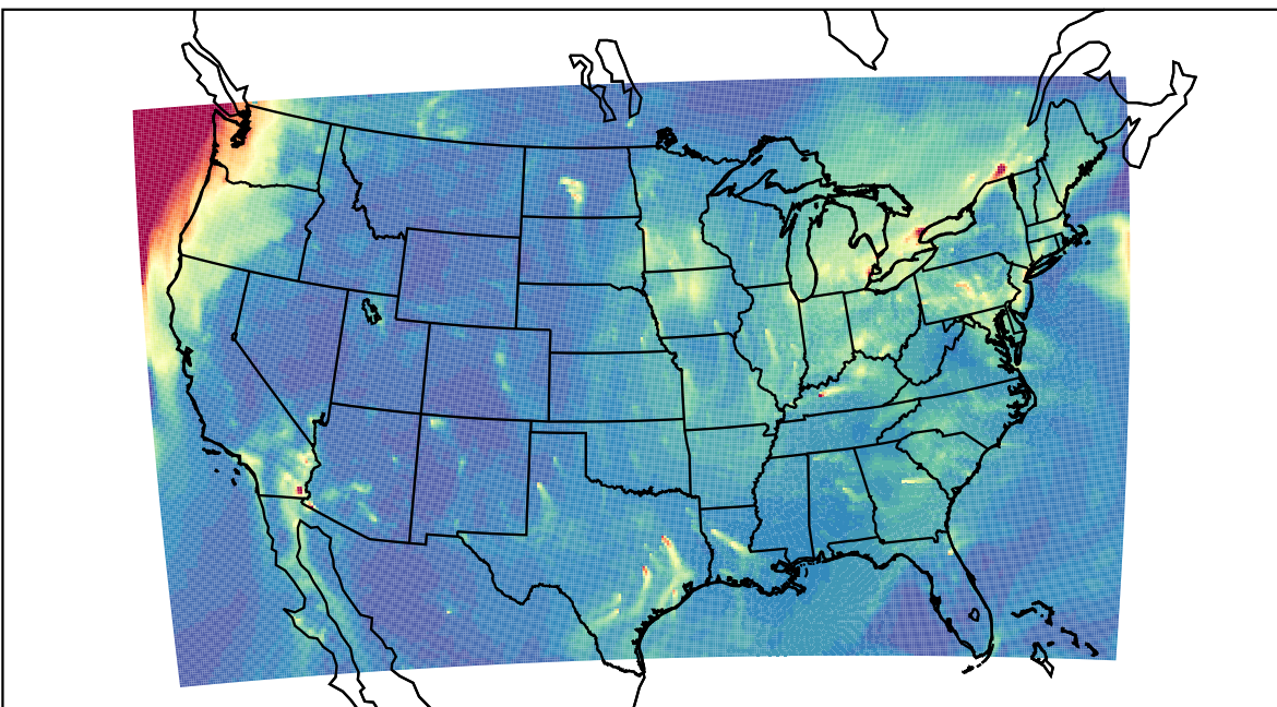
WRF 2023-12-28_16:00:00
