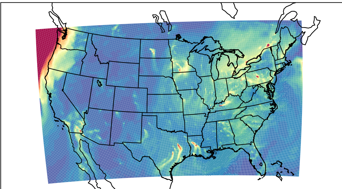
WRF 2023-12-28_13:00:00
