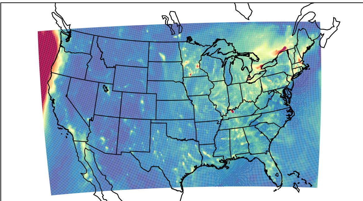
WRF 2023-12-28_01:00:00
