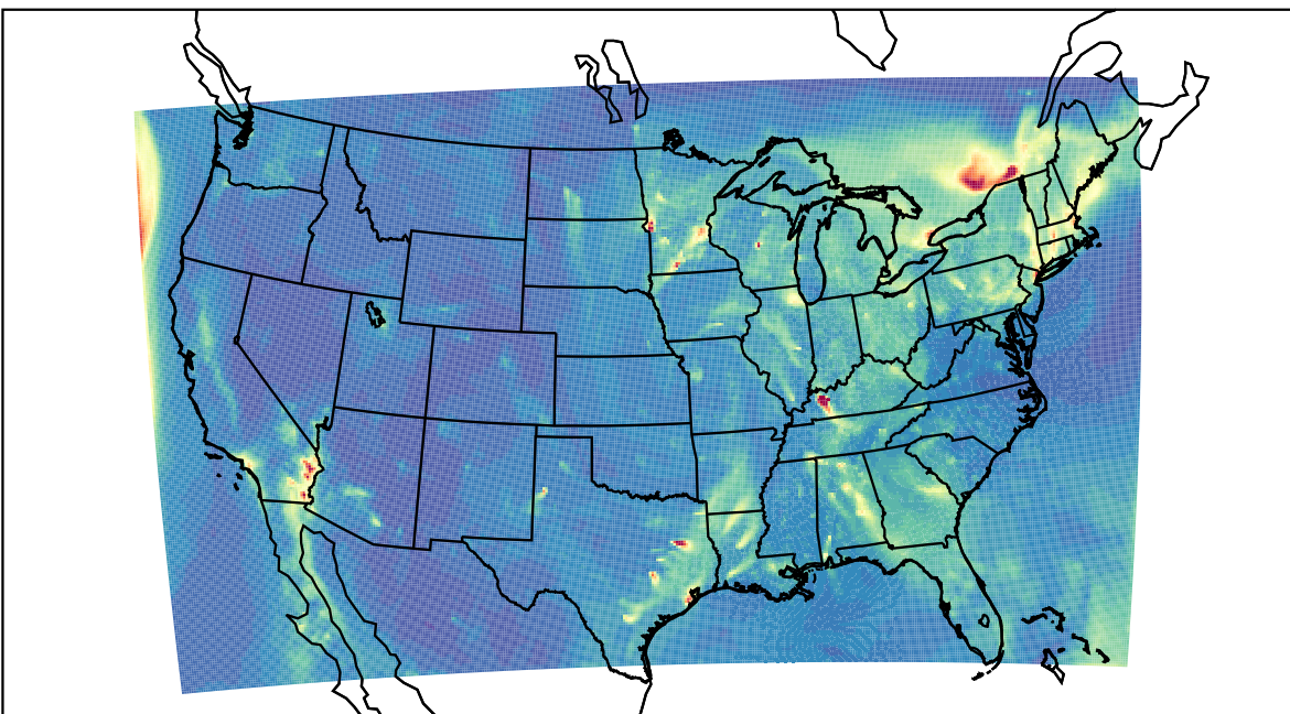
WRF 2023-12-27_12:00:00
