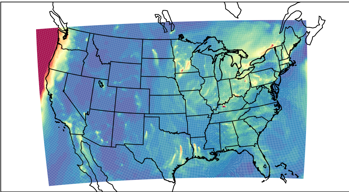
WRF 2023-12-28_07:00:00
