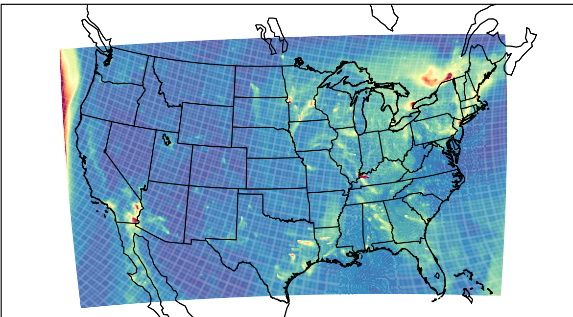
WRF 2023-12-27_15:00:00
