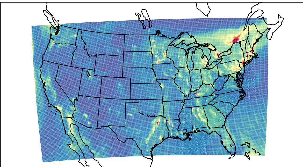
WRF 2023-12-27_04:00:00
