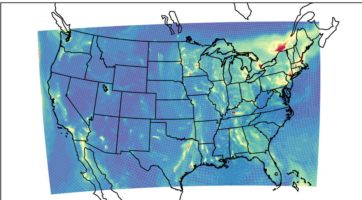
WRF 2023-12-27_05:00:00
