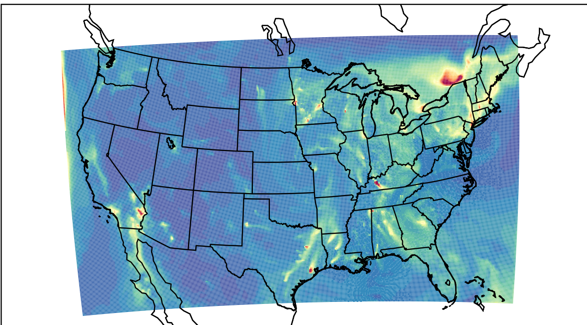
WRF 2023-12-27_09:00:00
