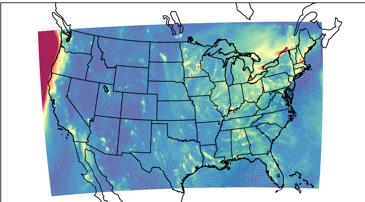
WRF 2023-12-28_02:00:00
