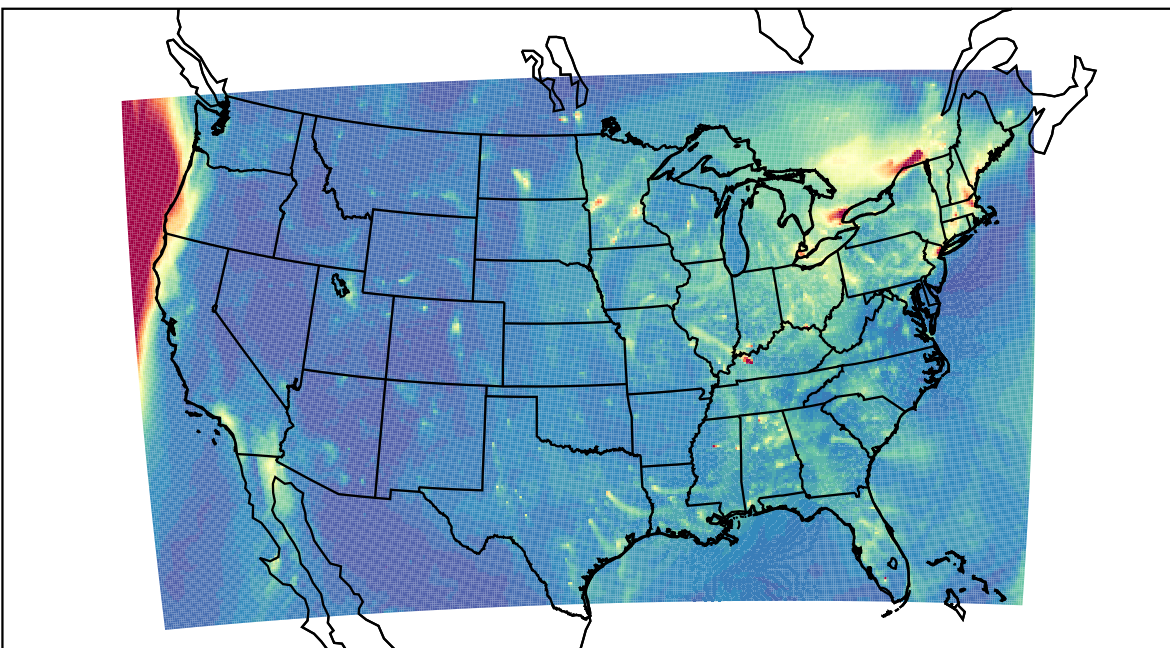
WRF 2023-12-27_23:00:00
