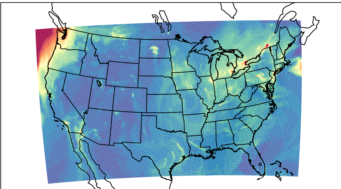
WRF 2023-12-28_19:00:00
