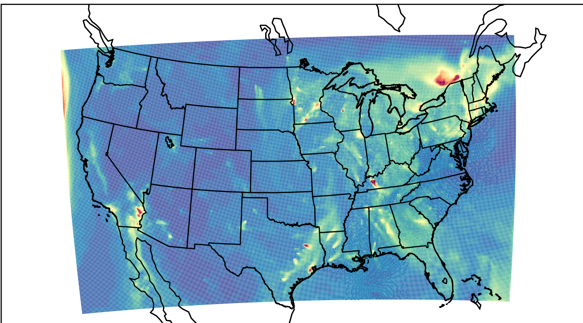
WRF 2023-12-27_11:00:00
