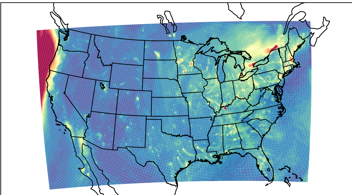
WRF 2023-12-28_00:00:00
