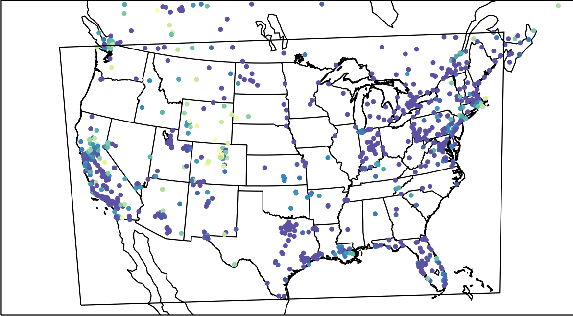
AirNOW (2023-12-28_08:00:00)
