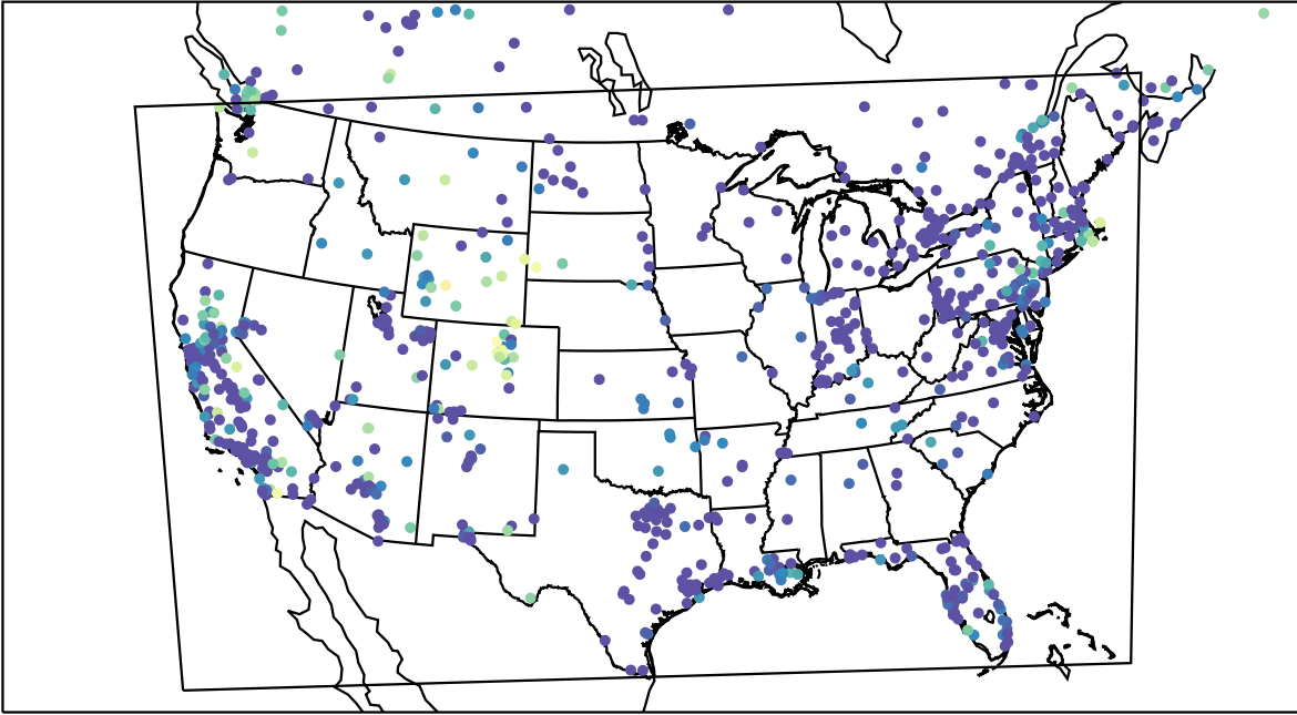
AirNOW (2023-12-28_09:00:00)
