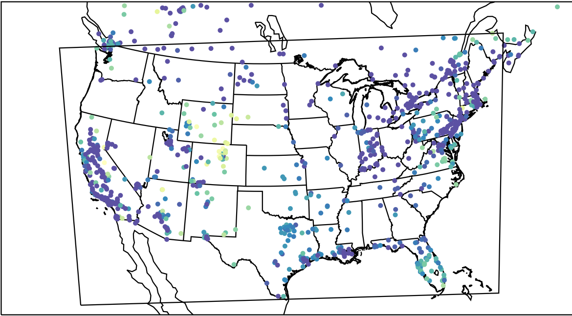
AirNOW (2023-12-27_16:00:00)
