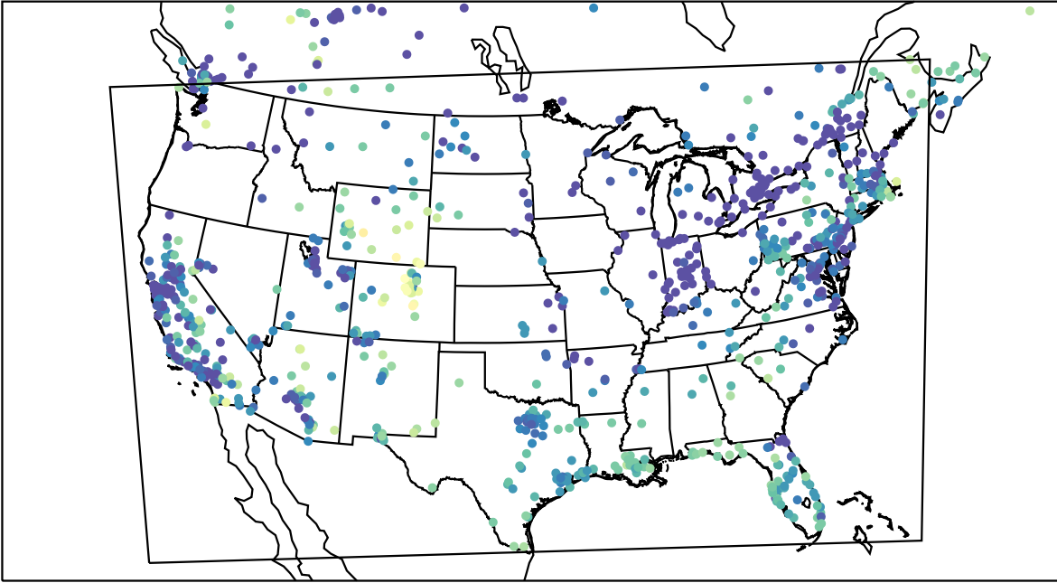
AirNOW (2023-12-28_18:00:00)
