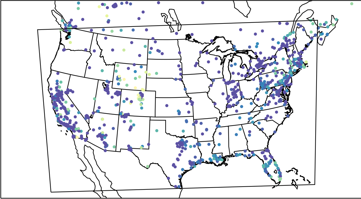
AirNOW (2023-12-28_15:00:00)
