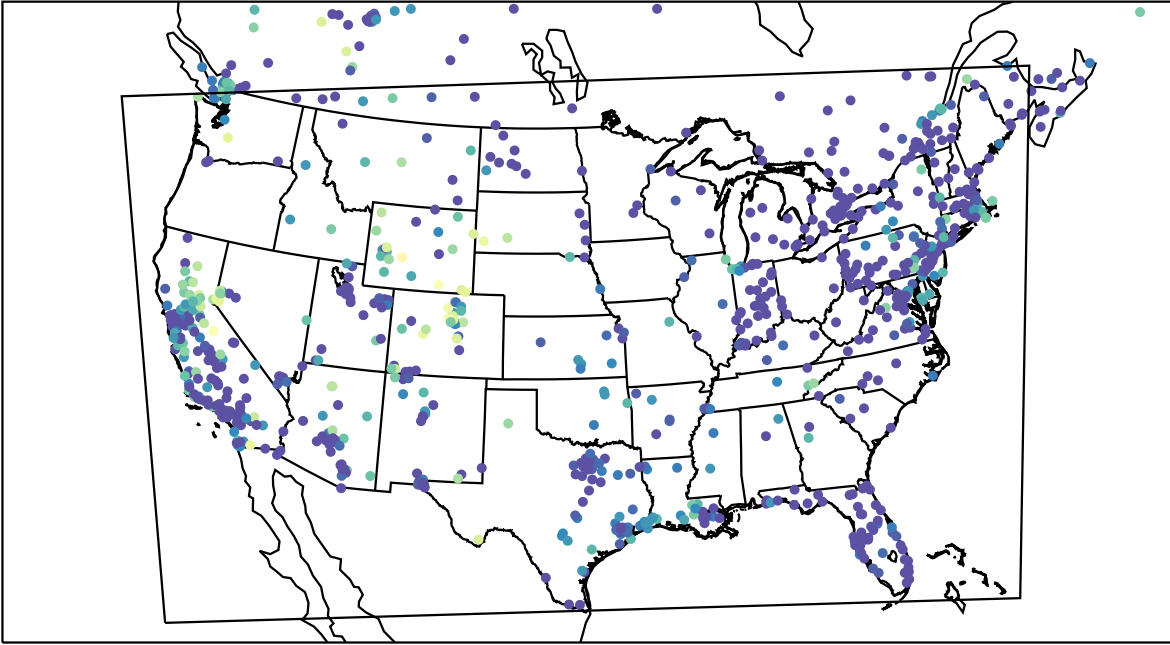
AirNOW (2023-12-28_04:00:00)
