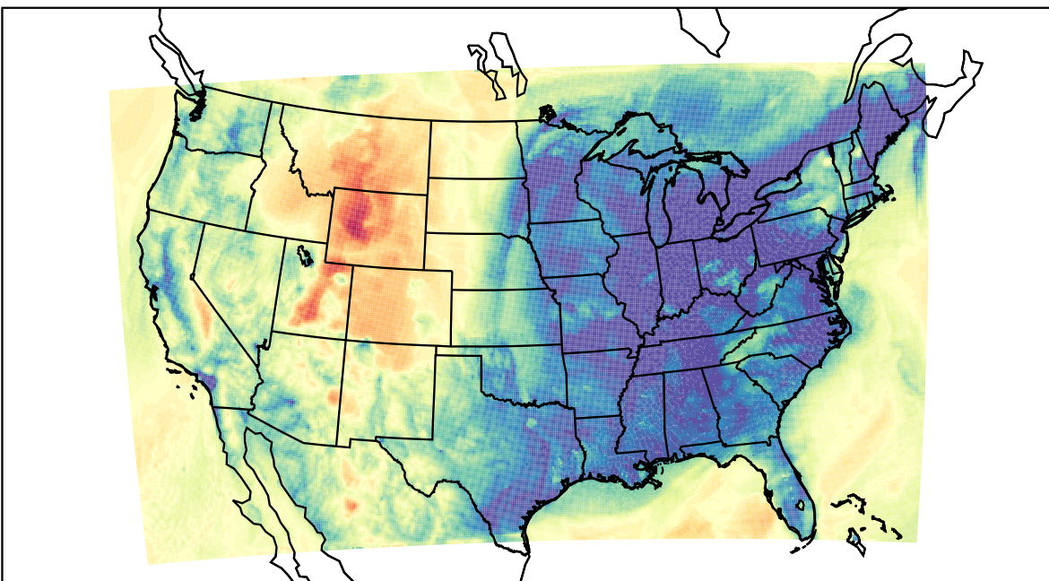
WRF (2023-12-28_09:00:00)
