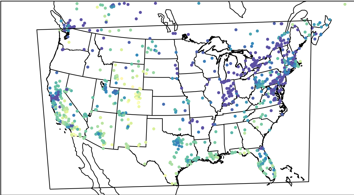
AirNOW (2023-12-28_21:00:00)
