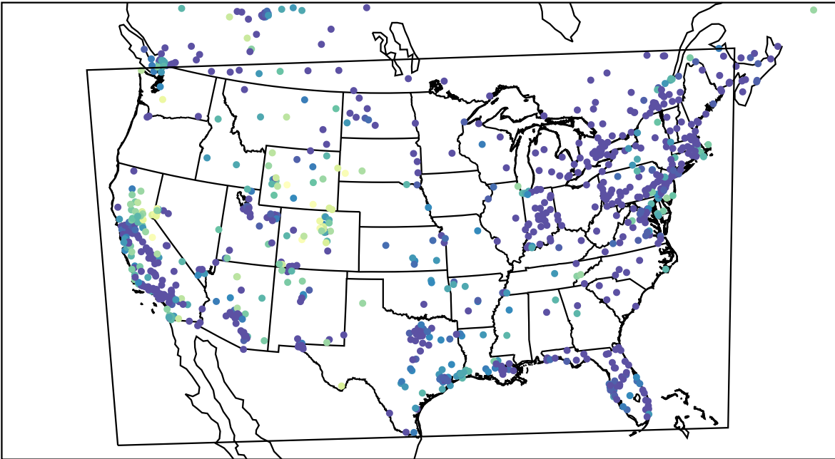
AirNOW (2023-12-28_03:00:00)
