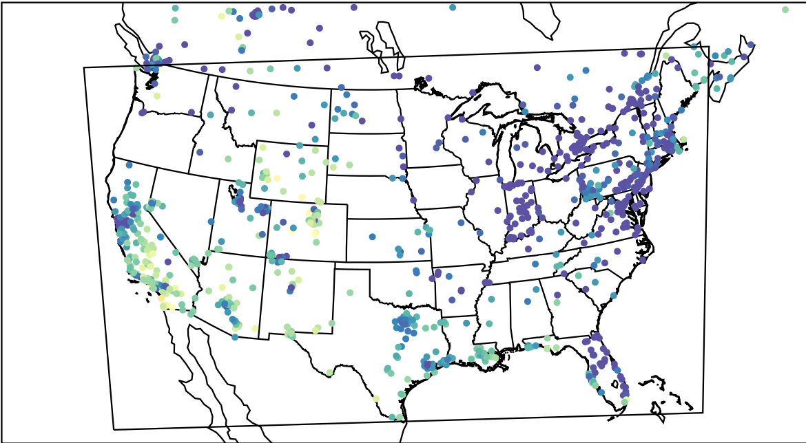
AirNOW (2023-12-28_23:00:00)
