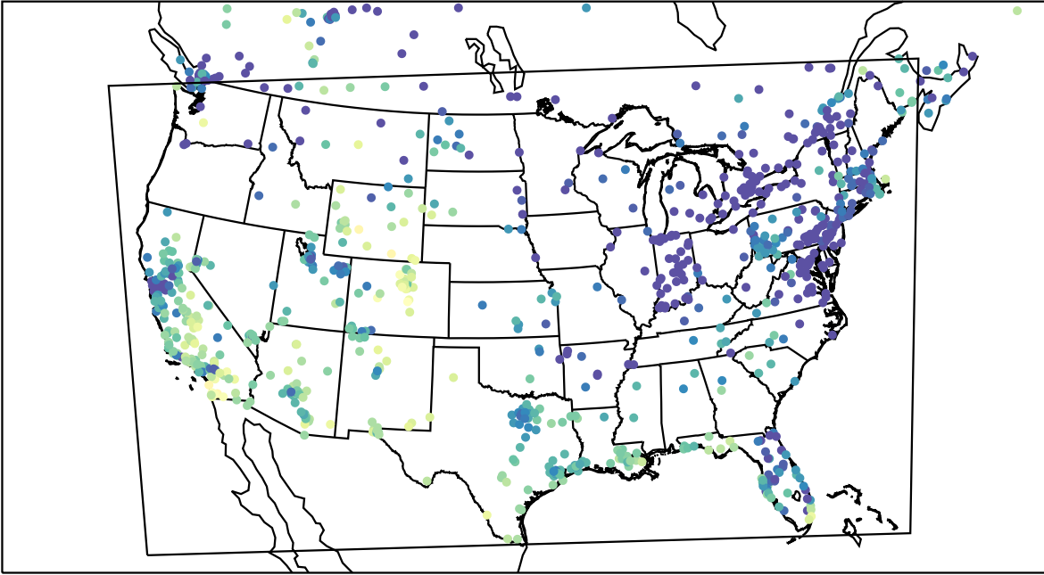
AirNOW (2023-12-28_22:00:00)
