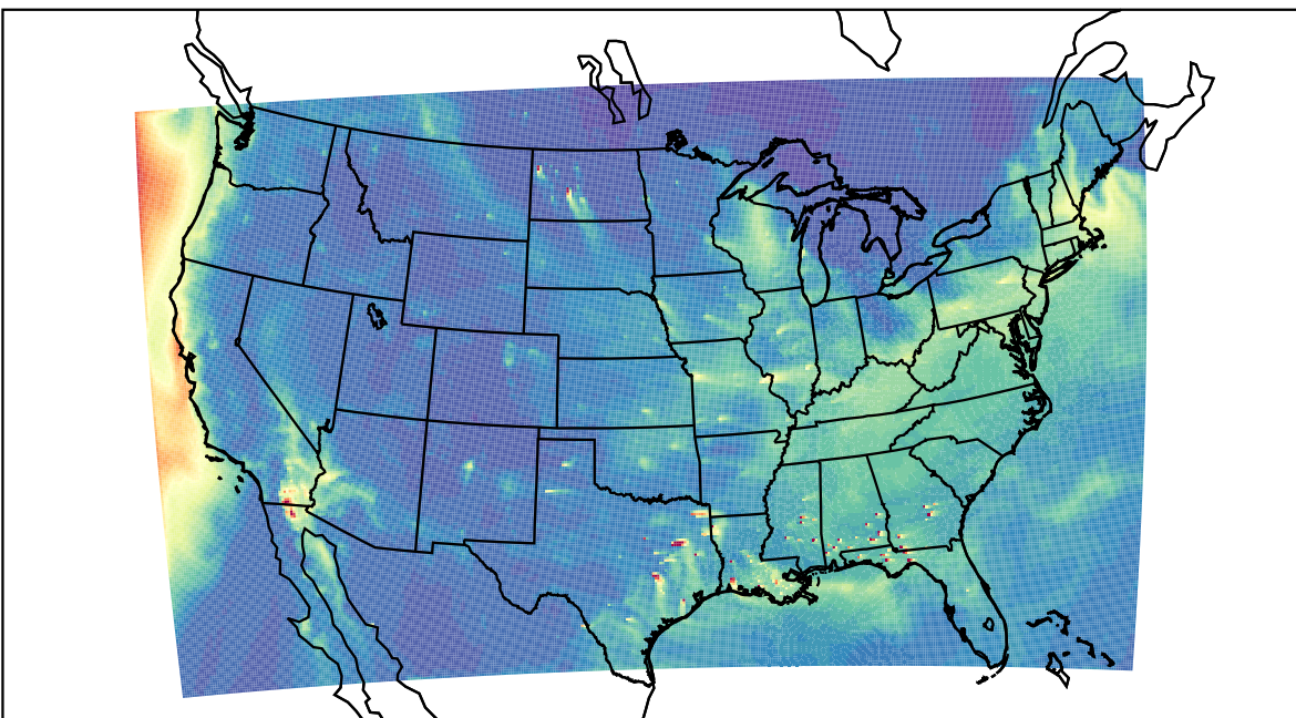
WRF 2023-12-30_17:00:00
