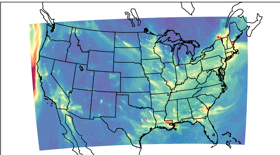
WRF 2023-12-30_07:00:00
