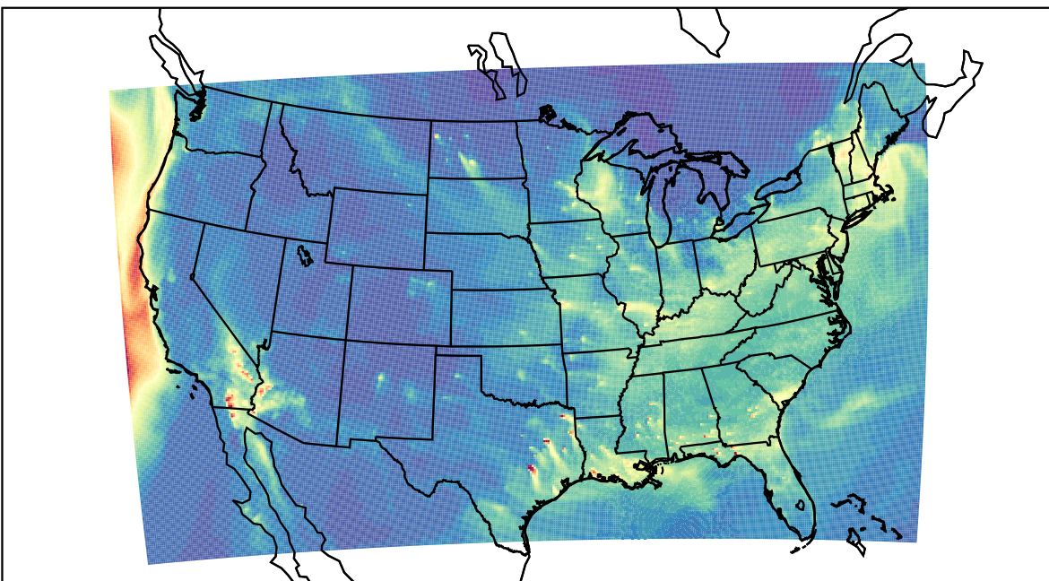
WRF 2023-12-30_13:00:00
