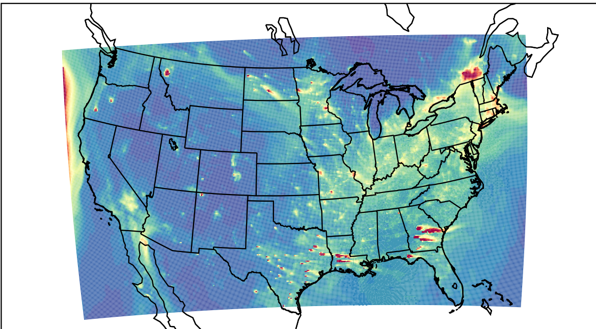
WRF 2023-12-30_00:00:00
