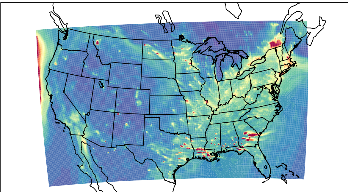
WRF 2023-12-30_01:00:00
