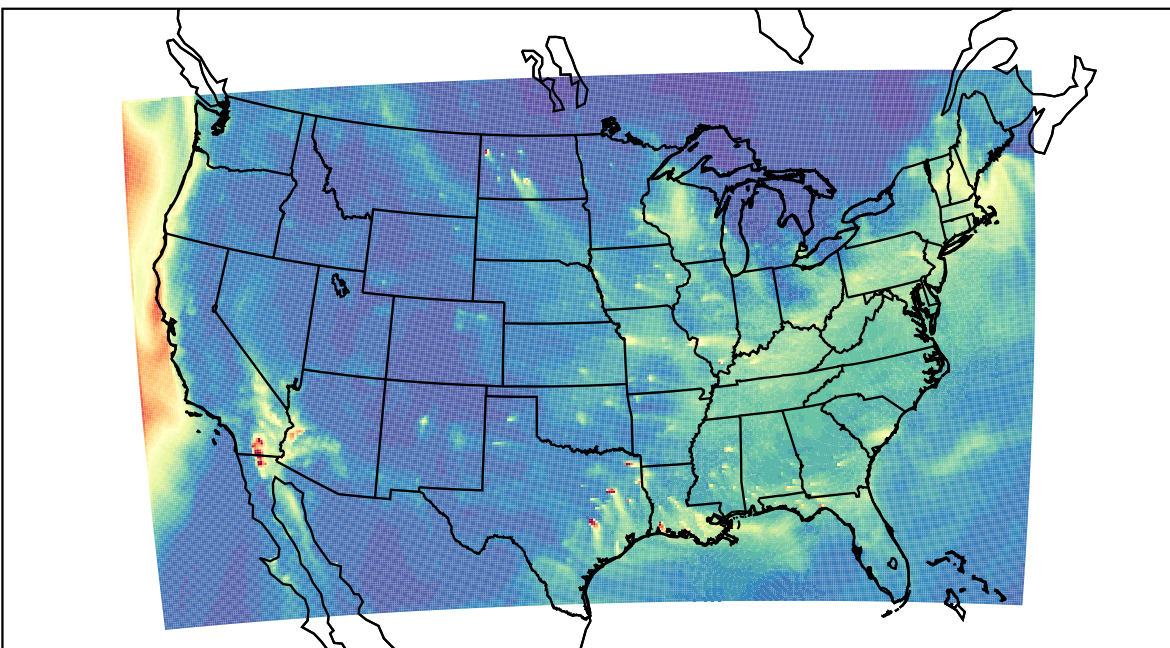
WRF 2023-12-30_15:00:00
