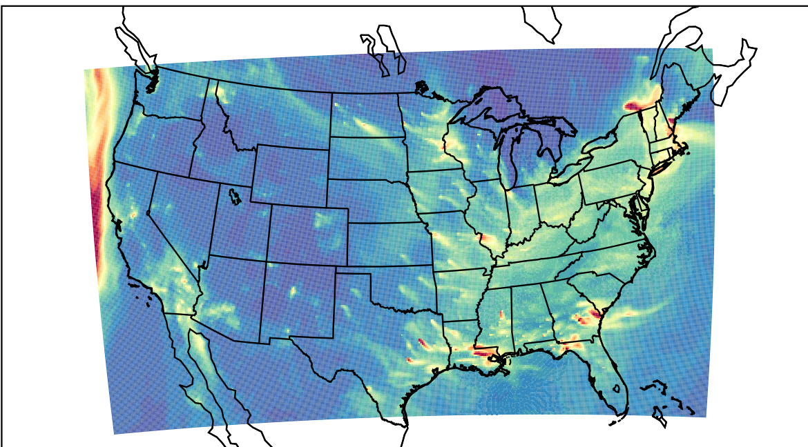
WRF 2023-12-30_06:00:00
