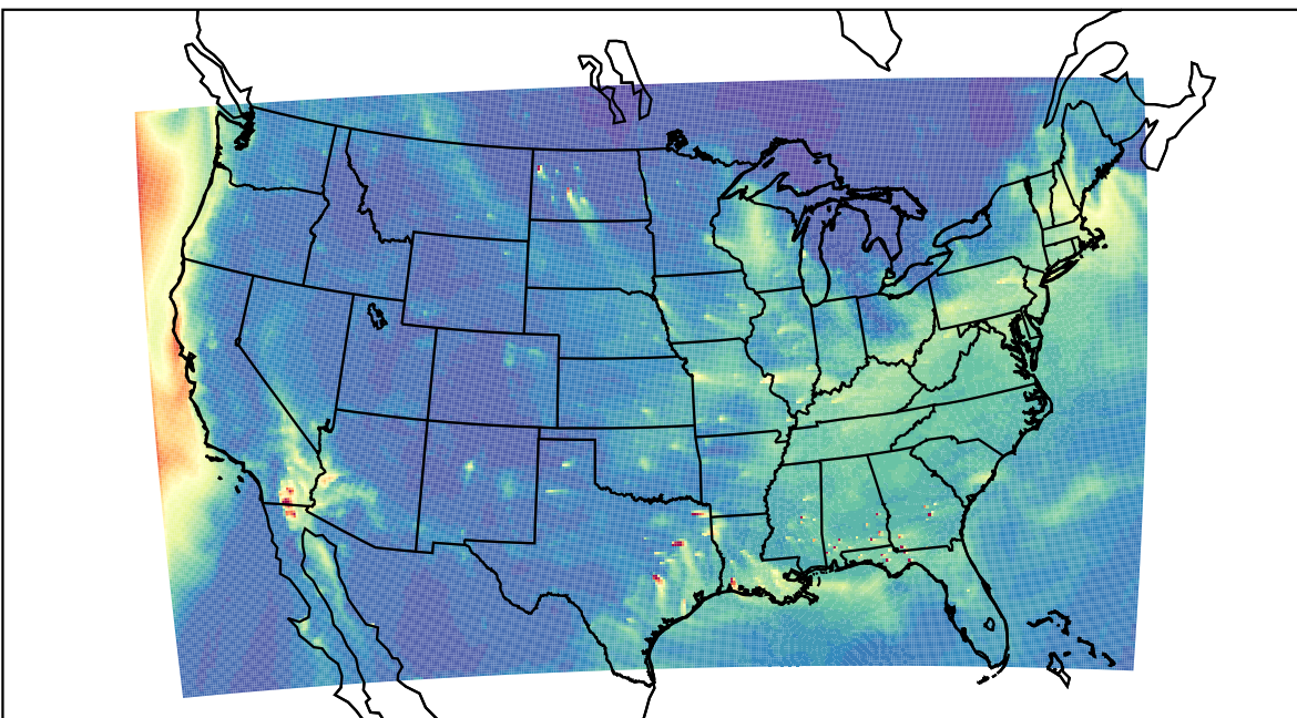
WRF 2023-12-30_16:00:00
