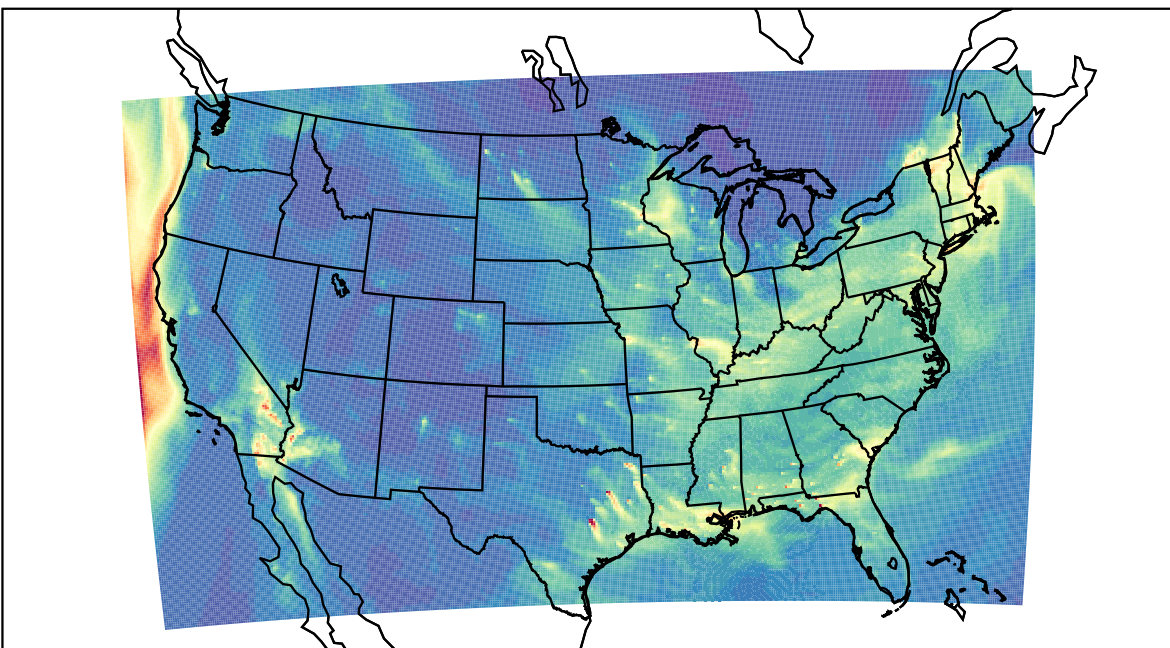
WRF 2023-12-30_11:00:00
