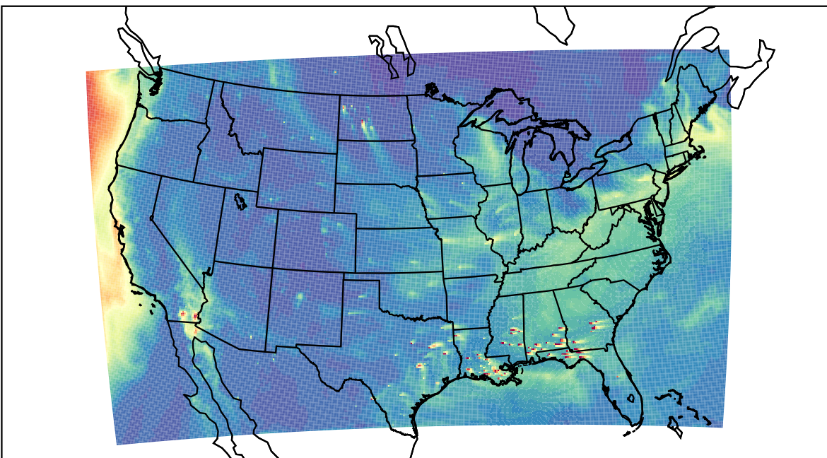
WRF 2023-12-30_19:00:00
