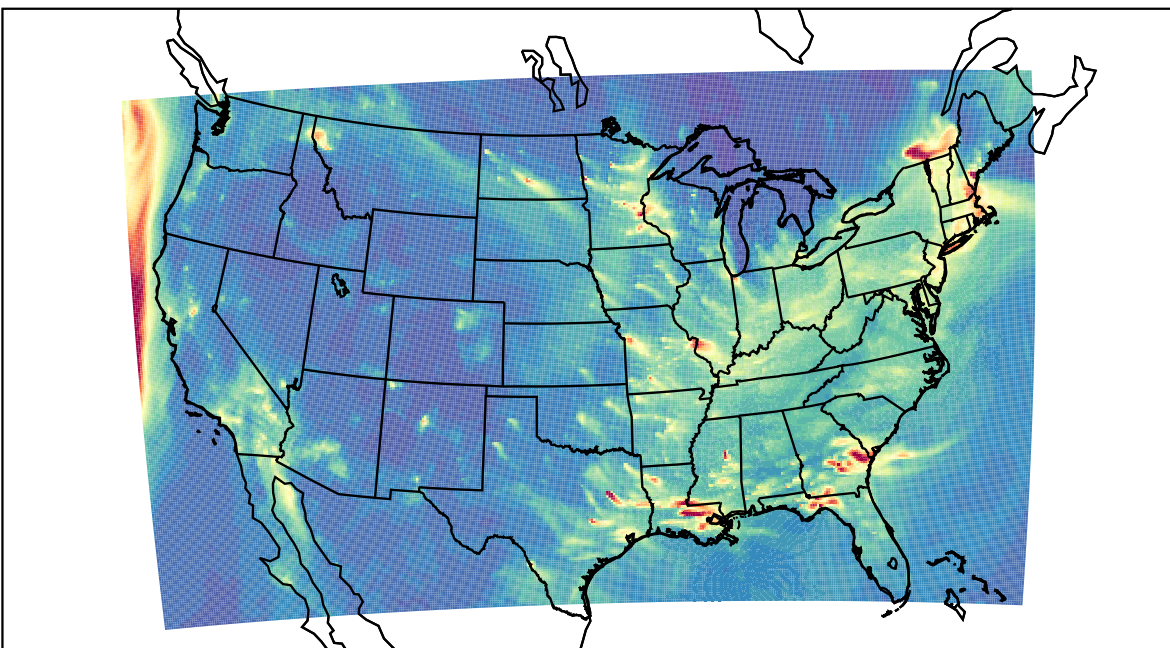
WRF 2023-12-30_05:00:00
