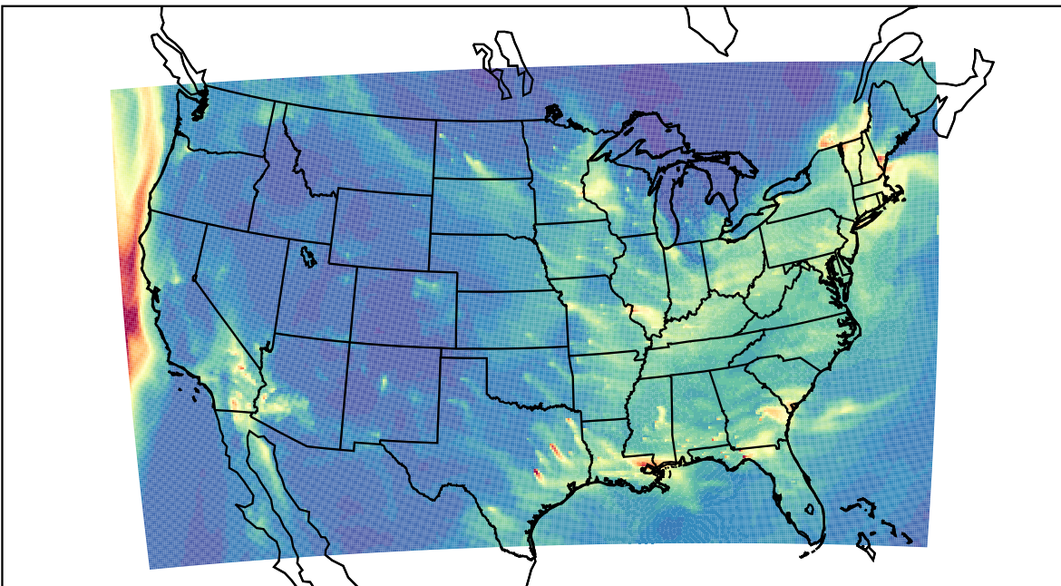
WRF 2023-12-30_09:00:00
