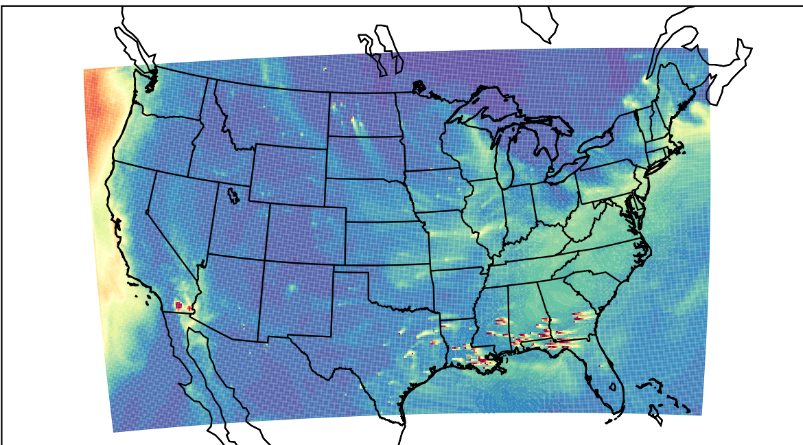
WRF 2023-12-30_21:00:00
