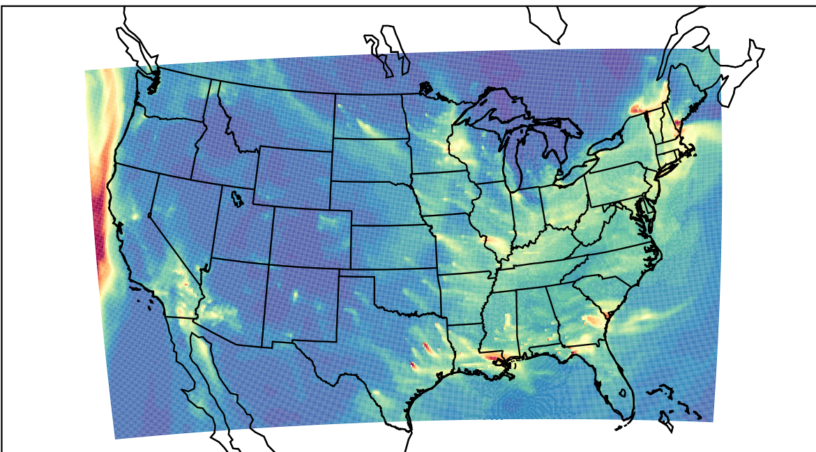
WRF 2023-12-30_08:00:00
