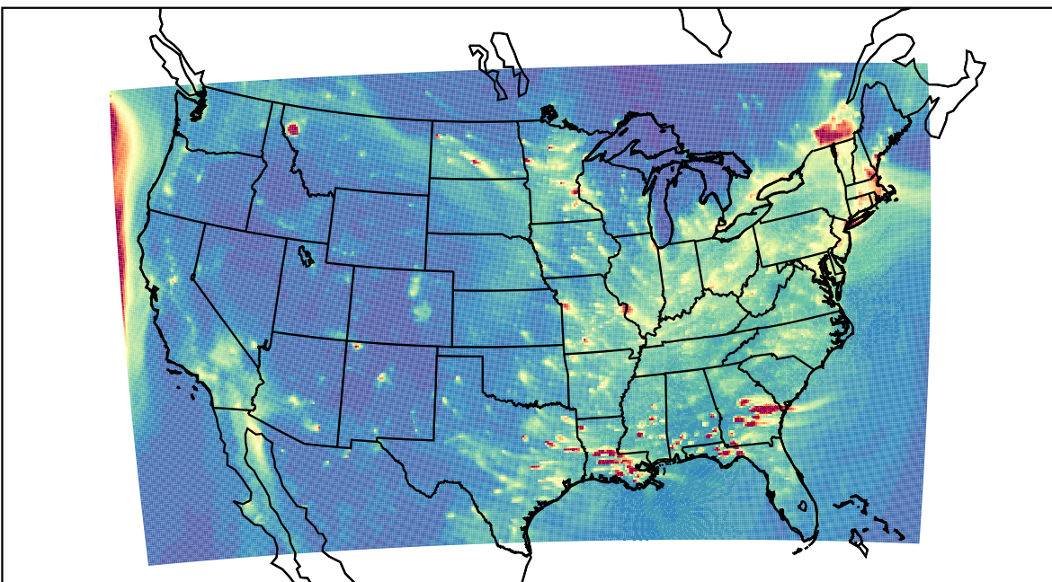
WRF 2023-12-30_02:00:00
