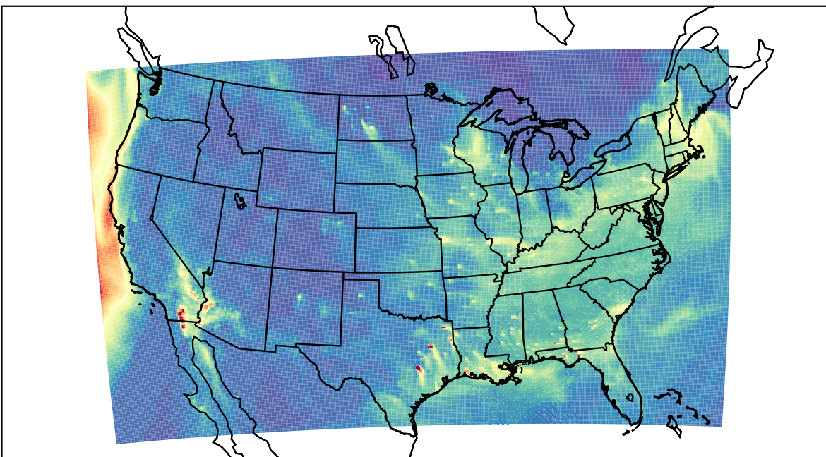
WRF 2023-12-30_14:00:00
