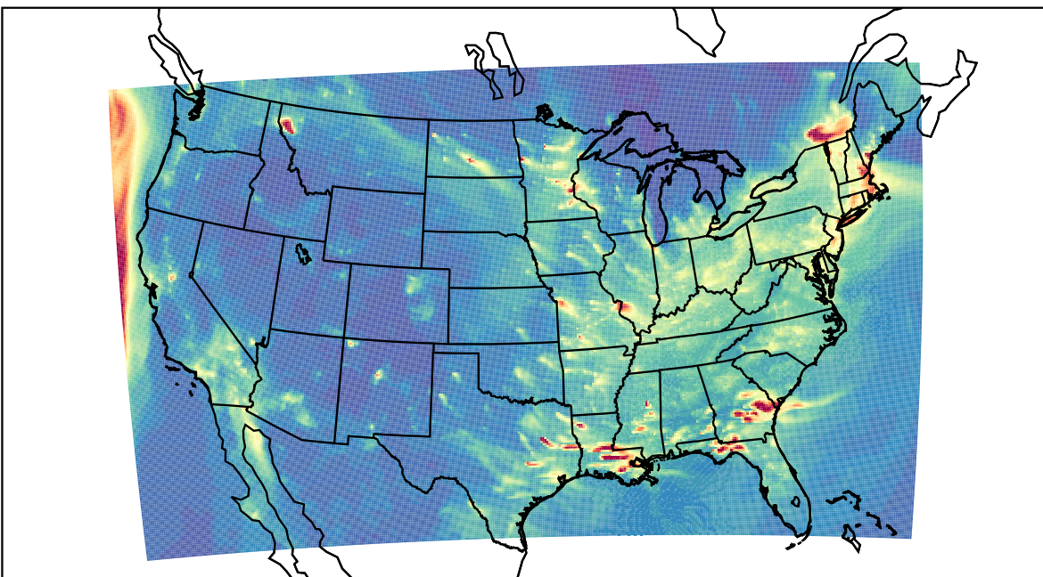
WRF 2023-12-30_04:00:00
