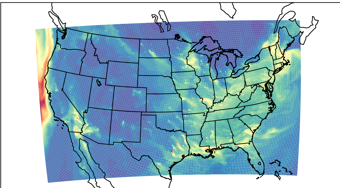
WRF 2023-12-30_10:00:00
