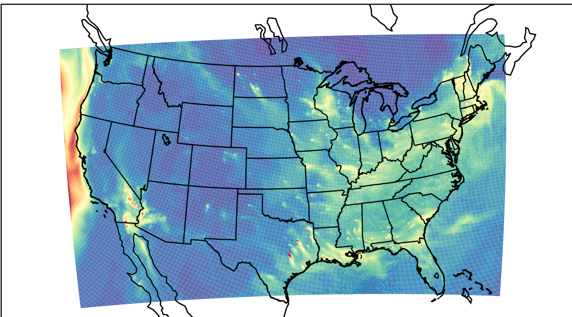
WRF 2023-12-30_12:00:00
