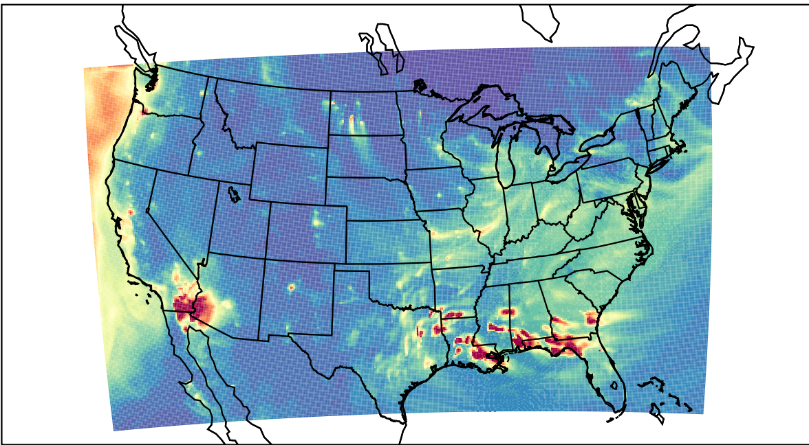
WRF 2023-12-31_05:00:00
