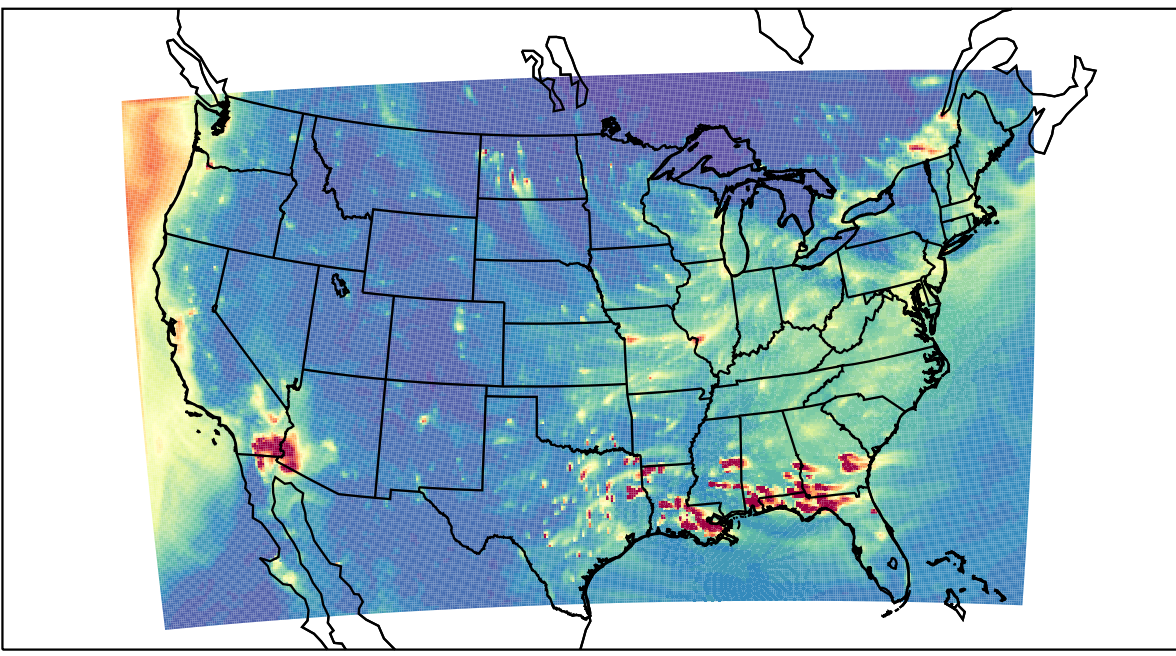
WRF 2023-12-31_02:00:00
