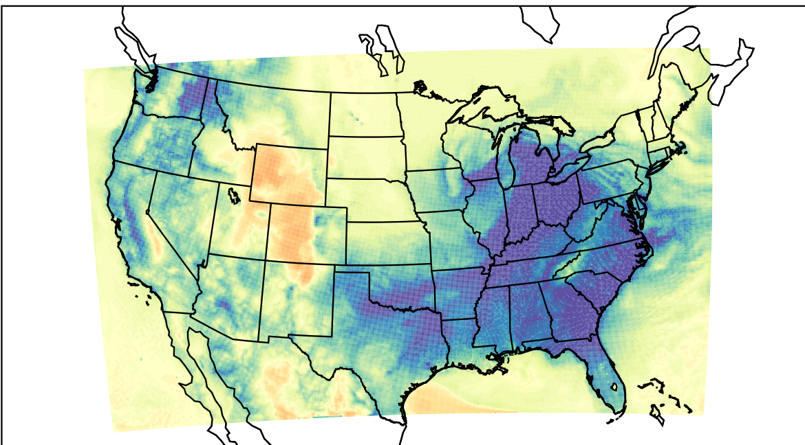
WRF (2023-12-31_14:00:00)
