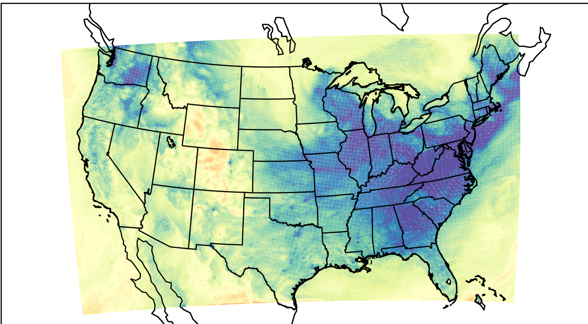
WRF (2023-12-31_00:00:00)
