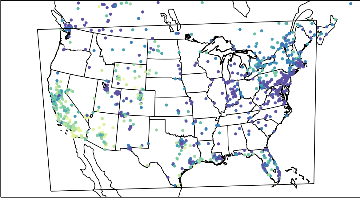
AirNOW (2023-12-31_00:00:00)
