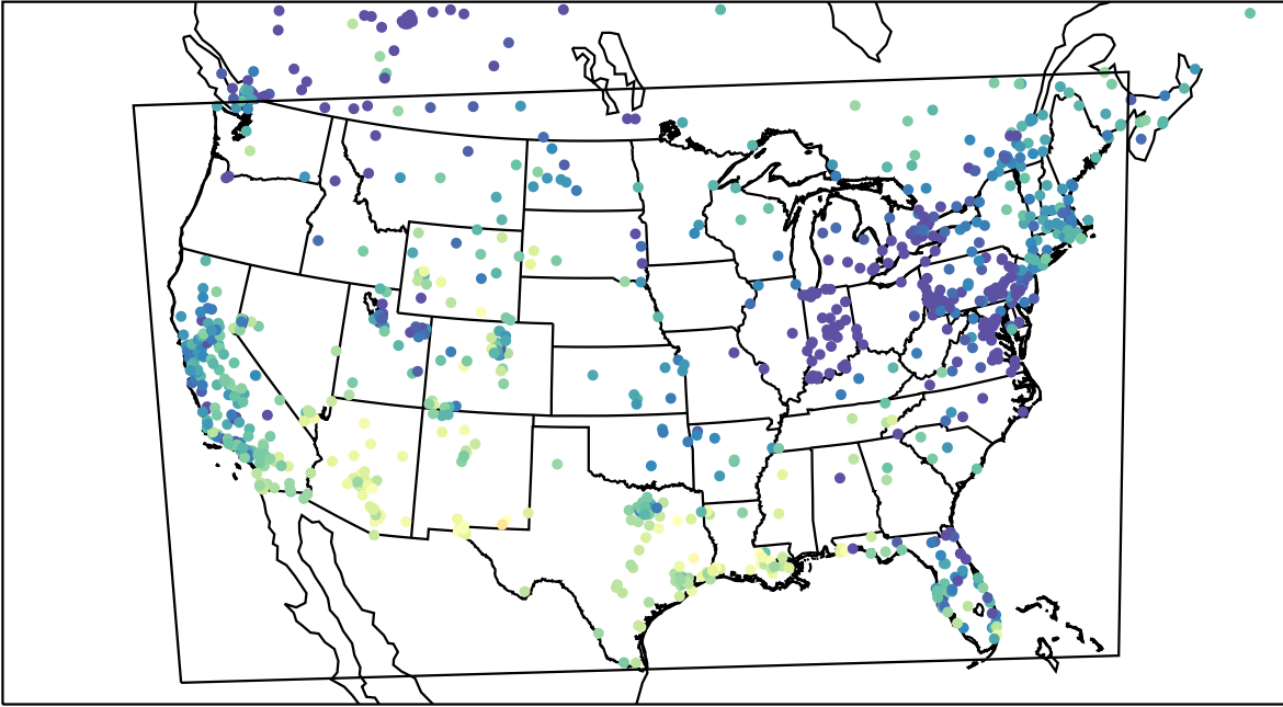
AirNOW (2023-12-31_23:00:00)
