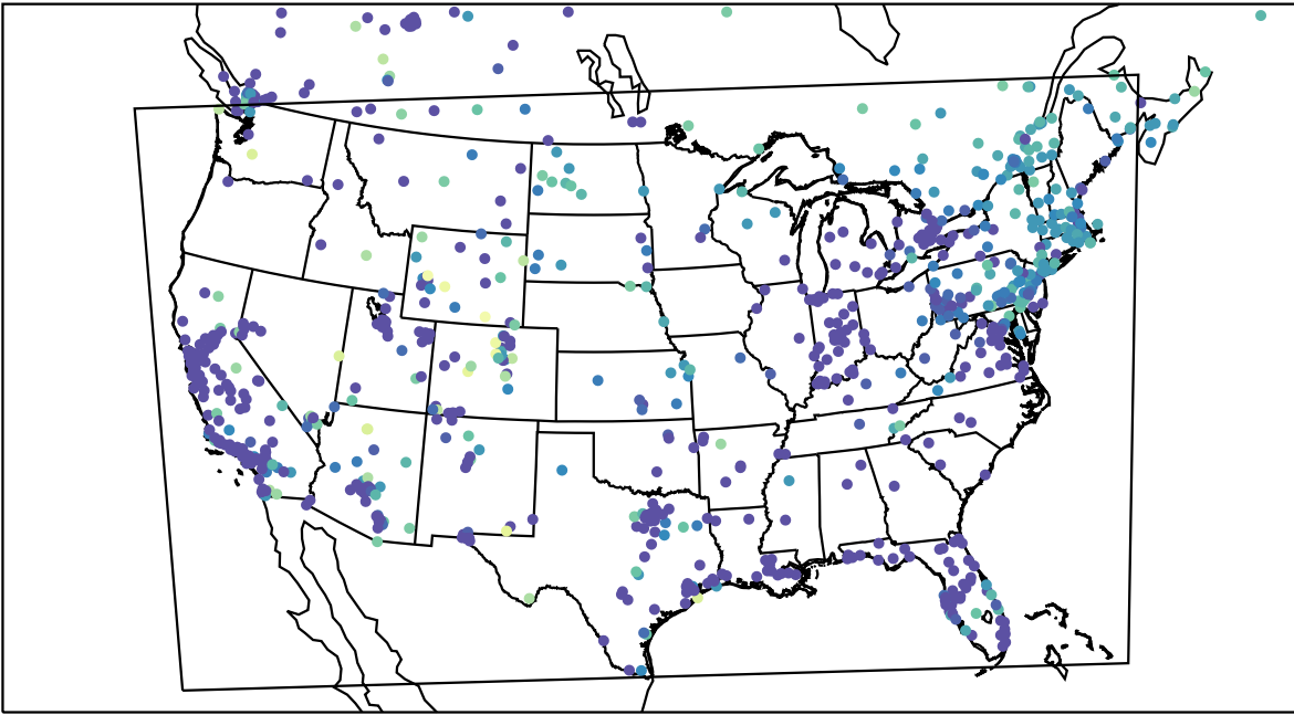
AirNOW (2023-12-31_12:00:00)
