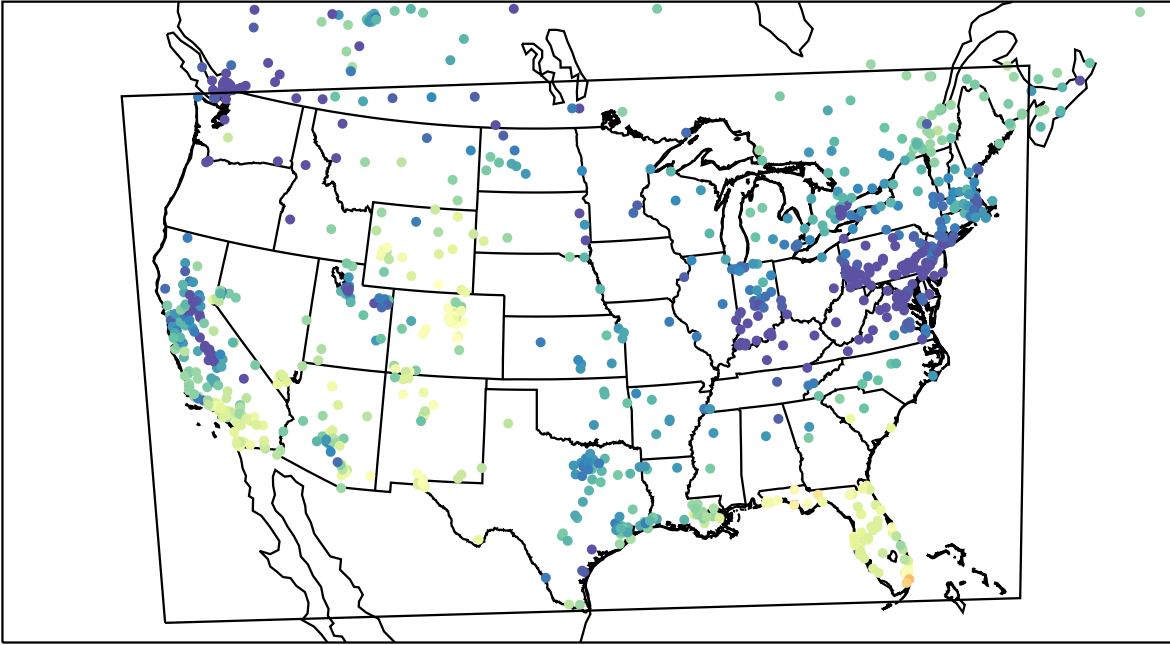
AirNOW (2024-01-01_21:00:00)
