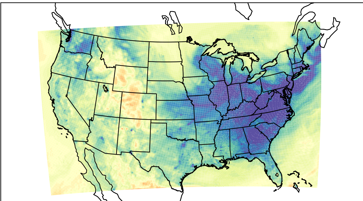
WRF (2023-12-31_01:00:00)
