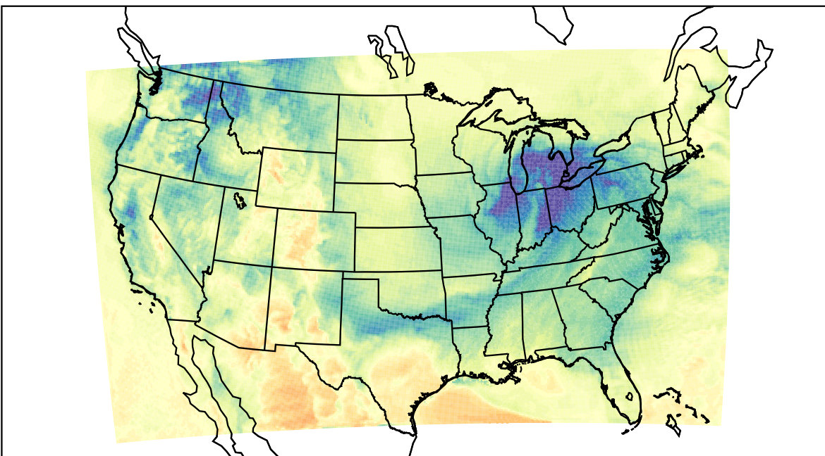
WRF (2023-12-31_20:00:00)
