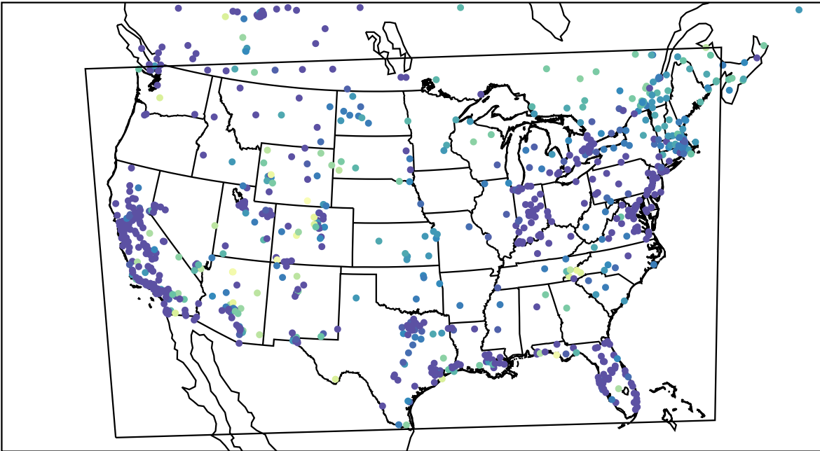
AirNOW (2024-01-01_06:00:00)
