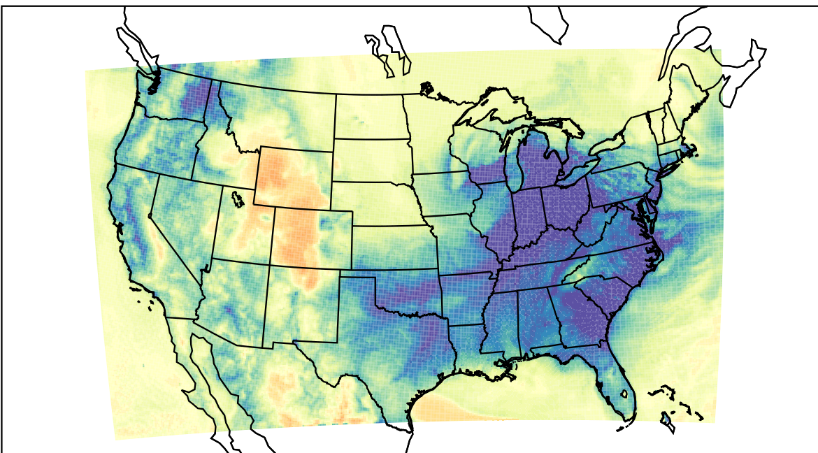
WRF (2023-12-31_12:00:00)
