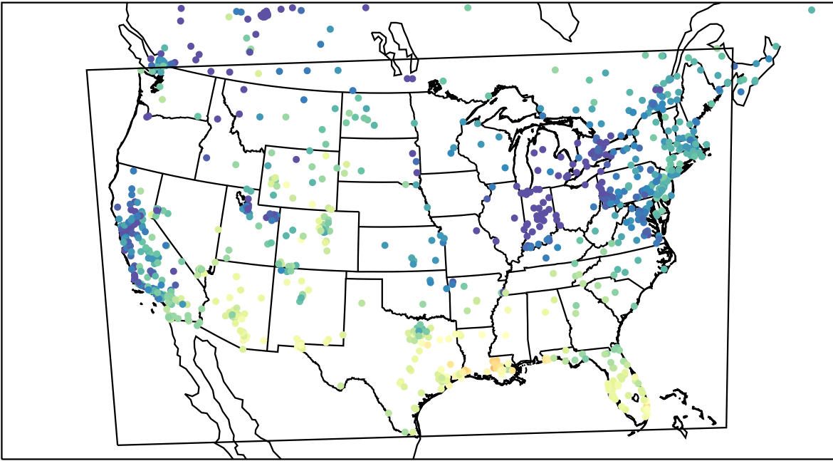
AirNOW (2023-12-31_20:00:00)
