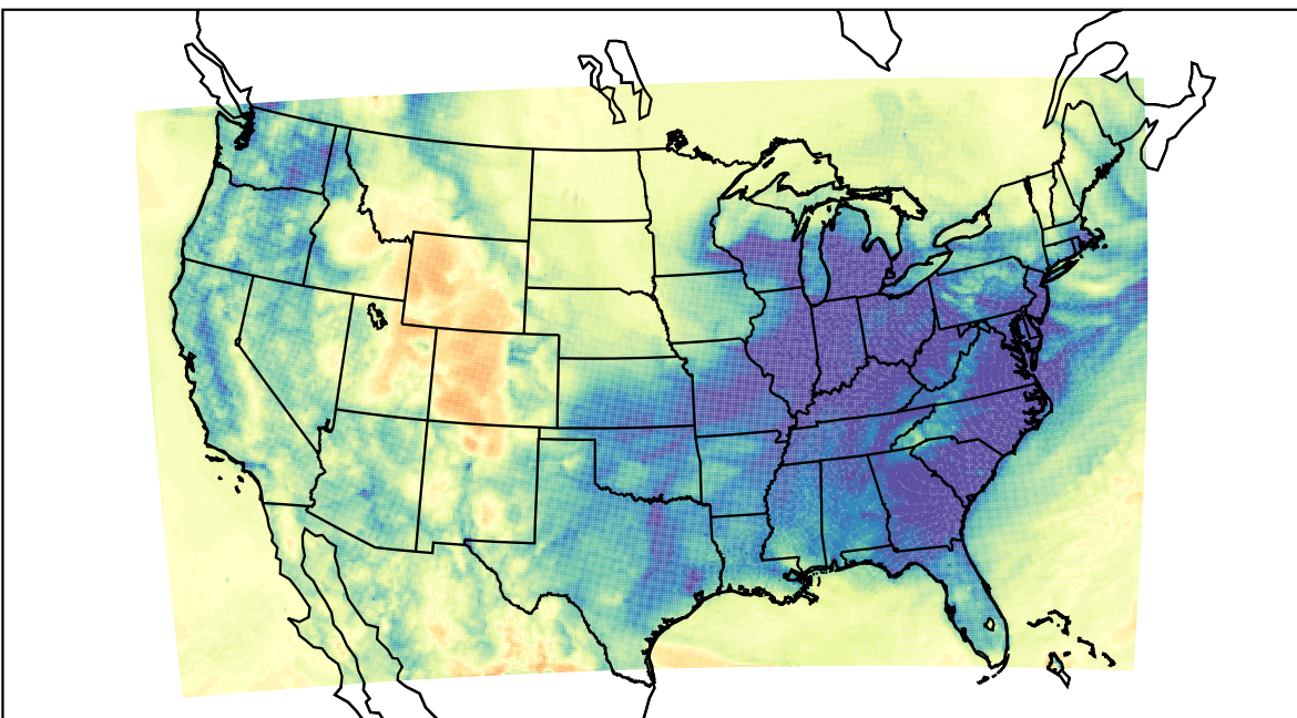
WRF (2023-12-31_07:00:00)
