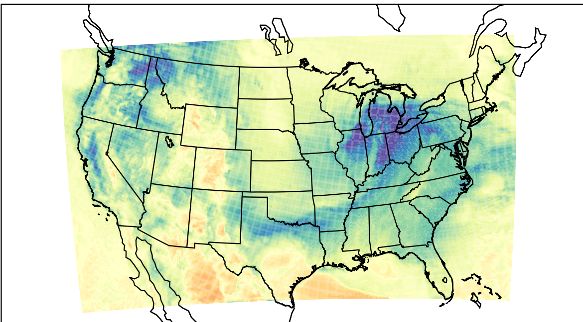
WRF (2023-12-31_19:00:00)
