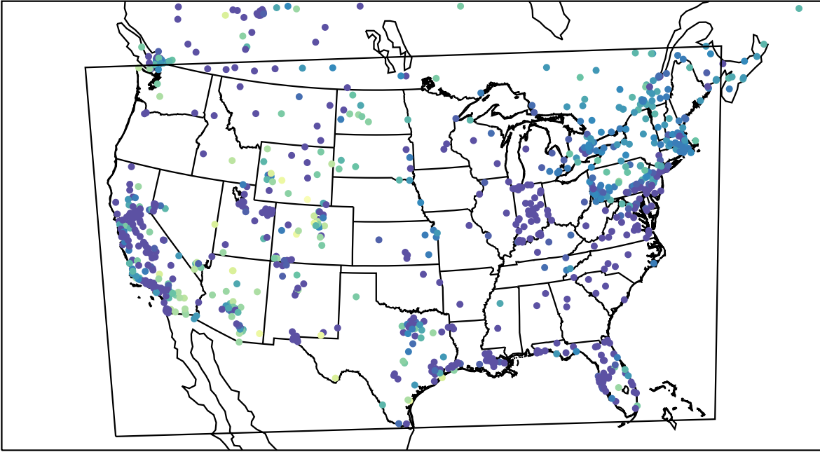
AirNOW (2023-12-31_05:00:00)
