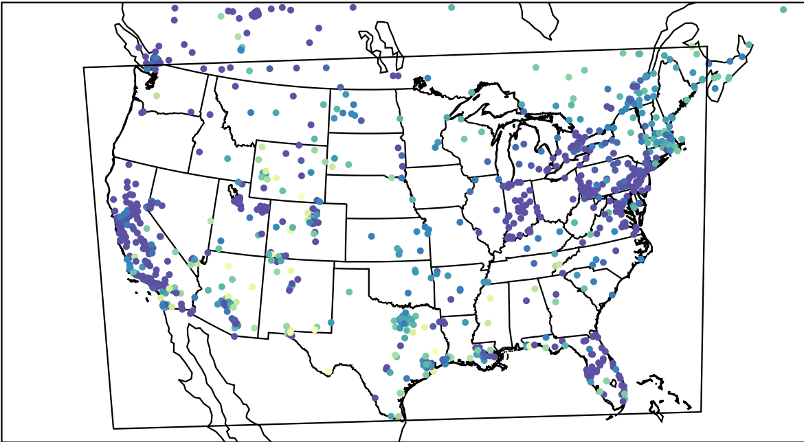
AirNOW (2024-01-01_02:00:00)
