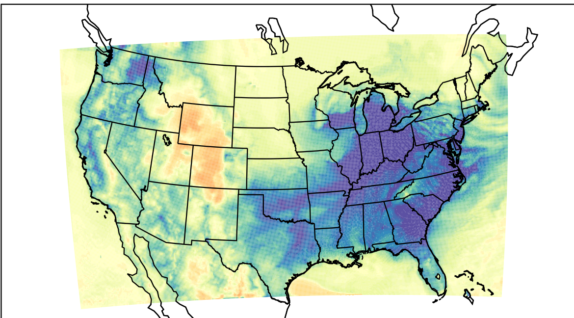
WRF (2023-12-31_11:00:00)
