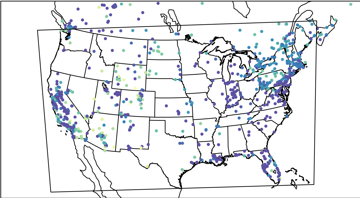
AirNOW (2023-12-31_04:00:00)
