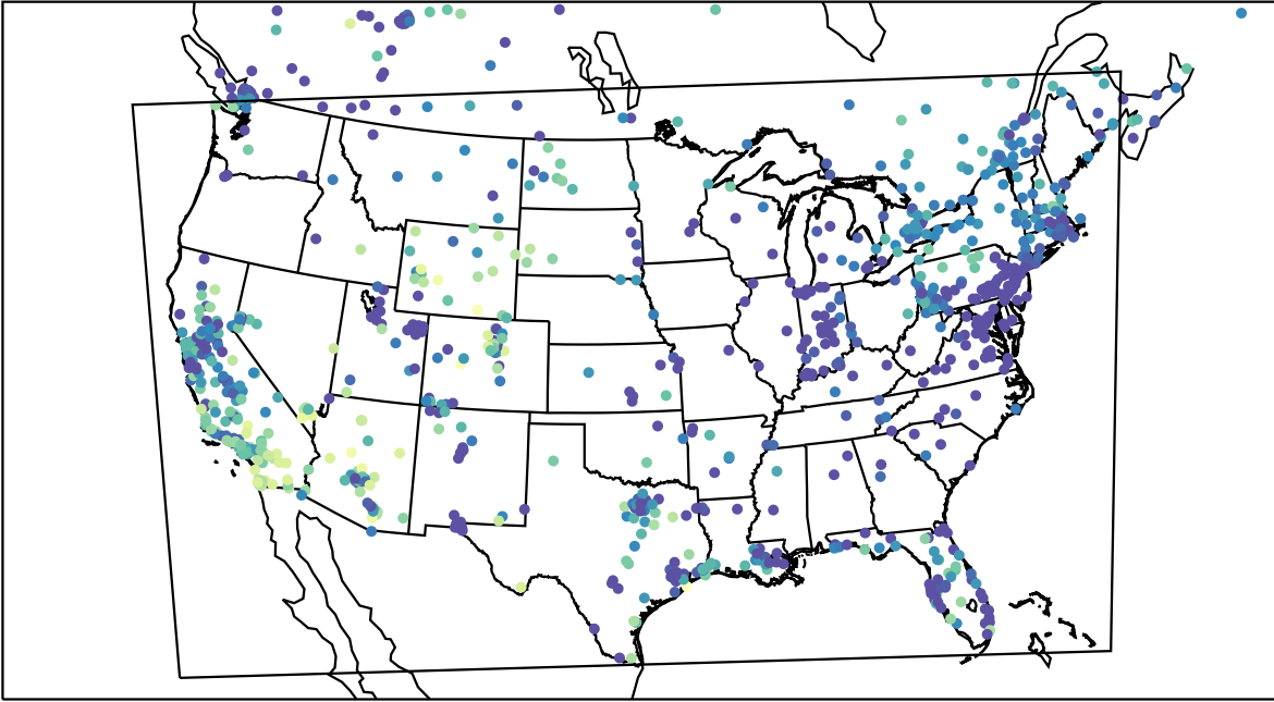
AirNOW (2023-12-31_01:00:00)
