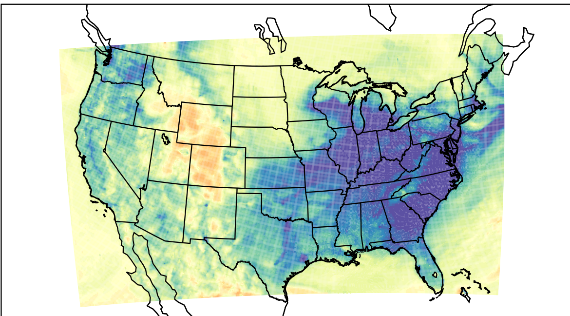
WRF (2023-12-31_05:00:00)
