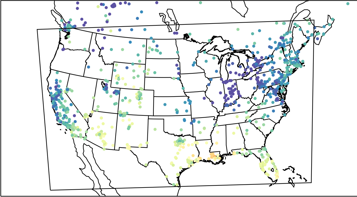
AirNOW (2023-12-31_21:00:00)
