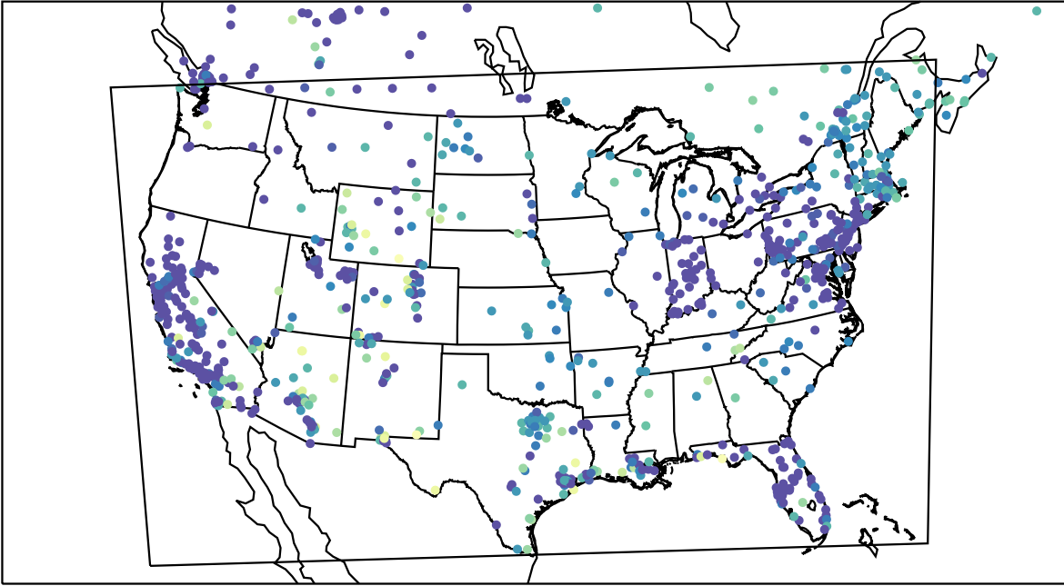
AirNOW (2024-01-01_03:00:00)
