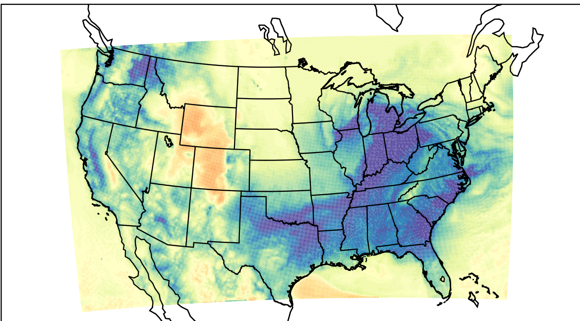
WRF (2023-12-31_15:00:00)
