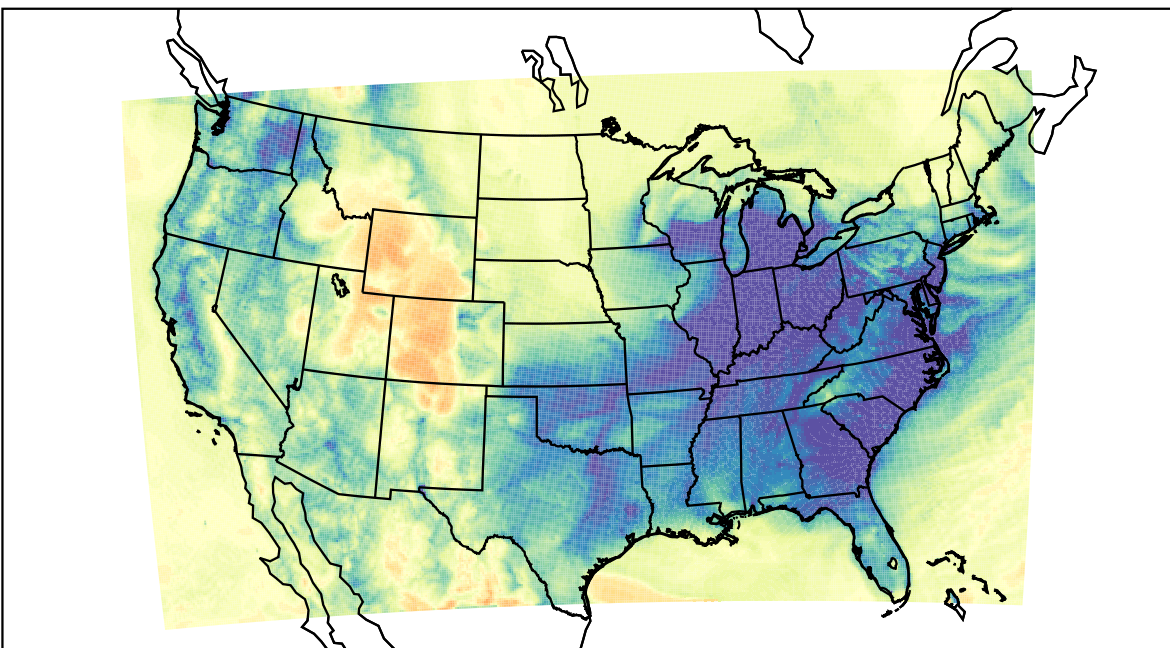
WRF (2023-12-31_09:00:00)
