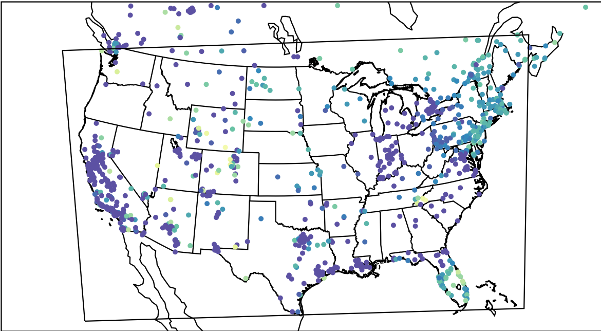
AirNOW (2023-12-31_14:00:00)
