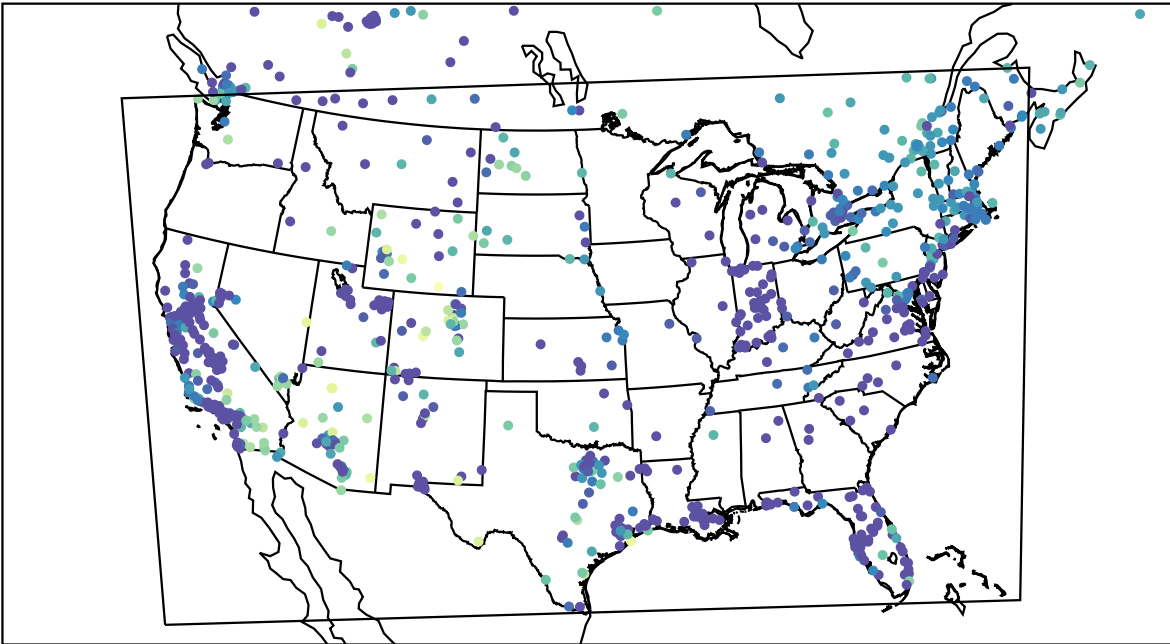
AirNOW (2023-12-31_06:00:00)
