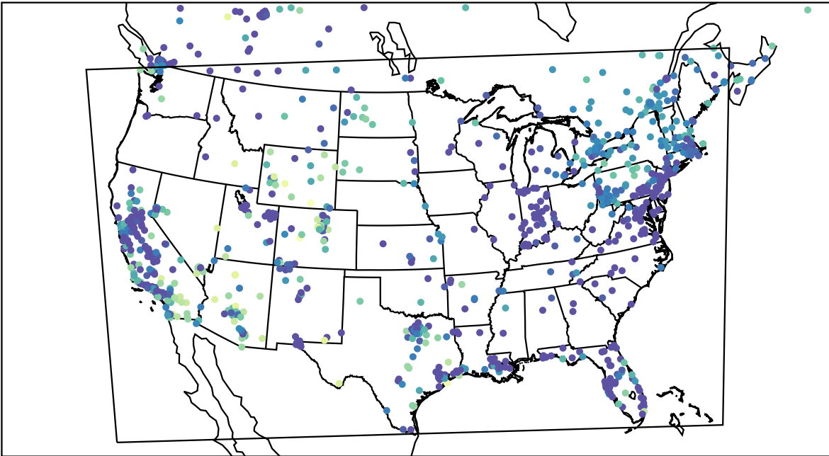
AirNOW (2023-12-31_03:00:00)
