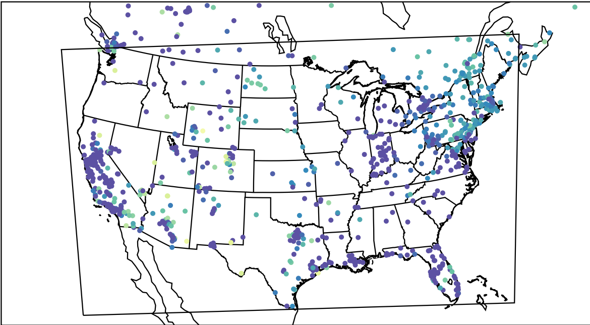
AirNOW (2023-12-31_09:00:00)
