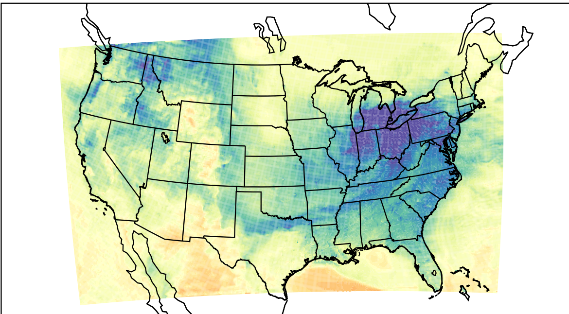
WRF (2023-12-31_23:00:00)
