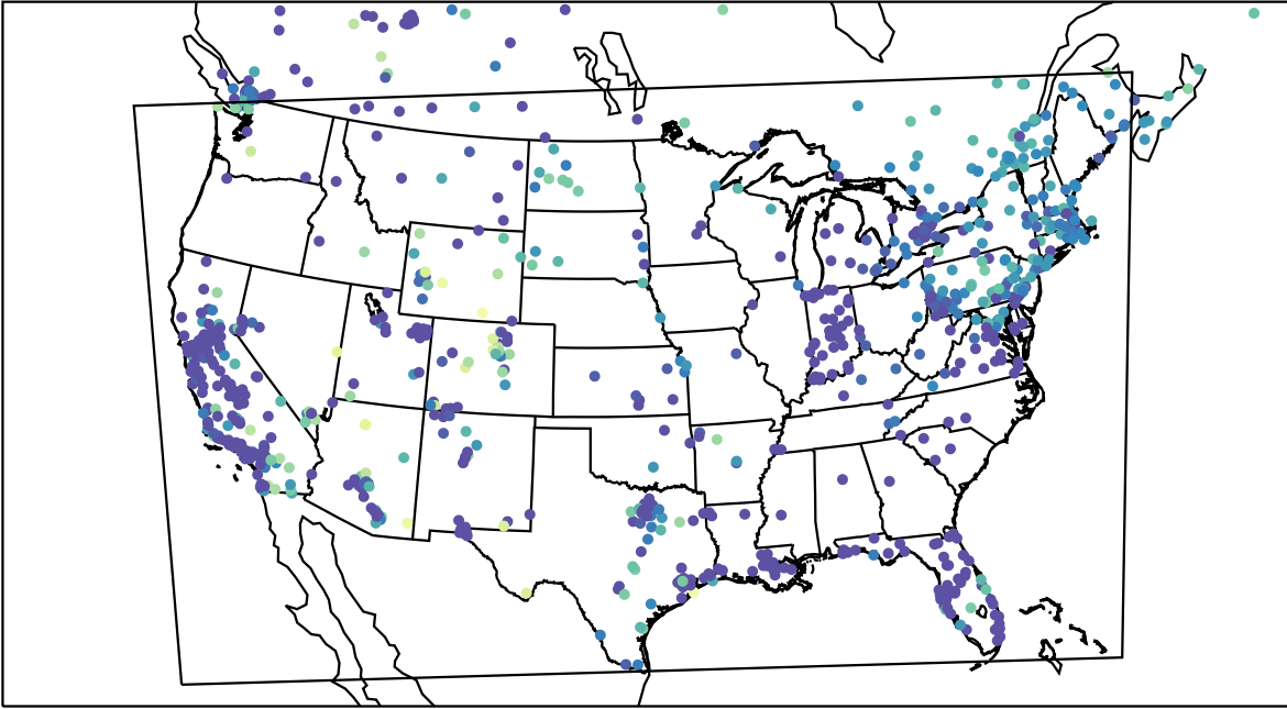
AirNOW (2023-12-31_08:00:00)
