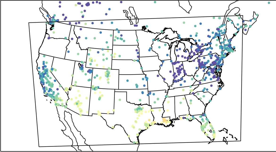
AirNOW (2023-12-31_22:00:00)
