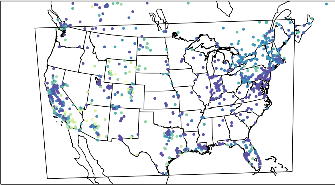
AirNOW (2023-12-31_02:00:00)
