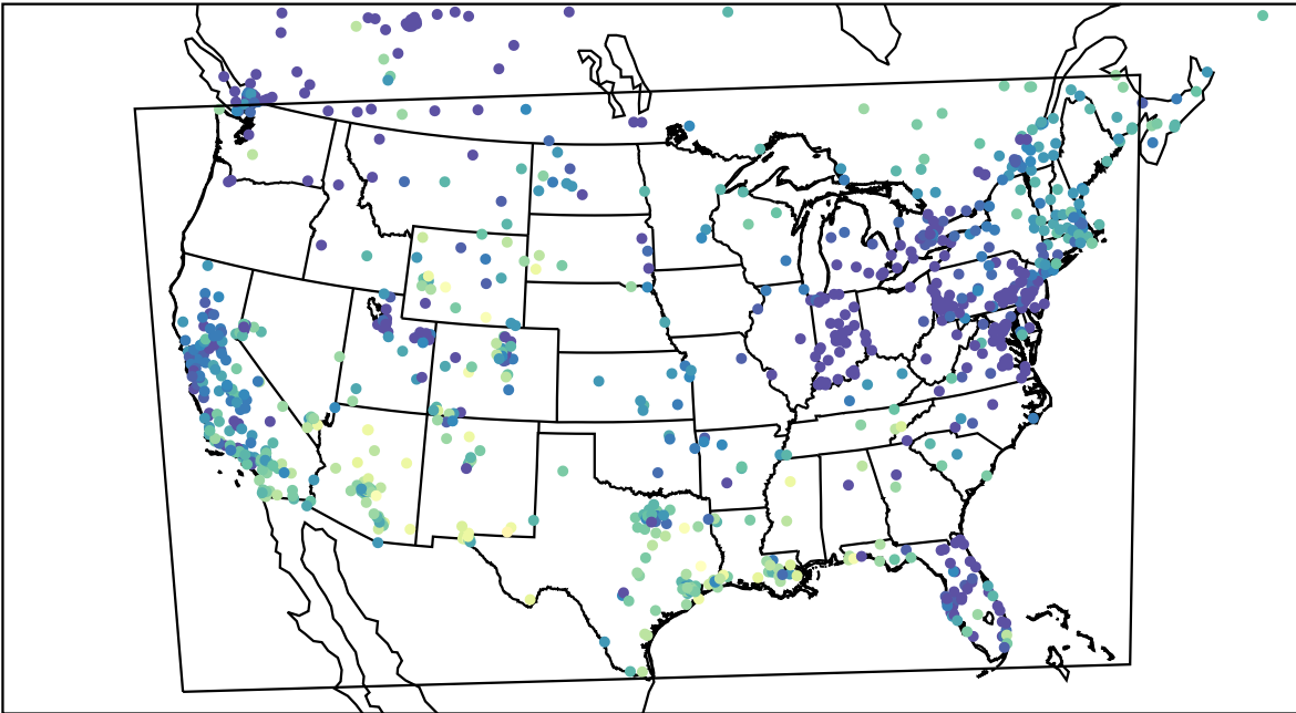
AirNOW (2024-01-01_00:00:00)
