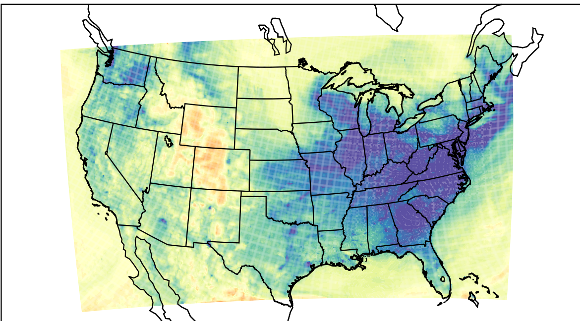
WRF (2023-12-31_02:00:00)
