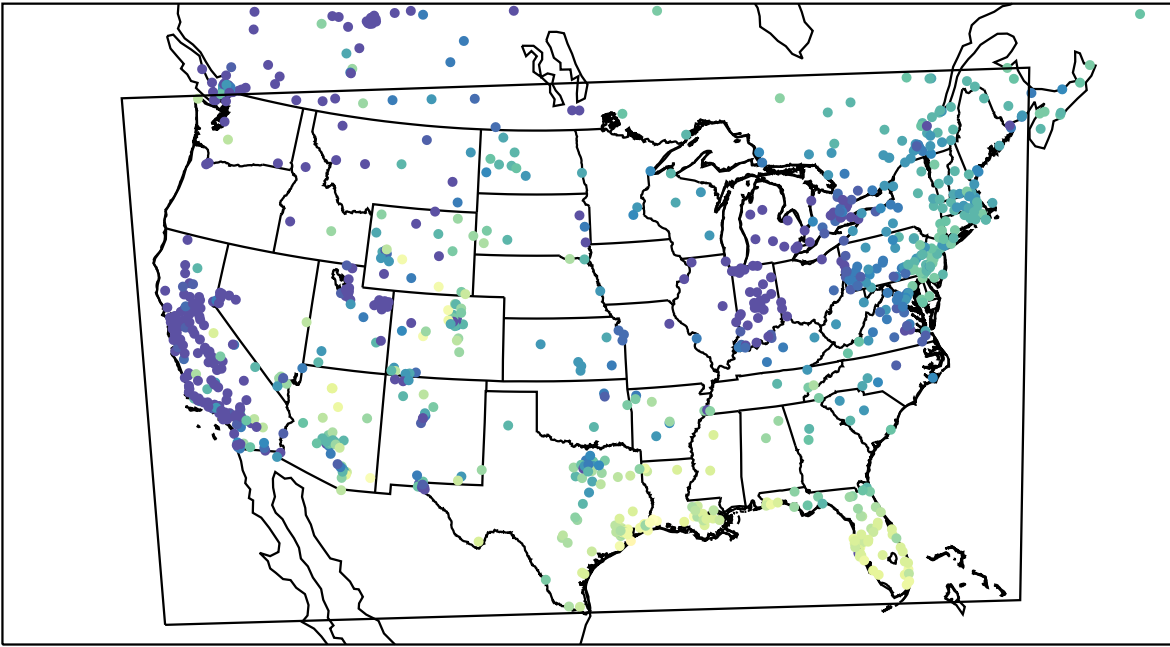
AirNOW (2023-12-31_17:00:00)
