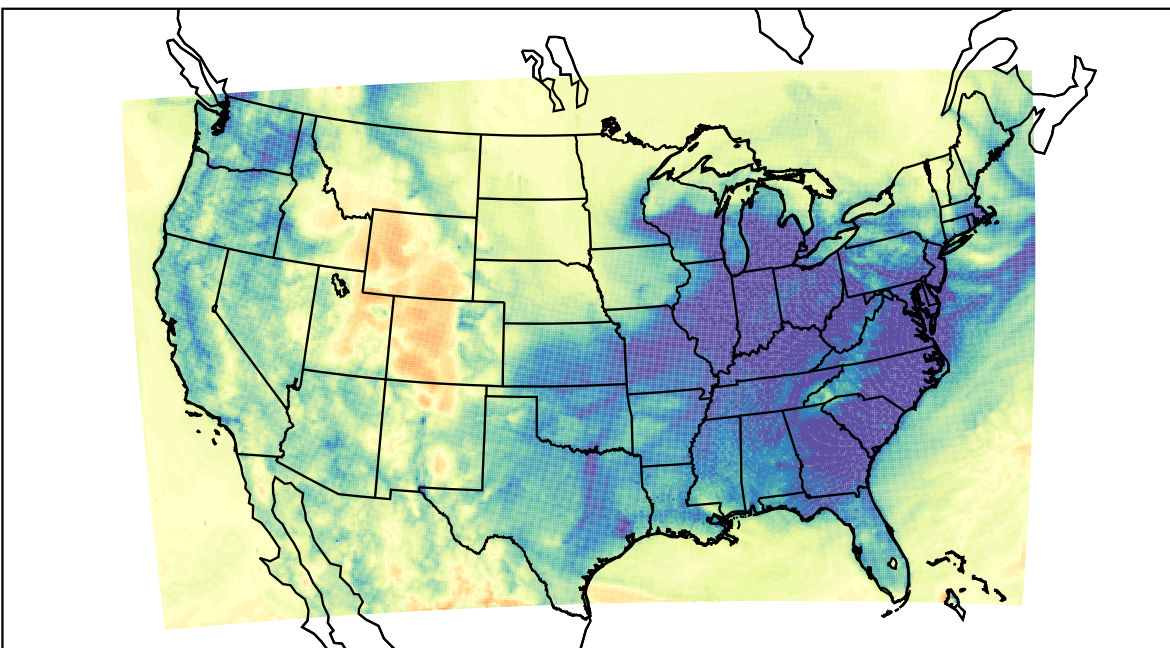
WRF (2023-12-31_06:00:00)
