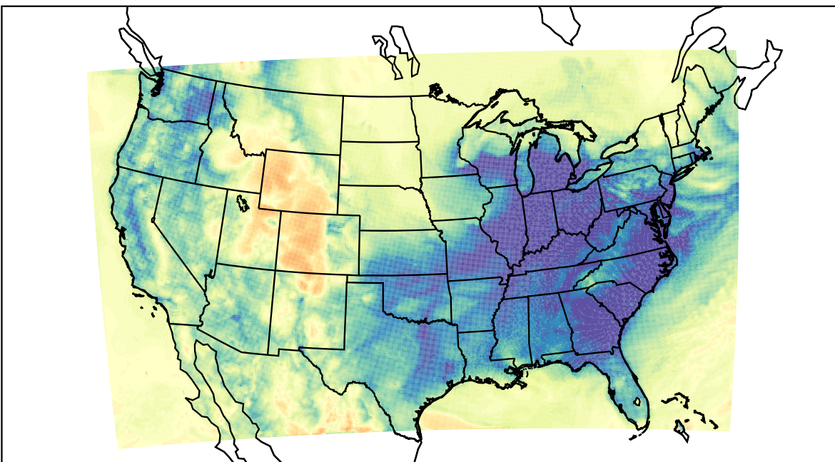
WRF (2023-12-31_08:00:00)
