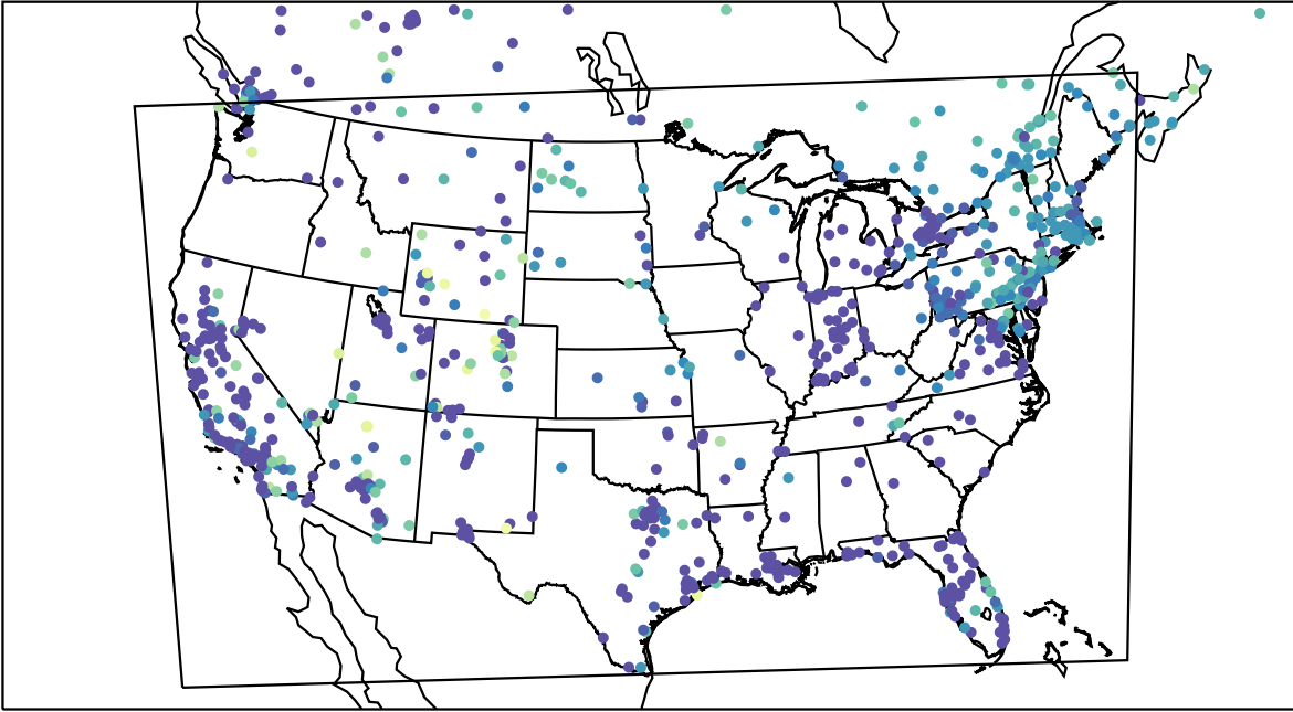
AirNOW (2023-12-31_11:00:00)
