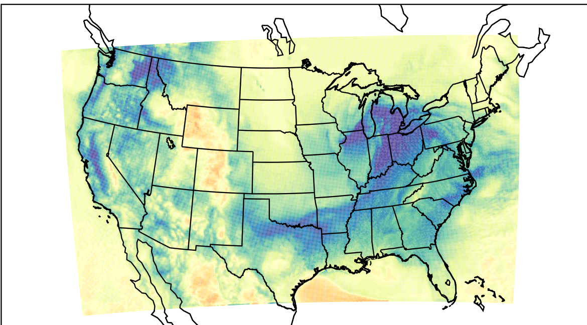
WRF (2023-12-31_17:00:00)
