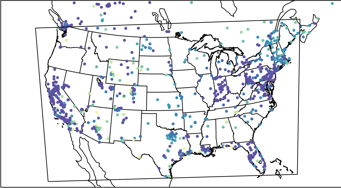
AirNOW (2024-01-01_04:00:00)
