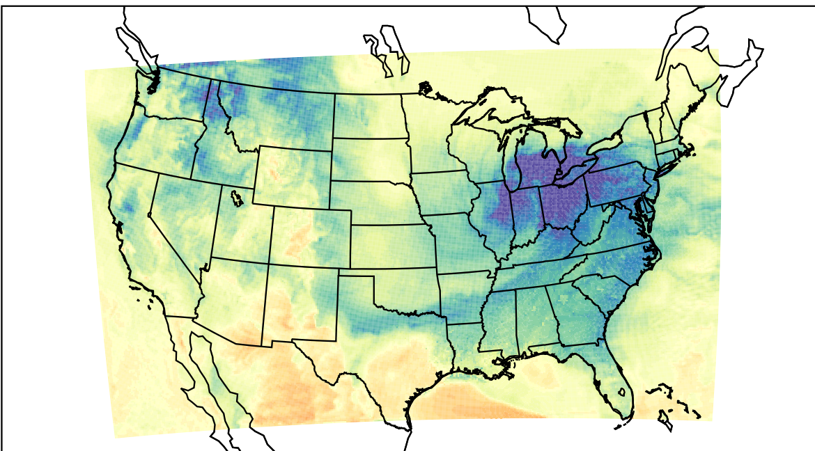
WRF (2023-12-31_22:00:00)
