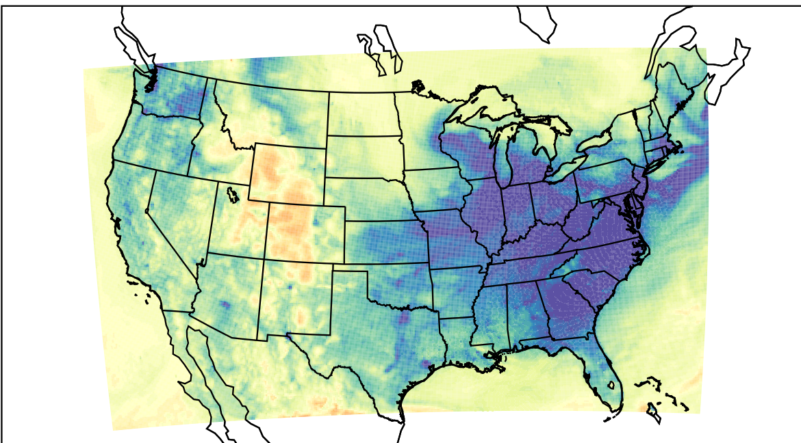
WRF (2023-12-31_03:00:00)
