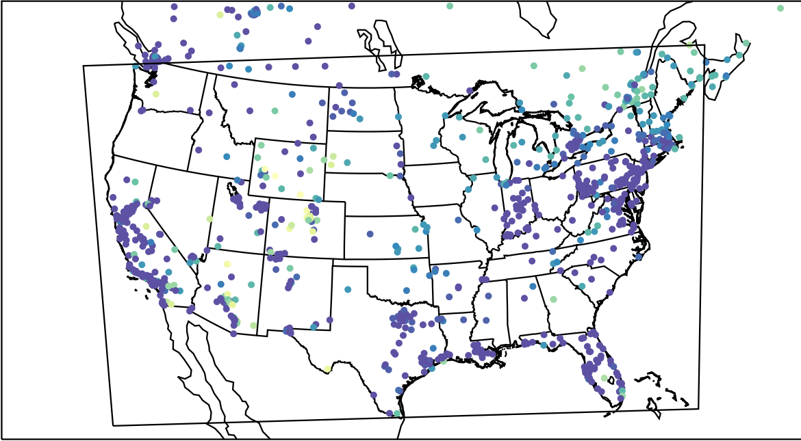
AirNOW (2024-01-01_12:00:00)
