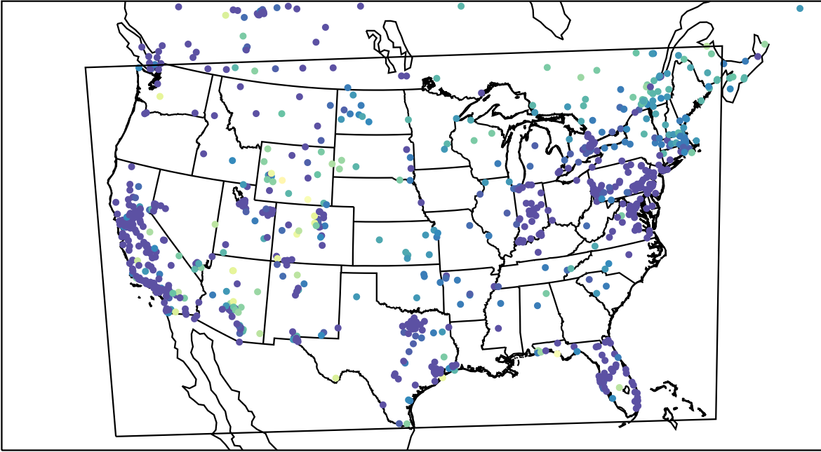
AirNOW (2024-01-01_07:00:00)
