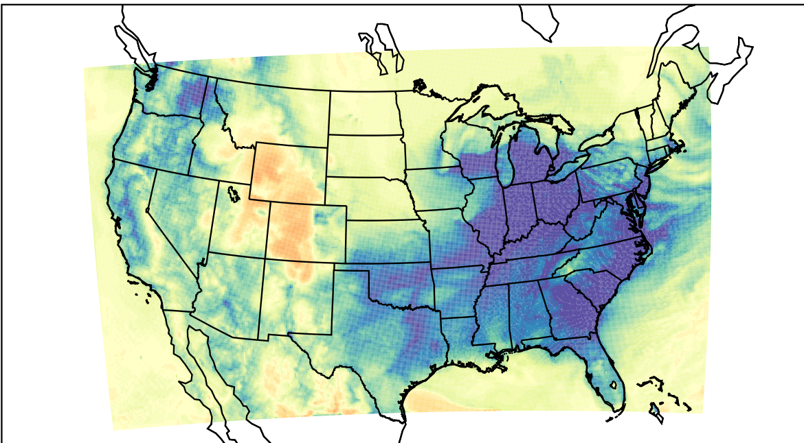
WRF (2023-12-31_10:00:00)
