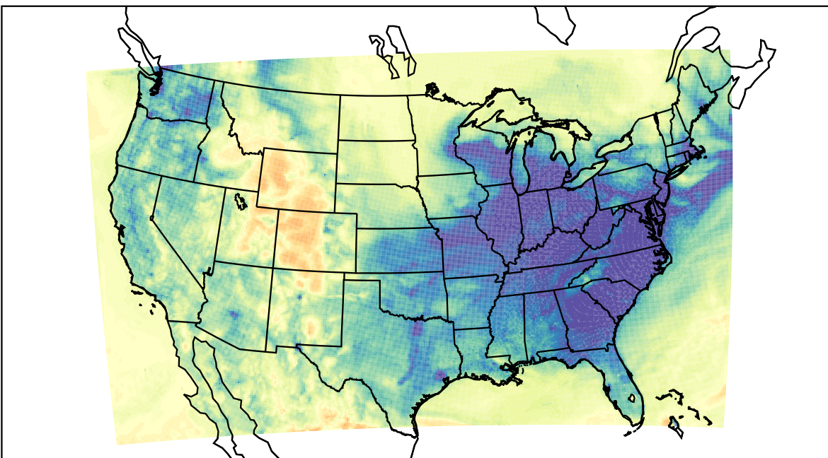
WRF (2023-12-31_04:00:00)
