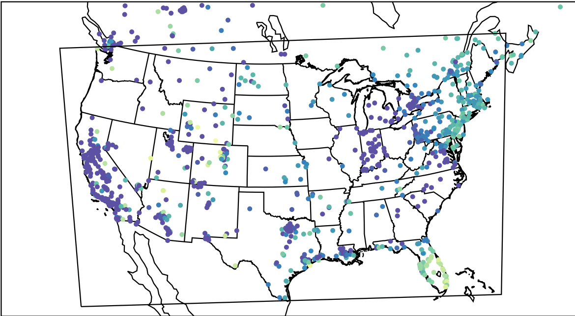
AirNOW (2023-12-31_15:00:00)
