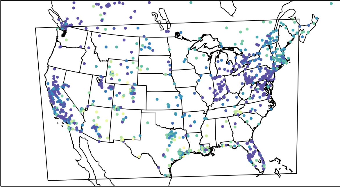
AirNOW (2024-01-01_01:00:00)
