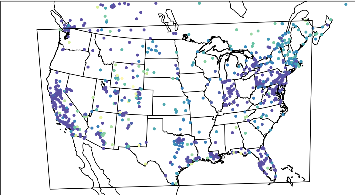
AirNOW (2024-01-01_05:00:00)
