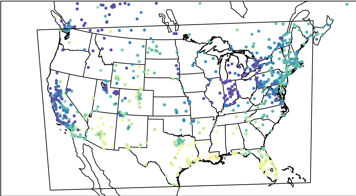
AirNOW (2023-12-31_19:00:00)
