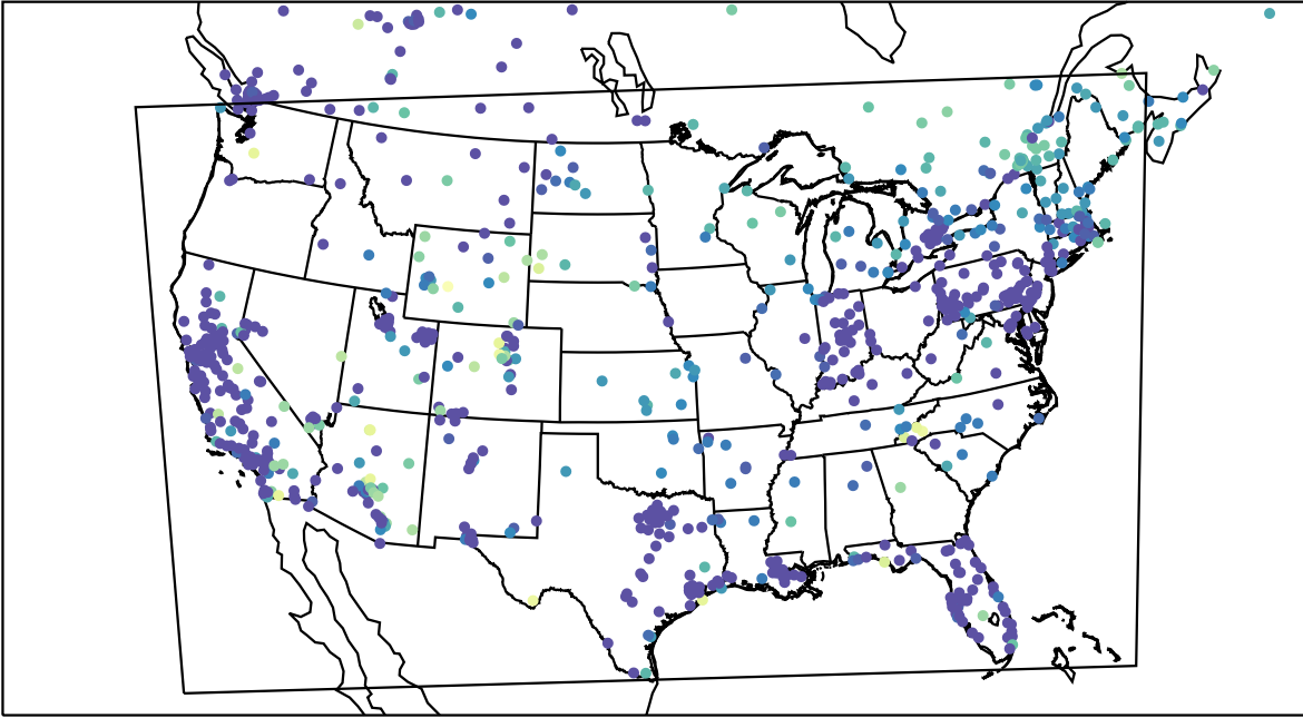
AirNOW (2024-01-01_09:00:00)
