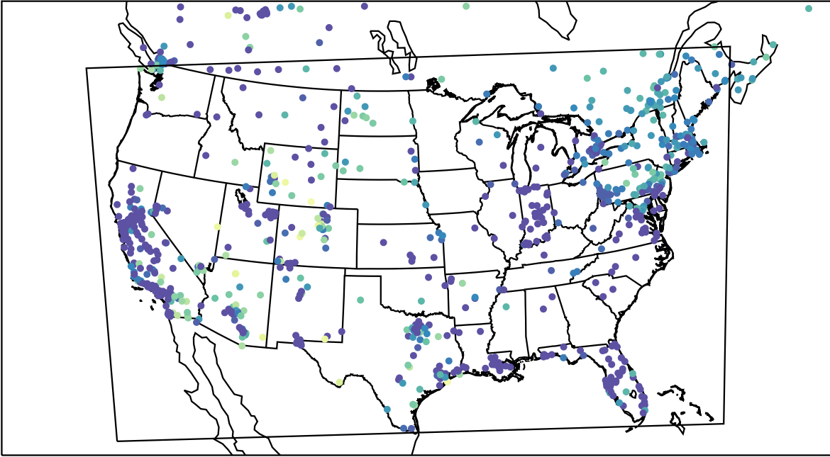
AirNOW (2023-12-31_07:00:00)
