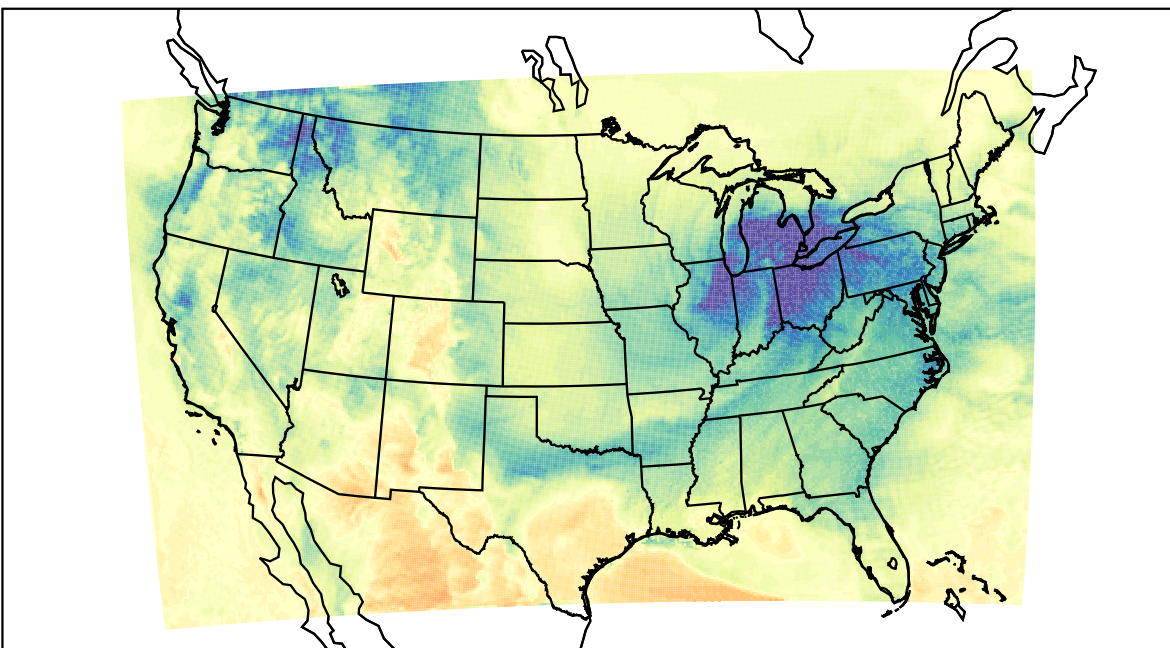
WRF (2023-12-31_21:00:00)
