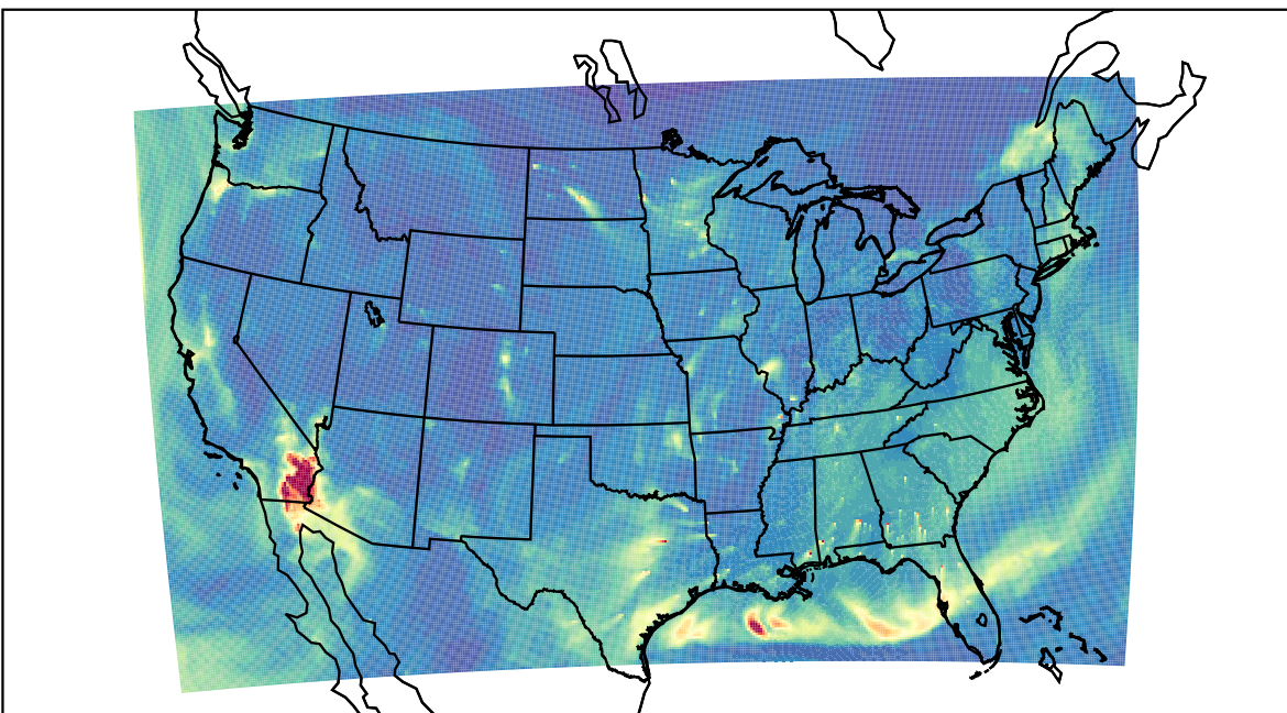
WRF 2024-01-02_11:00:00
