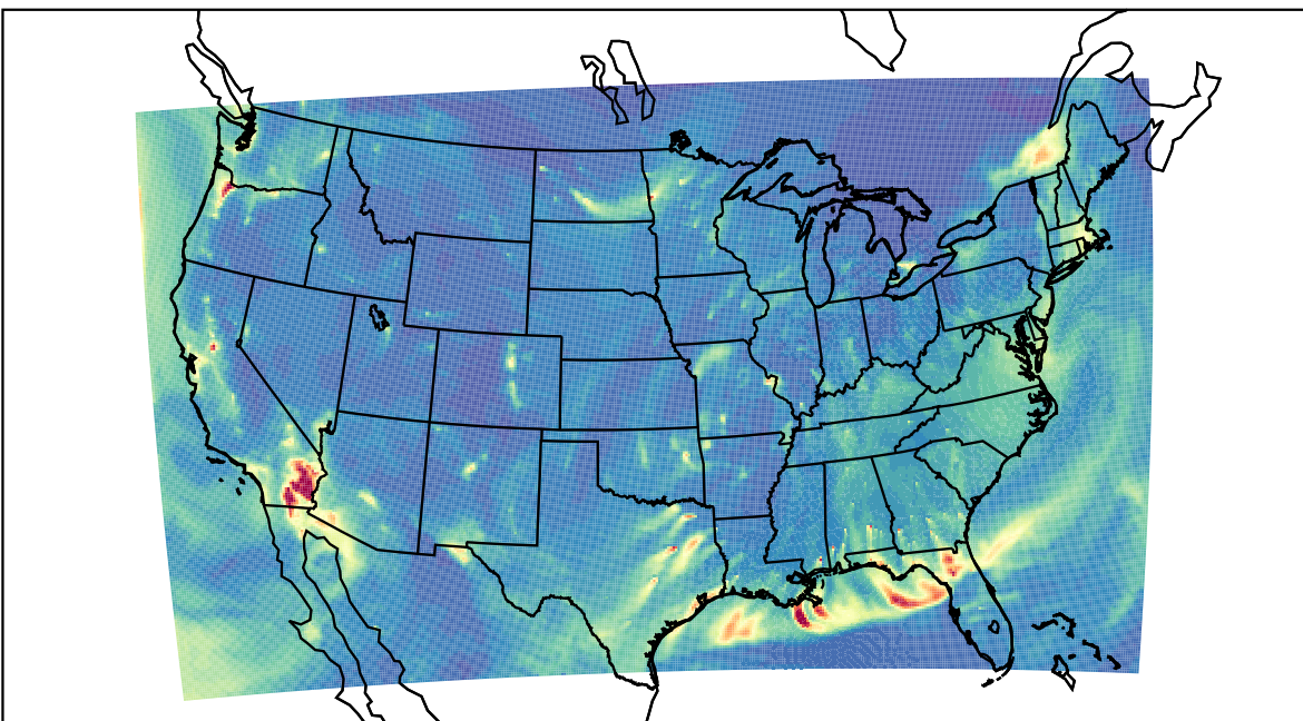
WRF 2024-01-02_06:00:00
