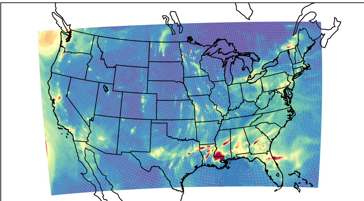
WRF 2024-01-01_05:00:00
