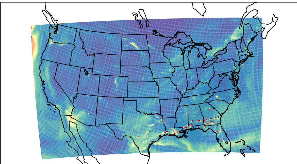
WRF 2024-01-02_21:00:00
