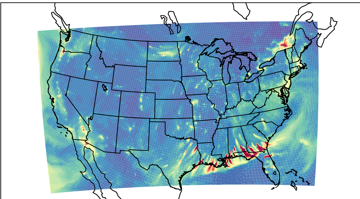
WRF 2024-01-02_02:00:00
