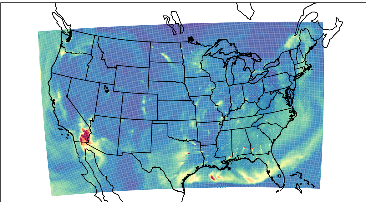
WRF 2024-01-02_12:00:00
