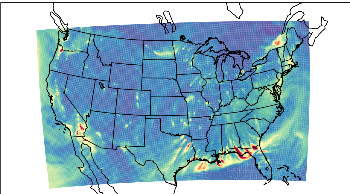
WRF 2024-01-02_04:00:00
