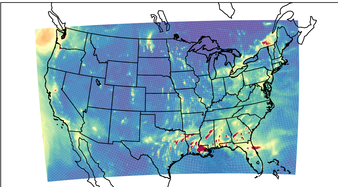
WRF 2024-01-01_02:00:00
