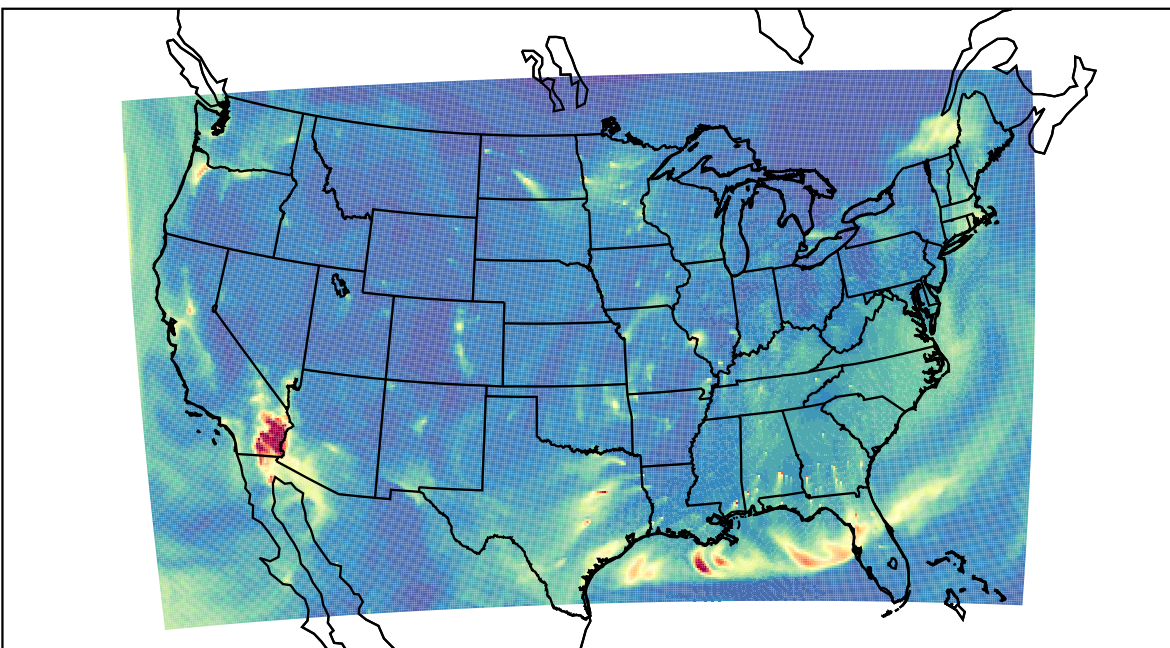
WRF 2024-01-02_09:00:00
