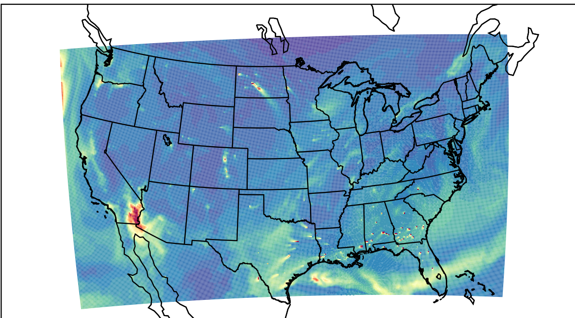
WRF 2024-01-02_17:00:00
