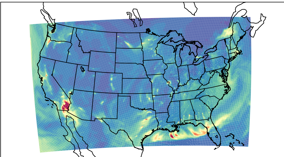
WRF 2024-01-02_08:00:00
