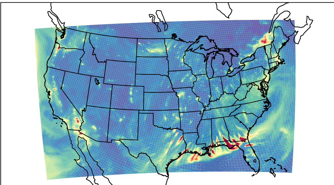
WRF 2024-01-02_03:00:00
