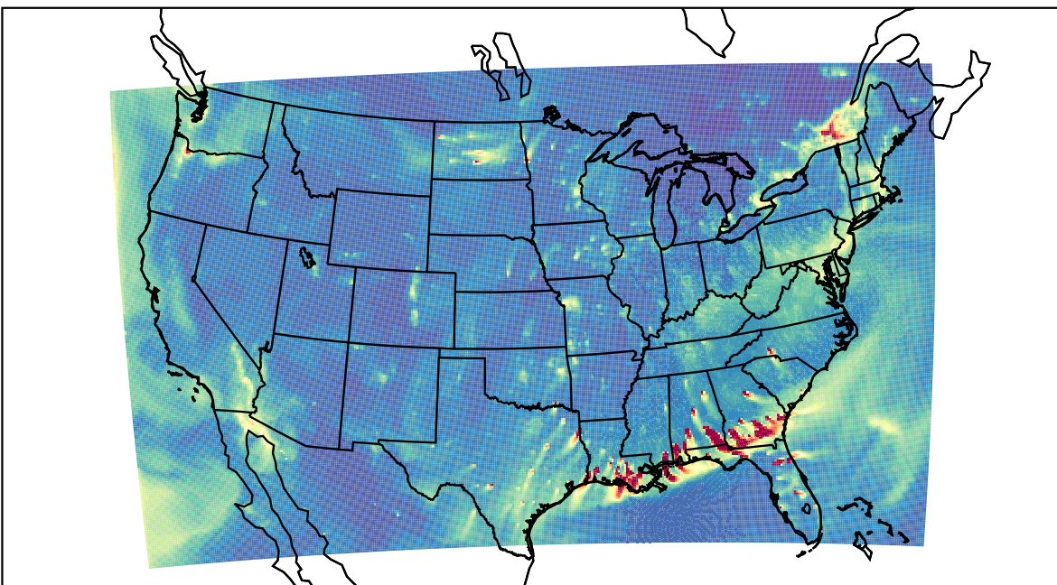
WRF 2024-01-02_00:00:00
