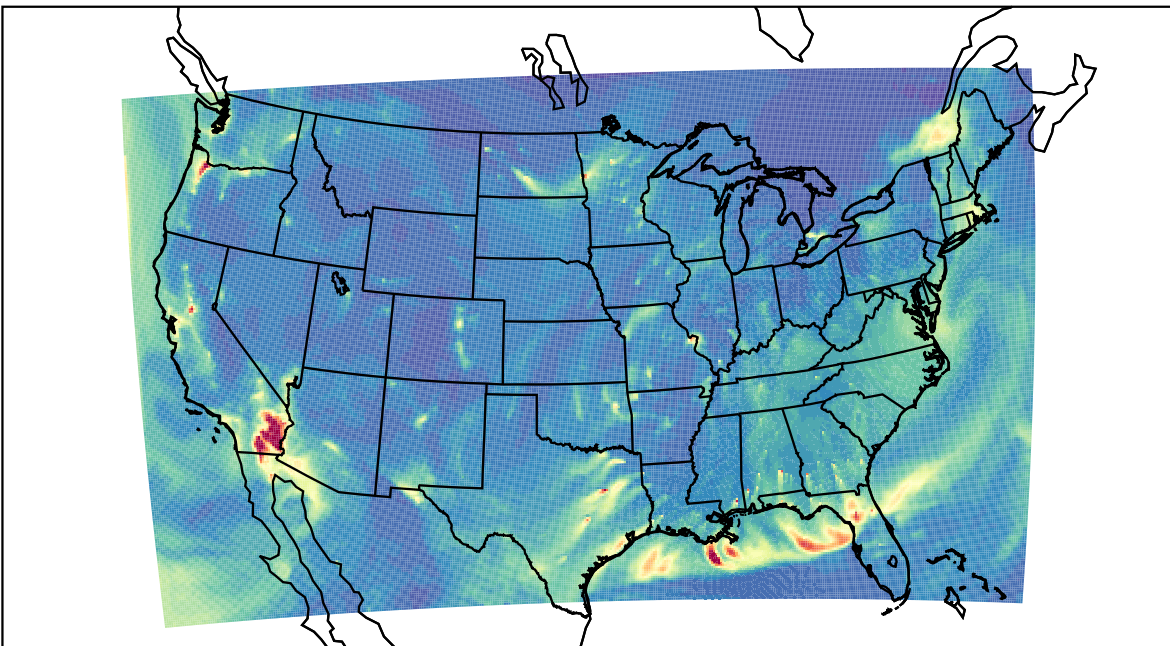
WRF 2024-01-02_07:00:00
