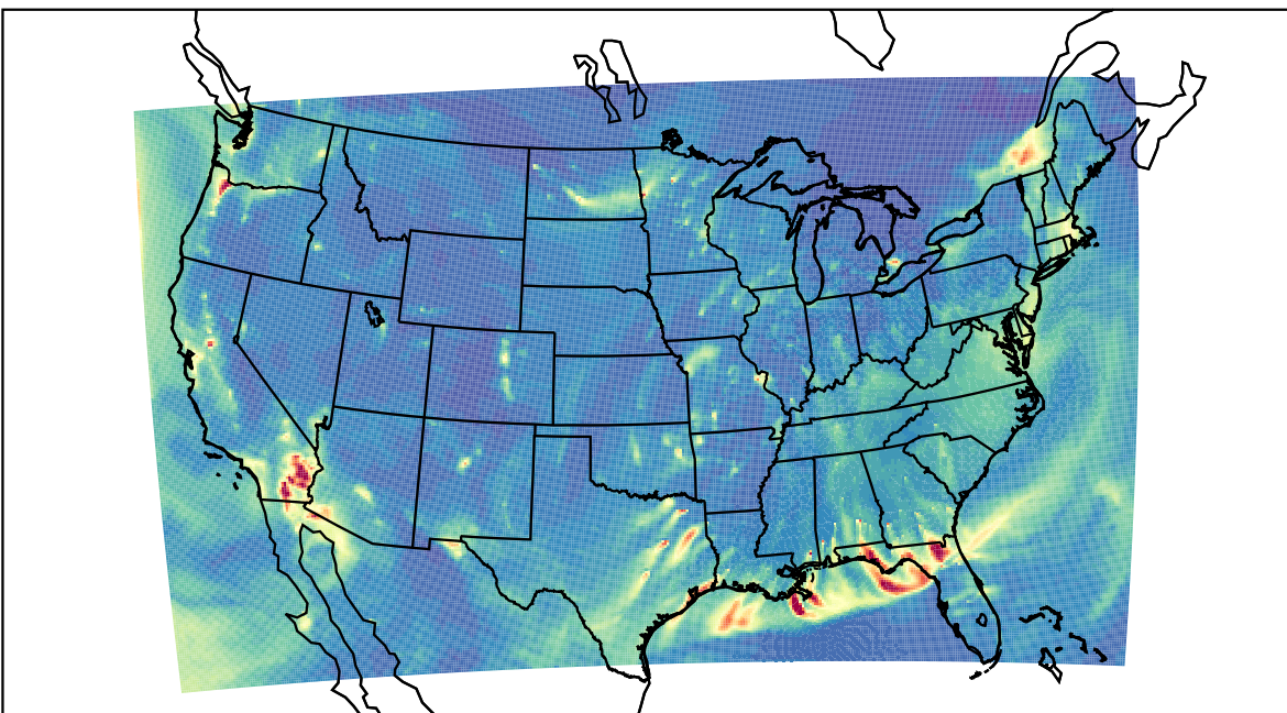
WRF 2024-01-02_05:00:00
