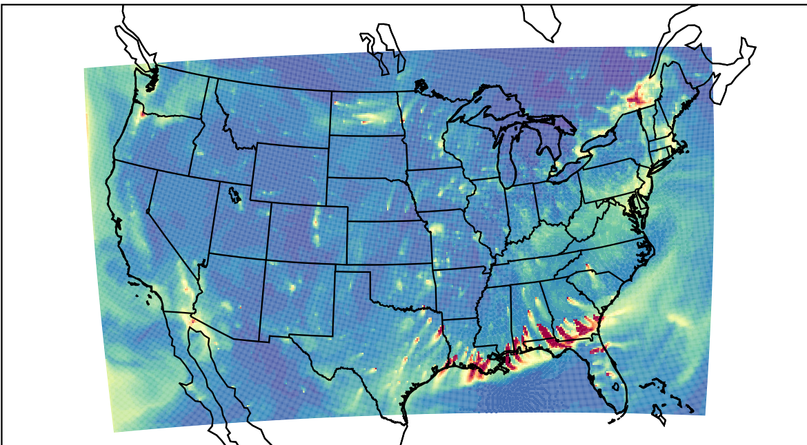
WRF 2024-01-02_01:00:00
