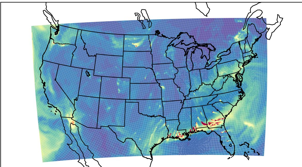
WRF 2024-01-01_21:00:00
