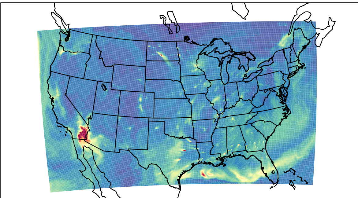
WRF 2024-01-02_14:00:00
