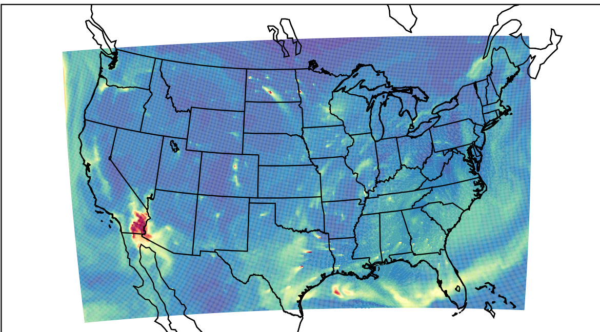
WRF 2024-01-02_15:00:00
