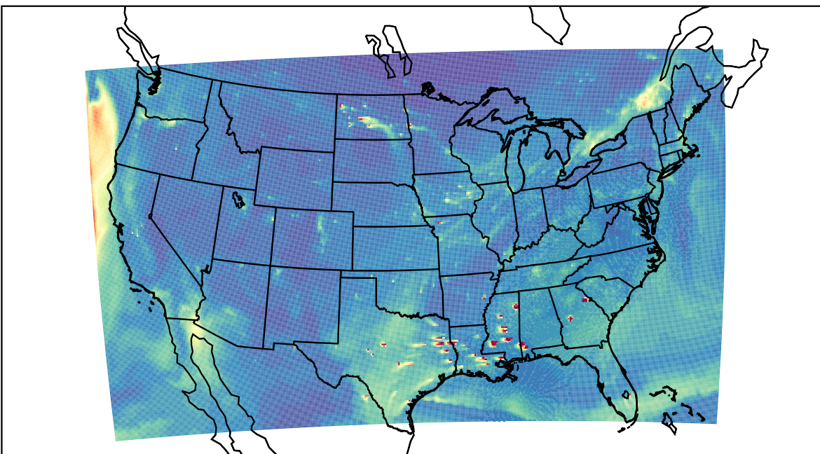
WRF 2024-01-02_22:00:00
