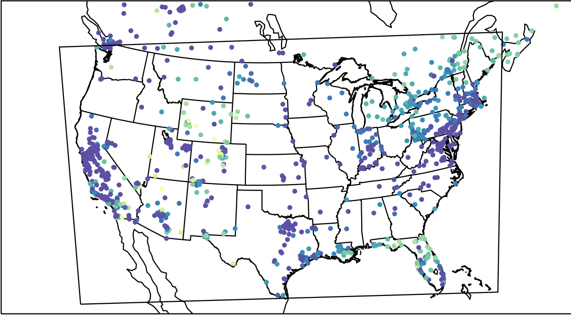
AirNOW (2024-01-02_03:00:00)
