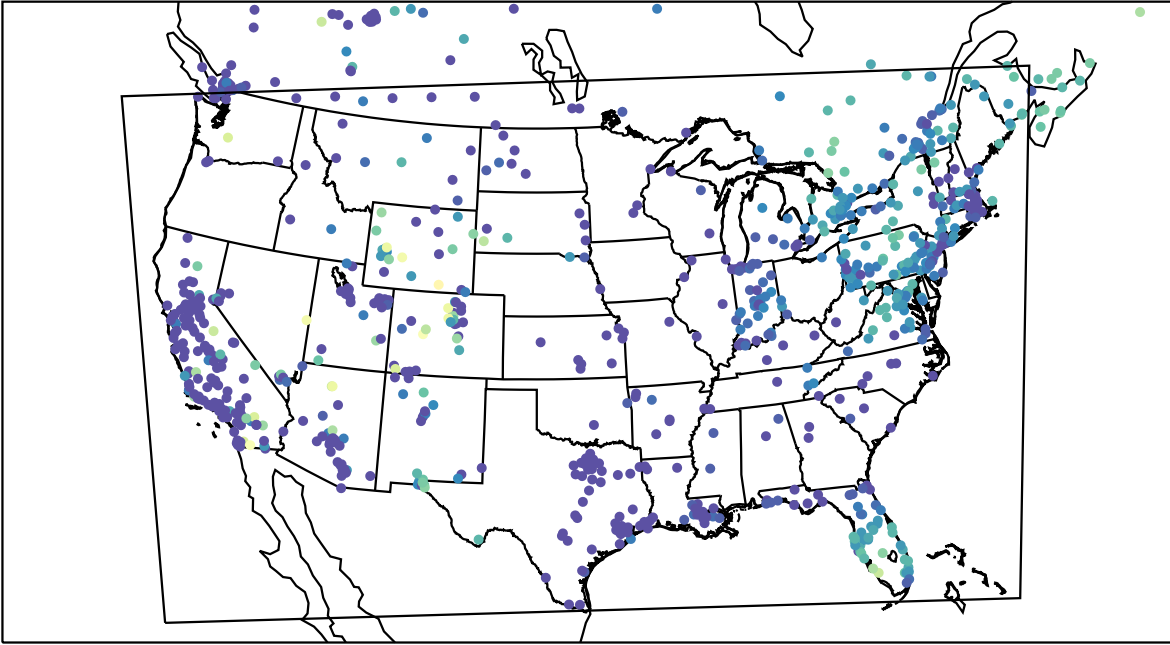
AirNOW (2024-01-02_14:00:00)
