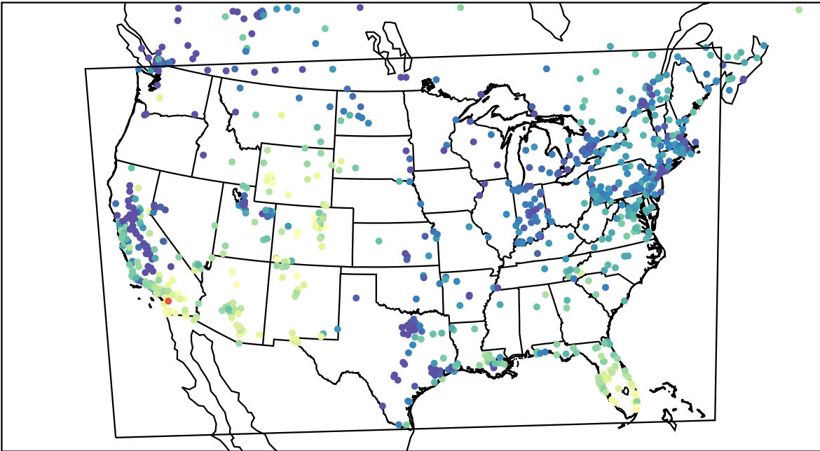
AirNOW (2024-01-02_21:00:00)
