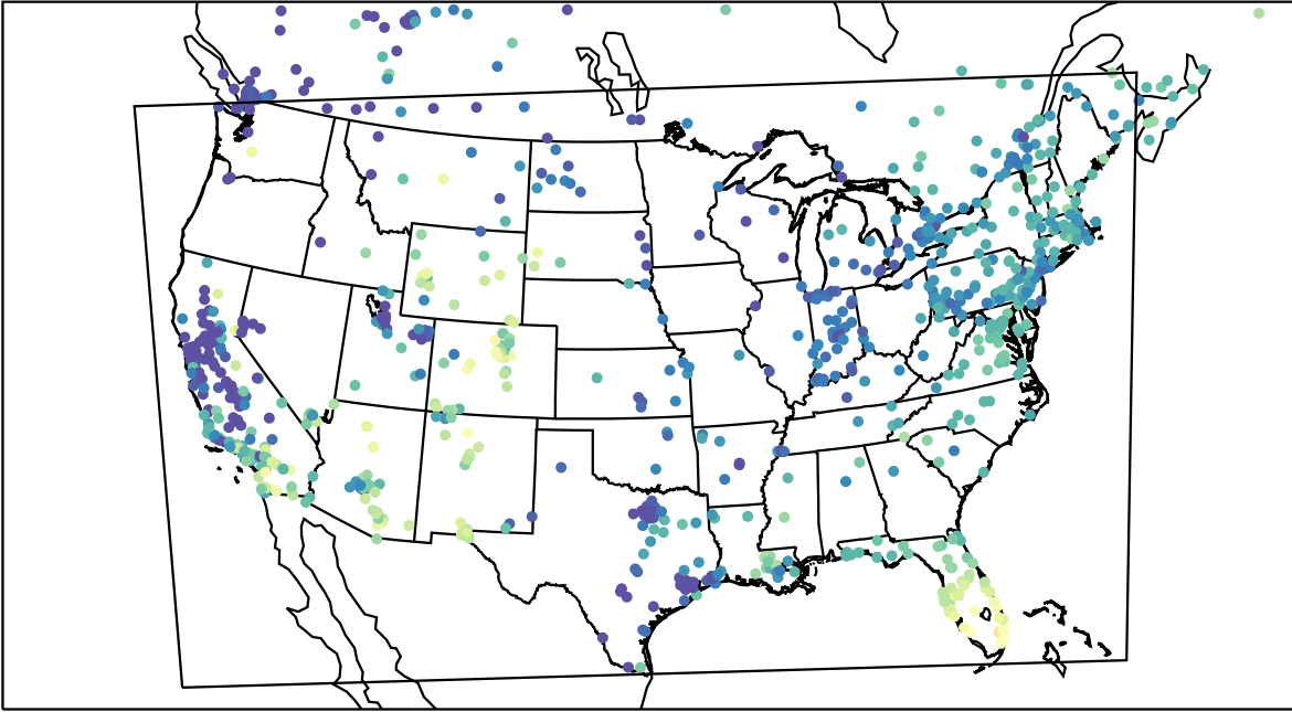
AirNOW (2024-01-02_19:00:00)
