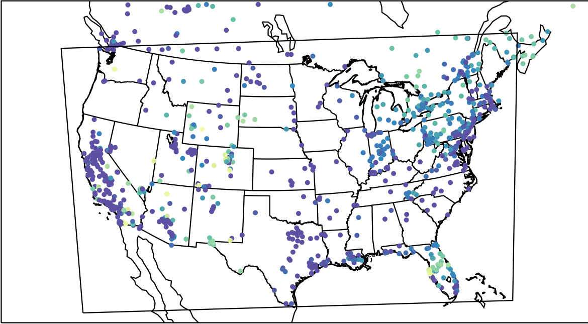
AirNOW (2024-01-02_09:00:00)
