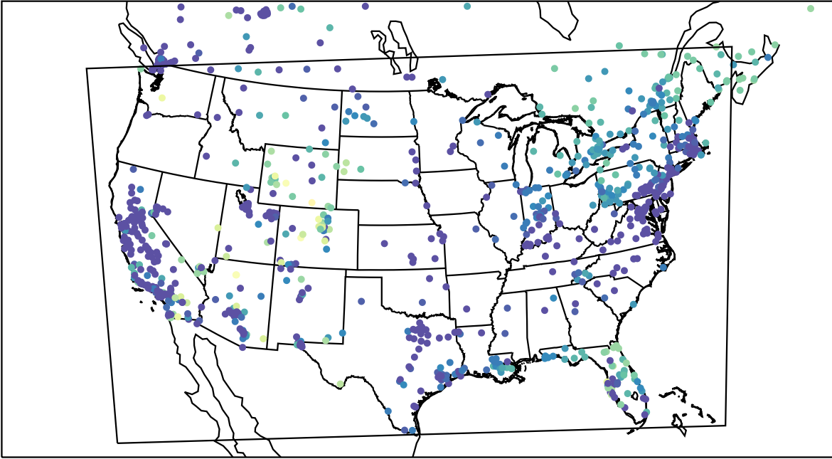
AirNOW (2024-01-02_05:00:00)
