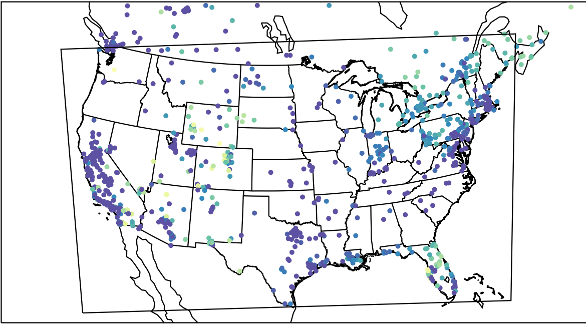
AirNOW (2024-01-02_07:00:00)
