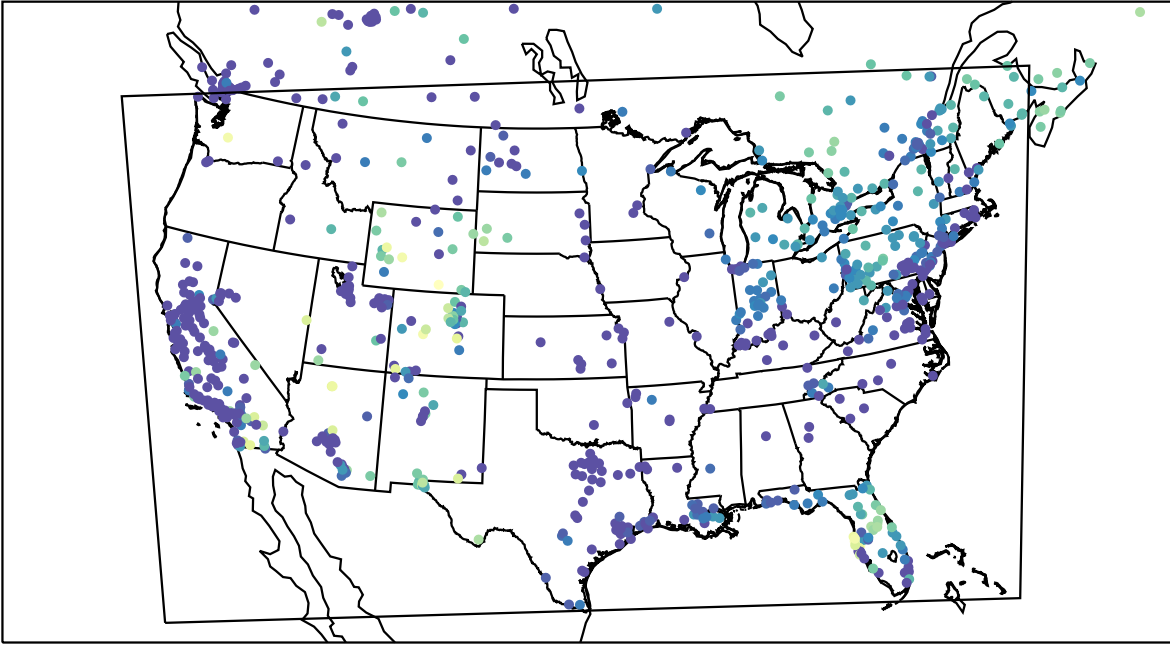
AirNOW (2024-01-02_08:00:00)
