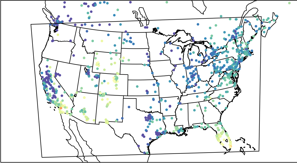
AirNOW (2024-01-02_20:00:00)
