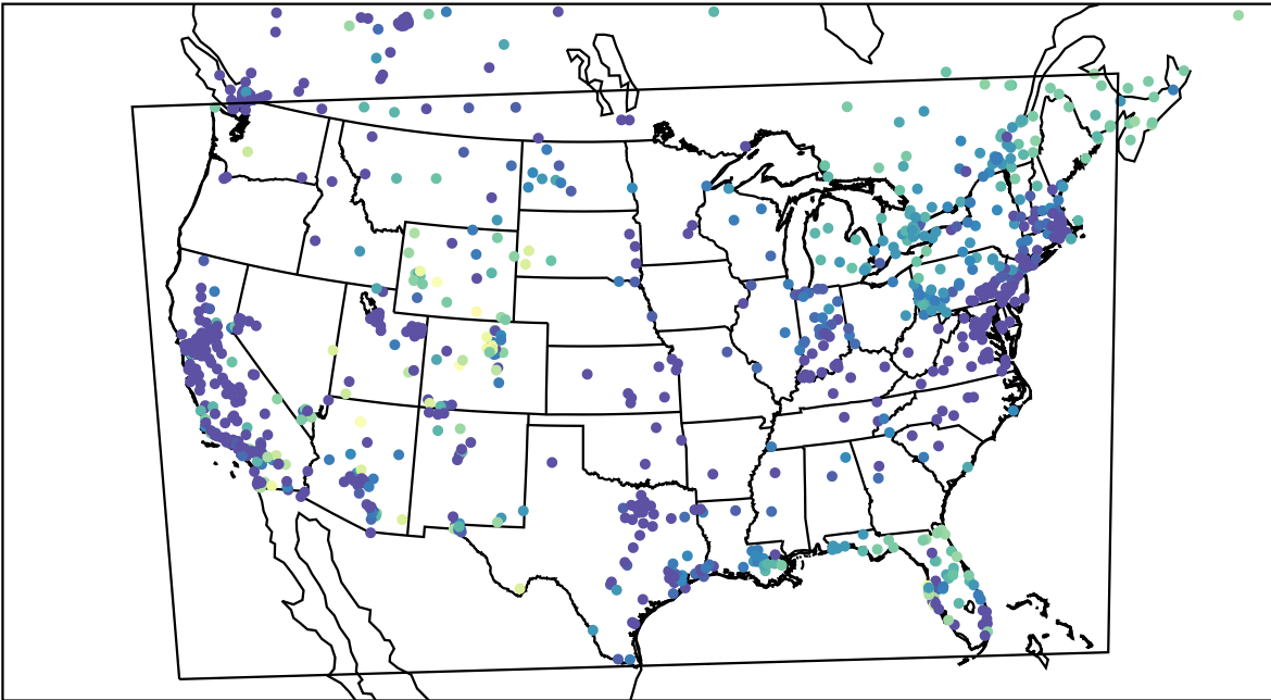
AirNOW (2024-01-02_04:00:00)
