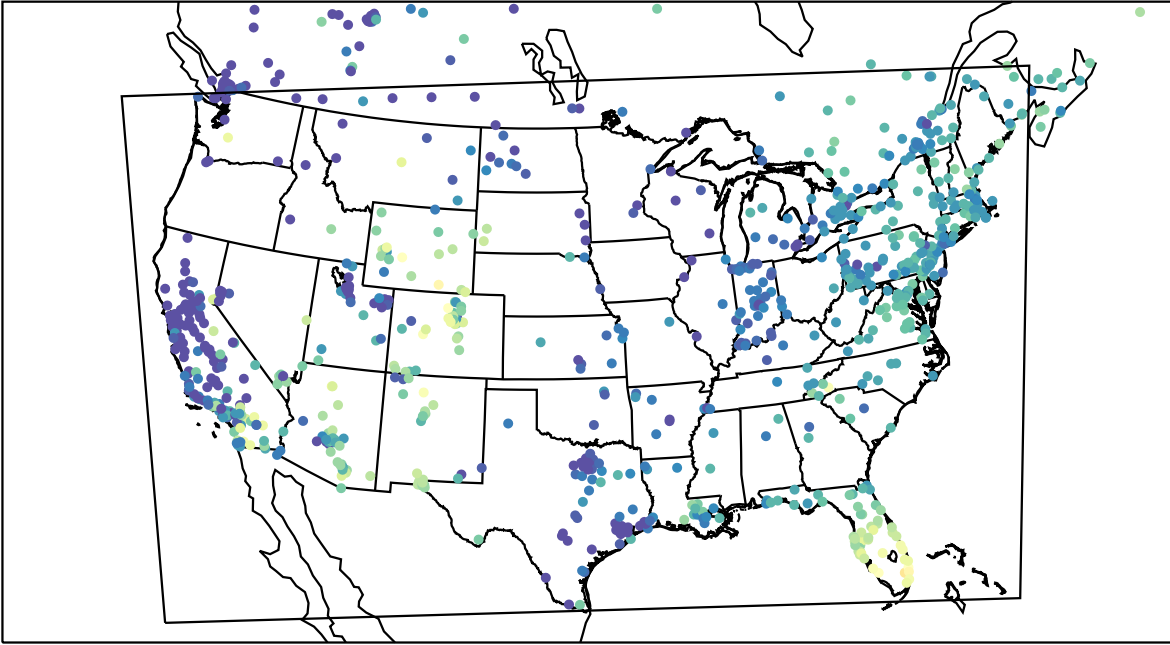
AirNOW (2024-01-02_18:00:00)
