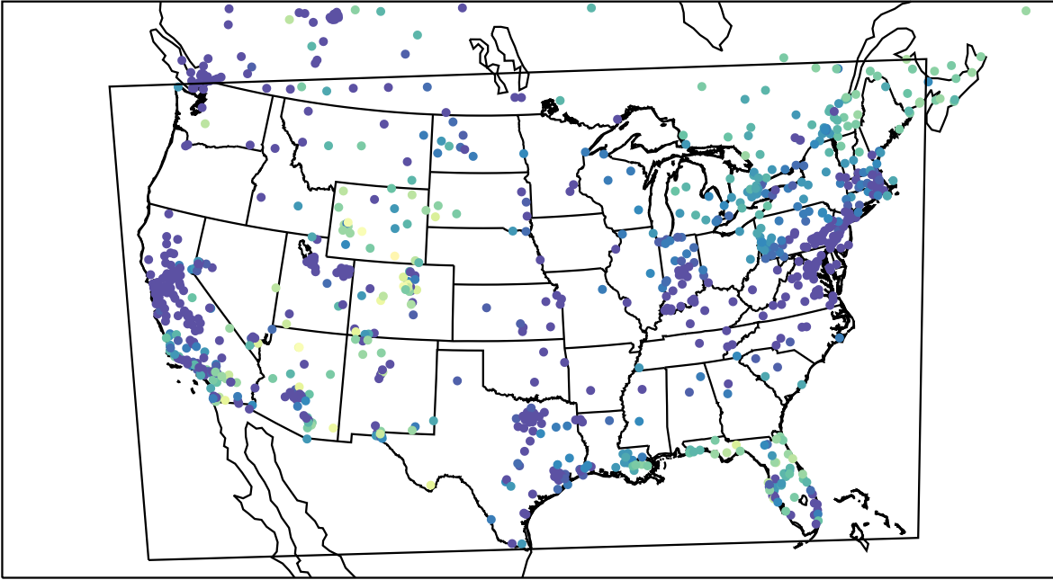
AirNOW (2024-01-02_02:00:00)
