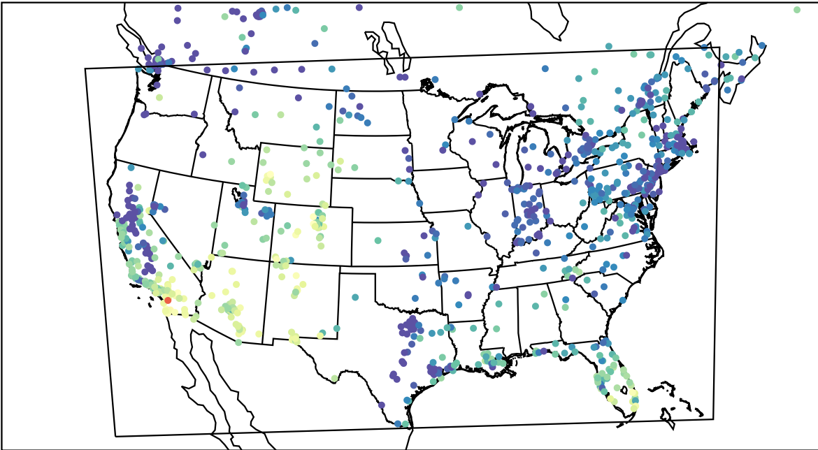
AirNOW (2024-01-02_22:00:00)
