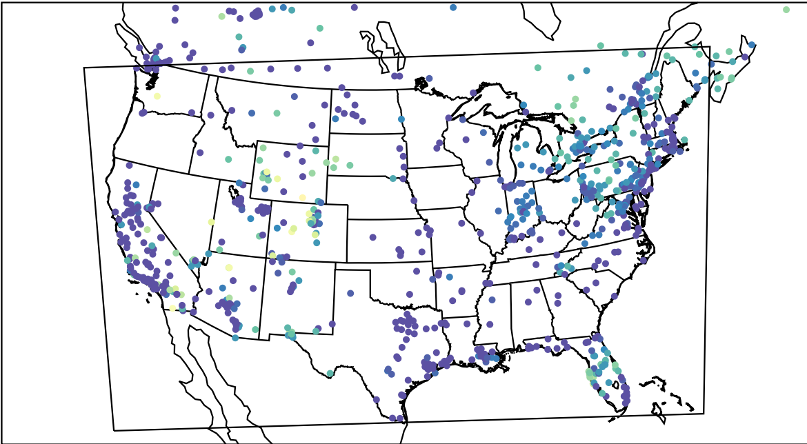
AirNOW (2024-01-02_11:00:00)
