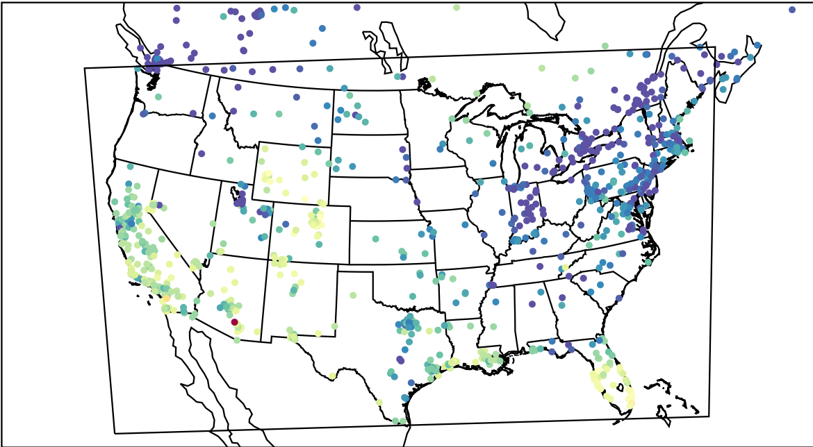
AirNOW (2024-01-03_21:00:00)
