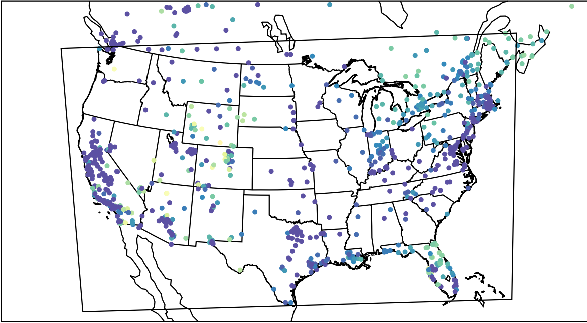
AirNOW (2024-01-02_06:00:00)
