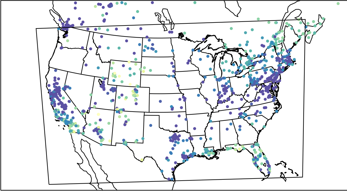
AirNOW (2024-01-02_01:00:00)
