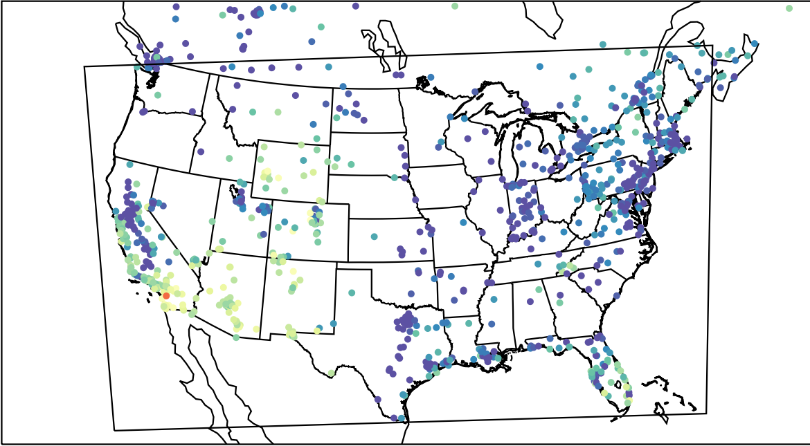
AirNOW (2024-01-02_23:00:00)
