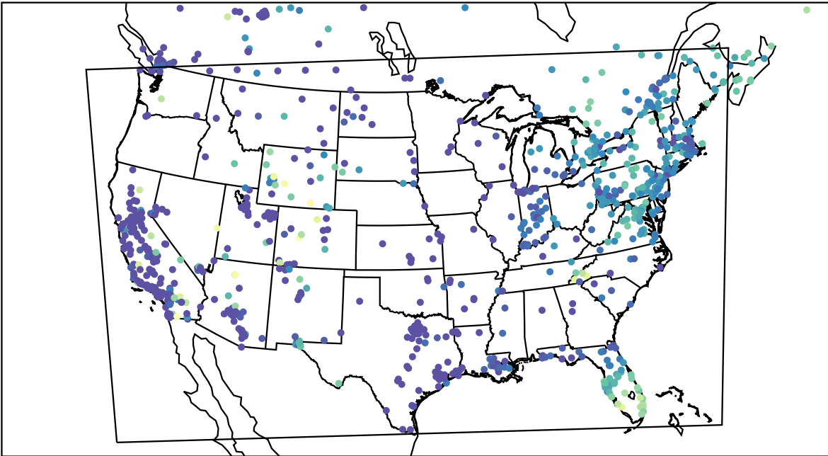
AirNOW (2024-01-02_15:00:00)
