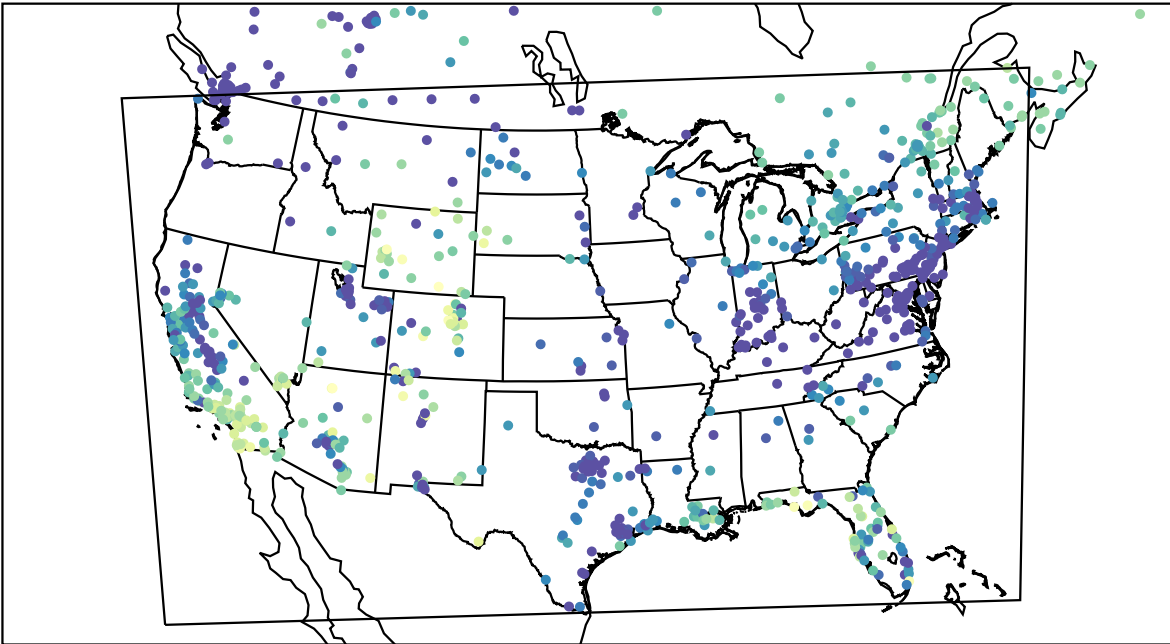
AirNOW (2024-01-02_00:00:00)
