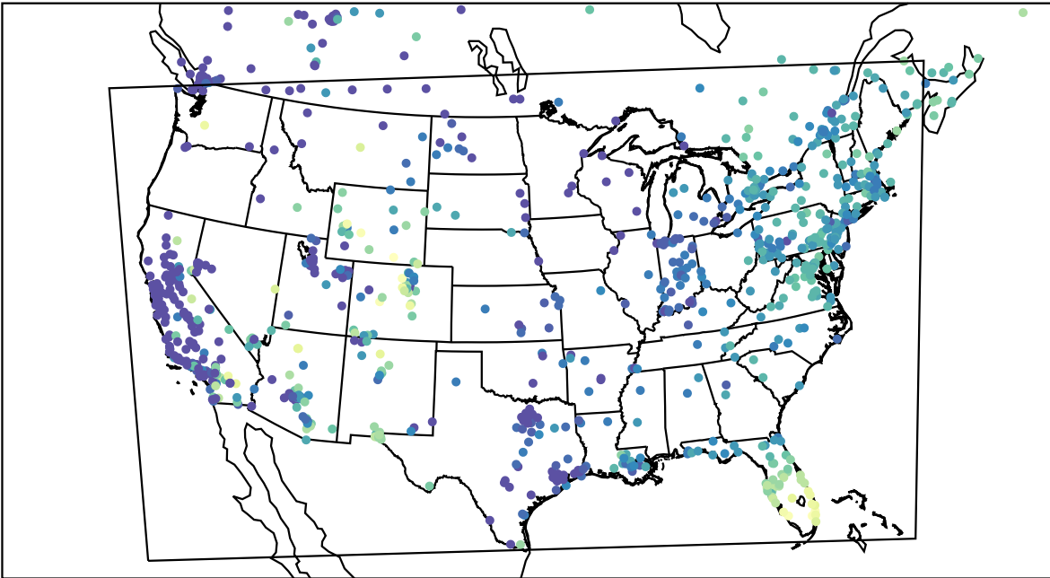
AirNOW (2024-01-02_17:00:00)
