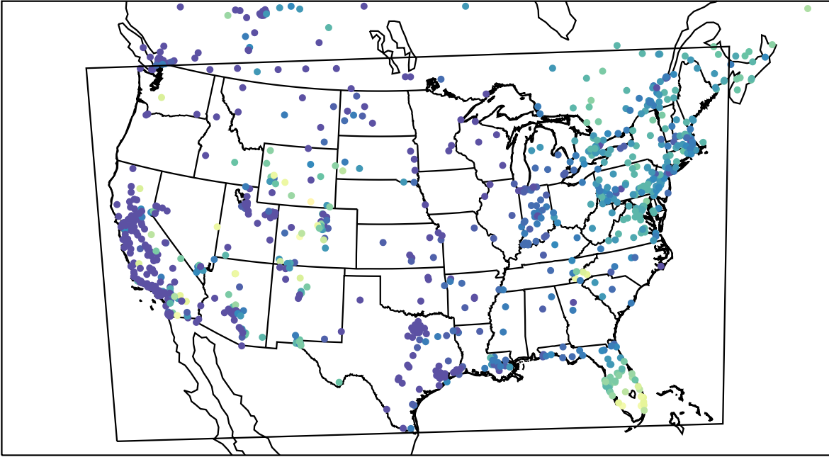
AirNOW (2024-01-02_16:00:00)
