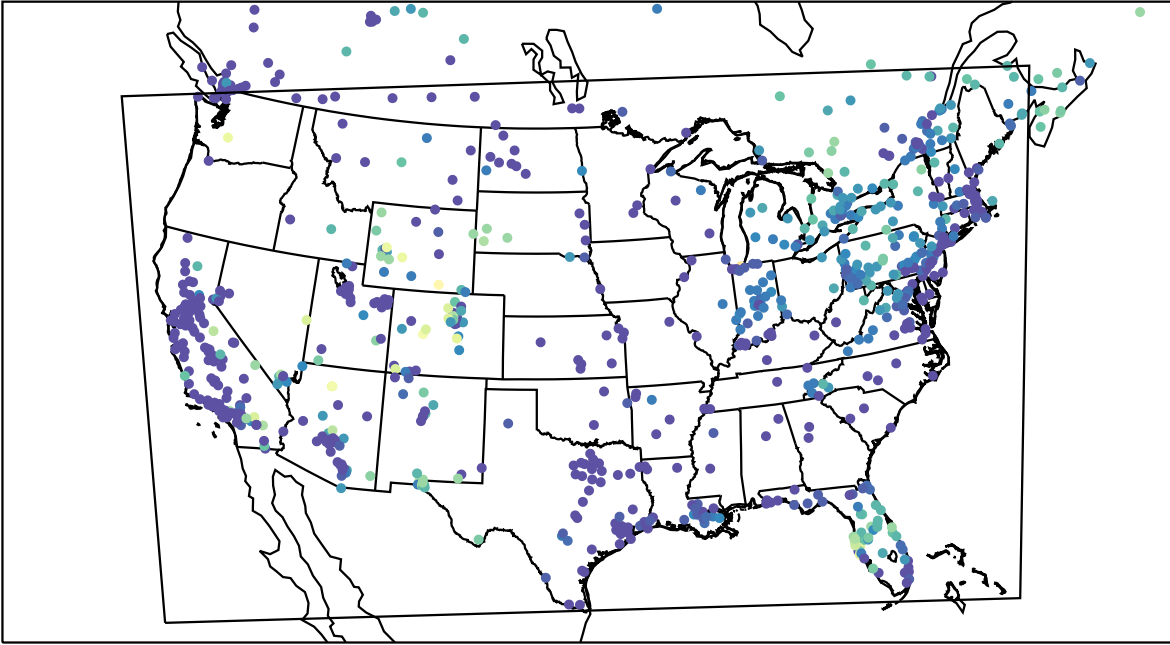
AirNOW (2024-01-02_10:00:00)
