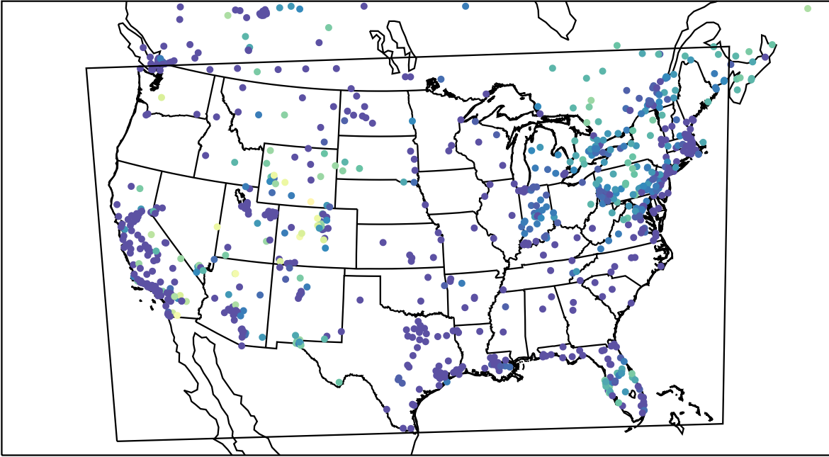
AirNOW (2024-01-02_12:00:00)
