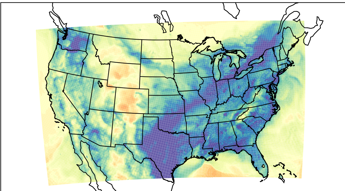
WRF (2024-01-03_13:00:00)
