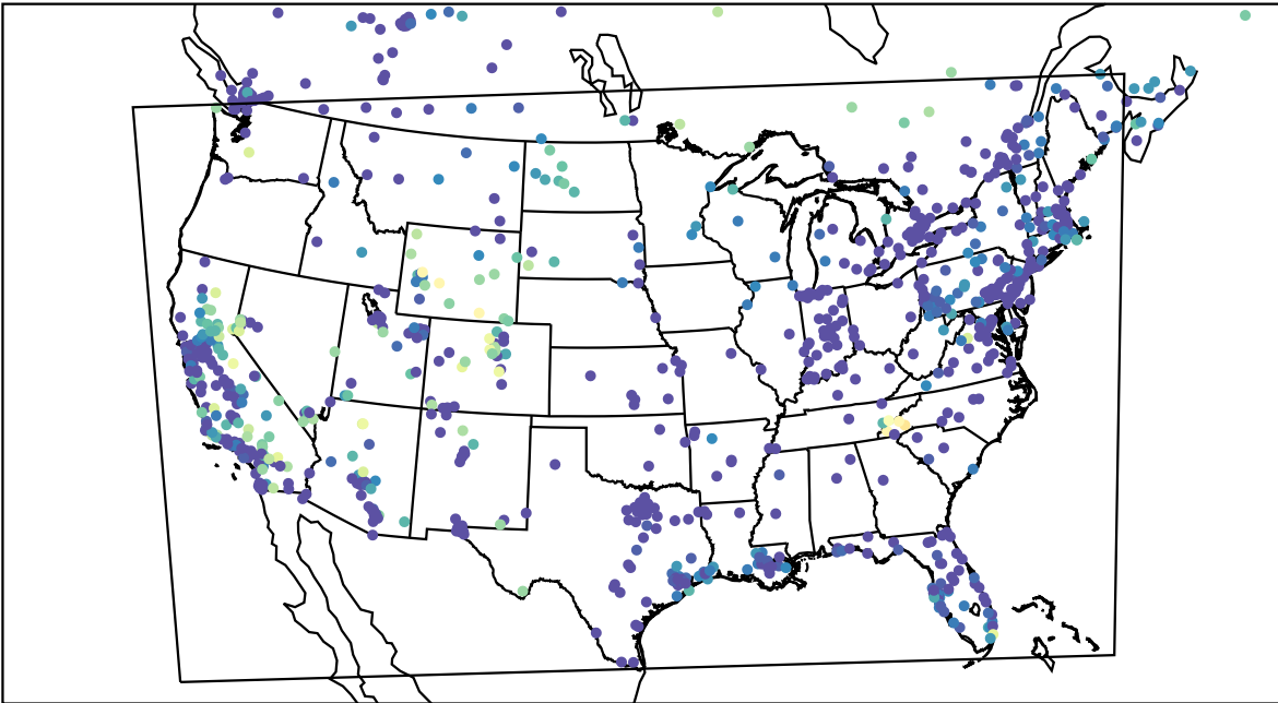
AirNOW (2024-01-03_14:00:00)
