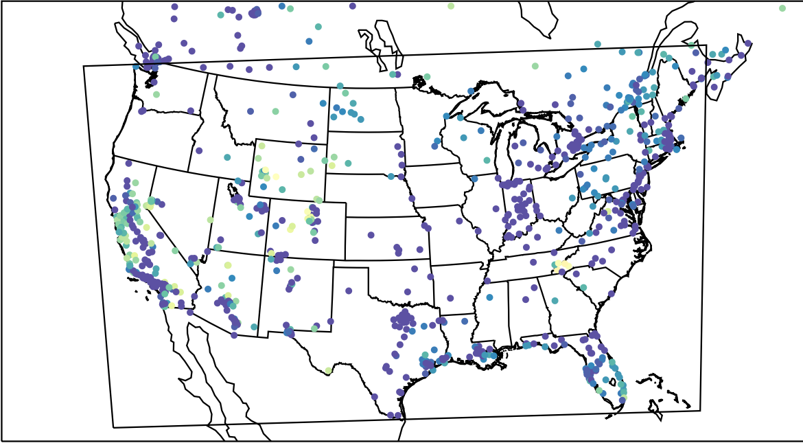
AirNOW (2024-01-03_06:00:00)
