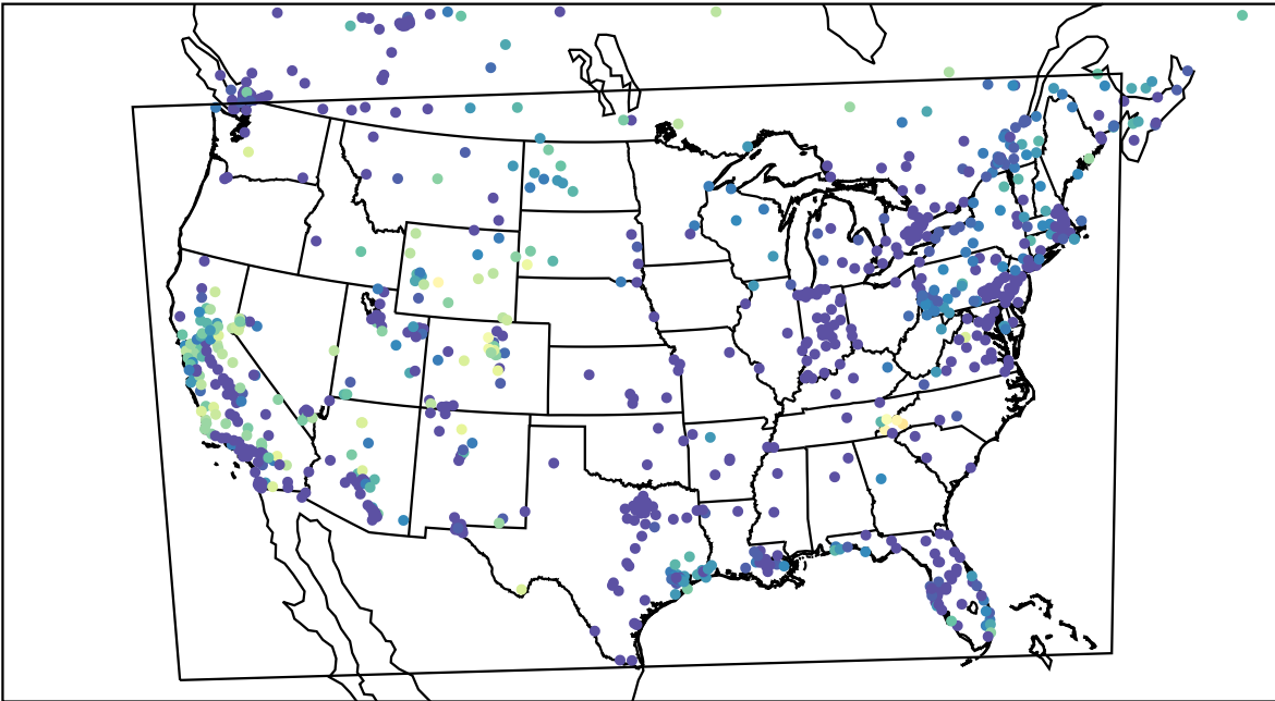
AirNOW (2024-01-03_09:00:00)
