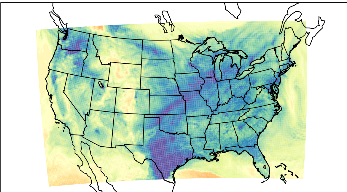
WRF (2024-01-03_00:00:00)
