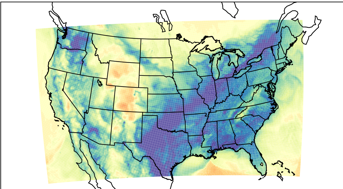
WRF (2024-01-03_15:00:00)
