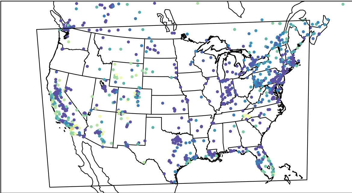
AirNOW (2024-01-03_01:00:00)
