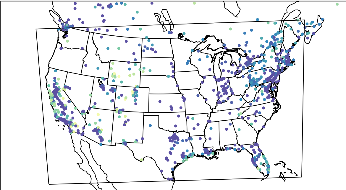
AirNOW (2024-01-03_03:00:00)
