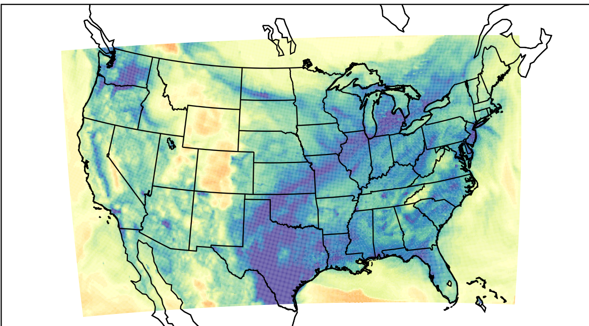
WRF (2024-01-03_06:00:00)
