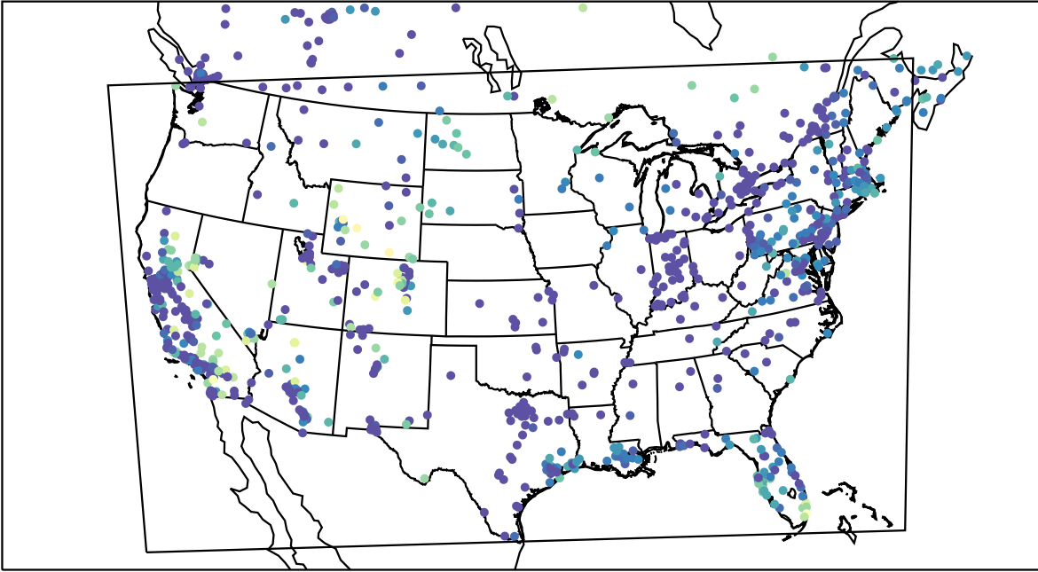
AirNOW (2024-01-03_15:00:00)
