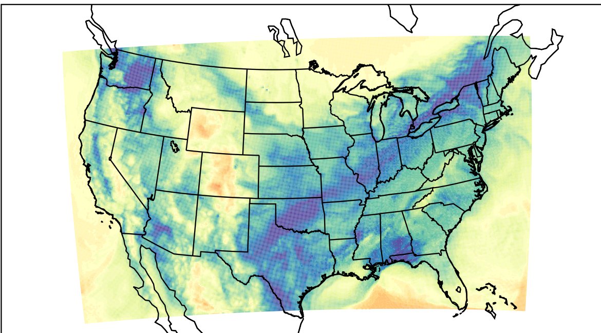
WRF (2024-01-03_17:00:00)
