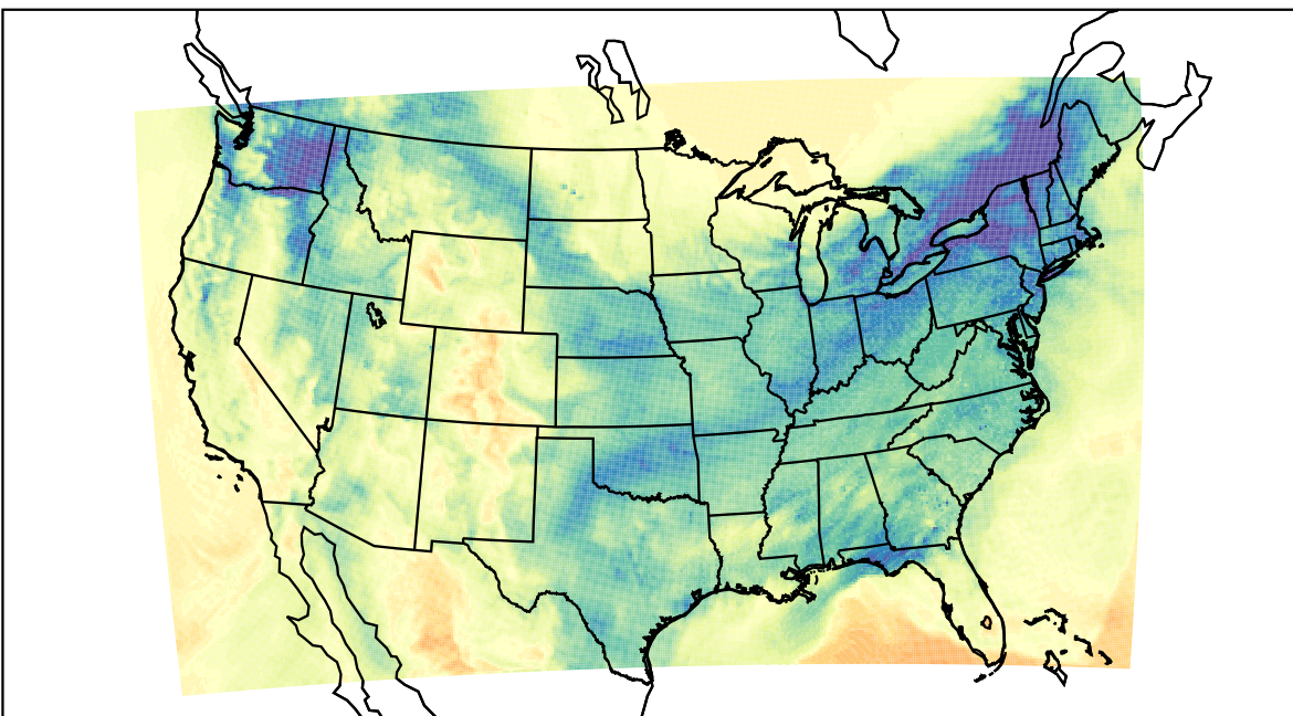
WRF (2024-01-03_21:00:00)
