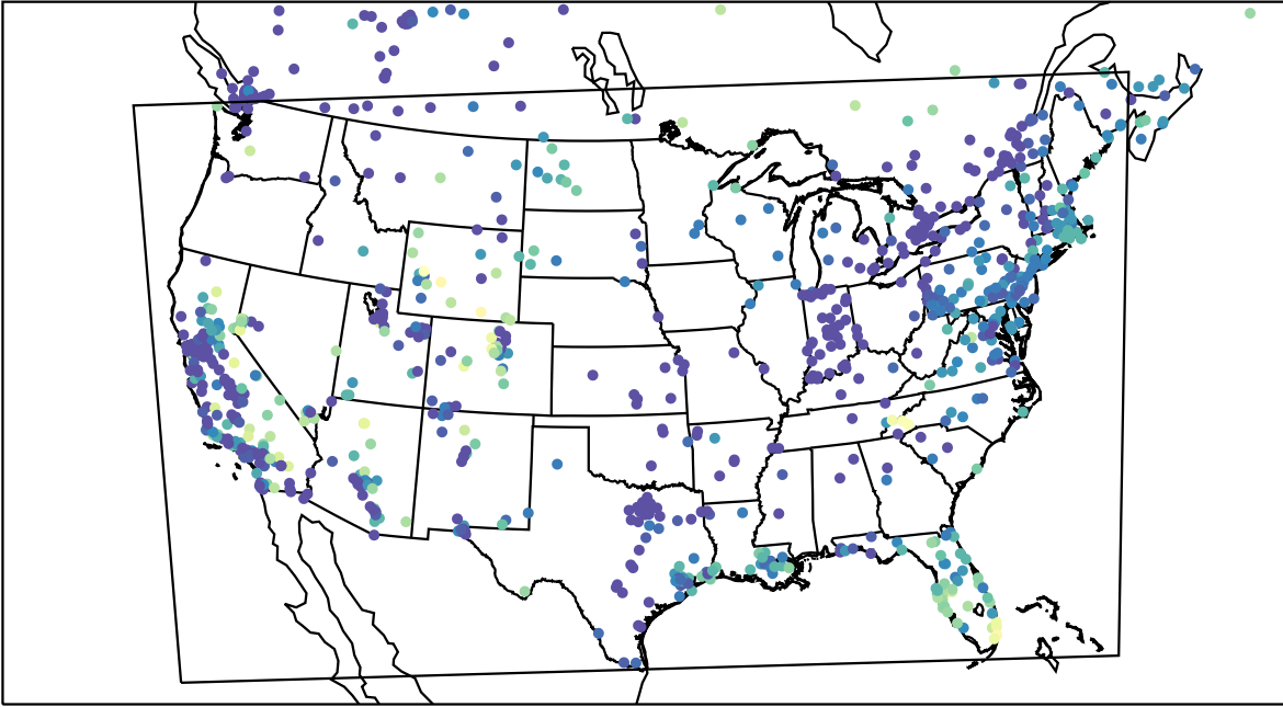
AirNOW (2024-01-03_16:00:00)
