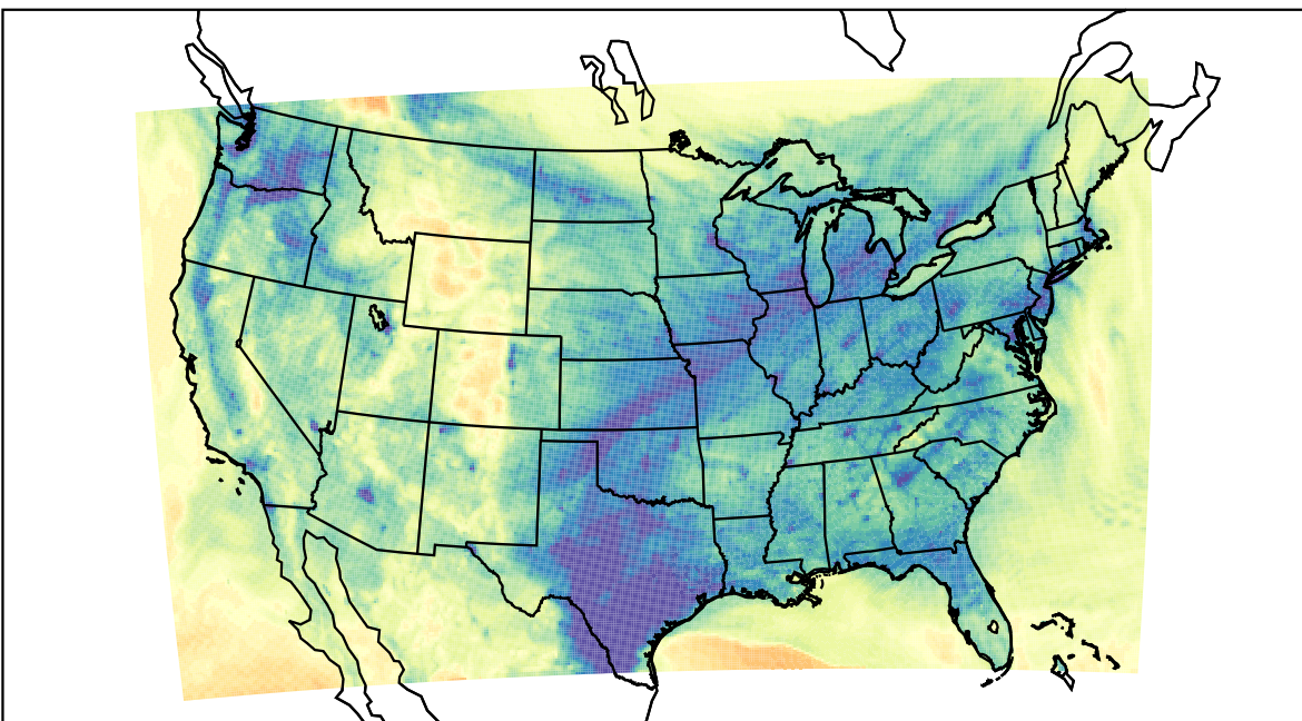
WRF (2024-01-03_01:00:00)
