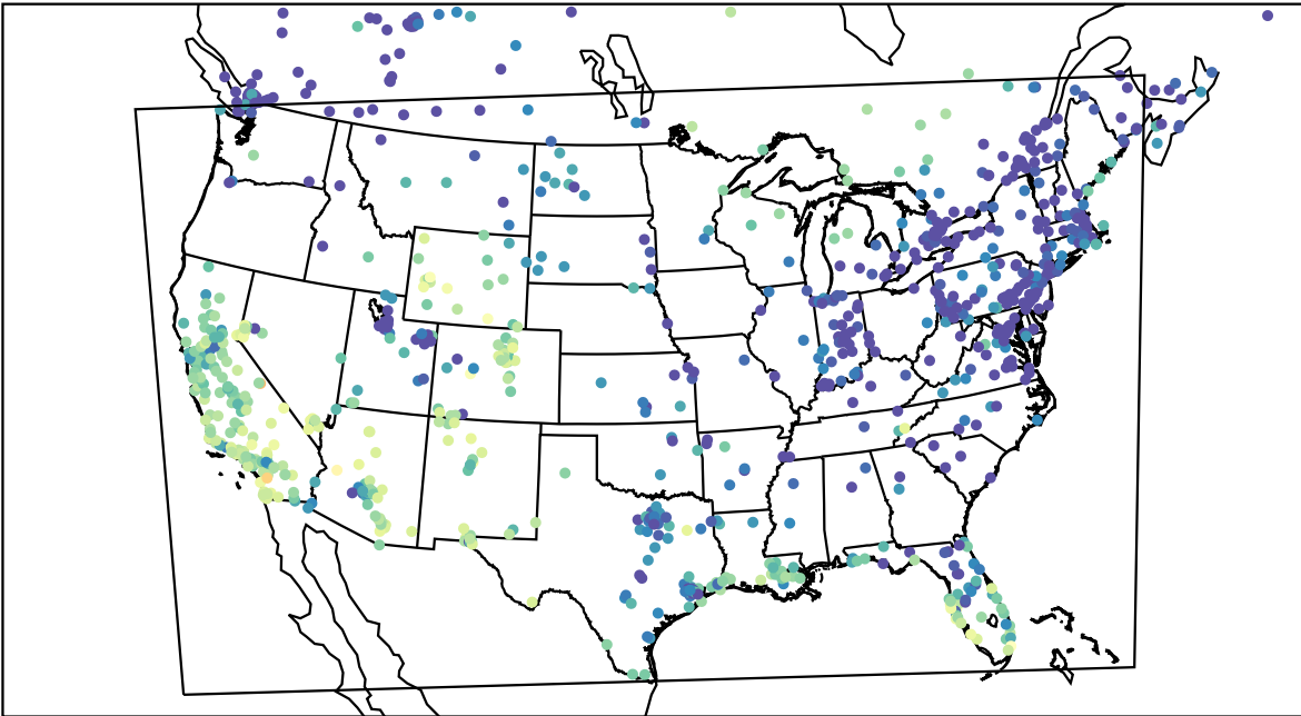
AirNOW (2024-01-03_23:00:00)
