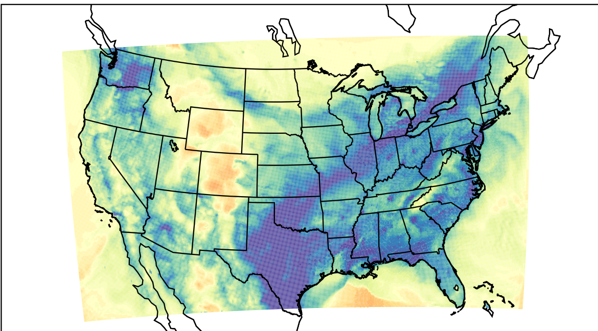
WRF (2024-01-03_12:00:00)
