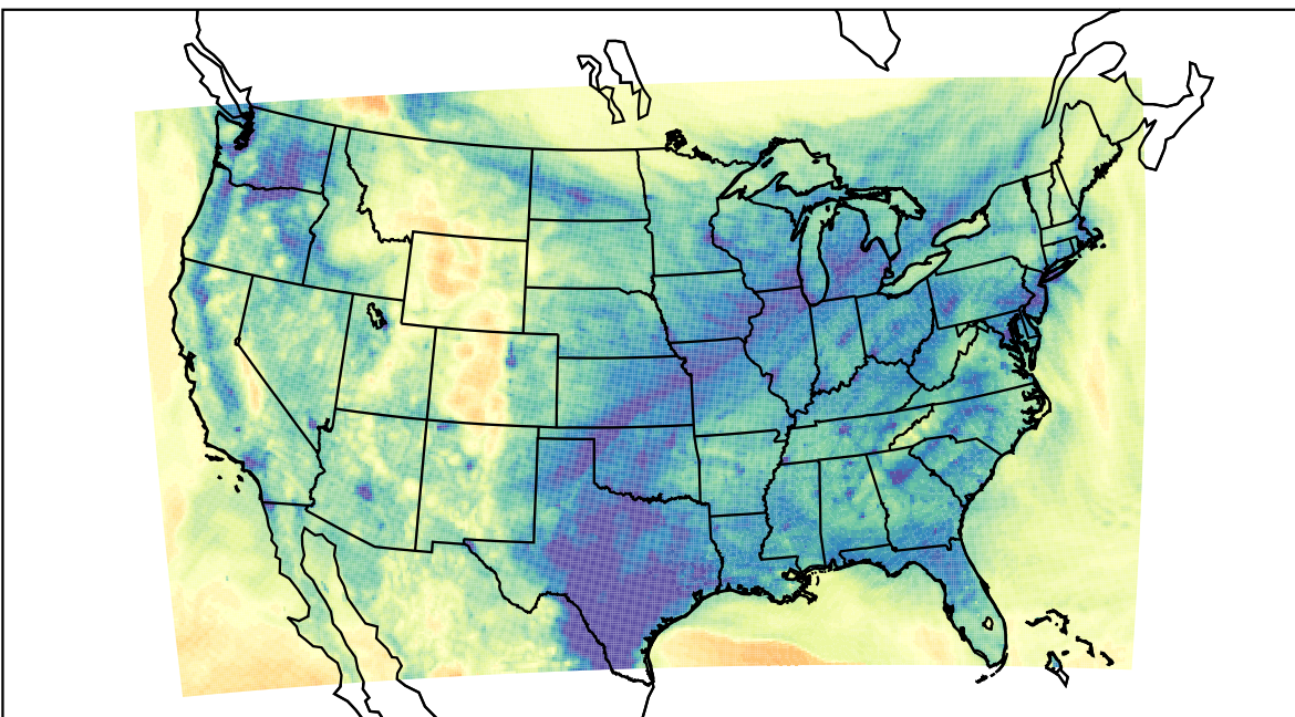
WRF (2024-01-03_02:00:00)
