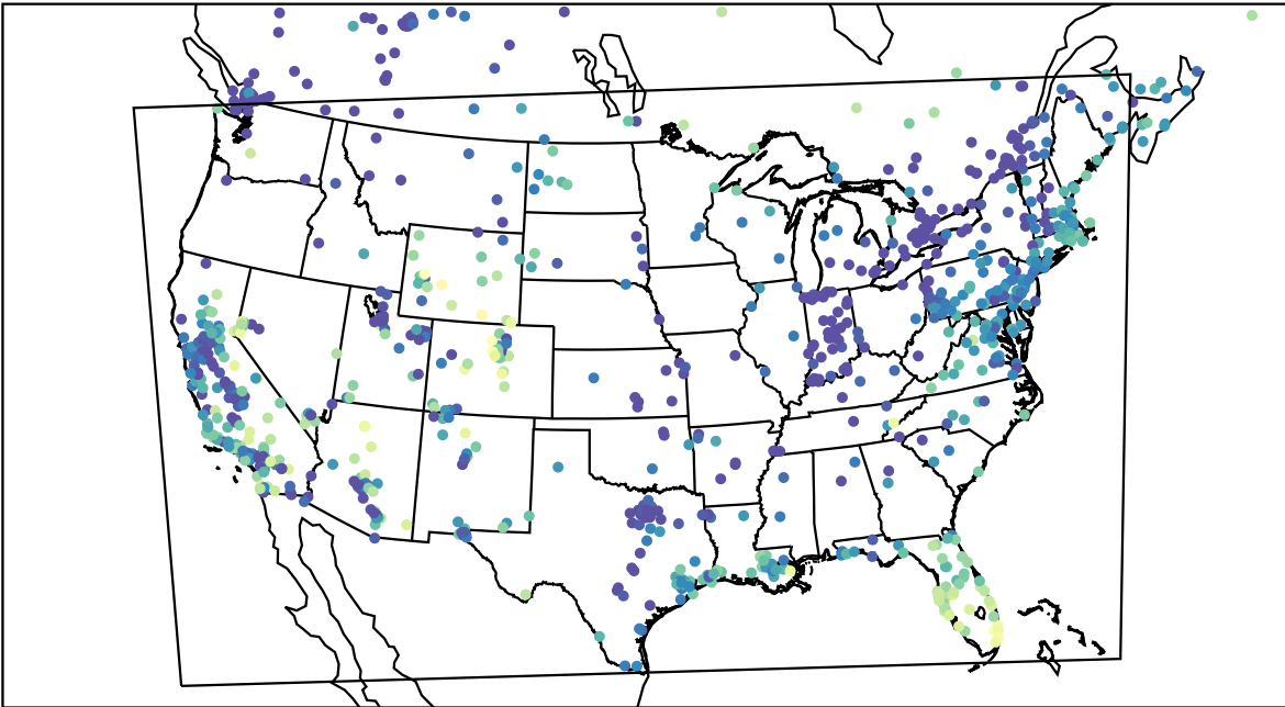
AirNOW (2024-01-03_17:00:00)
