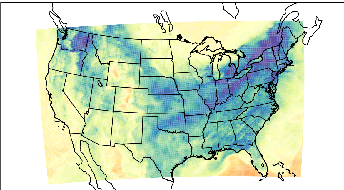
WRF (2024-01-03_23:00:00)
