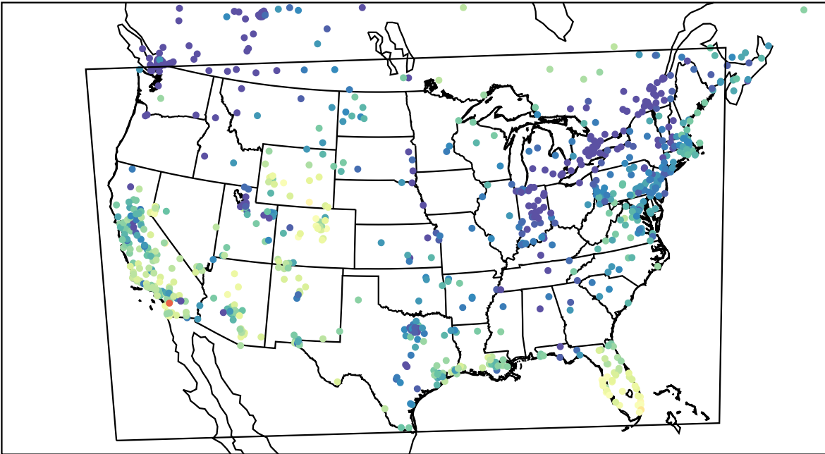
AirNOW (2024-01-03_19:00:00)
