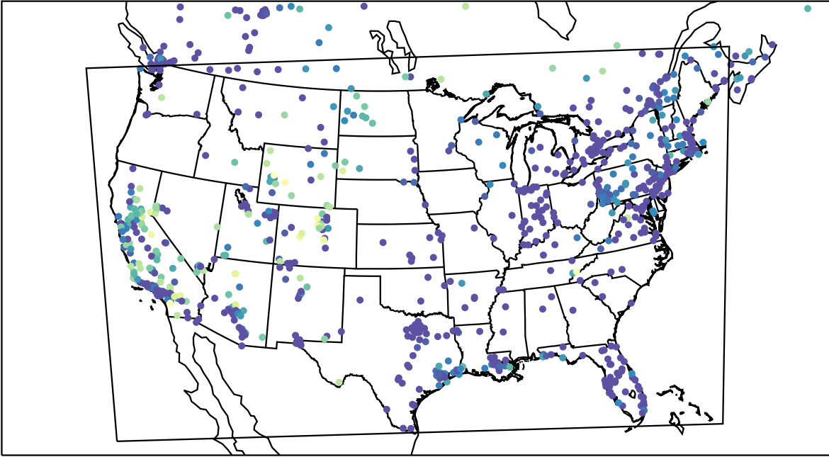
AirNOW (2024-01-03_11:00:00)
