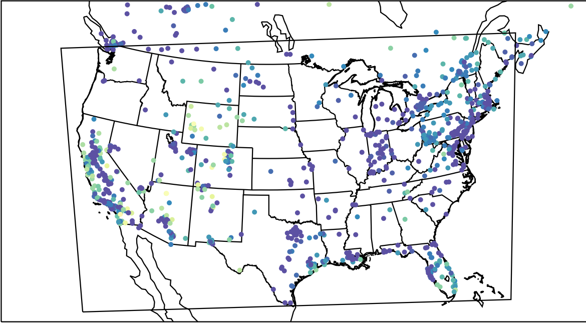
AirNOW (2024-01-03_02:00:00)
