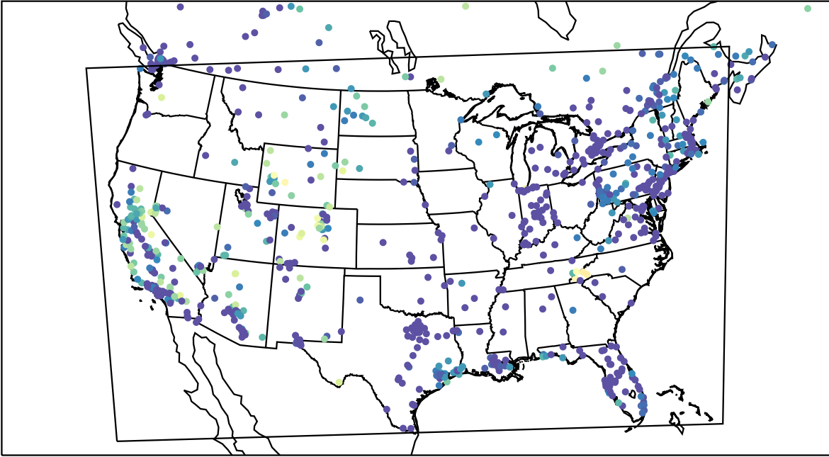
AirNOW (2024-01-03_10:00:00)
