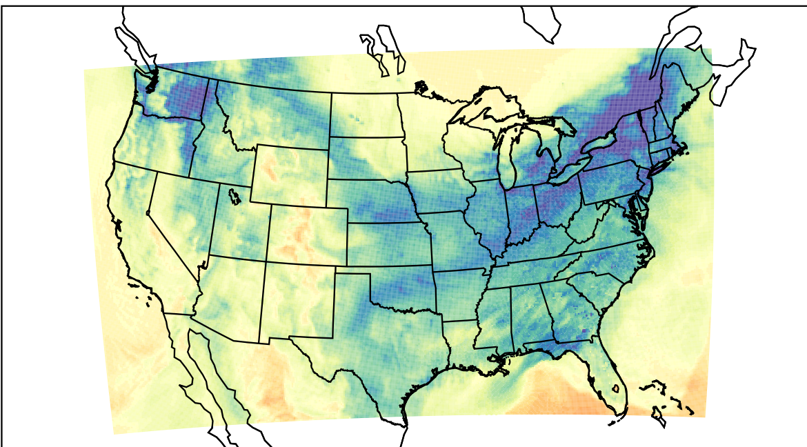
WRF (2024-01-03_22:00:00)
