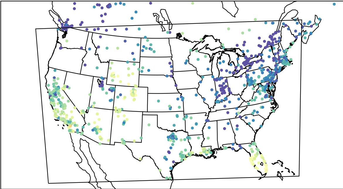
AirNOW (2024-01-03_20:00:00)
