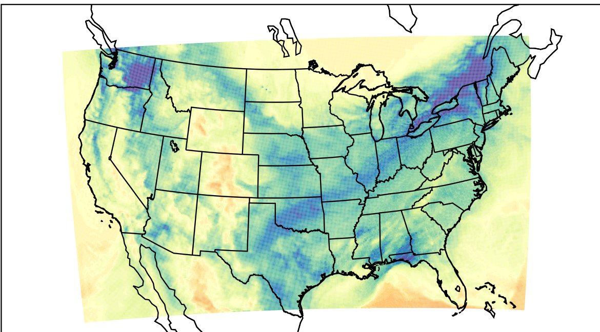
WRF (2024-01-03_19:00:00)
