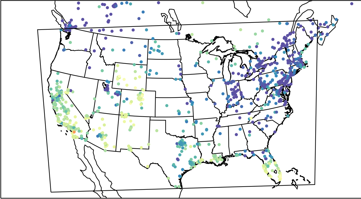
AirNOW (2024-01-03_22:00:00)
