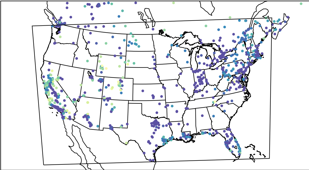
AirNOW (2024-01-03_08:00:00)
