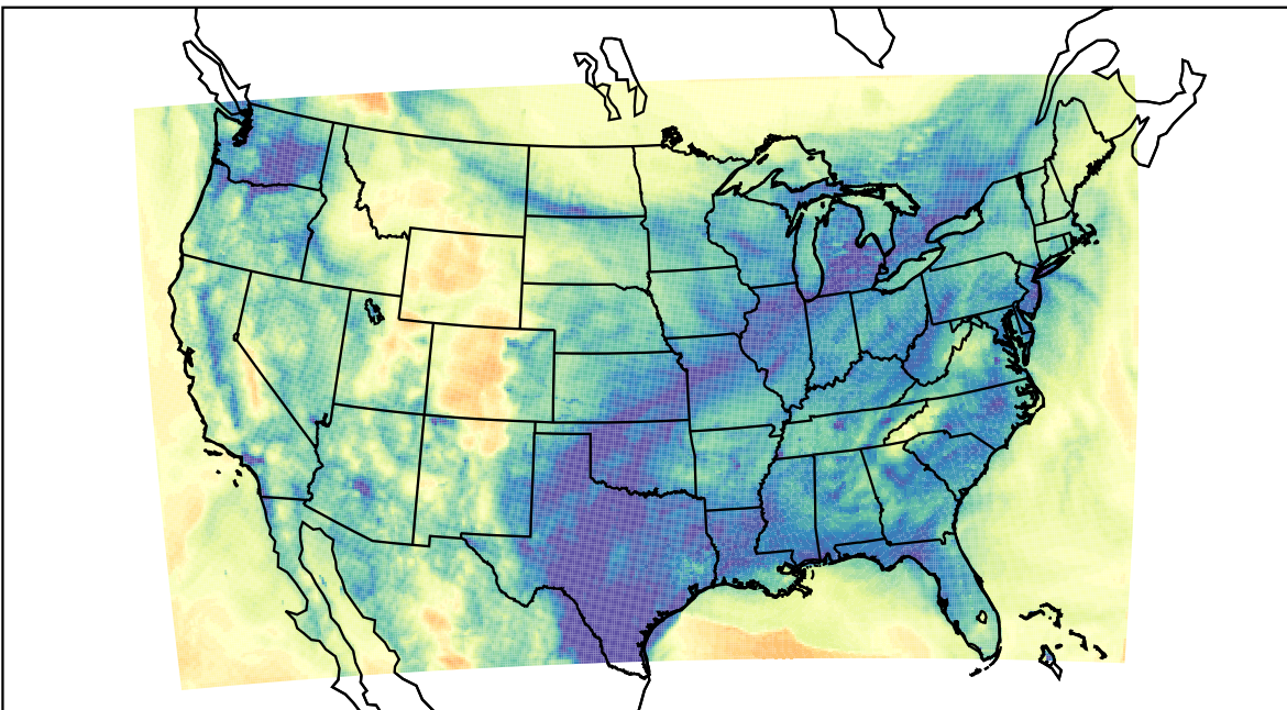
WRF (2024-01-03_07:00:00)
