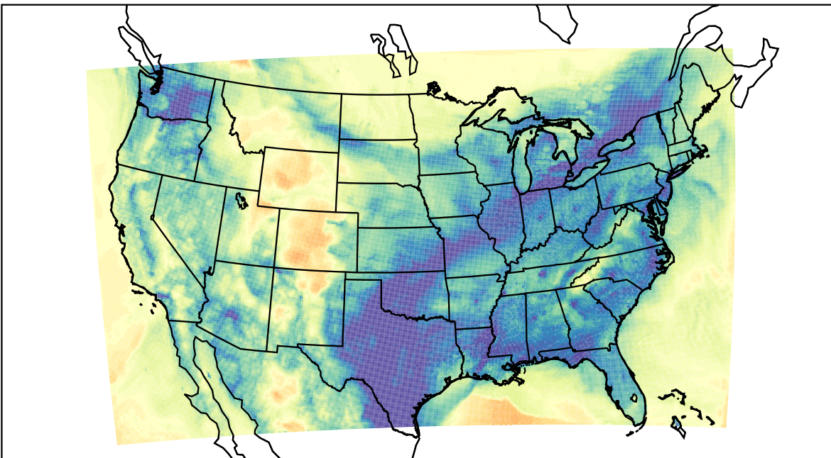
WRF (2024-01-03_11:00:00)
