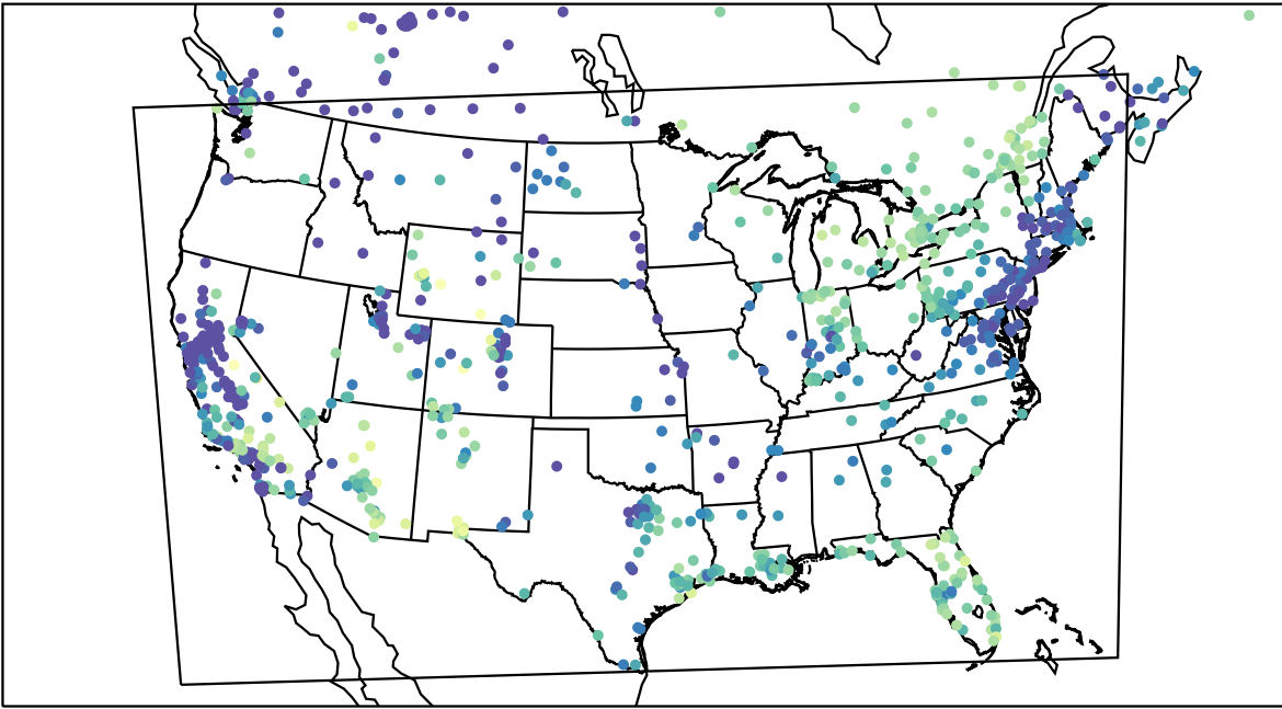
AirNOW (2024-01-04_17:00:00)
