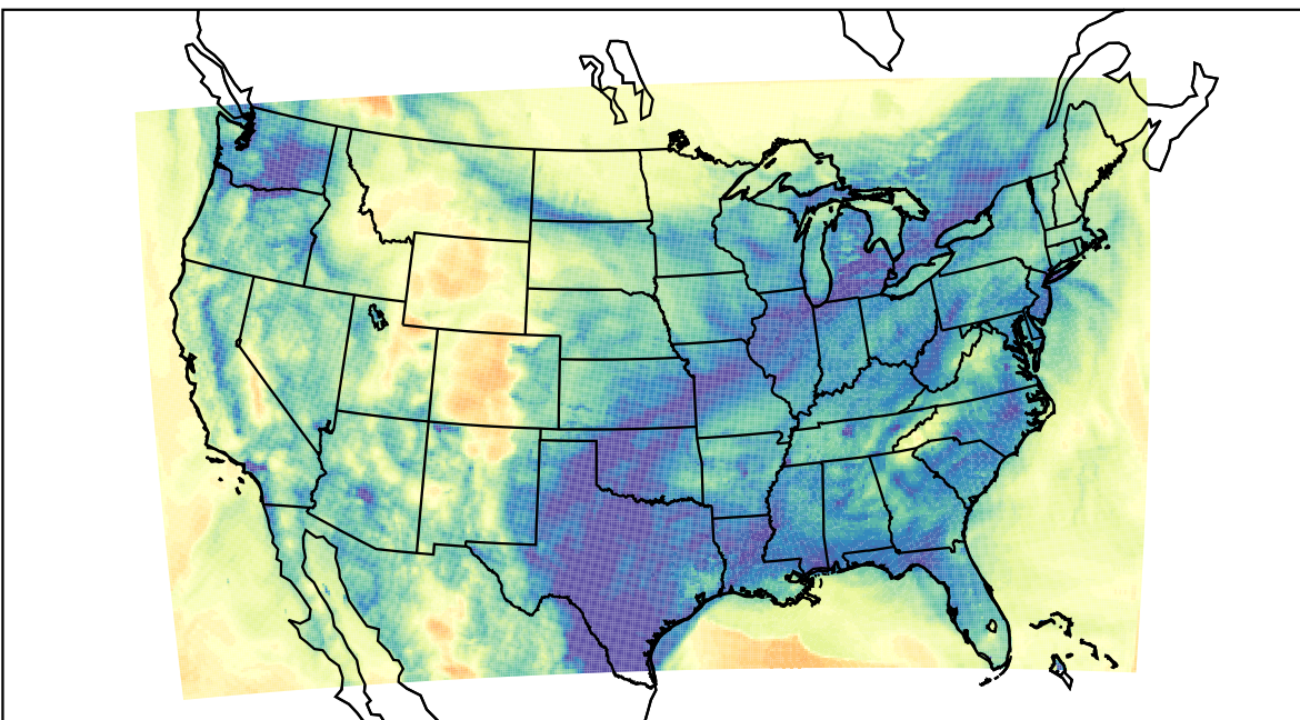
WRF (2024-01-03_08:00:00)
