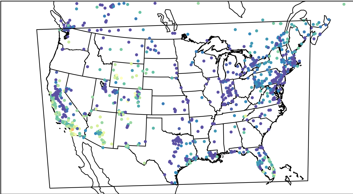
AirNOW (2024-01-03_00:00:00)
