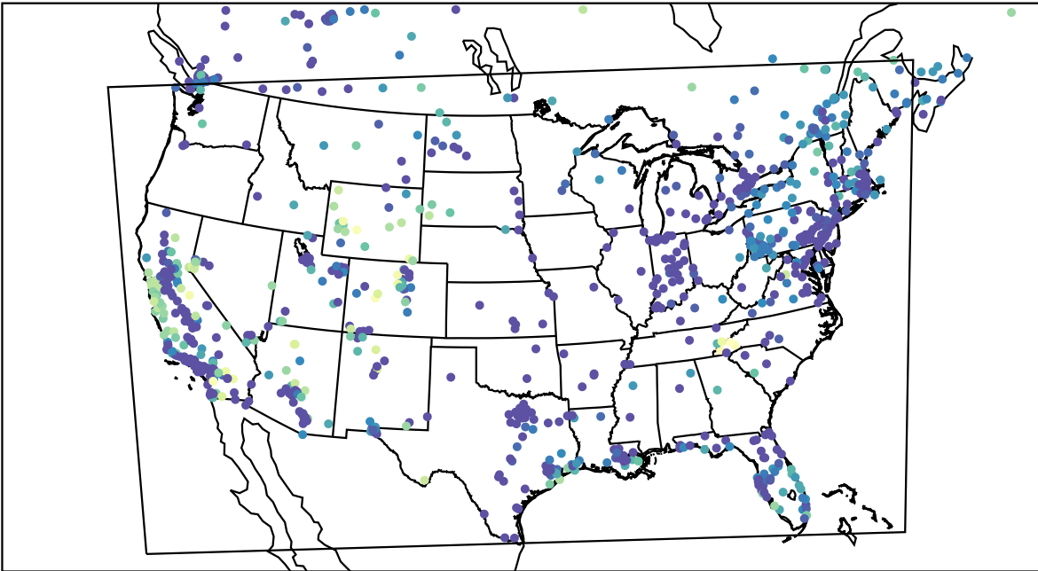
AirNOW (2024-01-03_04:00:00)
