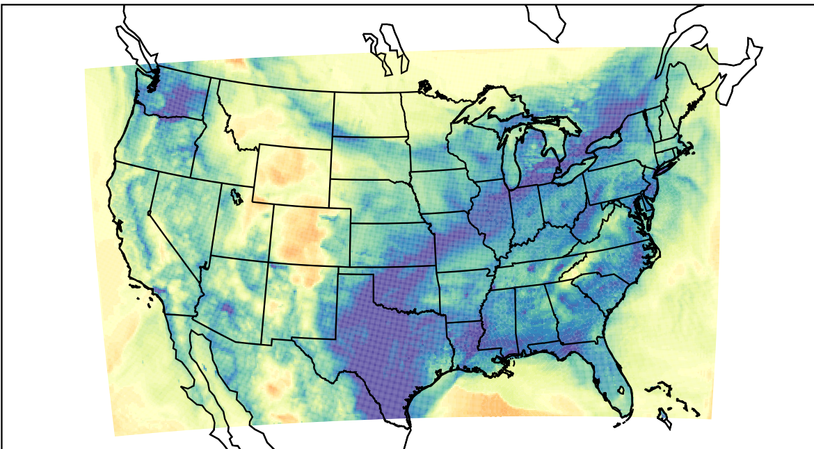
WRF (2024-01-03_10:00:00)
