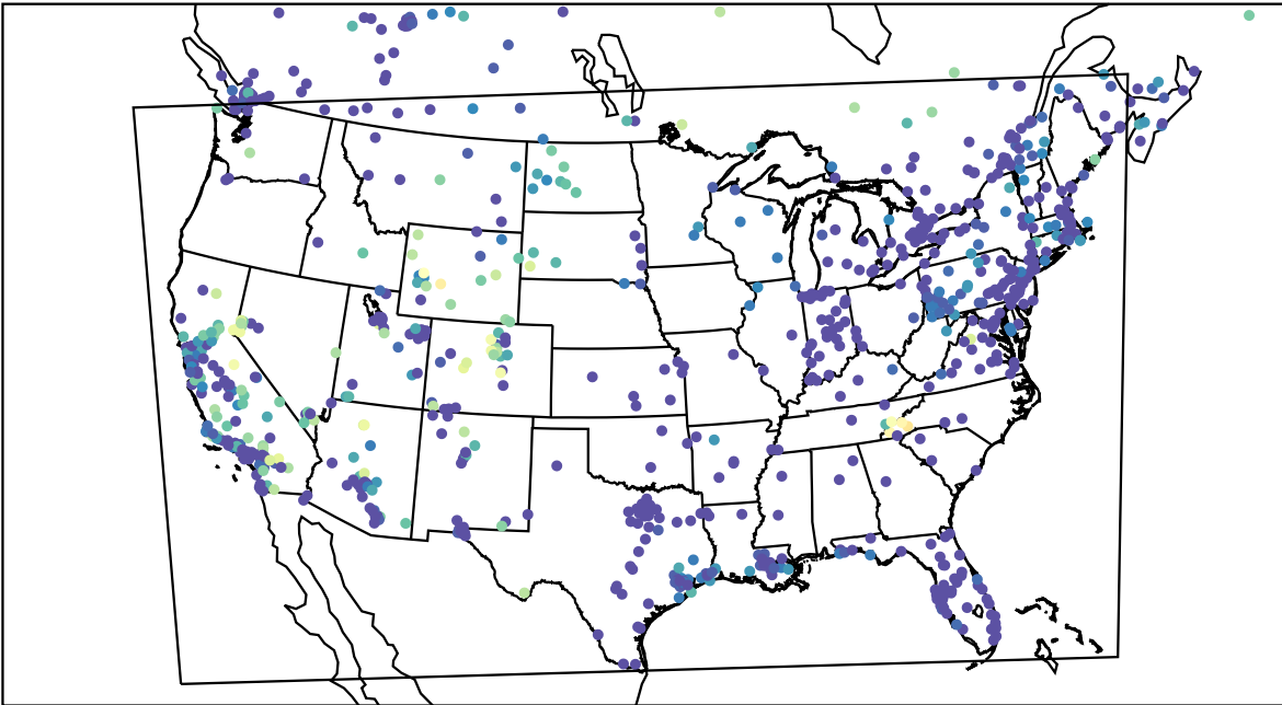
AirNOW (2024-01-03_12:00:00)
