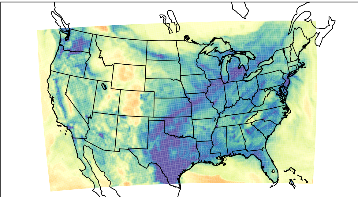
WRF (2024-01-03_05:00:00)
