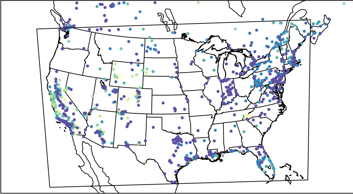
AirNOW (2024-01-03_05:00:00)
