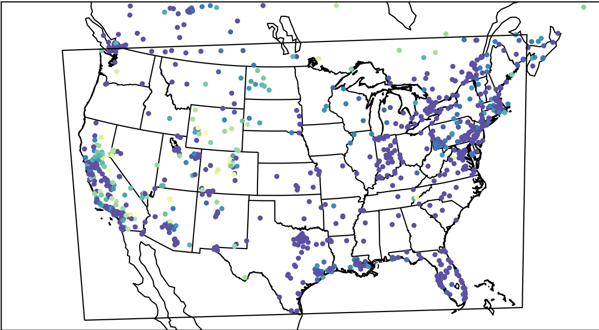
AirNOW (2024-01-03_13:00:00)
