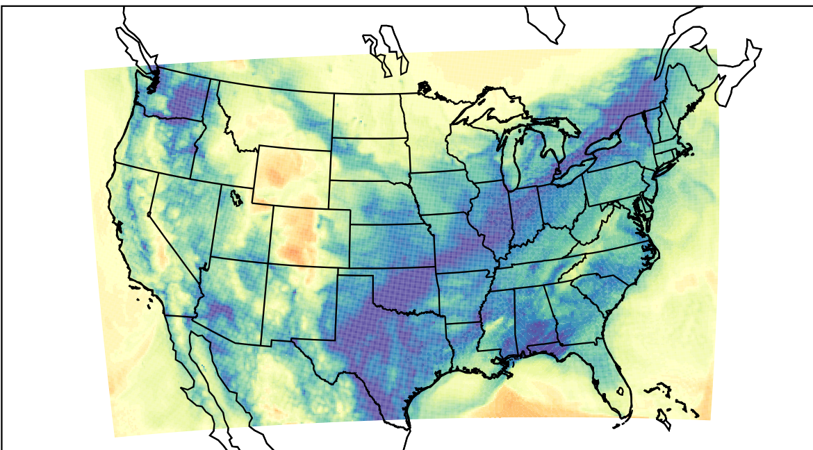
WRF (2024-01-03_16:00:00)
