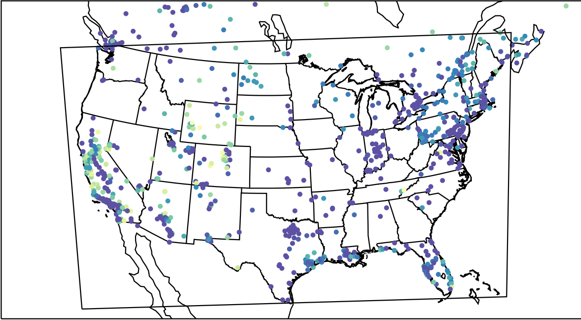
AirNOW (2024-01-03_07:00:00)
