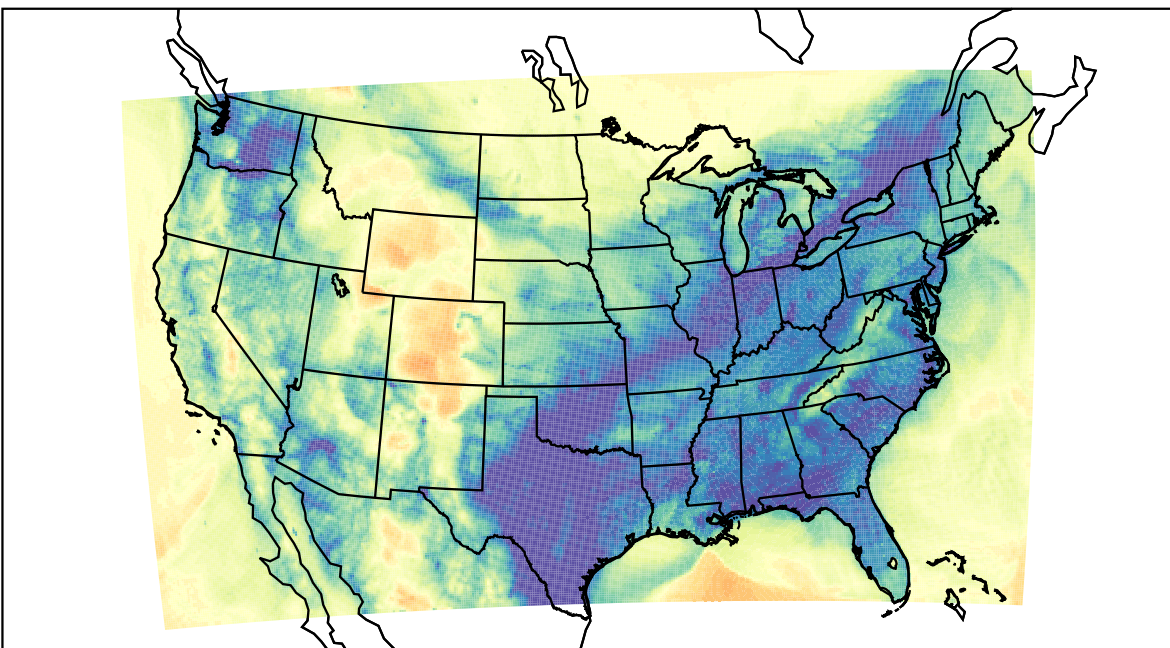
WRF (2024-01-03_14:00:00)
