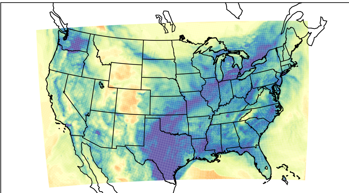
WRF (2024-01-03_09:00:00)
