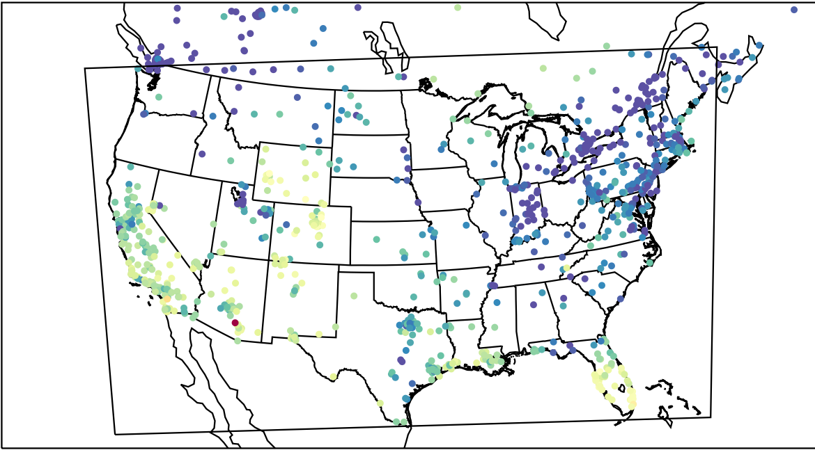
AirNOW (2024-01-03_21:00:00)
