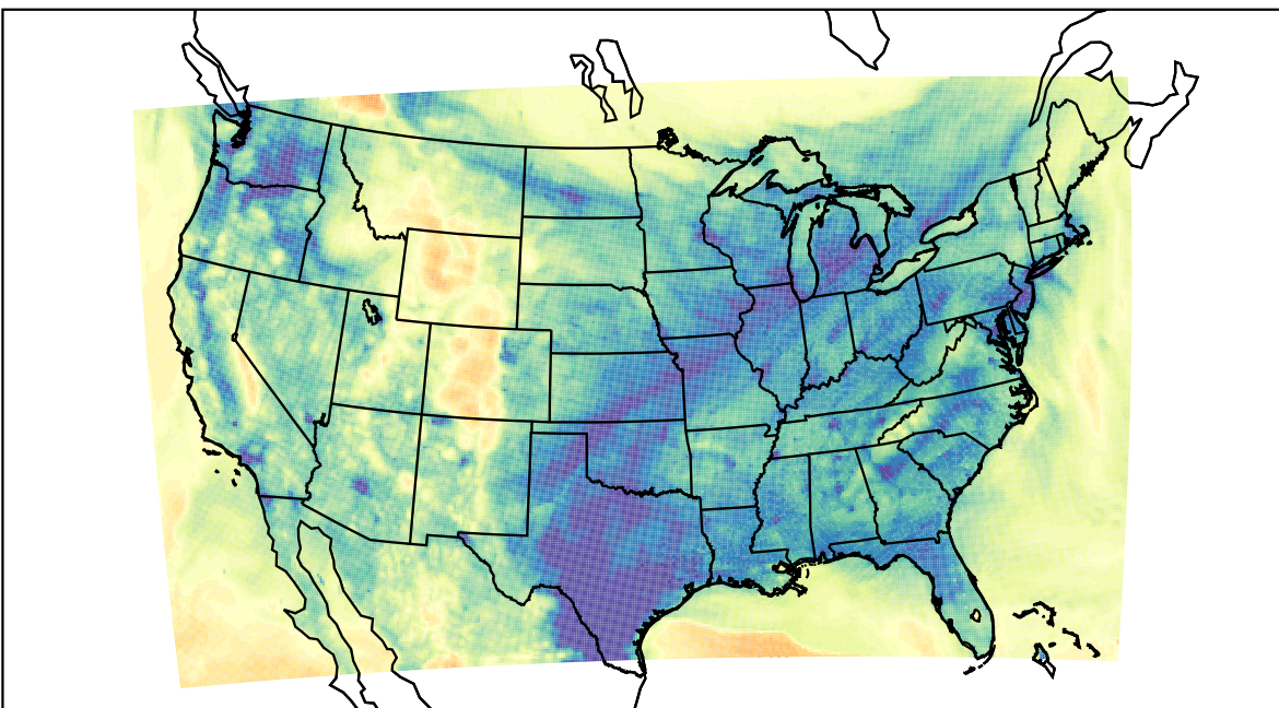
WRF (2024-01-03_03:00:00)
