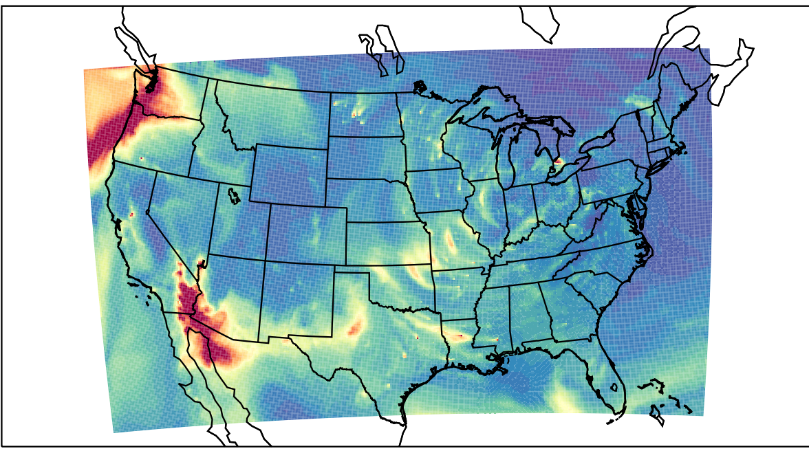
WRF 2024-01-05_09:00:00
