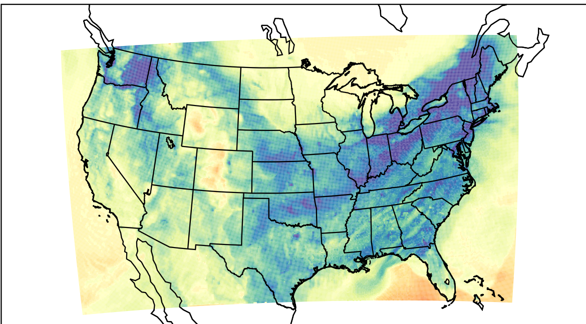
WRF (2024-01-04_00:00:00)
