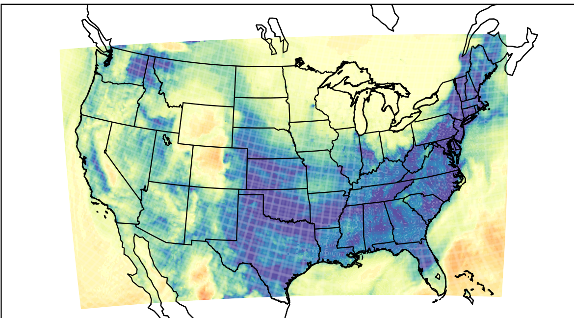
WRF (2024-01-04_13:00:00)
