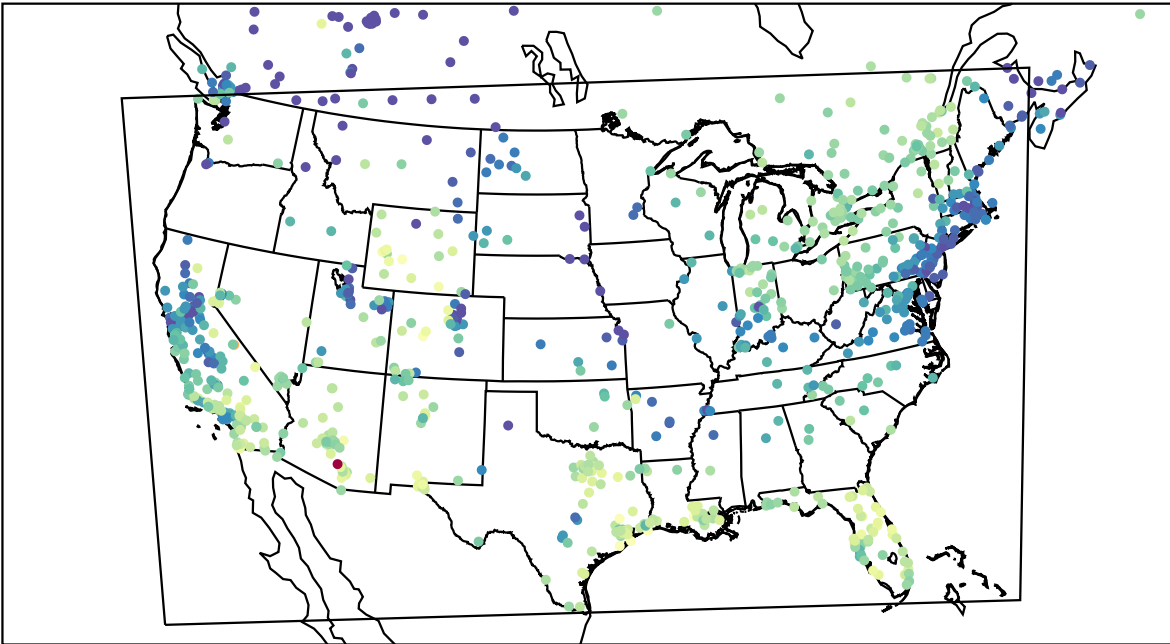
AirNOW (2024-01-04_20:00:00)
