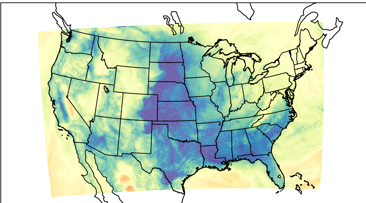
WRF (2024-01-05_08:00:00)
