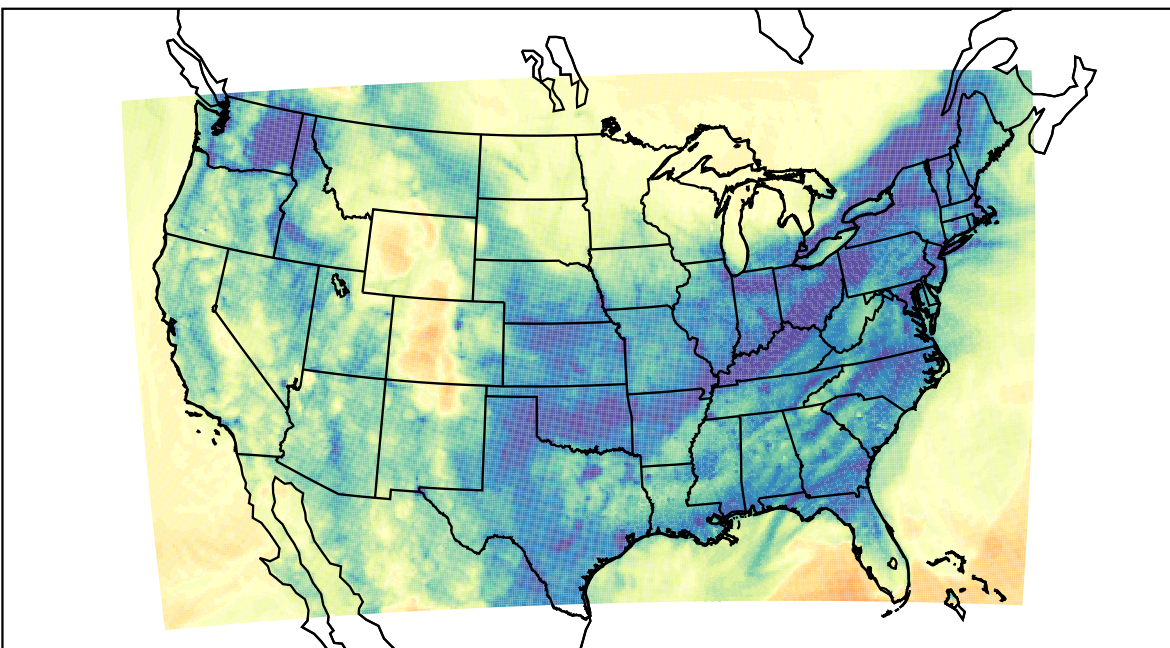
WRF (2024-01-04_03:00:00)
