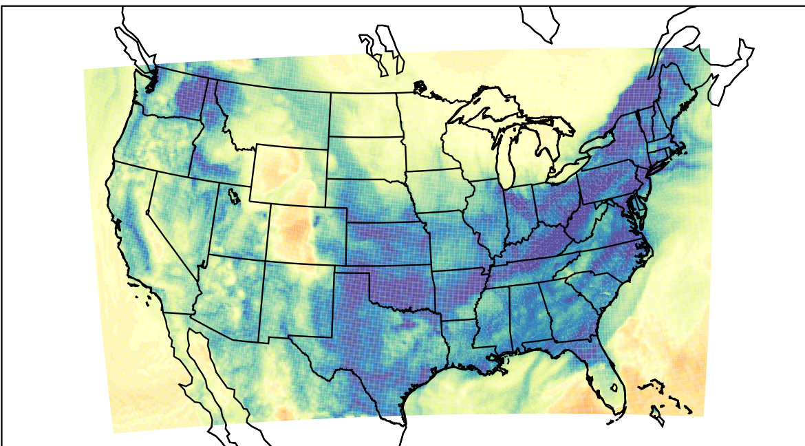
WRF (2024-01-04_07:00:00)
