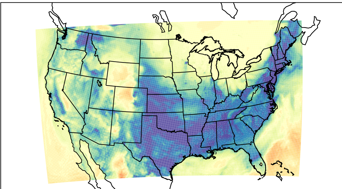
WRF (2024-01-04_14:00:00)
