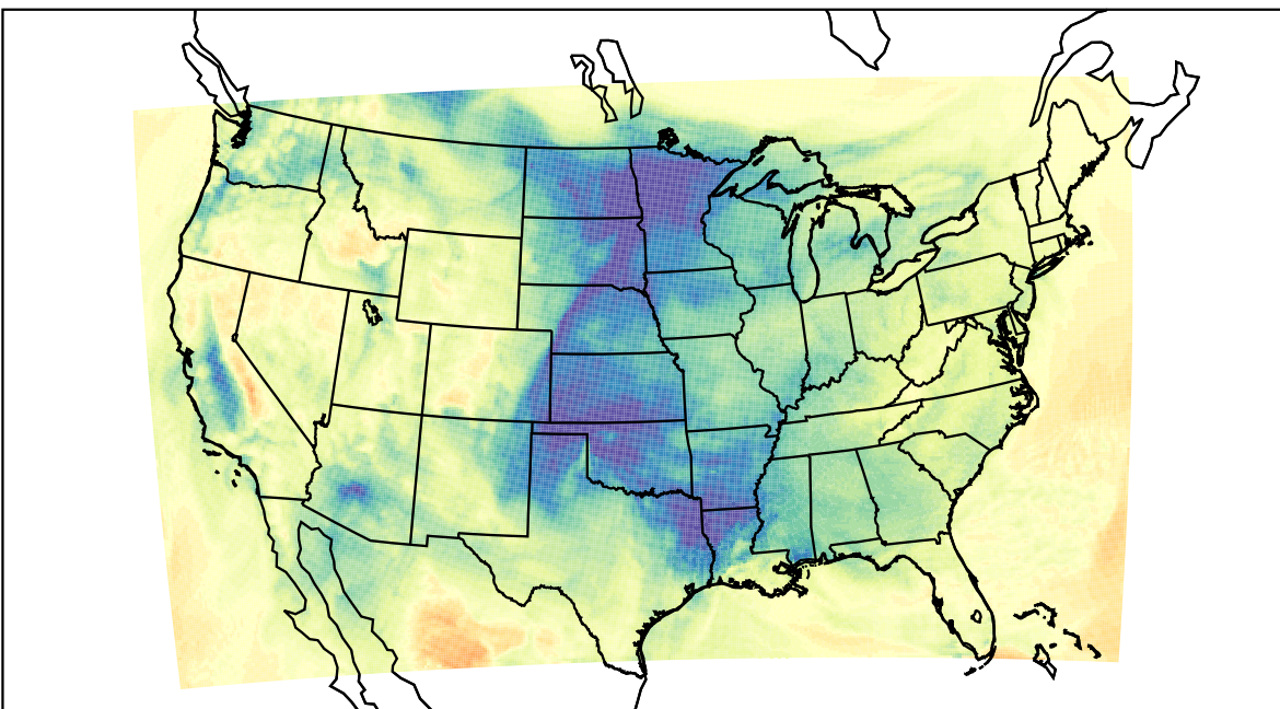
WRF (2024-01-05_19:00:00)
