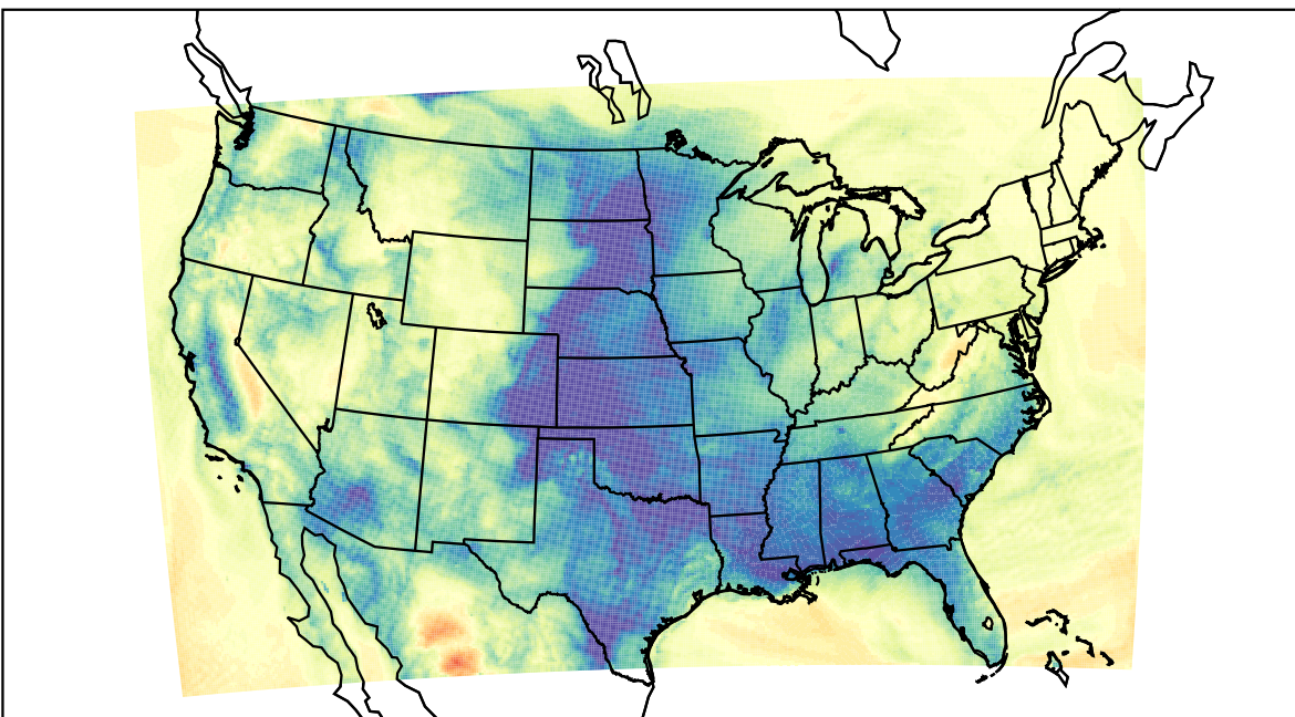
WRF (2024-01-05_11:00:00)
