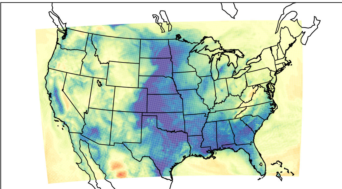
WRF (2024-01-05_12:00:00)
