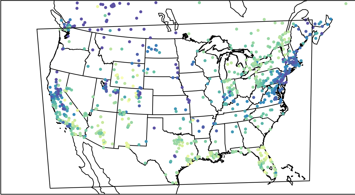
AirNOW (2024-01-04_19:00:00)
