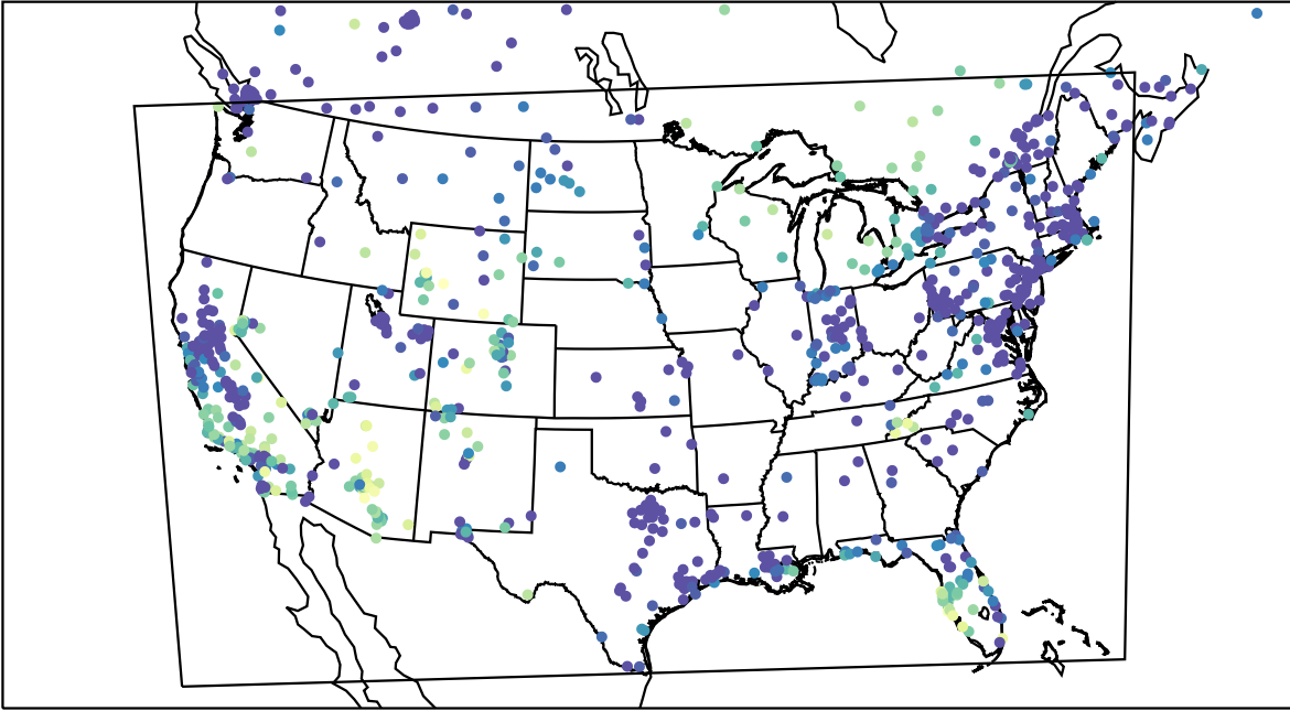
AirNOW (2024-01-04_05:00:00)
