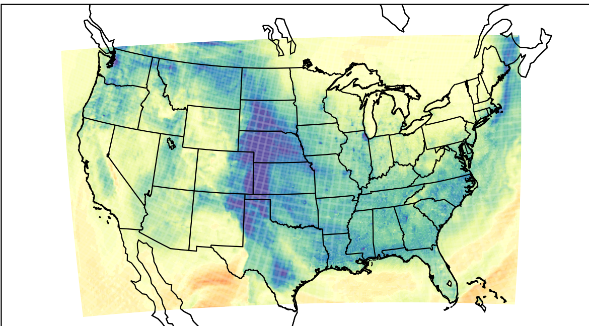
WRF (2024-01-04_23:00:00)
