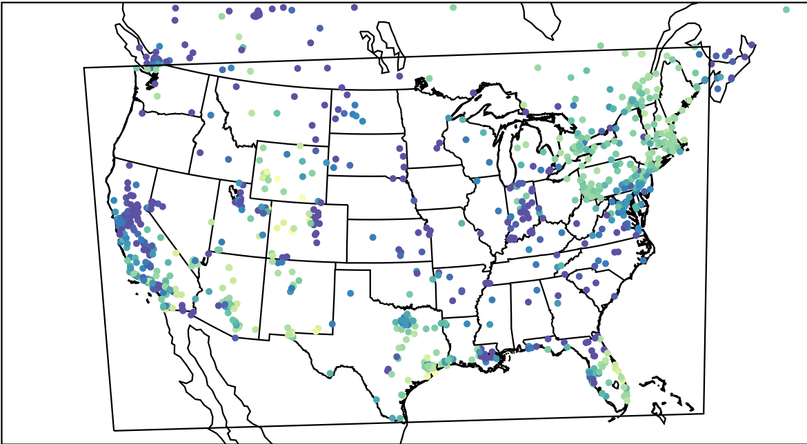
AirNOW (2024-01-05_01:00:00)
