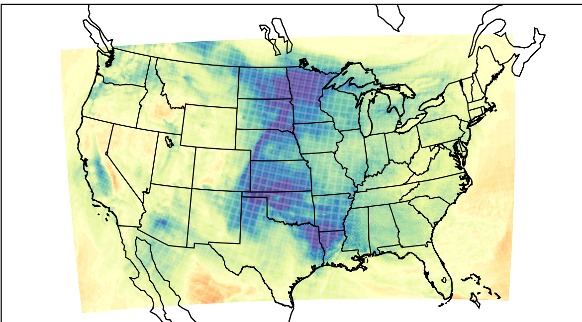
WRF (2024-01-05_20:00:00)
