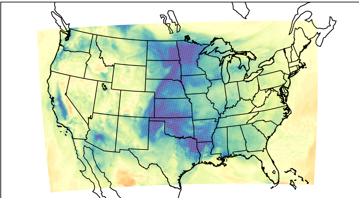
WRF (2024-01-05_18:00:00)
