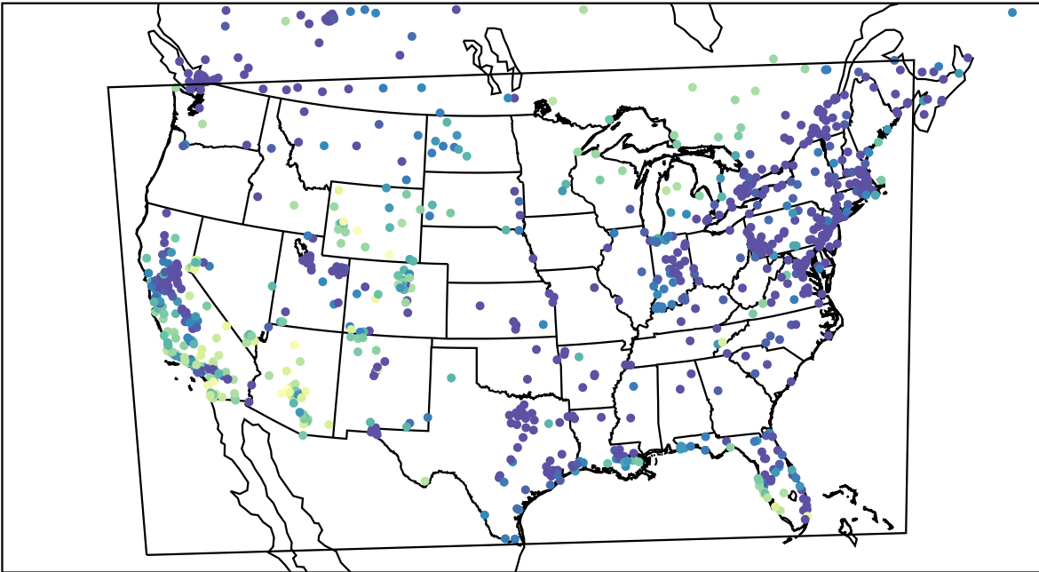
AirNOW (2024-01-04_02:00:00)
