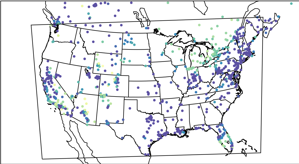
AirNOW (2024-01-04_11:00:00)
