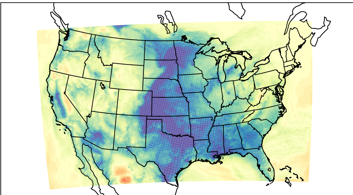
WRF (2024-01-05_14:00:00)
