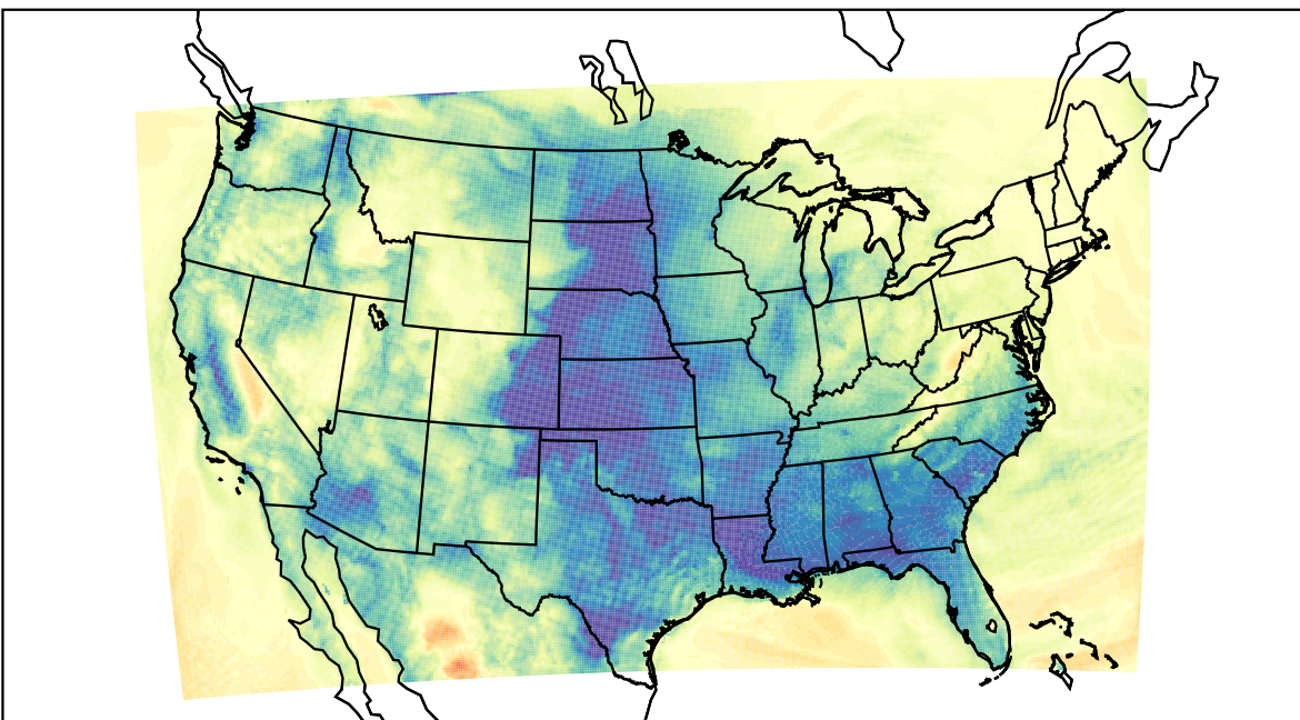
WRF (2024-01-05_09:00:00)
