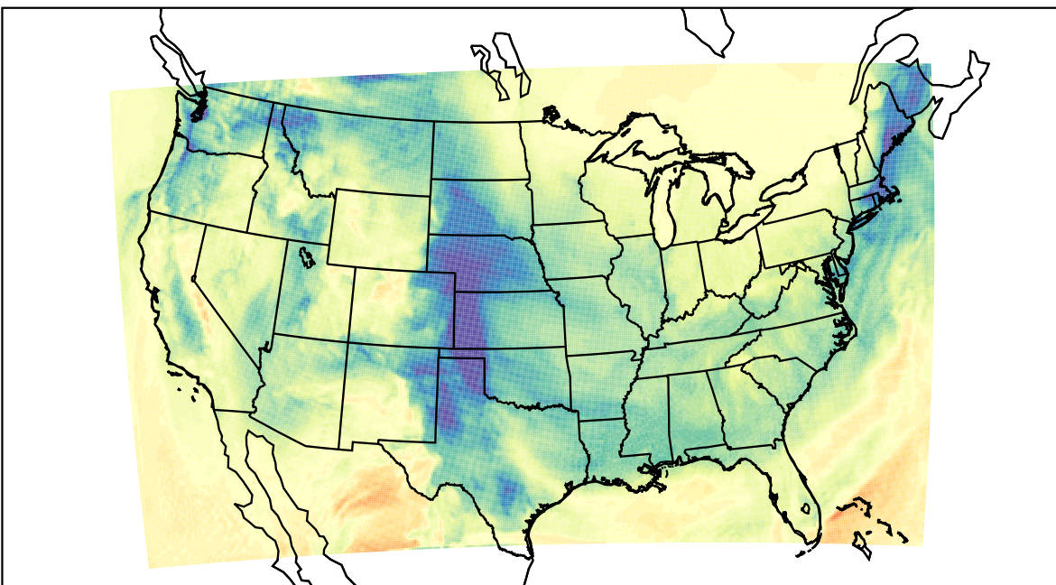
WRF (2024-01-04_20:00:00)
