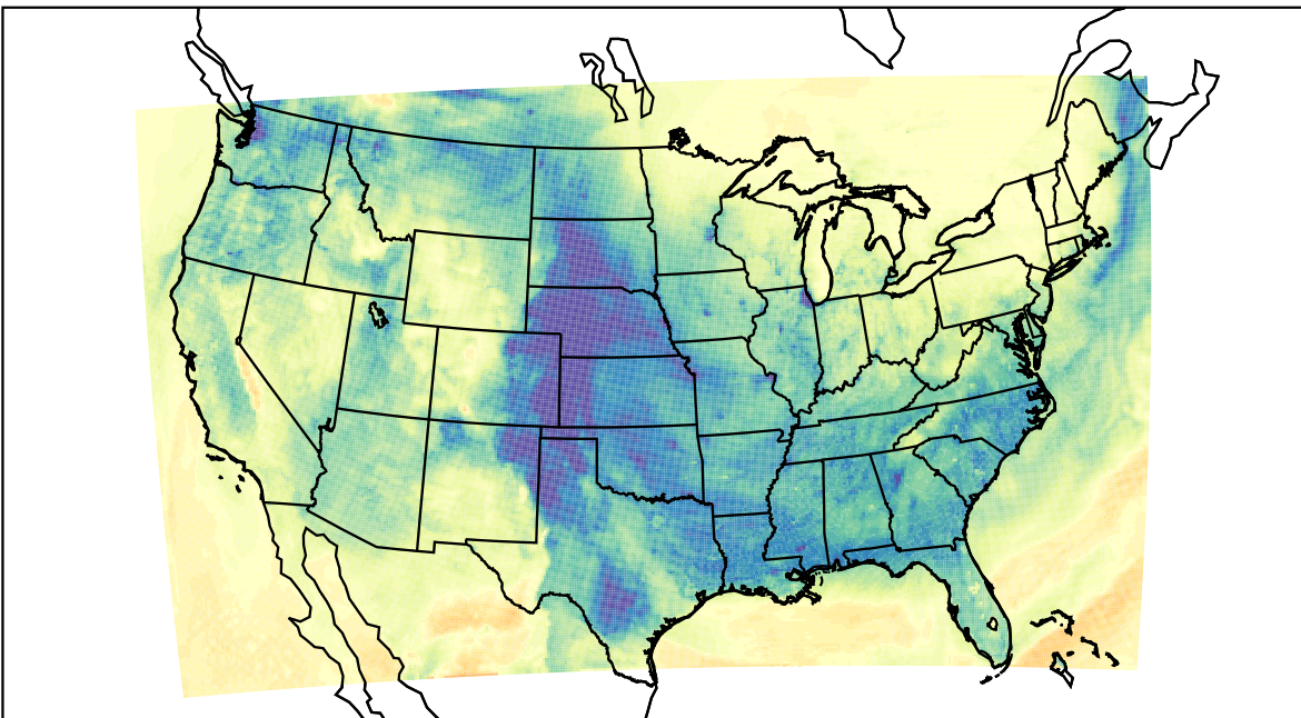
WRF (2024-01-05_00:00:00)
