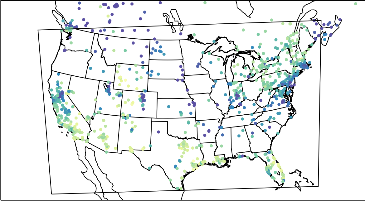
AirNOW (2024-01-04_22:00:00)
