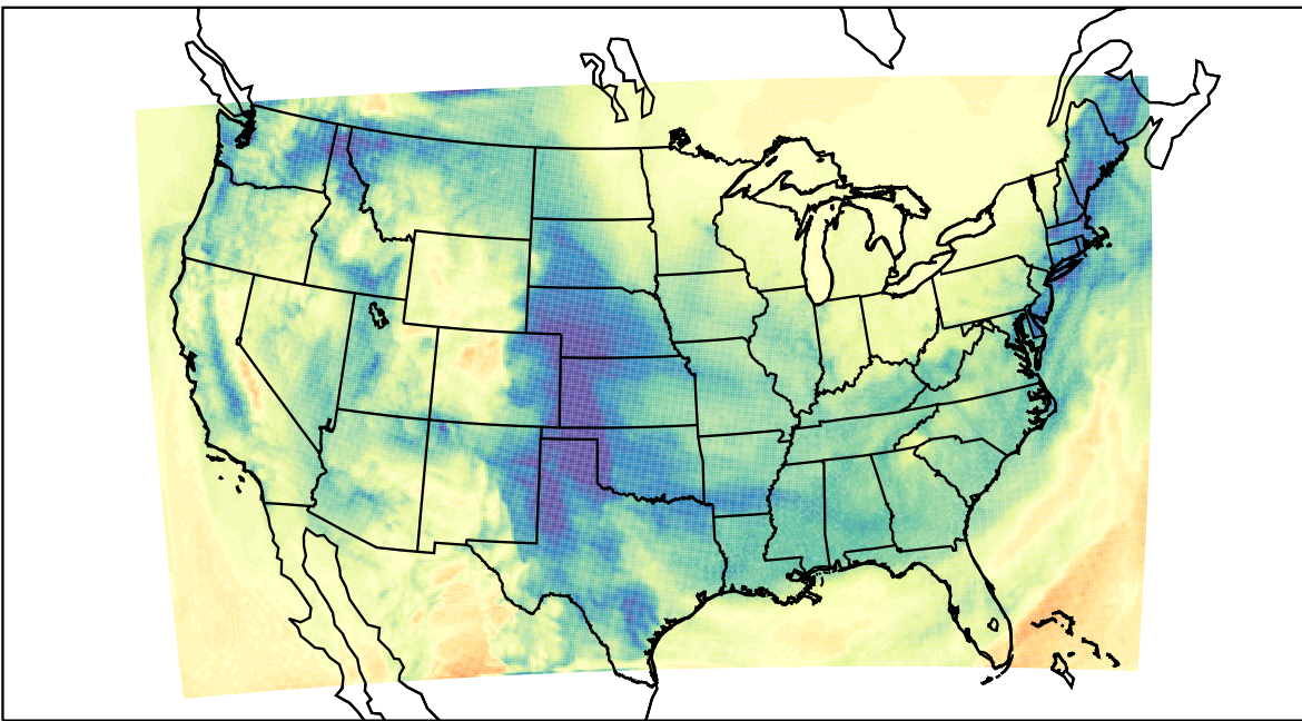
WRF (2024-01-04_18:00:00)
