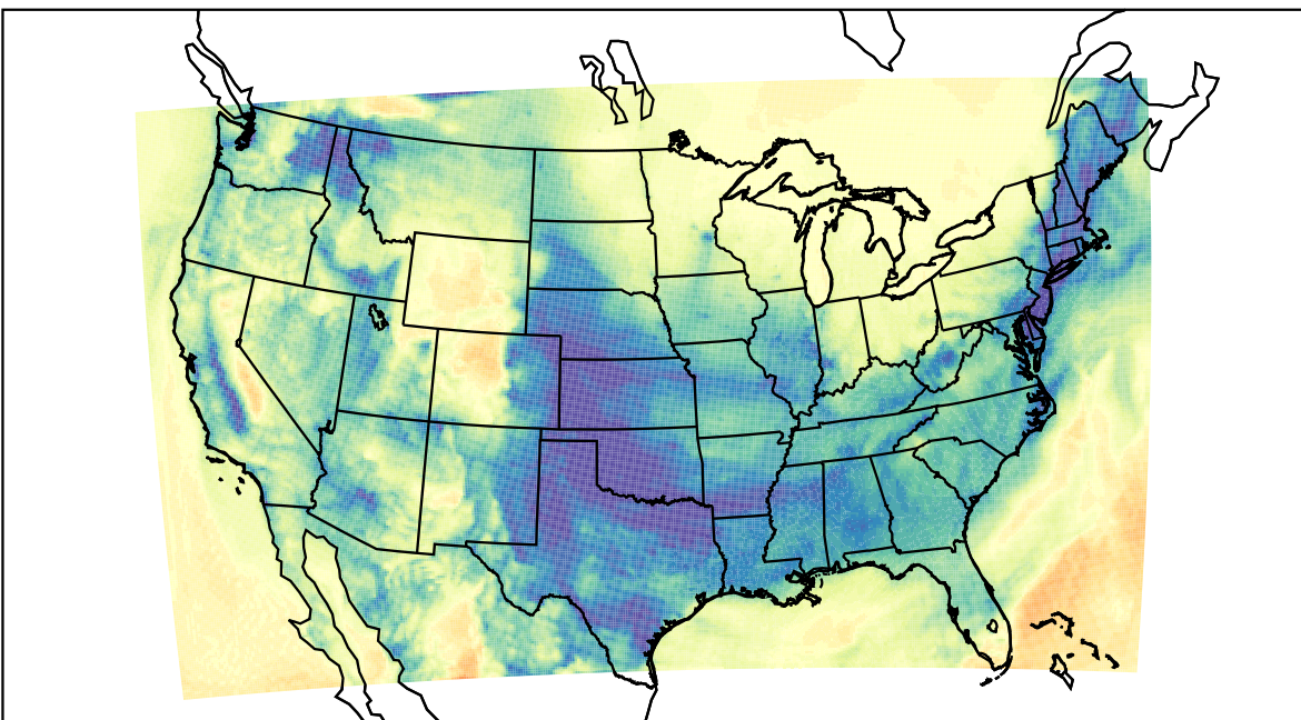
WRF (2024-01-04_16:00:00)
