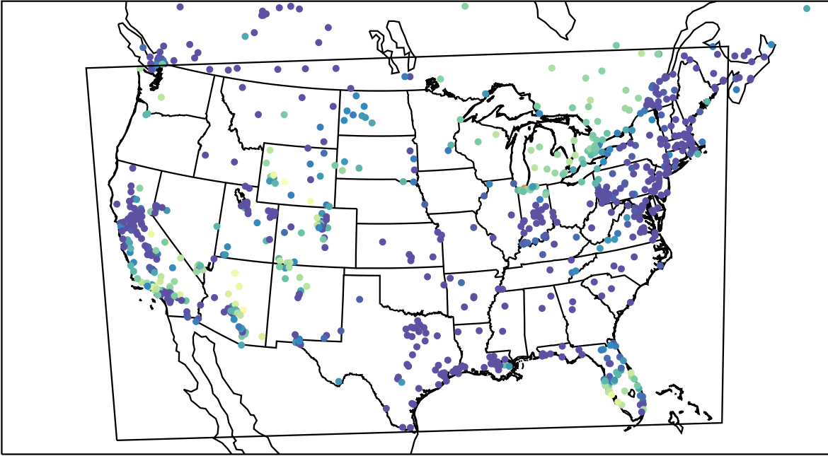
AirNOW (2024-01-04_10:00:00)
