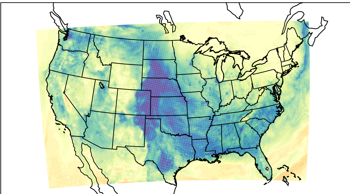
WRF (2024-01-05_01:00:00)
