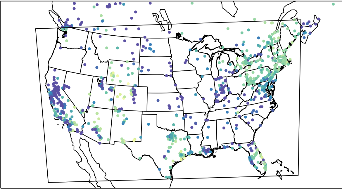
AirNOW (2024-01-05_02:00:00)
