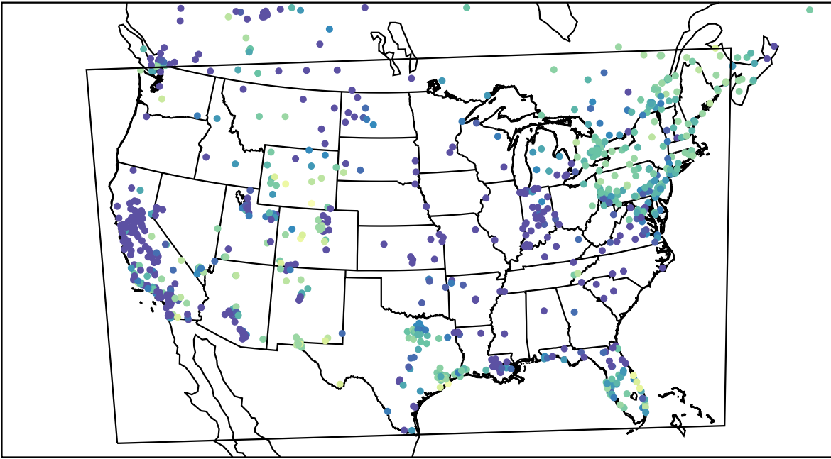
AirNOW (2024-01-05_08:00:00)
