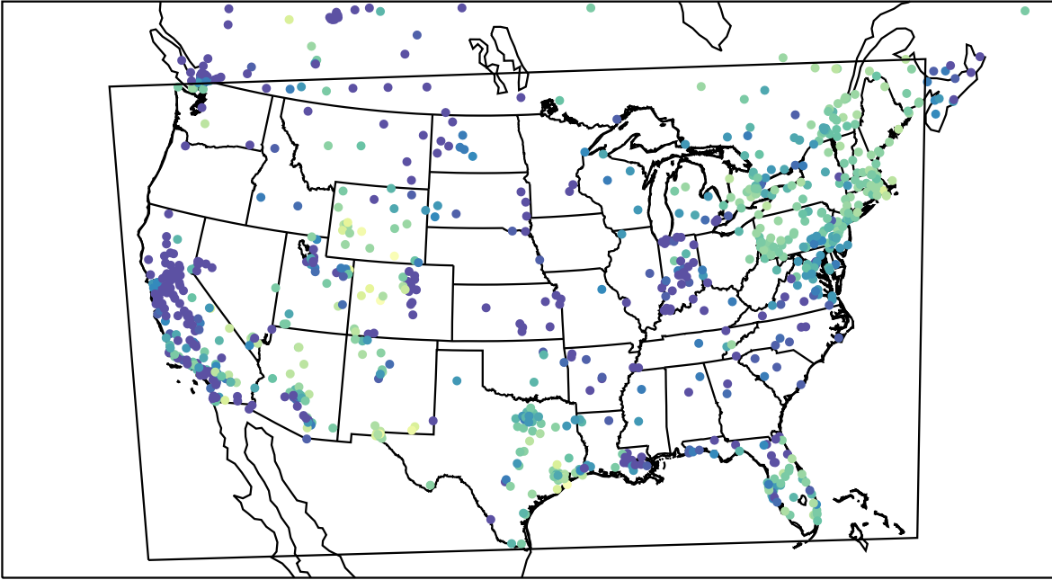
AirNOW (2024-01-05_03:00:00)
