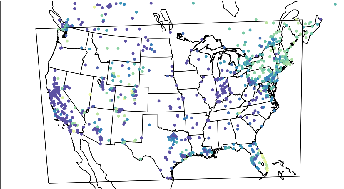
AirNOW (2024-01-05_14:00:00)
