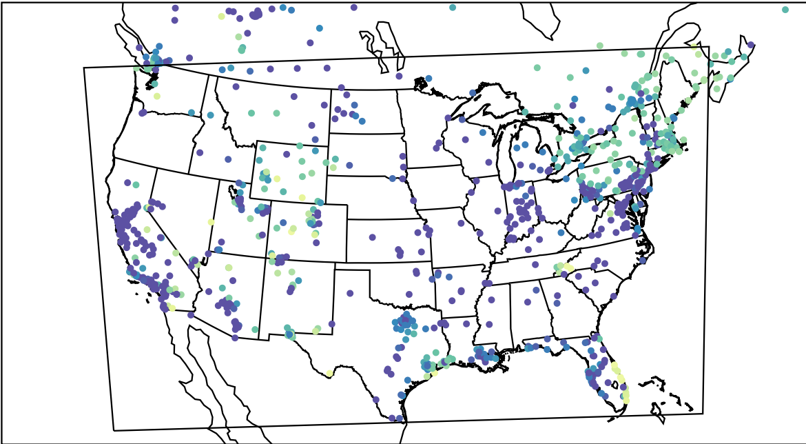
AirNOW (2024-01-05_12:00:00)
