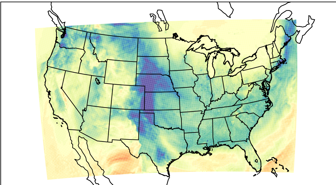
WRF (2024-01-04_22:00:00)
