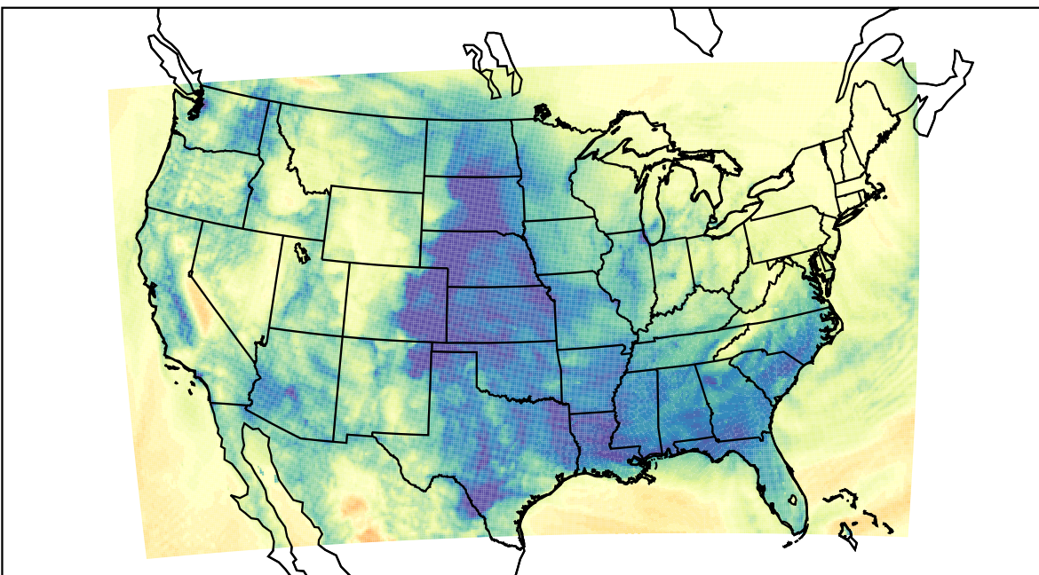
WRF (2024-01-05_06:00:00)
