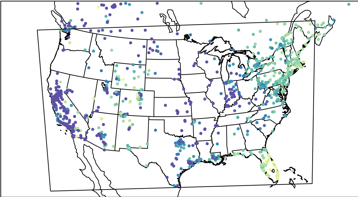
AirNOW (2024-01-05_16:00:00)
