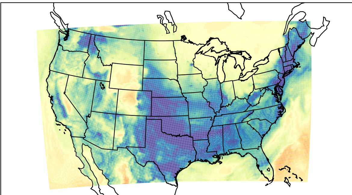
WRF (2024-01-04_15:00:00)
