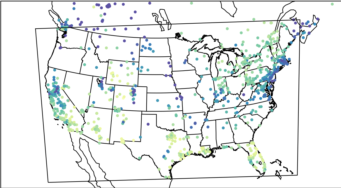
AirNOW (2024-01-04_21:00:00)
