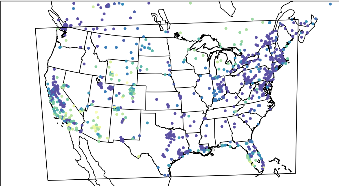
AirNOW (2024-01-04_03:00:00)
