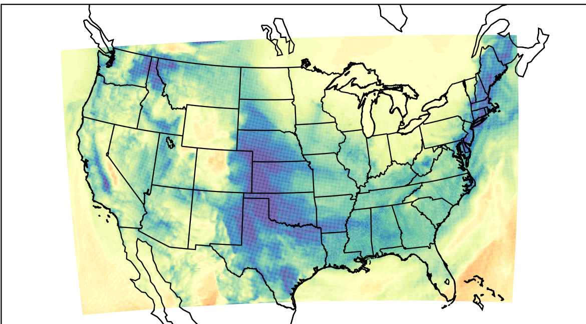
WRF (2024-01-04_17:00:00)
