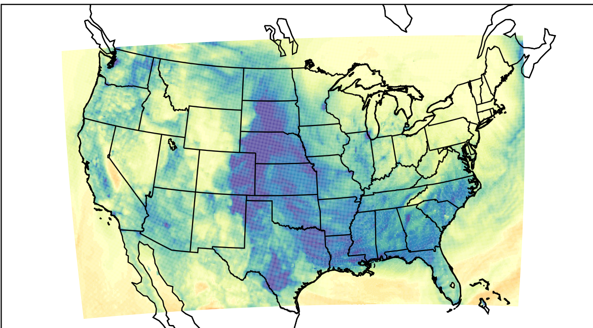
WRF (2024-01-05_03:00:00)
