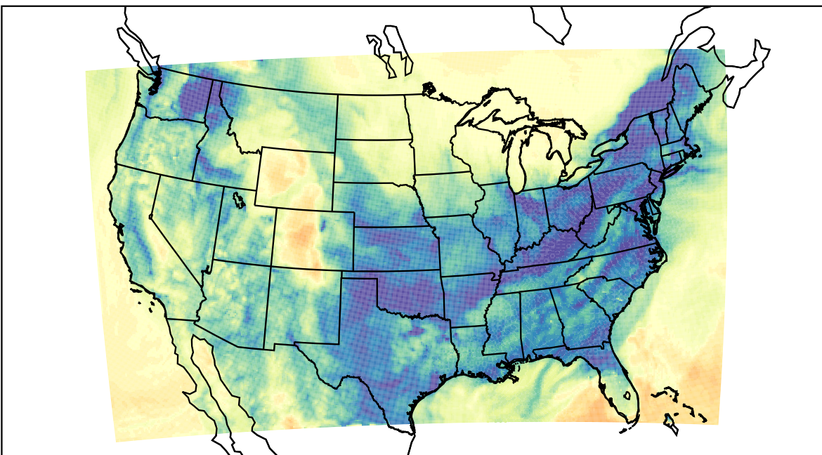
WRF (2024-01-04_06:00:00)
