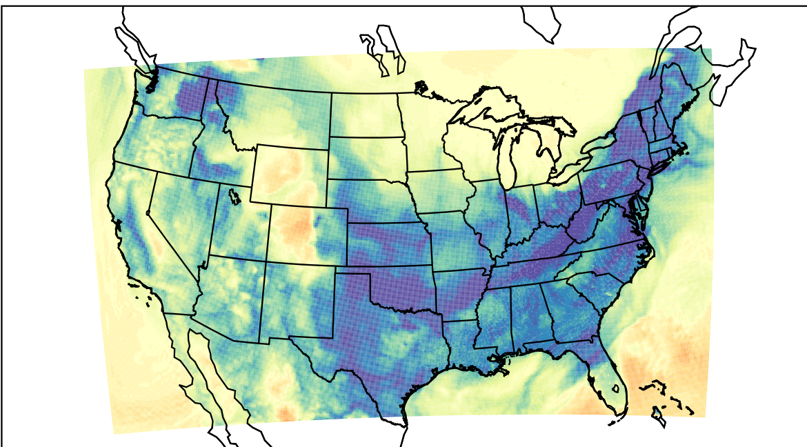
WRF (2024-01-04_09:00:00)
