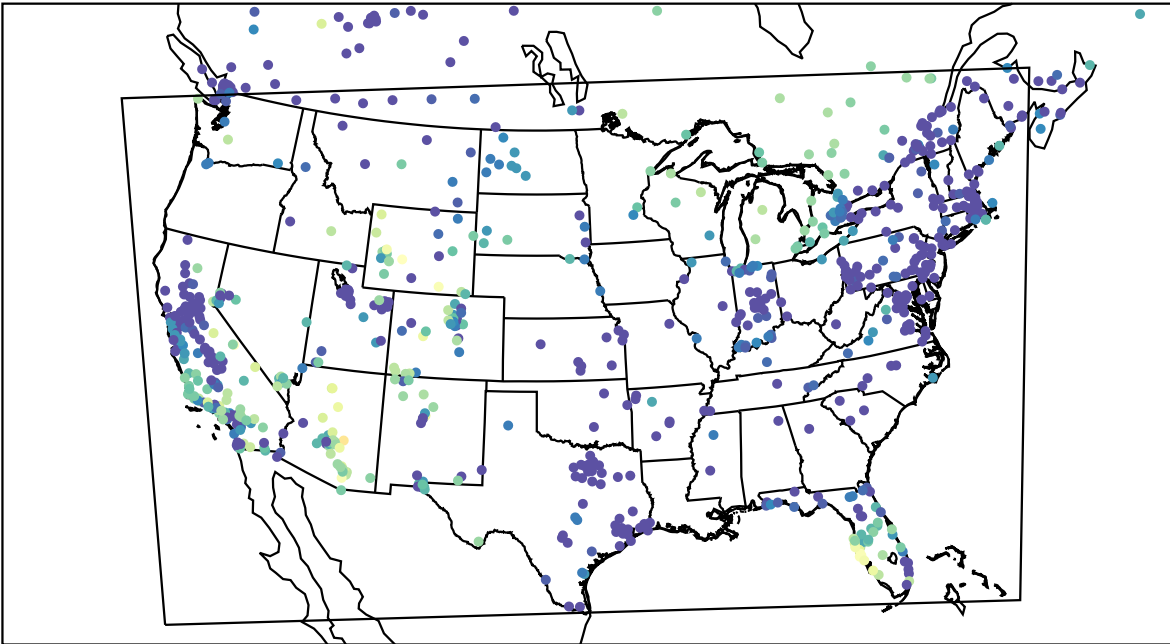
AirNOW (2024-01-04_07:00:00)
