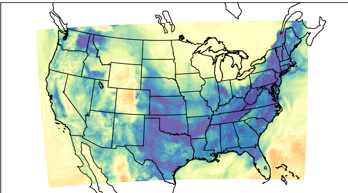
WRF (2024-01-04_11:00:00)
