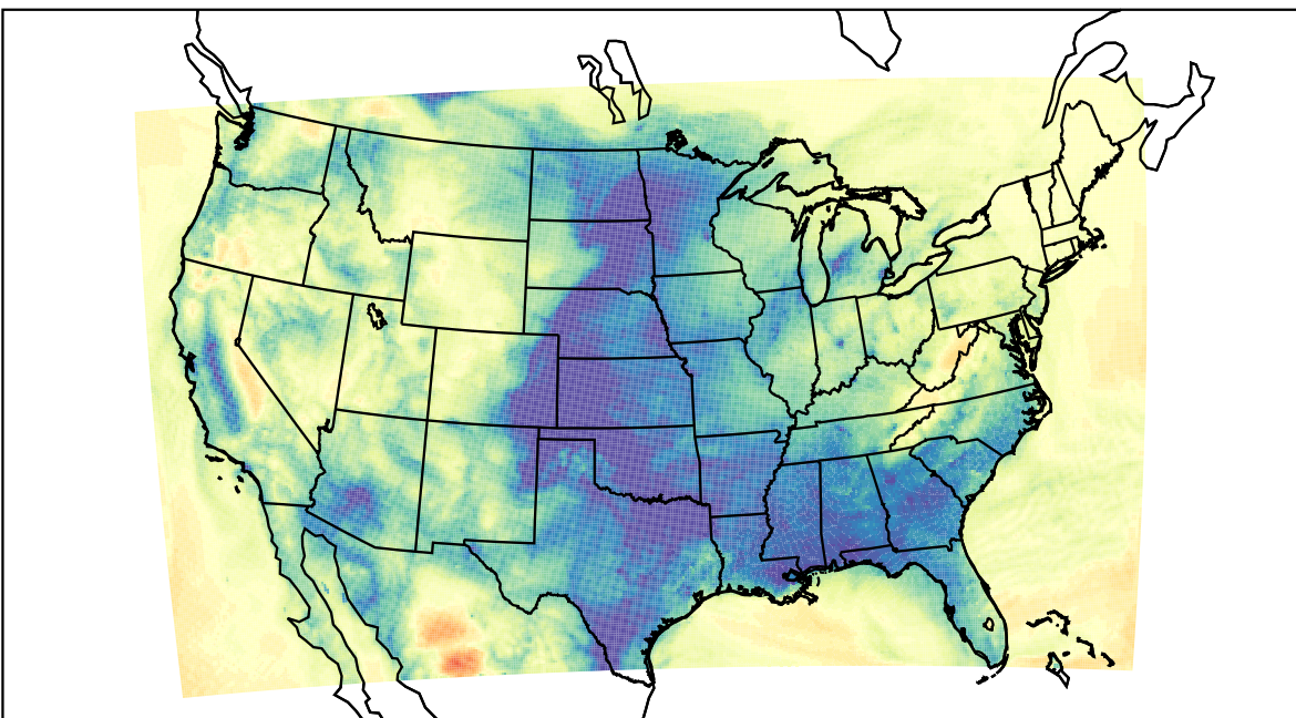
WRF (2024-01-05_13:00:00)
