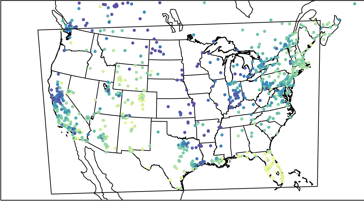
AirNOW (2024-01-05_20:00:00)
