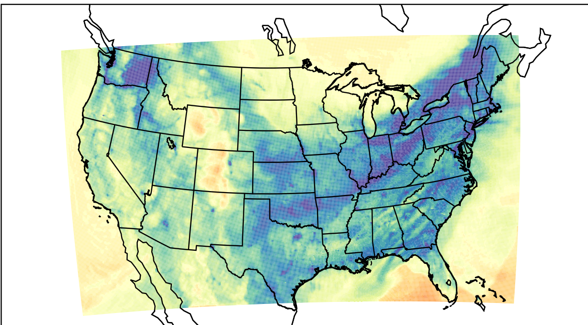
WRF (2024-01-04_01:00:00)
