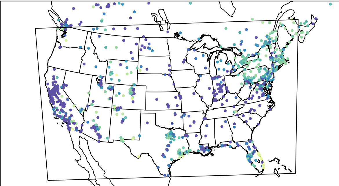
AirNOW (2024-01-05_09:00:00)
