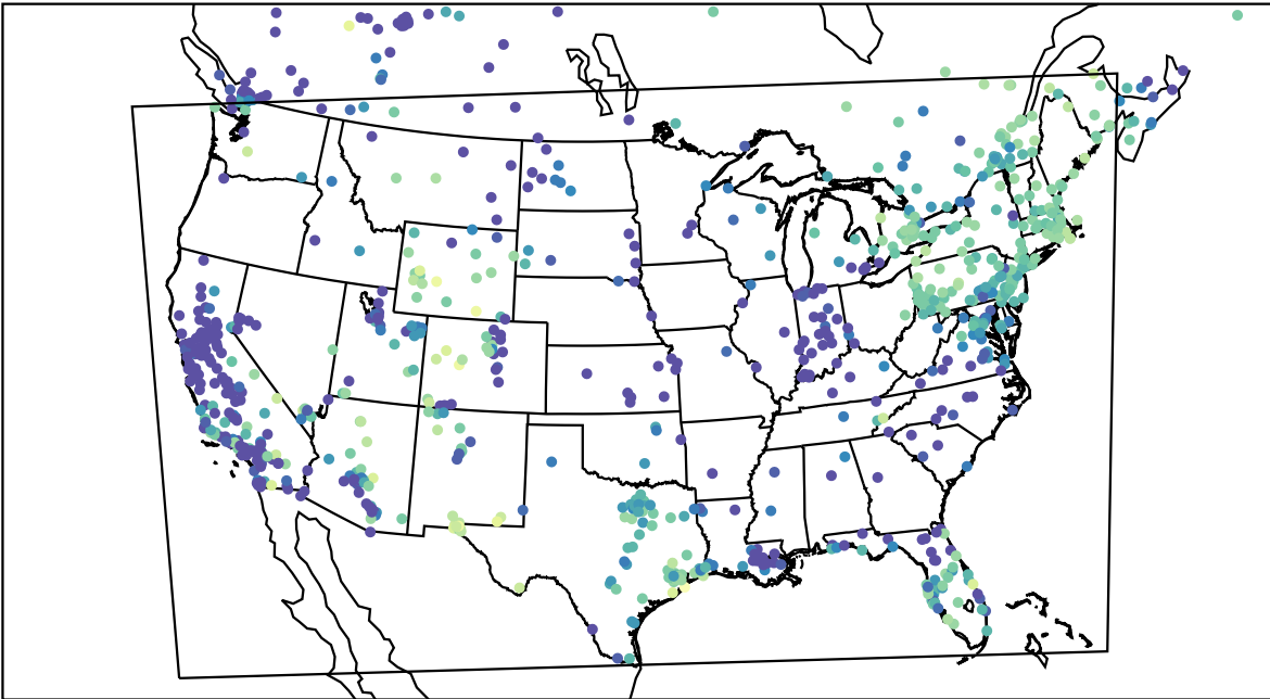
AirNOW (2024-01-05_05:00:00)
