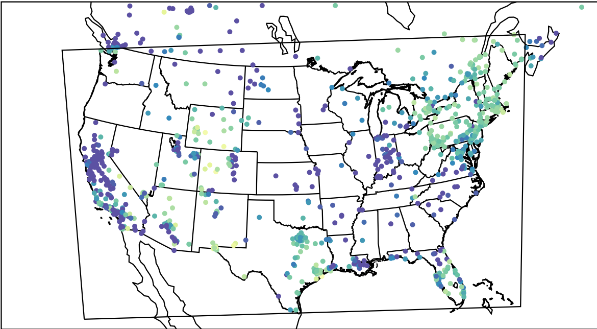
AirNOW (2024-01-05_04:00:00)
