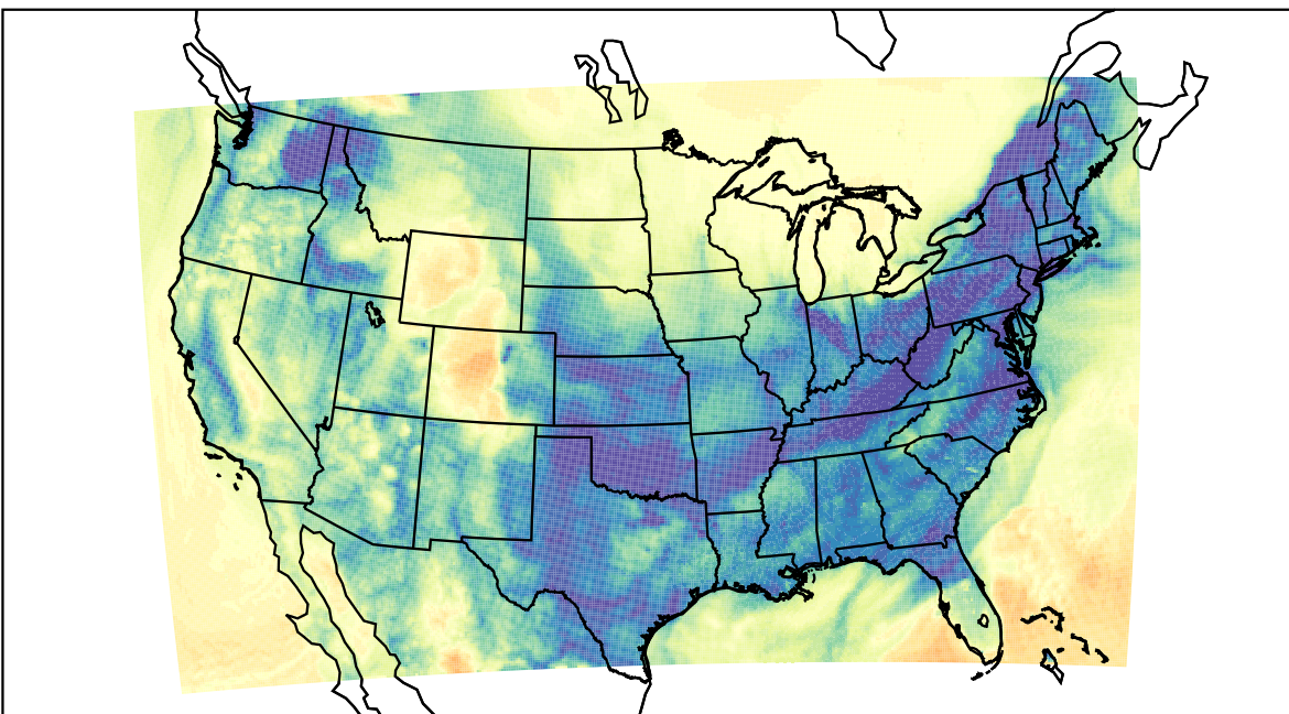
WRF (2024-01-04_08:00:00)
