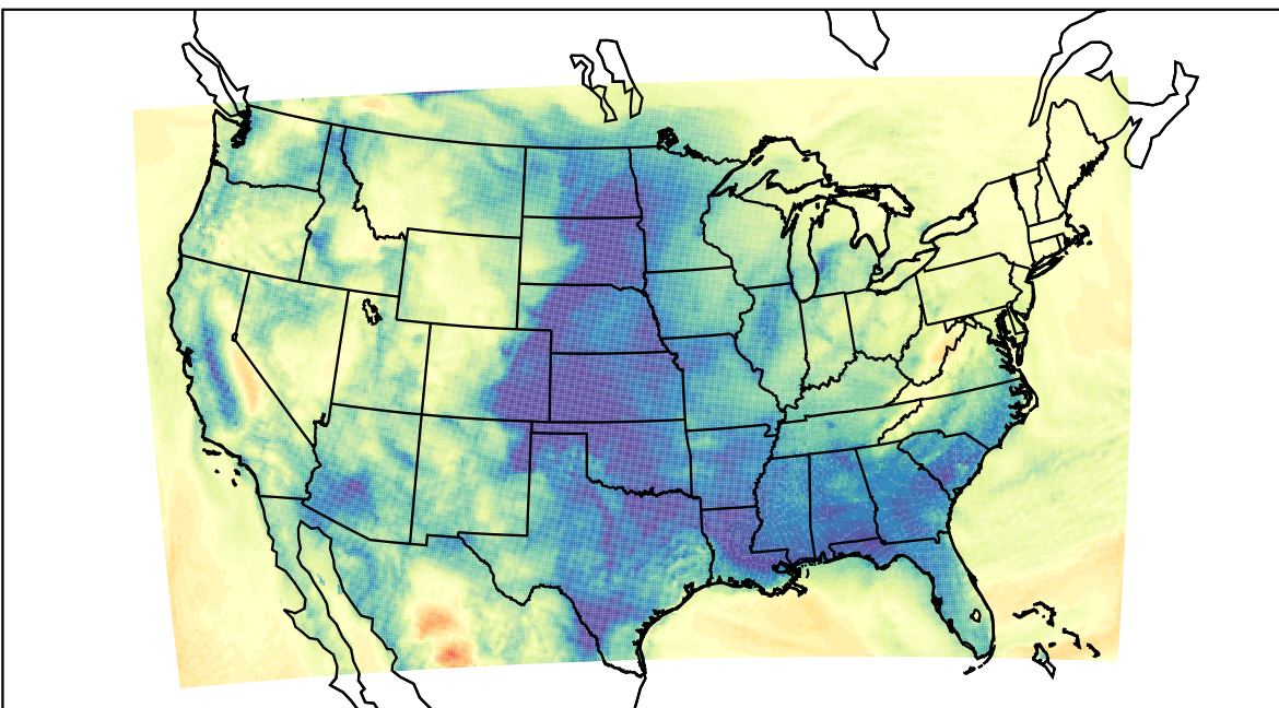
WRF (2024-01-05_10:00:00)
