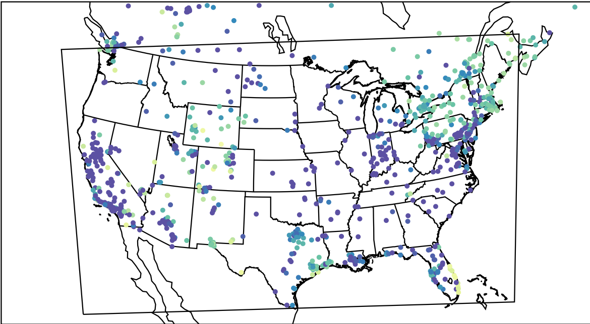
AirNOW (2024-01-05_11:00:00)
