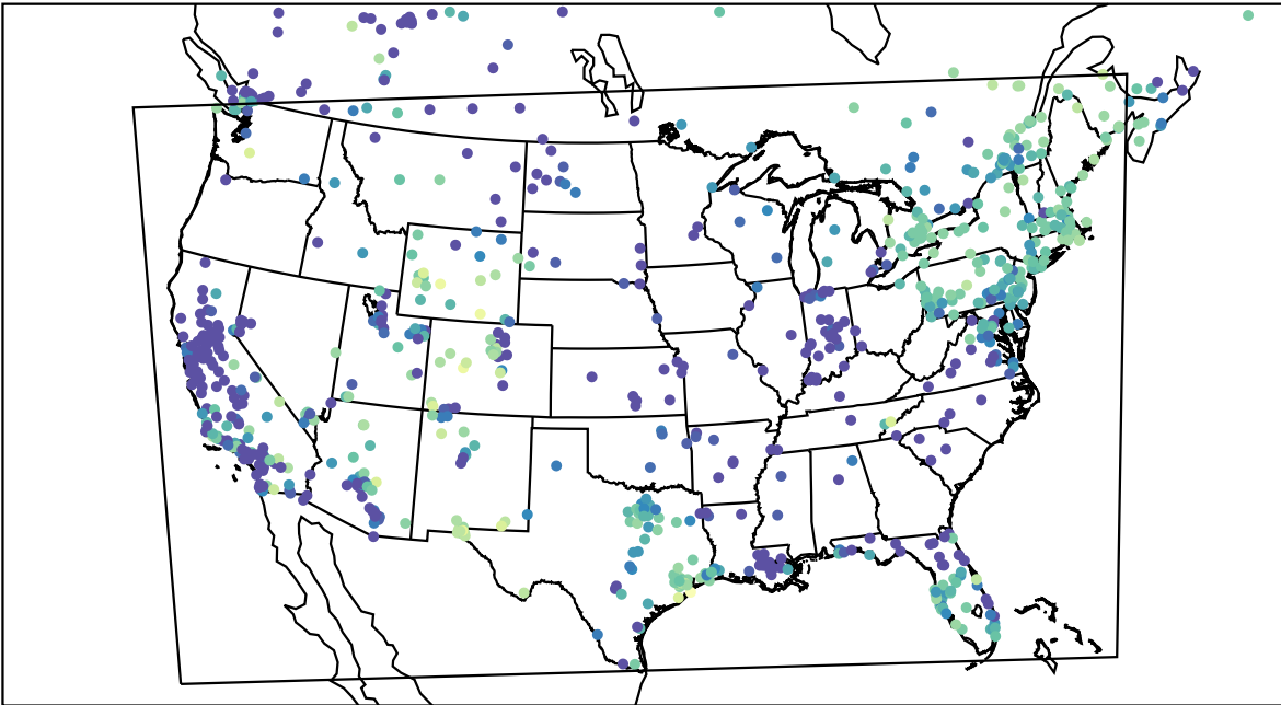
AirNOW (2024-01-05_07:00:00)
