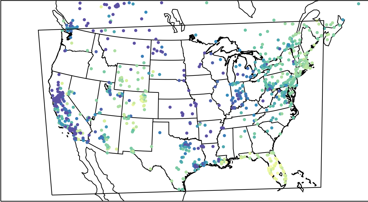
AirNOW (2024-01-05_18:00:00)
