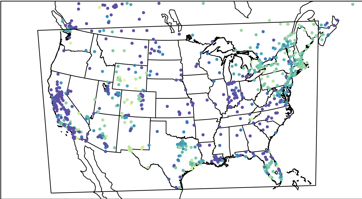
AirNOW (2024-01-05_06:00:00)
