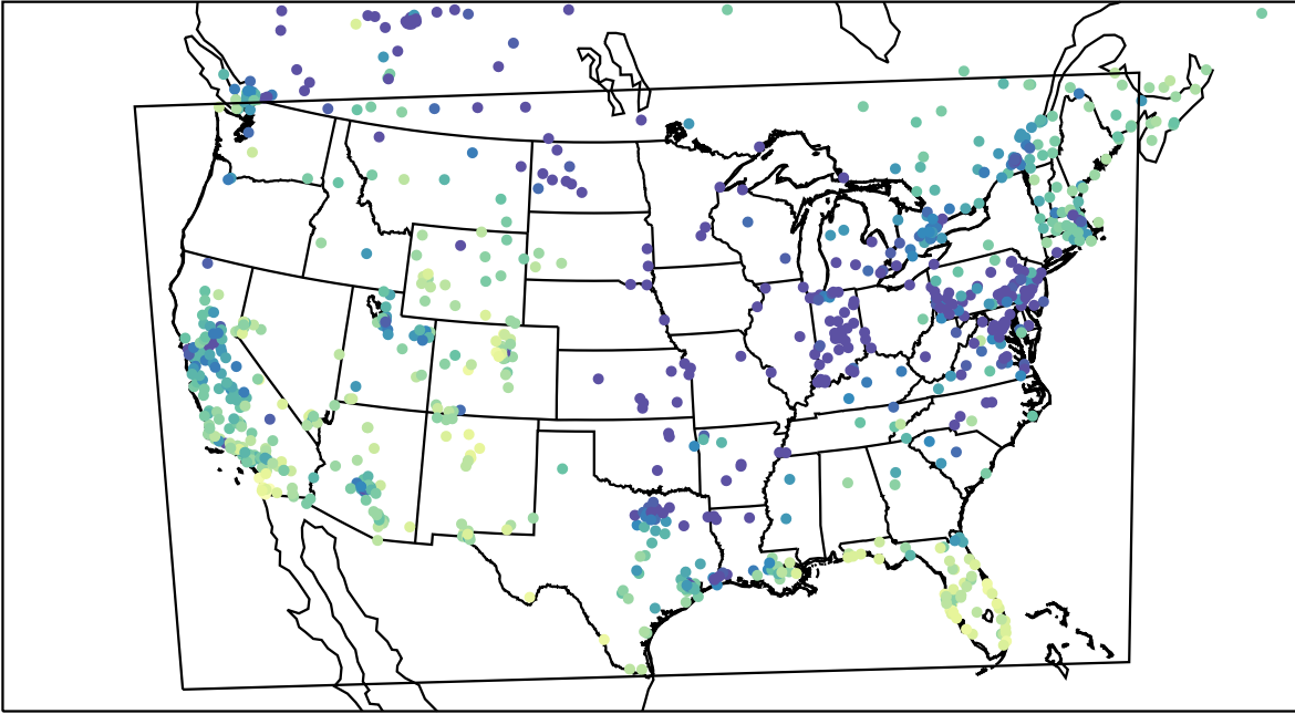
AirNOW (2024-01-05_23:00:00)
