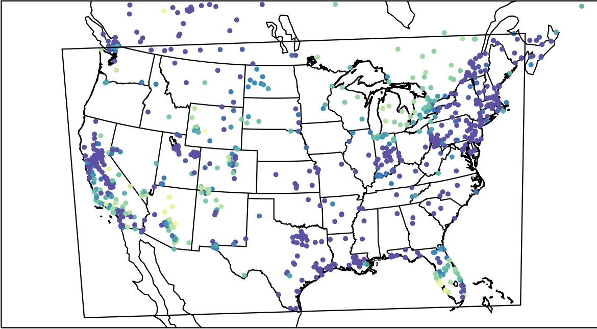
AirNOW (2024-01-04_09:00:00)
