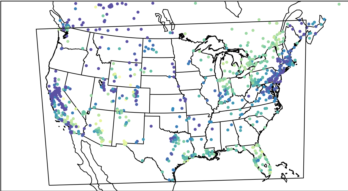
AirNOW (2024-01-04_17:00:00)
