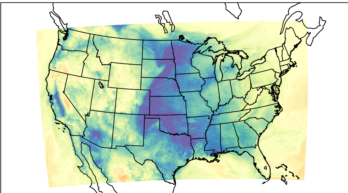
WRF (2024-01-05_16:00:00)
