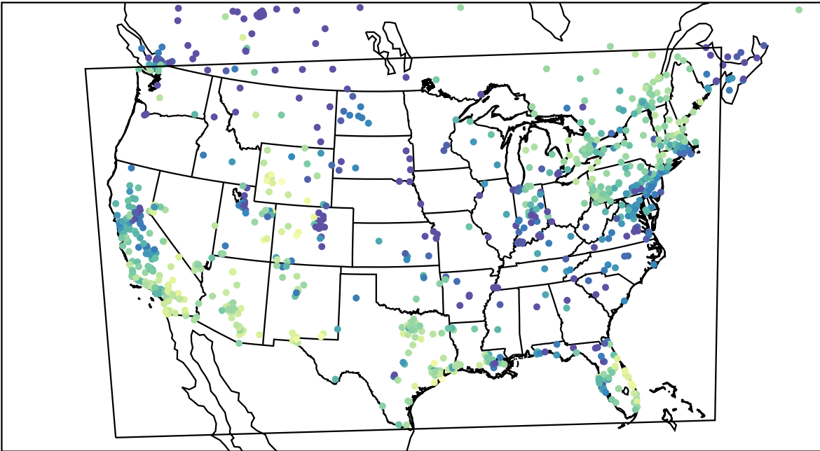
AirNOW (2024-01-04_23:00:00)
