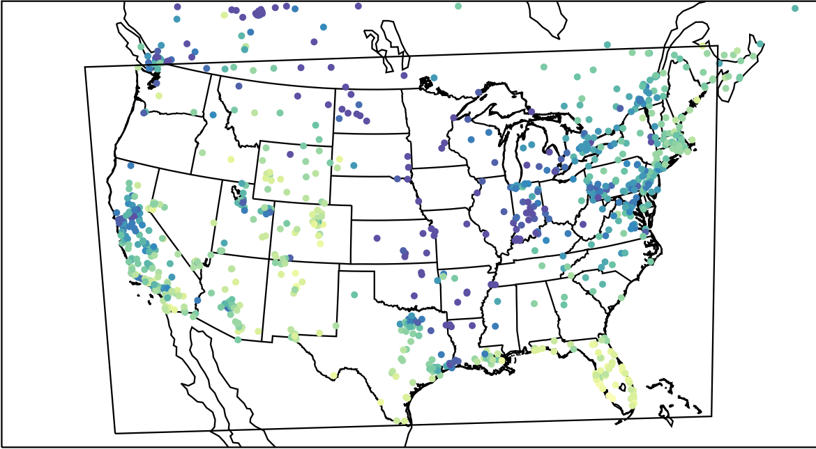
AirNOW (2024-01-05_21:00:00)
