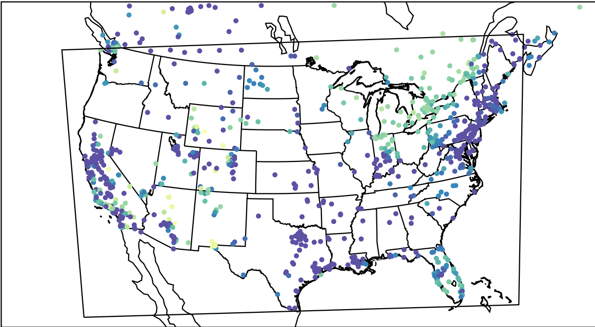
AirNOW (2024-01-04_14:00:00)
