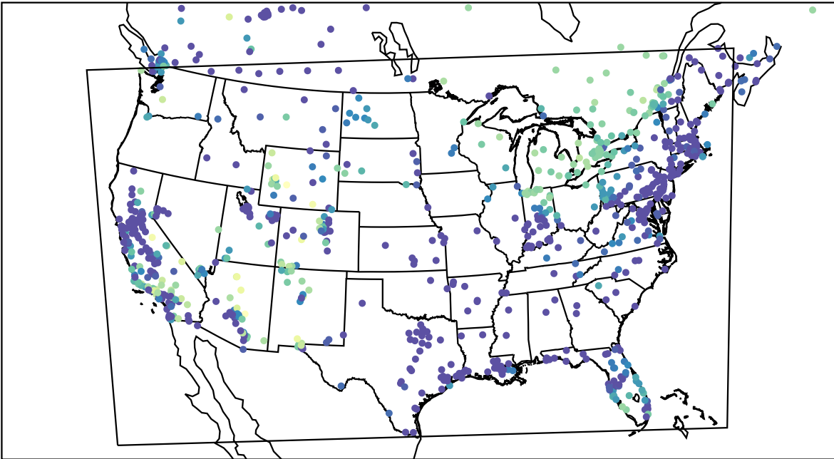
AirNOW (2024-01-04_13:00:00)
