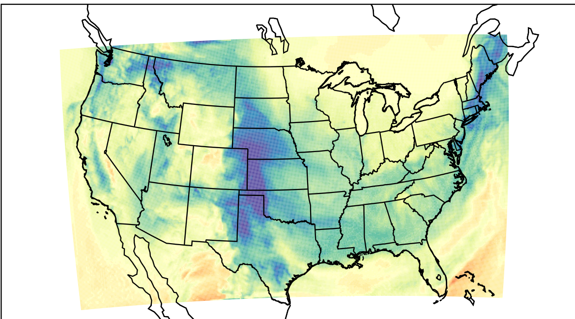
WRF (2024-01-04_19:00:00)
