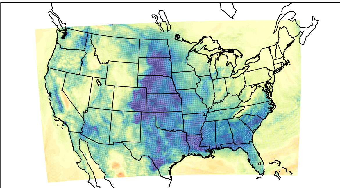
WRF (2024-01-05_07:00:00)
