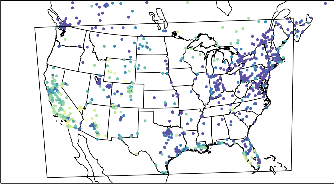
AirNOW (2024-01-04_00:00:00)
