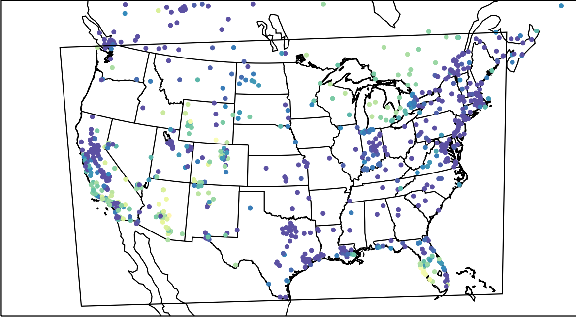
AirNOW (2024-01-04_06:00:00)
