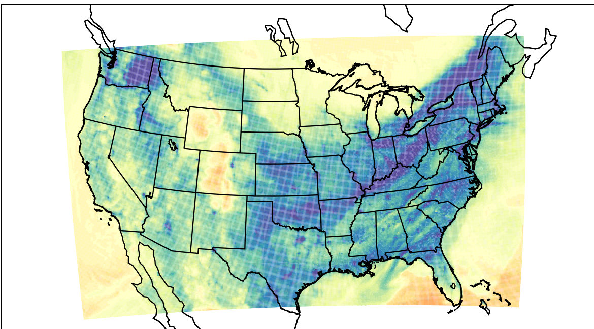
WRF (2024-01-04_02:00:00)
