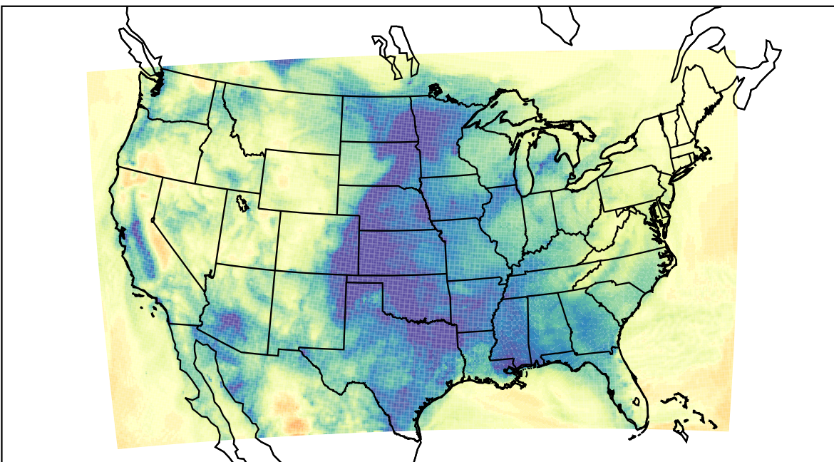
WRF (2024-01-05_15:00:00)
