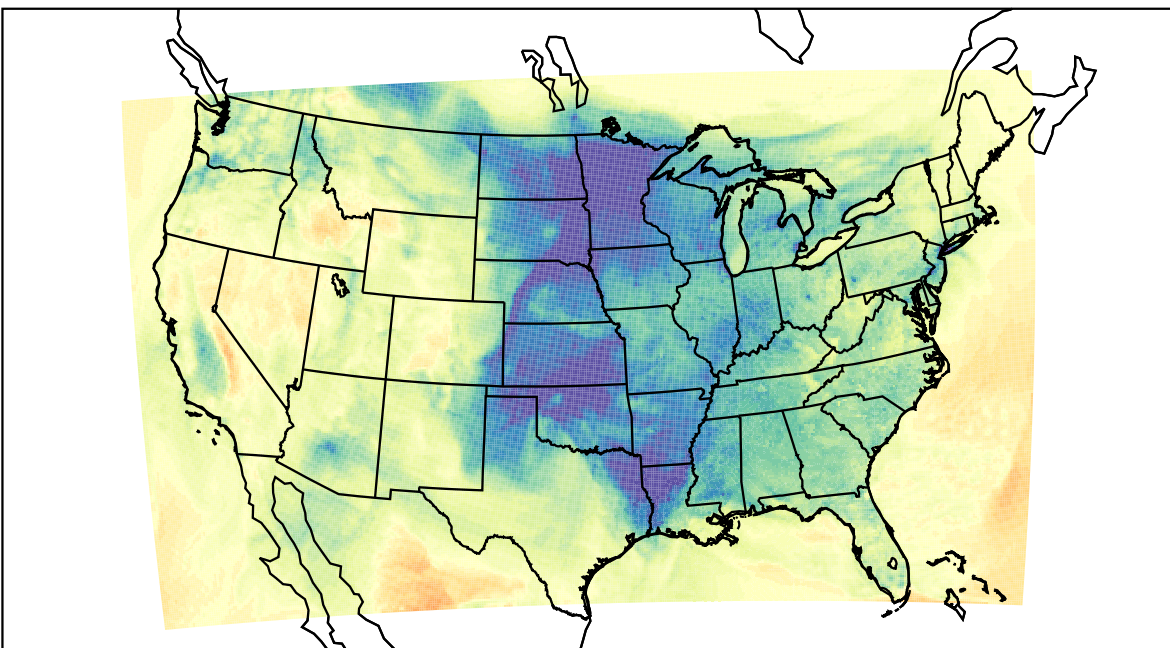
WRF (2024-01-05_22:00:00)
