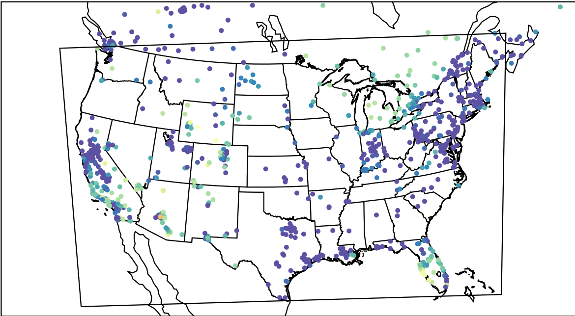
AirNOW (2024-01-04_08:00:00)
