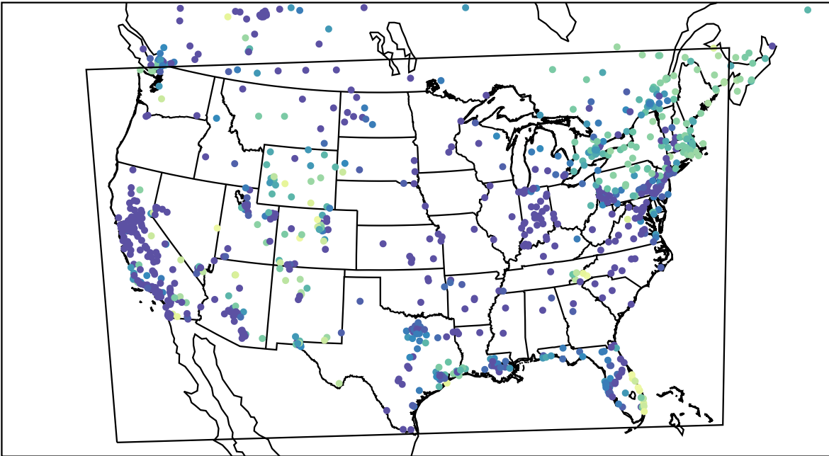
AirNOW (2024-01-05_13:00:00)
