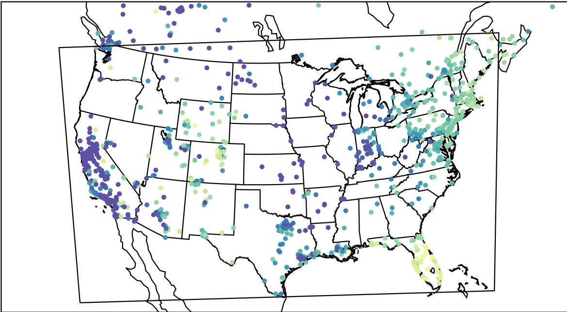
AirNOW (2024-01-05_17:00:00)
