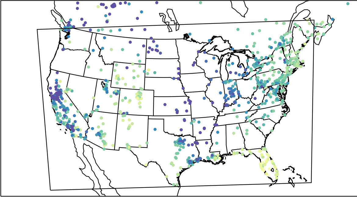
AirNOW (2024-01-05_19:00:00)
