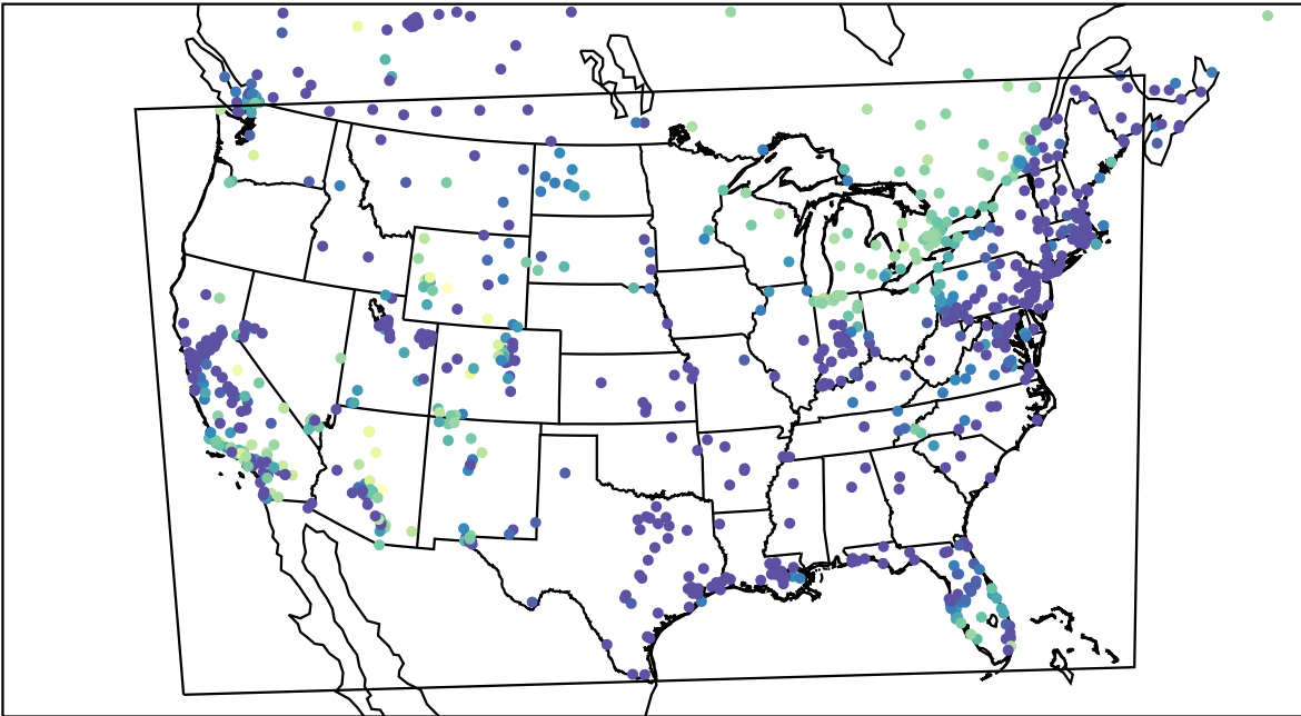
AirNOW (2024-01-04_12:00:00)
