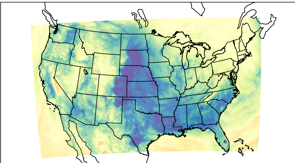
WRF (2024-01-05_05:00:00)
