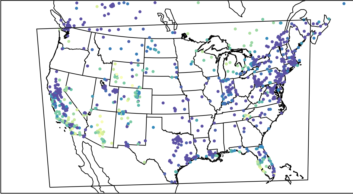
AirNOW (2024-01-04_04:00:00)
