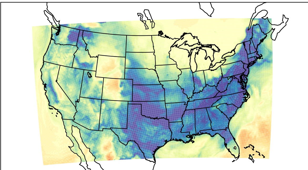
WRF (2024-01-04_12:00:00)
