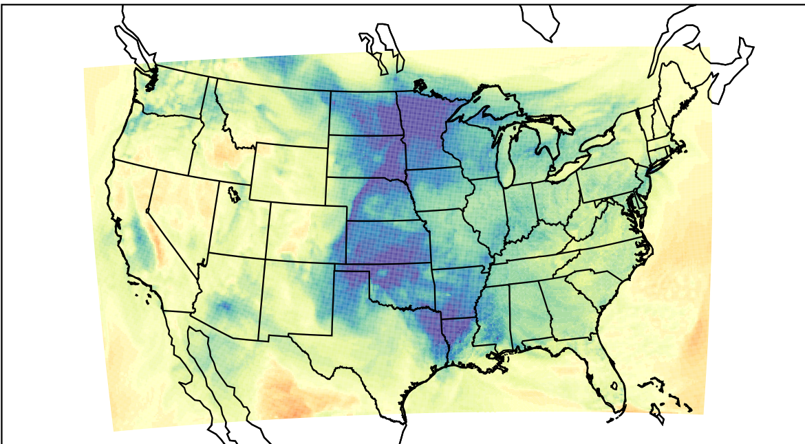
WRF (2024-01-05_21:00:00)
