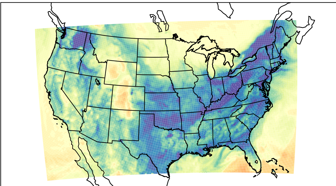
WRF (2024-01-04_04:00:00)
