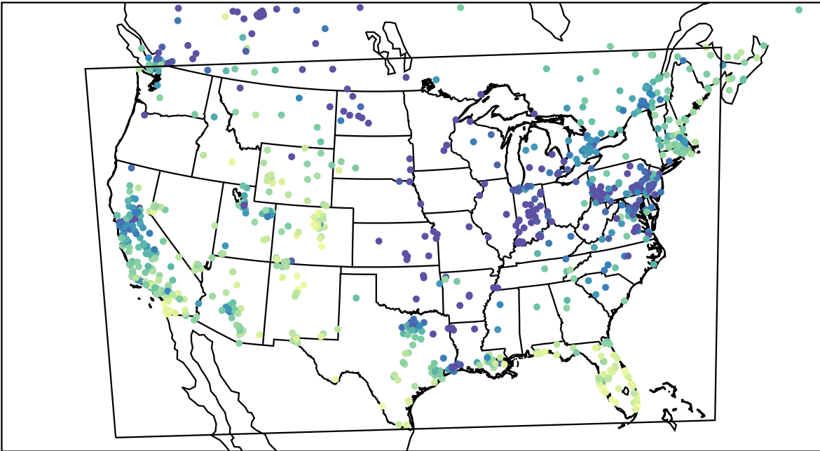
AirNOW (2024-01-05_22:00:00)
