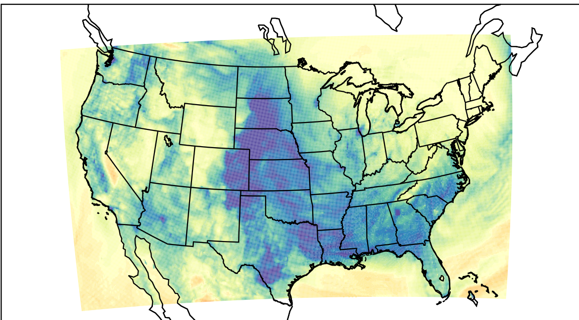
WRF (2024-01-05_04:00:00)
