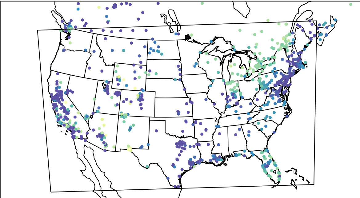
AirNOW (2024-01-04_15:00:00)
