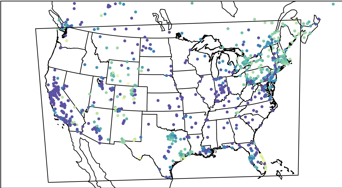
AirNOW (2024-01-05_10:00:00)
