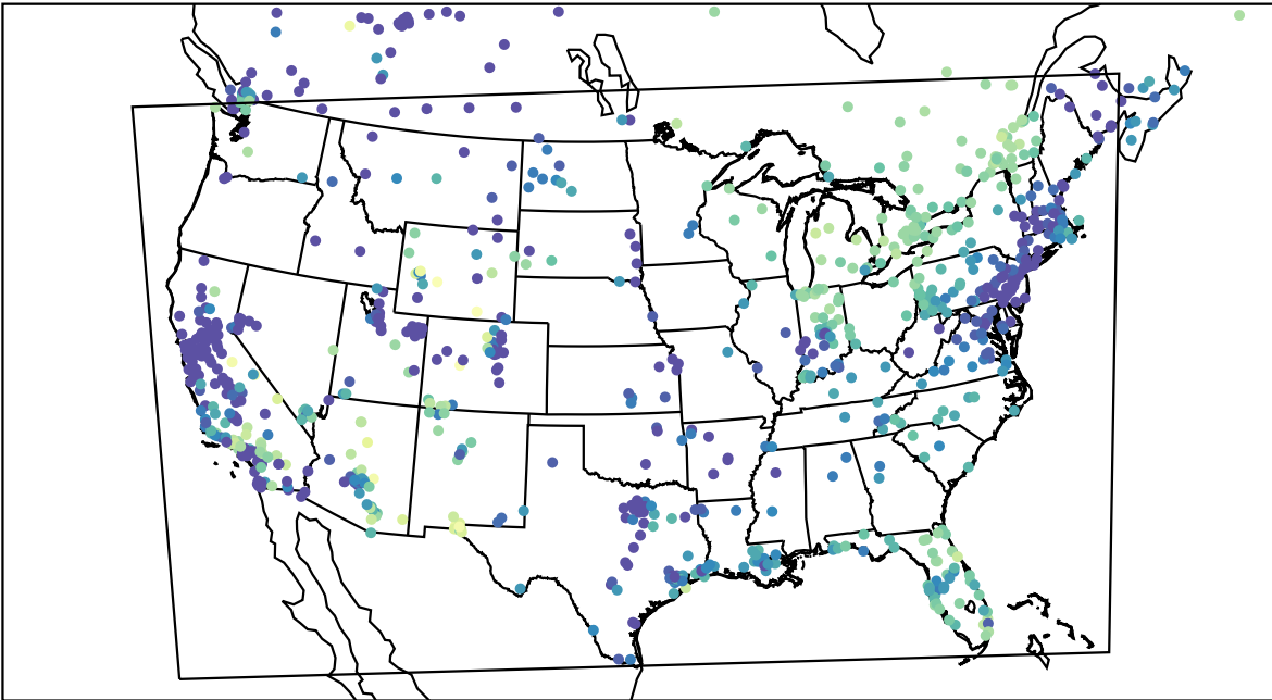
AirNOW (2024-01-04_16:00:00)
