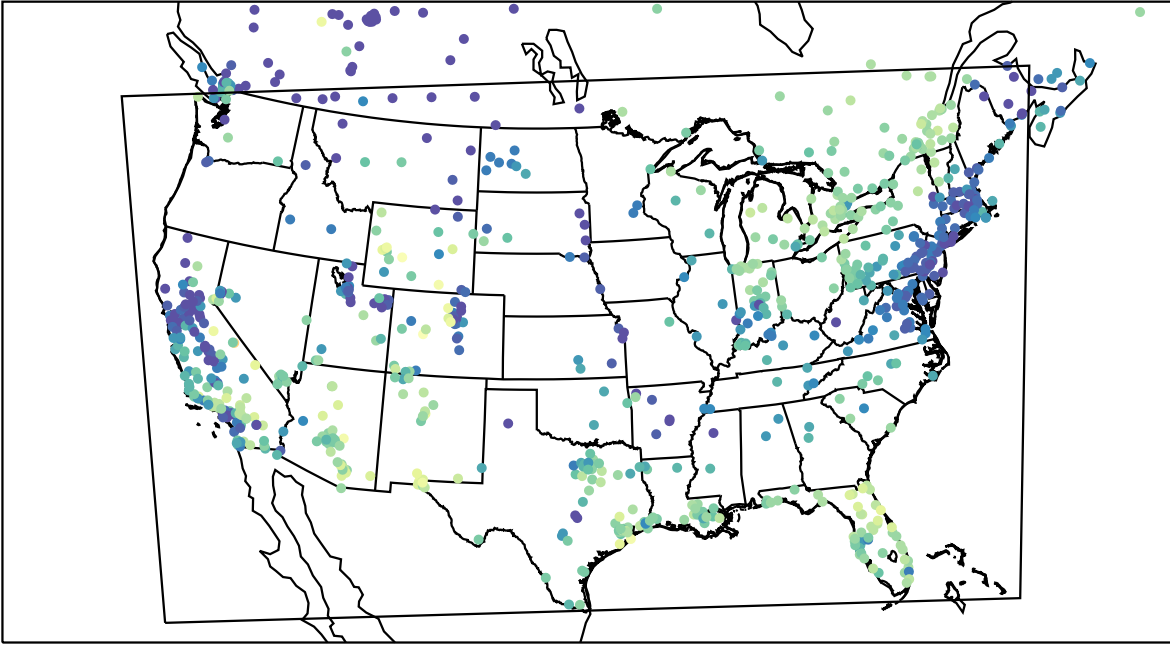
AirNOW (2024-01-04_18:00:00)
