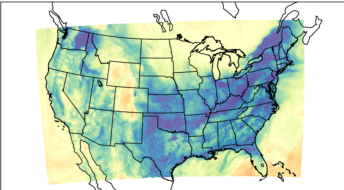
WRF (2024-01-04_05:00:00)
