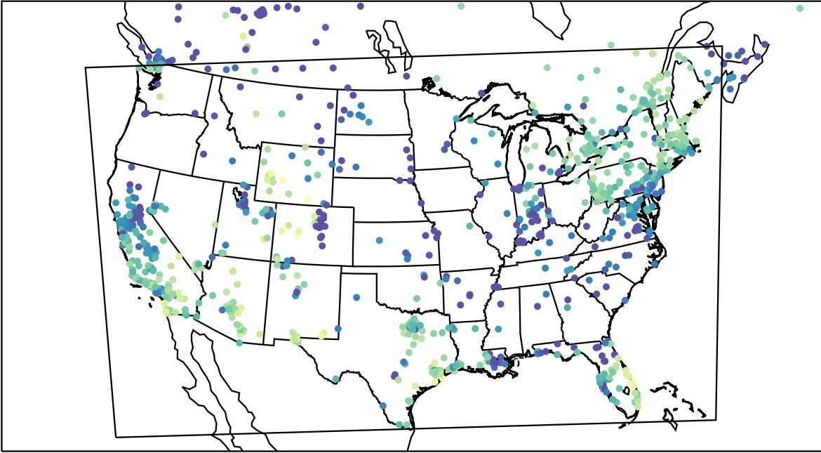
AirNOW (2024-01-05_00:00:00)
