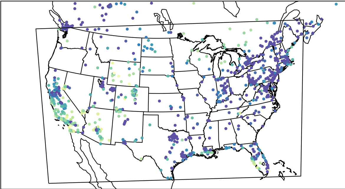
AirNOW (2024-01-04_01:00:00)
