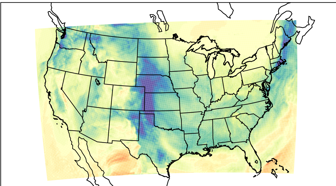
WRF (2024-01-04_21:00:00)
