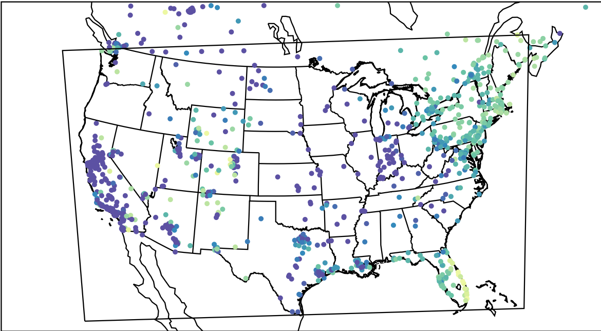
AirNOW (2024-01-05_15:00:00)
