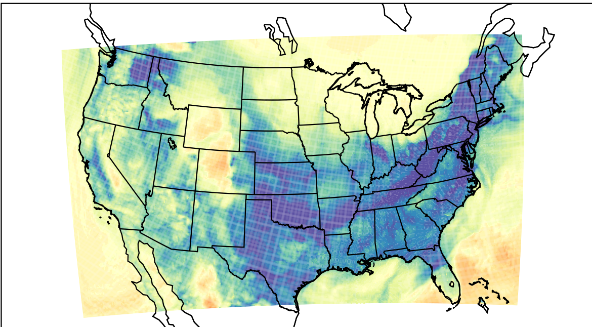
WRF (2024-01-04_10:00:00)
