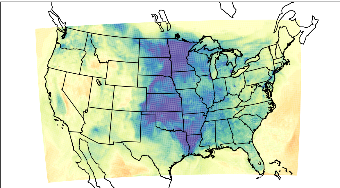
WRF (2024-01-05_23:00:00)
