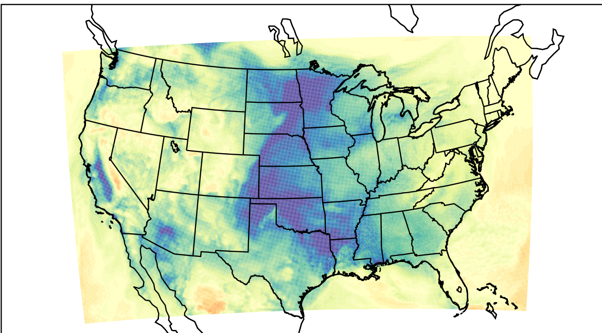
WRF (2024-01-05_17:00:00)
