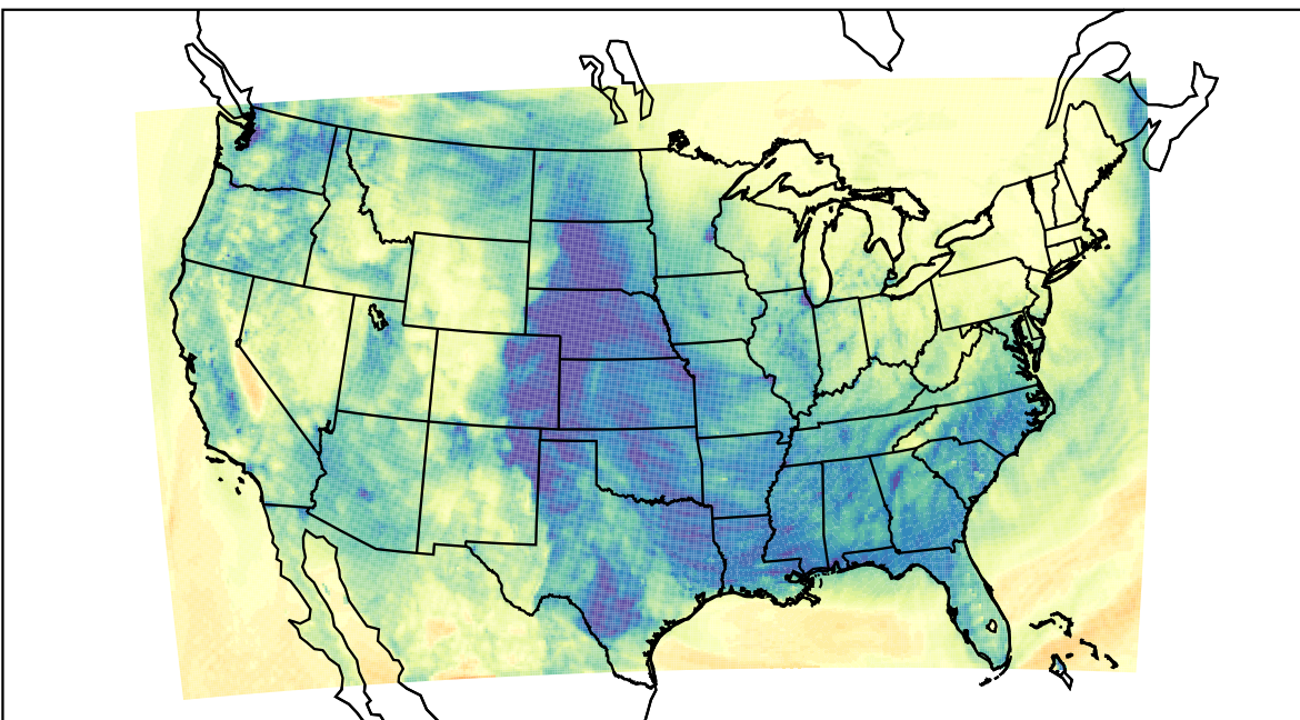
WRF (2024-01-05_02:00:00)
