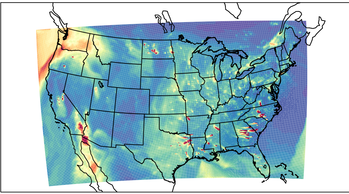
WRF 2024-01-05_23:00:00
