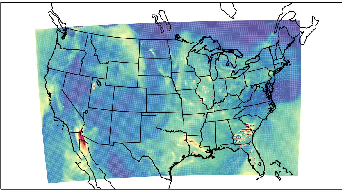
WRF 2024-01-06_19:00:00
