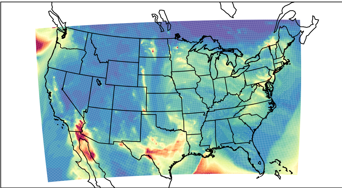
WRF 2024-01-09_06:00:00
